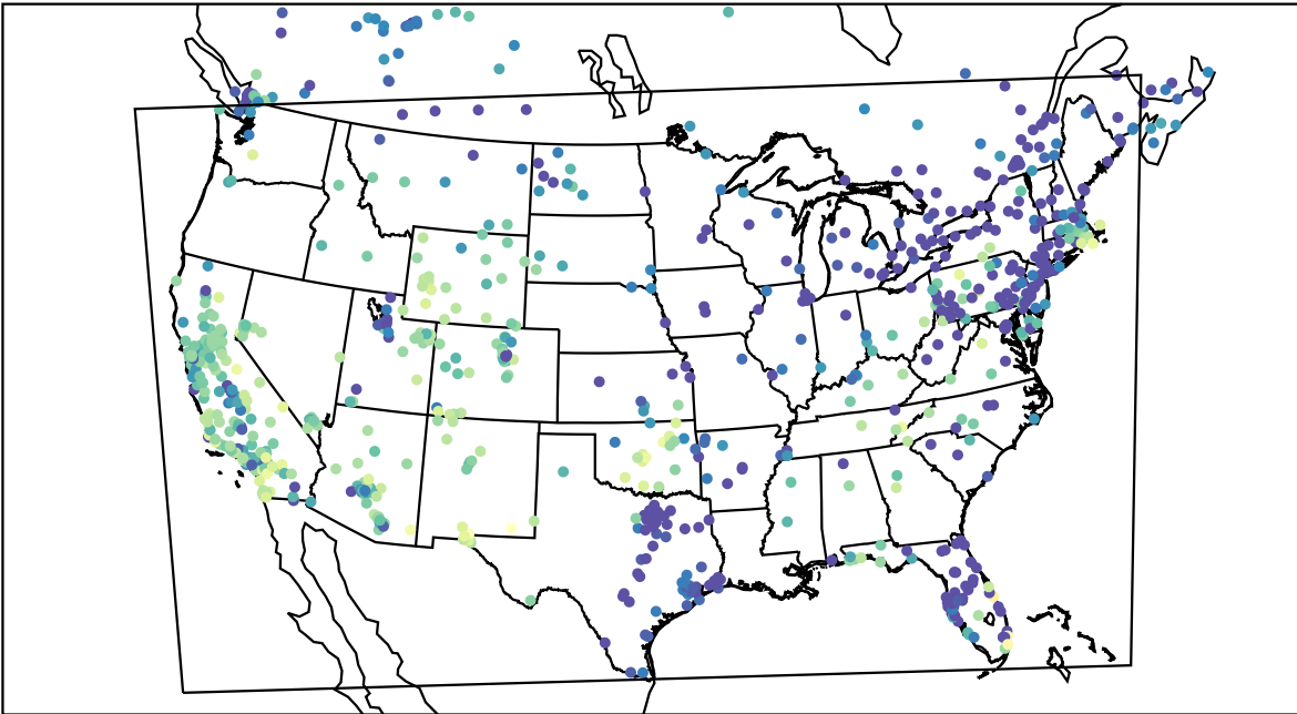
AirNOW (2019-11-27_00:00:00)
