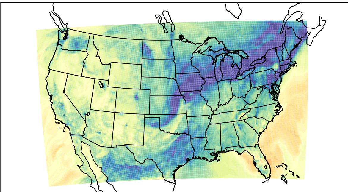
WRF (2019-11-27_02:00:00)
