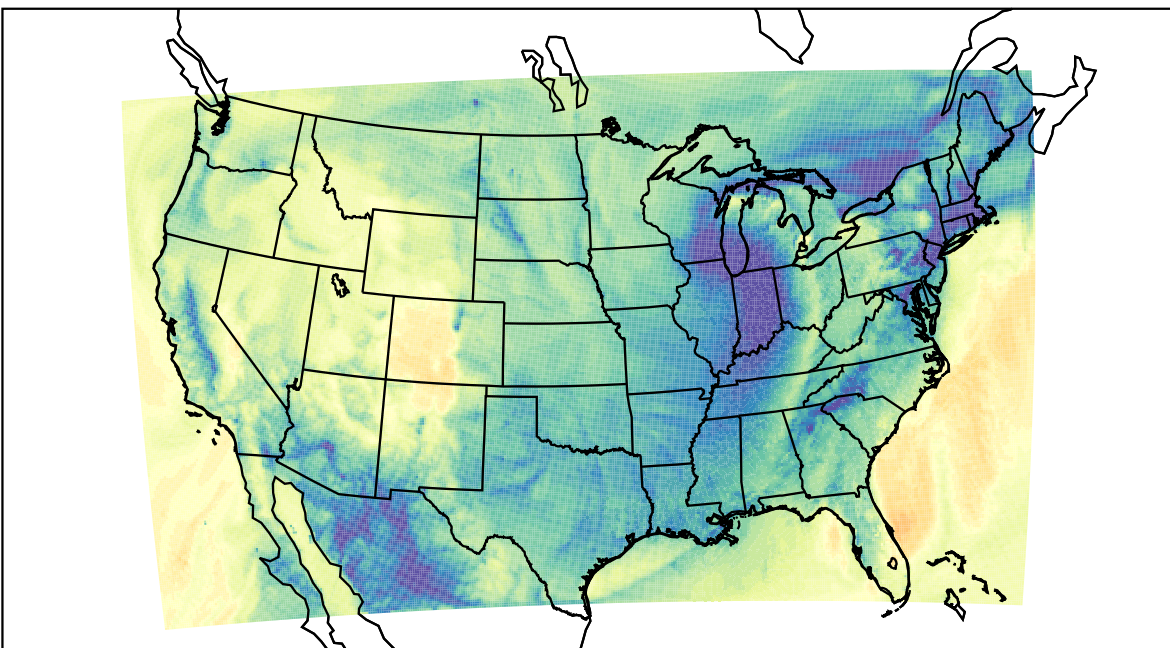
WRF (2019-11-27_15:00:00)
