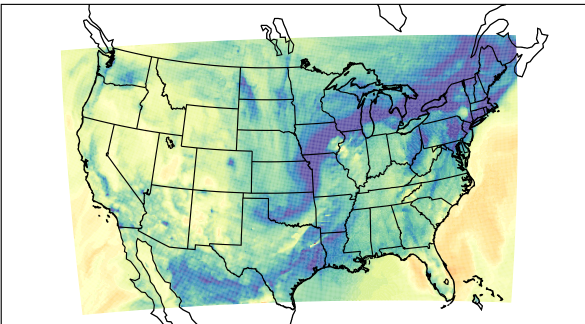
WRF (2019-11-27_05:00:00)
