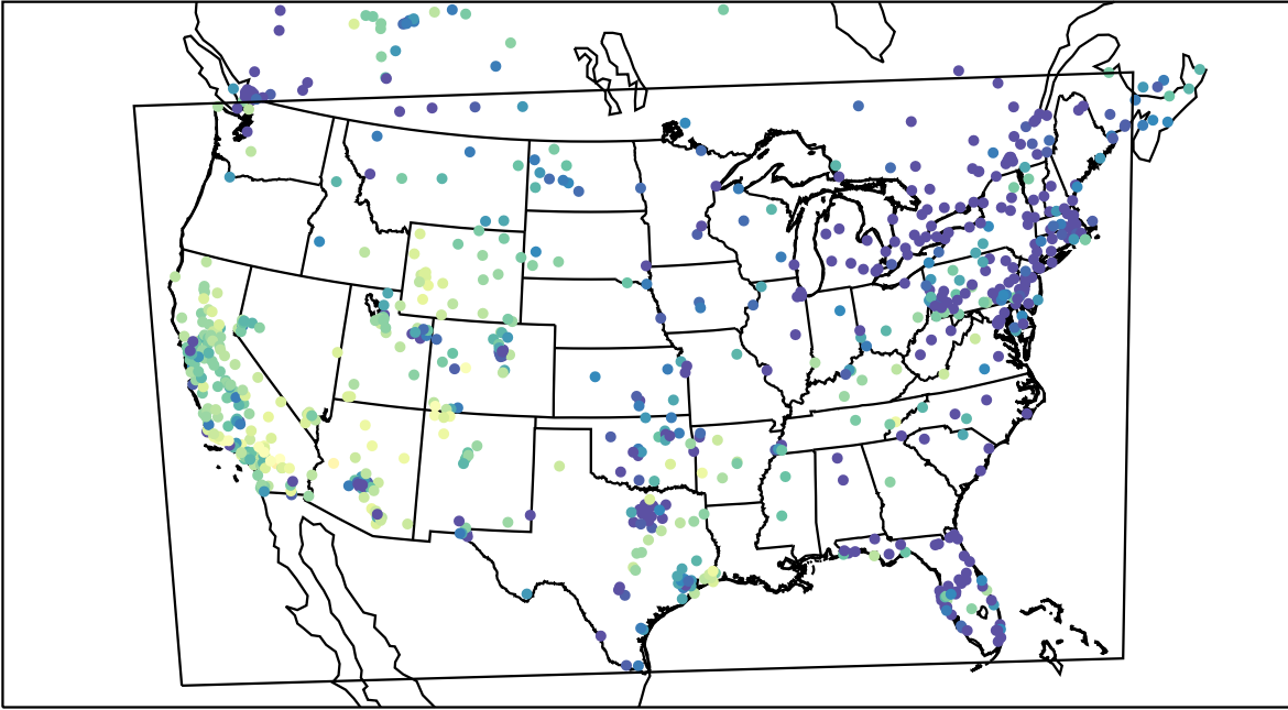
AirNOW (2019-11-26_01:00:00)
