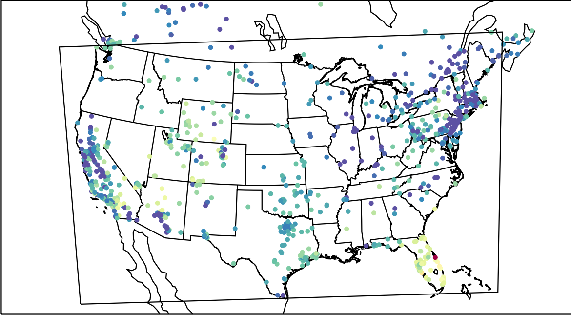
AirNOW (2019-11-27_16:00:00)
