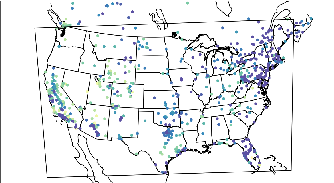
AirNOW (2019-11-27_10:00:00)
