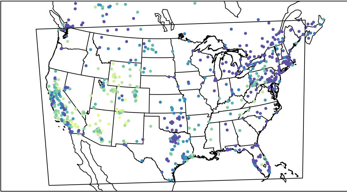
AirNOW (2019-11-26_05:00:00)
