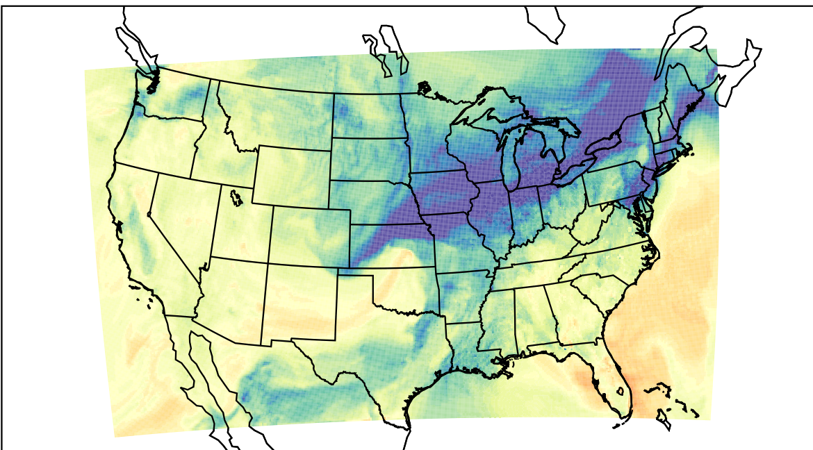
WRF (2019-11-26_21:00:00)
