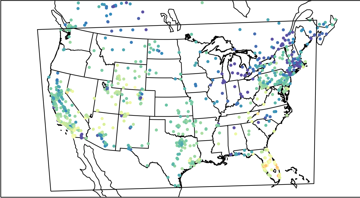
AirNOW (2019-11-27_19:00:00)
