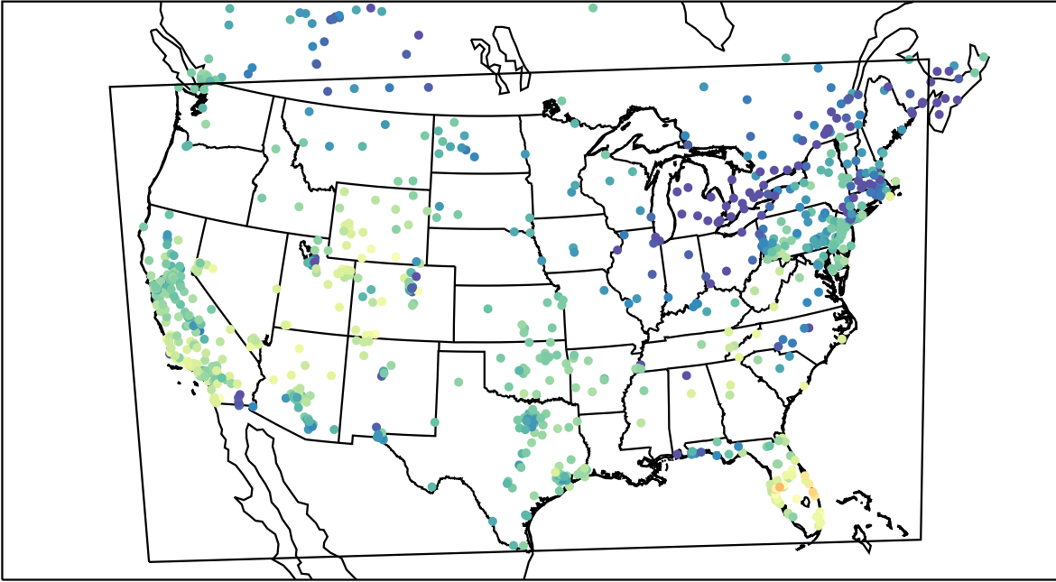
AirNOW (2019-11-27_21:00:00)
