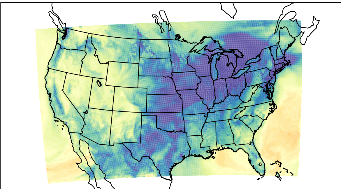
WRF (2019-11-26_09:00:00)
