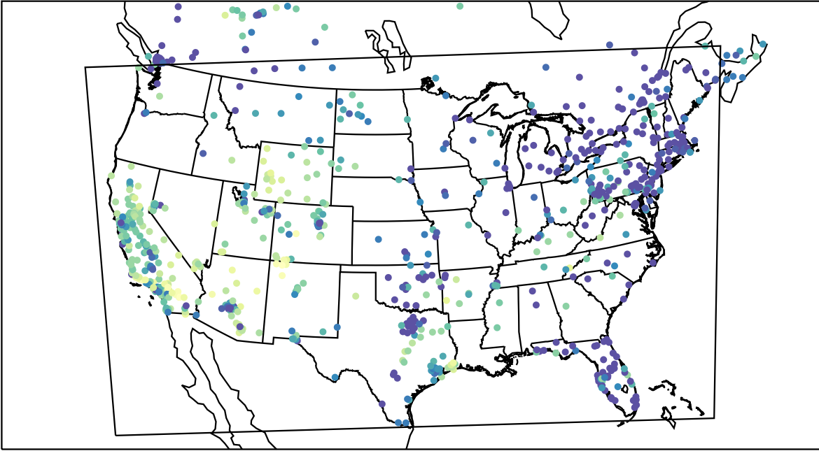
AirNOW (2019-11-26_02:00:00)
