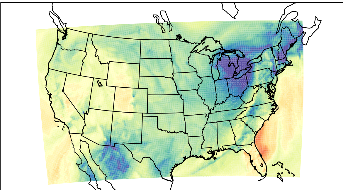
WRF (2019-11-27_21:00:00)
