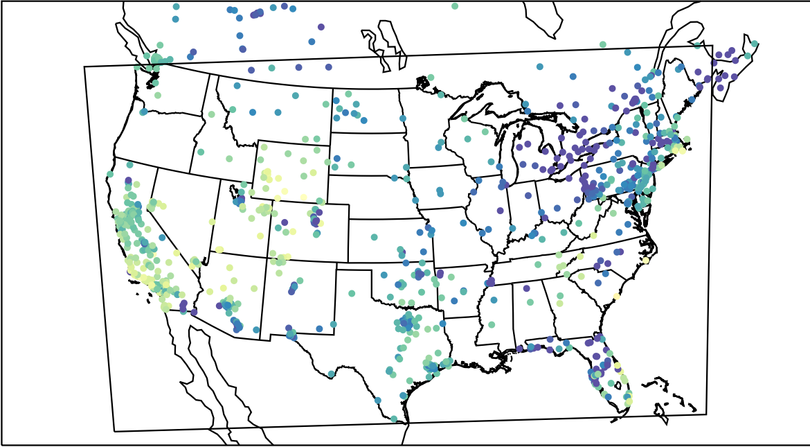
AirNOW (2019-11-27_23:00:00)
