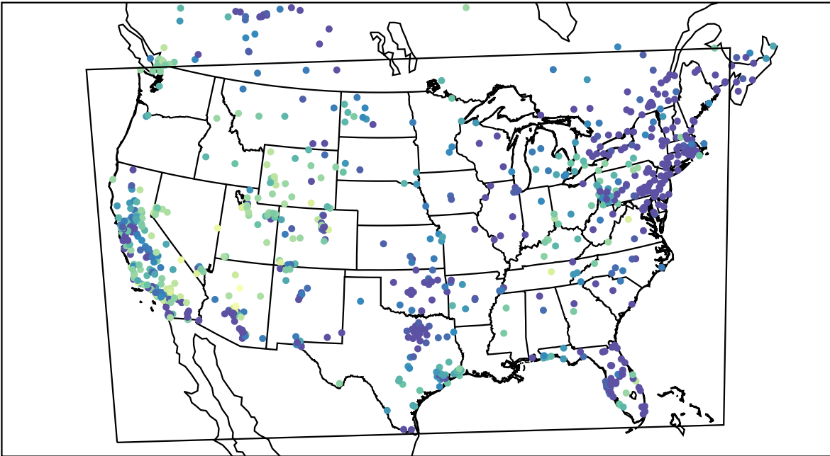
AirNOW (2019-11-27_13:00:00)
