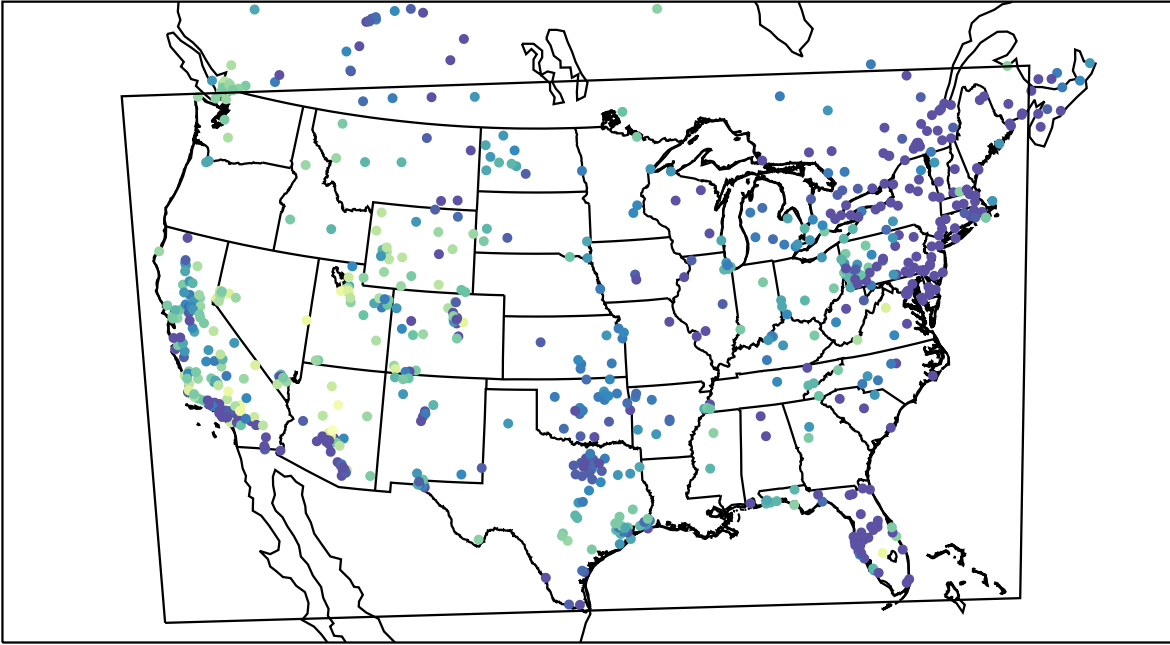
AirNOW (2019-11-27_11:00:00)
