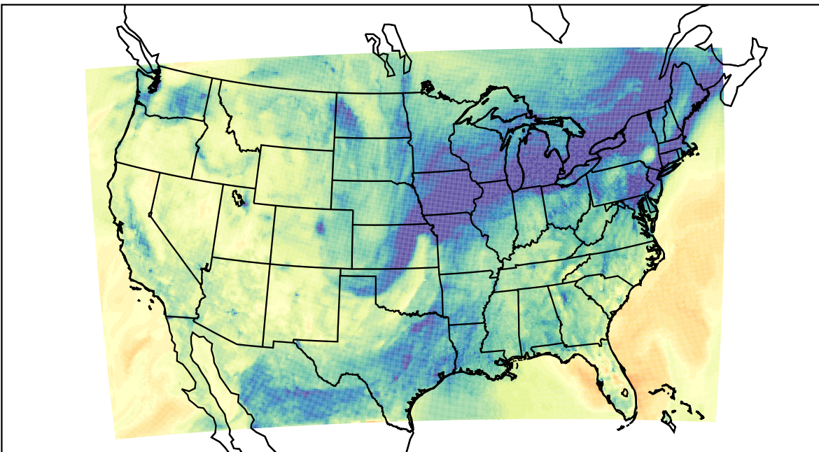
WRF (2019-11-27_01:00:00)
