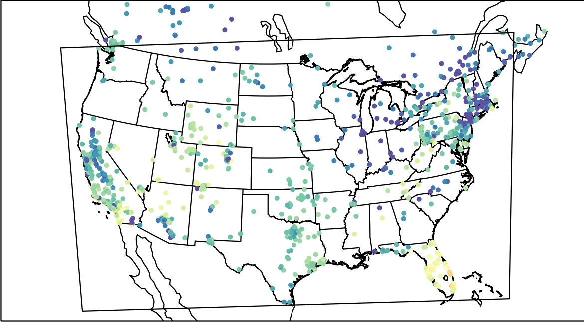
AirNOW (2019-11-27_18:00:00)
