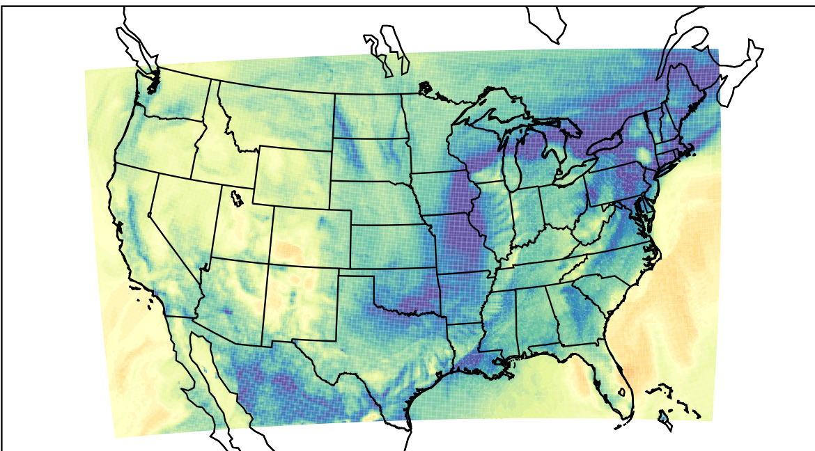
WRF (2019-11-27_09:00:00)
