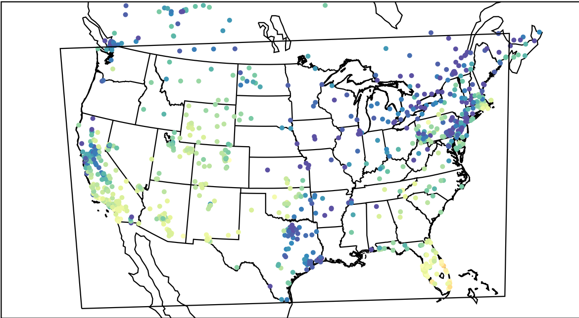
AirNOW (2019-11-26_21:00:00)
