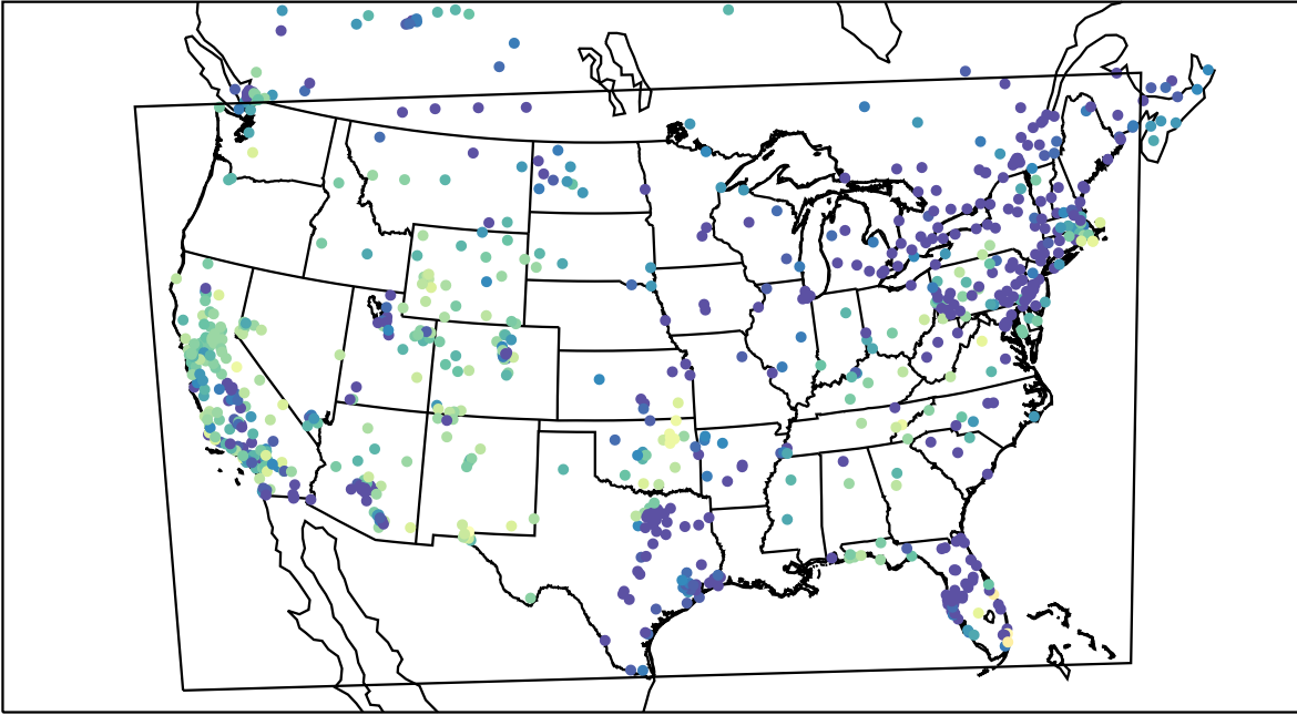
AirNOW (2019-11-27_01:00:00)
