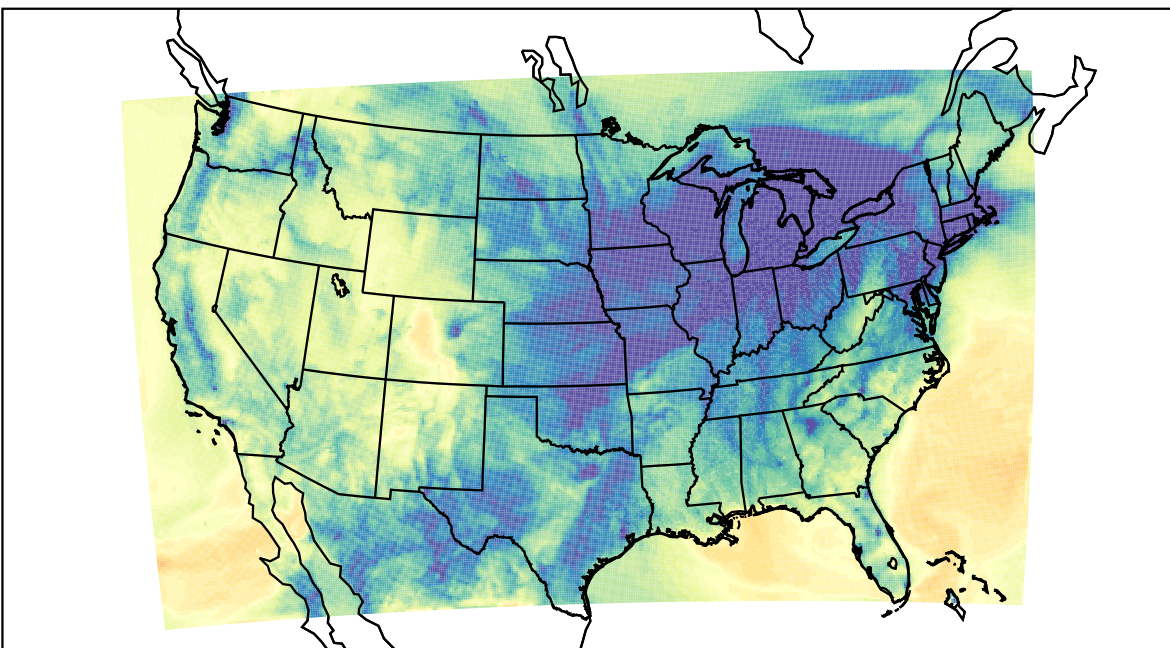
WRF (2019-11-26_05:00:00)
