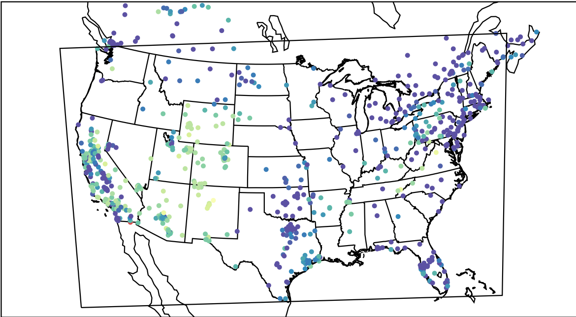
AirNOW (2019-11-26_09:00:00)
