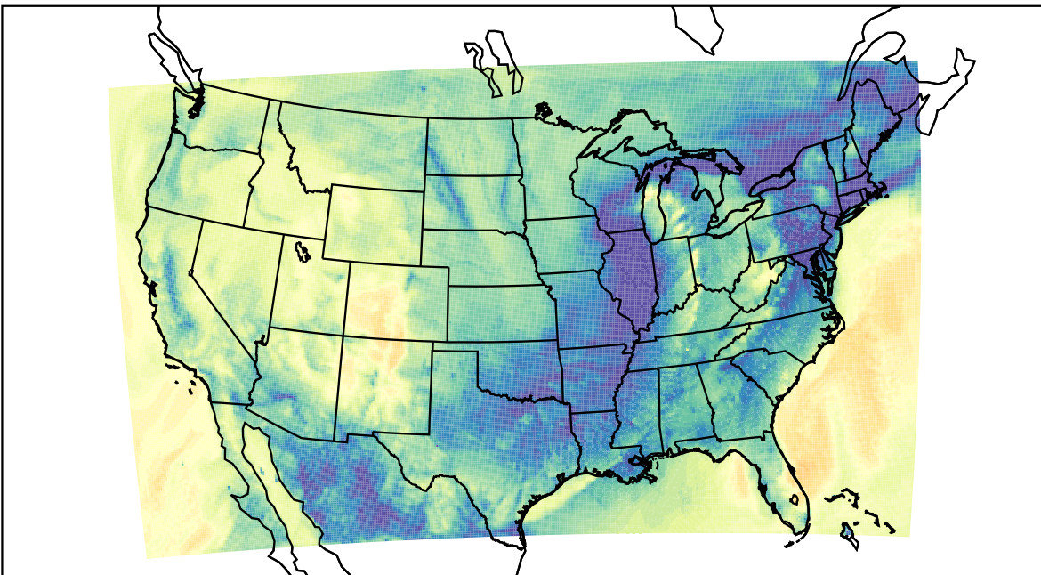
WRF (2019-11-27_12:00:00)
