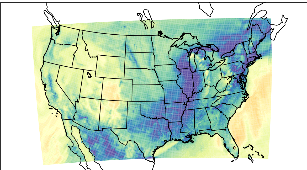
WRF (2019-11-27_13:00:00)
