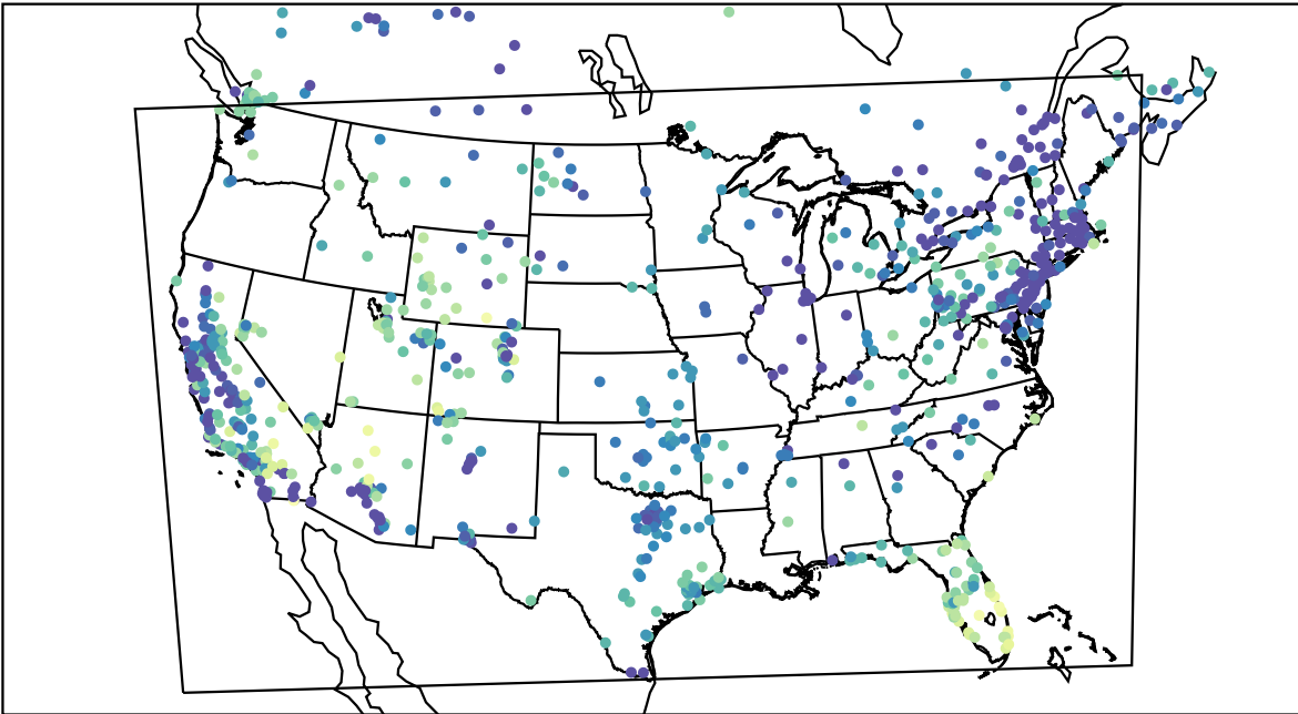
AirNOW (2019-11-27_15:00:00)
