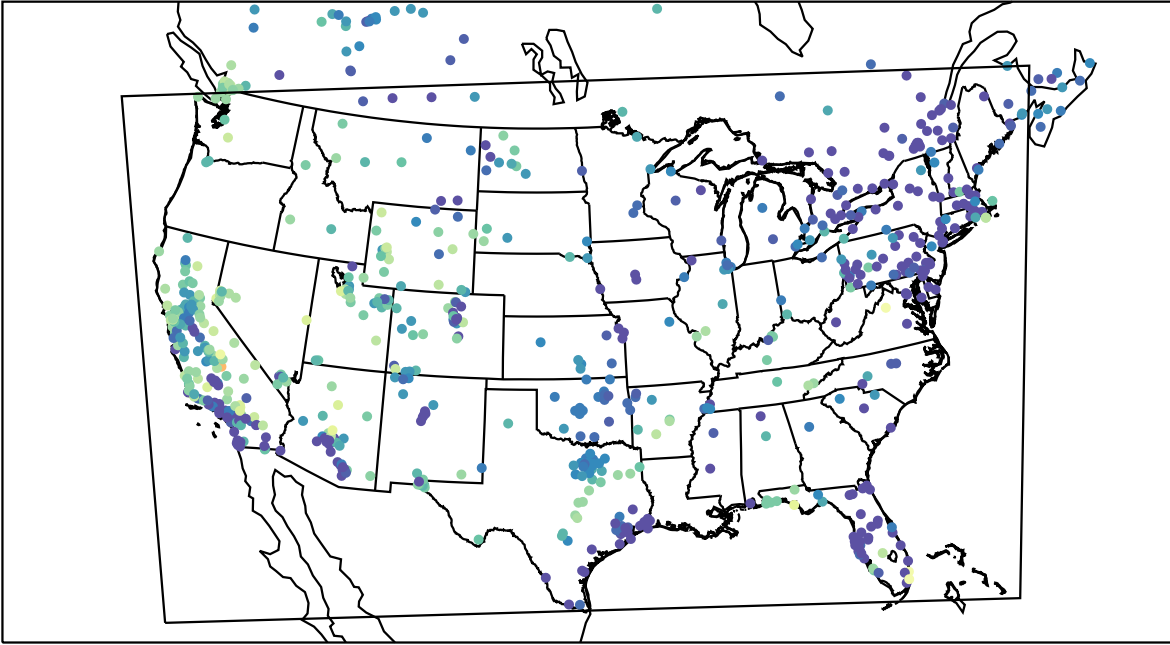
AirNOW (2019-11-27_07:00:00)
