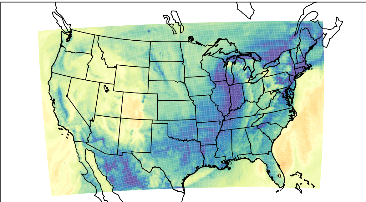
WRF (2019-11-27_14:00:00)
