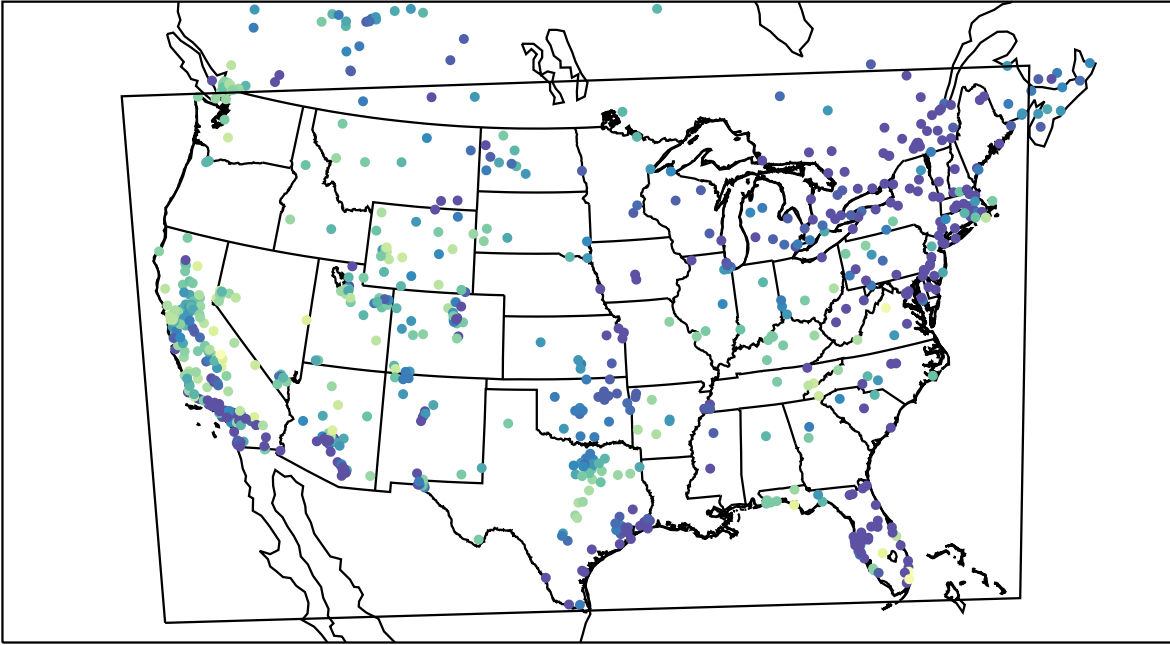
AirNOW (2019-11-27_06:00:00)
