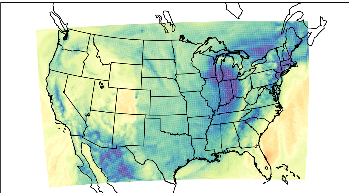
WRF (2019-11-27_16:00:00)
