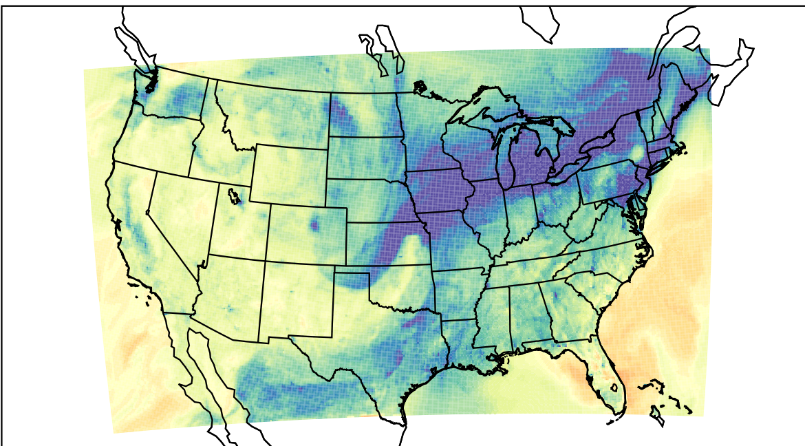
WRF (2019-11-27_00:00:00)
