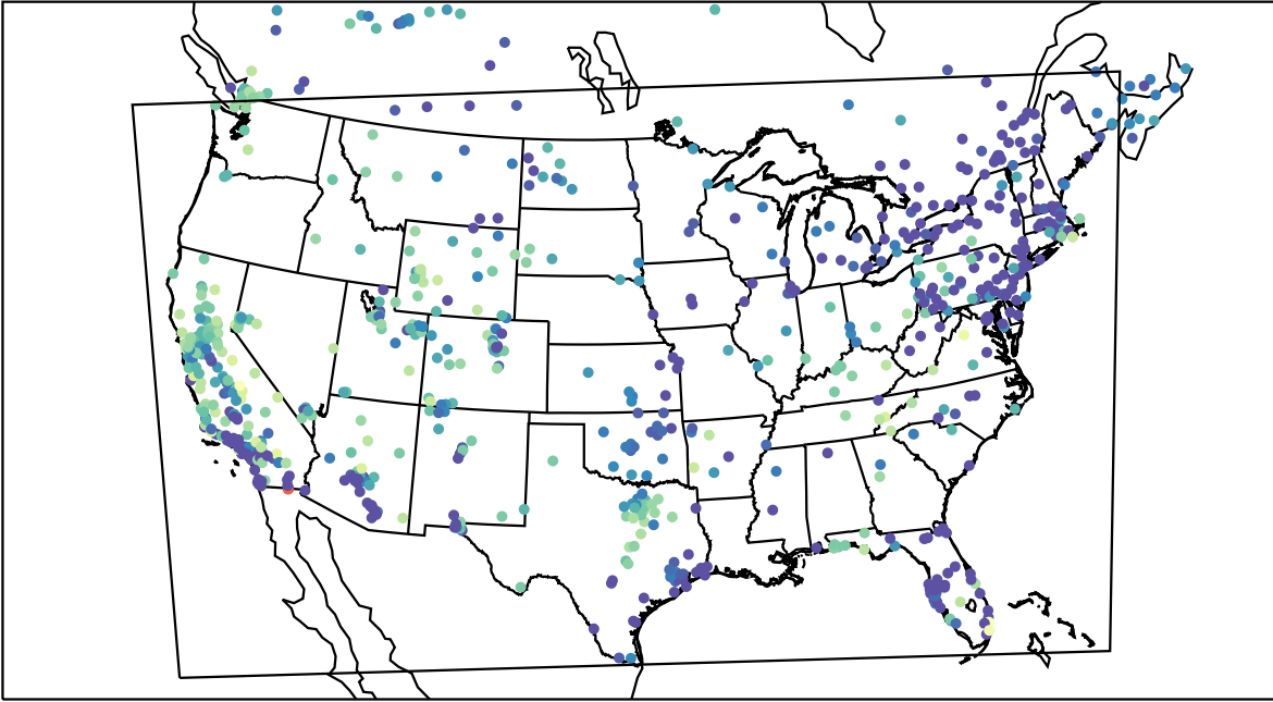
AirNOW (2019-11-27_05:00:00)
