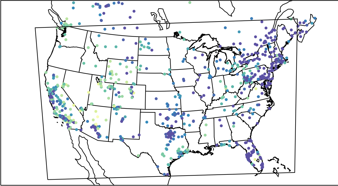
AirNOW (2019-11-27_12:00:00)
