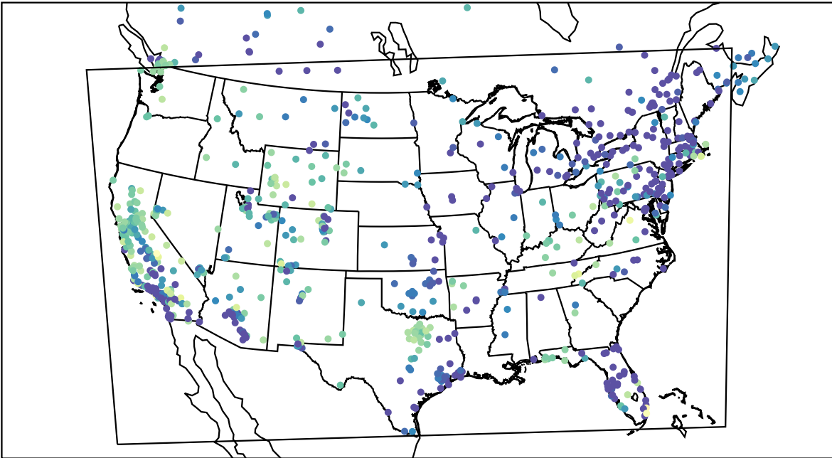
AirNOW (2019-11-27_04:00:00)
