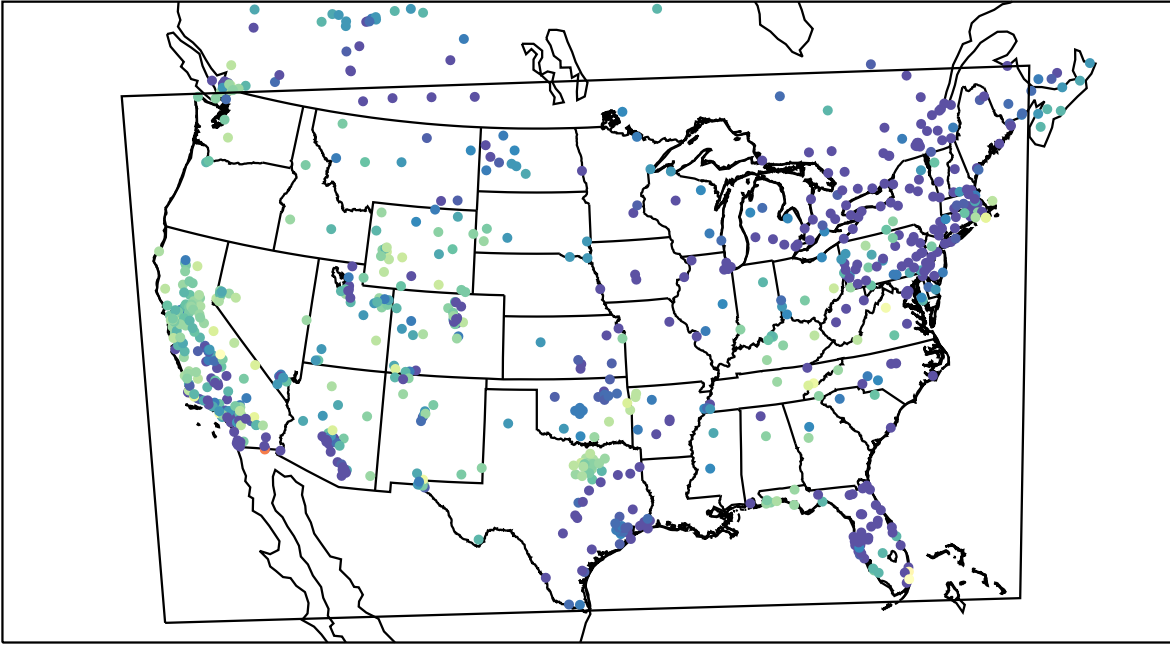
AirNOW (2019-11-27_03:00:00)
