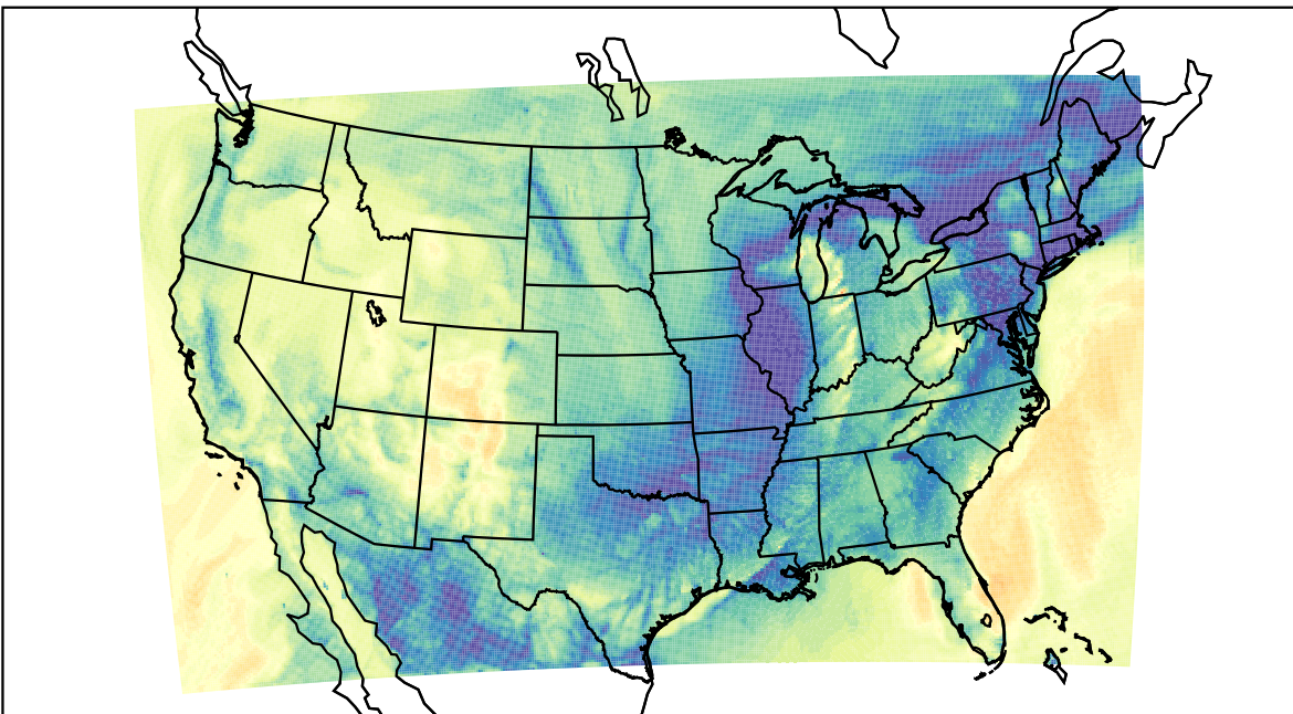
WRF (2019-11-27_11:00:00)
