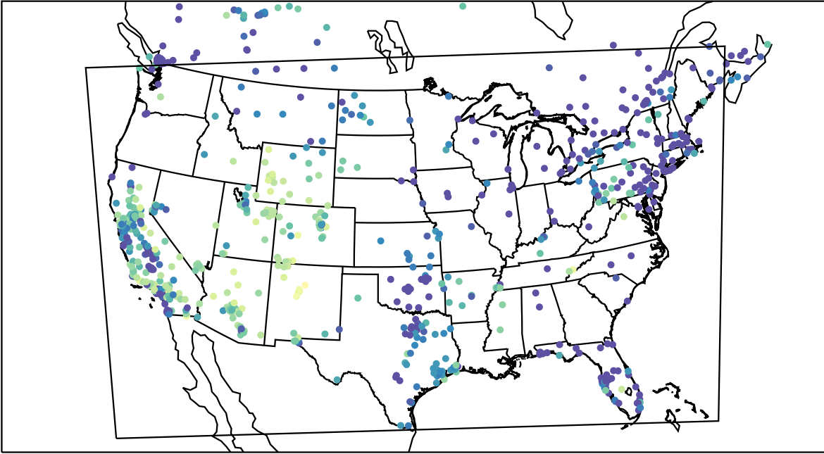
AirNOW (2019-11-26_07:00:00)
