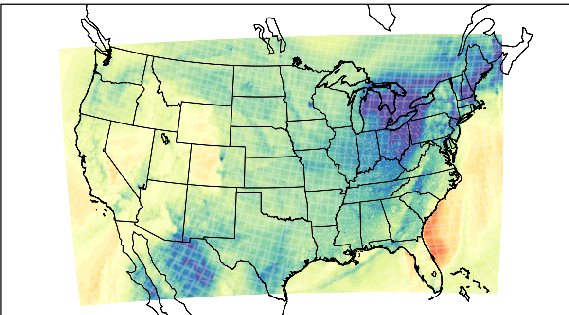
WRF (2019-11-27_22:00:00)
