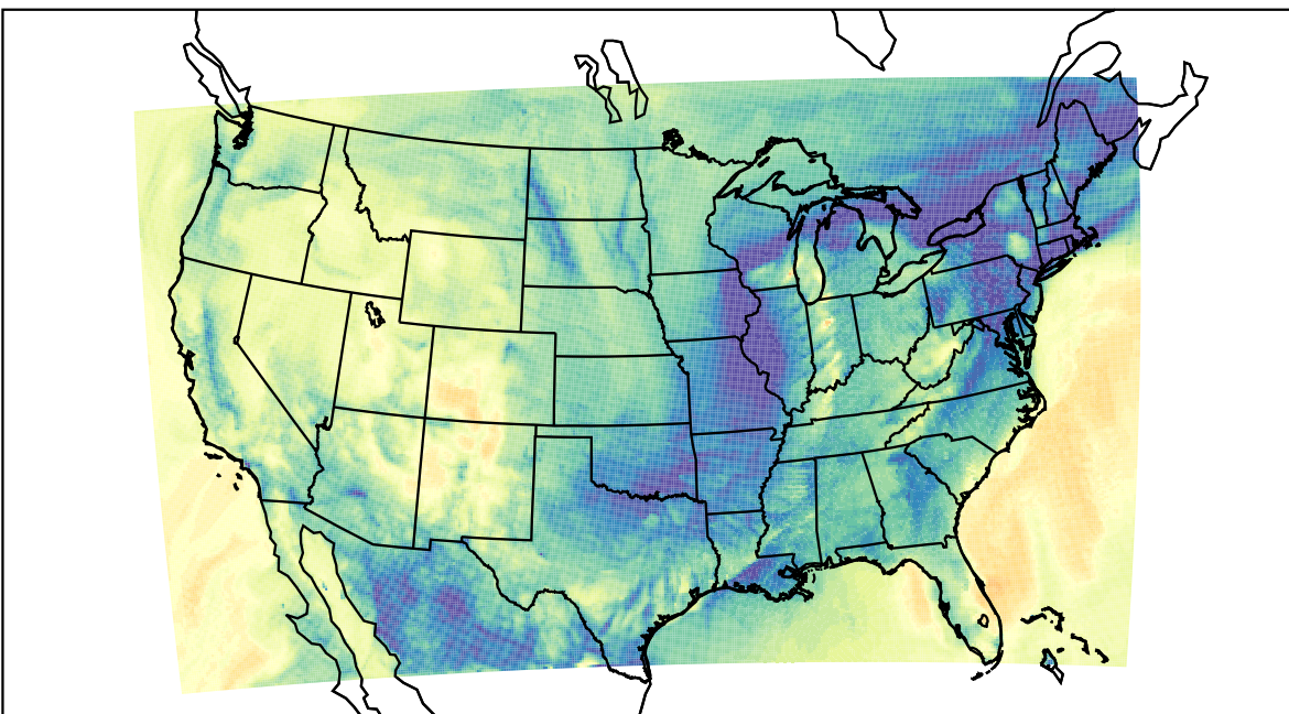
WRF (2019-11-27_10:00:00)
