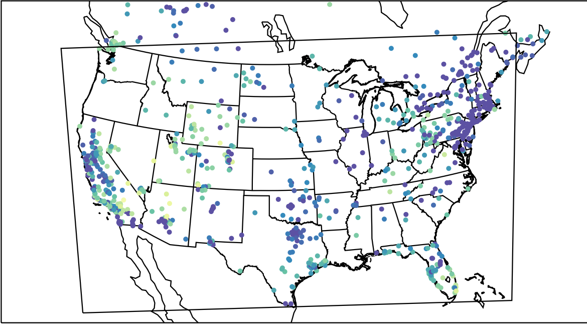
AirNOW (2019-11-27_14:00:00)
