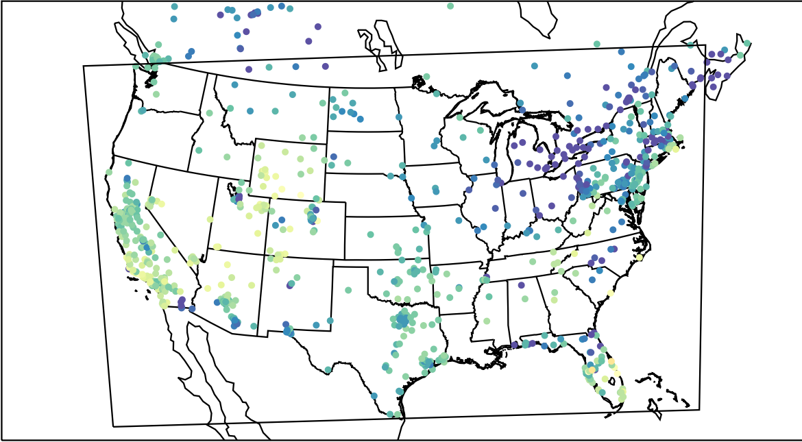
AirNOW (2019-11-27_22:00:00)
