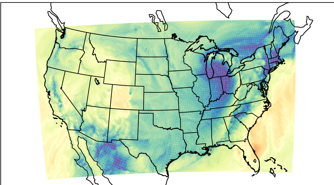
WRF (2019-11-27_17:00:00)
