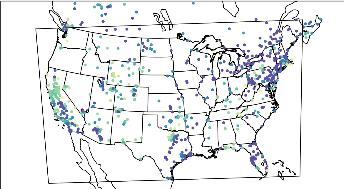
AirNOW (2019-11-27_02:00:00)
