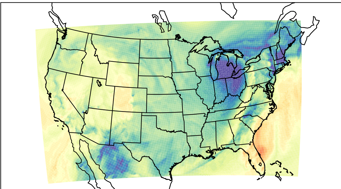
WRF (2019-11-27_19:00:00)
