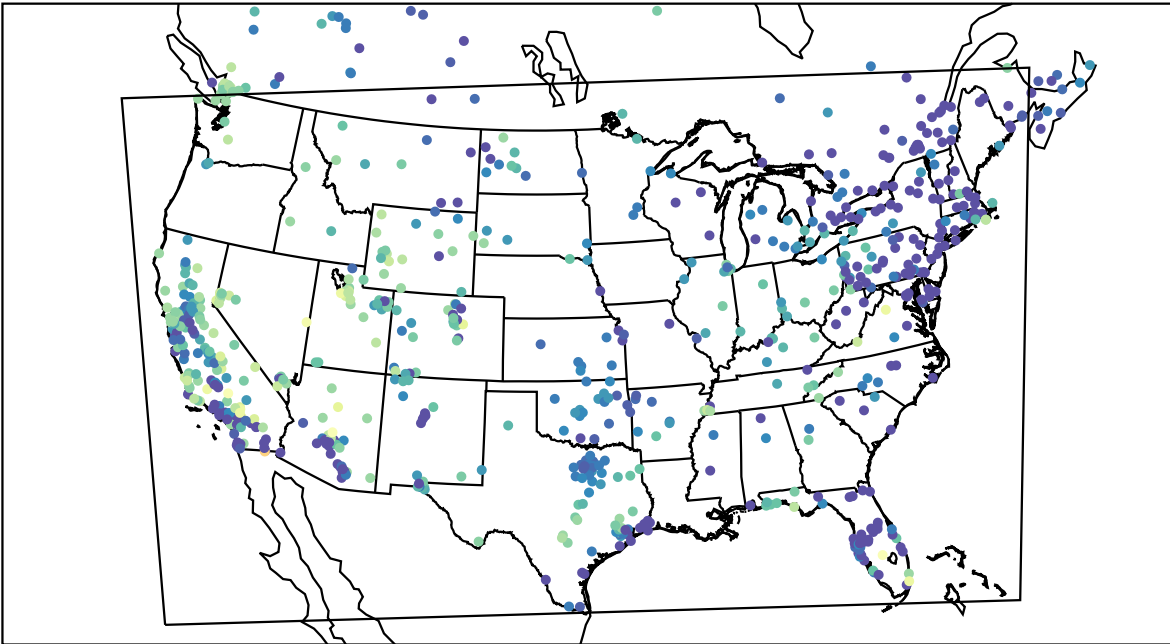
AirNOW (2019-11-27_09:00:00)
