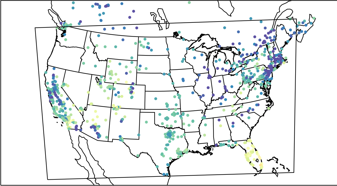
AirNOW (2019-11-27_17:00:00)
