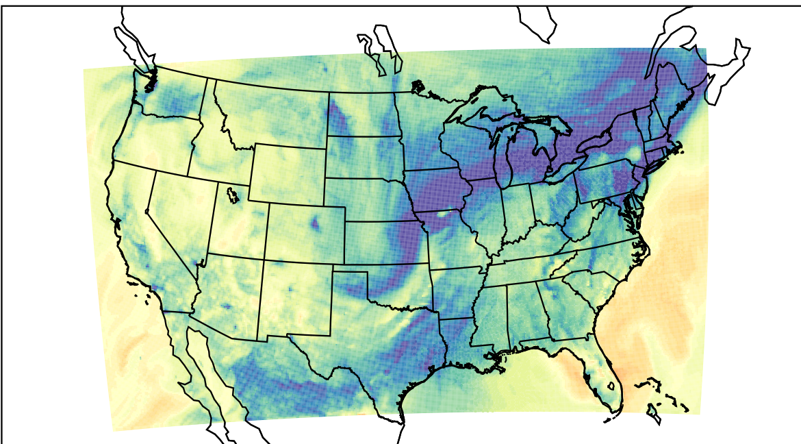
WRF (2019-11-27_03:00:00)
