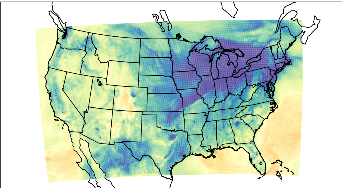
WRF (2019-11-26_02:00:00)
