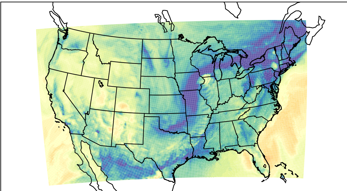
WRF (2019-11-27_07:00:00)
