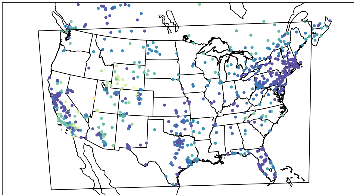
AirNOW (2019-11-28_12:00:00)
