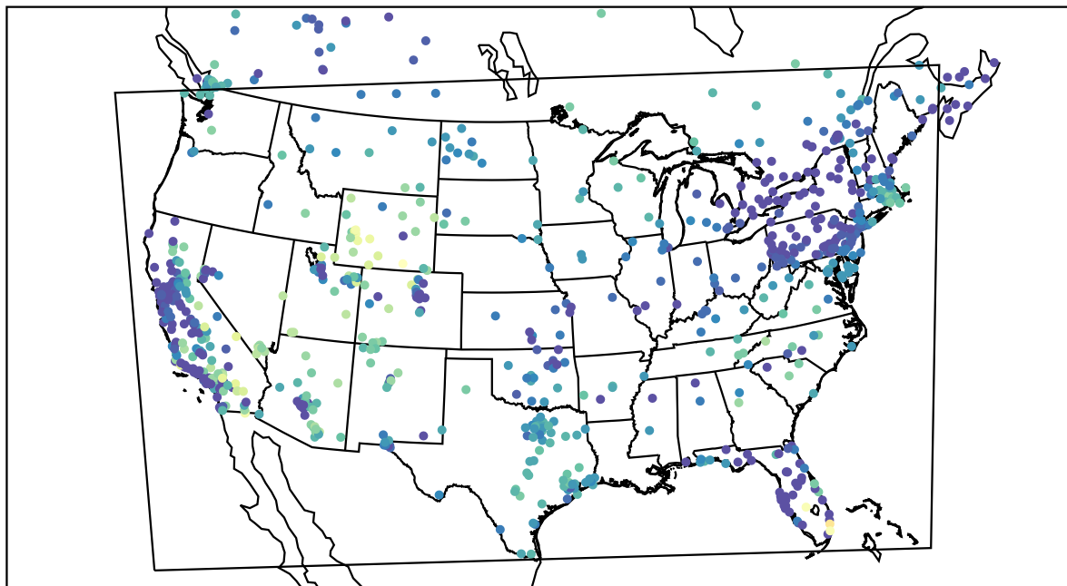
AirNOW (2019-11-28_05:00:00)
