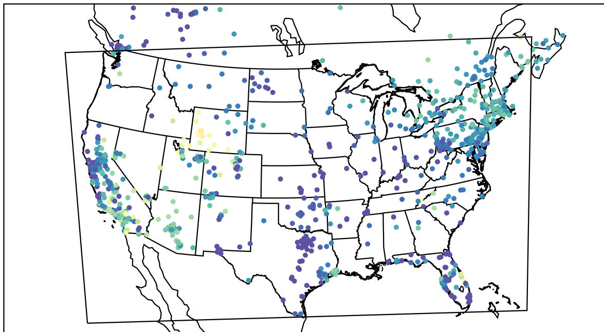
AirNOW (2019-11-29_02:00:00)
