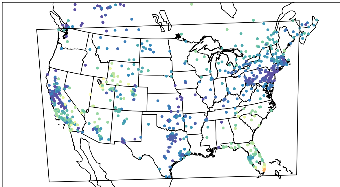
AirNOW (2019-11-28_17:00:00)
