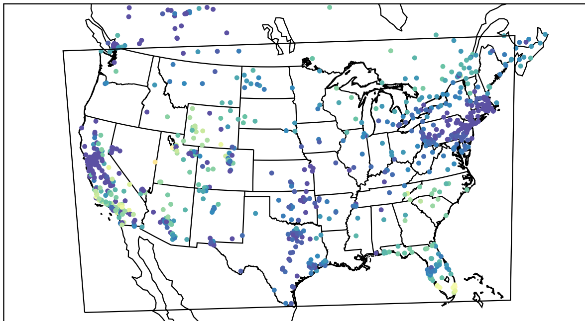
AirNOW (2019-11-28_15:00:00)
