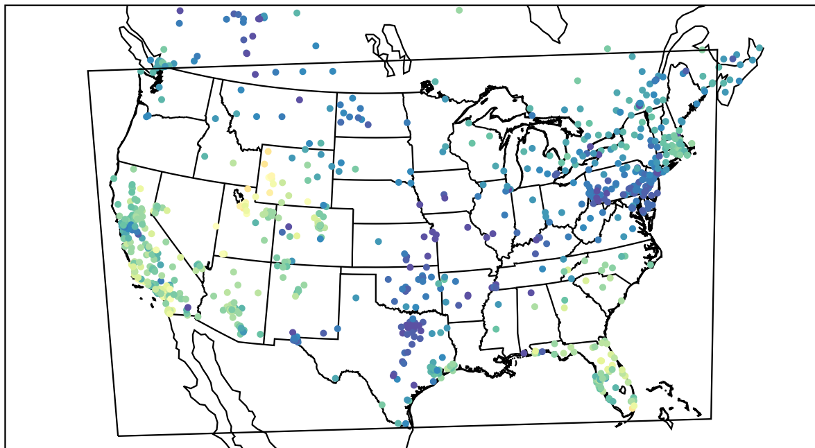
AirNOW (2019-11-28_21:00:00)
