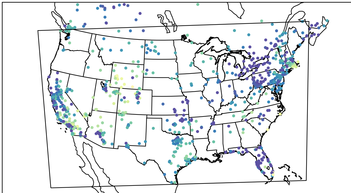
AirNOW (2019-11-28_02:00:00)
