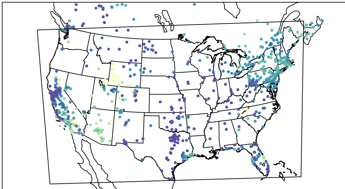
AirNOW (2019-11-29_05:00:00)
