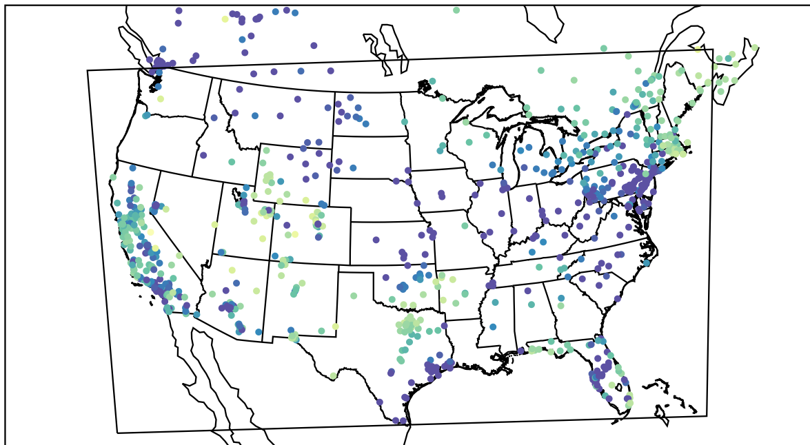
AirNOW (2019-12-01_02:00:00)
