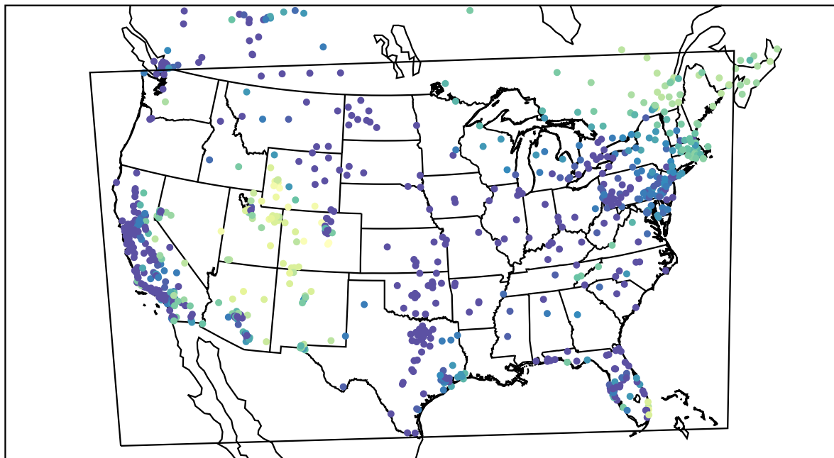
AirNOW (2019-11-30_05:00:00)
