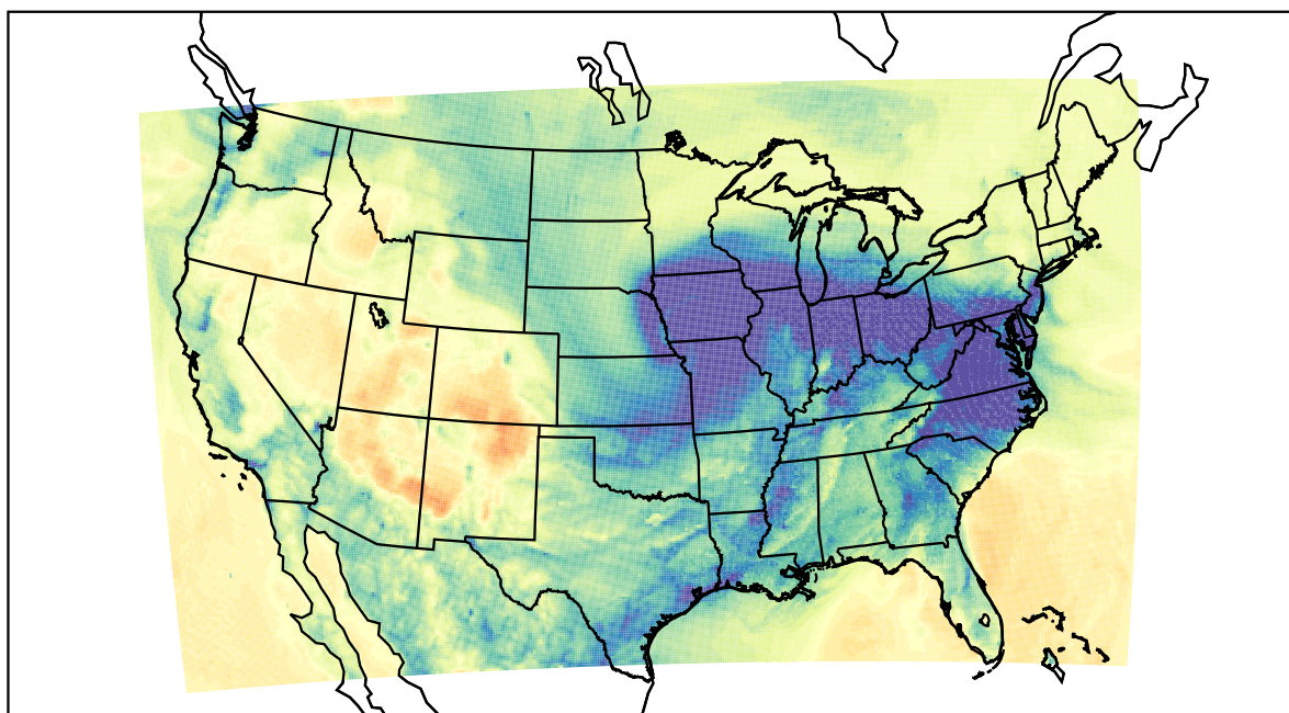
WRF (2019-12-01_05:00:00)
