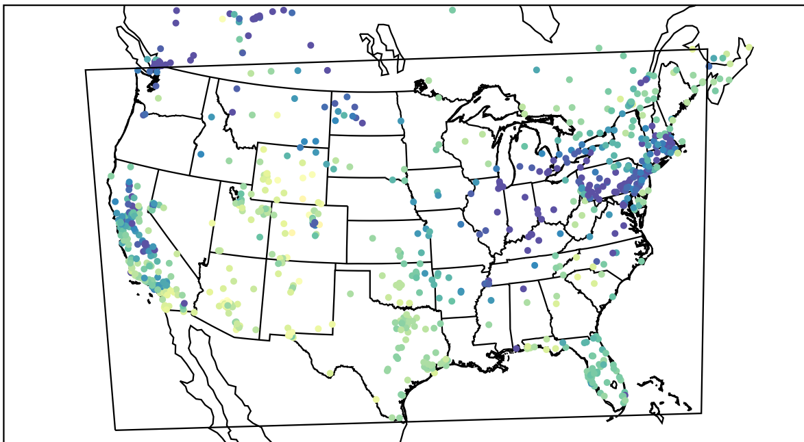
AirNOW (2019-12-01_21:00:00)
