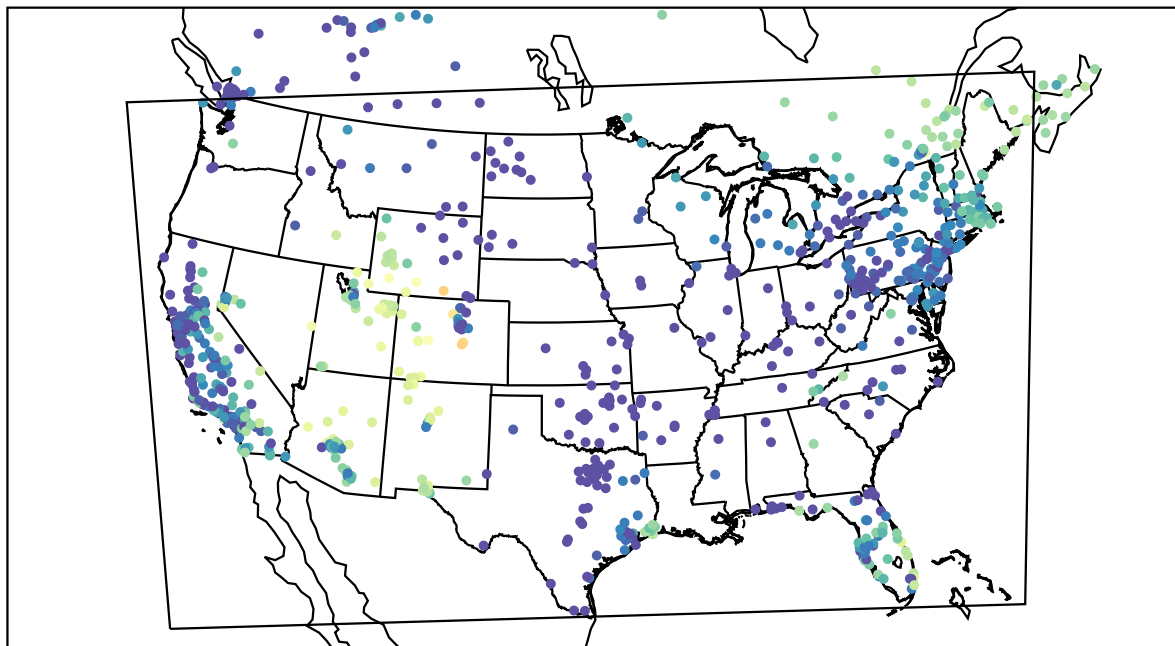
AirNOW (2019-11-30_02:00:00)
