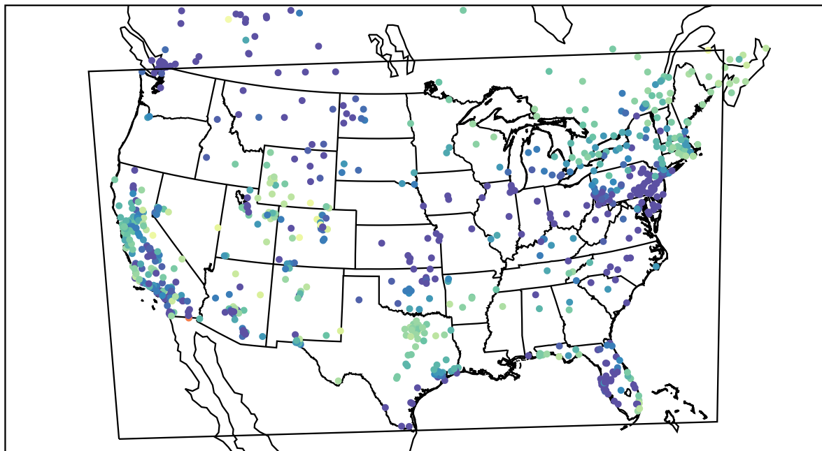
AirNOW (2019-12-01_05:00:00)
