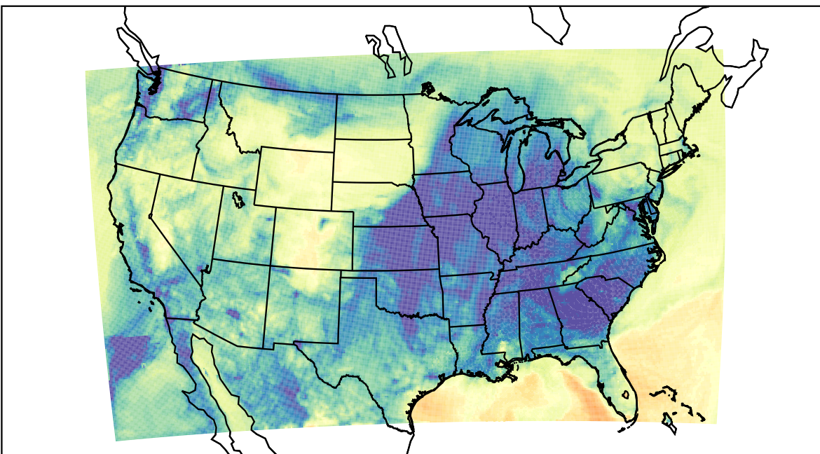
WRF (2019-12-08_05:00:00)
