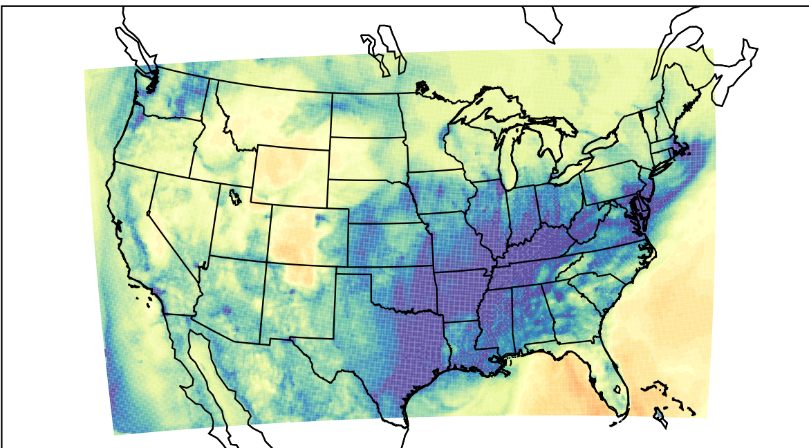
WRF (2019-12-07_05:00:00)
