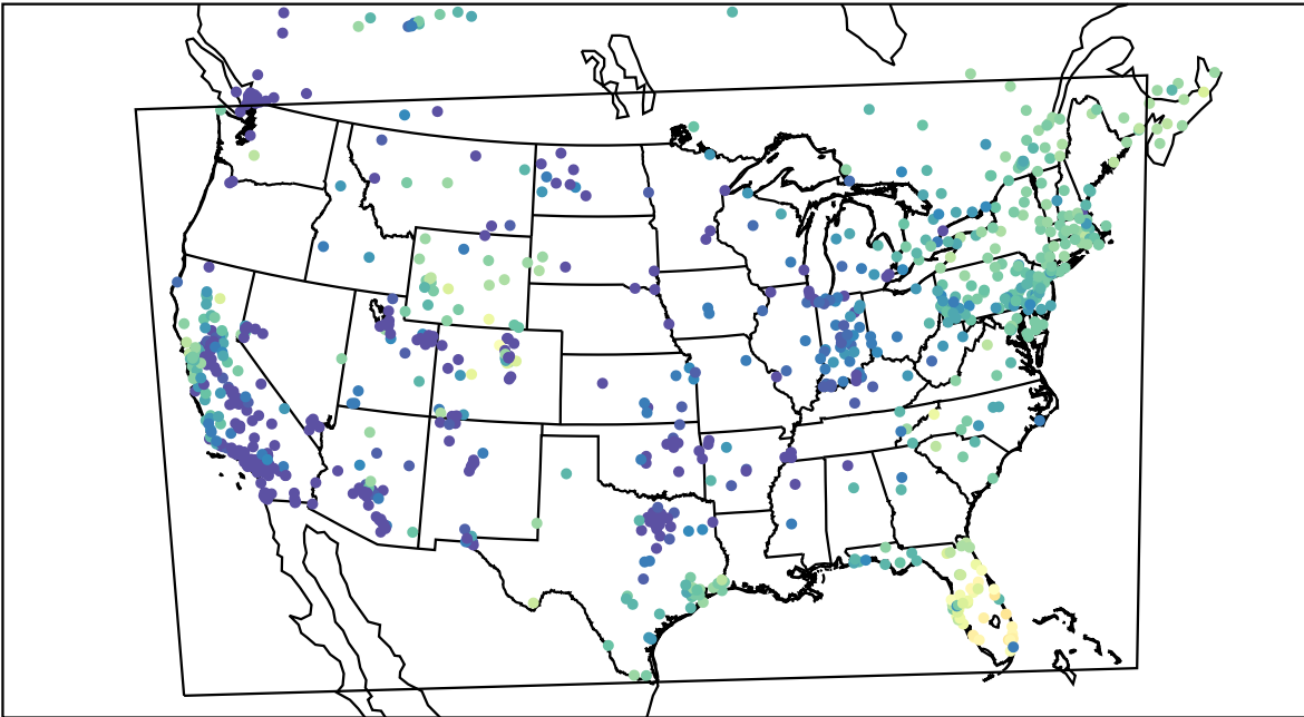
AirNOW (2019-12-07_16:00:00)
