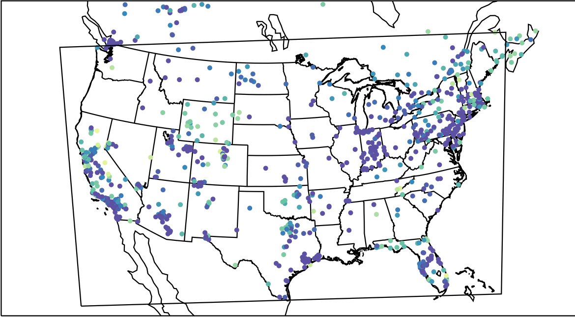
AirNOW (2019-12-08_12:00:00)
