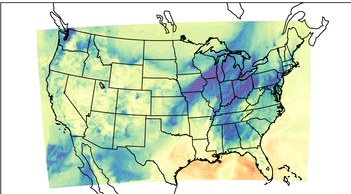
WRF (2019-12-08_21:00:00)
