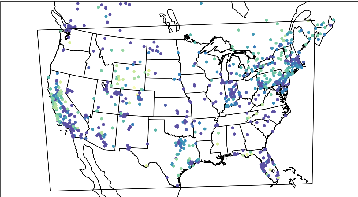
AirNOW (2019-12-07_03:00:00)
