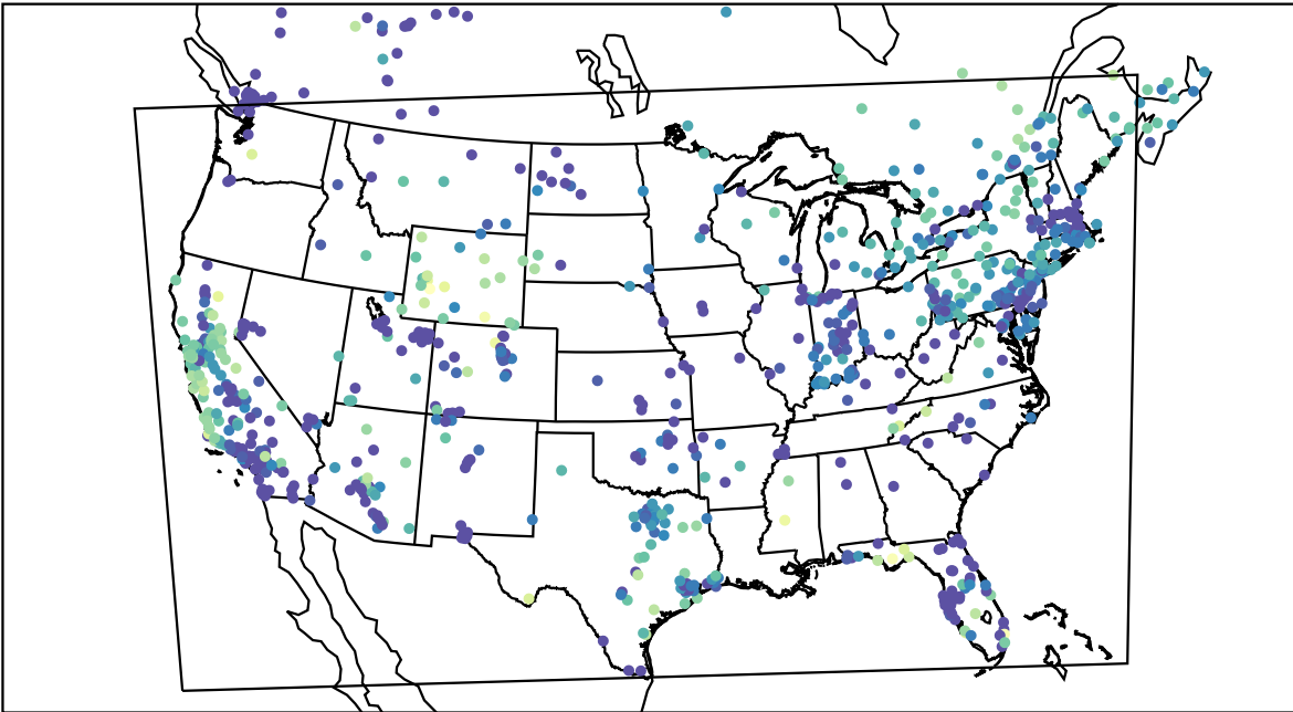
AirNOW (2019-12-07_02:00:00)
