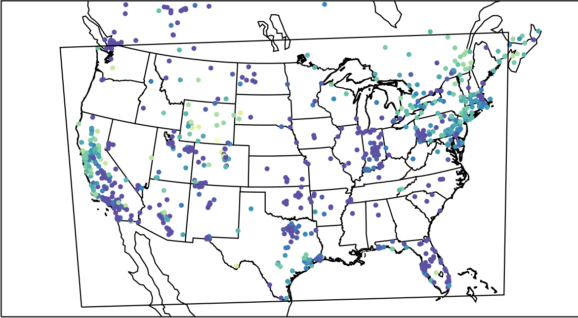
AirNOW (2019-12-07_07:00:00)
