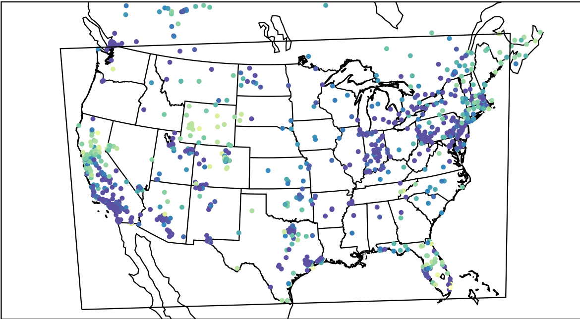
AirNOW (2019-12-08_02:00:00)
