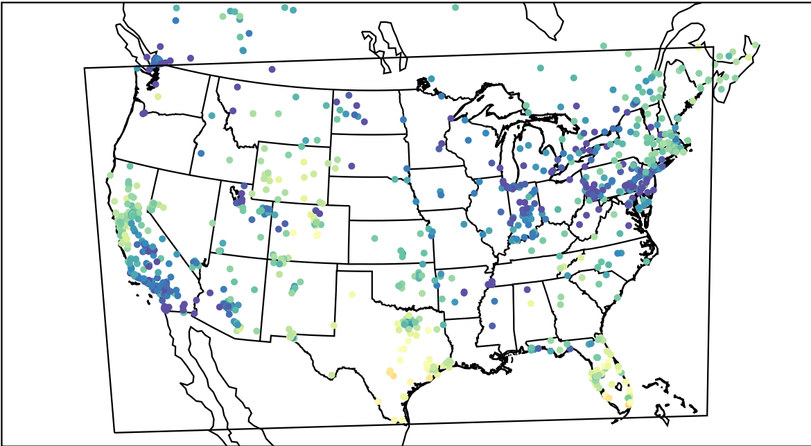
AirNOW (2019-12-07_22:00:00)
