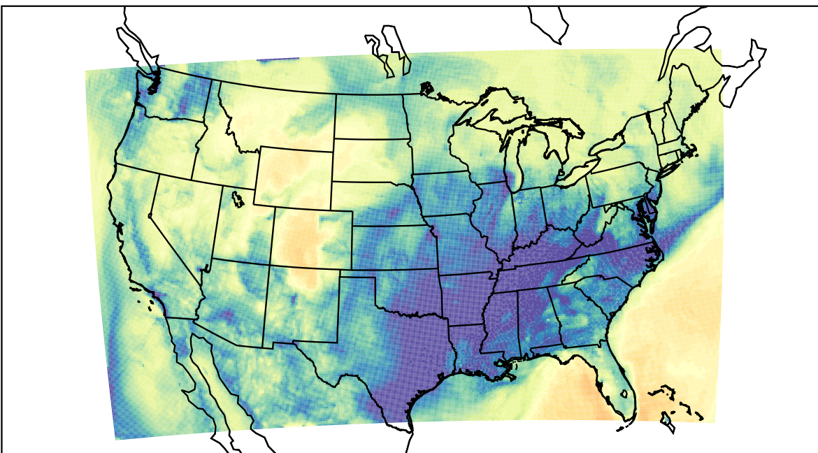
WRF (2019-12-07_10:00:00)
