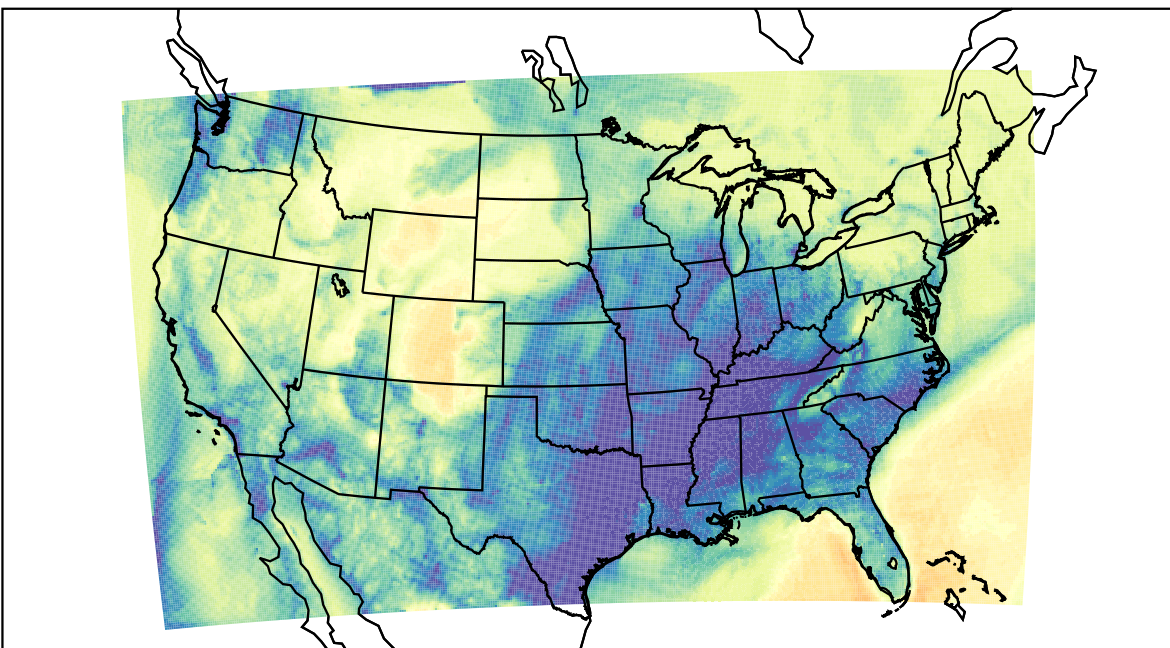
WRF (2019-12-07_14:00:00)
