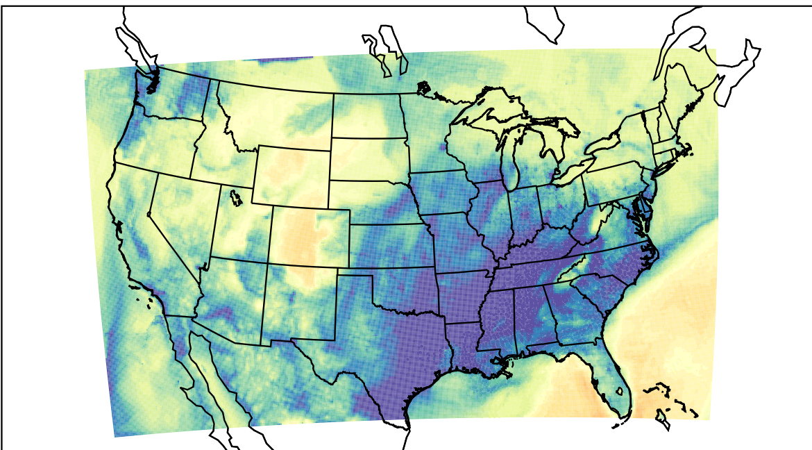
WRF (2019-12-07_13:00:00)
