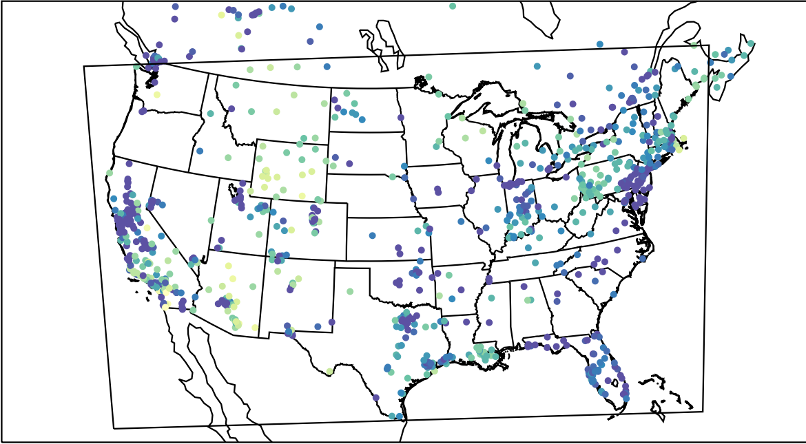
AirNOW (2019-12-18_01:00:00)
