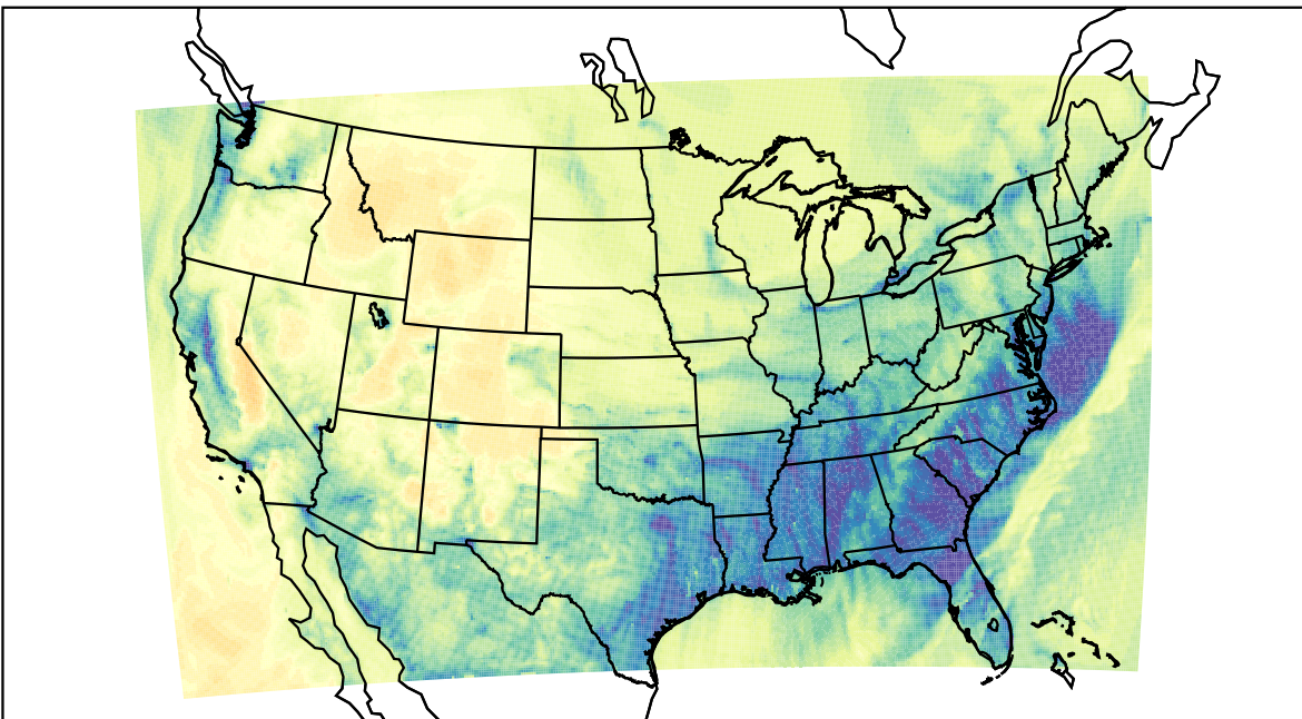
WRF (2019-12-18_05:00:00)
