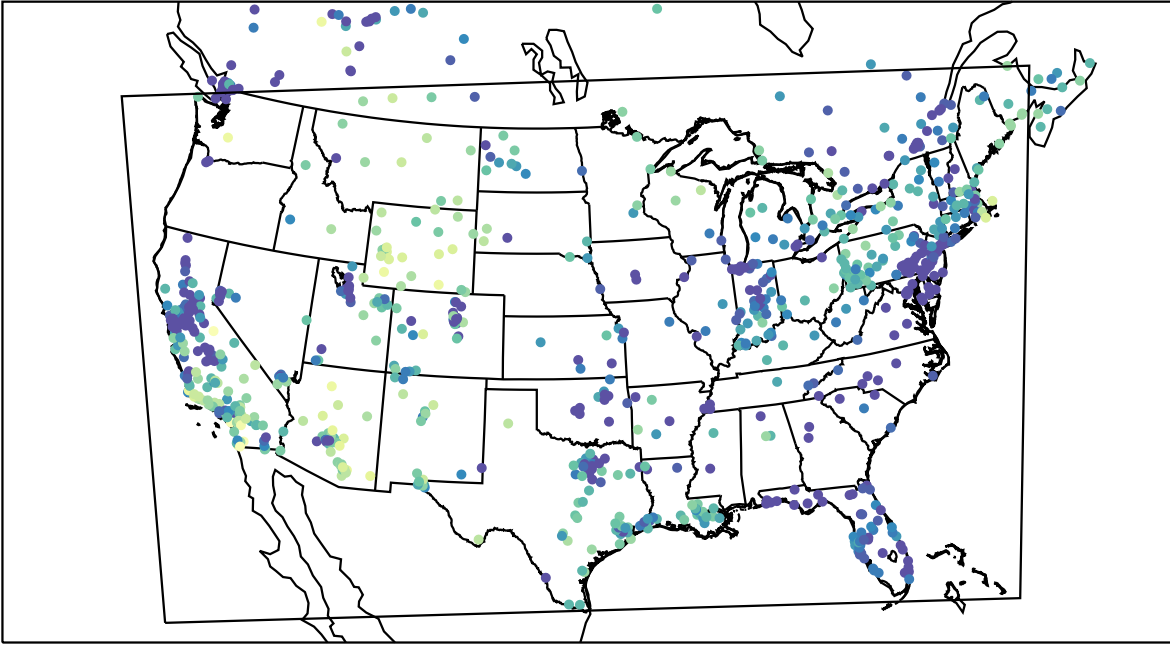
AirNOW (2019-12-18_00:00:00)
