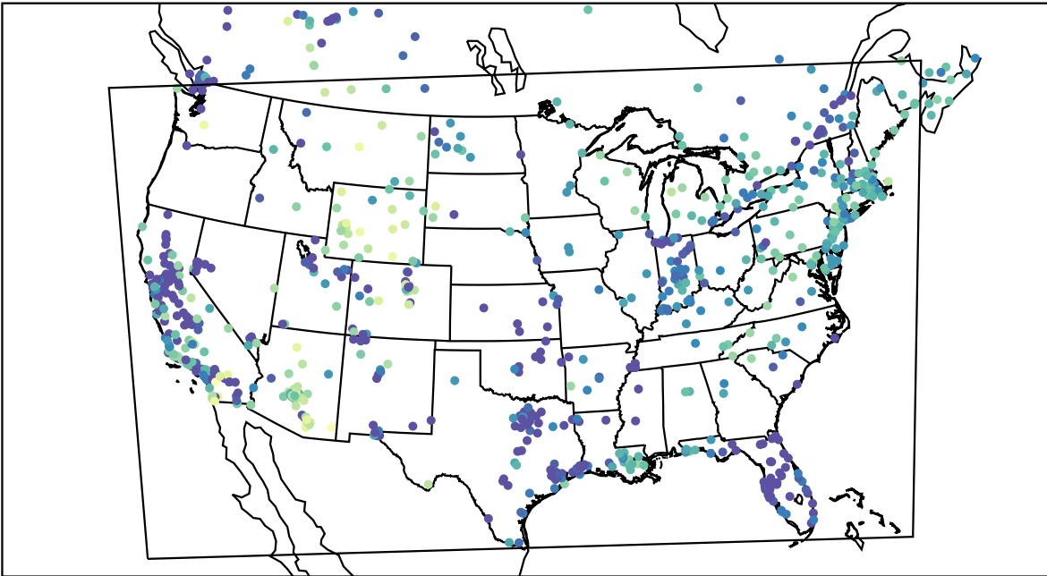
AirNOW (2019-12-18_06:00:00)
