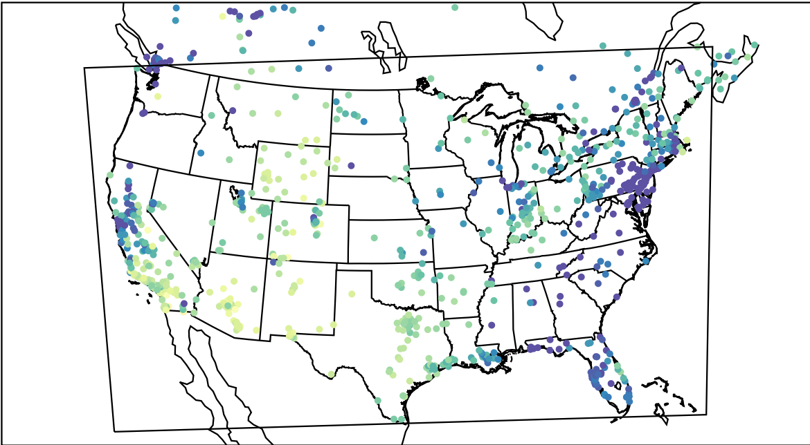
AirNOW (2019-12-17_21:00:00)
