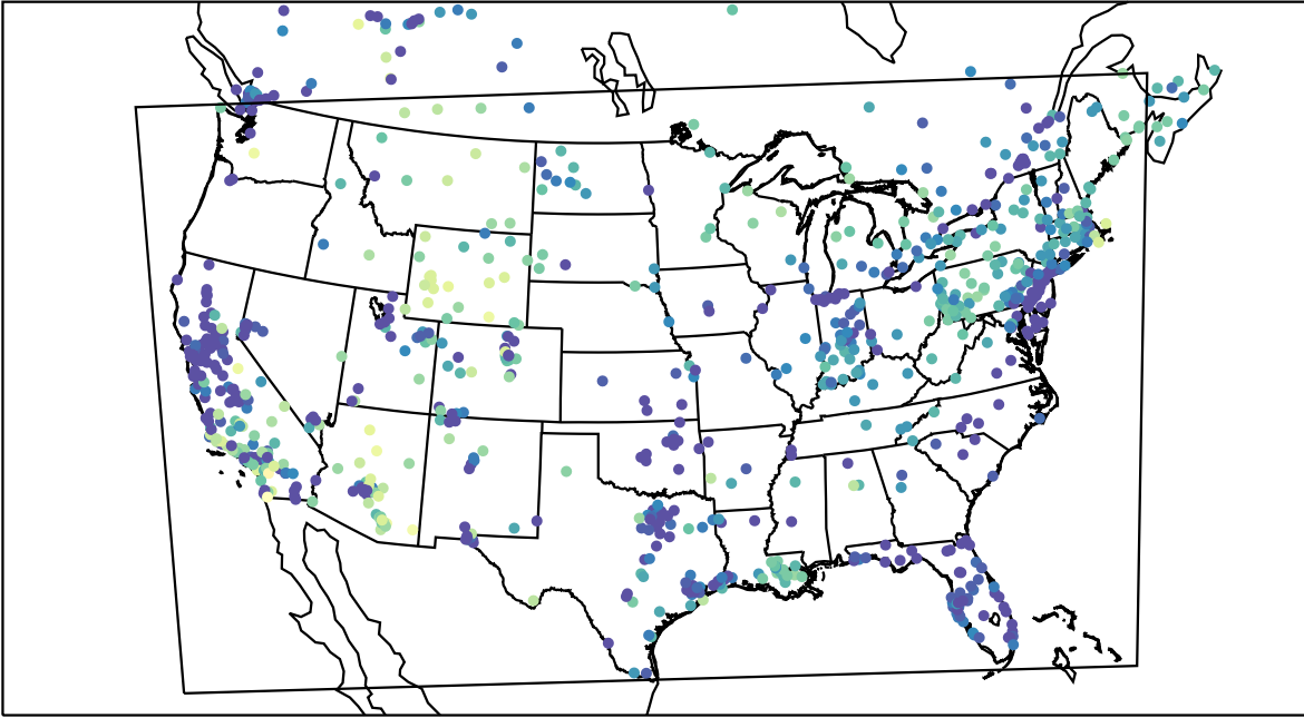
AirNOW (2019-12-18_02:00:00)
