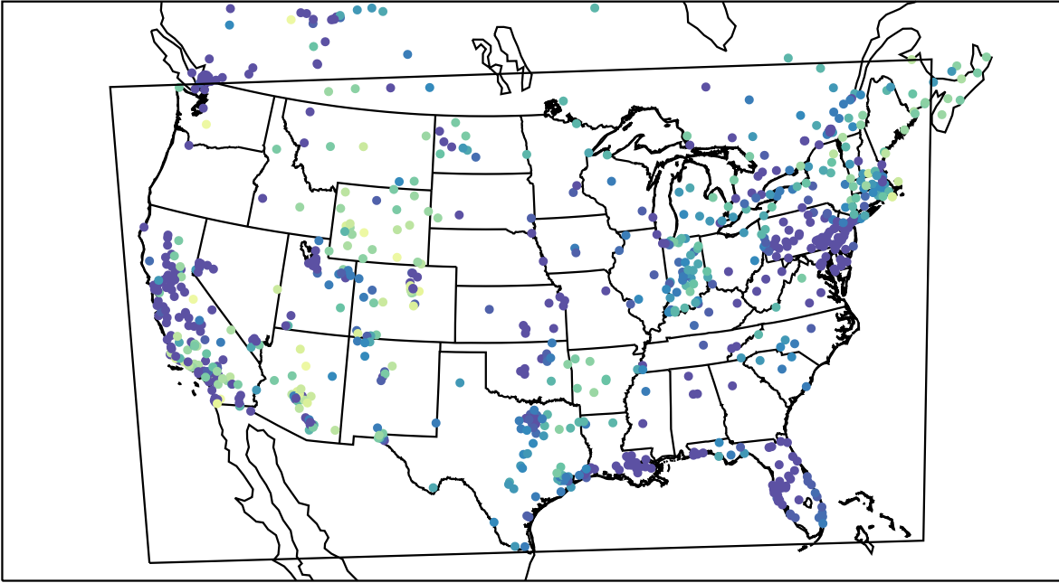
AirNOW (2019-12-17_15:00:00)
