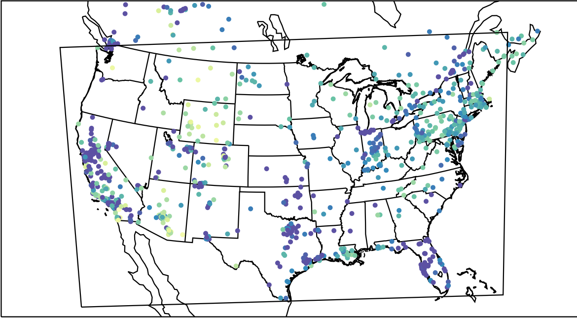
AirNOW (2019-12-18_05:00:00)
