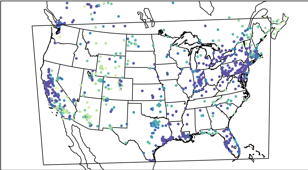
AirNOW (2019-12-17_05:00:00)
