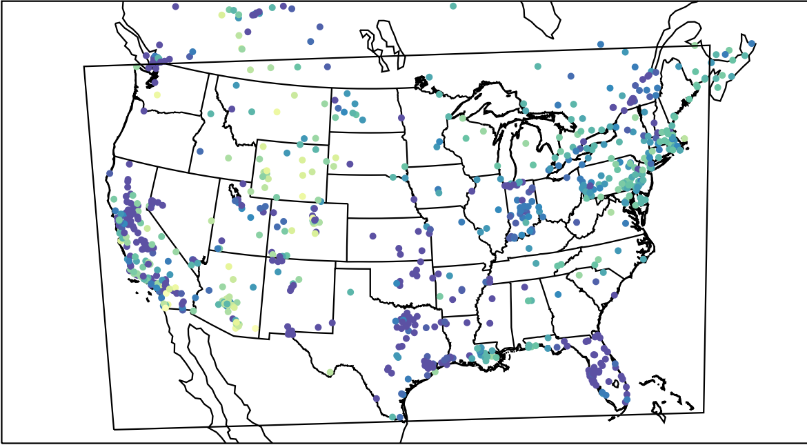
AirNOW (2019-12-18_07:00:00)
