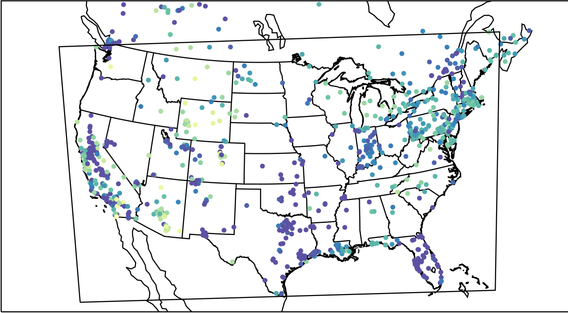
AirNOW (2019-12-18_09:00:00)
