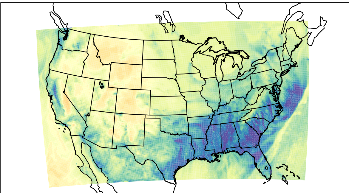
WRF (2019-12-18_07:00:00)
