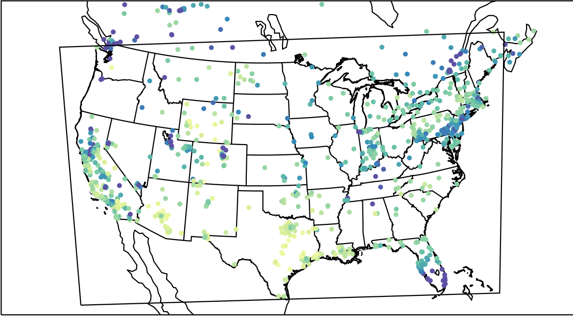
AirNOW (2019-12-18_21:00:00)
