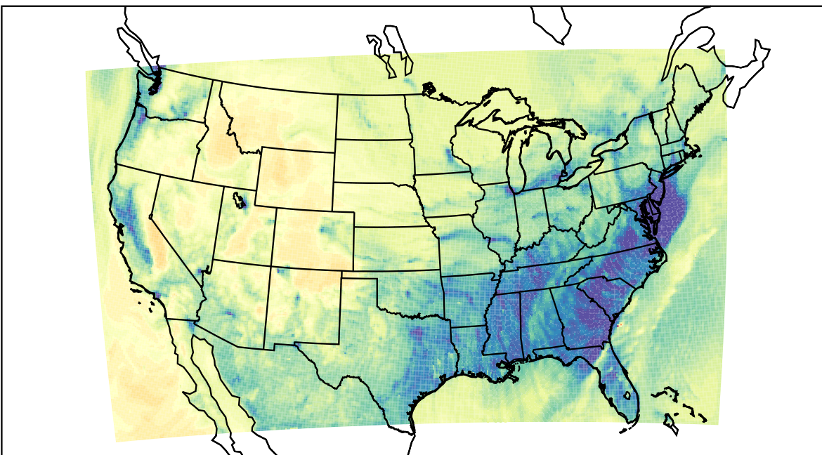
WRF (2019-12-18_02:00:00)
