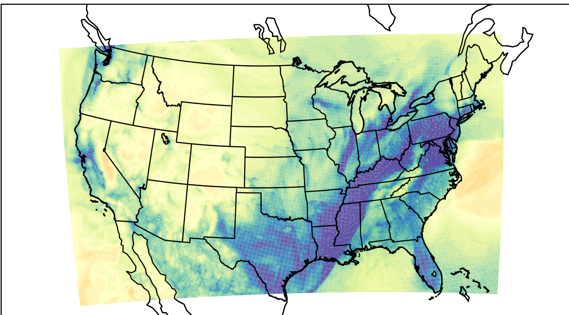
WRF (2019-12-17_05:00:00)
