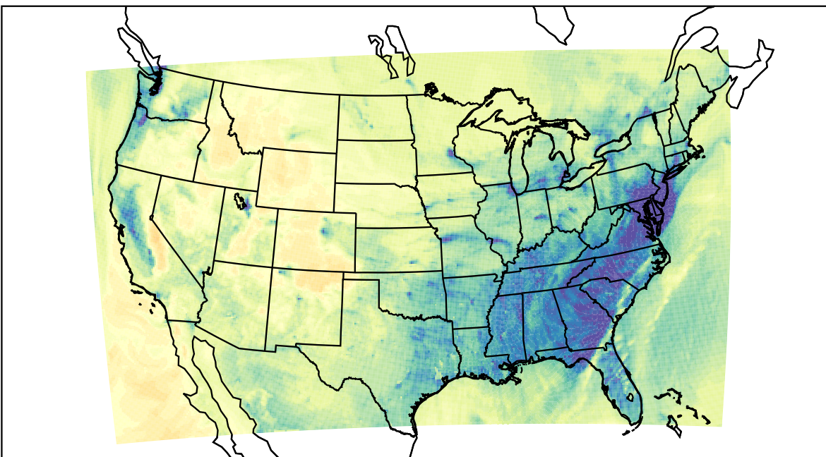
WRF (2019-12-18_00:00:00)
