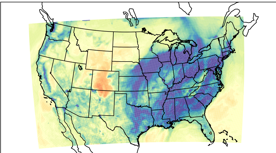
WRF (2019-12-22_02:00:00)
