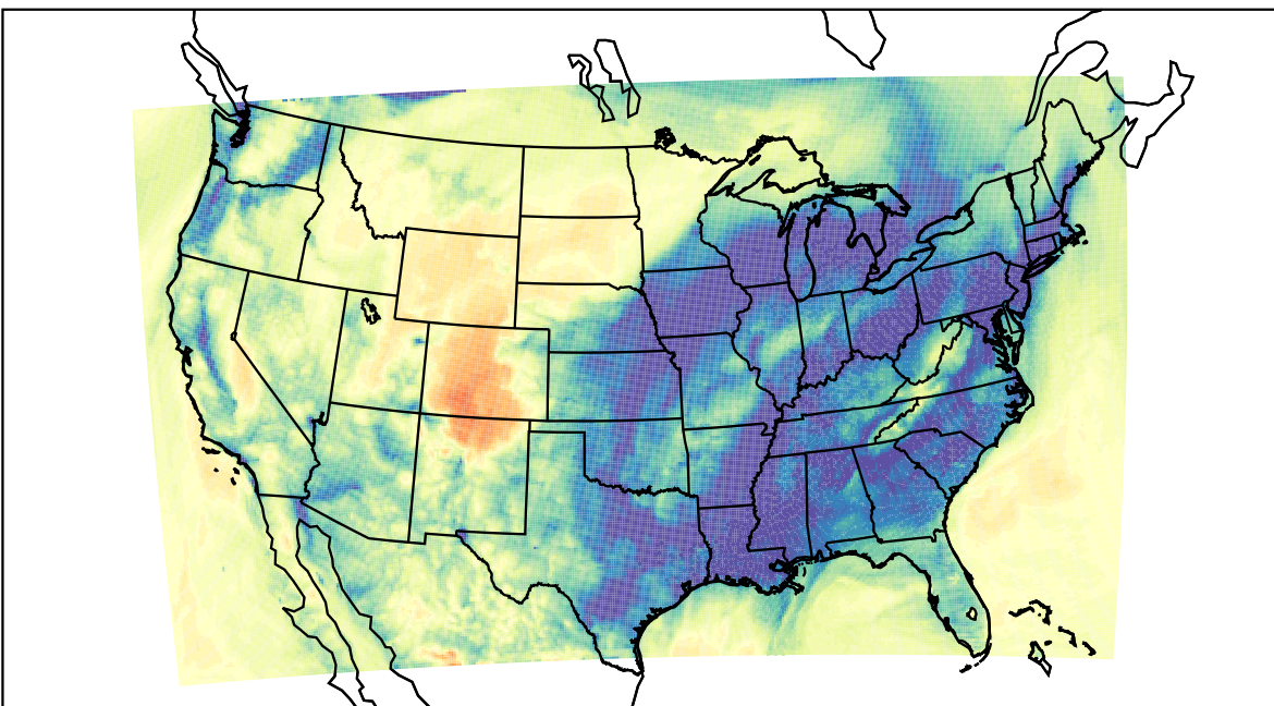
WRF (2019-12-22_07:00:00)
