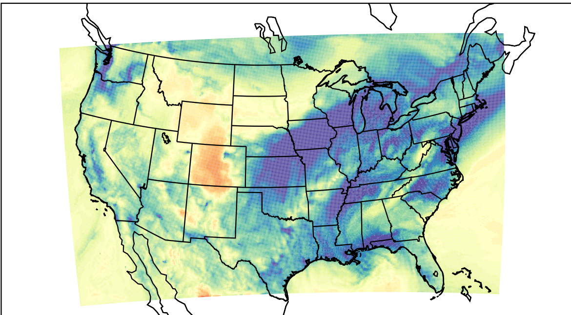
WRF (2019-12-23_05:00:00)
