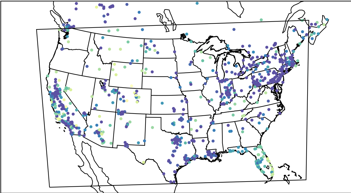
AirNOW (2019-12-22_01:00:00)
