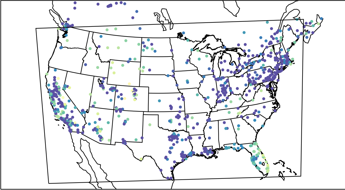
AirNOW (2019-12-22_03:00:00)
