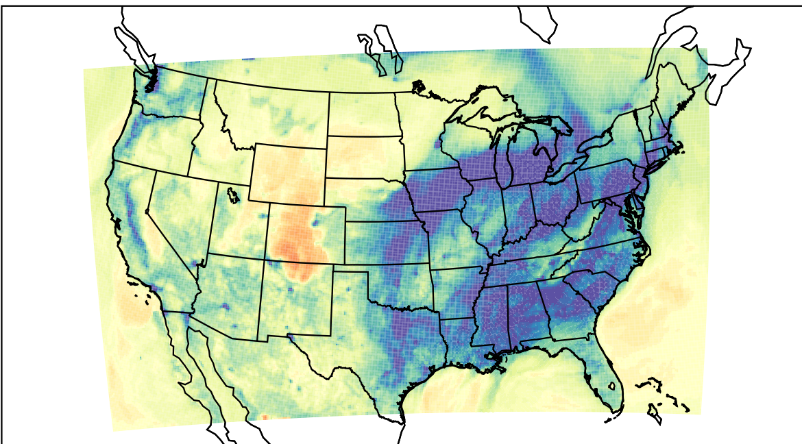
WRF (2019-12-22_01:00:00)
