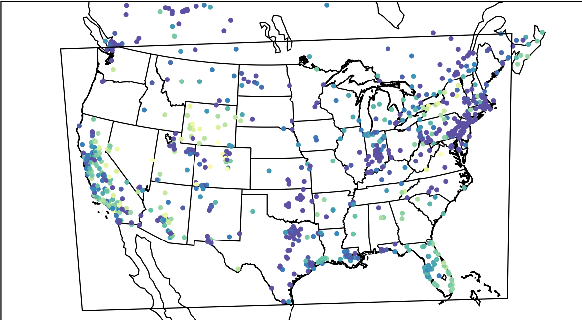
AirNOW (2019-12-23_02:00:00)
