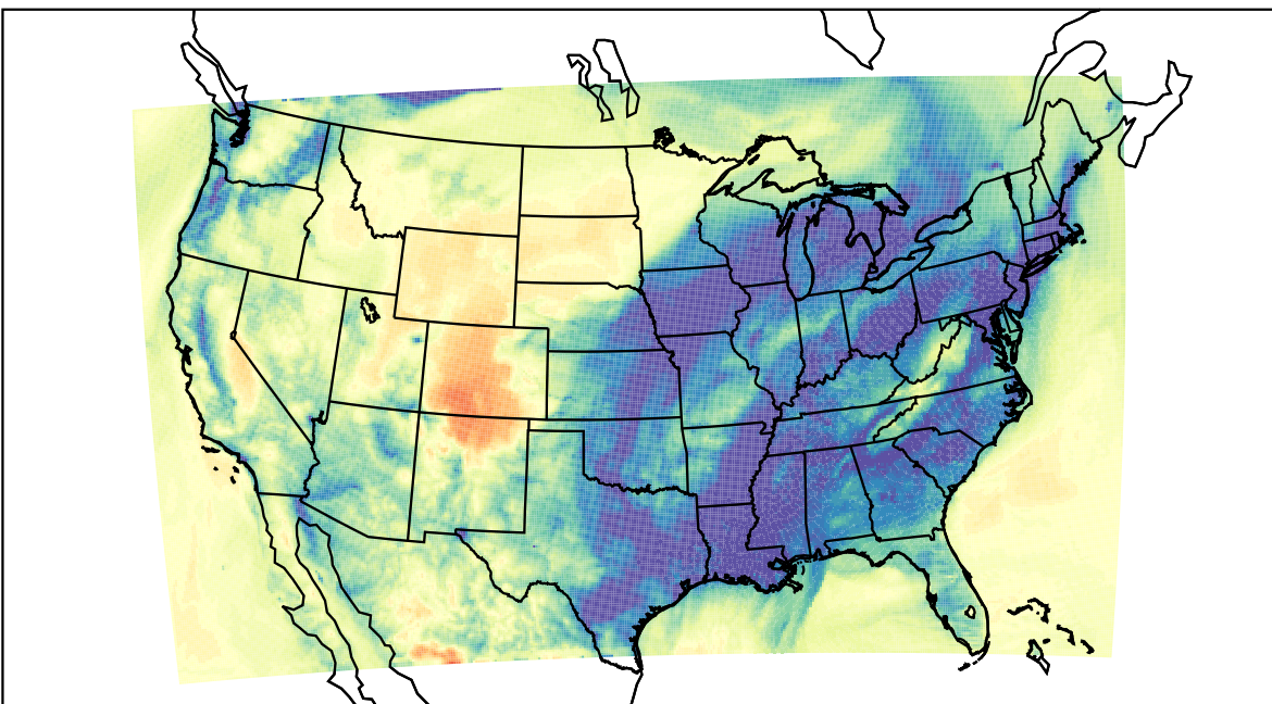
WRF (2019-12-22_09:00:00)
