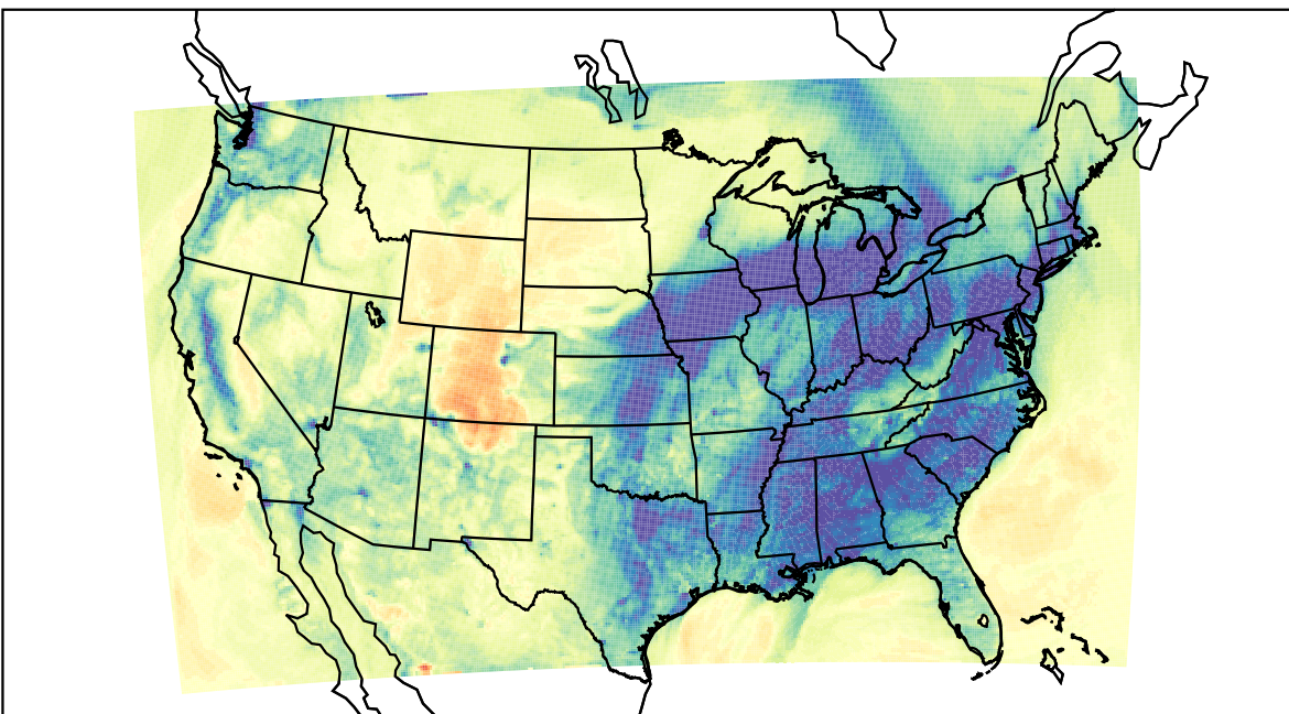
WRF (2019-12-22_00:00:00)
