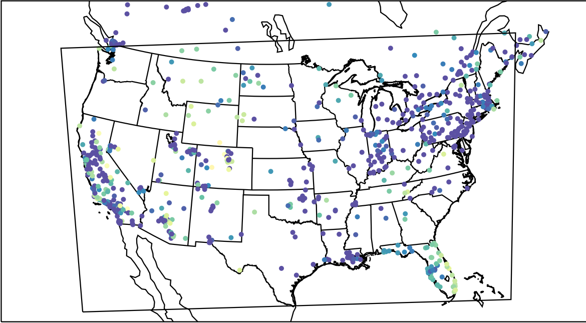
AirNOW (2019-12-22_04:00:00)
