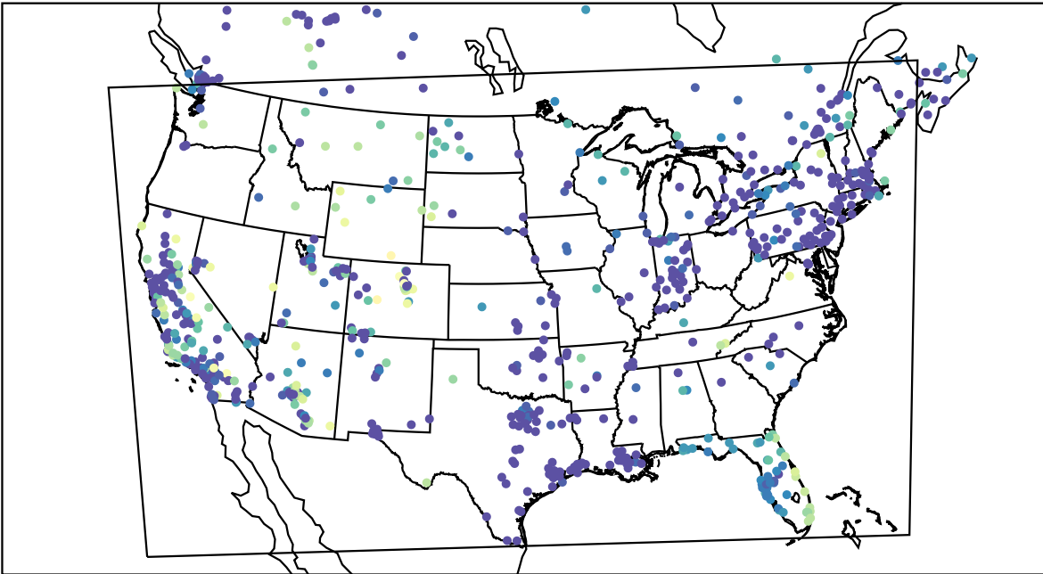
AirNOW (2019-12-22_07:00:00)
