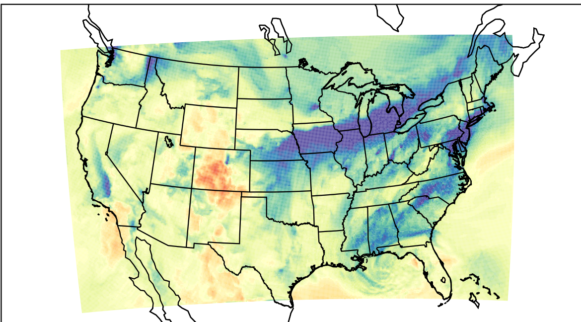
WRF (2019-12-23_21:00:00)
