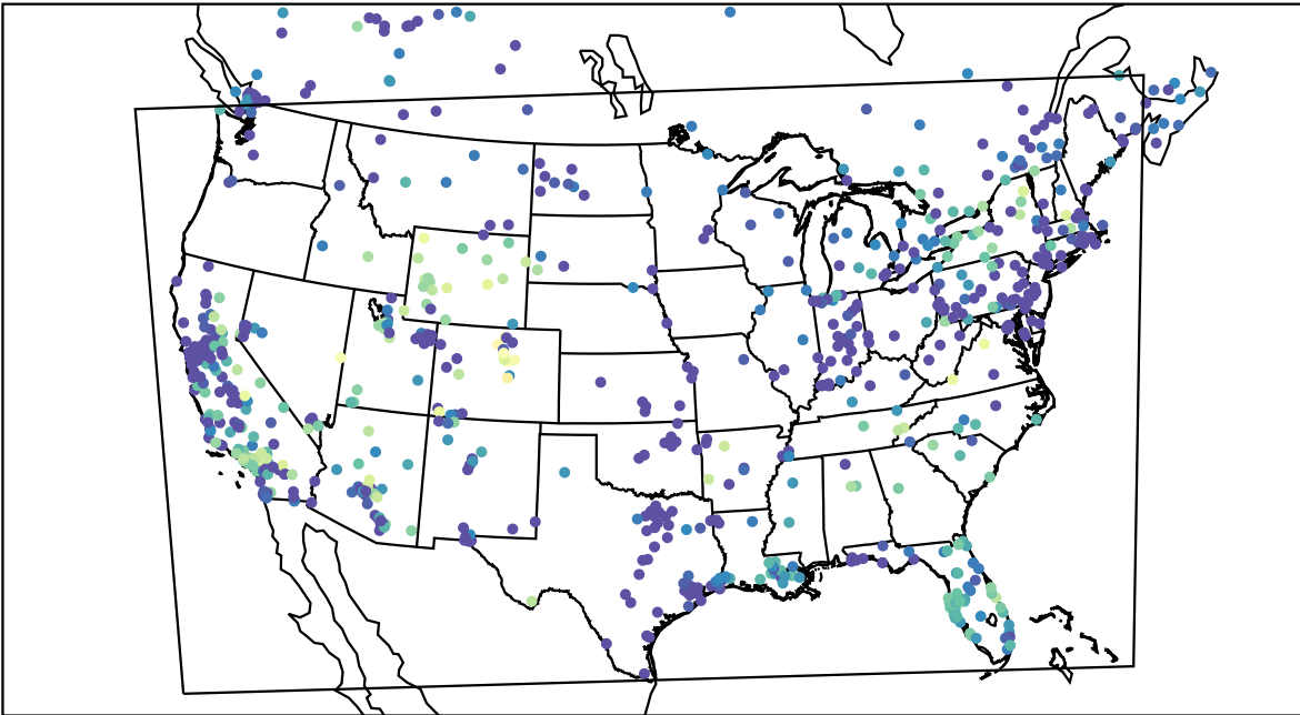
AirNOW (2019-12-23_09:00:00)
