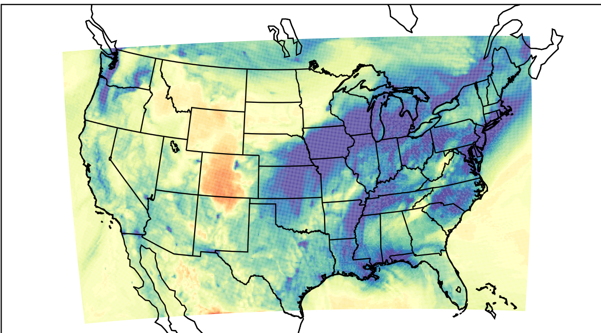
WRF (2019-12-23_02:00:00)
