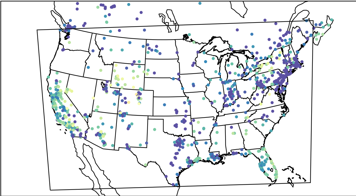
AirNOW (2019-12-23_01:00:00)
