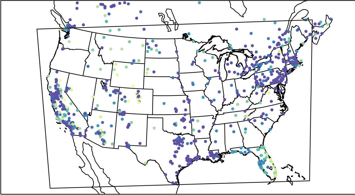
AirNOW (2019-12-22_05:00:00)
