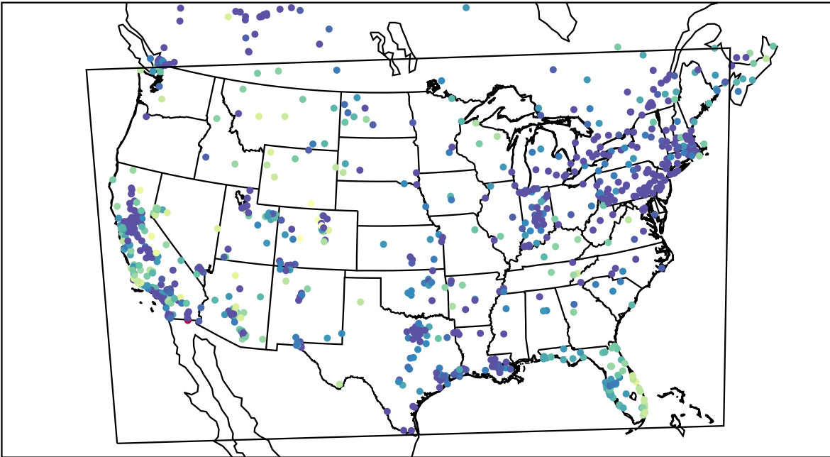
AirNOW (2019-12-22_00:00:00)
