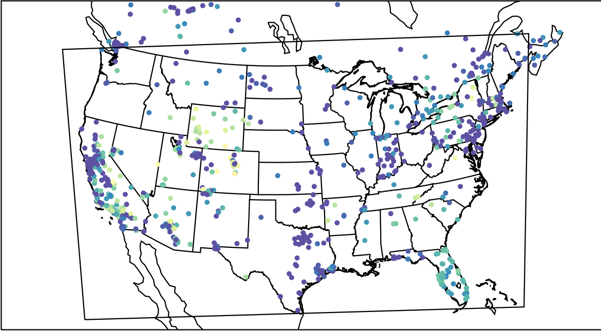
AirNOW (2019-12-23_07:00:00)
