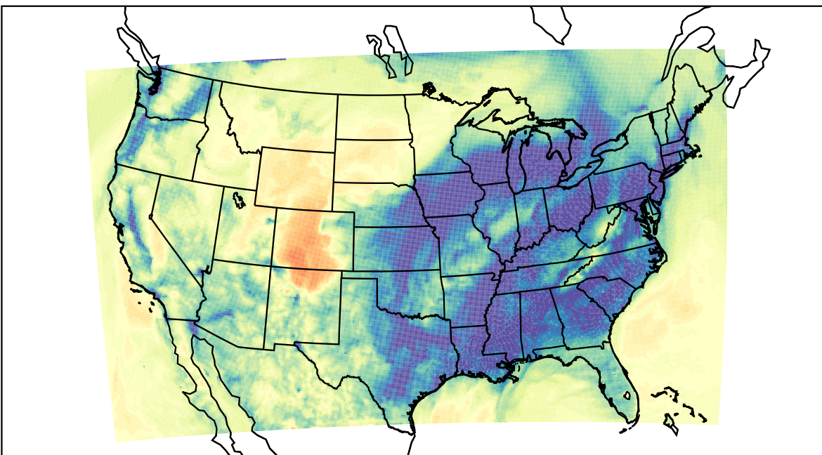
WRF (2019-12-22_05:00:00)
