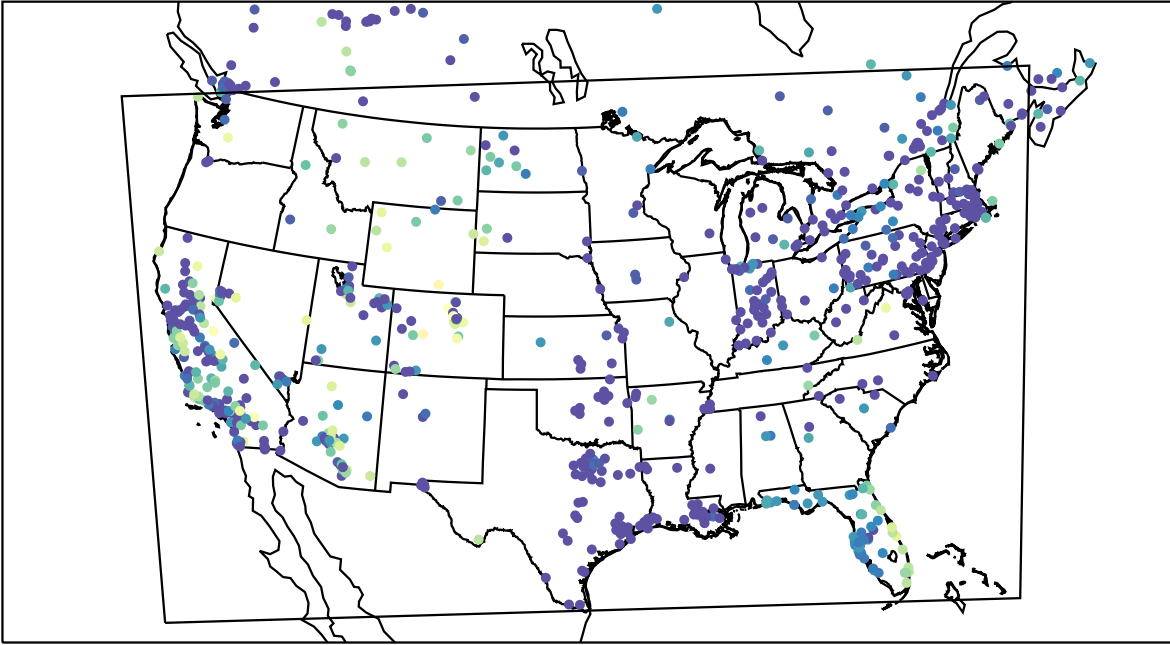
AirNOW (2019-12-22_08:00:00)
