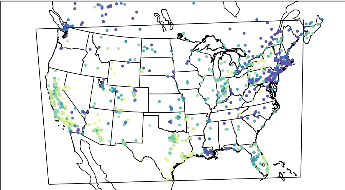
AirNOW (2019-12-22_21:00:00)
