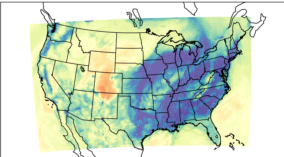
WRF (2019-12-22_04:00:00)
