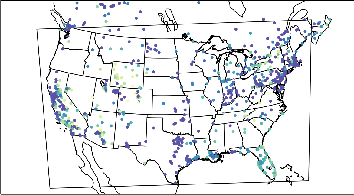
AirNOW (2019-12-23_05:00:00)
