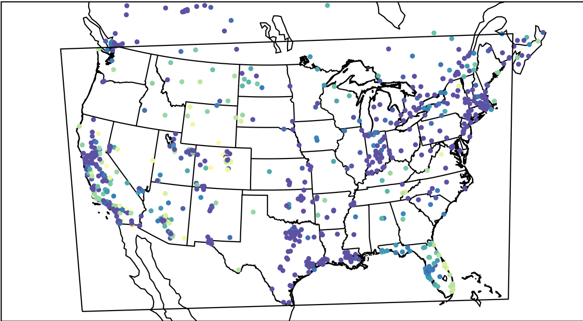
AirNOW (2019-12-22_06:00:00)
