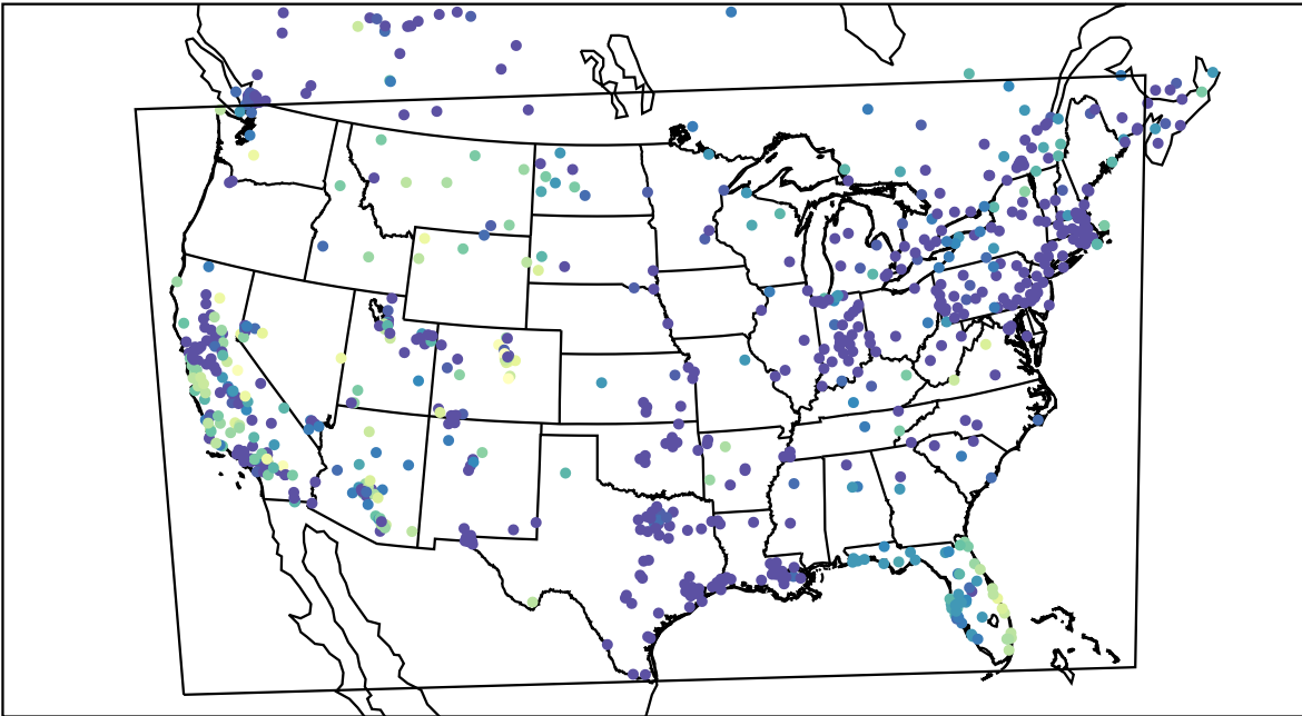
AirNOW (2019-12-22_09:00:00)
