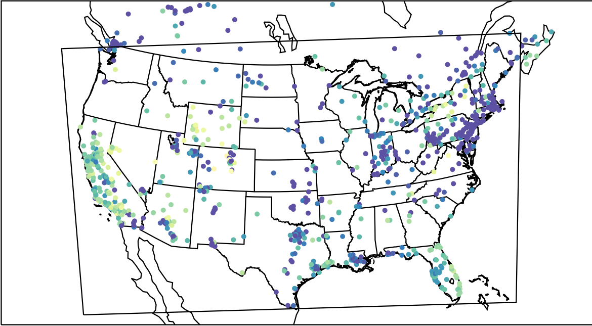
AirNOW (2019-12-23_00:00:00)
