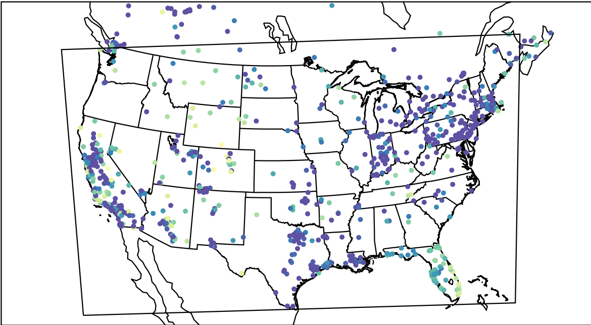
AirNOW (2019-12-22_02:00:00)
