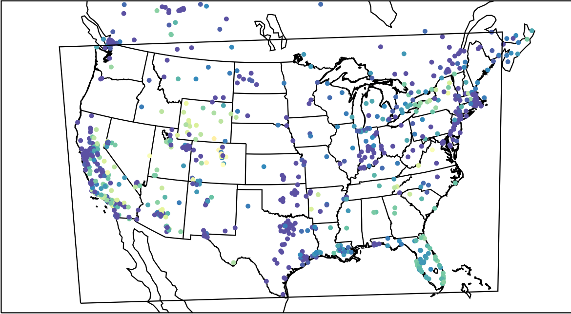
AirNOW (2019-12-23_06:00:00)
