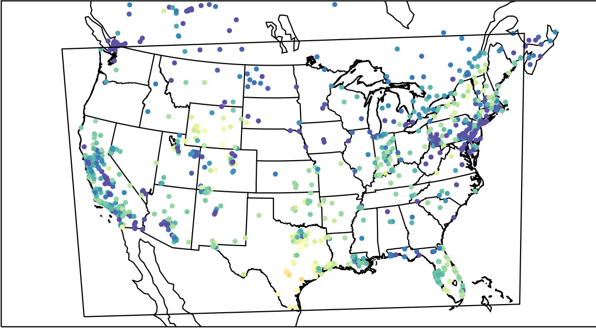
AirNOW (2019-12-23_21:00:00)
