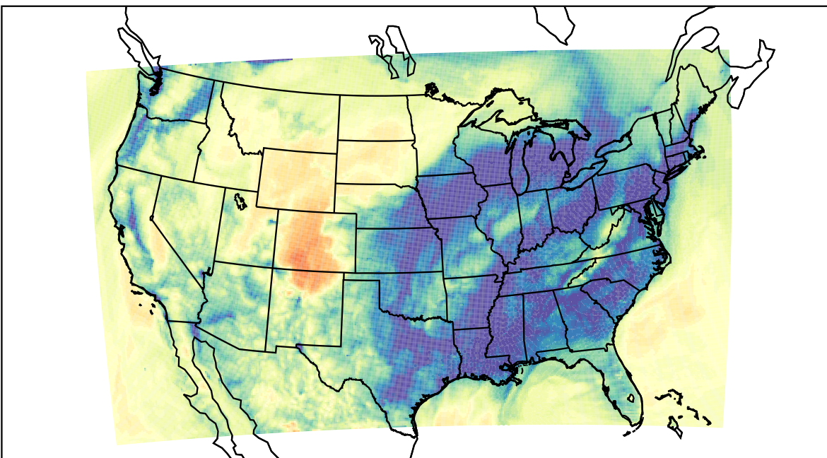
WRF (2019-12-22_06:00:00)
