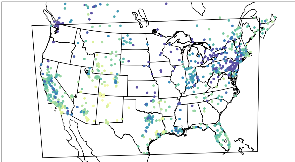
AirNOW (2019-12-26_21:00:00)
