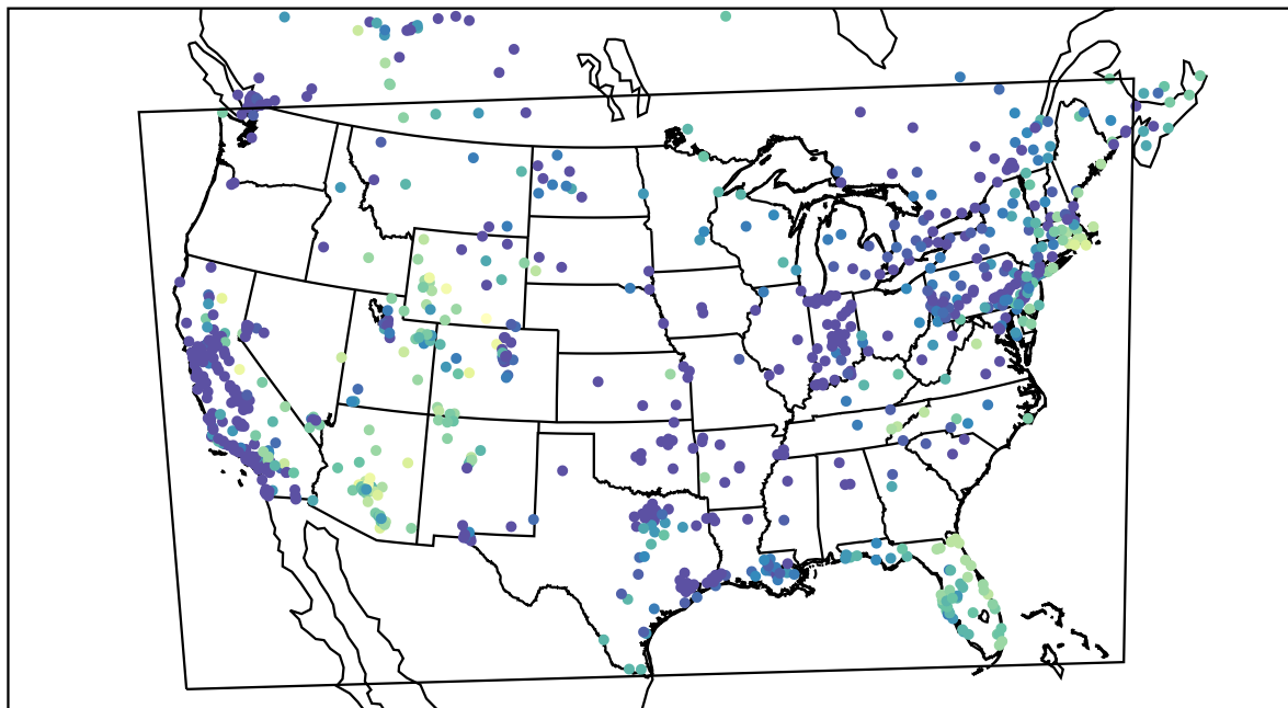
AirNOW (2019-12-27_16:00:00)
