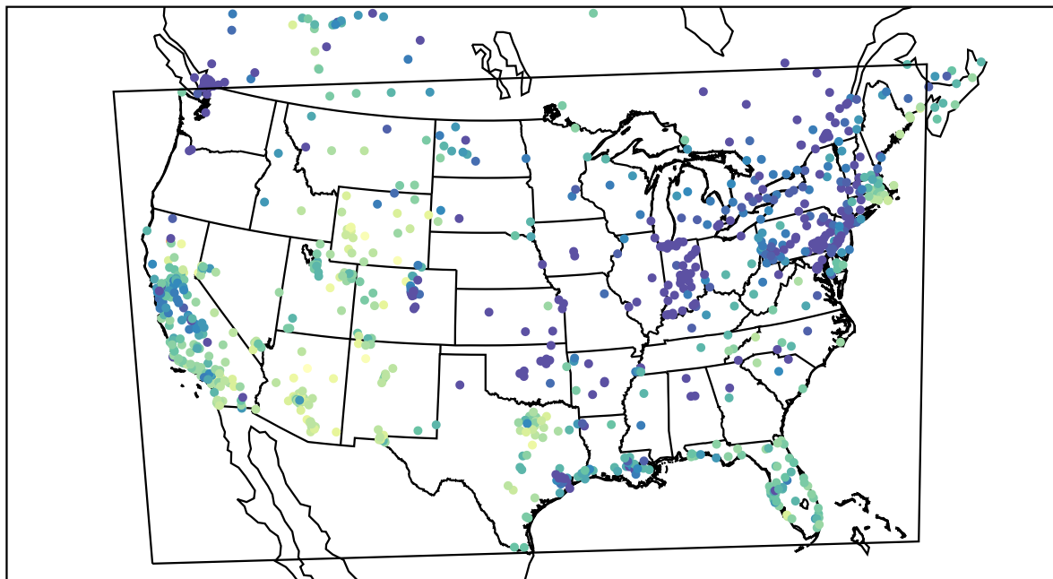
AirNOW (2019-12-27_21:00:00)
