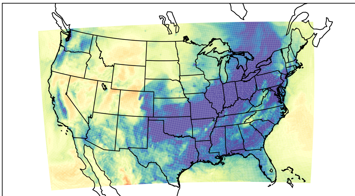
WRF (2019-12-27_14:00:00)
