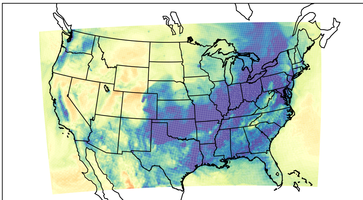
WRF (2019-12-27_15:00:00)
