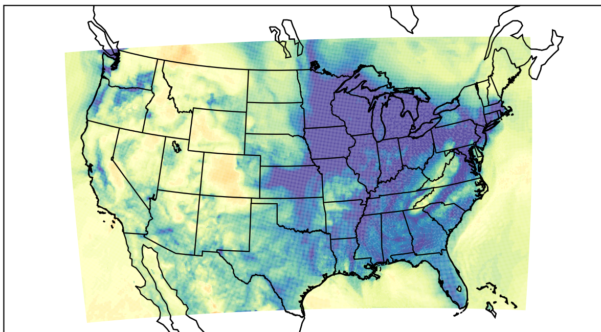
WRF (2019-12-26_09:00:00)
