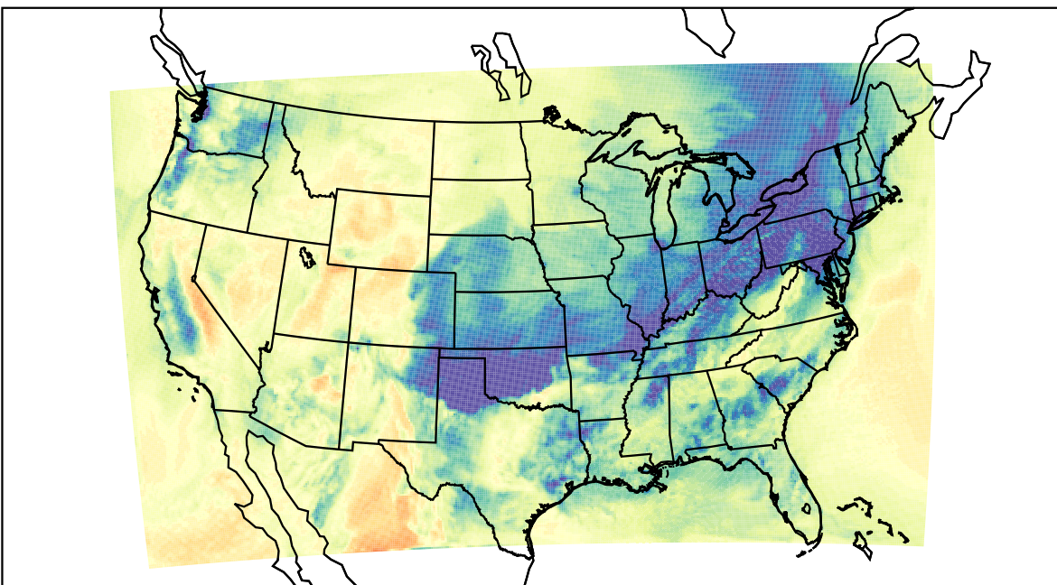
WRF (2019-12-27_19:00:00)
