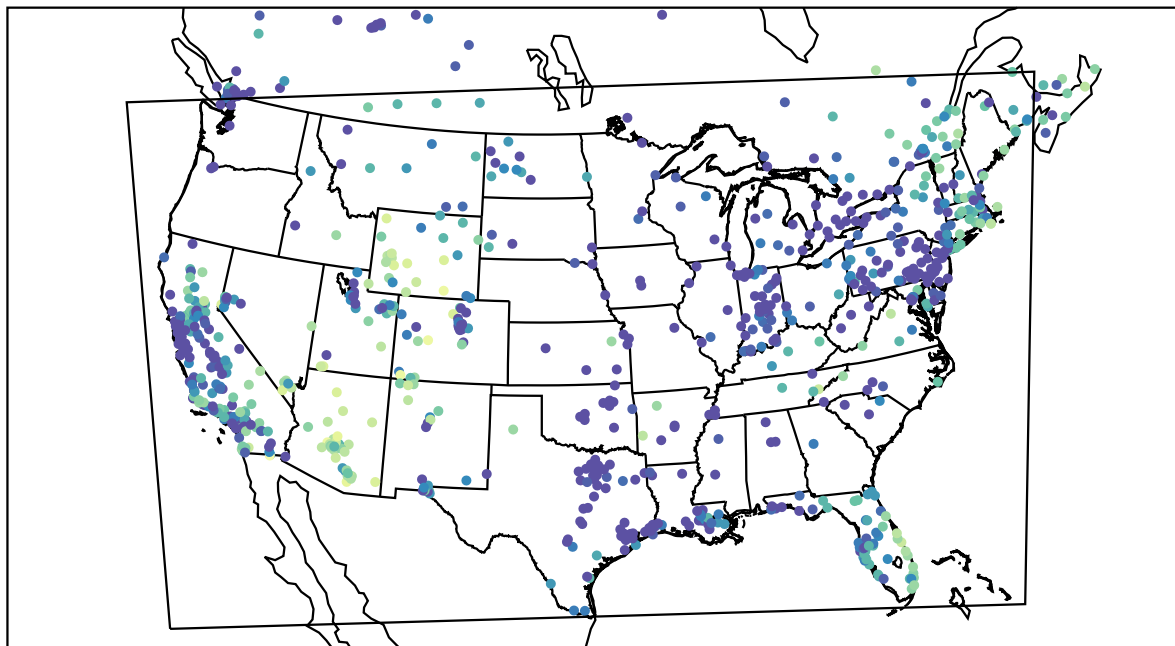
AirNOW (2019-12-27_02:00:00)
