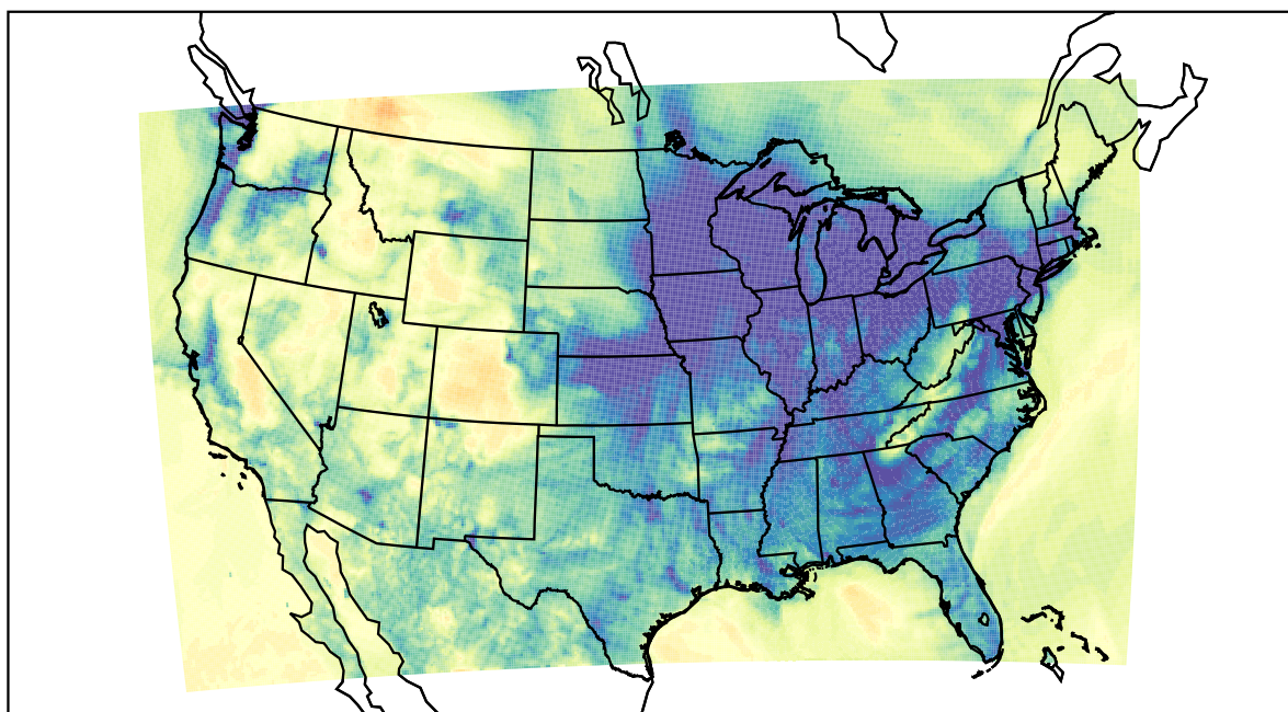
WRF (2019-12-26_05:00:00)
