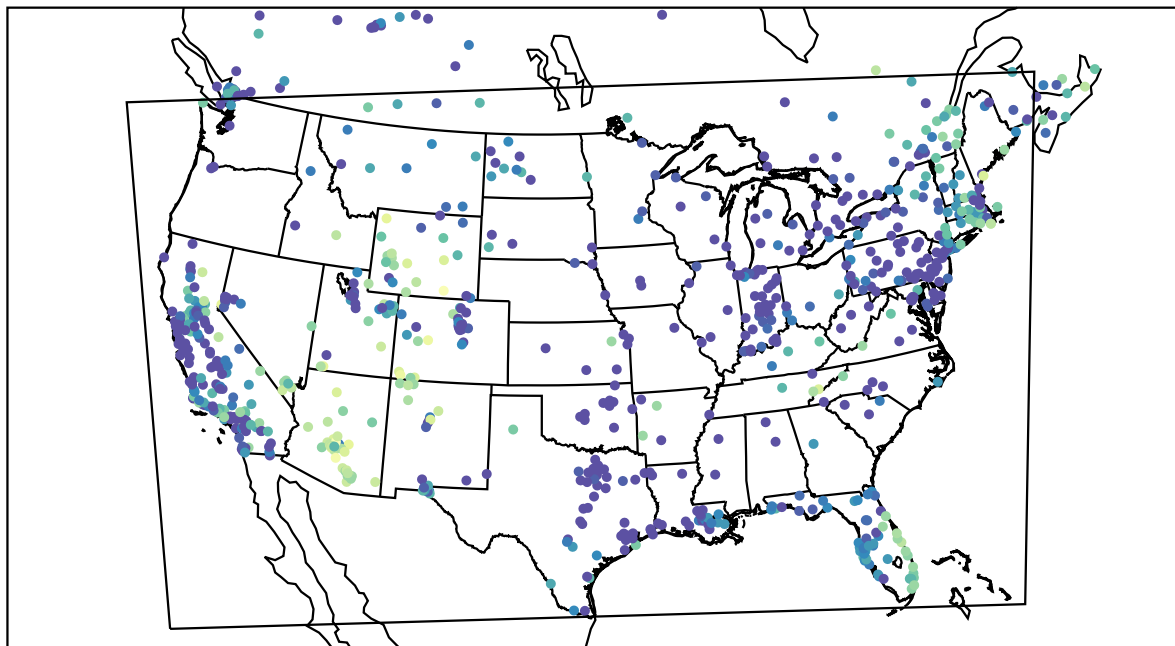
AirNOW (2019-12-27_05:00:00)
