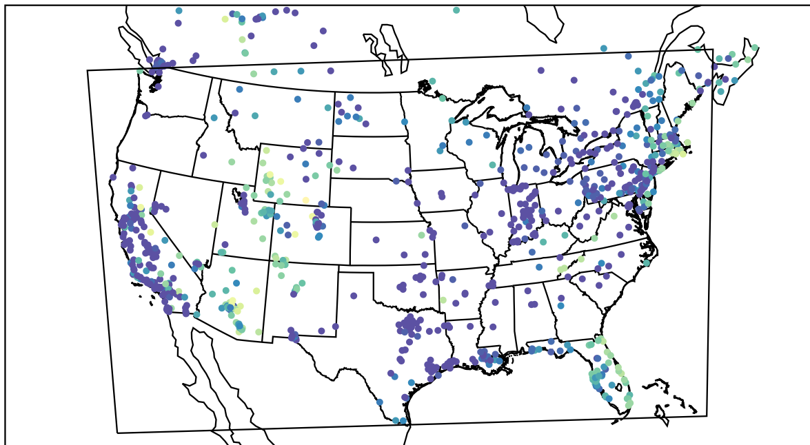
AirNOW (2019-12-27_15:00:00)
