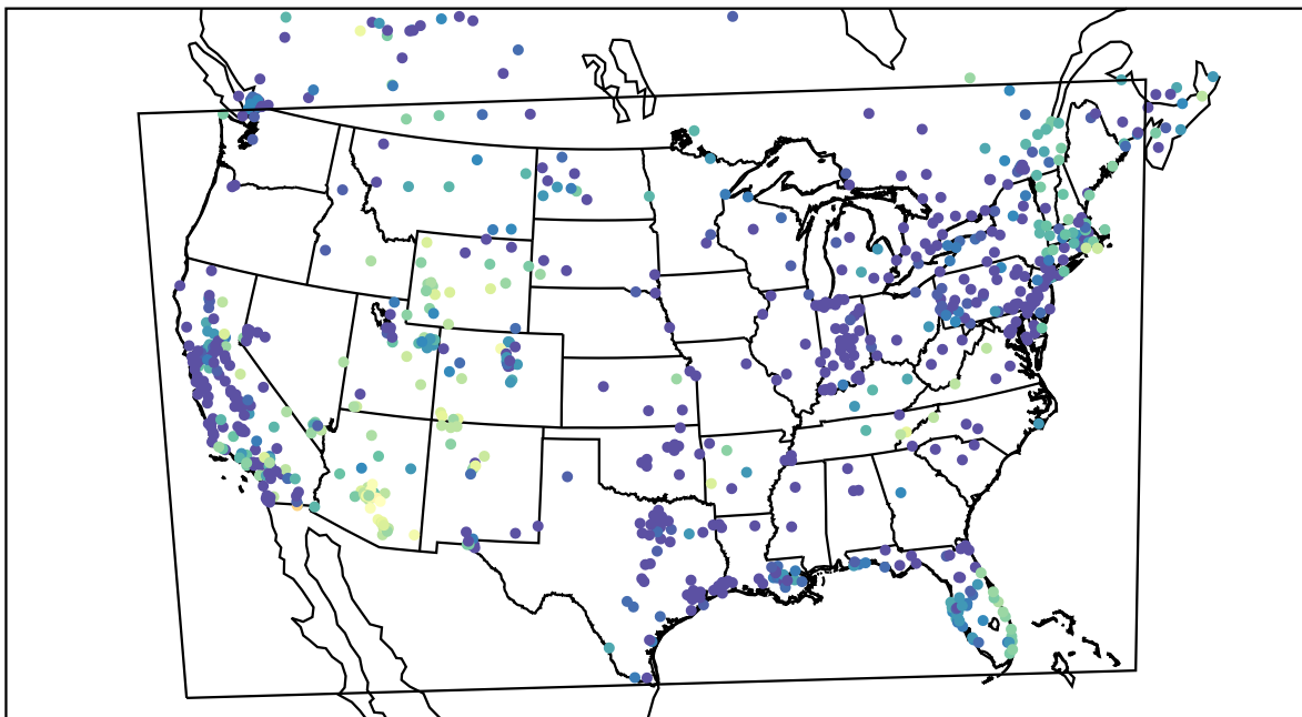
AirNOW (2019-12-27_09:00:00)
