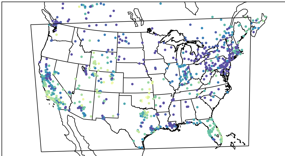
AirNOW (2019-12-26_02:00:00)
