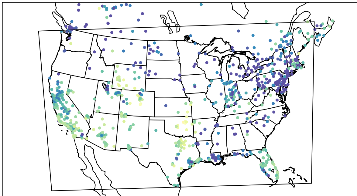
AirNOW (2019-12-26_00:00:00)
