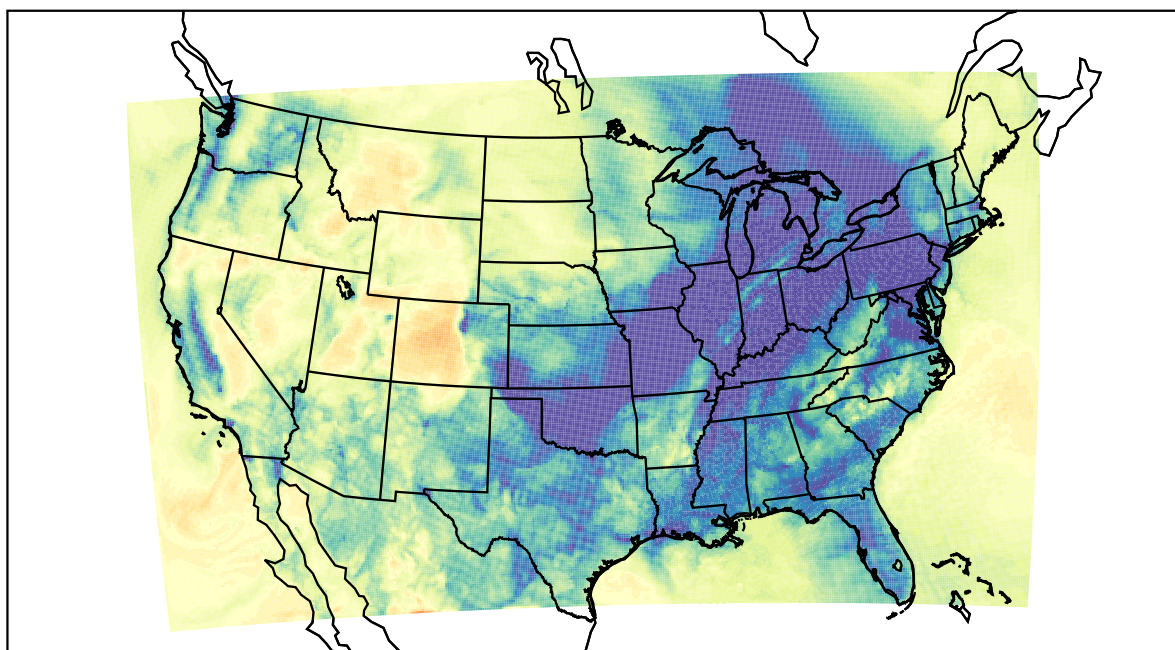
WRF (2019-12-27_05:00:00)
