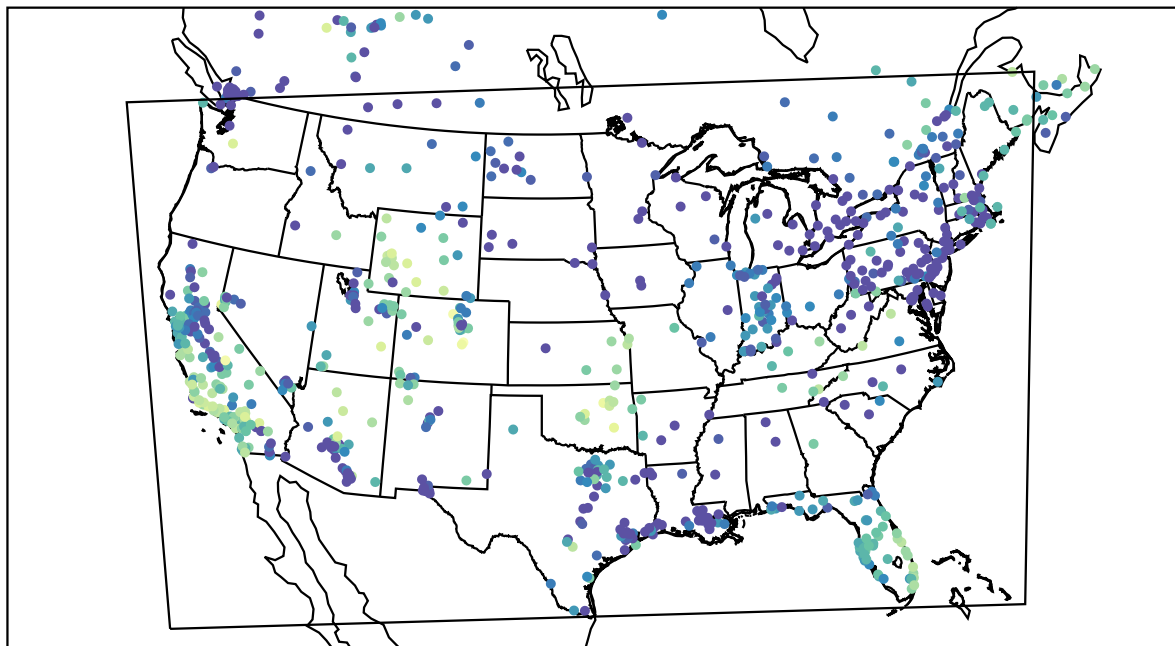
AirNOW (2019-12-26_05:00:00)
