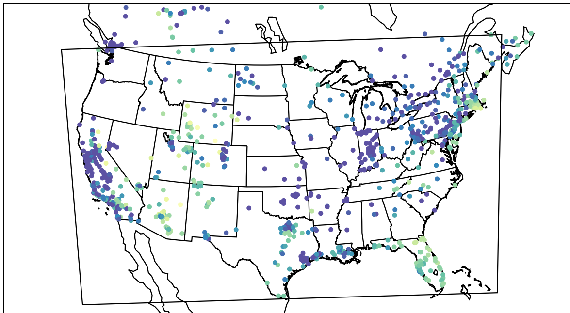
AirNOW (2019-12-27_17:00:00)
