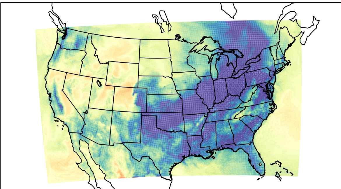
WRF (2019-12-27_12:00:00)
