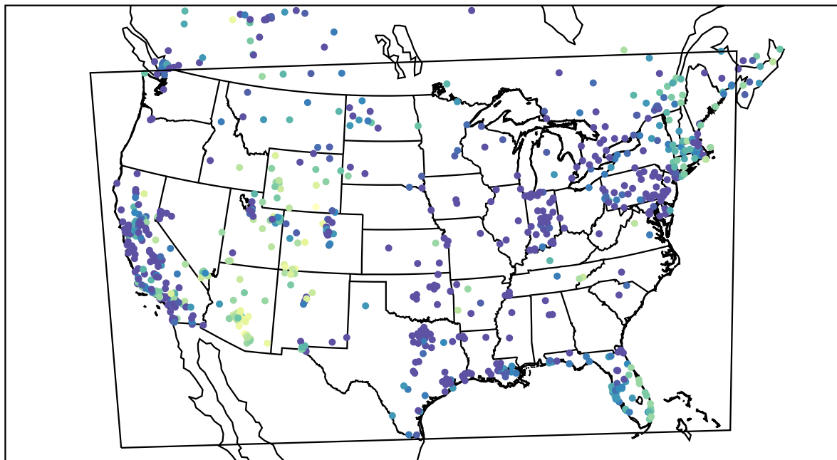
AirNOW (2019-12-27_07:00:00)
