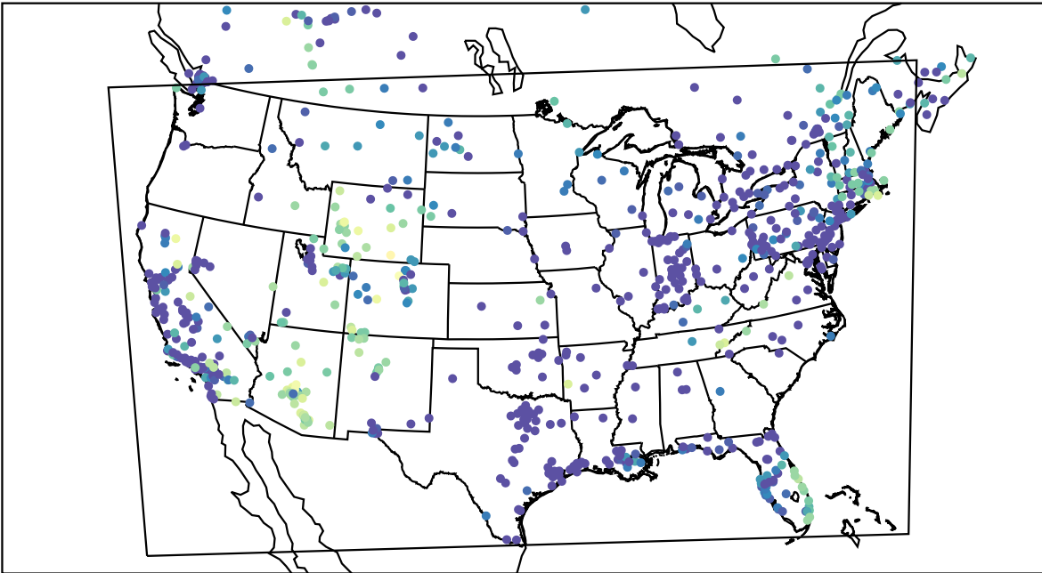
AirNOW (2019-12-27_12:00:00)
