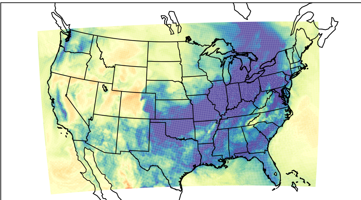
WRF (2019-12-27_11:00:00)
