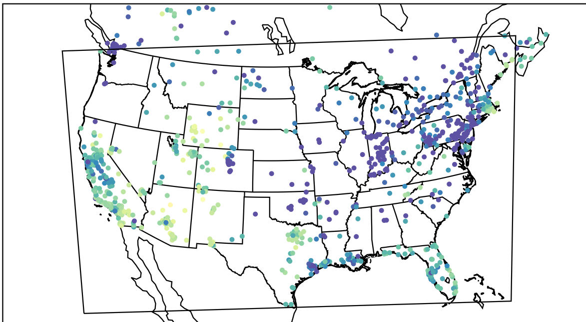
AirNOW (2019-12-27_22:00:00)
