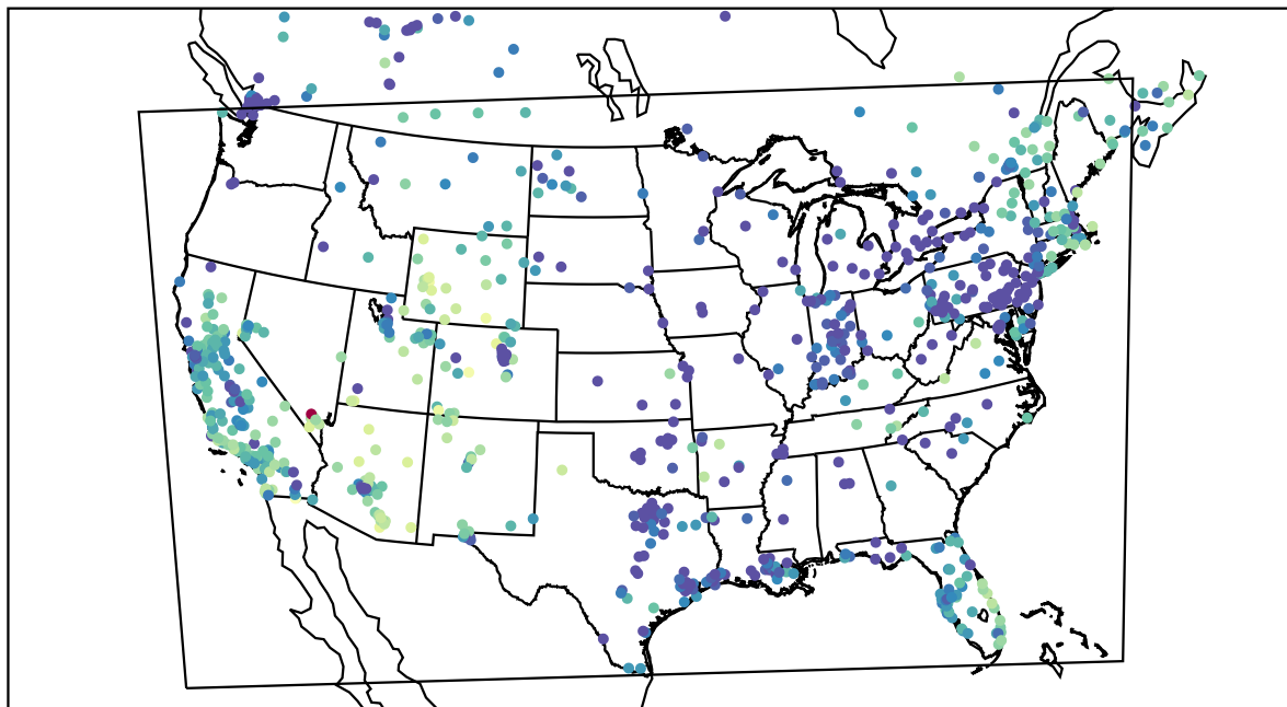
AirNOW (2019-12-27_00:00:00)
