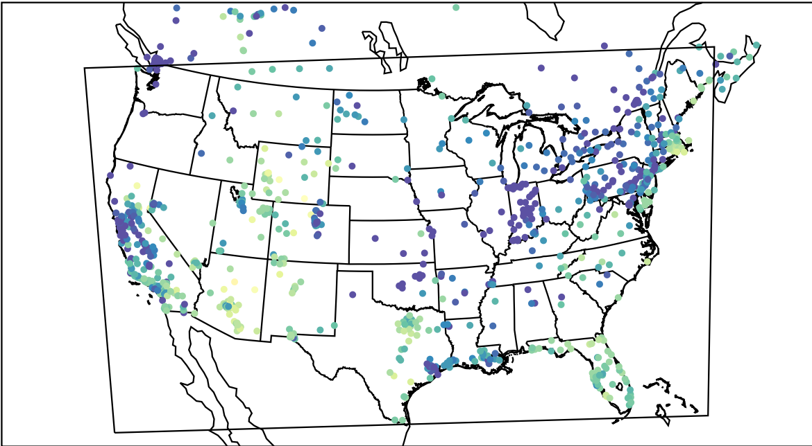
AirNOW (2019-12-27_19:00:00)
