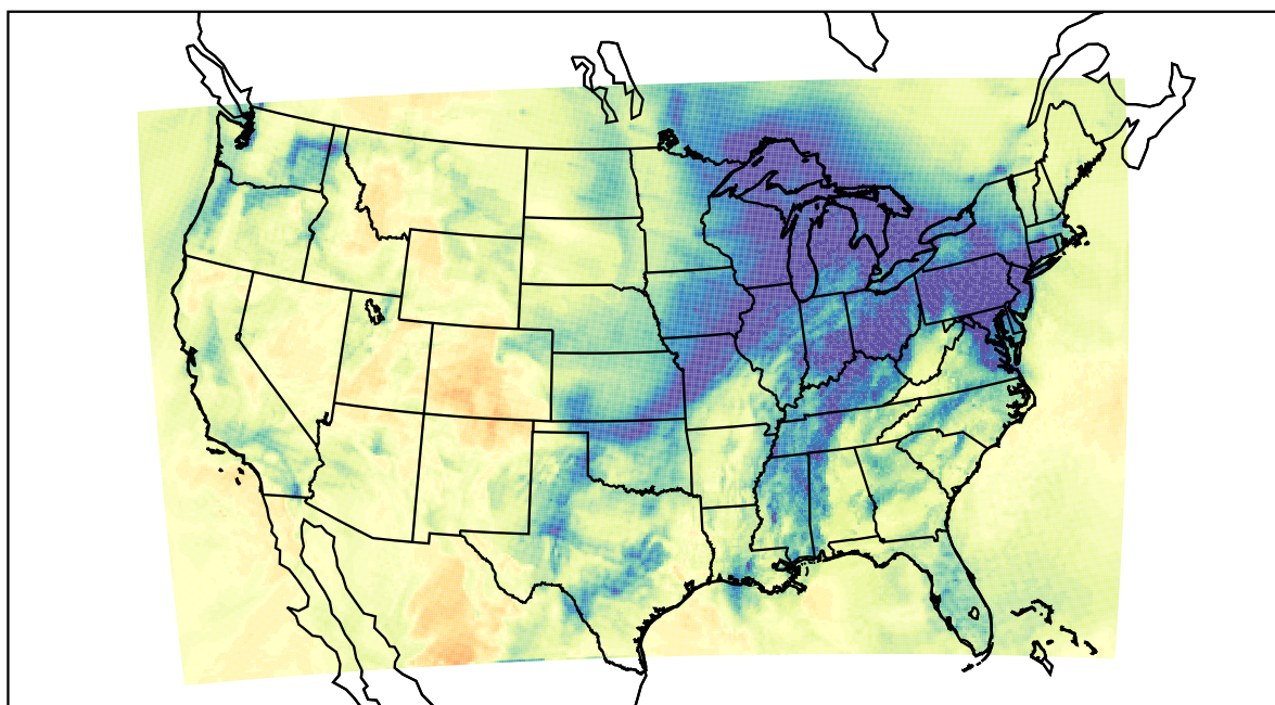
WRF (2019-12-26_21:00:00)
