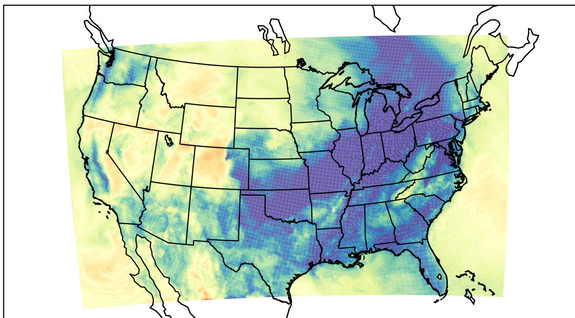
WRF (2019-12-27_10:00:00)
