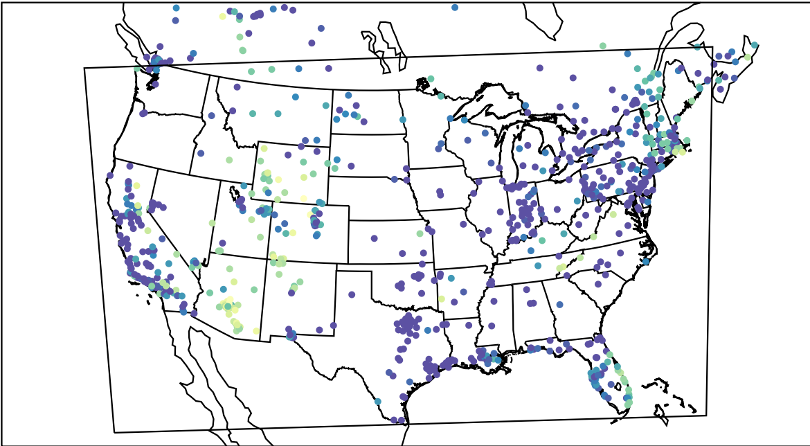
AirNOW (2019-12-27_11:00:00)
