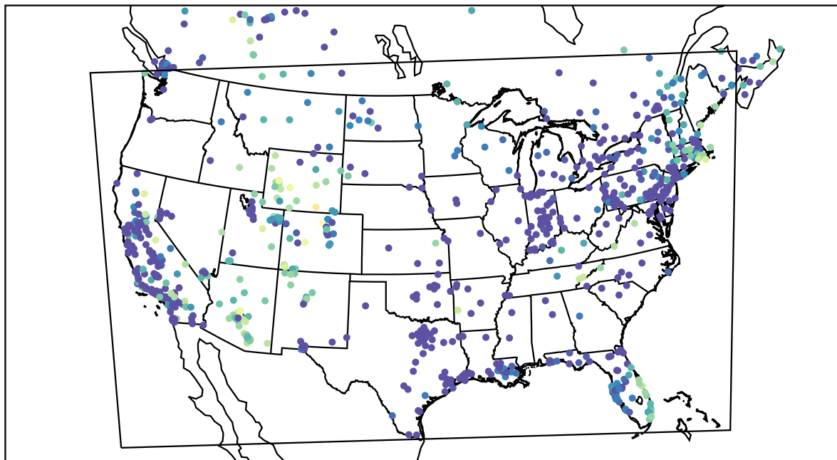
AirNOW (2019-12-27_13:00:00)
