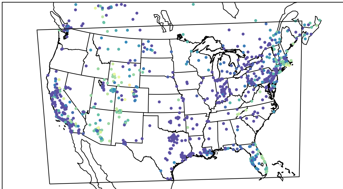
AirNOW (2019-12-27_14:00:00)
