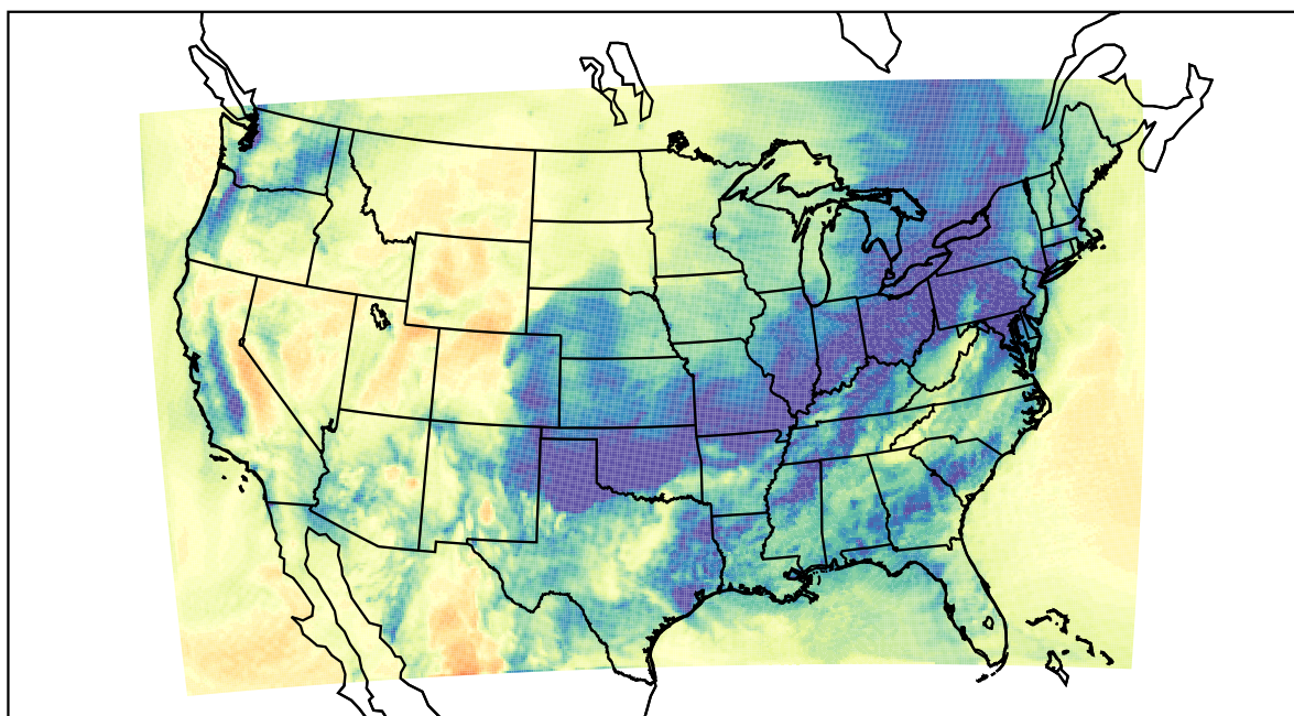
WRF (2019-12-27_17:00:00)
