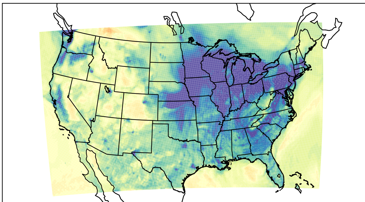
WRF (2019-12-26_02:00:00)
