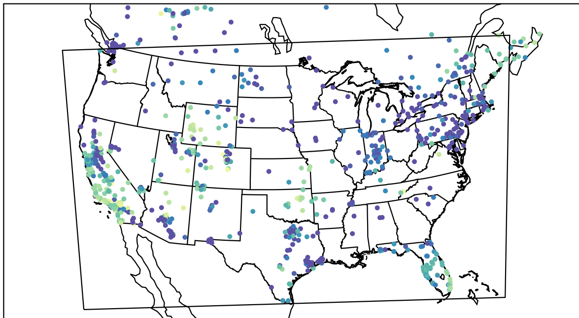
AirNOW (2019-12-26_07:00:00)
