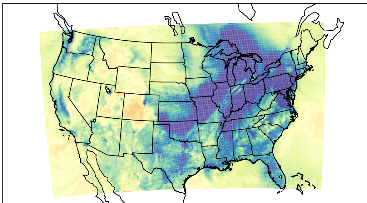
WRF (2019-12-27_02:00:00)
