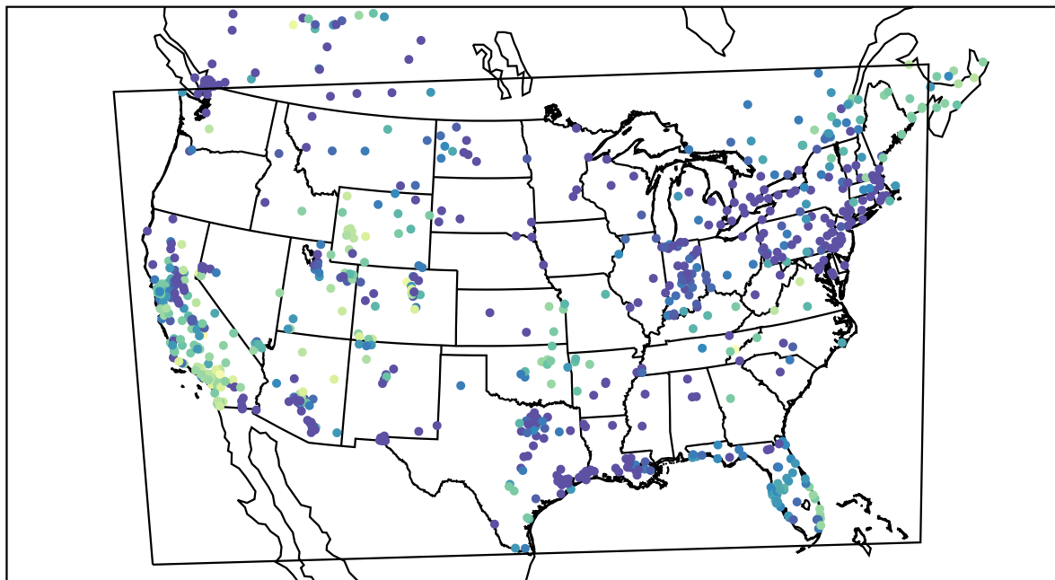
AirNOW (2019-12-26_09:00:00)
