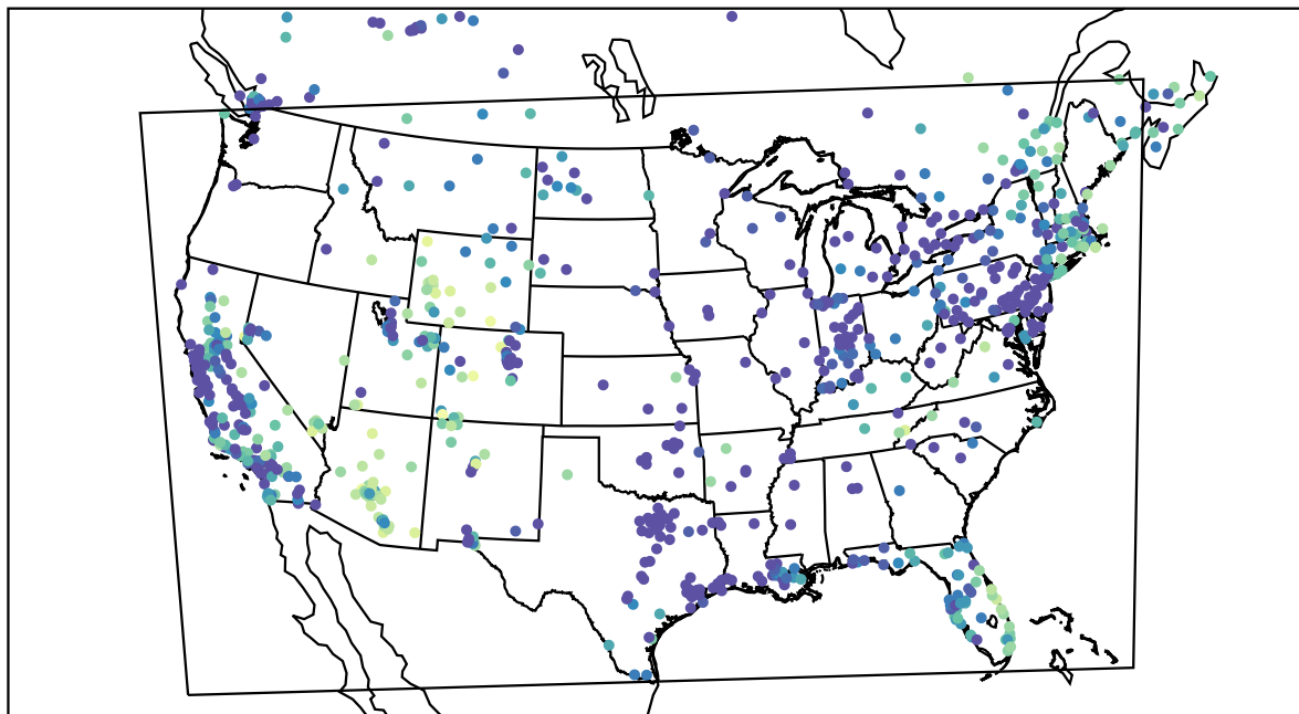
AirNOW (2019-12-27_03:00:00)
