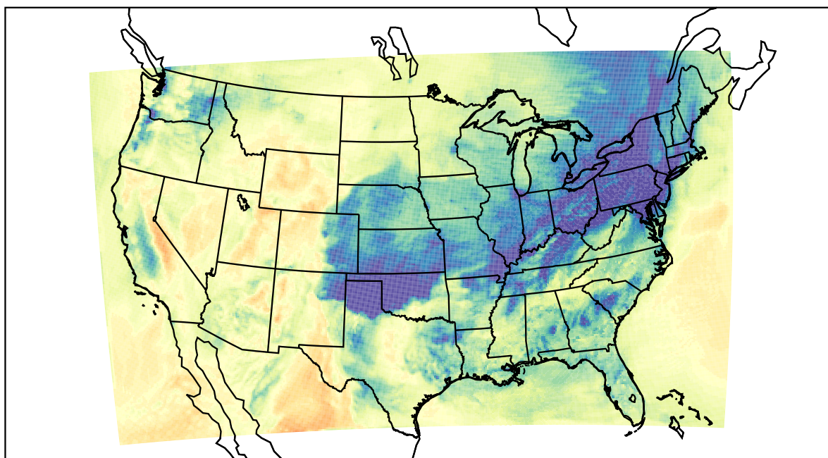
WRF (2019-12-27_21:00:00)
