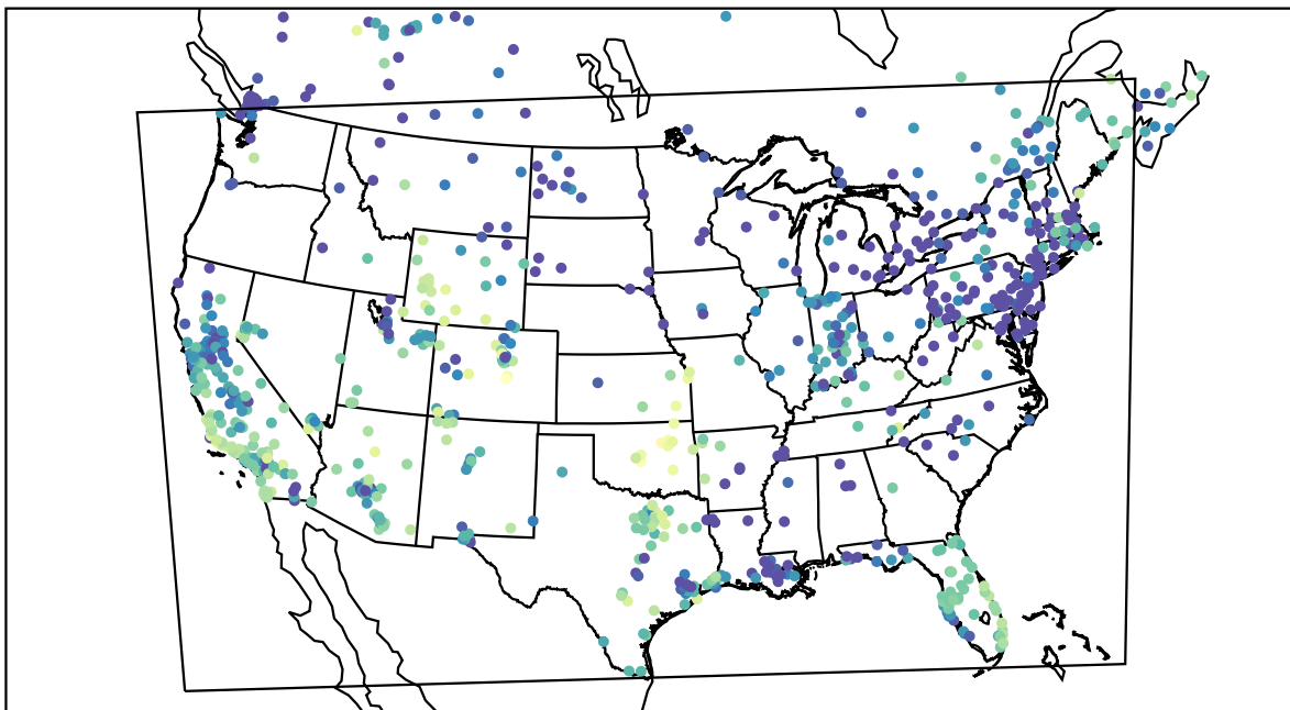
AirNOW (2019-12-26_01:00:00)
