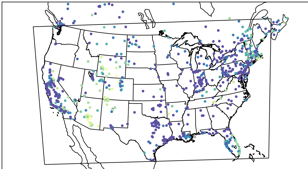
AirNOW (2019-12-27_10:00:00)
