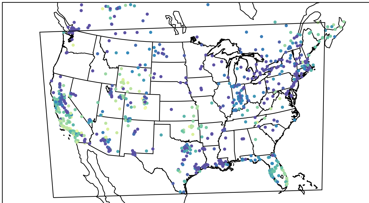
AirNOW (2019-12-26_06:00:00)
