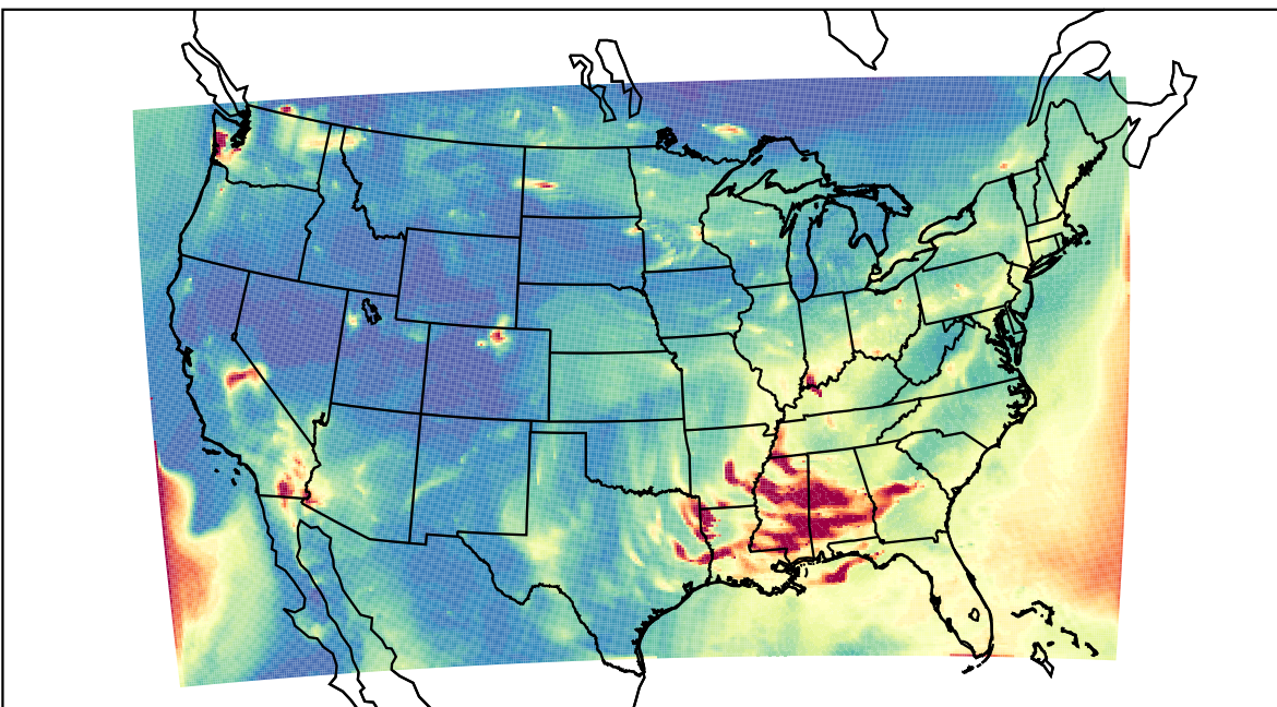
WRF 2020-10-22_05:00:00
