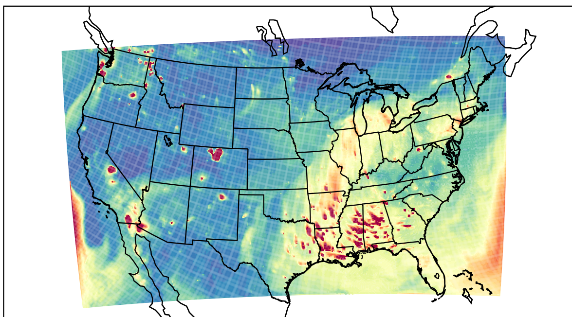
WRF 2020-10-23_02:00:00
