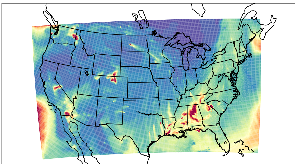
WRF 2020-10-24_05:00:00
