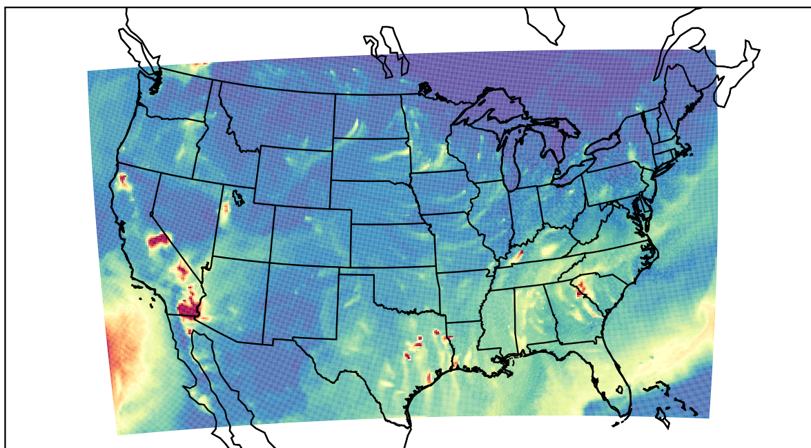
WRF 2020-10-25_05:00:00
