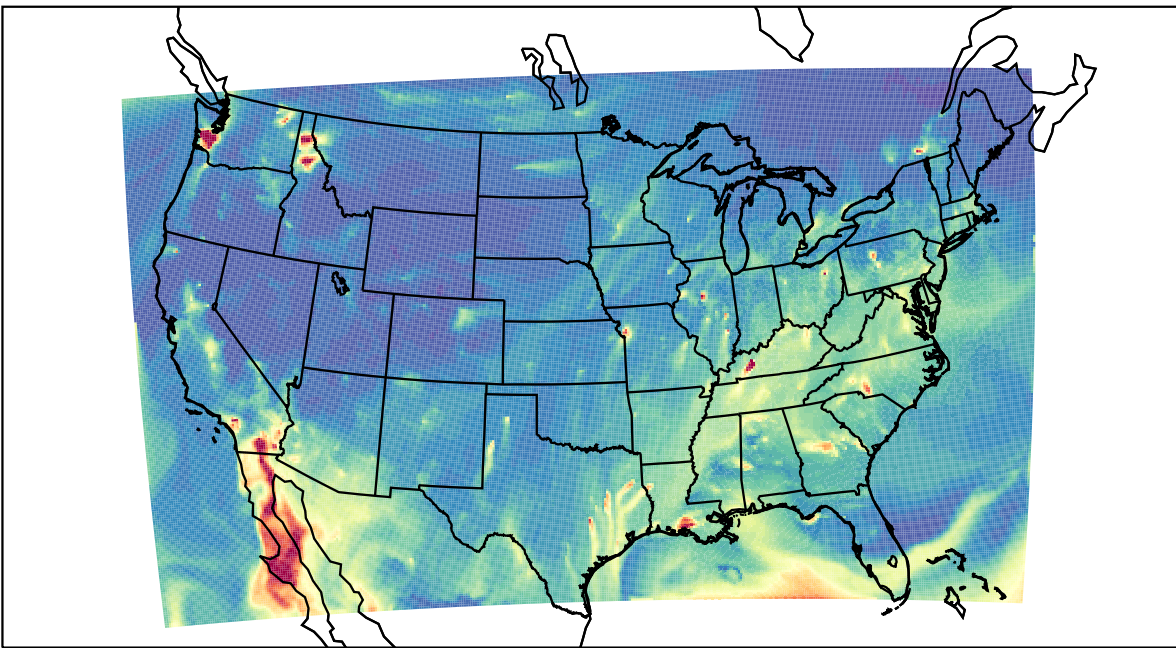
WRF 2020-10-28_05:00:00
