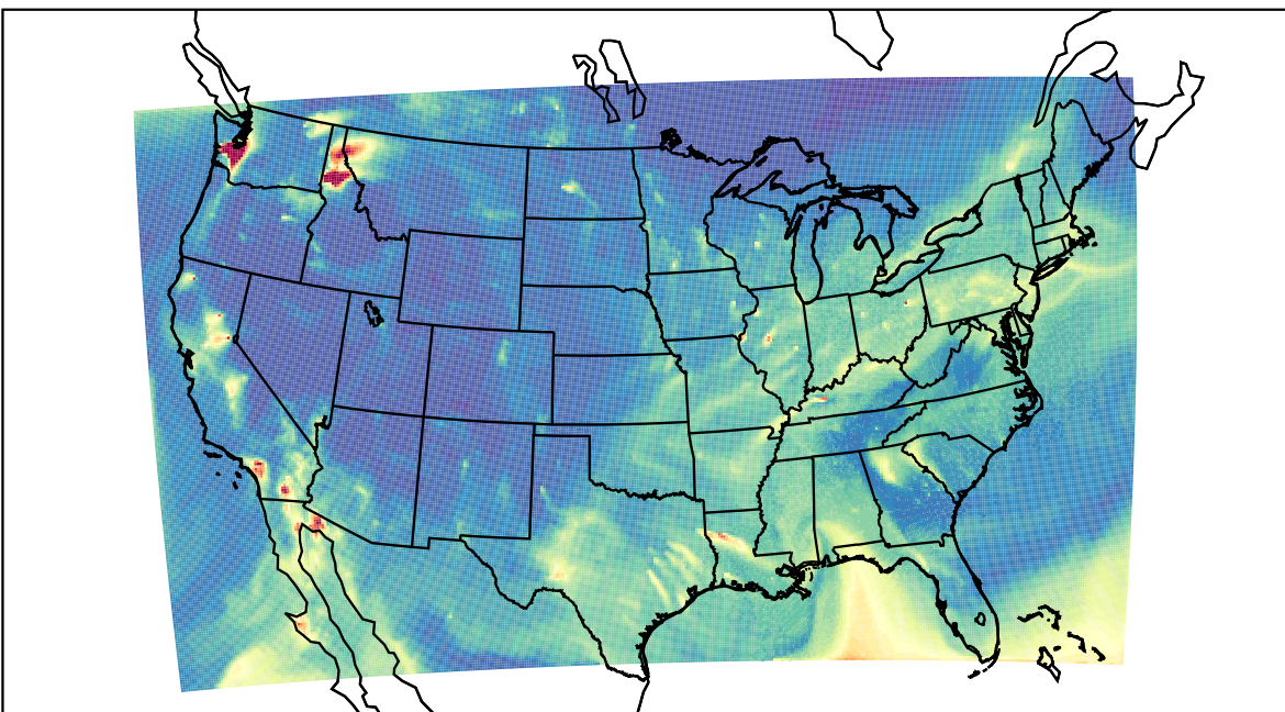
WRF 2020-10-29_05:00:00
