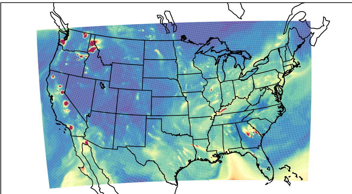
WRF 2020-10-29_02:00:00
