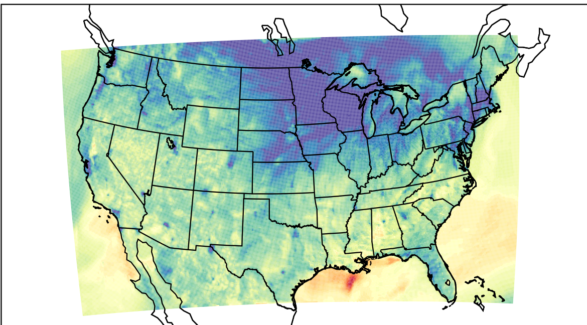
WRF (2020-11-05_02:00:00)
