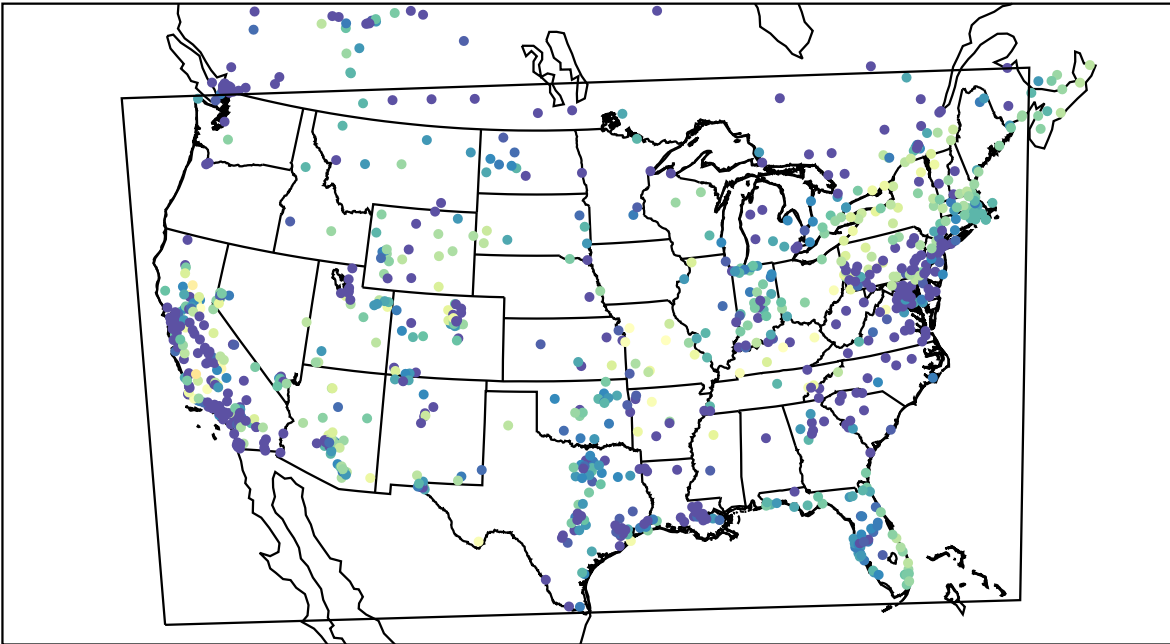
AirNOW (2020-11-06_03:00:00)
