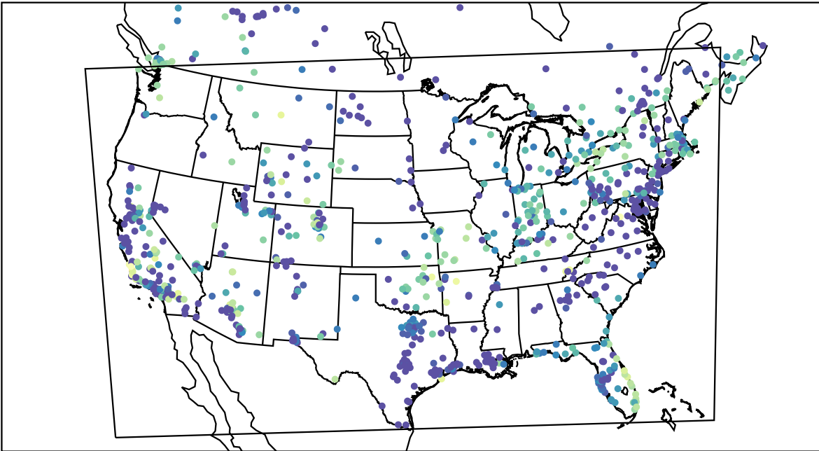
AirNOW (2020-11-05_11:00:00)
