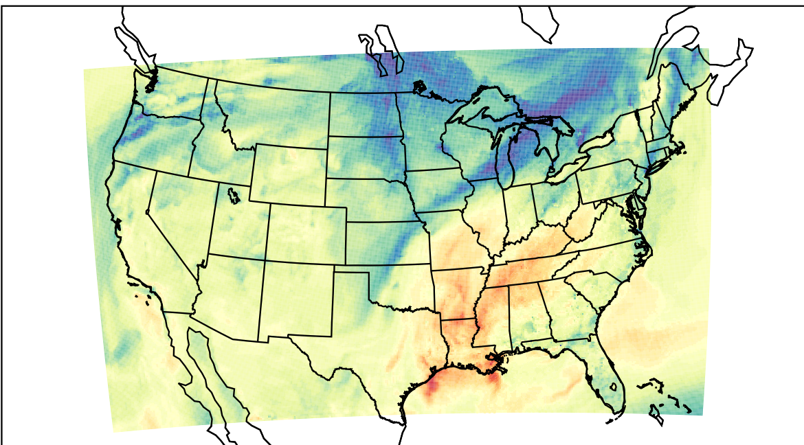
WRF (2020-11-05_21:00:00)
