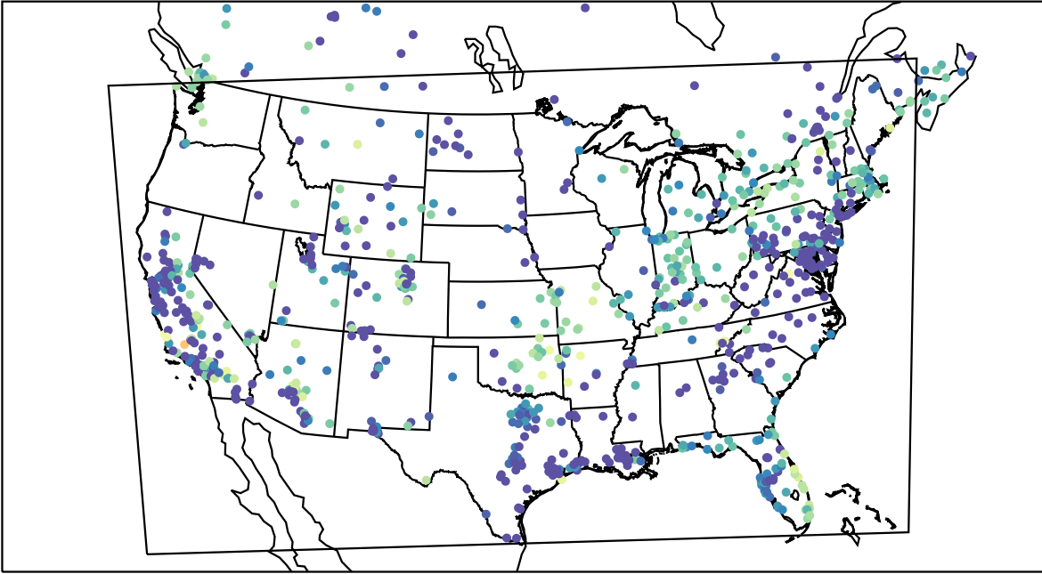
AirNOW (2020-11-05_10:00:00)
