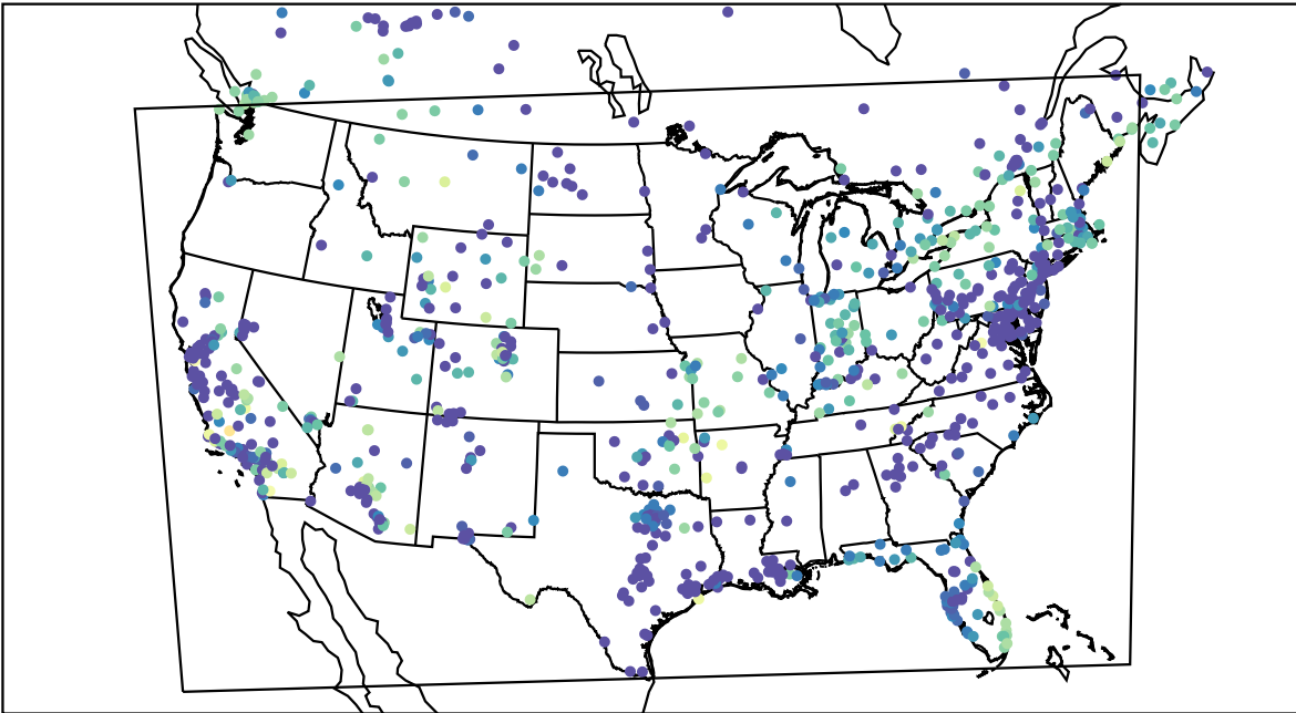
AirNOW (2020-11-05_12:00:00)
