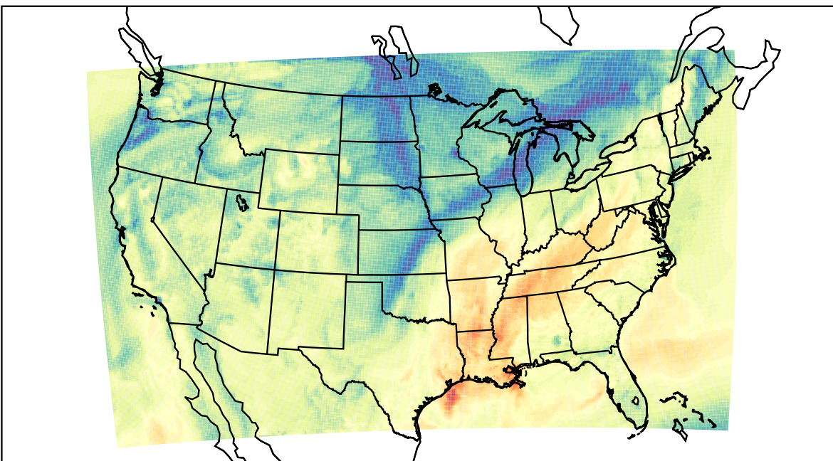
WRF (2020-11-05_19:00:00)
