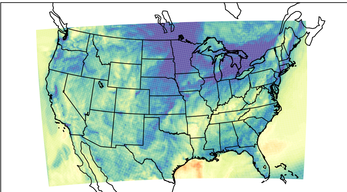
WRF (2020-11-06_07:00:00)
