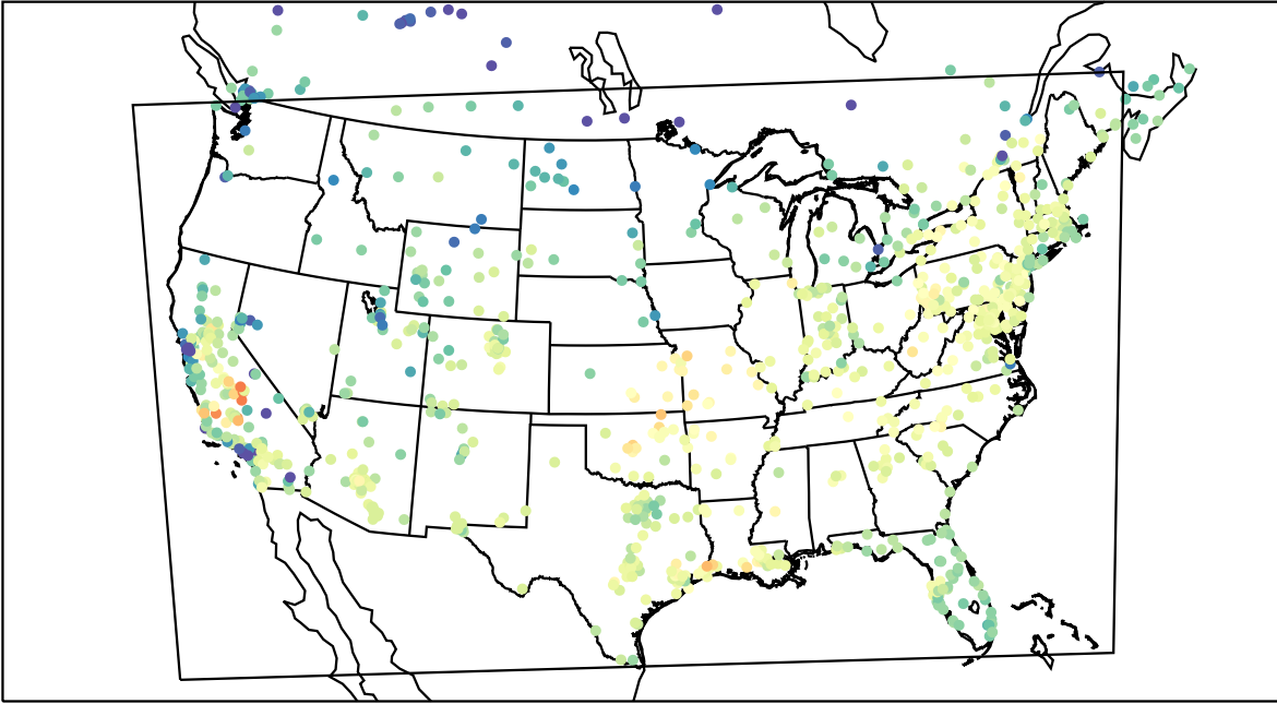
AirNOW (2020-11-05_19:00:00)
