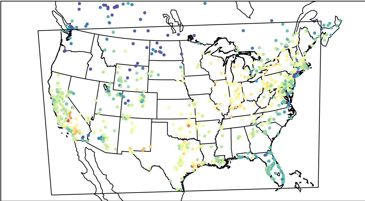
AirNOW (2020-11-06_21:00:00)
