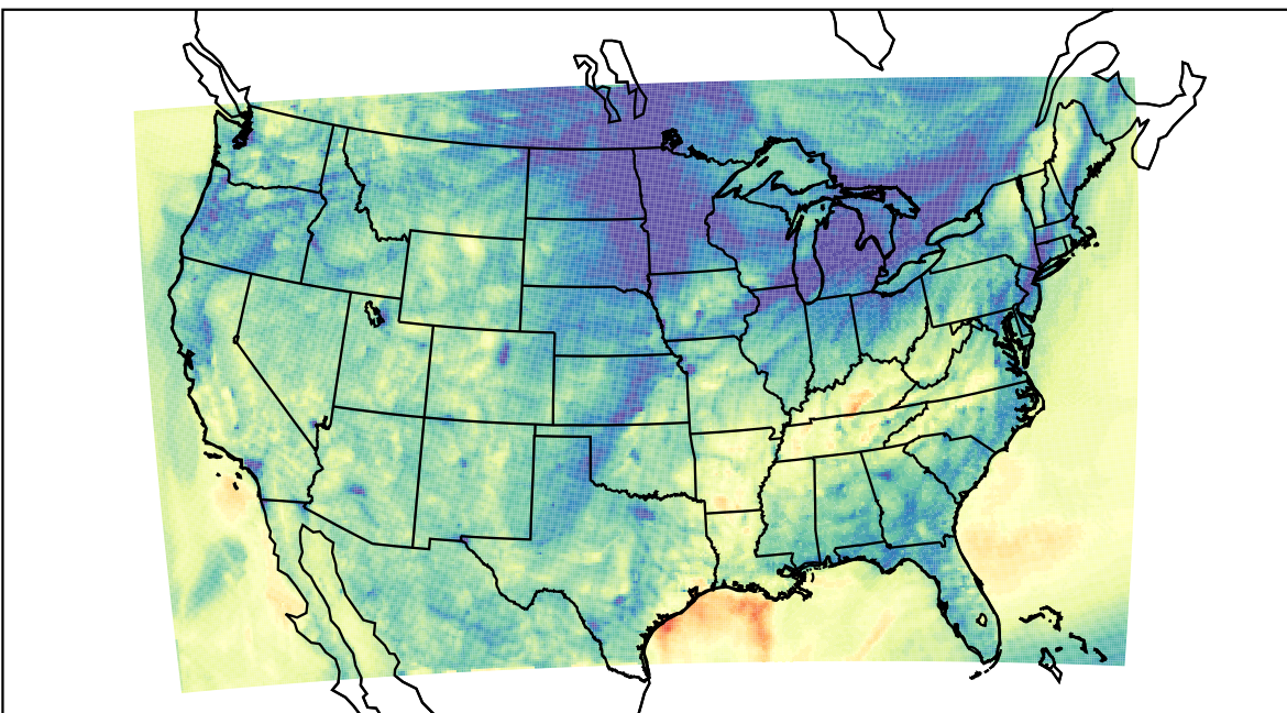
WRF (2020-11-06_03:00:00)
