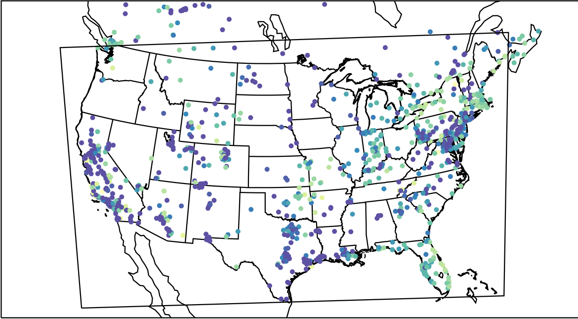
AirNOW (2020-11-05_14:00:00)
