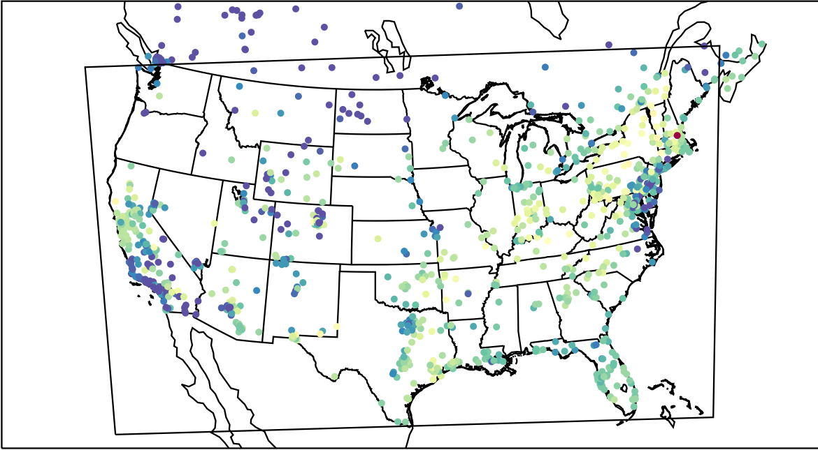
AirNOW (2020-11-06_16:00:00)
