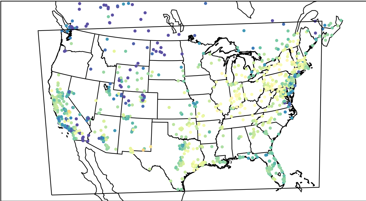
AirNOW (2020-11-06_17:00:00)
