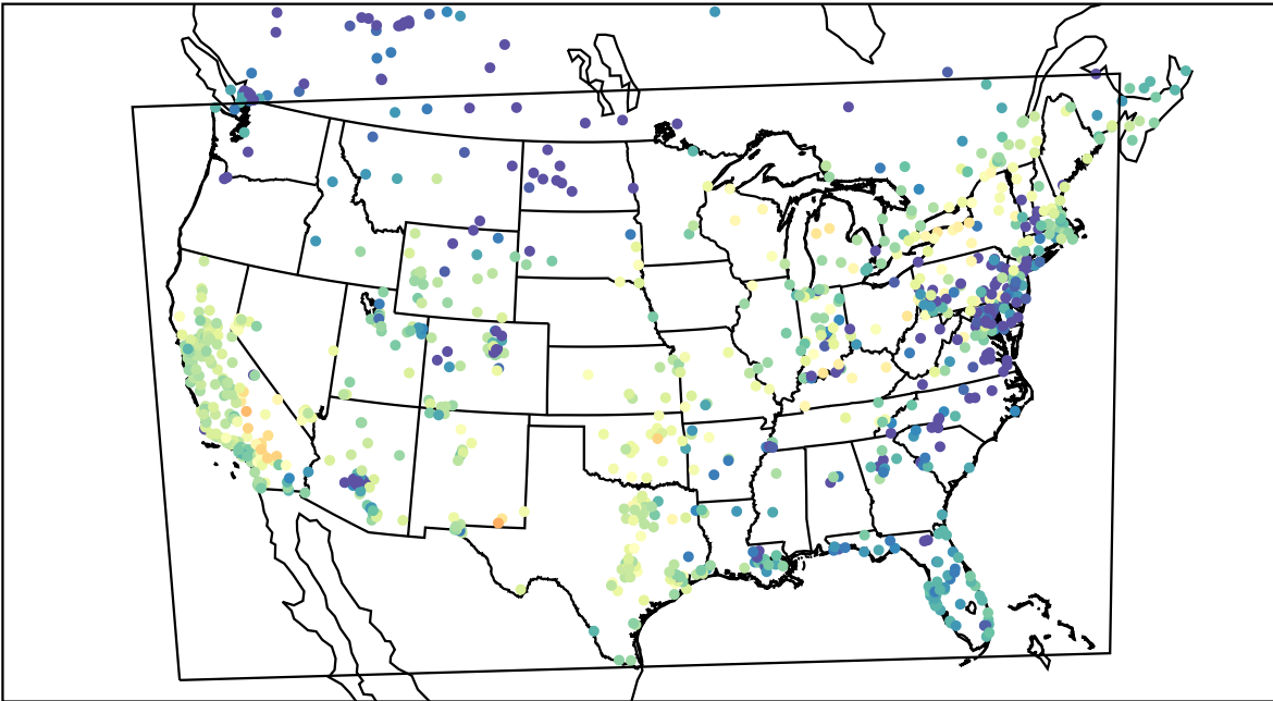
AirNOW (2020-11-06_23:00:00)
