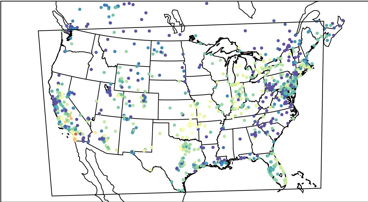
AirNOW (2020-11-05_01:00:00)
