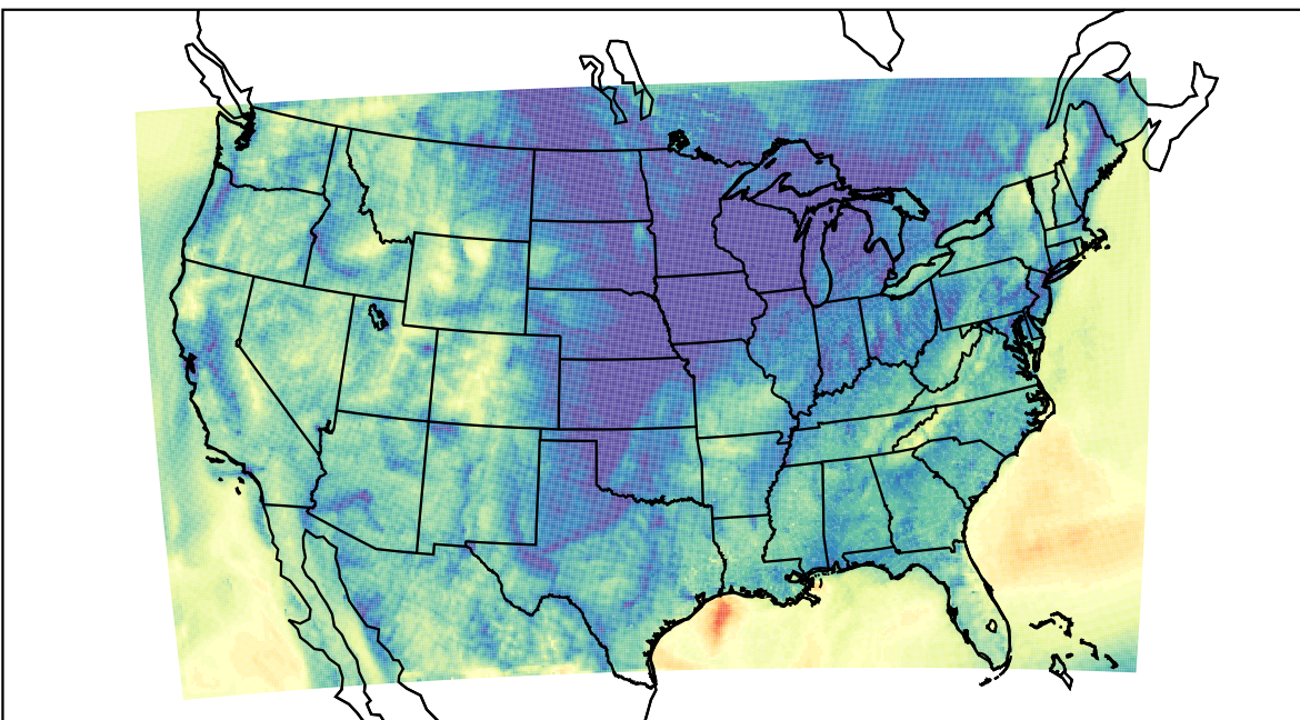
WRF (2020-11-05_14:00:00)
