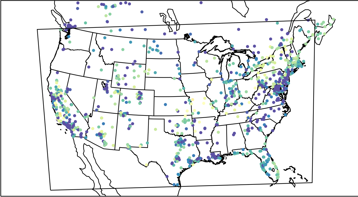
AirNOW (2020-11-06_01:00:00)
