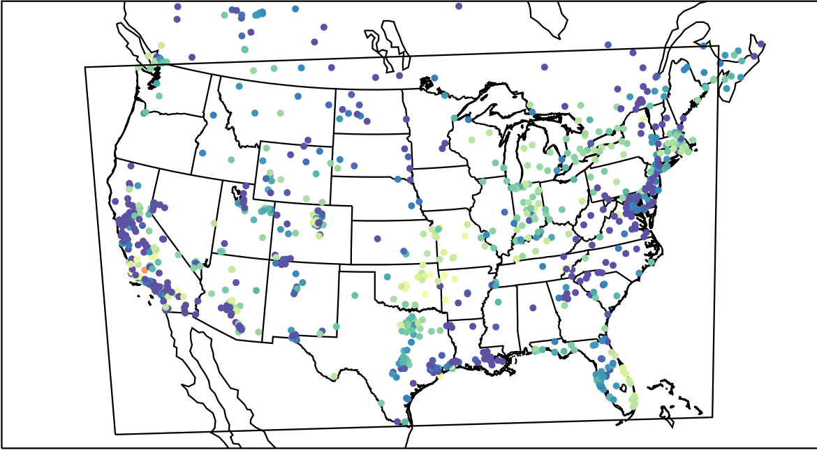
AirNOW (2020-11-05_06:00:00)
