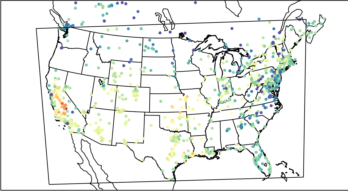
AirNOW (2020-11-05_22:00:00)
