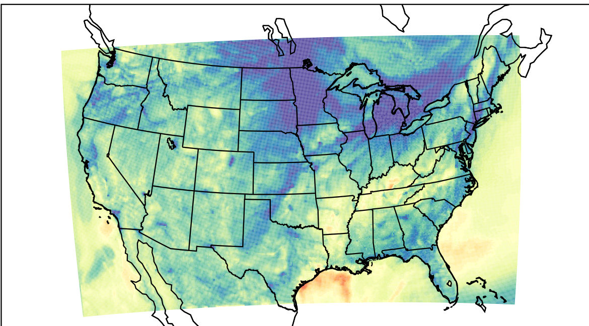
WRF (2020-11-06_04:00:00)
