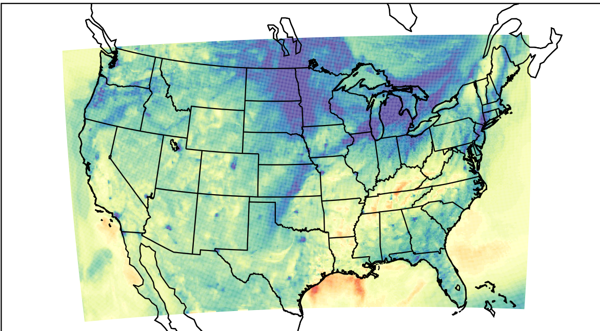
WRF (2020-11-06_01:00:00)
