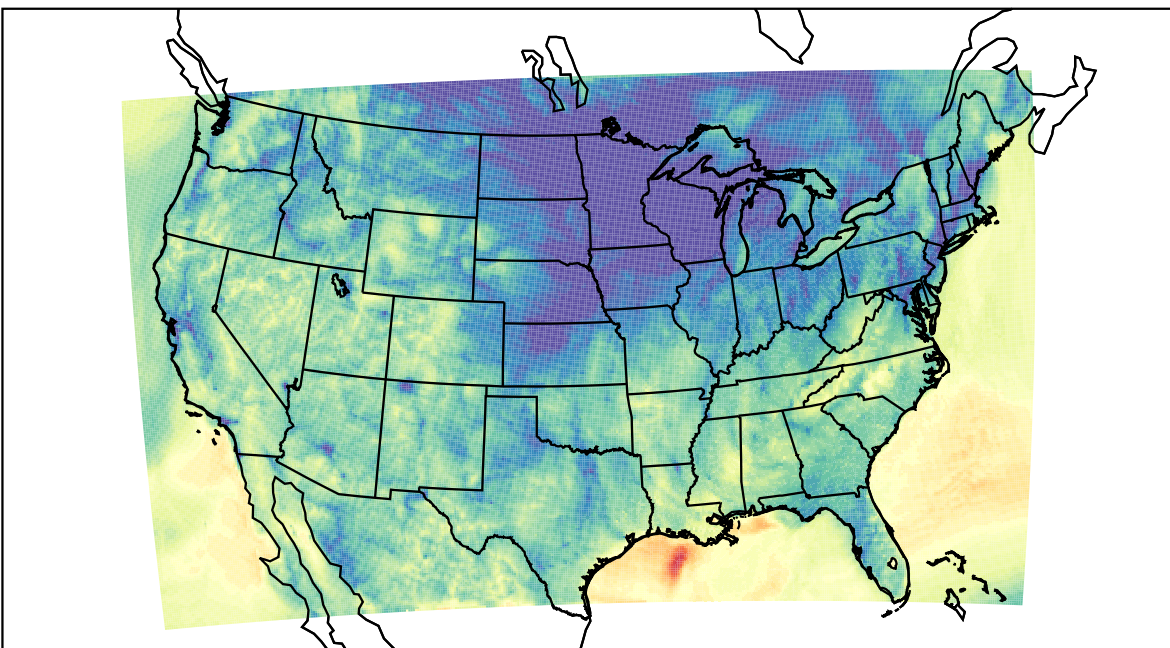
WRF (2020-11-05_06:00:00)
