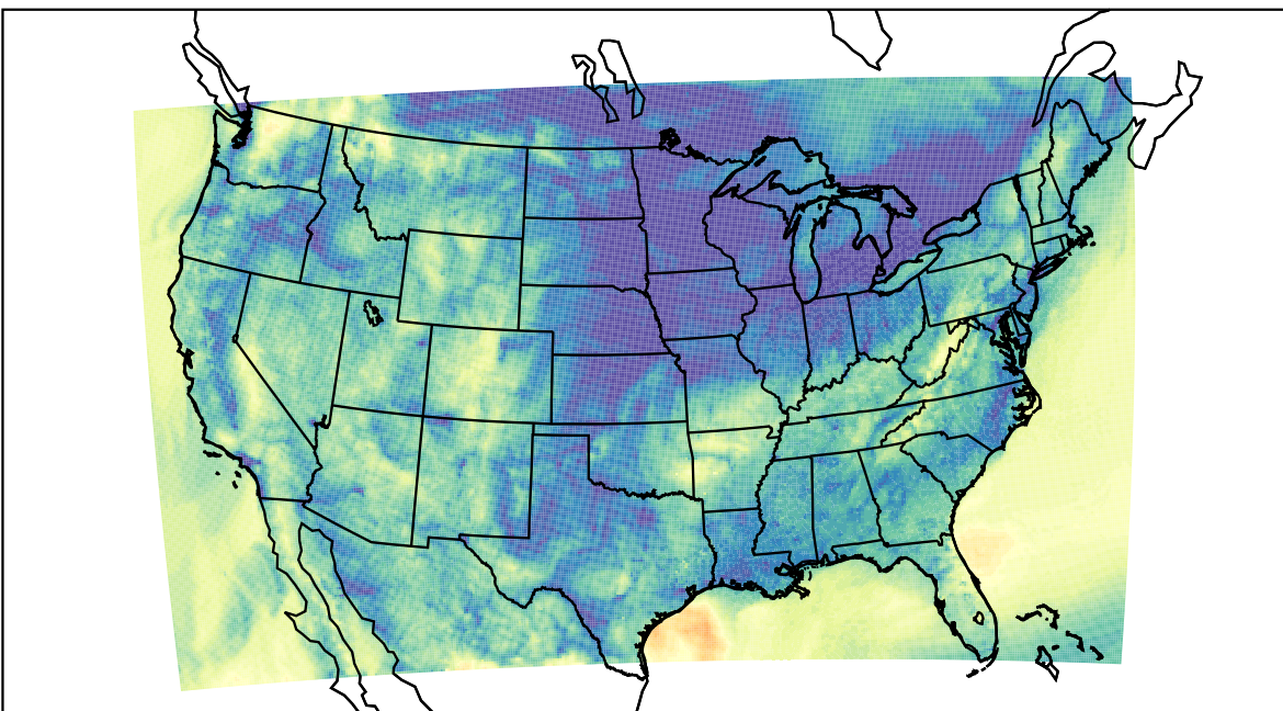
WRF (2020-11-06_14:00:00)
