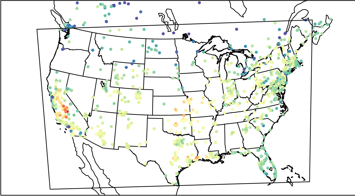
AirNOW (2020-11-05_21:00:00)
