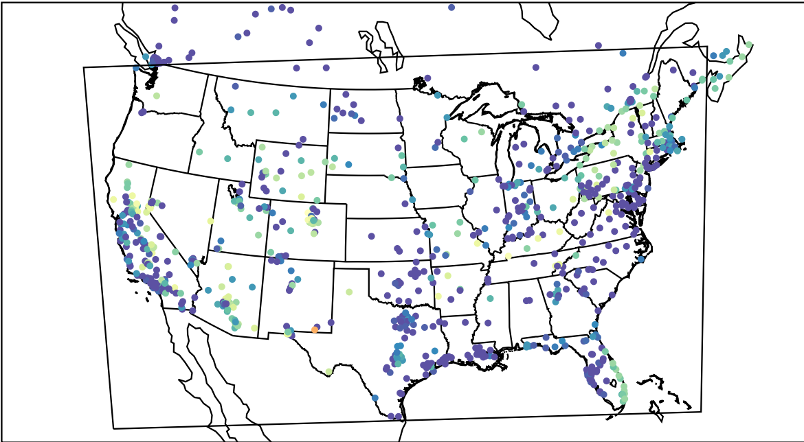
AirNOW (2020-11-06_10:00:00)
