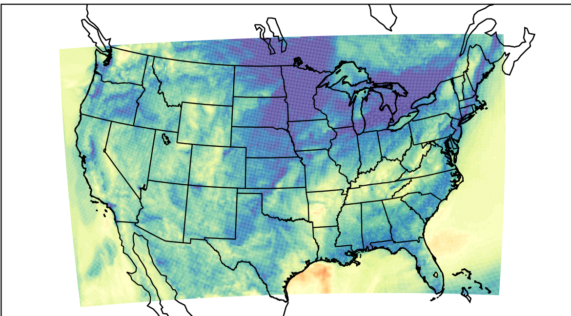
WRF (2020-11-06_08:00:00)
