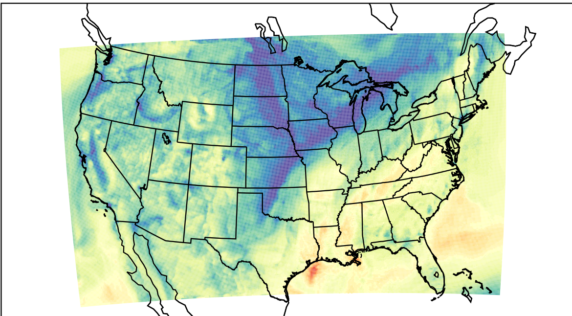
WRF (2020-11-05_17:00:00)
