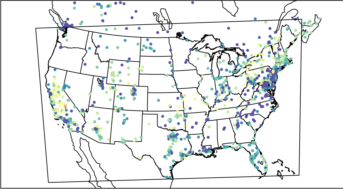
AirNOW (2020-11-06_00:00:00)
