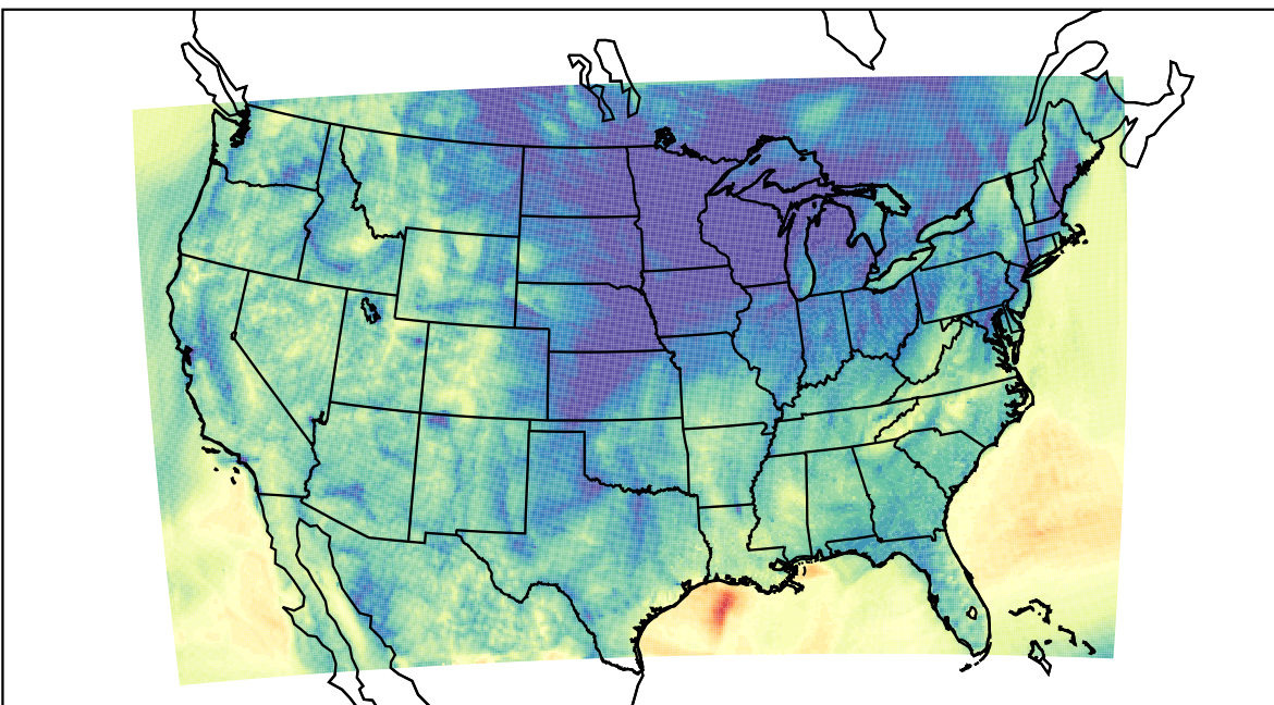
WRF (2020-11-05_09:00:00)
