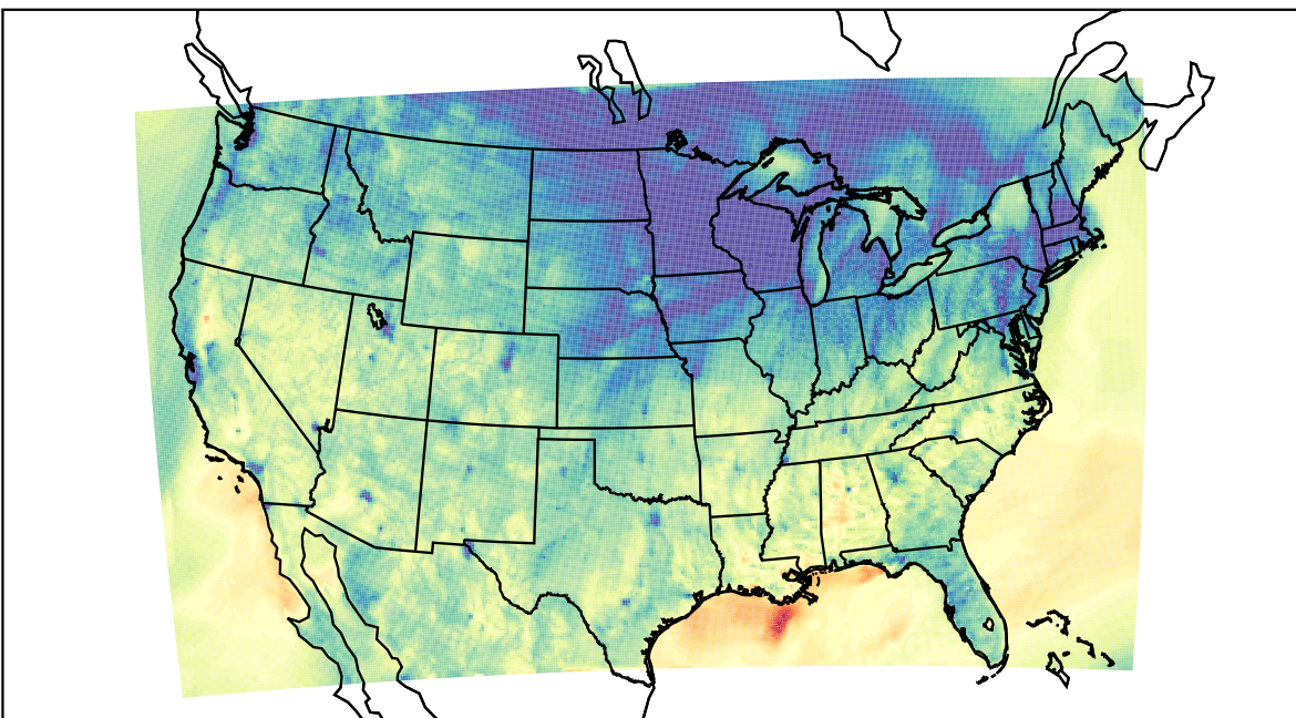
WRF (2020-11-05_01:00:00)
