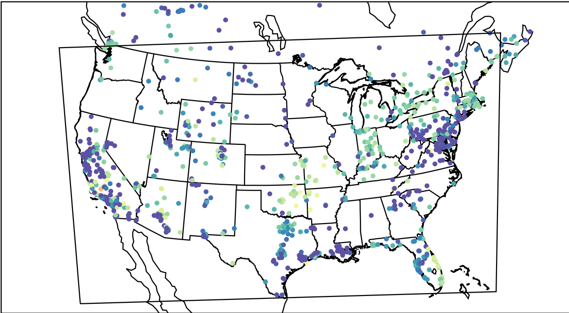
AirNOW (2020-11-05_08:00:00)
