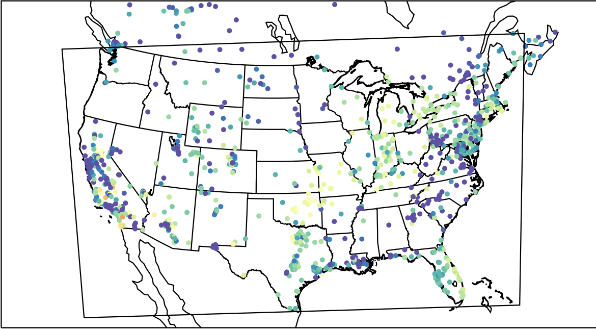
AirNOW (2020-11-05_02:00:00)
