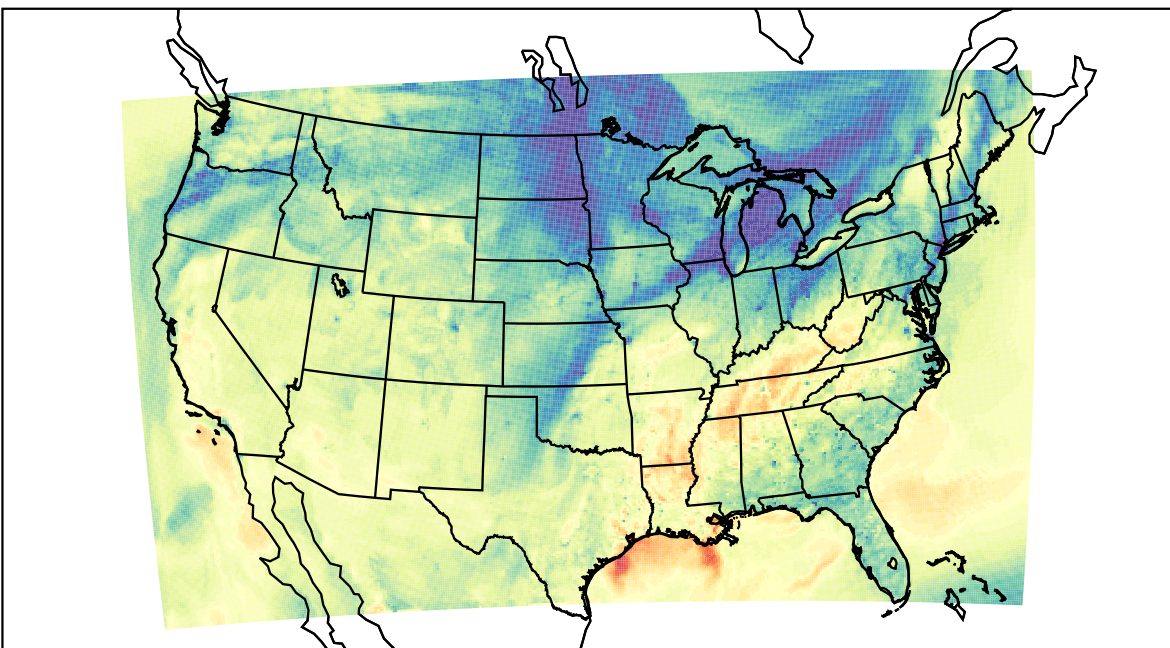
WRF (2020-11-05_23:00:00)
