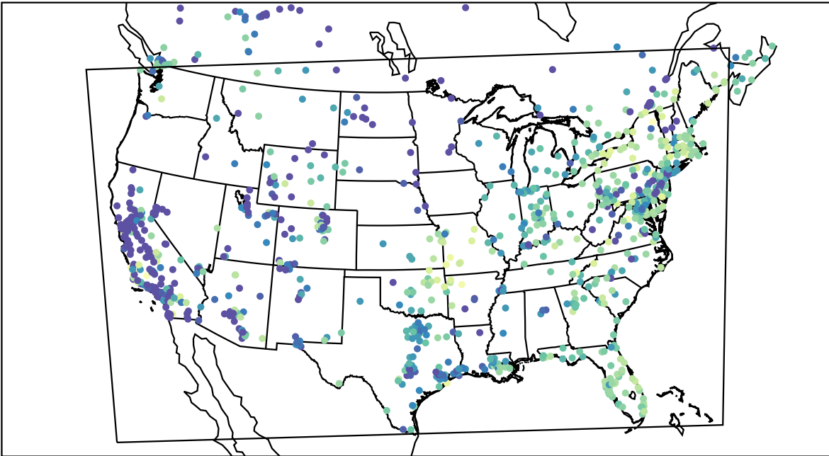
AirNOW (2020-11-05_15:00:00)
