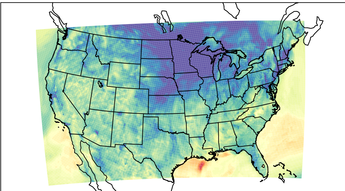
WRF (2020-11-05_05:00:00)
