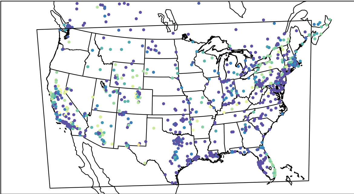
AirNOW (2020-11-06_11:00:00)
