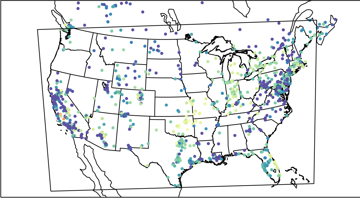
AirNOW (2020-11-05_04:00:00)
