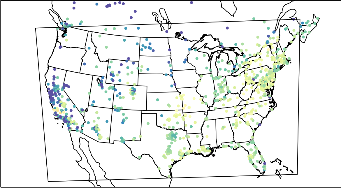
AirNOW (2020-11-05_17:00:00)
