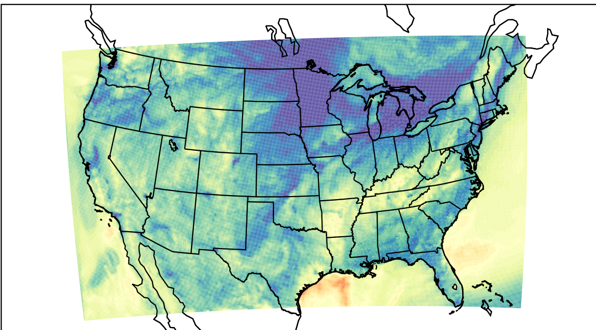
WRF (2020-11-06_06:00:00)
