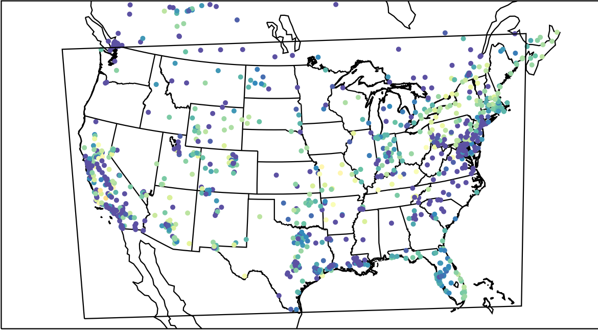
AirNOW (2020-11-06_02:00:00)
