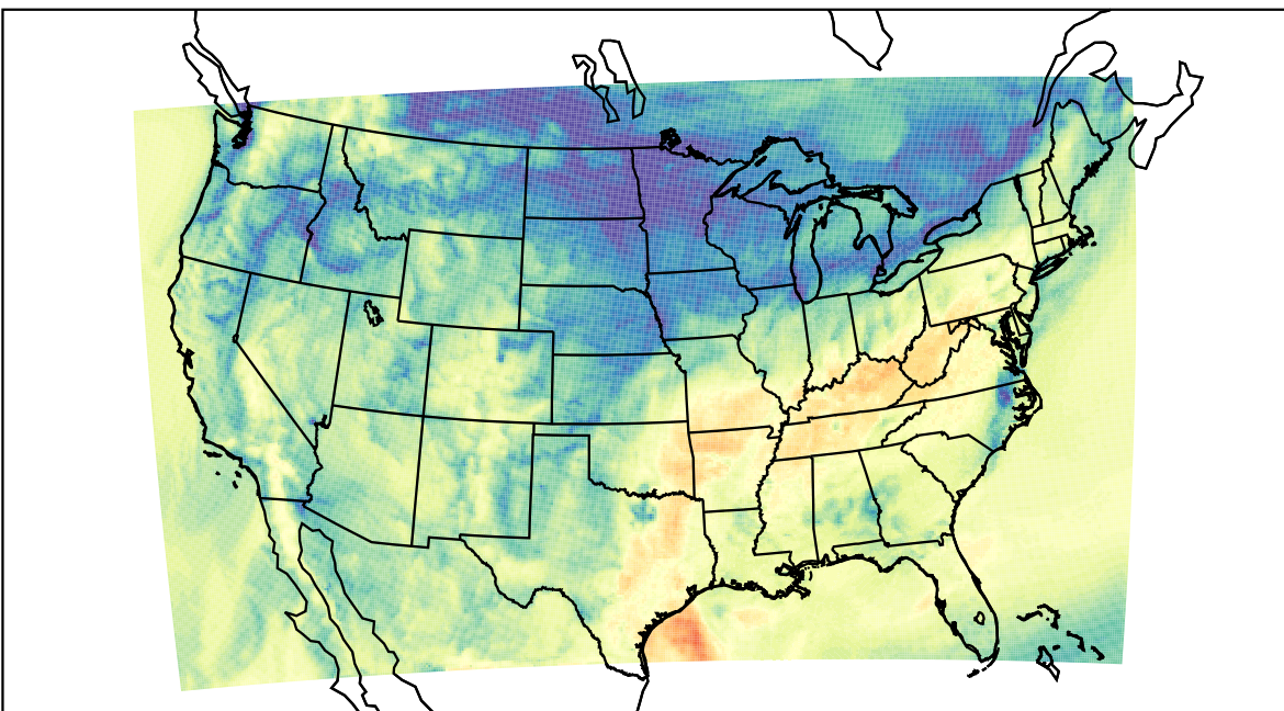
WRF (2020-11-06_17:00:00)
