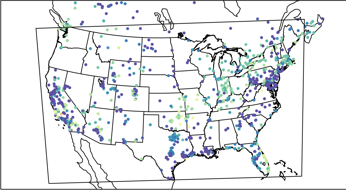
AirNOW (2020-11-05_09:00:00)
