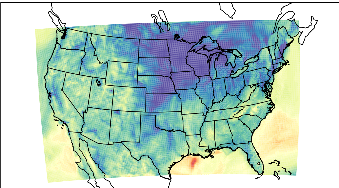
WRF (2020-11-05_08:00:00)
