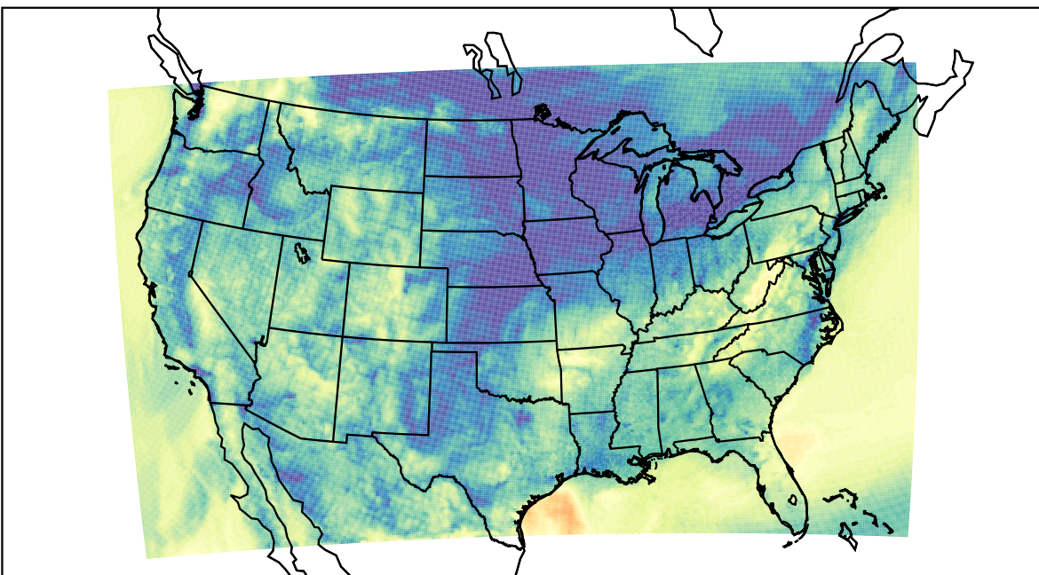
WRF (2020-11-06_15:00:00)
