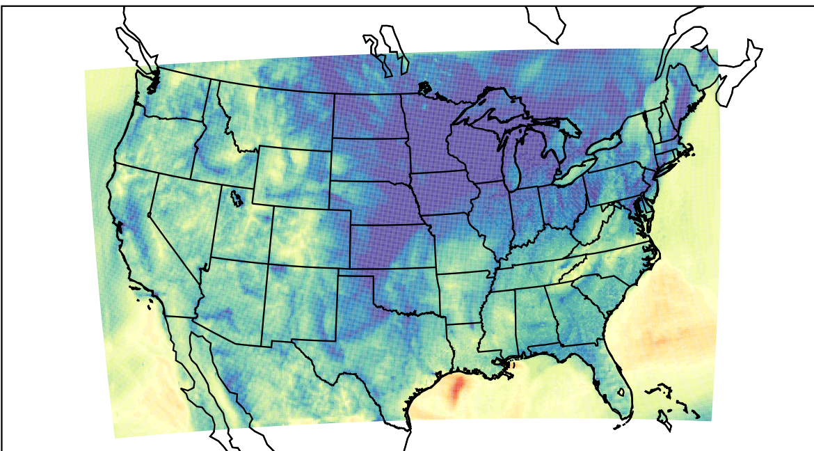
WRF (2020-11-05_11:00:00)
