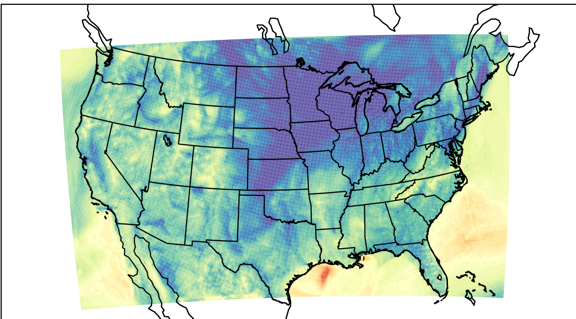
WRF (2020-11-05_10:00:00)
