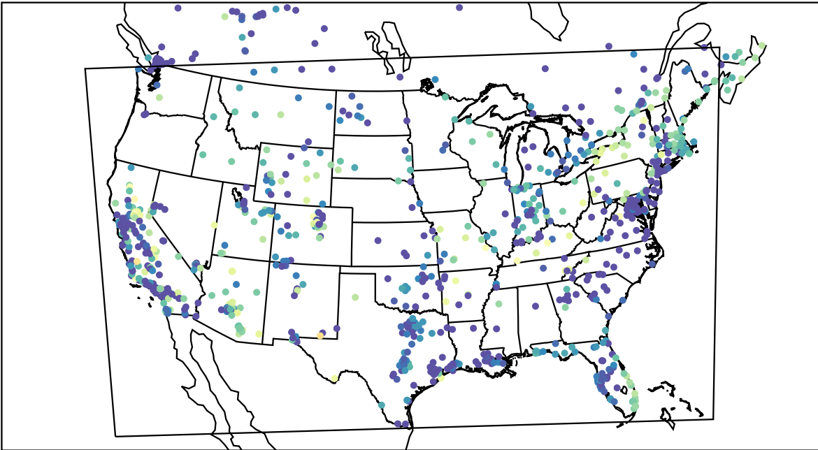
AirNOW (2020-11-06_06:00:00)
