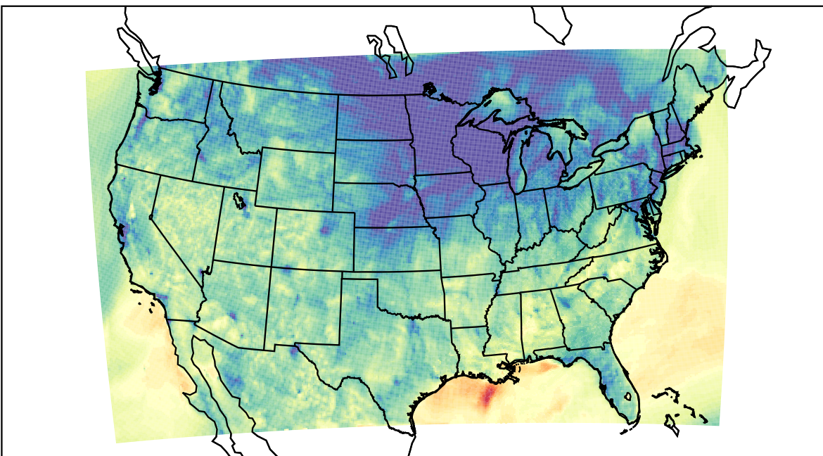
WRF (2020-11-05_03:00:00)
