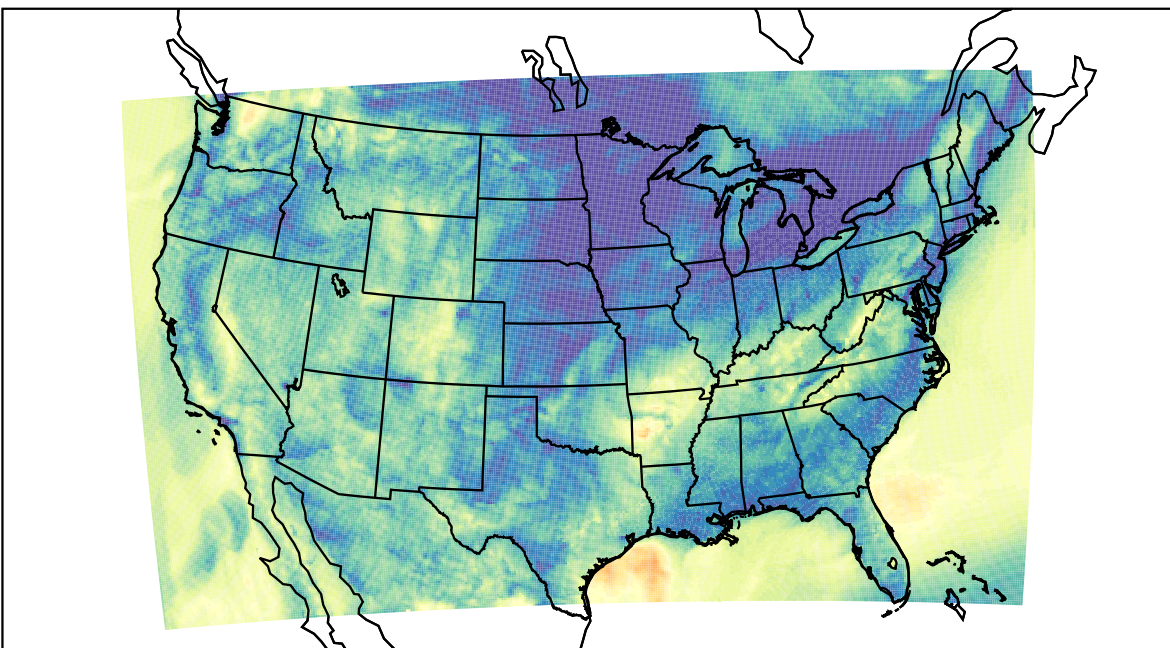
WRF (2020-11-06_11:00:00)
