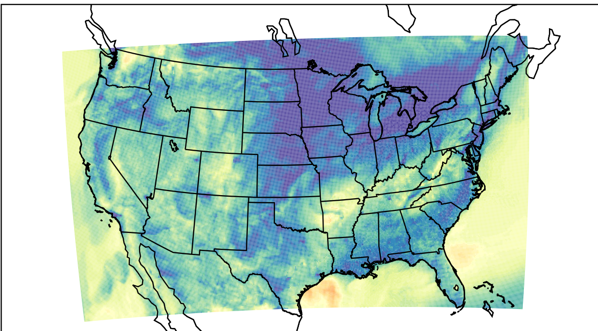
WRF (2020-11-06_12:00:00)
