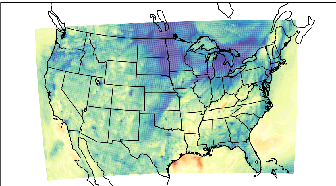
WRF (2020-11-06_02:00:00)
