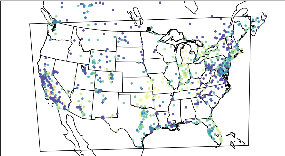
AirNOW (2020-11-05_03:00:00)
