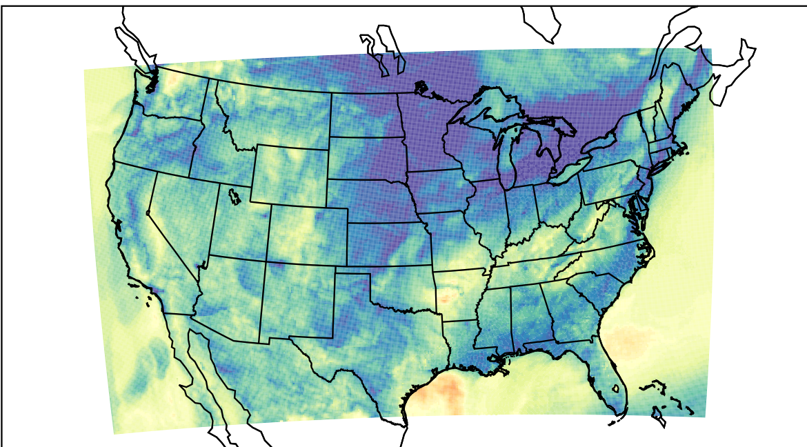
WRF (2020-11-06_10:00:00)
