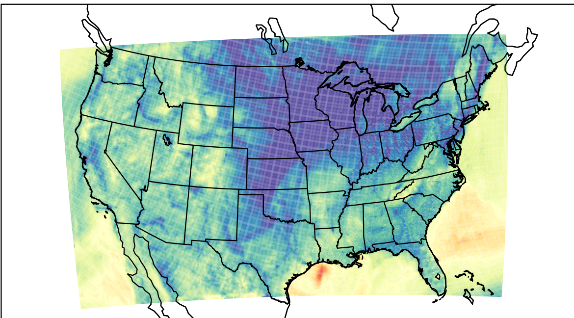
WRF (2020-11-05_12:00:00)
