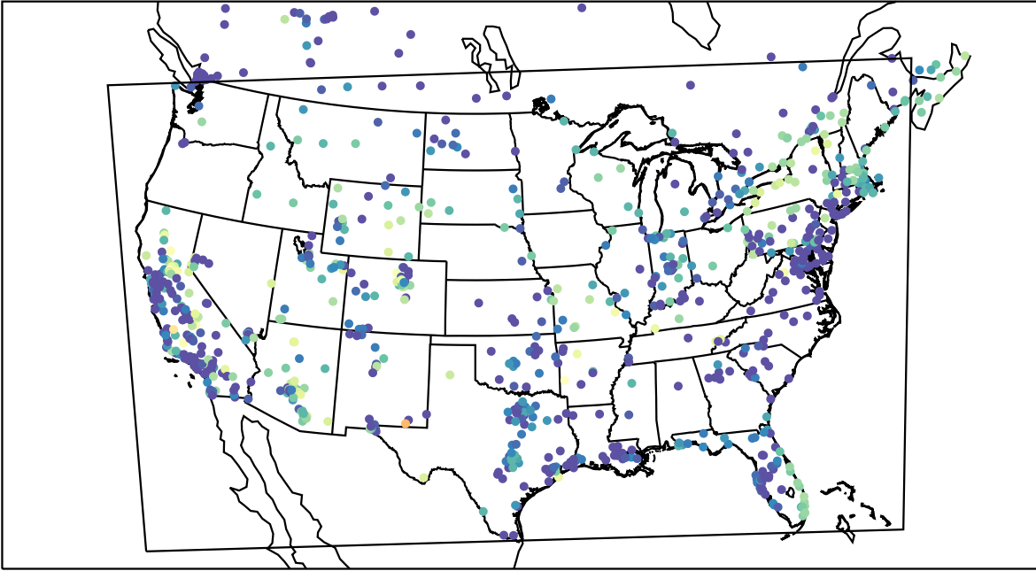
AirNOW (2020-11-06_07:00:00)
