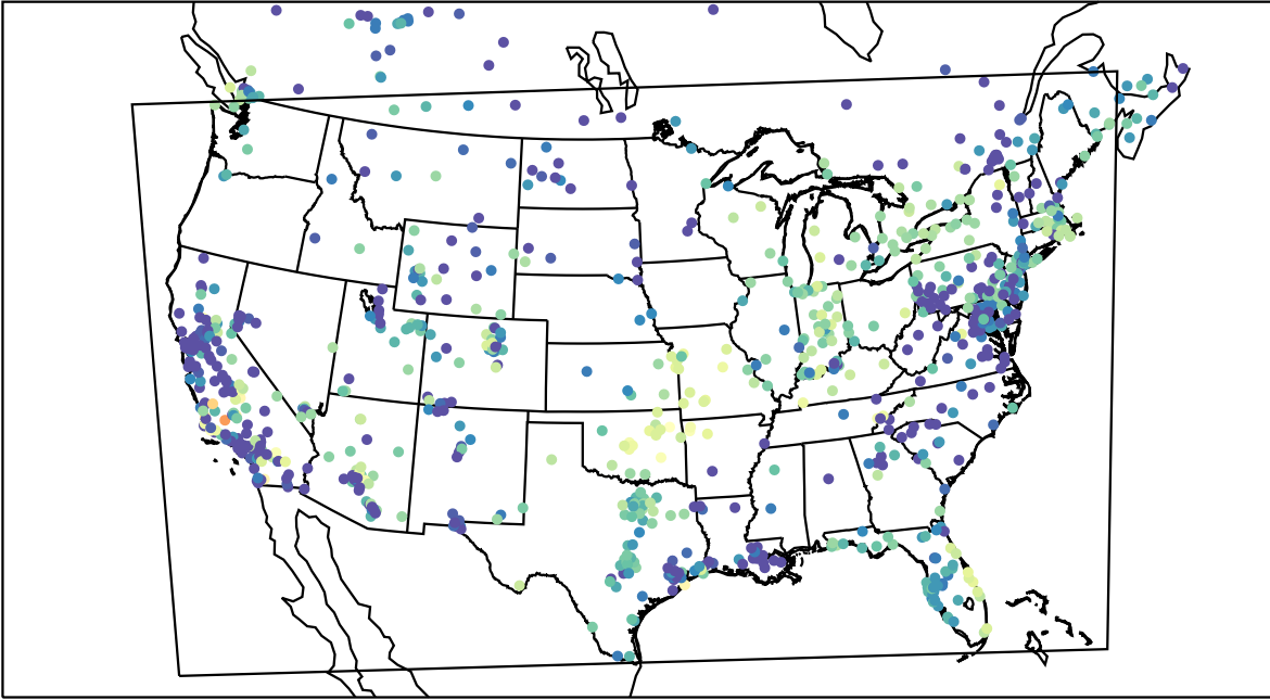
AirNOW (2020-11-05_05:00:00)
