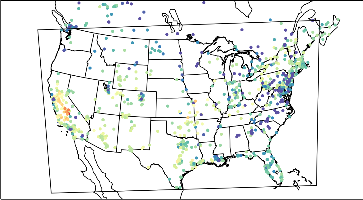
AirNOW (2020-11-05_23:00:00)
