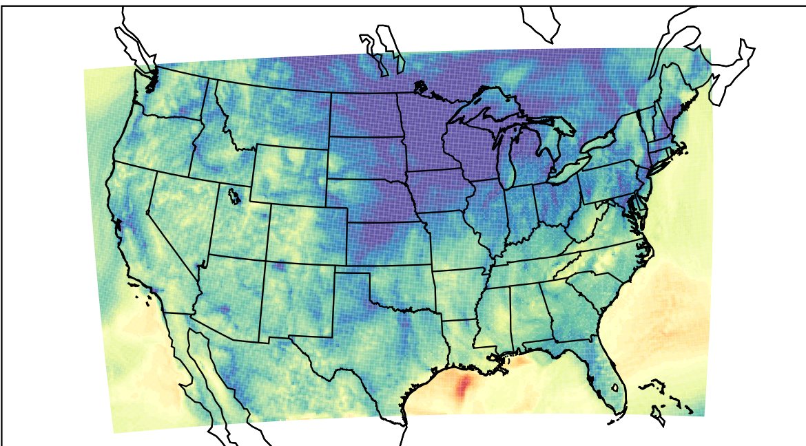
WRF (2020-11-05_07:00:00)
