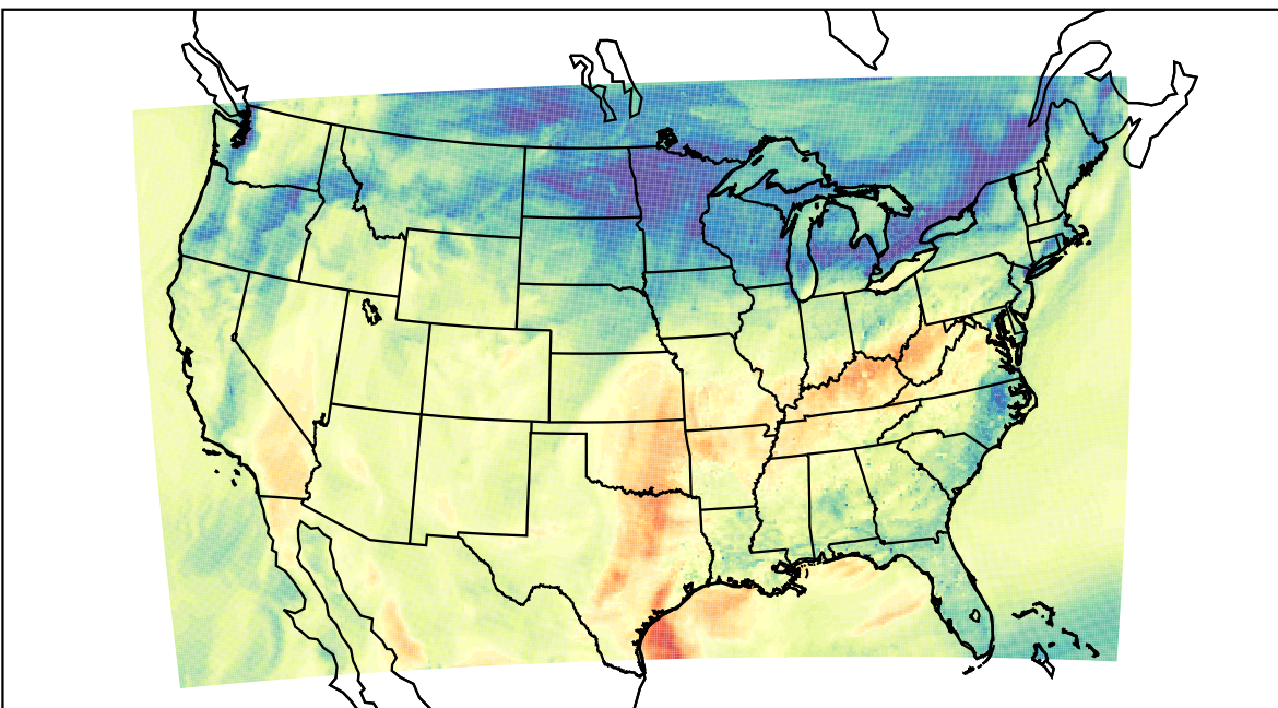
WRF (2020-11-06_22:00:00)
