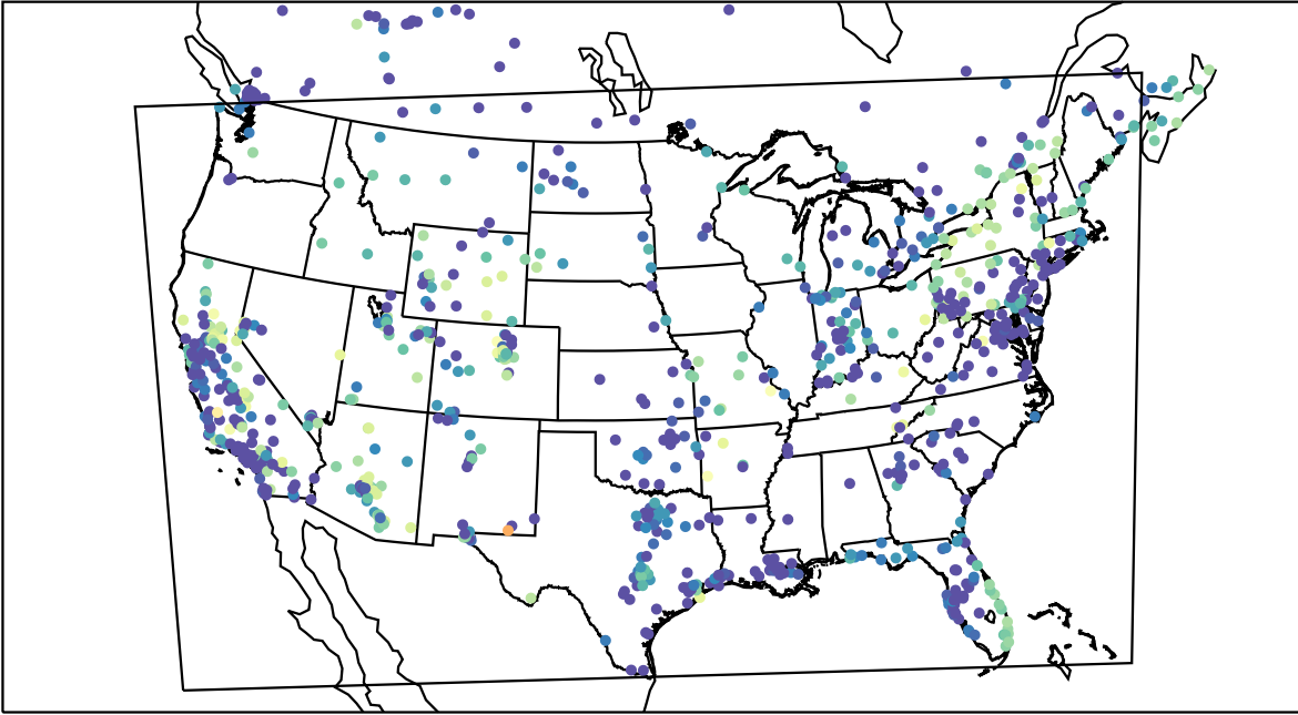
AirNOW (2020-11-06_08:00:00)
