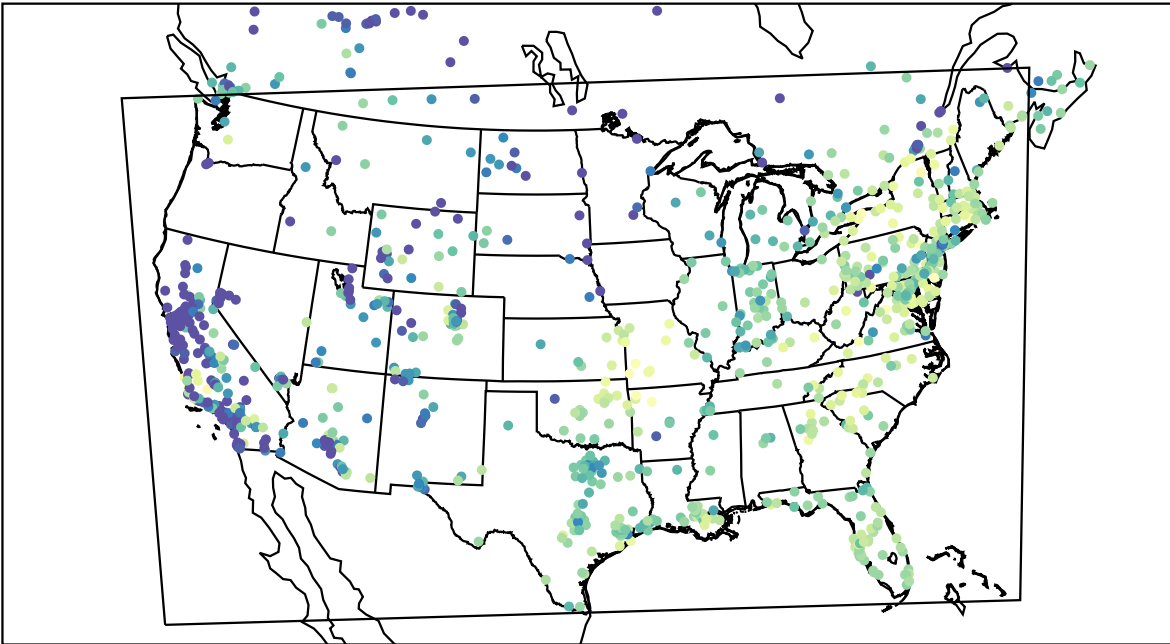
AirNOW (2020-11-05_16:00:00)
