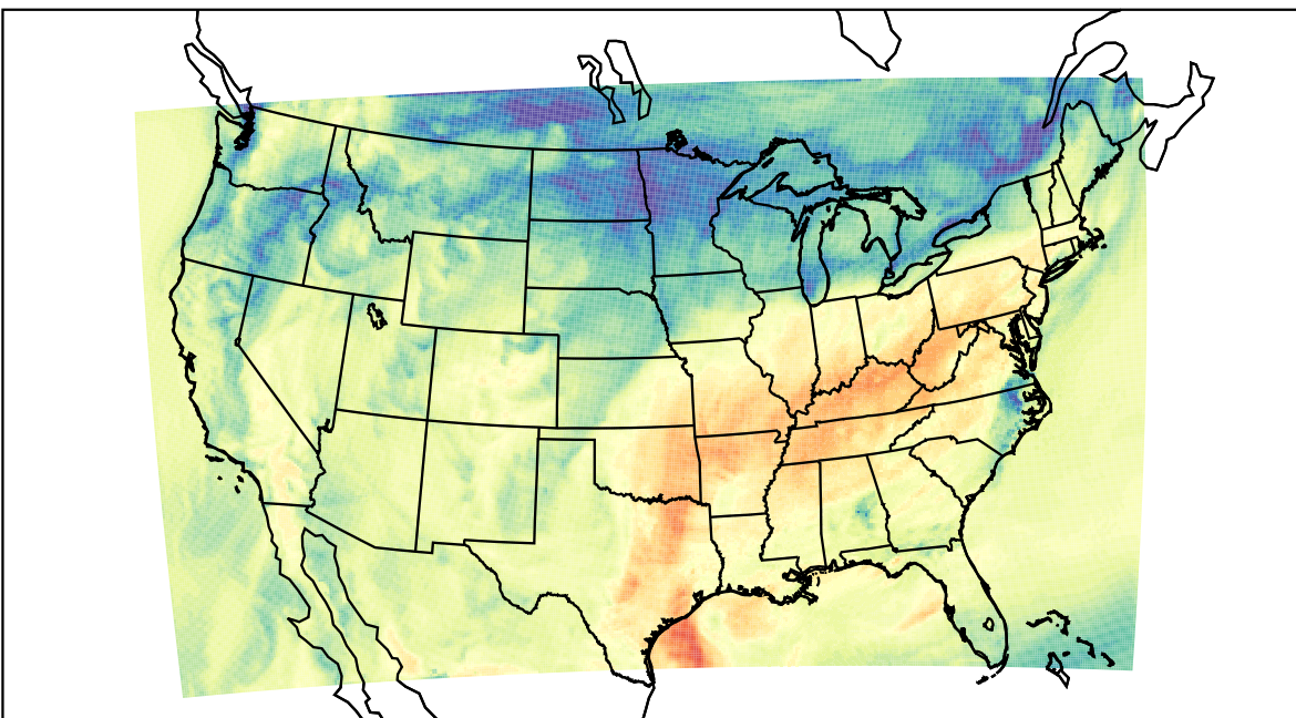
WRF (2020-11-06_19:00:00)
