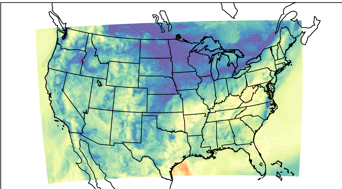
WRF (2020-11-06_16:00:00)
