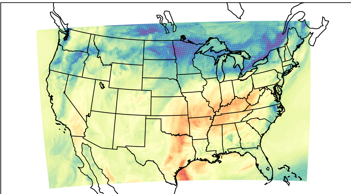
WRF (2020-11-06_21:00:00)
