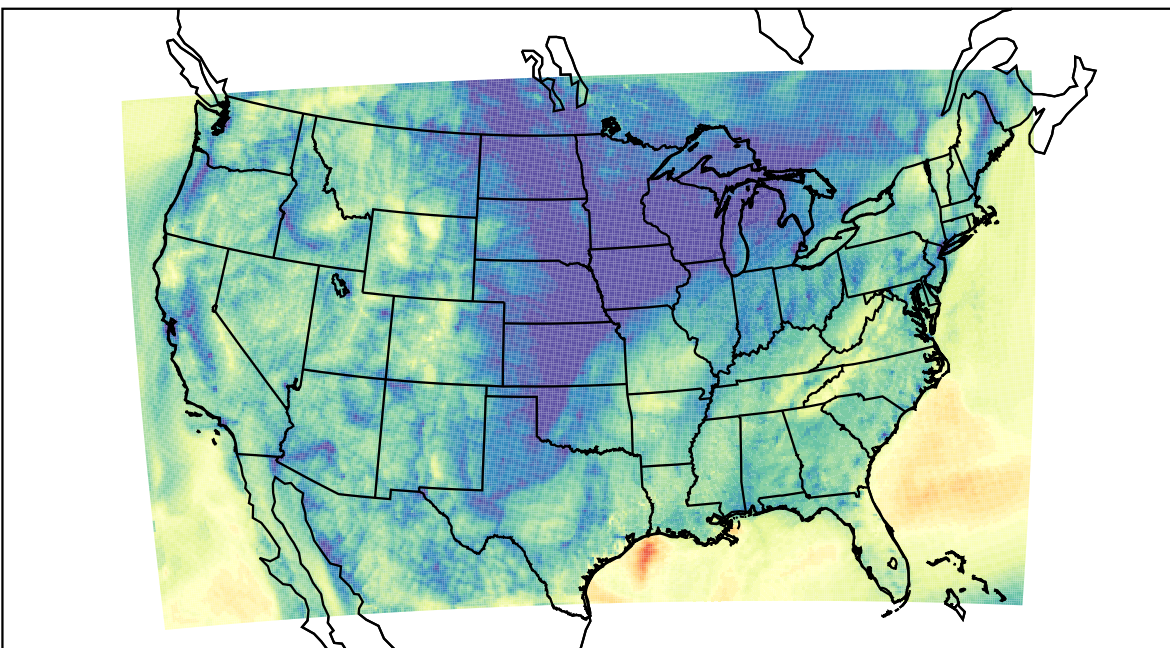
WRF (2020-11-05_15:00:00)
