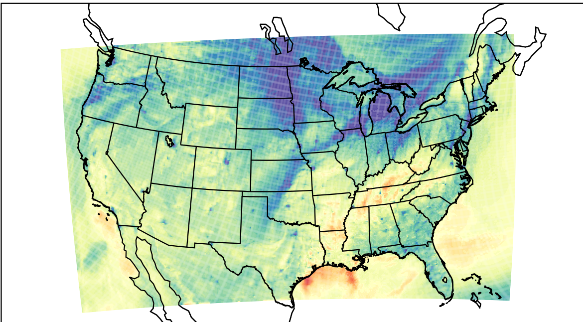
WRF (2020-11-06_00:00:00)
