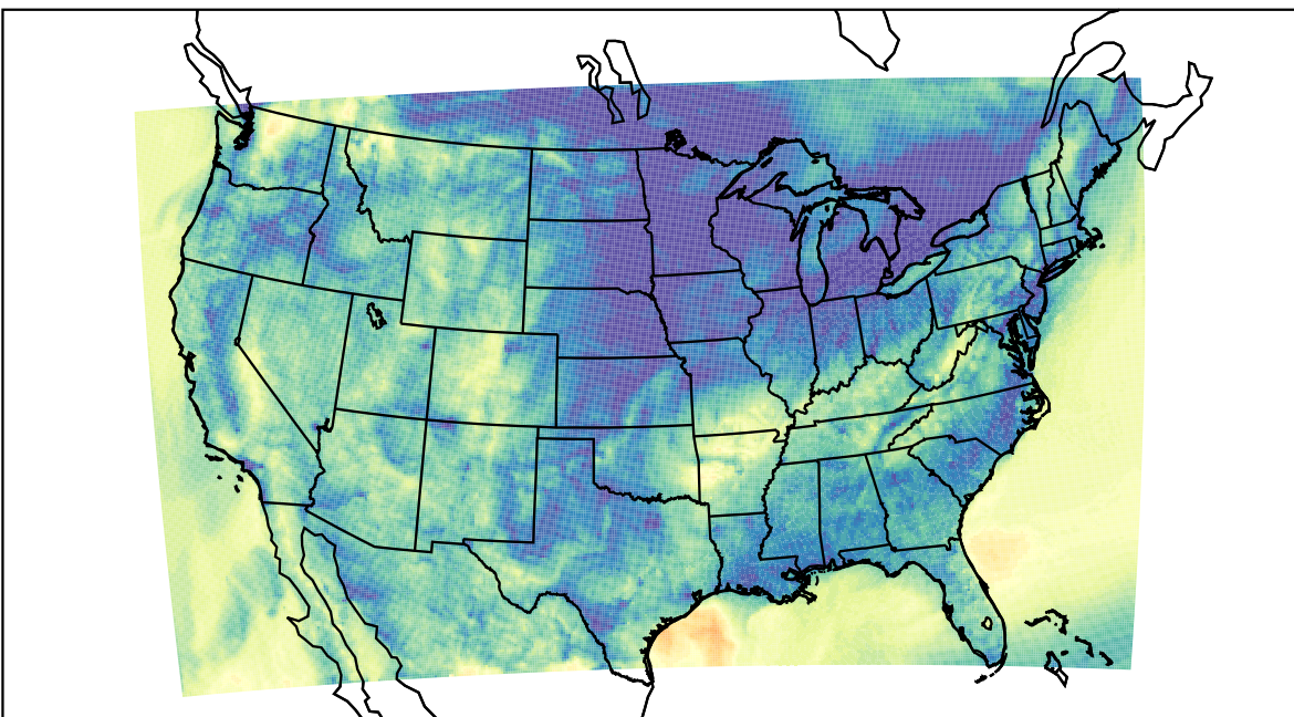
WRF (2020-11-06_13:00:00)
