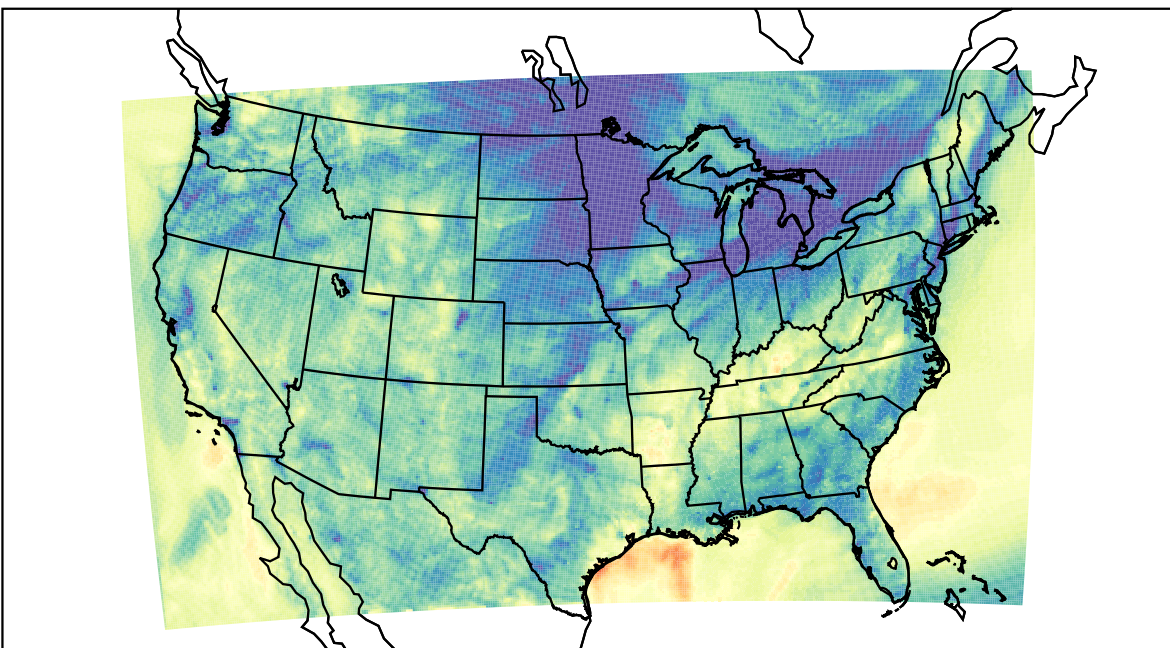
WRF (2020-11-06_05:00:00)
