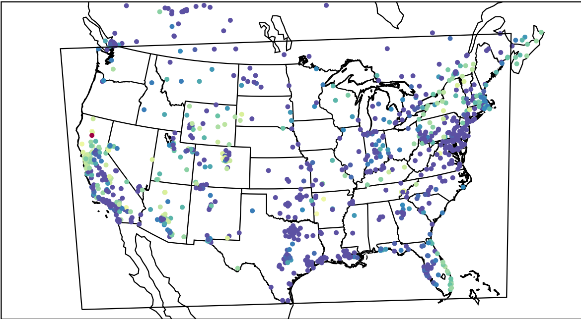
AirNOW (2020-11-06_13:00:00)
