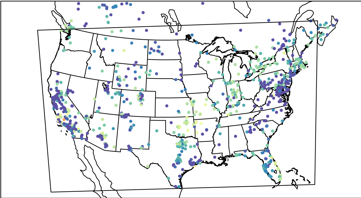
AirNOW (2020-11-05_07:00:00)
