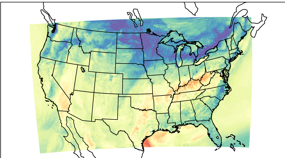
WRF (2020-11-06_23:00:00)
