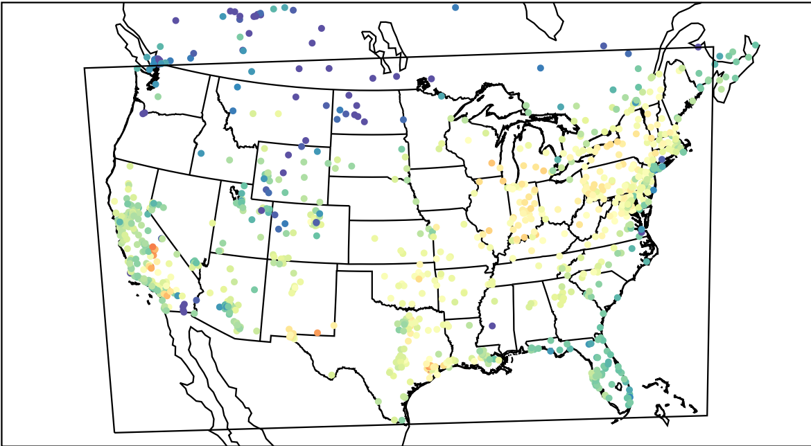
AirNOW (2020-11-06_19:00:00)
