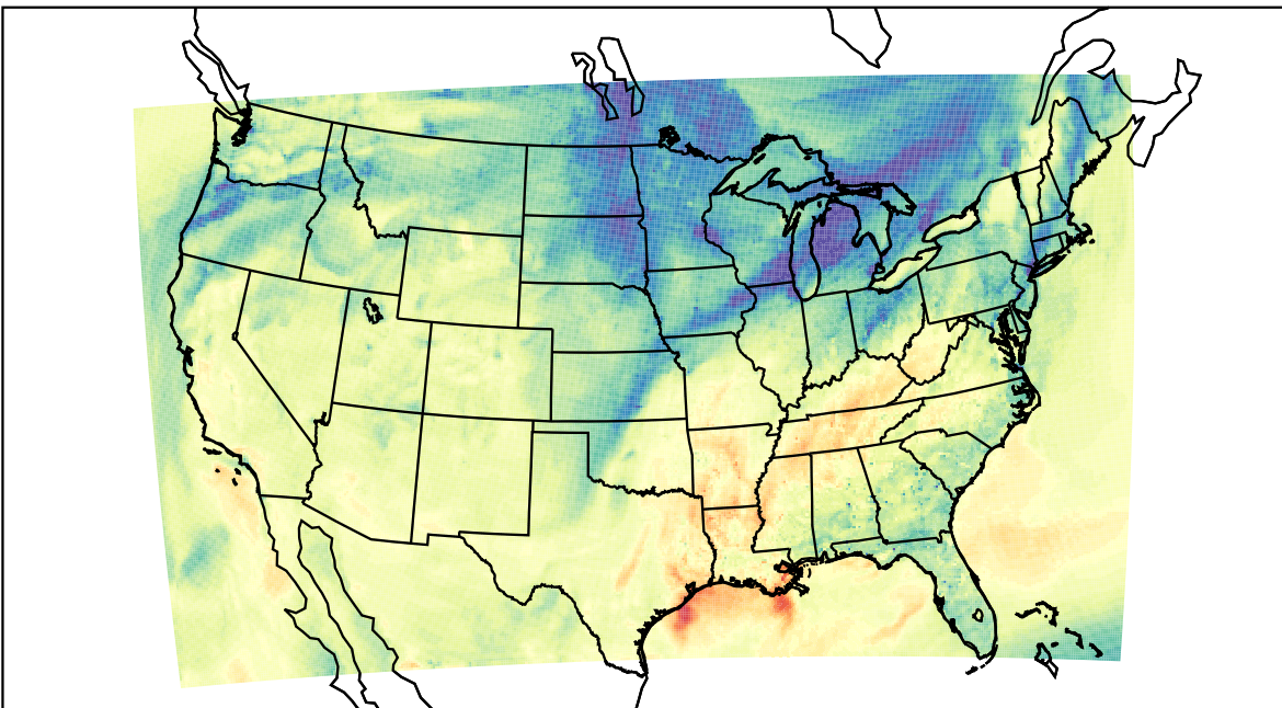
WRF (2020-11-05_22:00:00)
