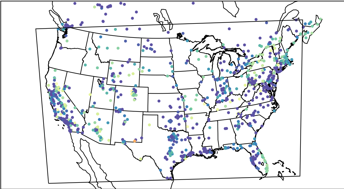
AirNOW (2020-11-06_09:00:00)
