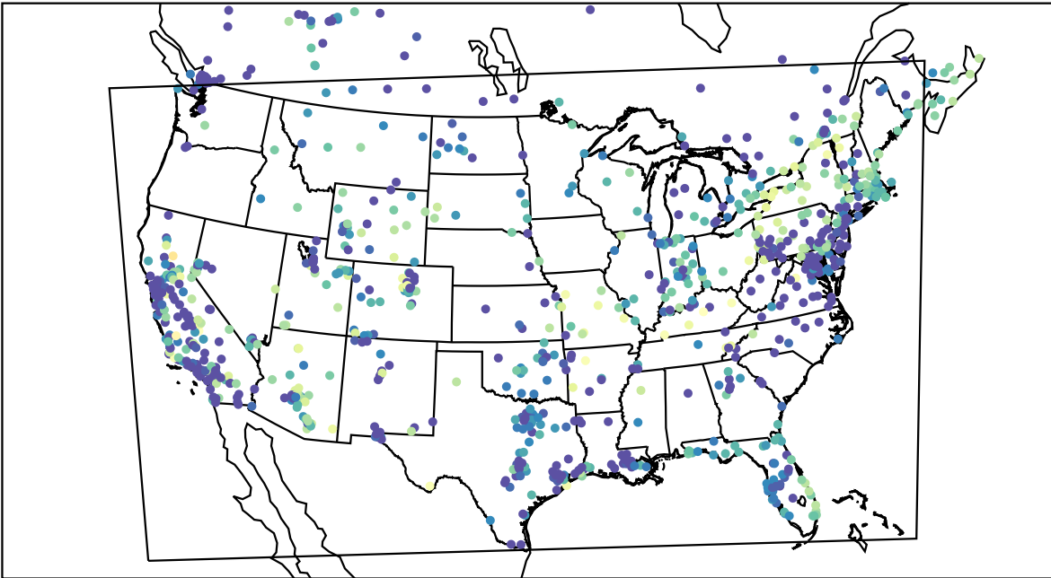
AirNOW (2020-11-06_04:00:00)
