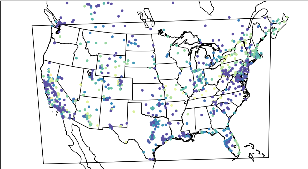
AirNOW (2020-11-06_05:00:00)
