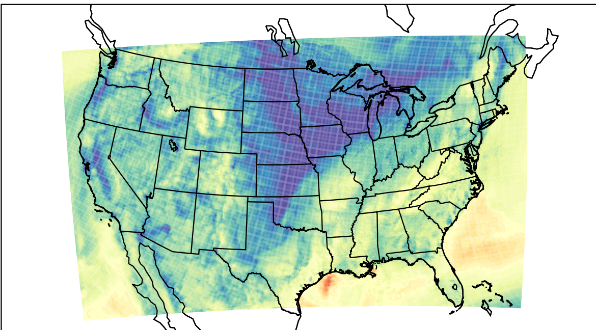
WRF (2020-11-05_16:00:00)
