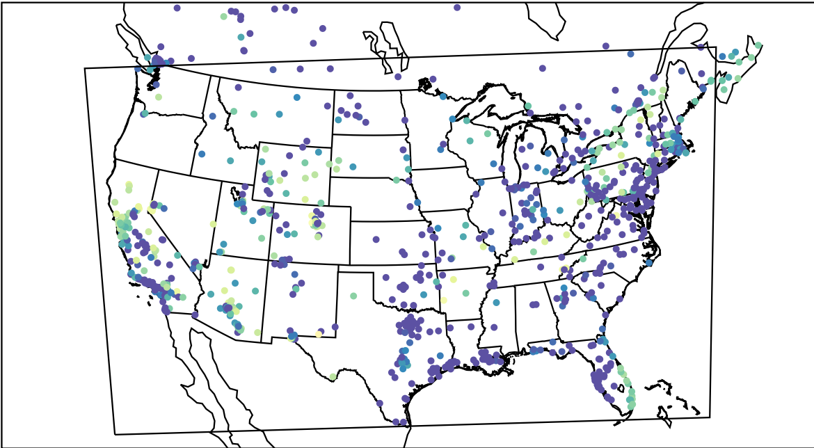
AirNOW (2020-11-06_12:00:00)
