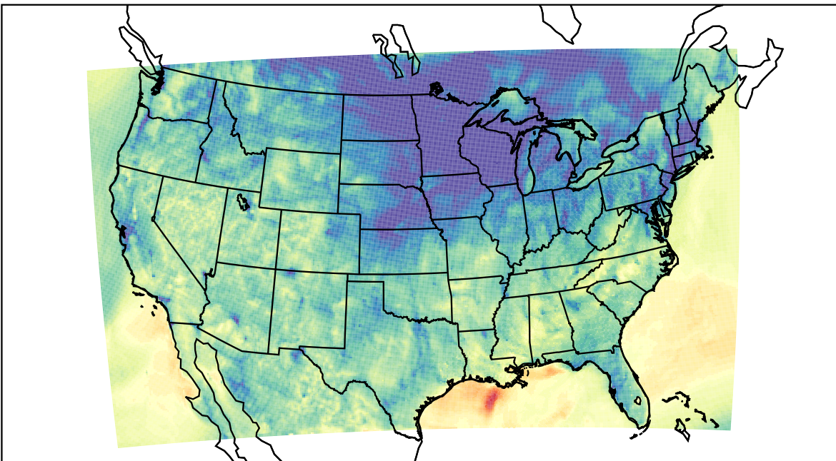
WRF (2020-11-05_04:00:00)
