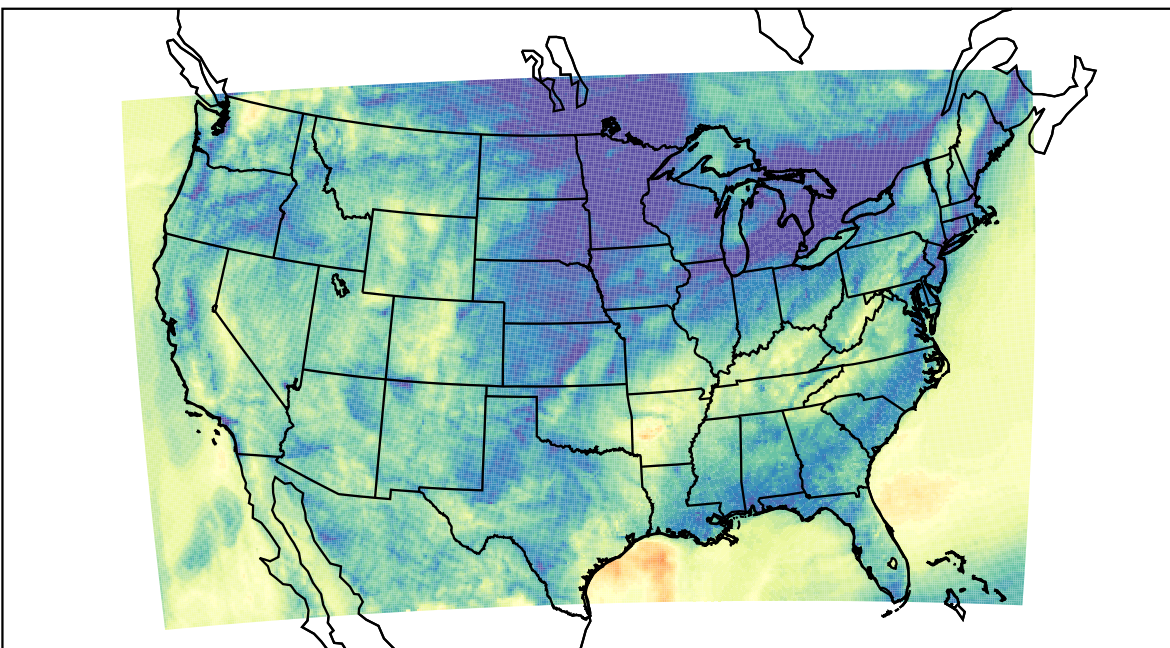
WRF (2020-11-06_09:00:00)
