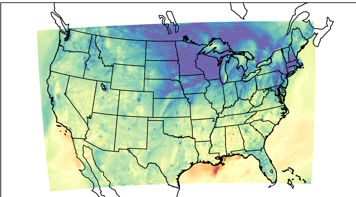
WRF (2020-11-05_00:00:00)
