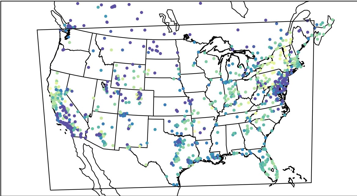
AirNOW (2020-11-06_15:00:00)
