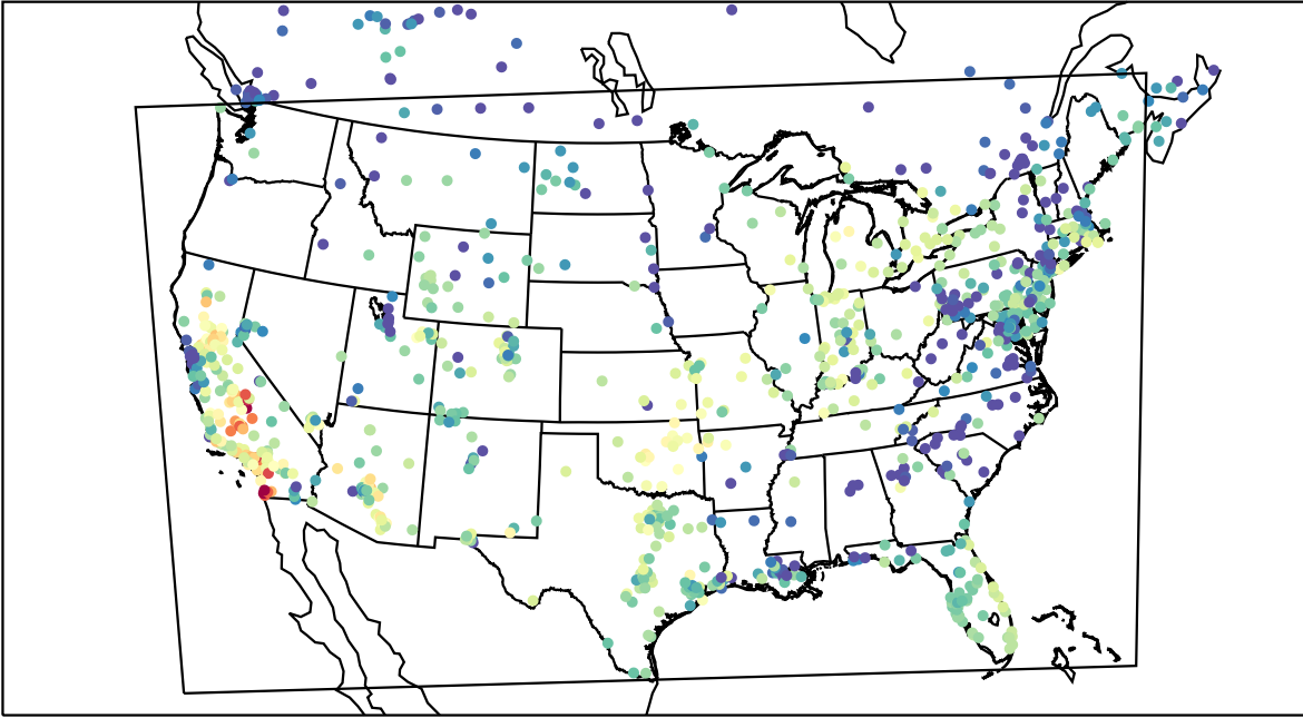
AirNOW (2020-11-05_00:00:00)
