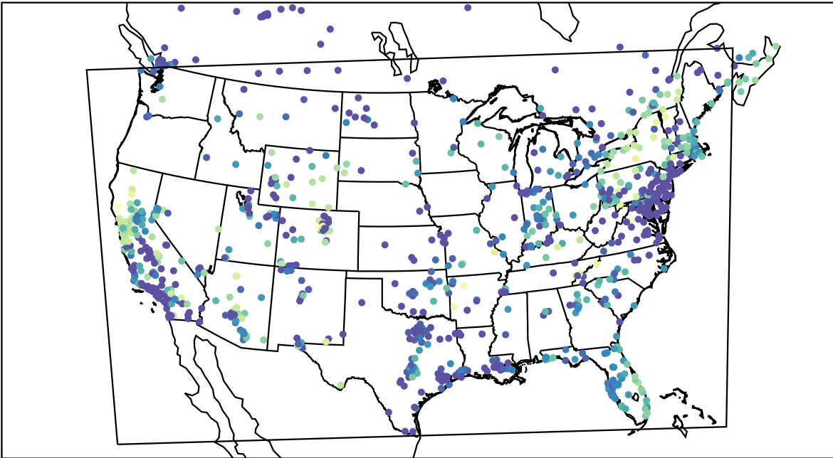
AirNOW (2020-11-06_14:00:00)
