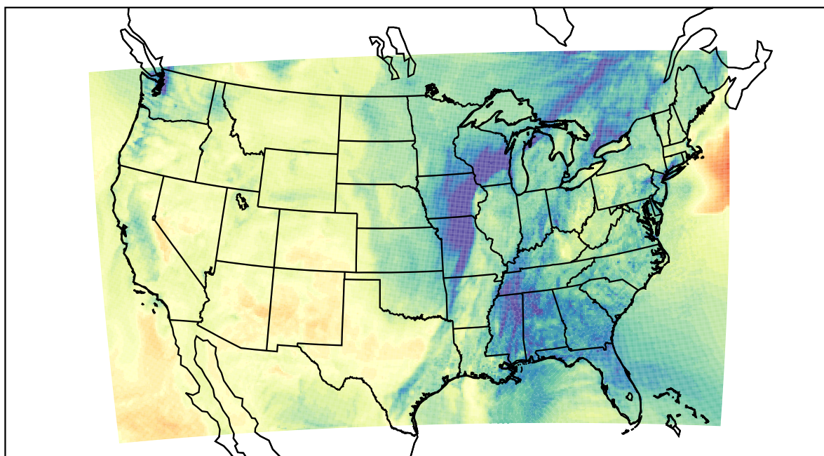
WRF (2020-11-10_21:00:00)
