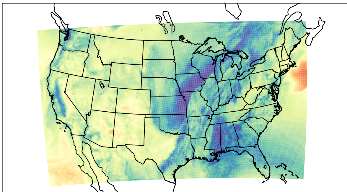
WRF (2020-11-10_17:00:00)
