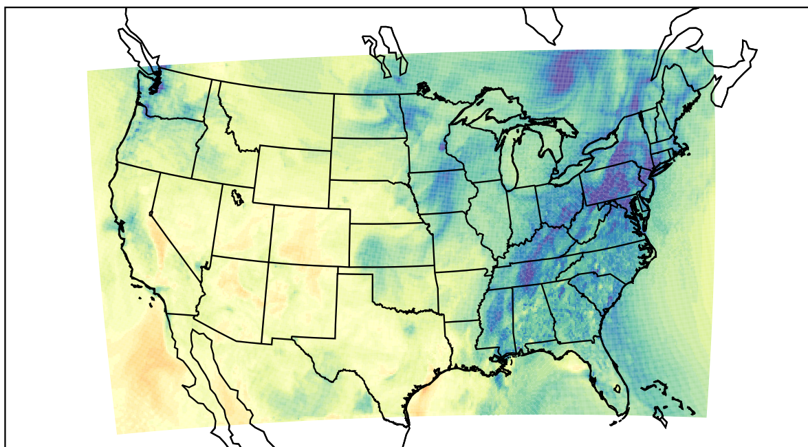
WRF (2020-11-11_21:00:00)
