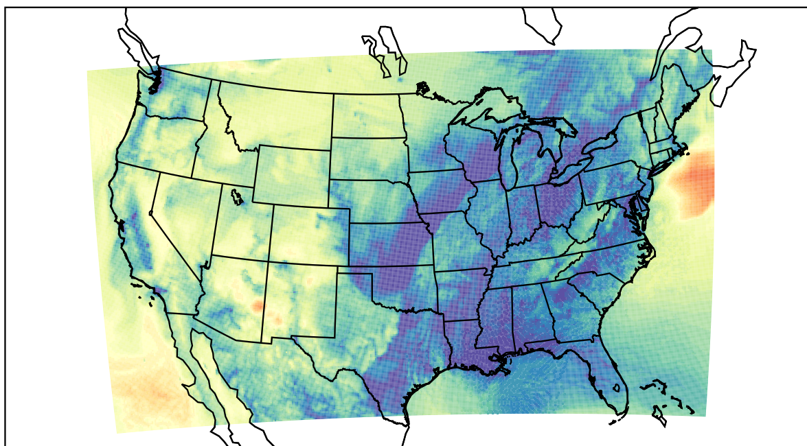
WRF (2020-11-10_14:00:00)
