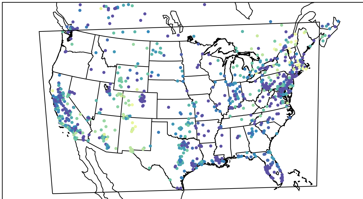
AirNOW (2020-11-10_01:00:00)
