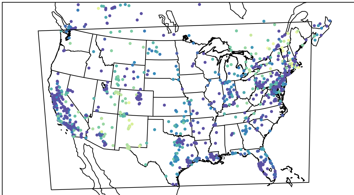
AirNOW (2020-11-10_02:00:00)
