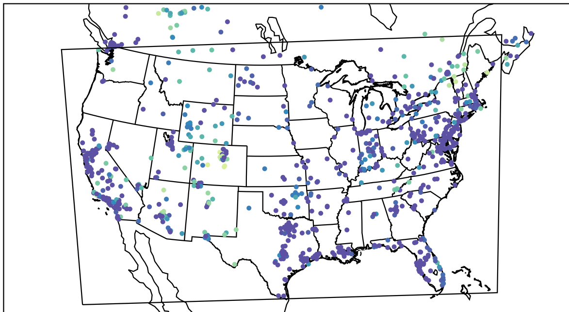
AirNOW (2020-11-10_12:00:00)
