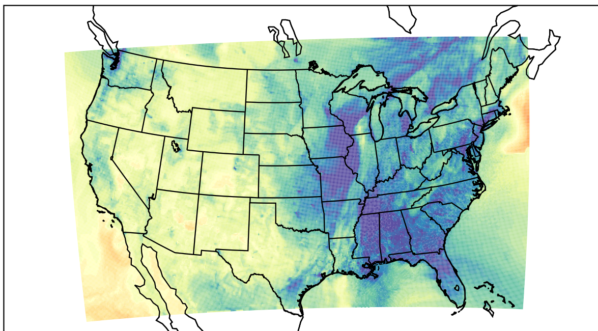
WRF (2020-11-11_00:00:00)
