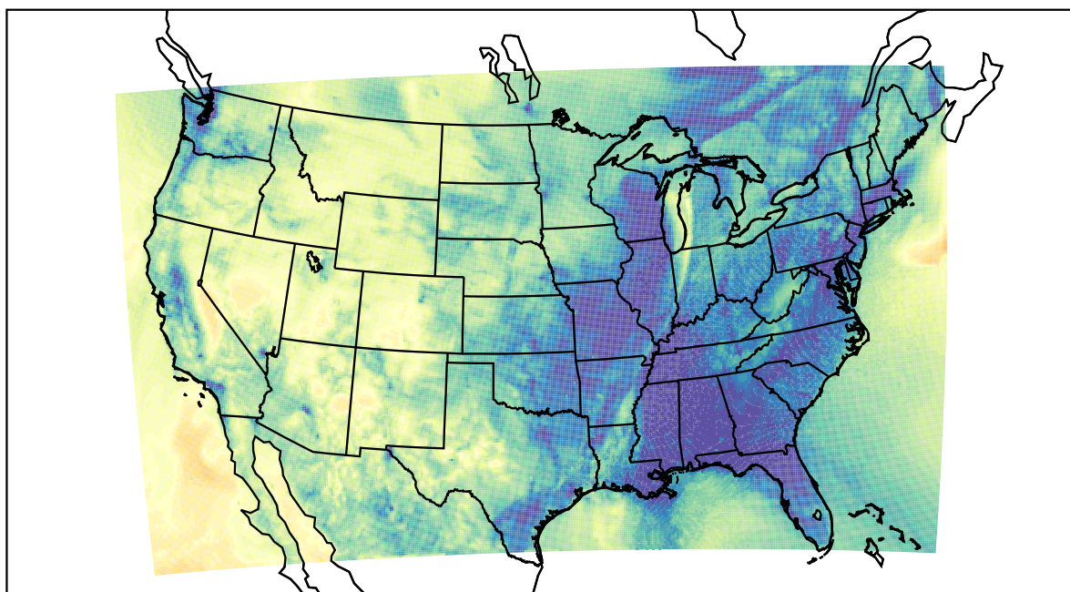
WRF (2020-11-11_04:00:00)
