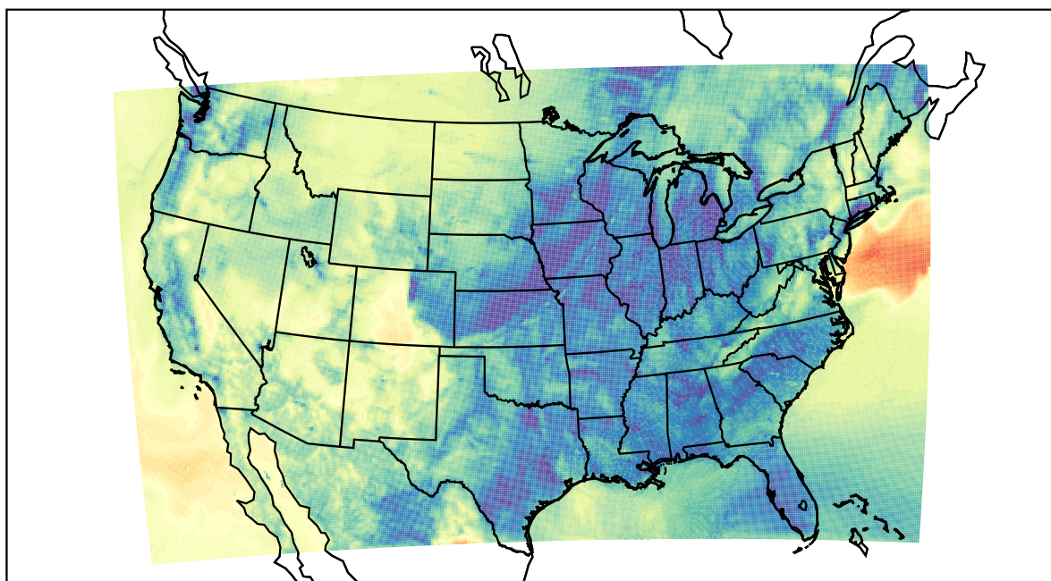
WRF (2020-11-10_04:00:00)
