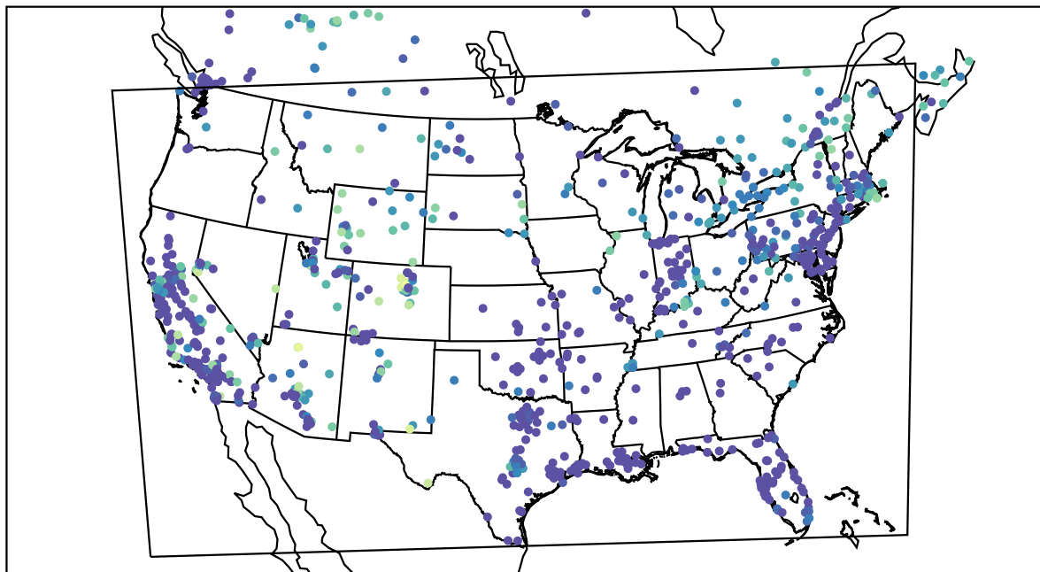
AirNOW (2020-11-11_09:00:00)
