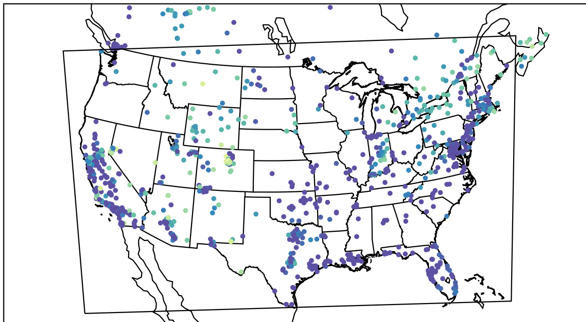
AirNOW (2020-11-11_06:00:00)
