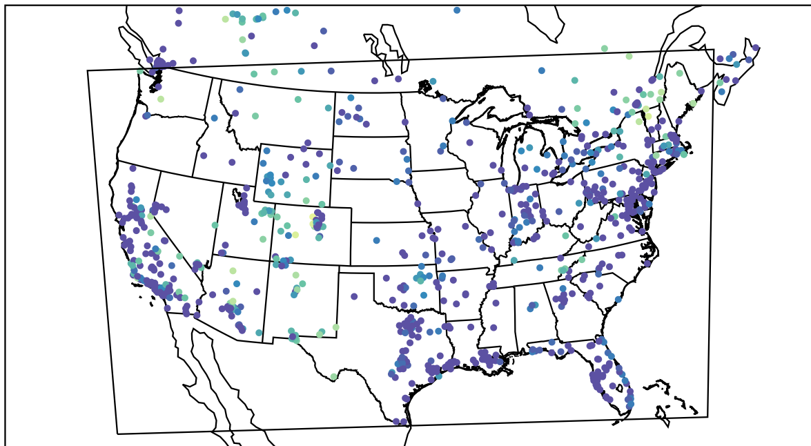
AirNOW (2020-11-10_11:00:00)
