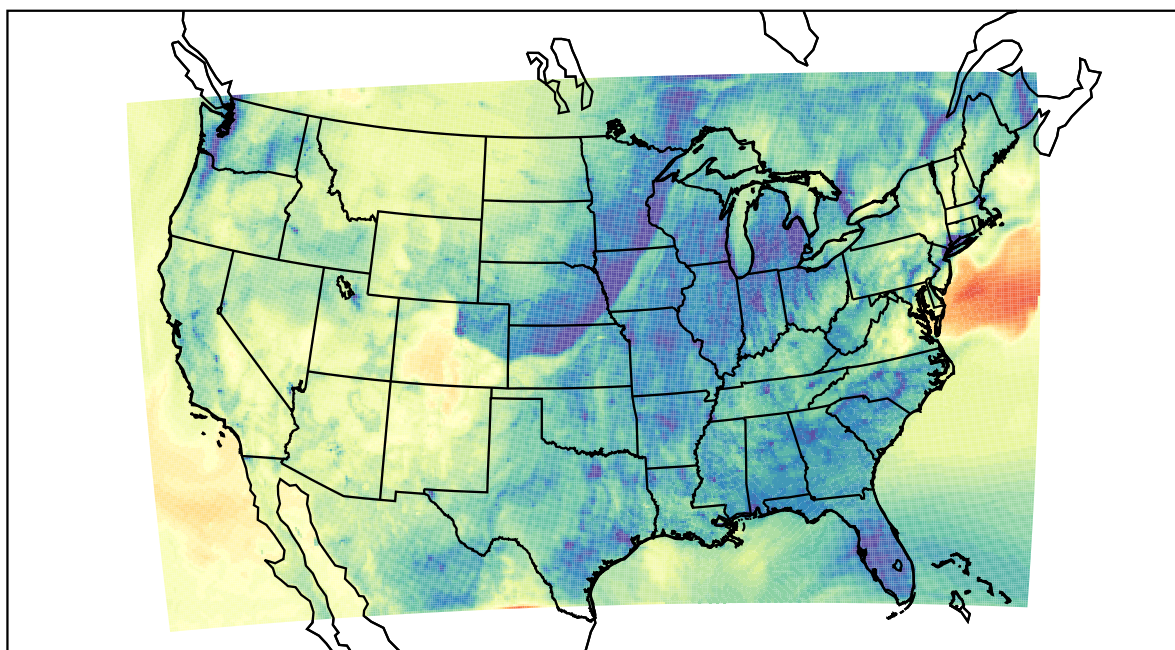
WRF (2020-11-10_01:00:00)
