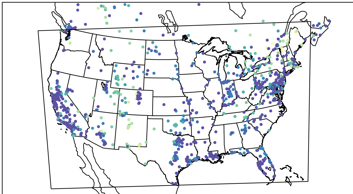
AirNOW (2020-11-10_05:00:00)
