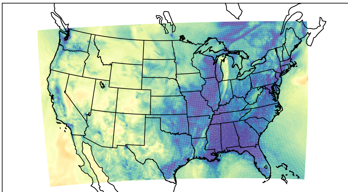
WRF (2020-11-11_05:00:00)
