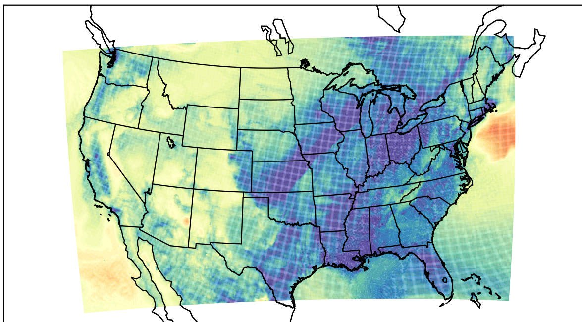
WRF (2020-11-10_11:00:00)
