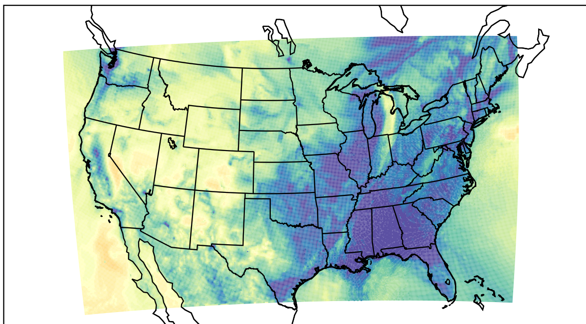
WRF (2020-11-11_07:00:00)
