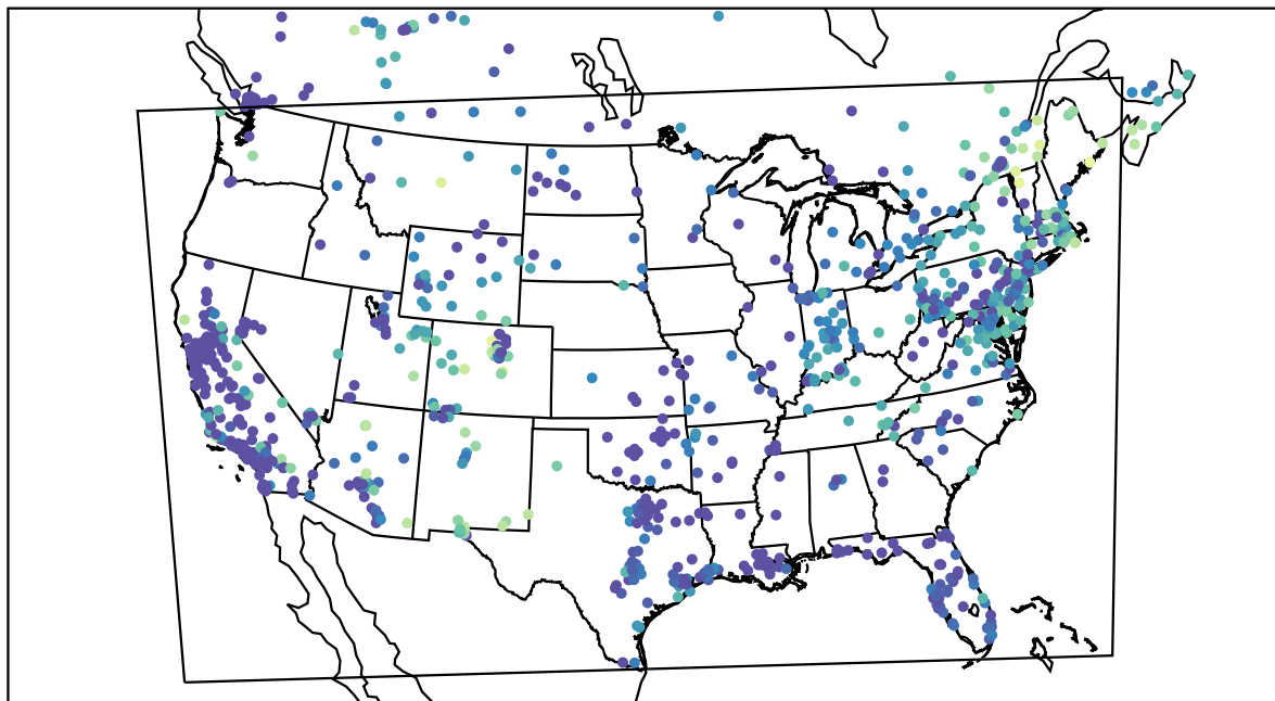
AirNOW (2020-11-10_15:00:00)
