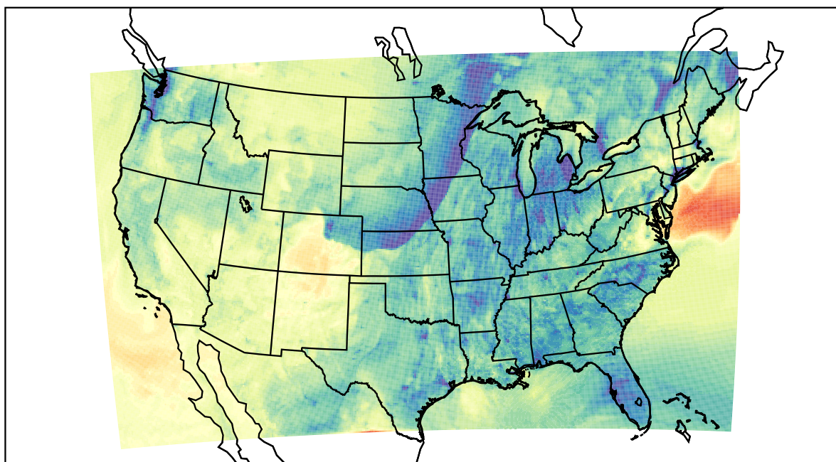
WRF (2020-11-10_00:00:00)
