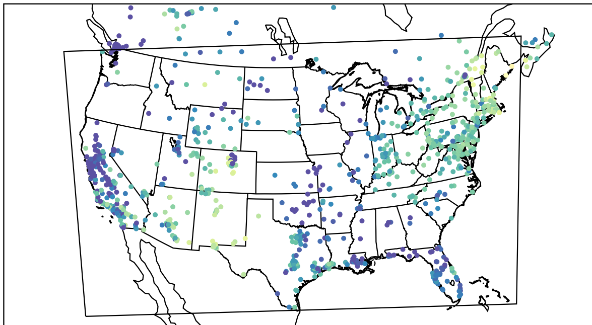
AirNOW (2020-11-10_17:00:00)
