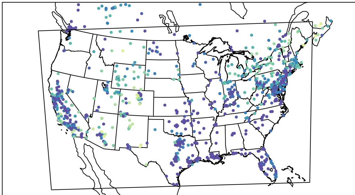
AirNOW (2020-11-11_02:00:00)
