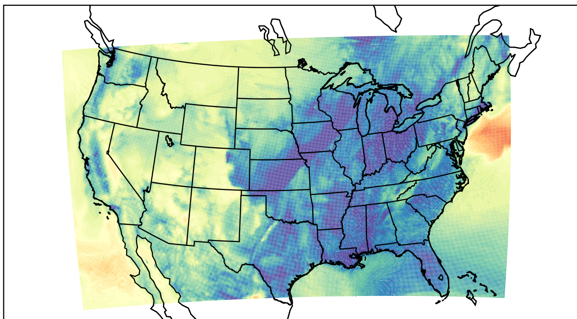
WRF (2020-11-10_09:00:00)
