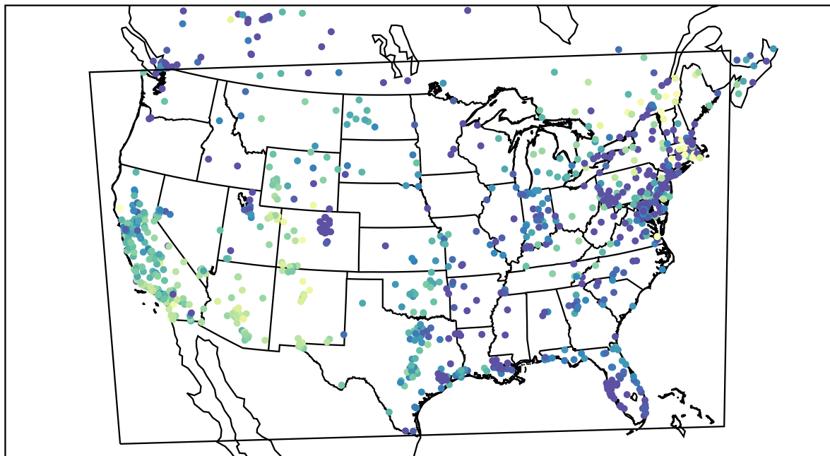
AirNOW (2020-11-10_00:00:00)
