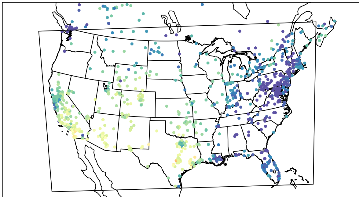
AirNOW (2020-11-11_21:00:00)
