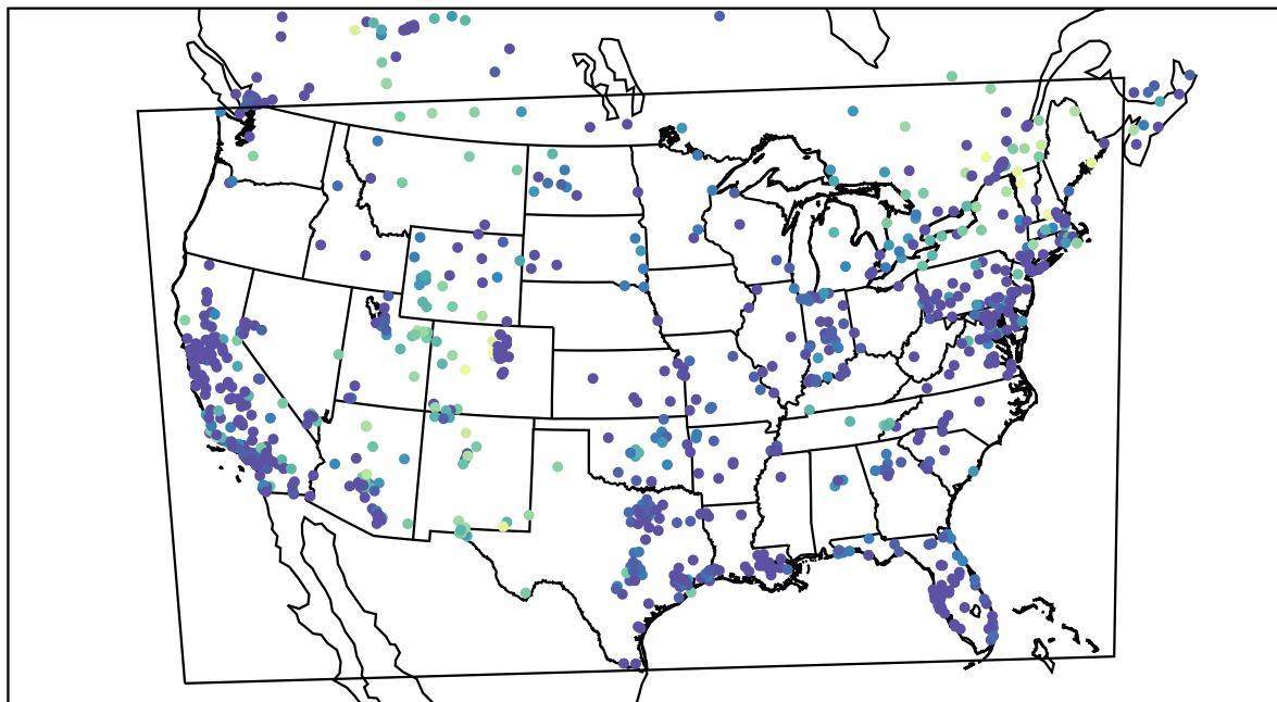
AirNOW (2020-11-10_07:00:00)
