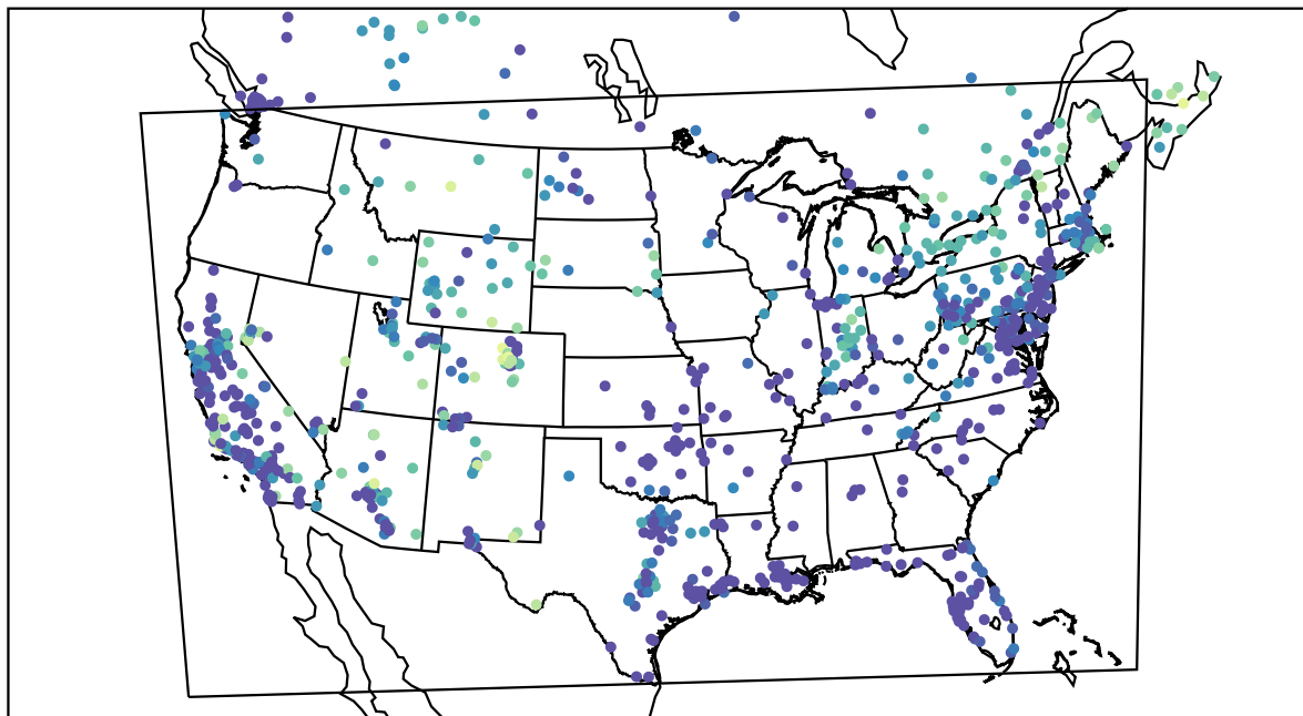
AirNOW (2020-11-11_05:00:00)
