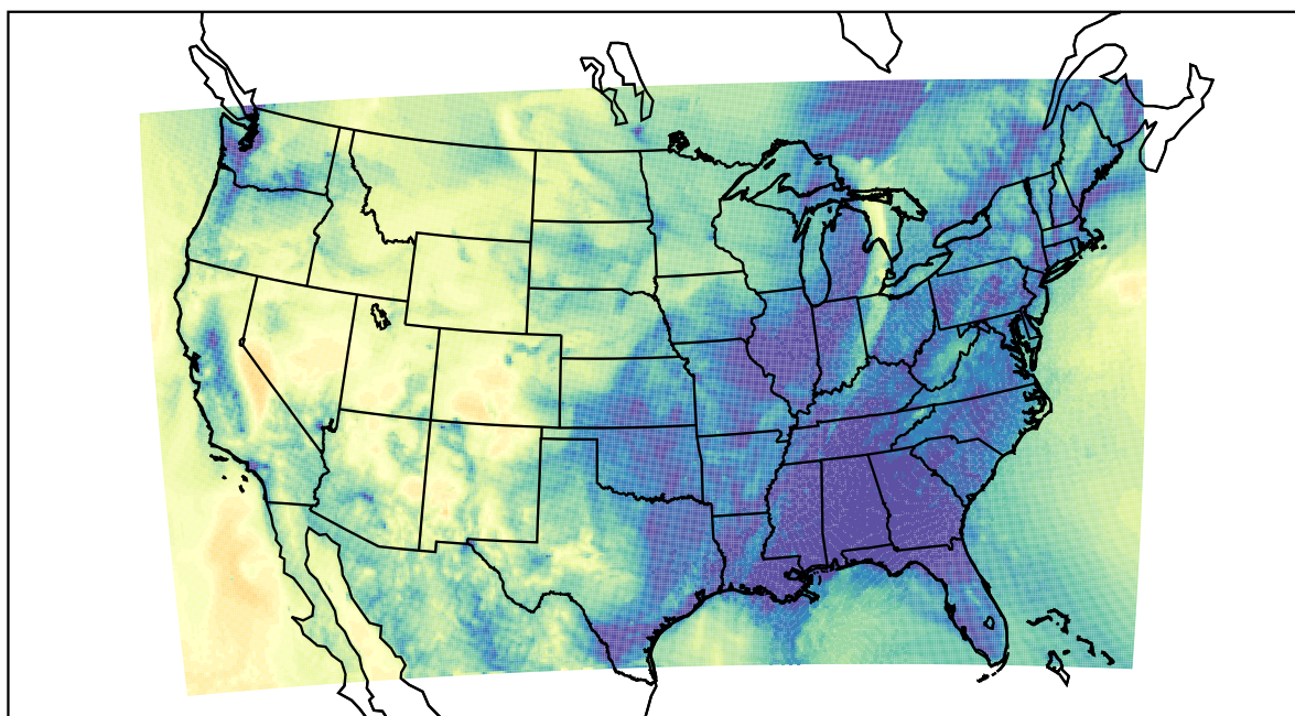
WRF (2020-11-11_09:00:00)
