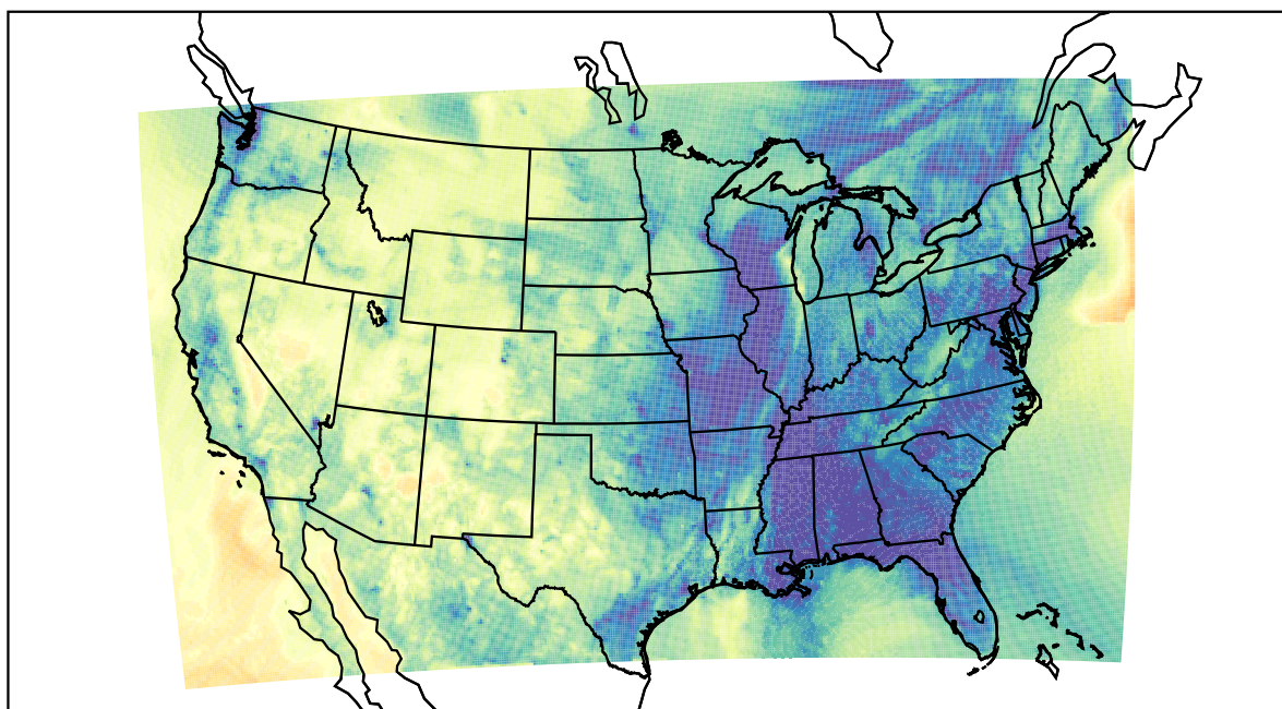
WRF (2020-11-11_02:00:00)
