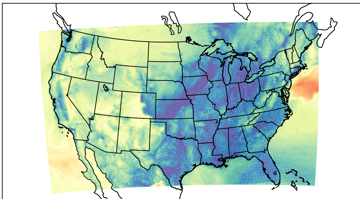
WRF (2020-11-10_07:00:00)
