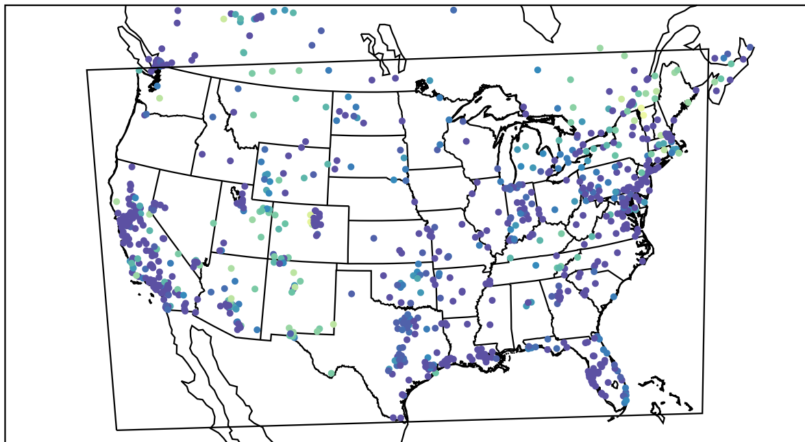
AirNOW (2020-11-10_09:00:00)
