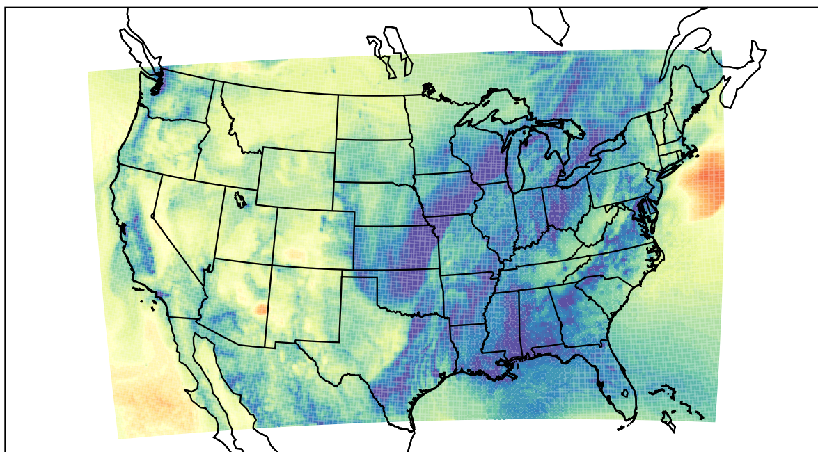
WRF (2020-11-10_15:00:00)
