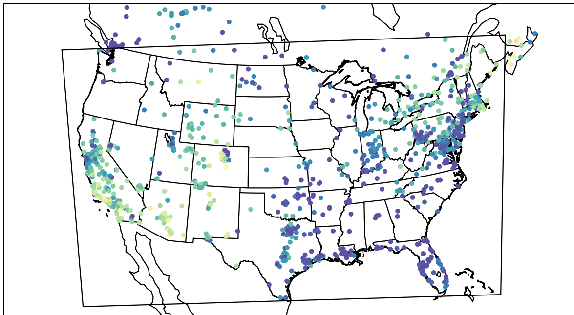
AirNOW (2020-11-11_00:00:00)
