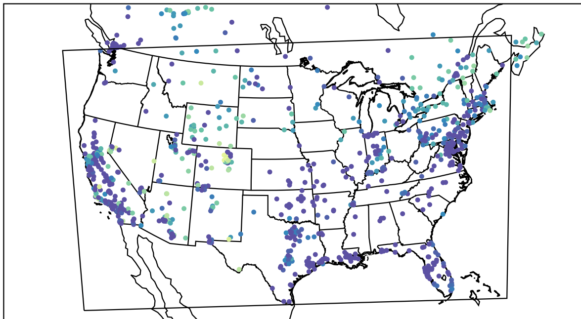
AirNOW (2020-11-11_07:00:00)
