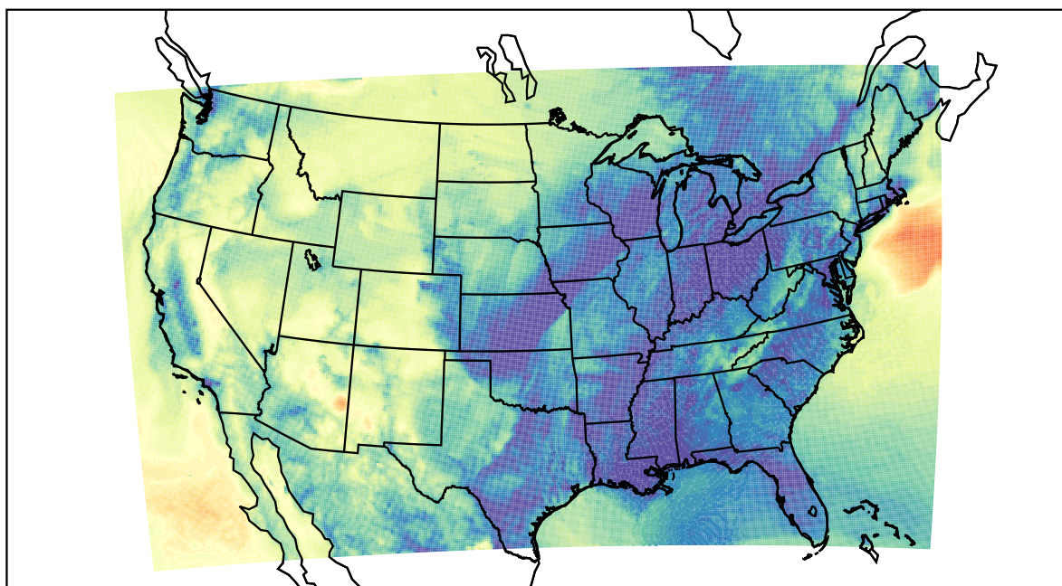
WRF (2020-11-10_12:00:00)
