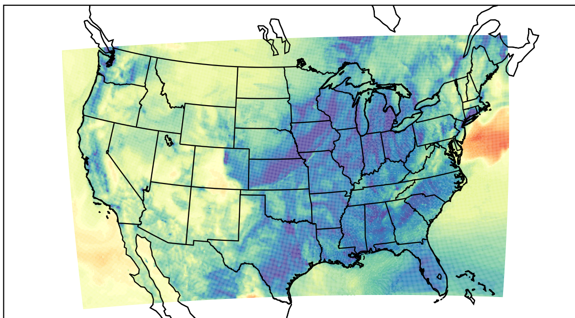
WRF (2020-11-10_05:00:00)
