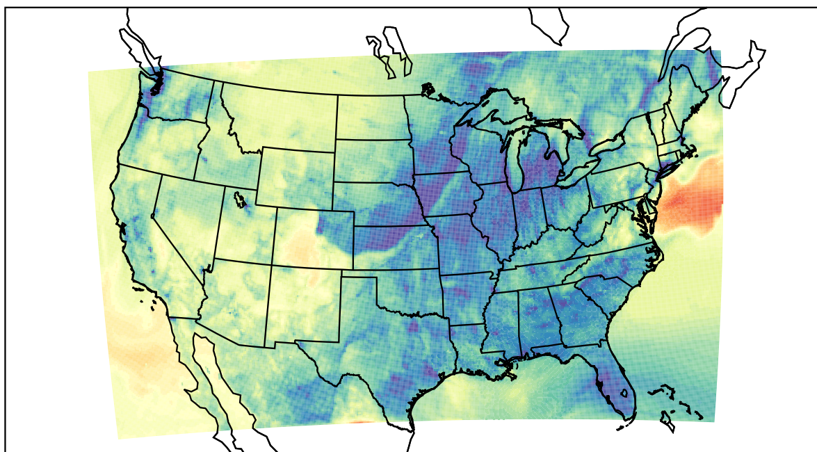
WRF (2020-11-10_02:00:00)
