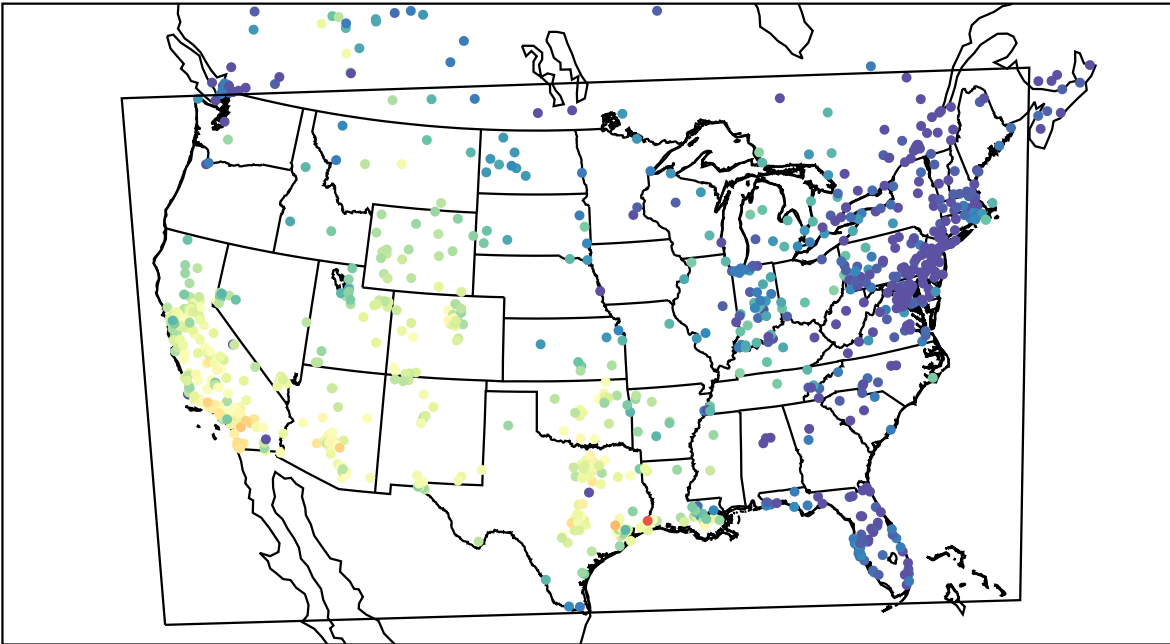
AirNOW (2020-11-12_22:00:00)
