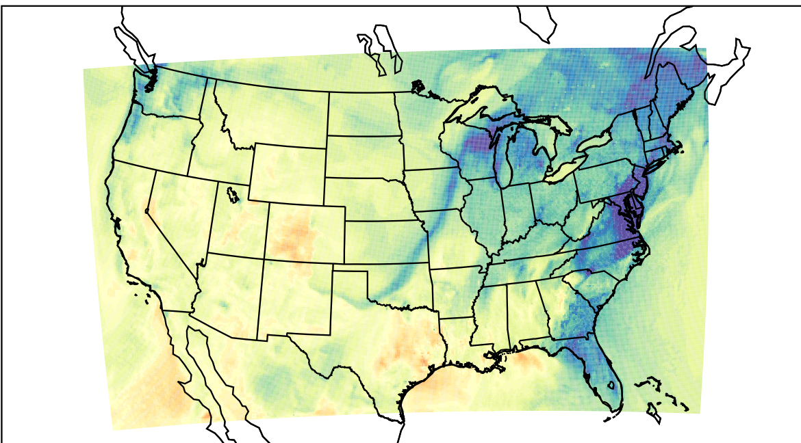
WRF (2020-11-12_21:00:00)
