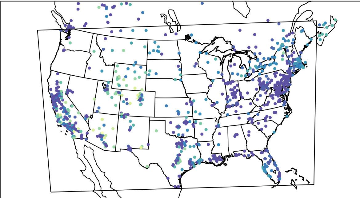
AirNOW (2020-11-12_02:00:00)
