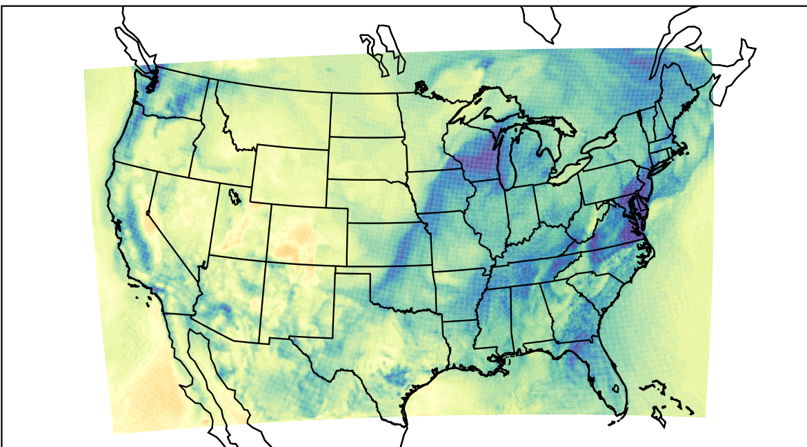
WRF (2020-11-12_17:00:00)
