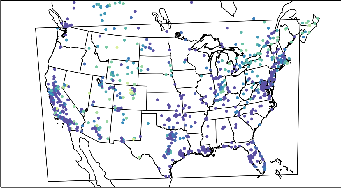
AirNOW (2020-11-11_06:00:00)
