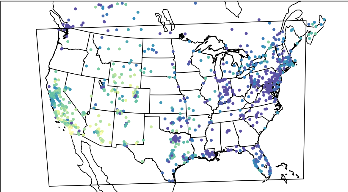
AirNOW (2020-11-12_00:00:00)
