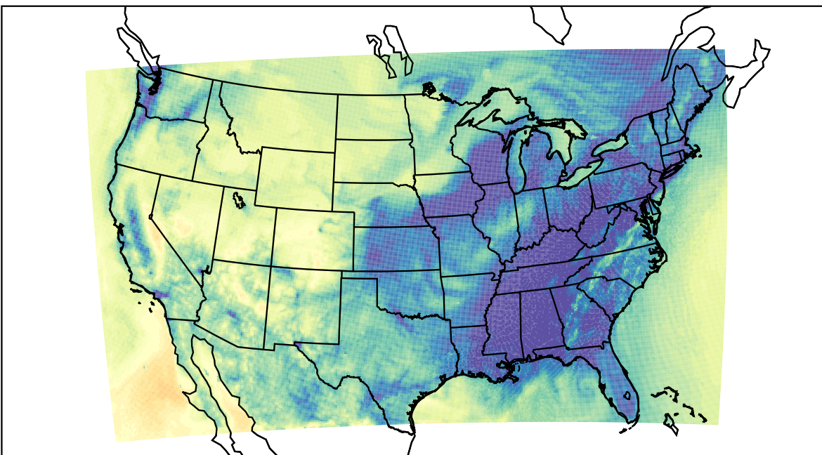
WRF (2020-11-12_08:00:00)
