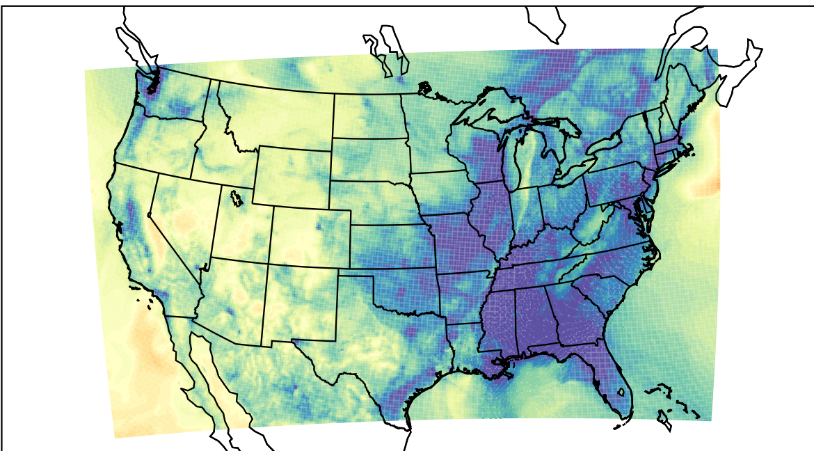
WRF (2020-11-11_04:00:00)
