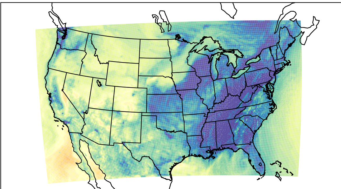
WRF (2020-11-12_05:00:00)
