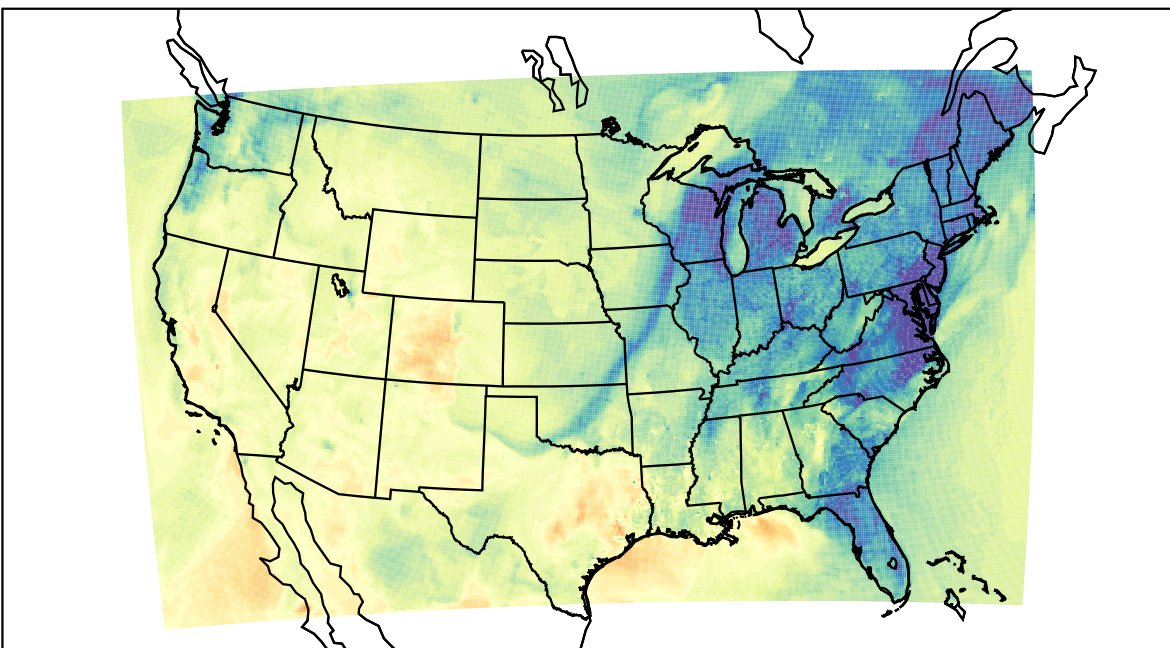
WRF (2020-11-12_22:00:00)
