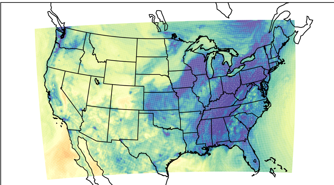
WRF (2020-11-12_03:00:00)
