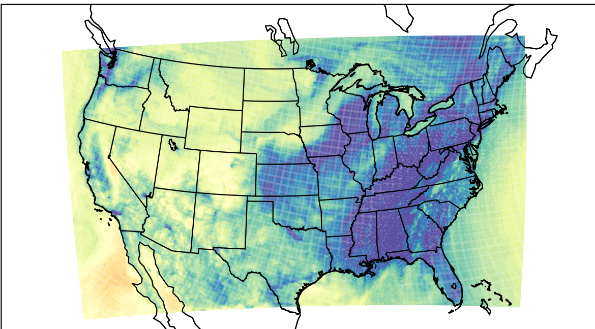
WRF (2020-11-12_06:00:00)
