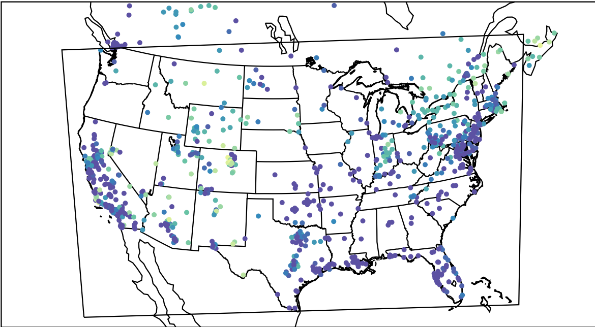
AirNOW (2020-11-11_05:00:00)
