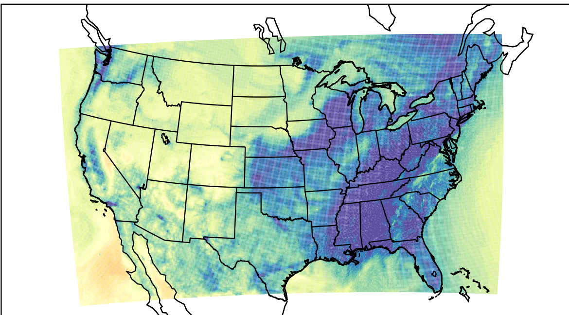
WRF (2020-11-12_07:00:00)
