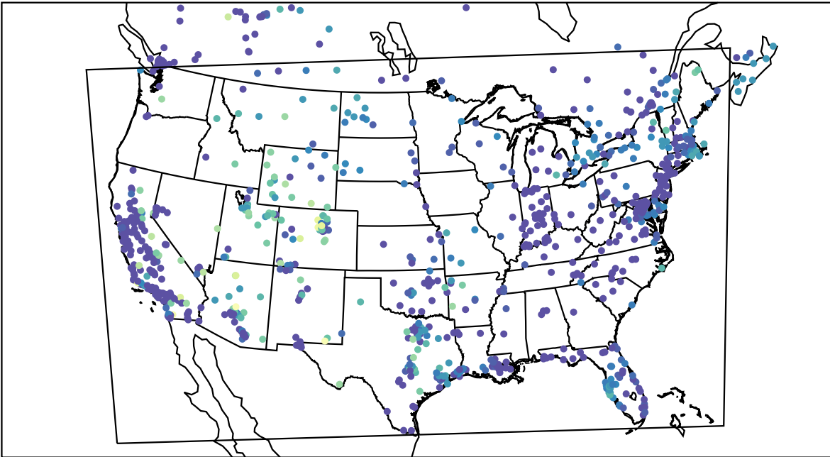
AirNOW (2020-11-12_06:00:00)
