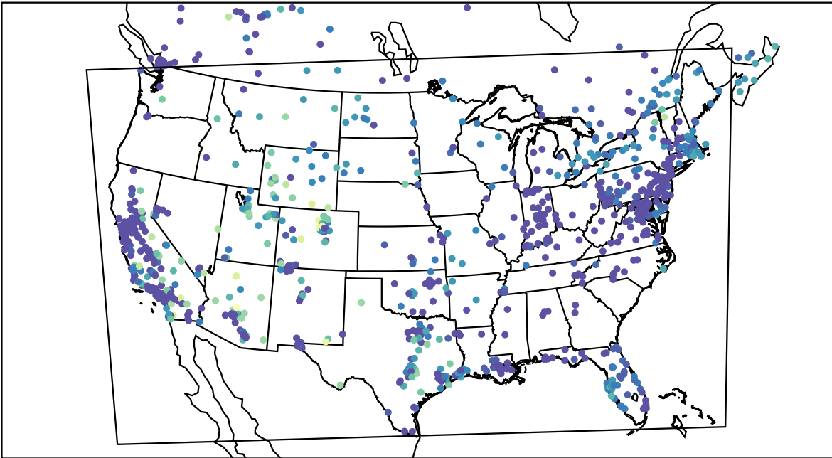
AirNOW (2020-11-12_04:00:00)
