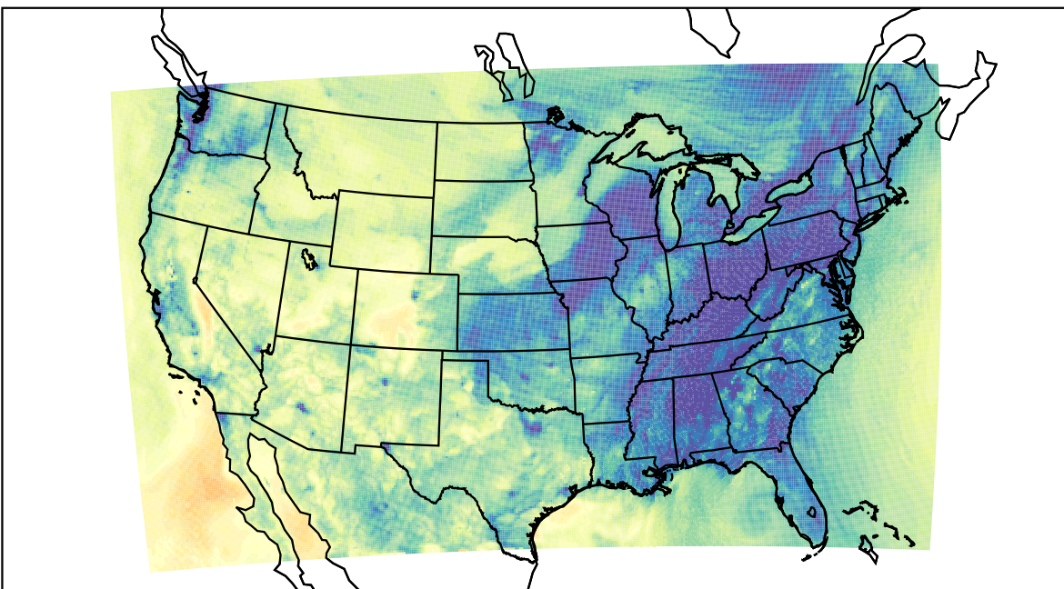
WRF (2020-11-12_02:00:00)
