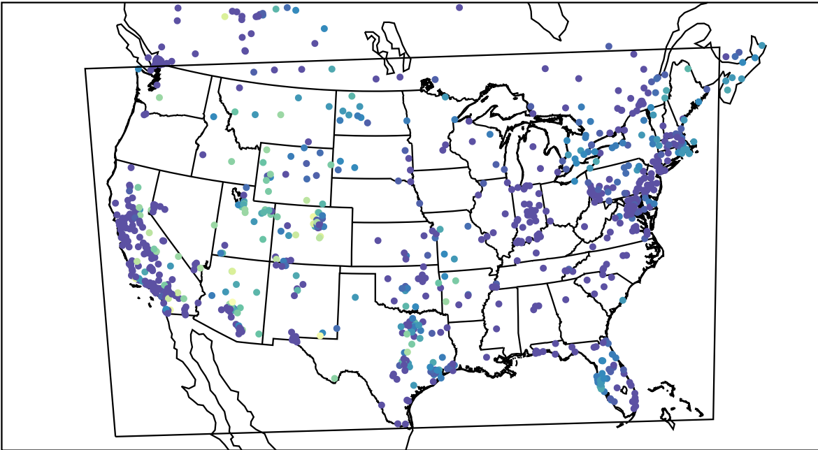
AirNOW (2020-11-12_07:00:00)
