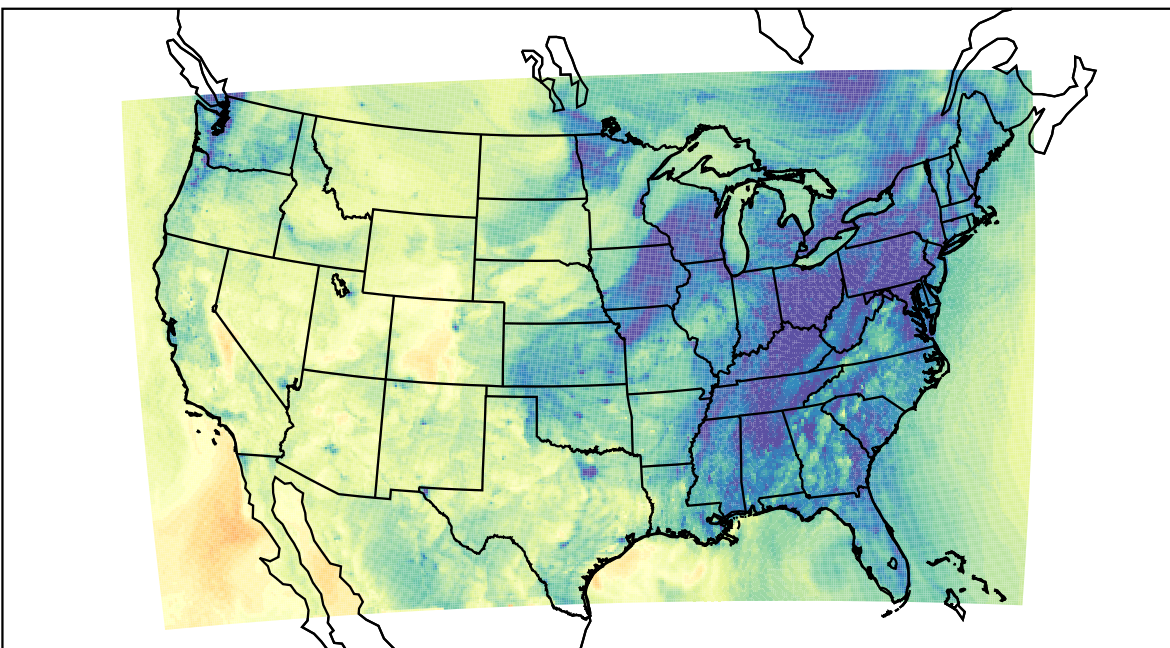
WRF (2020-11-12_00:00:00)
