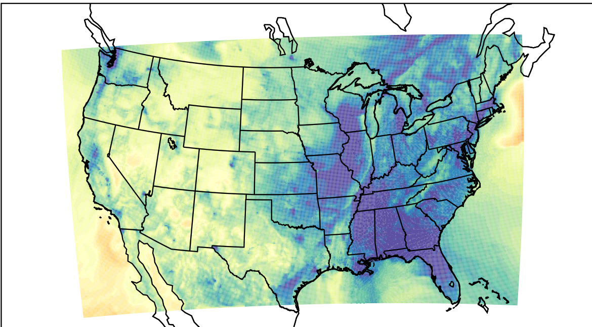
WRF (2020-11-11_02:00:00)
