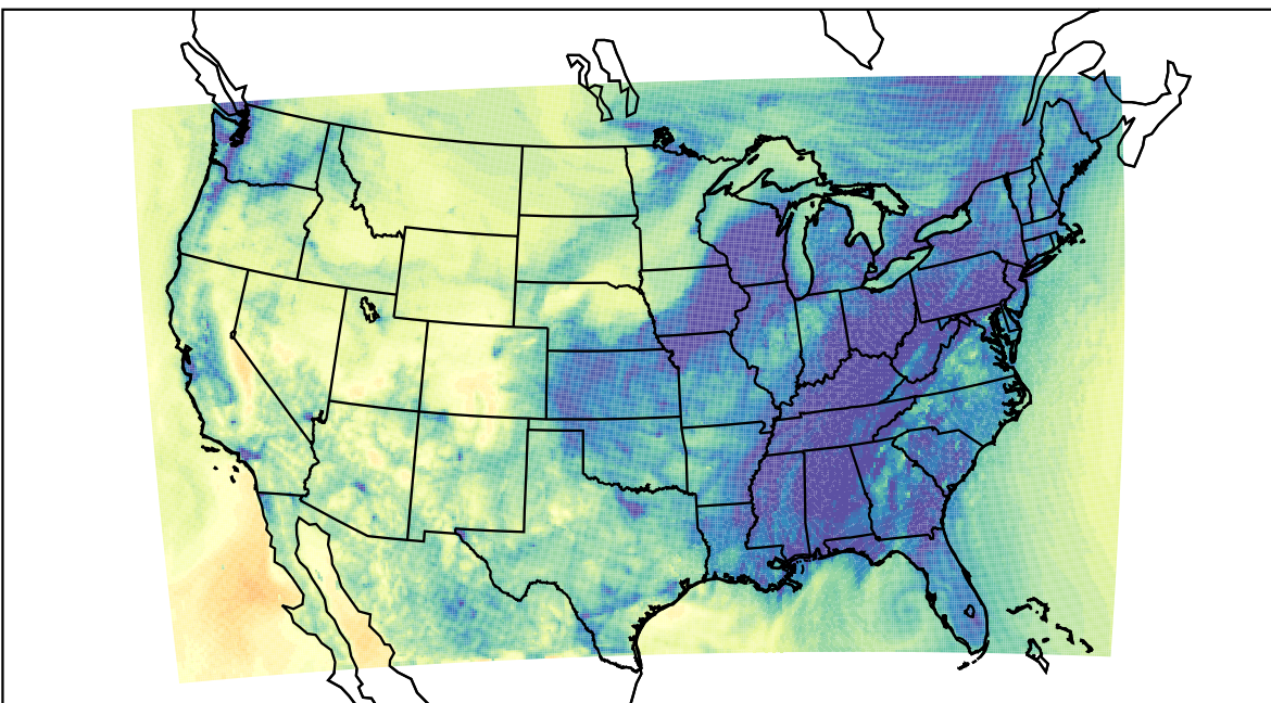
WRF (2020-11-12_04:00:00)
