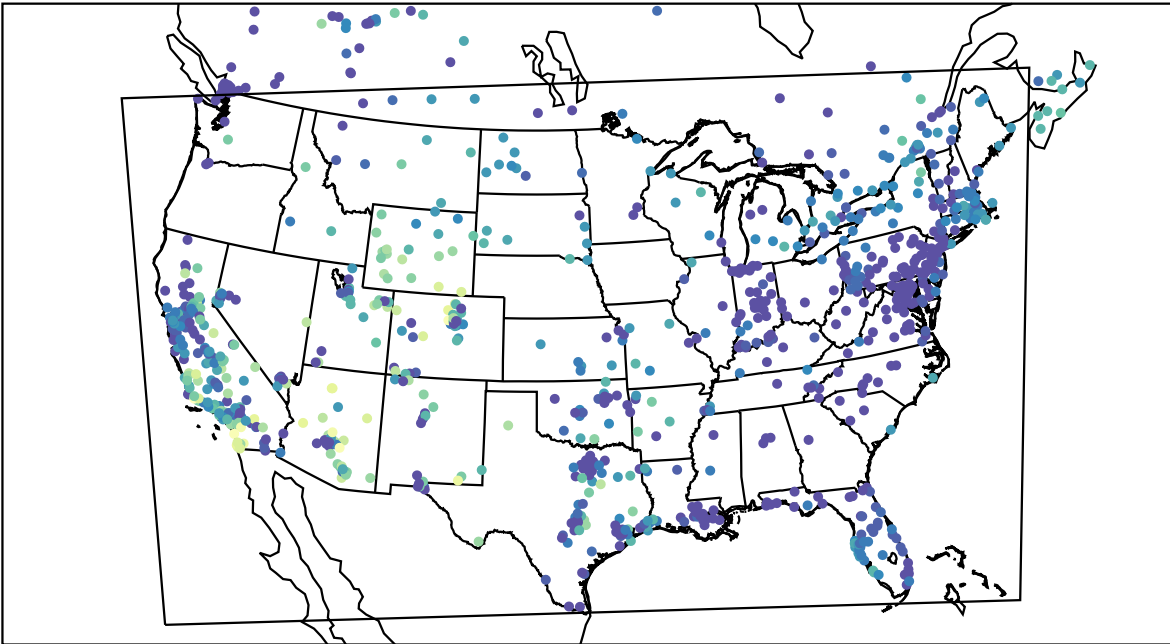
AirNOW (2020-11-12_01:00:00)
