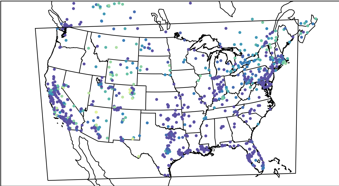
AirNOW (2020-11-11_09:00:00)
