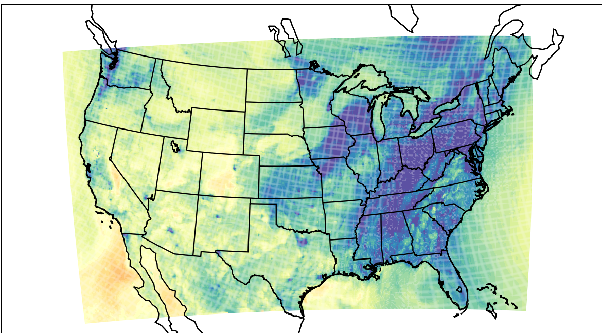
WRF (2020-11-12_01:00:00)
