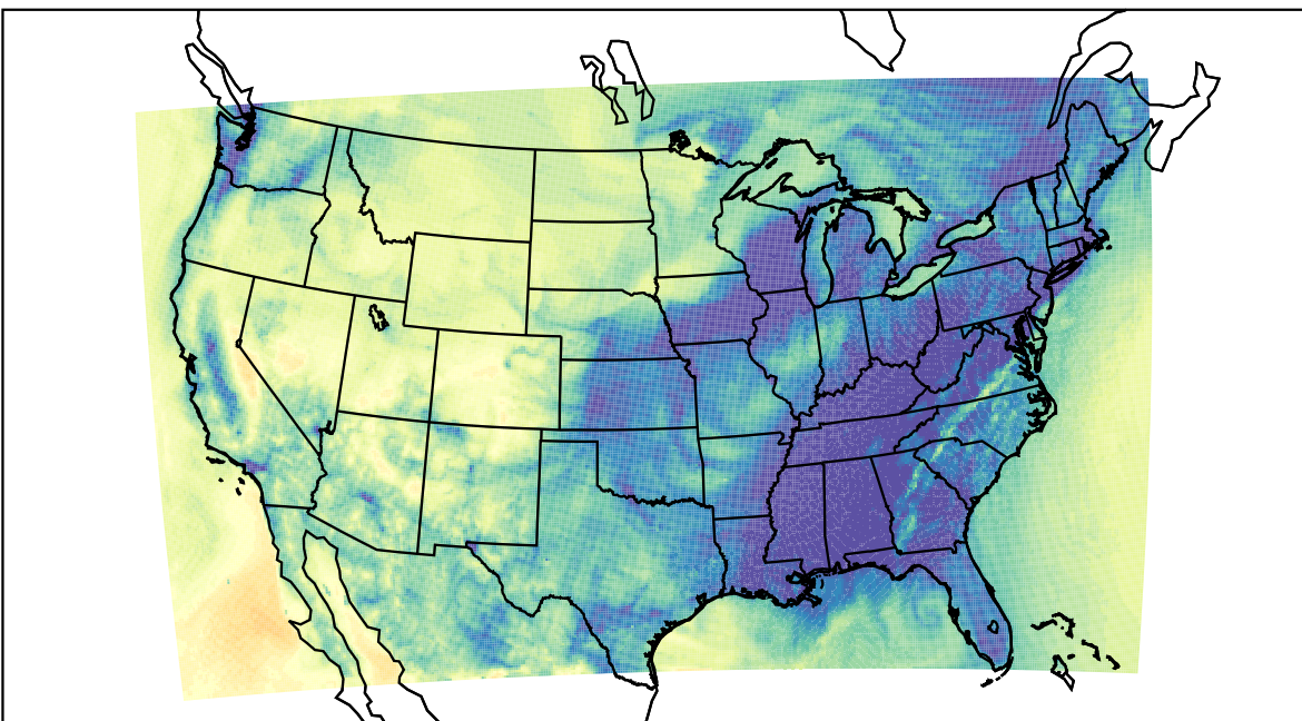
WRF (2020-11-12_09:00:00)
