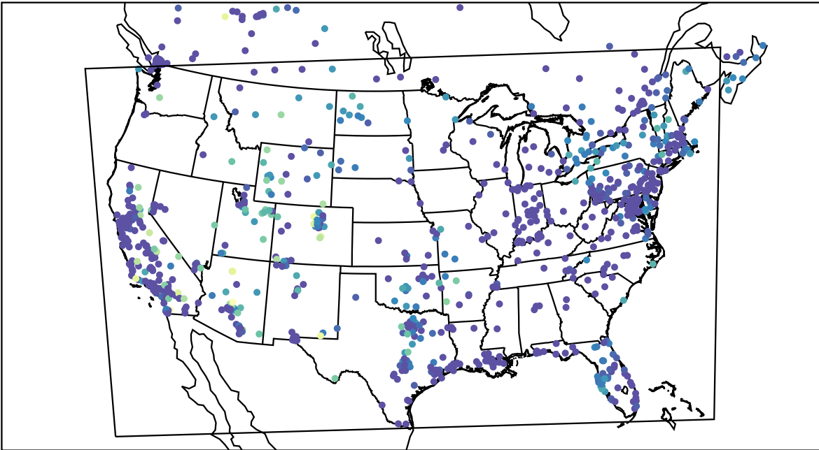
AirNOW (2020-11-12_09:00:00)
