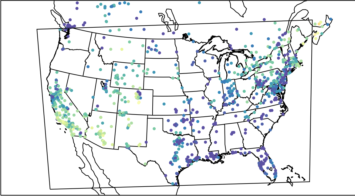
AirNOW (2020-11-11_00:00:00)
