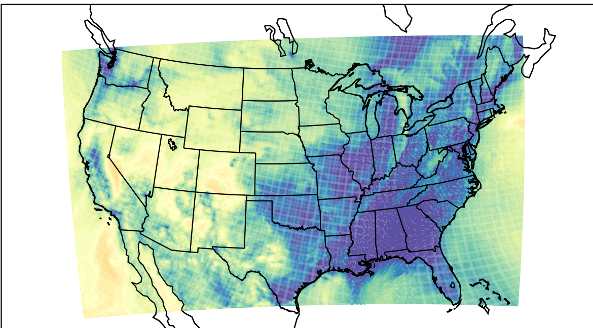
WRF (2020-11-11_09:00:00)
