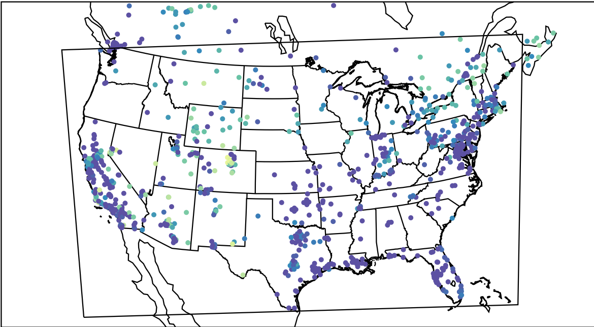
AirNOW (2020-11-11_07:00:00)
