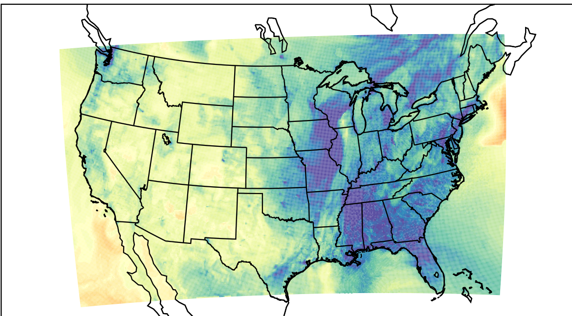
WRF (2020-11-11_00:00:00)
