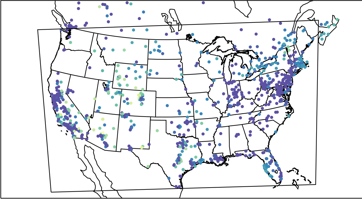
AirNOW (2020-11-12_03:00:00)
