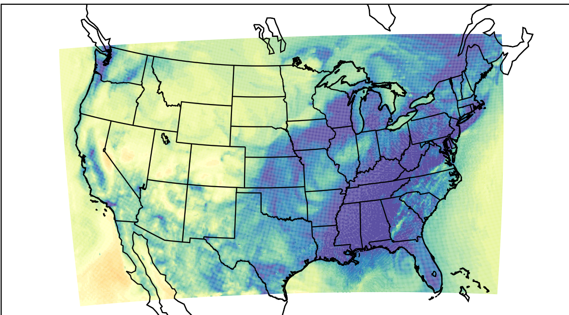
WRF (2020-11-12_11:00:00)
