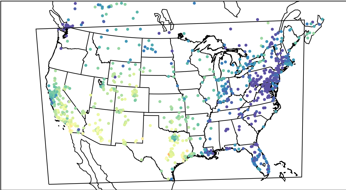
AirNOW (2020-11-11_21:00:00)
