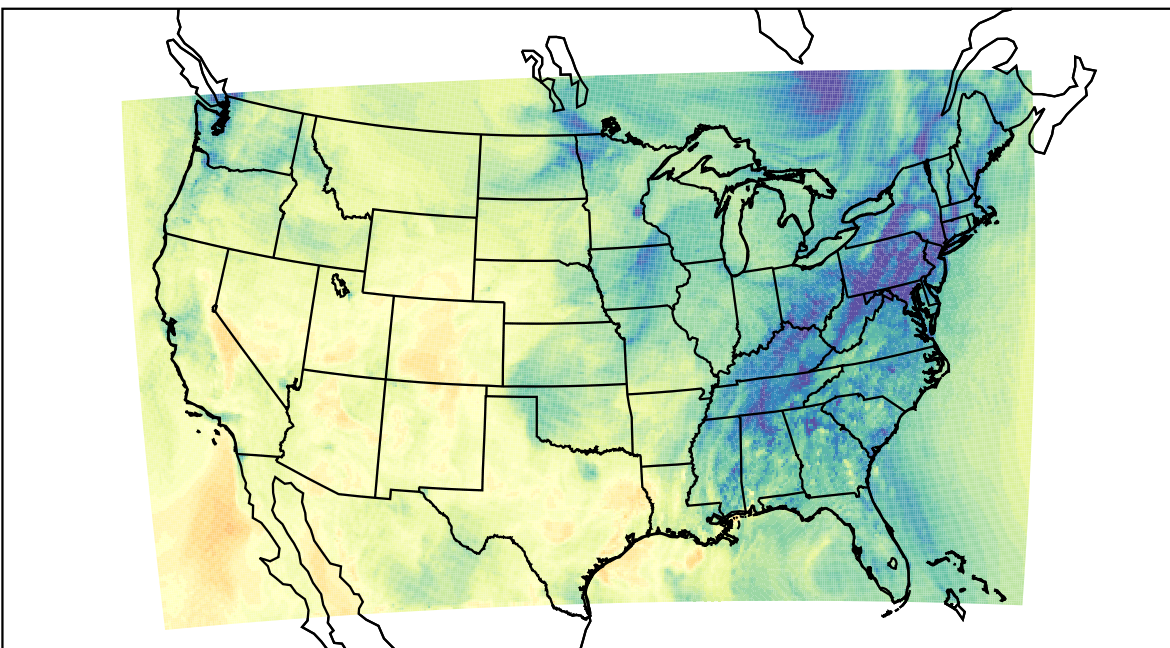
WRF (2020-11-11_21:00:00)
