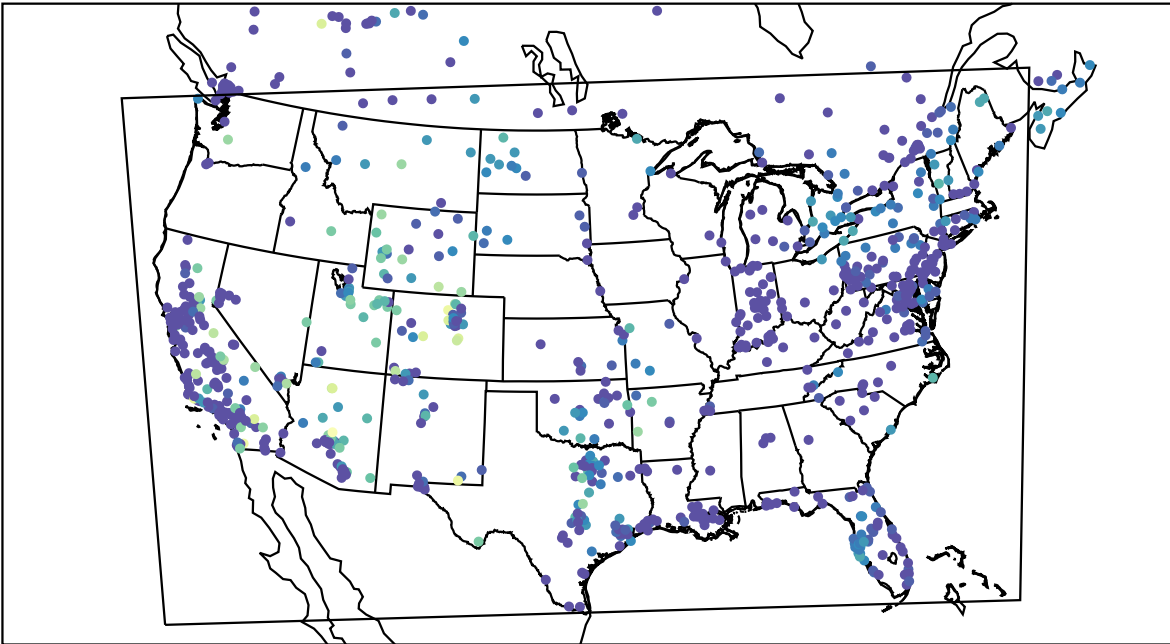
AirNOW (2020-11-12_08:00:00)
