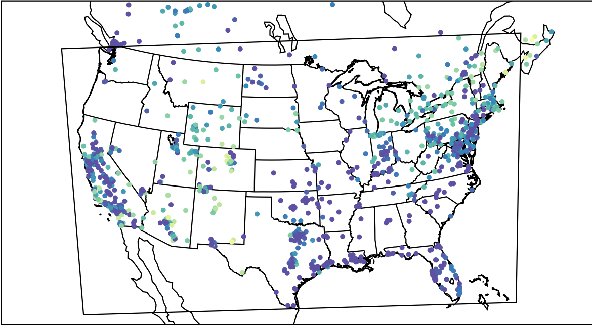
AirNOW (2020-11-11_02:00:00)
