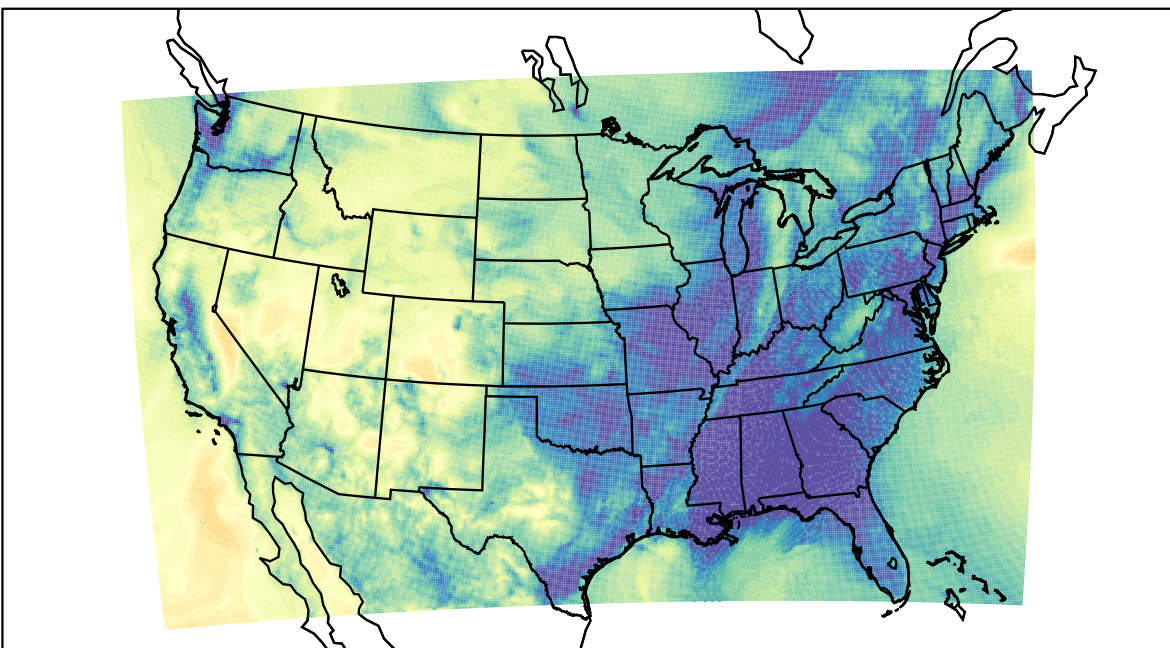
WRF (2020-11-11_07:00:00)
