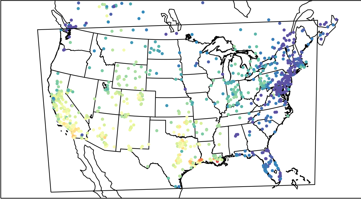
AirNOW (2020-11-12_21:00:00)
