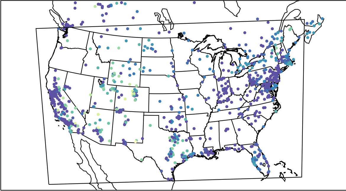
AirNOW (2020-11-12_05:00:00)
