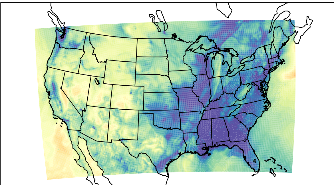
WRF (2020-11-11_05:00:00)
