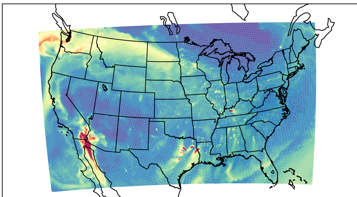
WRF 2020-11-16_14:00:00
