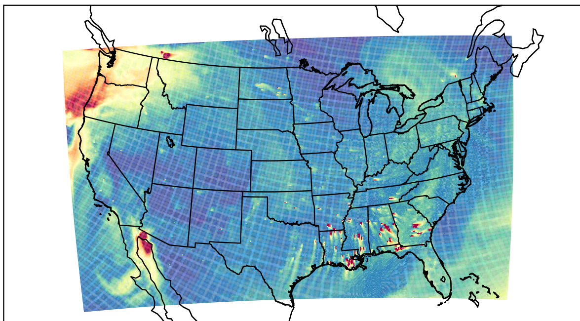
WRF 2020-11-15_23:00:00
