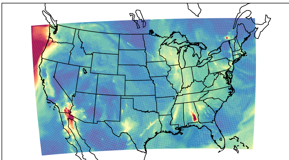
WRF 2020-11-15_09:00:00
