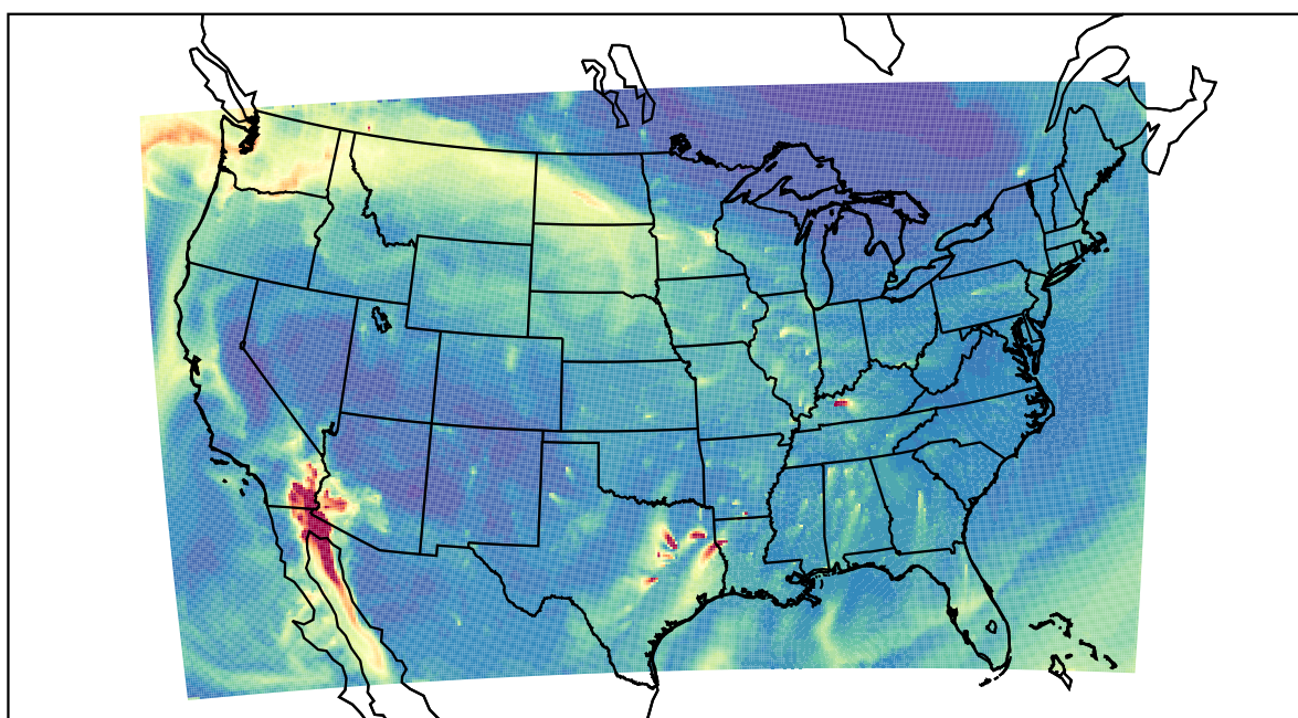
WRF 2020-11-16_15:00:00
