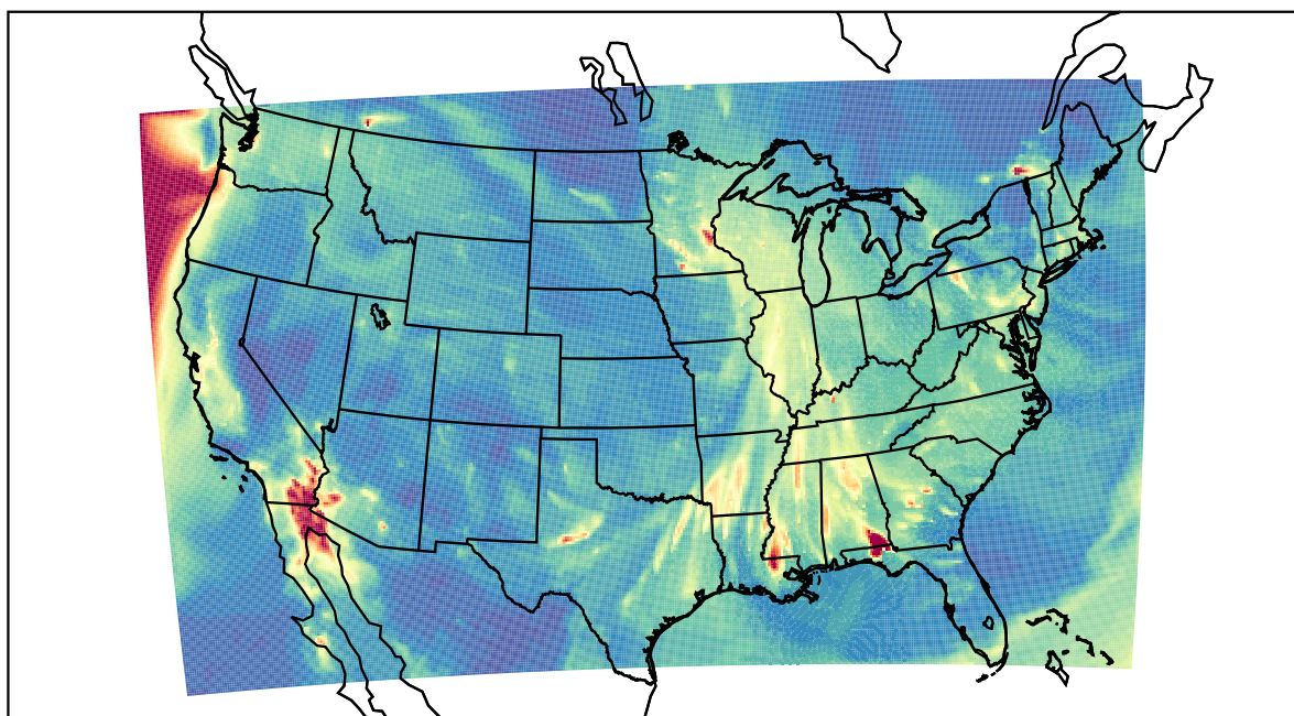
WRF 2020-11-15_05:00:00
