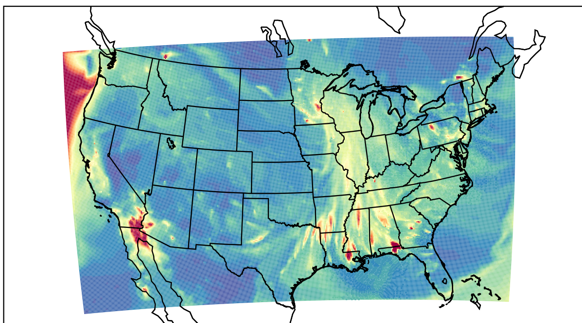
WRF 2020-11-15_04:00:00
