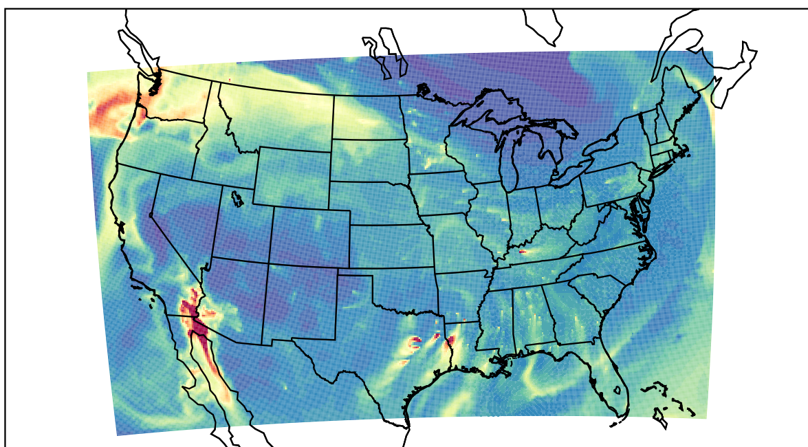
WRF 2020-11-16_11:00:00
