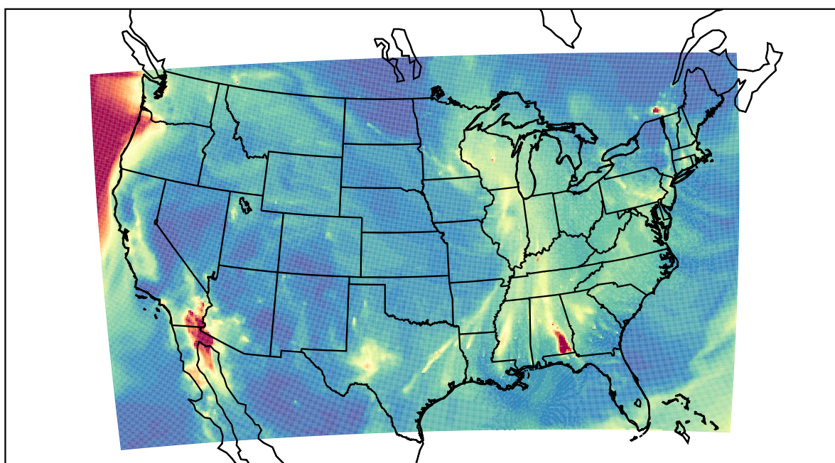
WRF 2020-11-15_08:00:00
