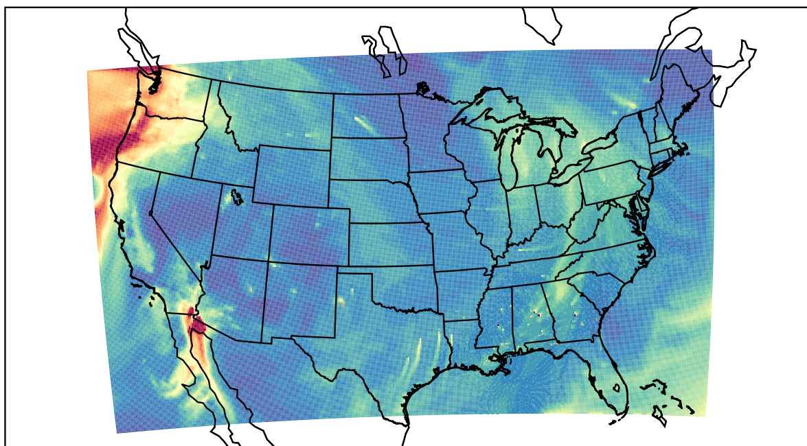
WRF 2020-11-15_17:00:00
