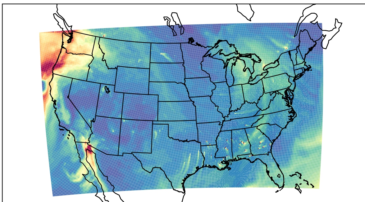
WRF 2020-11-15_19:00:00
