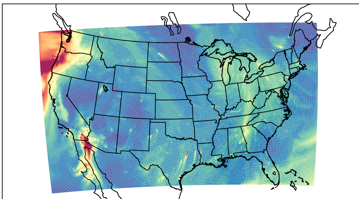
WRF 2020-11-15_15:00:00
