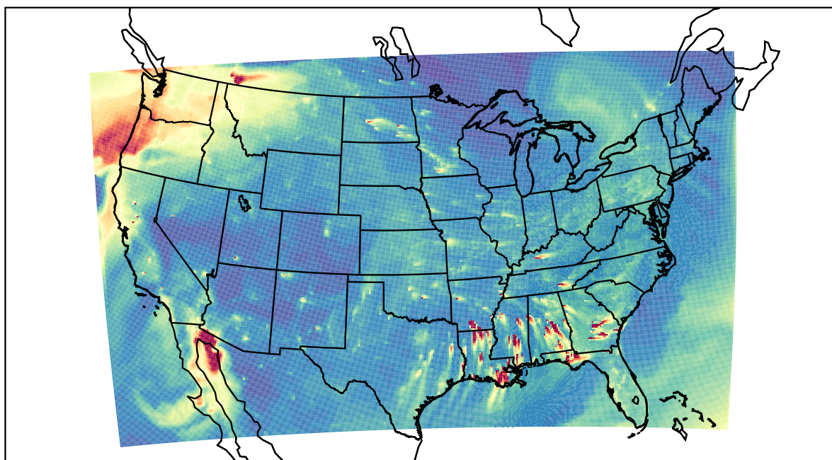
WRF 2020-11-16_01:00:00
