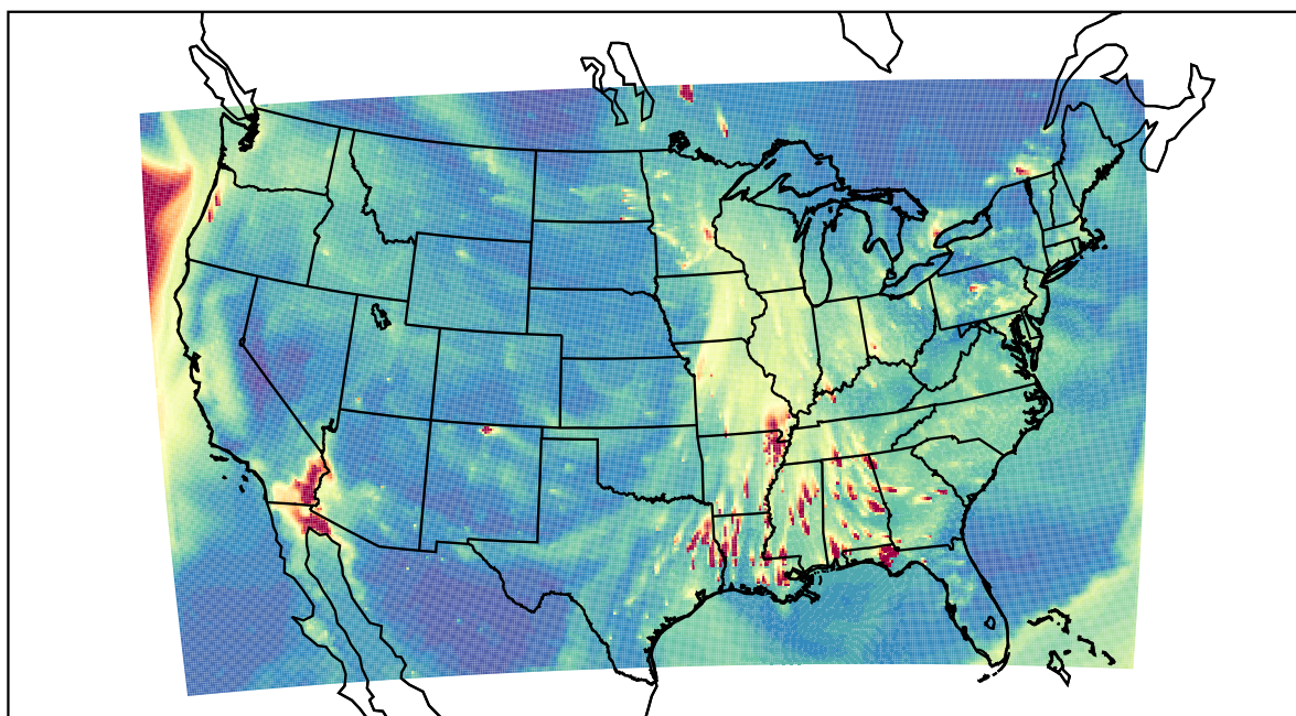
WRF 2020-11-15_00:00:00
