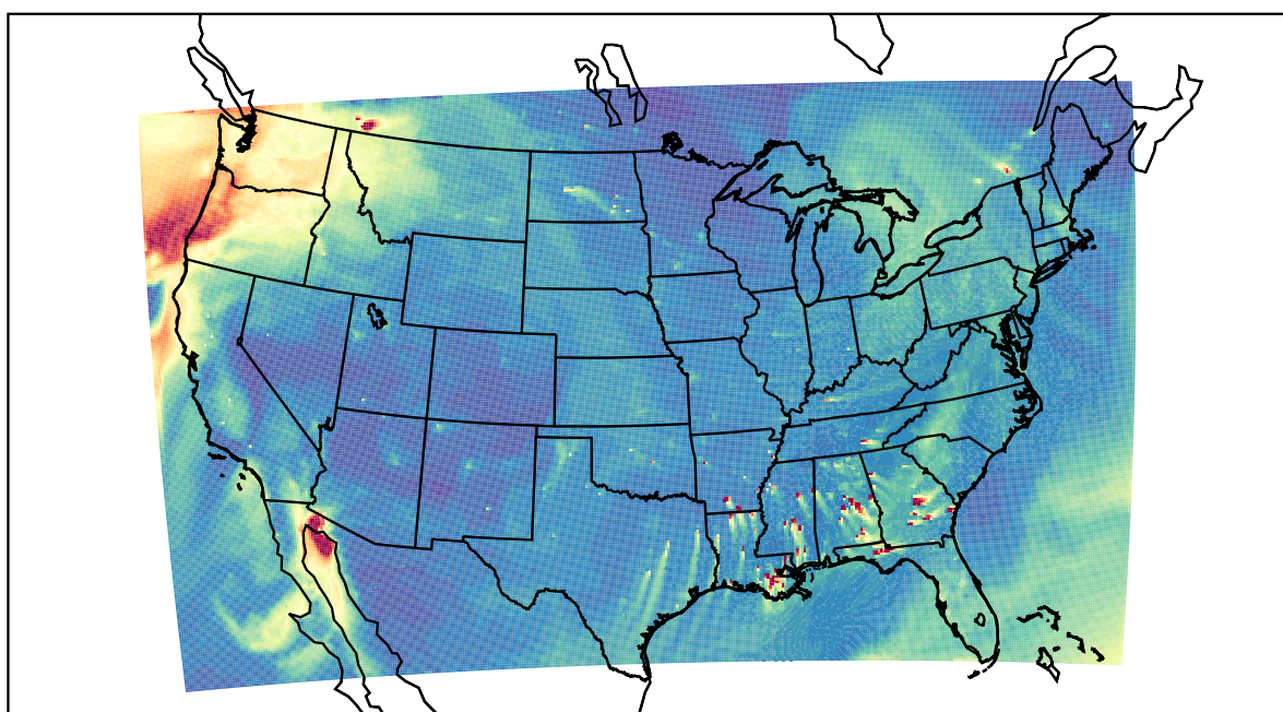
WRF 2020-11-15_22:00:00
