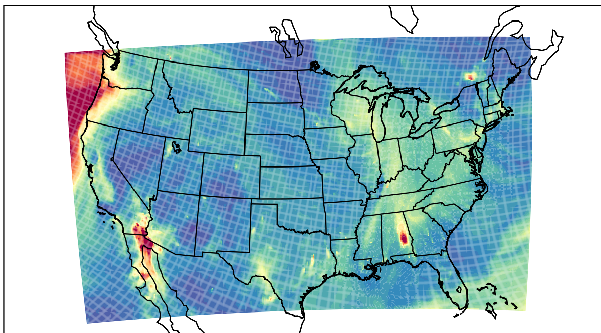
WRF 2020-11-15_11:00:00
