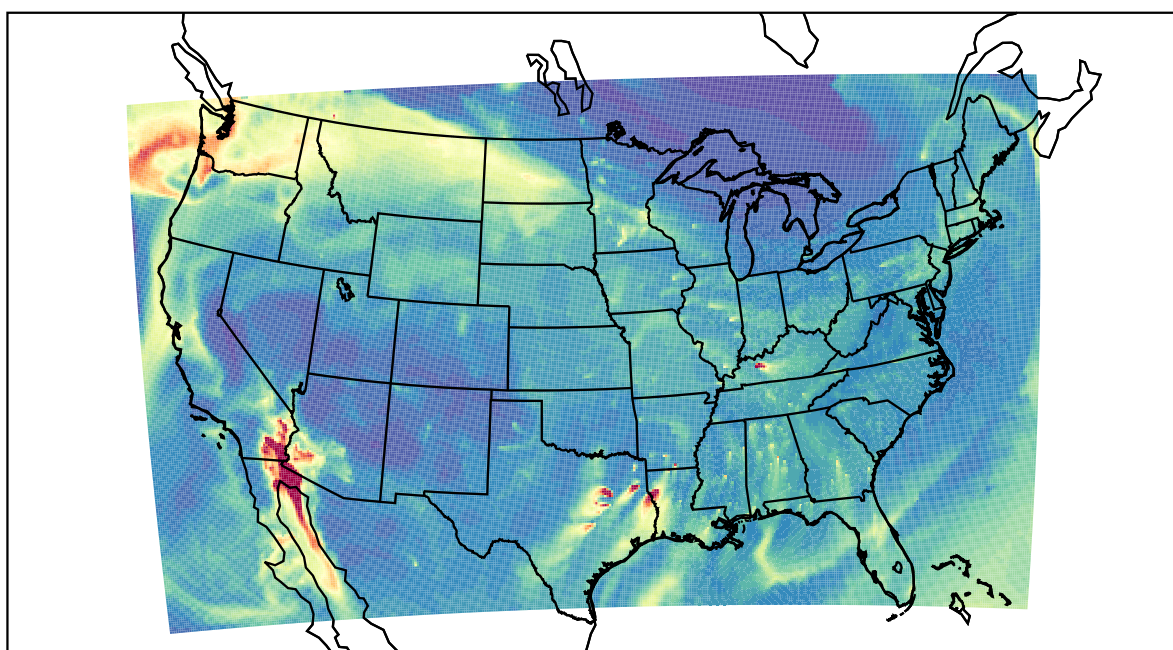
WRF 2020-11-16_12:00:00
