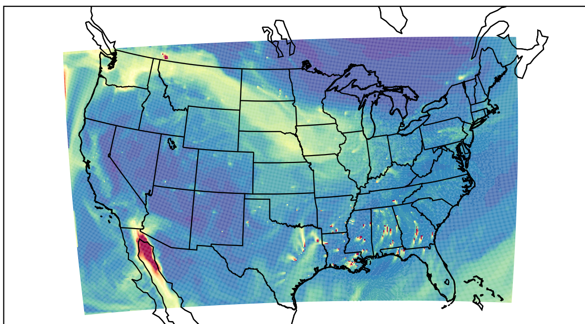
WRF 2020-11-16_21:00:00
