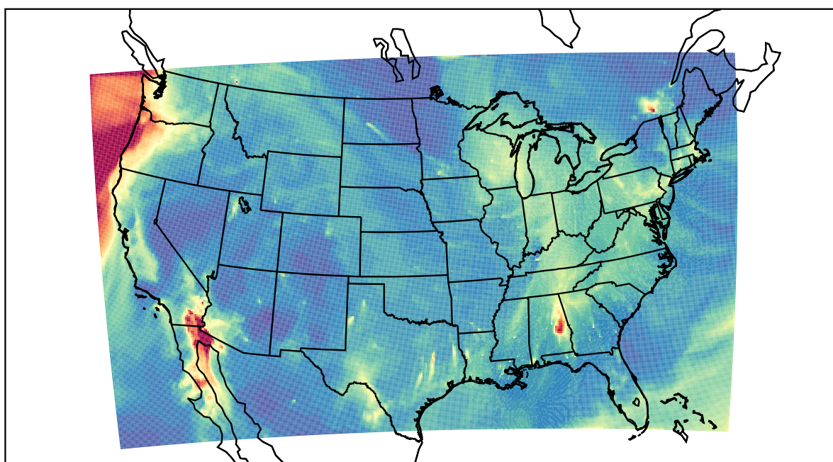
WRF 2020-11-15_12:00:00
