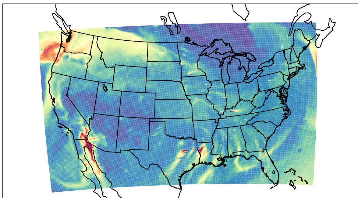
WRF 2020-11-16_09:00:00
