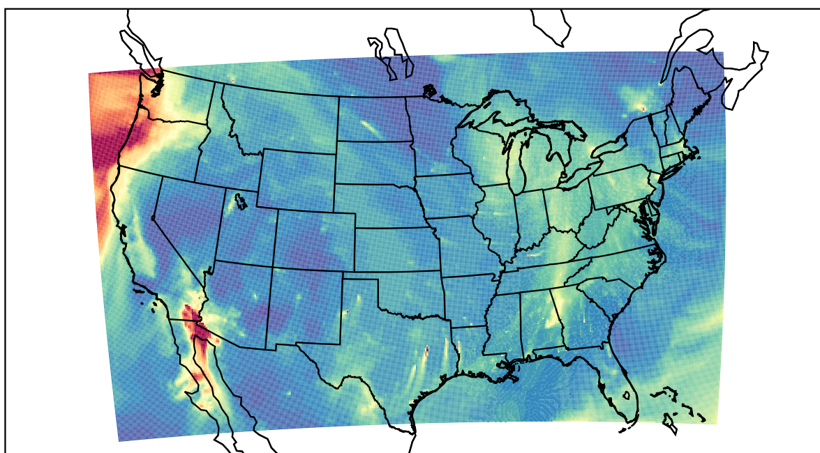
WRF 2020-11-15_14:00:00
