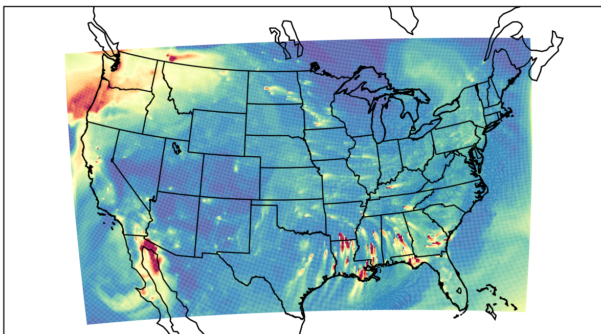
WRF 2020-11-16_02:00:00
