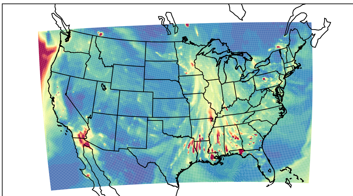
WRF 2020-11-15_02:00:00
