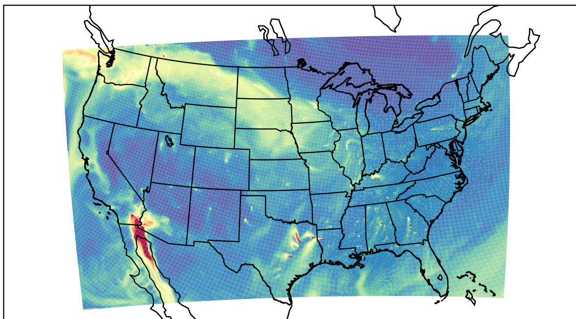
WRF 2020-11-16_17:00:00
