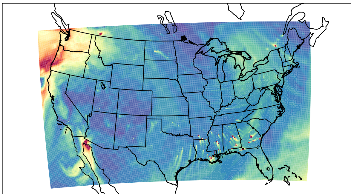
WRF 2020-11-15_21:00:00
