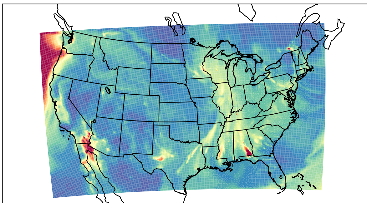
WRF 2020-11-15_07:00:00
