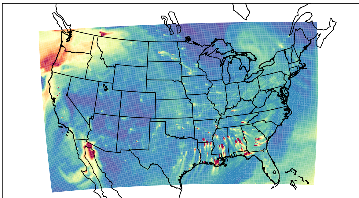
WRF 2020-11-16_00:00:00
