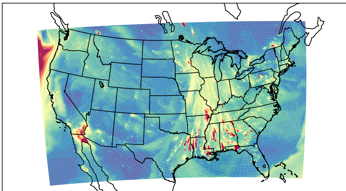
WRF 2020-11-15_01:00:00
