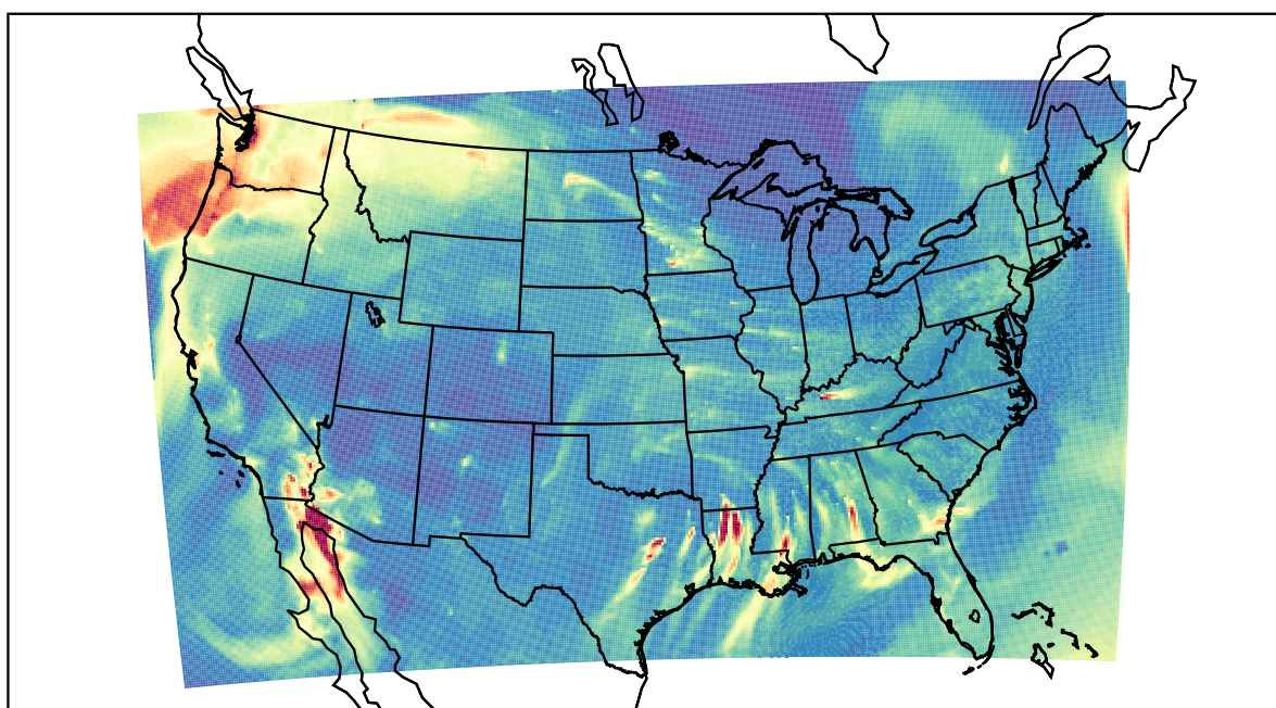
WRF 2020-11-16_05:00:00
