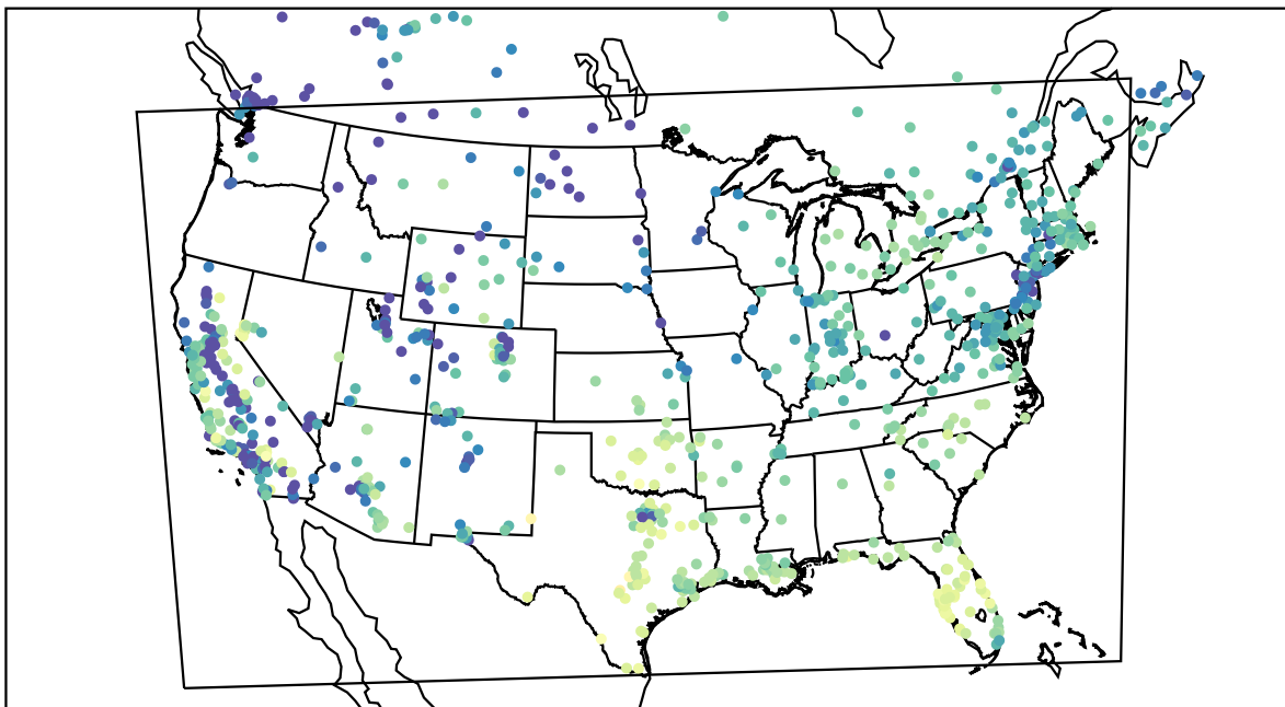
AirNOW (2020-11-17_17:00:00)
