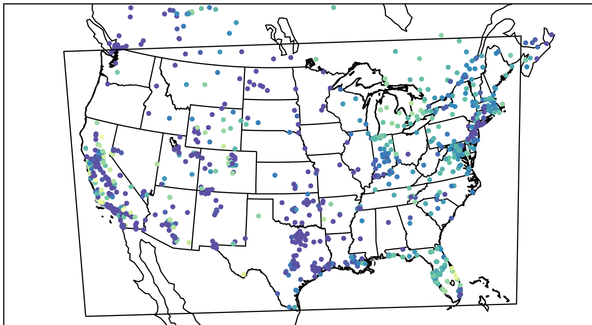
AirNOW (2020-11-17_14:00:00)
