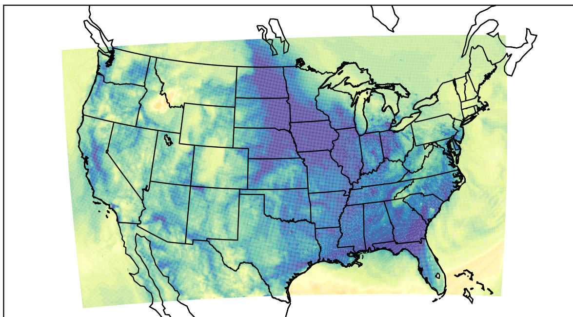
WRF (2020-11-18_12:00:00)
