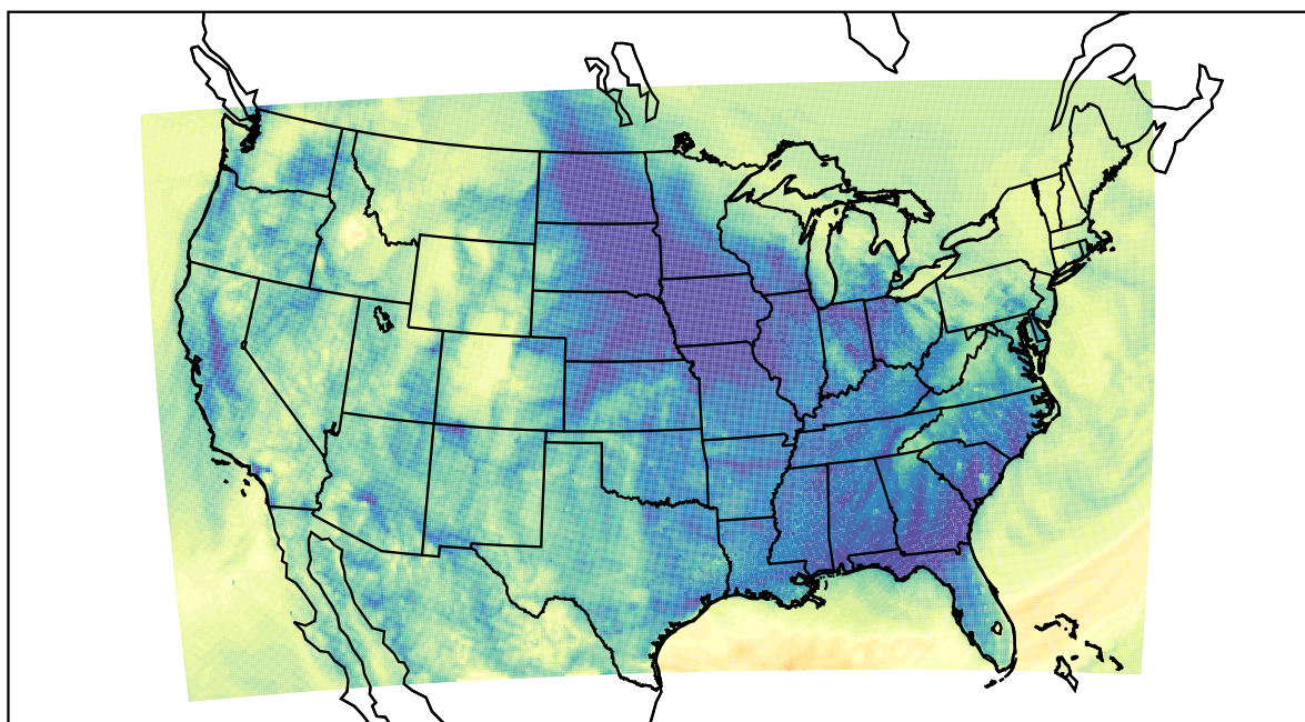
WRF (2020-11-18_09:00:00)
