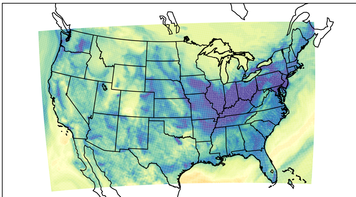
WRF (2020-11-17_09:00:00)
