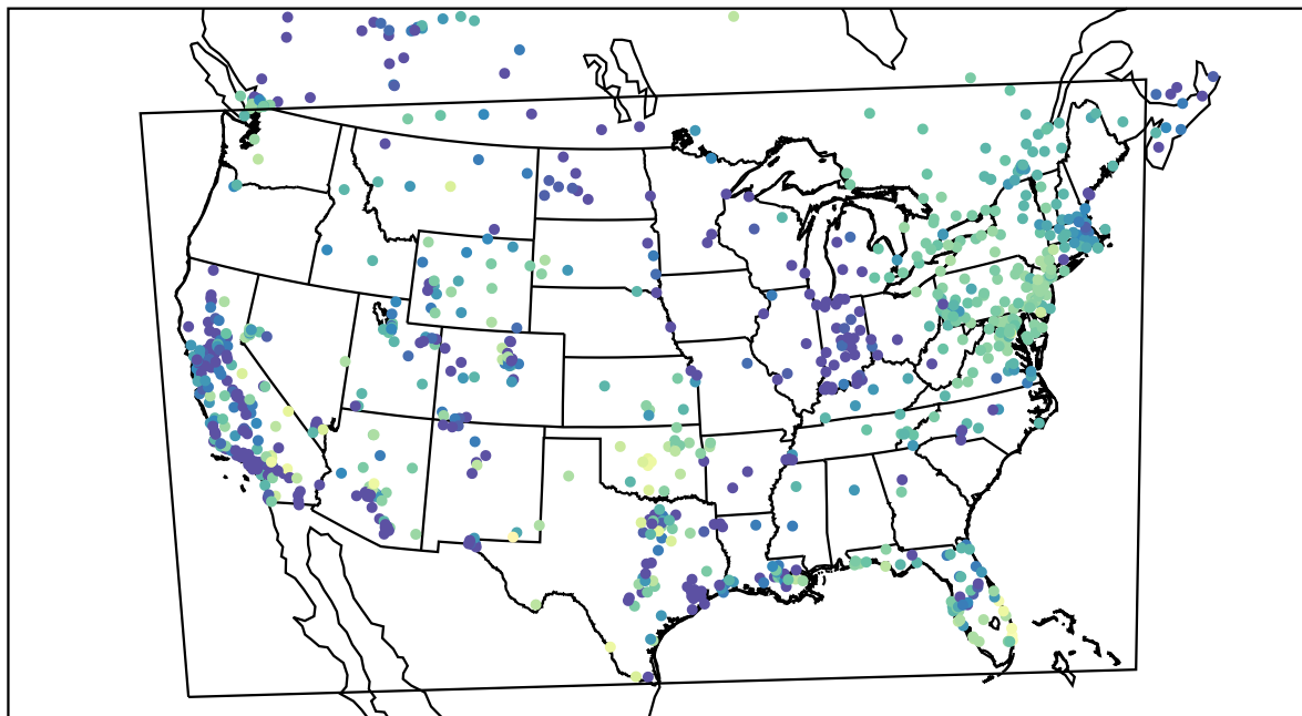
AirNOW (2020-11-18_04:00:00)
