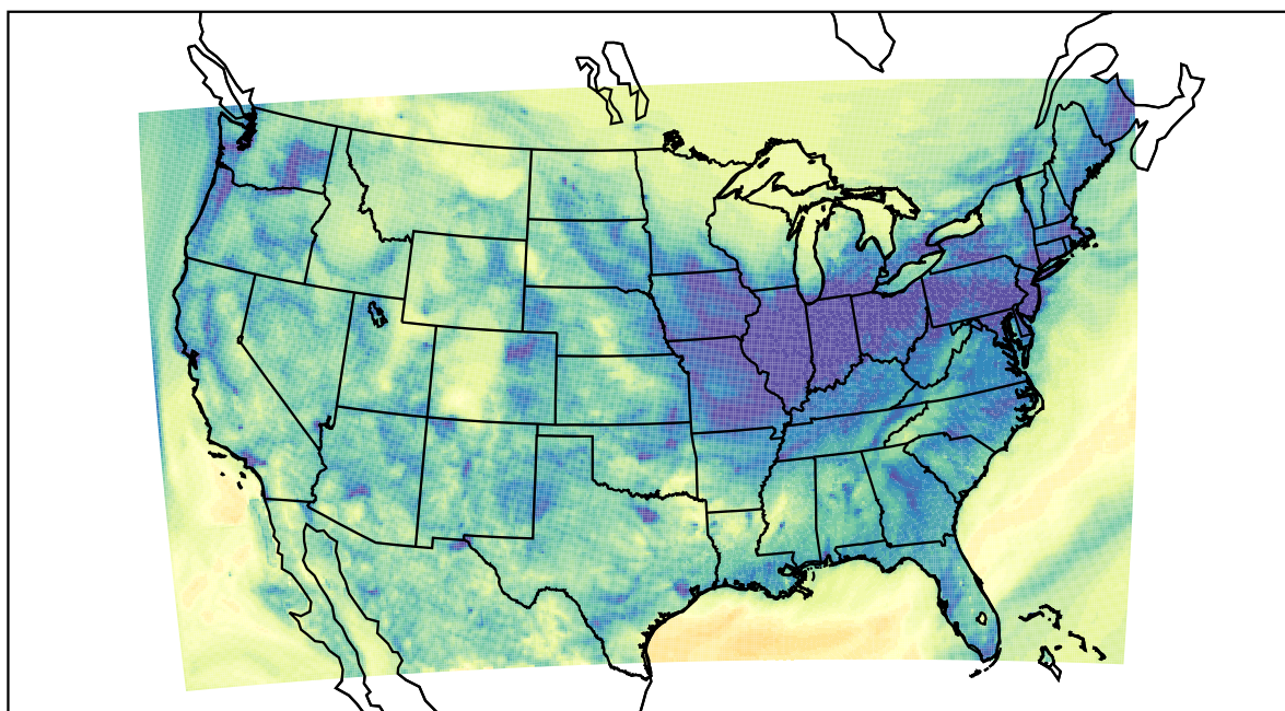
WRF (2020-11-17_05:00:00)
