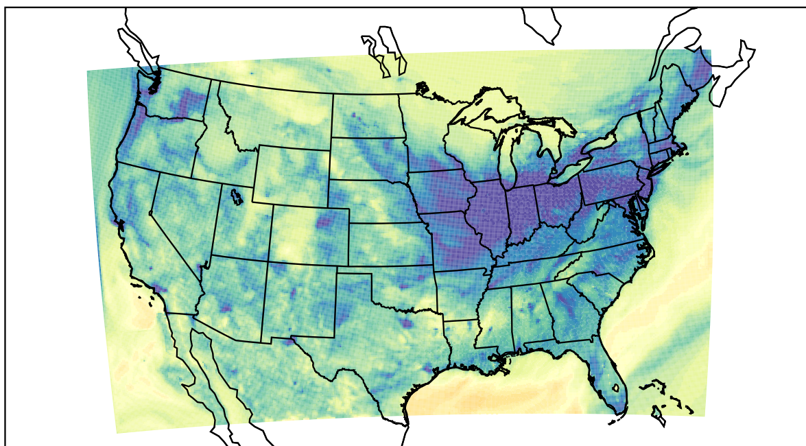
WRF (2020-11-17_04:00:00)
