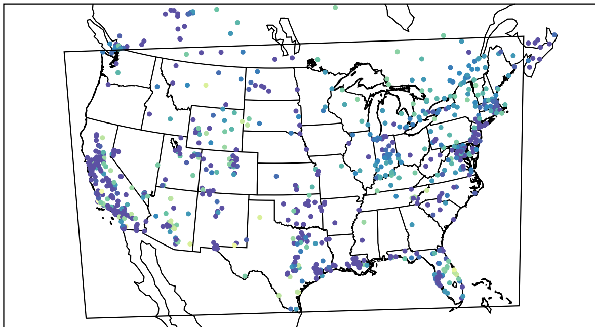
AirNOW (2020-11-17_05:00:00)
