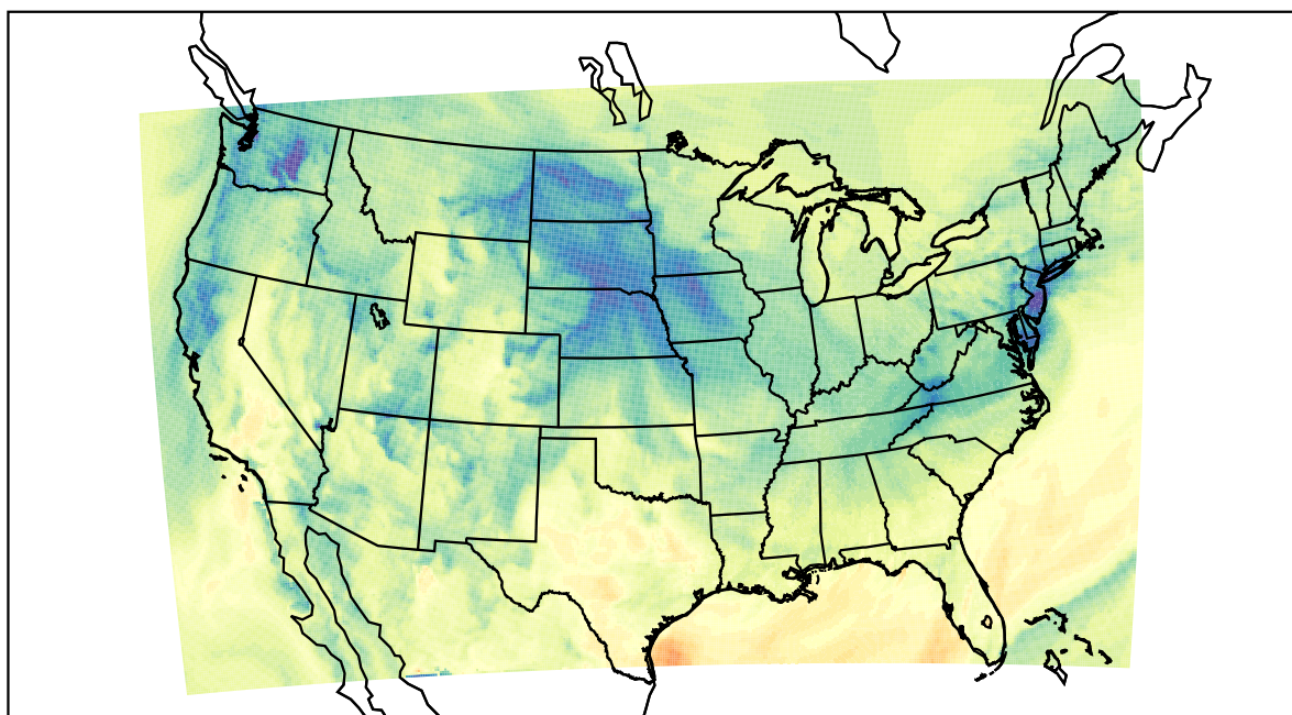
WRF (2020-11-17_19:00:00)
