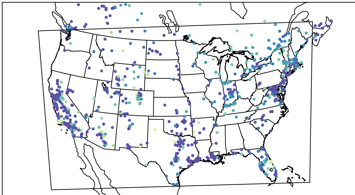
AirNOW (2020-11-17_07:00:00)
