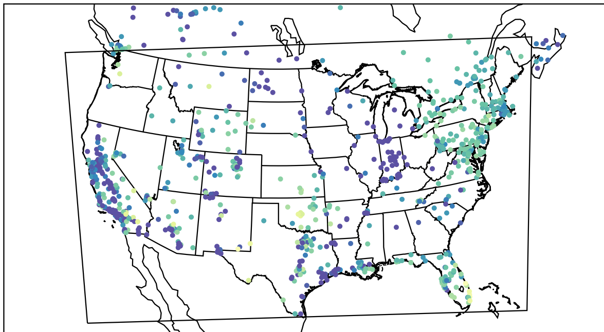
AirNOW (2020-11-18_07:00:00)
