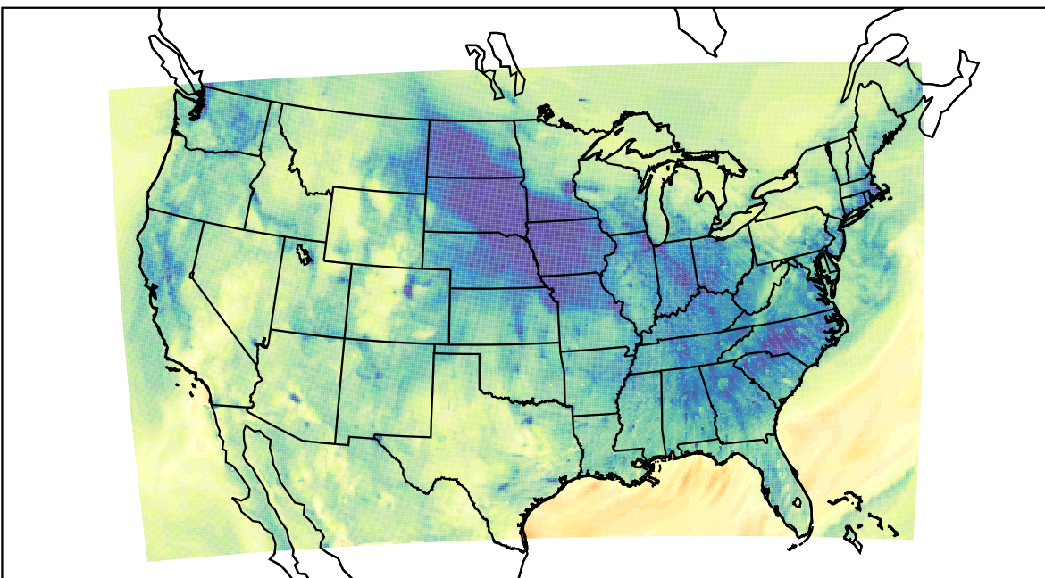
WRF (2020-11-18_00:00:00)
