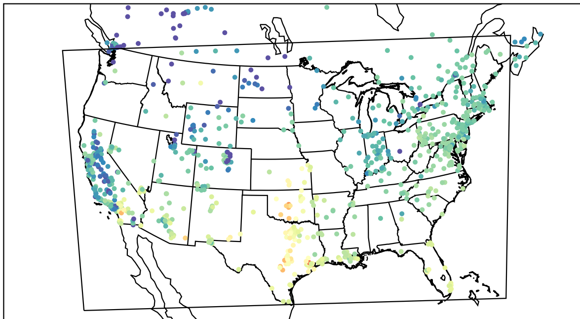
AirNOW (2020-11-18_19:00:00)
