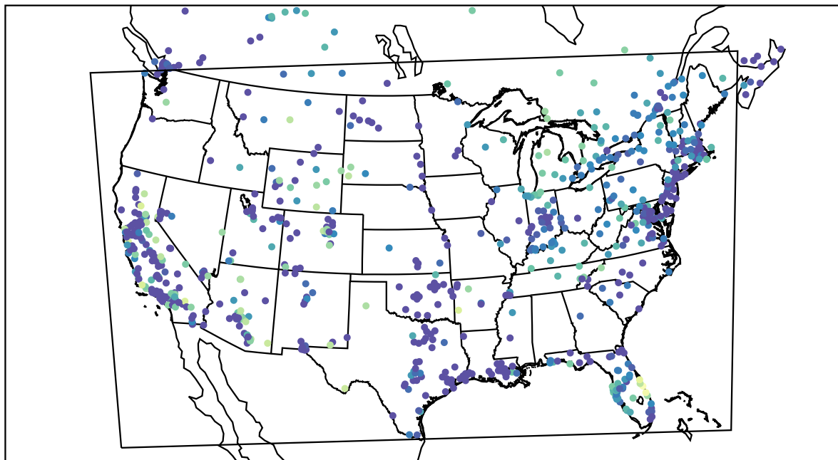
AirNOW (2020-11-17_10:00:00)
