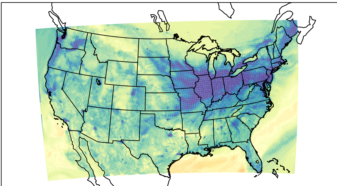
WRF (2020-11-17_02:00:00)
