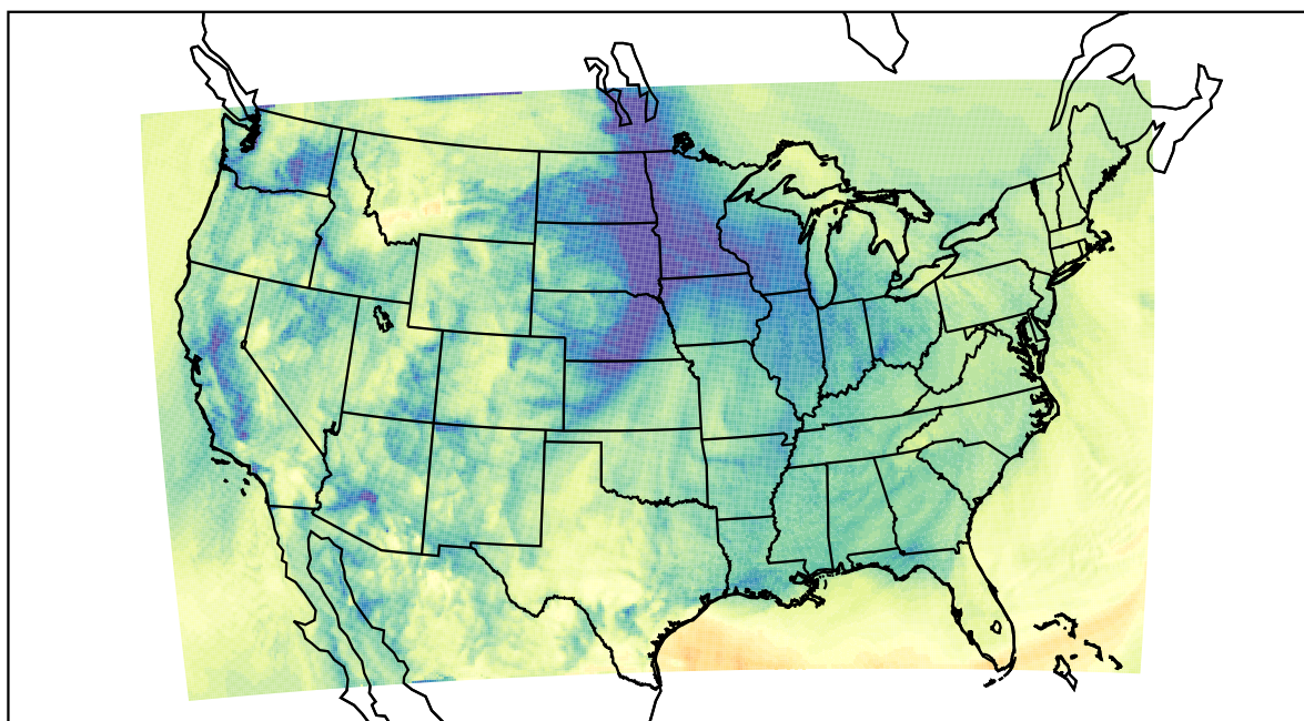
WRF (2020-11-18_17:00:00)
