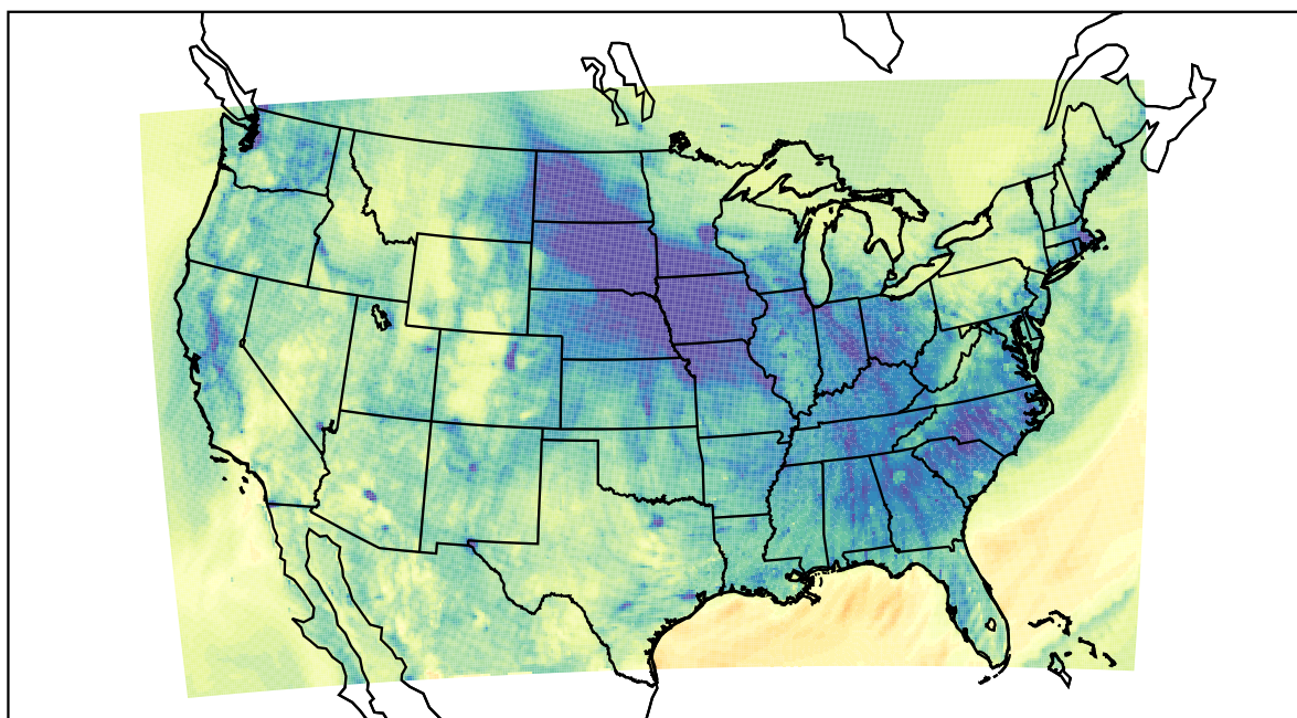
WRF (2020-11-18_01:00:00)
