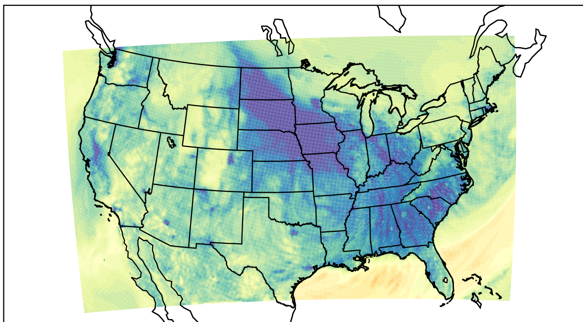
WRF (2020-11-18_03:00:00)
