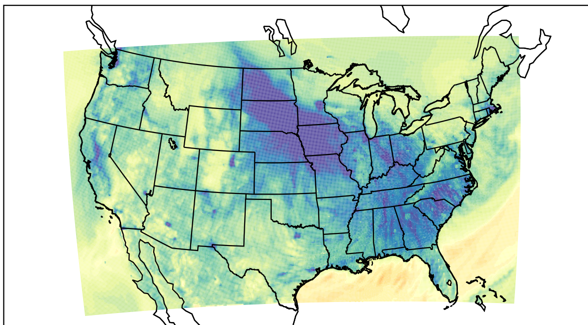
WRF (2020-11-18_02:00:00)
