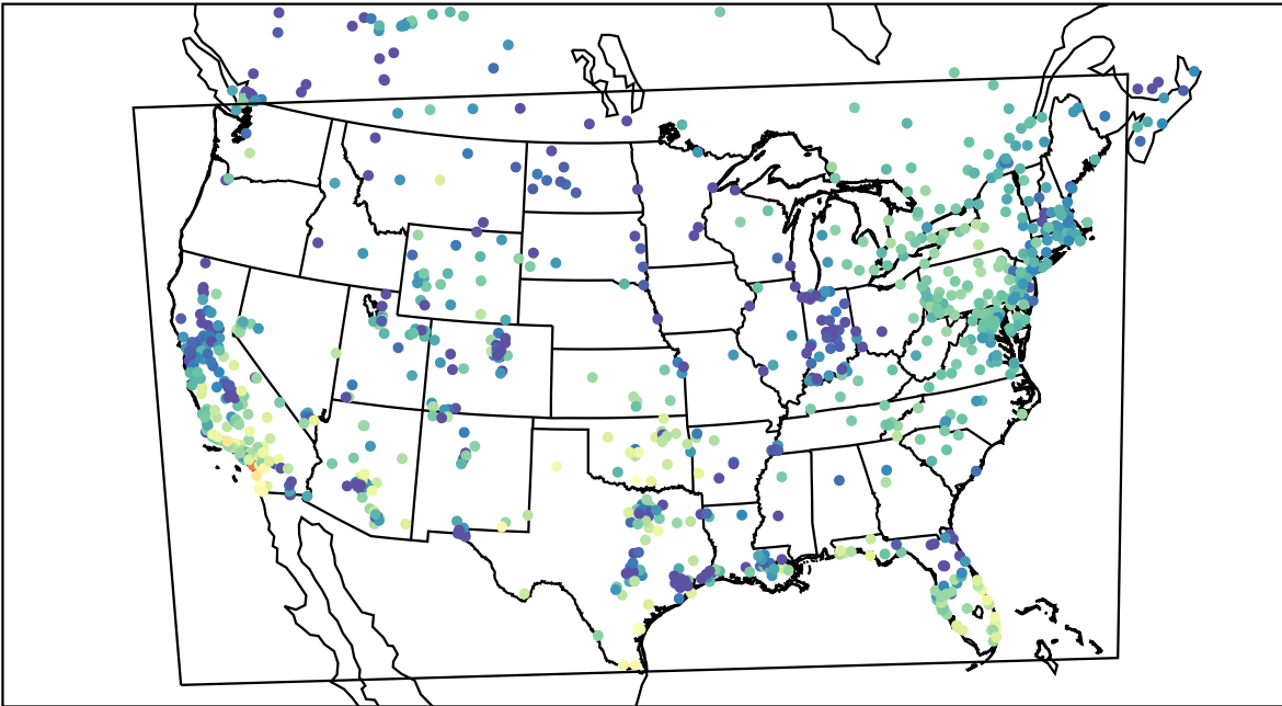
AirNOW (2020-11-18_00:00:00)
