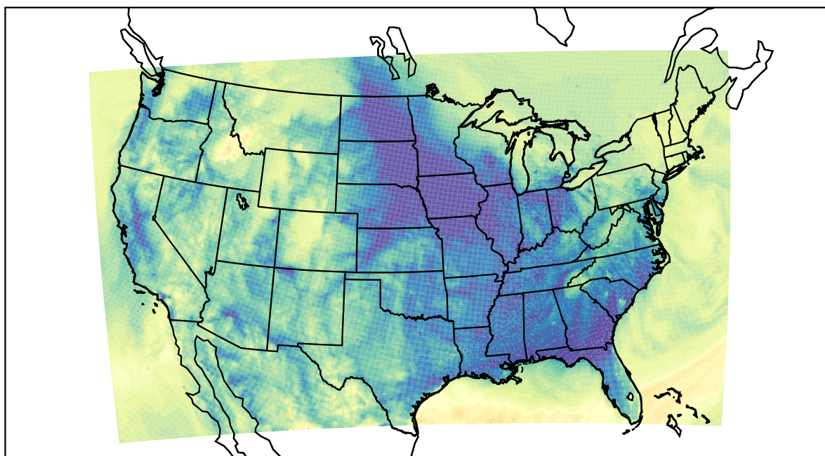
WRF (2020-11-18_11:00:00)
