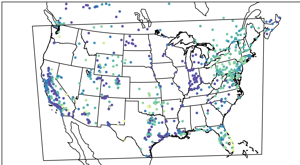
AirNOW (2020-11-18_08:00:00)
