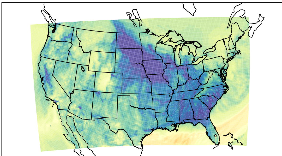
WRF (2020-11-18_06:00:00)
