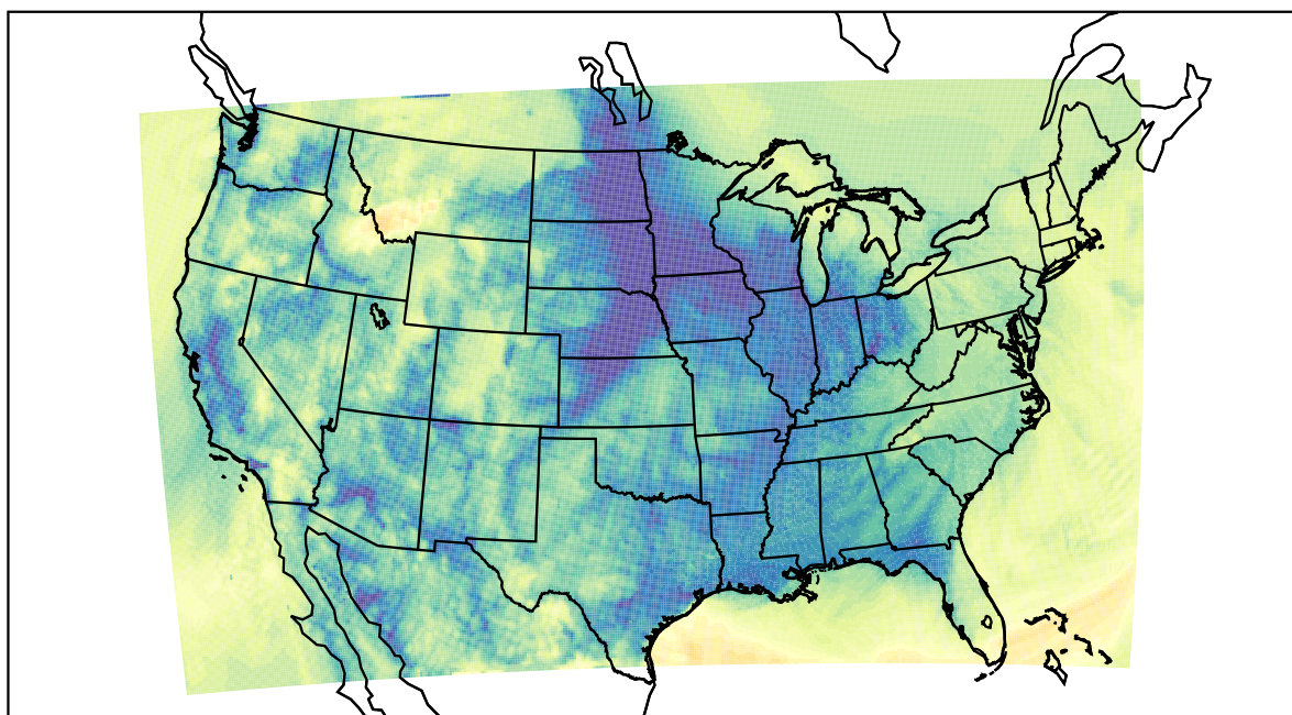
WRF (2020-11-18_15:00:00)
