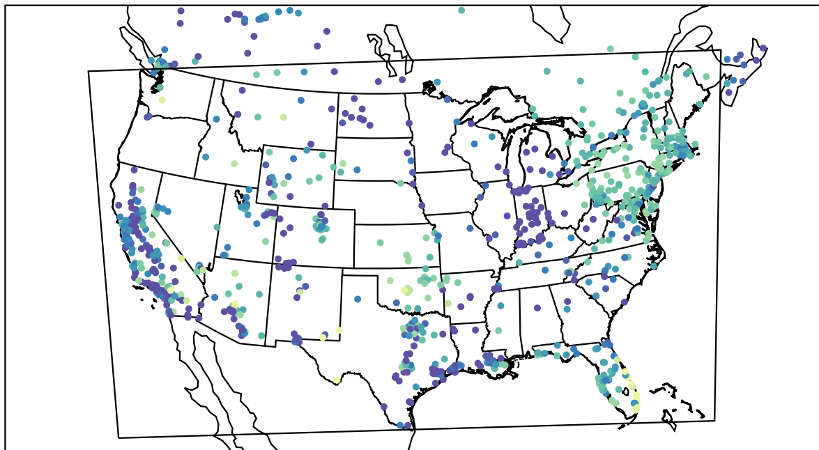
AirNOW (2020-11-18_09:00:00)
