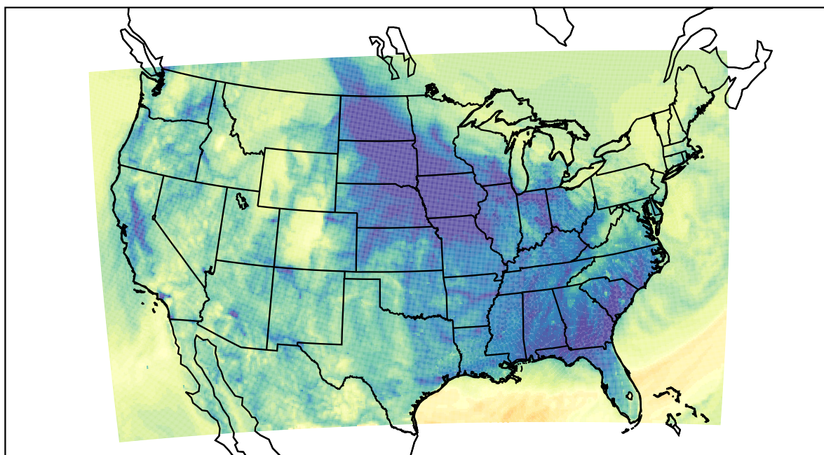
WRF (2020-11-18_07:00:00)
