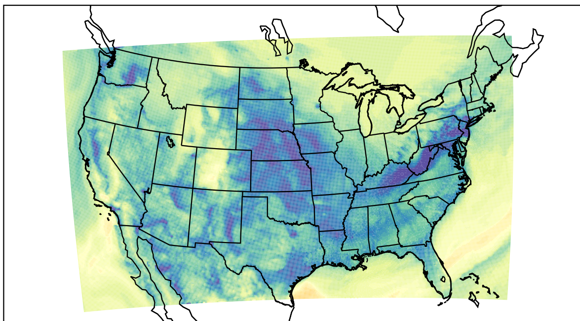
WRF (2020-11-17_15:00:00)
