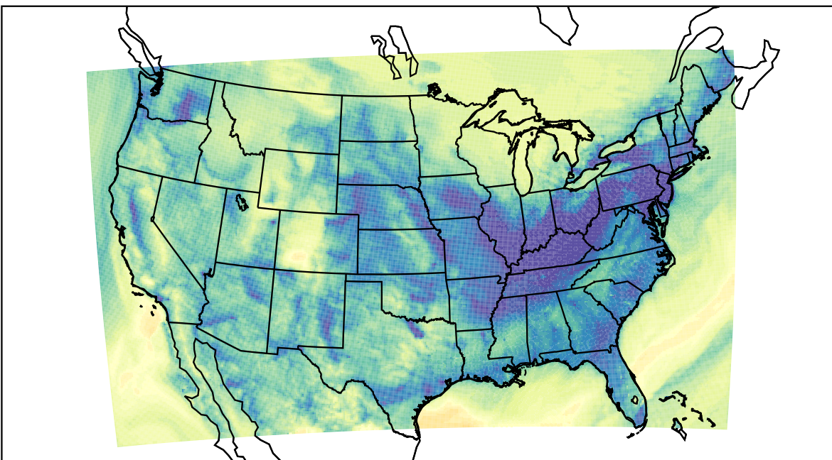
WRF (2020-11-17_11:00:00)
