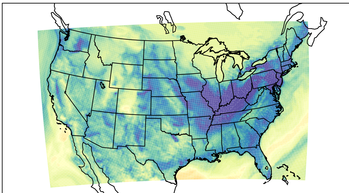
WRF (2020-11-17_10:00:00)
