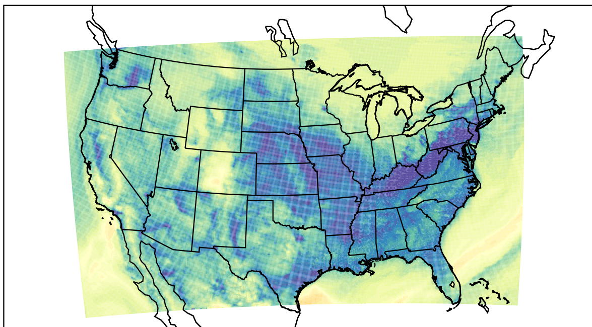
WRF (2020-11-17_14:00:00)
