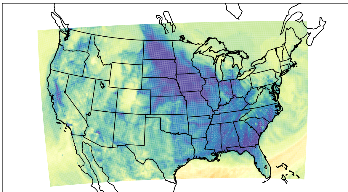
WRF (2020-11-18_08:00:00)
