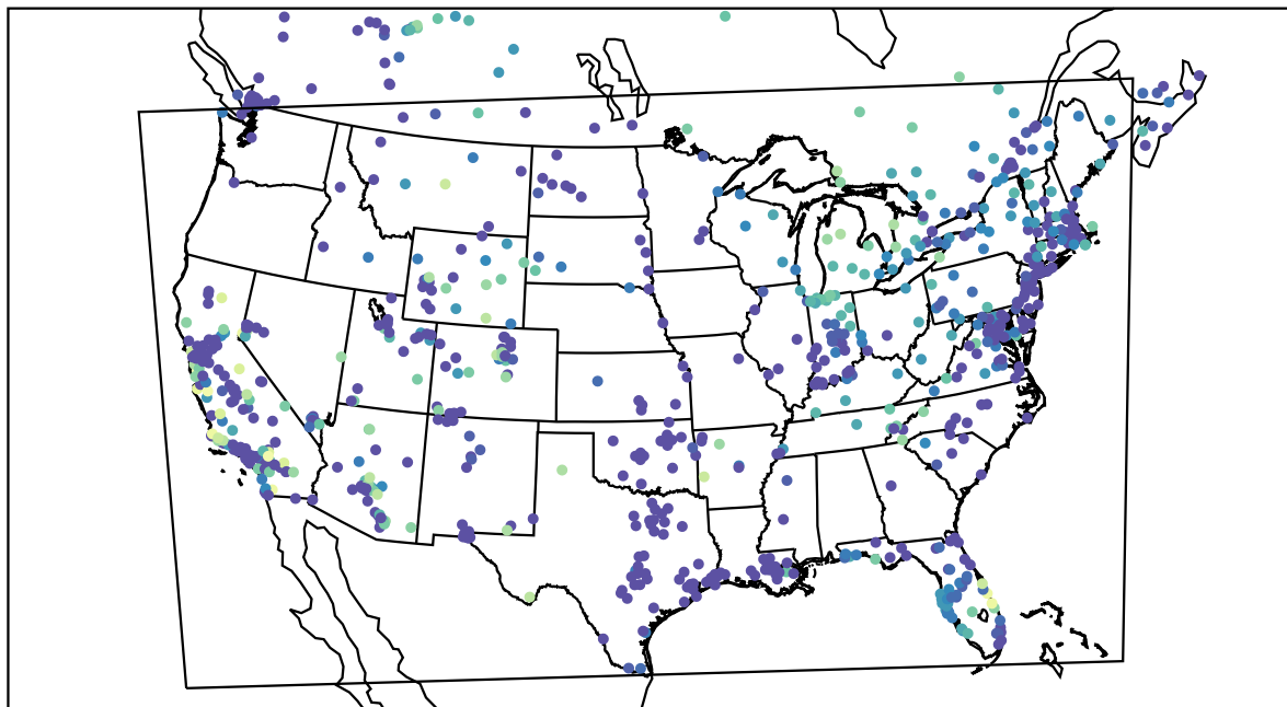
AirNOW (2020-11-17_12:00:00)
