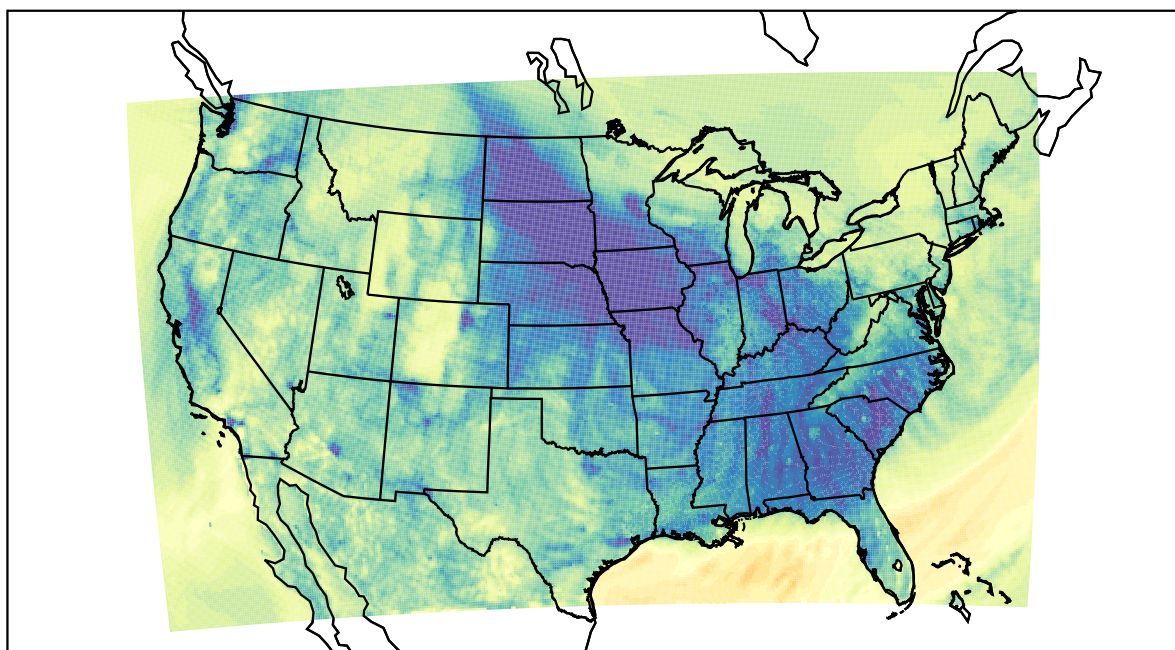
WRF (2020-11-18_04:00:00)
