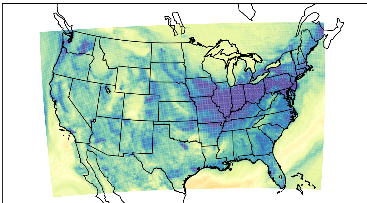
WRF (2020-11-17_07:00:00)
