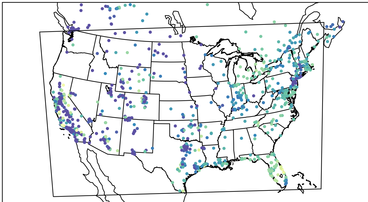
AirNOW (2020-11-17_15:00:00)
