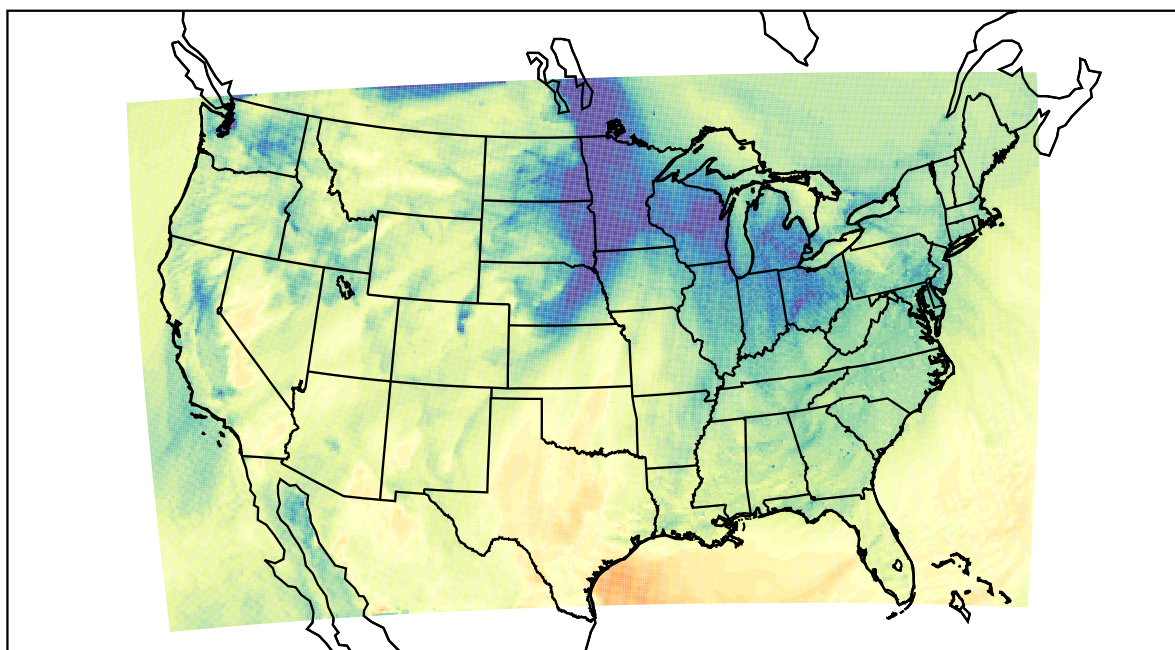
WRF (2020-11-18_21:00:00)
