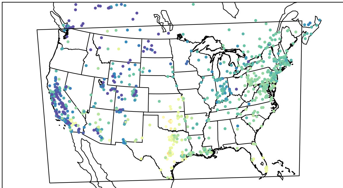
AirNOW (2020-11-18_17:00:00)
