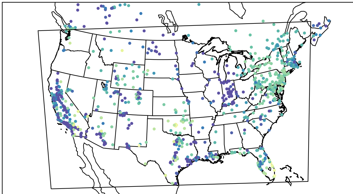
AirNOW (2020-11-18_05:00:00)
