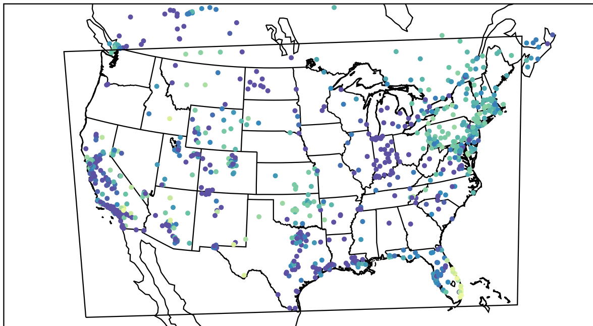
AirNOW (2020-11-18_12:00:00)
