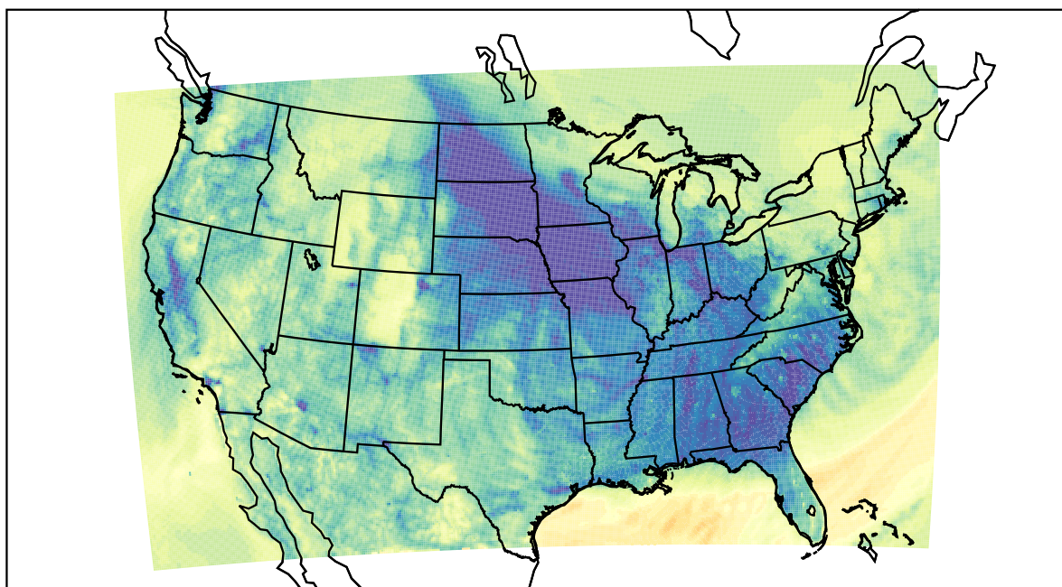
WRF (2020-11-18_05:00:00)
