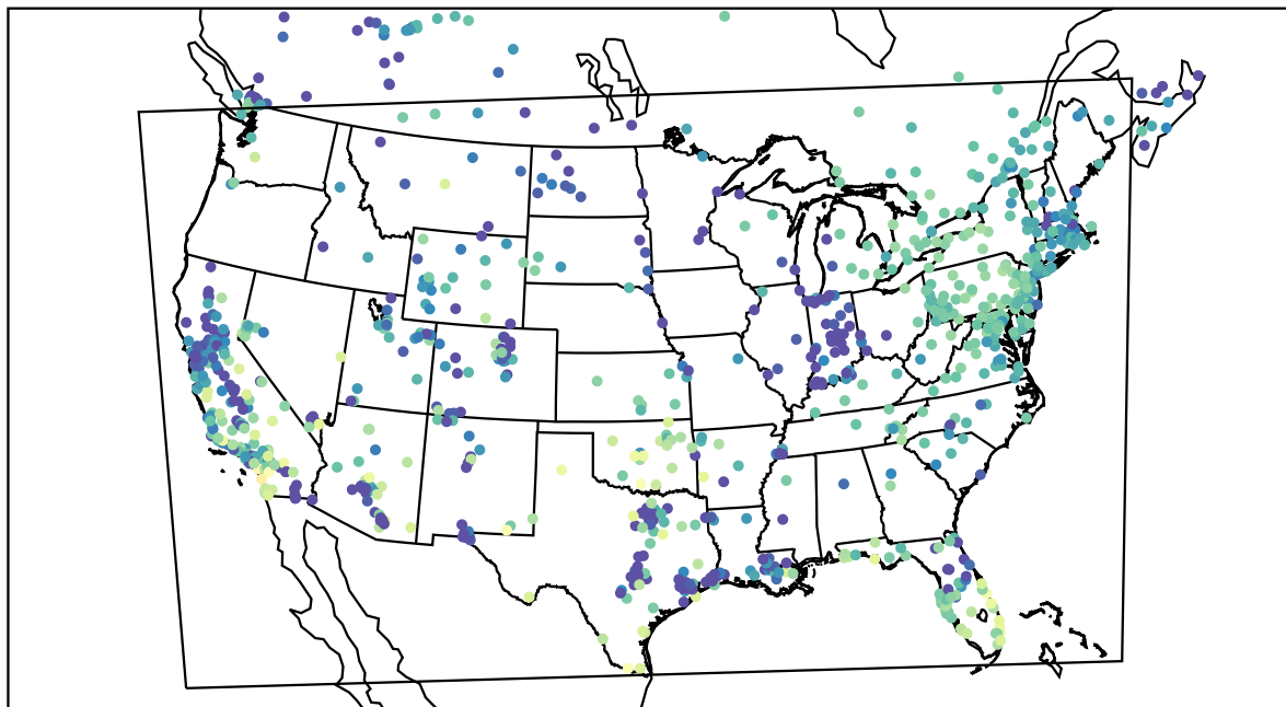
AirNOW (2020-11-18_01:00:00)
