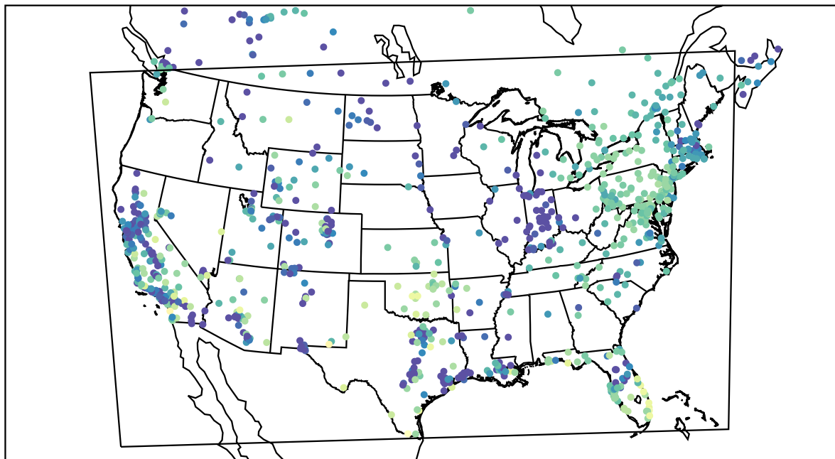
AirNOW (2020-11-18_02:00:00)
