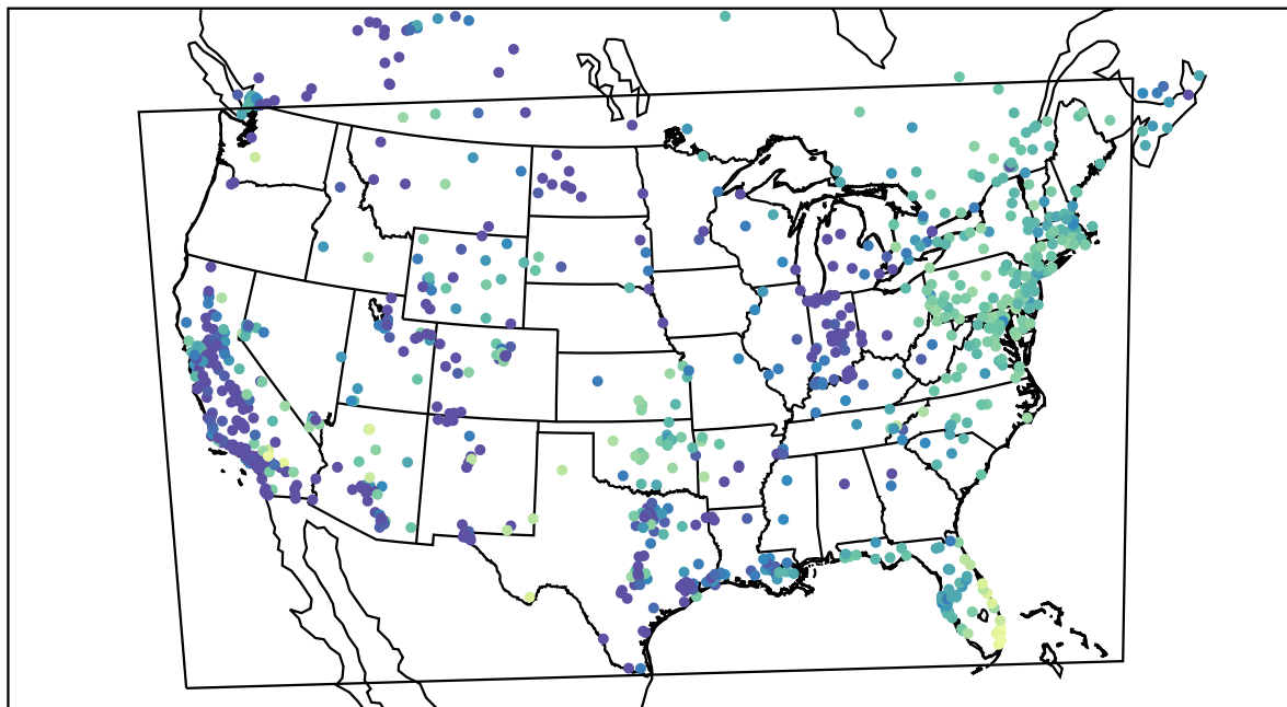
AirNOW (2020-11-18_14:00:00)
