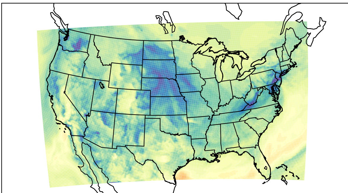
WRF (2020-11-17_17:00:00)
