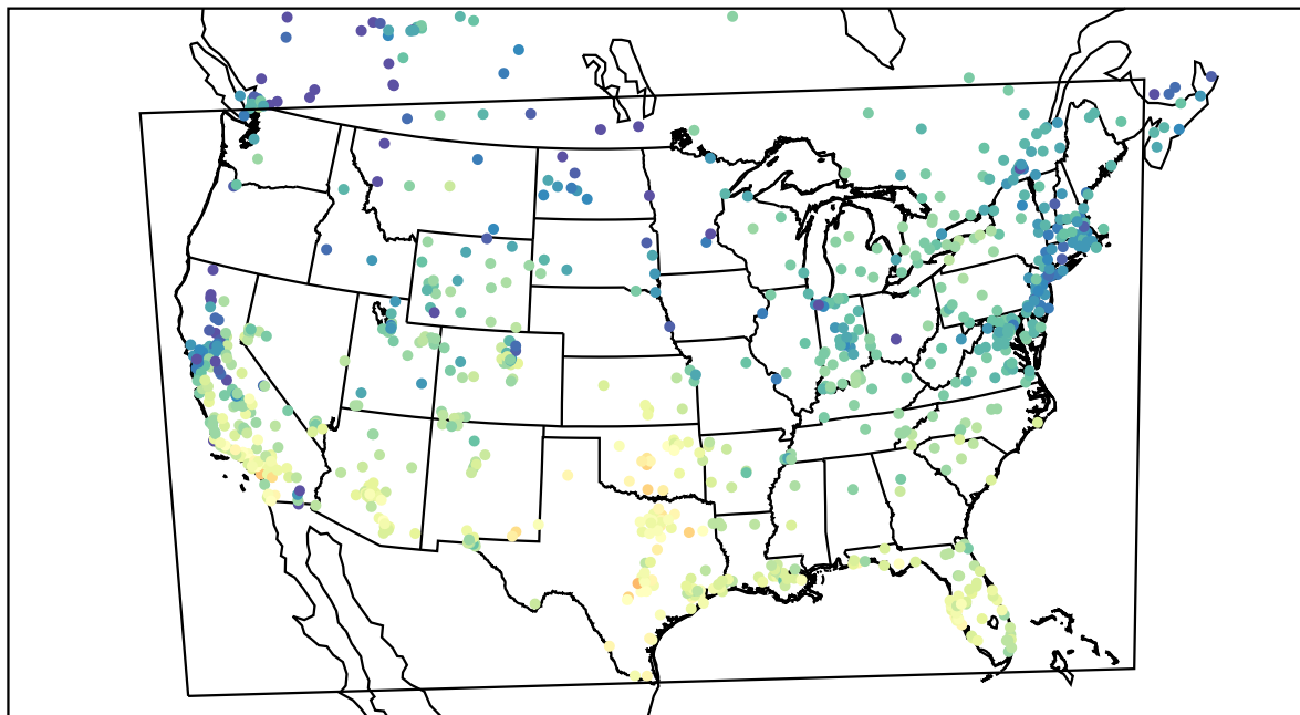
AirNOW (2020-11-17_21:00:00)
