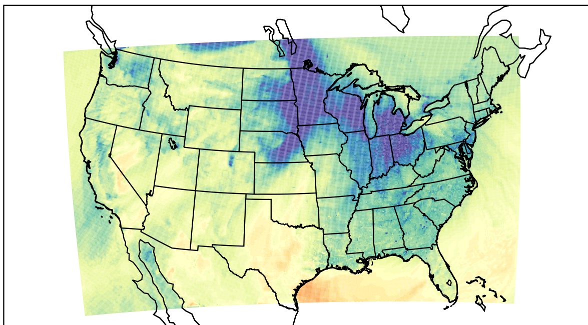
WRF (2020-11-18_22:00:00)
