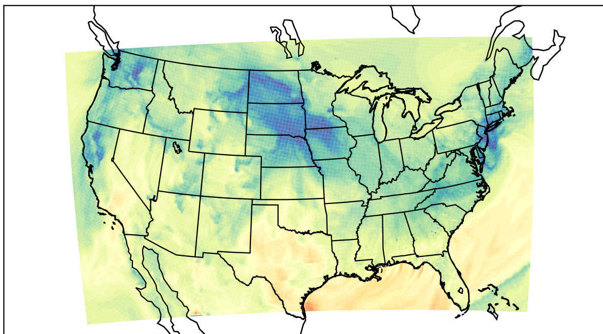
WRF (2020-11-17_21:00:00)
