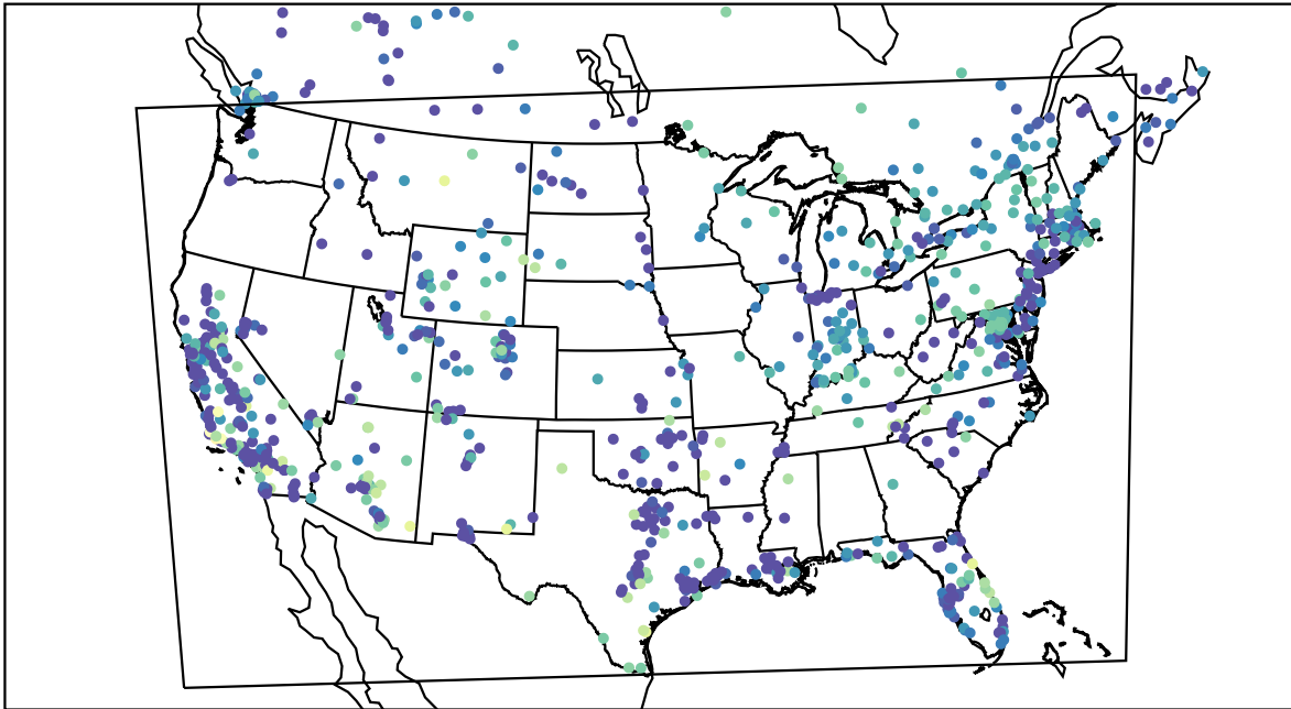
AirNOW (2020-11-17_02:00:00)
