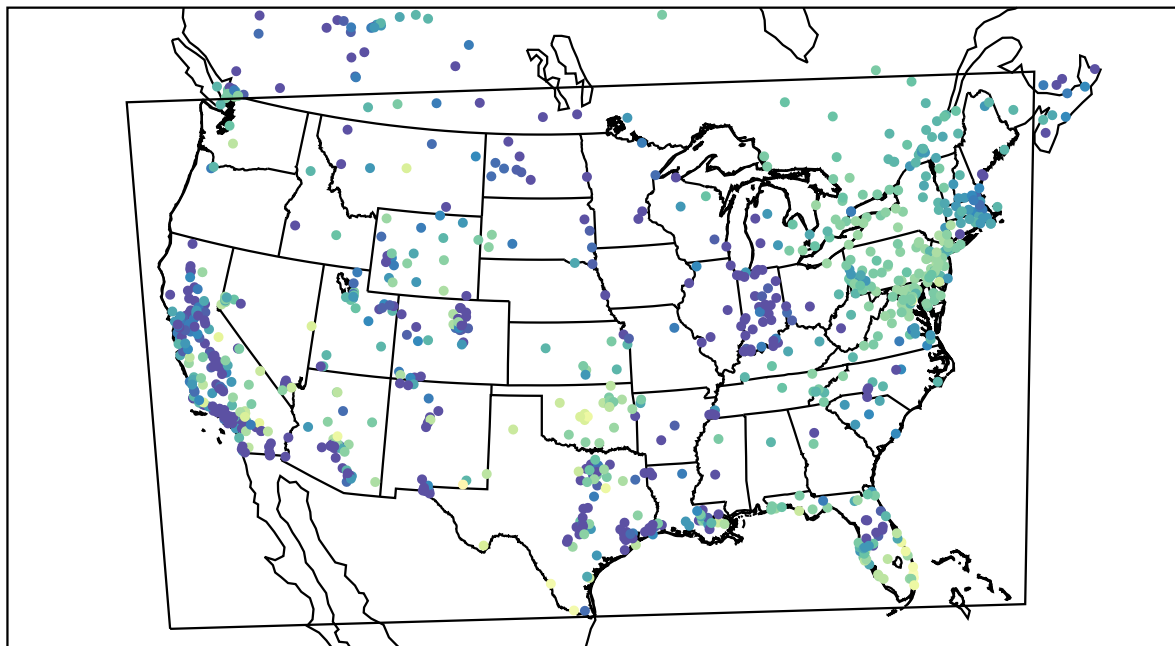
AirNOW (2020-11-18_03:00:00)
