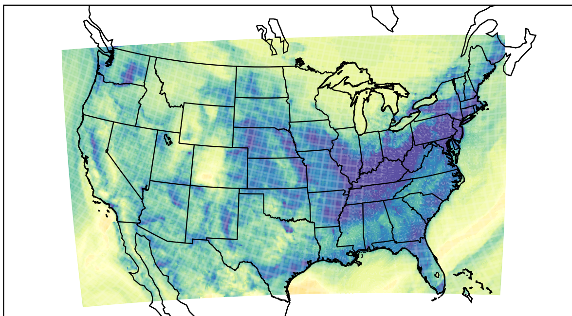
WRF (2020-11-17_12:00:00)
