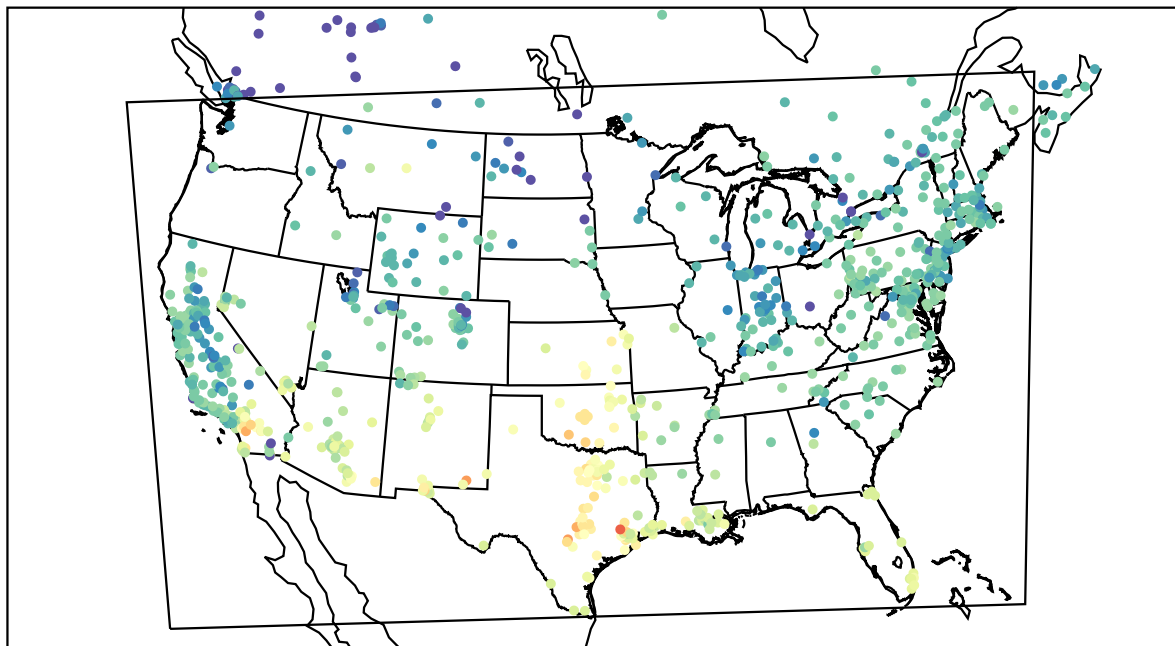
AirNOW (2020-11-18_21:00:00)
