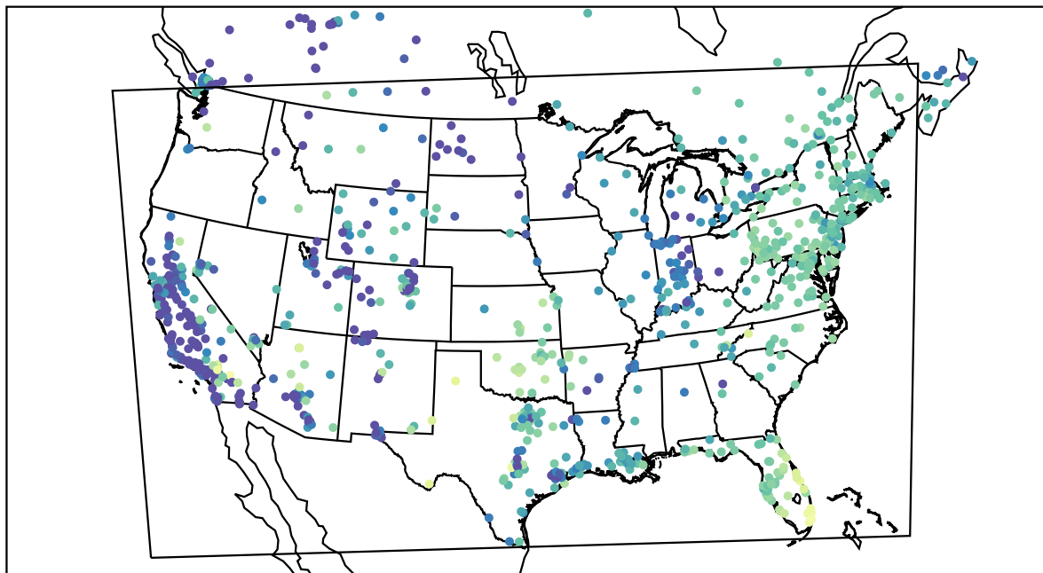
AirNOW (2020-11-18_15:00:00)
