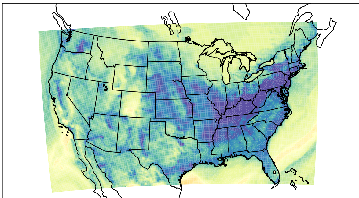
WRF (2020-11-17_13:00:00)
