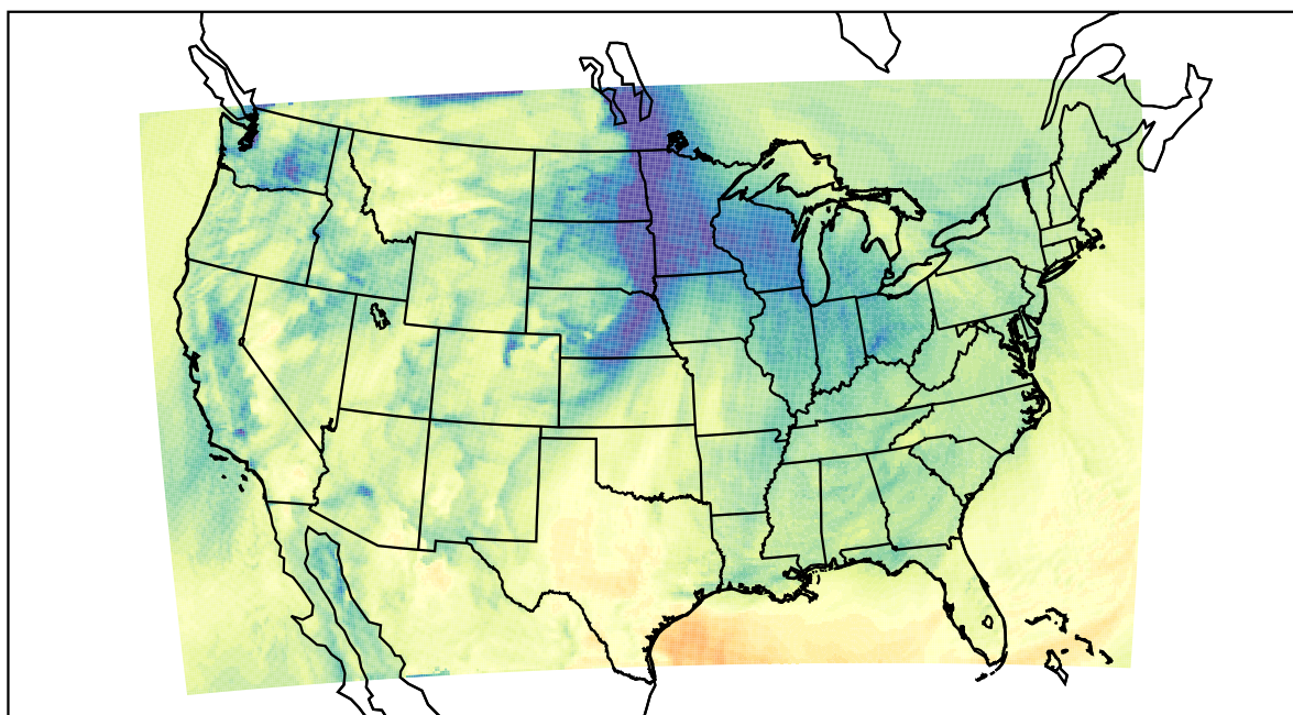
WRF (2020-11-18_19:00:00)
