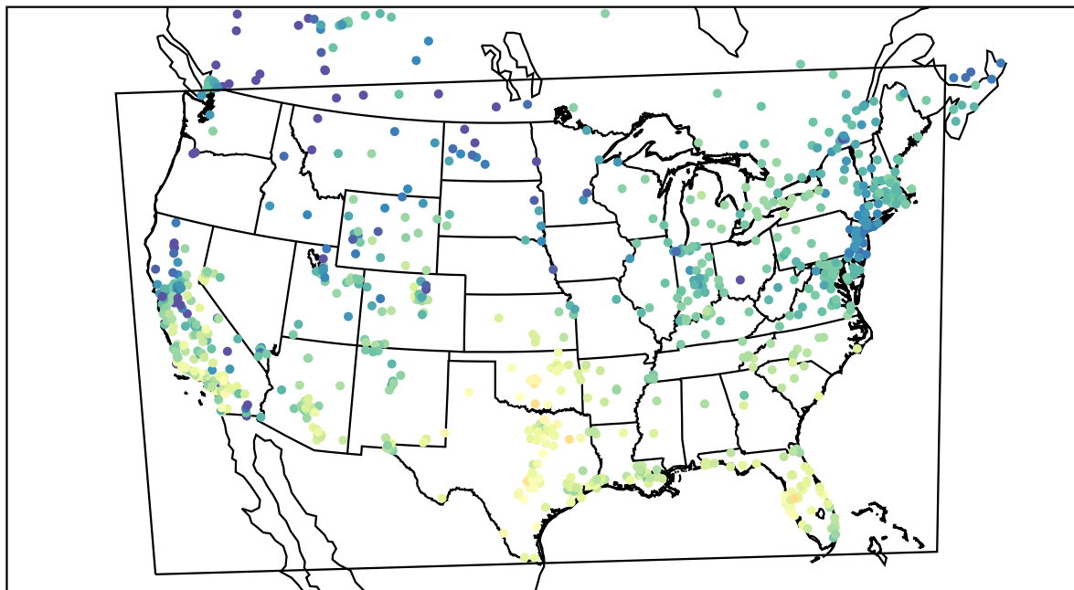
AirNOW (2020-11-17_19:00:00)
