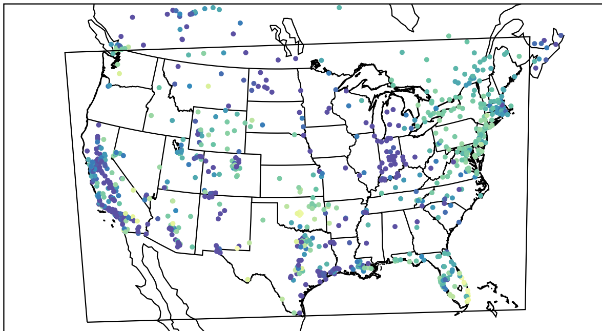
AirNOW (2020-11-18_06:00:00)
