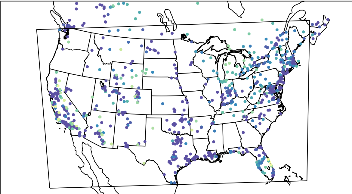
AirNOW (2020-11-17_11:00:00)
