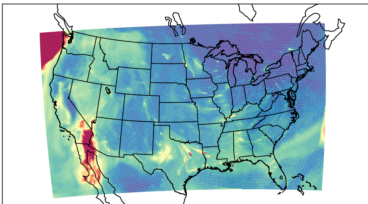
WRF 2020-12-15_16:00:00
