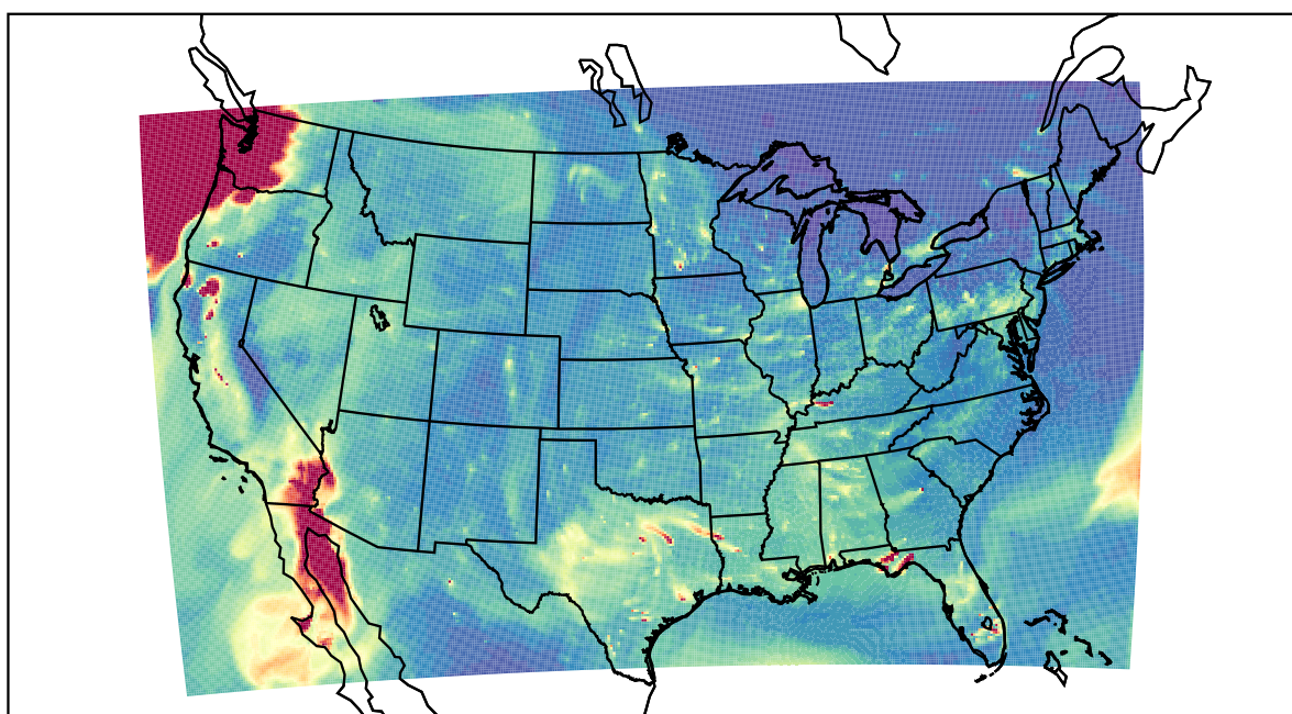
WRF 2020-12-16_00:00:00
