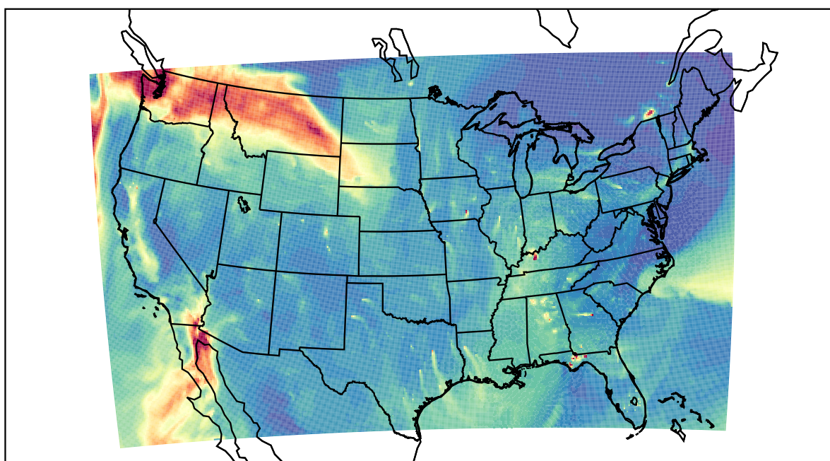
WRF 2020-12-16_19:00:00
