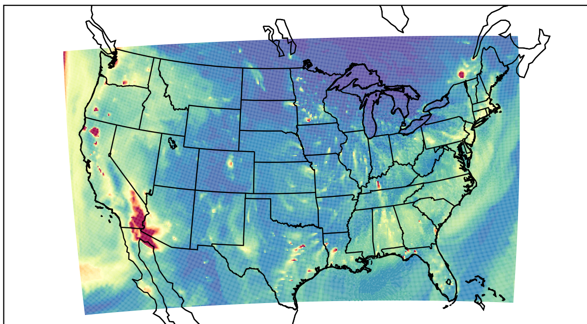
WRF 2020-12-15_02:00:00
