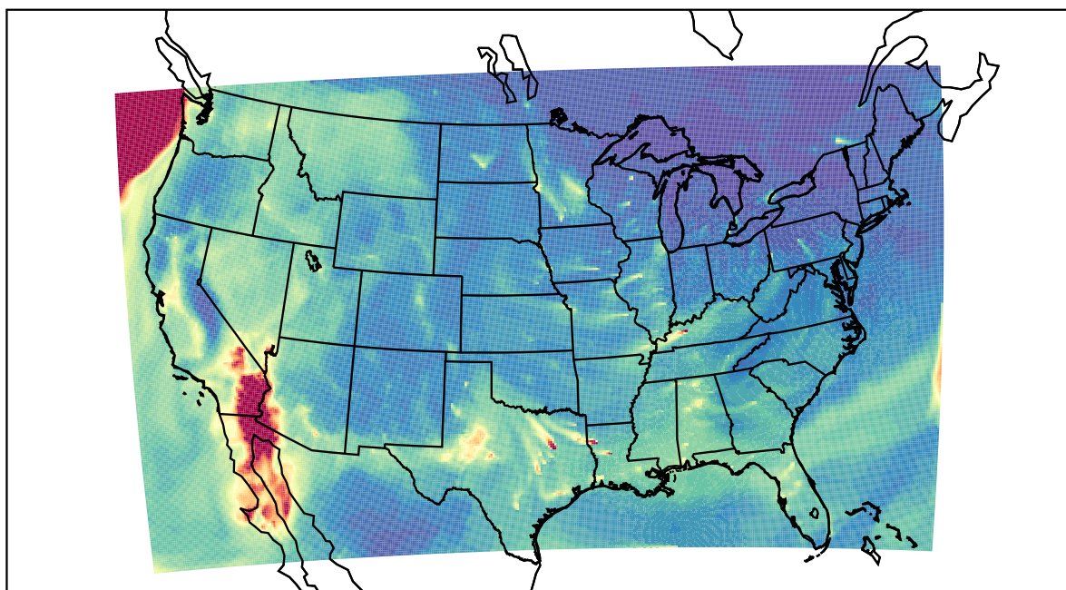
WRF 2020-12-15_15:00:00
