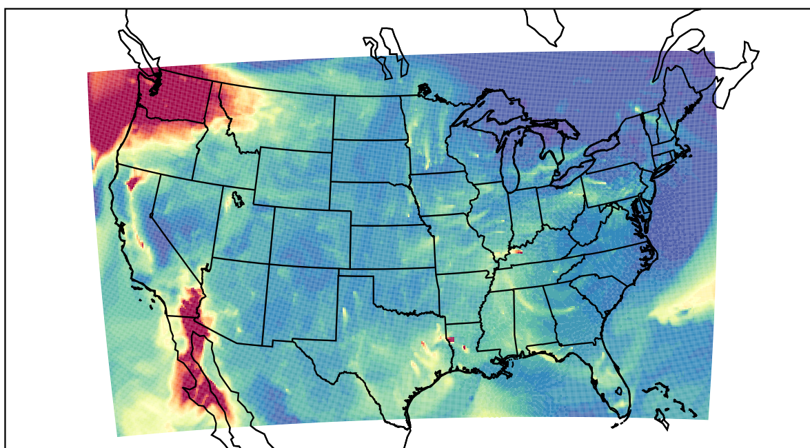
WRF 2020-12-16_08:00:00
