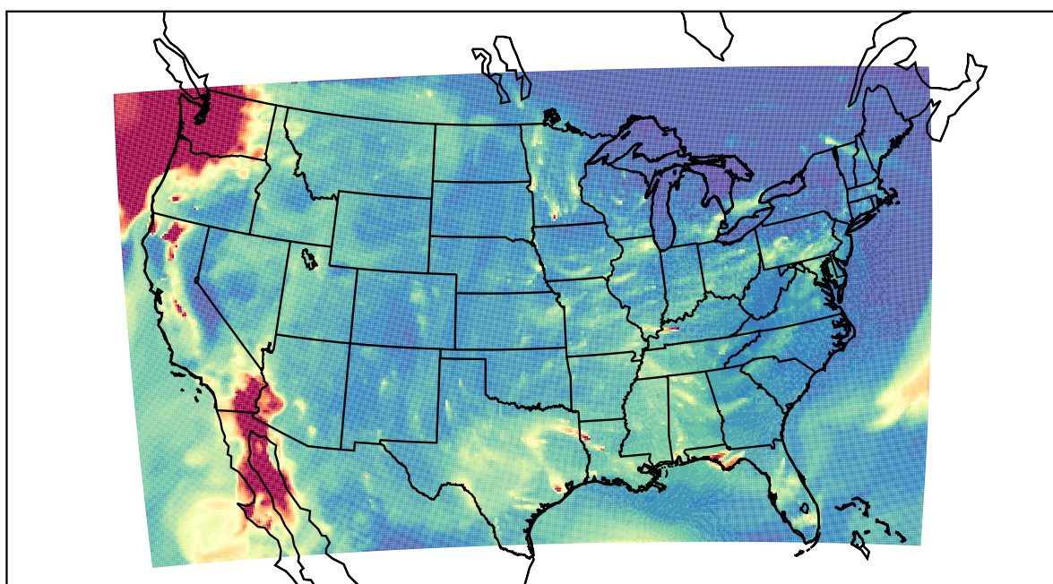
WRF 2020-12-16_03:00:00
