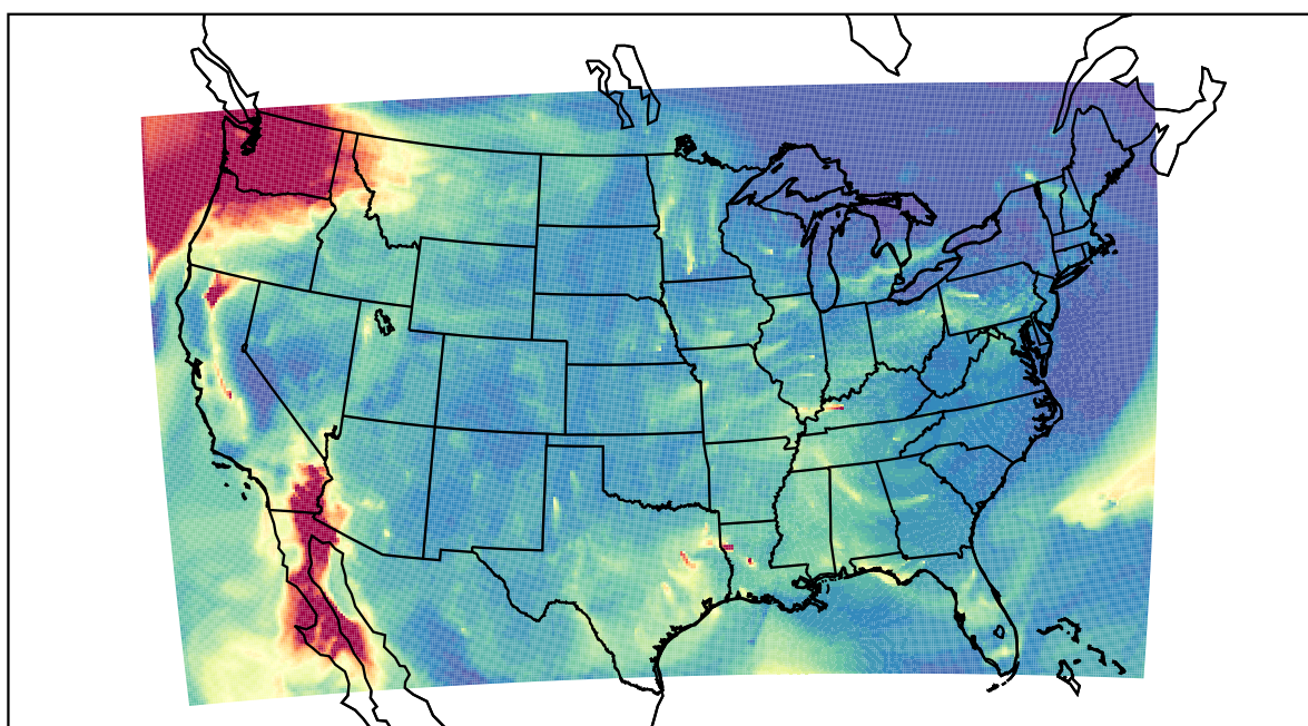
WRF 2020-12-16_07:00:00
