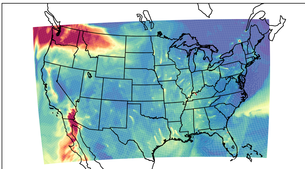
WRF 2020-12-16_14:00:00
