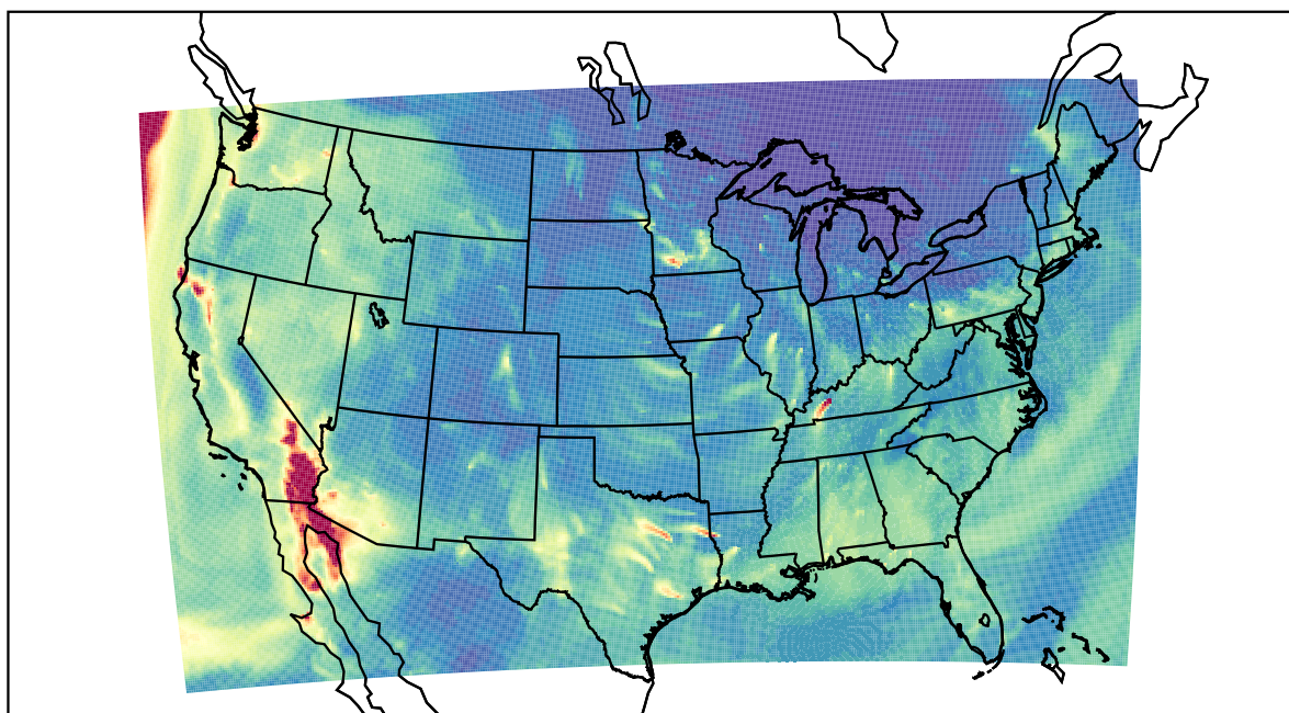
WRF 2020-12-15_07:00:00
