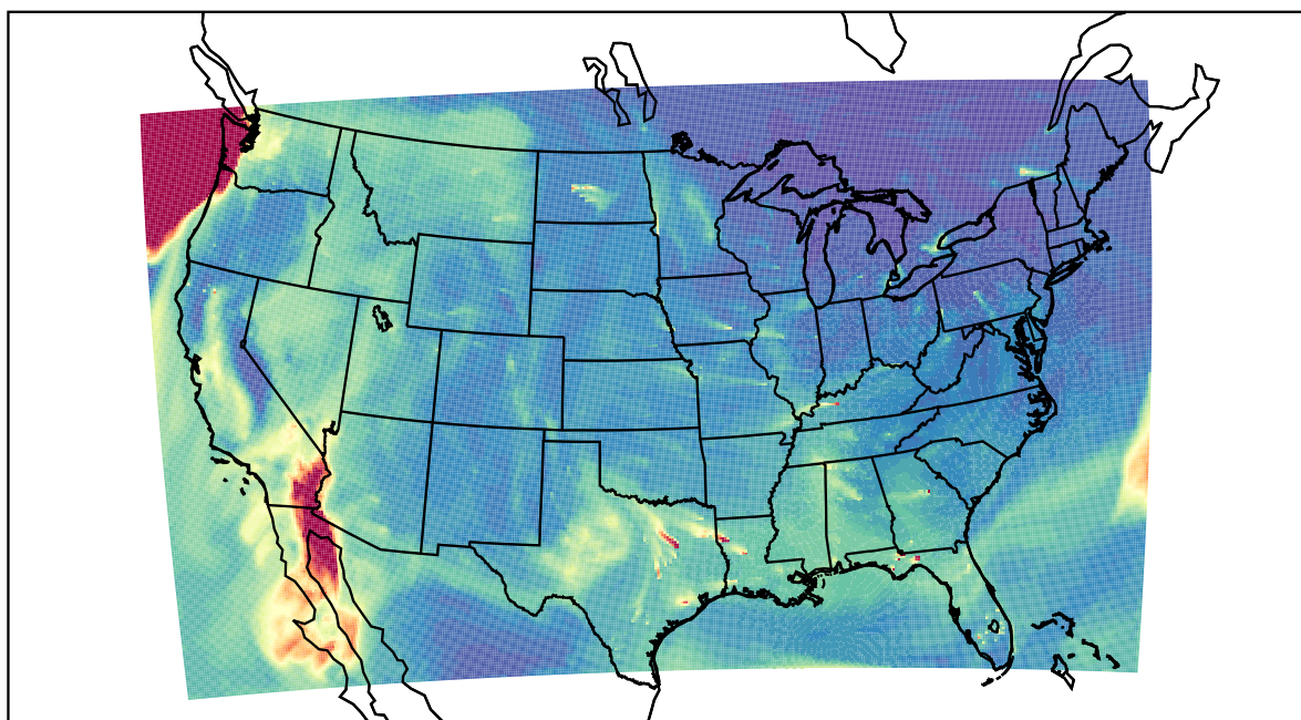
WRF 2020-12-15_19:00:00
