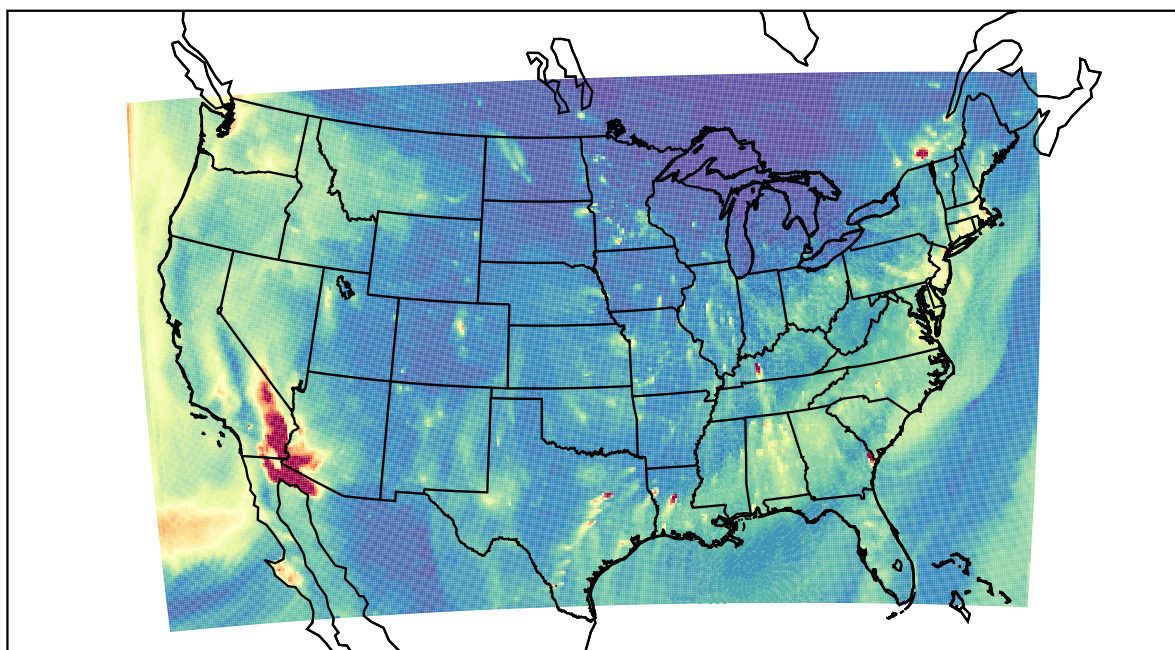
WRF 2020-12-15_00:00:00
