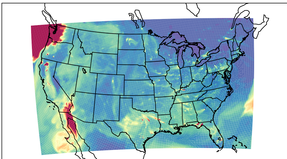
WRF 2020-12-15_23:00:00
