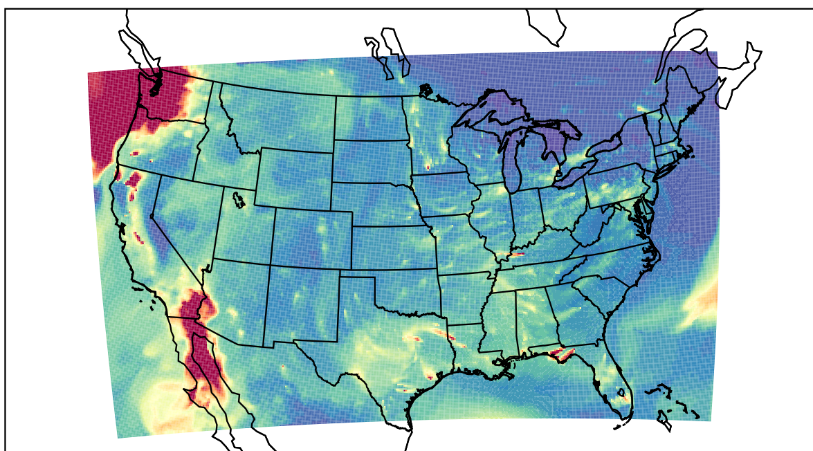
WRF 2020-12-16_02:00:00
