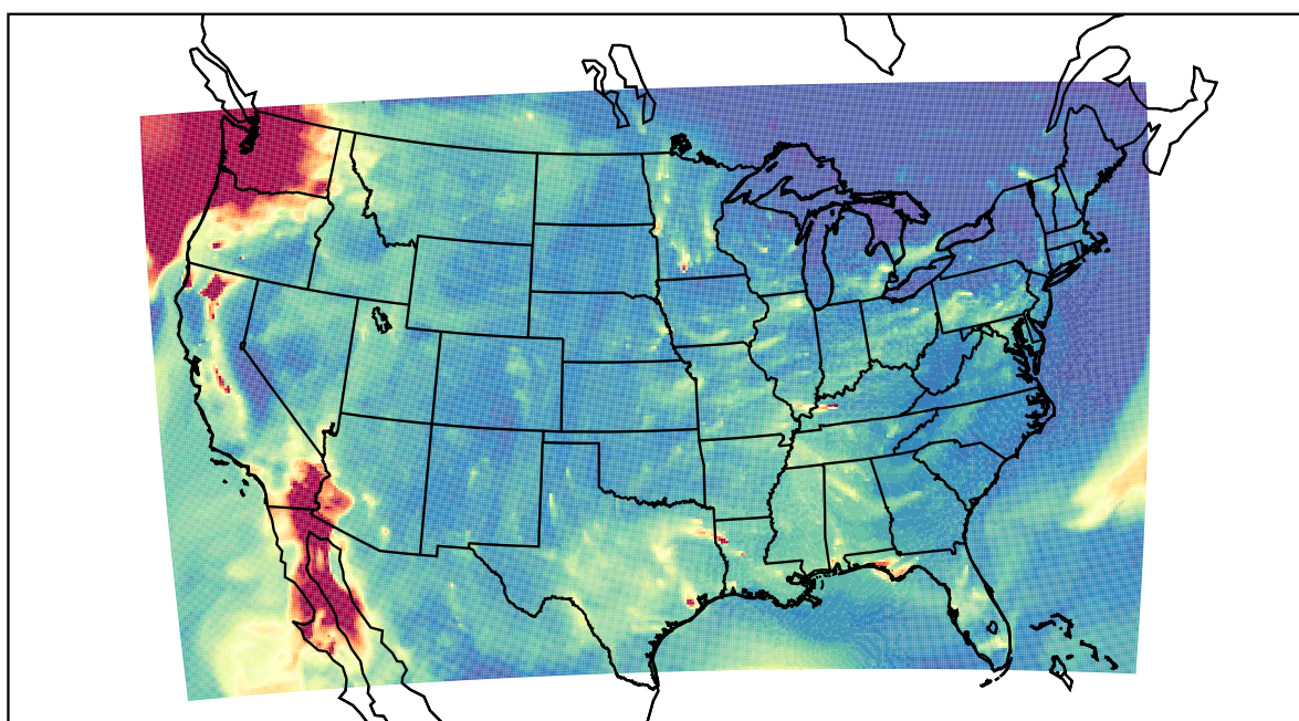
WRF 2020-12-16_04:00:00
