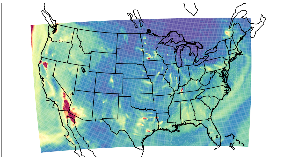
WRF 2020-12-15_05:00:00
