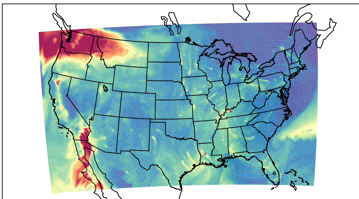
WRF 2020-12-16_12:00:00
