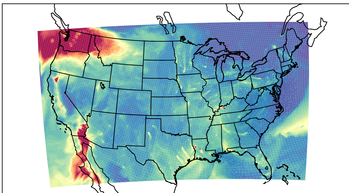
WRF 2020-12-16_11:00:00
