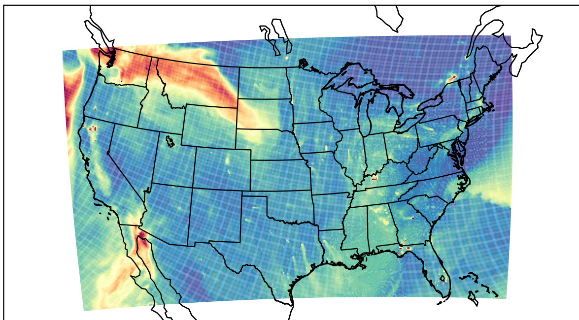
WRF 2020-12-16_21:00:00
