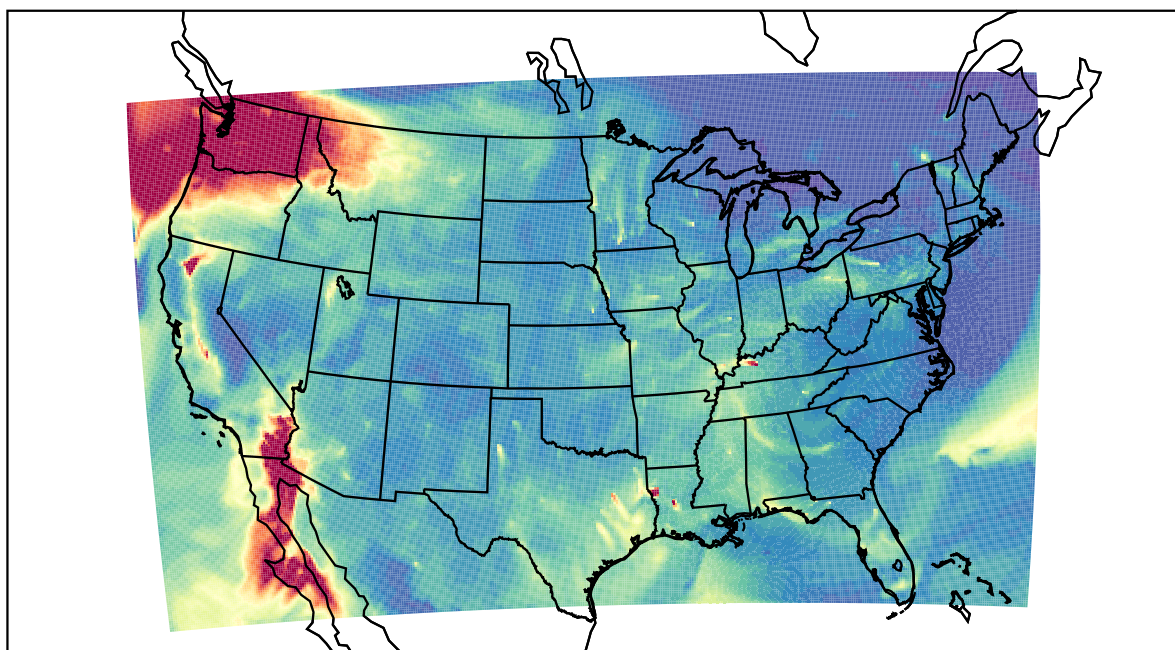
WRF 2020-12-16_09:00:00
