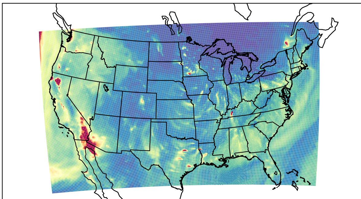
WRF 2020-12-15_04:00:00
