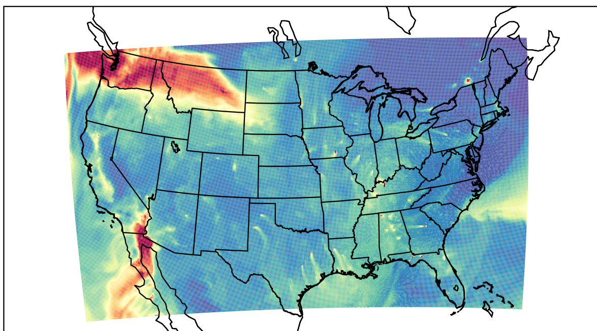
WRF 2020-12-16_17:00:00
