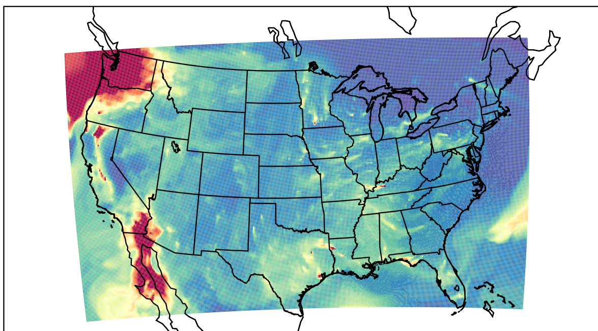
WRF 2020-12-16_05:00:00
