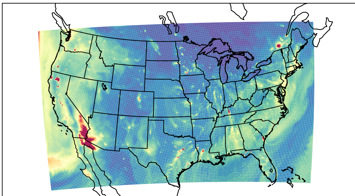
WRF 2020-12-15_01:00:00
