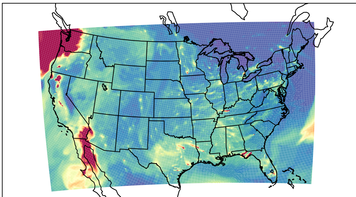
WRF 2020-12-16_01:00:00
