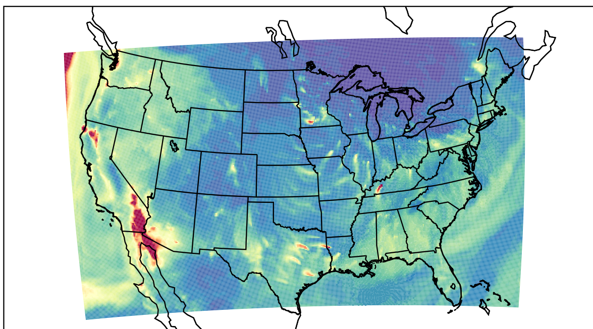
WRF 2020-12-15_06:00:00
