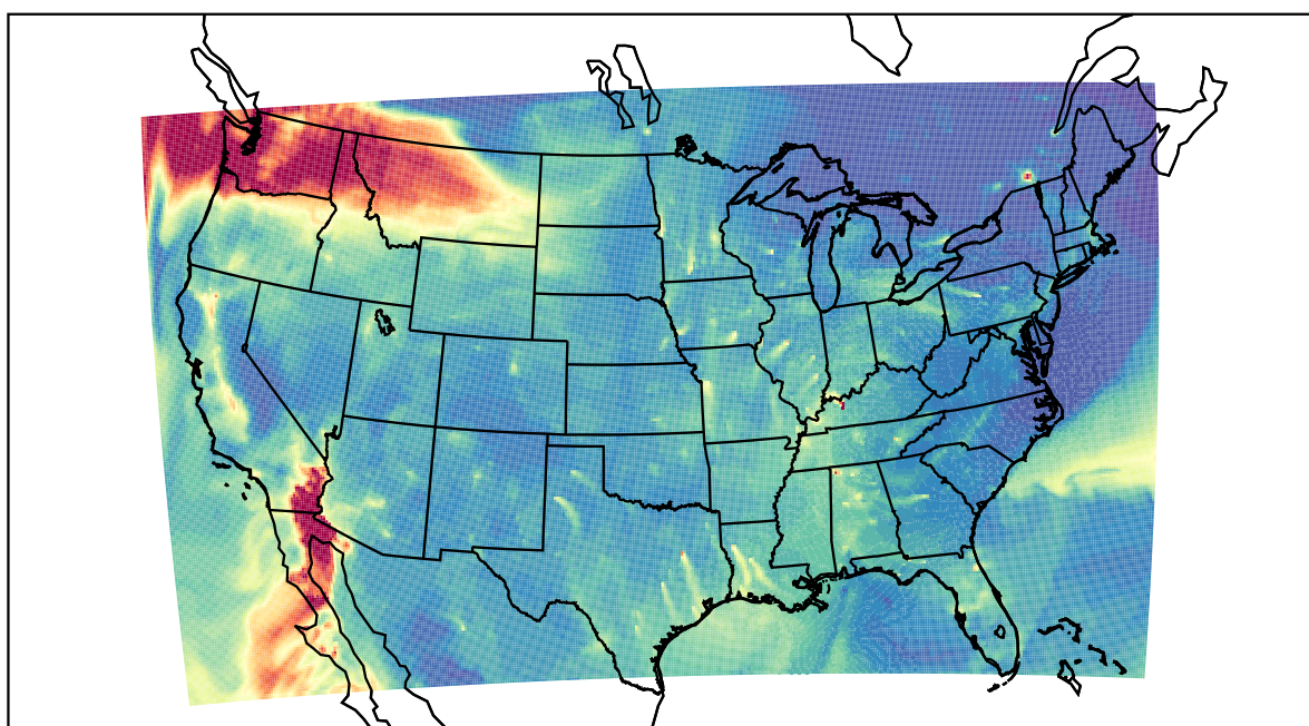
WRF 2020-12-16_15:00:00
