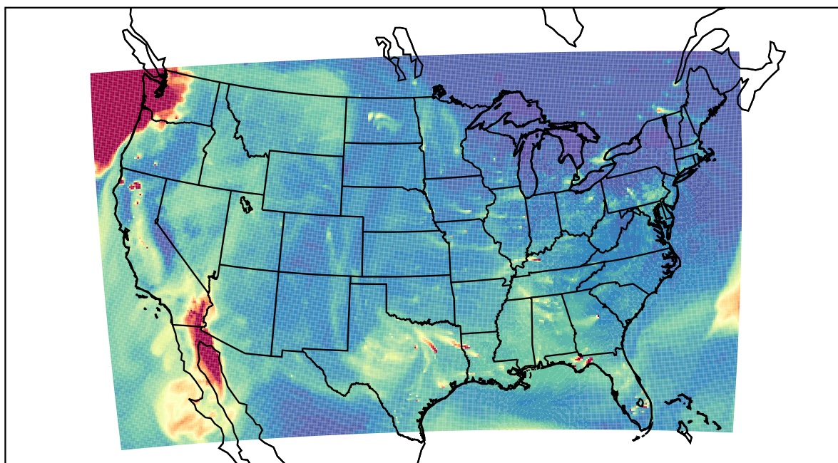
WRF 2020-12-15_22:00:00
