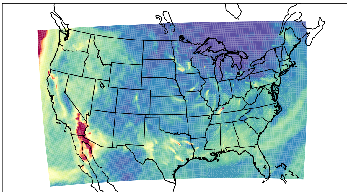
WRF 2020-12-15_08:00:00
