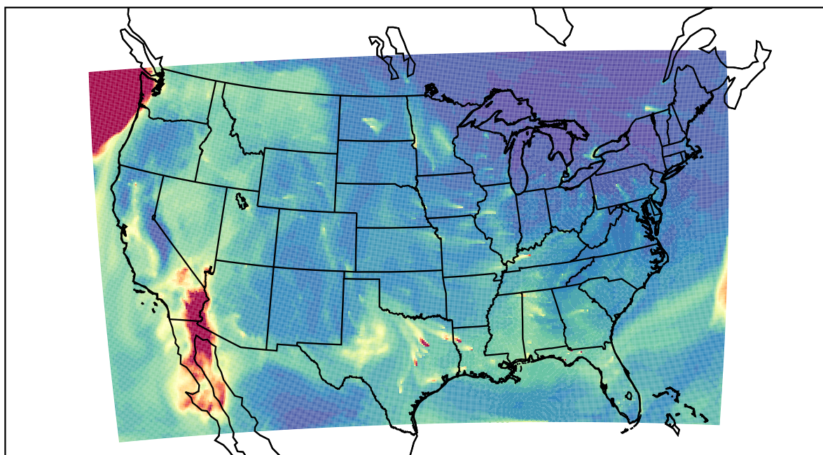
WRF 2020-12-15_17:00:00
