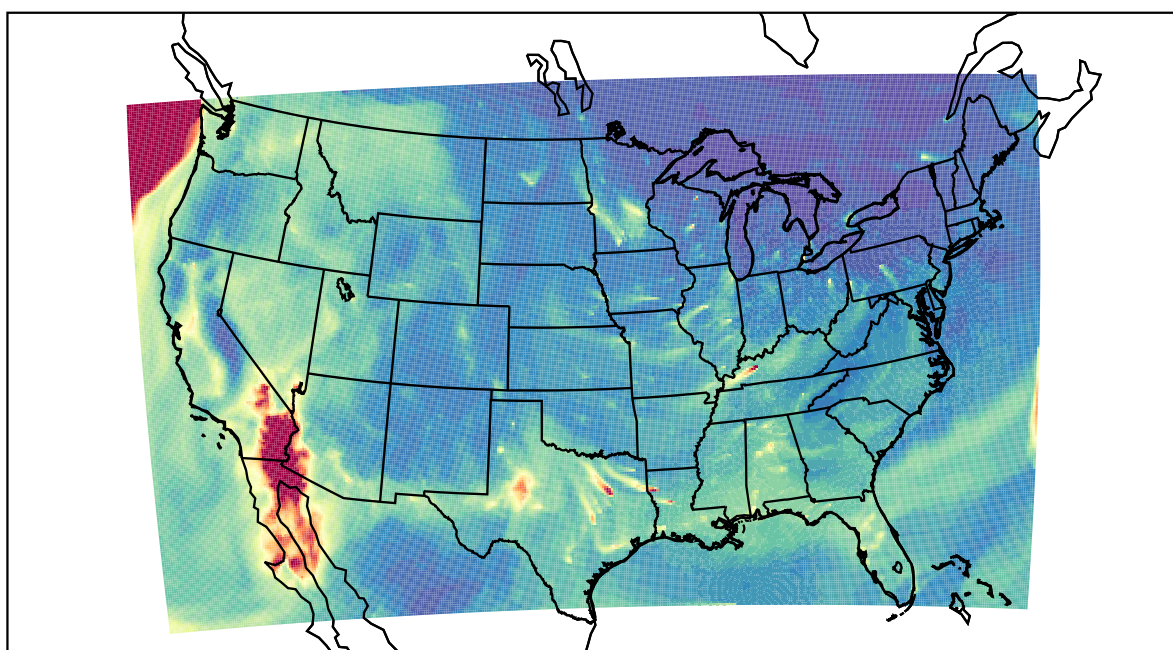
WRF 2020-12-15_14:00:00
