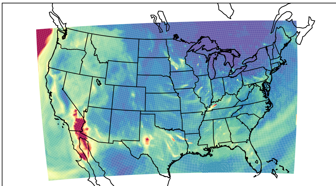
WRF 2020-12-15_11:00:00
