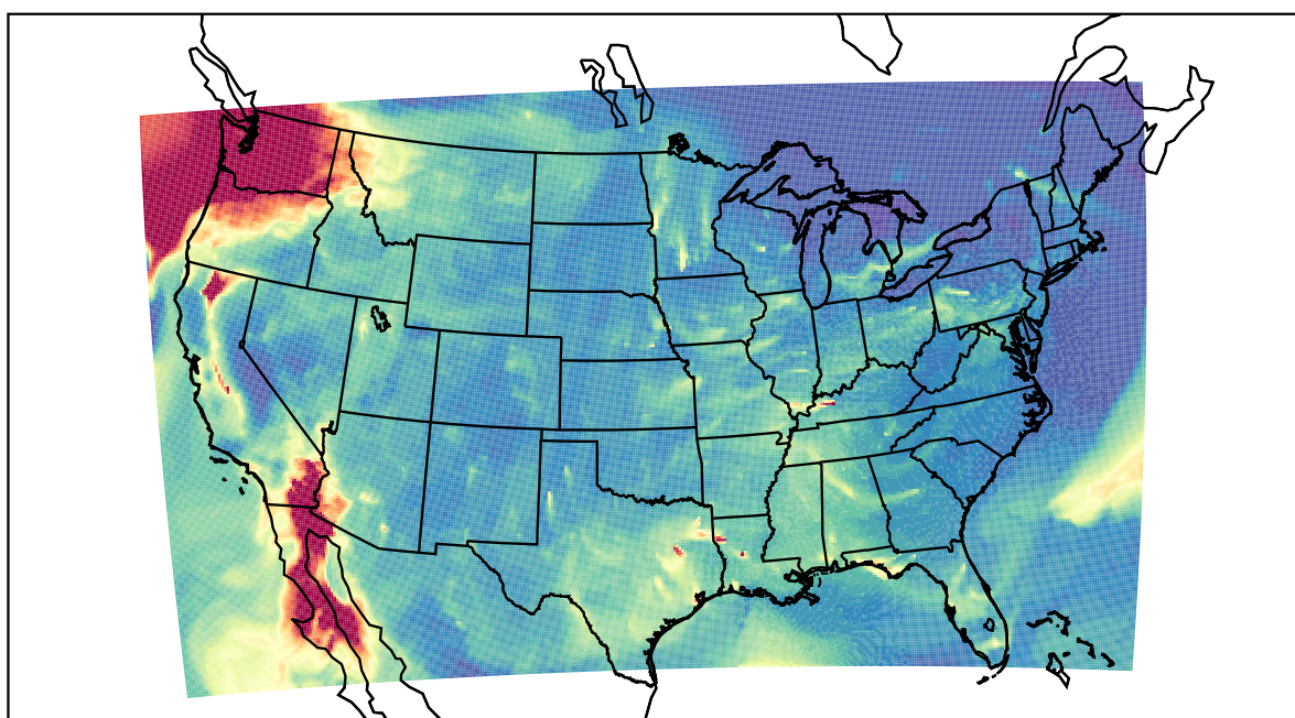
WRF 2020-12-16_06:00:00
