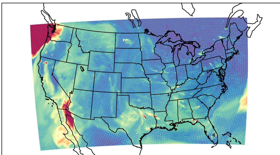
WRF 2020-12-15_21:00:00
