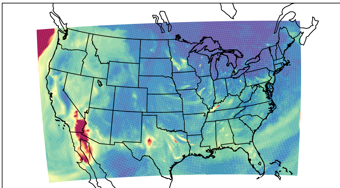
WRF 2020-12-15_12:00:00
