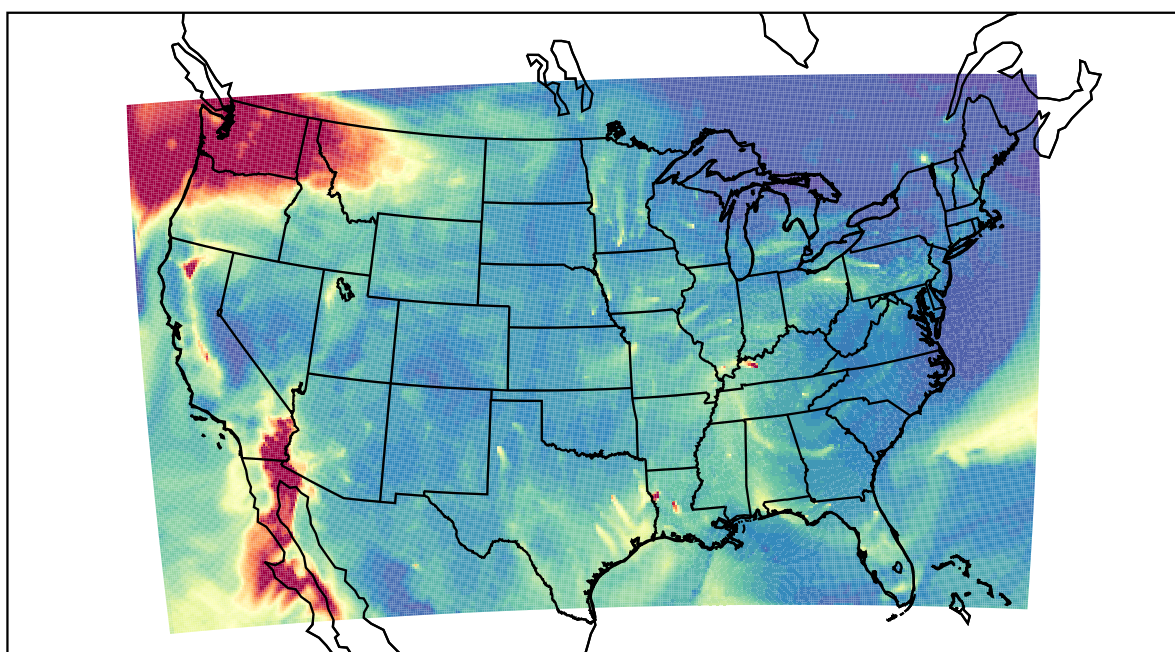
WRF 2020-12-16_10:00:00
