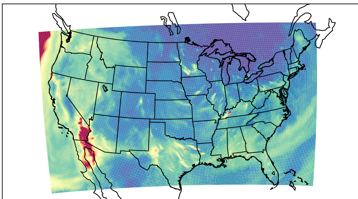
WRF 2020-12-15_09:00:00
