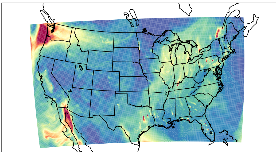
WRF 2020-12-19_20:00:00
