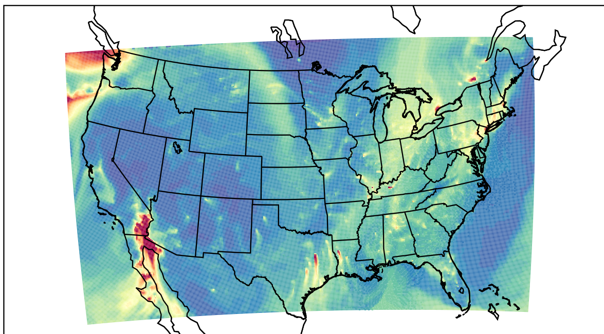
WRF 2020-12-20_14:00:00
