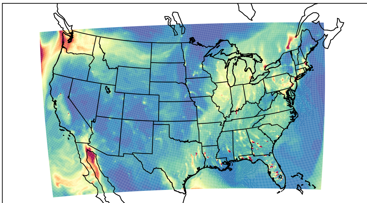
WRF 2020-12-19_23:00:00
