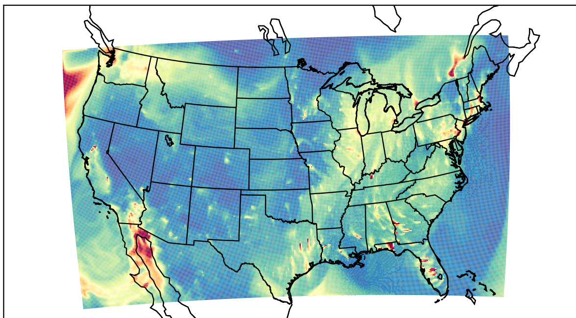
WRF 2020-12-20_02:00:00
