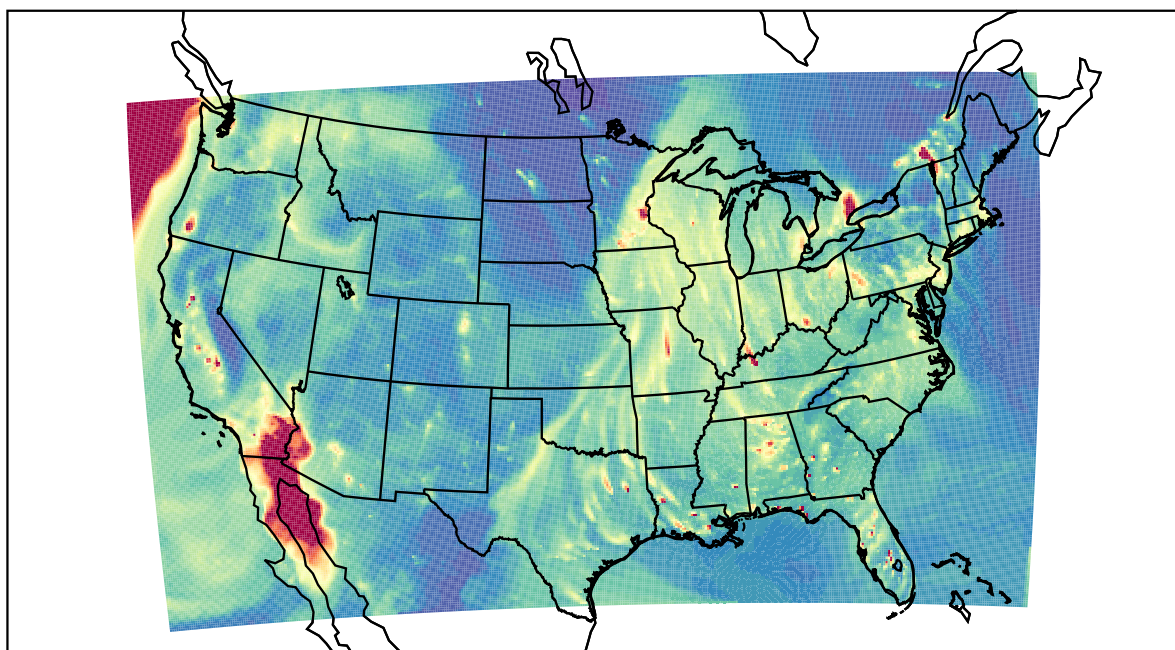
WRF 2020-12-19_02:00:00
