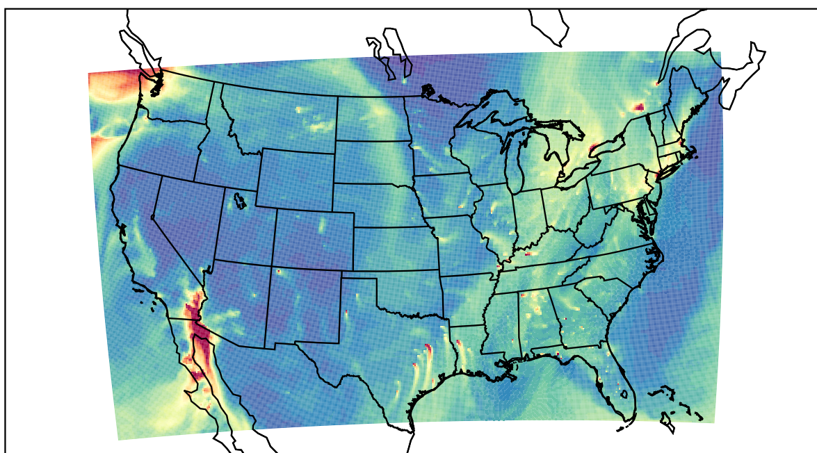
WRF 2020-12-20_17:00:00
