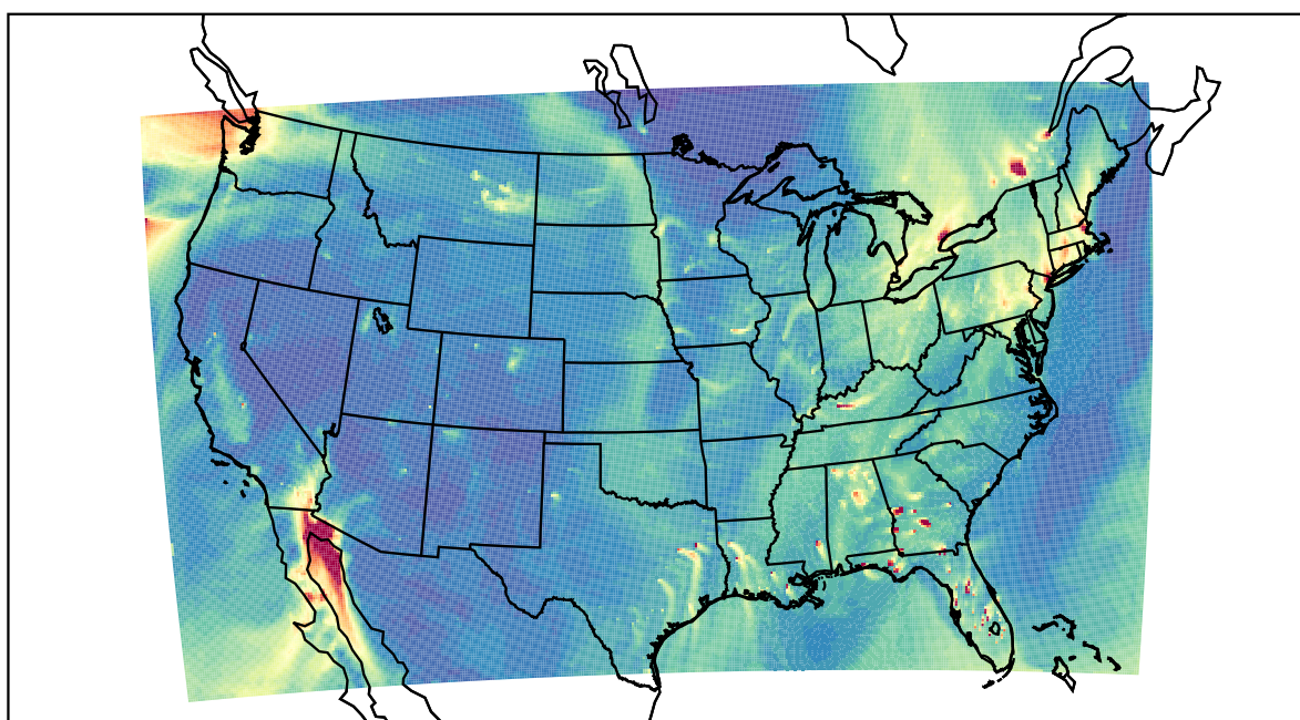
WRF 2020-12-20_21:00:00
