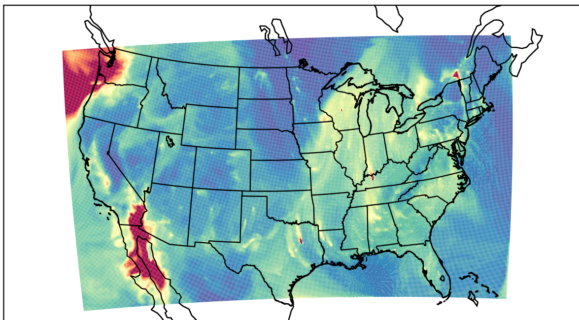
WRF 2020-12-19_09:00:00
