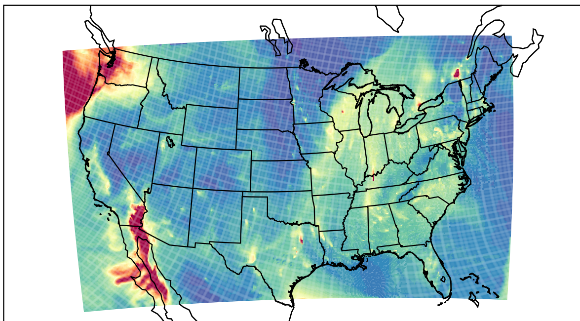
WRF 2020-12-19_13:00:00
