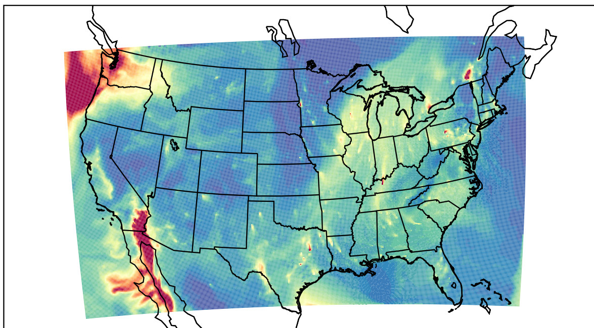
WRF 2020-12-19_15:00:00
