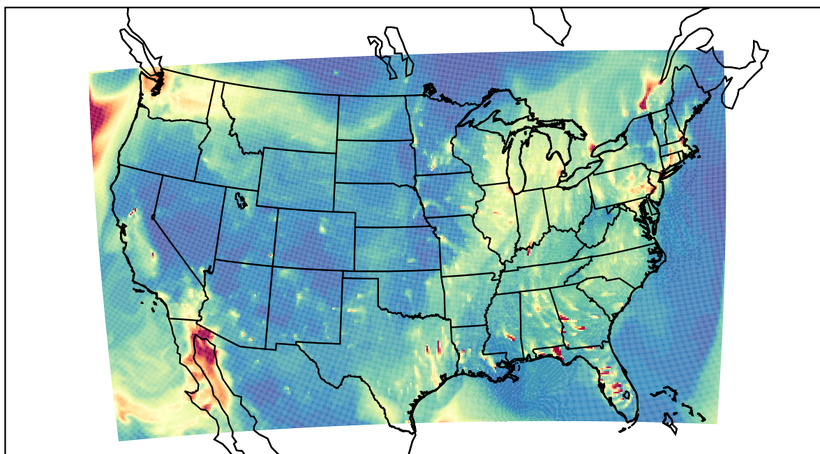
WRF 2020-12-20_01:00:00
