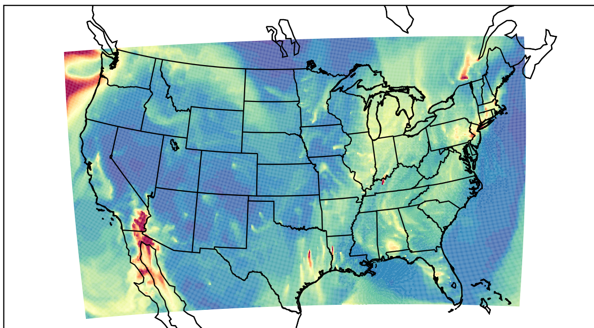
WRF 2020-12-20_07:00:00
