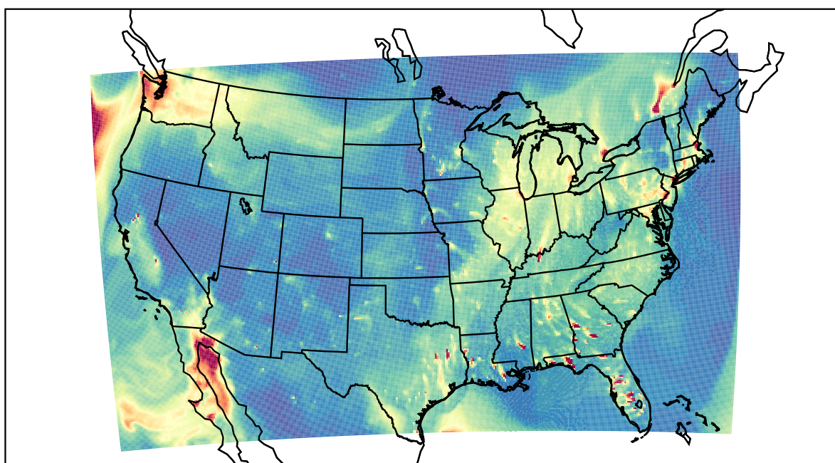
WRF 2020-12-20_00:00:00
