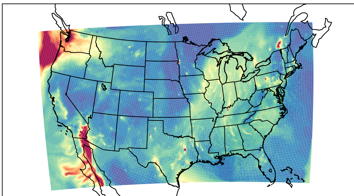
WRF 2020-12-19_16:00:00
