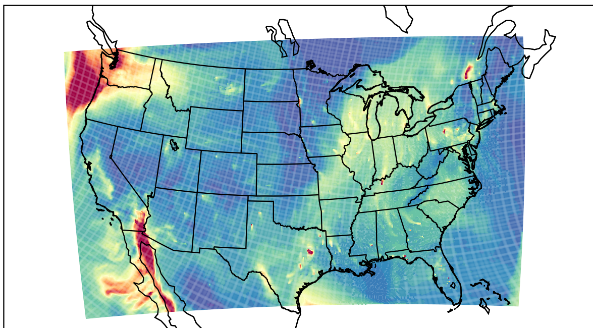
WRF 2020-12-19_17:00:00
