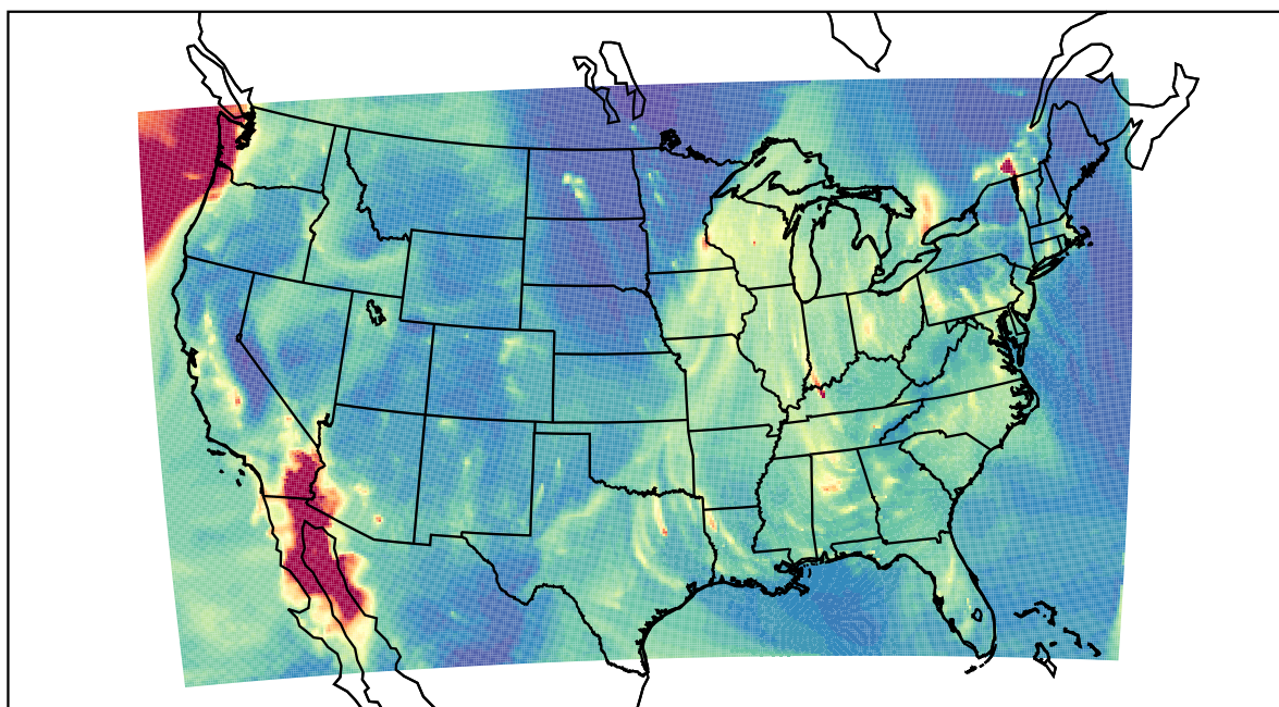
WRF 2020-12-19_06:00:00
