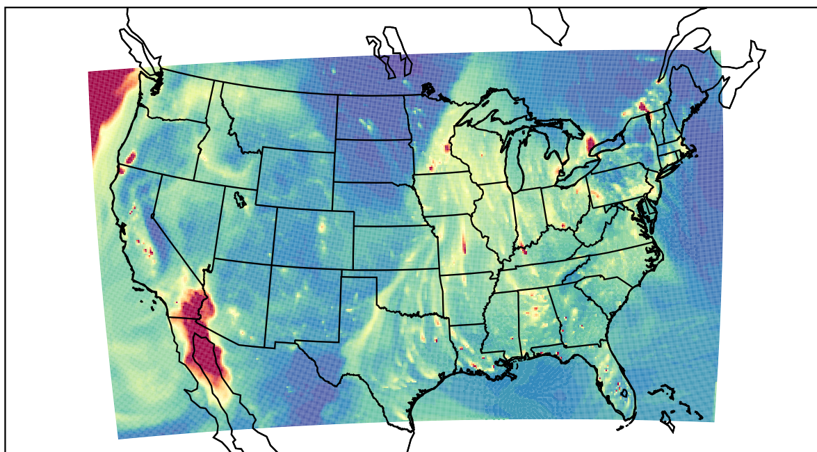
WRF 2020-12-19_01:00:00
