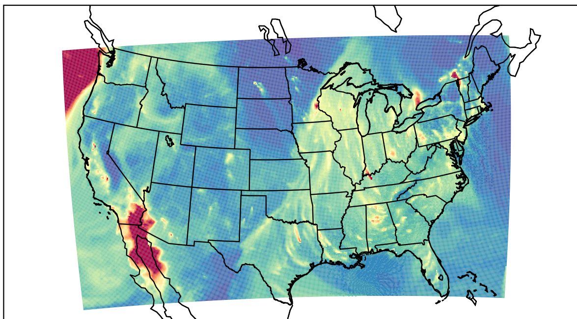
WRF 2020-12-19_04:00:00
