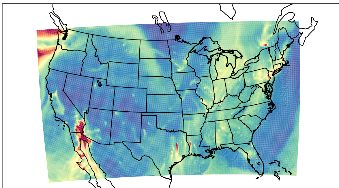
WRF 2020-12-20_11:00:00
