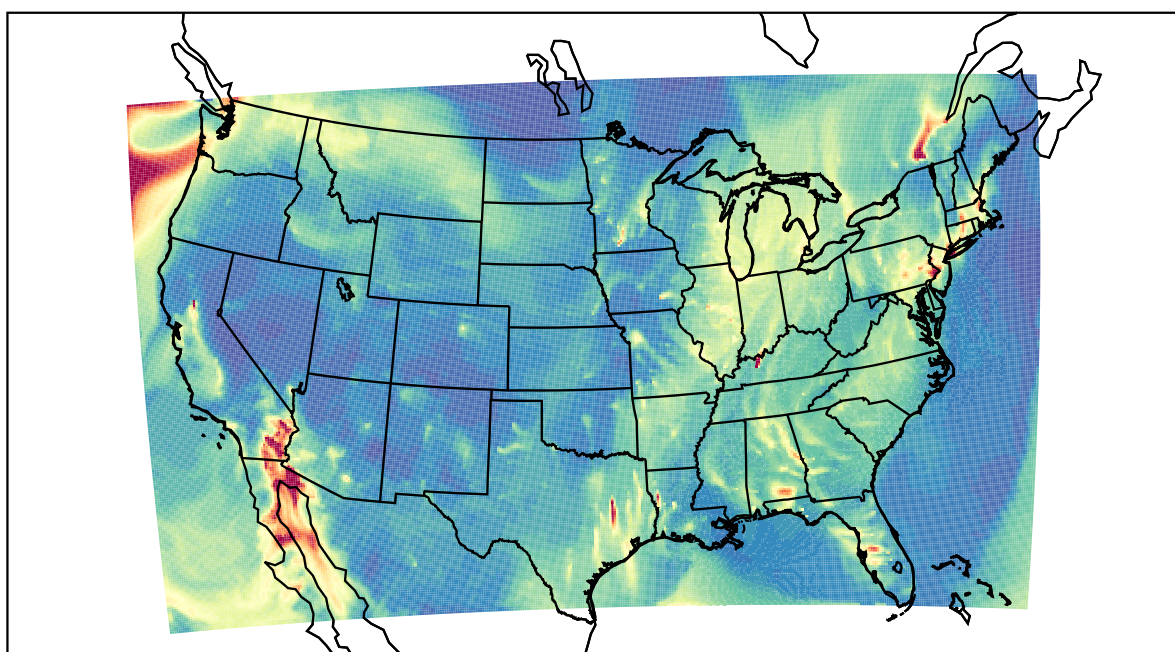
WRF 2020-12-20_05:00:00
