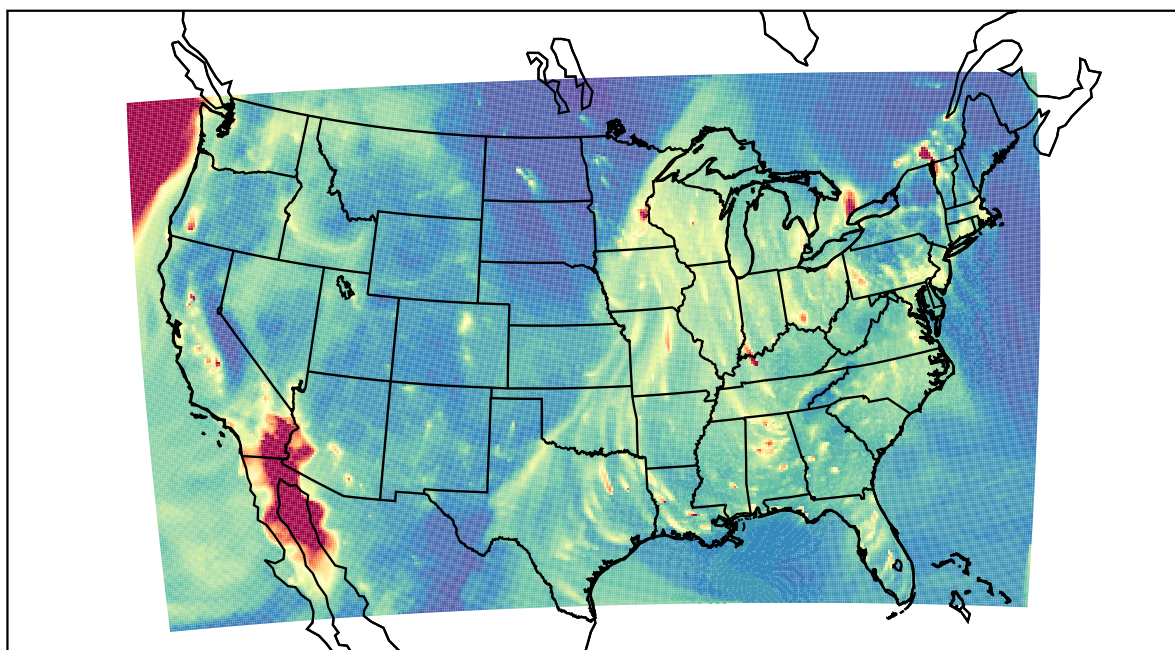
WRF 2020-12-19_03:00:00
