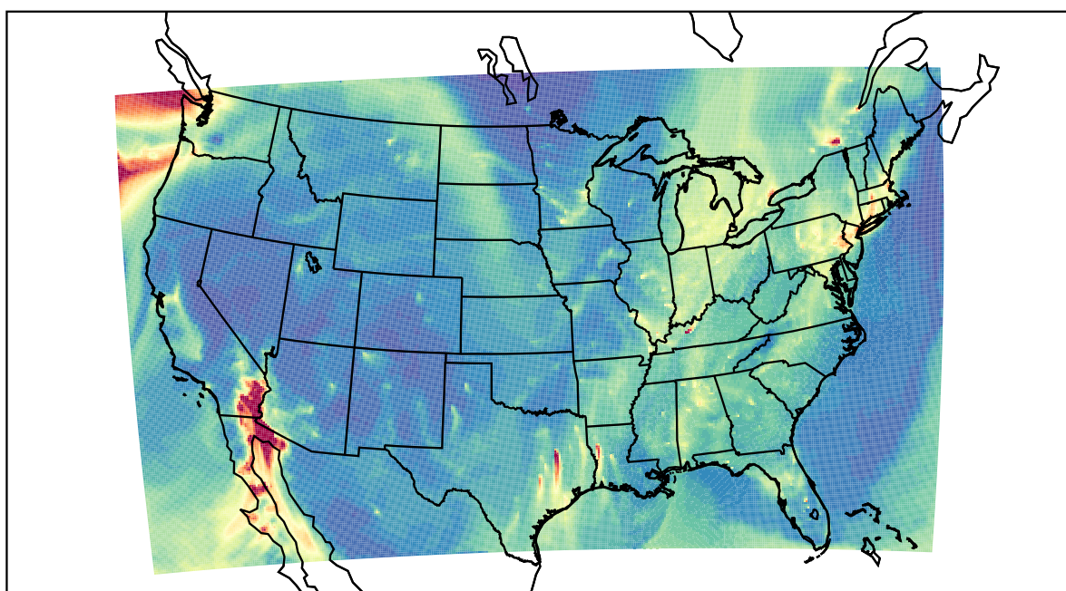
WRF 2020-12-20_12:00:00
