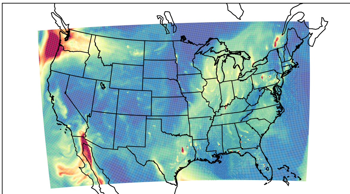
WRF 2020-12-19_19:00:00
