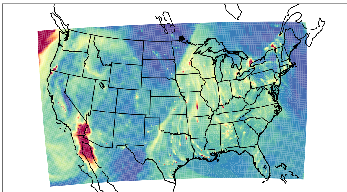
WRF 2020-12-19_00:00:00
