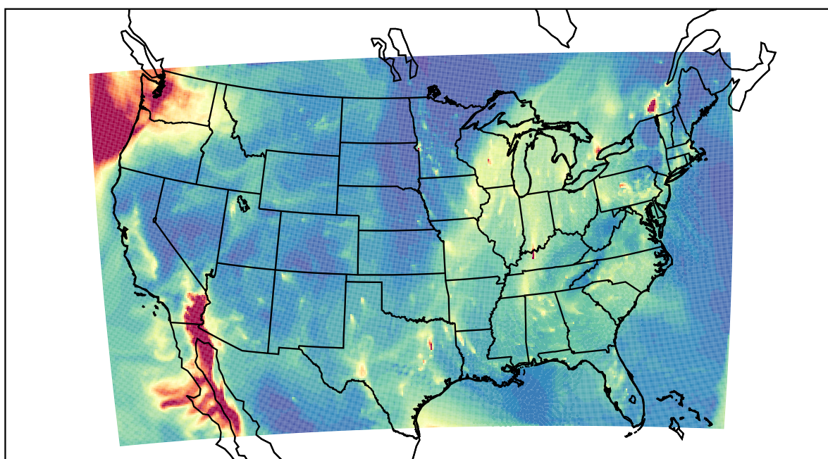
WRF 2020-12-19_14:00:00
