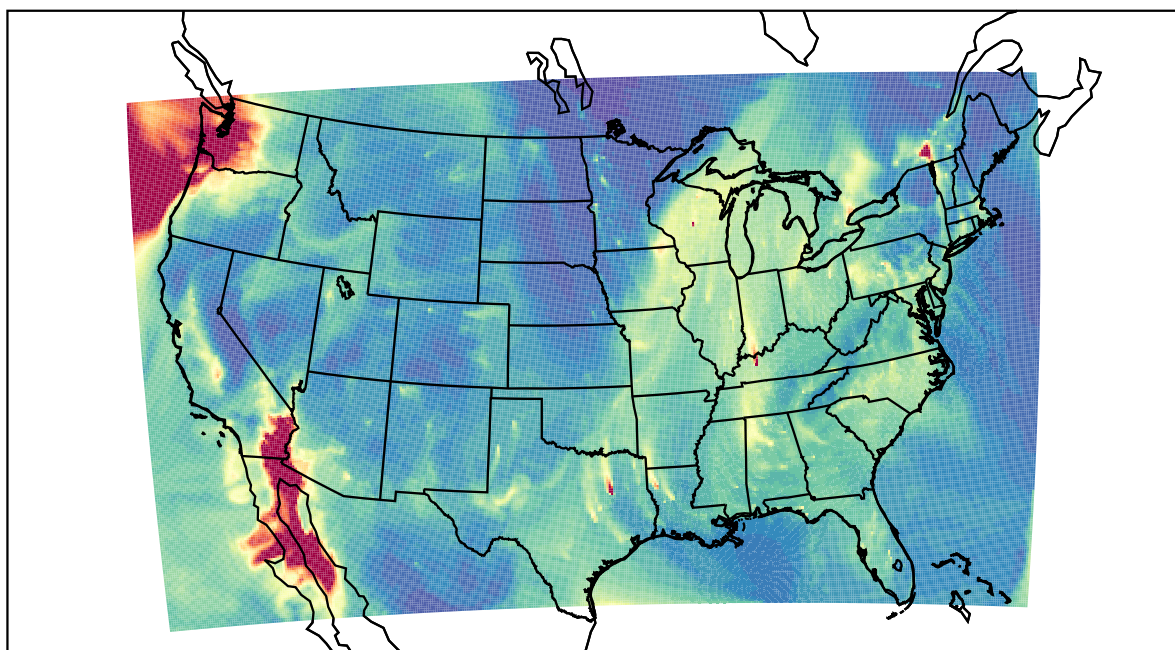
WRF 2020-12-19_10:00:00
