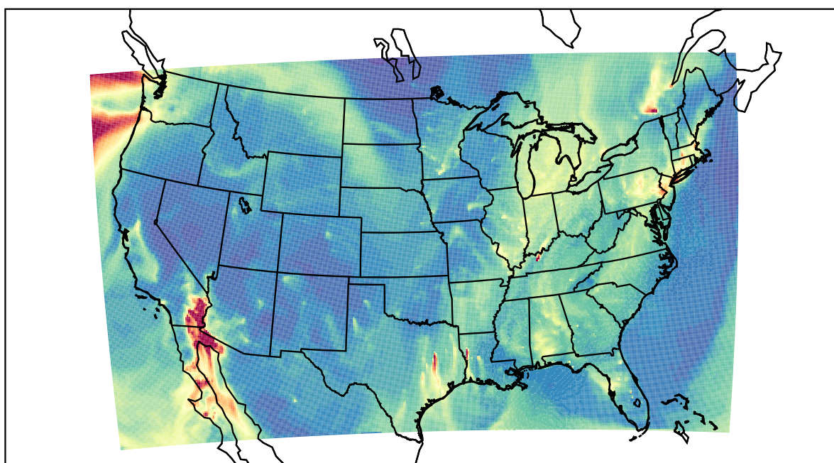
WRF 2020-12-20_09:00:00
