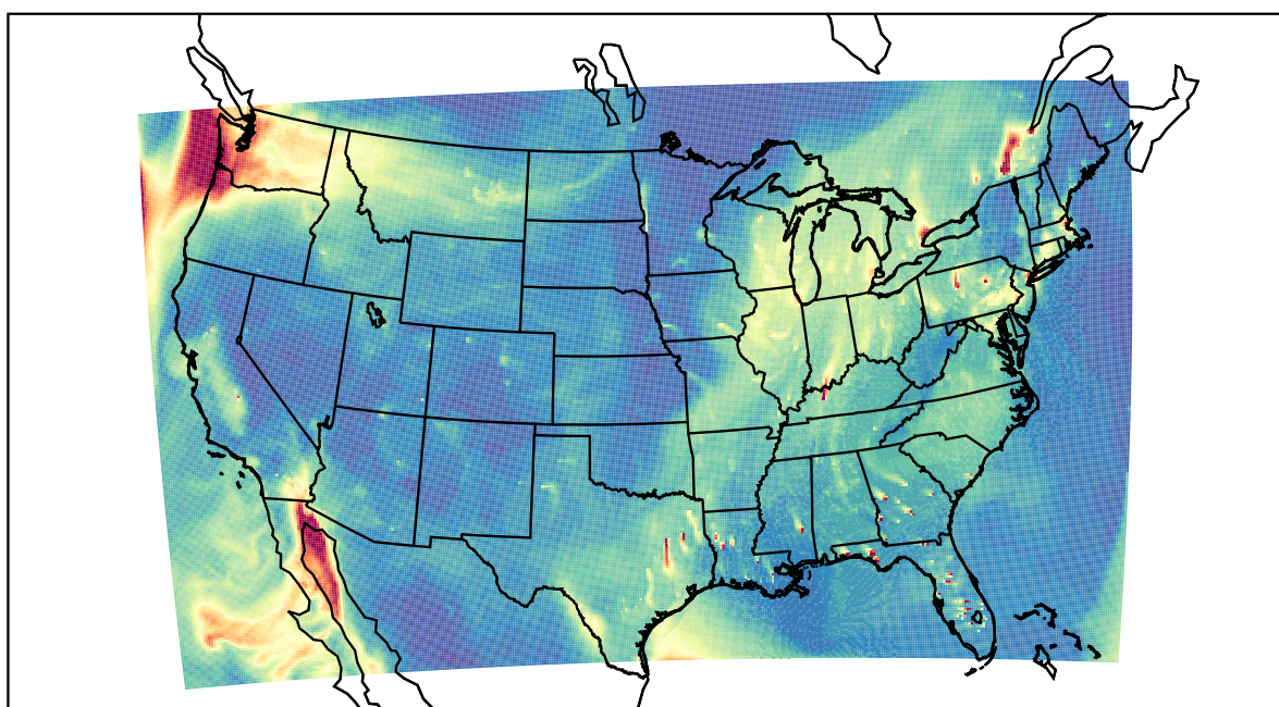
WRF 2020-12-19_21:00:00
