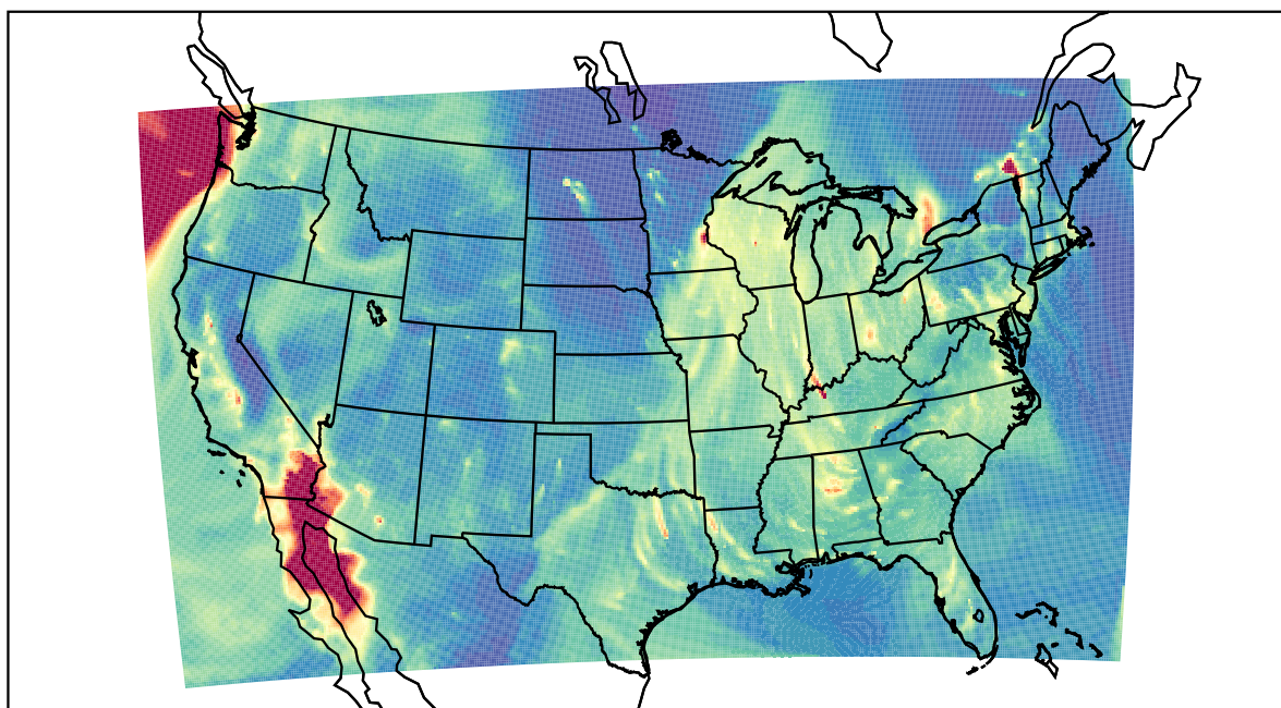
WRF 2020-12-19_05:00:00
