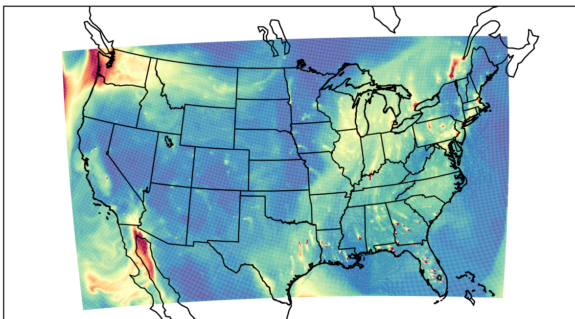
WRF 2020-12-19_22:00:00
