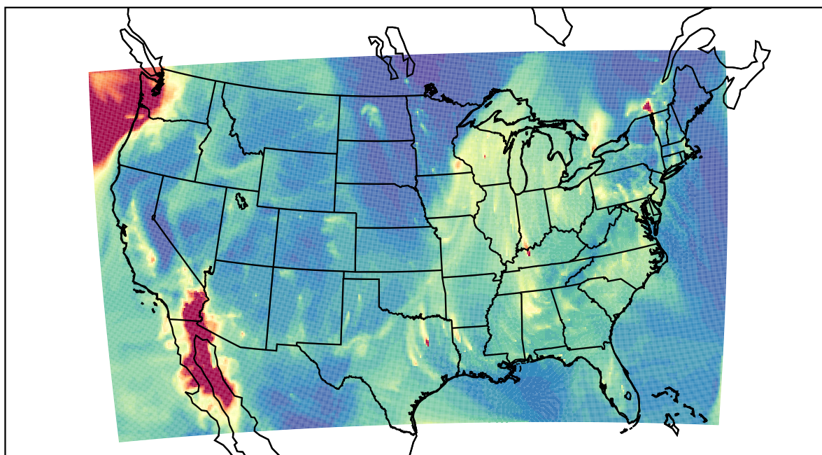
WRF 2020-12-19_08:00:00
