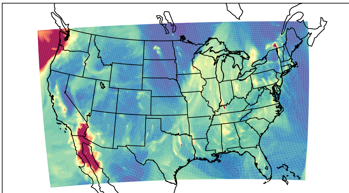
WRF 2020-12-19_07:00:00
