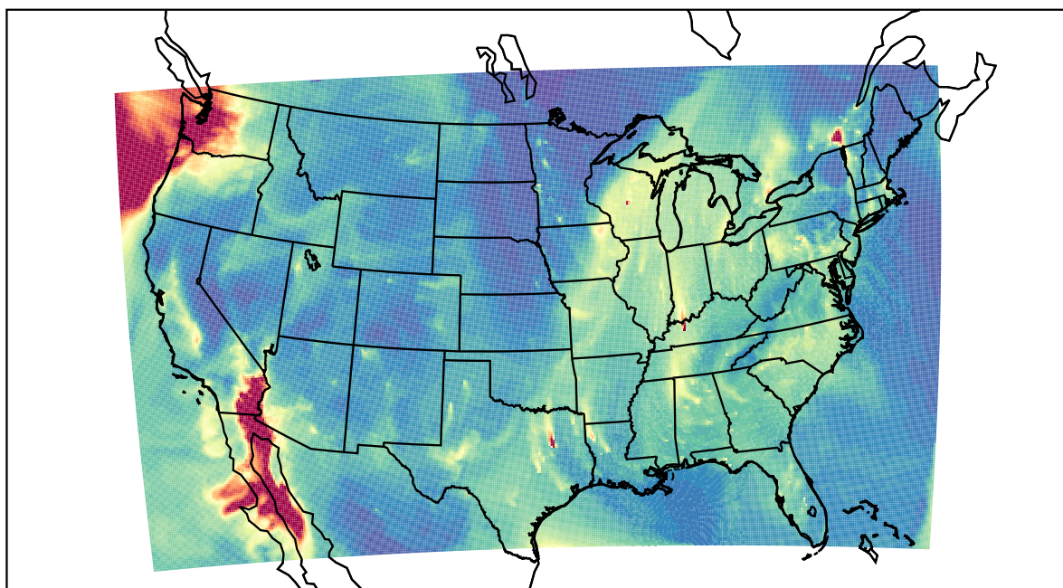
WRF 2020-12-19_11:00:00
