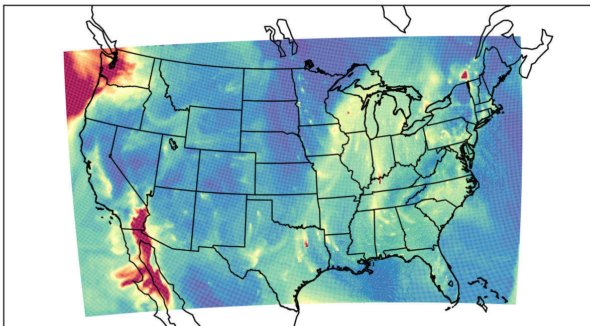
WRF 2020-12-19_12:00:00
