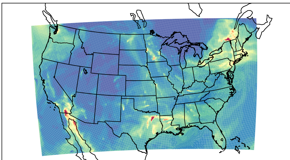
WRF 2020-12-22_09:00:00
