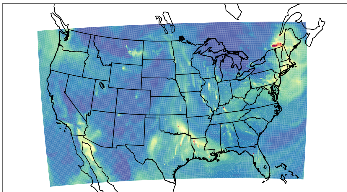
WRF 2020-12-22_21:00:00
