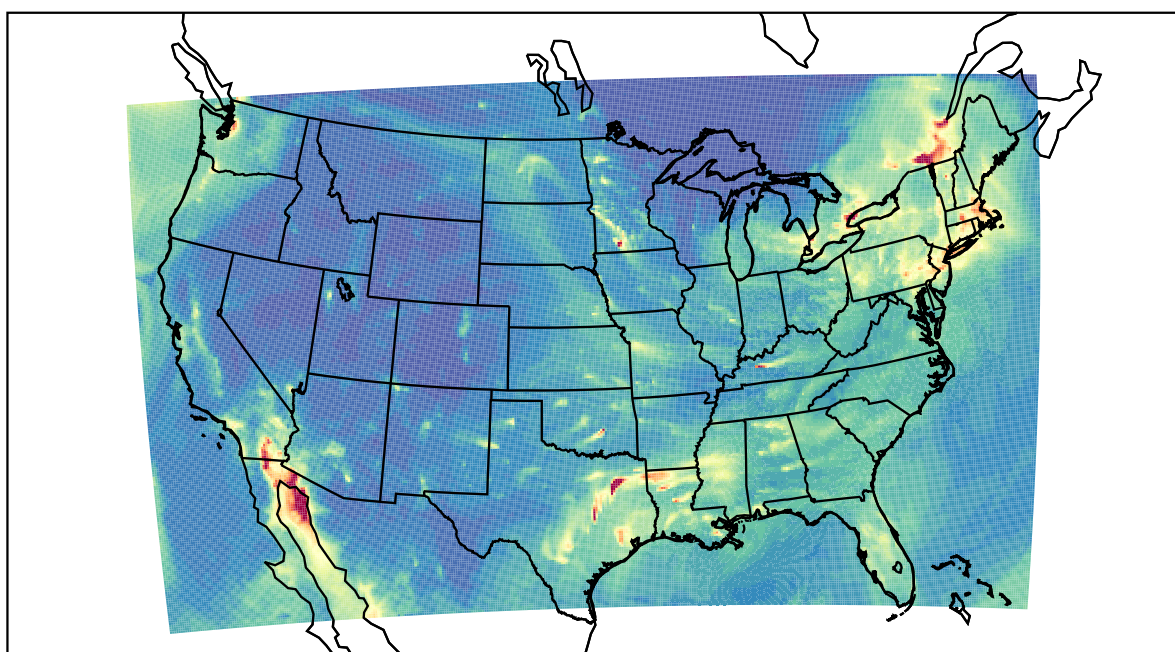
WRF 2020-12-22_04:00:00
