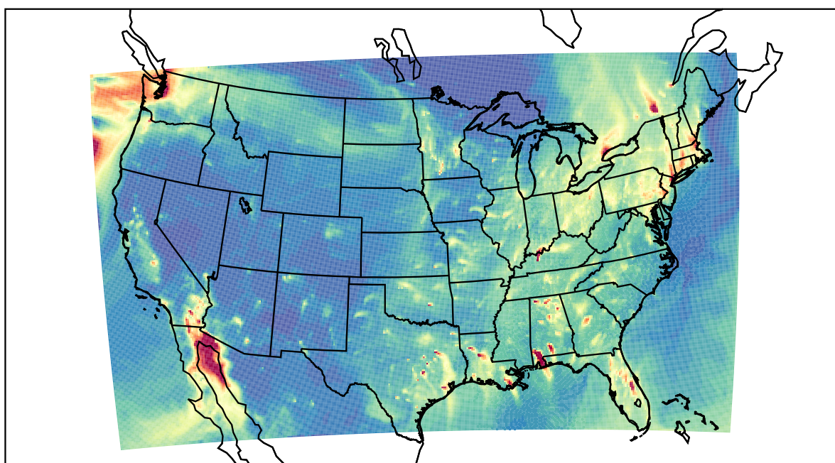
WRF 2020-12-21_02:00:00
