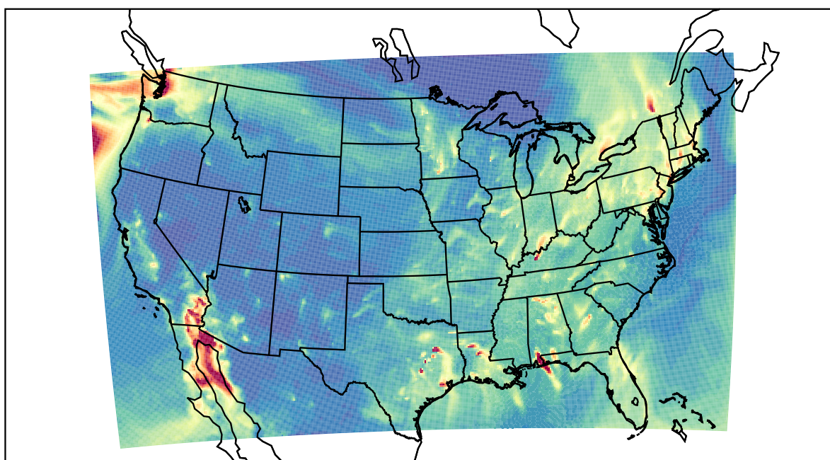
WRF 2020-12-21_05:00:00
