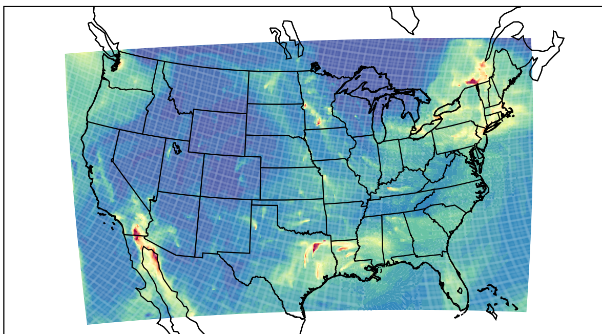
WRF 2020-12-22_08:00:00
