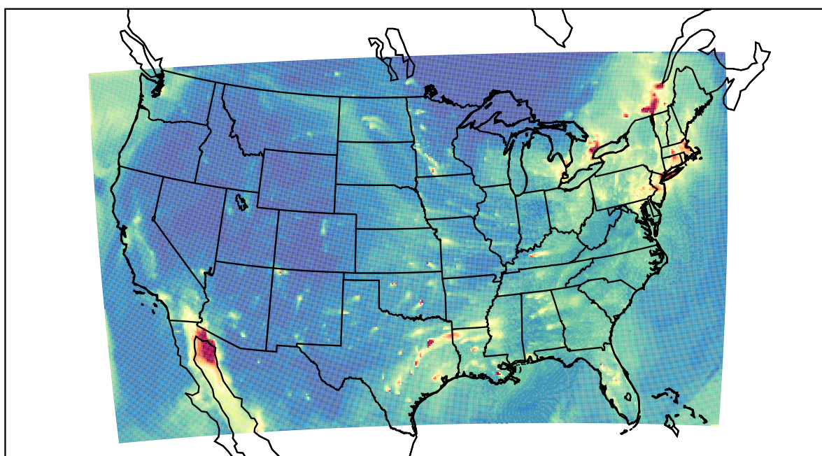
WRF 2020-12-22_01:00:00
