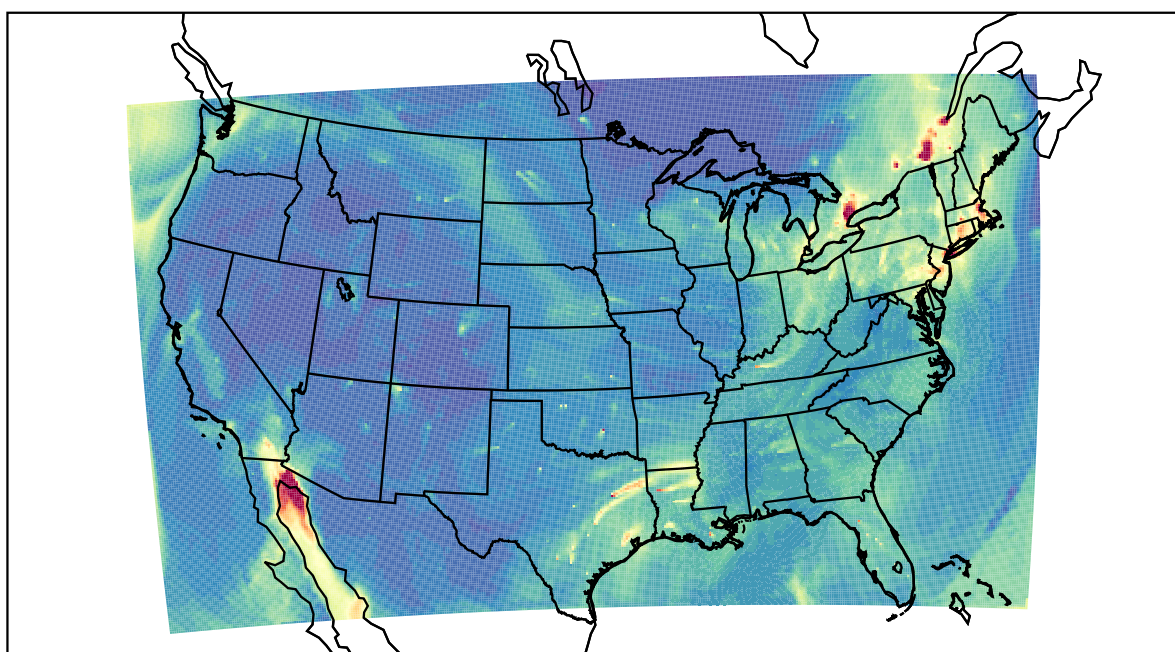
WRF 2020-12-21_21:00:00
