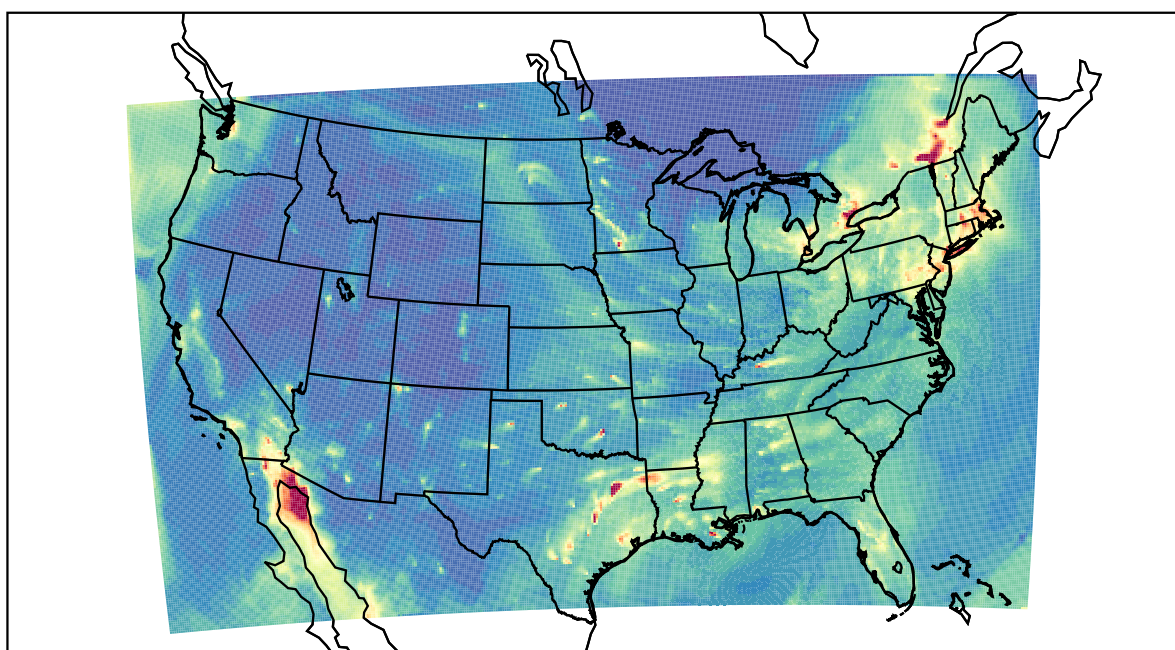
WRF 2020-12-22_02:00:00
