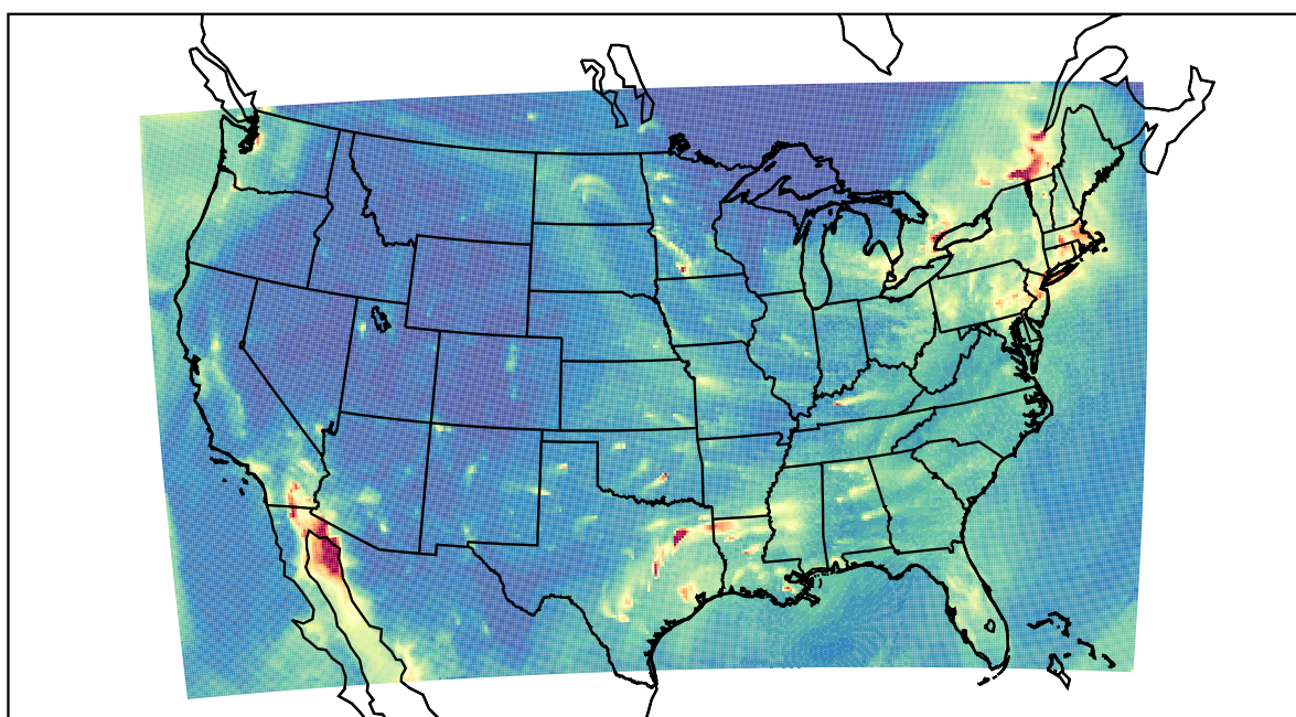
WRF 2020-12-22_03:00:00
