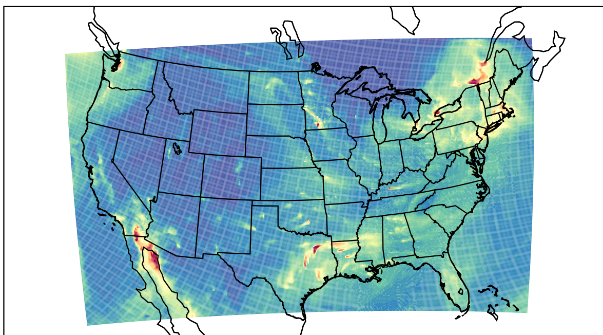
WRF 2020-12-22_05:00:00
