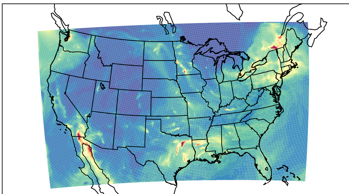
WRF 2020-12-22_07:00:00
