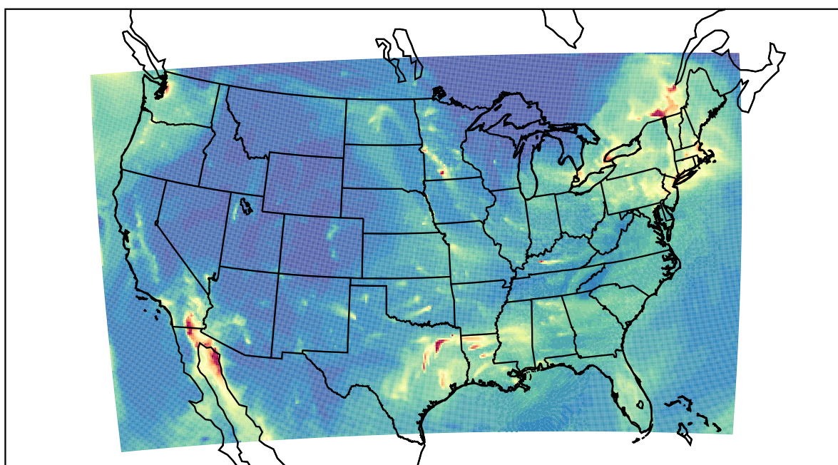
WRF 2020-12-22_06:00:00
