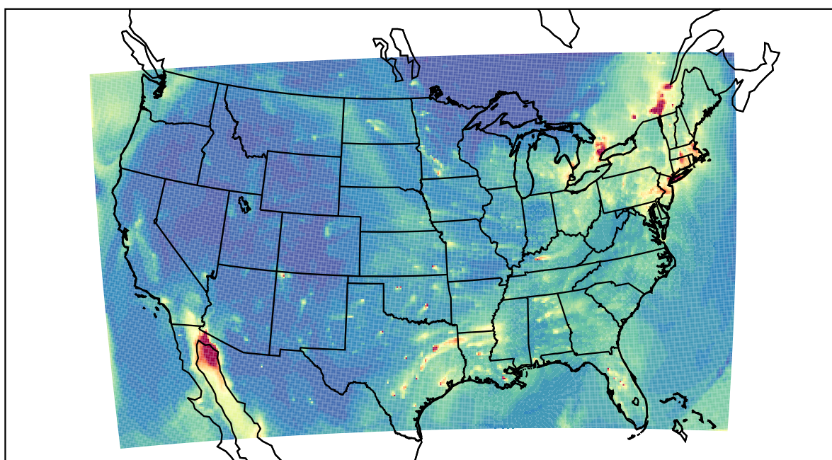
WRF 2020-12-22_00:00:00
