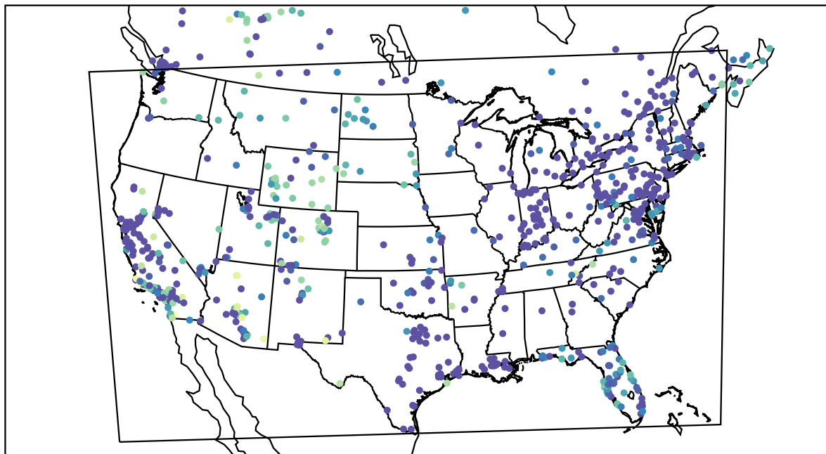
AirNOW (2020-12-21_12:00:00)
