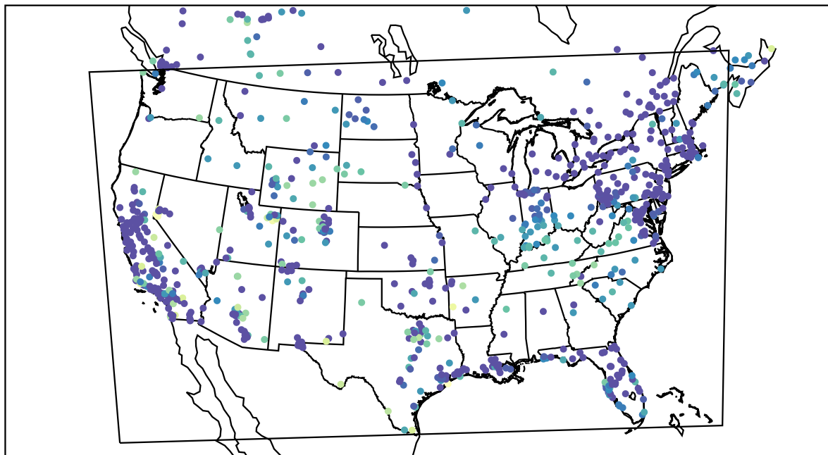
AirNOW (2020-12-22_05:00:00)
