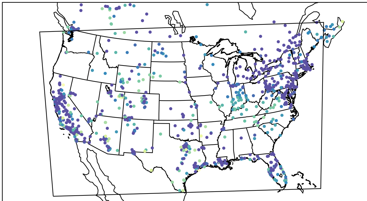
AirNOW (2020-12-22_03:00:00)
