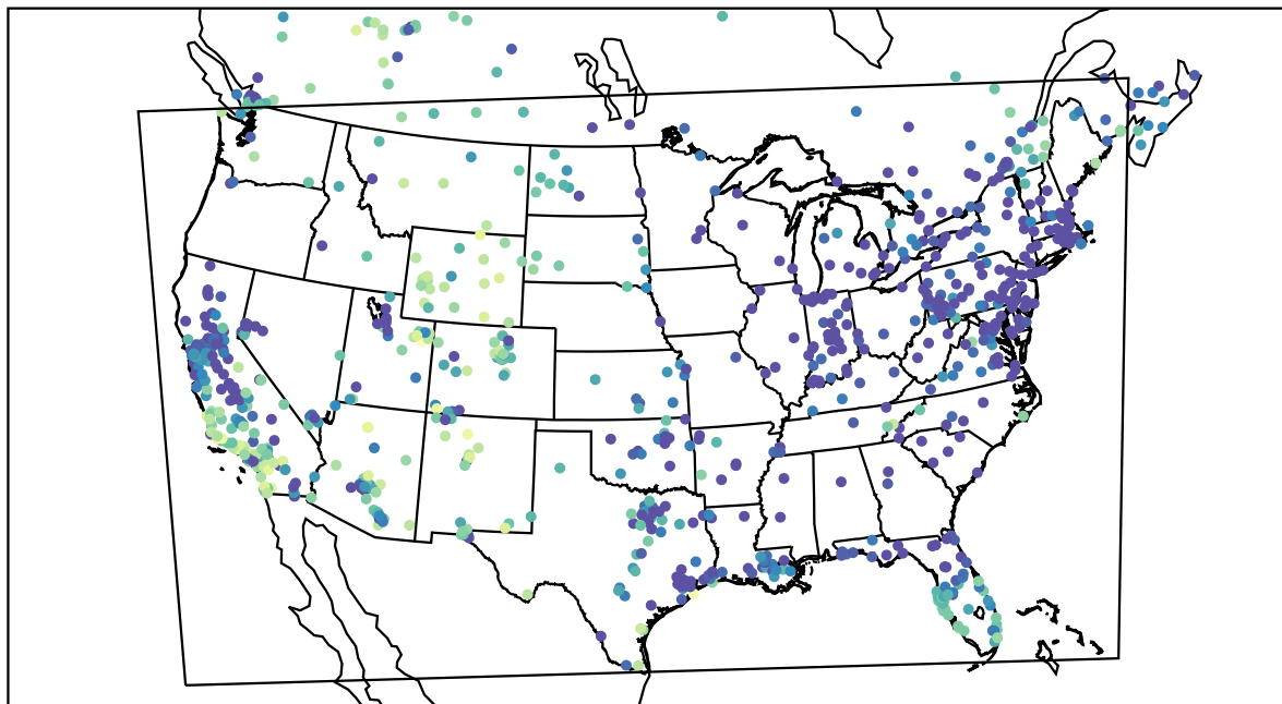
AirNOW (2020-12-21_00:00:00)
