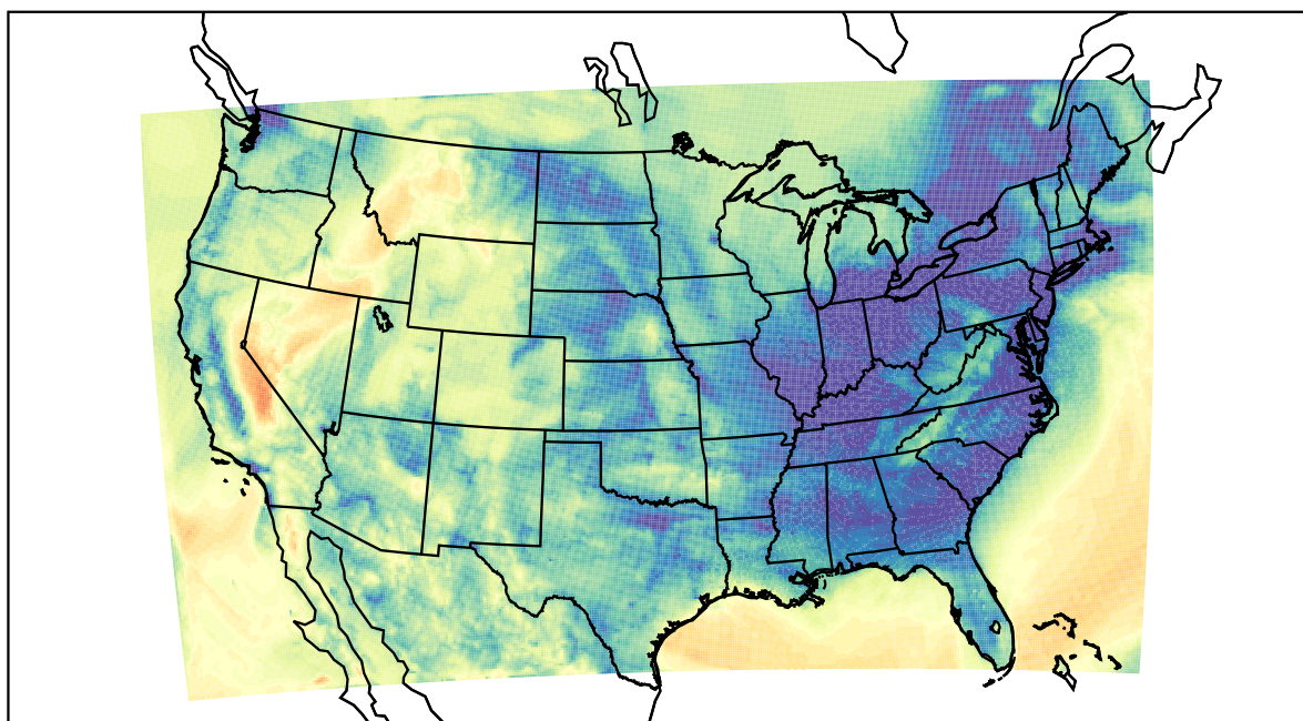
WRF (2020-12-22_09:00:00)
