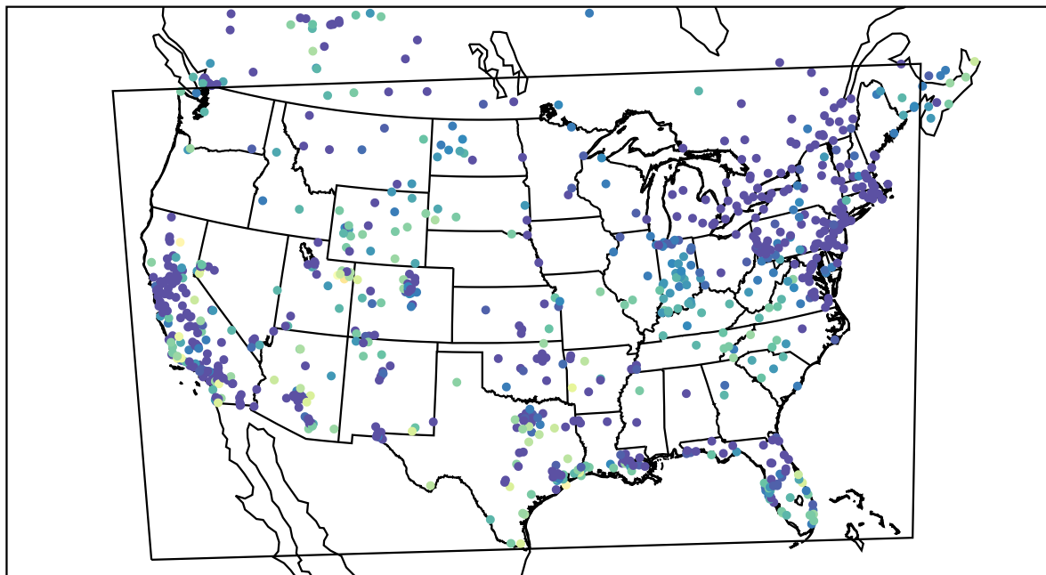
AirNOW (2020-12-22_01:00:00)
