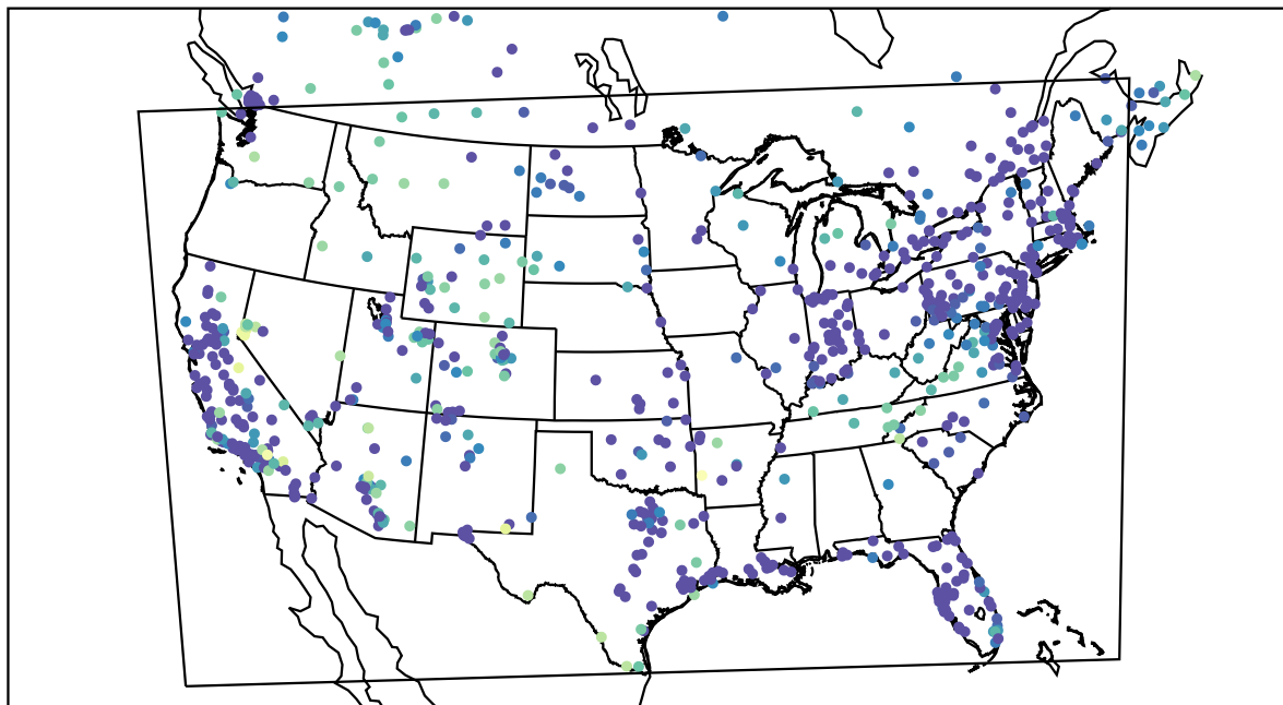
AirNOW (2020-12-22_11:00:00)
