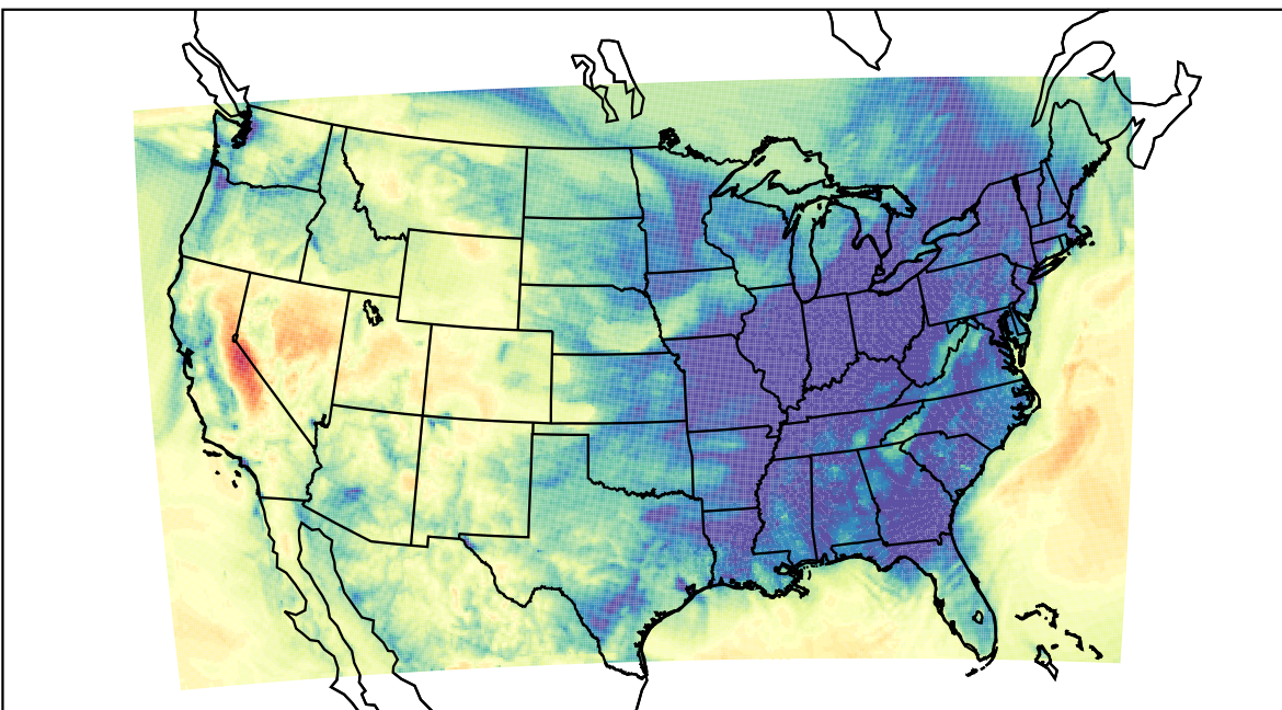
WRF (2020-12-21_07:00:00)
