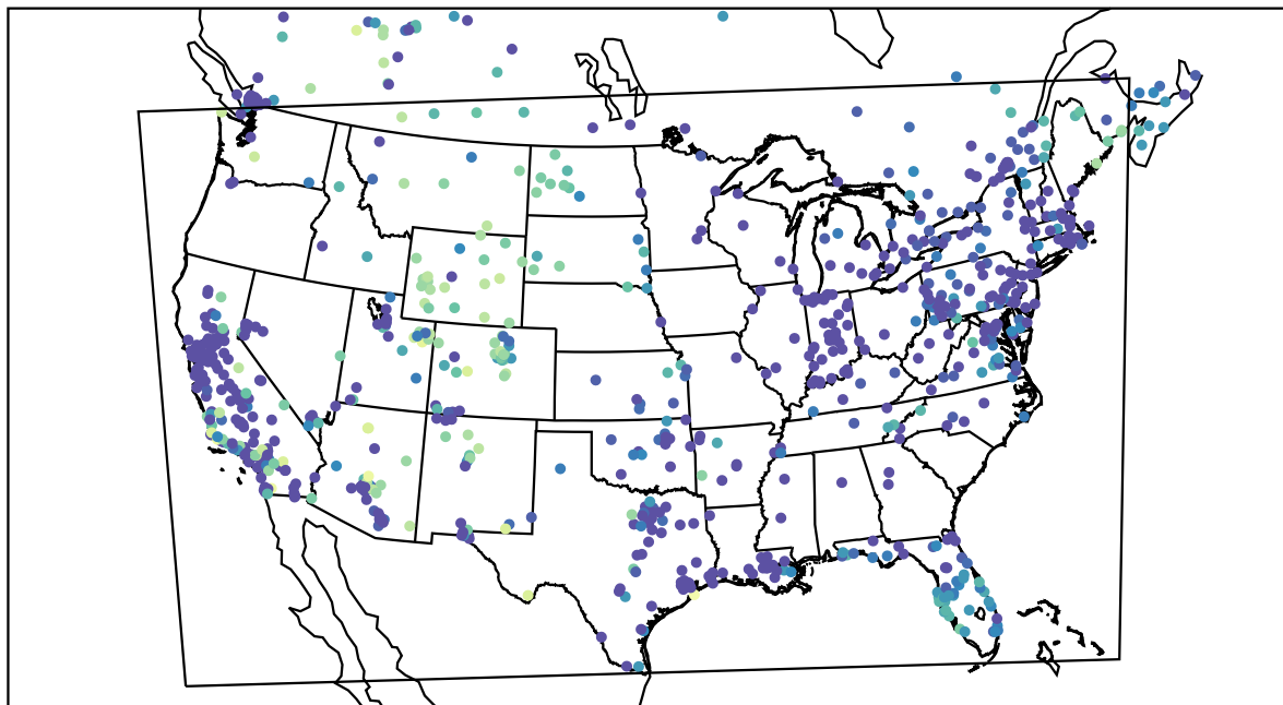
AirNOW (2020-12-21_04:00:00)
