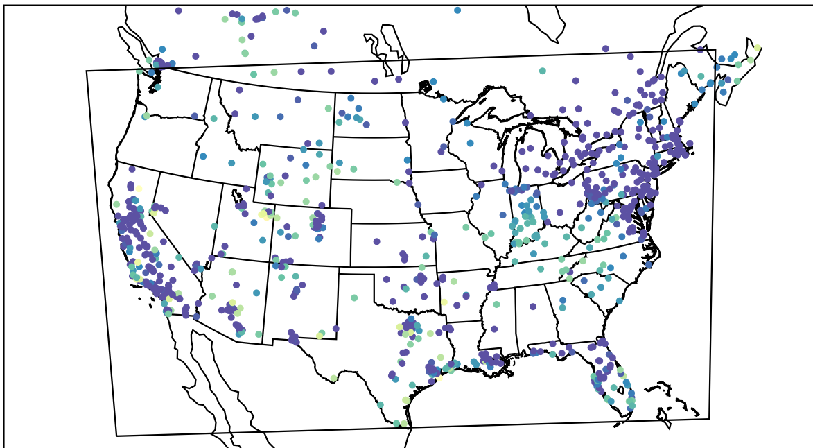
AirNOW (2020-12-22_02:00:00)
