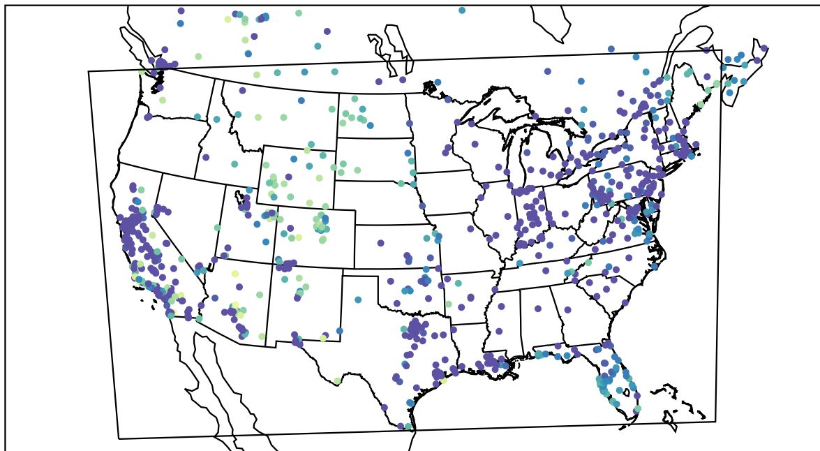
AirNOW (2020-12-21_05:00:00)
