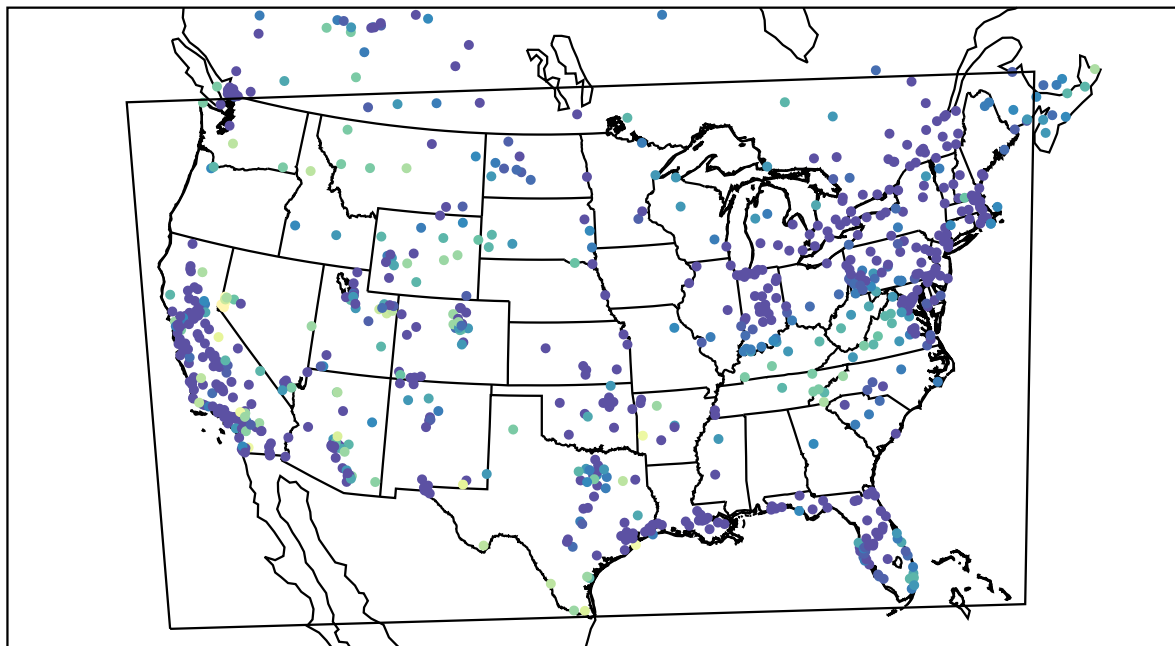
AirNOW (2020-12-22_09:00:00)
