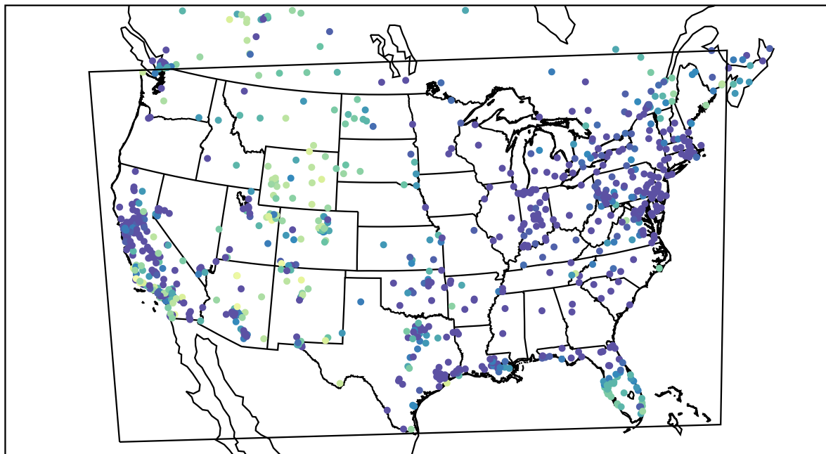
AirNOW (2020-12-21_01:00:00)
