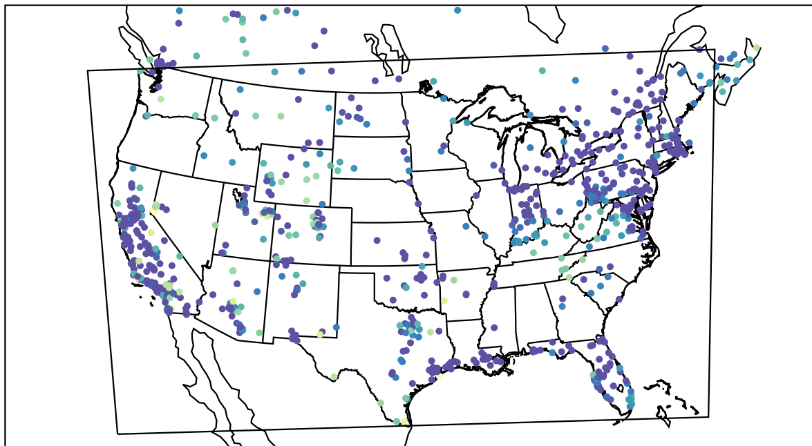
AirNOW (2020-12-22_08:00:00)
