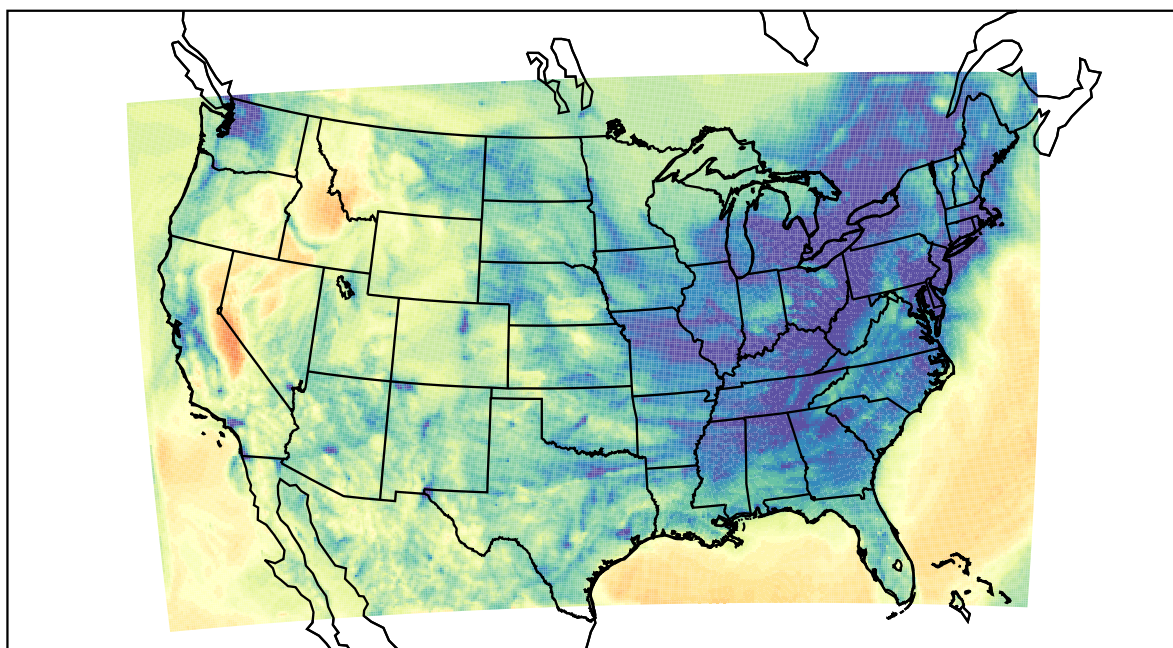
WRF (2020-12-22_03:00:00)
