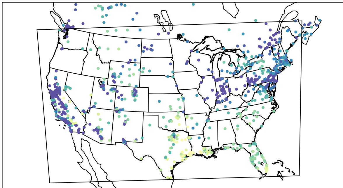
AirNOW (2020-12-22_17:00:00)
