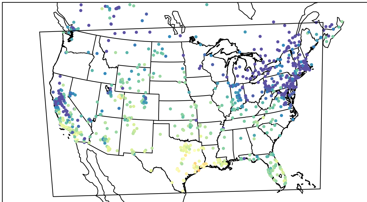
AirNOW (2020-12-21_21:00:00)
