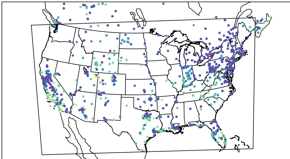
AirNOW (2020-12-22_00:00:00)
