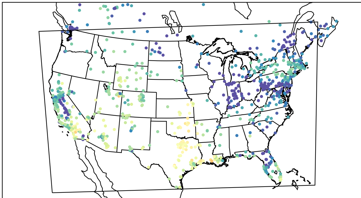
AirNOW (2020-12-22_22:00:00)
