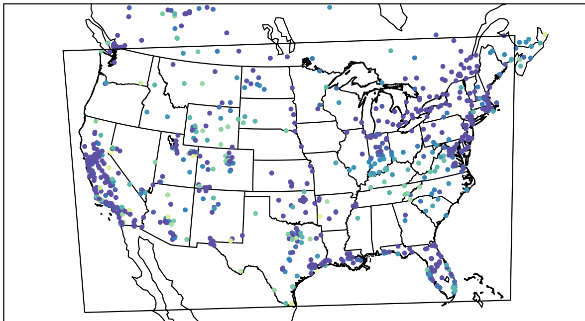
AirNOW (2020-12-22_06:00:00)
