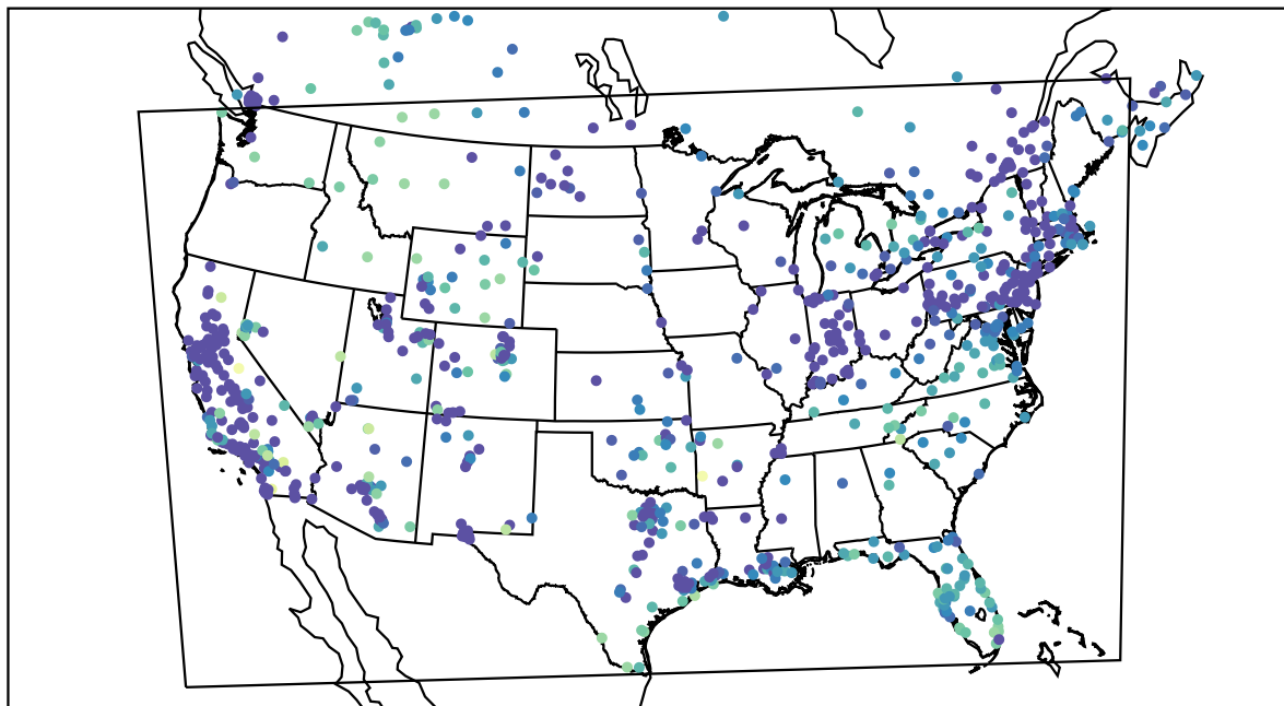
AirNOW (2020-12-22_15:00:00)
