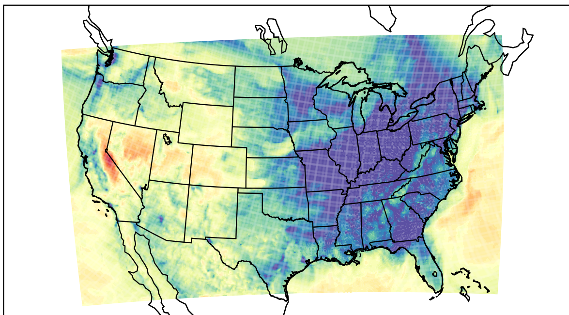
WRF (2020-12-21_05:00:00)
