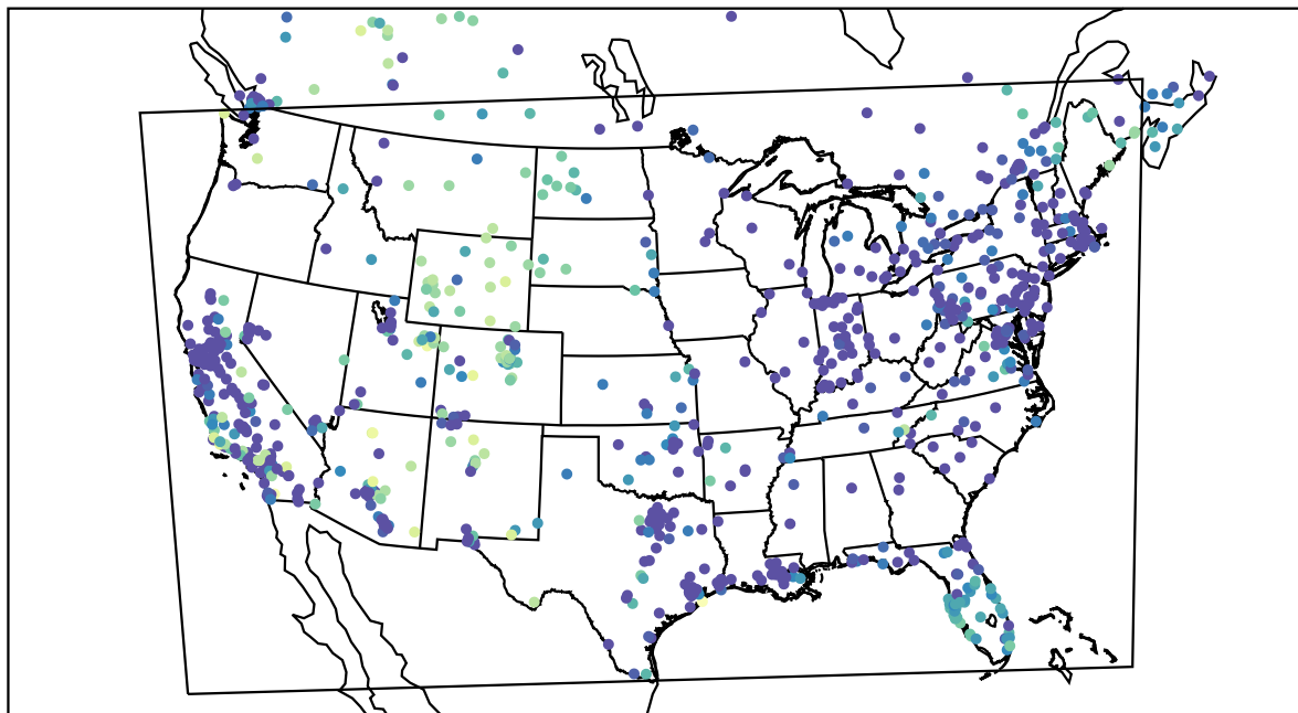
AirNOW (2020-12-21_03:00:00)
