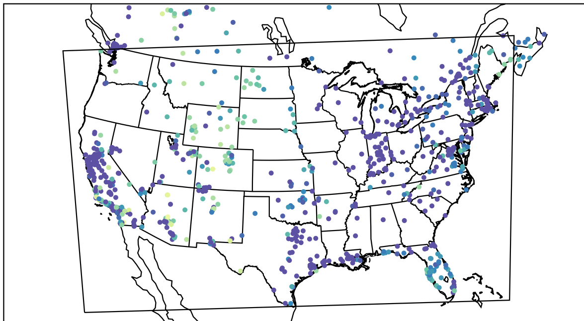
AirNOW (2020-12-21_06:00:00)
