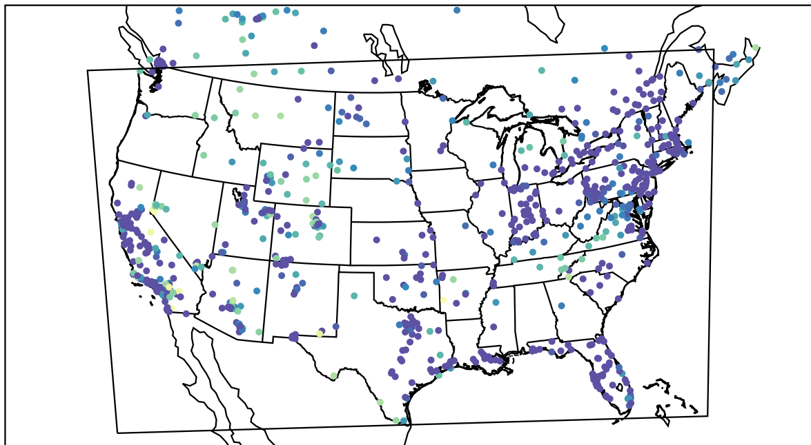
AirNOW (2020-12-22_12:00:00)
