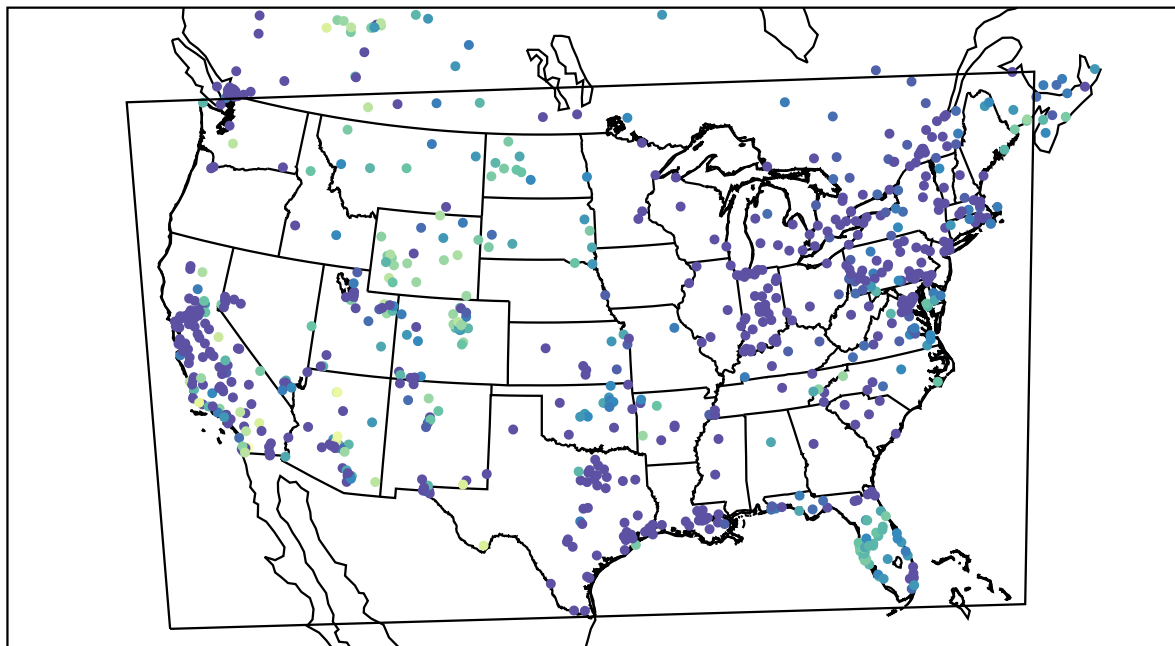
AirNOW (2020-12-21_09:00:00)
