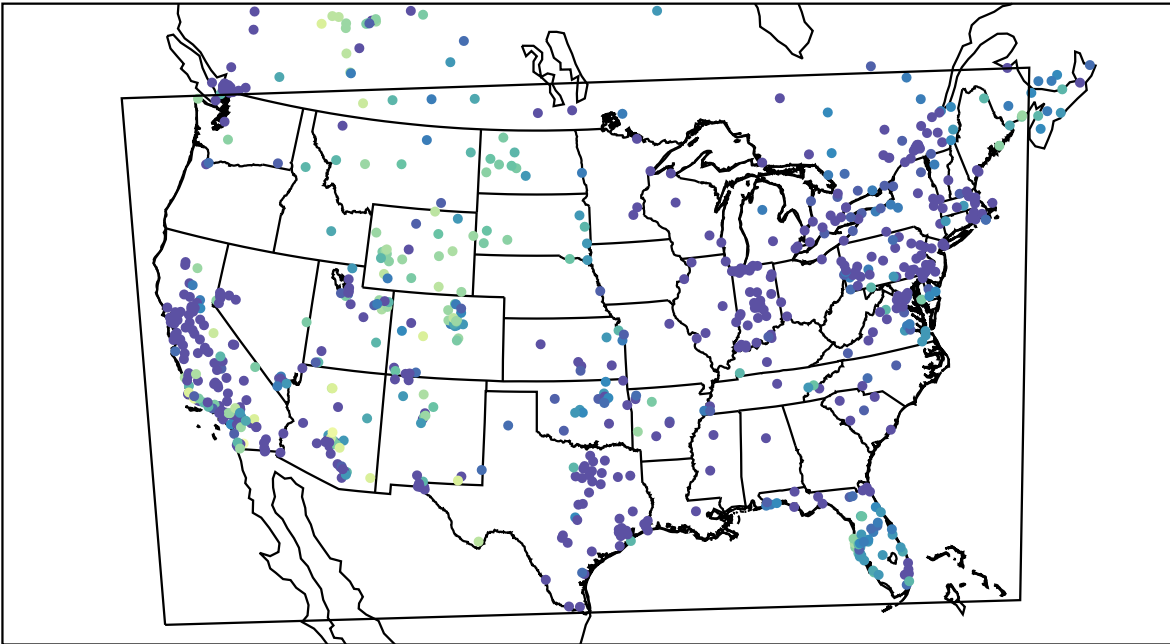
AirNOW (2020-12-21_07:00:00)
