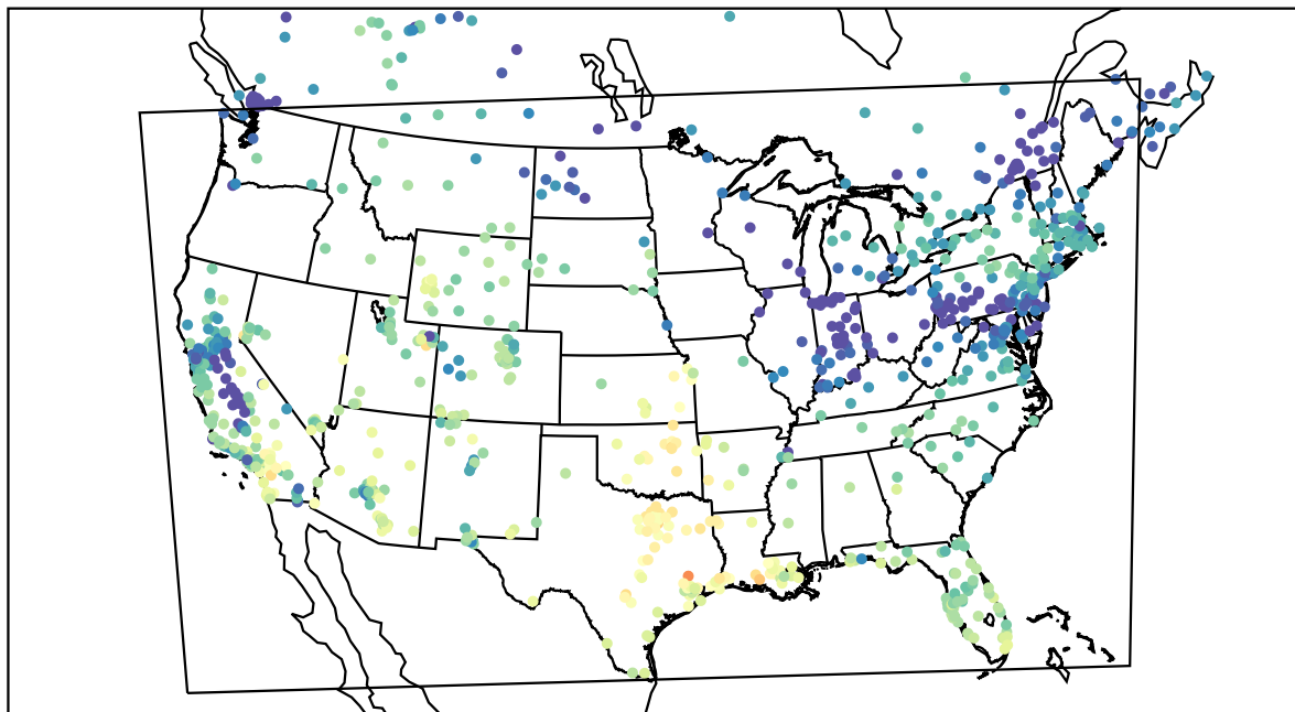
AirNOW (2020-12-22_21:00:00)
