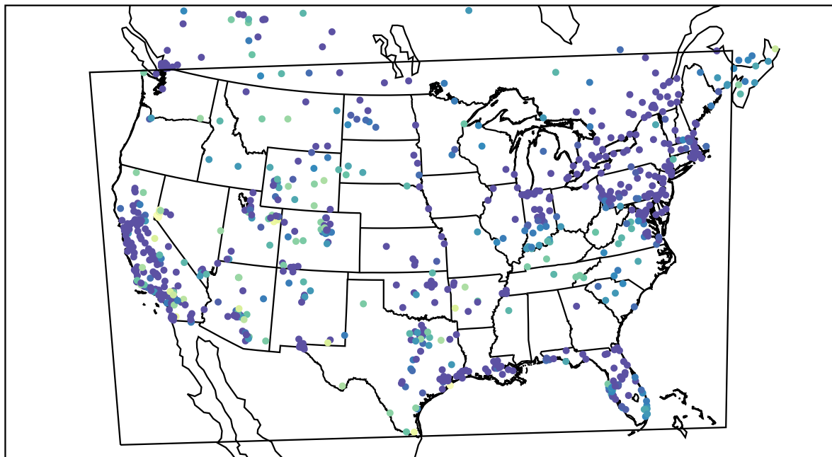
AirNOW (2020-12-22_07:00:00)
