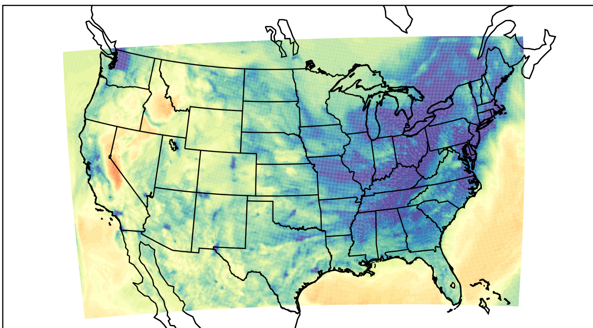
WRF (2020-12-22_02:00:00)
