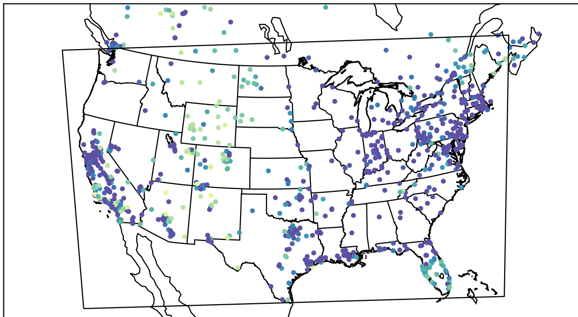
AirNOW (2020-12-21_02:00:00)
