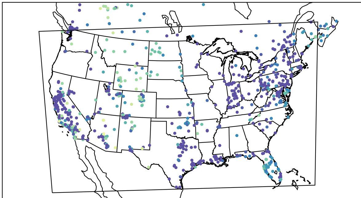
AirNOW (2020-12-21_08:00:00)
