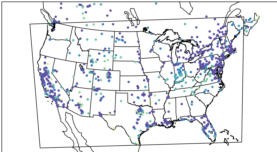
AirNOW (2020-12-22_04:00:00)
