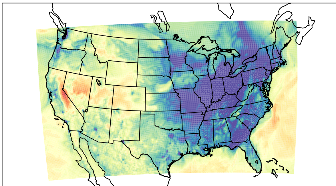
WRF (2020-12-21_03:00:00)
