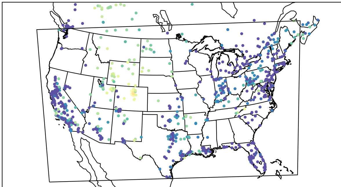
AirNOW (2021-01-14_08:00:00)
