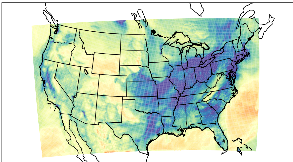
WRF (2021-01-14_05:00:00)
