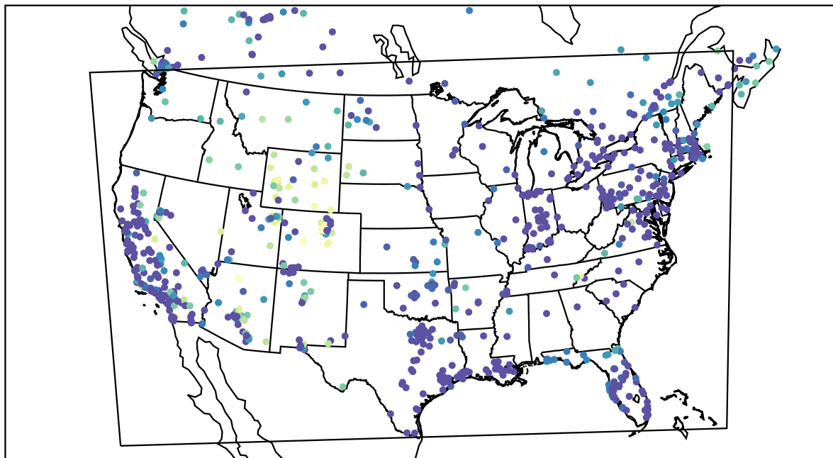
AirNOW (2021-01-13_07:00:00)
