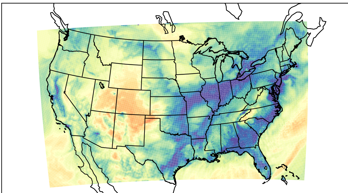
WRF (2021-01-13_09:00:00)
