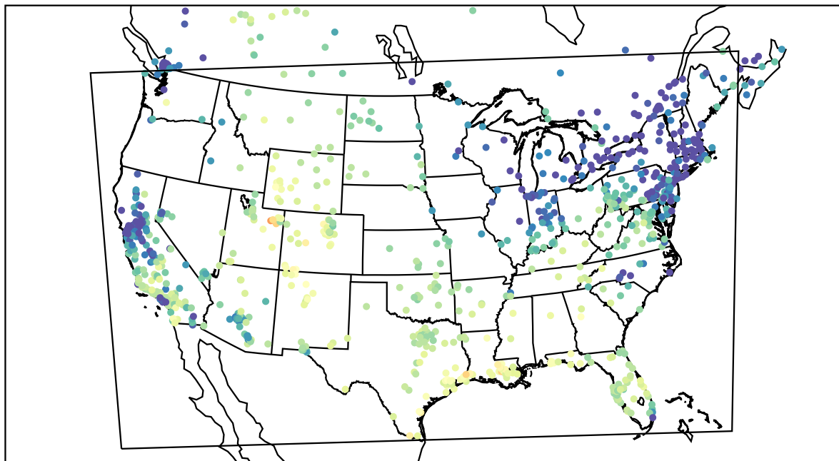
AirNOW (2021-01-14_21:00:00)
