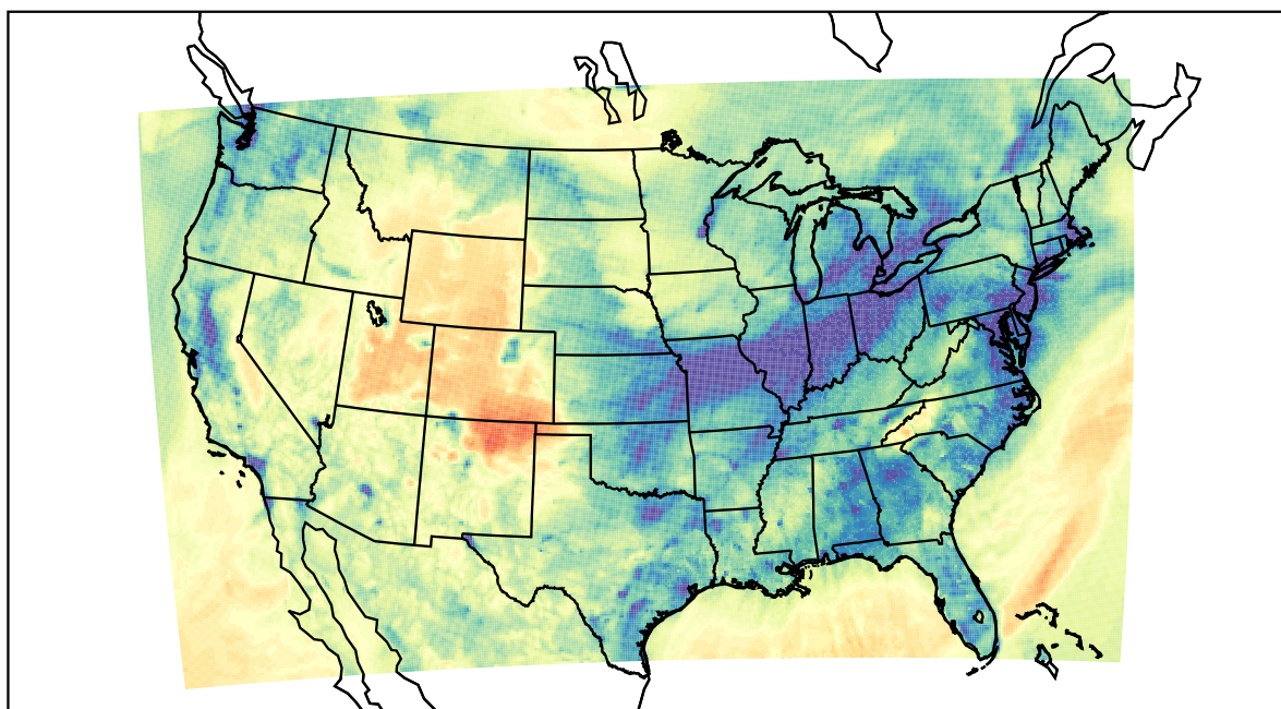
WRF (2021-01-13_02:00:00)
