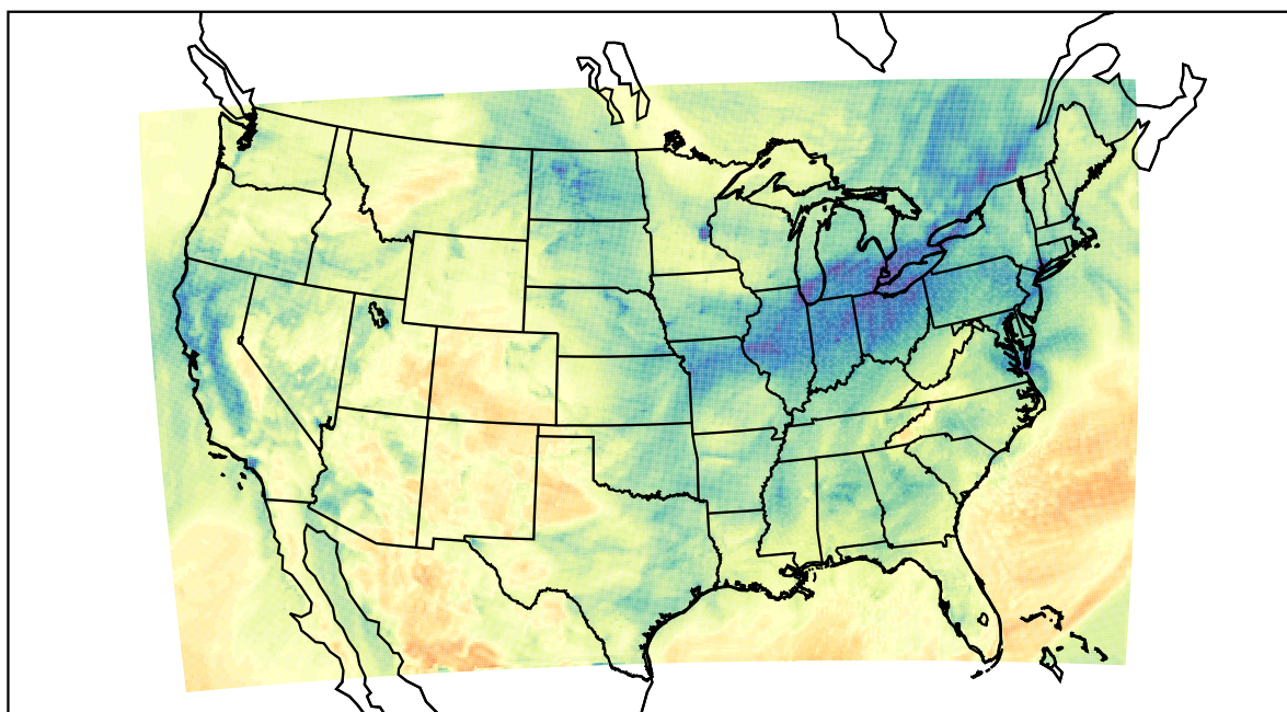
WRF (2021-01-13_19:00:00)
