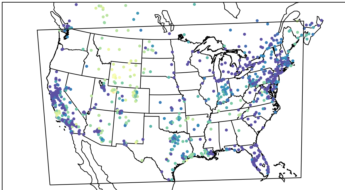
AirNOW (2021-01-14_01:00:00)
