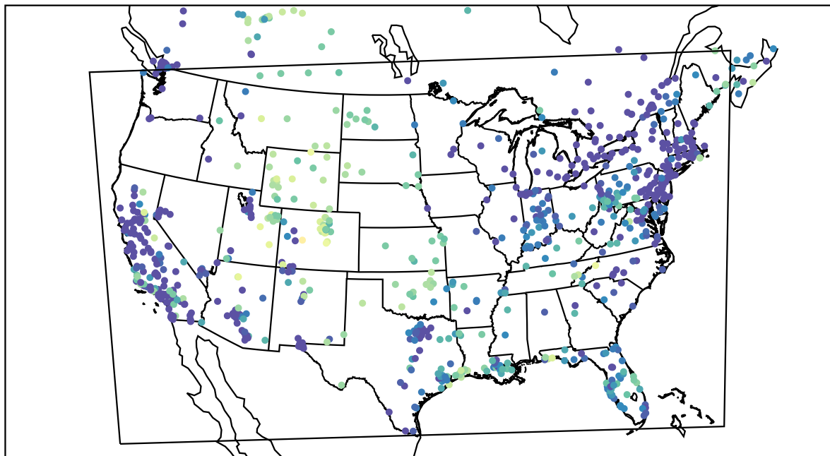
AirNOW (2021-01-14_15:00:00)
