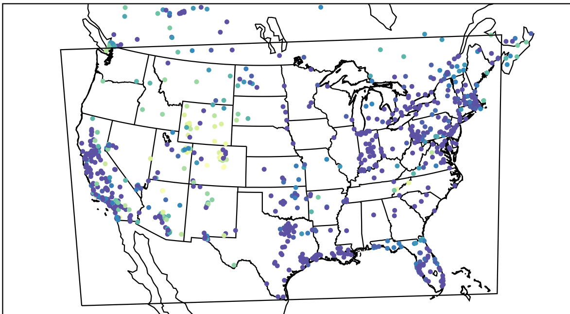
AirNOW (2021-01-13_08:00:00)
