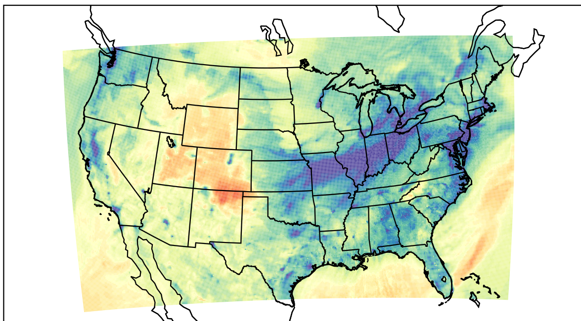
WRF (2021-01-13_01:00:00)
