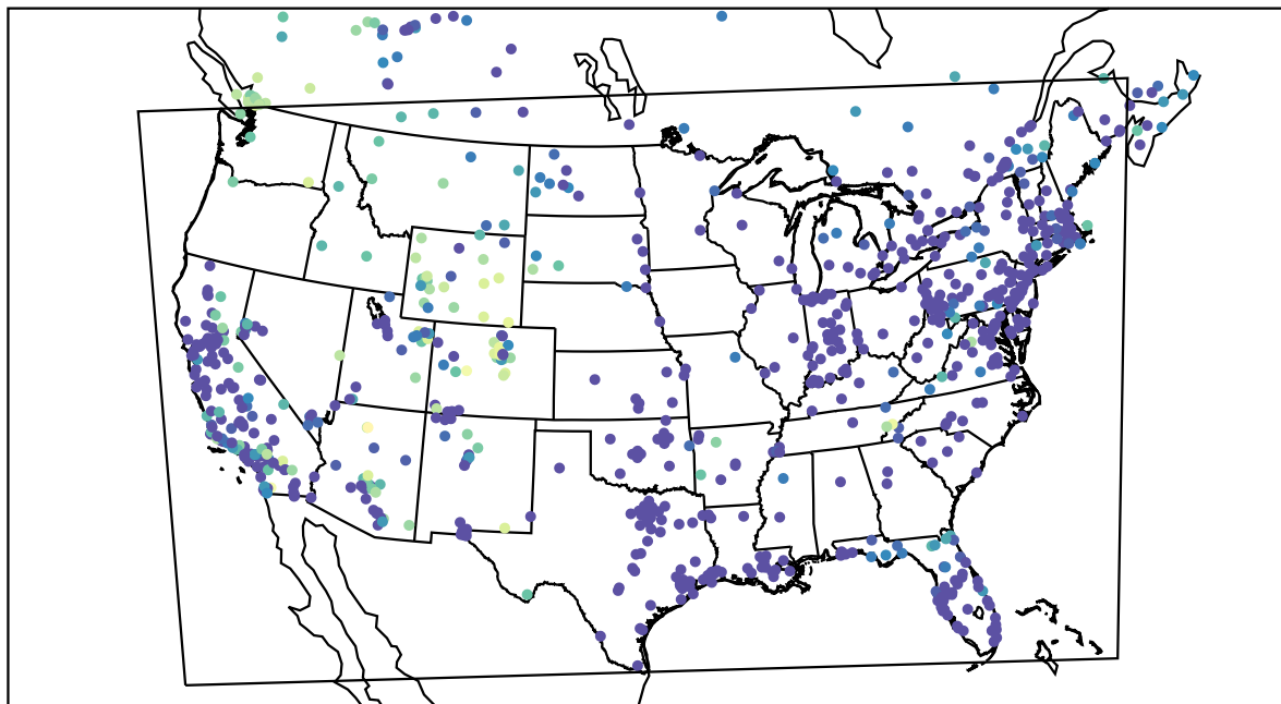
AirNOW (2021-01-13_13:00:00)
