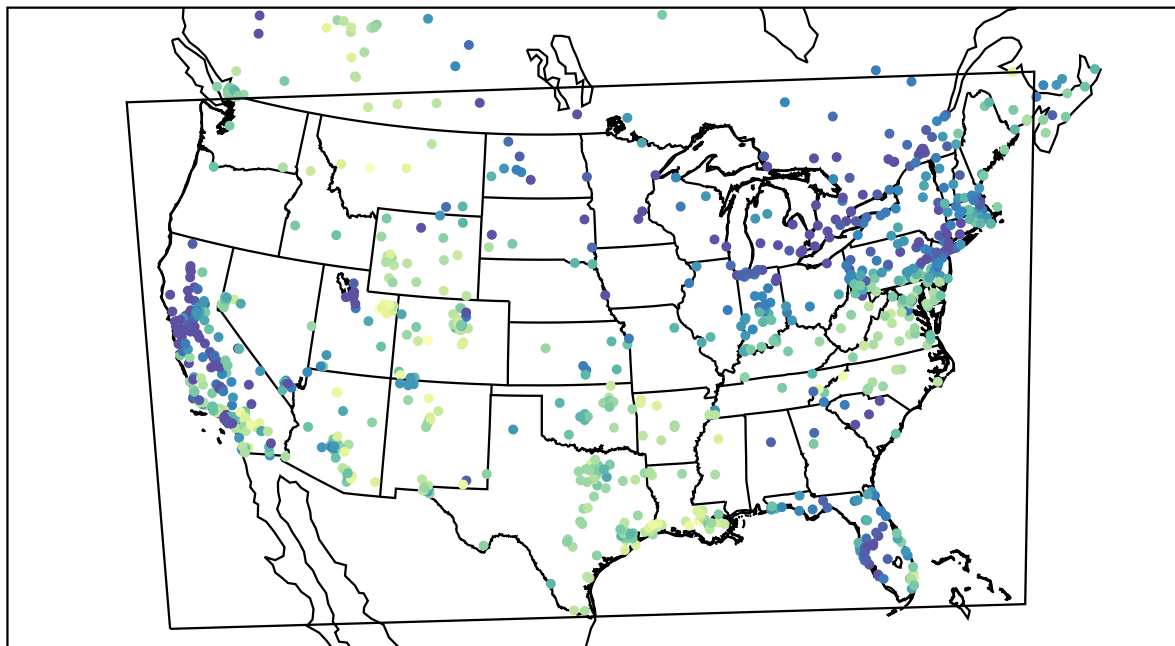
AirNOW (2021-01-13_19:00:00)
