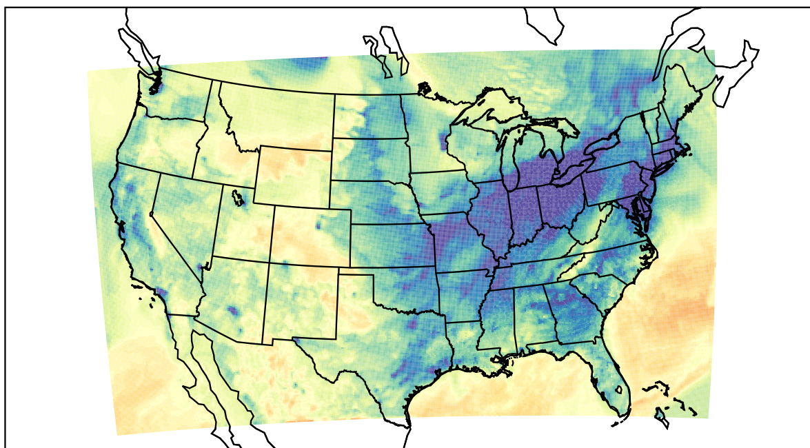
WRF (2021-01-14_01:00:00)
