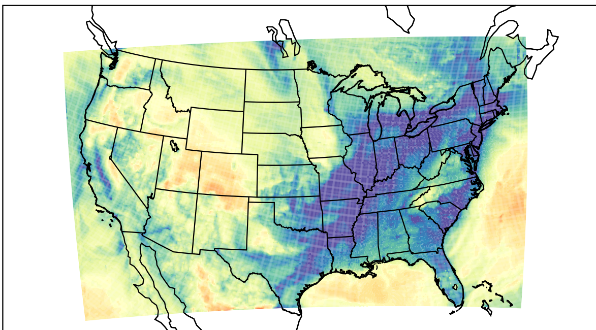
WRF (2021-01-14_13:00:00)
