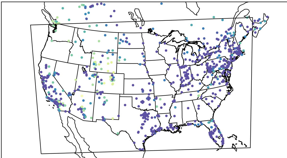
AirNOW (2021-01-13_12:00:00)
