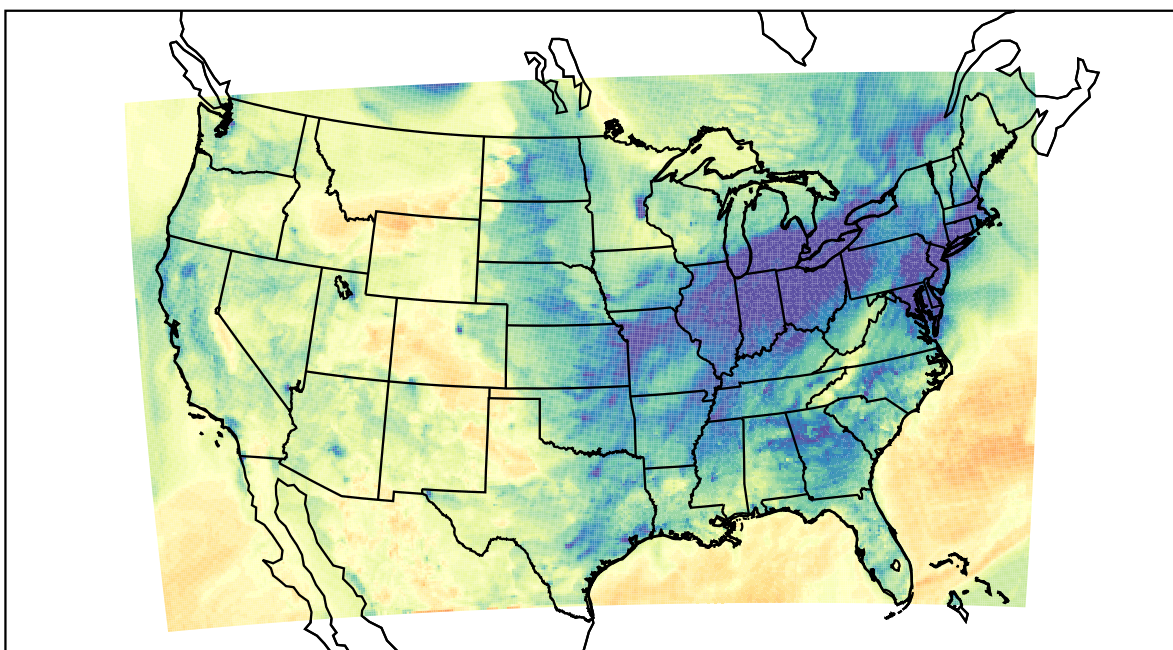
WRF (2021-01-14_00:00:00)
