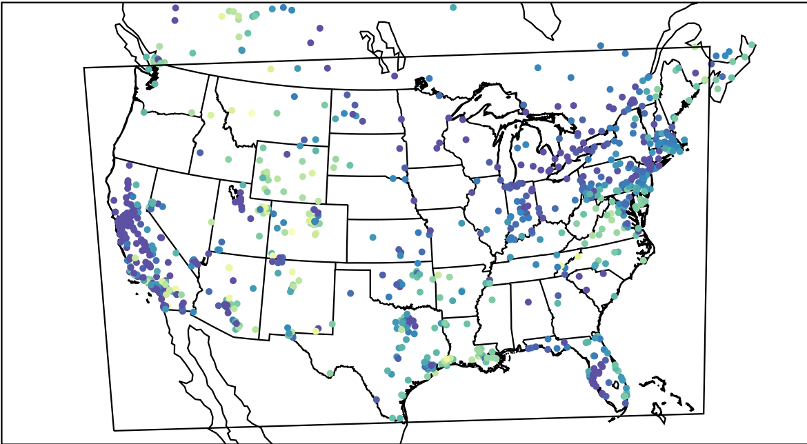
AirNOW (2021-01-13_17:00:00)
