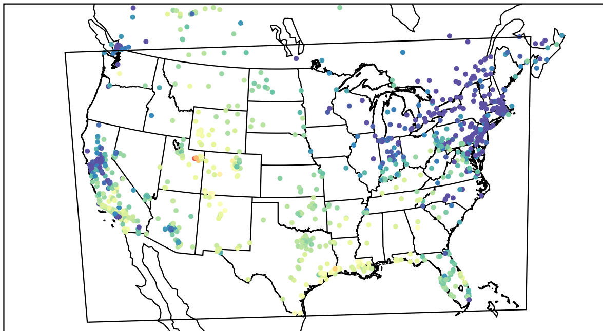
AirNOW (2021-01-14_22:00:00)
