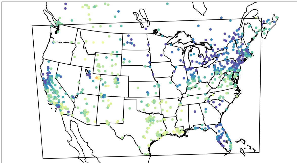
AirNOW (2021-01-13_21:00:00)
