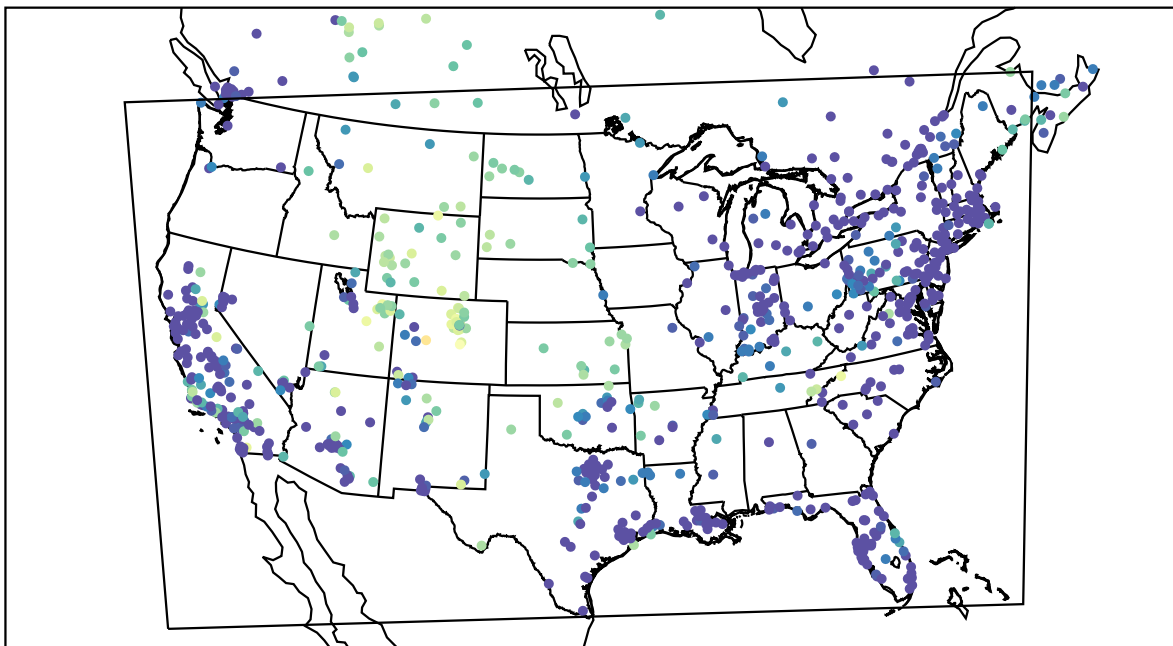
AirNOW (2021-01-14_13:00:00)
