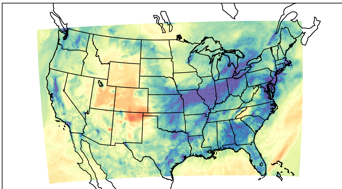
WRF (2021-01-13_04:00:00)
