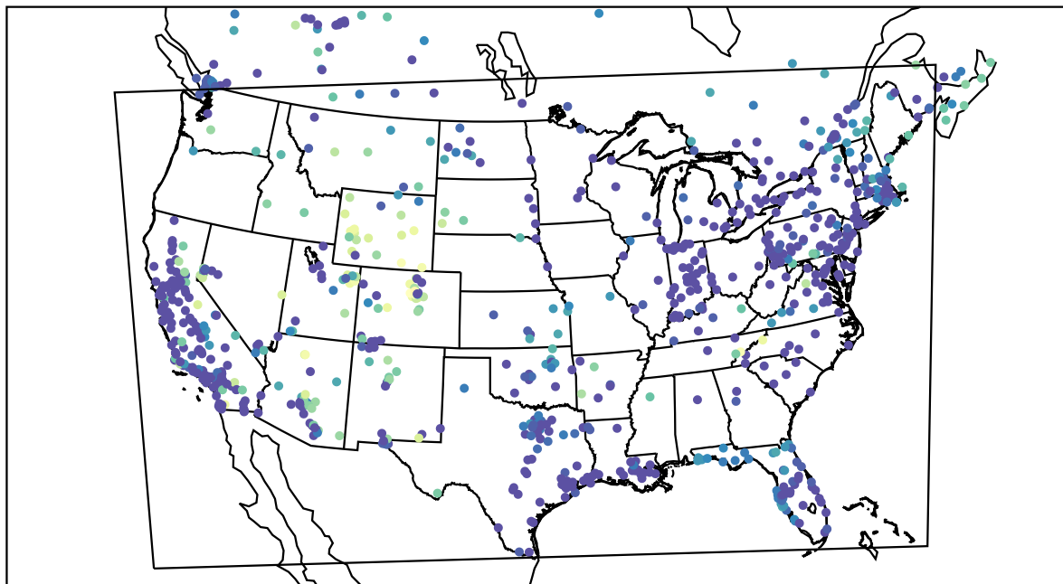
AirNOW (2021-01-13_05:00:00)
