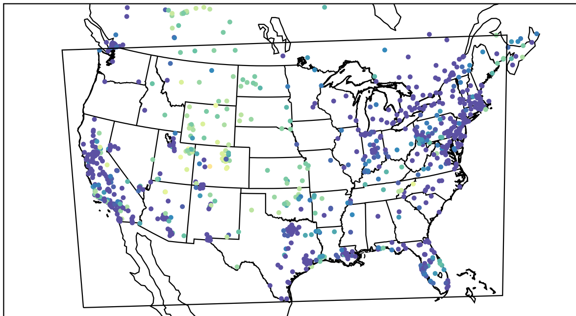
AirNOW (2021-01-14_14:00:00)
