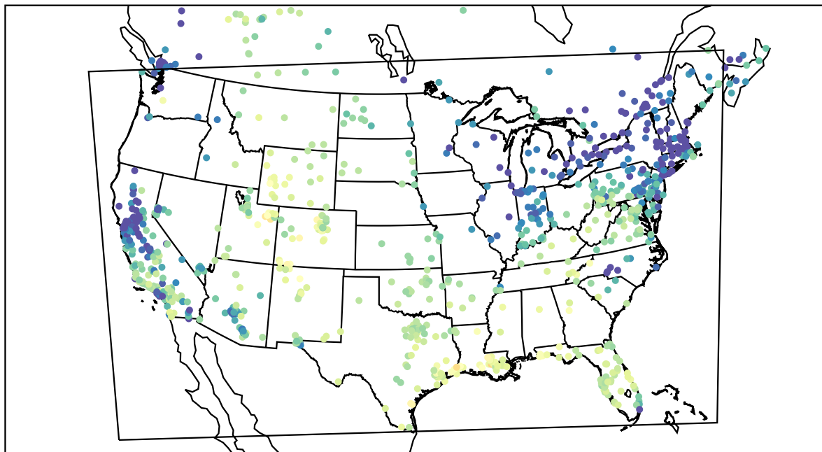
AirNOW (2021-01-14_20:00:00)
