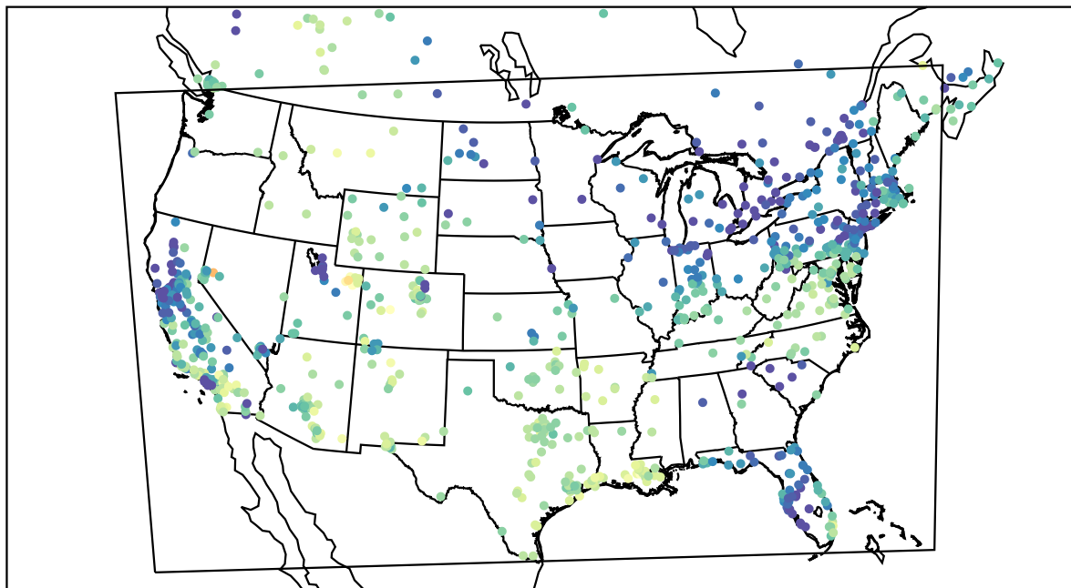
AirNOW (2021-01-13_20:00:00)
