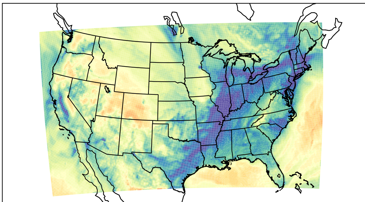
WRF (2021-01-14_15:00:00)
