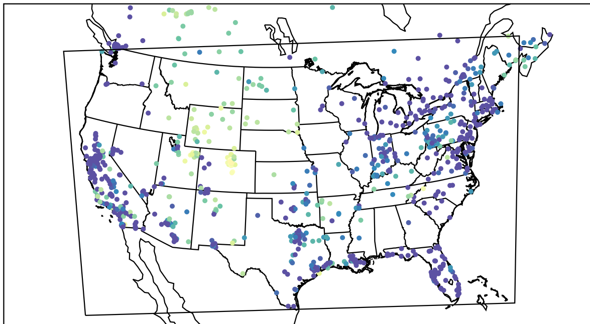
AirNOW (2021-01-14_09:00:00)
