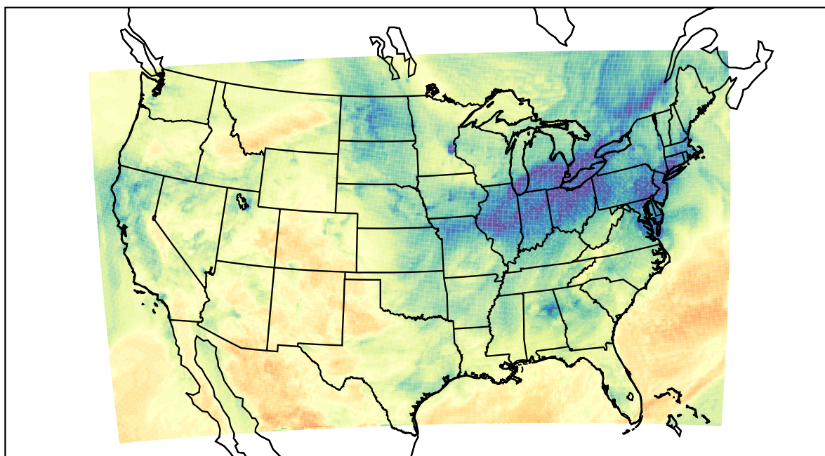
WRF (2021-01-13_21:00:00)
