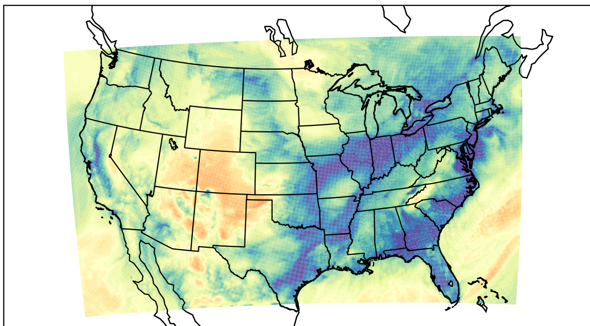
WRF (2021-01-13_11:00:00)
