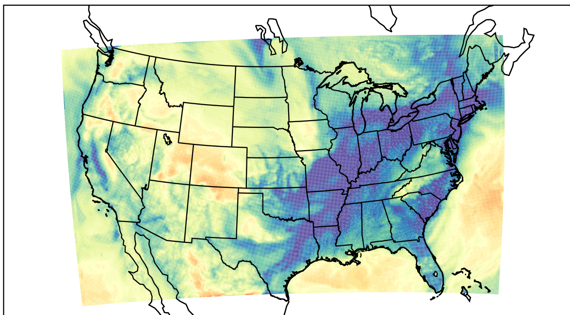
WRF (2021-01-14_12:00:00)
