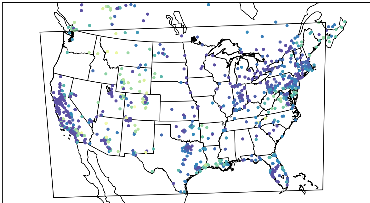
AirNOW (2021-01-13_16:00:00)
