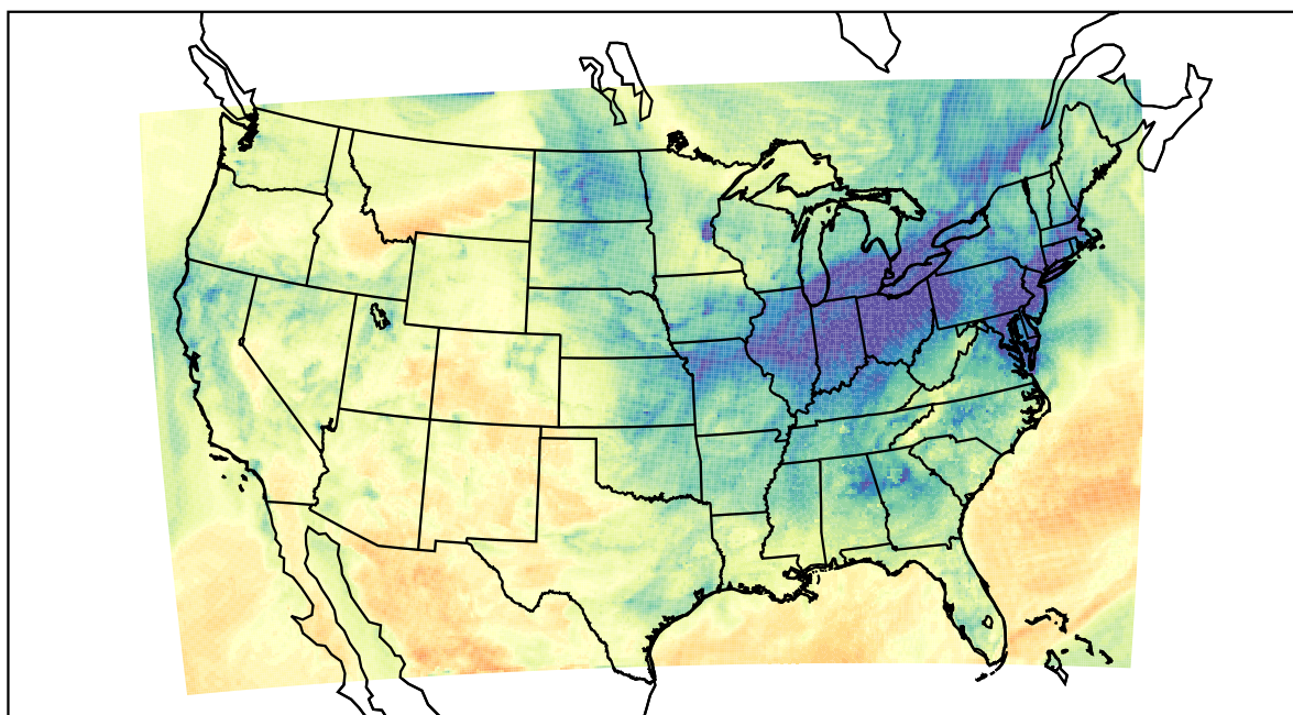
WRF (2021-01-13_22:00:00)
