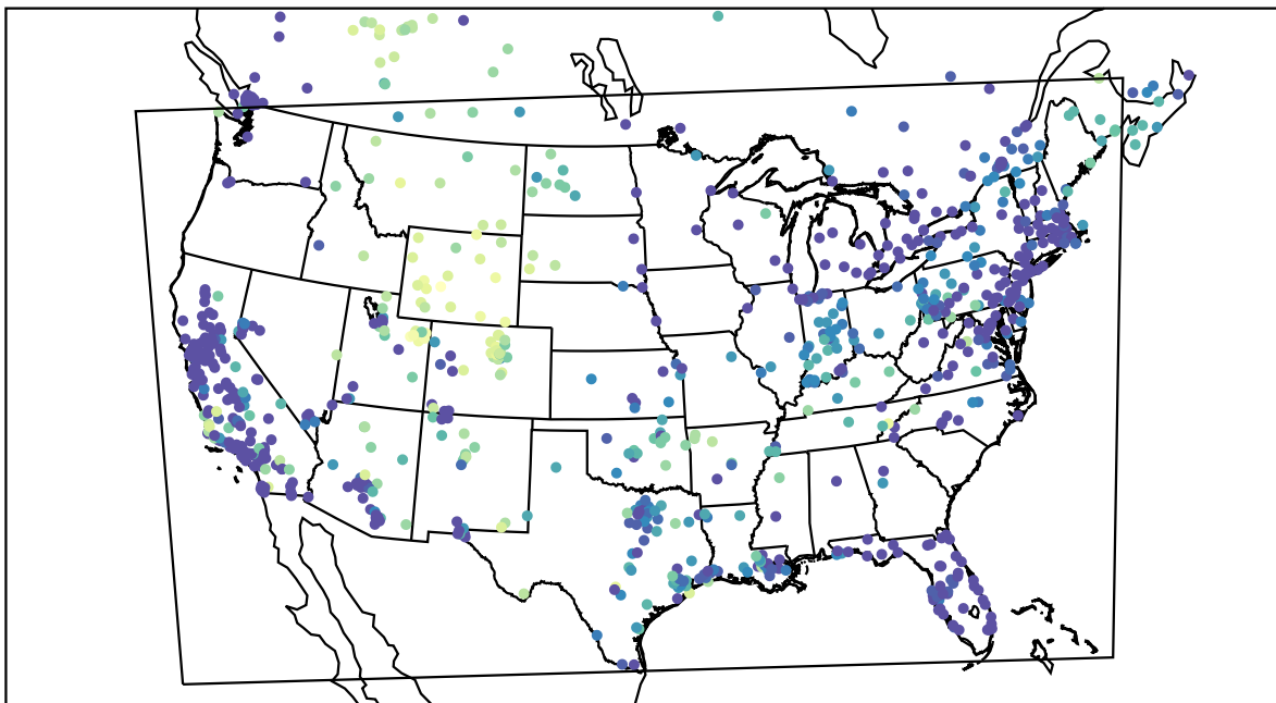
AirNOW (2021-01-14_04:00:00)
