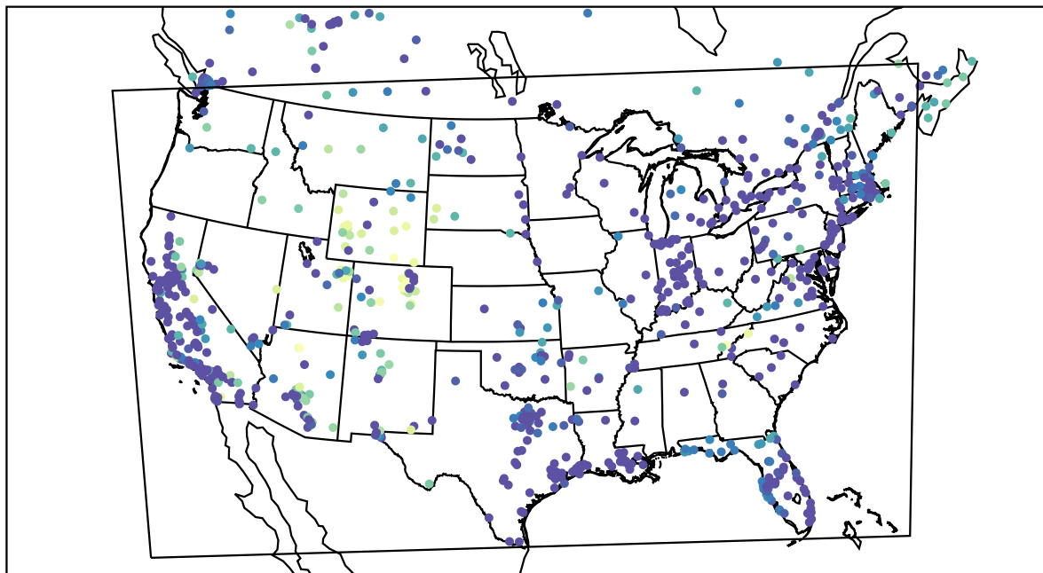
AirNOW (2021-01-13_06:00:00)
