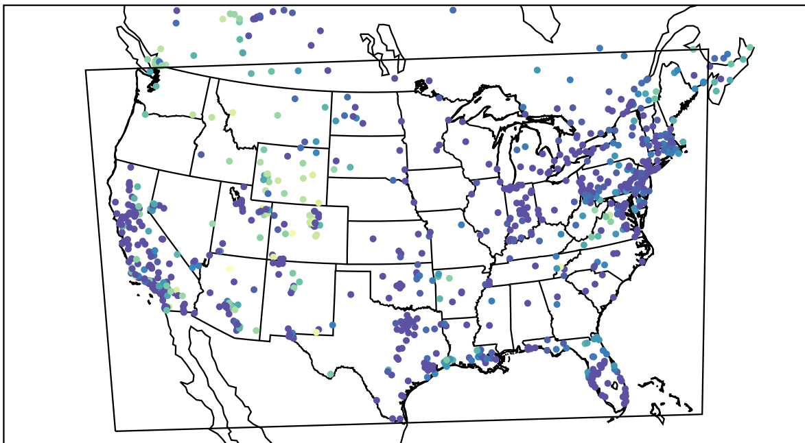
AirNOW (2021-01-13_15:00:00)
