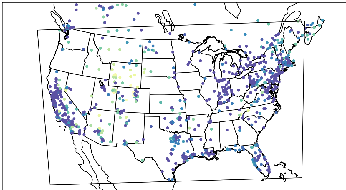
AirNOW (2021-01-13_02:00:00)
