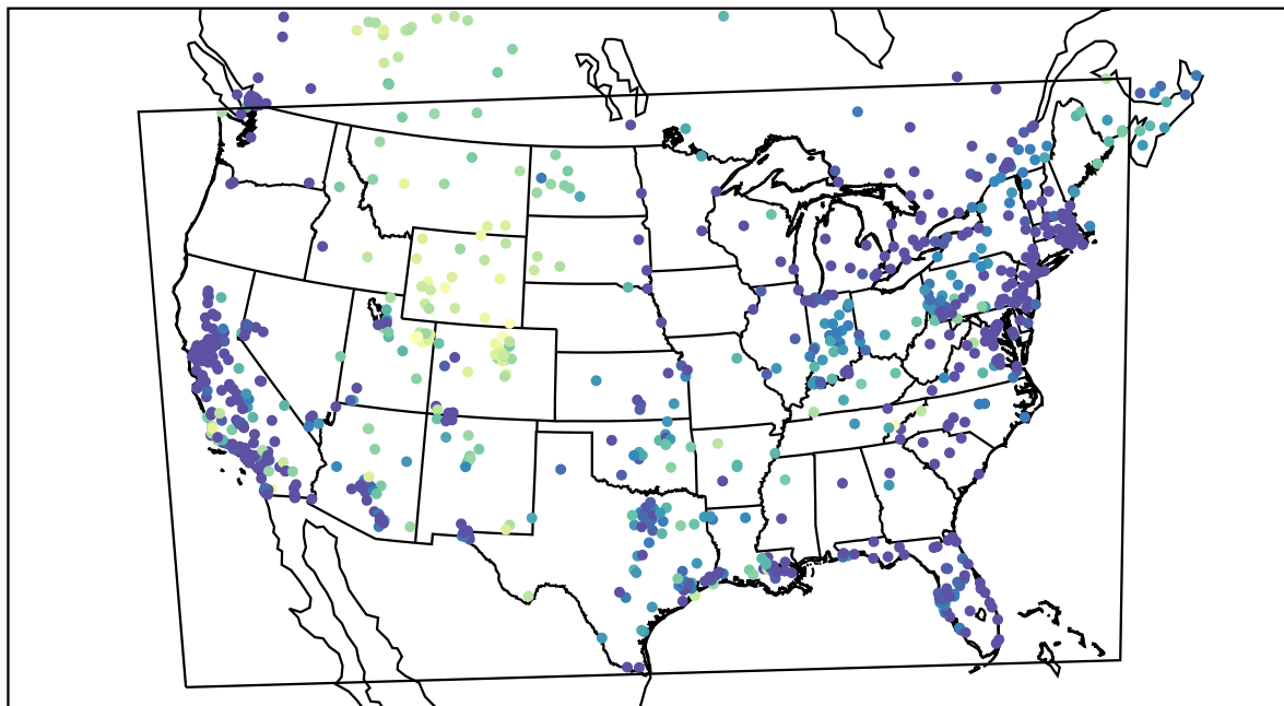
AirNOW (2021-01-14_05:00:00)
