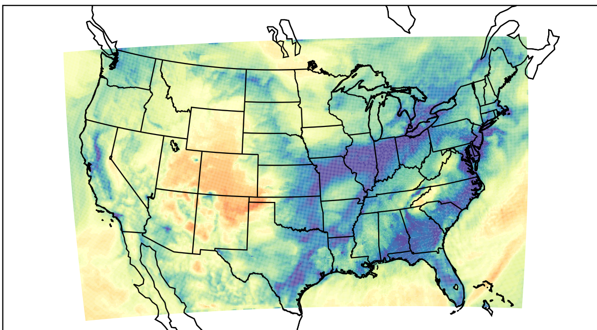
WRF (2021-01-13_08:00:00)
