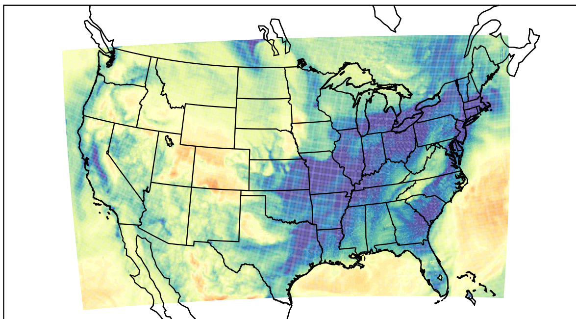
WRF (2021-01-14_09:00:00)
