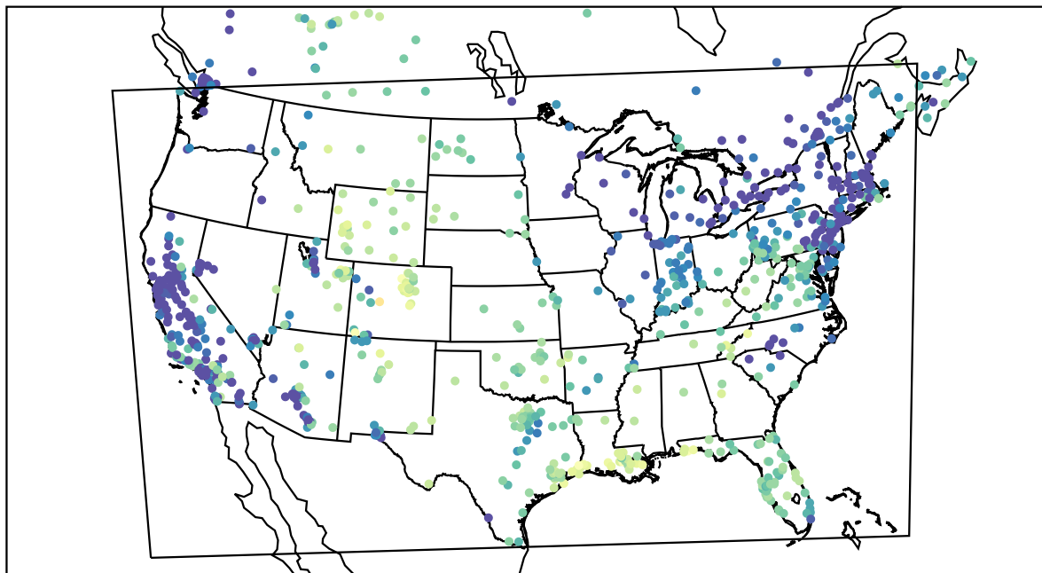
AirNOW (2021-01-14_17:00:00)
