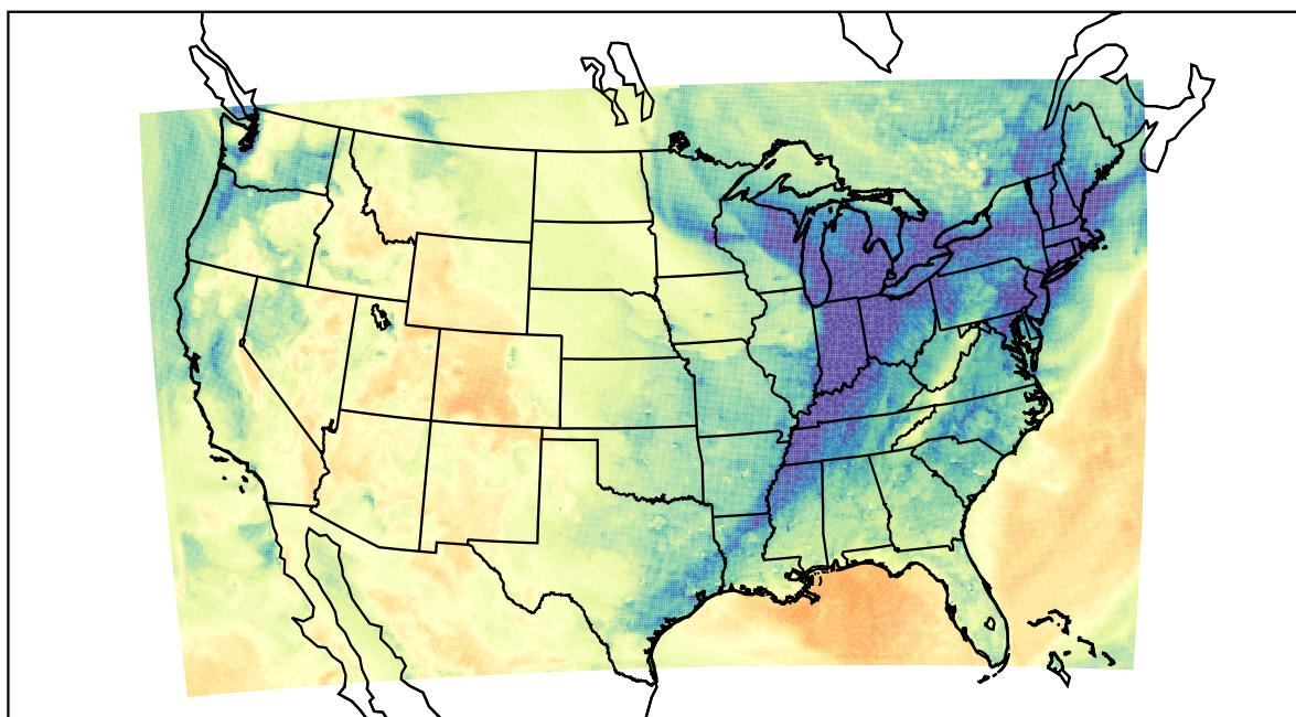
WRF (2021-01-14_23:00:00)
