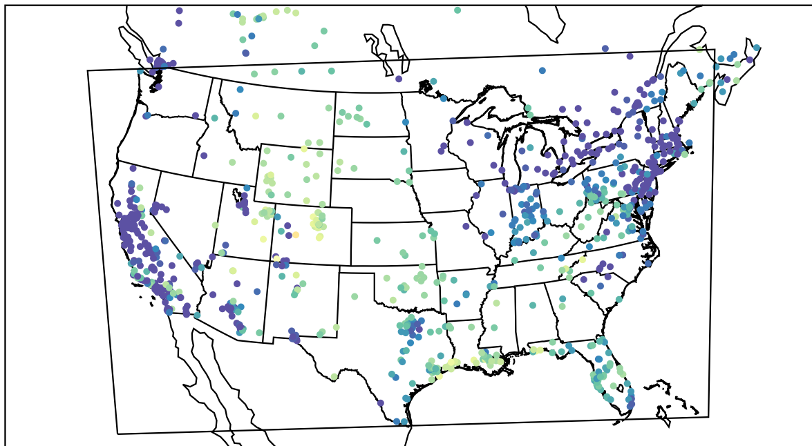
AirNOW (2021-01-14_16:00:00)
