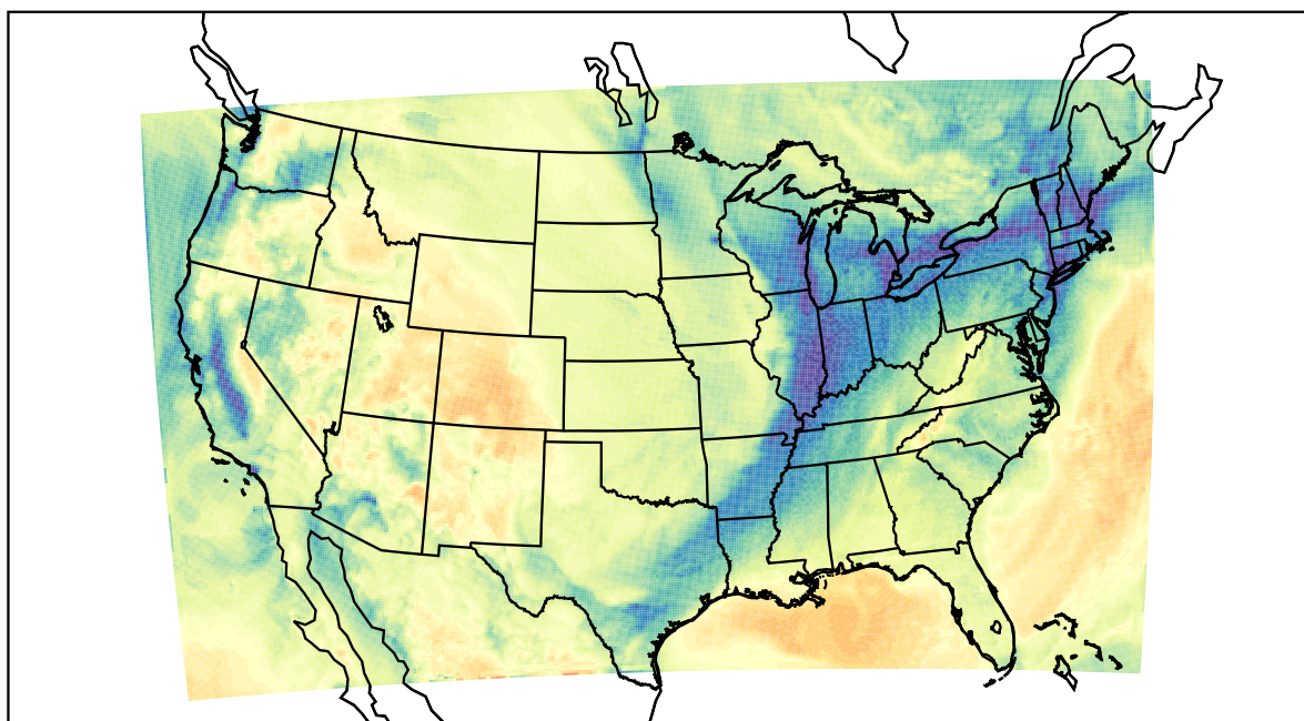
WRF (2021-01-14_18:00:00)
