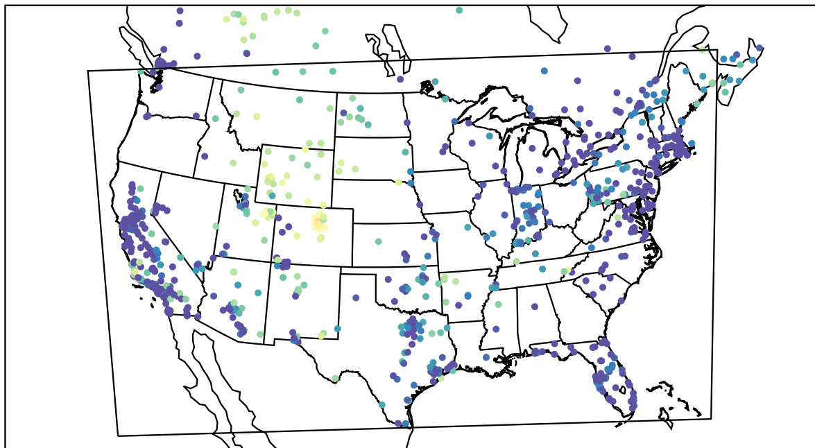
AirNOW (2021-01-14_07:00:00)
