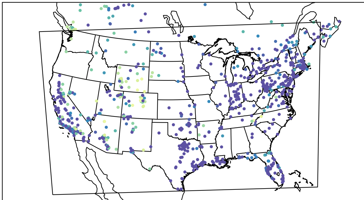
AirNOW (2021-01-13_11:00:00)
