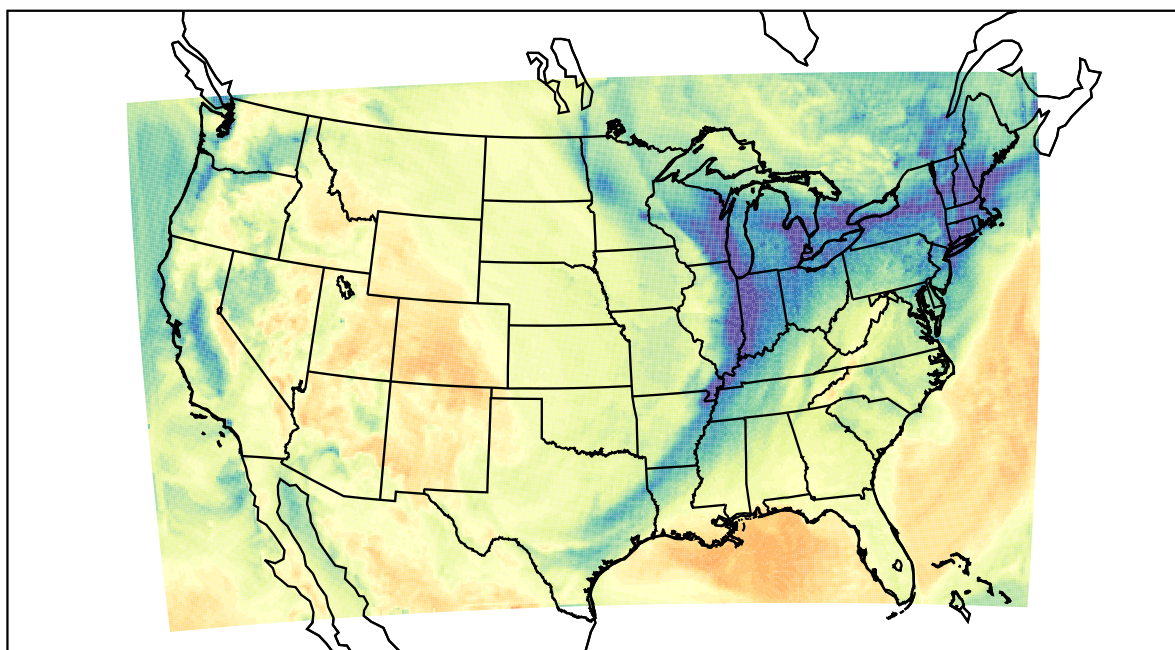
WRF (2021-01-14_20:00:00)
