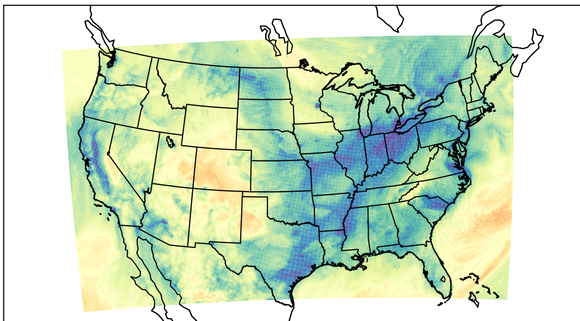
WRF (2021-01-13_16:00:00)
