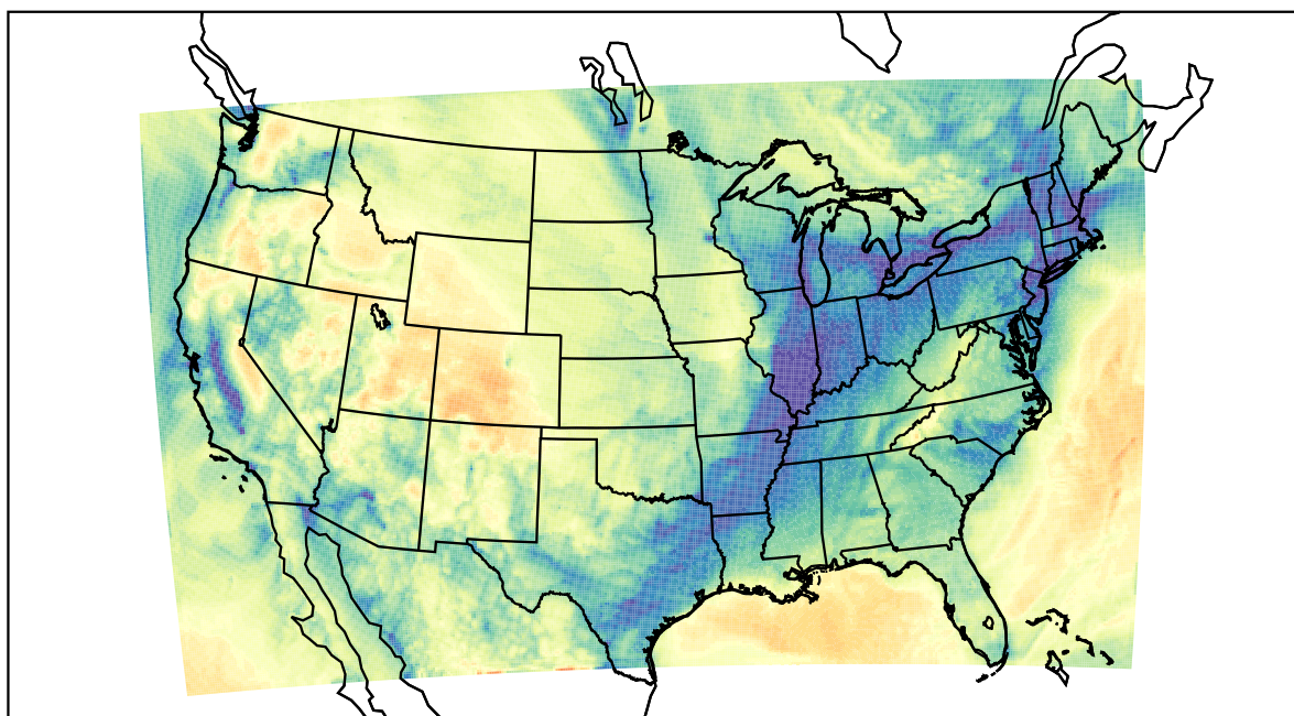
WRF (2021-01-14_16:00:00)
