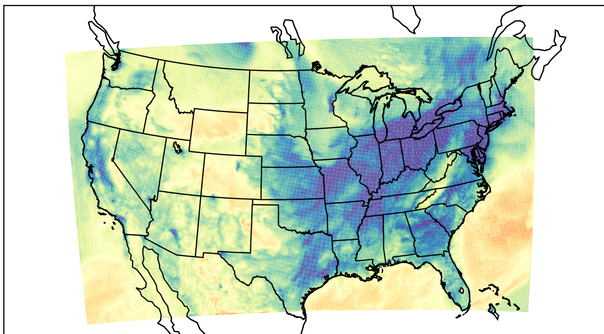
WRF (2021-01-14_03:00:00)
