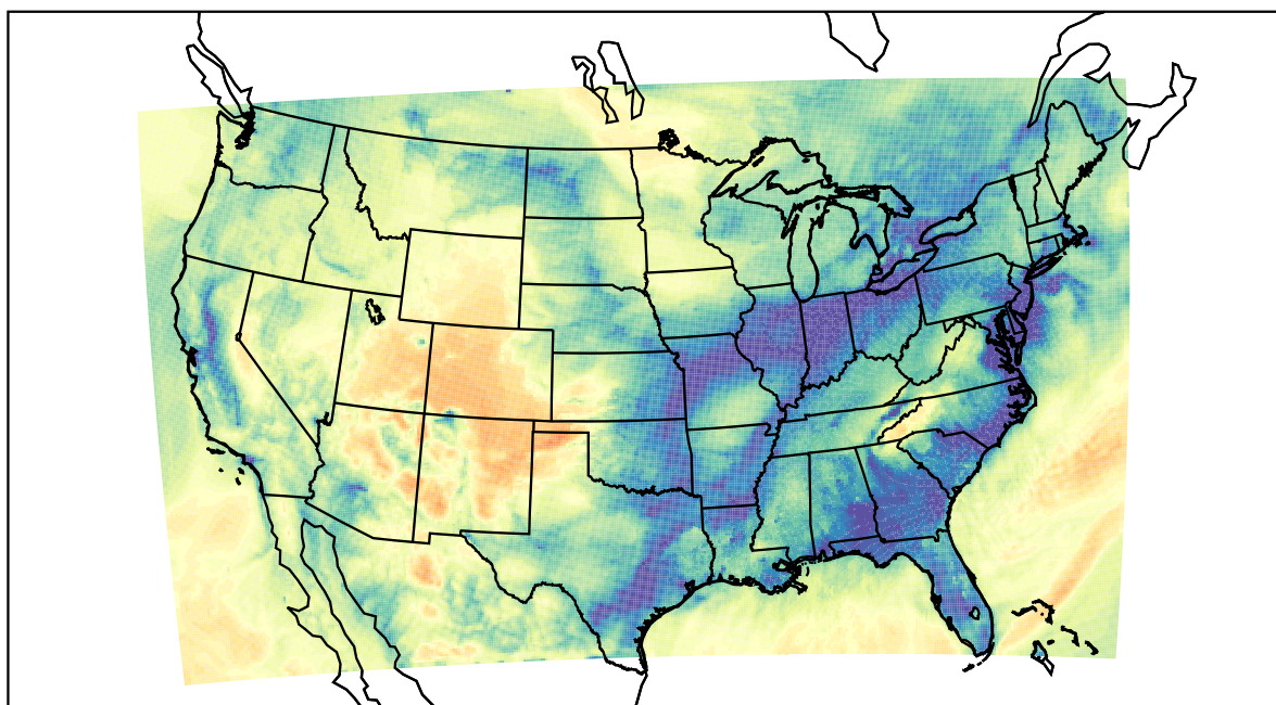
WRF (2021-01-13_10:00:00)
