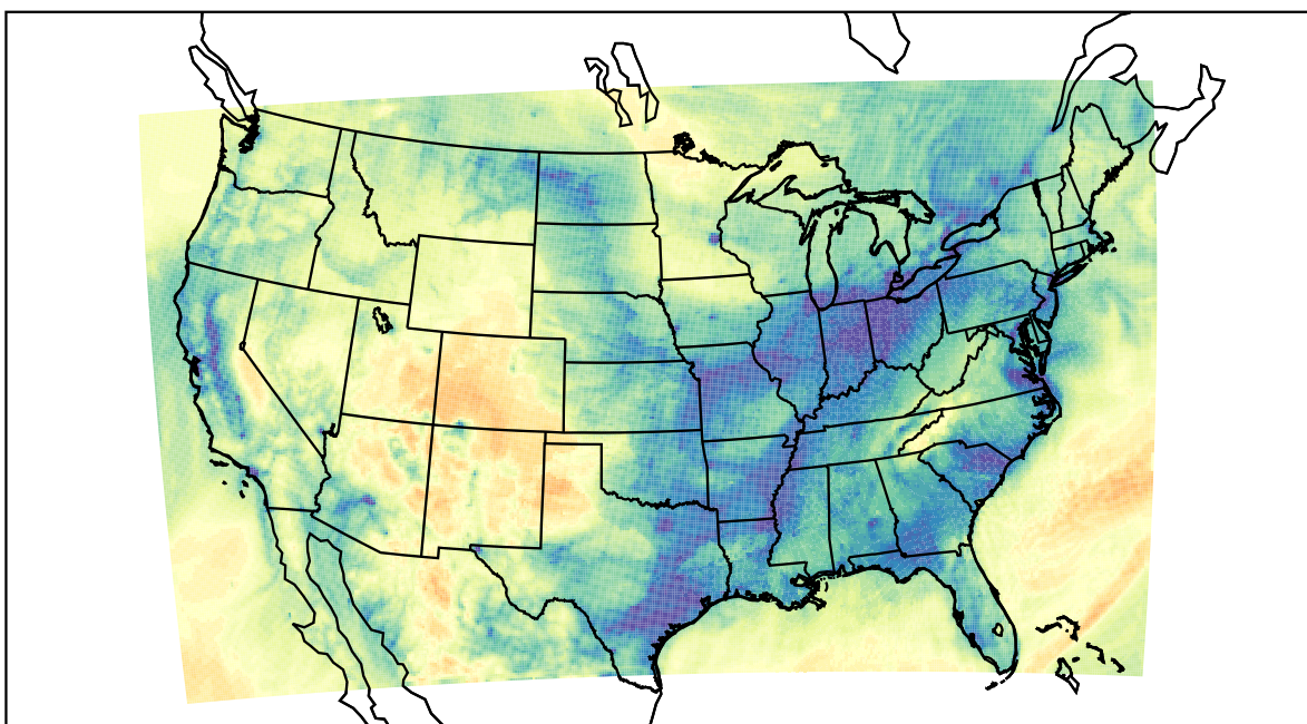
WRF (2021-01-13_15:00:00)
