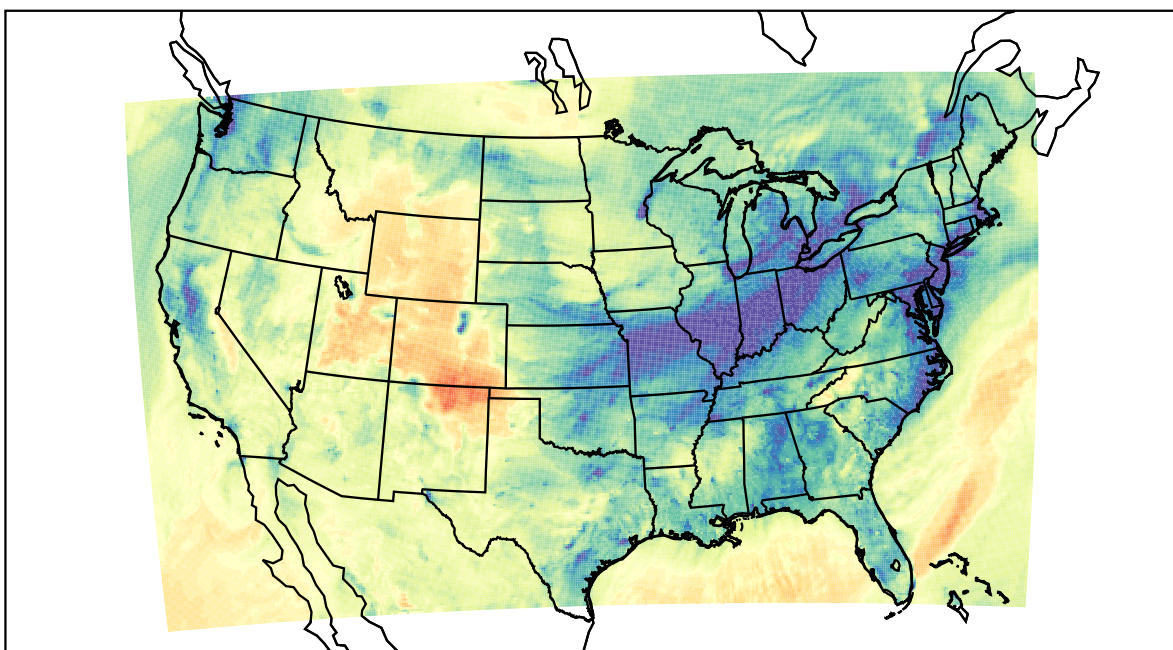
WRF (2021-01-13_00:00:00)
