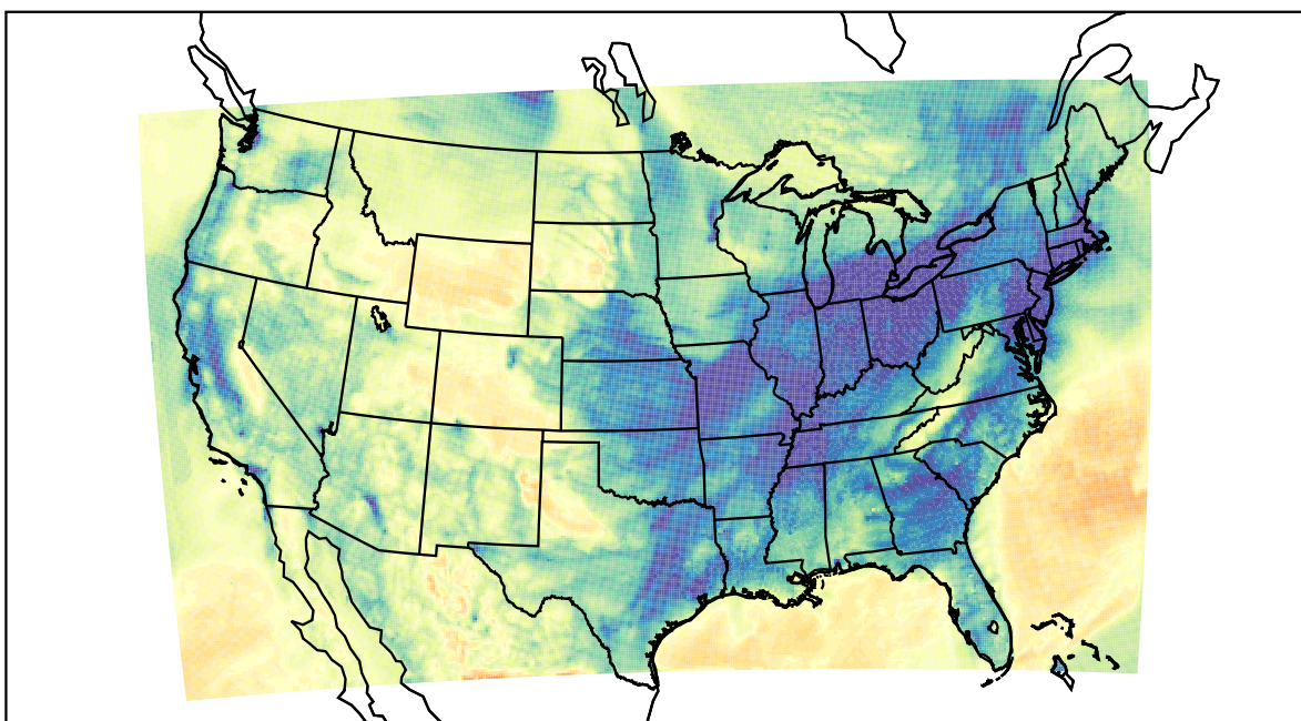
WRF (2021-01-14_04:00:00)
