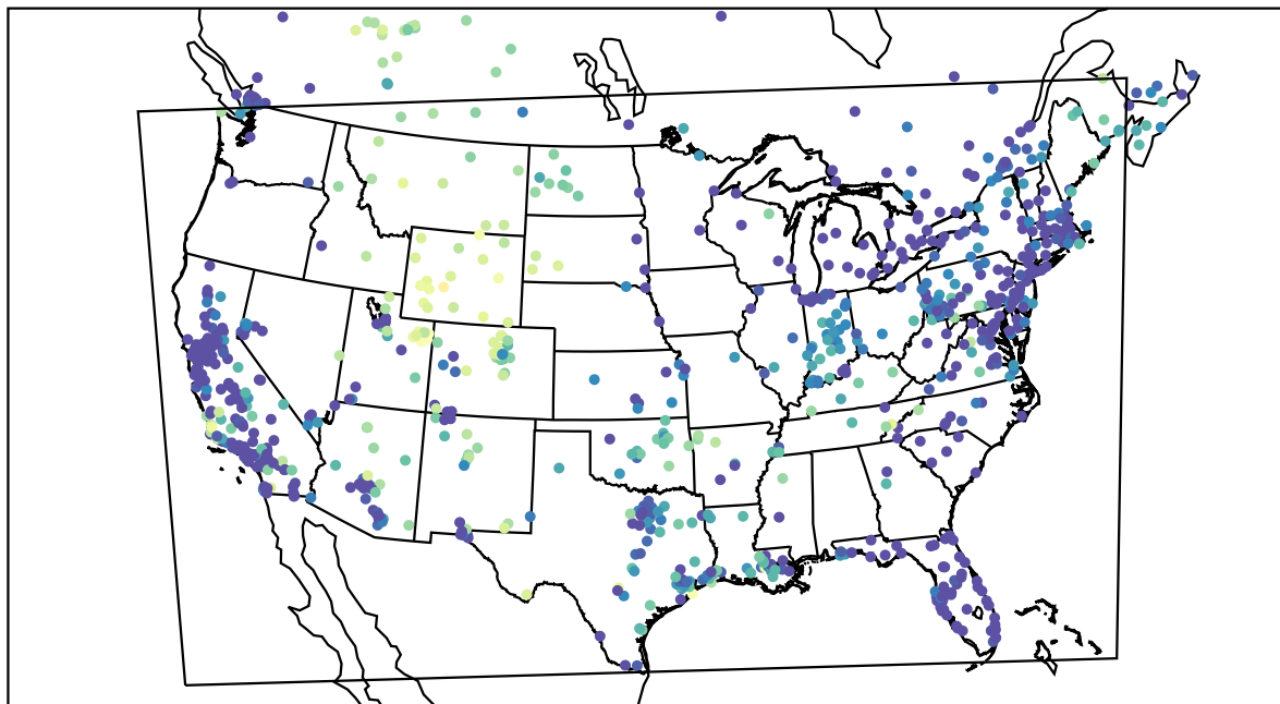
AirNOW (2021-01-14_03:00:00)
