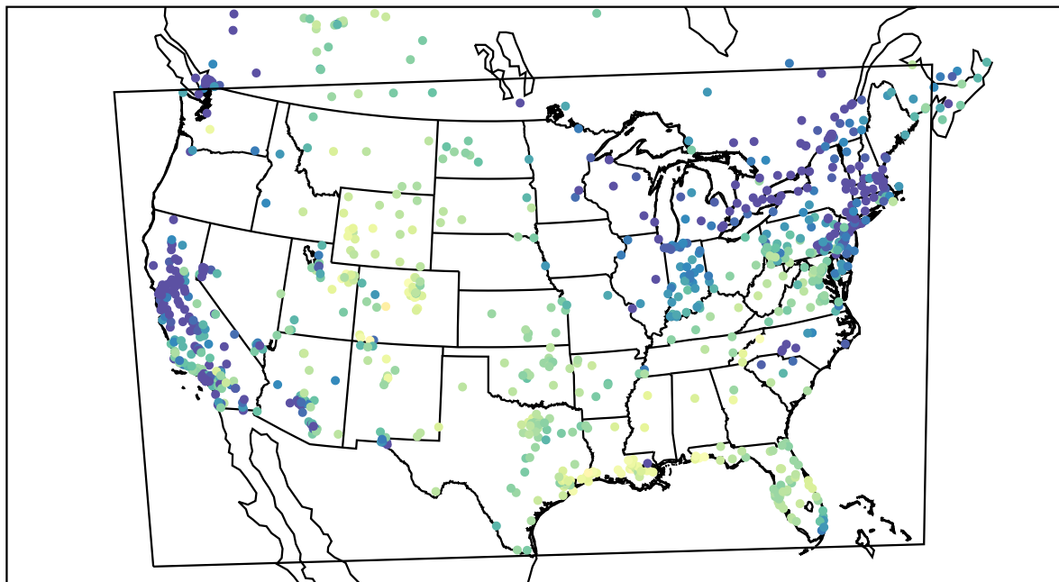
AirNOW (2021-01-14_18:00:00)
