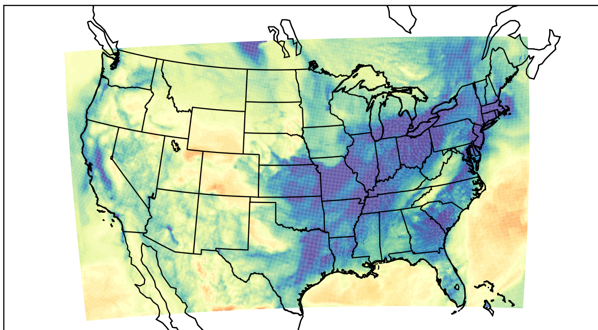
WRF (2021-01-14_07:00:00)
