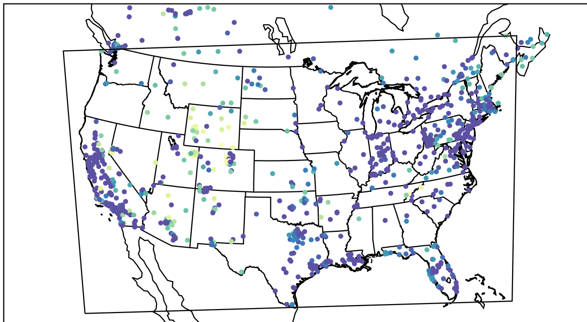
AirNOW (2021-01-13_03:00:00)
