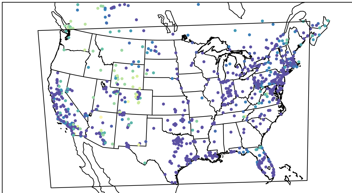
AirNOW (2021-01-13_14:00:00)
