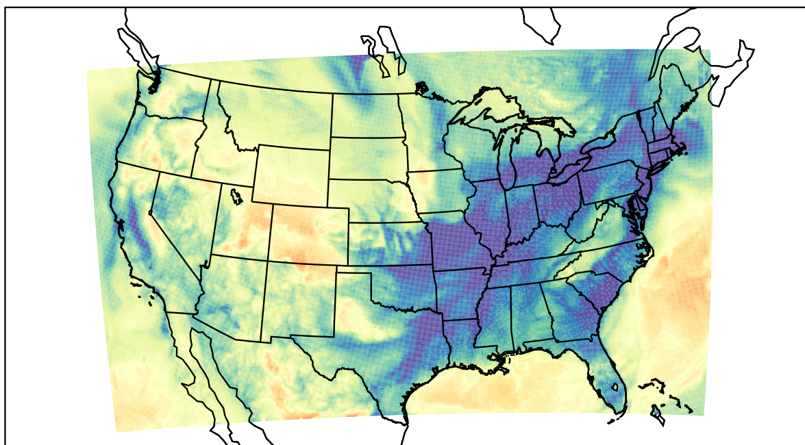
WRF (2021-01-14_10:00:00)
