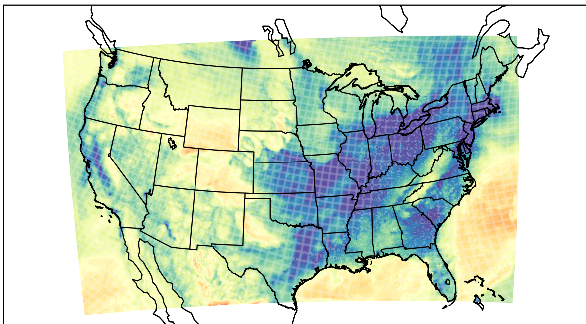
WRF (2021-01-14_06:00:00)
