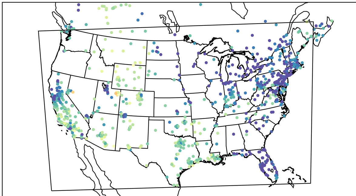
AirNOW (2021-01-13_23:00:00)
