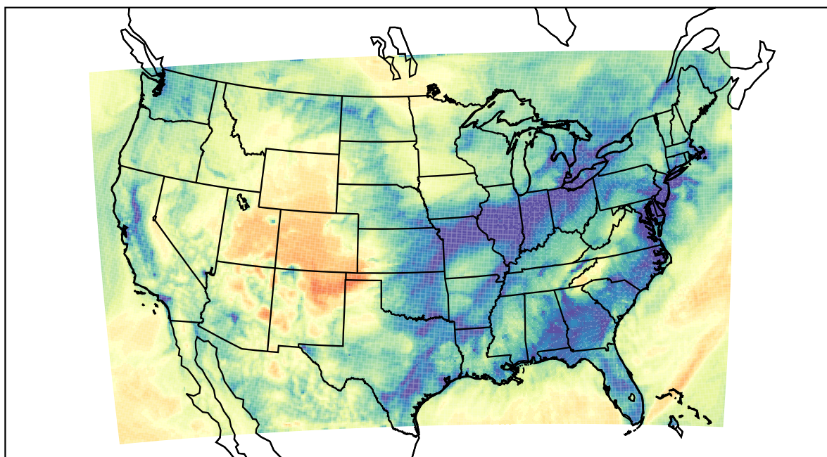
WRF (2021-01-13_07:00:00)
