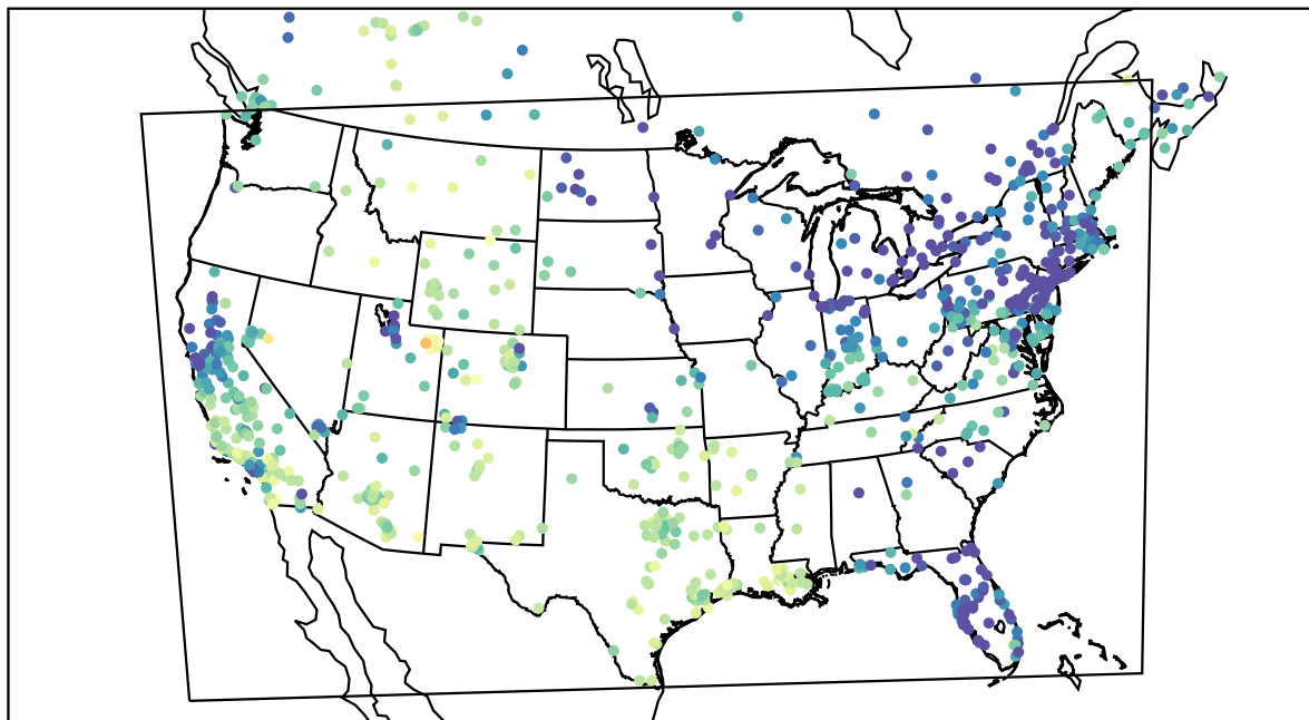
AirNOW (2021-01-13_22:00:00)
