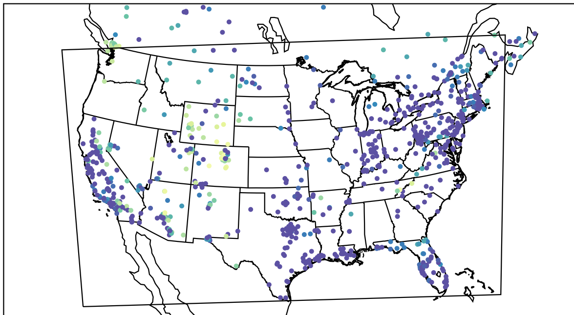
AirNOW (2021-01-13_10:00:00)
