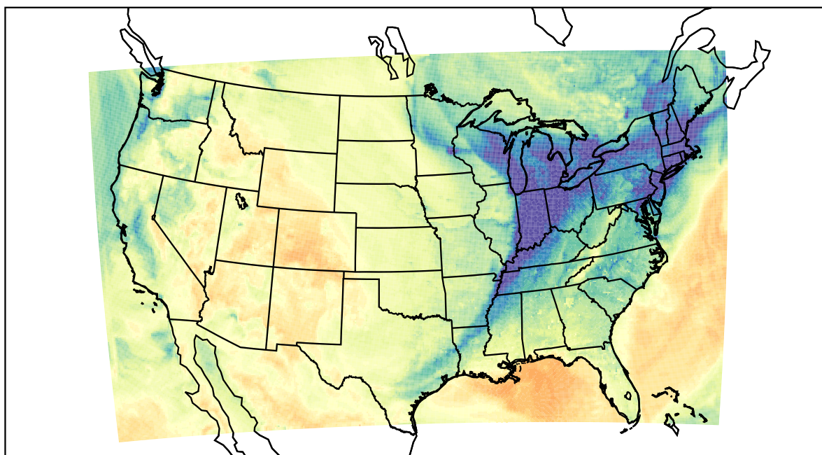
WRF (2021-01-14_22:00:00)
