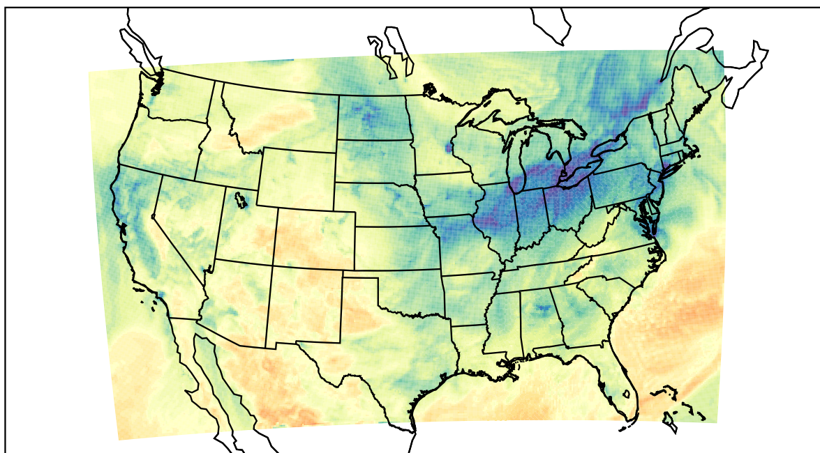
WRF (2021-01-13_20:00:00)
