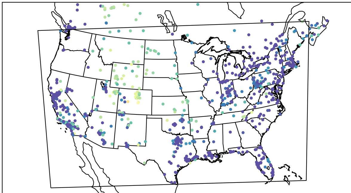
AirNOW (2021-01-14_12:00:00)
