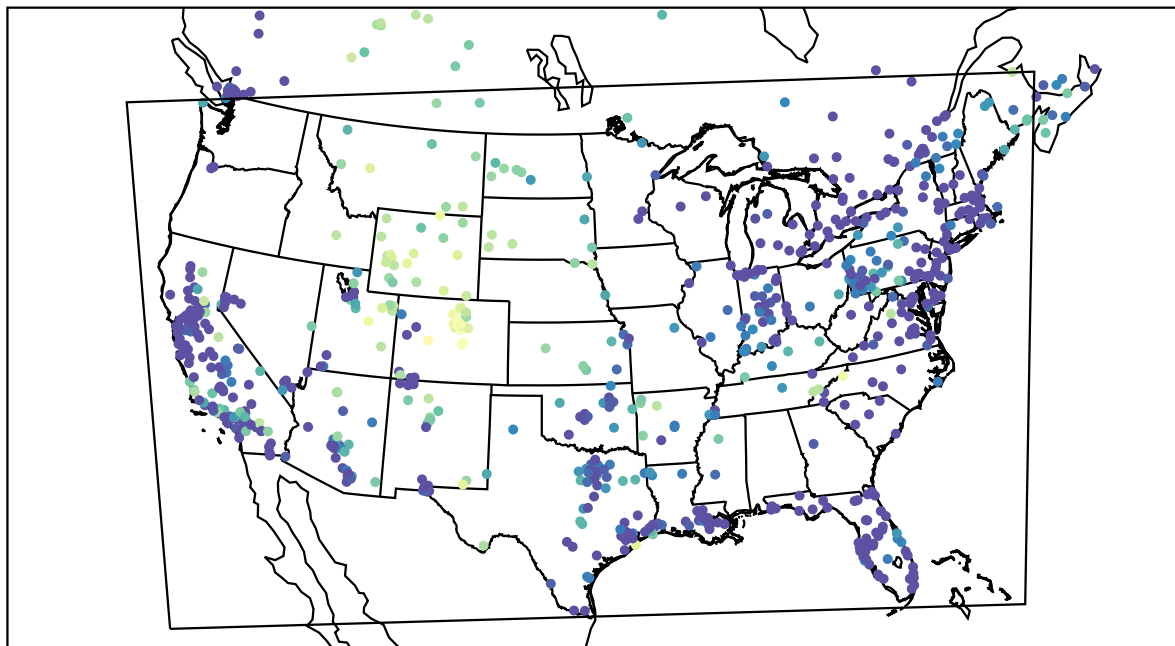
AirNOW (2021-01-14_10:00:00)
