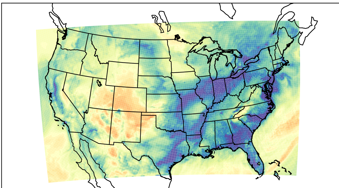
WRF (2021-01-13_12:00:00)
