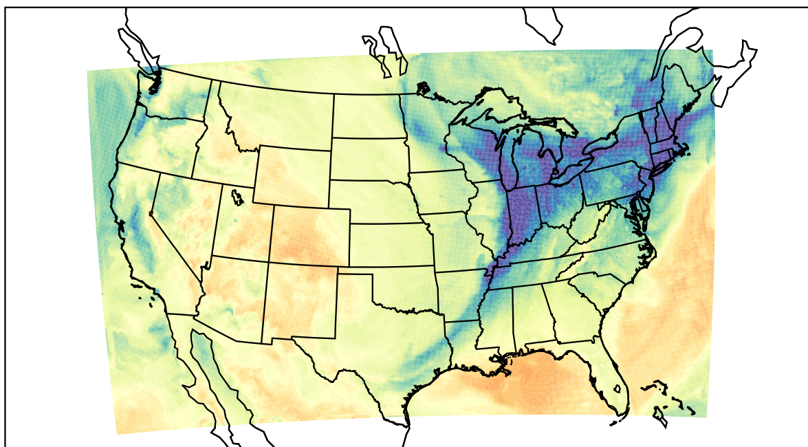
WRF (2021-01-14_21:00:00)
