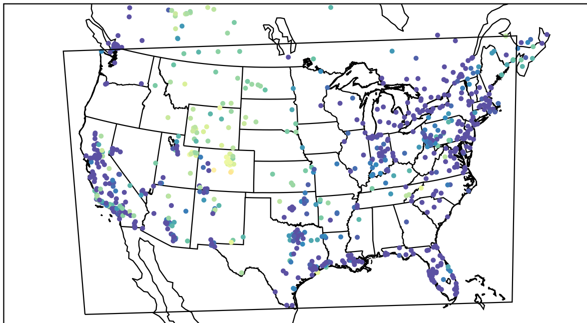
AirNOW (2021-01-14_11:00:00)
