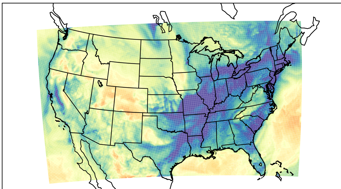
WRF (2021-01-14_11:00:00)
