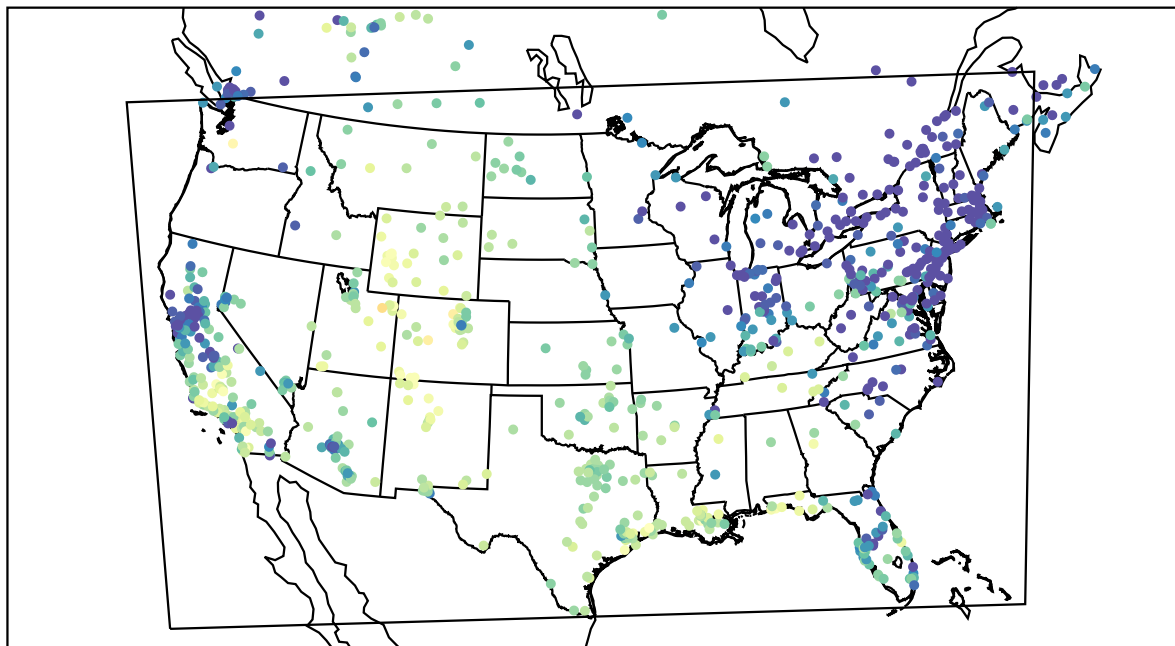
AirNOW (2021-01-14_23:00:00)
