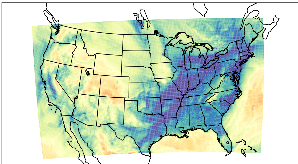
WRF (2021-01-14_14:00:00)
