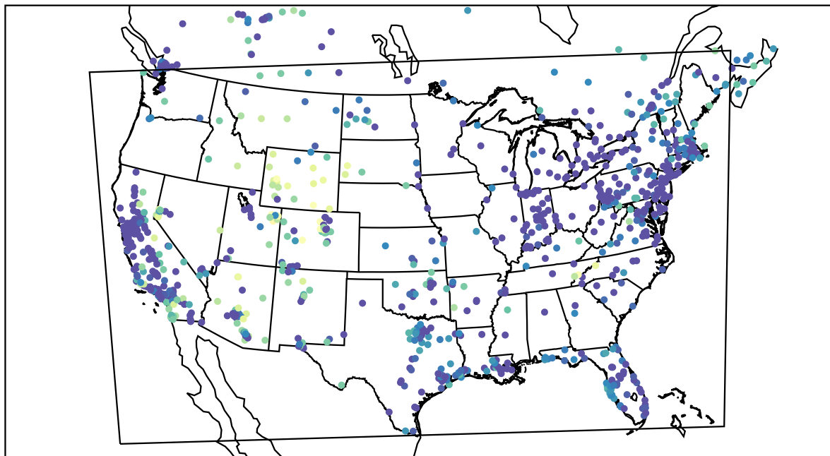
AirNOW (2021-01-13_01:00:00)
