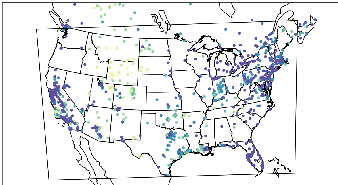
AirNOW (2021-01-14_02:00:00)
