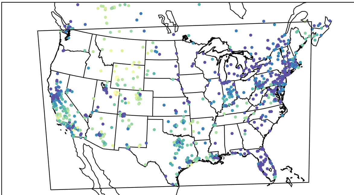
AirNOW (2021-01-14_00:00:00)
