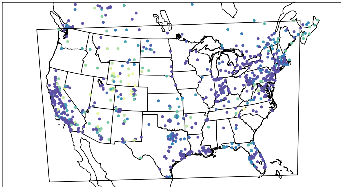
AirNOW (2021-01-13_04:00:00)
