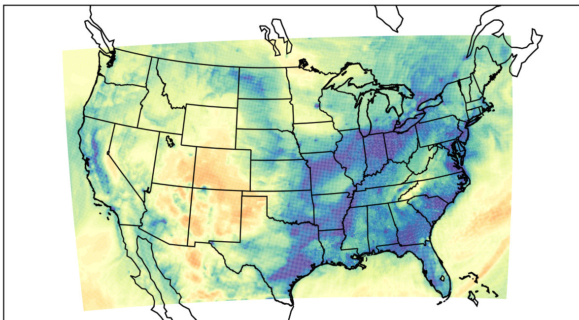
WRF (2021-01-13_14:00:00)
