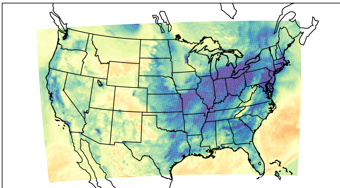
WRF (2021-01-14_02:00:00)
