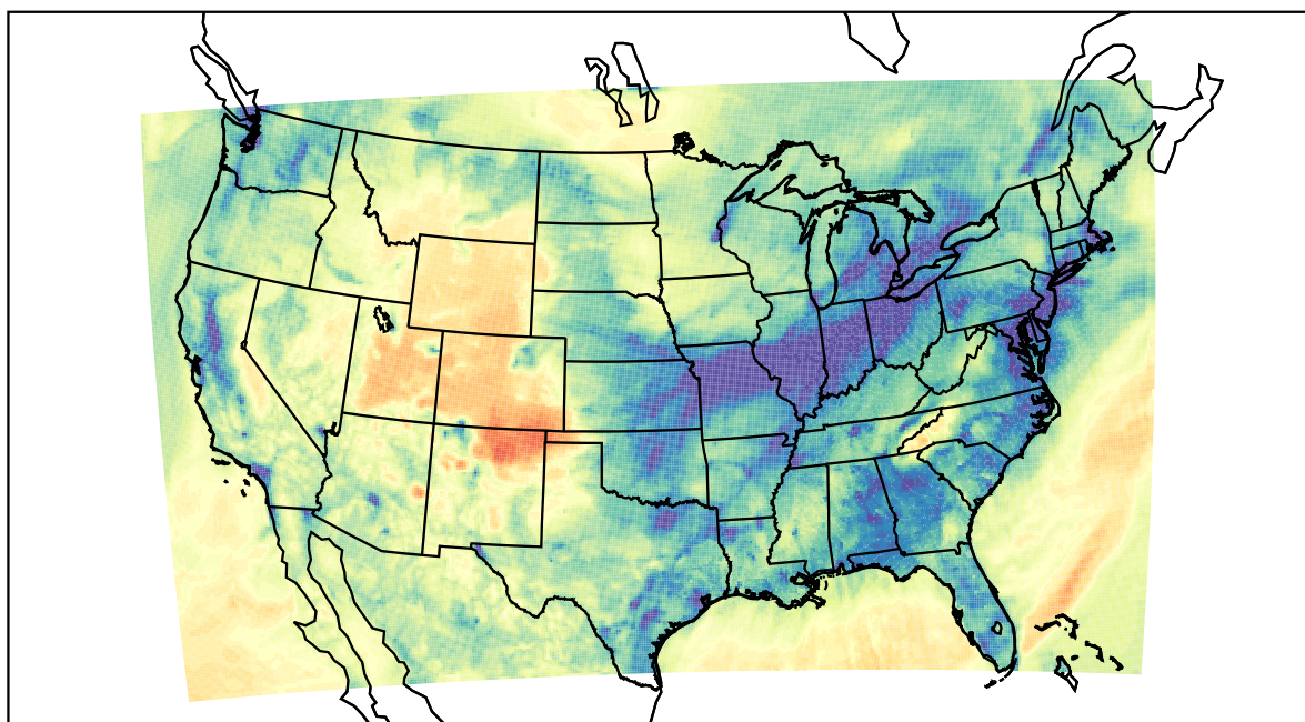
WRF (2021-01-13_03:00:00)
