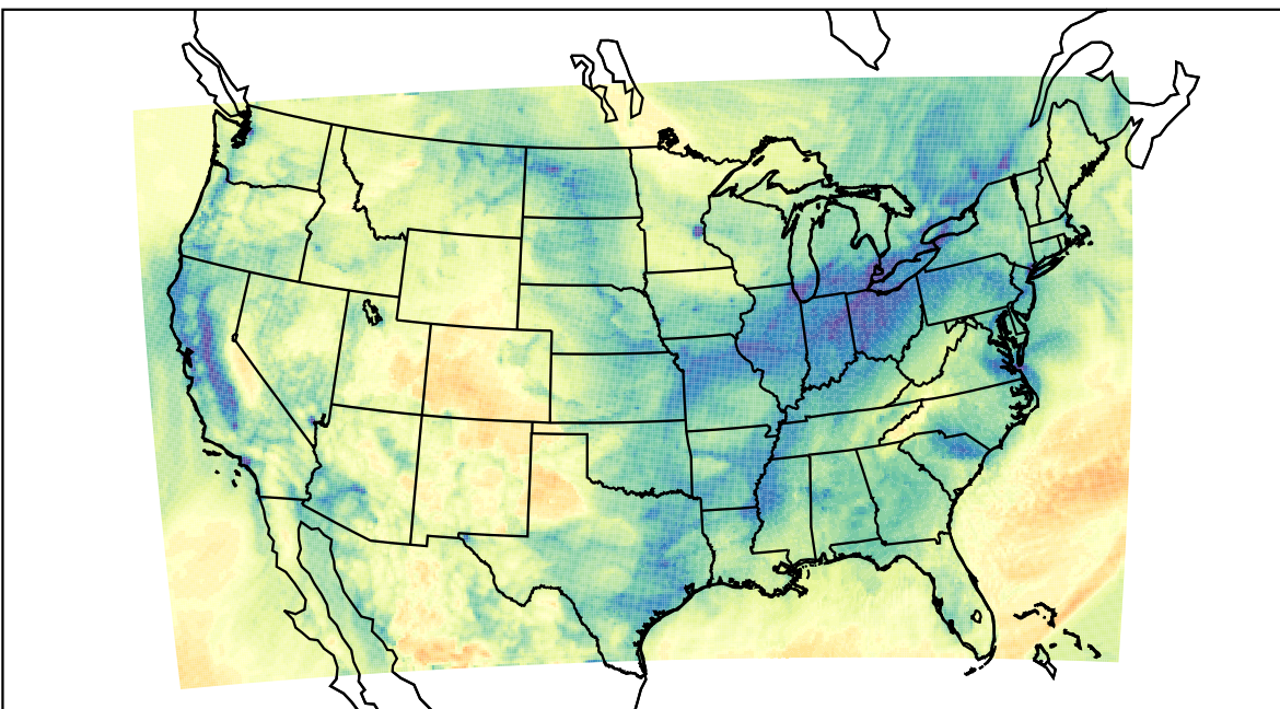
WRF (2021-01-13_17:00:00)
