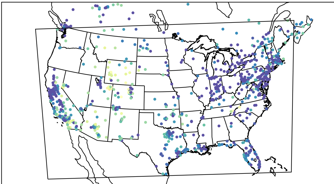
AirNOW (2021-01-13_00:00:00)
