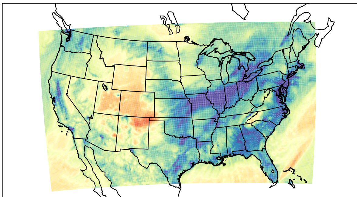
WRF (2021-01-13_05:00:00)
