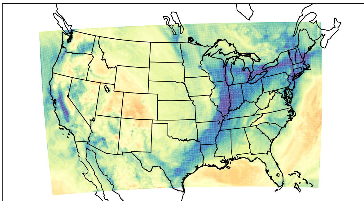
WRF (2021-01-14_17:00:00)
