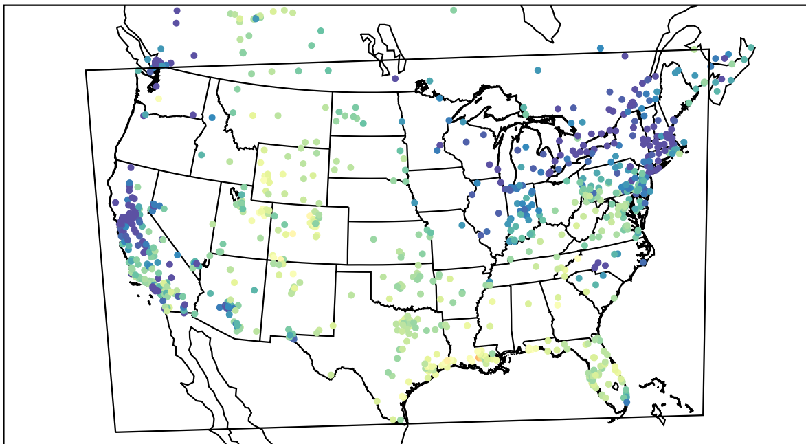
AirNOW (2021-01-14_19:00:00)
