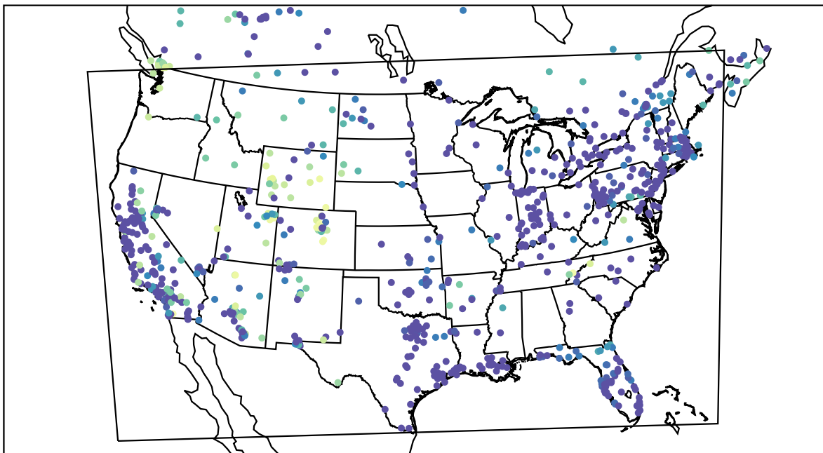
AirNOW (2021-01-13_09:00:00)
