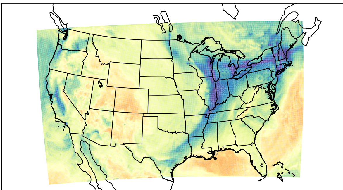
WRF (2021-01-14_19:00:00)
