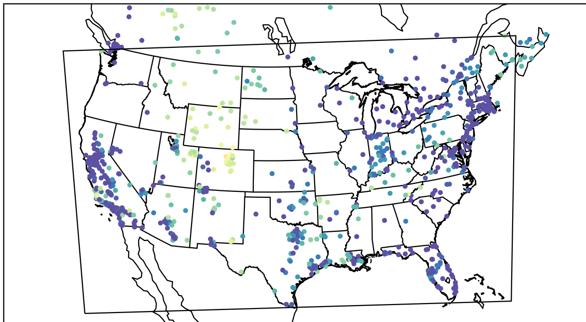
AirNOW (2021-01-14_06:00:00)
