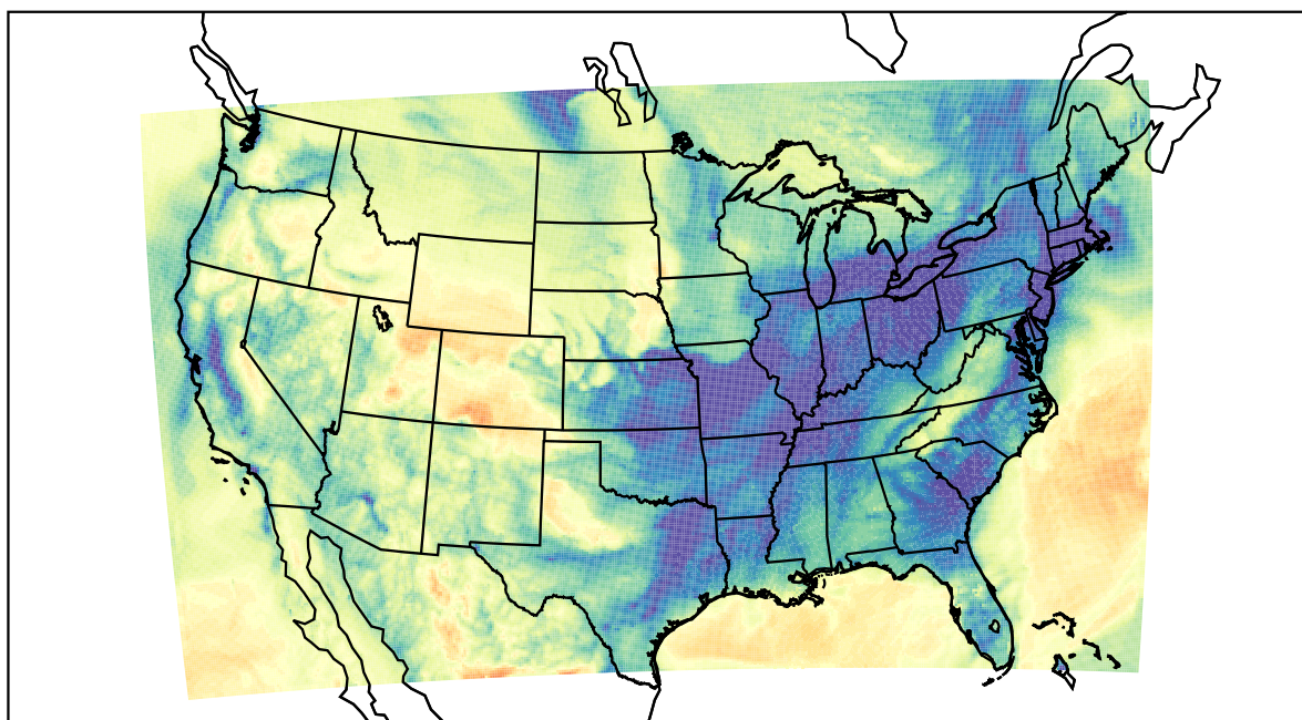
WRF (2021-01-14_08:00:00)
