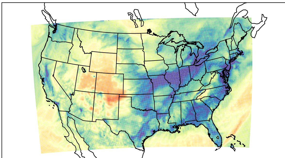
WRF (2021-01-13_06:00:00)
