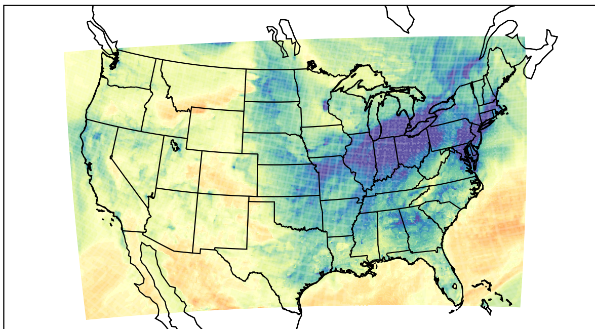
WRF (2021-01-13_23:00:00)
