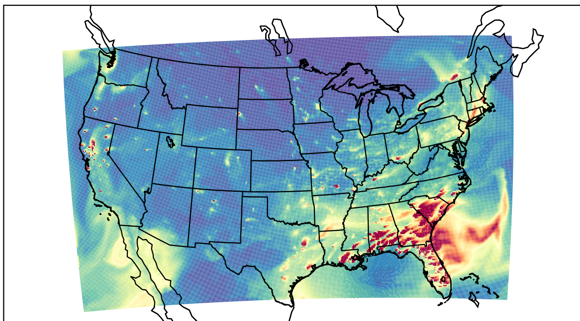
WRF 2021-01-22_00:00:00
