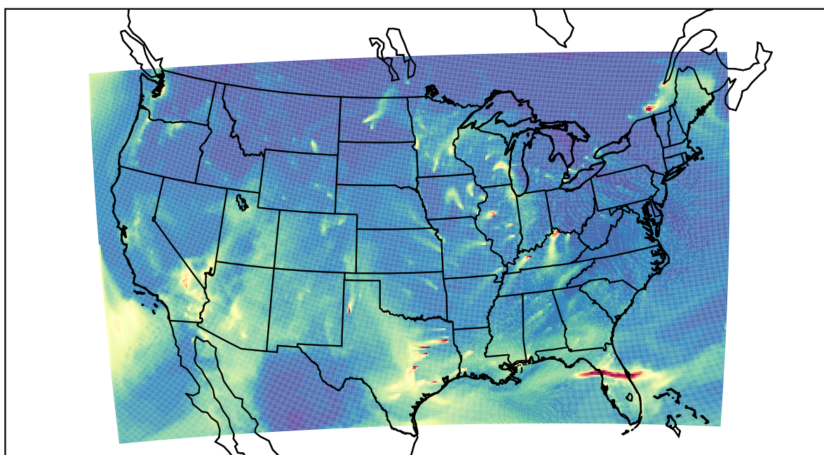
WRF 2021-01-23_15:00:00
