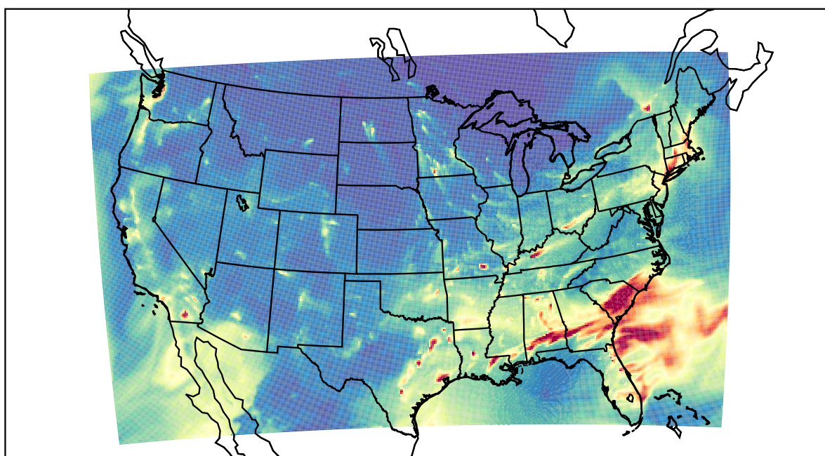
WRF 2021-01-22_05:00:00
