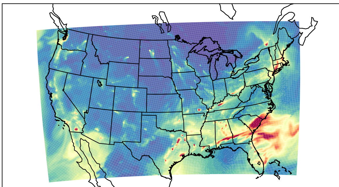
WRF 2021-01-22_06:00:00
