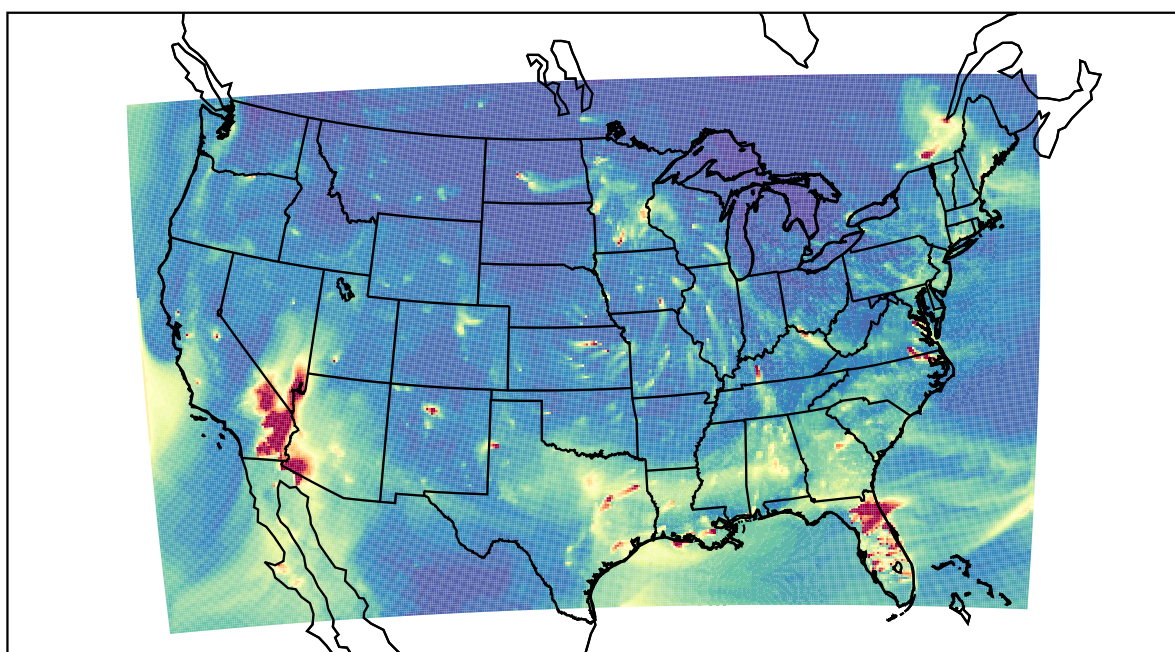
WRF 2021-01-23_01:00:00
