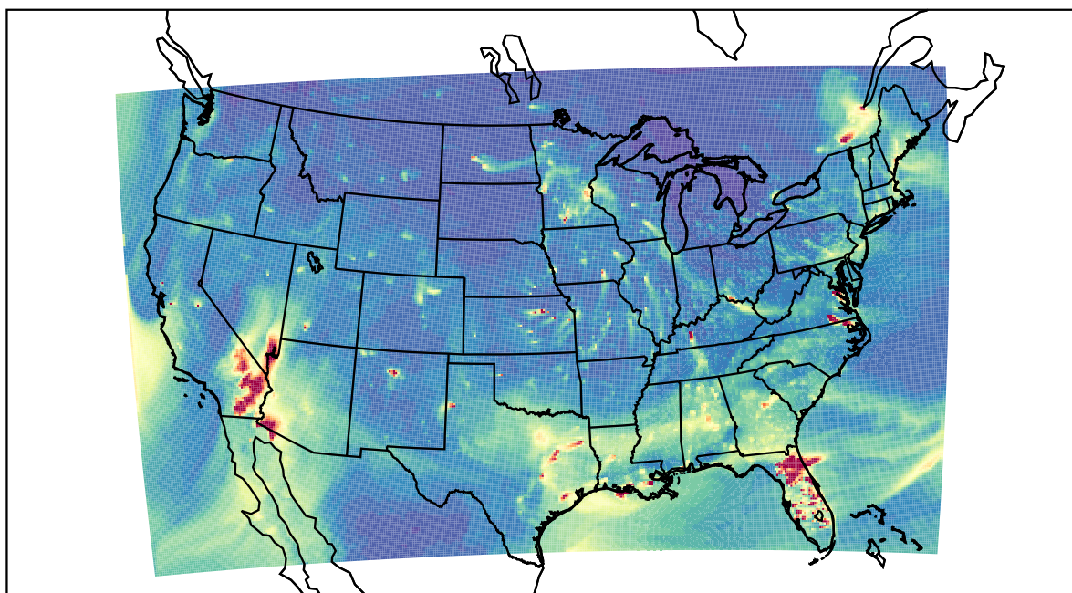
WRF 2021-01-23_00:00:00
