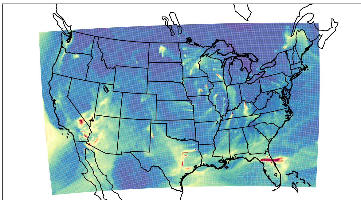
WRF 2021-01-23_10:00:00
