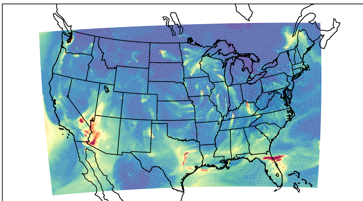
WRF 2021-01-23_07:00:00
