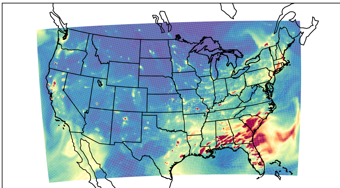
WRF 2021-01-22_01:00:00
