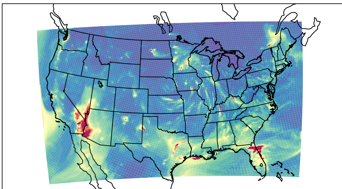
WRF 2021-01-23_04:00:00
