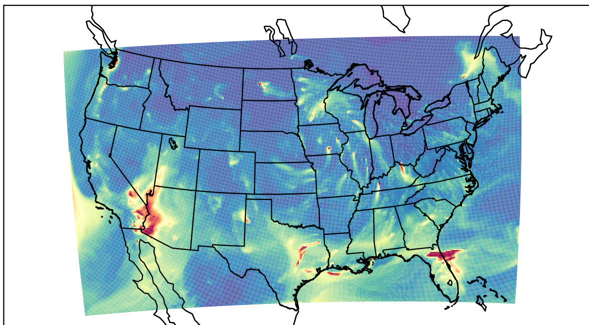
WRF 2021-01-23_06:00:00
