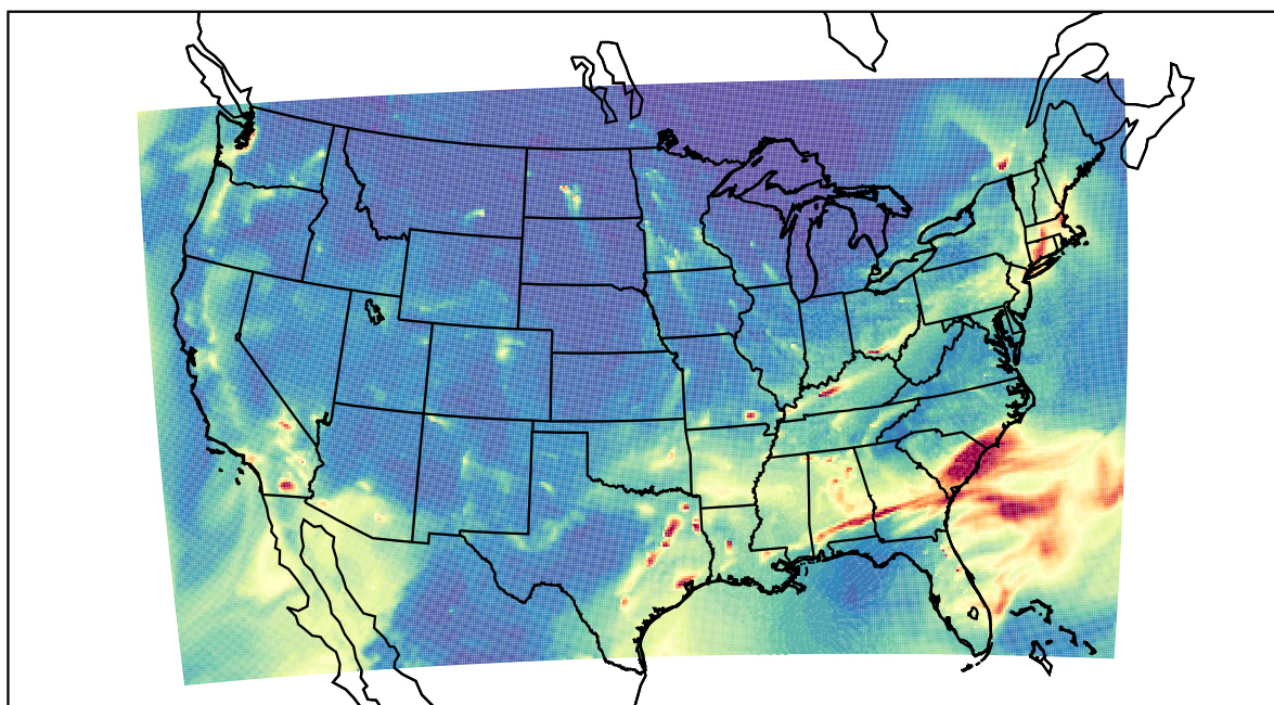
WRF 2021-01-22_07:00:00
