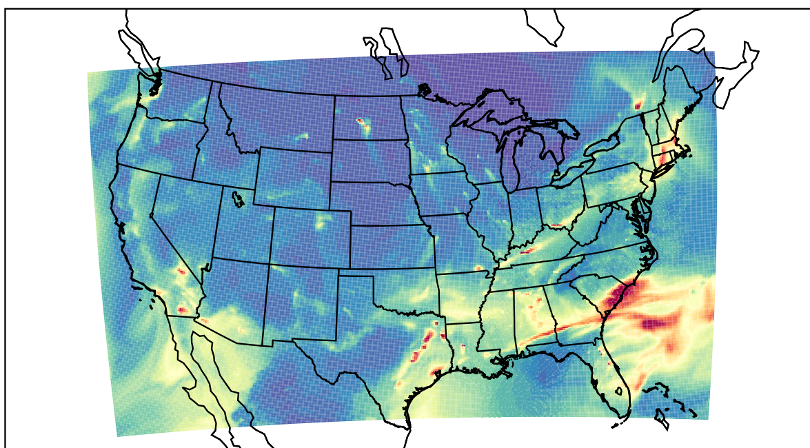
WRF 2021-01-22_08:00:00
