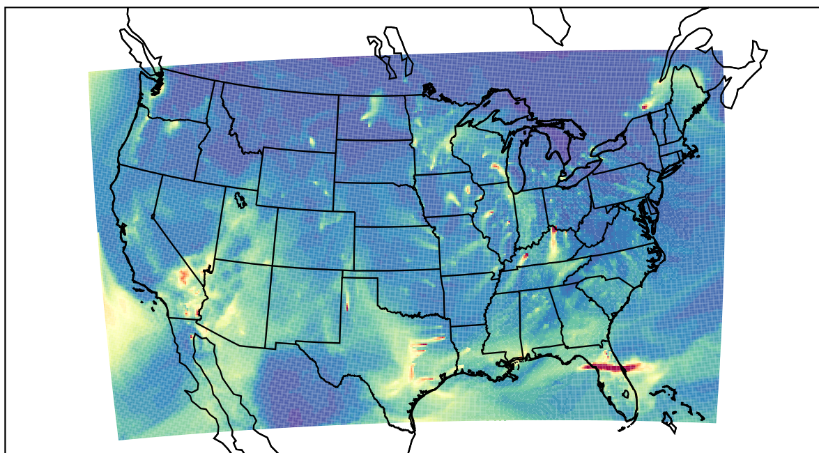
WRF 2021-01-23_13:00:00
