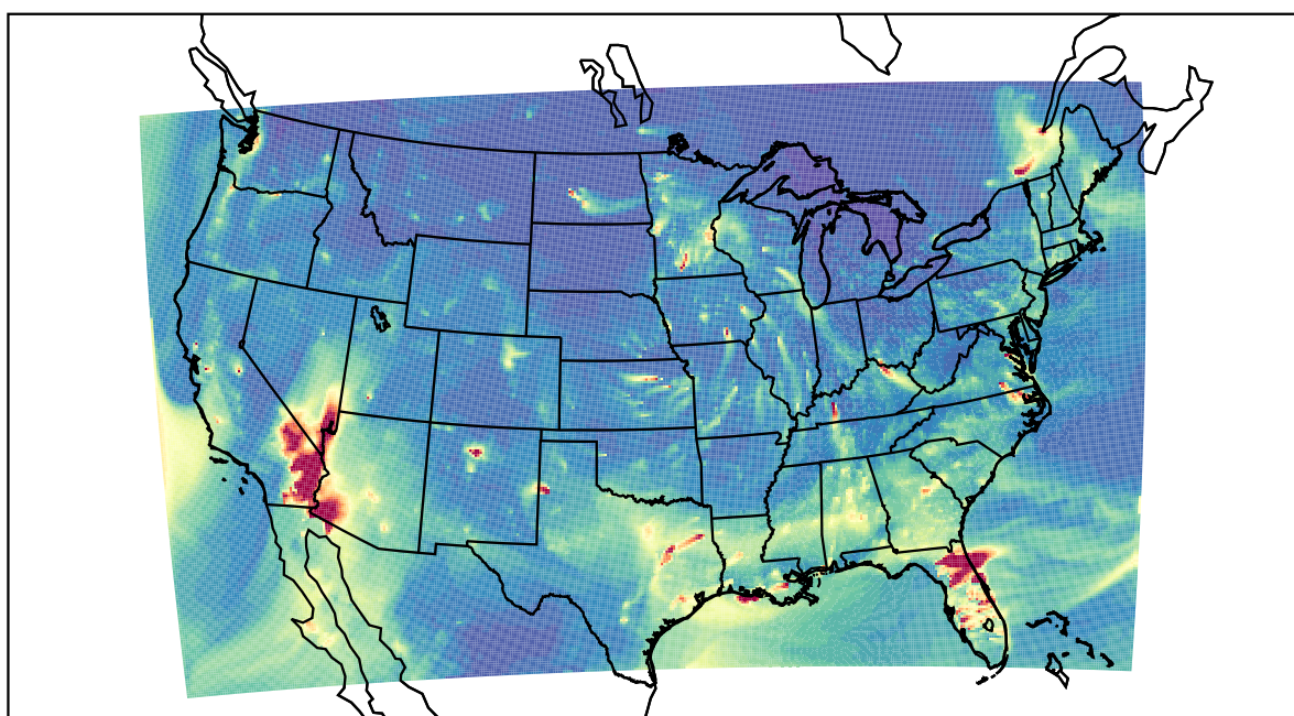
WRF 2021-01-23_02:00:00
