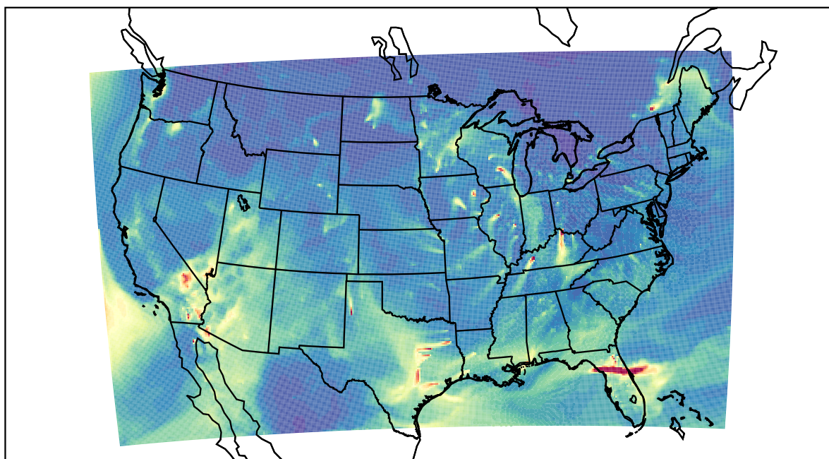
WRF 2021-01-23_12:00:00
