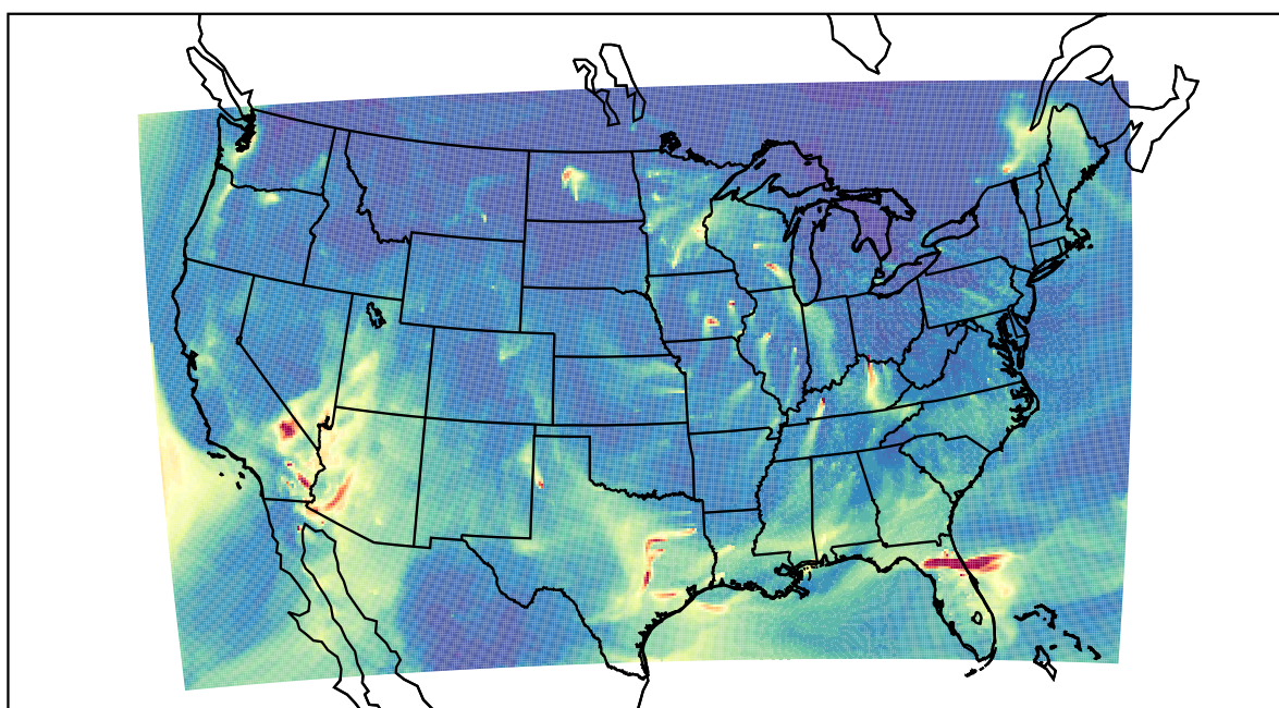
WRF 2021-01-23_09:00:00
