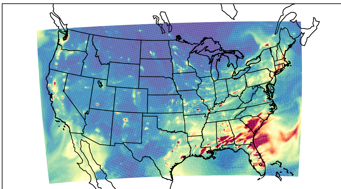
WRF 2021-01-22_02:00:00
