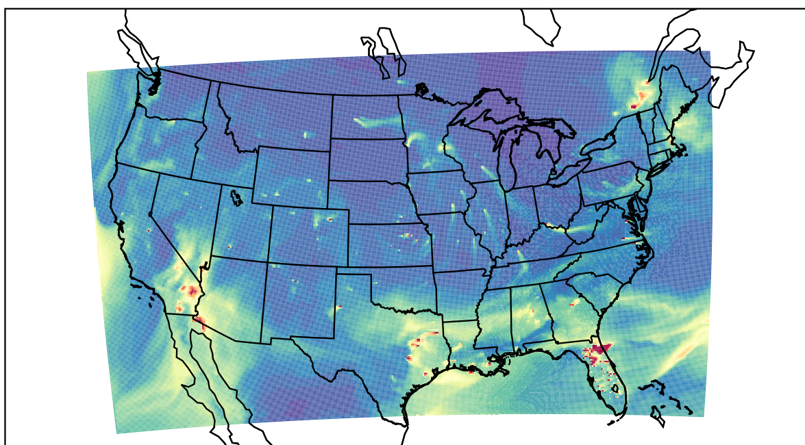
WRF 2021-01-22_21:00:00
