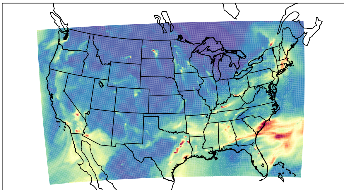
WRF 2021-01-22_09:00:00
