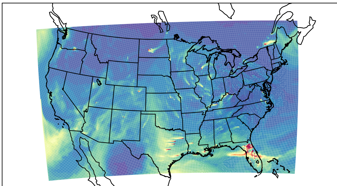
WRF 2021-01-23_20:00:00
