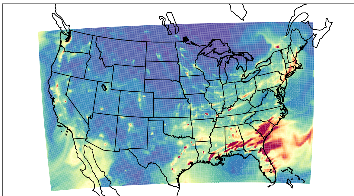
WRF 2021-01-22_03:00:00
