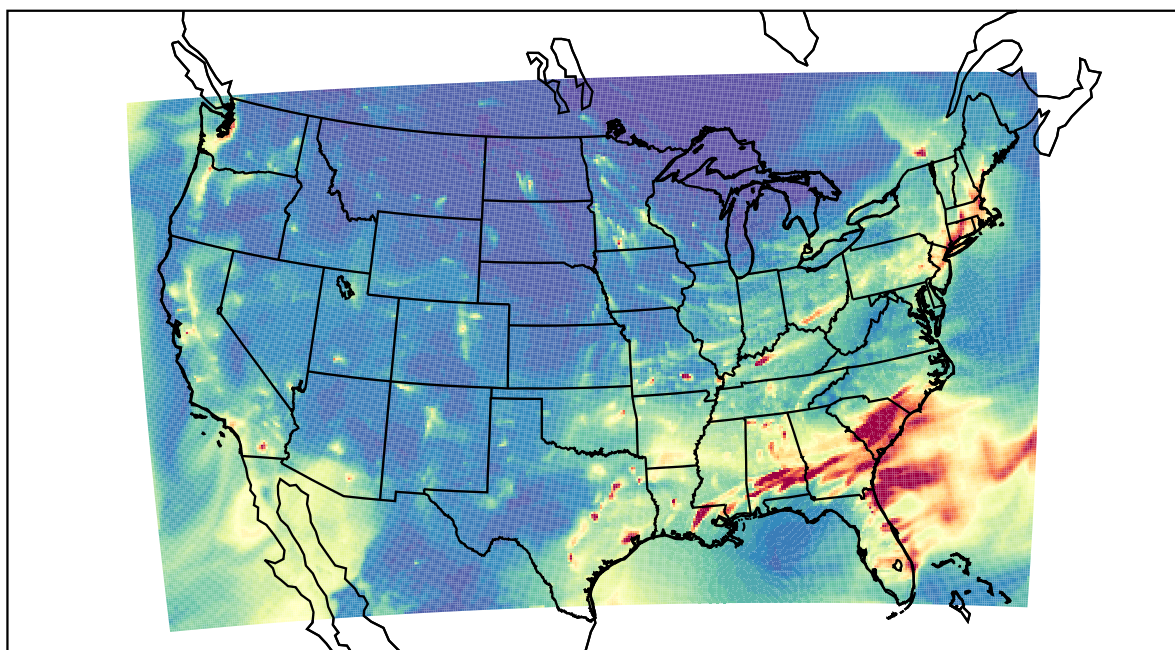
WRF 2021-01-22_04:00:00
