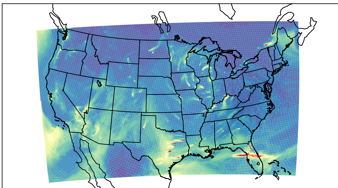
WRF 2021-01-23_17:00:00
