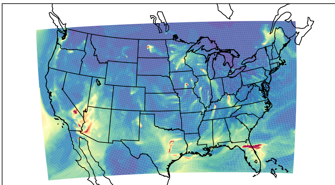
WRF 2021-01-23_08:00:00
