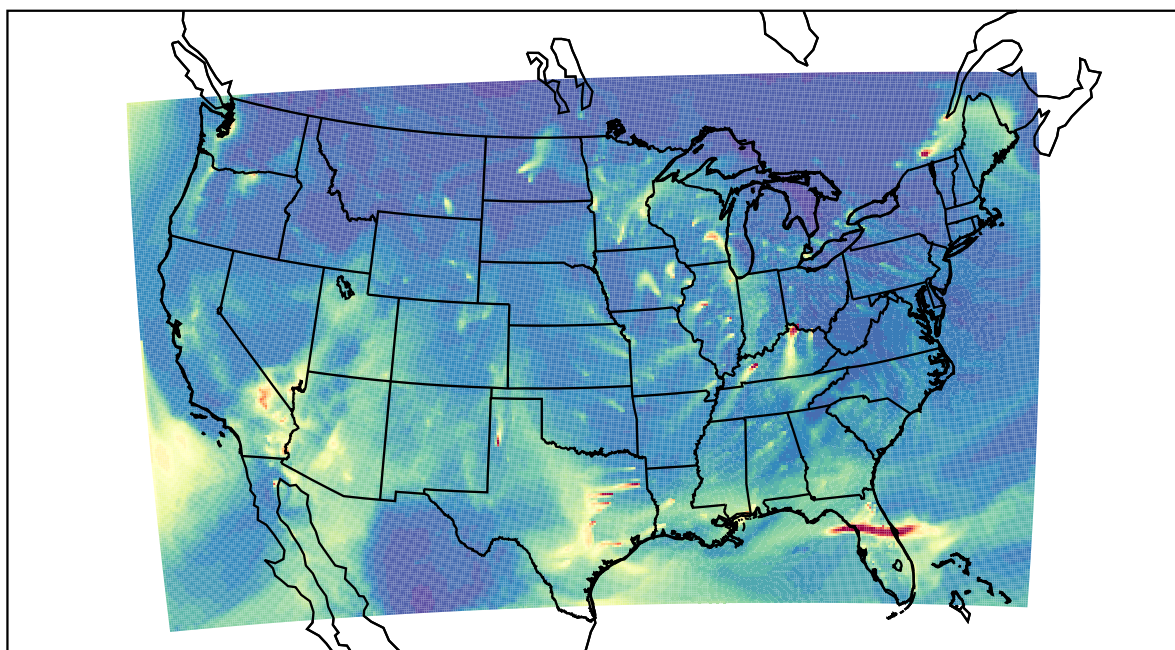
WRF 2021-01-23_14:00:00
