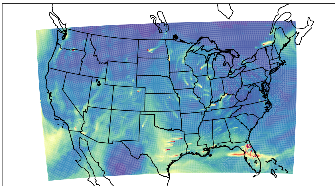
WRF 2021-01-23_19:00:00
