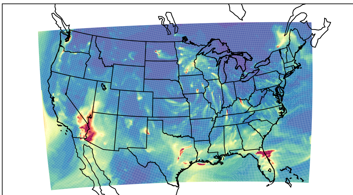
WRF 2021-01-23_05:00:00
