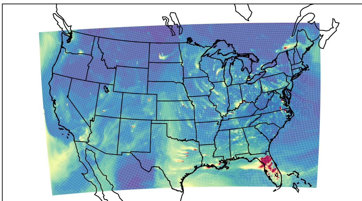
WRF 2021-01-23_23:00:00
