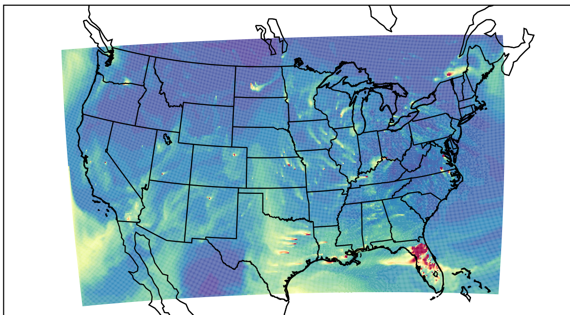
WRF 2021-01-23_22:00:00
