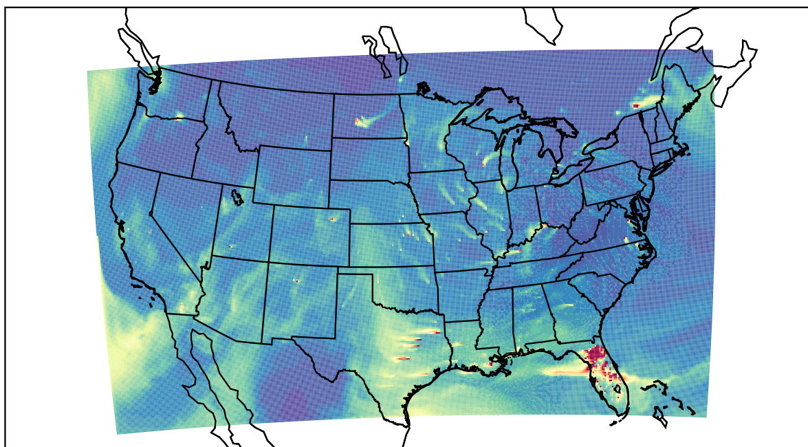
WRF 2021-01-23_21:00:00
