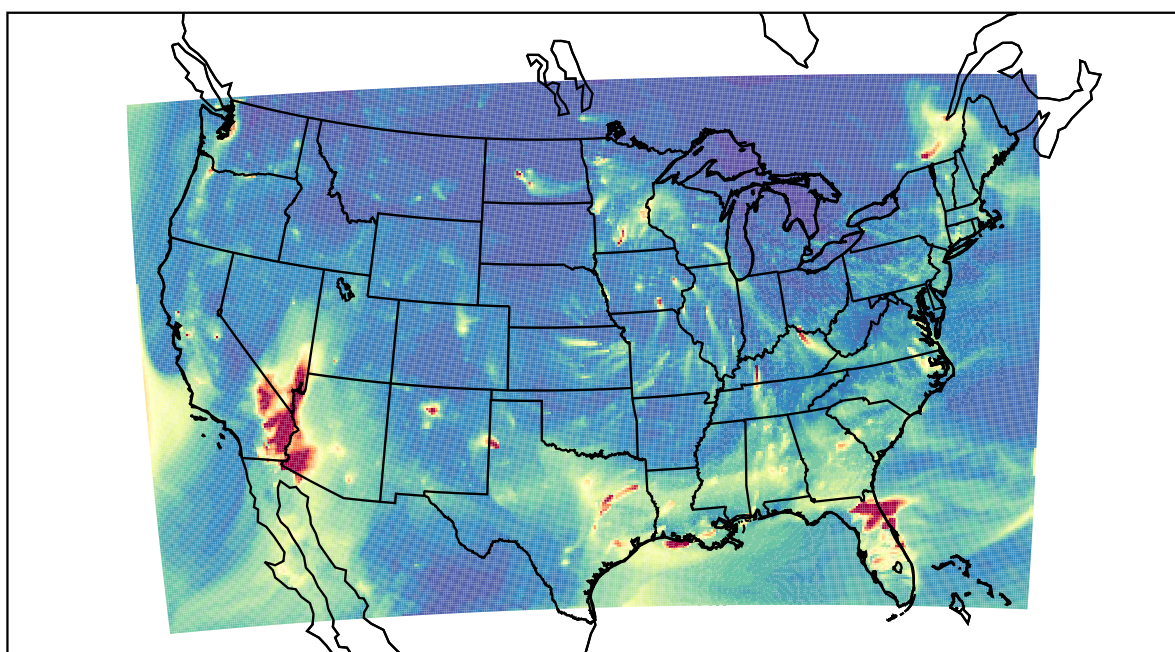
WRF 2021-01-23_03:00:00
