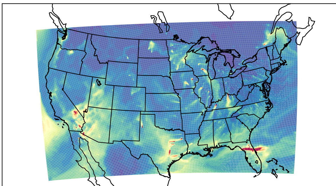
WRF 2021-01-23_11:00:00
