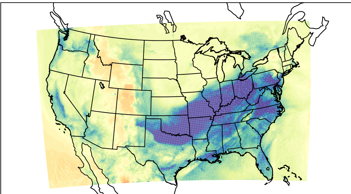
WRF (2021-01-26_11:00:00)
