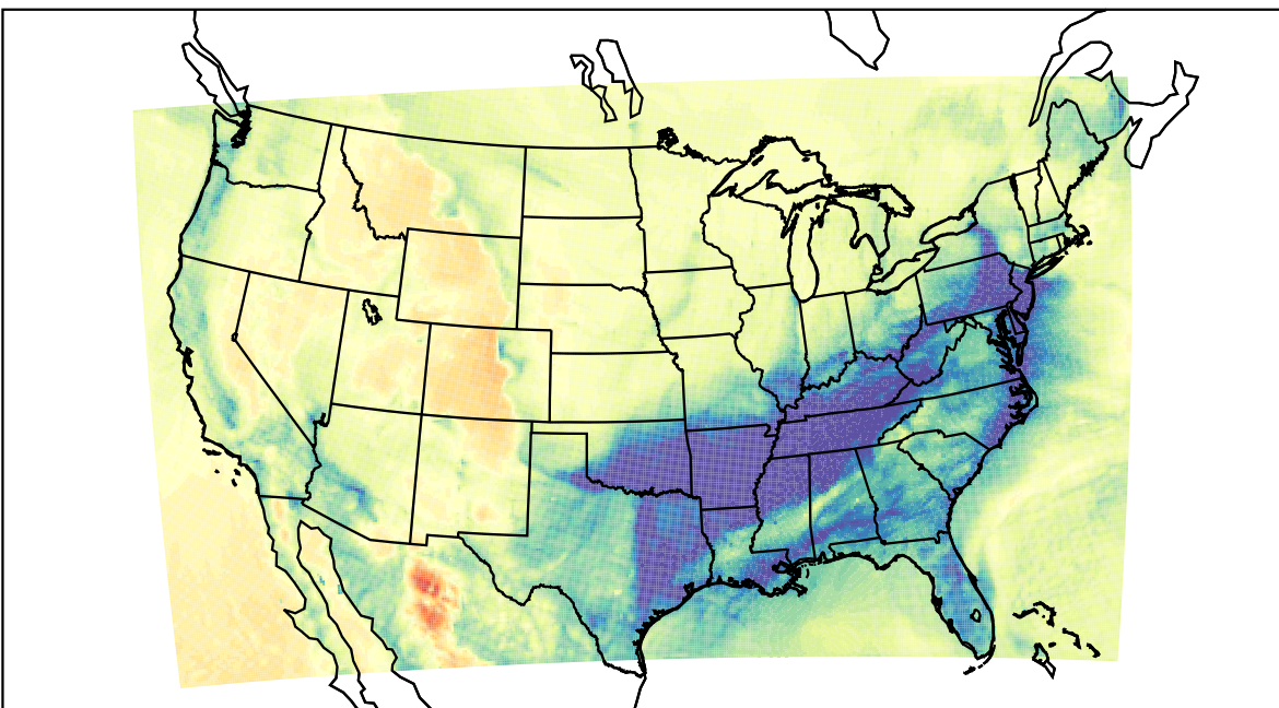
WRF (2021-01-27_09:00:00)
