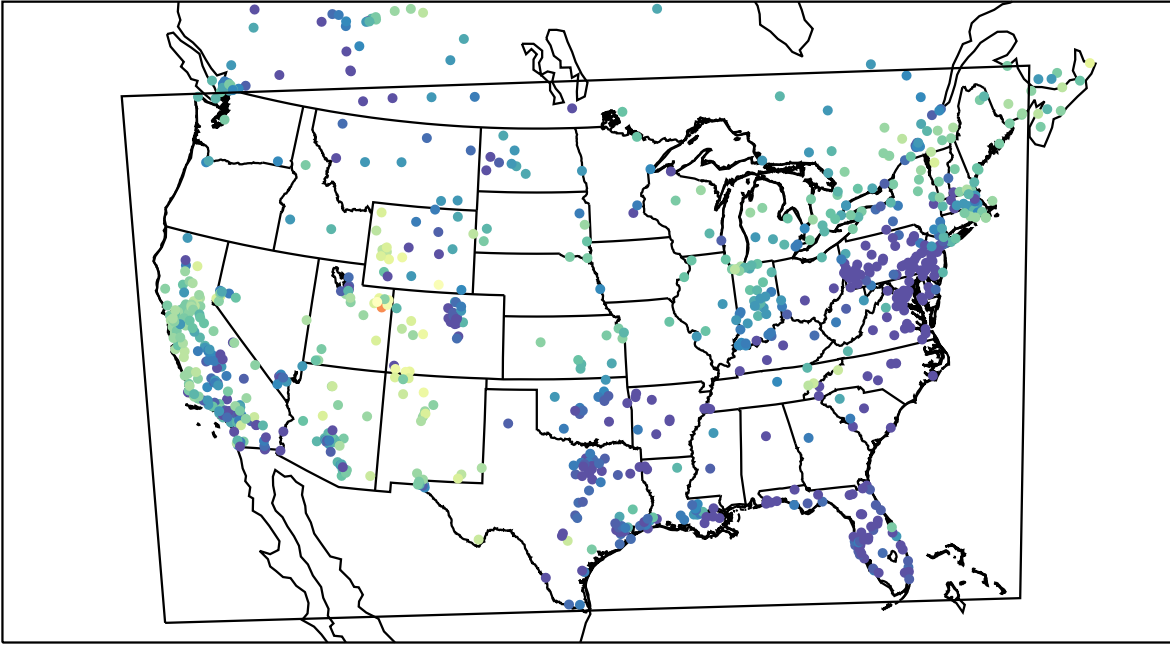
AirNOW (2021-01-27_02:00:00)
