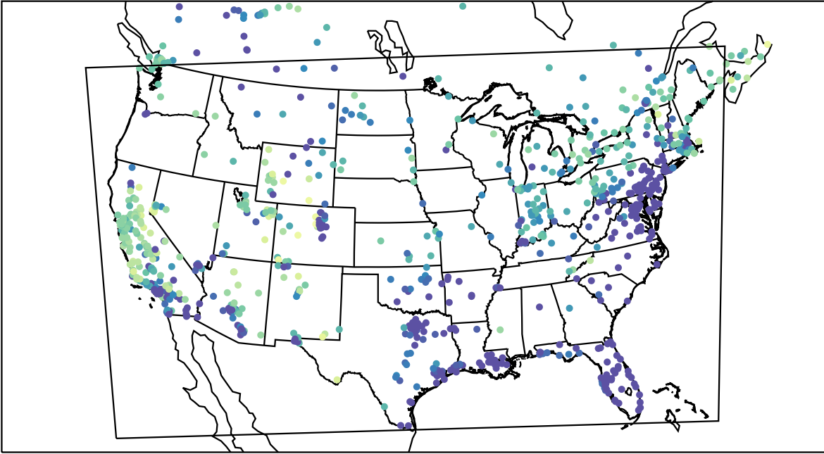
AirNOW (2021-01-27_08:00:00)
