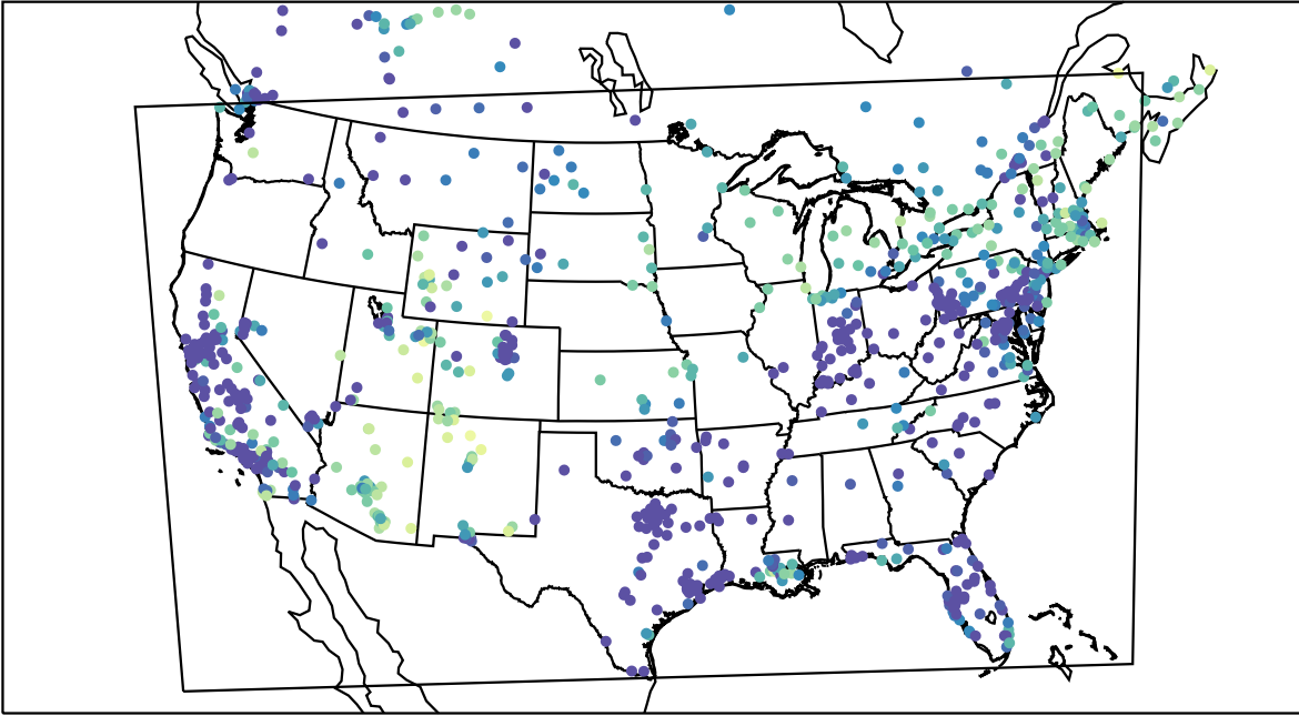
AirNOW (2021-01-26_14:00:00)
