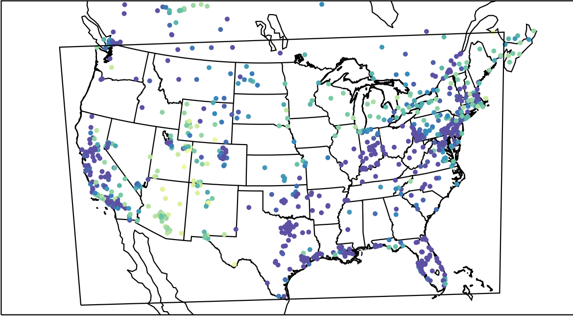
AirNOW (2021-01-26_11:00:00)
