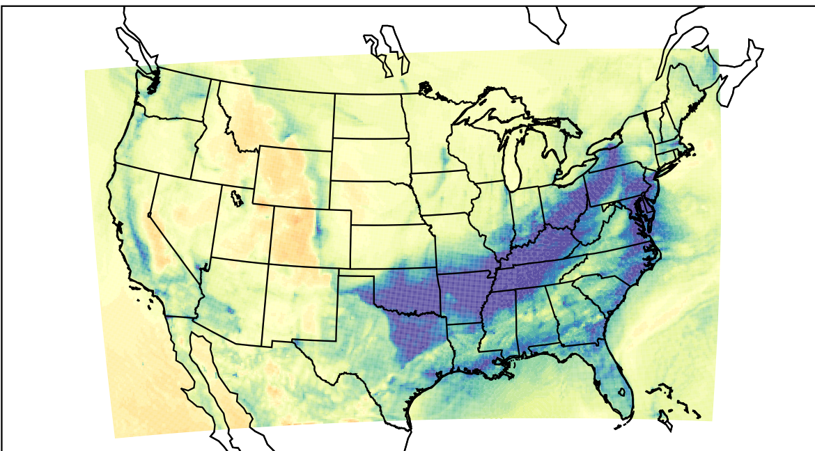
WRF (2021-01-27_04:00:00)
