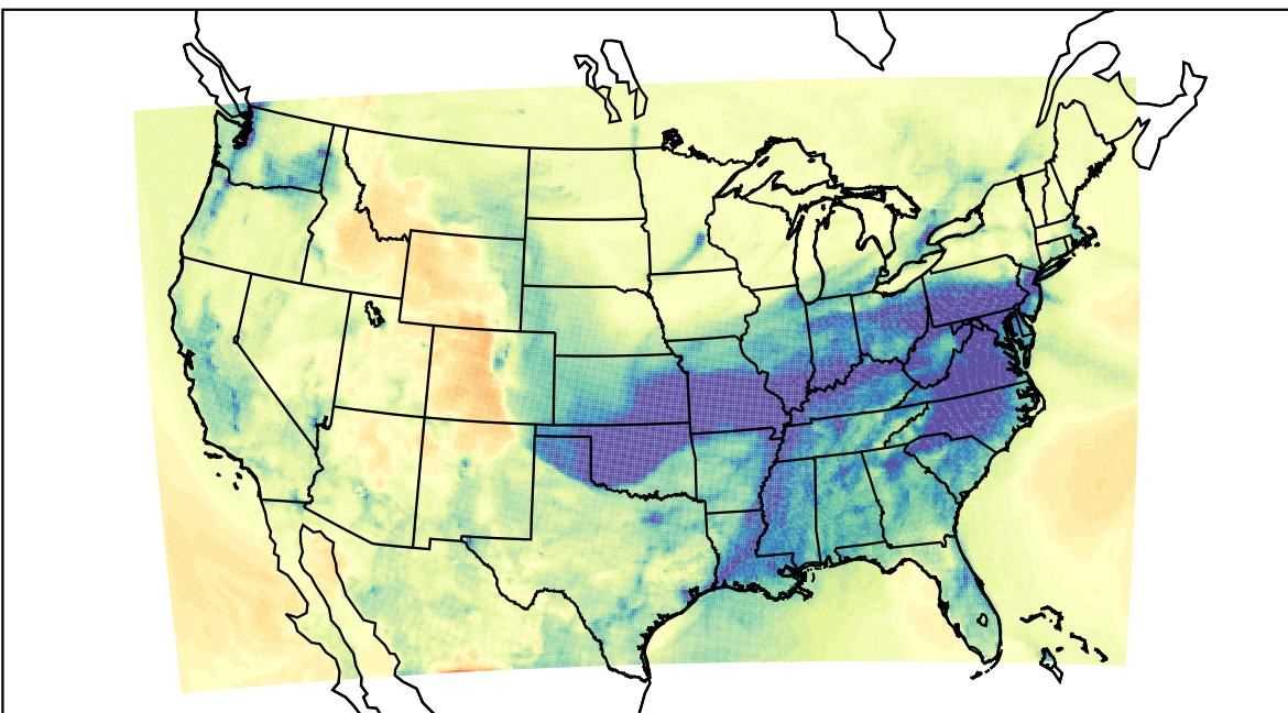
WRF (2021-01-26_02:00:00)
