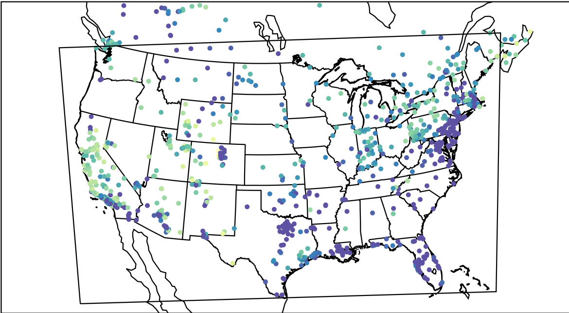
AirNOW (2021-01-27_11:00:00)
