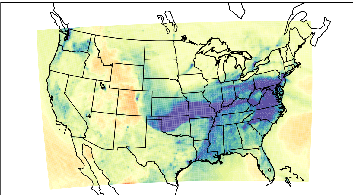
WRF (2021-01-26_01:00:00)
