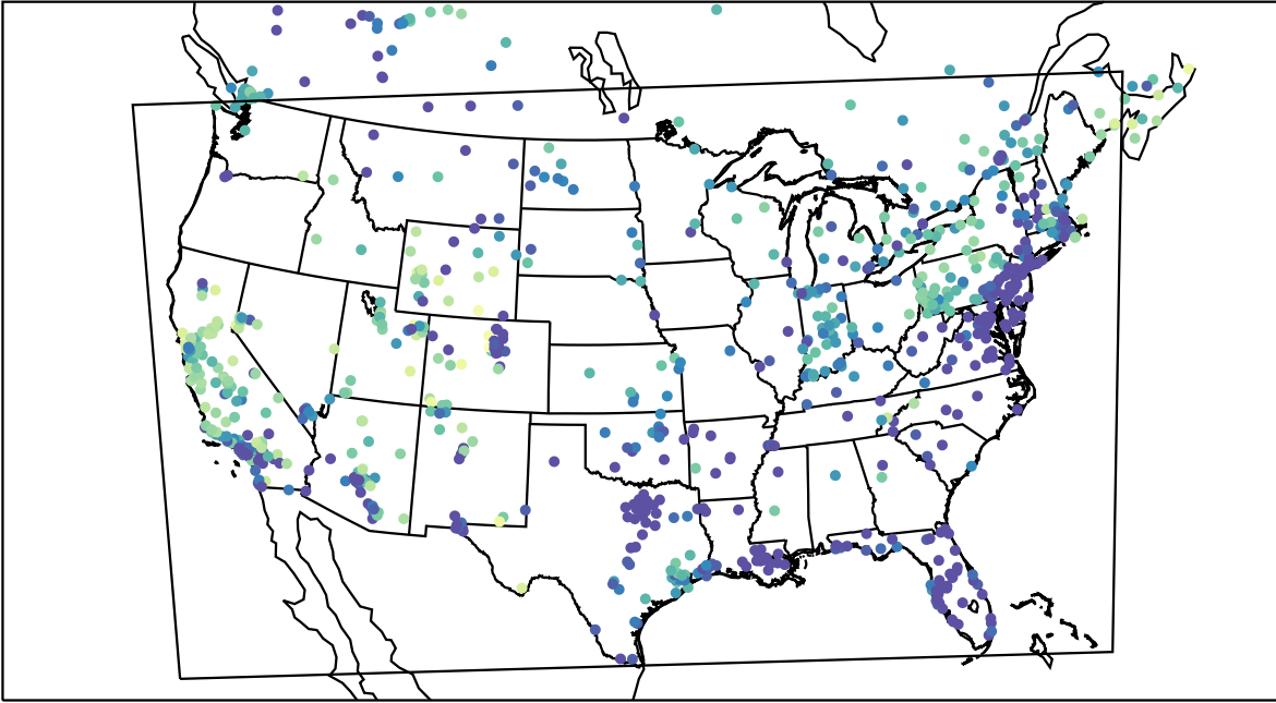
AirNOW (2021-01-27_12:00:00)
