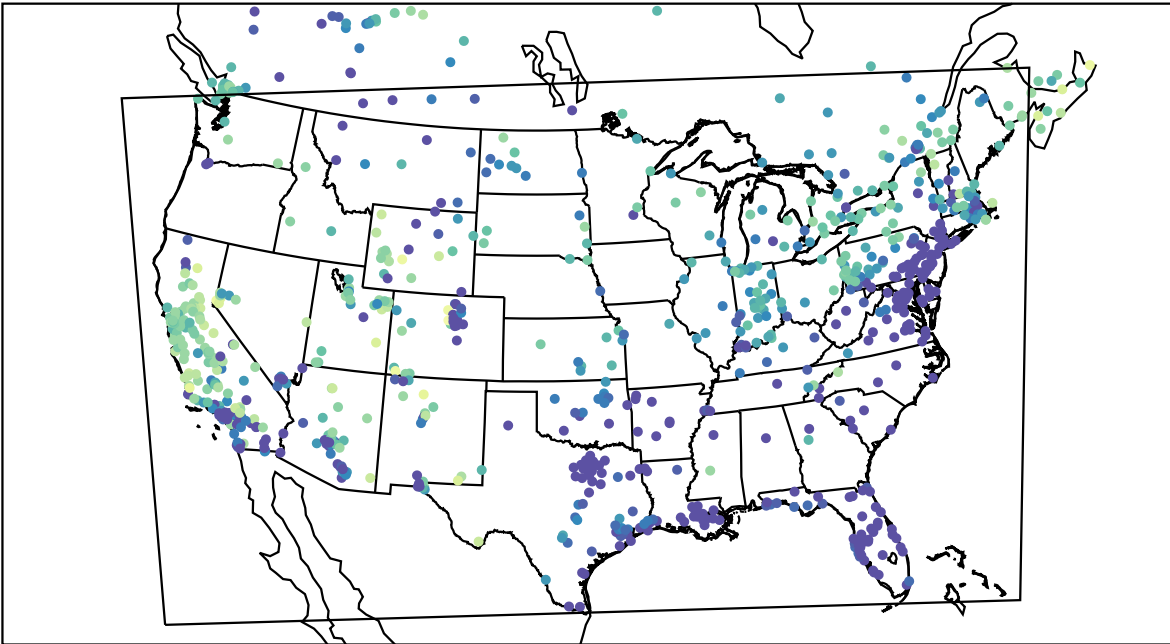
AirNOW (2021-01-27_09:00:00)
