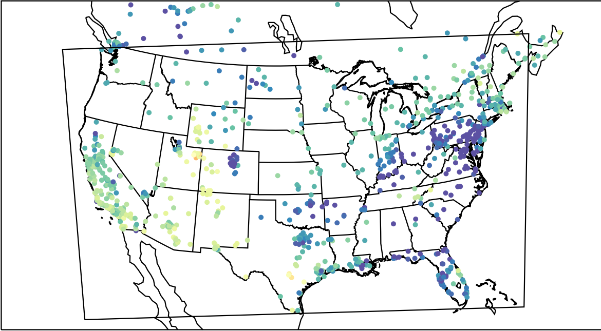
AirNOW (2021-01-26_23:00:00)
