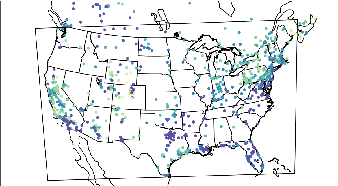
AirNOW (2021-01-27_15:00:00)
