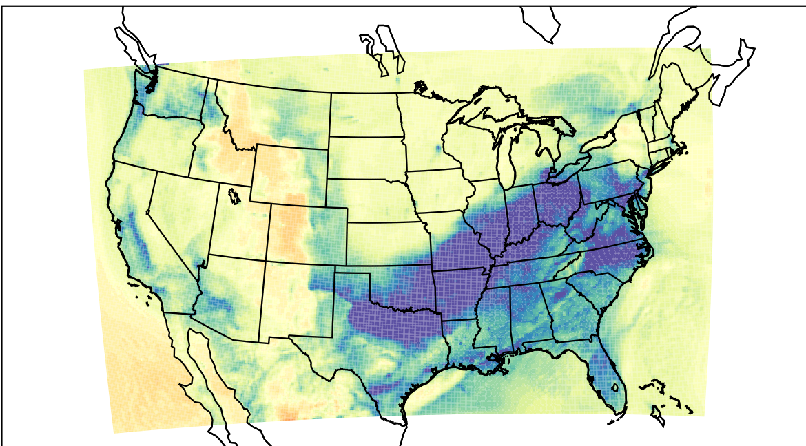
WRF (2021-01-26_14:00:00)
