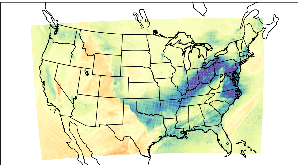
WRF (2021-01-26_22:00:00)
