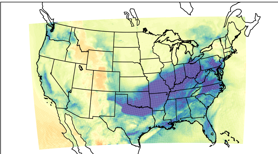
WRF (2021-01-26_12:00:00)
