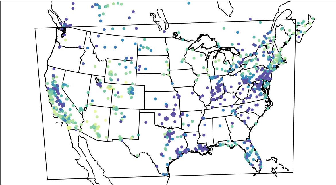
AirNOW (2021-01-26_02:00:00)
