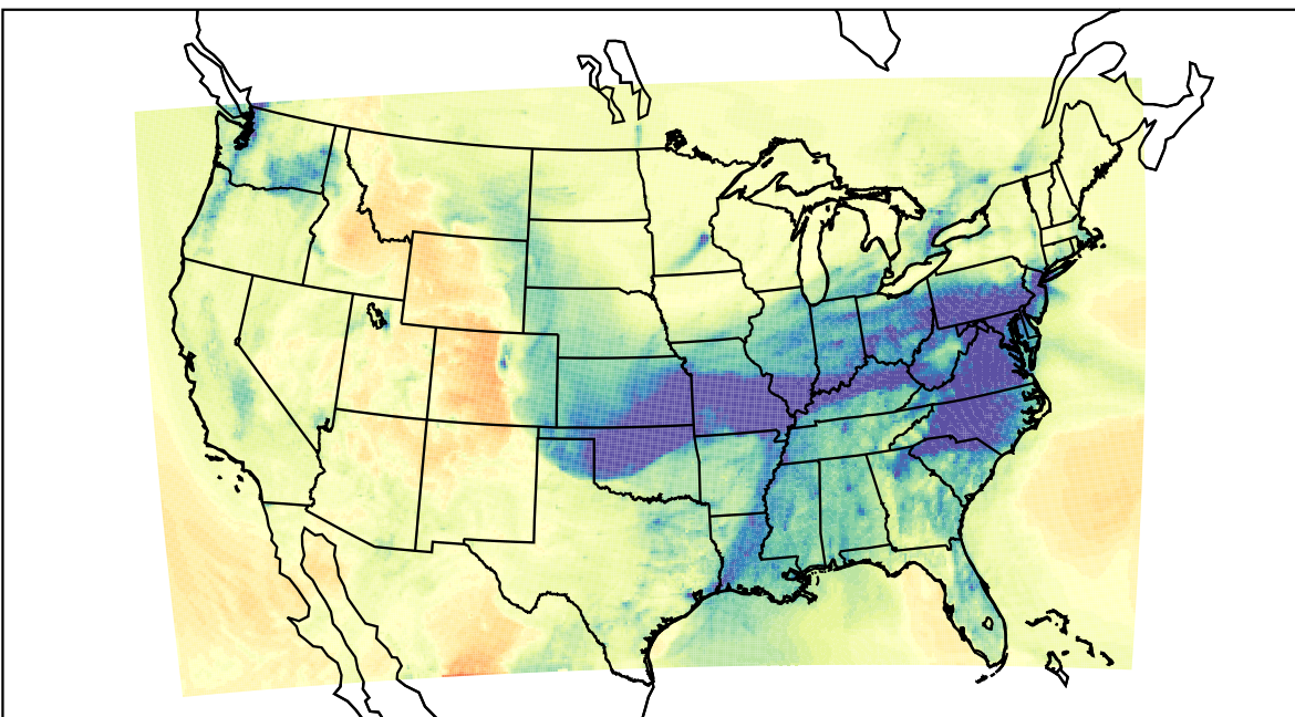
WRF (2021-01-26_00:00:00)
