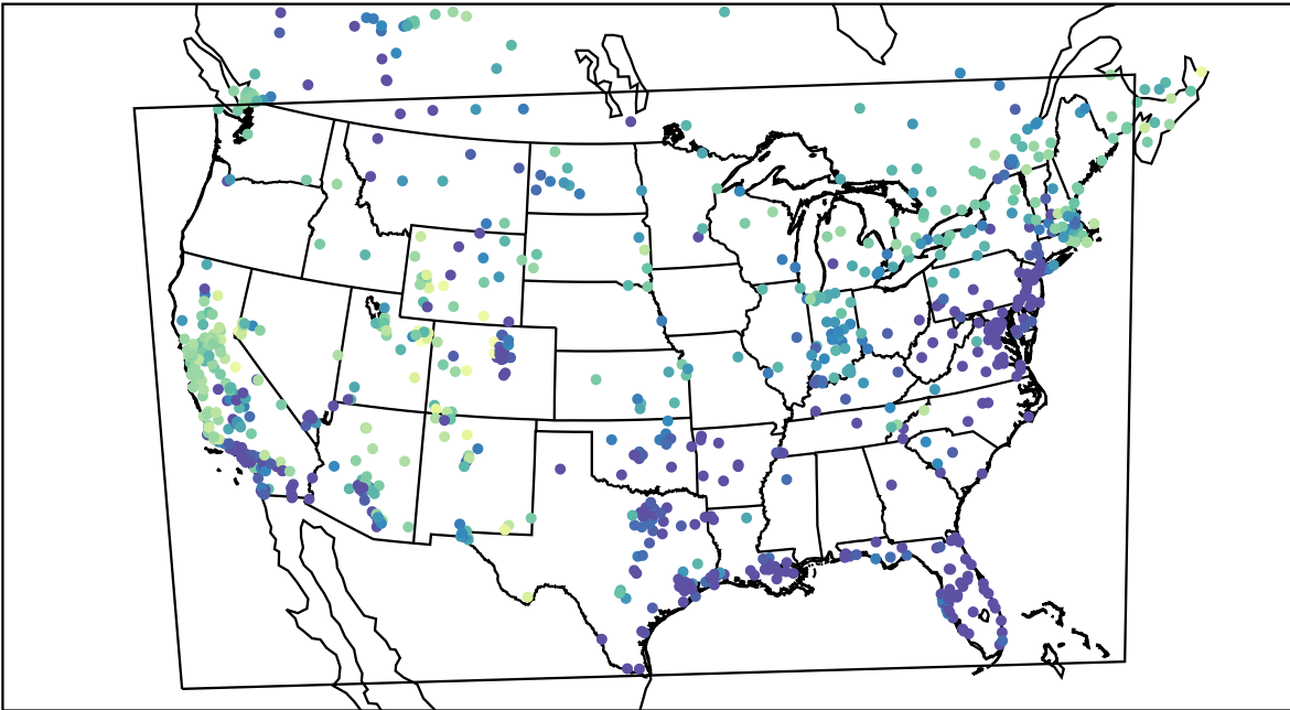
AirNOW (2021-01-27_06:00:00)
