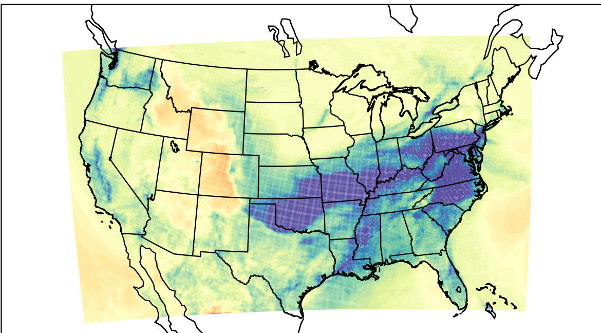
WRF (2021-01-26_04:00:00)
