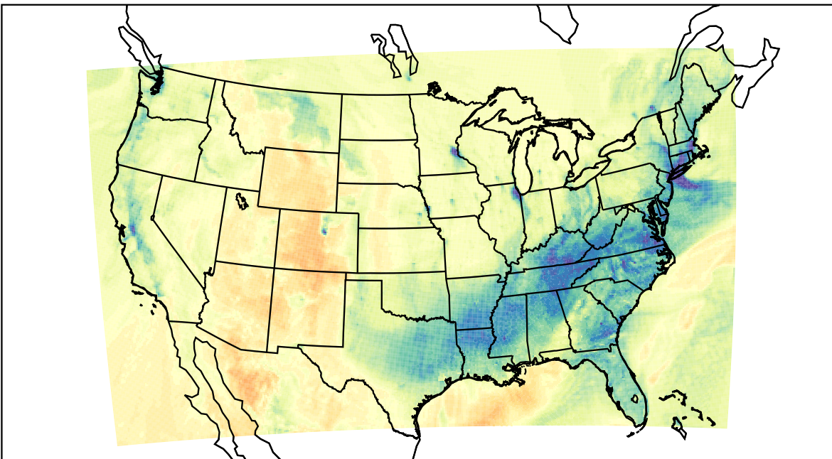
WRF (2021-01-27_23:00:00)
