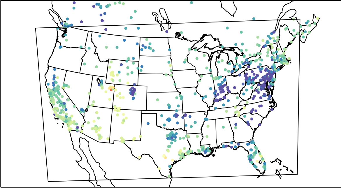
AirNOW (2021-01-26_21:00:00)
