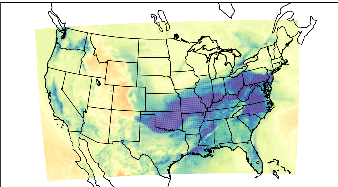
WRF (2021-01-26_06:00:00)
