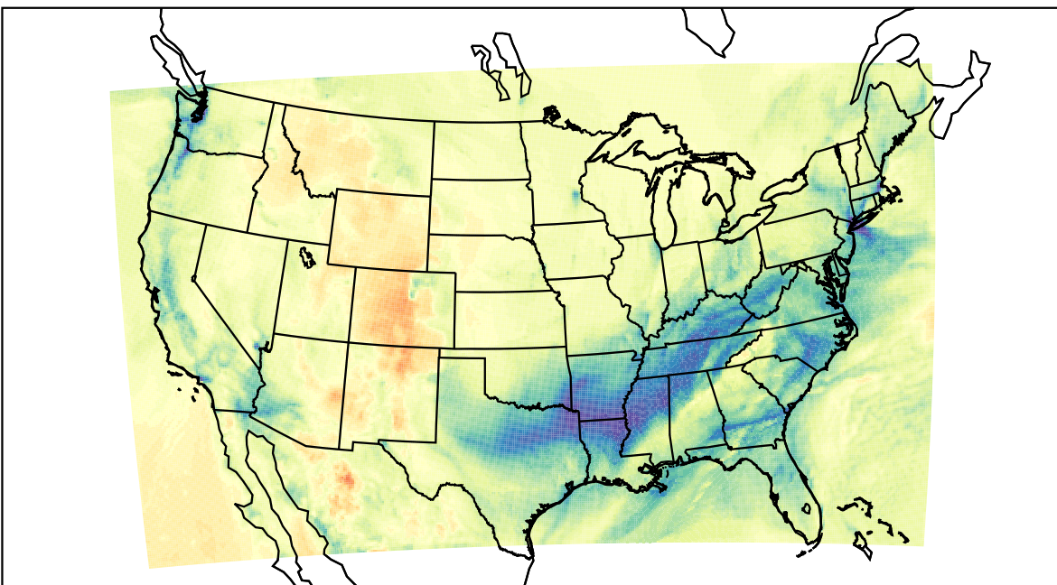
WRF (2021-01-27_17:00:00)
