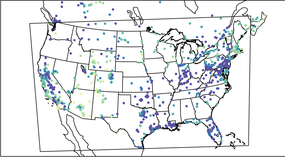
AirNOW (2021-01-26_05:00:00)
