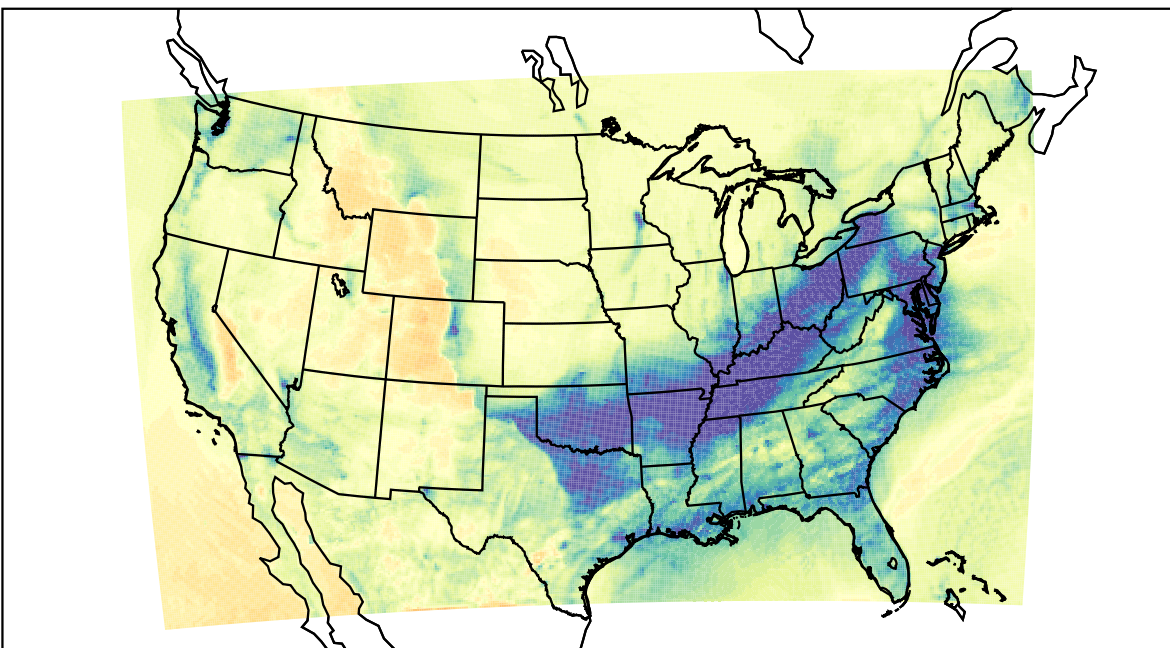
WRF (2021-01-27_02:00:00)
