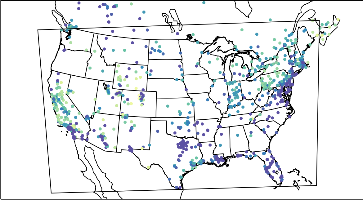
AirNOW (2021-01-27_14:00:00)
