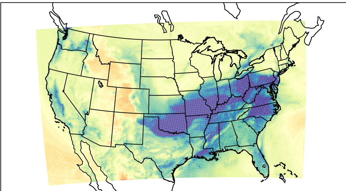
WRF (2021-01-26_07:00:00)
