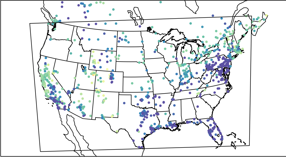
AirNOW (2021-01-27_04:00:00)
