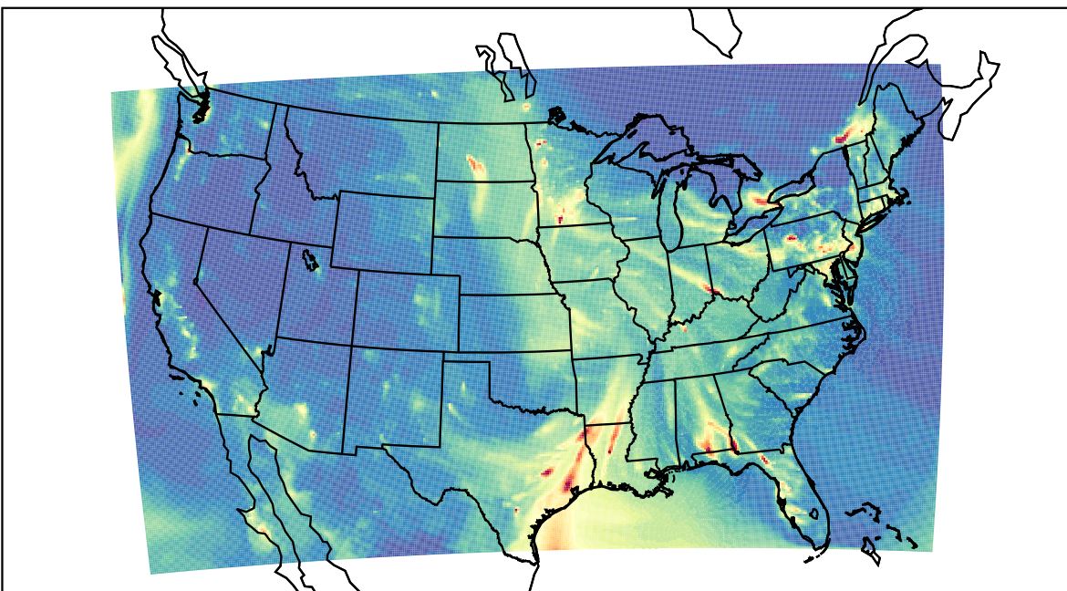
WRF 2021-01-31_04:00:00
