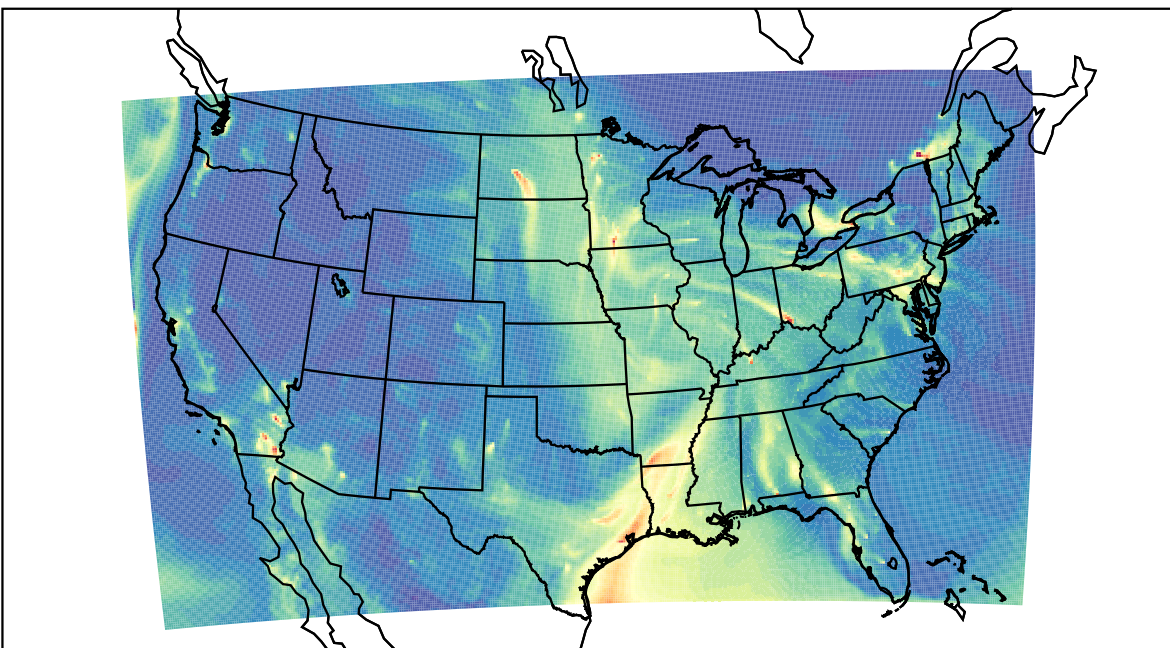
WRF 2021-01-31_07:00:00
