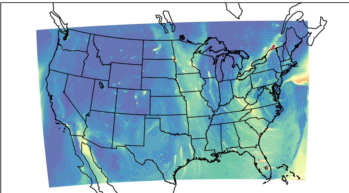
WRF 2021-02-01_21:00:00
