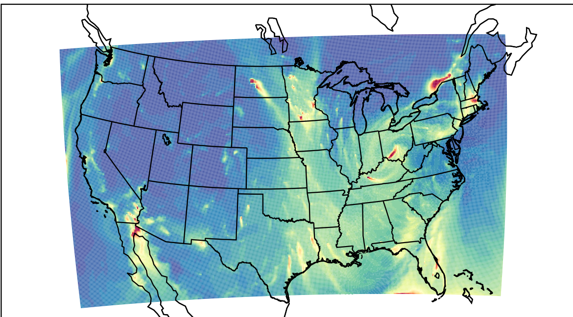
WRF 2021-02-01_05:00:00
