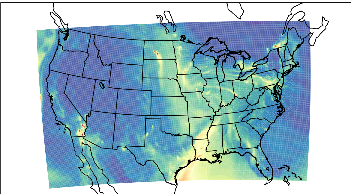
WRF 2021-01-31_09:00:00
