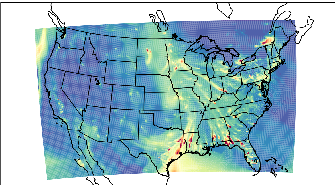
WRF 2021-01-31_01:00:00
