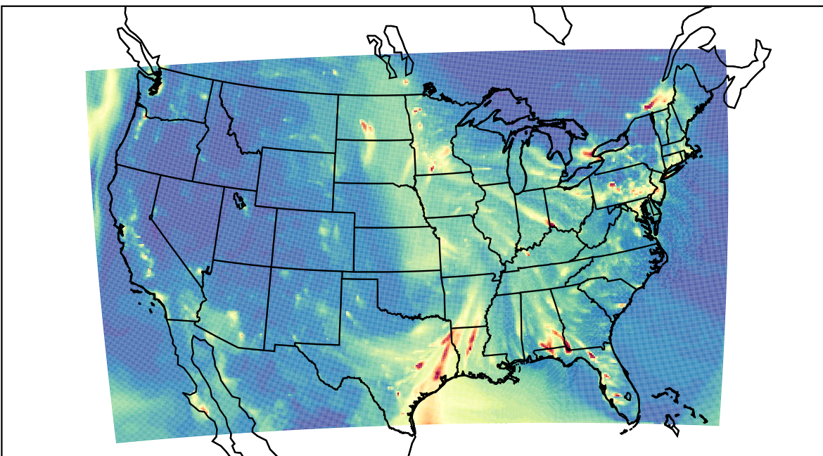
WRF 2021-01-31_03:00:00
