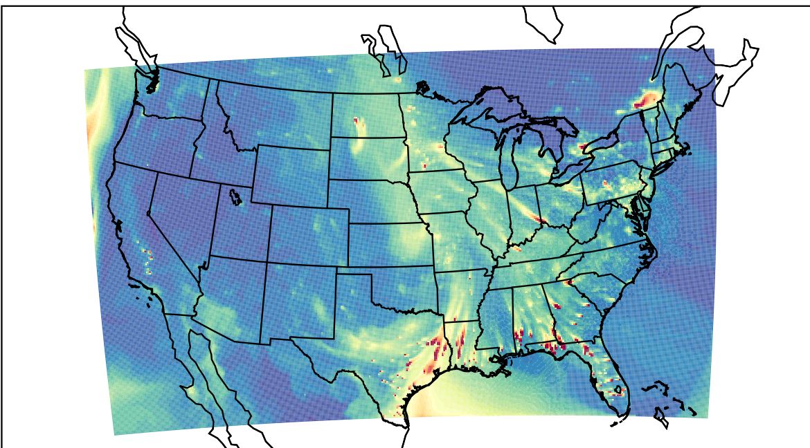
WRF 2021-01-31_00:00:00
