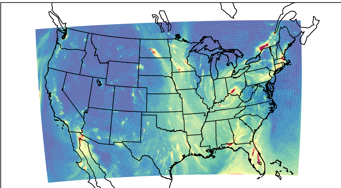
WRF 2021-02-01_02:00:00
