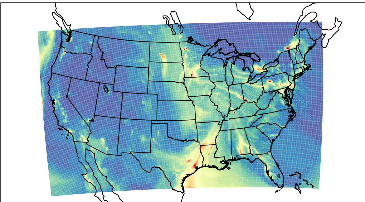
WRF 2021-01-31_05:00:00
