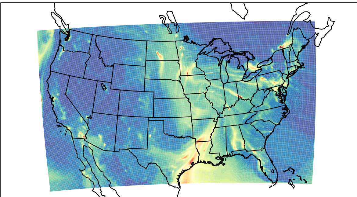
WRF 2021-01-31_06:00:00
