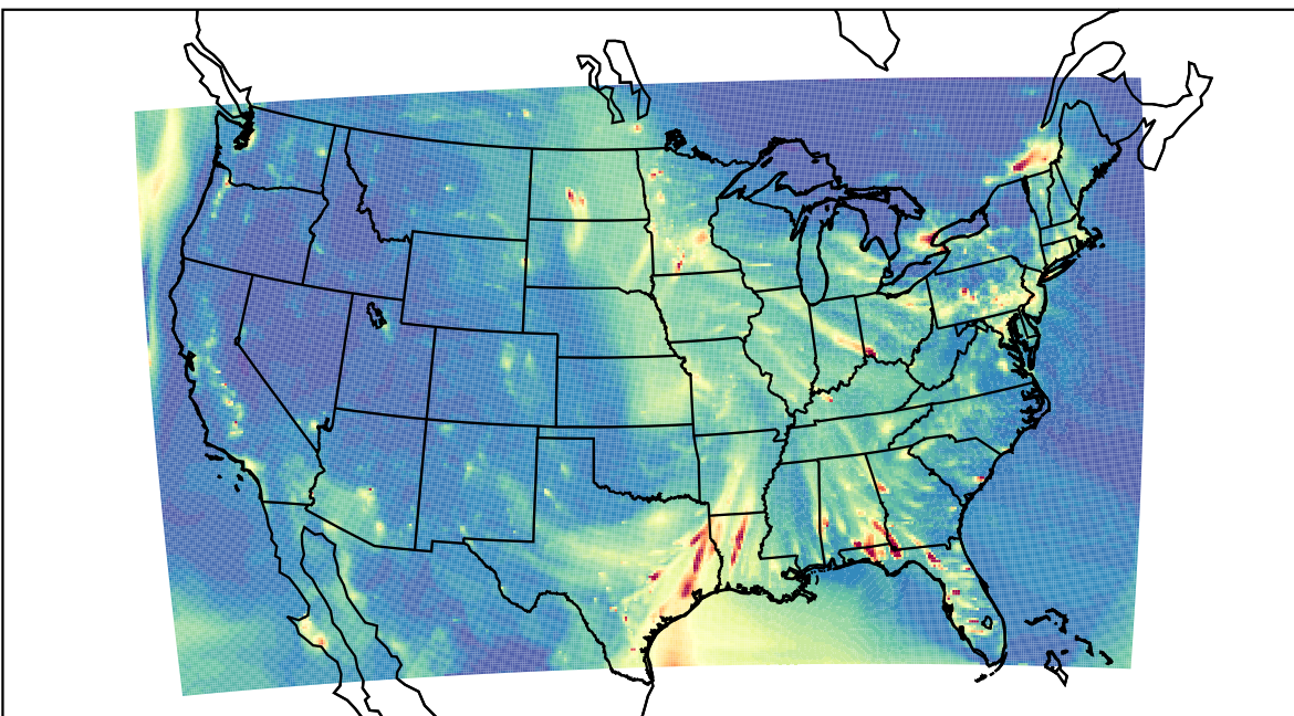
WRF 2021-01-31_02:00:00
