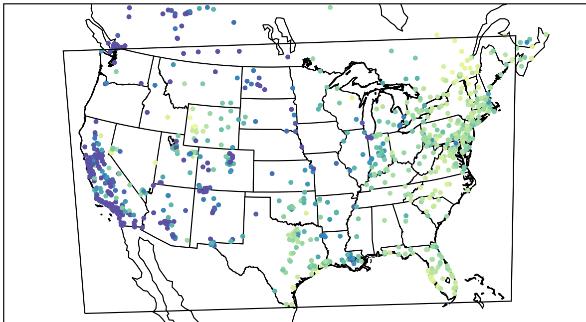
AirNOW (2021-02-03_16:00:00)
