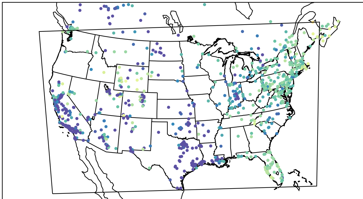
AirNOW (2021-02-02_12:00:00)
