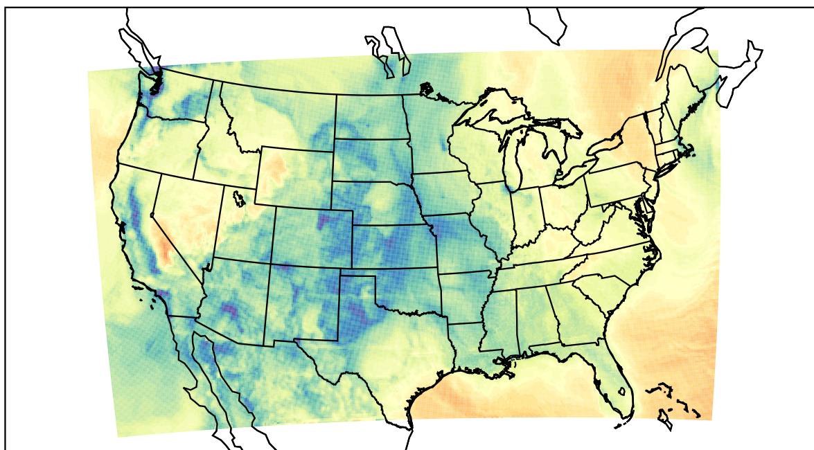
WRF (2021-02-03_17:00:00)
