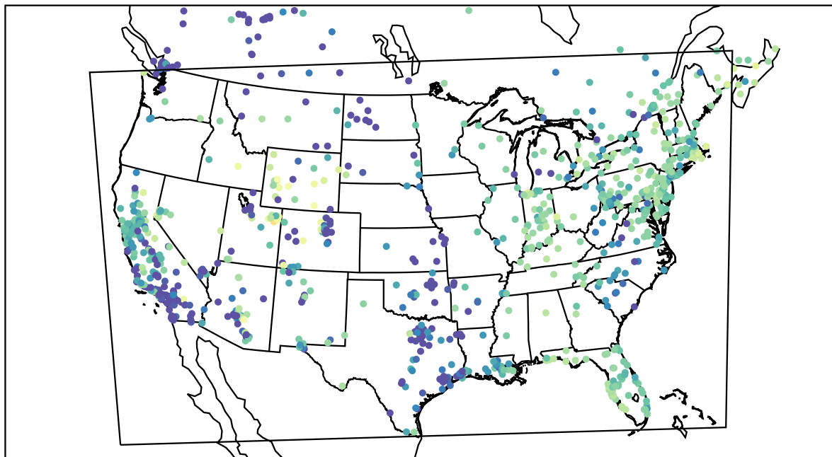
AirNOW (2021-02-02_03:00:00)
