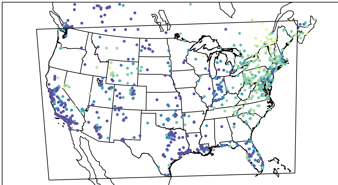
AirNOW (2021-02-03_12:00:00)
