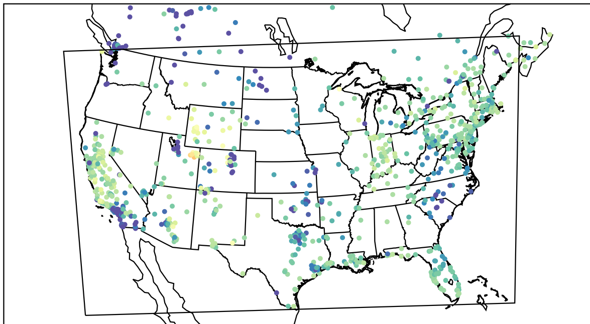
AirNOW (2021-02-02_00:00:00)
