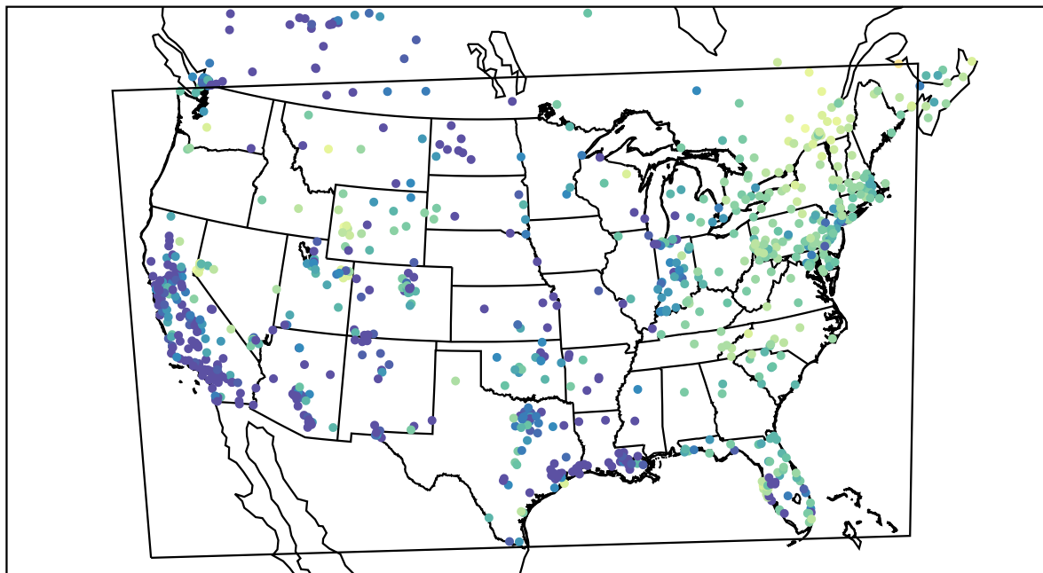
AirNOW (2021-02-03_09:00:00)
