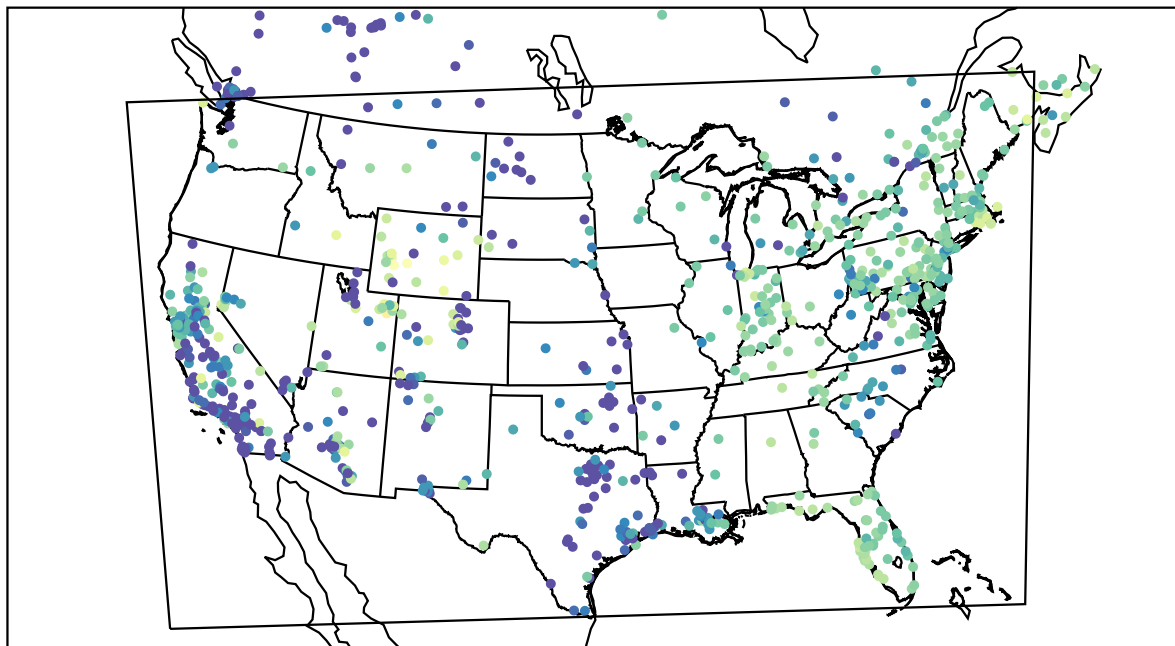
AirNOW (2021-02-02_05:00:00)
