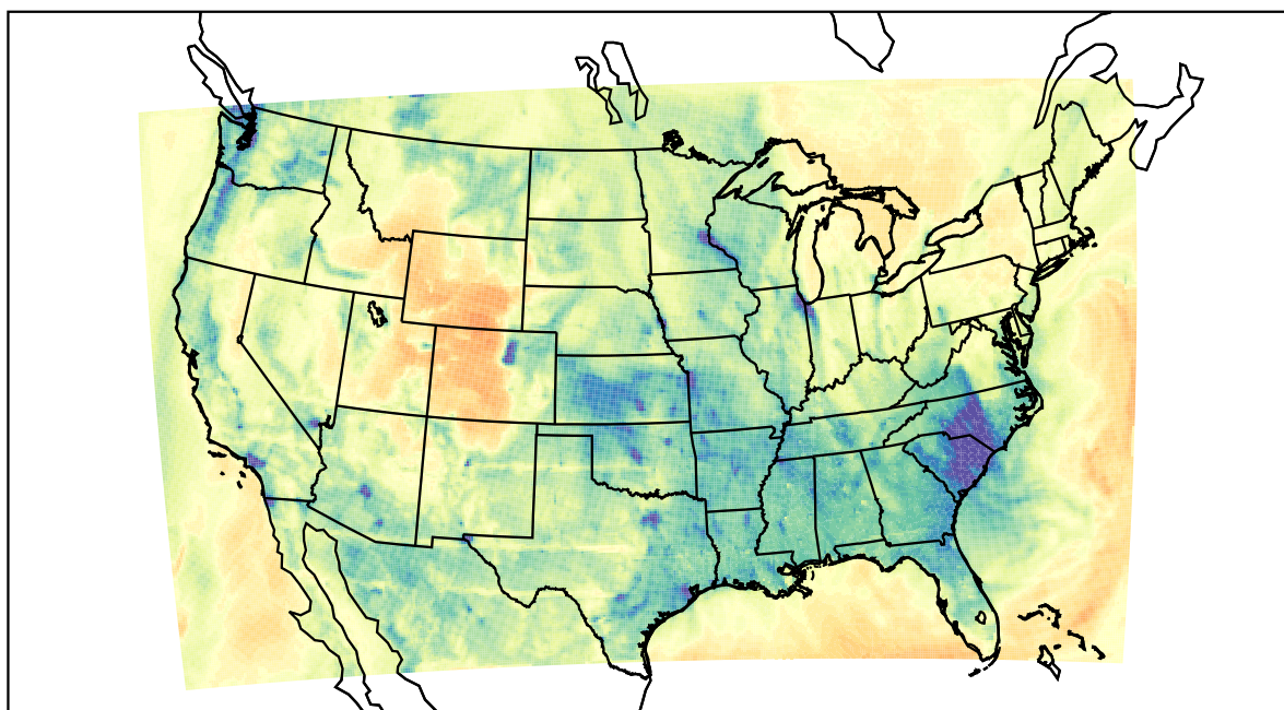
WRF (2021-02-02_02:00:00)
