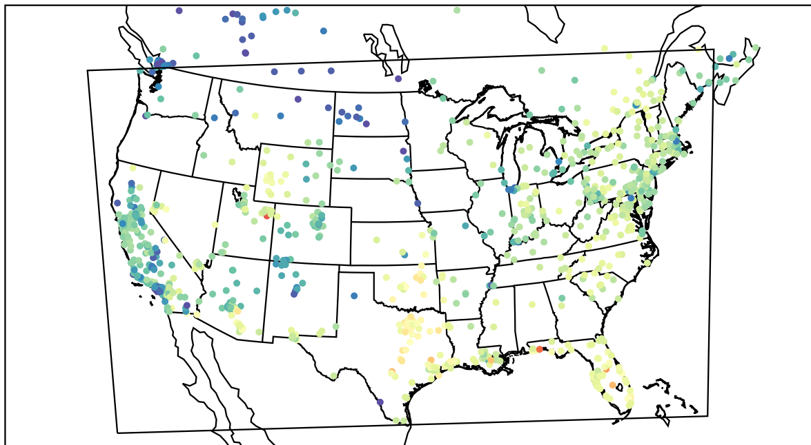
AirNOW (2021-02-03_20:00:00)
