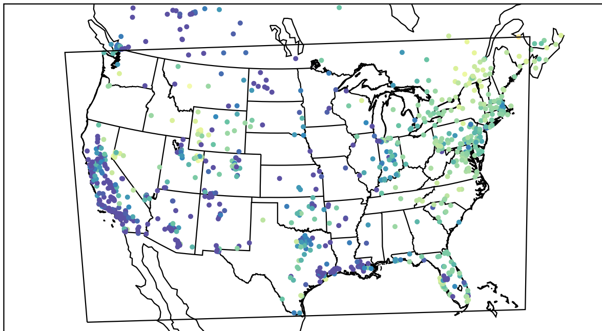
AirNOW (2021-02-03_07:00:00)
