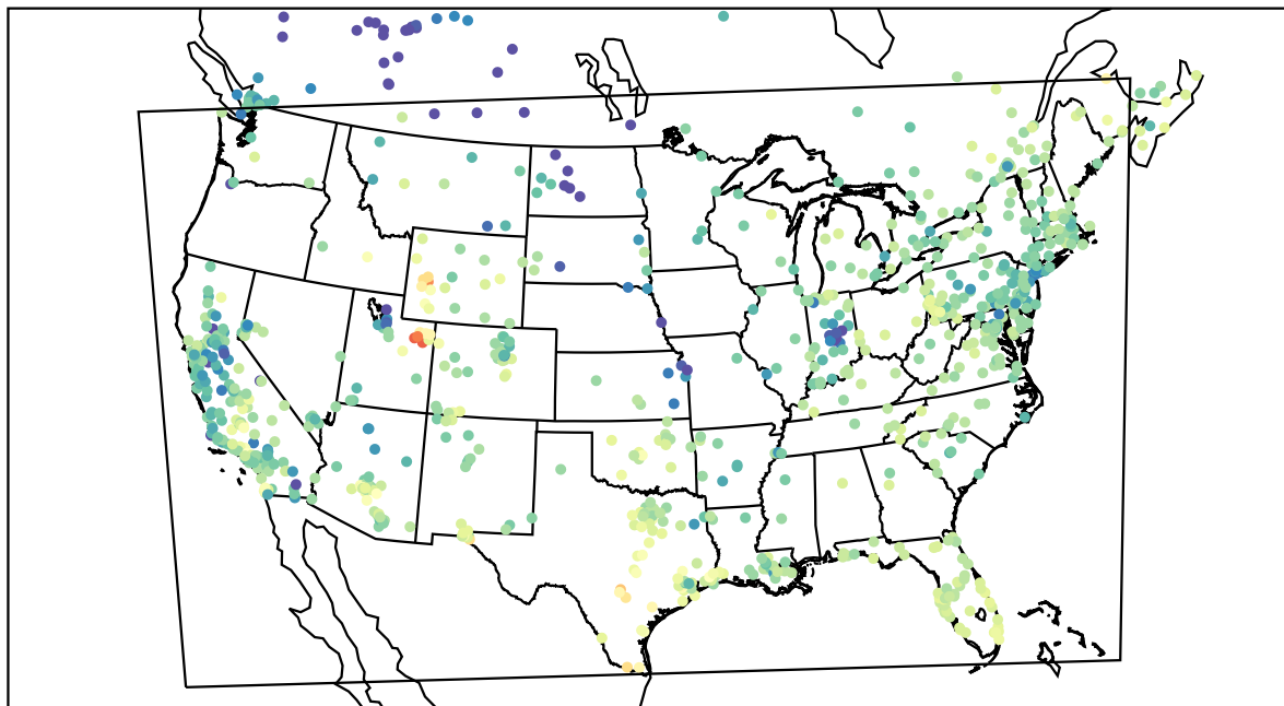
AirNOW (2021-02-02_22:00:00)
