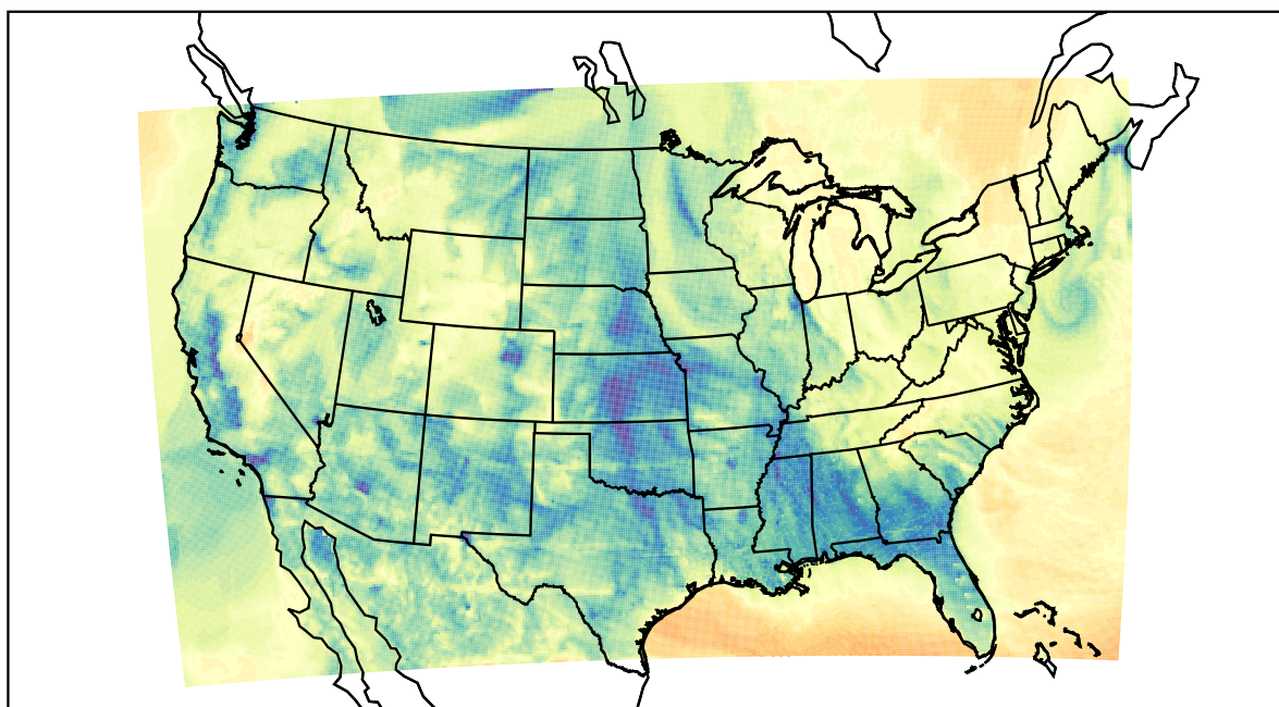
WRF (2021-02-03_05:00:00)
