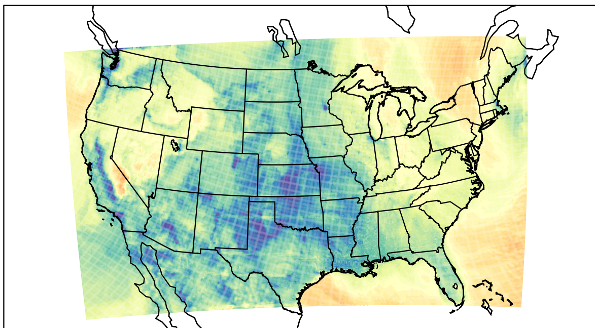
WRF (2021-02-03_15:00:00)
