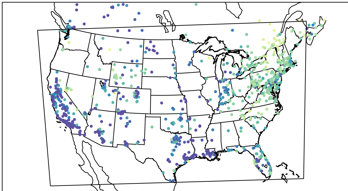
AirNOW (2021-02-03_10:00:00)
