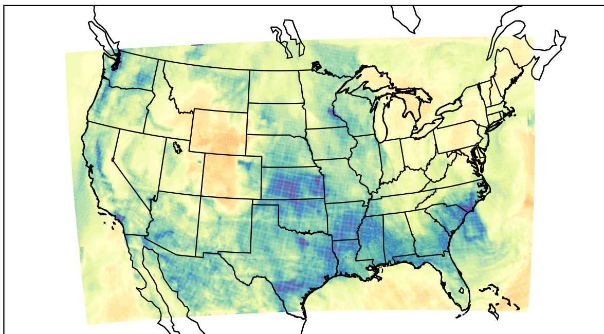
WRF (2021-02-02_09:00:00)
