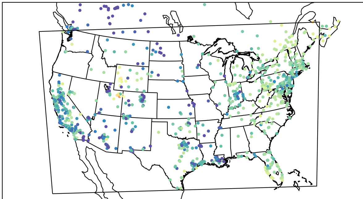
AirNOW (2021-02-03_01:00:00)
