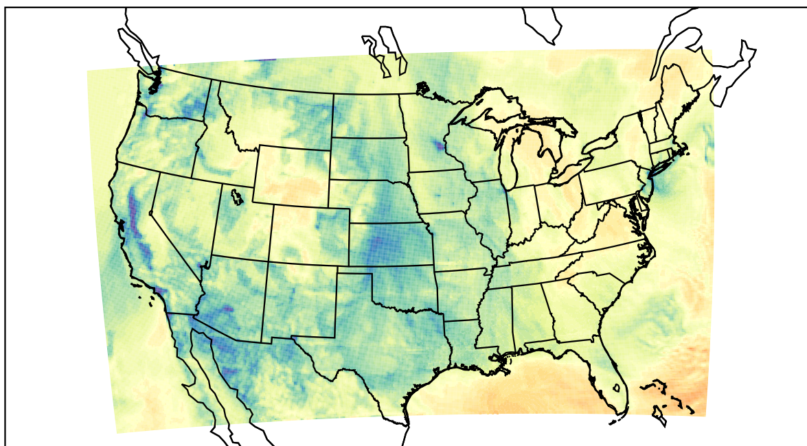
WRF (2021-02-02_17:00:00)
