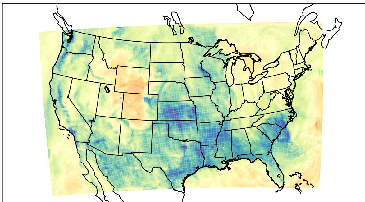
WRF (2021-02-02_07:00:00)
