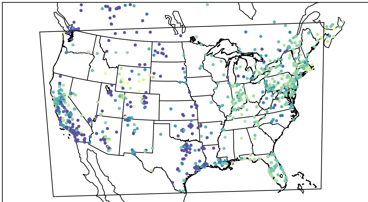
AirNOW (2021-02-02_04:00:00)
