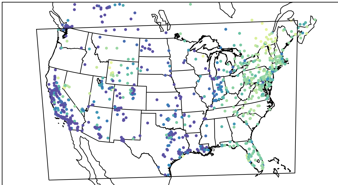
AirNOW (2021-02-03_14:00:00)
