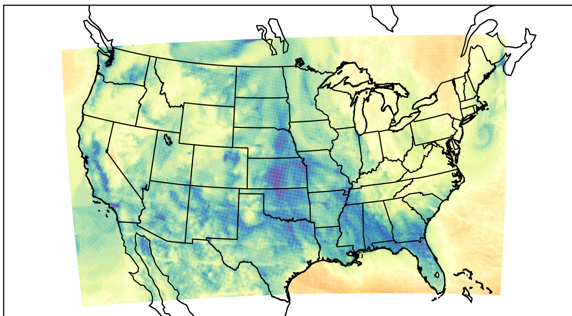
WRF (2021-02-03_08:00:00)
