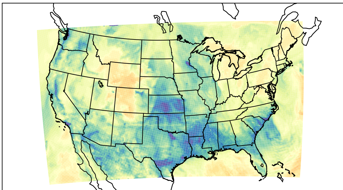
WRF (2021-02-02_11:00:00)
