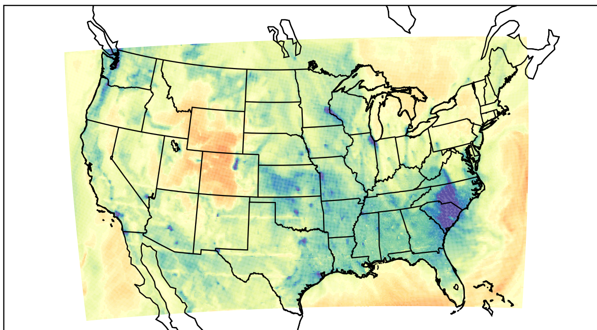
WRF (2021-02-02_01:00:00)
