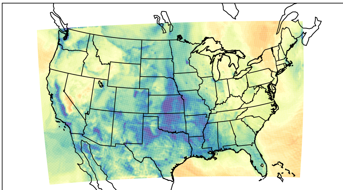
WRF (2021-02-03_14:00:00)
