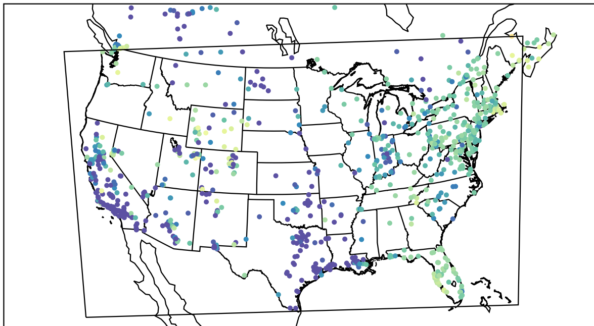
AirNOW (2021-02-02_11:00:00)
