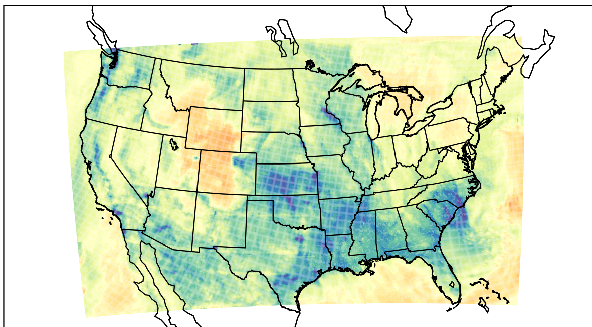
WRF (2021-02-02_06:00:00)
