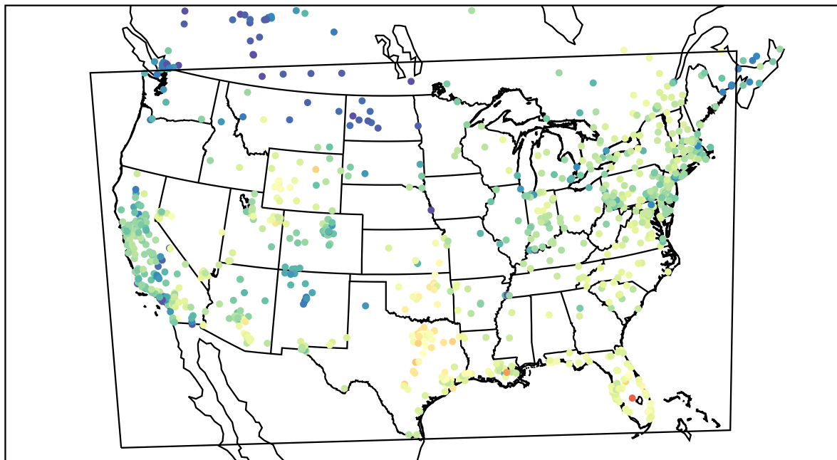
AirNOW (2021-02-03_21:00:00)
