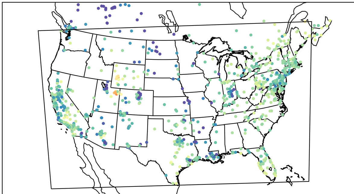
AirNOW (2021-02-03_00:00:00)
