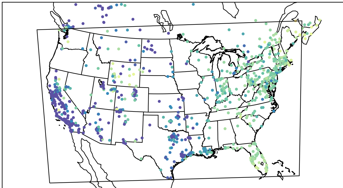
AirNOW (2021-02-02_15:00:00)
