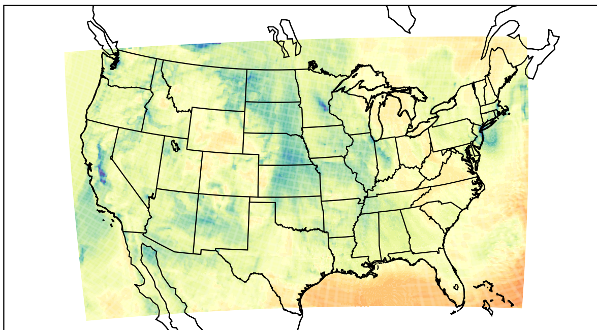
WRF (2021-02-02_21:00:00)
