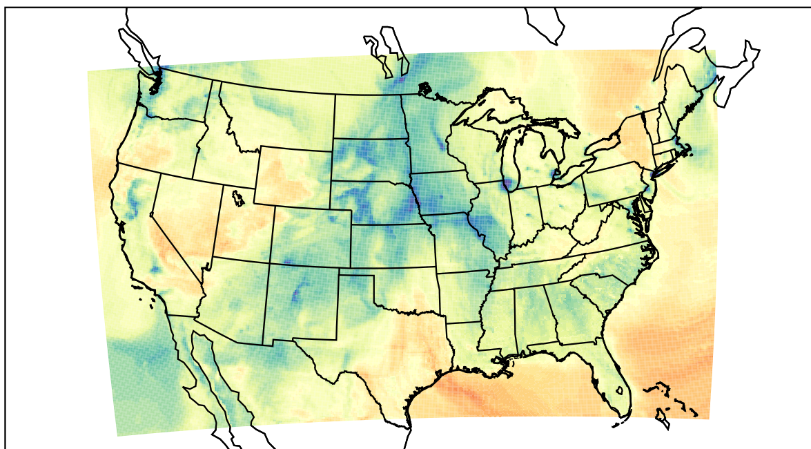
WRF (2021-02-03_22:00:00)
