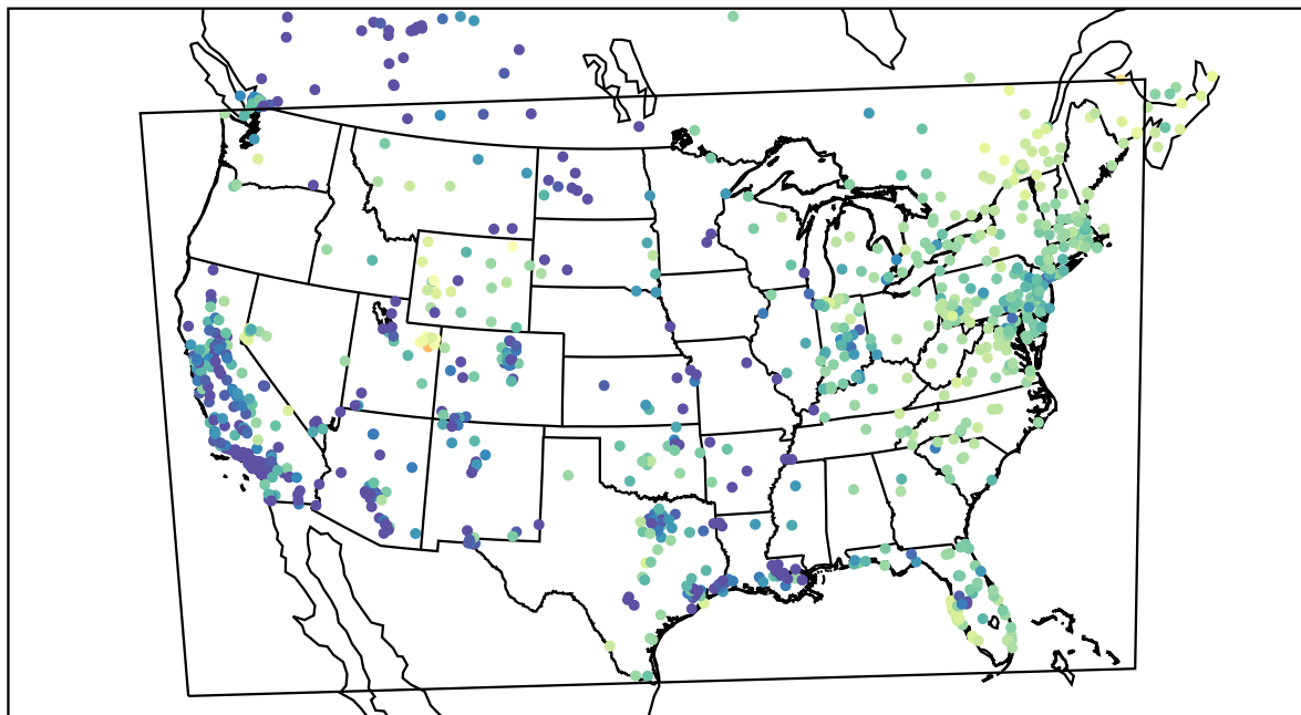
AirNOW (2021-02-03_03:00:00)
