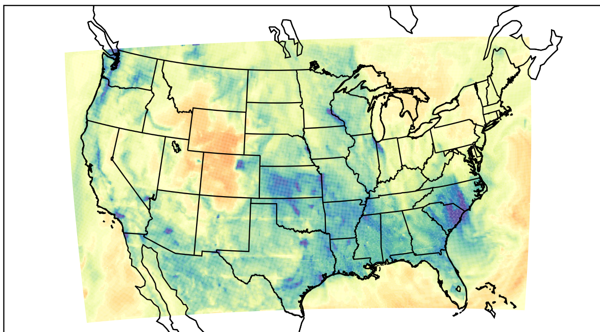
WRF (2021-02-02_04:00:00)
