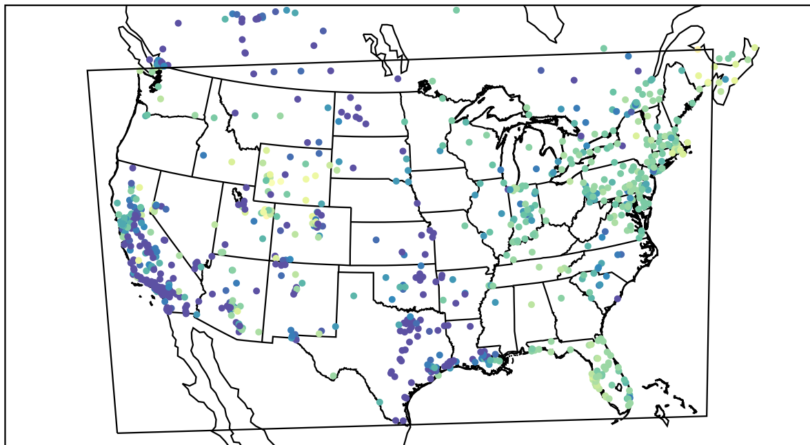
AirNOW (2021-02-02_07:00:00)
