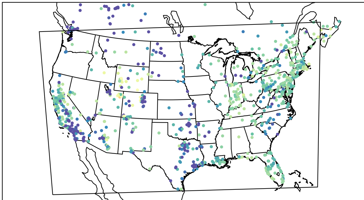
AirNOW (2021-02-02_02:00:00)
