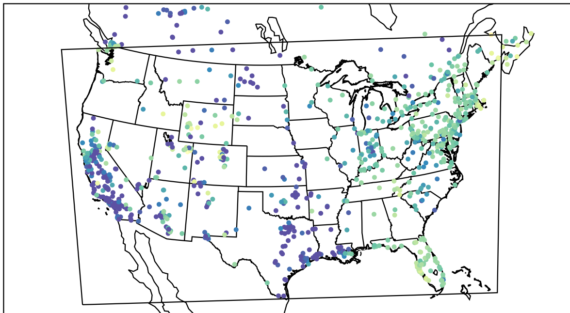
AirNOW (2021-02-02_09:00:00)
