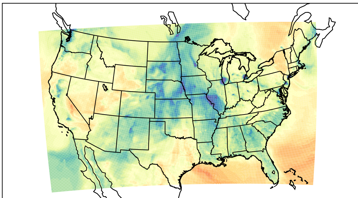
WRF (2021-02-03_23:00:00)
