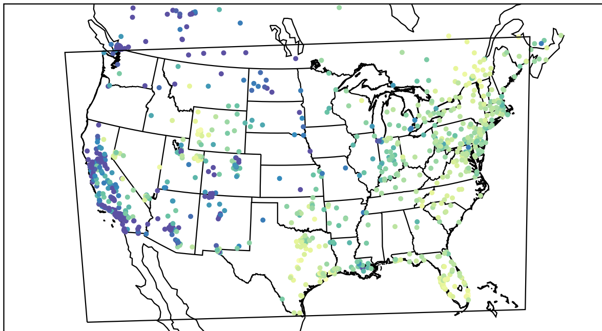
AirNOW (2021-02-03_17:00:00)
