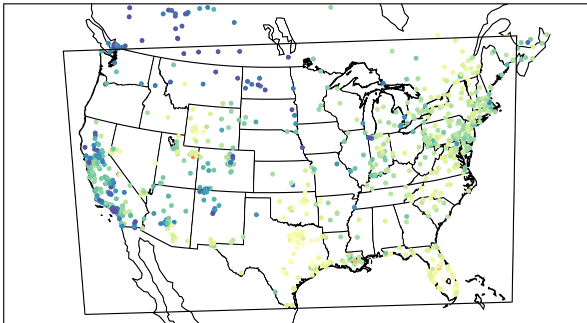
AirNOW (2021-02-03_19:00:00)
