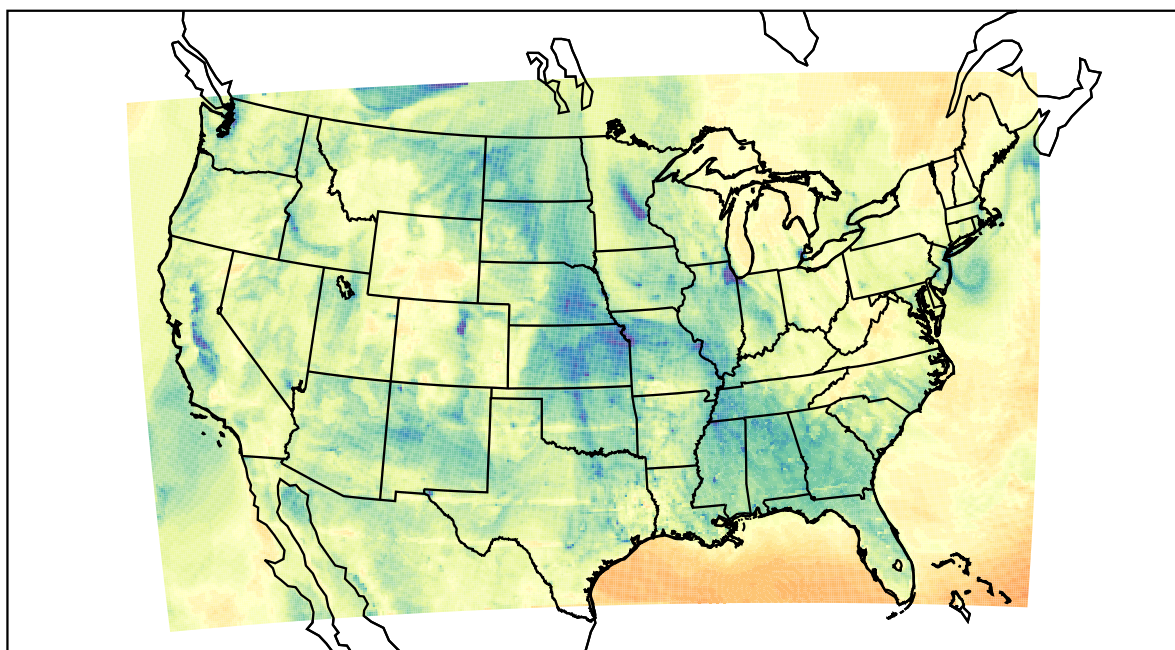
WRF (2021-02-03_00:00:00)
