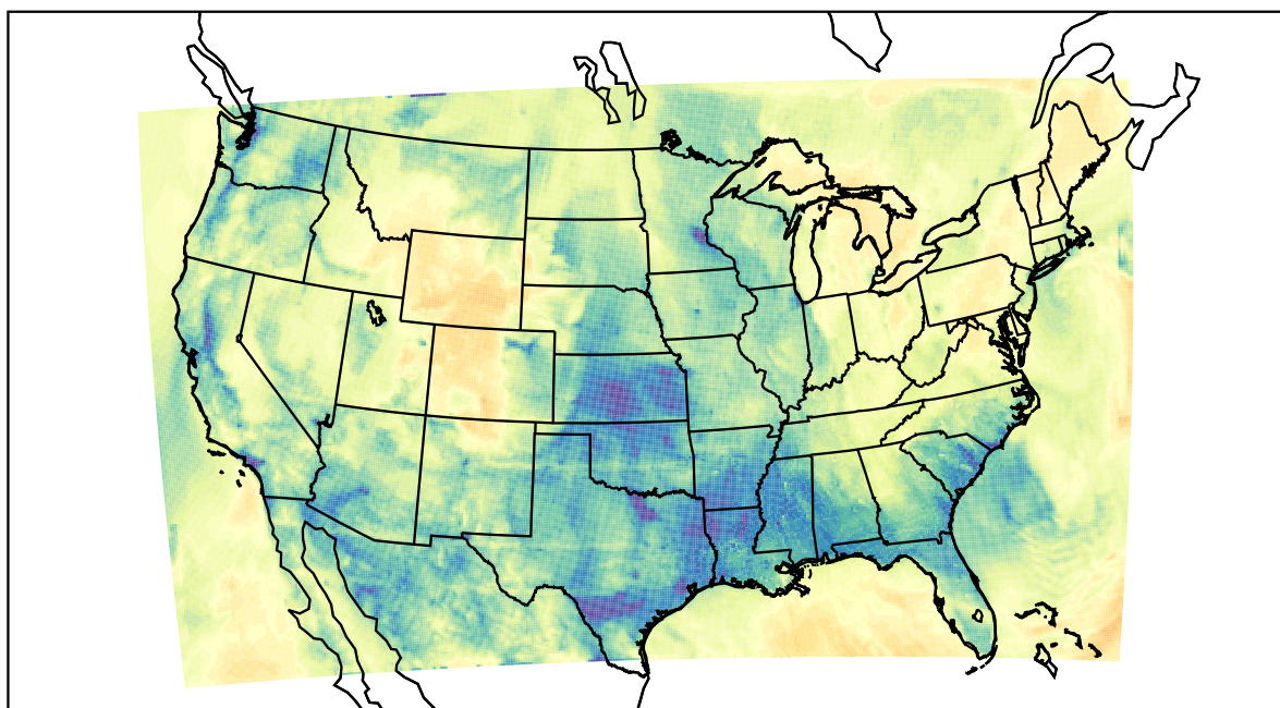
WRF (2021-02-02_12:00:00)
