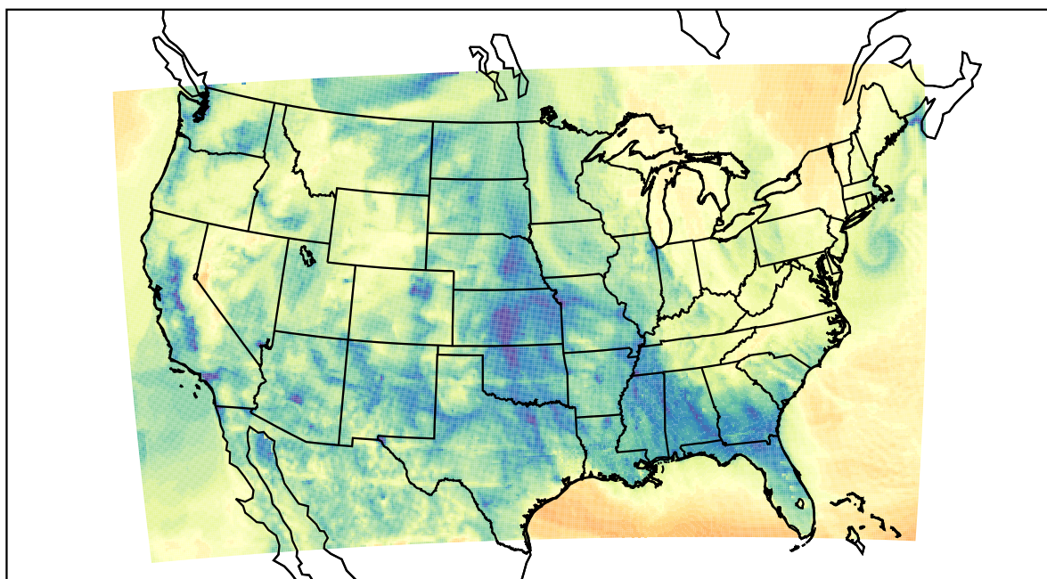
WRF (2021-02-03_06:00:00)
