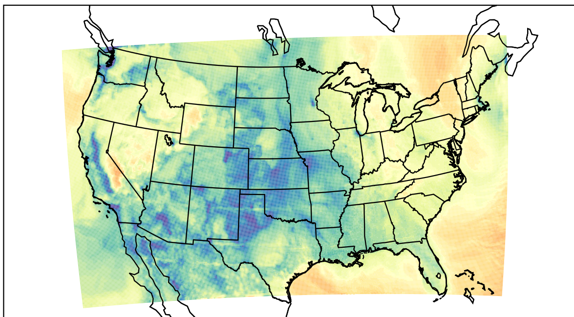
WRF (2021-02-03_16:00:00)
