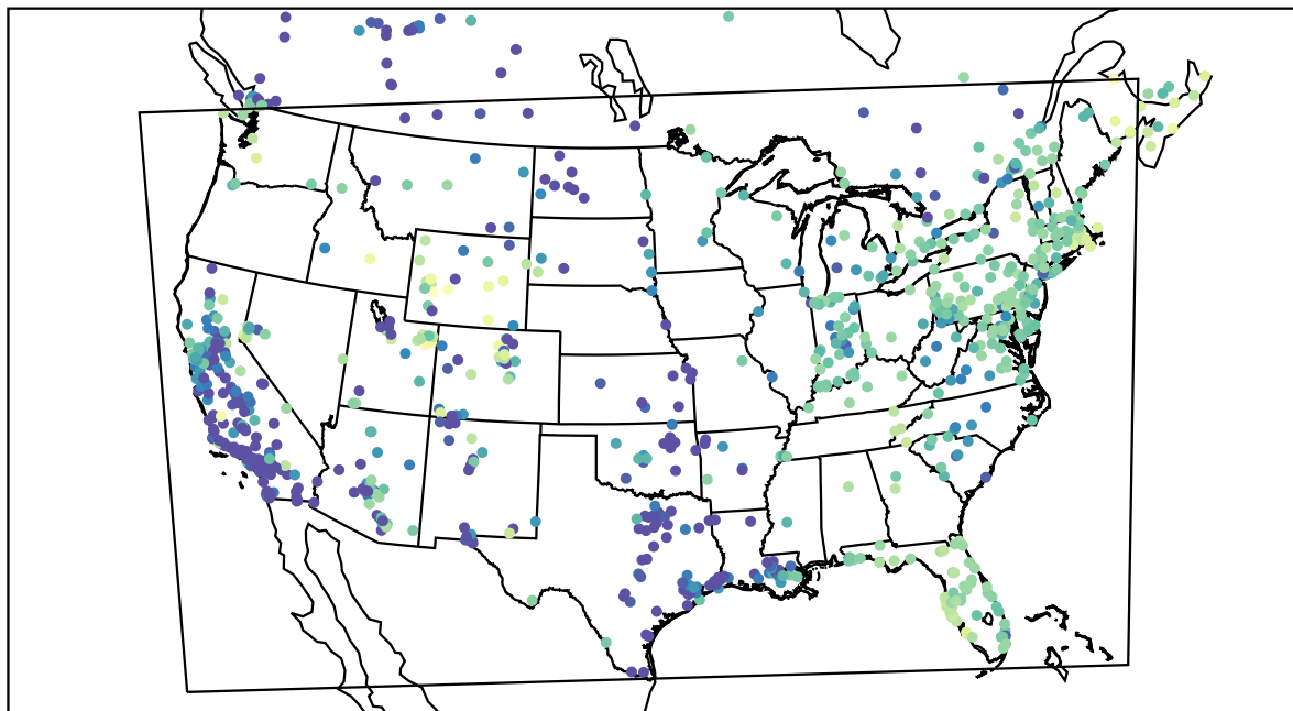
AirNOW (2021-02-02_08:00:00)
