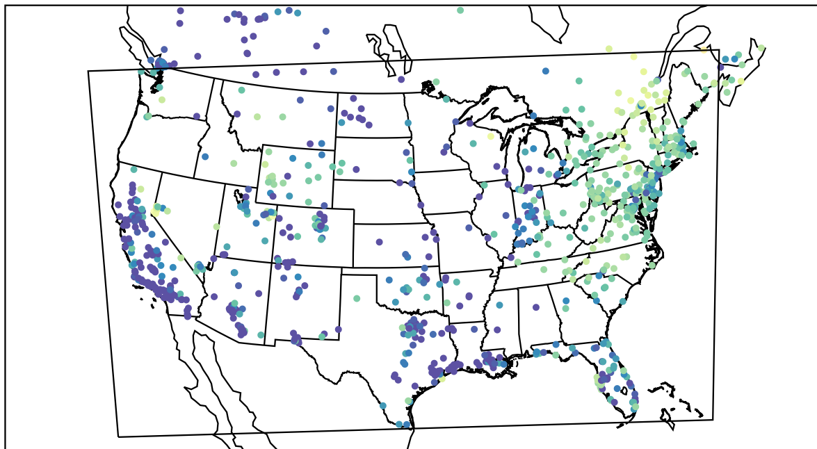
AirNOW (2021-02-03_11:00:00)
