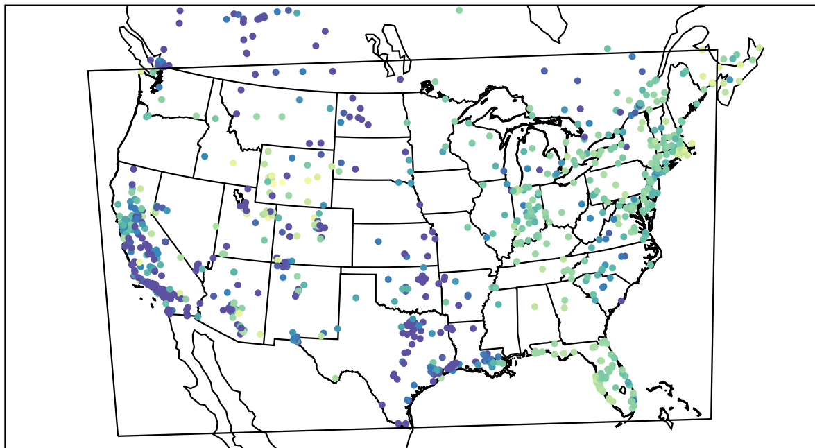
AirNOW (2021-02-02_06:00:00)
