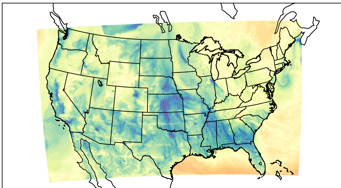
WRF (2021-02-03_04:00:00)
