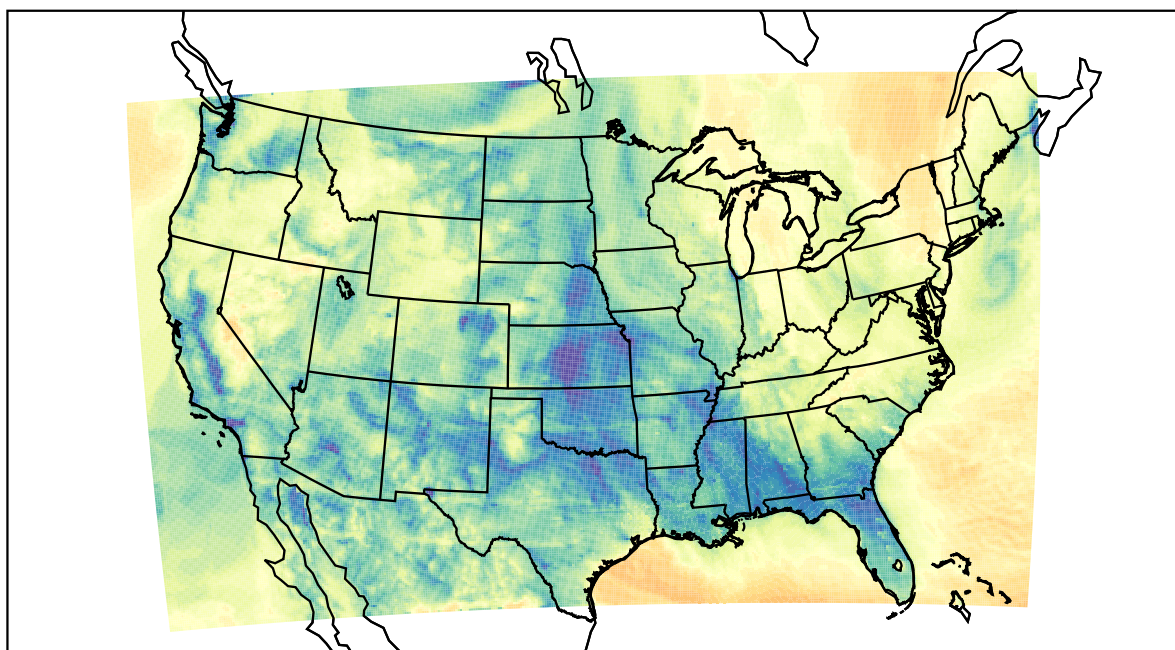
WRF (2021-02-03_09:00:00)
