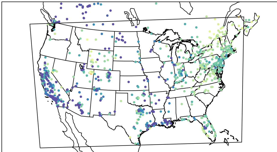
AirNOW (2021-02-03_04:00:00)
