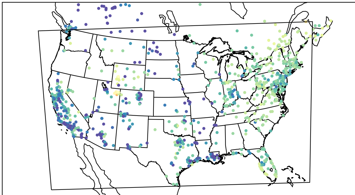
AirNOW (2021-02-03_02:00:00)
