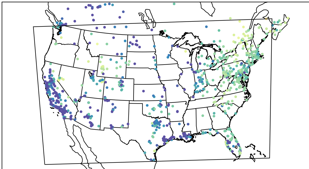
AirNOW (2021-02-03_08:00:00)
