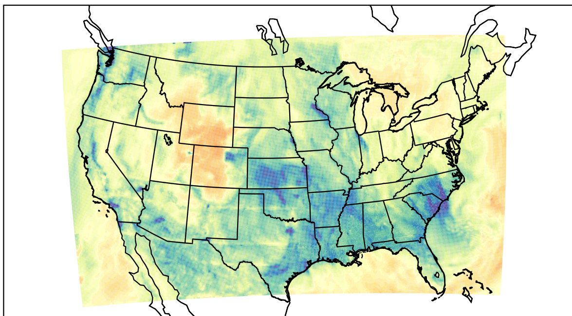
WRF (2021-02-02_05:00:00)
