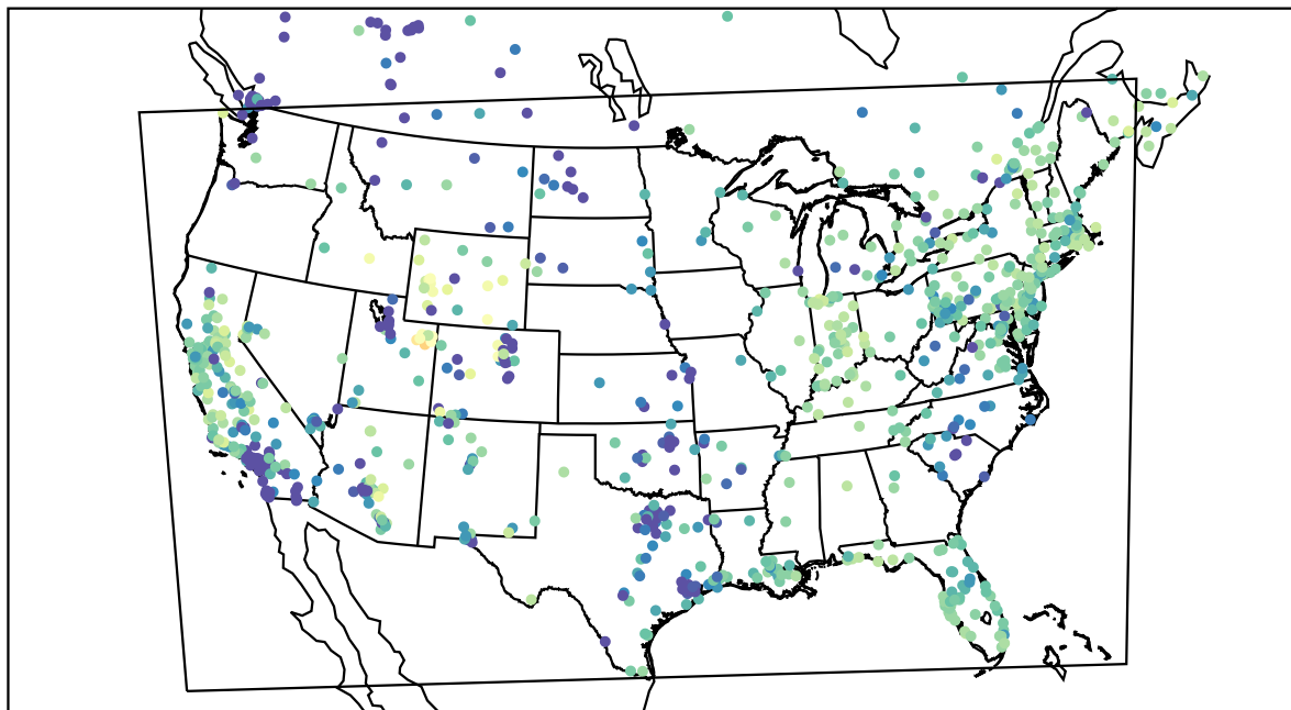
AirNOW (2021-02-02_01:00:00)
