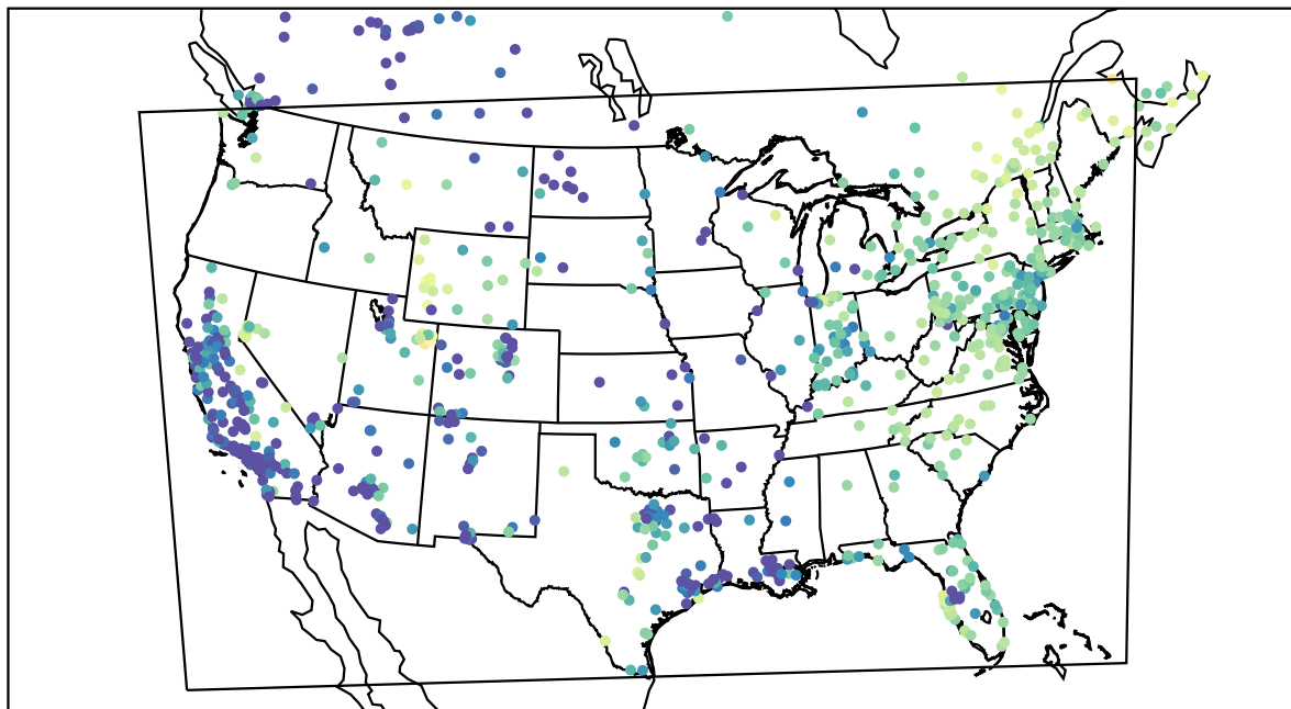
AirNOW (2021-02-03_05:00:00)
