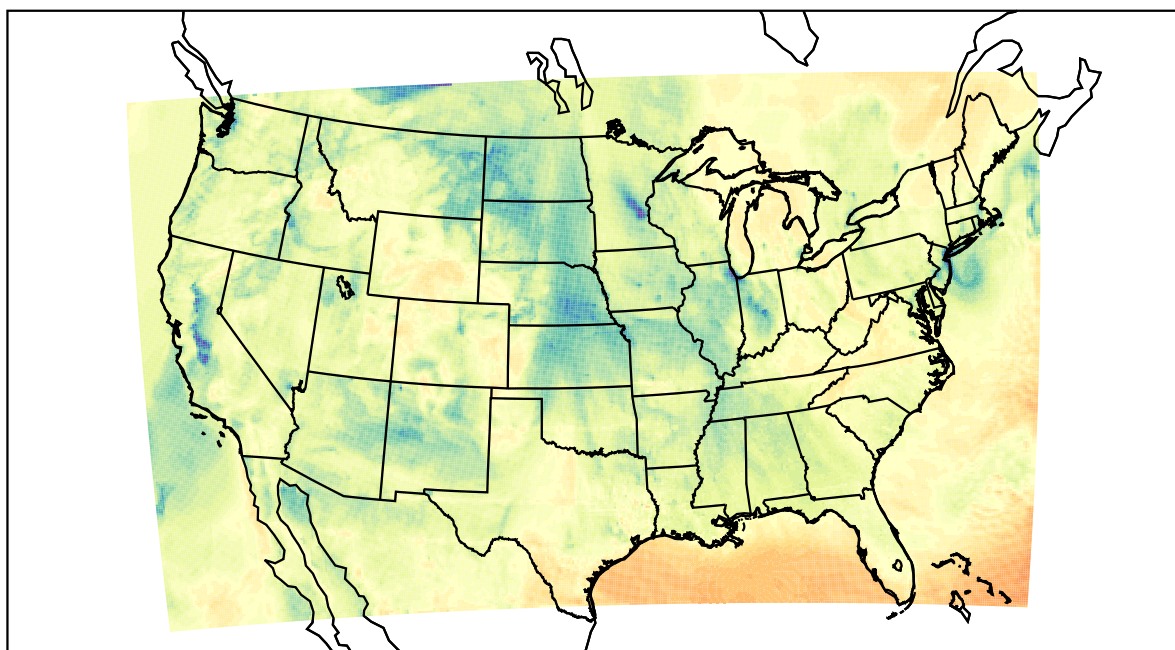
WRF (2021-02-02_22:00:00)
