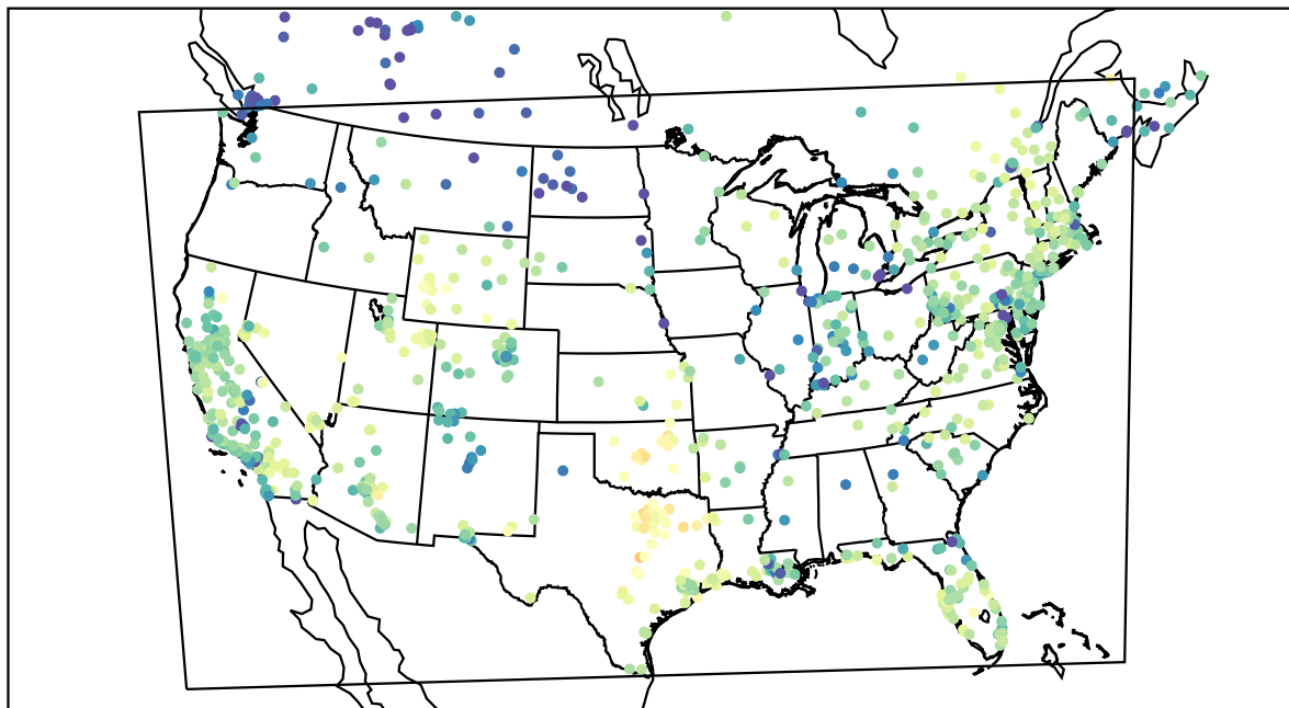
AirNOW (2021-02-03_23:00:00)
