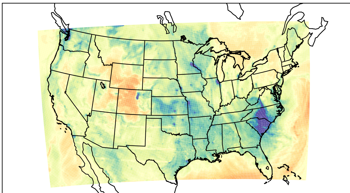
WRF (2021-02-02_00:00:00)
