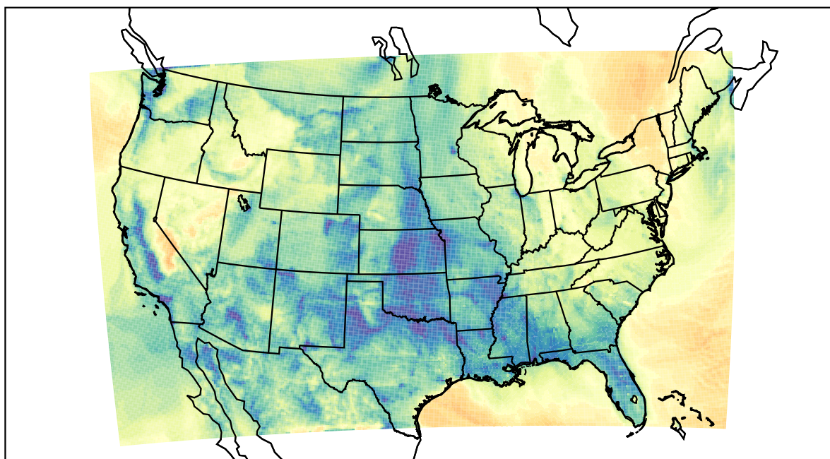
WRF (2021-02-03_13:00:00)
