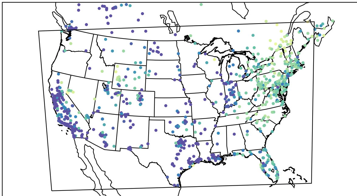
AirNOW (2021-02-03_13:00:00)
