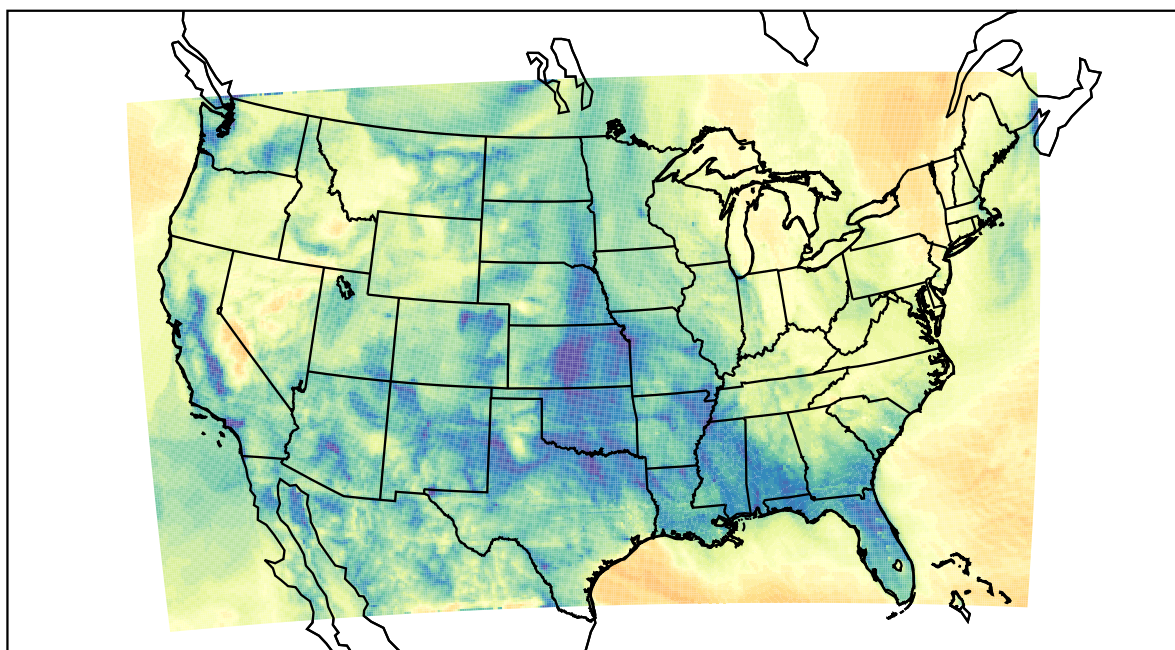
WRF (2021-02-03_11:00:00)
