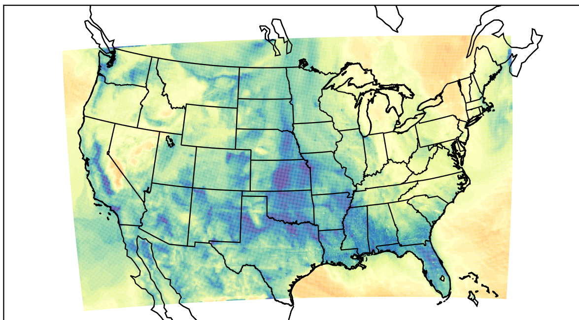
WRF (2021-02-03_12:00:00)
