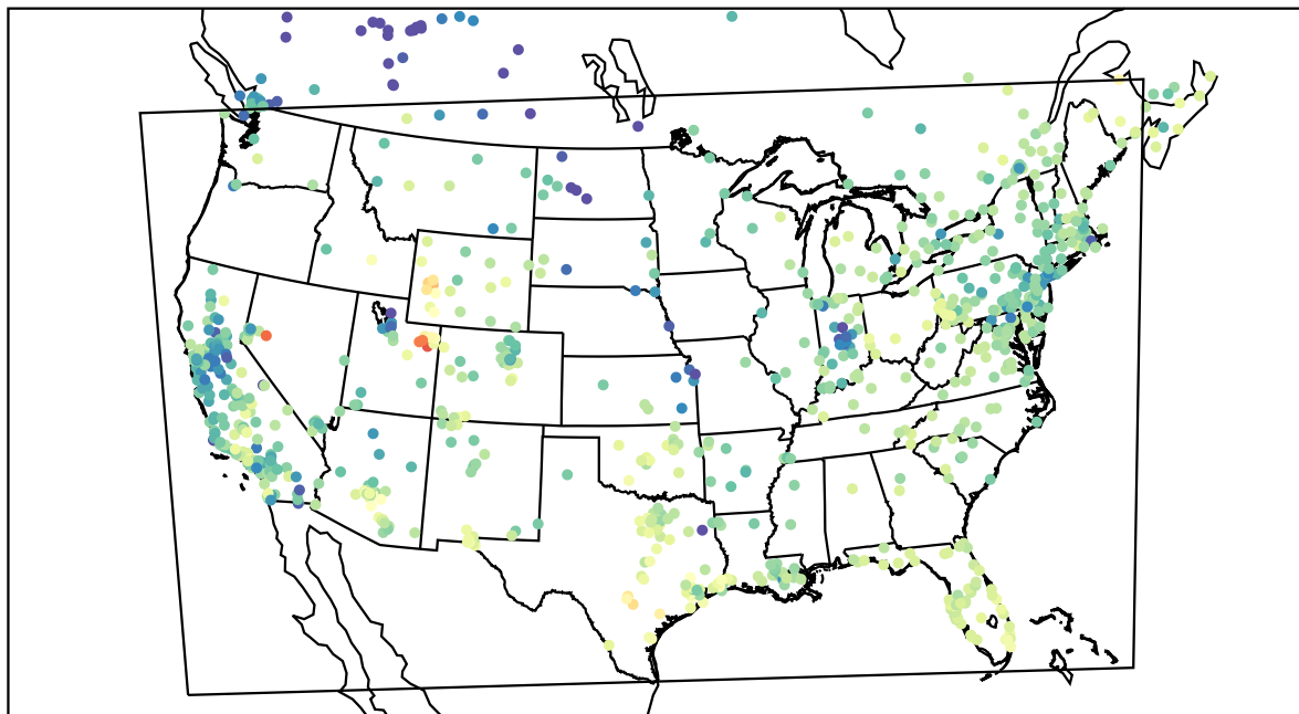
AirNOW (2021-02-02_21:00:00)
