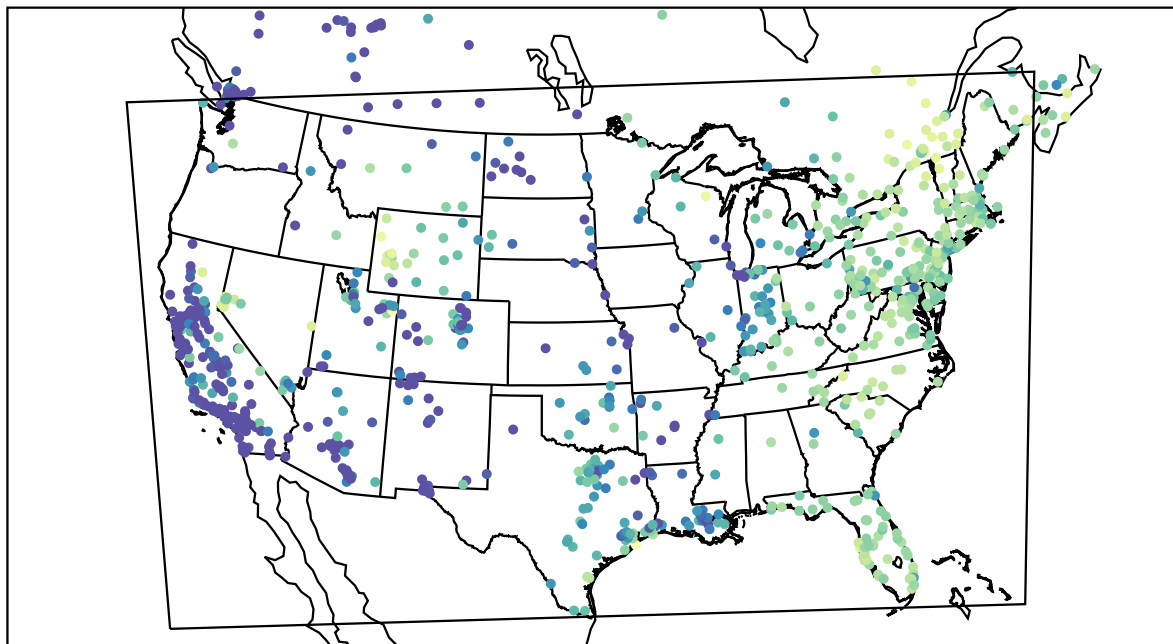
AirNOW (2021-02-03_15:00:00)
