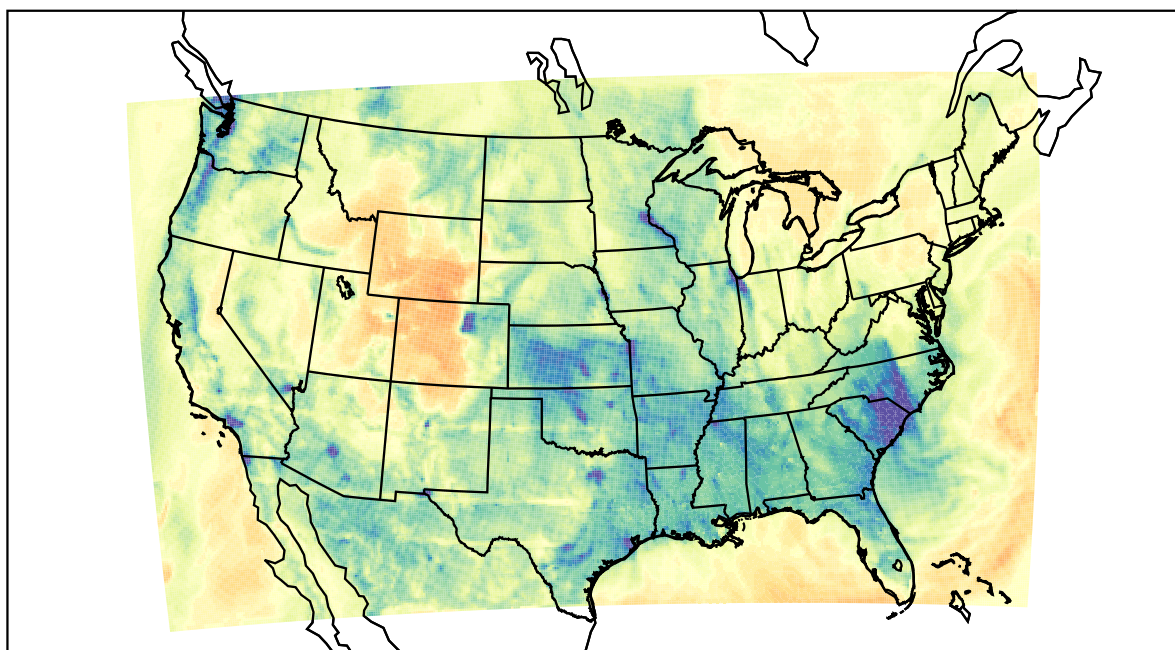
WRF (2021-02-02_03:00:00)
