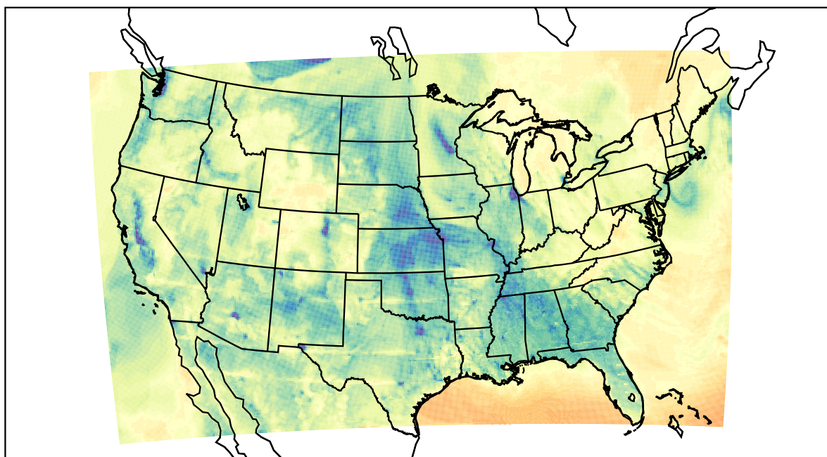
WRF (2021-02-03_01:00:00)
