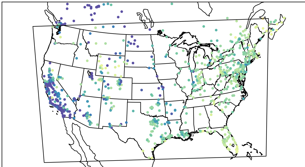
AirNOW (2021-02-02_17:00:00)
