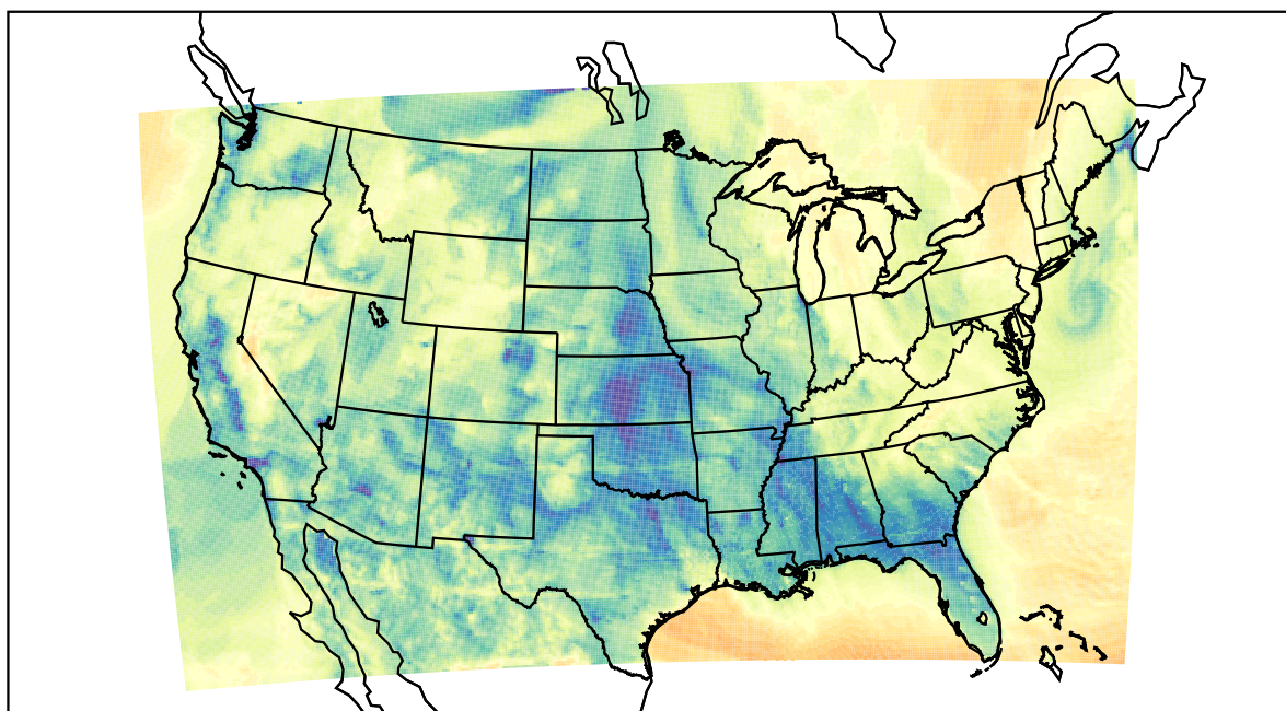
WRF (2021-02-03_07:00:00)
