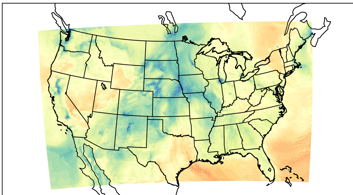
WRF (2021-02-03_21:00:00)
