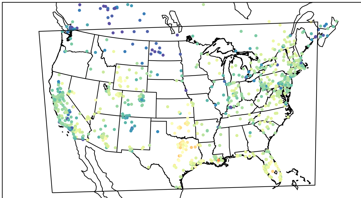
AirNOW (2021-02-03_22:00:00)
