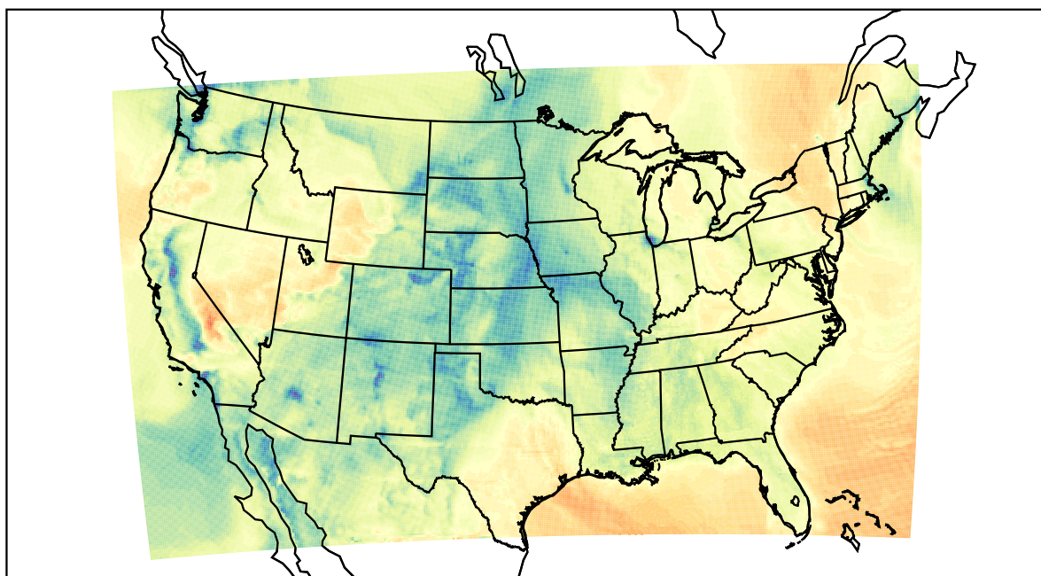
WRF (2021-02-03_19:00:00)
