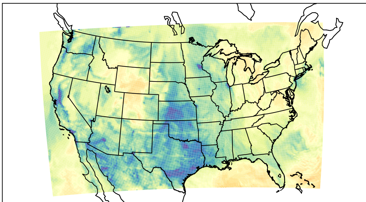
WRF (2021-02-02_15:00:00)
