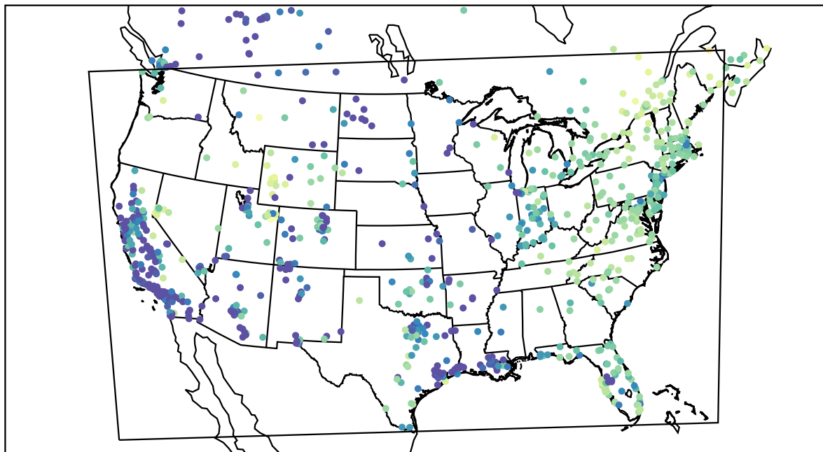
AirNOW (2021-02-03_06:00:00)
