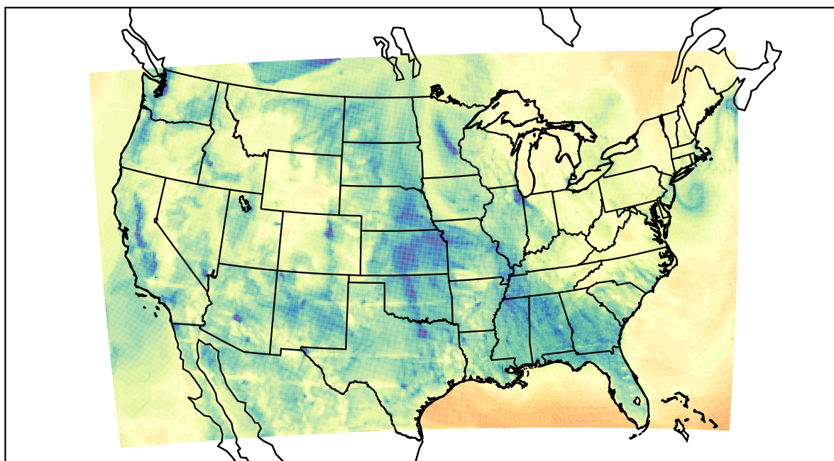
WRF (2021-02-03_02:00:00)
