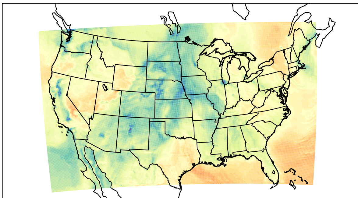
WRF (2021-02-03_20:00:00)
