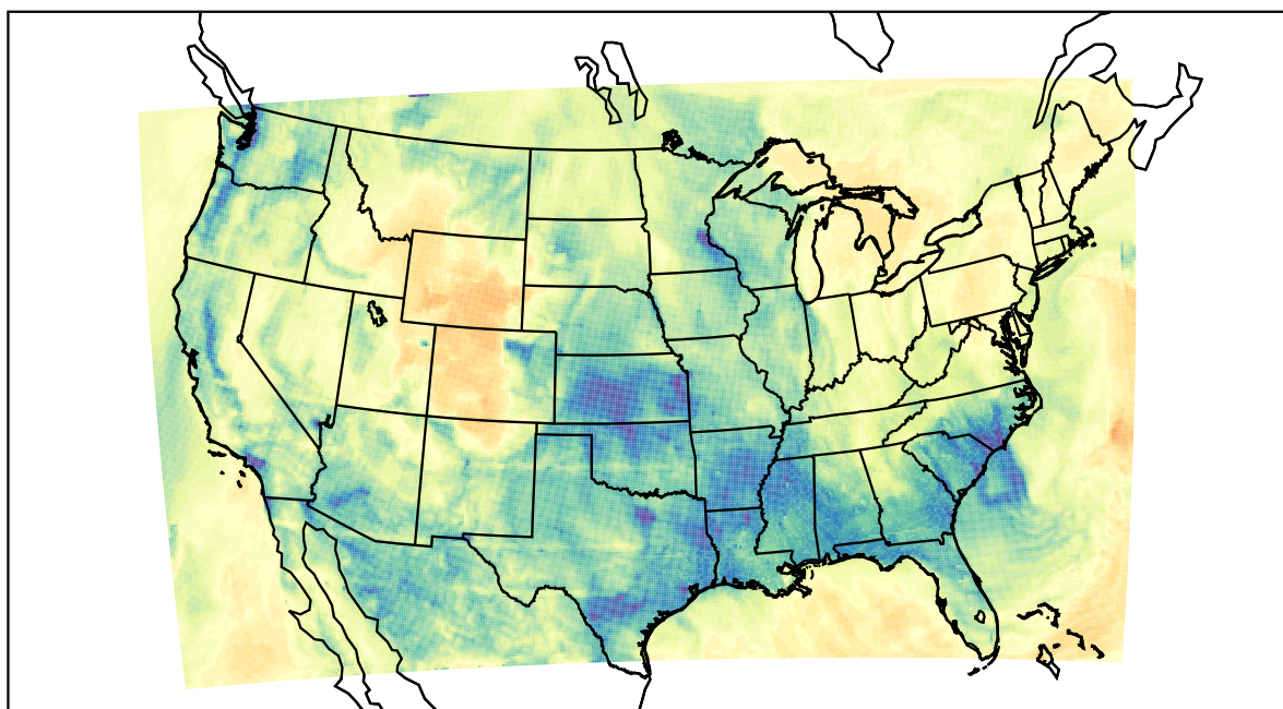
WRF (2021-02-02_08:00:00)
