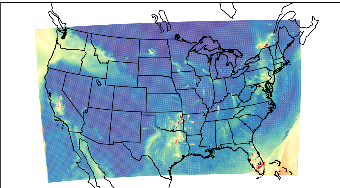
WRF 2021-02-07_22:00:00
