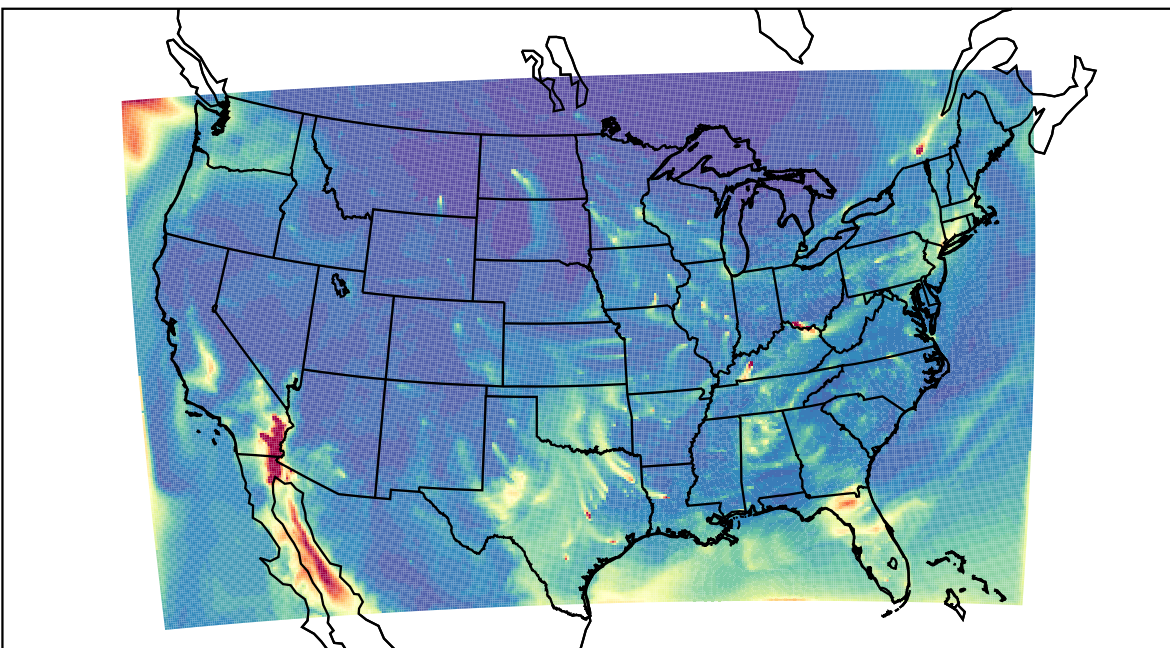
WRF 2021-02-06_14:00:00
