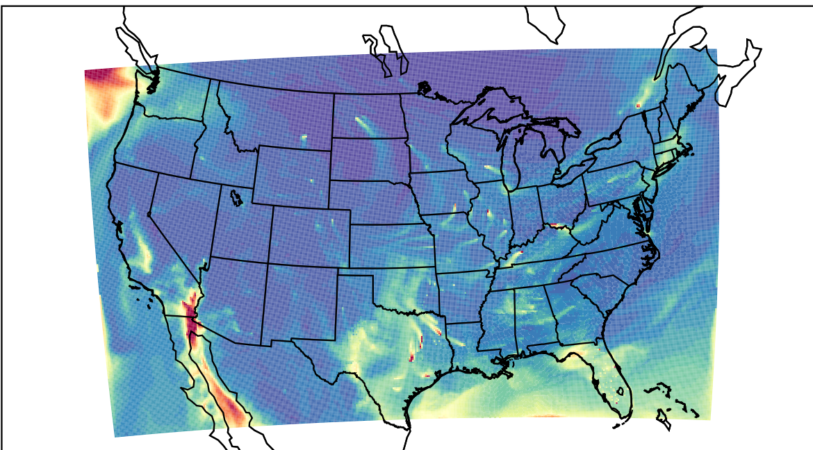
WRF 2021-02-06_17:00:00
