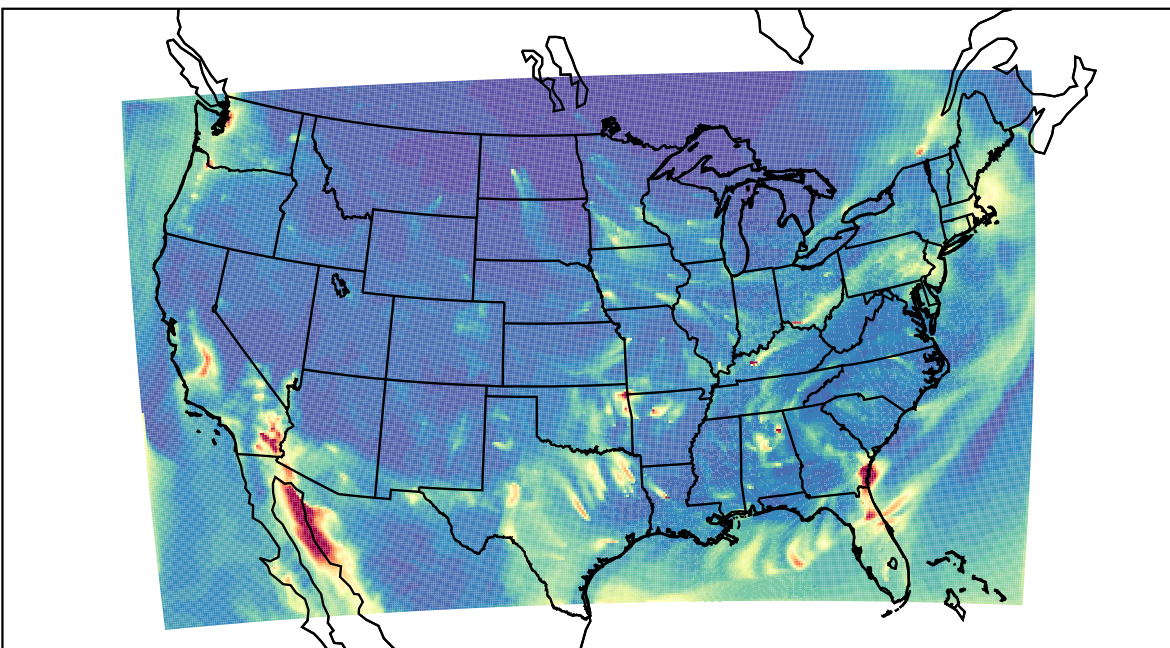
WRF 2021-02-06_07:00:00
