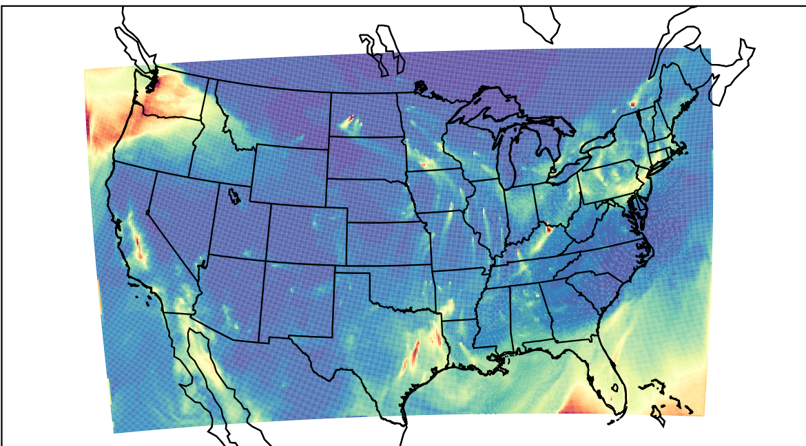
WRF 2021-02-07_09:00:00
