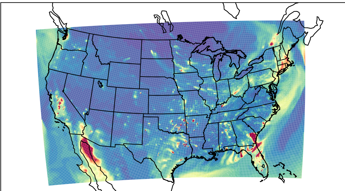
WRF 2021-02-06_02:00:00
