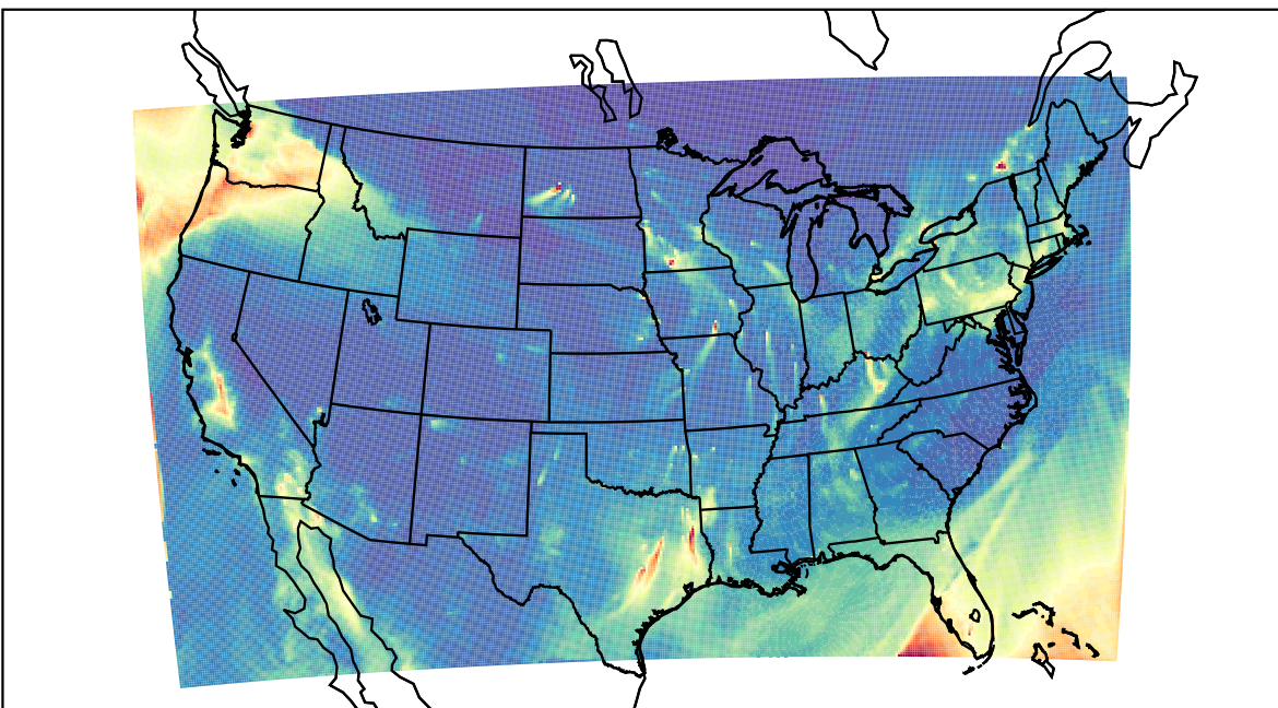
WRF 2021-02-07_12:00:00
