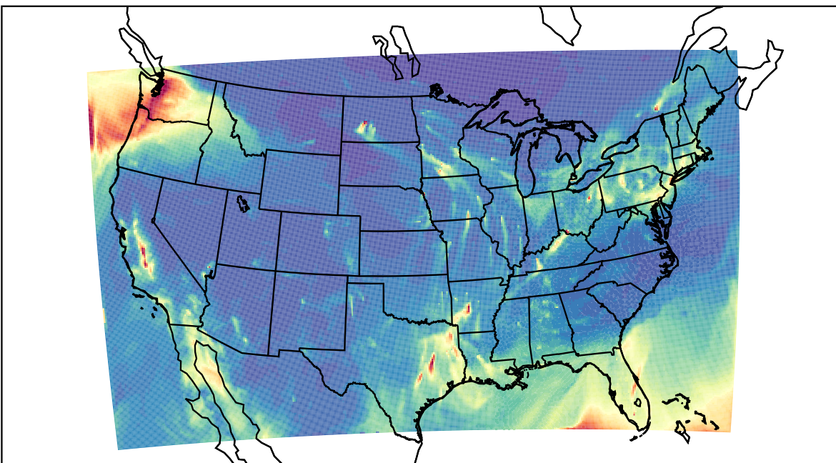
WRF 2021-02-07_07:00:00
