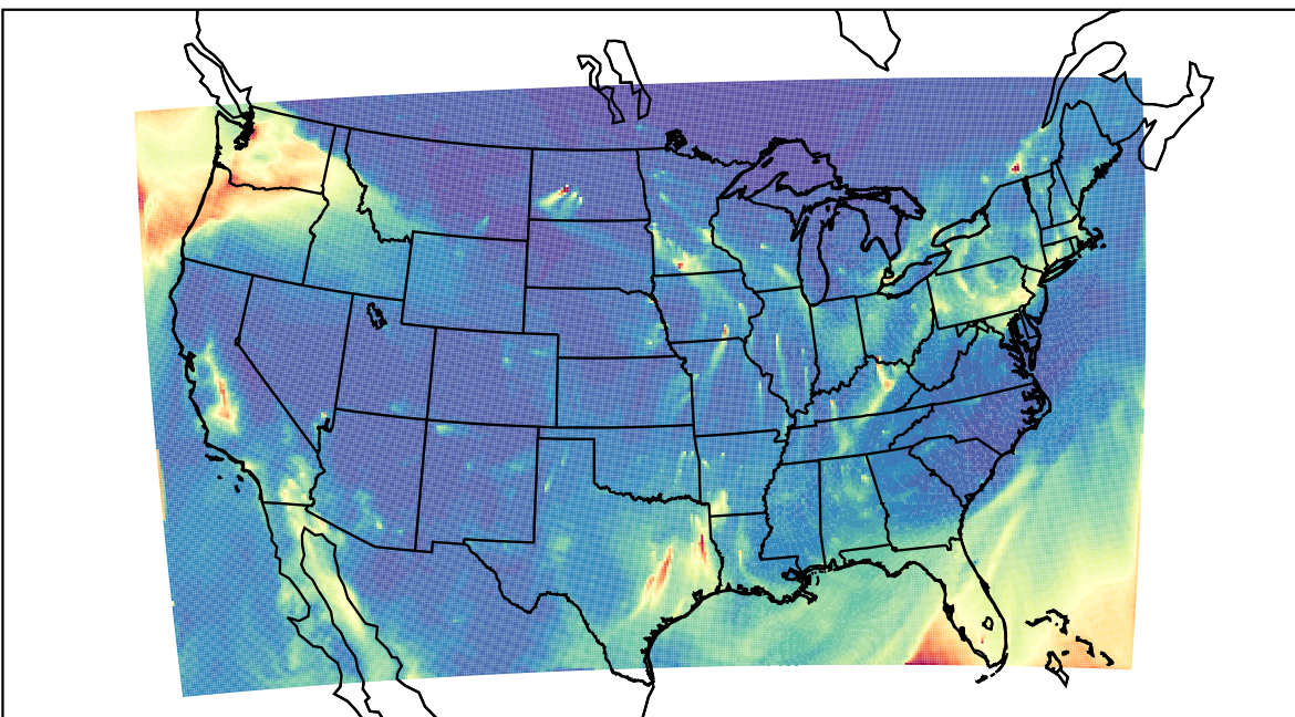
WRF 2021-02-07_11:00:00
