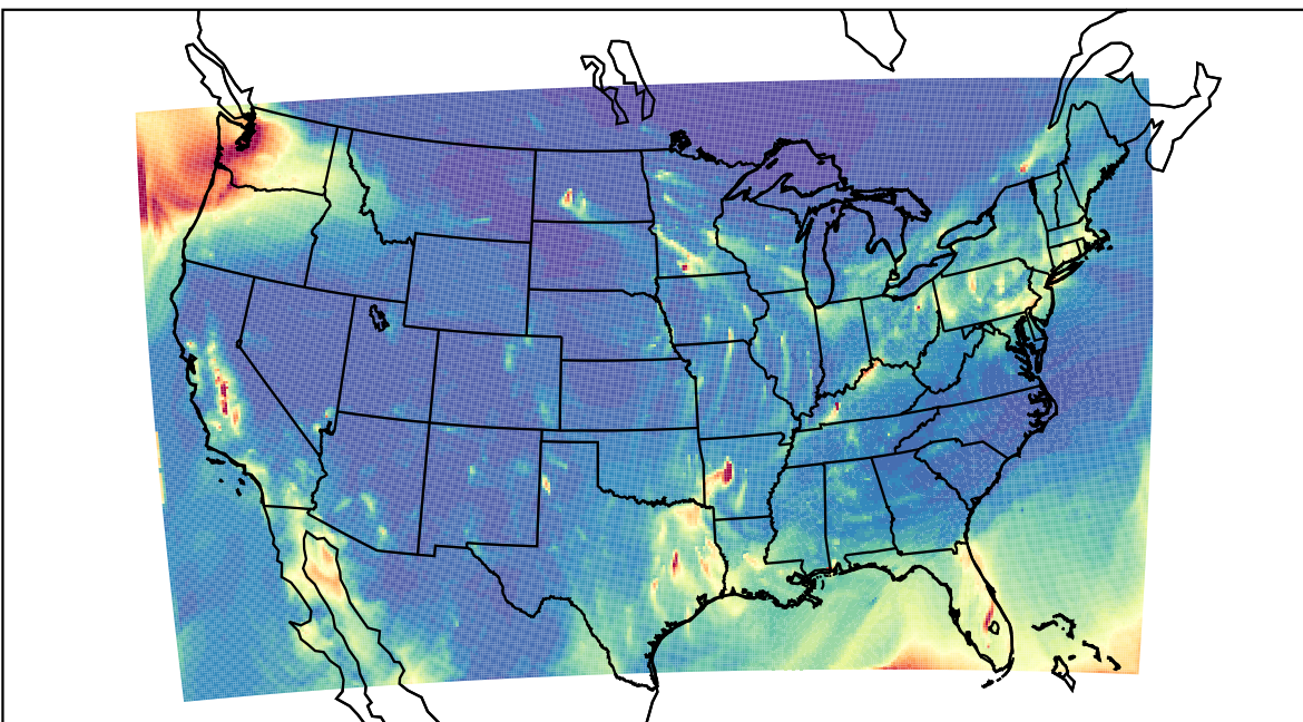
WRF 2021-02-07_05:00:00
