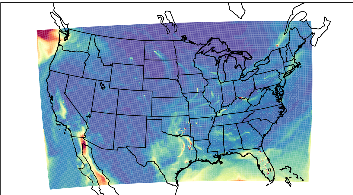
WRF 2021-02-06_19:00:00
