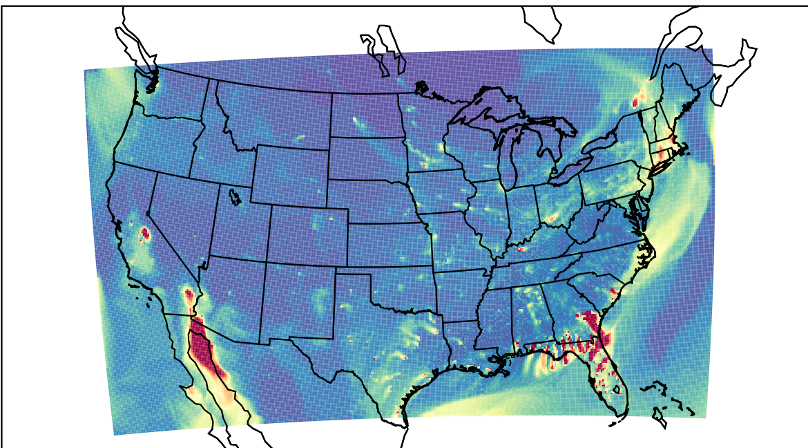
WRF 2021-02-06_00:00:00
