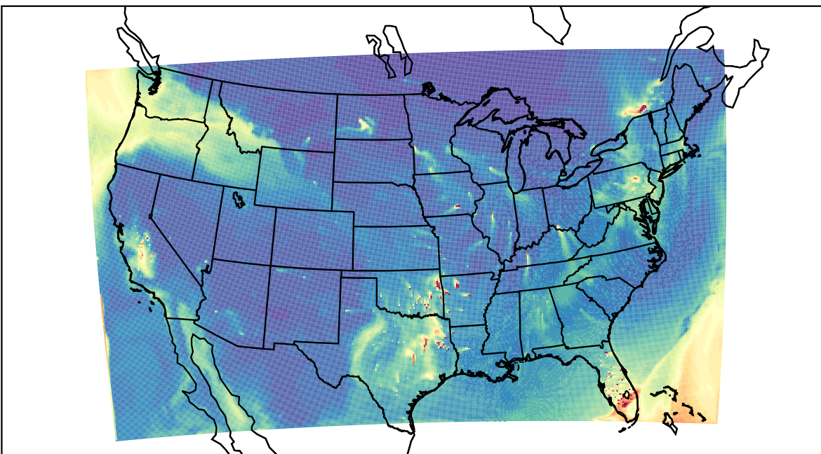
WRF 2021-02-07_21:00:00
