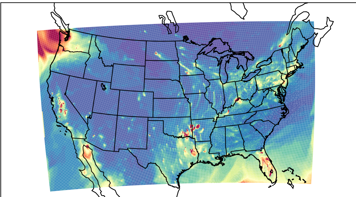
WRF 2021-02-07_02:00:00
