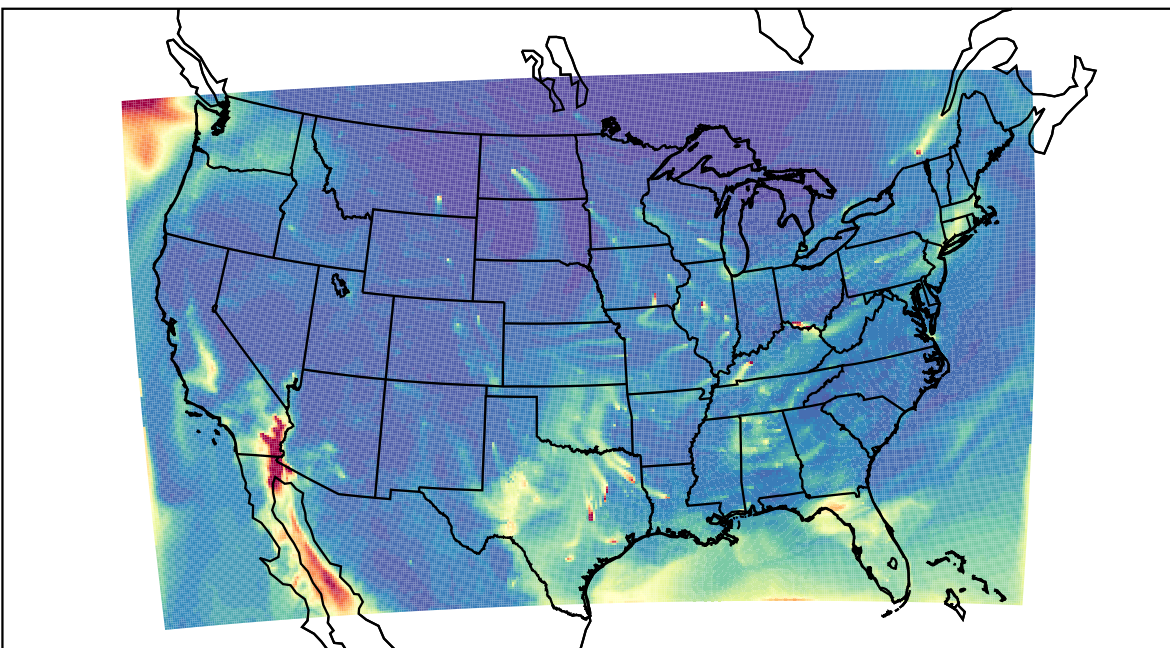
WRF 2021-02-06_16:00:00
