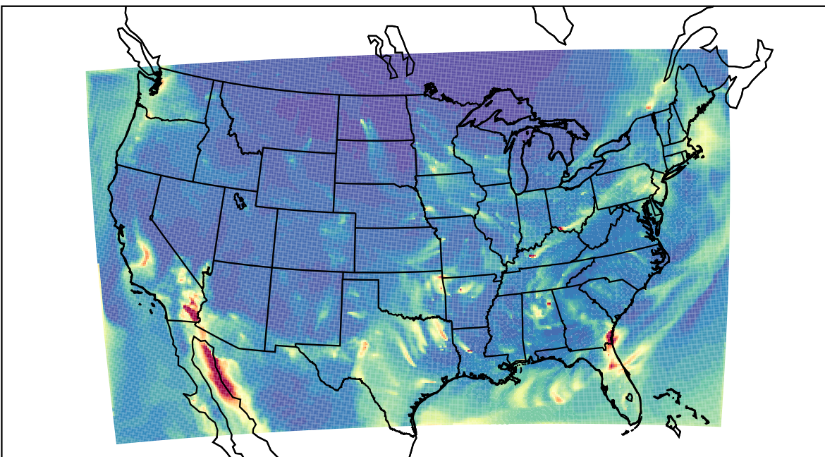
WRF 2021-02-06_08:00:00
