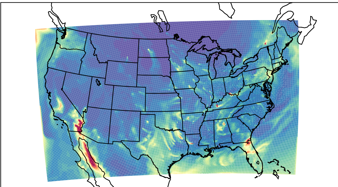
WRF 2021-02-06_11:00:00
