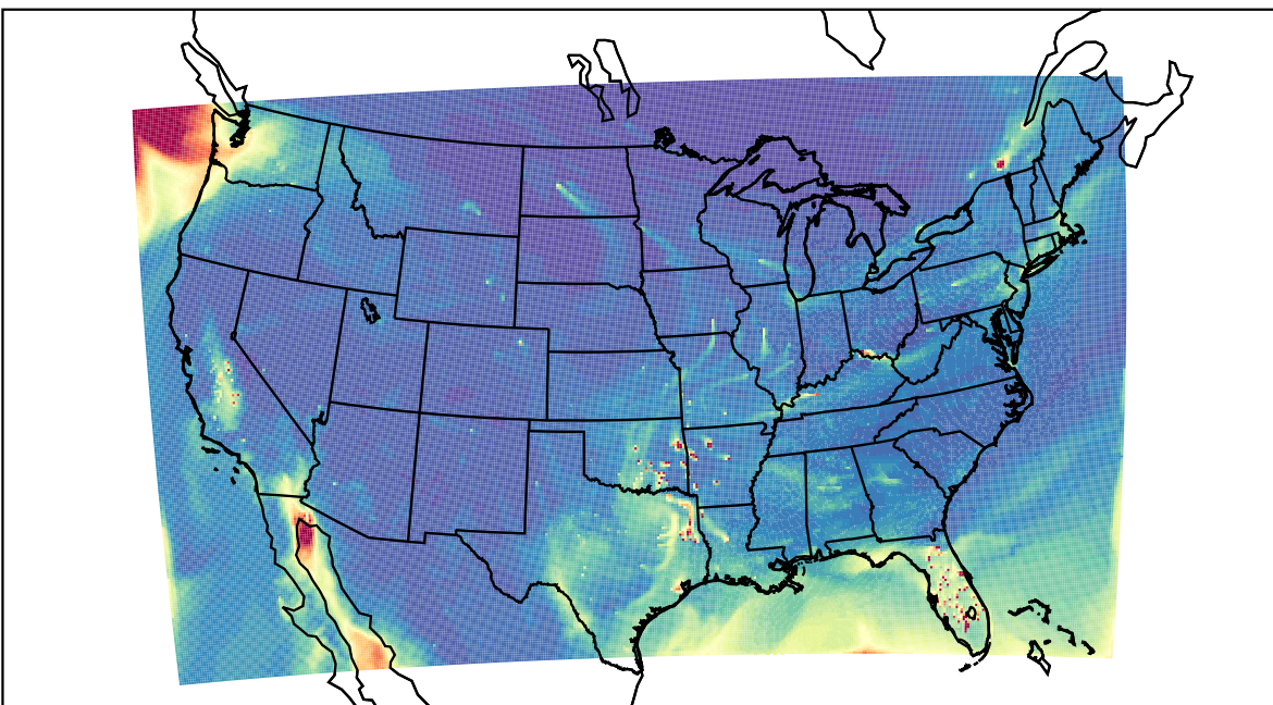
WRF 2021-02-06_21:00:00
