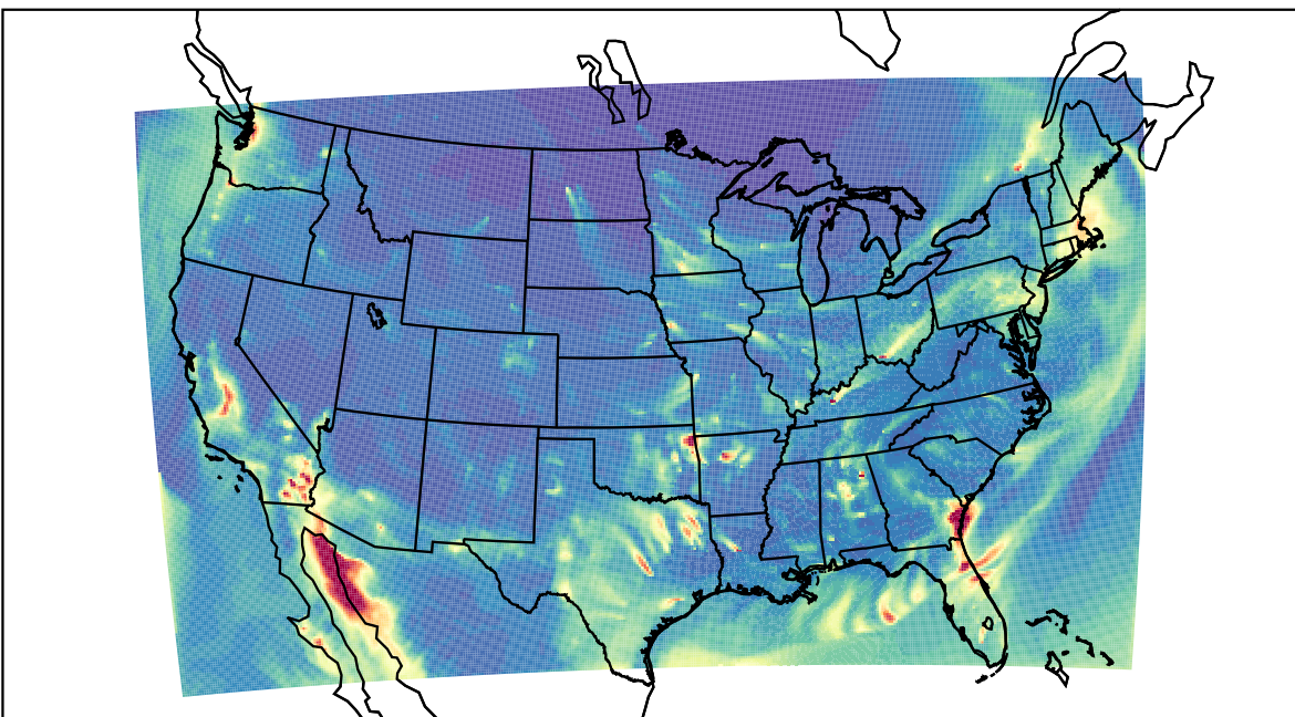
WRF 2021-02-06_06:00:00
