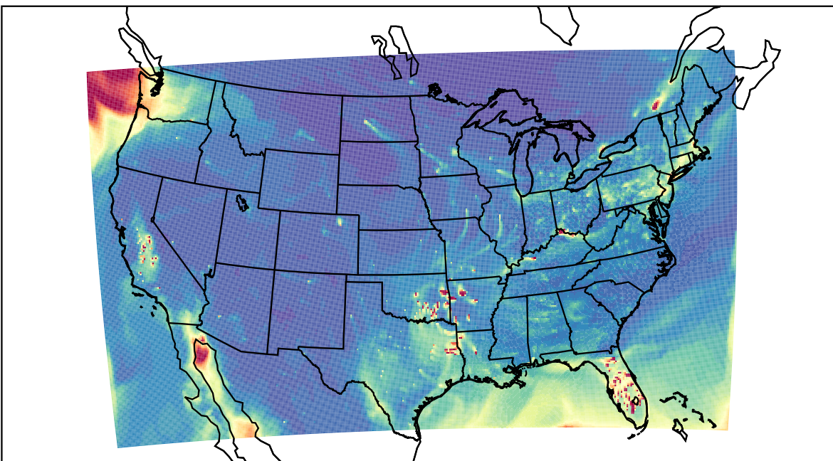
WRF 2021-02-06_23:00:00
