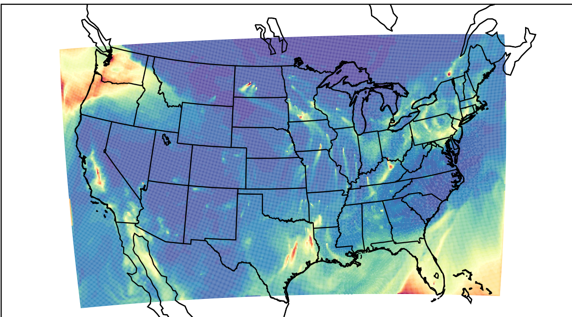
WRF 2021-02-07_10:00:00
