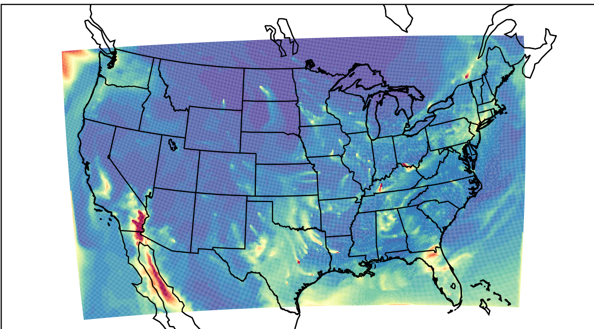
WRF 2021-02-06_13:00:00
