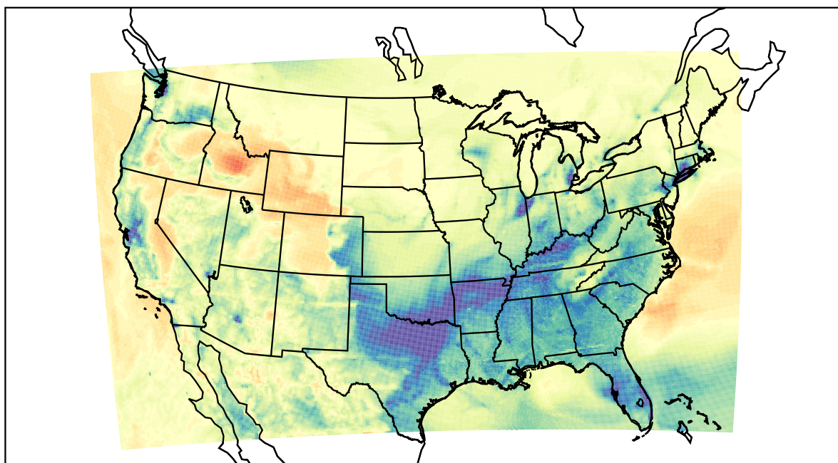
WRF (2021-02-09_06:00:00)
