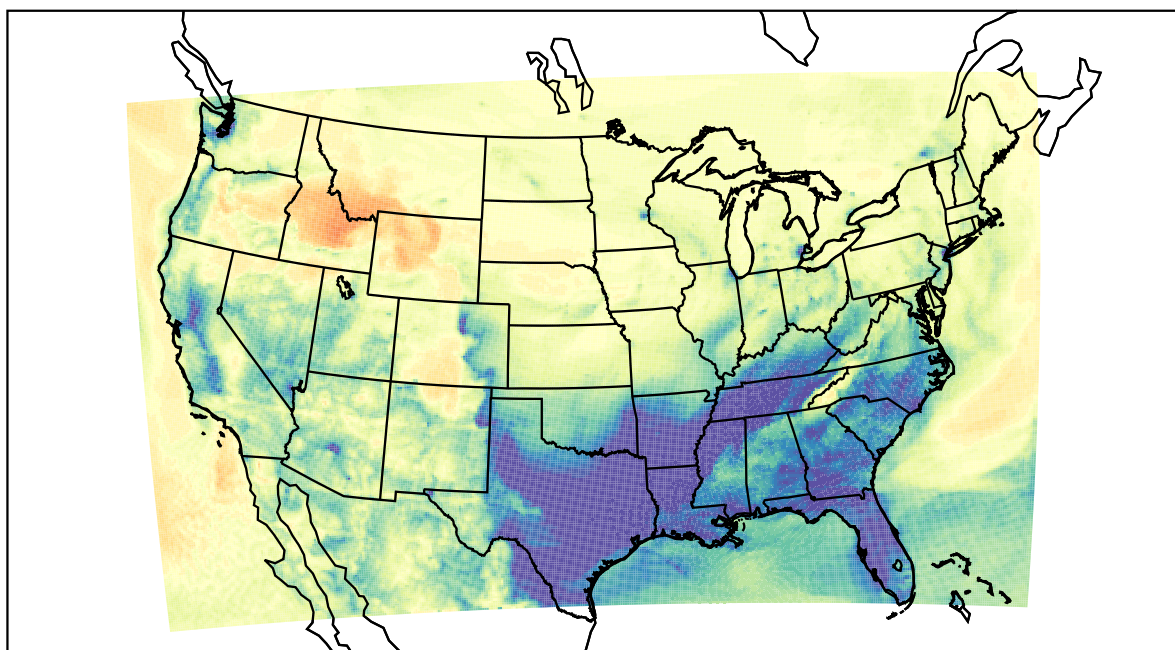
WRF (2021-02-10_13:00:00)
