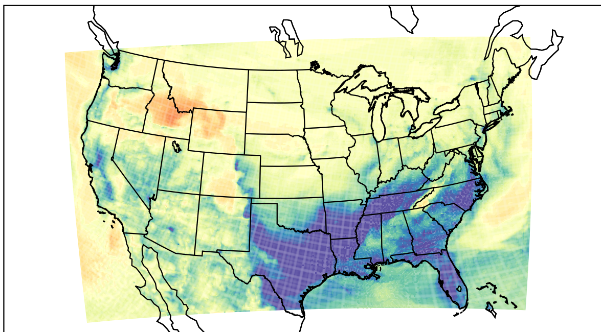
WRF (2021-02-10_12:00:00)
