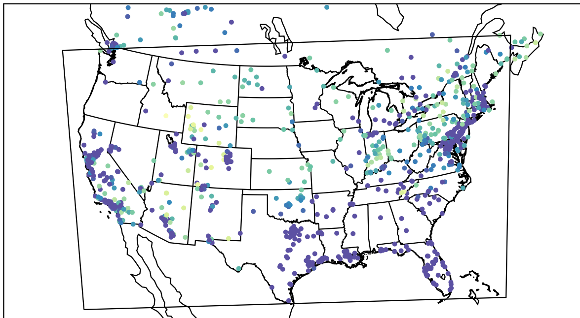
AirNOW (2021-02-10_12:00:00)
