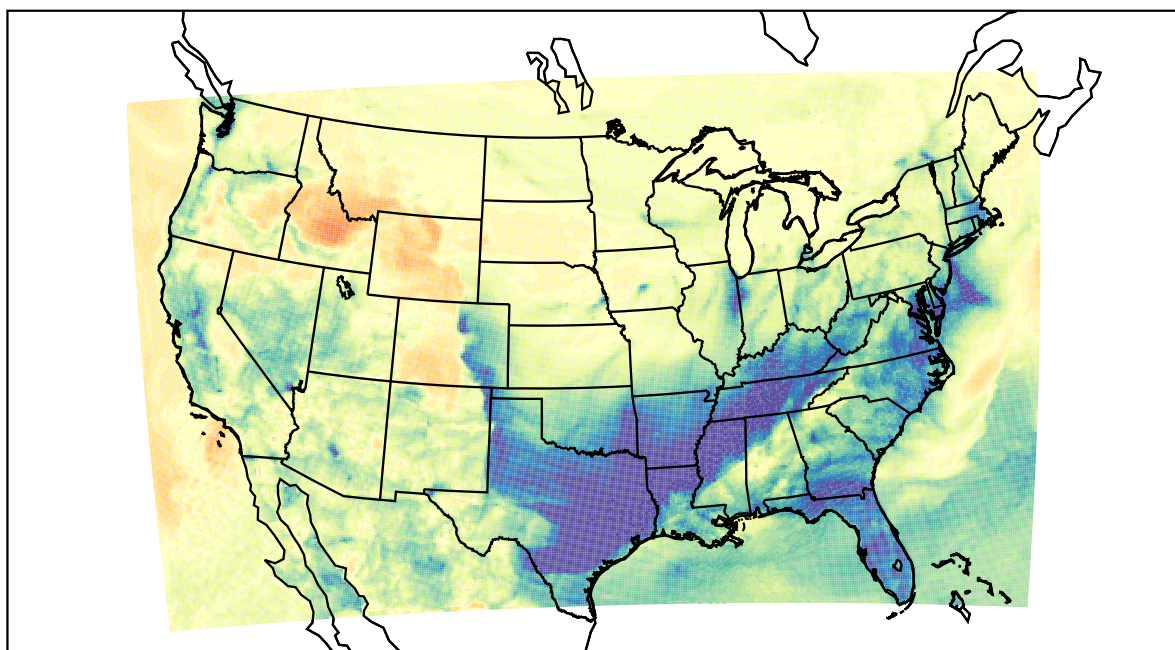
WRF (2021-02-10_05:00:00)
