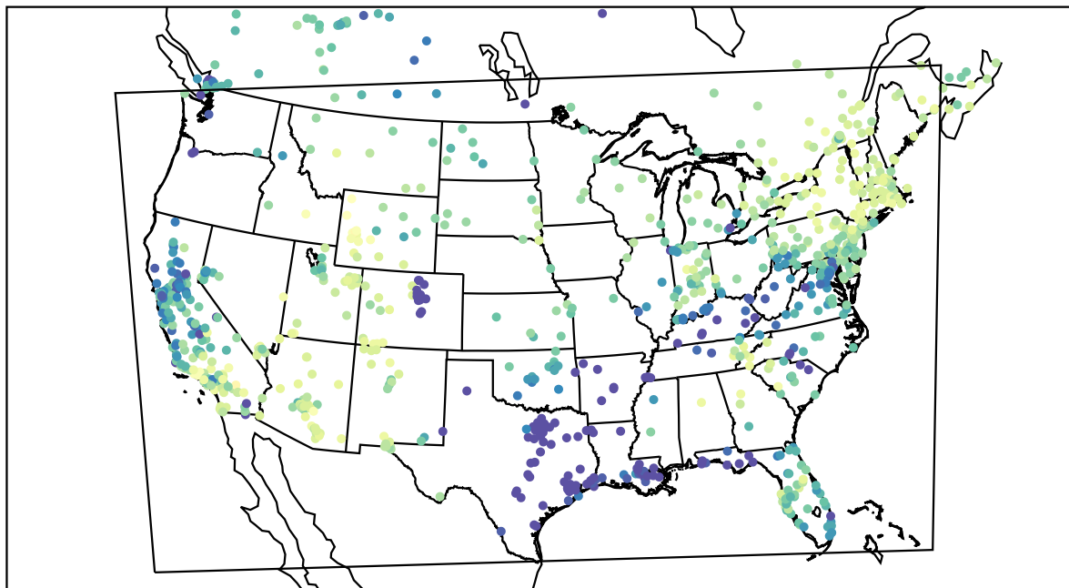
AirNOW (2021-02-10_19:00:00)
