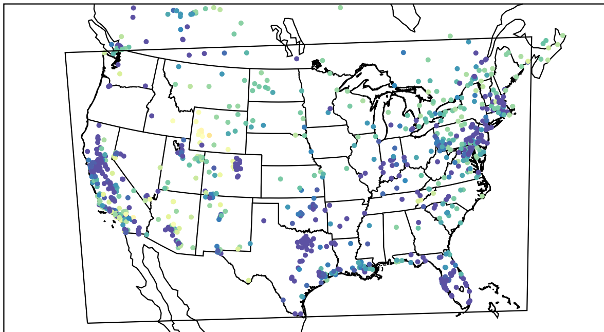
AirNOW (2021-02-09_05:00:00)
