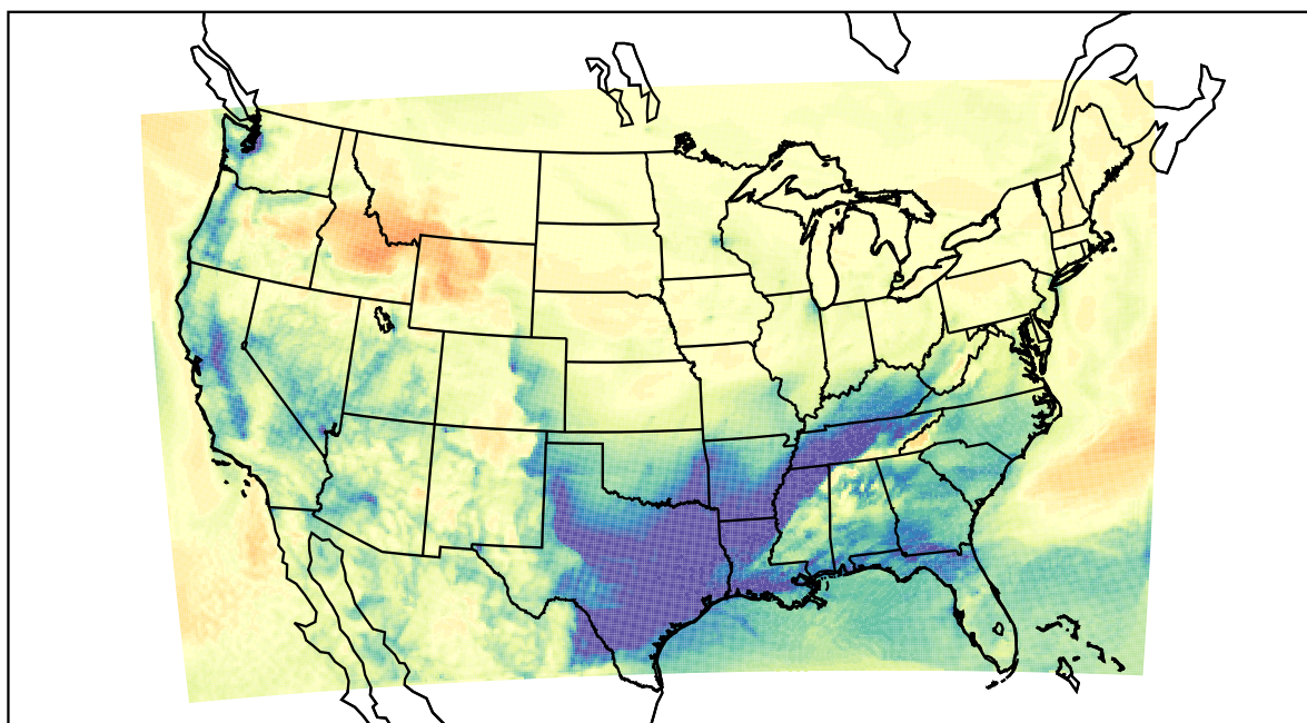
WRF (2021-02-10_17:00:00)
