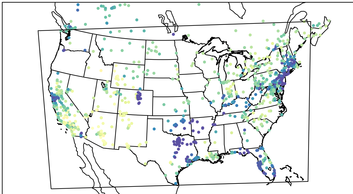
AirNOW (2021-02-09_21:00:00)
