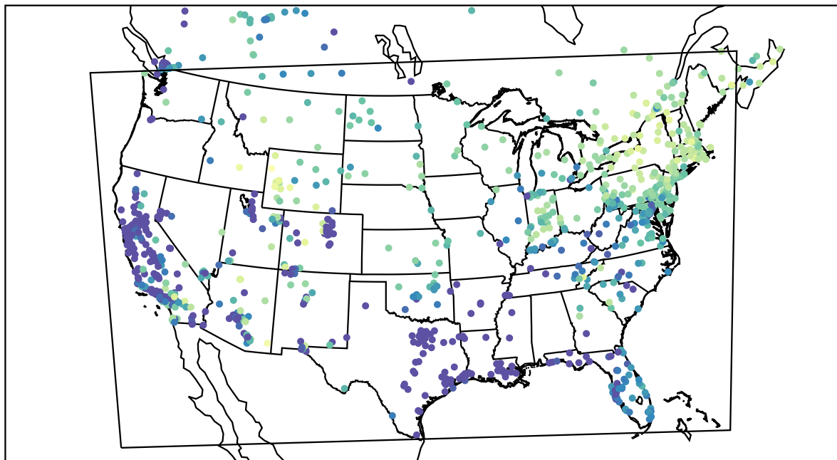
AirNOW (2021-02-10_16:00:00)
