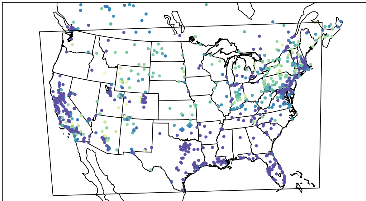
AirNOW (2021-02-10_09:00:00)
