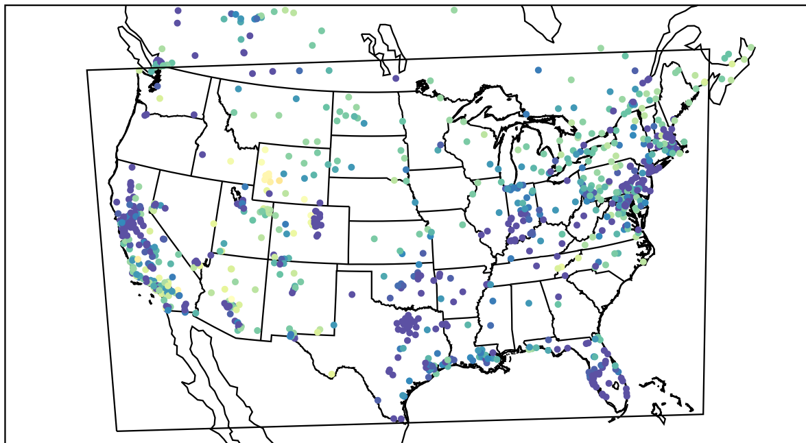
AirNOW (2021-02-09_04:00:00)
