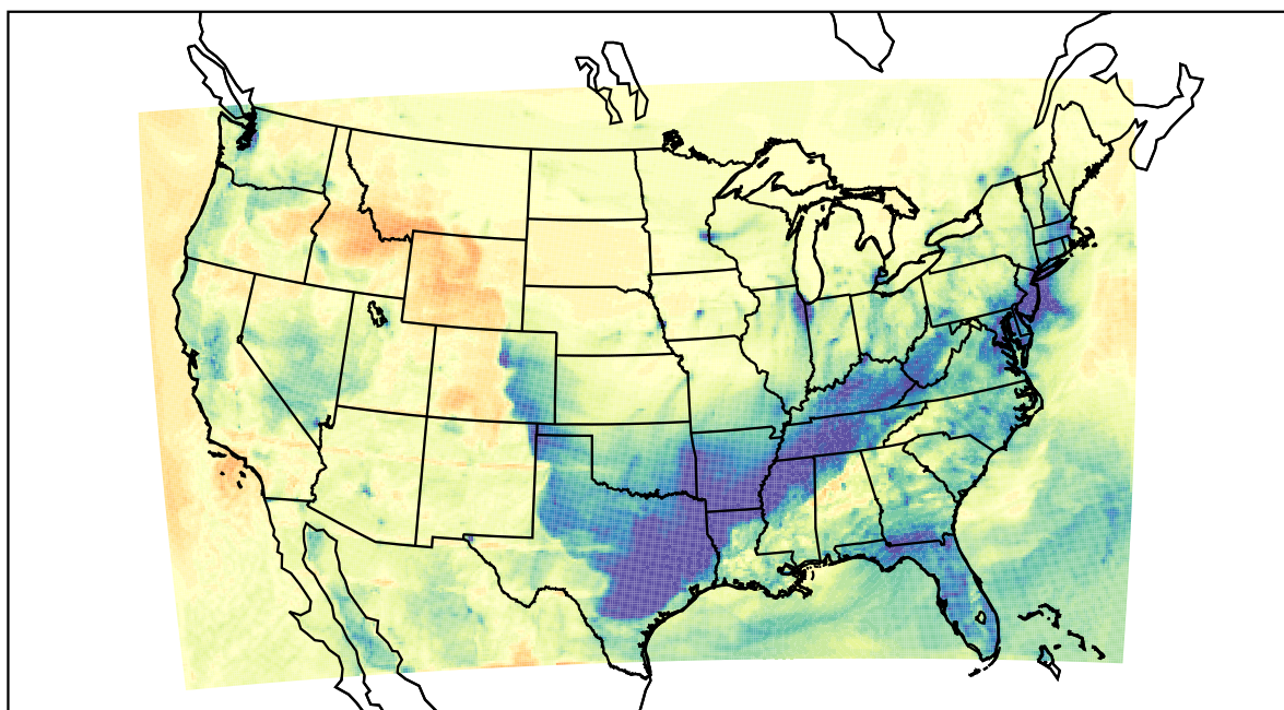
WRF (2021-02-10_01:00:00)
