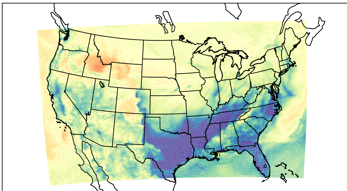
WRF (2021-02-10_09:00:00)
