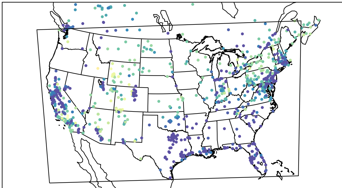
AirNOW (2021-02-10_05:00:00)
