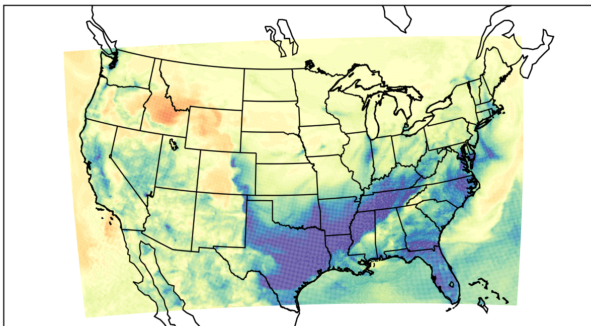
WRF (2021-02-10_07:00:00)
