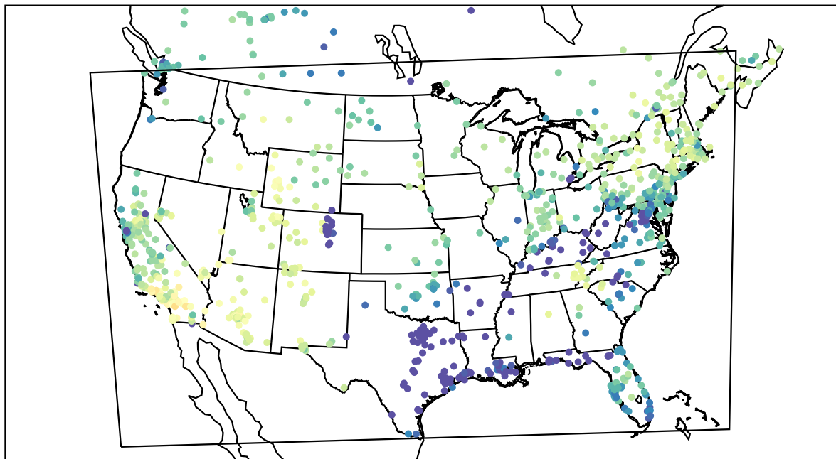
AirNOW (2021-02-10_22:00:00)
