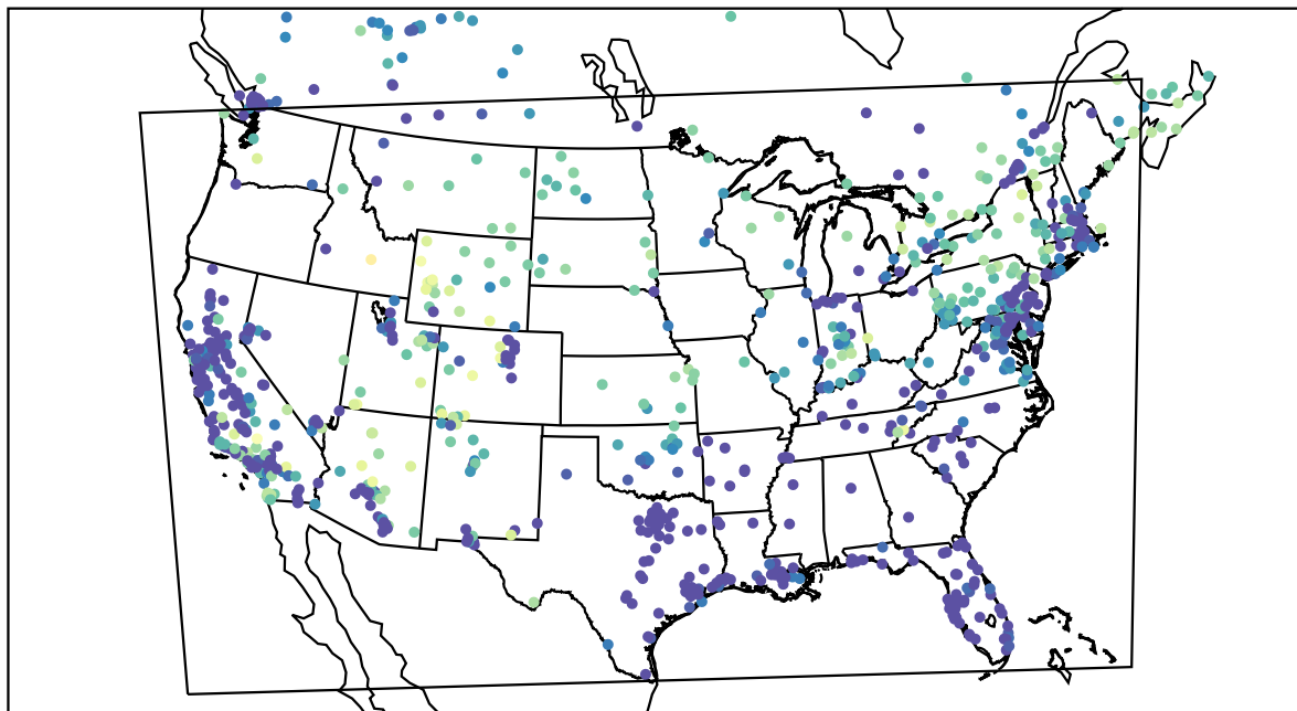
AirNOW (2021-02-10_07:00:00)
