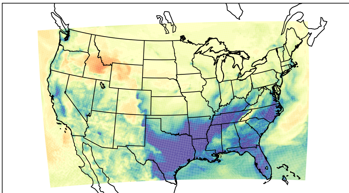
WRF (2021-02-10_11:00:00)
