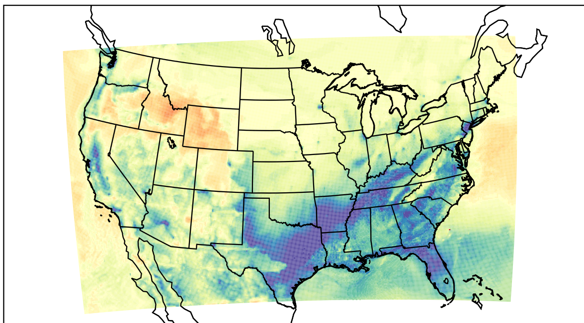
WRF (2021-02-09_15:00:00)
