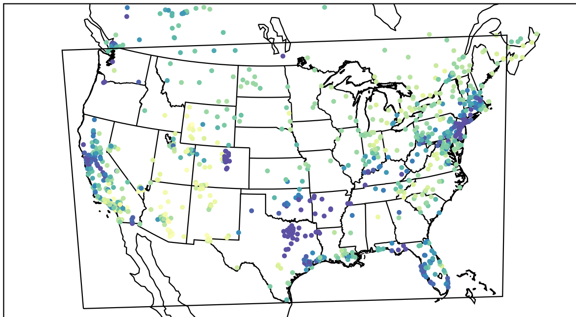
AirNOW (2021-02-09_19:00:00)
