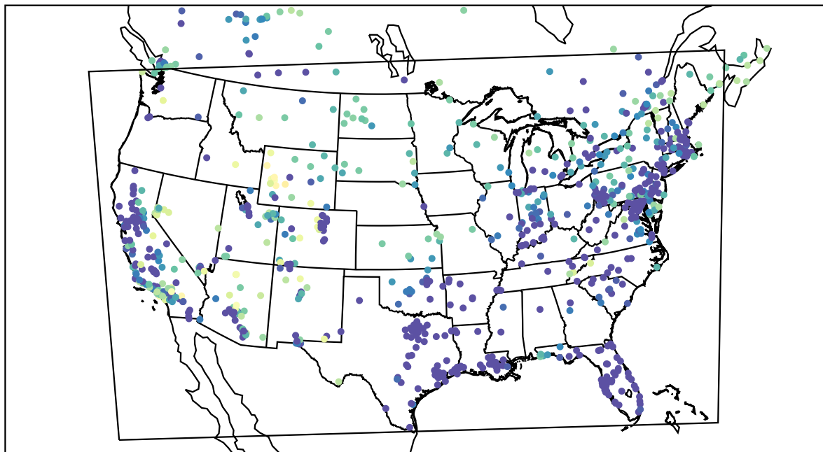
AirNOW (2021-02-09_11:00:00)
