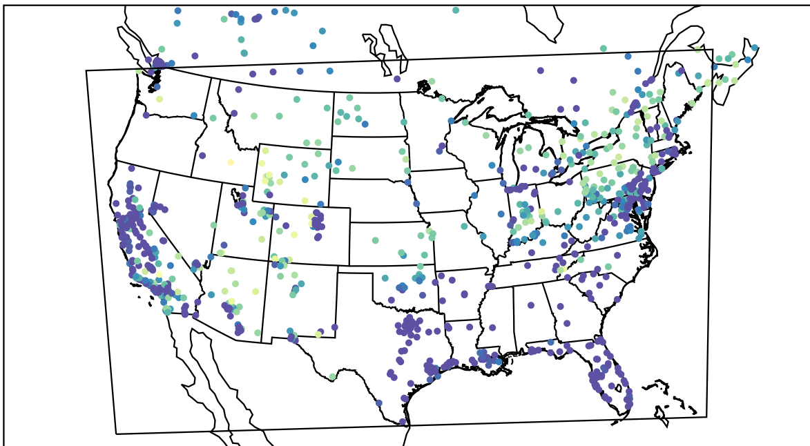
AirNOW (2021-02-10_08:00:00)
