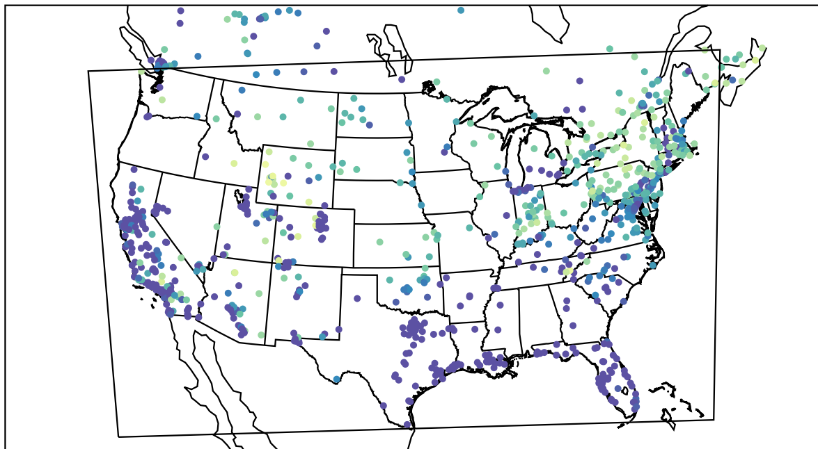
AirNOW (2021-02-10_14:00:00)
