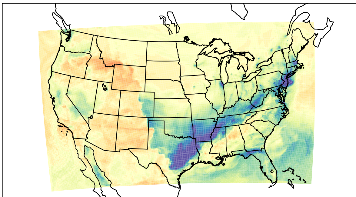
WRF (2021-02-09_22:00:00)
