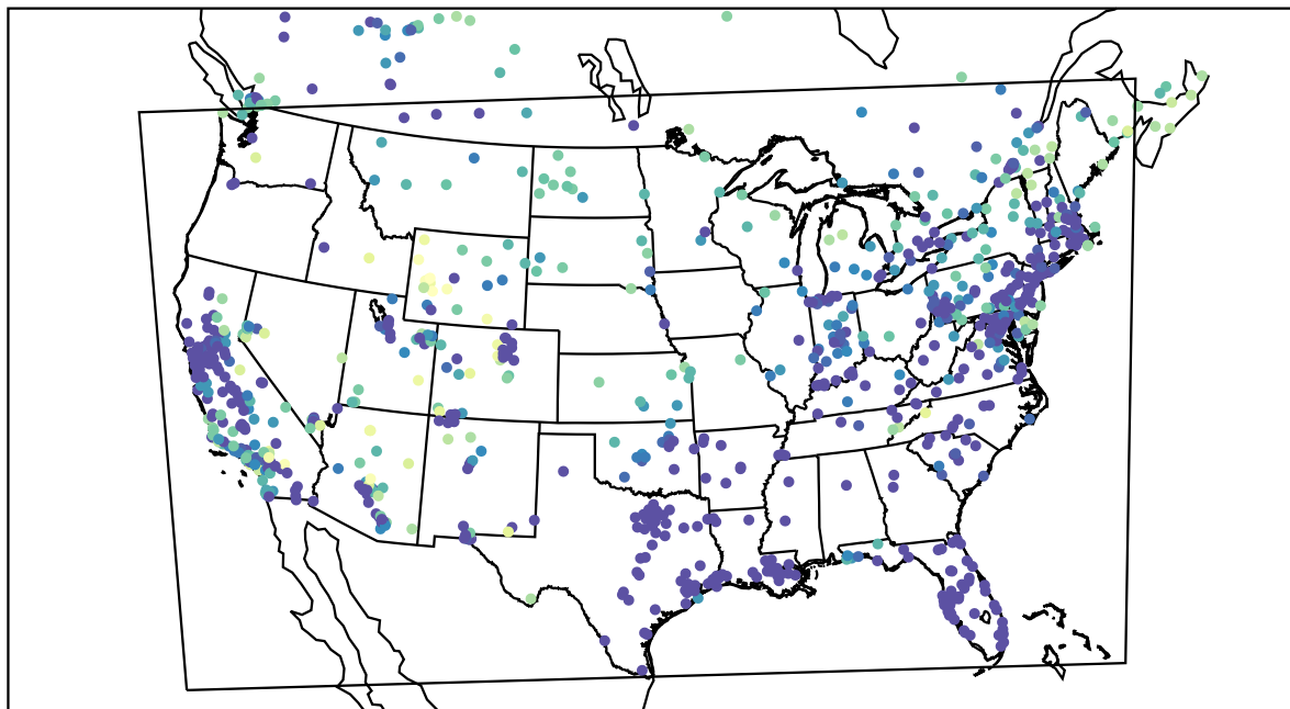
AirNOW (2021-02-09_13:00:00)
