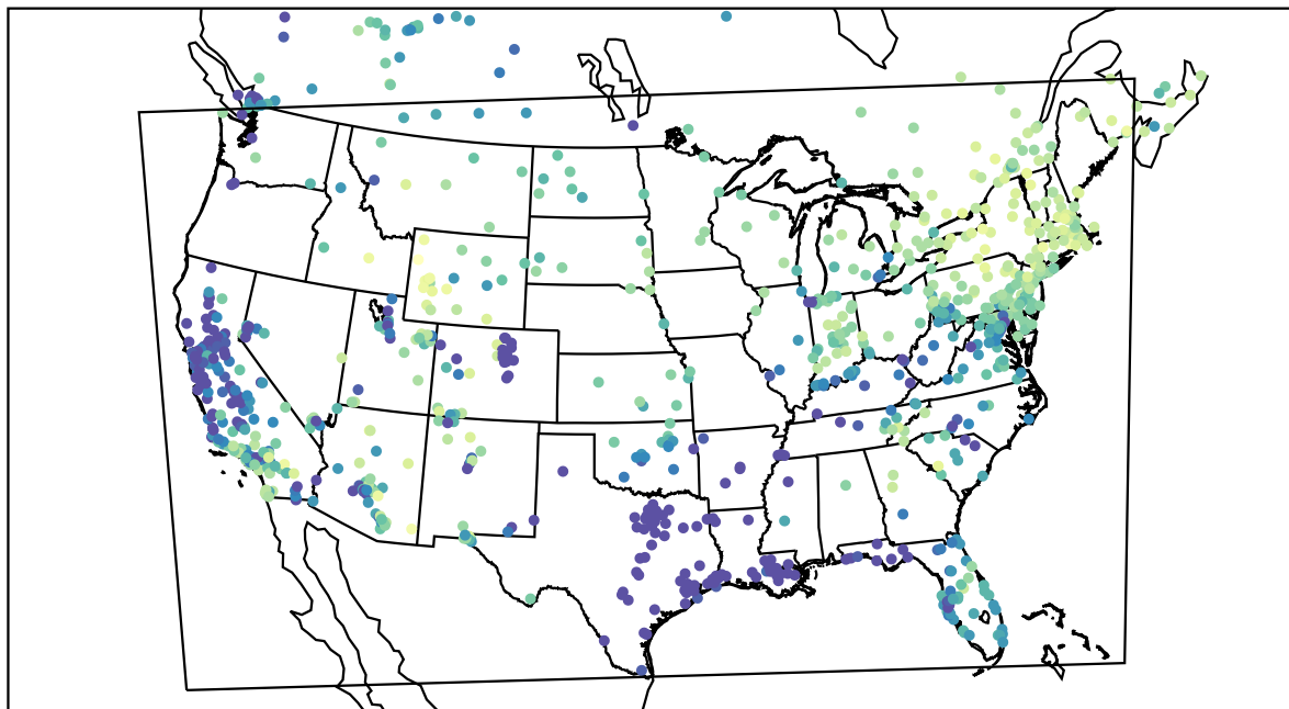
AirNOW (2021-02-10_17:00:00)
