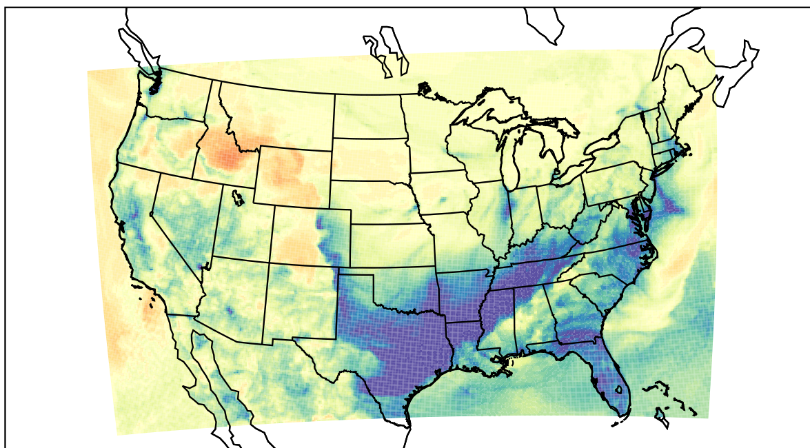
WRF (2021-02-10_06:00:00)
