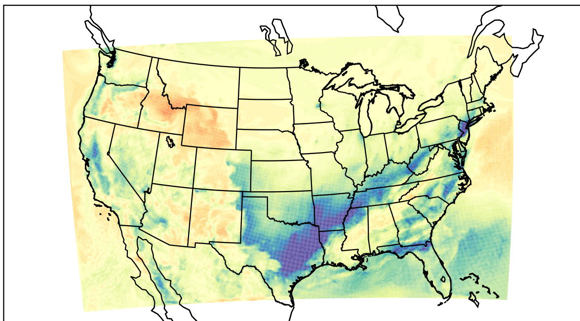
WRF (2021-02-09_18:00:00)
