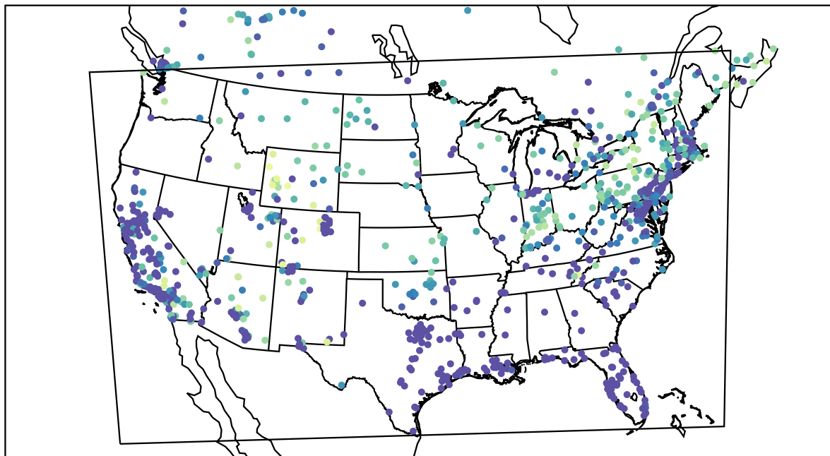
AirNOW (2021-02-10_13:00:00)
