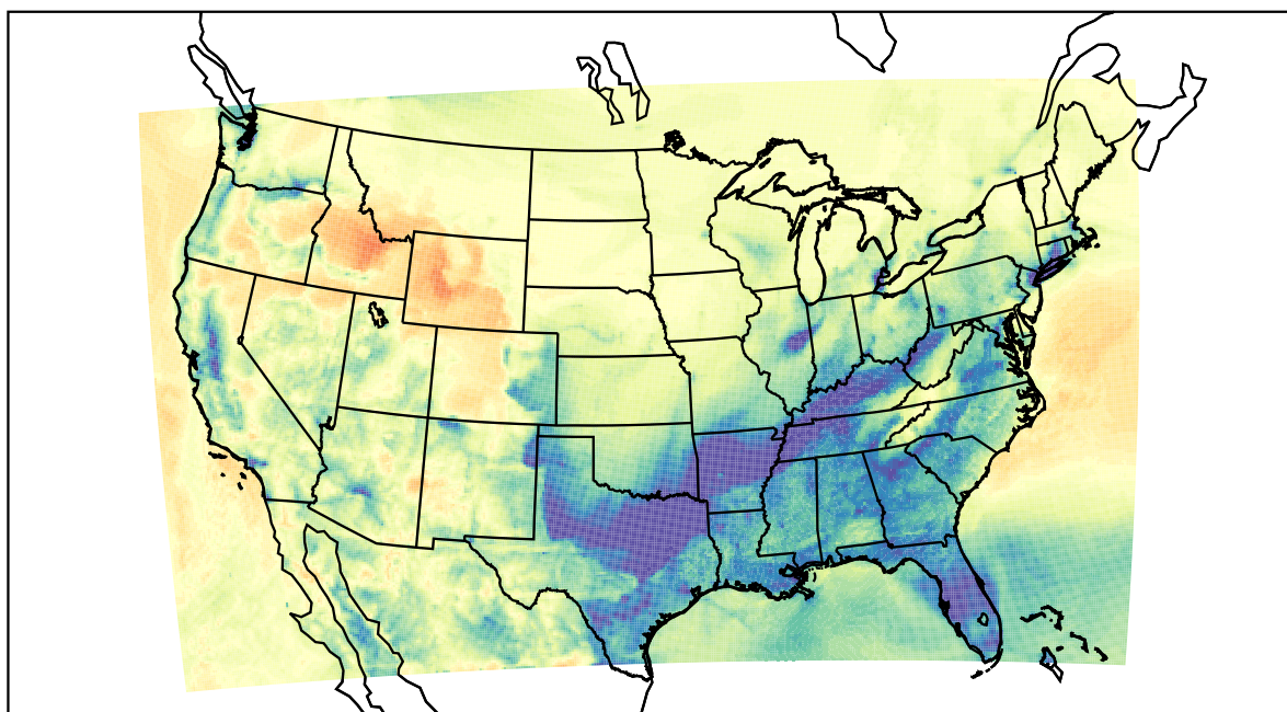
WRF (2021-02-09_11:00:00)
