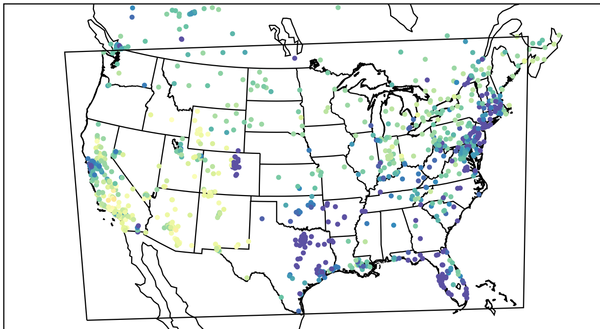
AirNOW (2021-02-09_23:00:00)
