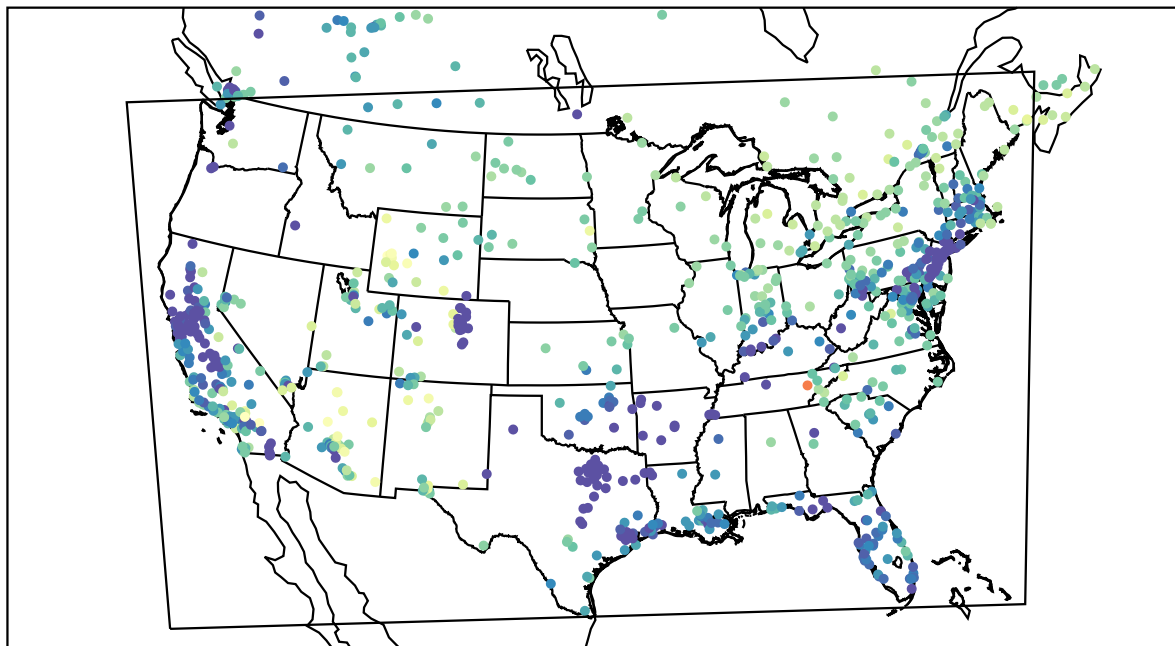
AirNOW (2021-02-09_17:00:00)
