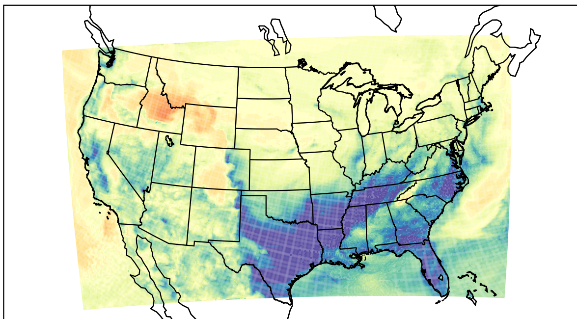
WRF (2021-02-10_10:00:00)
