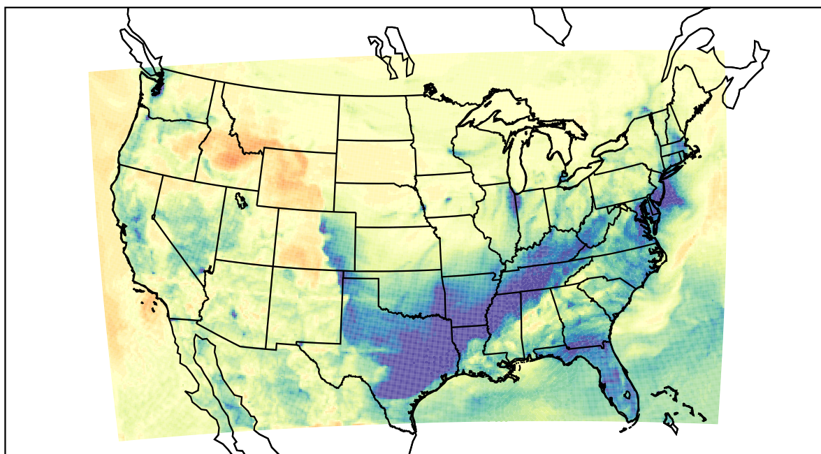
WRF (2021-02-10_03:00:00)
