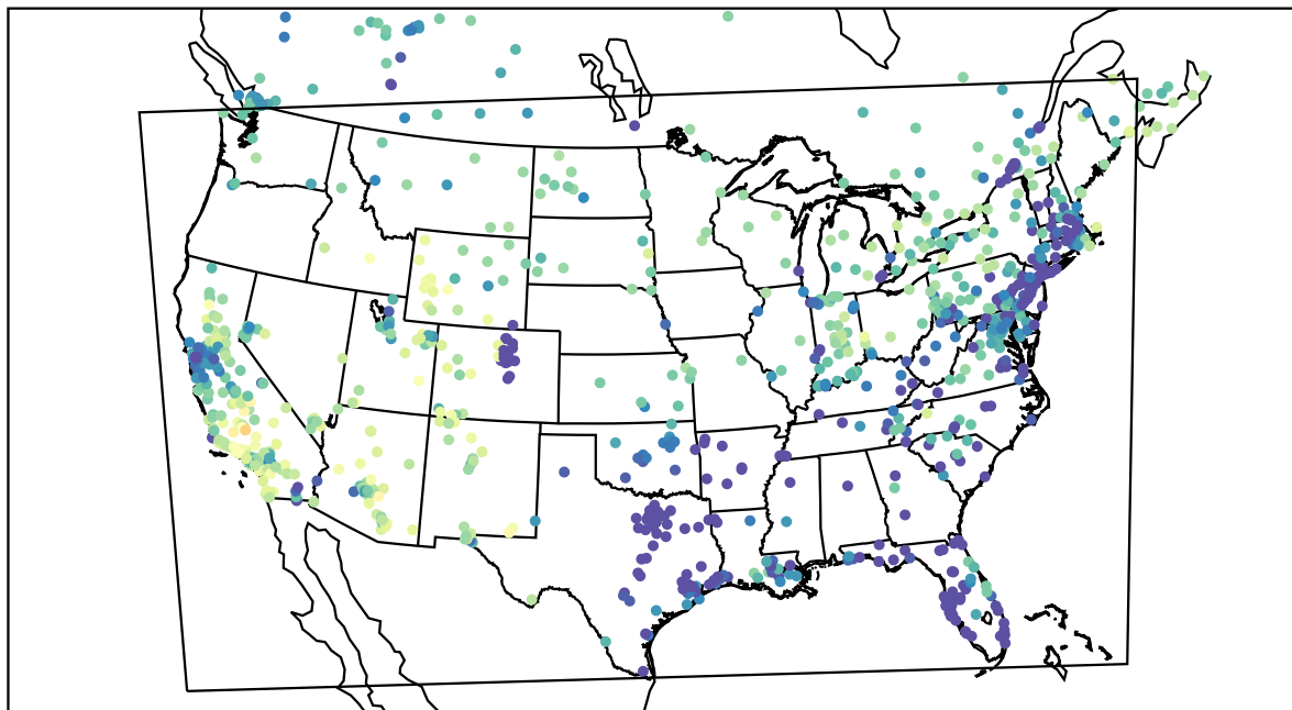
AirNOW (2021-02-10_00:00:00)
