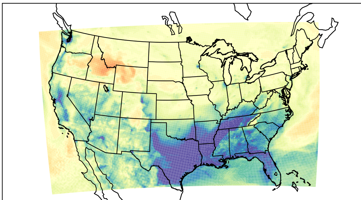
WRF (2021-02-10_15:00:00)
