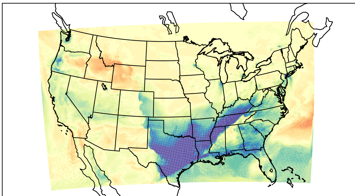
WRF (2021-02-10_22:00:00)
