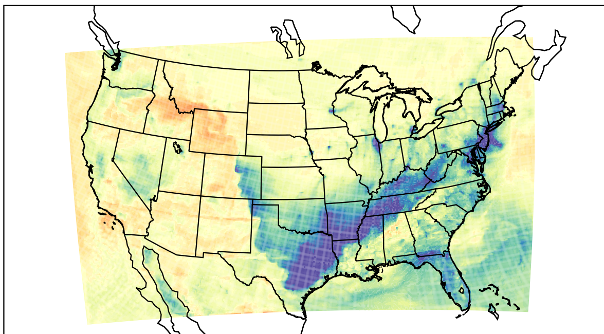
WRF (2021-02-10_00:00:00)
