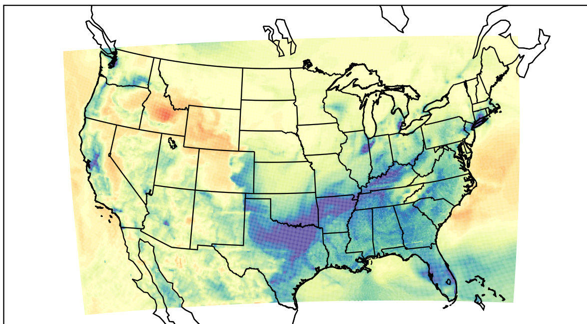
WRF (2021-02-09_07:00:00)
