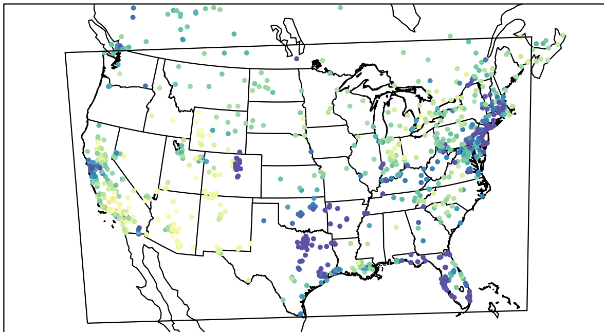
AirNOW (2021-02-09_22:00:00)
