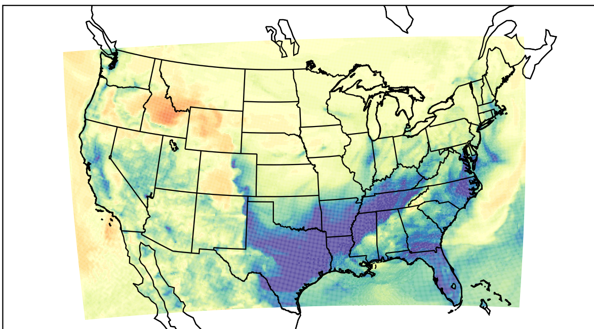
WRF (2021-02-10_08:00:00)
