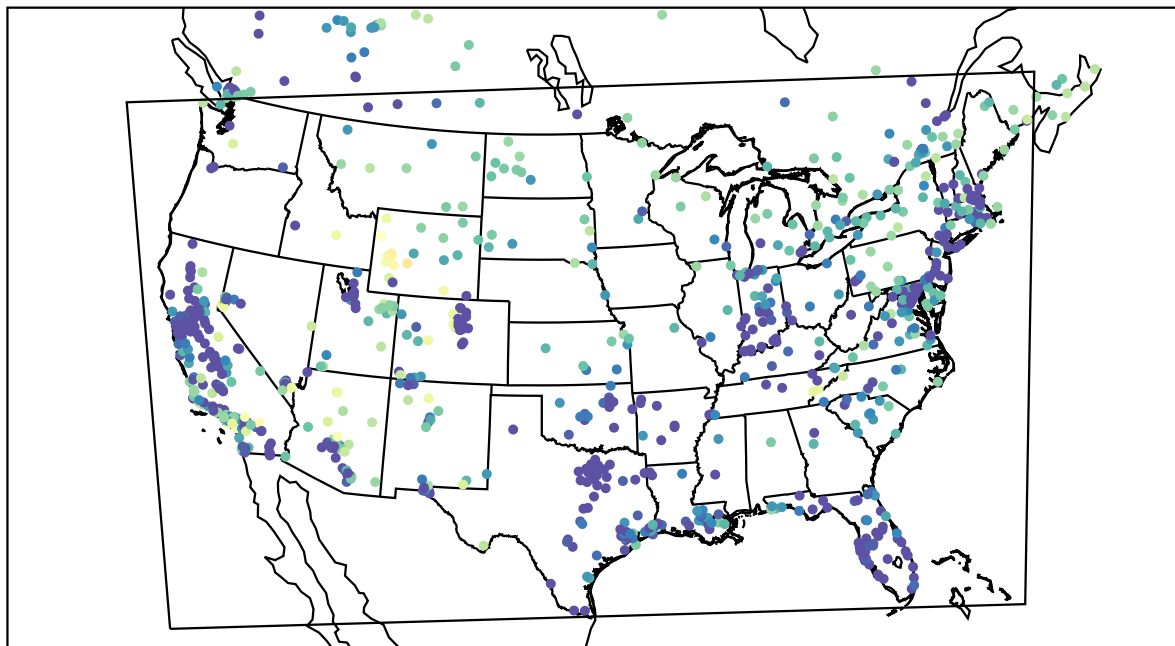
AirNOW (2021-02-09_06:00:00)
