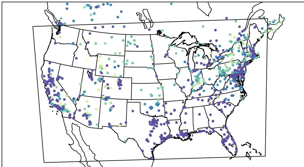
AirNOW (2021-02-10_11:00:00)
