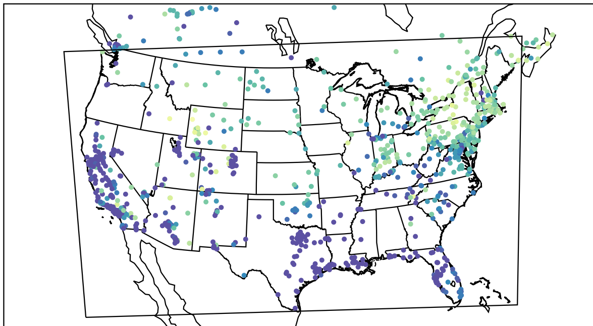
AirNOW (2021-02-10_15:00:00)
