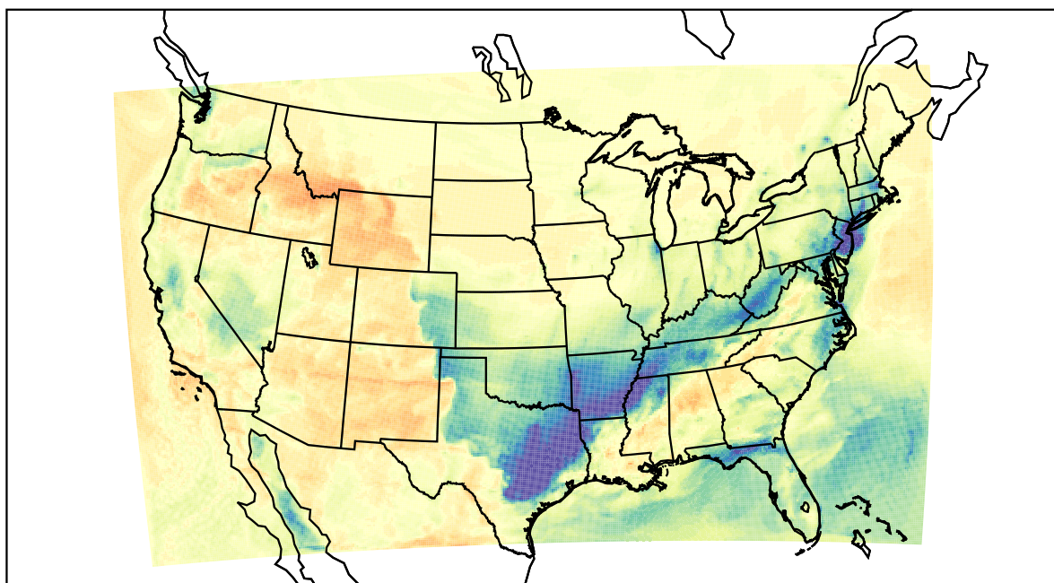
WRF (2021-02-09_21:00:00)
