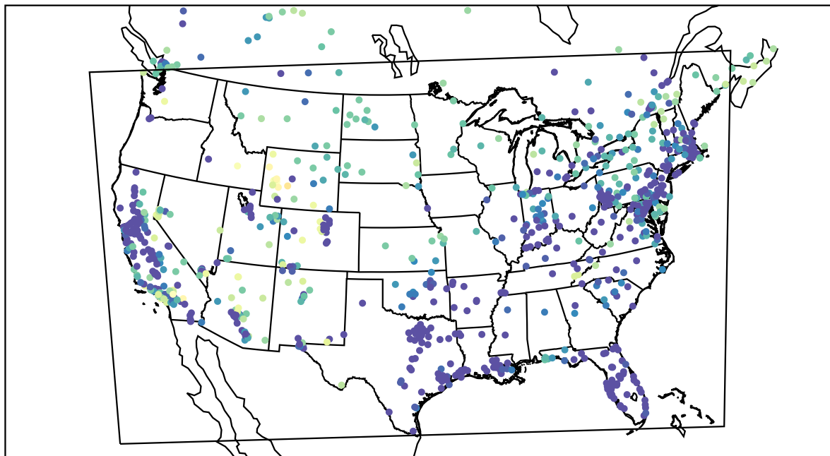
AirNOW (2021-02-09_10:00:00)
