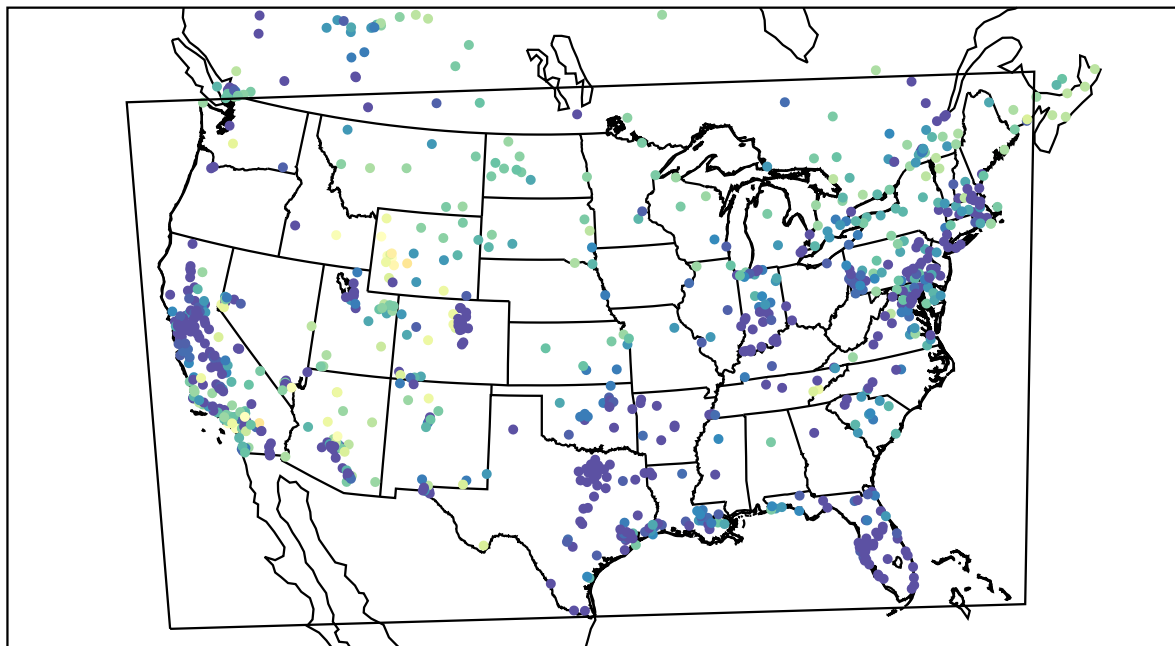
AirNOW (2021-02-09_07:00:00)
