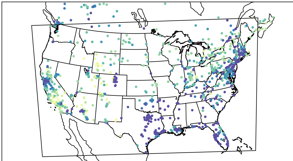
AirNOW (2021-02-10_01:00:00)
