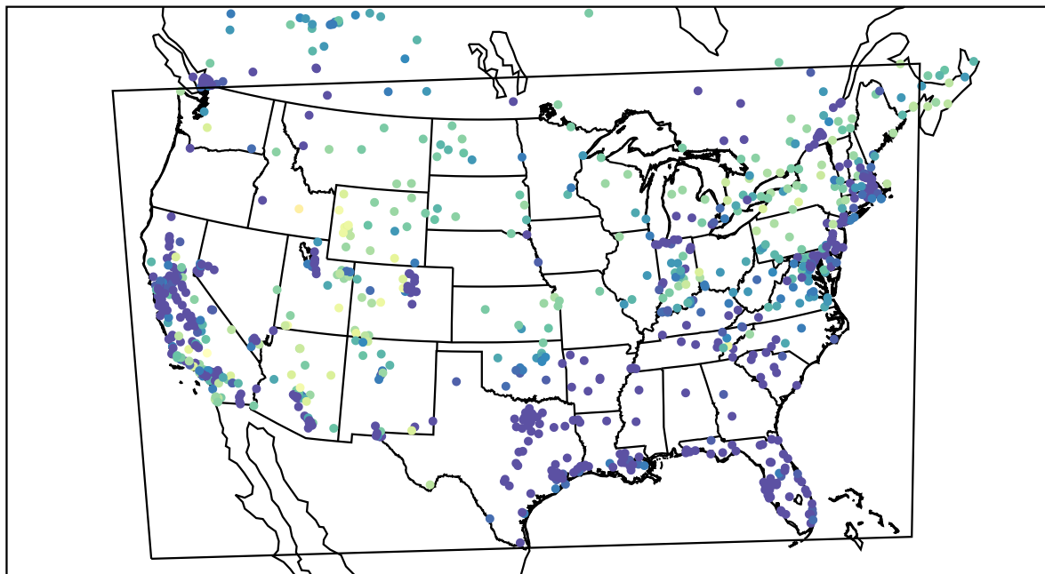
AirNOW (2021-02-10_06:00:00)
