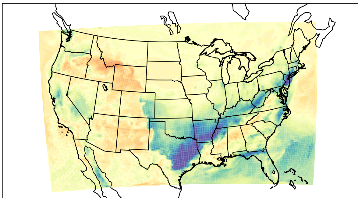
WRF (2021-02-09_20:00:00)
