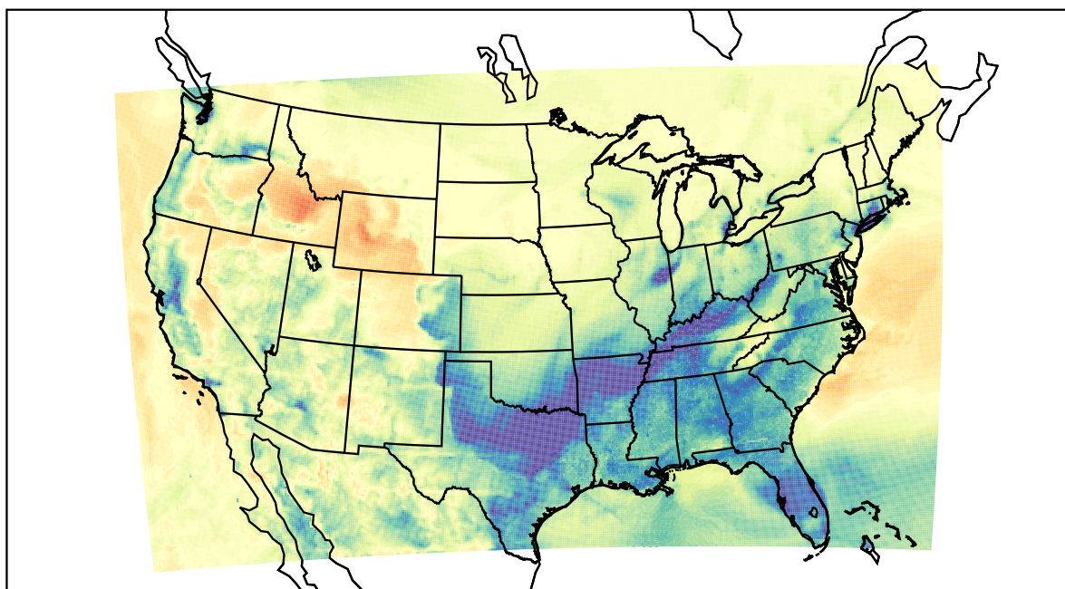
WRF (2021-02-09_09:00:00)
