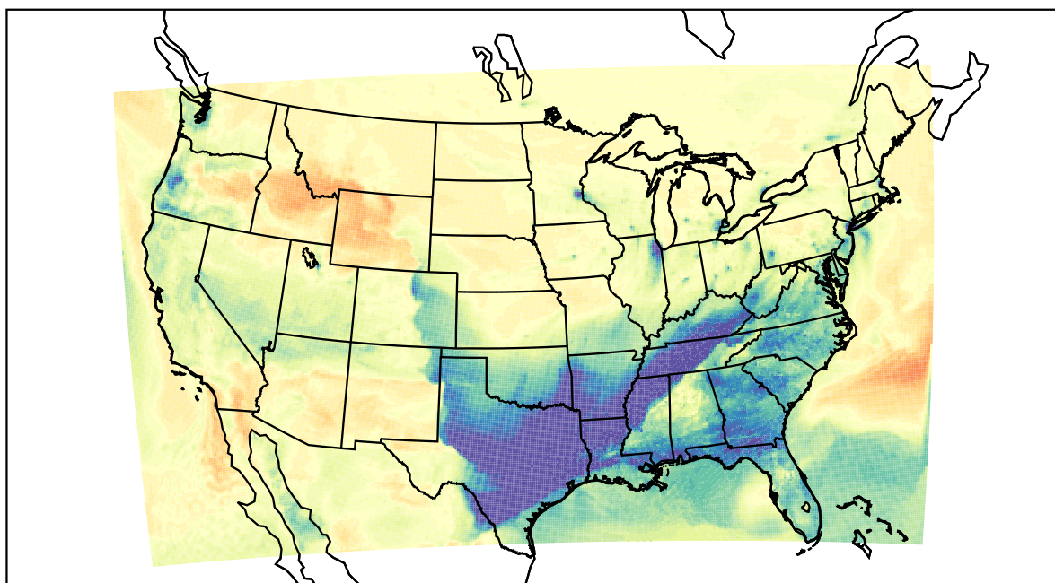
WRF (2021-02-10_23:00:00)
