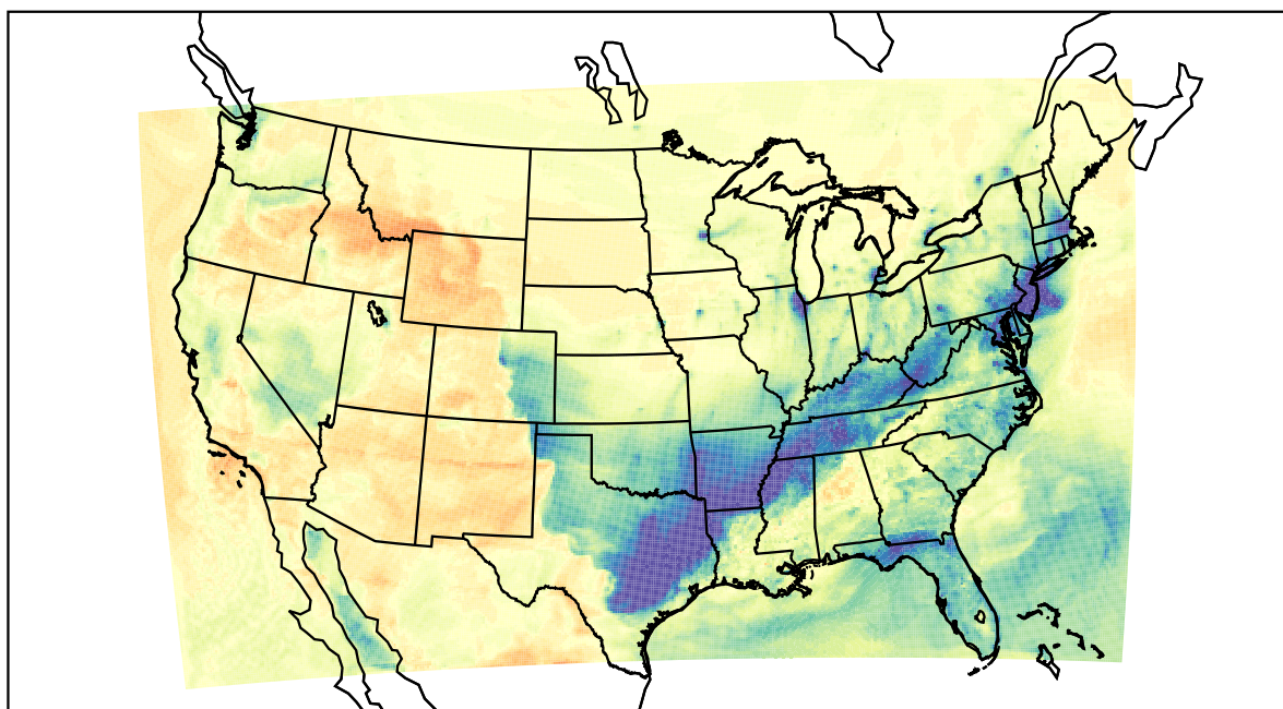
WRF (2021-02-09_23:00:00)
