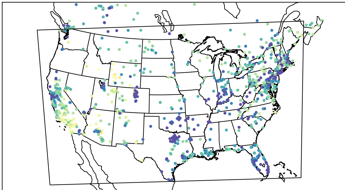
AirNOW (2021-02-09_01:00:00)
