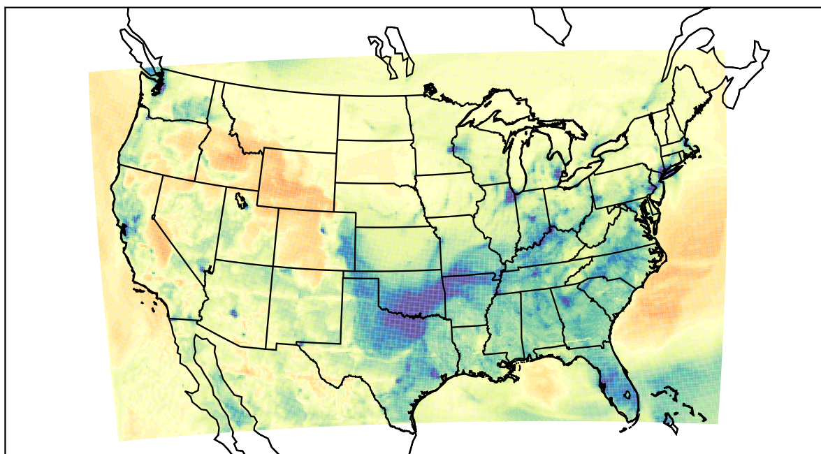
WRF (2021-02-09_02:00:00)
