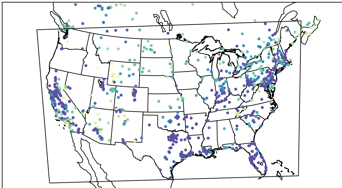
AirNOW (2021-02-09_09:00:00)
