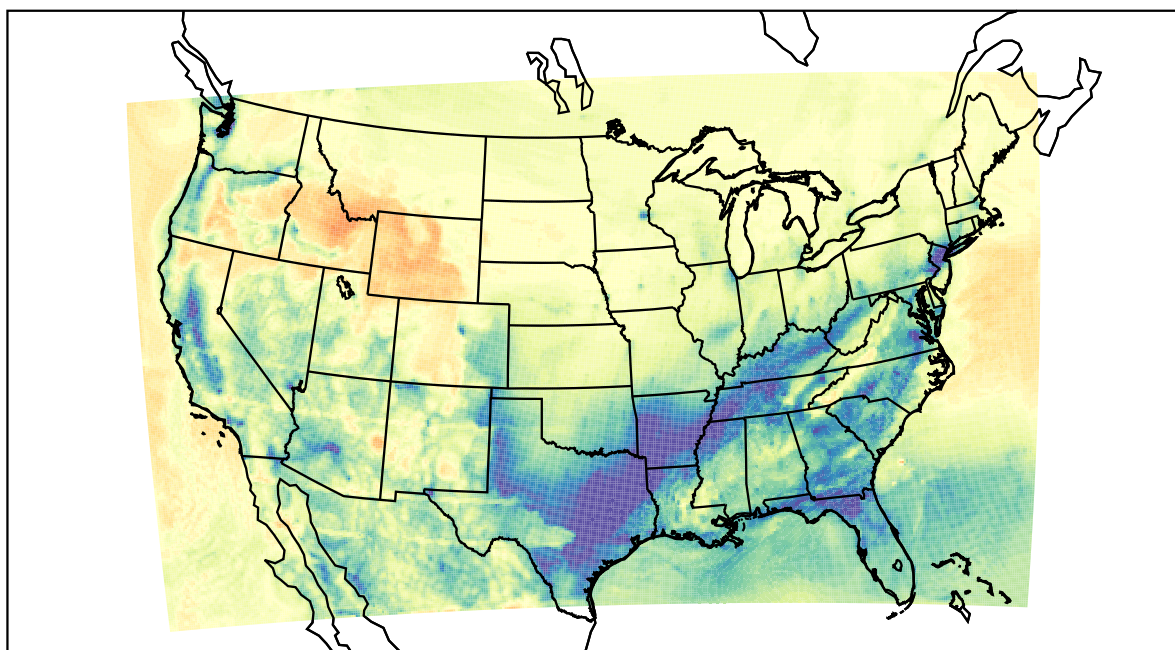
WRF (2021-02-09_16:00:00)
