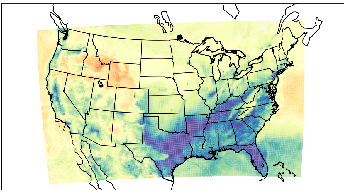
WRF (2021-02-09_14:00:00)
