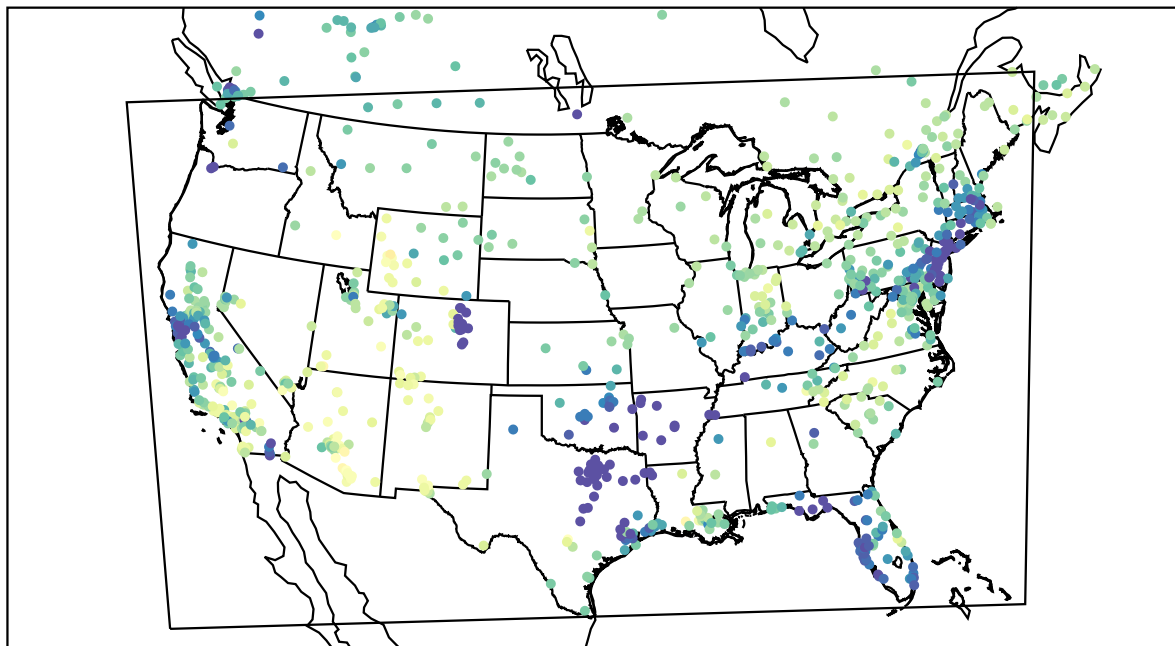
AirNOW (2021-02-09_20:00:00)
