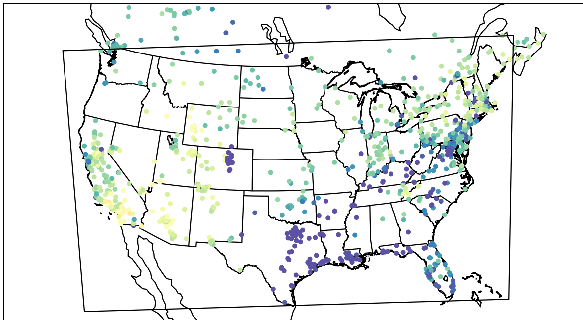
AirNOW (2021-02-10_23:00:00)
