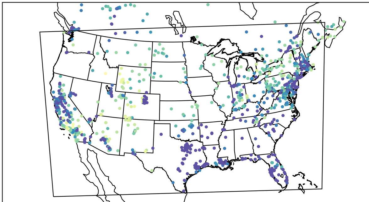
AirNOW (2021-02-10_03:00:00)
