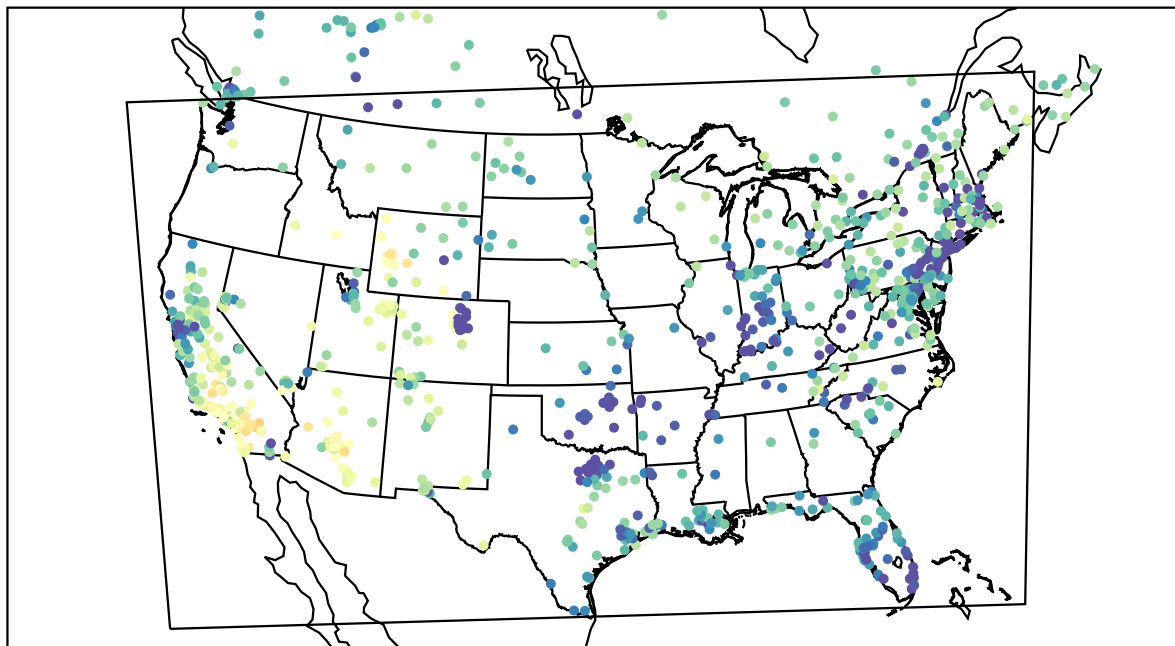
AirNOW (2021-02-09_00:00:00)
