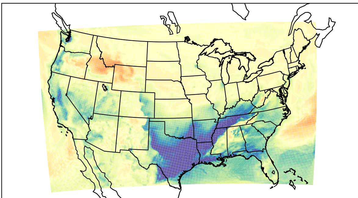
WRF (2021-02-10_18:00:00)
