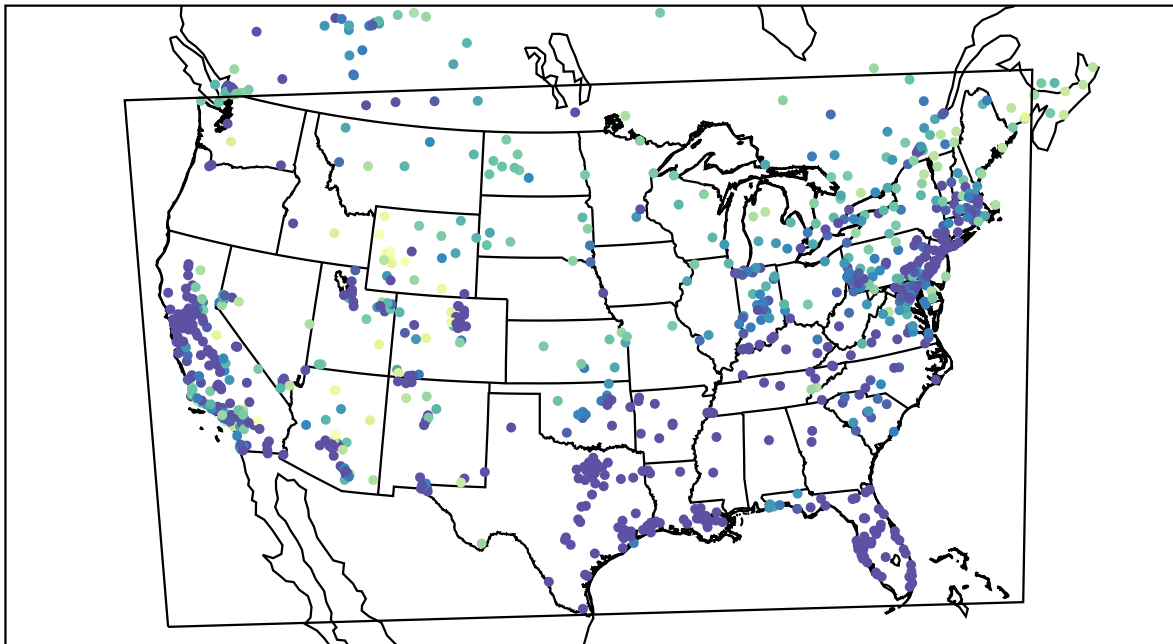
AirNOW (2021-02-09_14:00:00)
