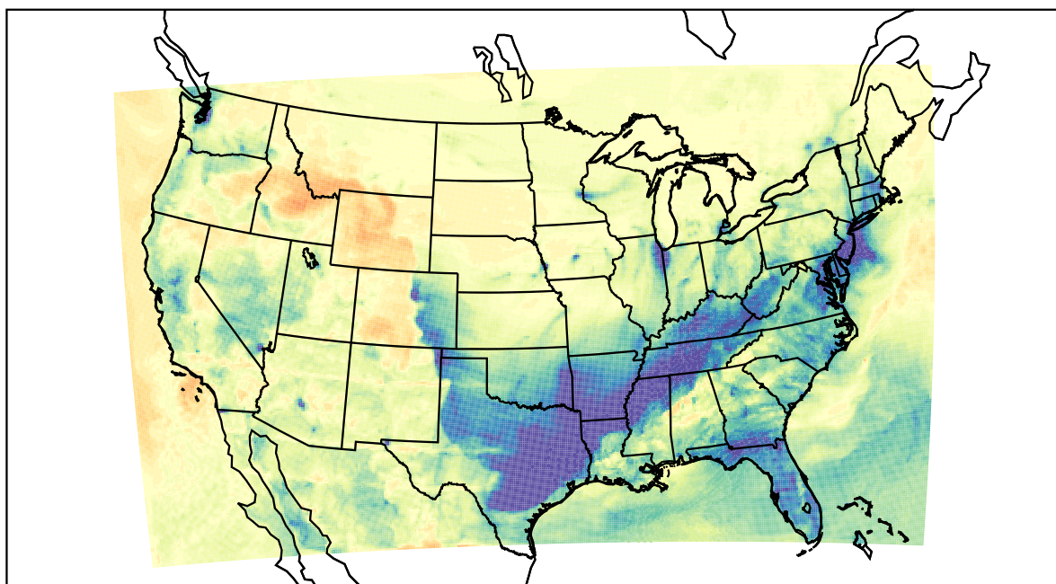
WRF (2021-02-10_02:00:00)
