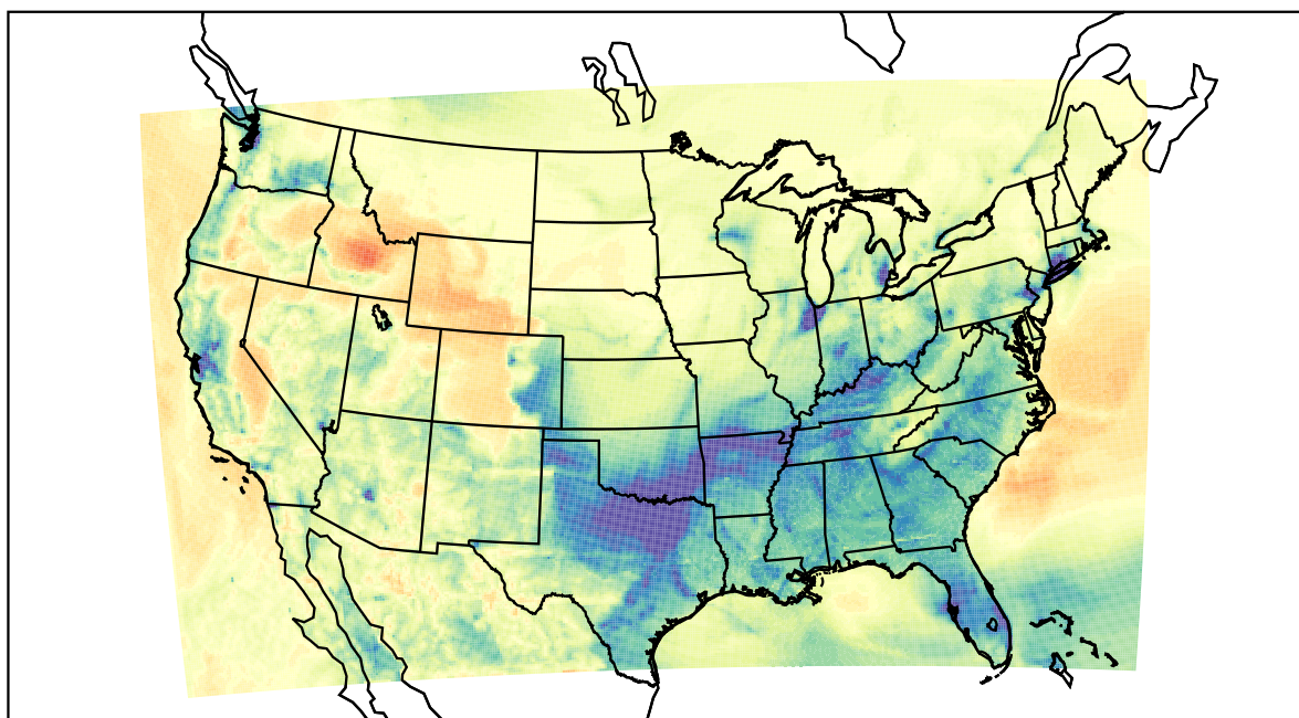
WRF (2021-02-09_05:00:00)
