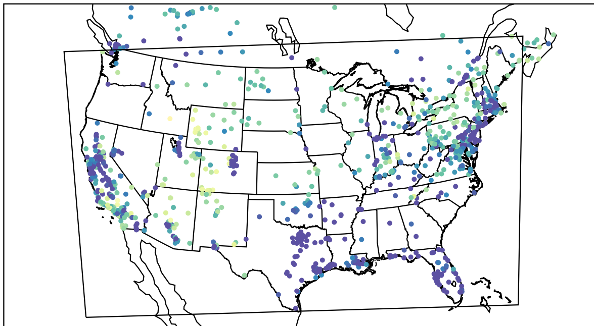
AirNOW (2021-02-10_04:00:00)
