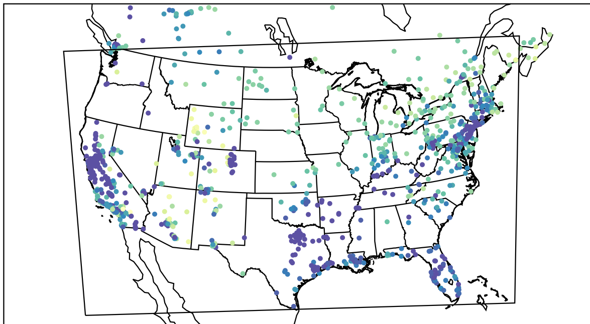
AirNOW (2021-02-09_16:00:00)
