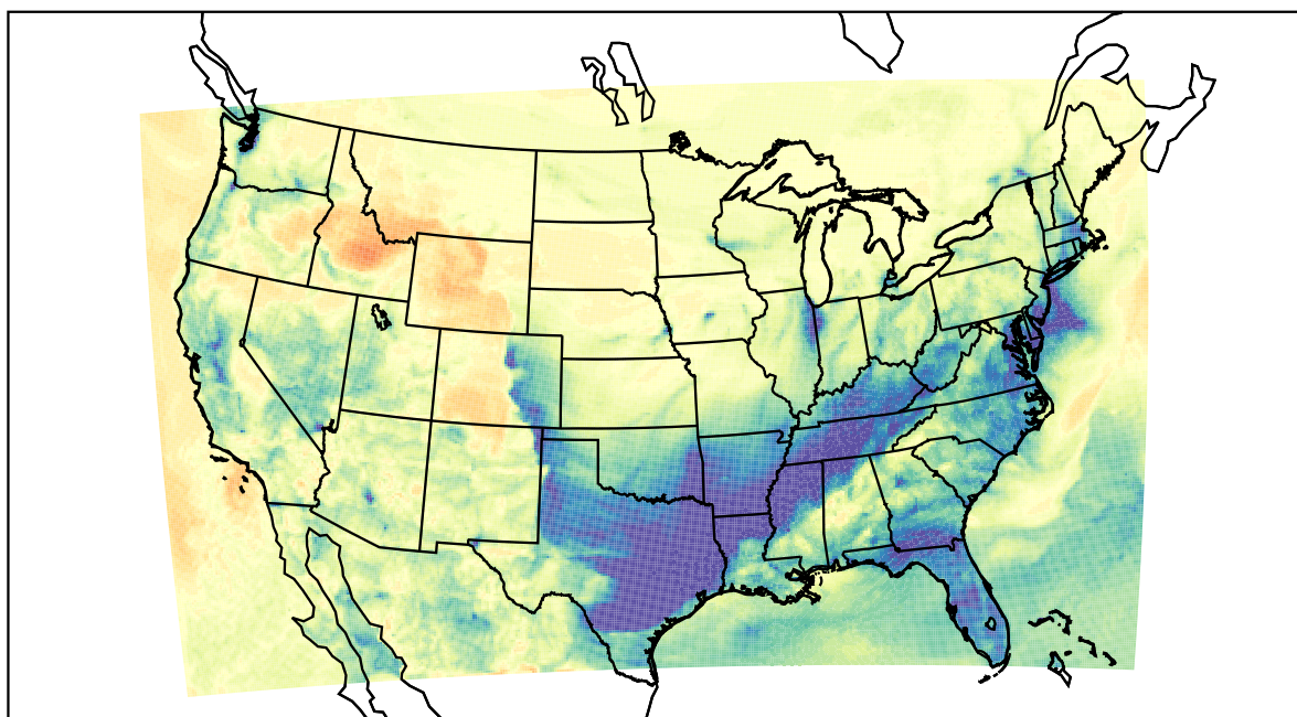
WRF (2021-02-10_04:00:00)
