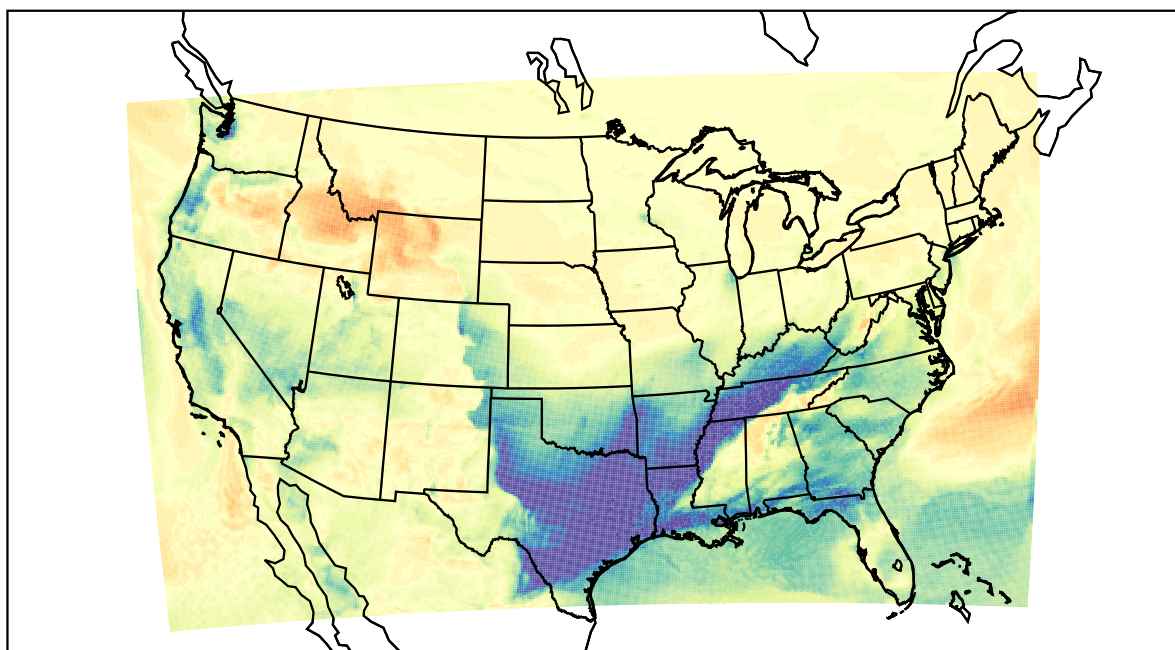
WRF (2021-02-10_19:00:00)
