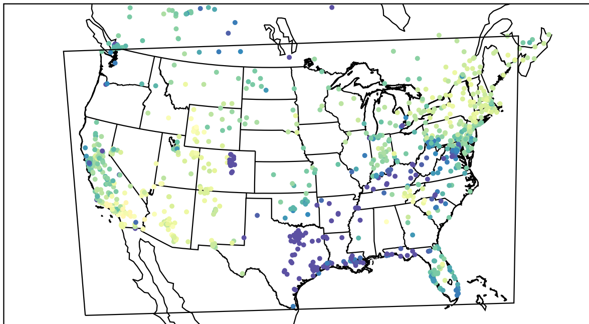
AirNOW (2021-02-10_21:00:00)
