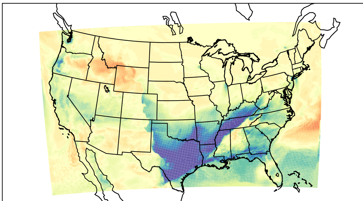
WRF (2021-02-10_21:00:00)
