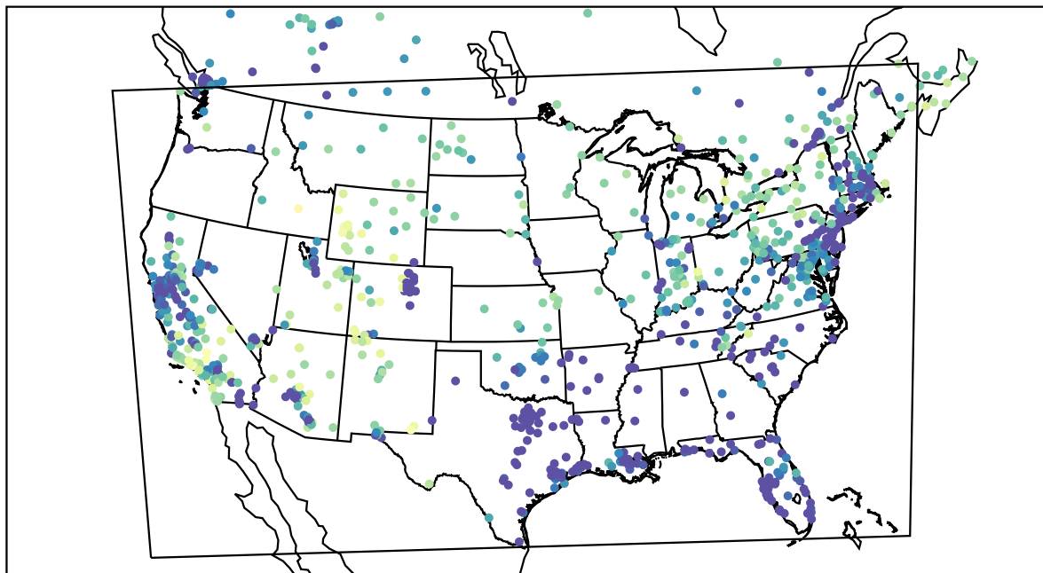
AirNOW (2021-02-10_02:00:00)
