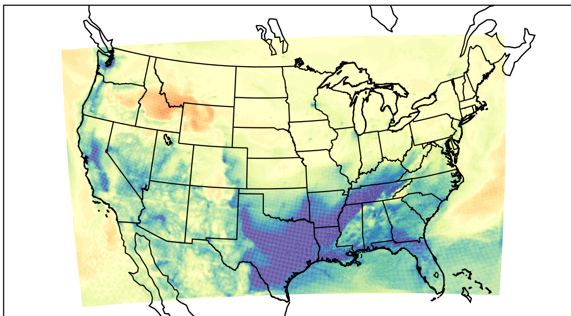
WRF (2021-02-10_16:00:00)
