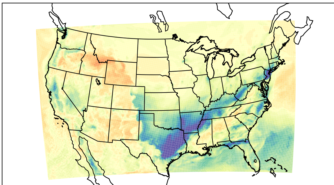
WRF (2021-02-09_19:00:00)
