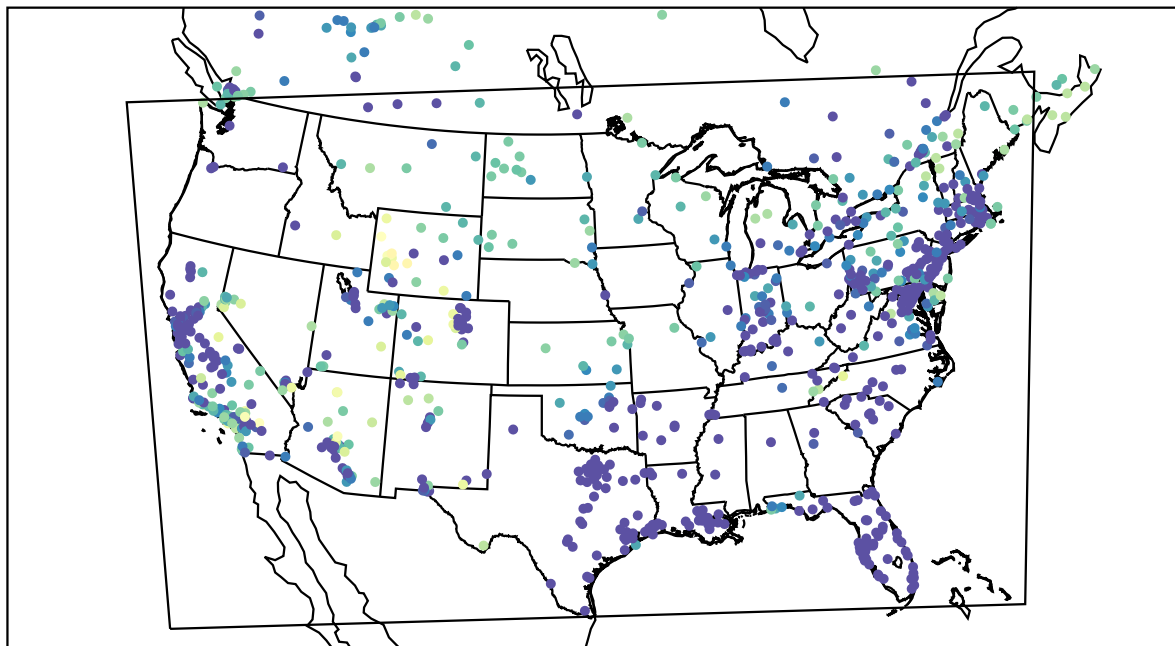
AirNOW (2021-02-09_12:00:00)
