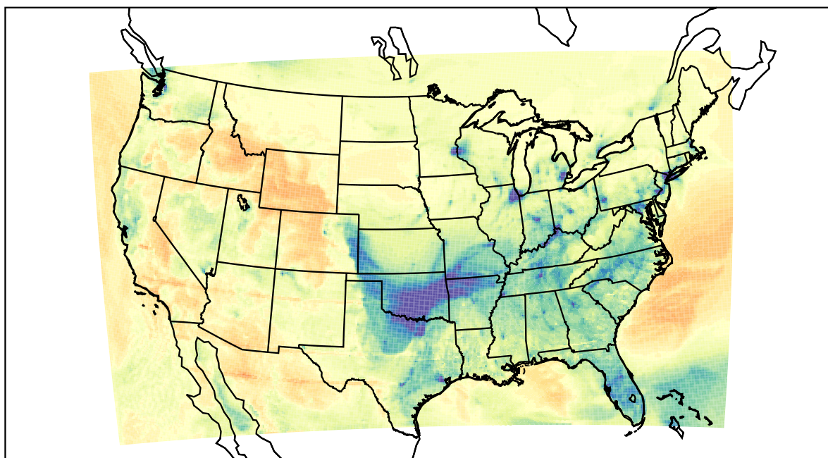
WRF (2021-02-09_00:00:00)
