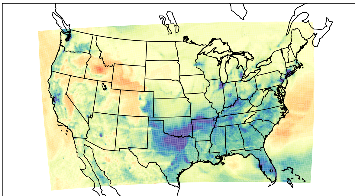
WRF (2021-02-09_04:00:00)
