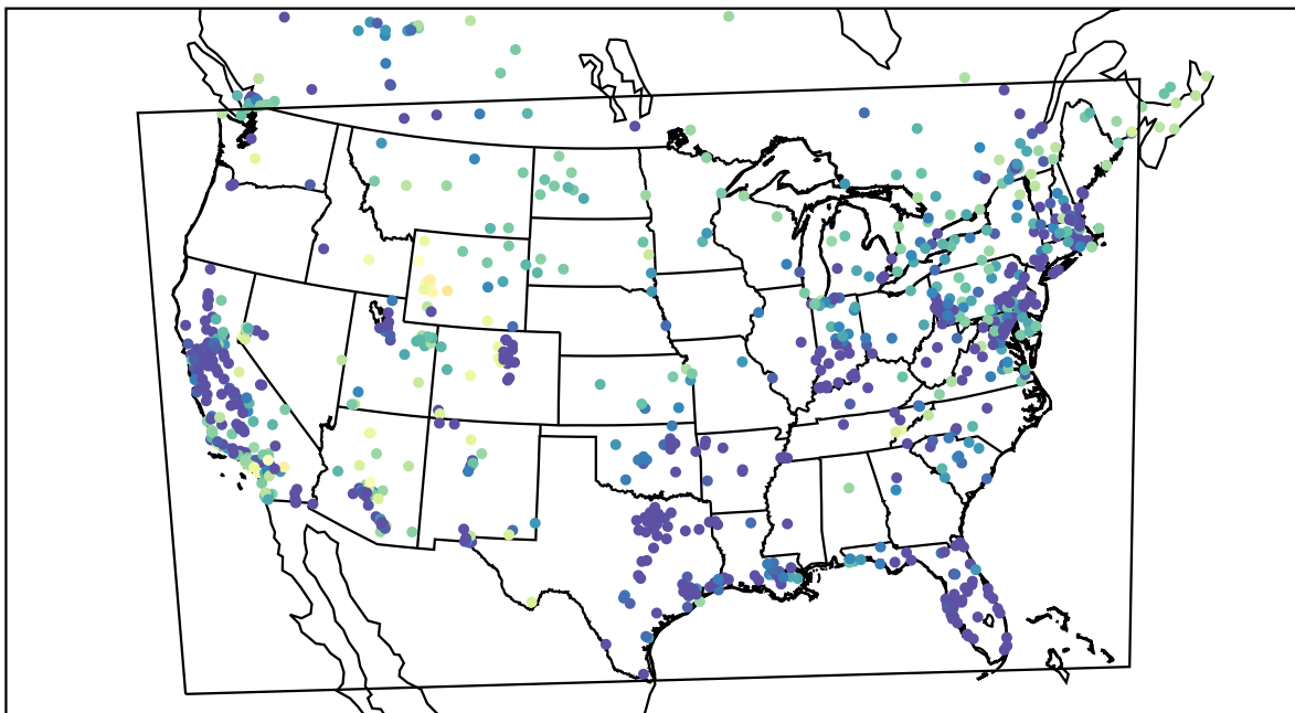
AirNOW (2021-02-09_08:00:00)
