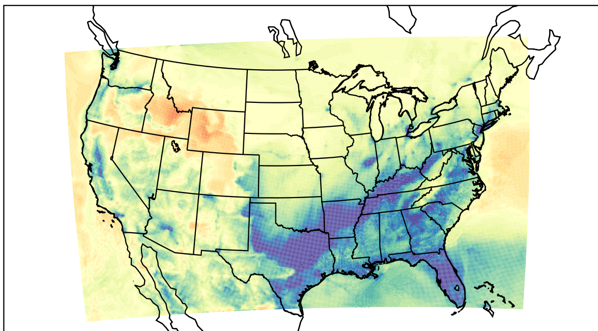
WRF (2021-02-09_13:00:00)
