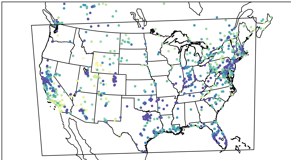
AirNOW (2021-02-09_02:00:00)
