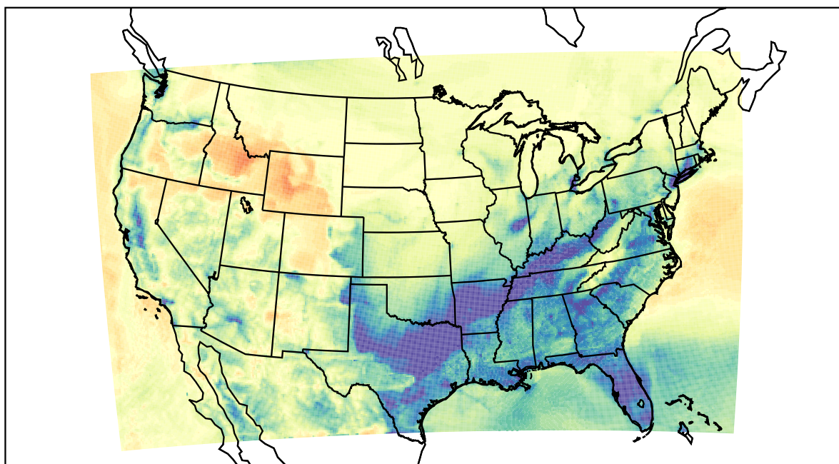
WRF (2021-02-09_12:00:00)
