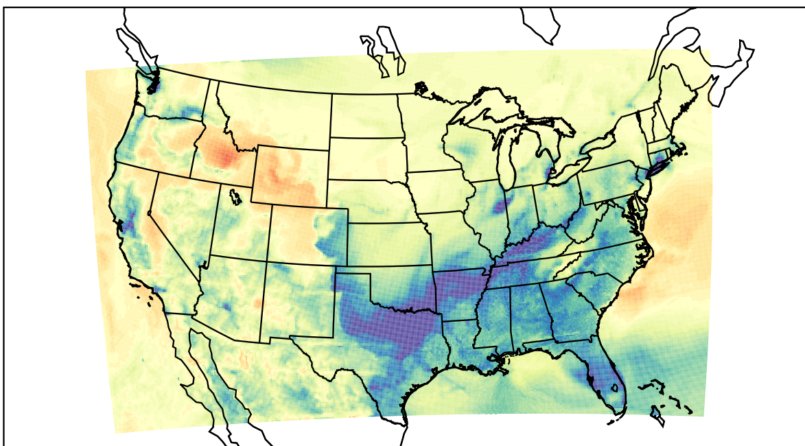
WRF (2021-02-09_08:00:00)
