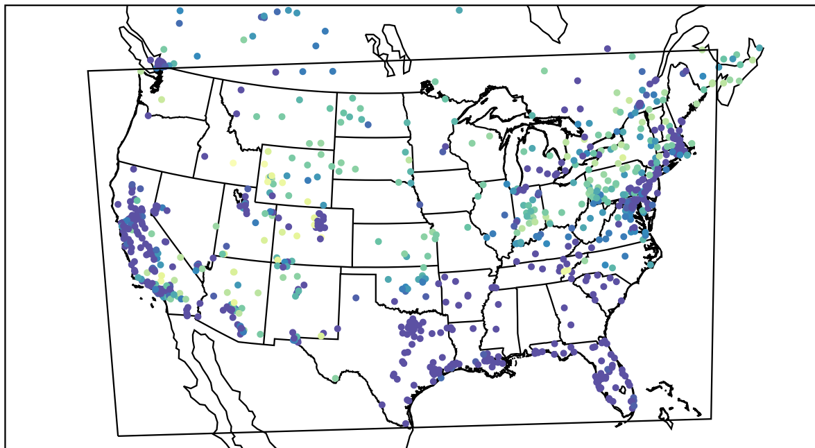
AirNOW (2021-02-10_10:00:00)
