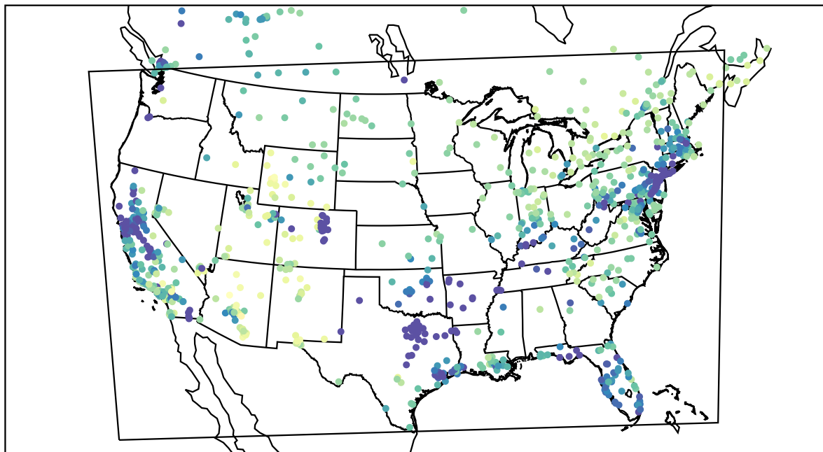
AirNOW (2021-02-09_18:00:00)
