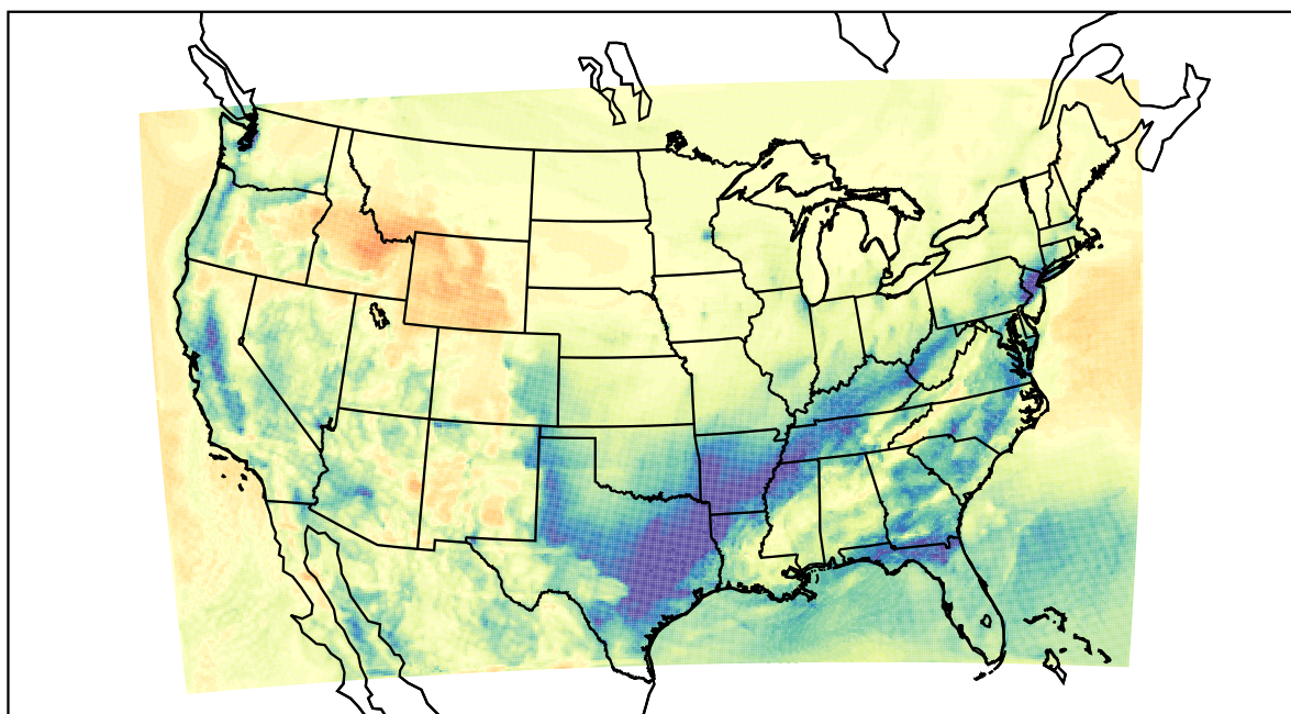
WRF (2021-02-09_17:00:00)
