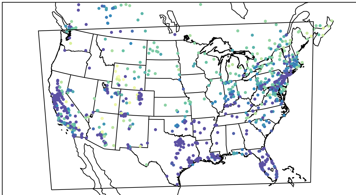
AirNOW (2021-02-09_15:00:00)
