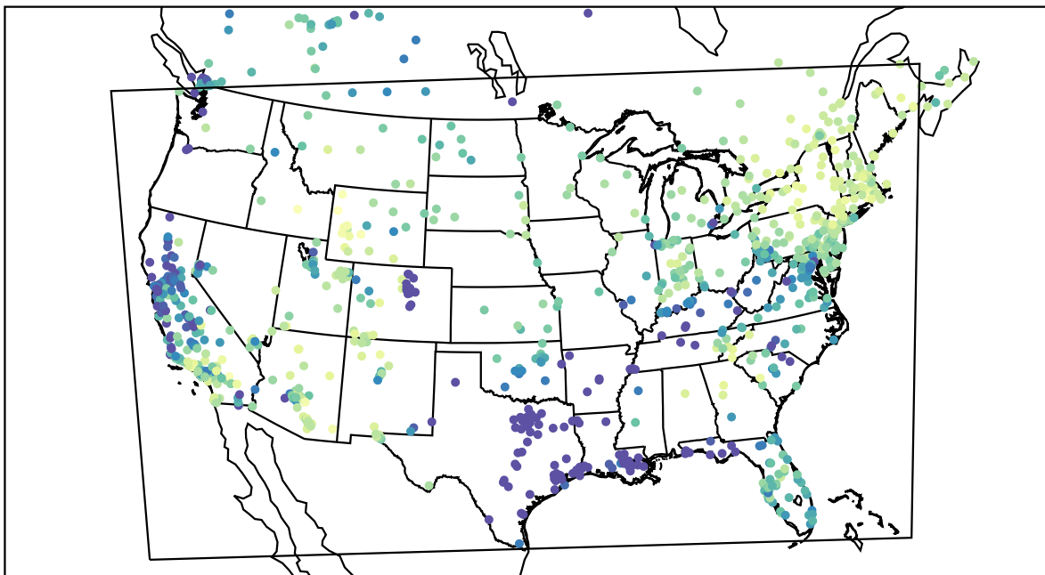
AirNOW (2021-02-10_18:00:00)
