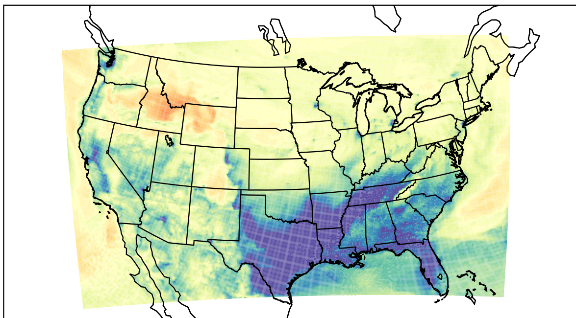
WRF (2021-02-10_14:00:00)
