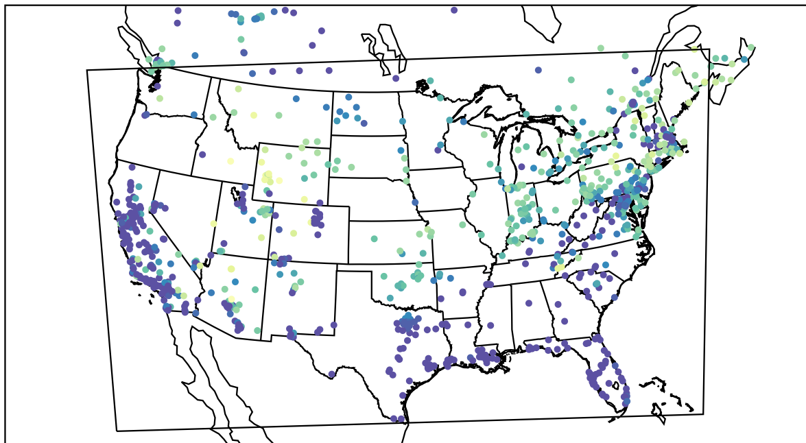
AirNOW (2021-02-11_08:00:00)
