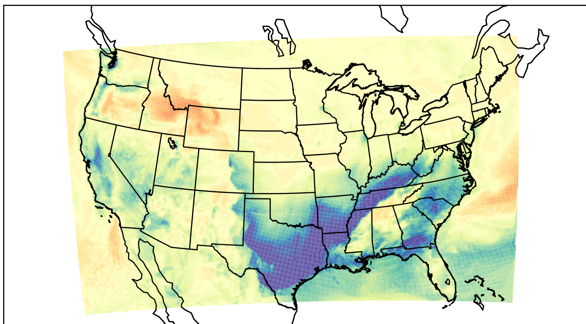
WRF (2021-02-10_18:00:00)
