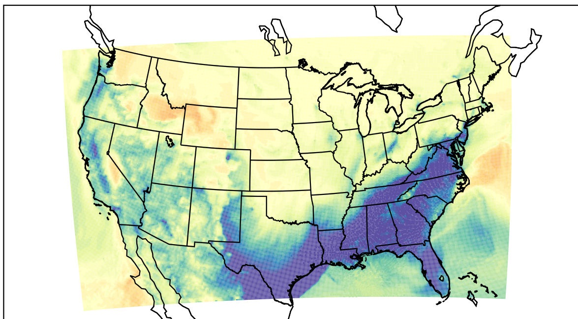
WRF (2021-02-11_12:00:00)
