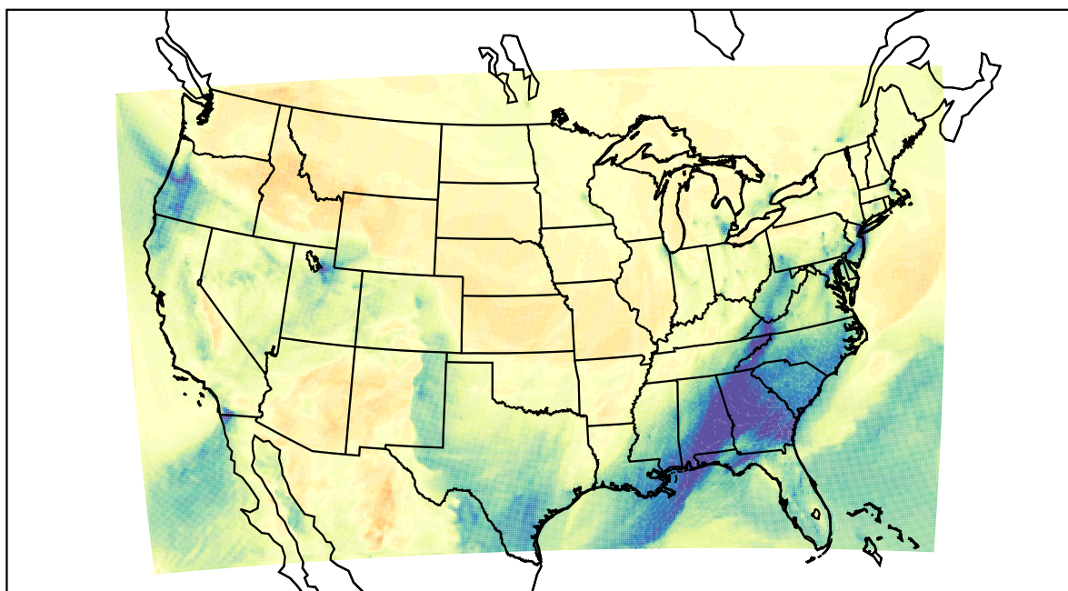
WRF (2021-02-12_22:00:00)
