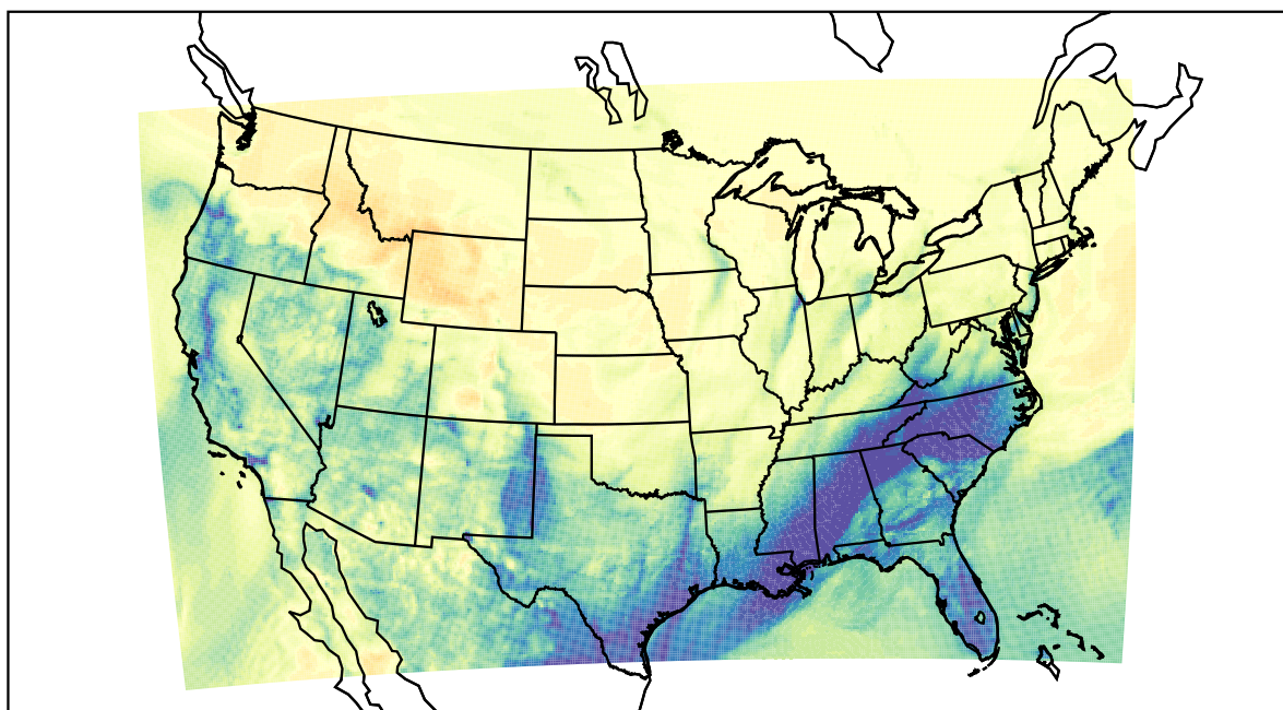
WRF (2021-02-12_06:00:00)
