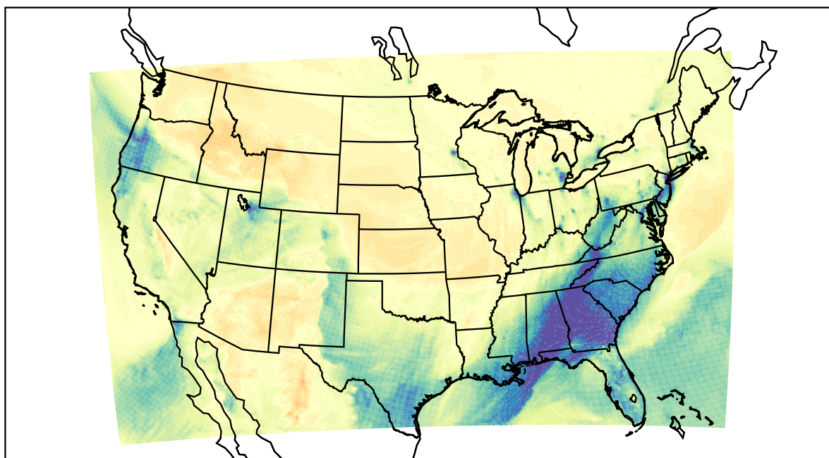
WRF (2021-02-12_23:00:00)
