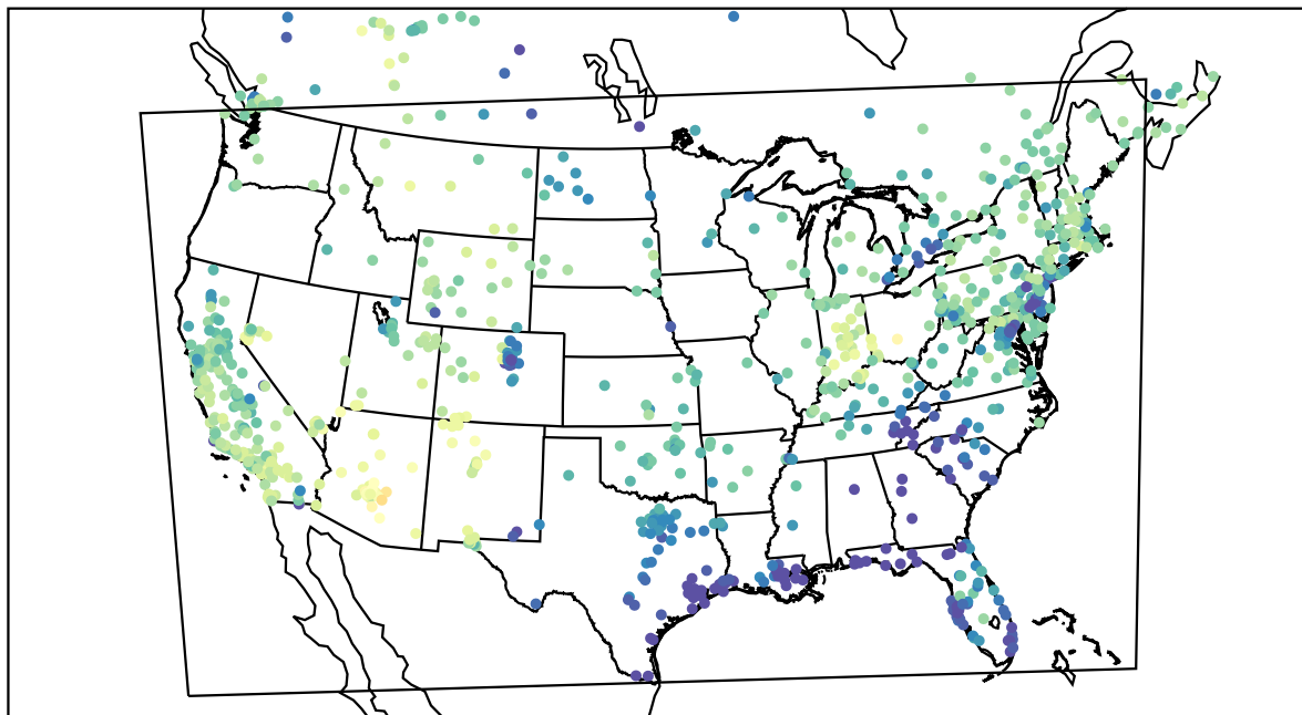
AirNOW (2021-02-12_22:00:00)
