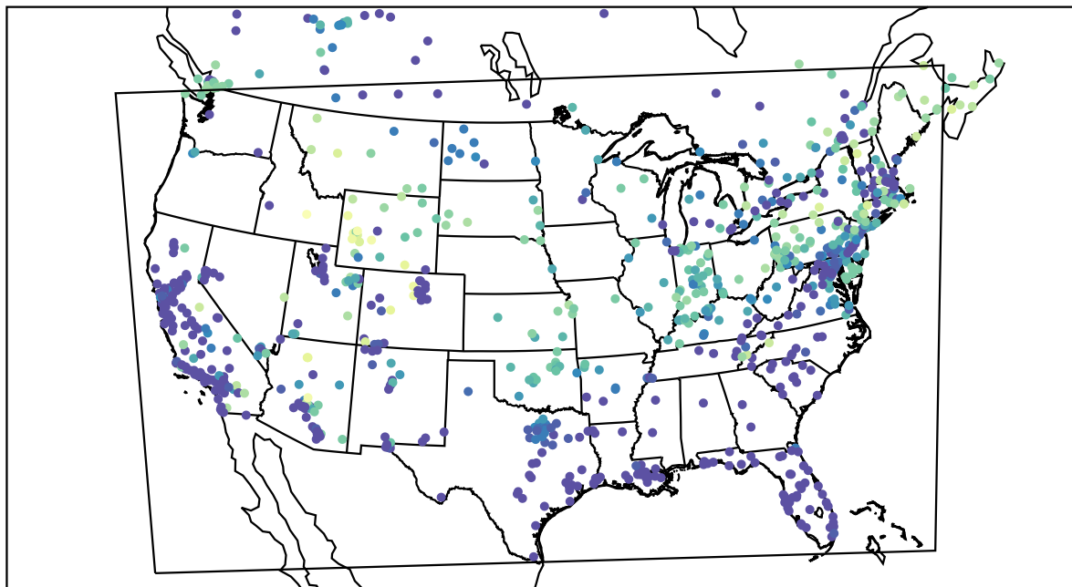
AirNOW (2021-02-11_12:00:00)
