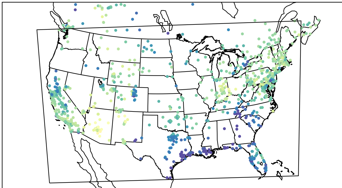
AirNOW (2021-02-12_19:00:00)
