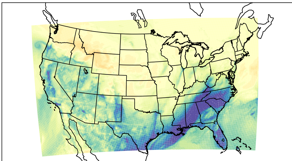
WRF (2021-02-12_09:00:00)
