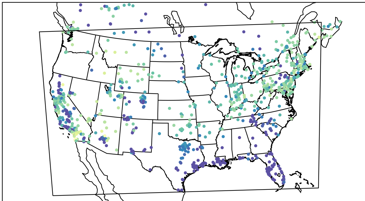
AirNOW (2021-02-12_09:00:00)
