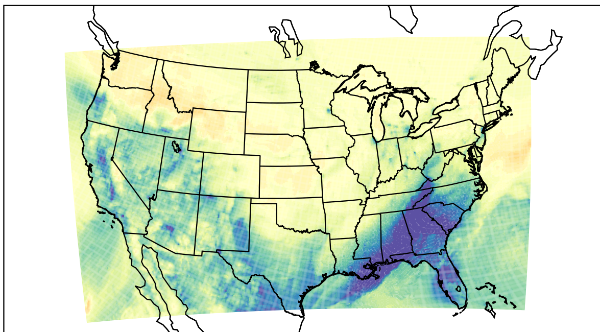
WRF (2021-02-12_14:00:00)
