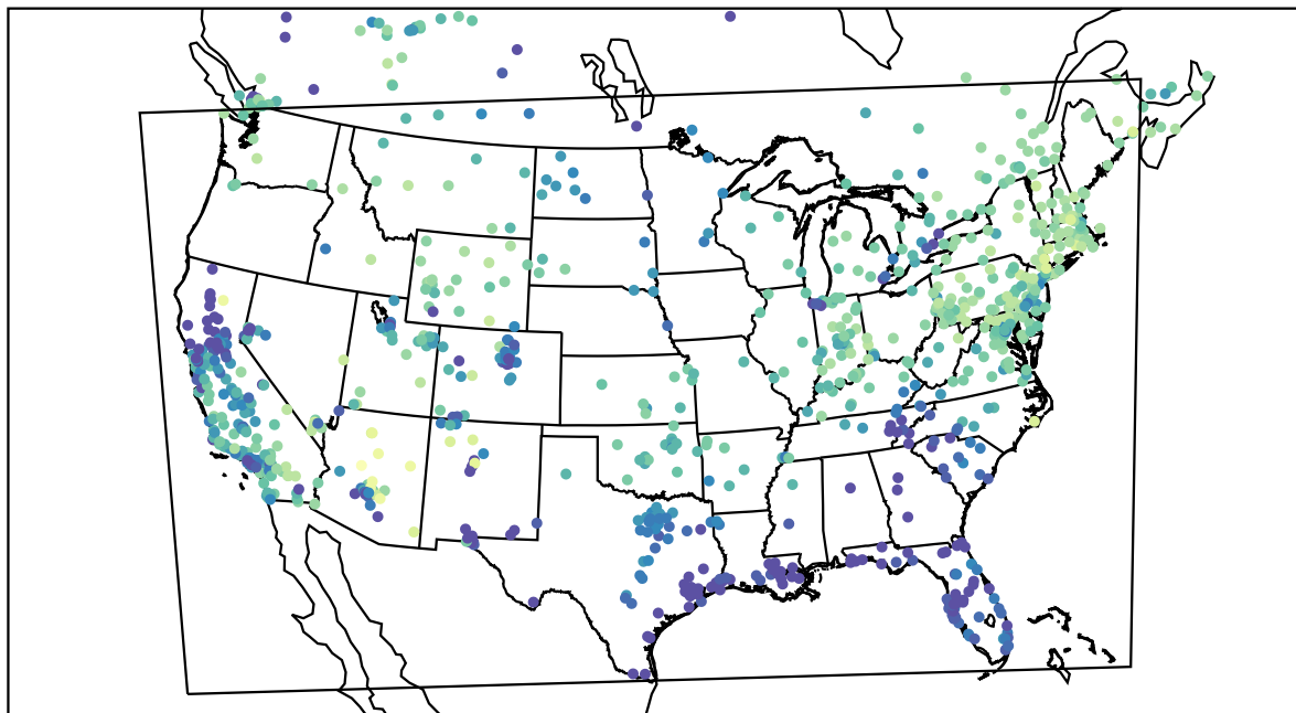
AirNOW (2021-02-12_16:00:00)
