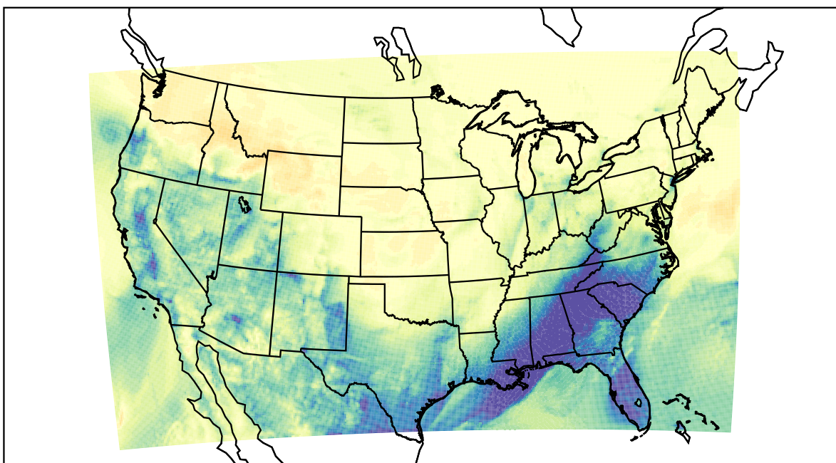
WRF (2021-02-12_12:00:00)
