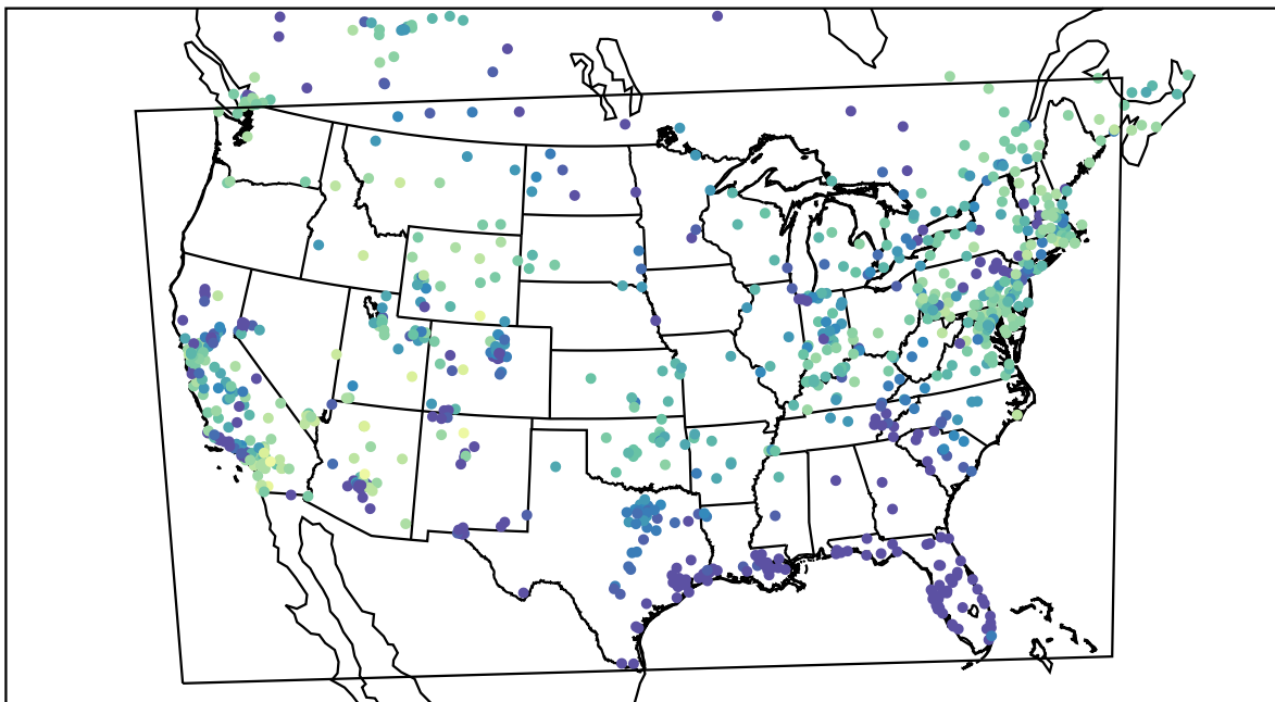
AirNOW (2021-02-12_12:00:00)
