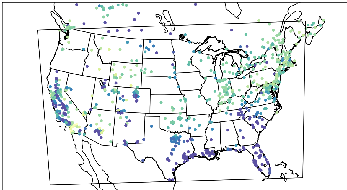
AirNOW (2021-02-12_06:00:00)
