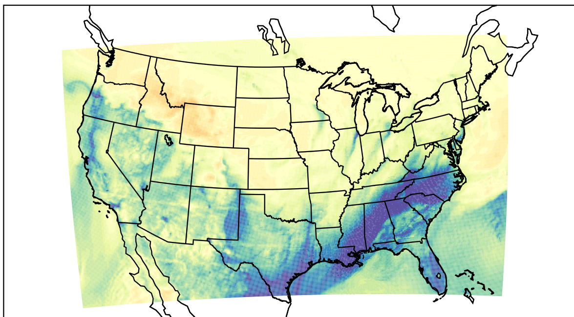
WRF (2021-02-12_05:00:00)
