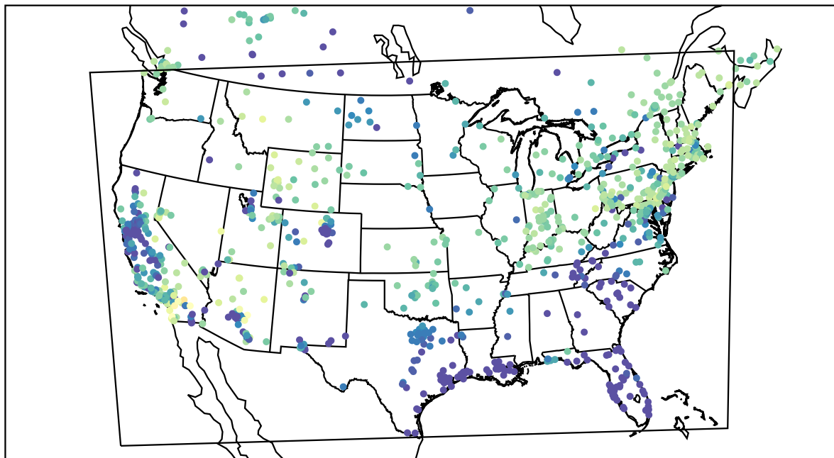
AirNOW (2021-02-12_03:00:00)
