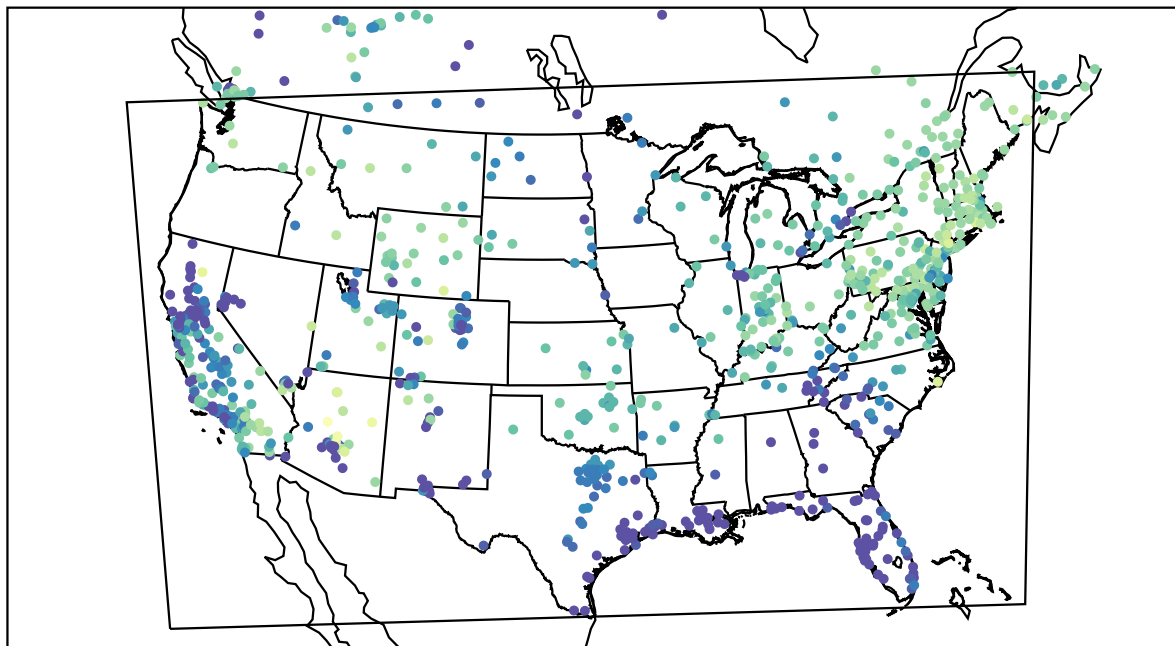
AirNOW (2021-02-12_15:00:00)
