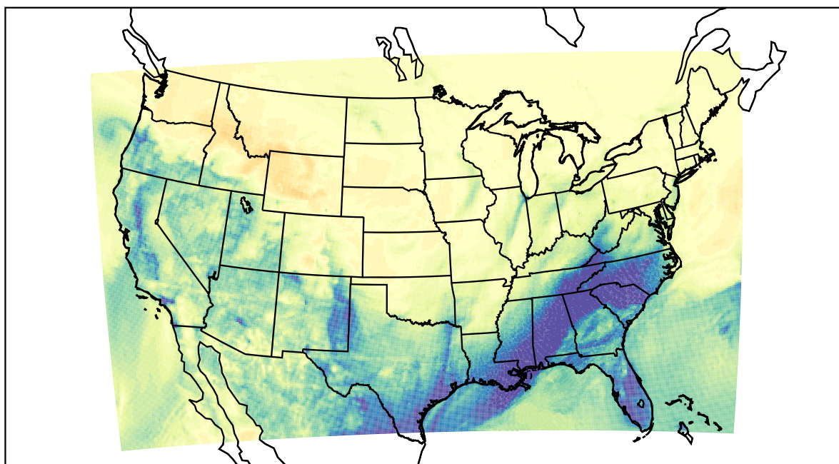
WRF (2021-02-12_08:00:00)
