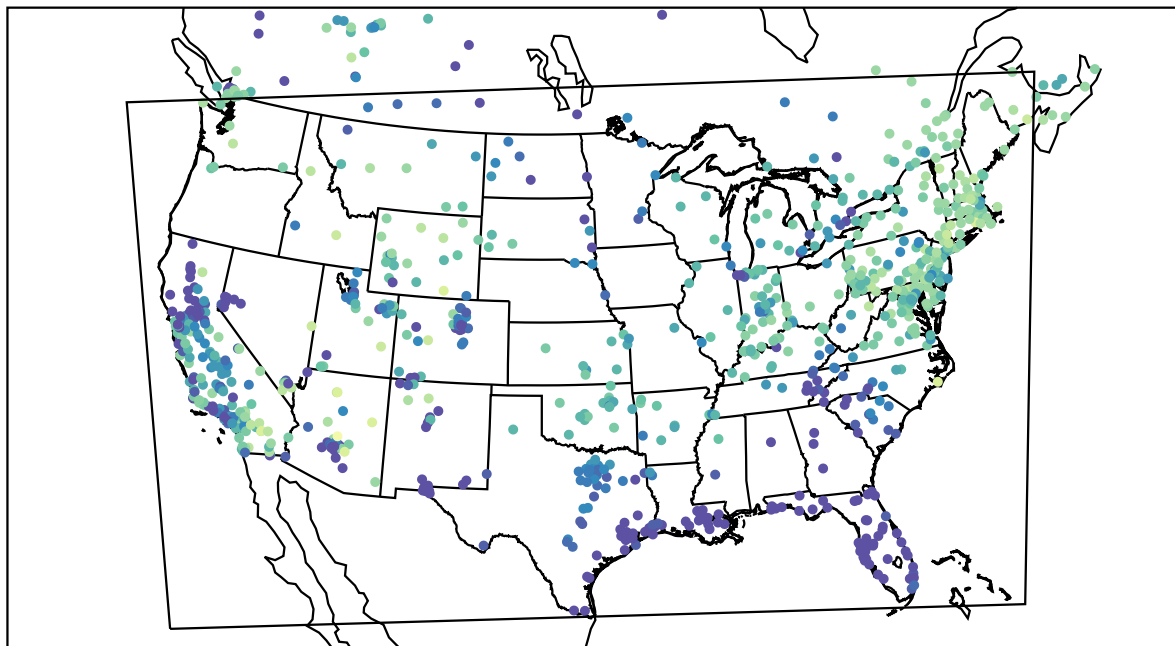
AirNOW (2021-02-12_14:00:00)
