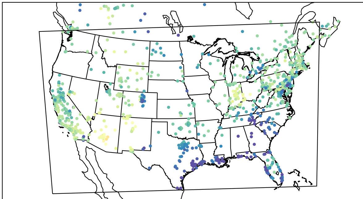
AirNOW (2021-02-12_21:00:00)
