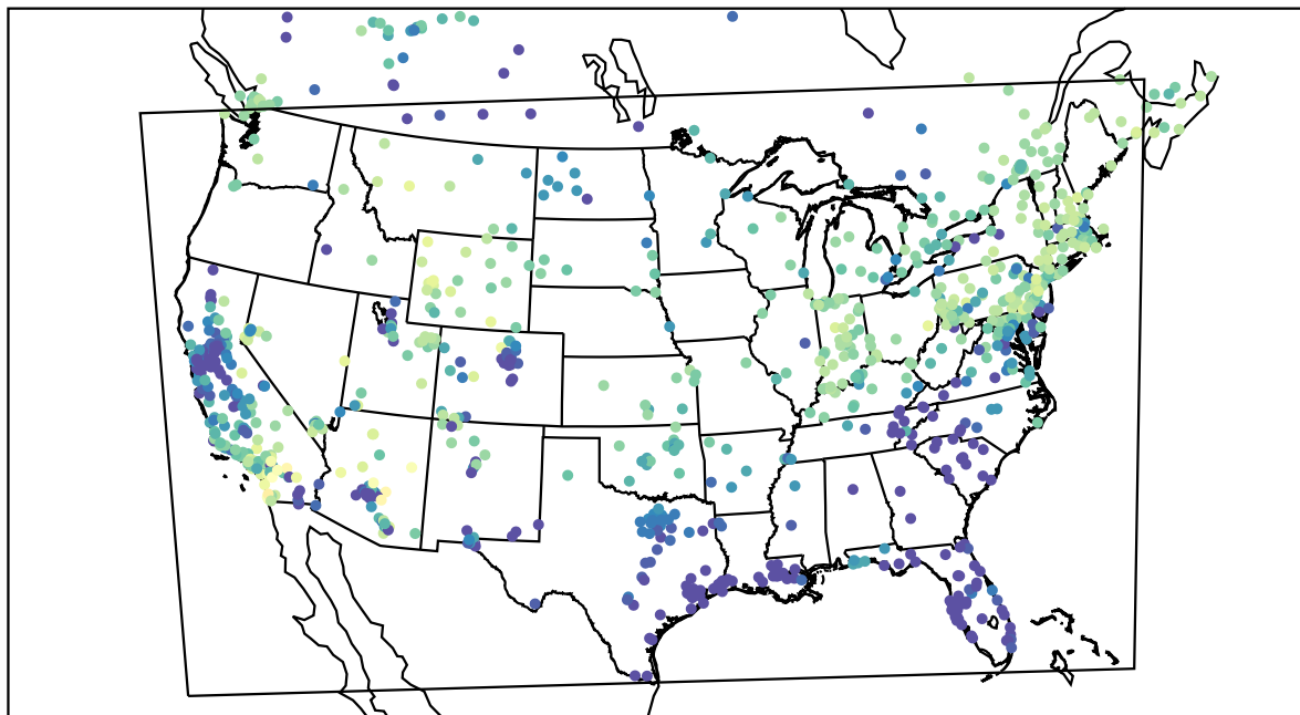
AirNOW (2021-02-12_02:00:00)
