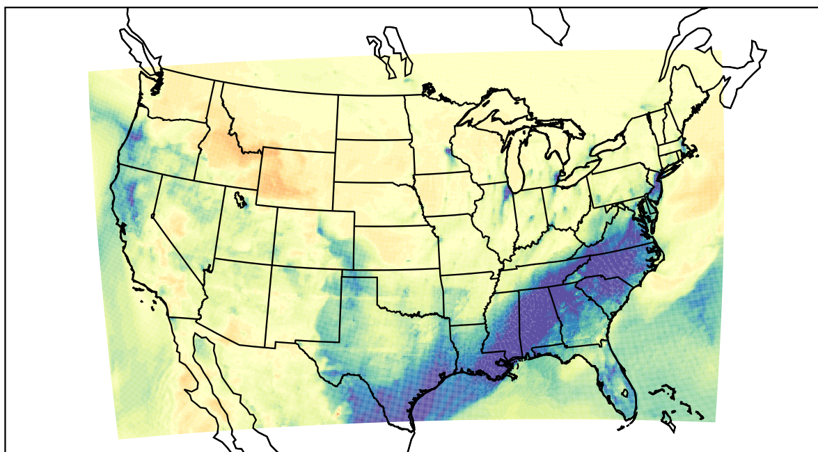
WRF (2021-02-12_00:00:00)
