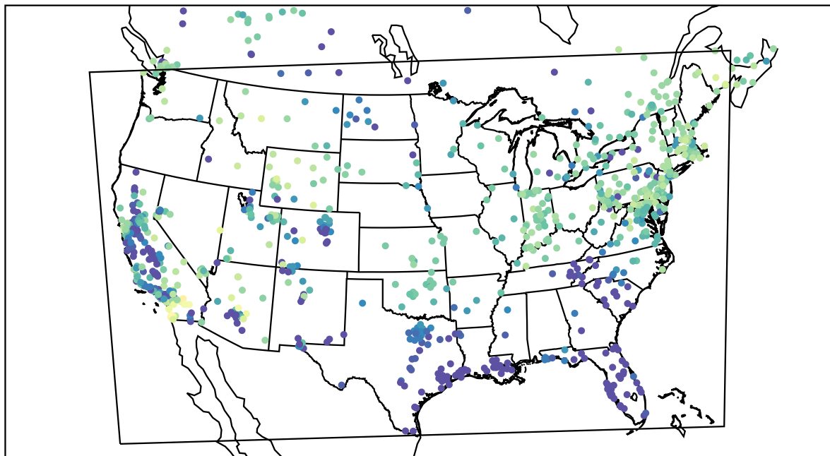
AirNOW (2021-02-12_05:00:00)
