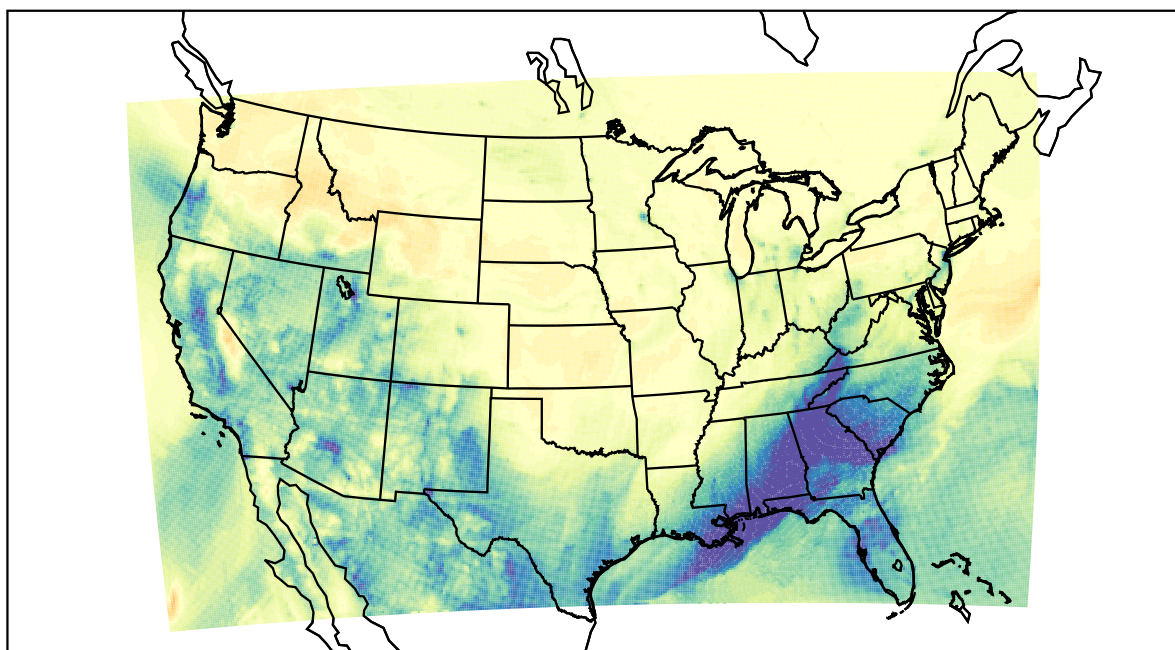
WRF (2021-02-12_15:00:00)
