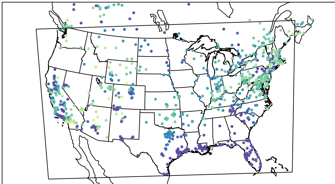
AirNOW (2021-02-12_11:00:00)
