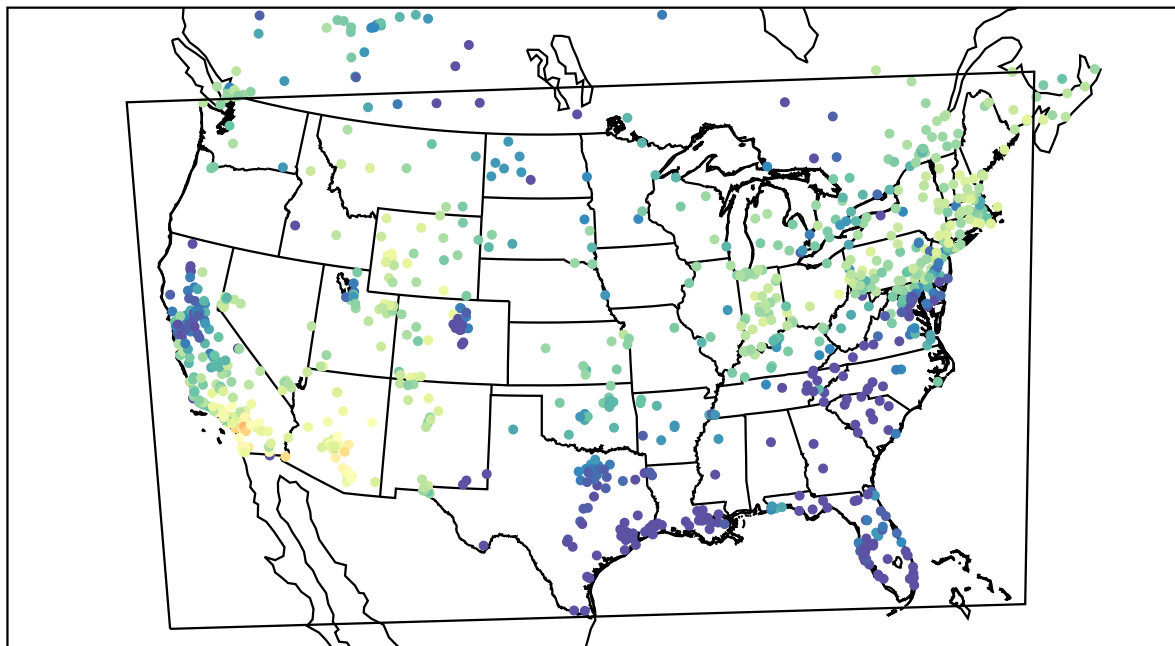
AirNOW (2021-02-12_00:00:00)
