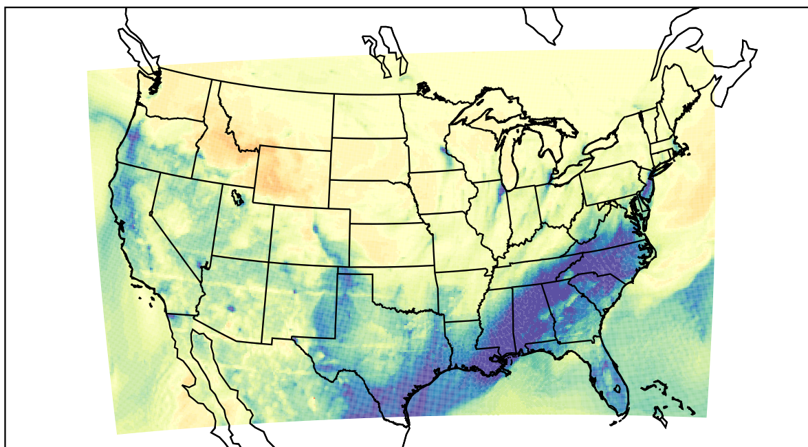
WRF (2021-02-12_02:00:00)
