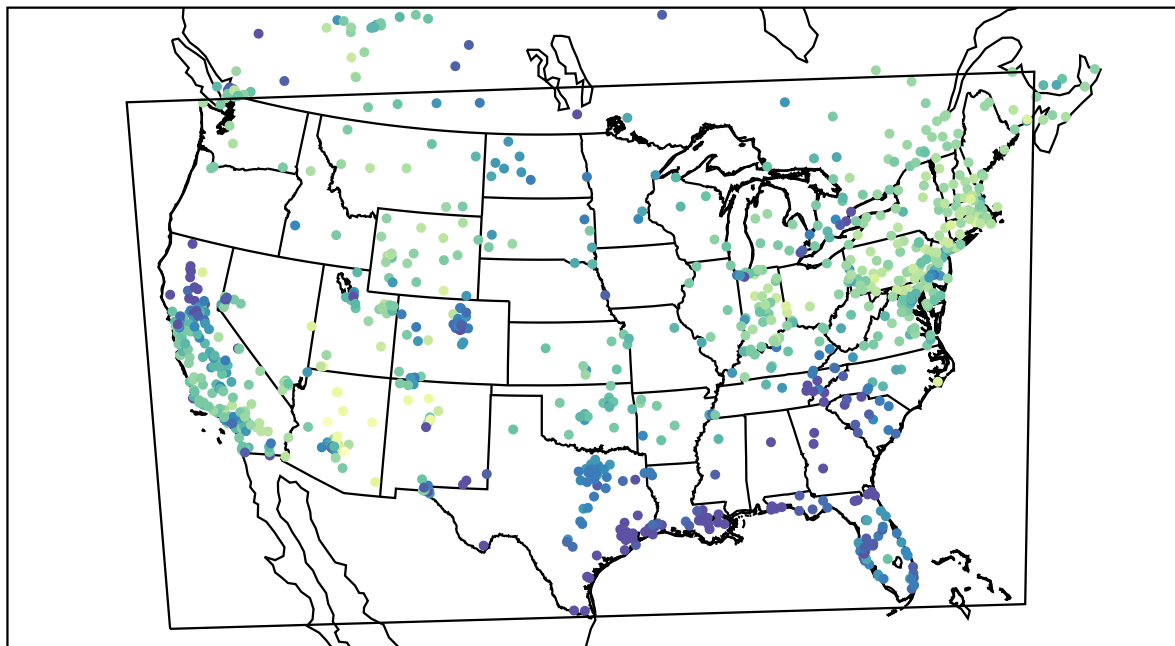
AirNOW (2021-02-12_17:00:00)
