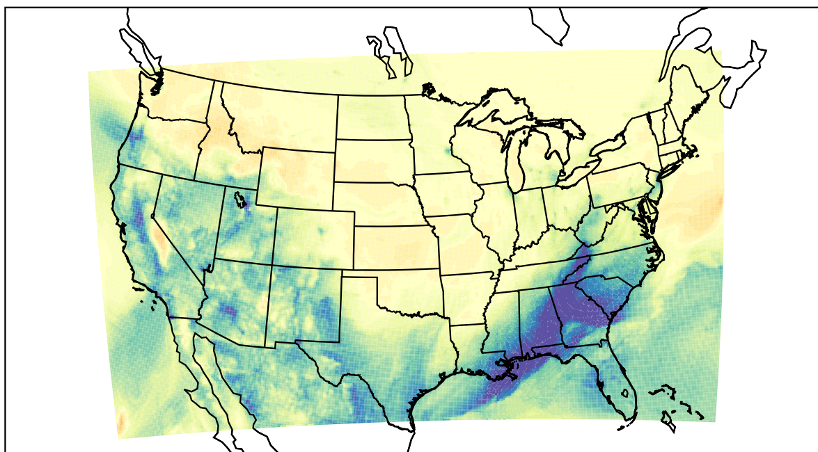
WRF (2021-02-12_16:00:00)
