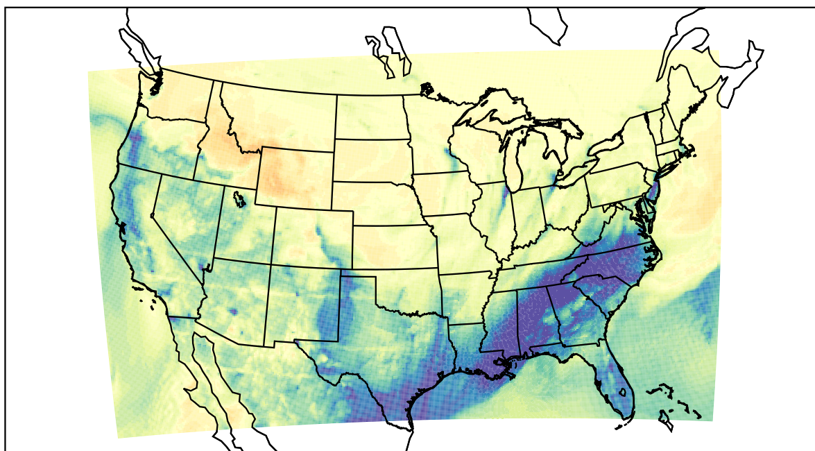
WRF (2021-02-12_03:00:00)
