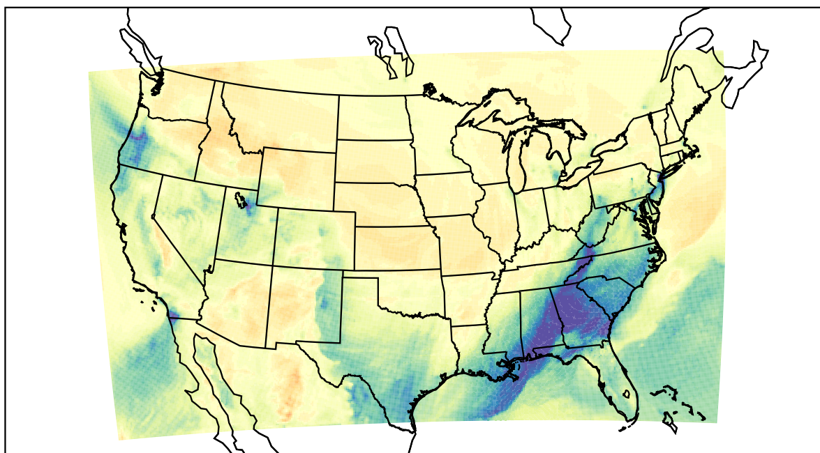
WRF (2021-02-12_21:00:00)
