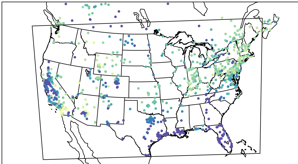
AirNOW (2021-02-12_04:00:00)
