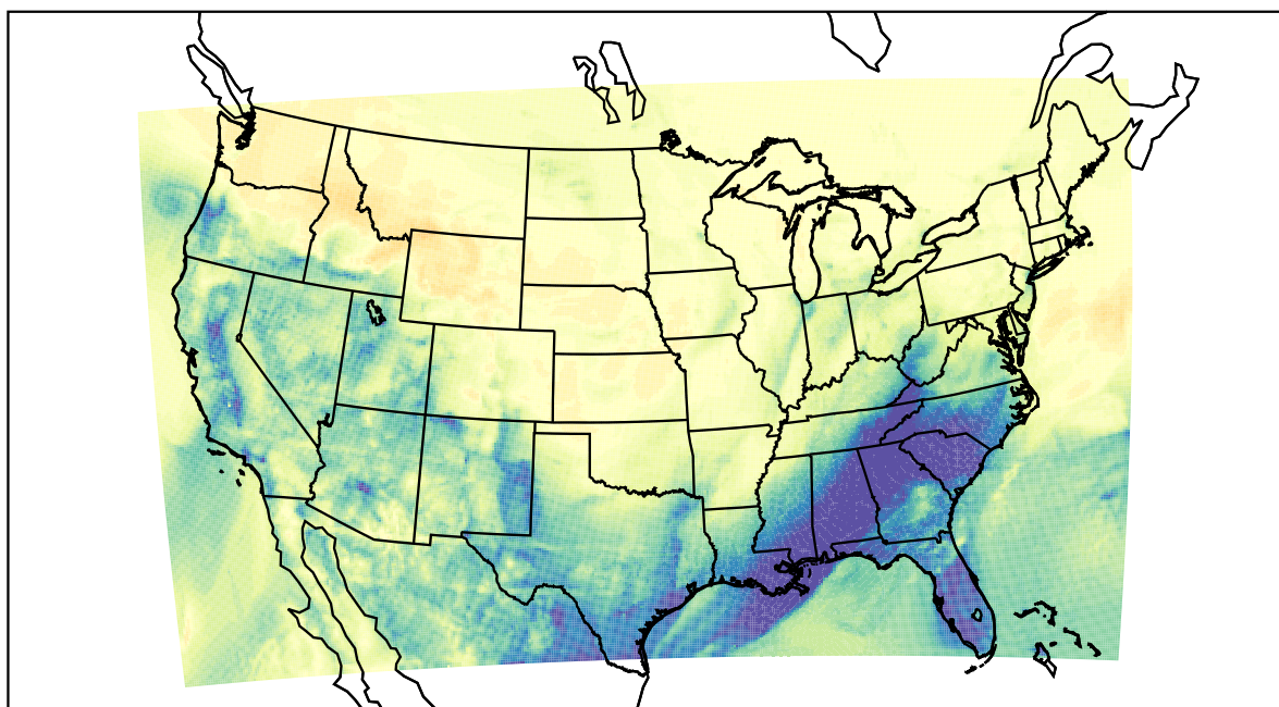
WRF (2021-02-12_11:00:00)
