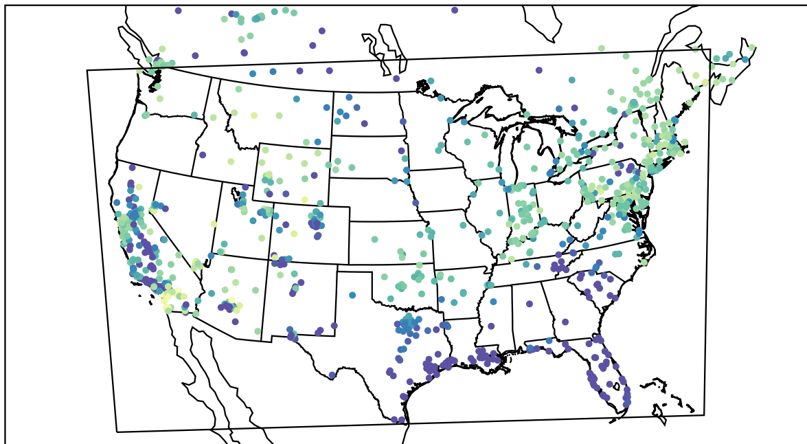
AirNOW (2021-02-12_07:00:00)
