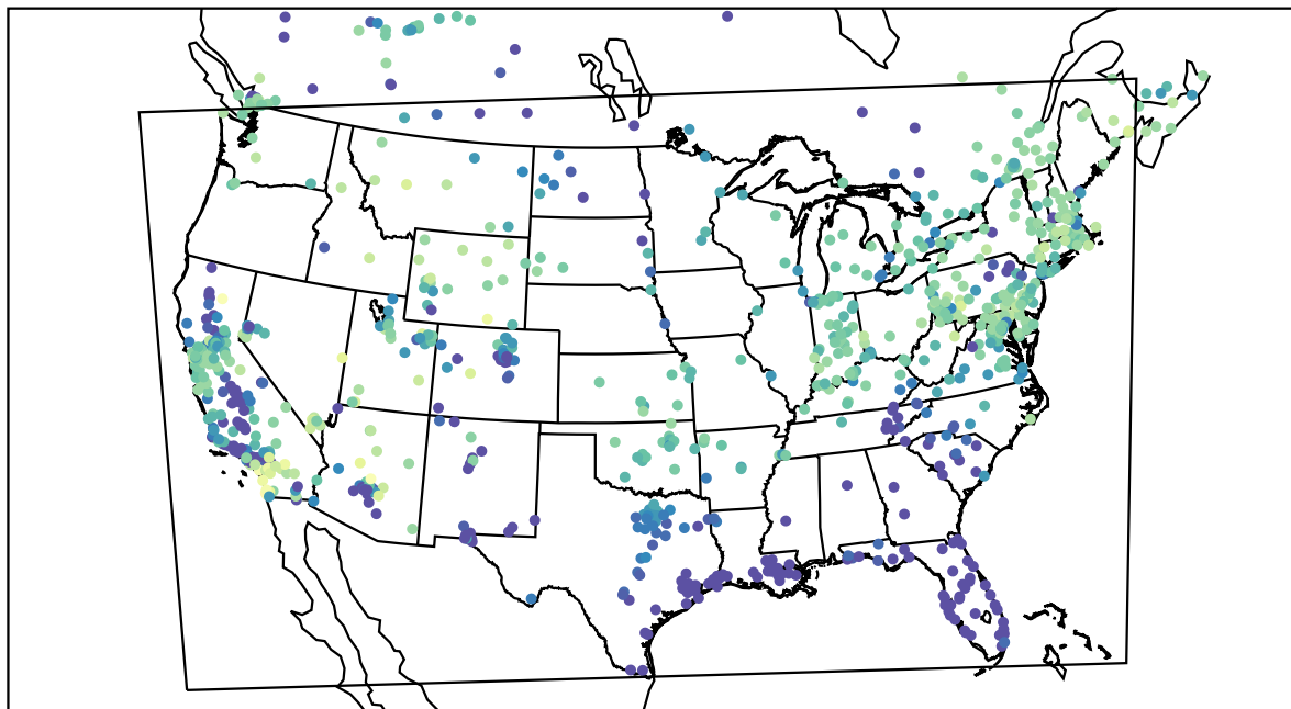
AirNOW (2021-02-12_08:00:00)
