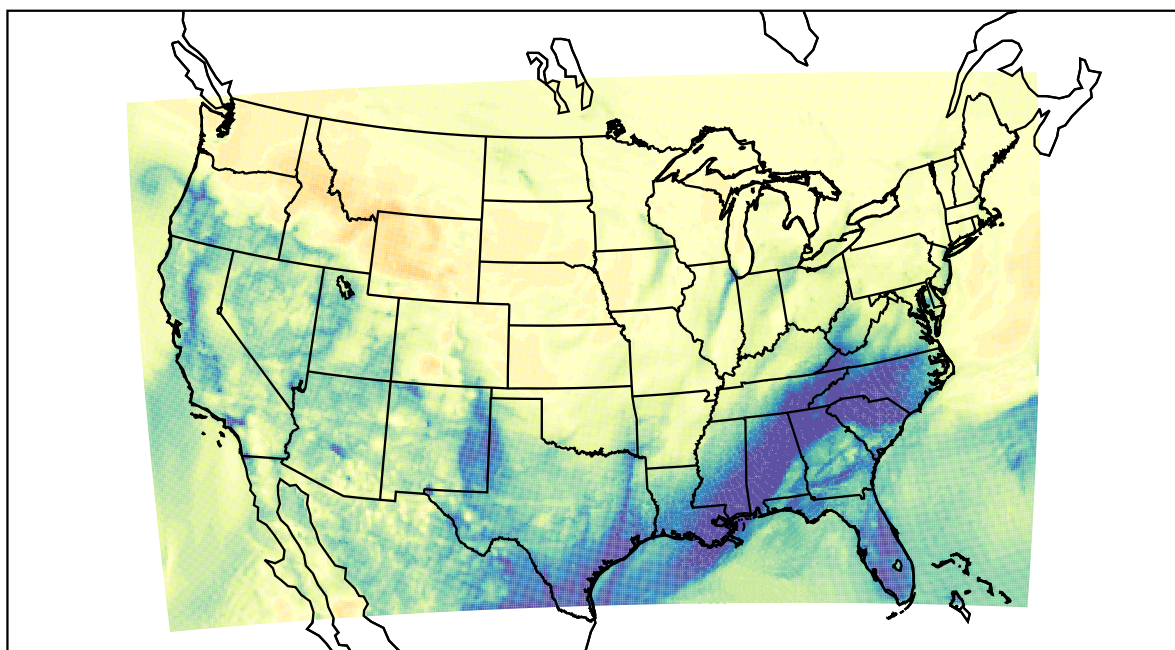
WRF (2021-02-12_07:00:00)
