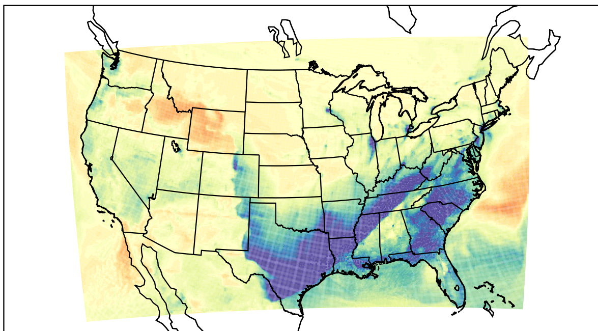
WRF (2021-02-11_00:00:00)
