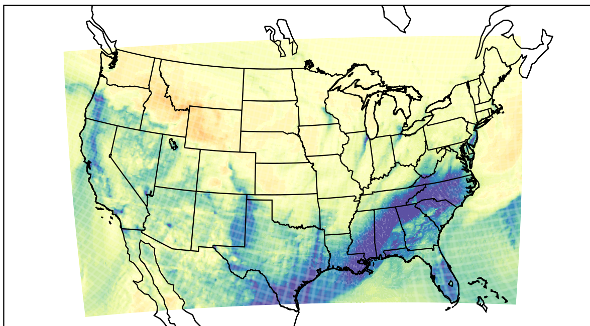
WRF (2021-02-12_04:00:00)
