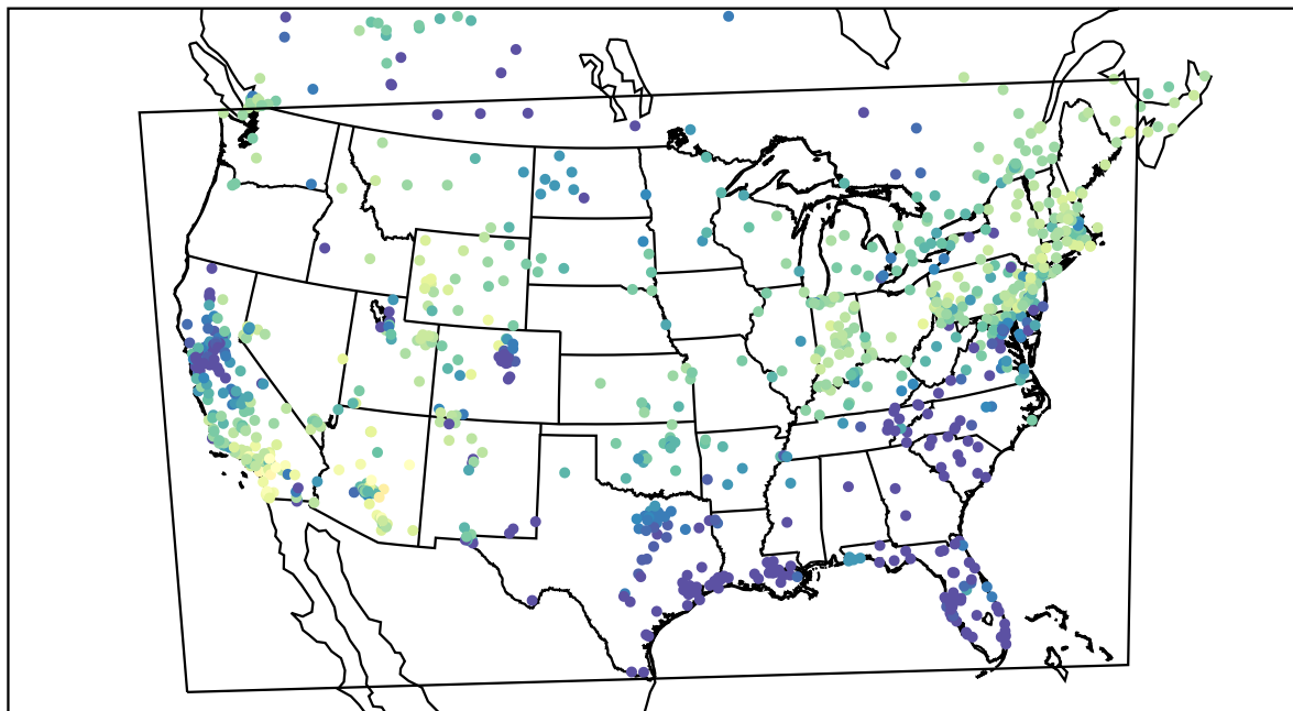
AirNOW (2021-02-12_01:00:00)
