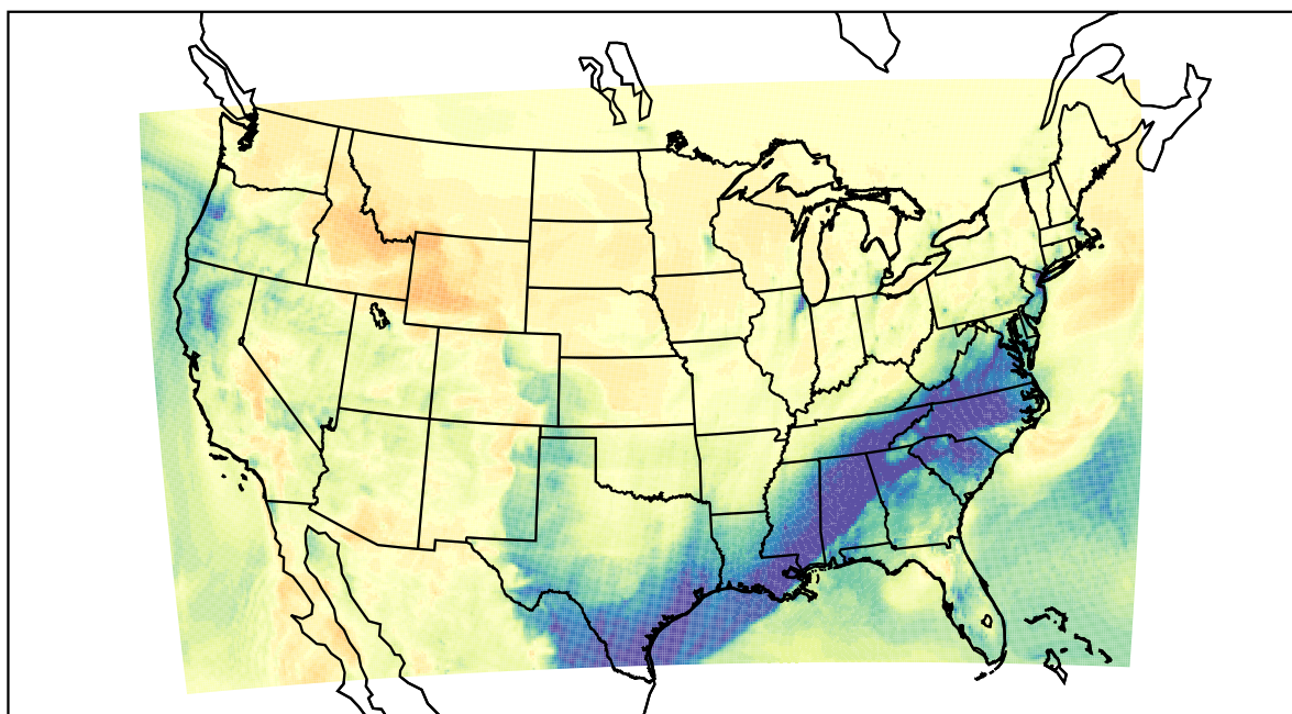
WRF (2021-02-11_22:00:00)
