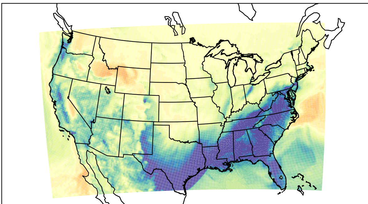
WRF (2021-02-11_10:00:00)
