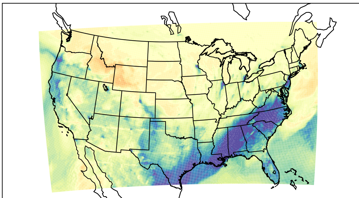
WRF (2021-02-12_01:00:00)
