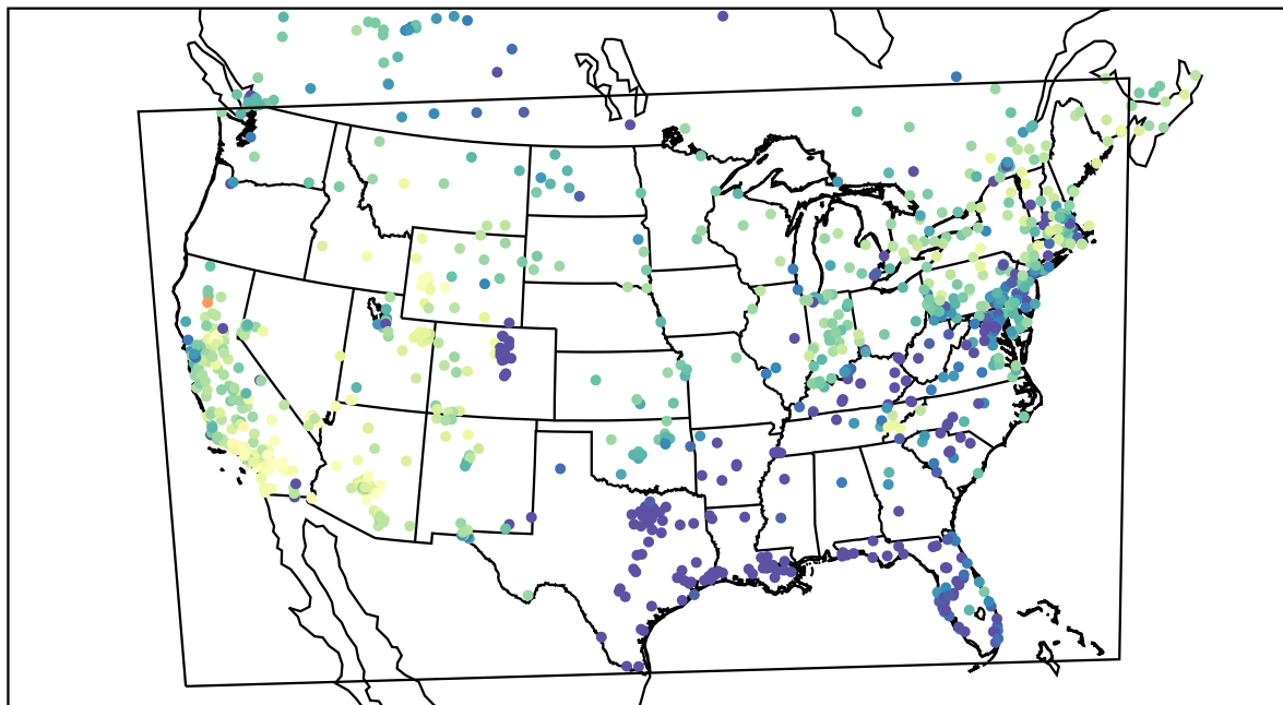
AirNOW (2021-02-11_00:00:00)
