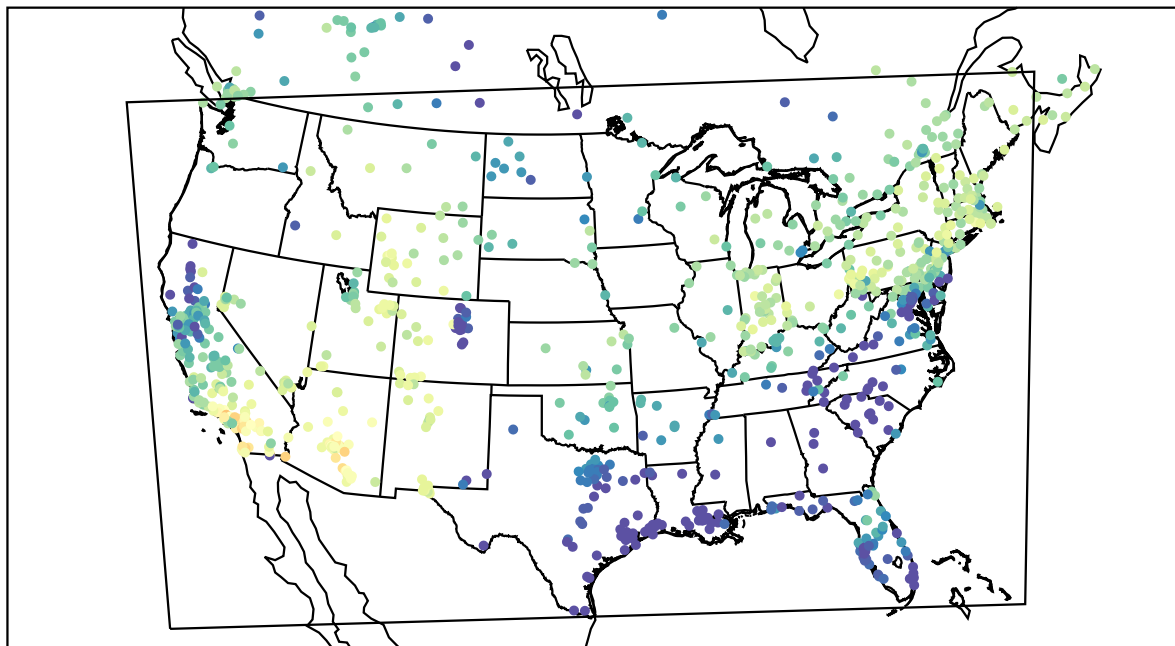
AirNOW (2021-02-11_22:00:00)
