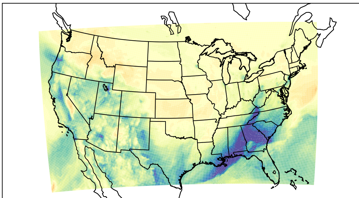
WRF (2021-02-12_17:00:00)
