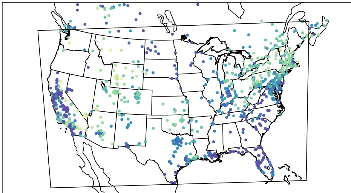
AirNOW (2021-02-14_15:00:00)
