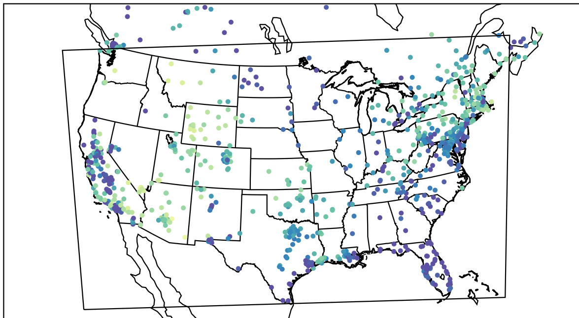
AirNOW (2021-02-14_10:00:00)
