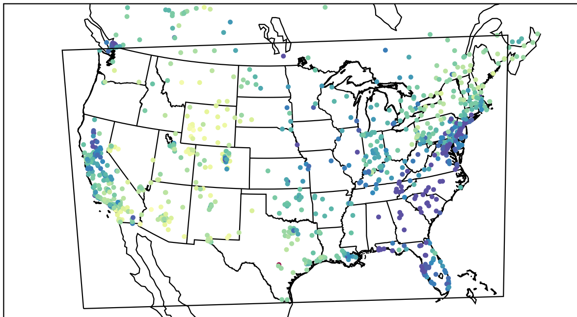
AirNOW (2021-02-15_22:00:00)
