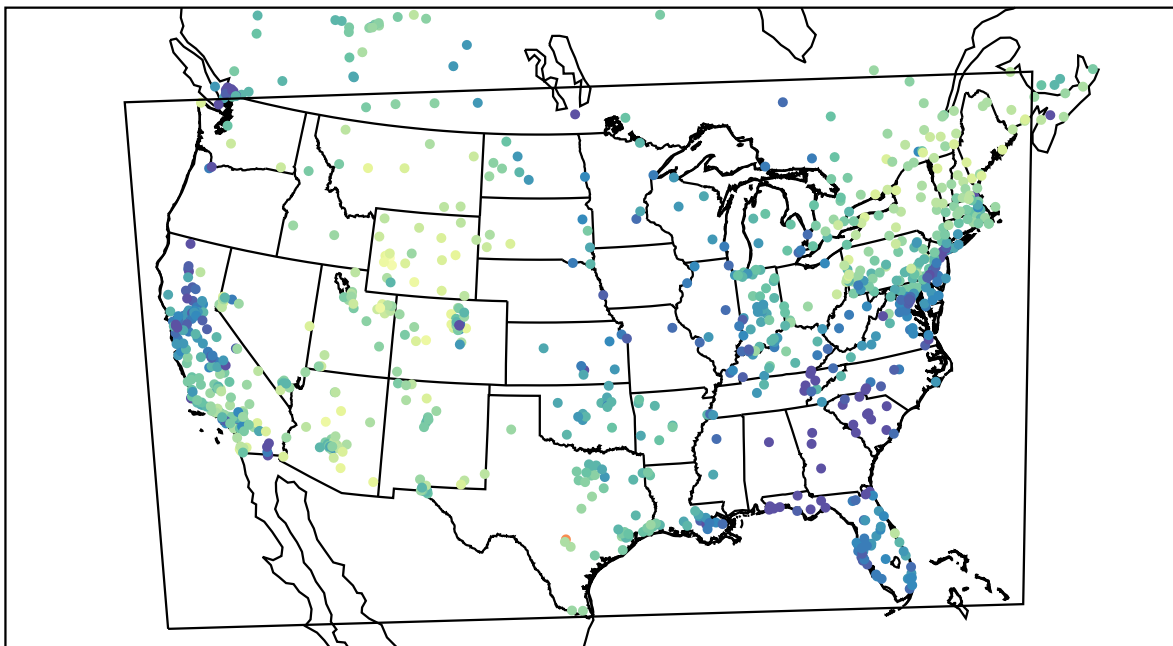
AirNOW (2021-02-15_19:00:00)
