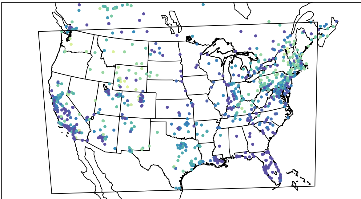
AirNOW (2021-02-15_12:00:00)
