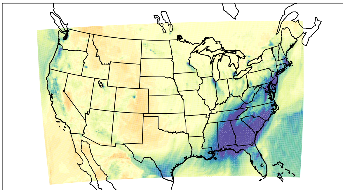
WRF (2021-02-15_01:00:00)
