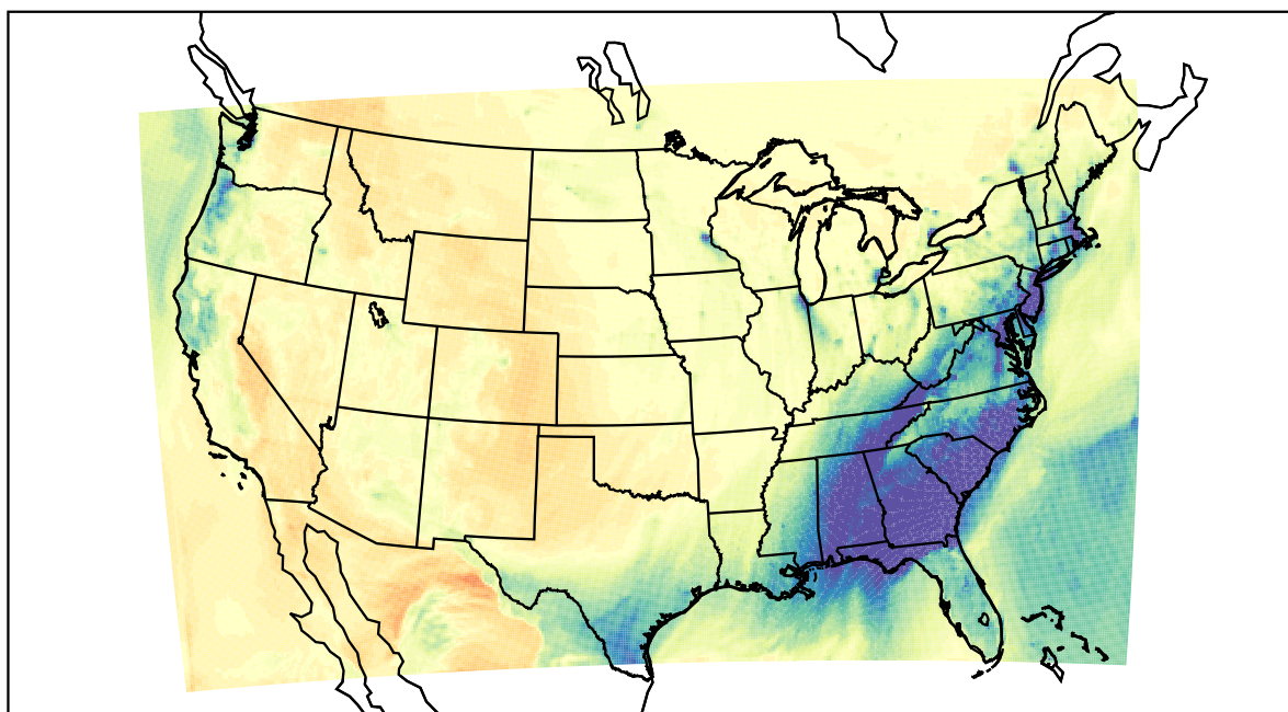
WRF (2021-02-14_23:00:00)
