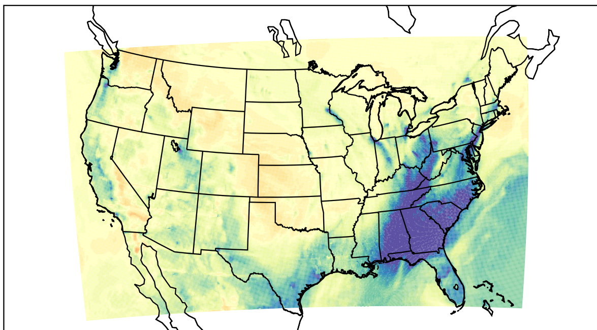
WRF (2021-02-14_02:00:00)
