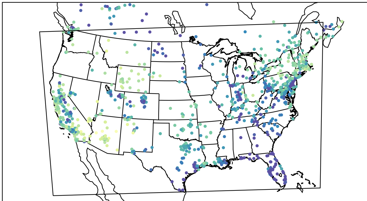
AirNOW (2021-02-14_03:00:00)
