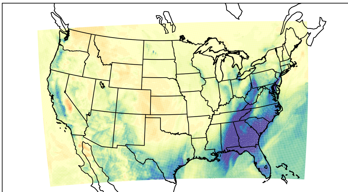
WRF (2021-02-14_07:00:00)
