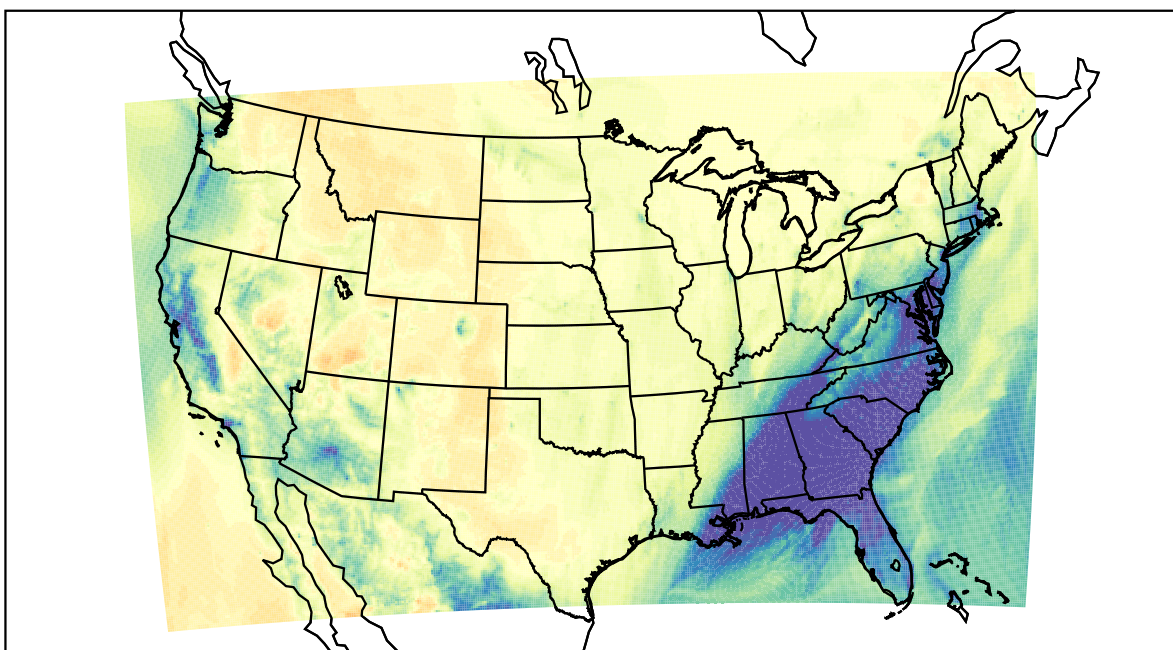
WRF (2021-02-15_12:00:00)
