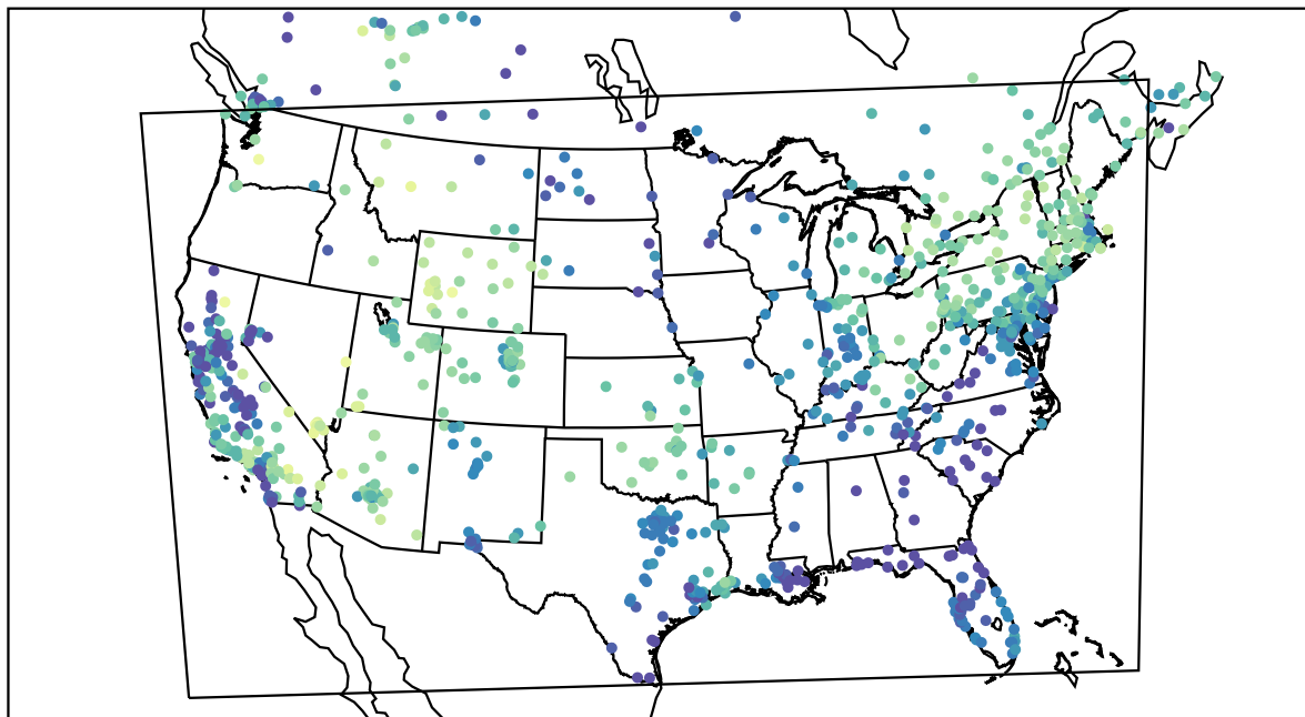
AirNOW (2021-02-14_16:00:00)
