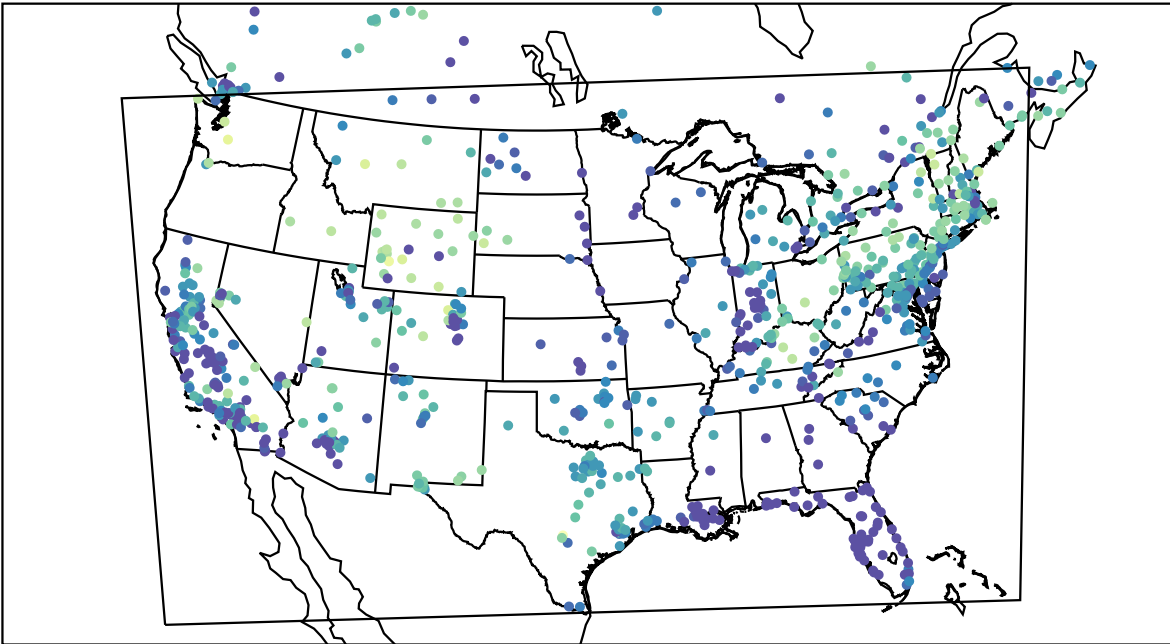
AirNOW (2021-02-15_10:00:00)
