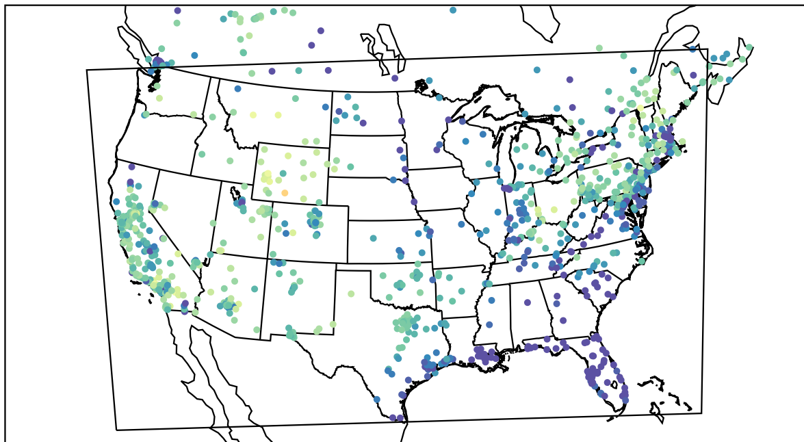
AirNOW (2021-02-15_02:00:00)
