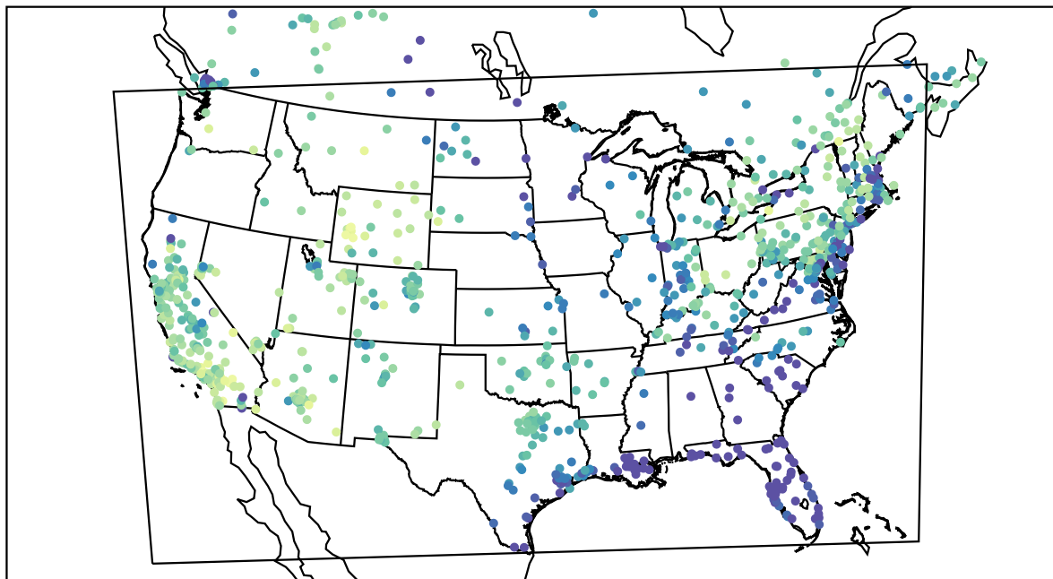
AirNOW (2021-02-15_01:00:00)
