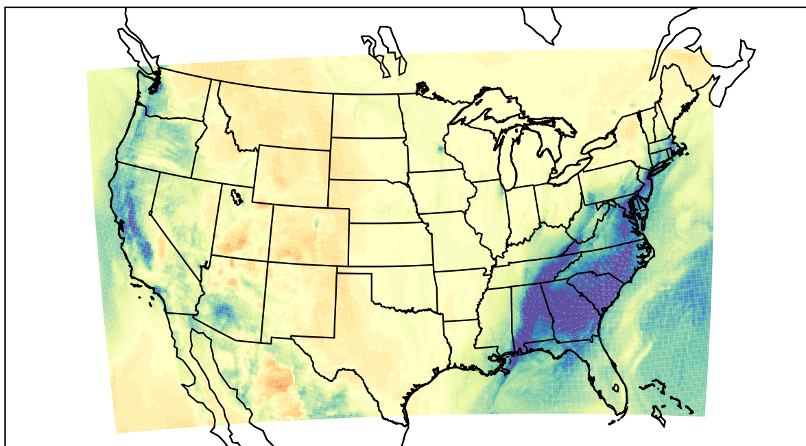
WRF (2021-02-15_17:00:00)
