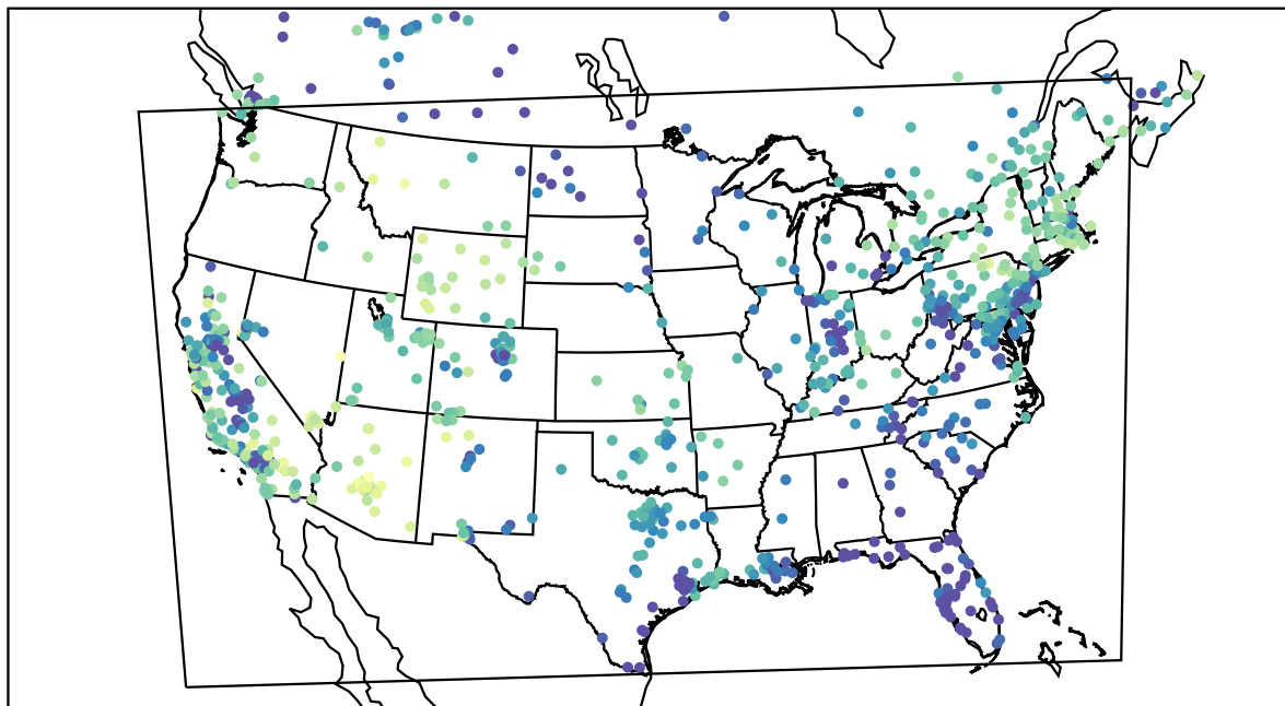
AirNOW (2021-02-14_05:00:00)
