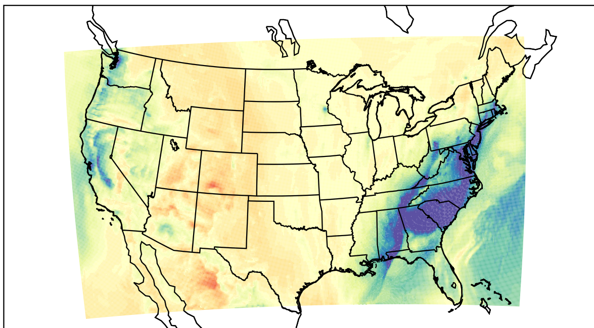
WRF (2021-02-15_20:00:00)
