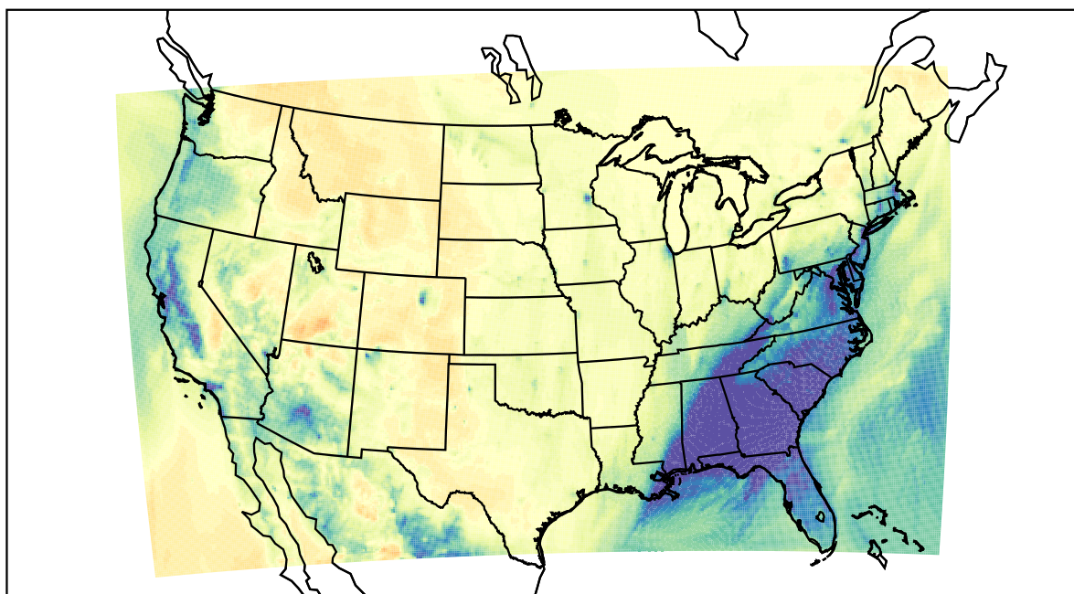
WRF (2021-02-15_14:00:00)
