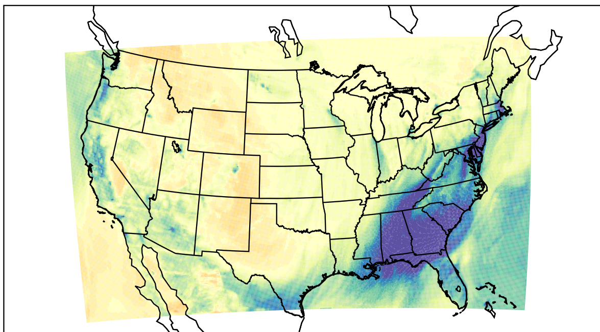
WRF (2021-02-15_04:00:00)
