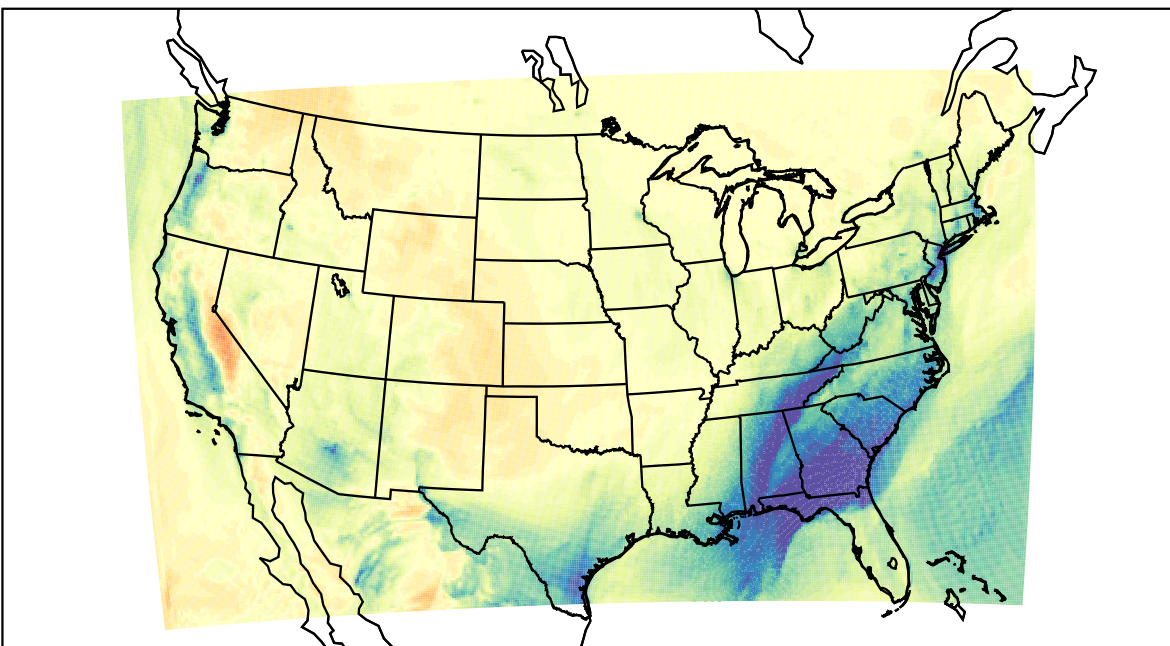
WRF (2021-02-14_17:00:00)
