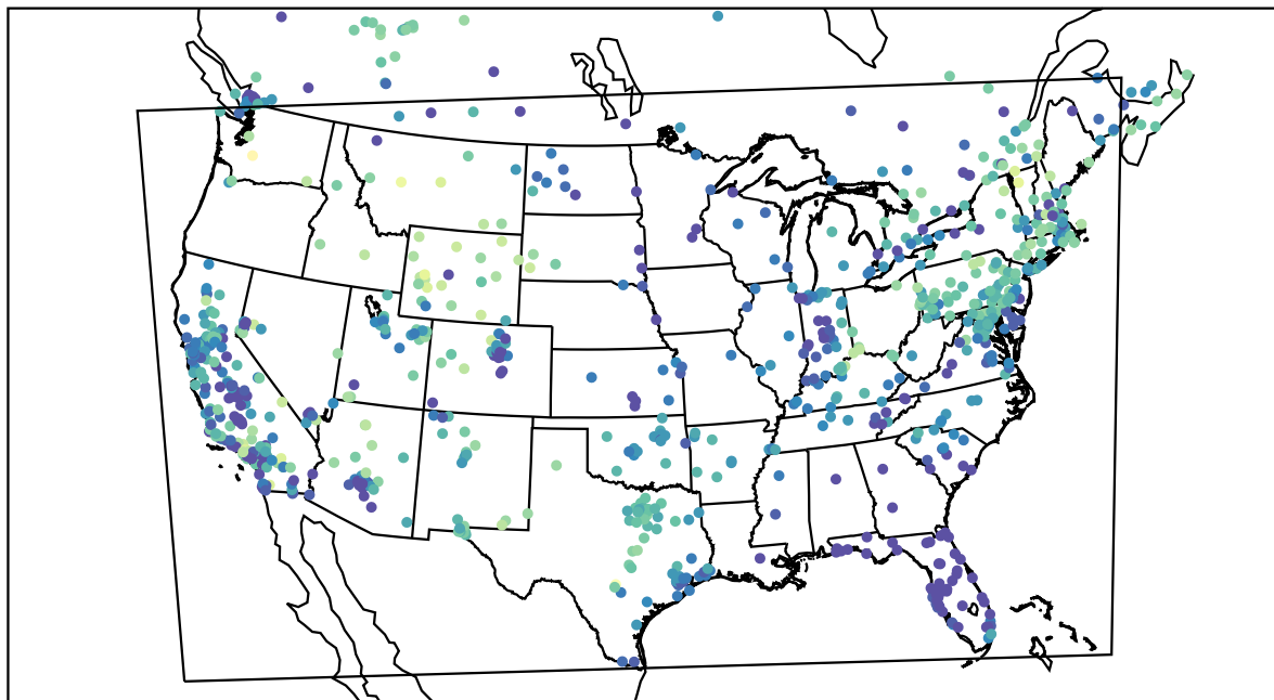
AirNOW (2021-02-15_07:00:00)
