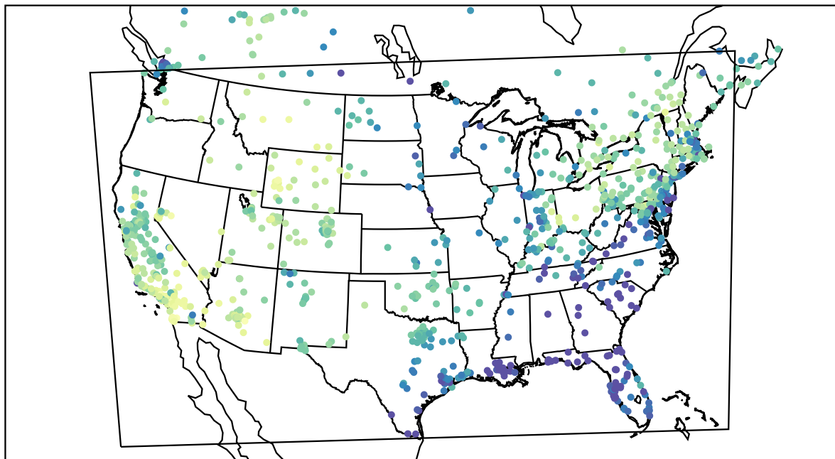
AirNOW (2021-02-14_23:00:00)
