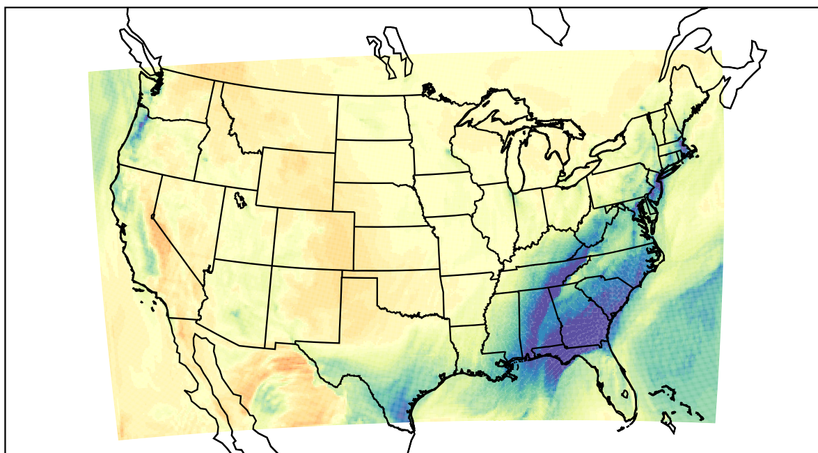
WRF (2021-02-14_20:00:00)
