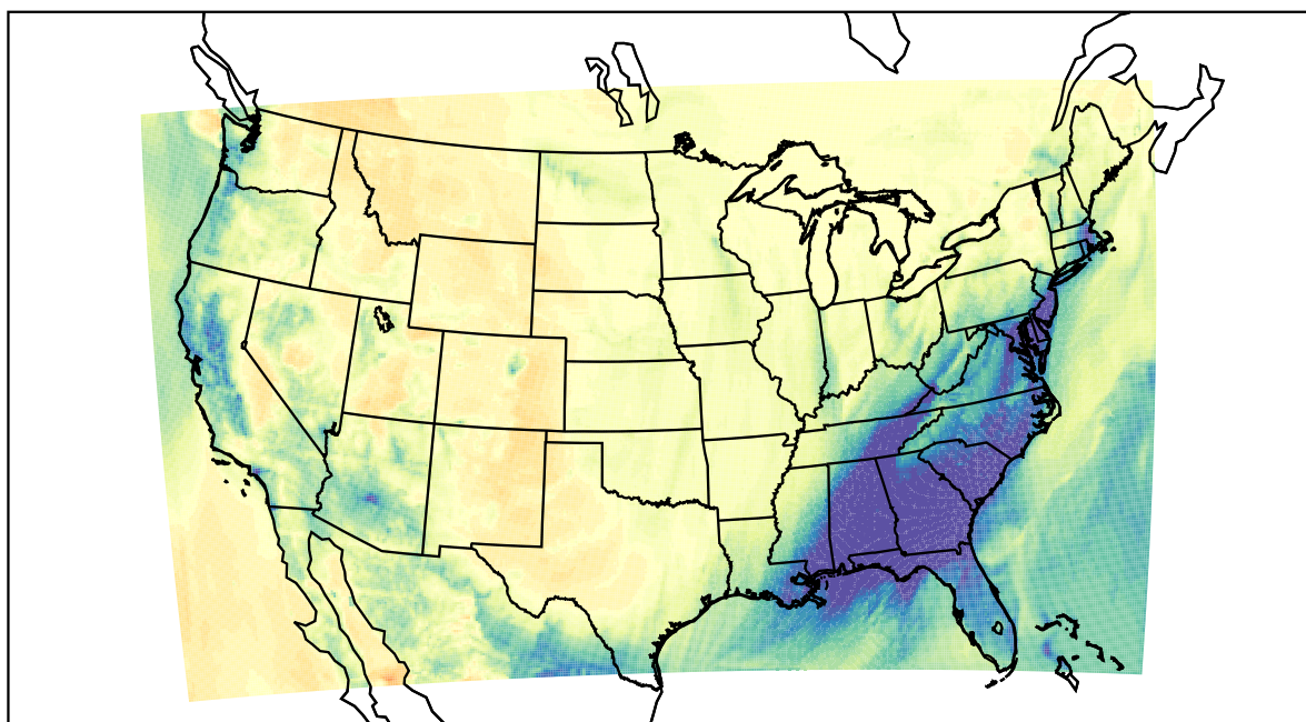
WRF (2021-02-15_08:00:00)
