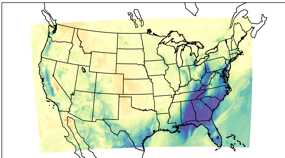
WRF (2021-02-14_06:00:00)
