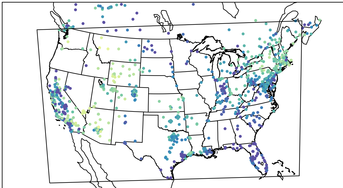
AirNOW (2021-02-14_08:00:00)
