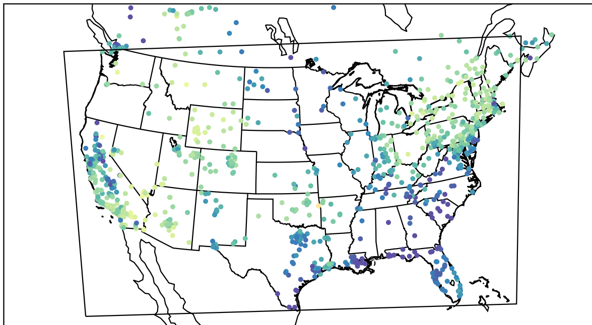
AirNOW (2021-02-14_18:00:00)
