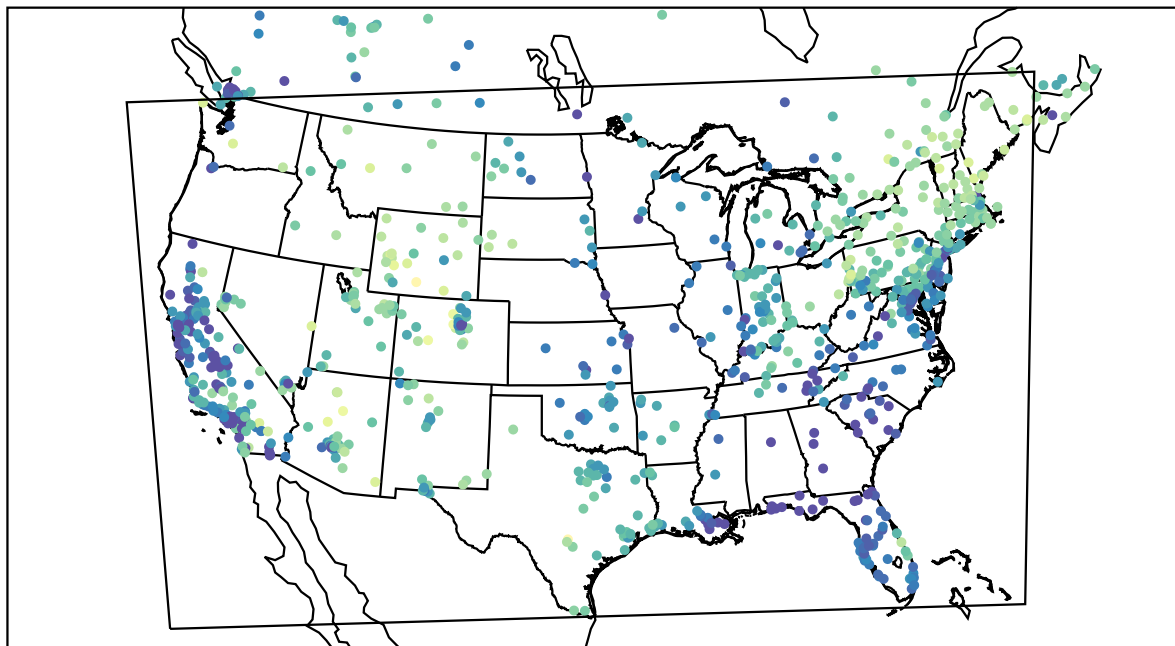
AirNOW (2021-02-15_17:00:00)
