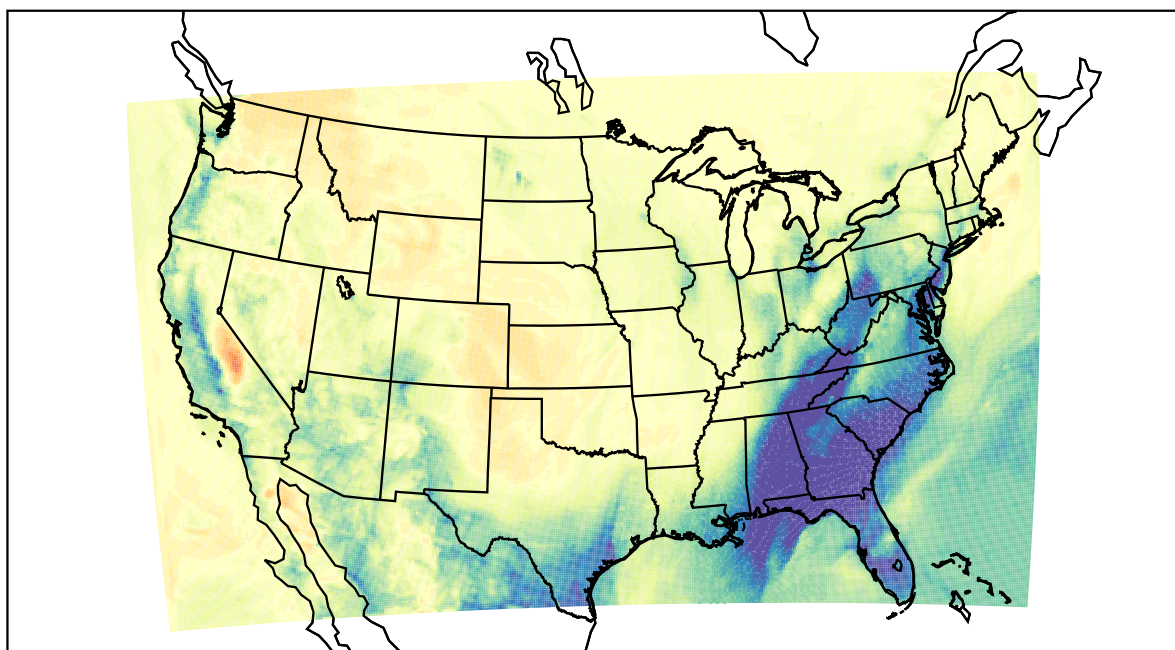
WRF (2021-02-14_09:00:00)
