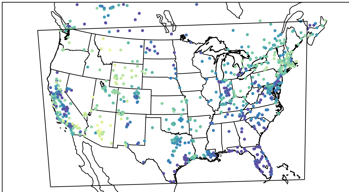
AirNOW (2021-02-14_06:00:00)
