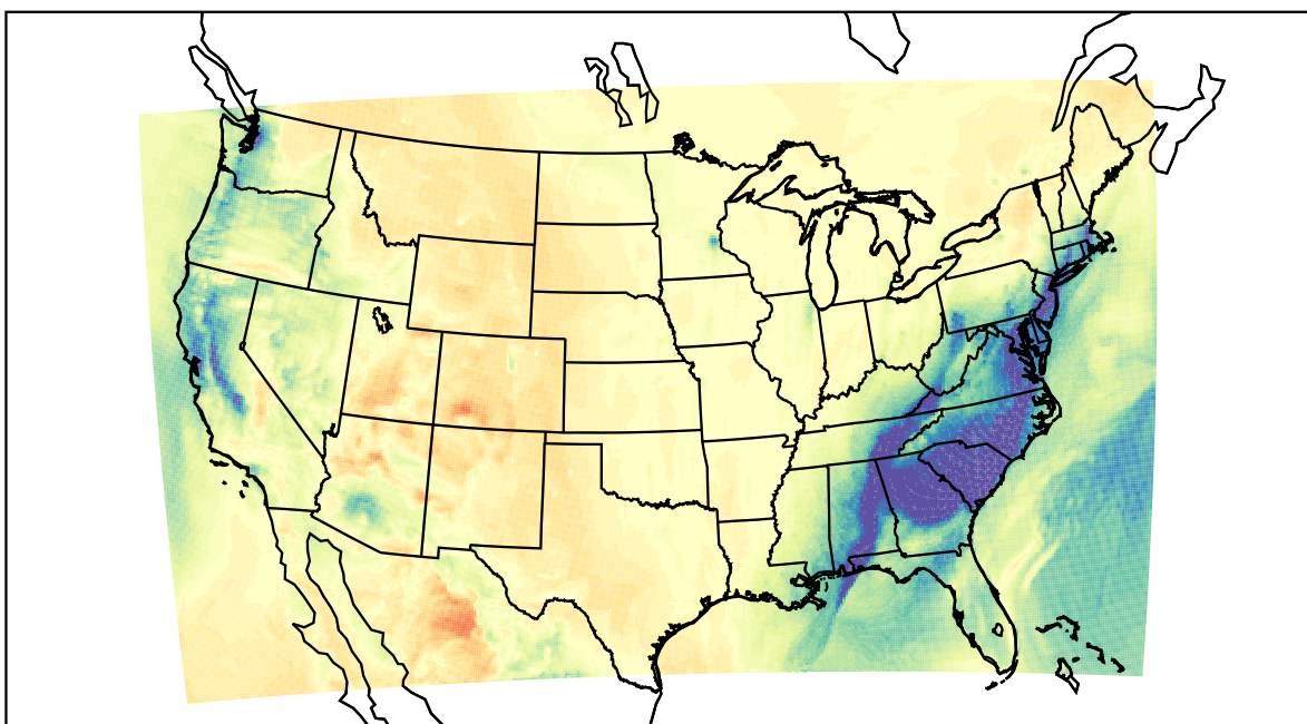
WRF (2021-02-15_19:00:00)
