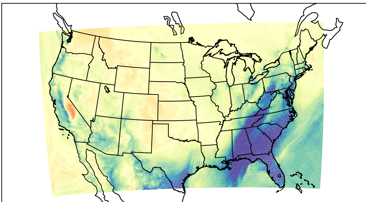
WRF (2021-02-14_12:00:00)
