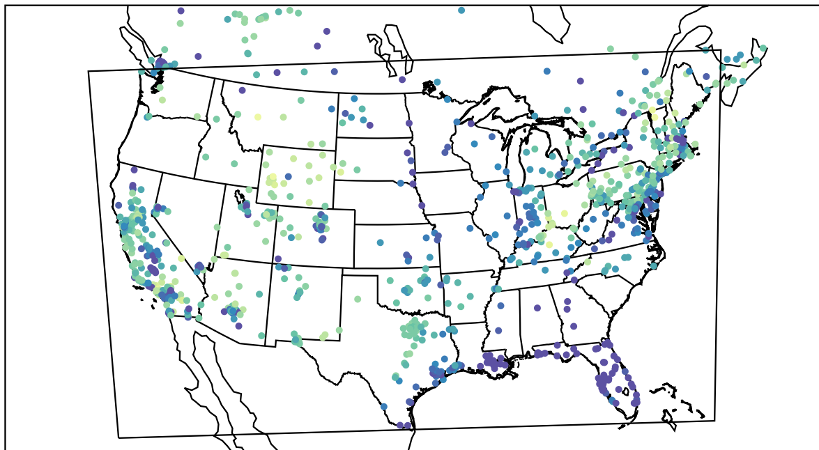
AirNOW (2021-02-15_04:00:00)
