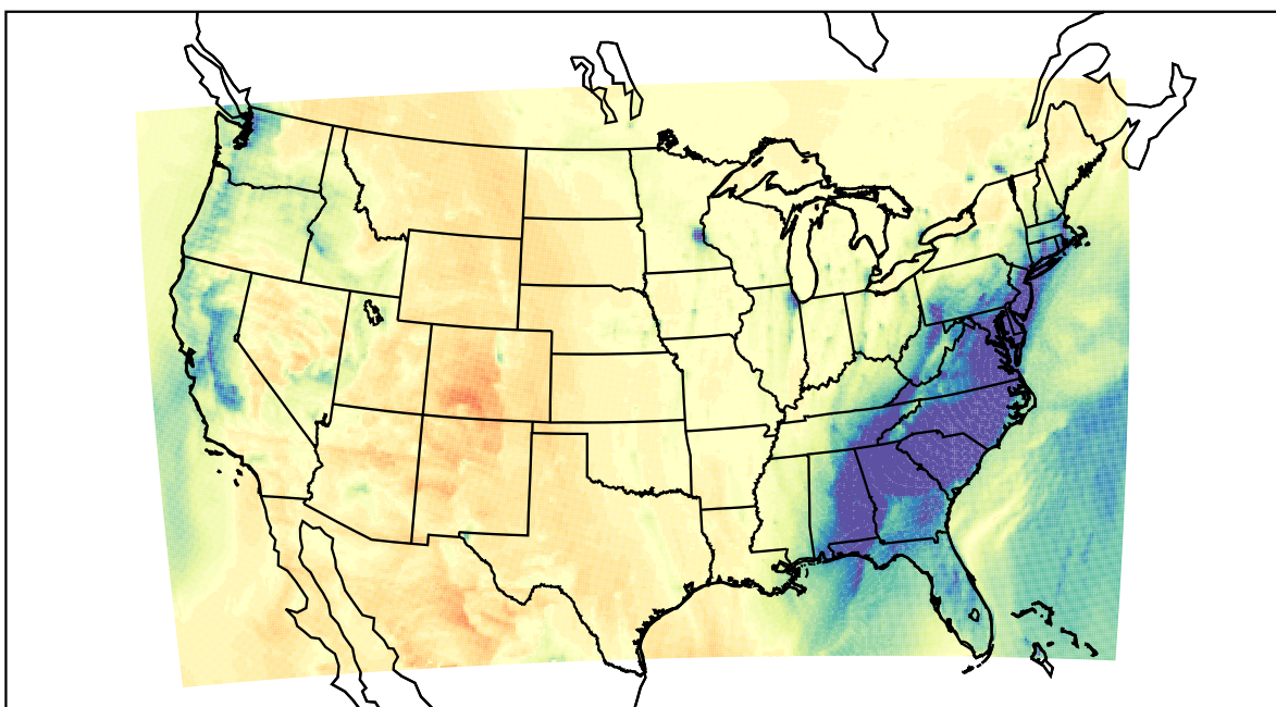
WRF (2021-02-15_23:00:00)
