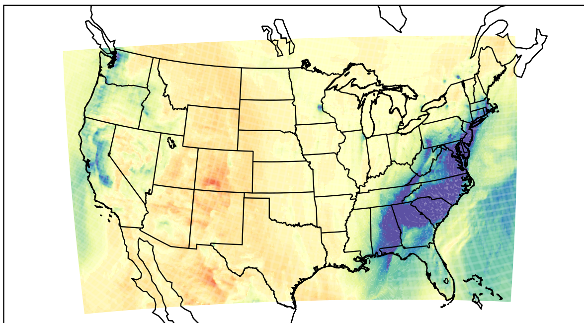
WRF (2021-02-15_22:00:00)
