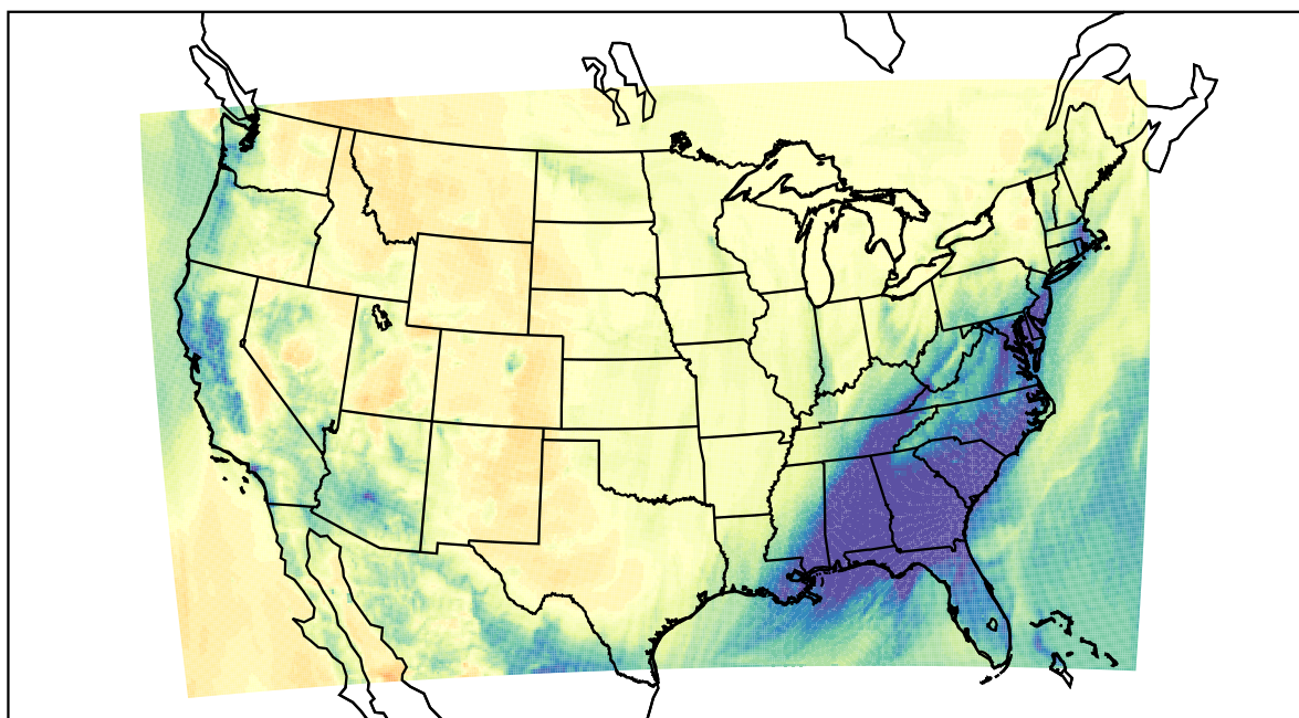
WRF (2021-02-15_09:00:00)
