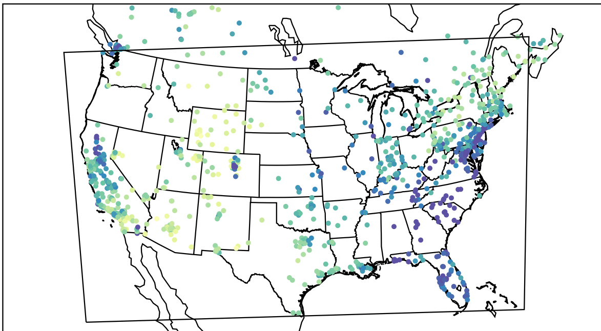
AirNOW (2021-02-15_23:00:00)
