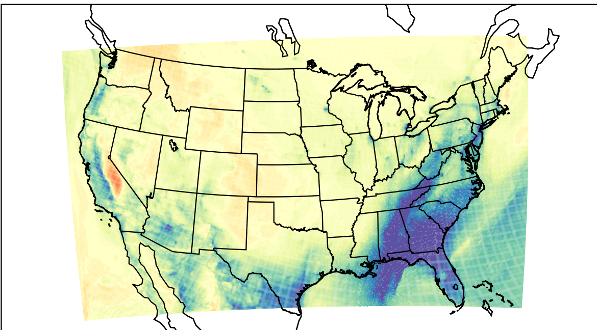
WRF (2021-02-14_14:00:00)
