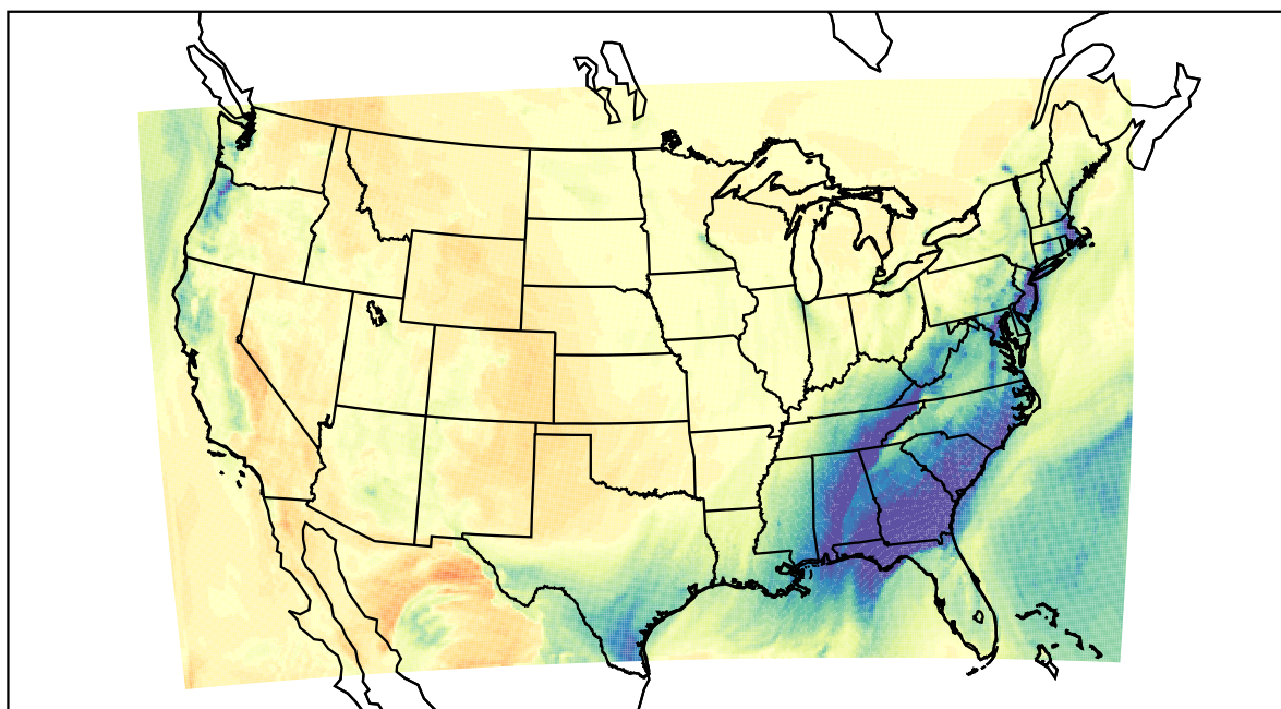
WRF (2021-02-14_21:00:00)
