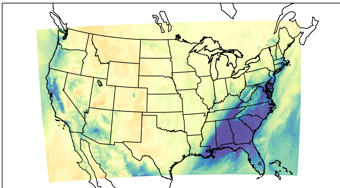
WRF (2021-02-15_11:00:00)
