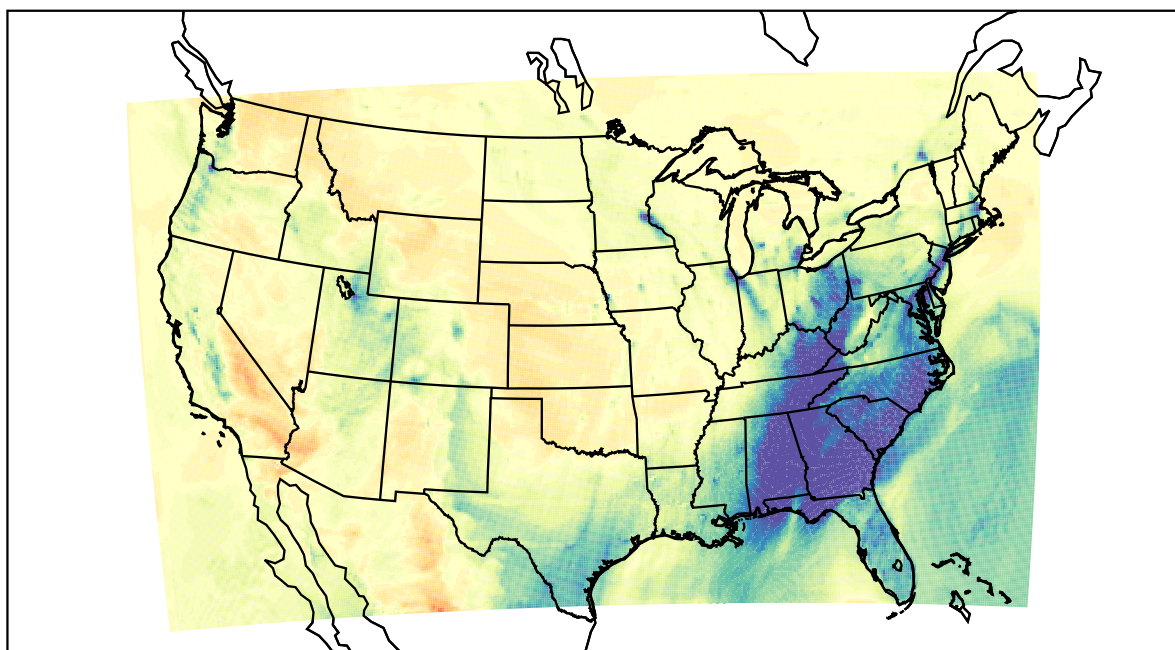
WRF (2021-02-14_00:00:00)
