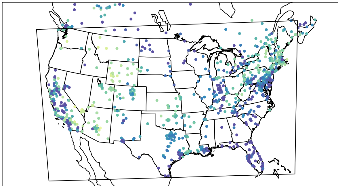
AirNOW (2021-02-14_11:00:00)
