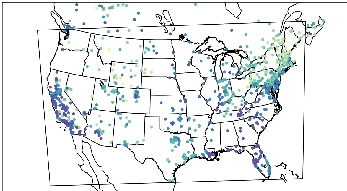
AirNOW (2021-02-15_16:00:00)
