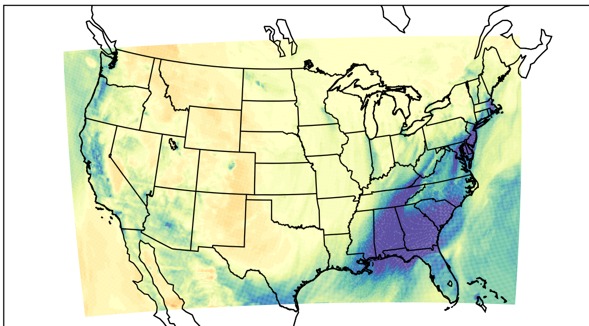
WRF (2021-02-15_05:00:00)
