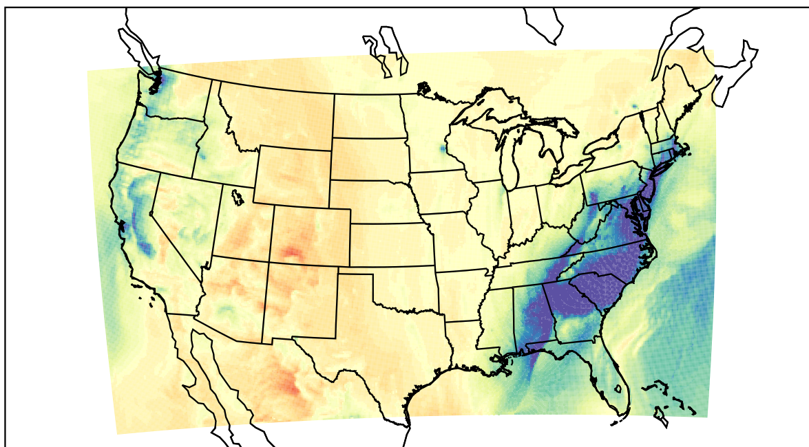
WRF (2021-02-15_21:00:00)
