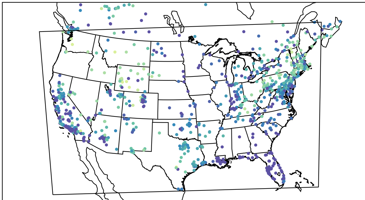
AirNOW (2021-02-15_11:00:00)
