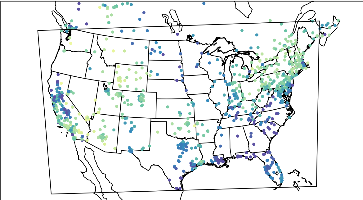
AirNOW (2021-02-14_17:00:00)
