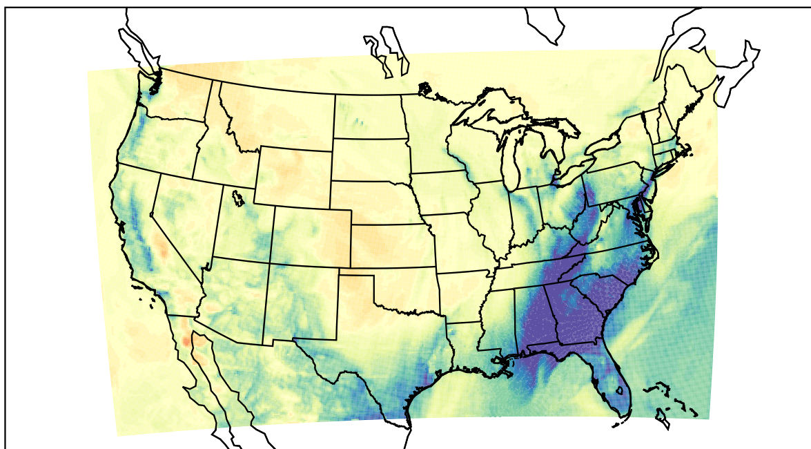
WRF (2021-02-14_05:00:00)
