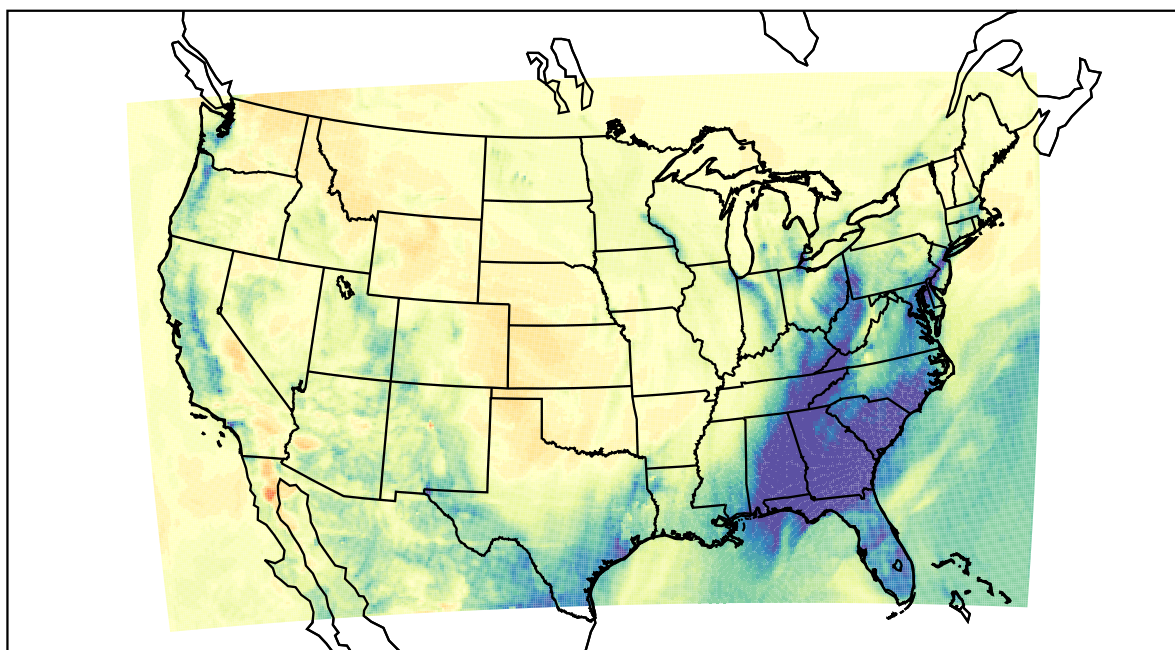
WRF (2021-02-14_04:00:00)
