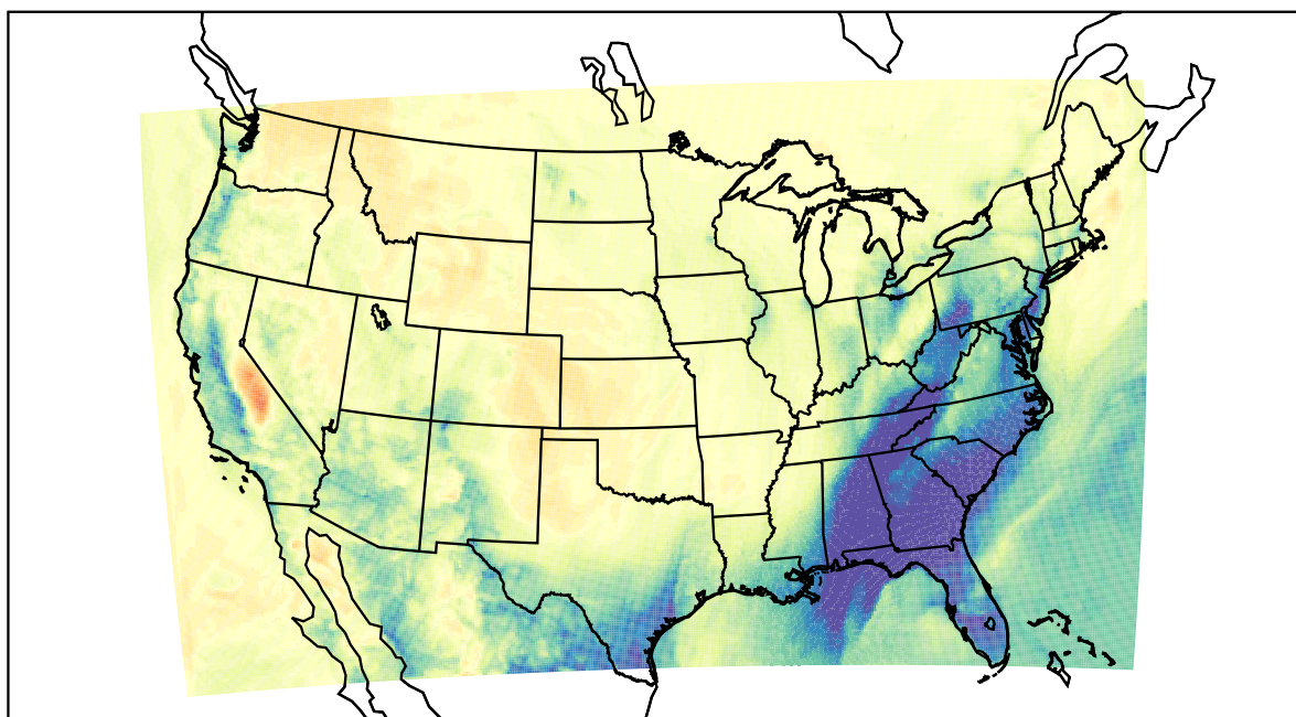
WRF (2021-02-14_10:00:00)
