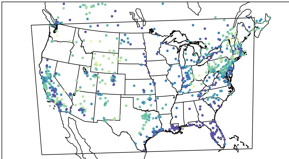
AirNOW (2021-02-15_05:00:00)
