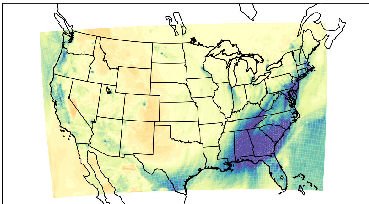
WRF (2021-02-15_02:00:00)
