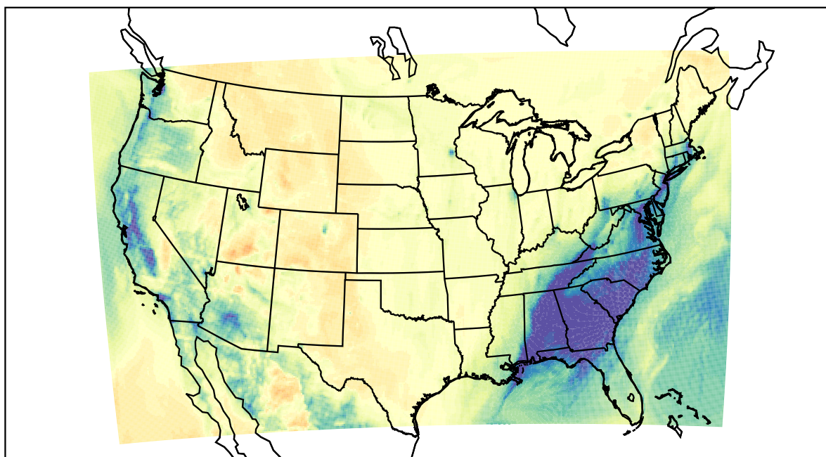
WRF (2021-02-15_16:00:00)
