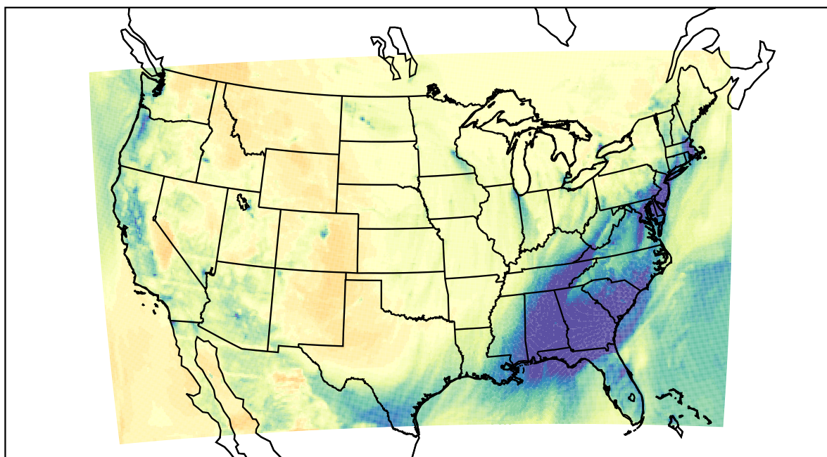
WRF (2021-02-15_03:00:00)
