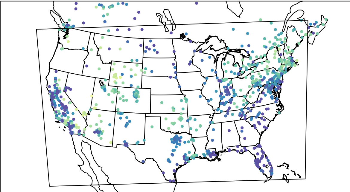
AirNOW (2021-02-14_14:00:00)
