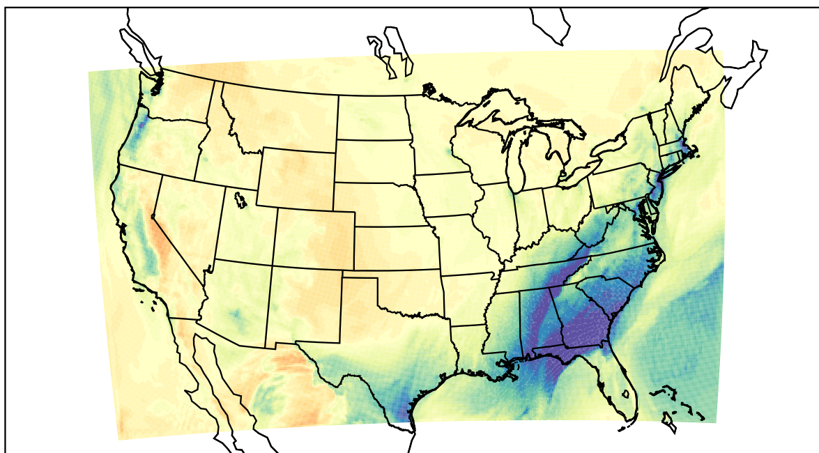
WRF (2021-02-14_19:00:00)
