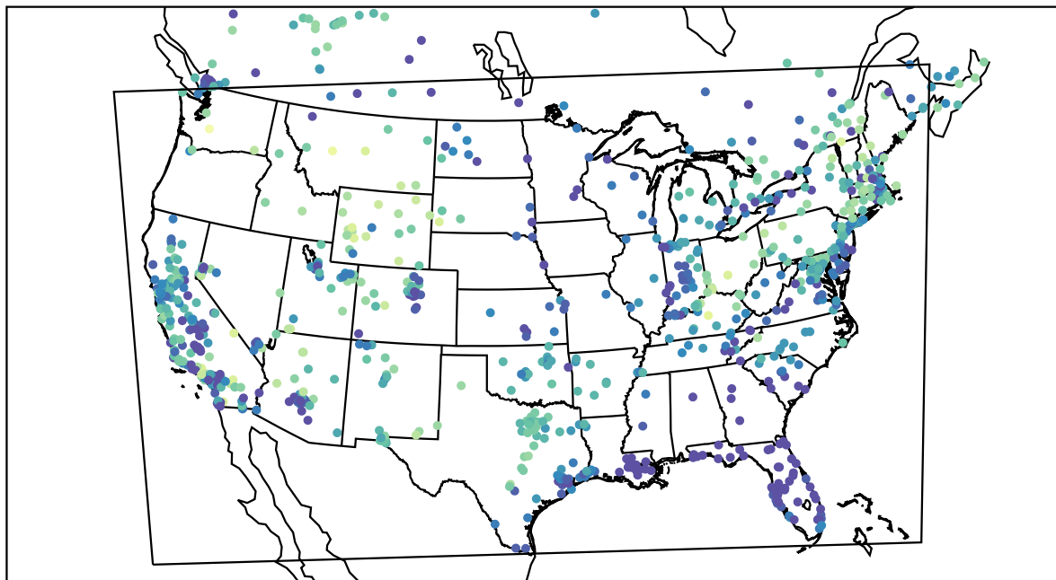
AirNOW (2021-02-15_06:00:00)
