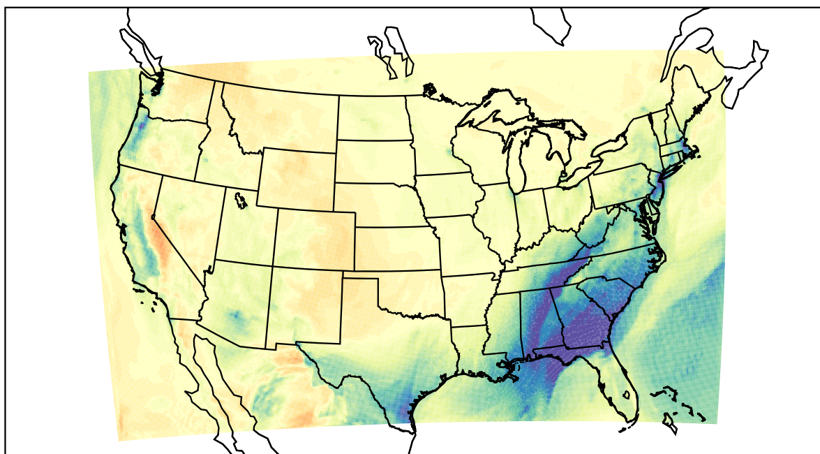
WRF (2021-02-14_18:00:00)
