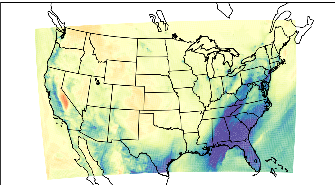
WRF (2021-02-14_13:00:00)
