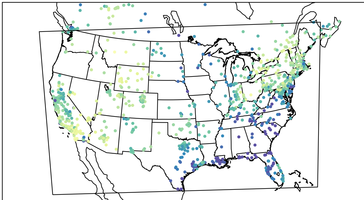
AirNOW (2021-02-14_21:00:00)
