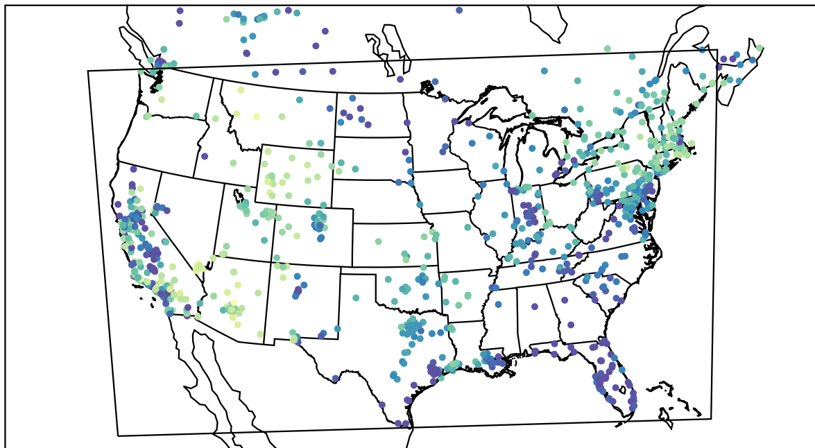
AirNOW (2021-02-14_07:00:00)
