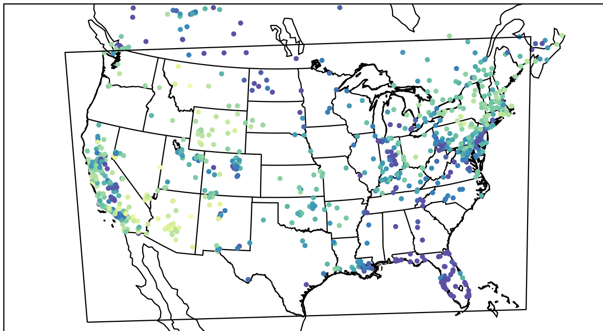
AirNOW (2021-02-14_04:00:00)
