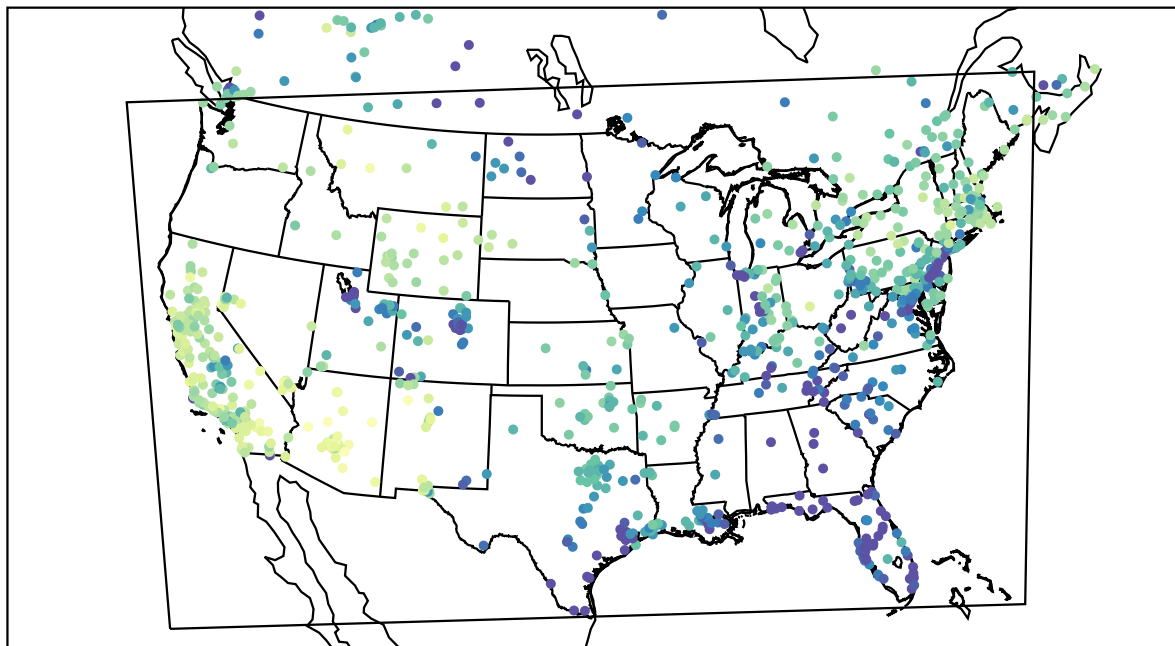
AirNOW (2021-02-14_00:00:00)
