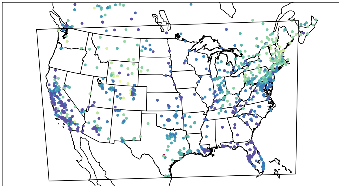
AirNOW (2021-02-15_15:00:00)
