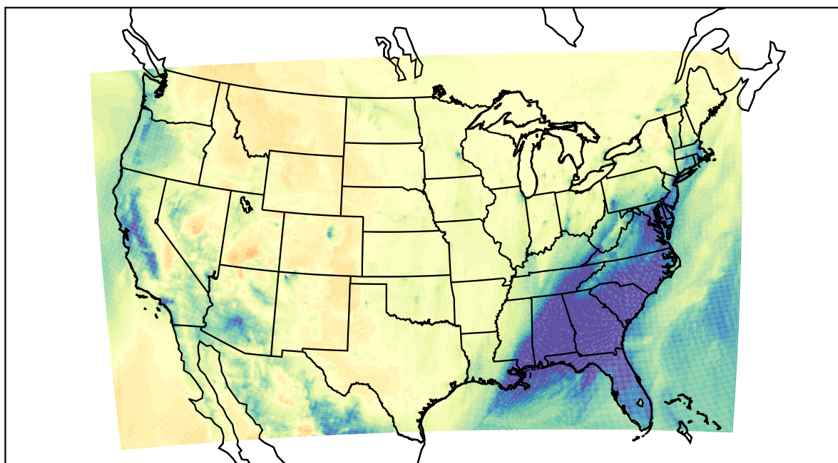
WRF (2021-02-15_13:00:00)
