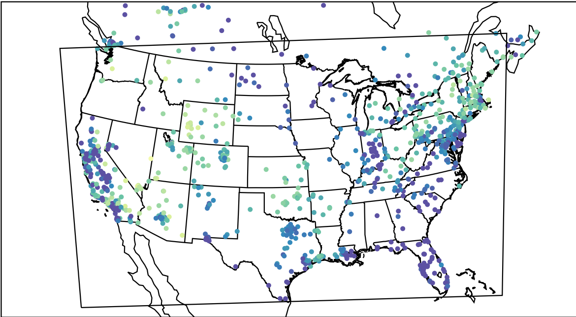
AirNOW (2021-02-14_13:00:00)
