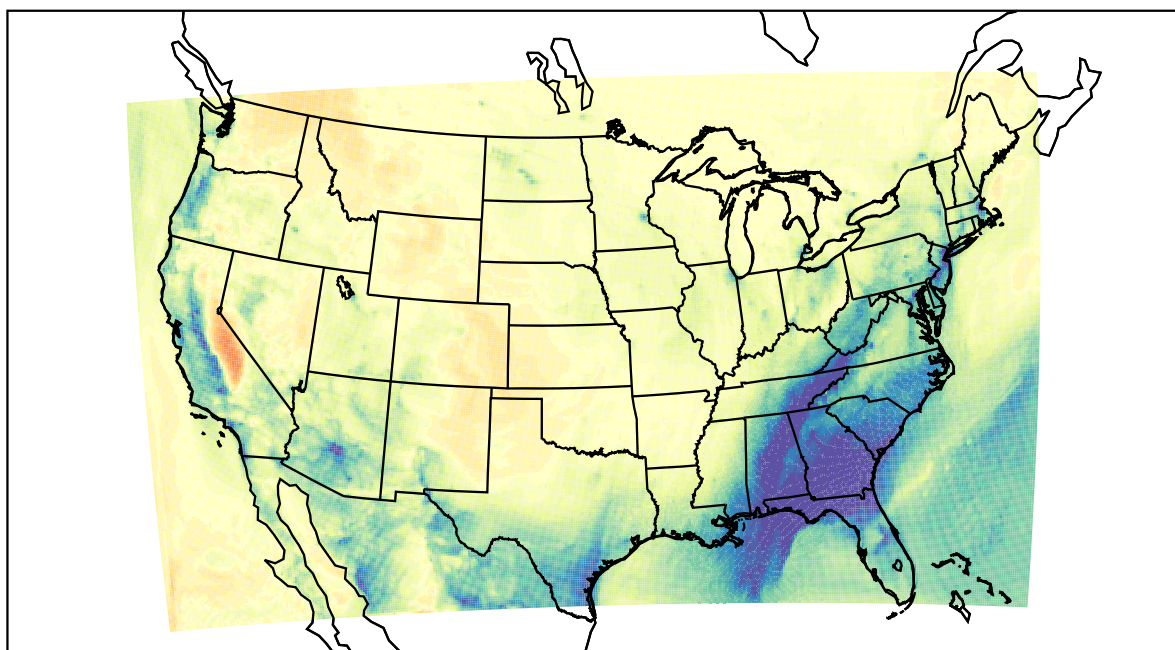
WRF (2021-02-14_15:00:00)
