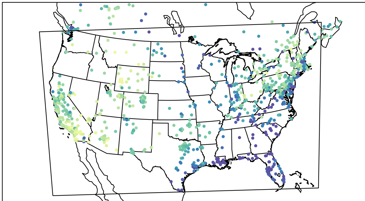
AirNOW (2021-02-15_00:00:00)
