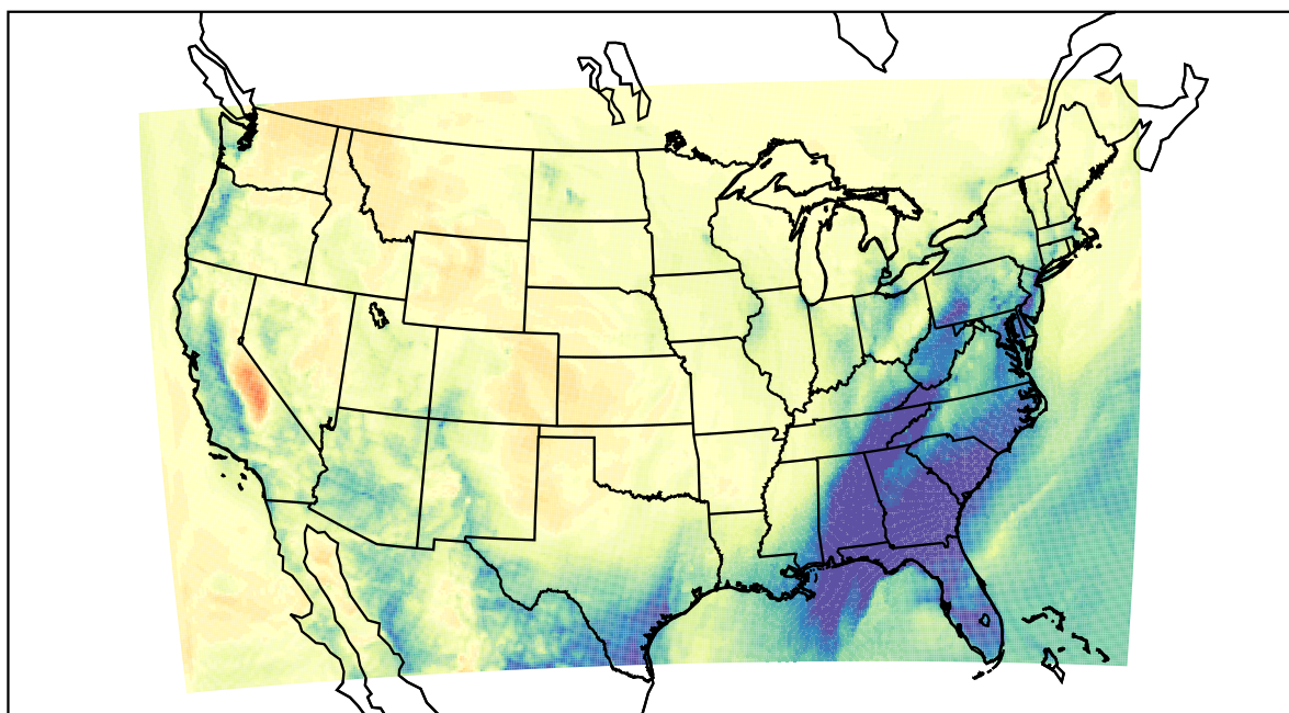
WRF (2021-02-14_11:00:00)
