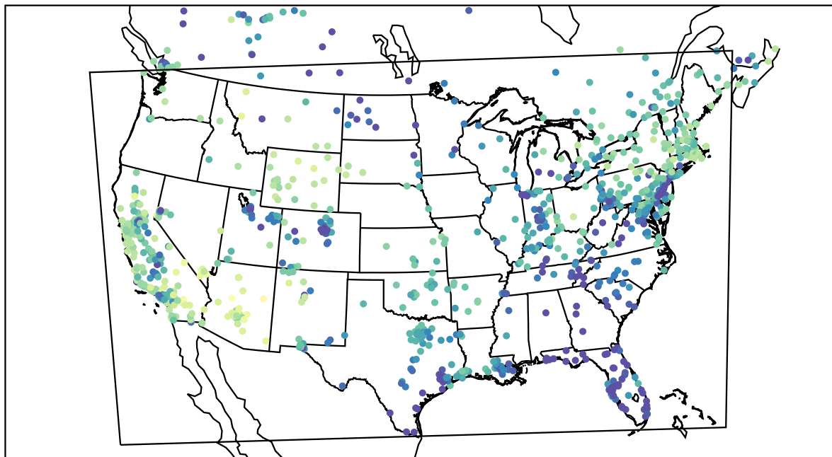
AirNOW (2021-02-14_02:00:00)
