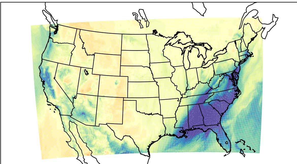
WRF (2021-02-15_10:00:00)
