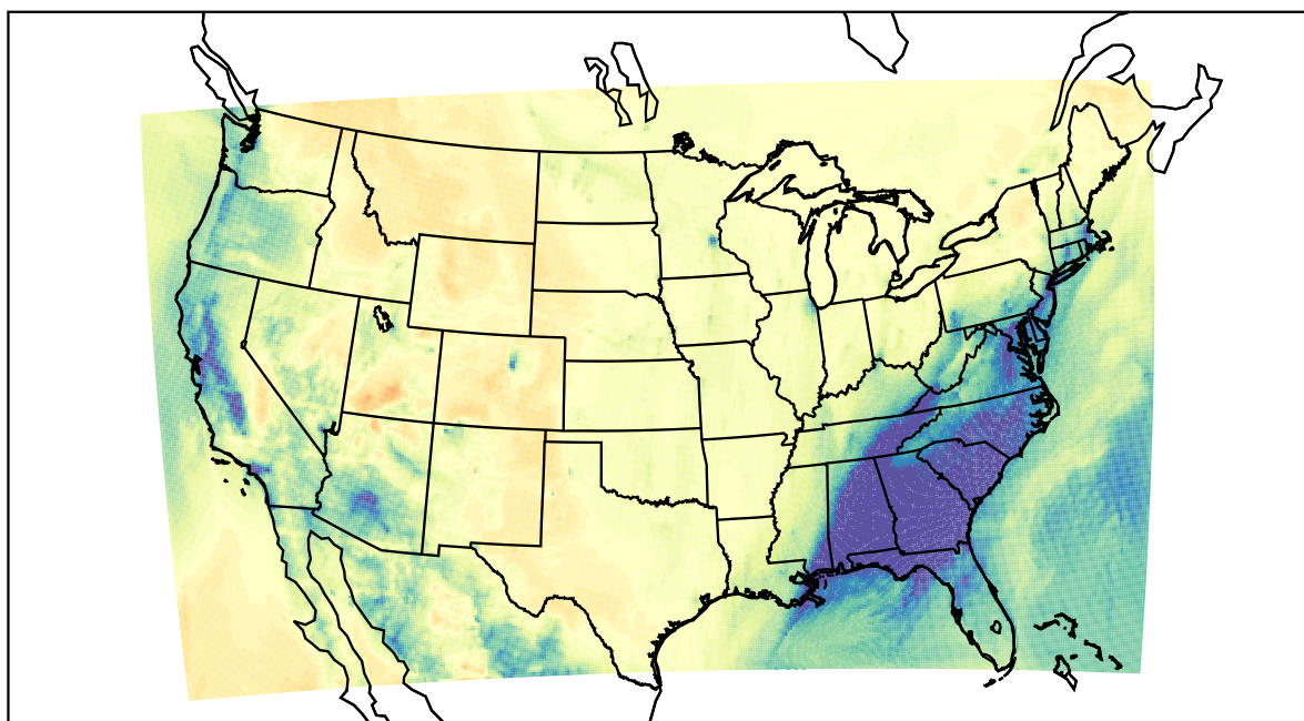
WRF (2021-02-15_15:00:00)
