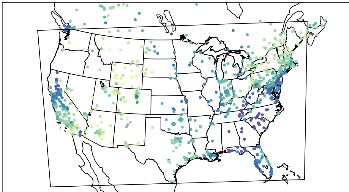
AirNOW (2021-02-15_20:00:00)
