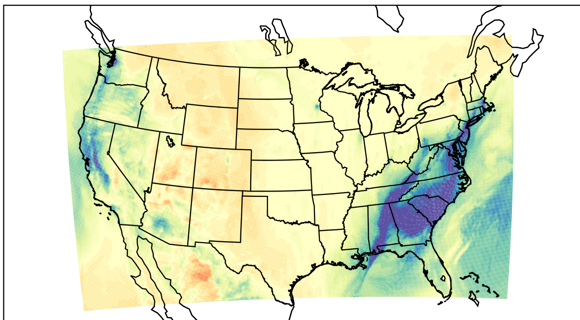
WRF (2021-02-15_18:00:00)
