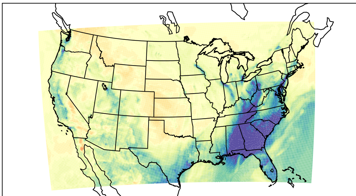
WRF (2021-02-14_03:00:00)
