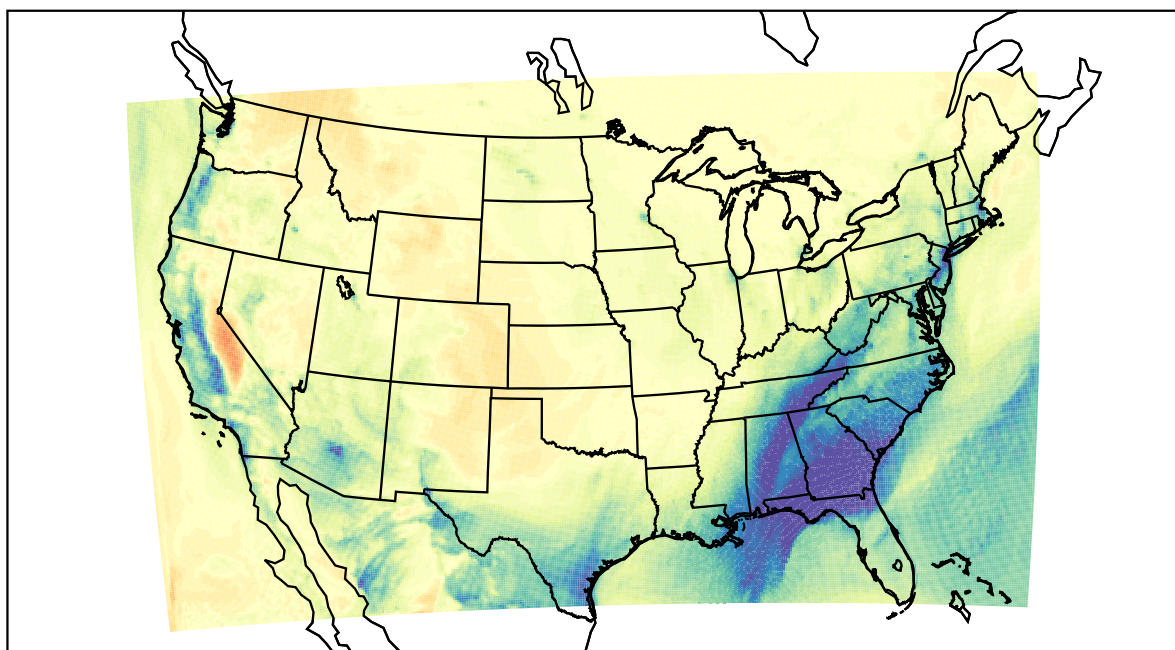
WRF (2021-02-14_16:00:00)
