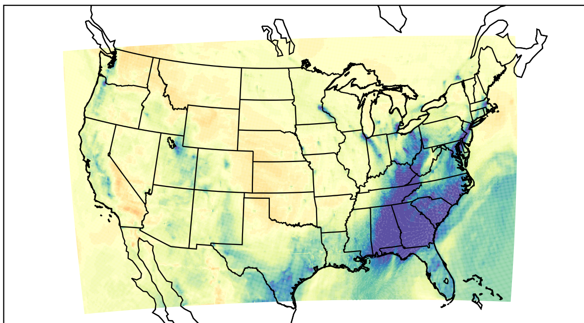
WRF (2021-02-14_01:00:00)
