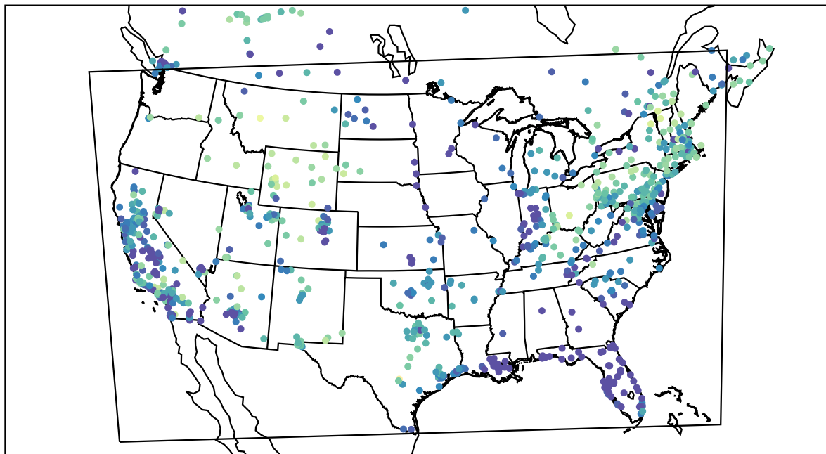
AirNOW (2021-02-15_08:00:00)
