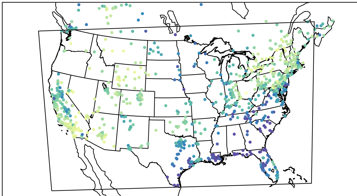
AirNOW (2021-02-14_20:00:00)
