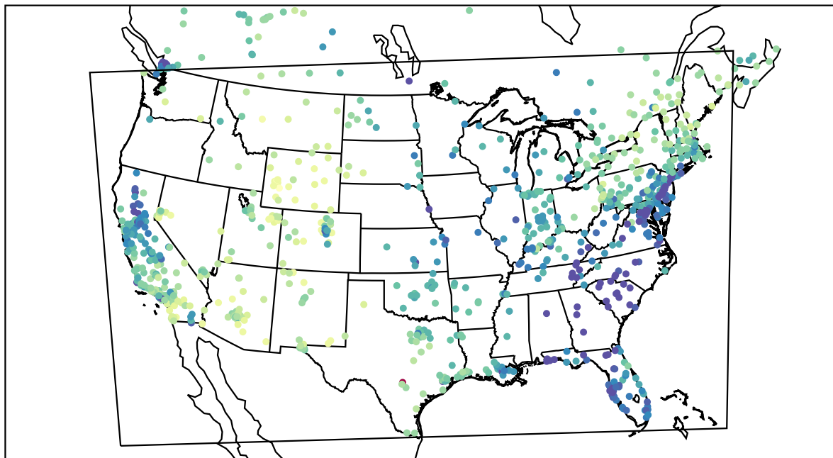
AirNOW (2021-02-15_21:00:00)
