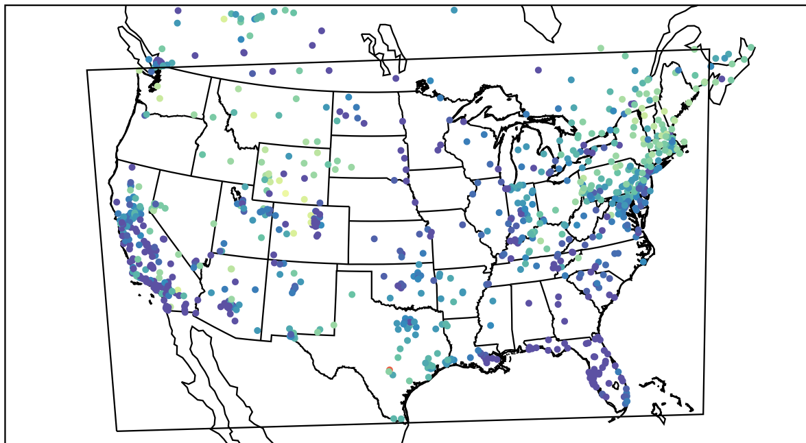
AirNOW (2021-02-15_14:00:00)
