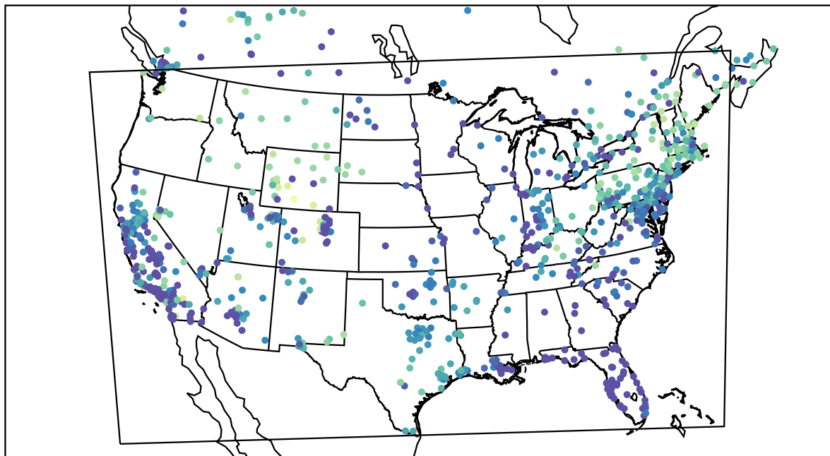
AirNOW (2021-02-15_13:00:00)
