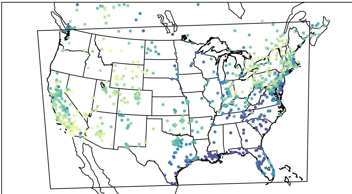
AirNOW (2021-02-14_22:00:00)
