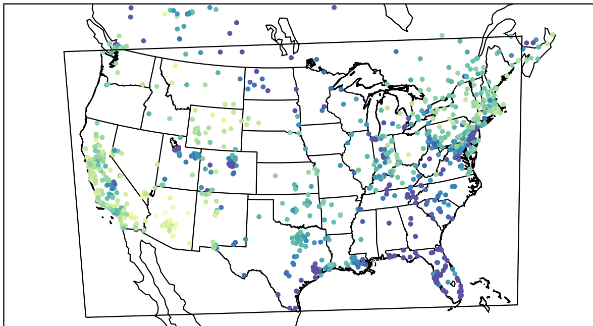
AirNOW (2021-02-14_01:00:00)
