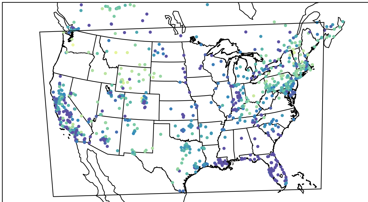
AirNOW (2021-02-15_09:00:00)
