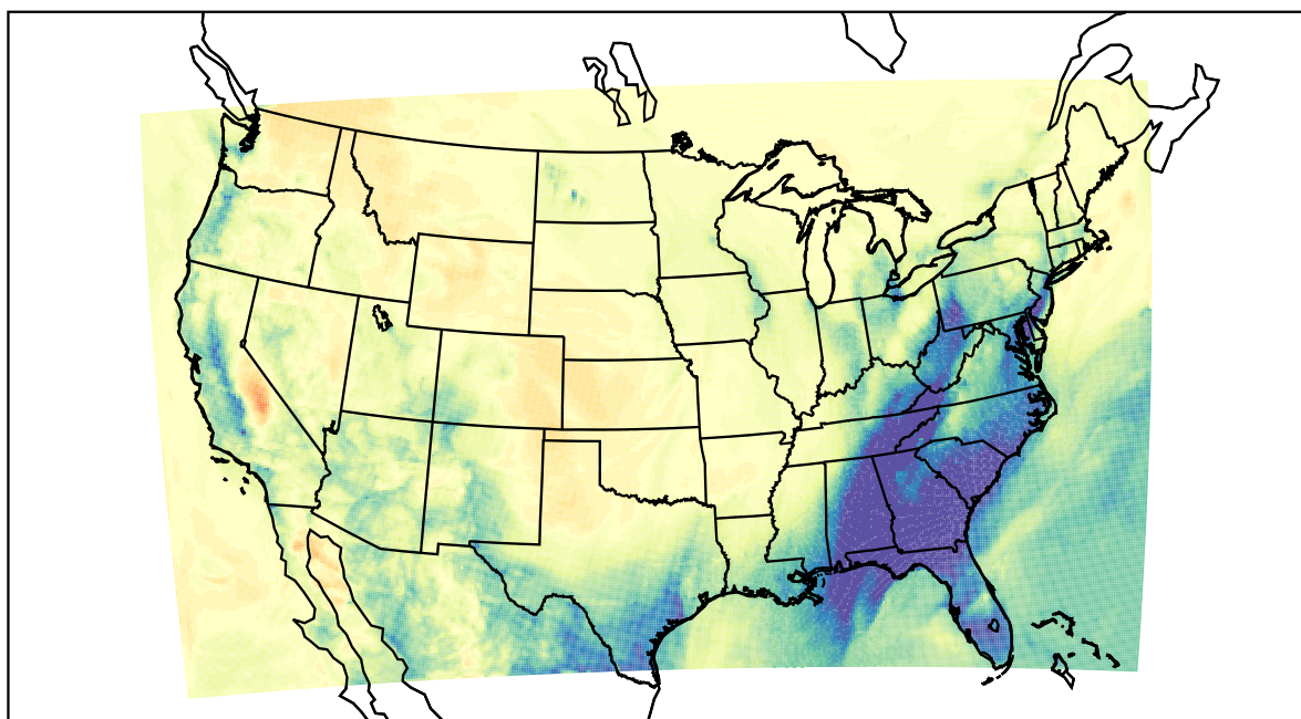
WRF (2021-02-14_08:00:00)
