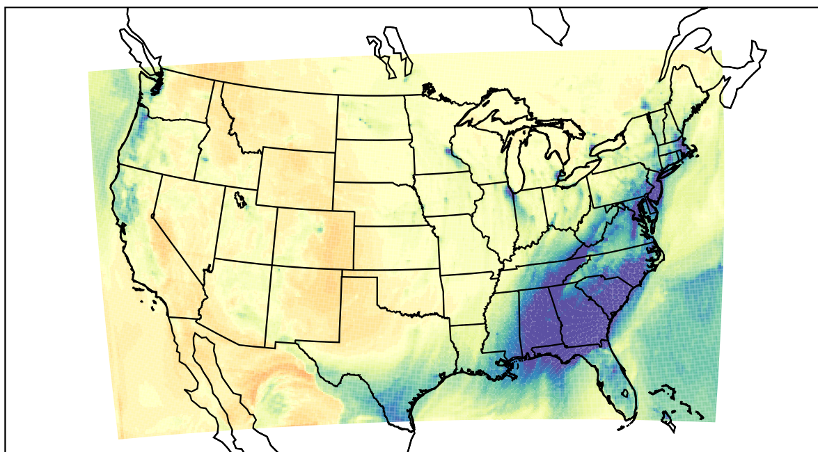
WRF (2021-02-15_00:00:00)
