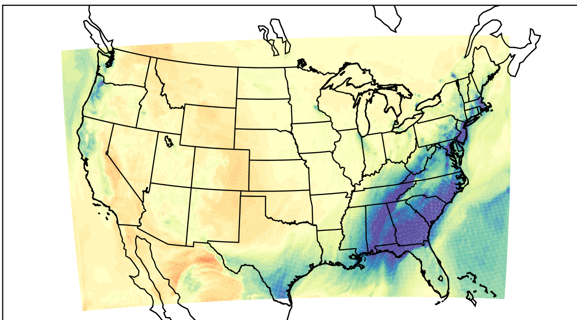
WRF (2021-02-14_22:00:00)
