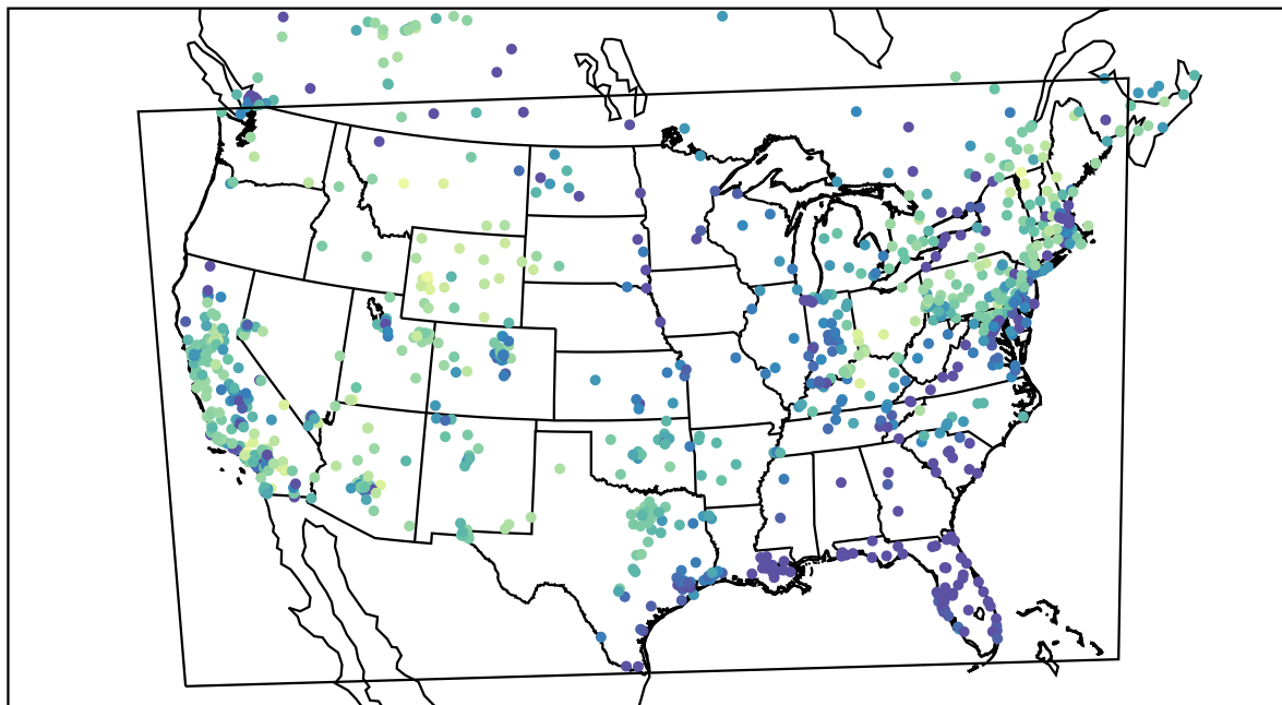
AirNOW (2021-02-15_03:00:00)
