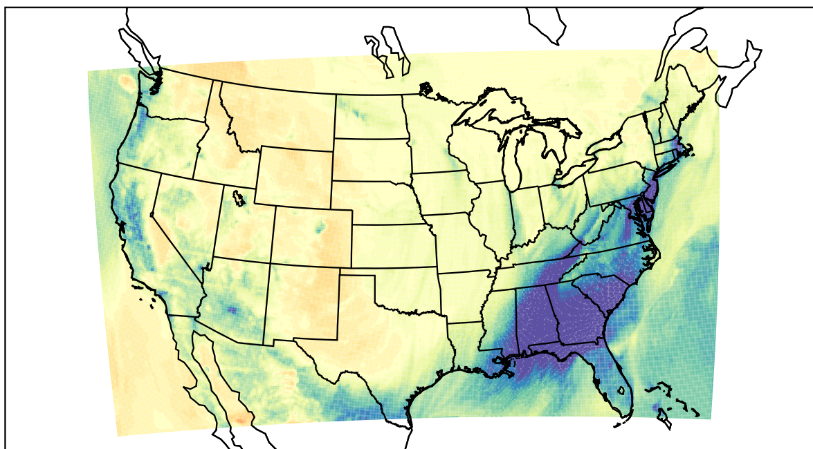
WRF (2021-02-15_06:00:00)
