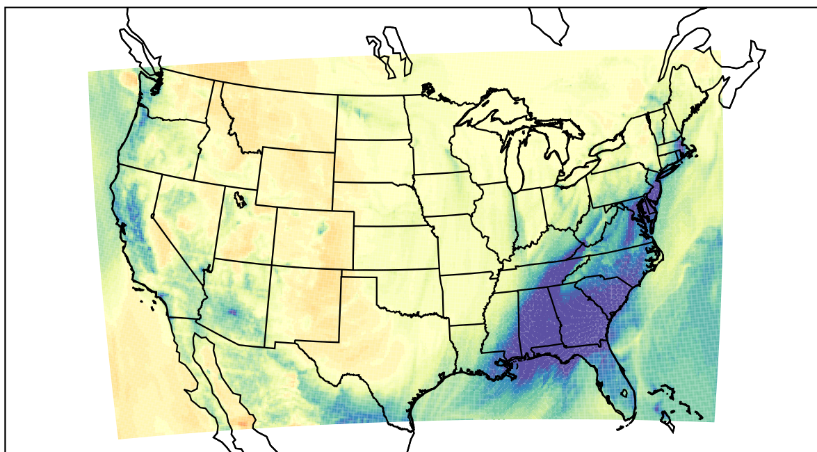
WRF (2021-02-15_07:00:00)
