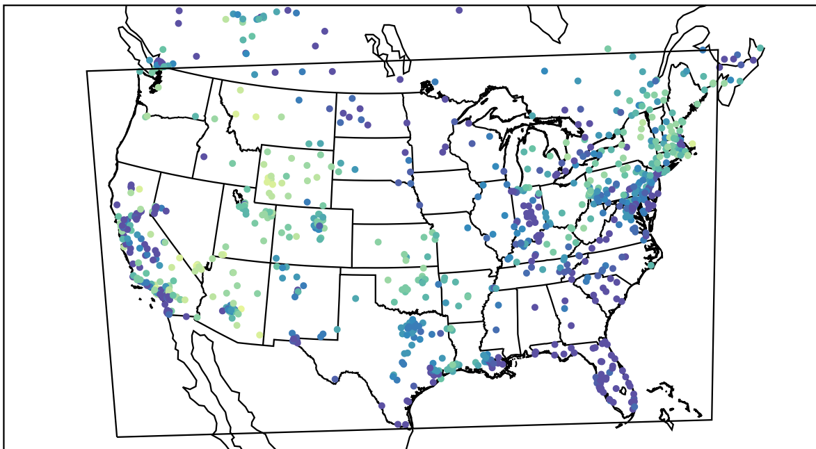
AirNOW (2021-02-14_12:00:00)
