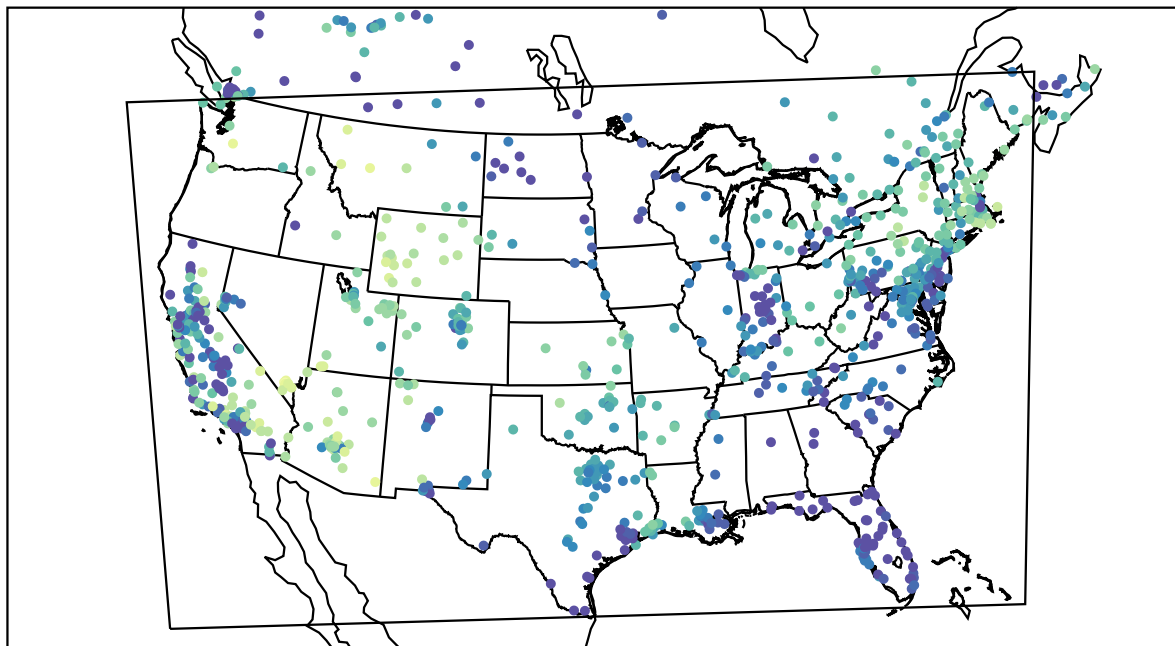
AirNOW (2021-02-14_09:00:00)
