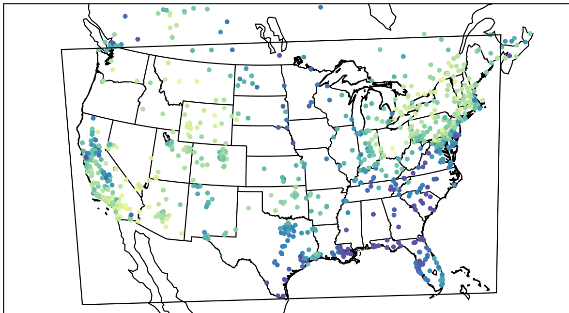
AirNOW (2021-02-14_19:00:00)
