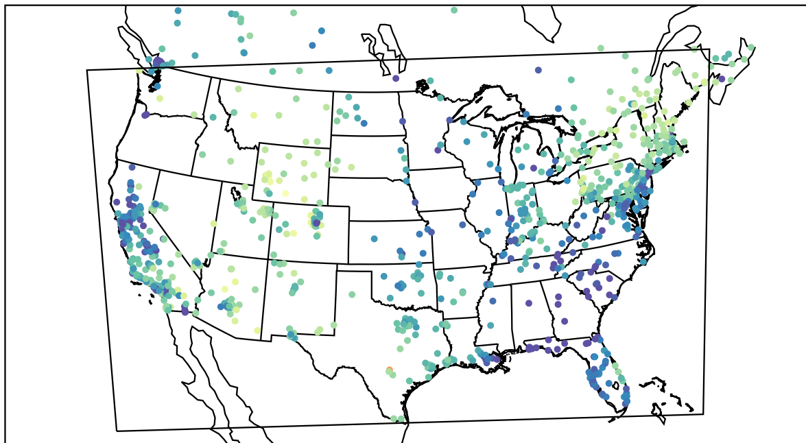
AirNOW (2021-02-15_18:00:00)
