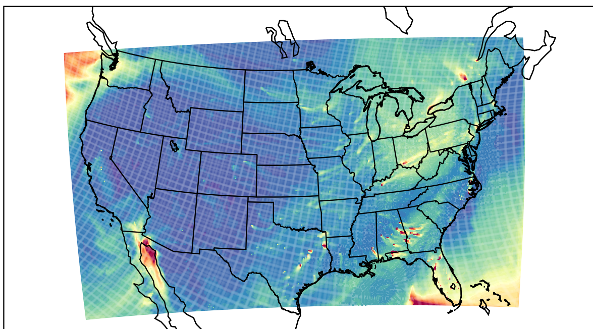
WRF 2021-02-22_22:00:00
