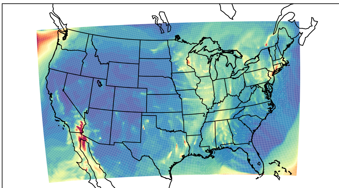
WRF 2021-02-22_08:00:00
