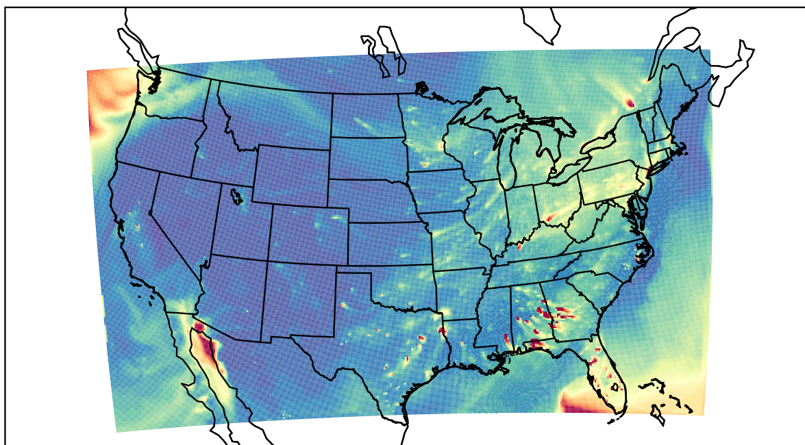
WRF 2021-02-23_00:00:00
