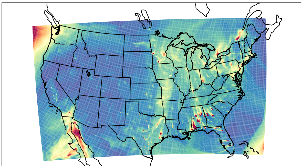
WRF 2021-02-22_00:00:00
