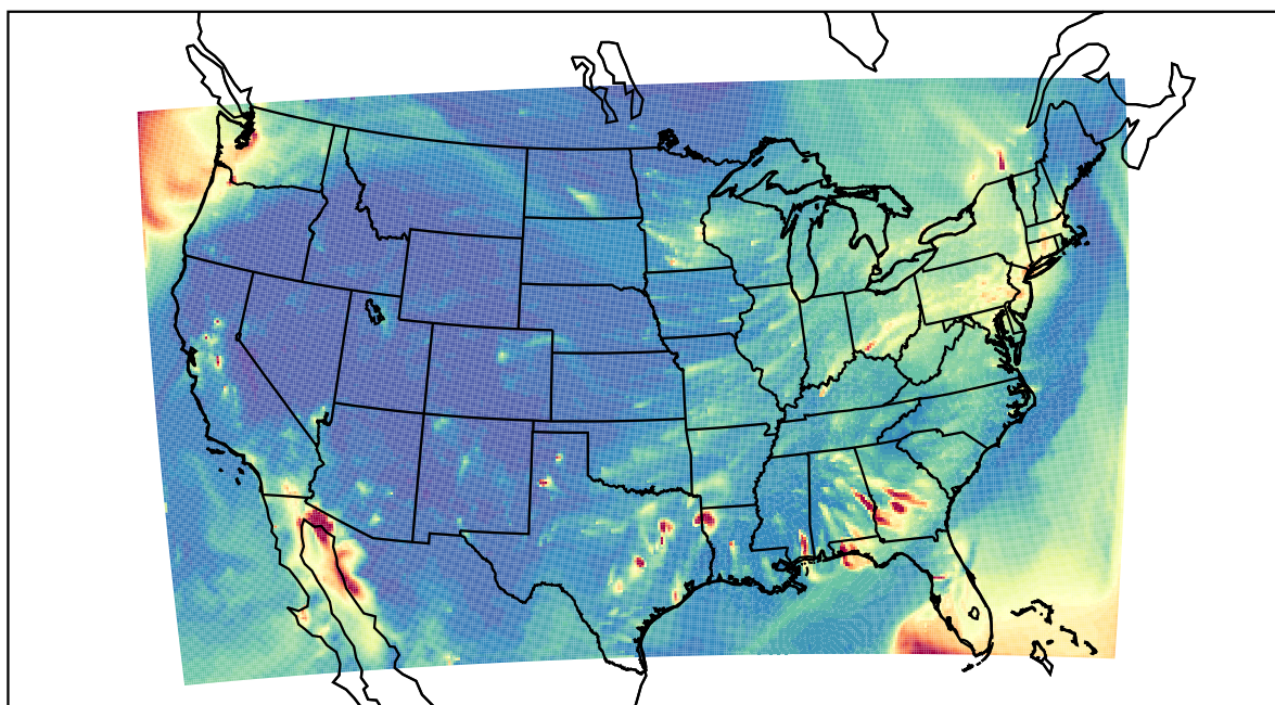
WRF 2021-02-23_03:00:00
