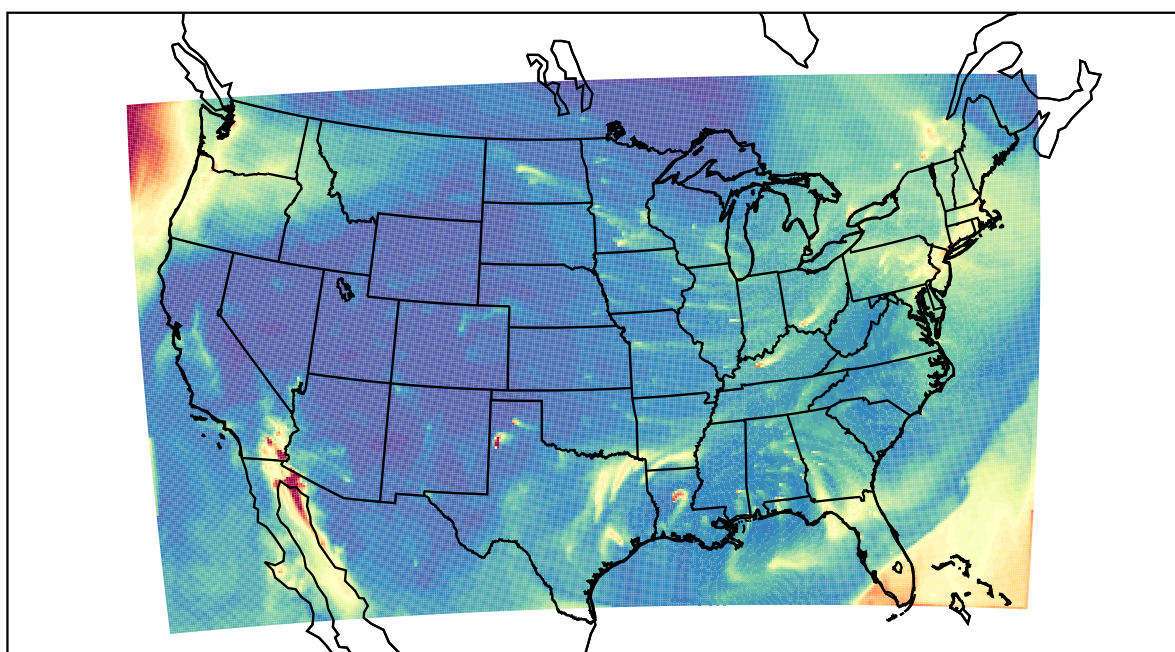
WRF 2021-02-23_11:00:00
