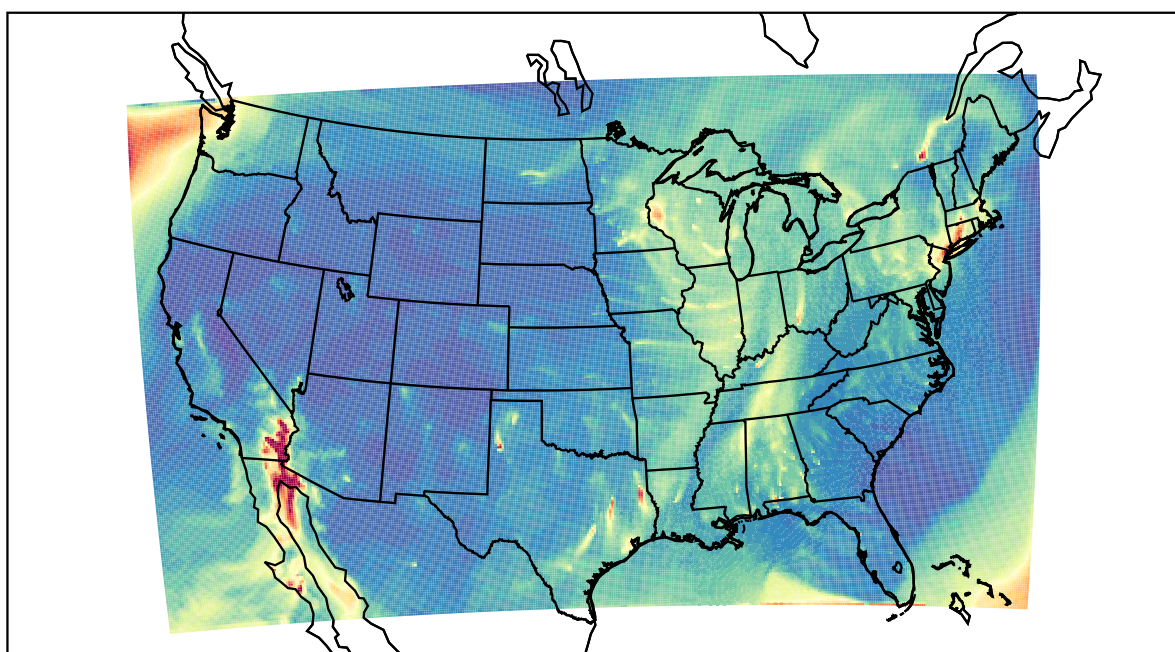
WRF 2021-02-22_09:00:00
