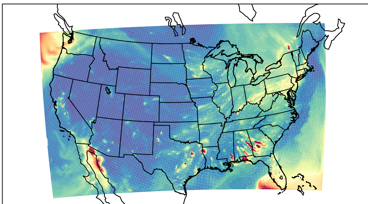
WRF 2021-02-23_02:00:00
