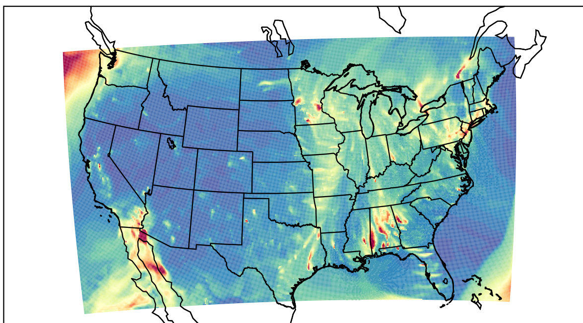
WRF 2021-02-22_03:00:00
