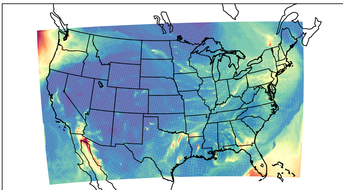
WRF 2021-02-23_08:00:00
