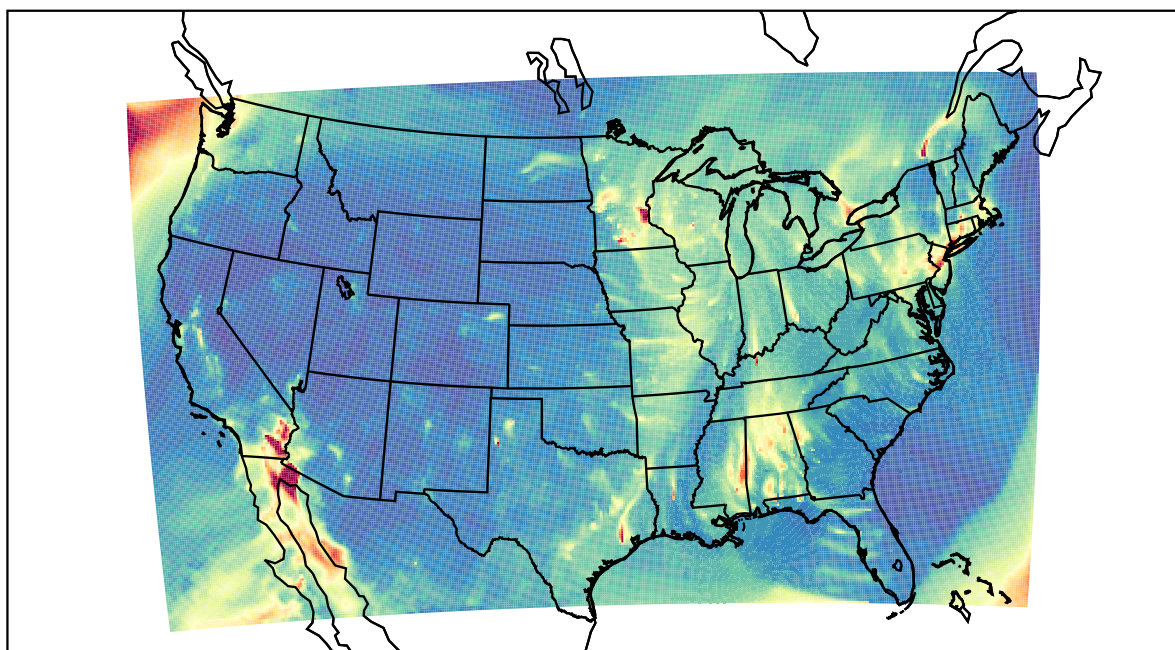
WRF 2021-02-22_05:00:00
