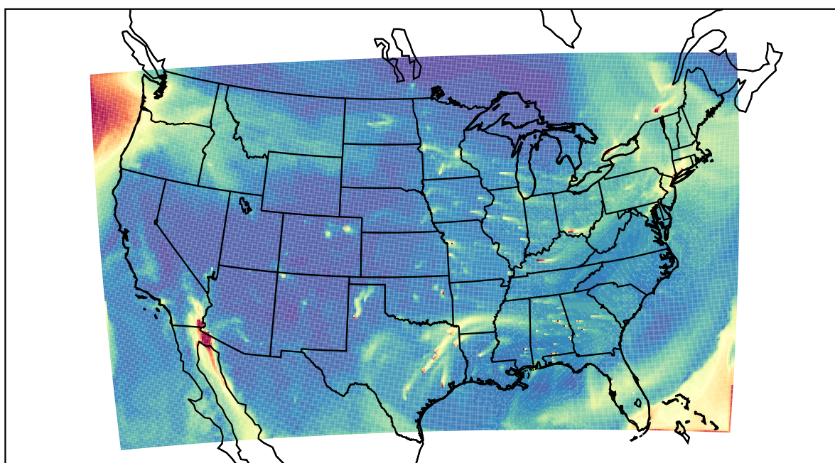
WRF 2021-02-23_17:00:00
