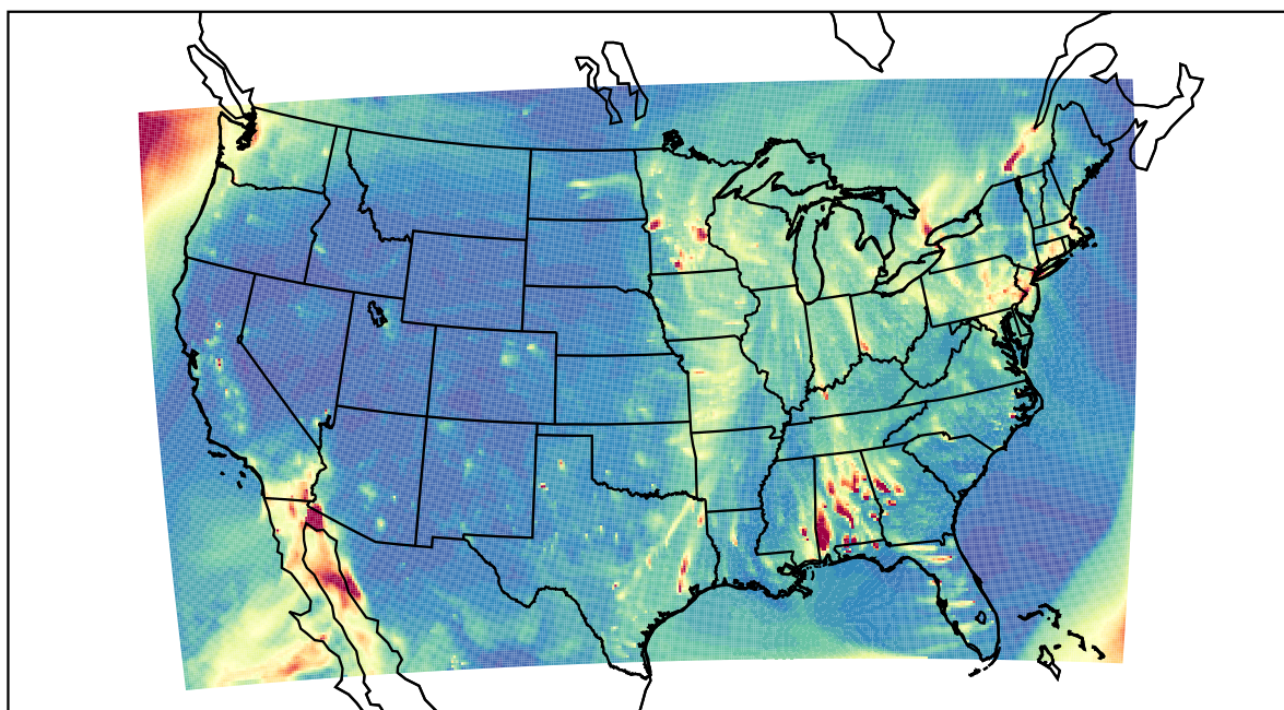
WRF 2021-02-22_02:00:00
