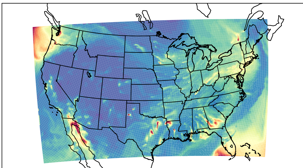
WRF 2021-02-23_05:00:00
