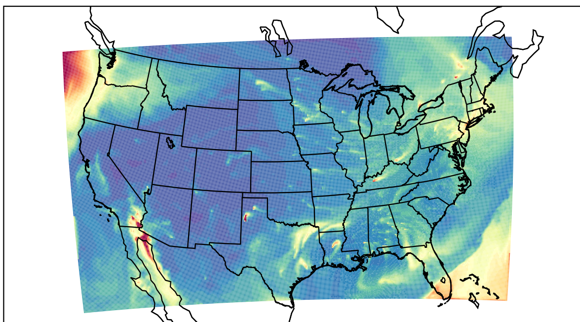
WRF 2021-02-23_12:00:00
