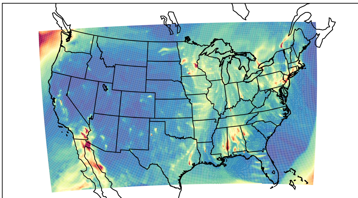
WRF 2021-02-22_04:00:00
