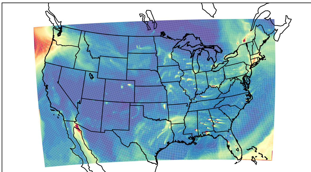
WRF 2021-02-23_21:00:00
