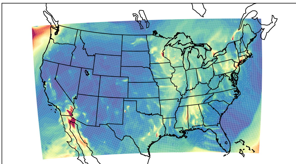
WRF 2021-02-22_06:00:00
