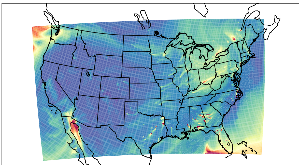
WRF 2021-02-22_21:00:00
