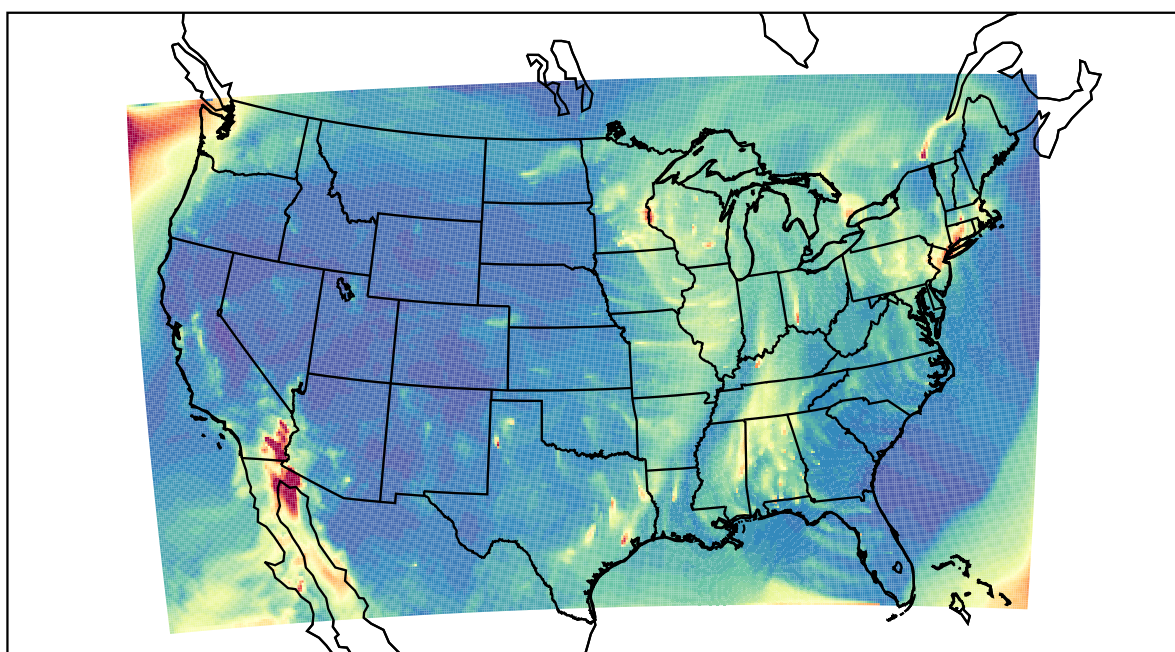
WRF 2021-02-22_07:00:00
