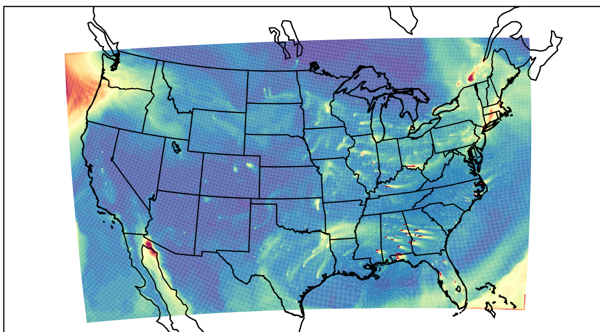
WRF 2021-02-23_22:00:00
