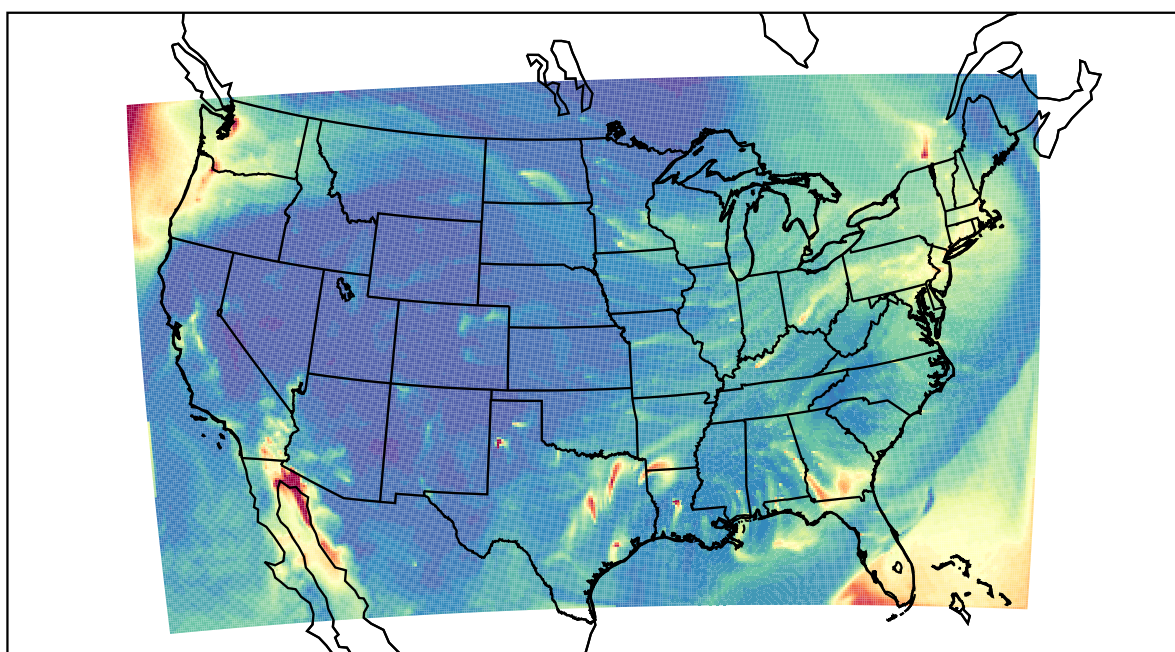
WRF 2021-02-23_07:00:00
