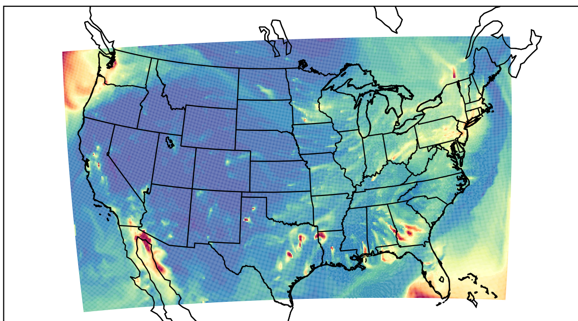
WRF 2021-02-23_04:00:00
