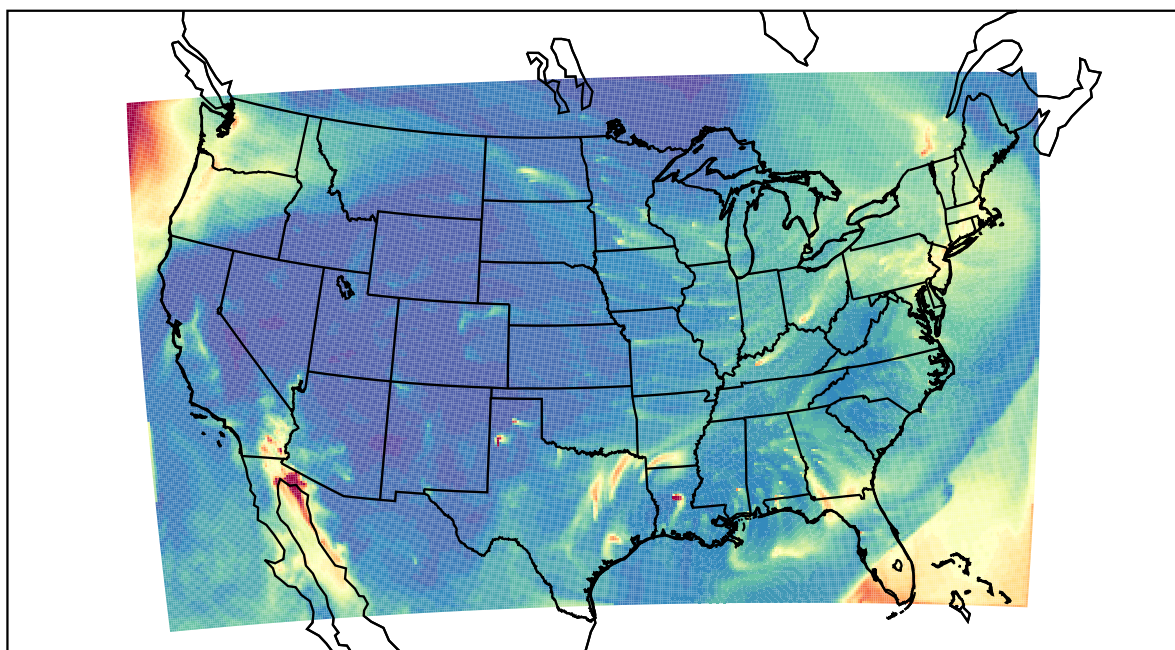
WRF 2021-02-23_09:00:00
