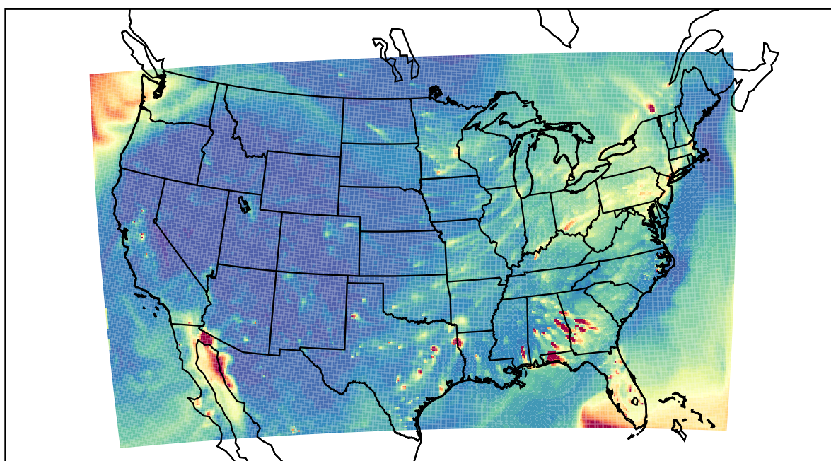
WRF 2021-02-23_01:00:00
