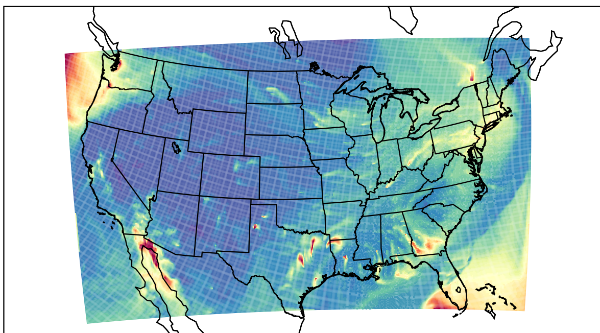
WRF 2021-02-23_06:00:00
