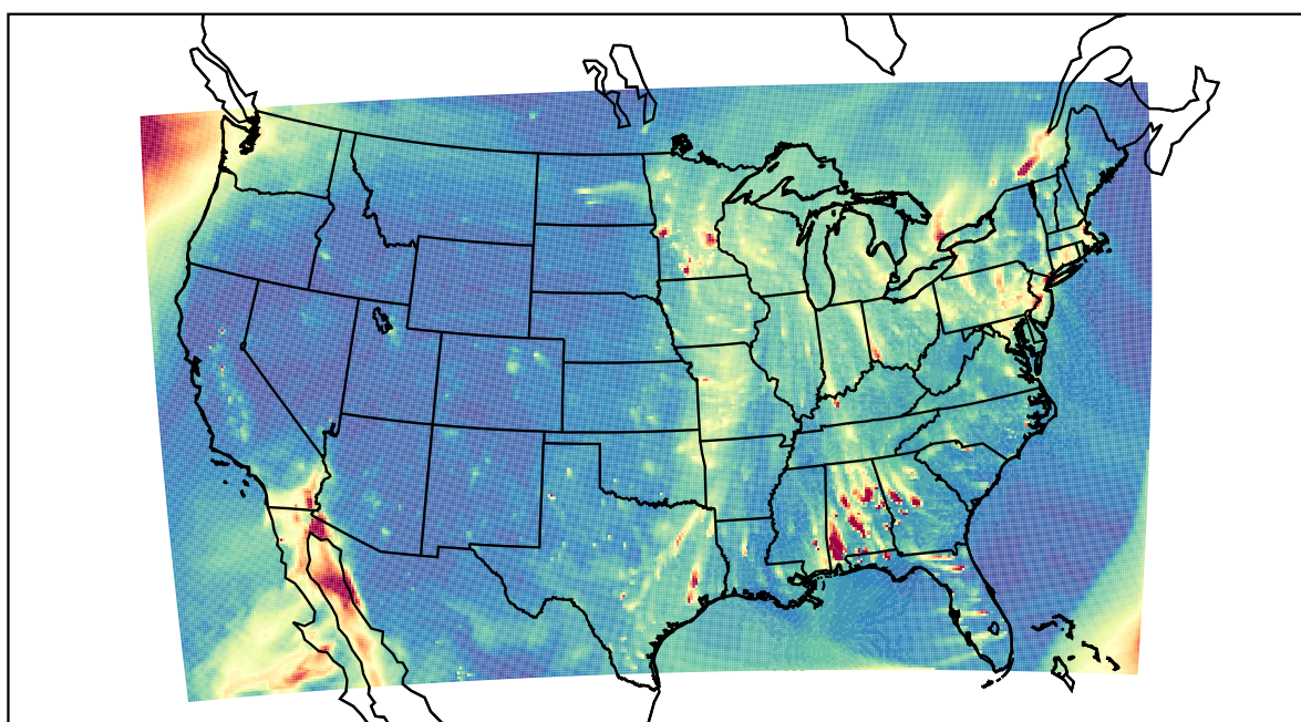
WRF 2021-02-22_01:00:00
