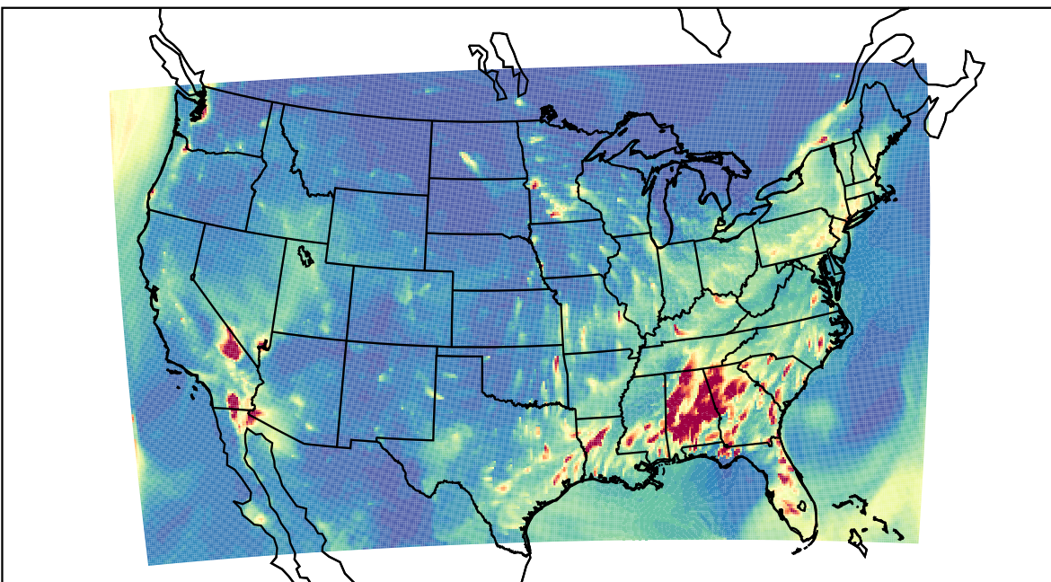
WRF 2021-02-25_03:00:00
