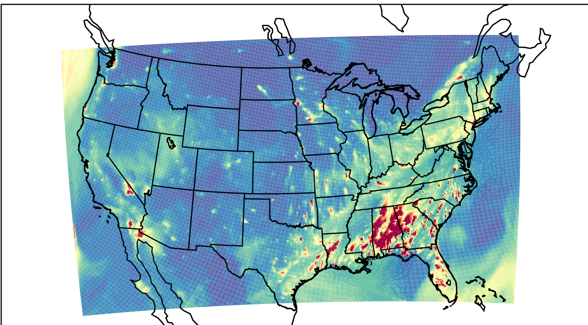
WRF 2021-02-25_02:00:00
