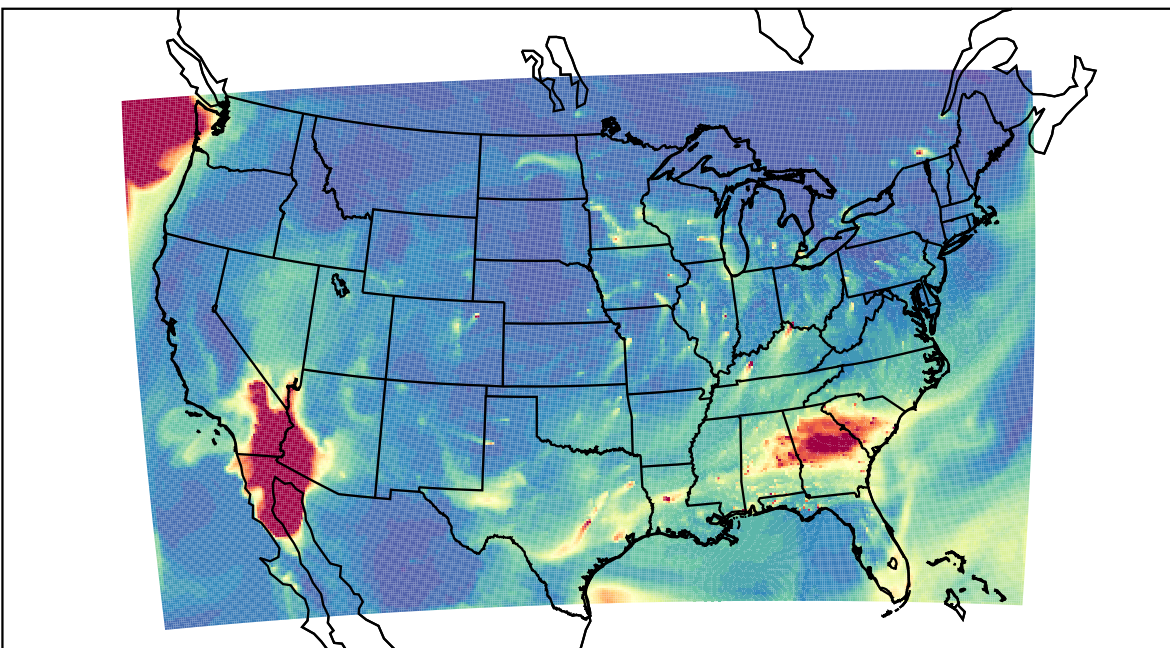
WRF 2021-02-25_14:00:00
