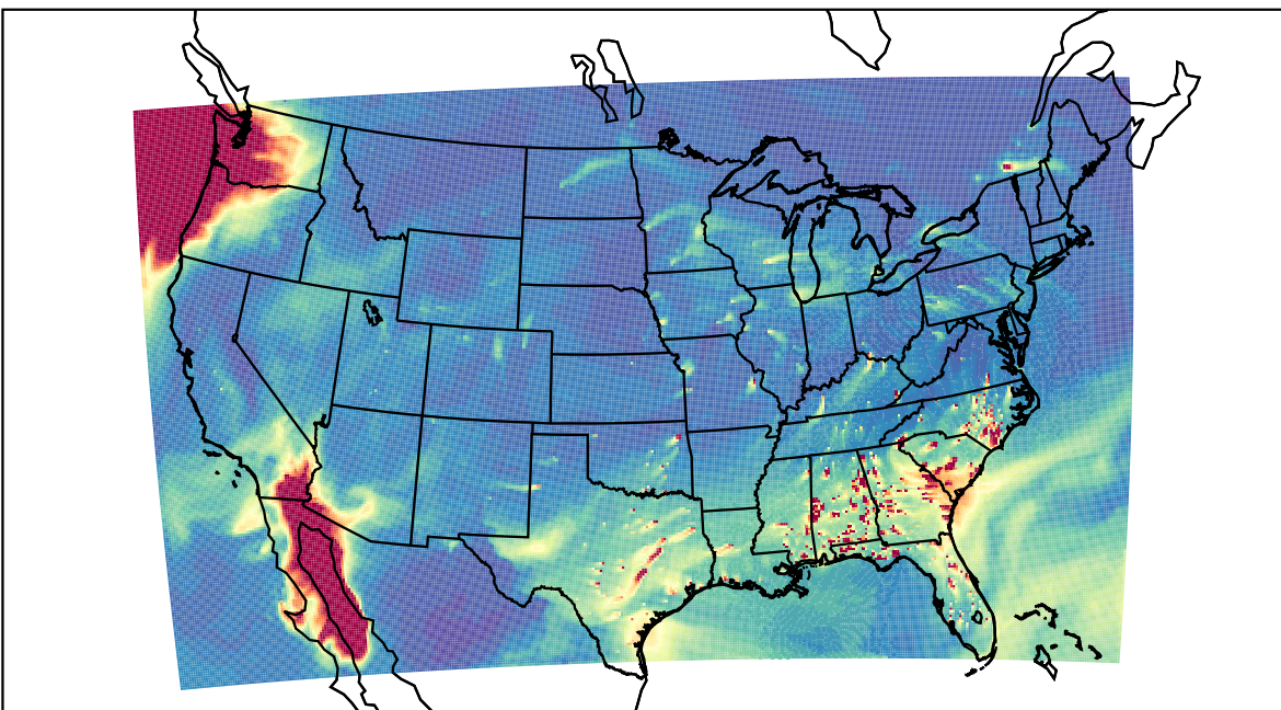
WRF 2021-02-25_21:00:00
