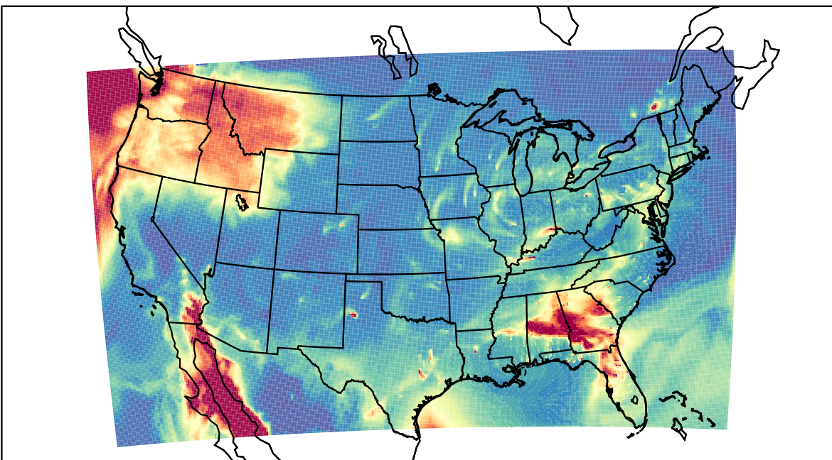
WRF 2021-02-26_12:00:00
