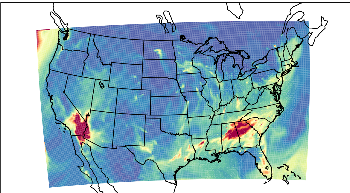
WRF 2021-02-25_08:00:00
