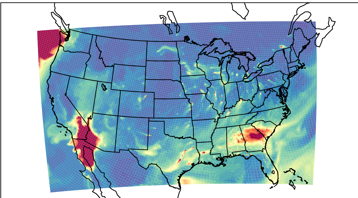
WRF 2021-02-25_15:00:00
