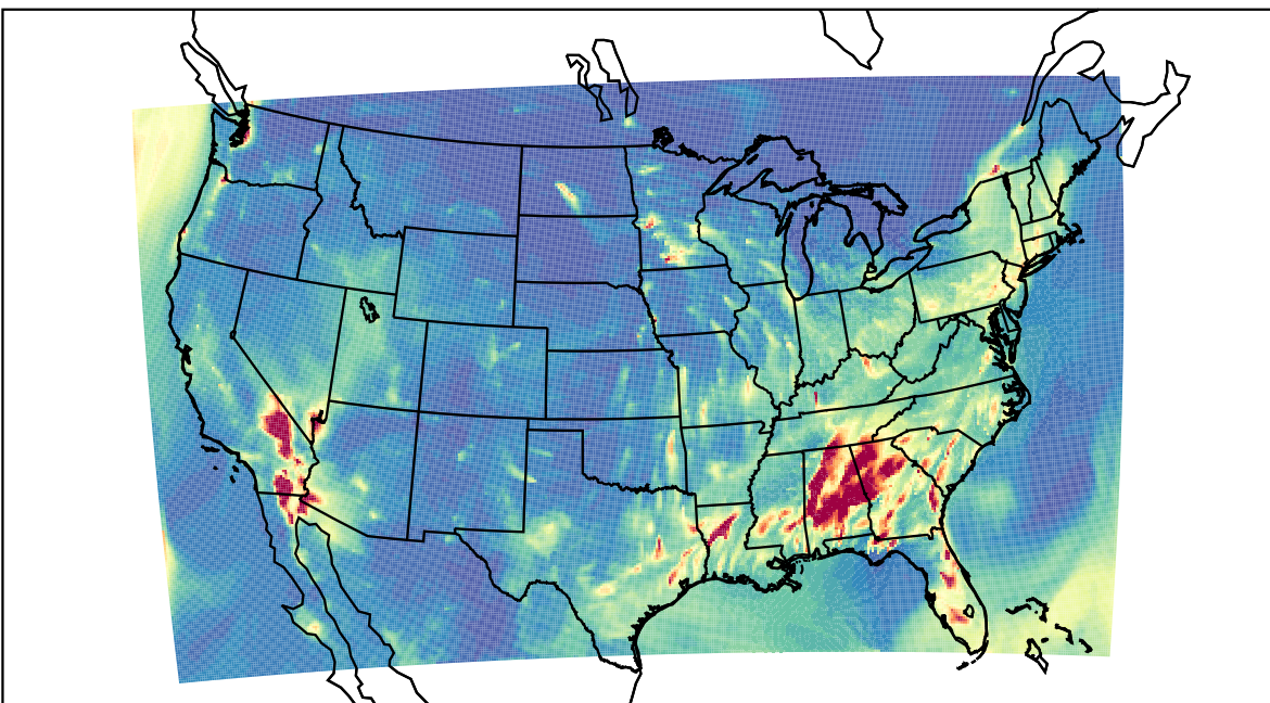
WRF 2021-02-25_04:00:00
