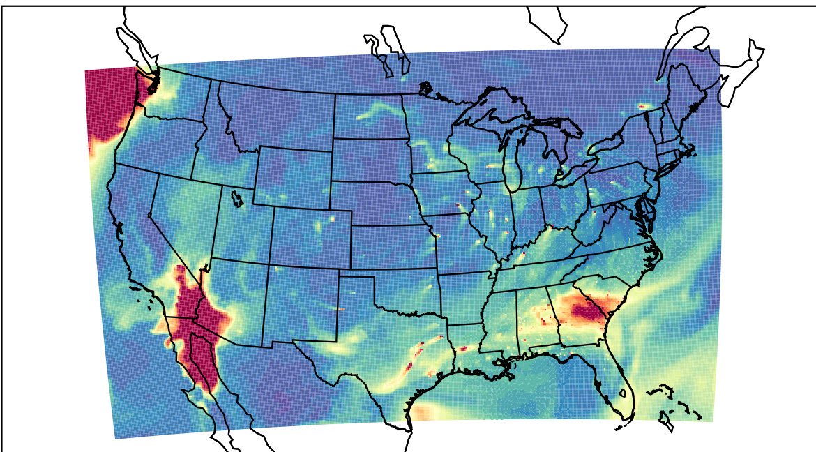
WRF 2021-02-25_16:00:00
