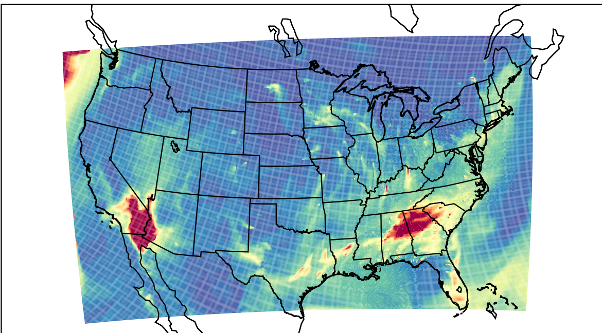
WRF 2021-02-25_09:00:00
