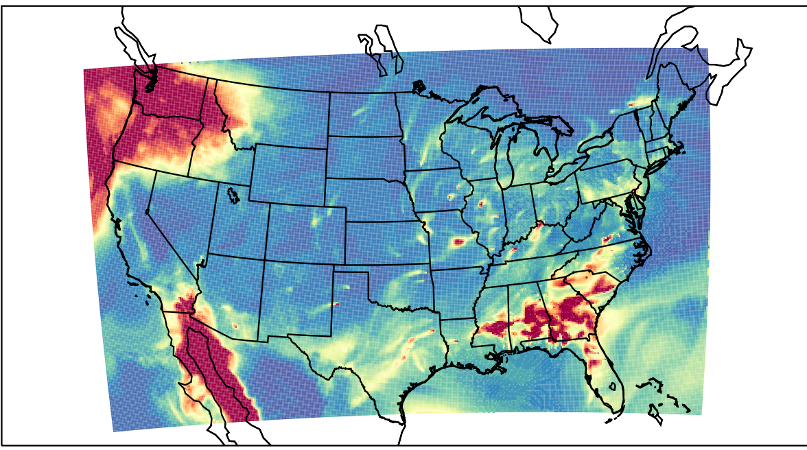
WRF 2021-02-26_06:00:00
