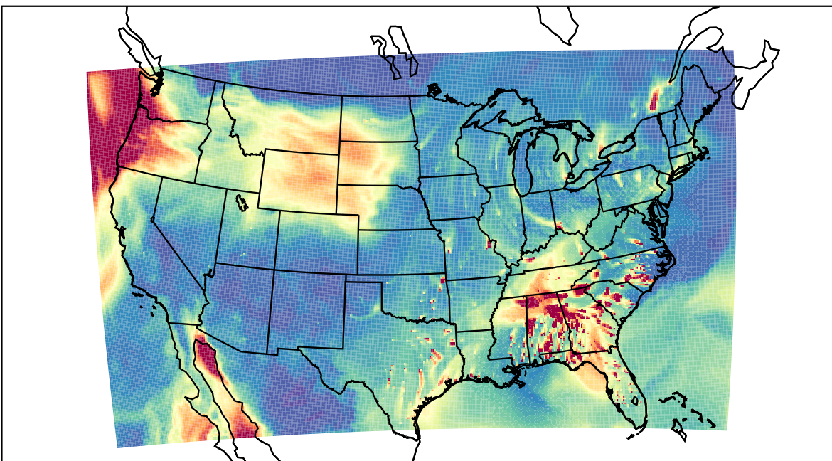
WRF 2021-02-26_22:00:00
