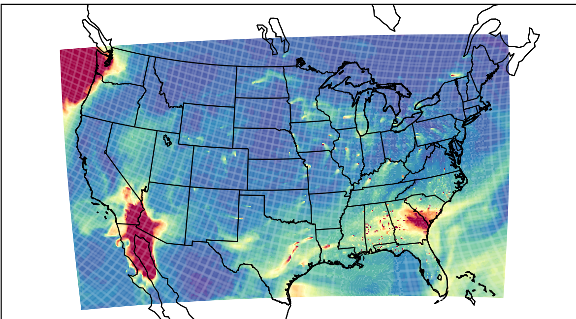
WRF 2021-02-25_17:00:00
