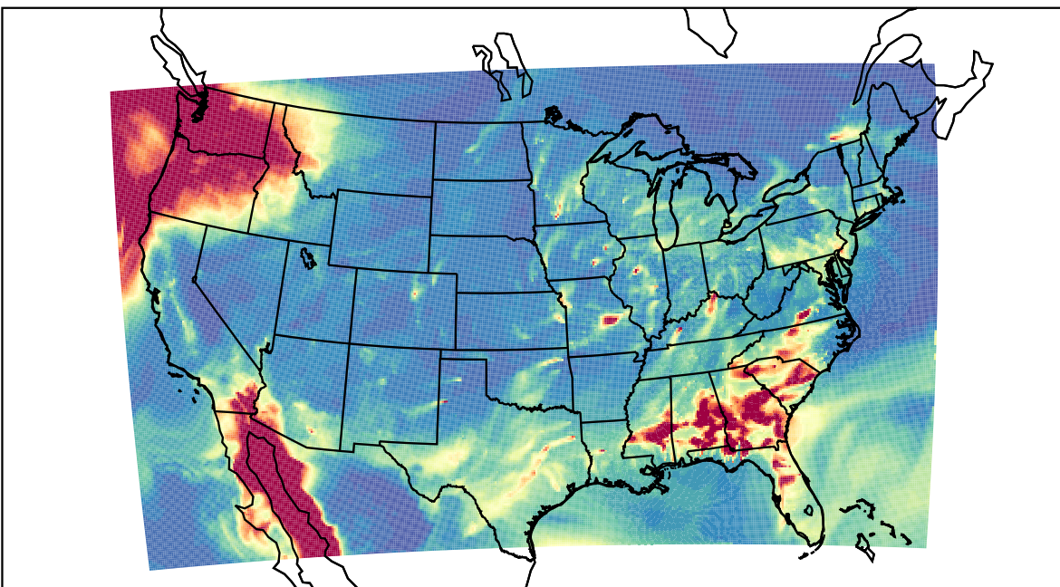
WRF 2021-02-26_05:00:00
