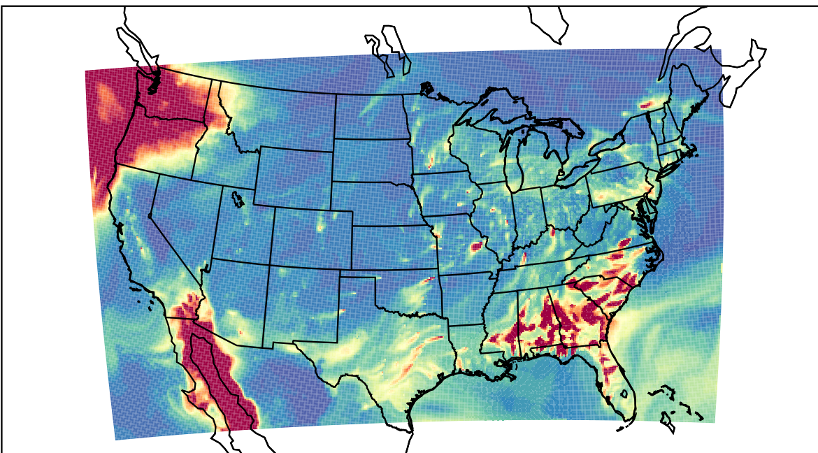
WRF 2021-02-26_03:00:00
