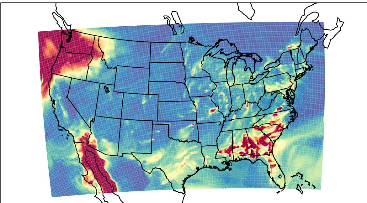
WRF 2021-02-26_04:00:00
