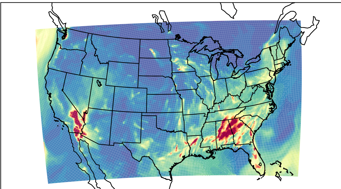
WRF 2021-02-25_05:00:00
