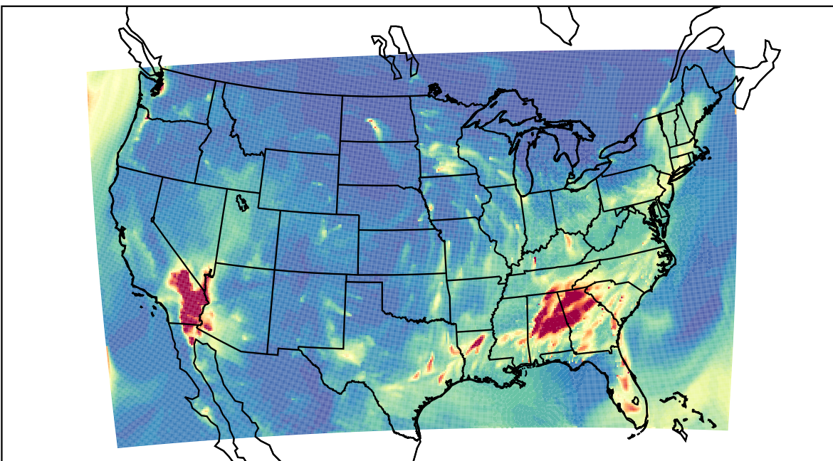
WRF 2021-02-25_06:00:00
