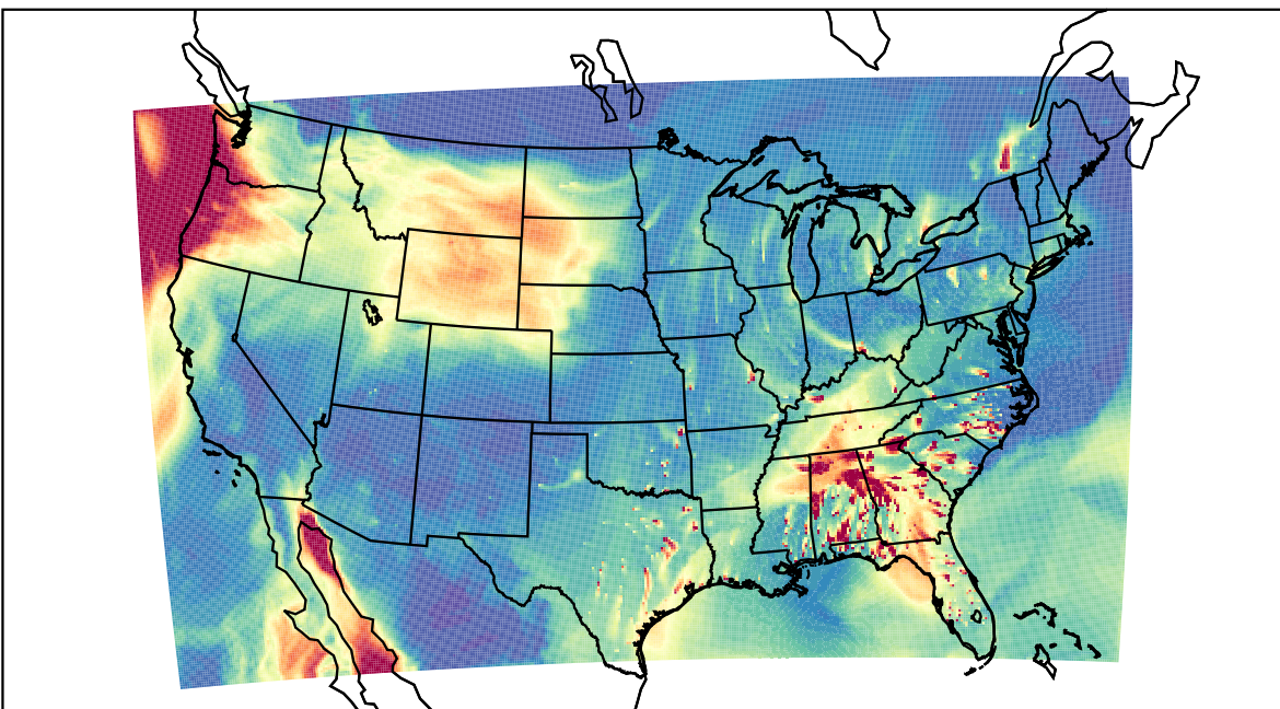
WRF 2021-02-26_21:00:00
