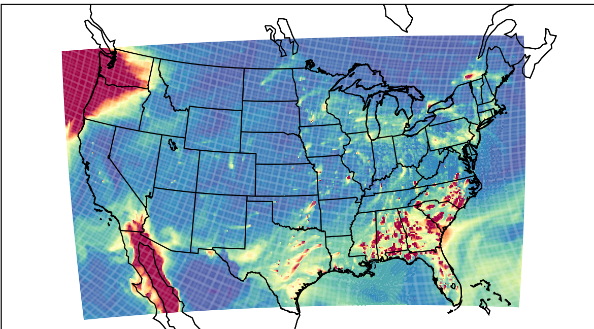
WRF 2021-02-26_00:00:00
