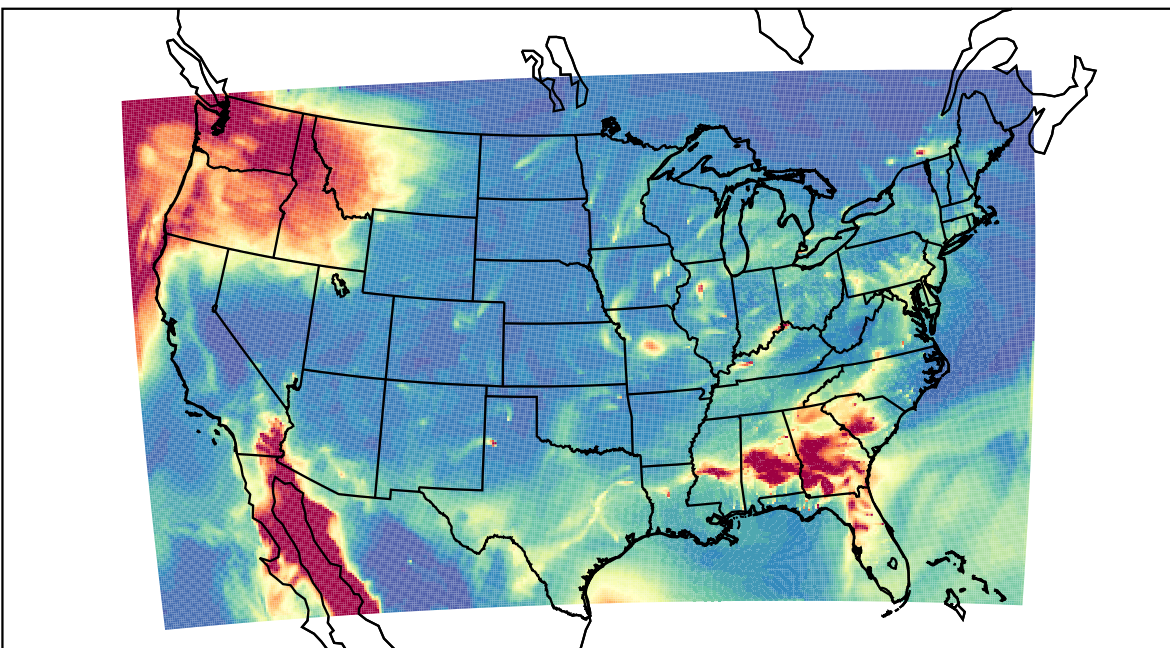
WRF 2021-02-26_09:00:00
