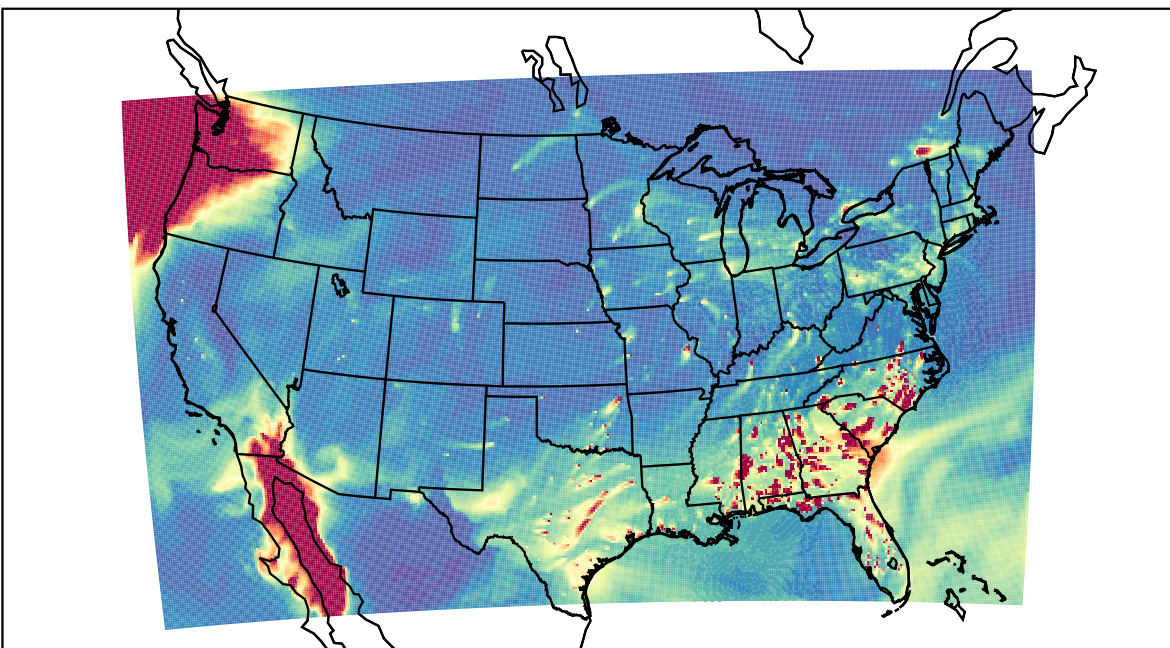
WRF 2021-02-25_23:00:00
