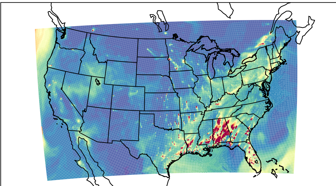
WRF 2021-02-25_00:00:00
