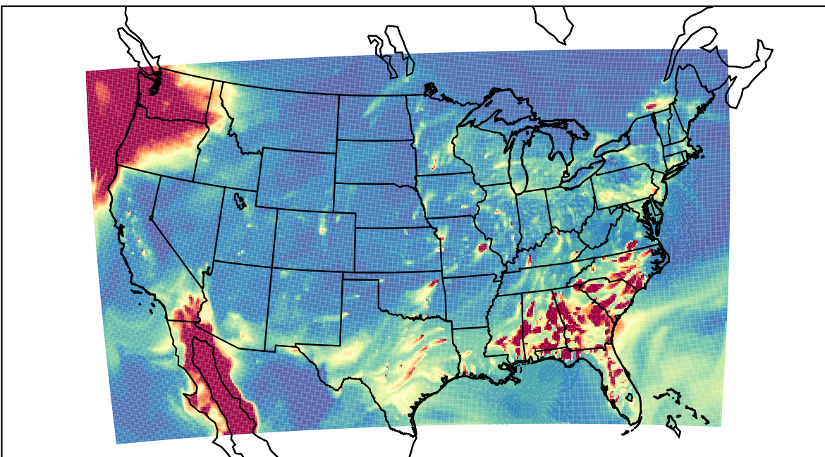
WRF 2021-02-26_02:00:00
