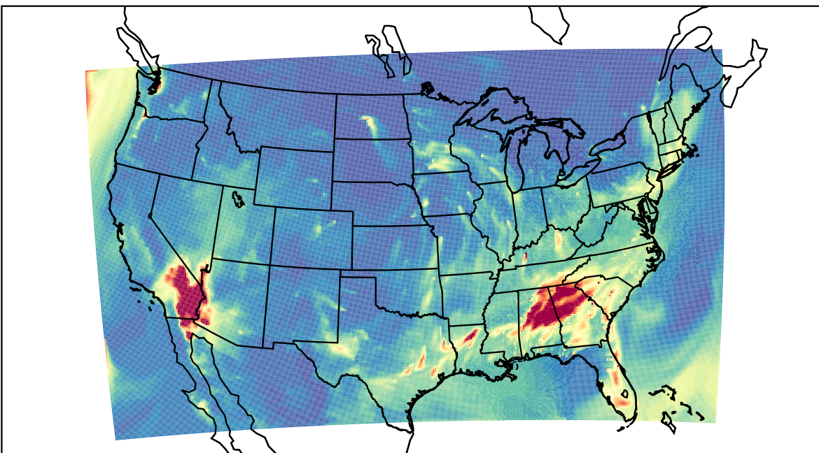
WRF 2021-02-25_07:00:00
