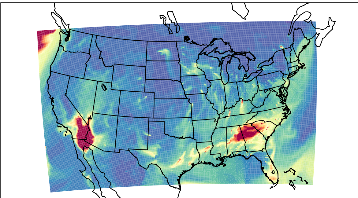
WRF 2021-02-25_10:00:00
