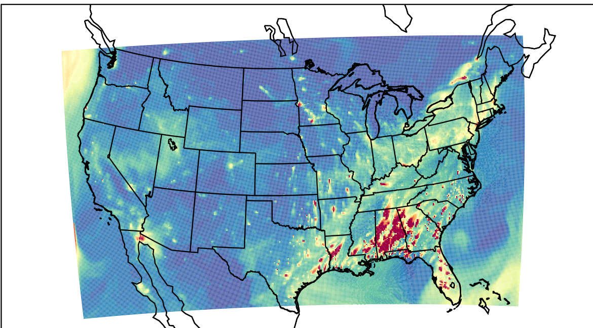
WRF 2021-02-25_01:00:00
