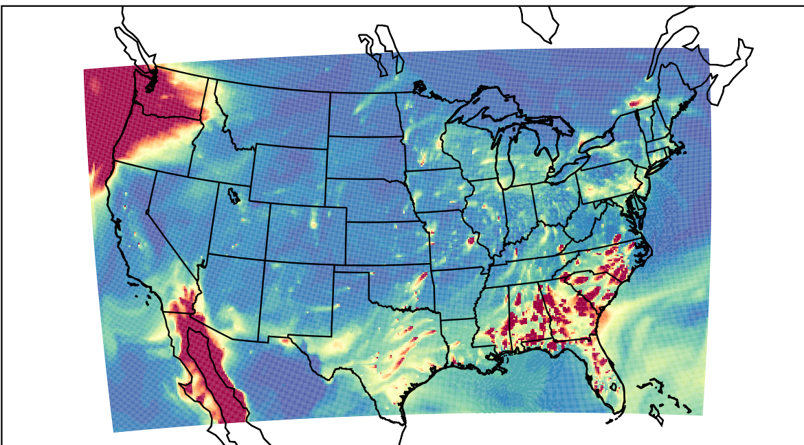
WRF 2021-02-26_01:00:00
