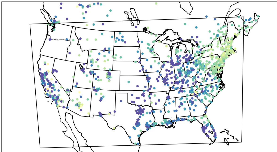
AirNOW (2021-03-02_12:00:00)
