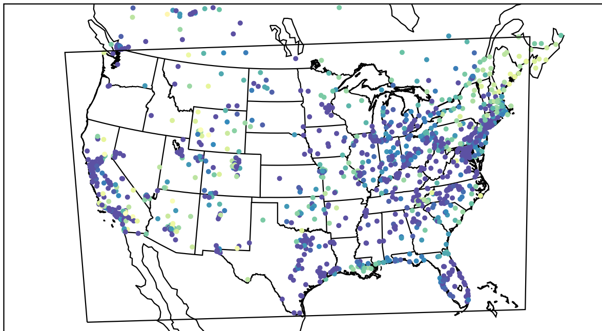
AirNOW (2021-03-03_12:00:00)
