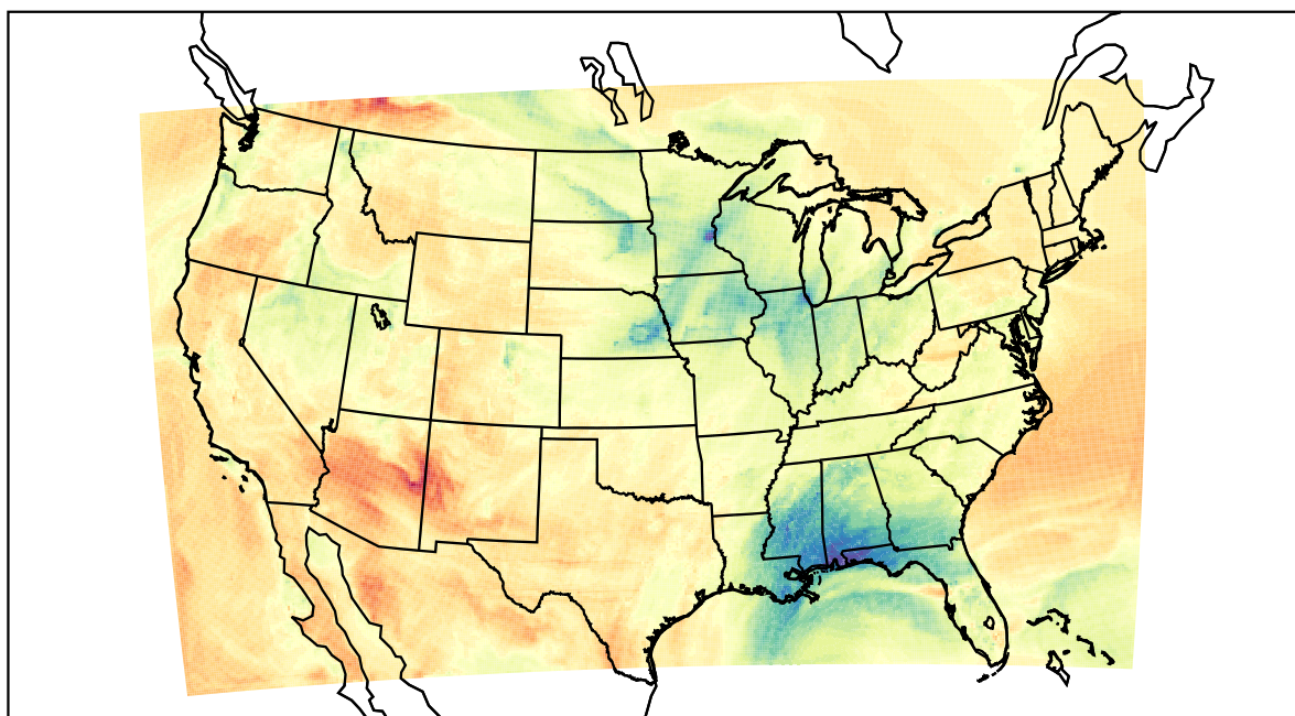
WRF (2021-03-02_22:00:00)
