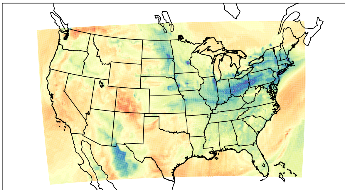
WRF (2021-03-03_23:00:00)
