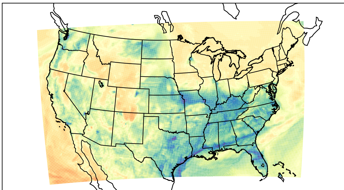
WRF (2021-03-02_05:00:00)
