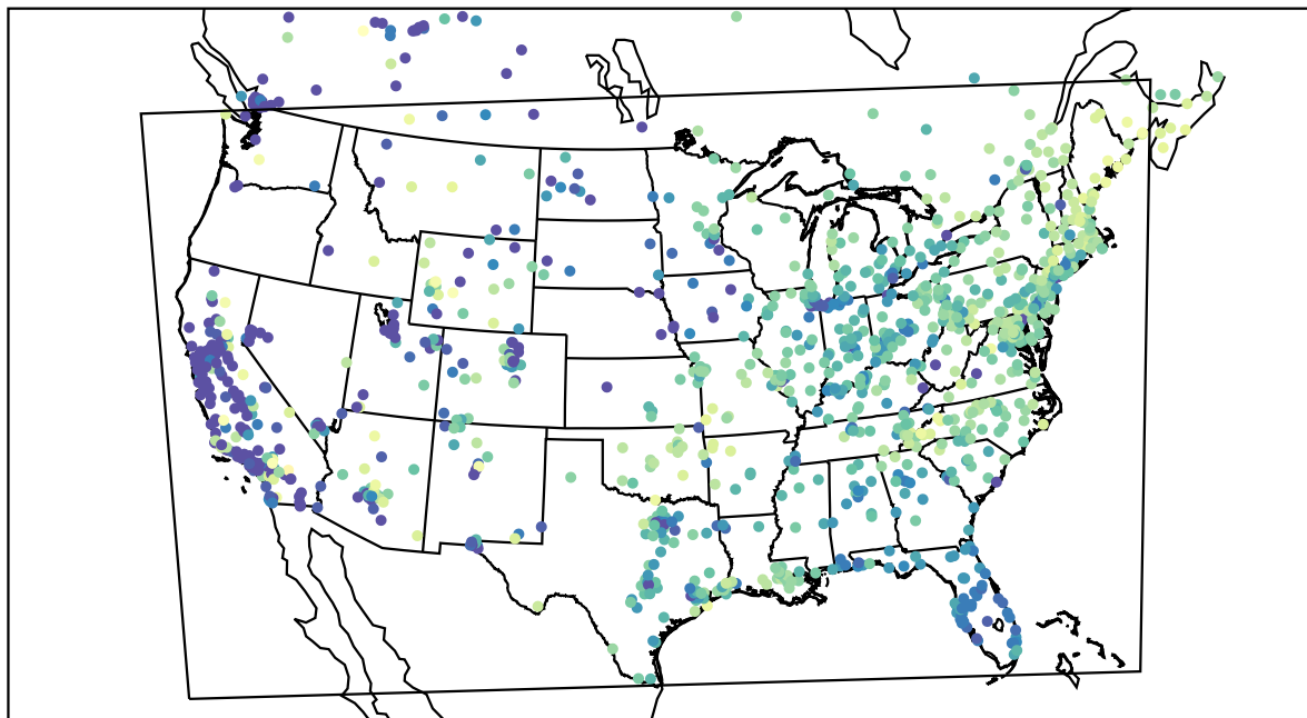
AirNOW (2021-03-03_15:00:00)
