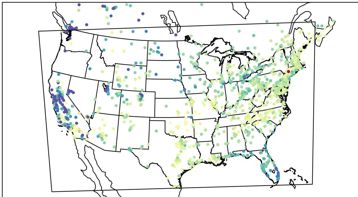
AirNOW (2021-03-03_17:00:00)
