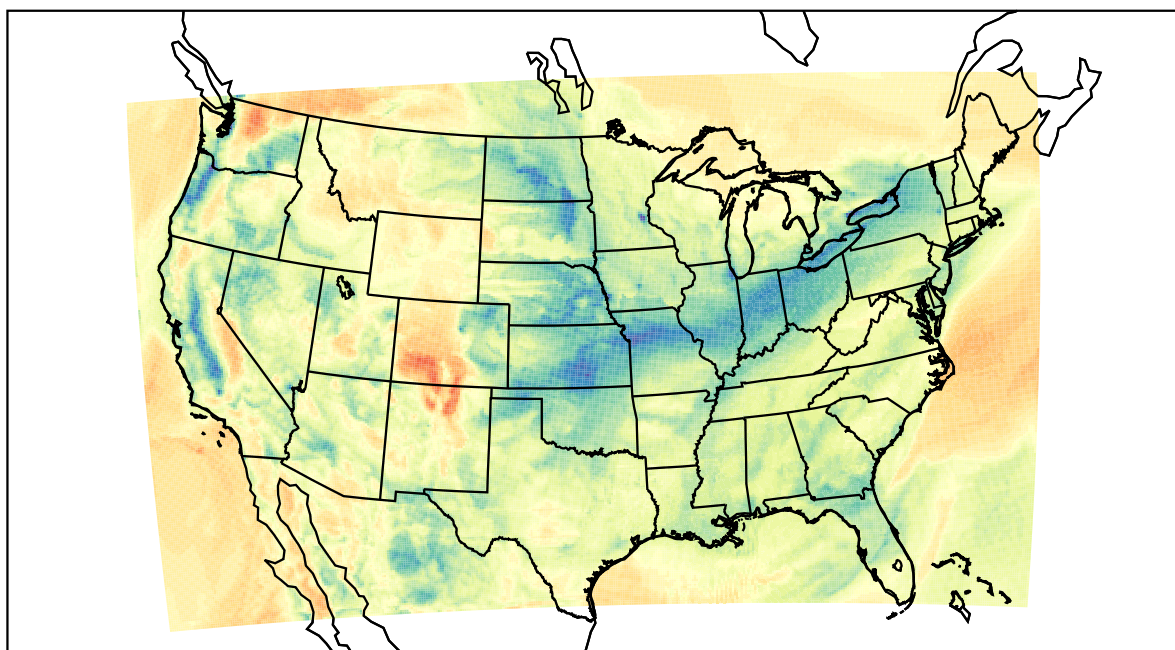
WRF (2021-03-03_17:00:00)
