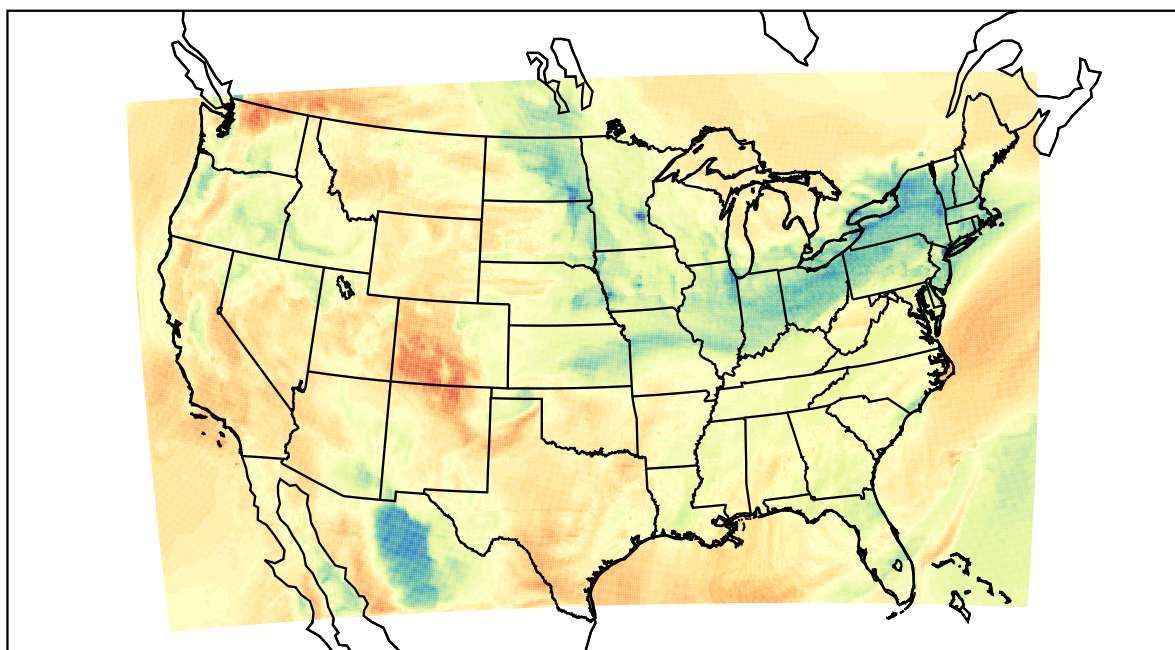
WRF (2021-03-03_21:00:00)
