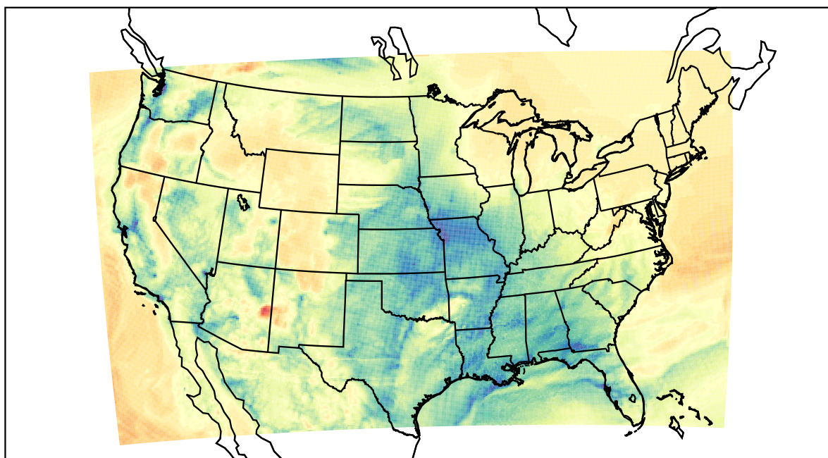
WRF (2021-03-02_15:00:00)
