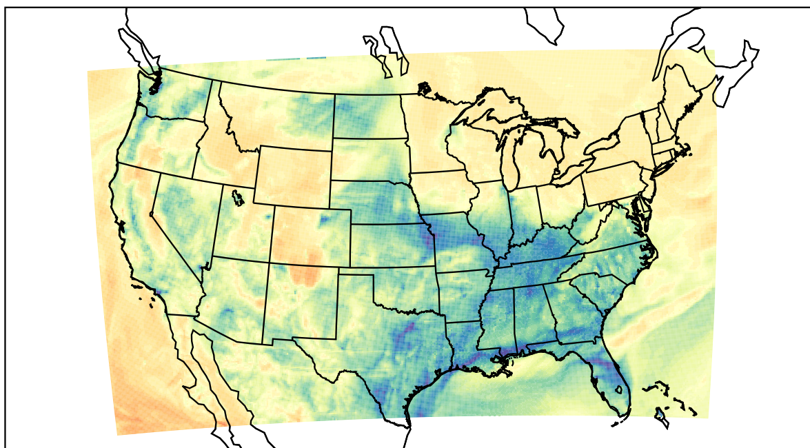
WRF (2021-03-02_07:00:00)
