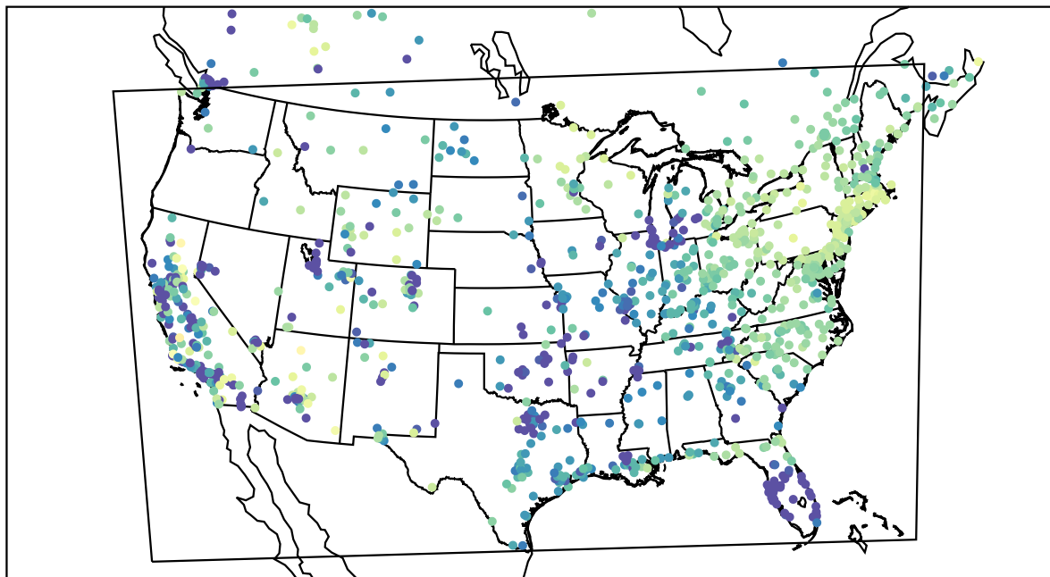
AirNOW (2021-03-02_06:00:00)
