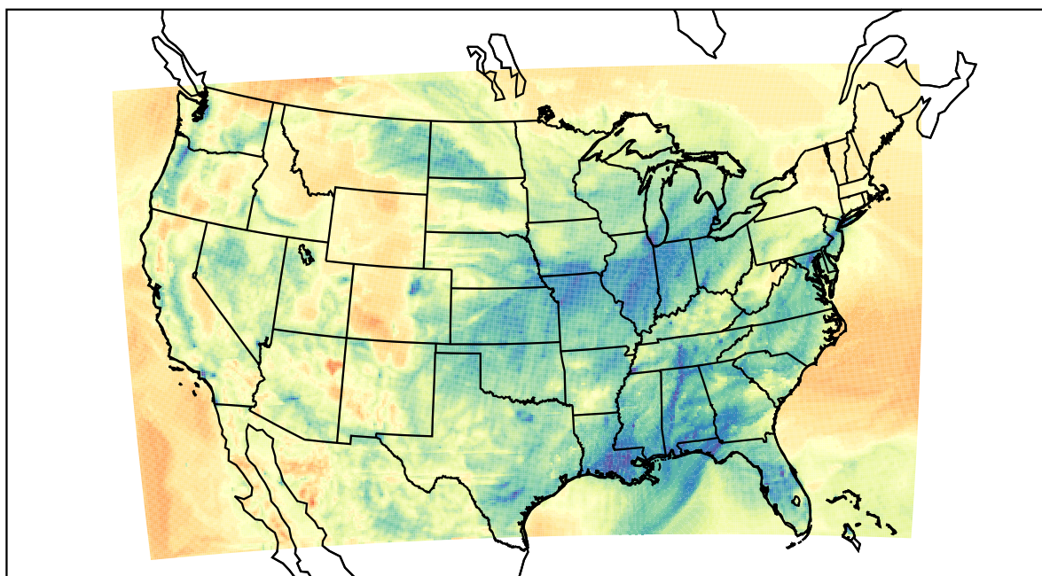
WRF (2021-03-03_05:00:00)
