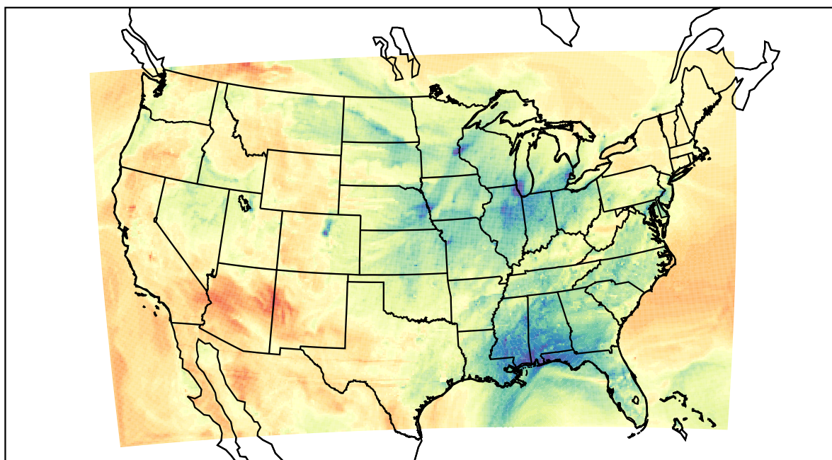
WRF (2021-03-03_00:00:00)
