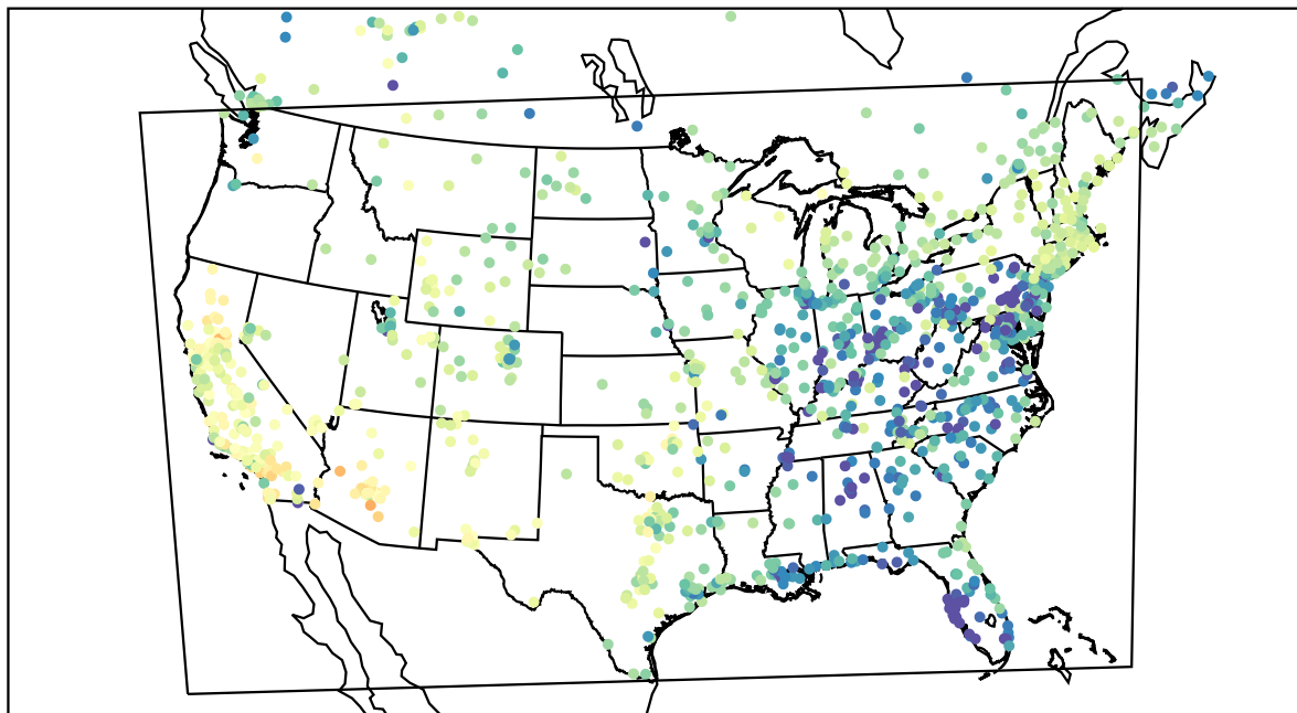
AirNOW (2021-03-03_00:00:00)
