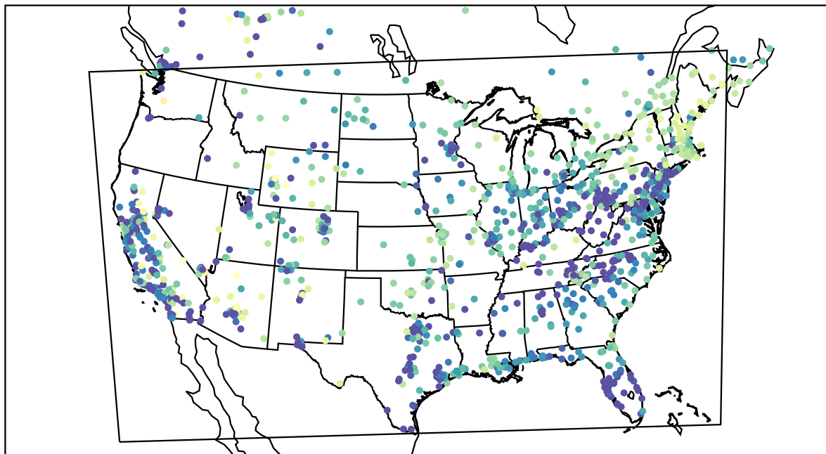
AirNOW (2021-03-03_05:00:00)
