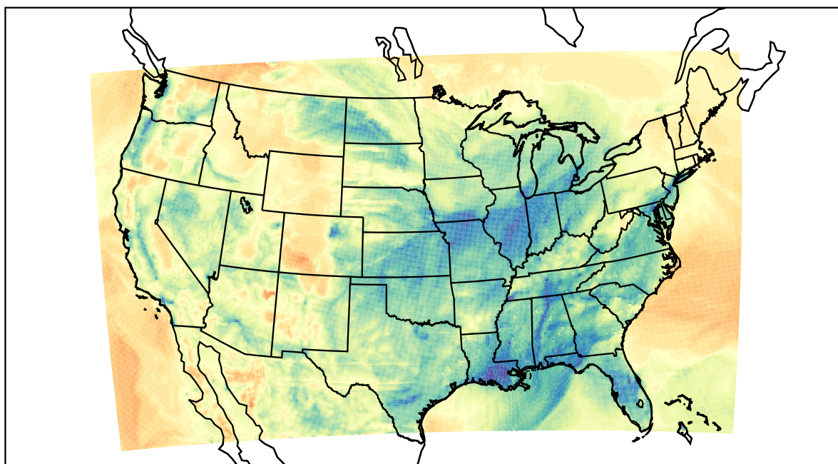
WRF (2021-03-03_06:00:00)
