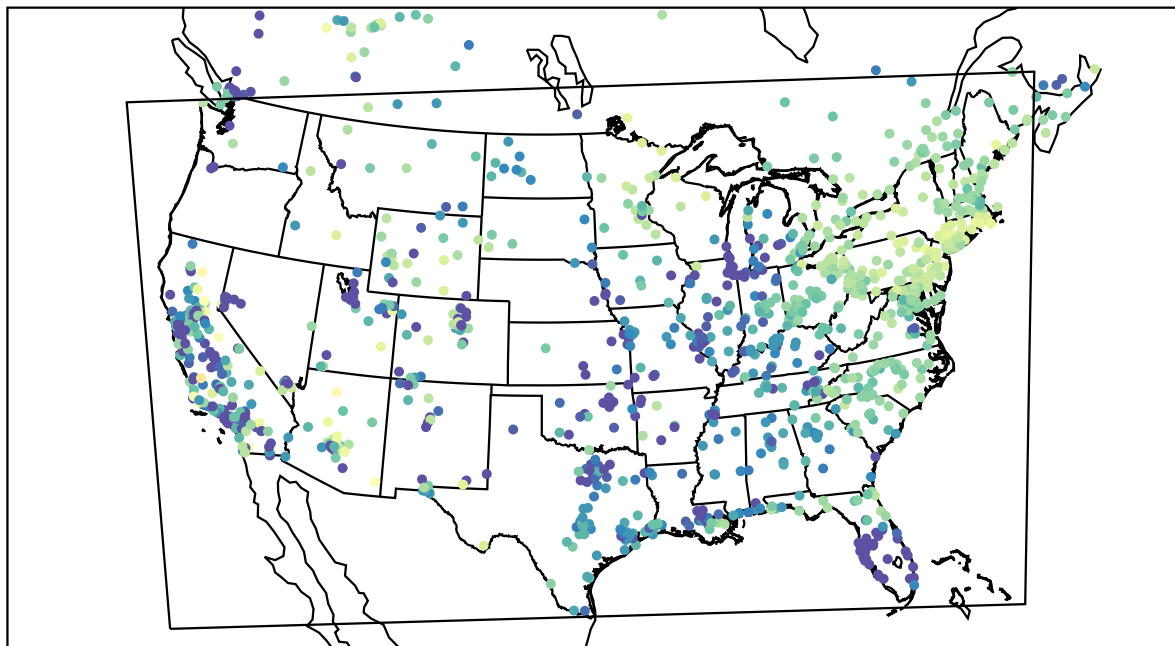
AirNOW (2021-03-02_07:00:00)
