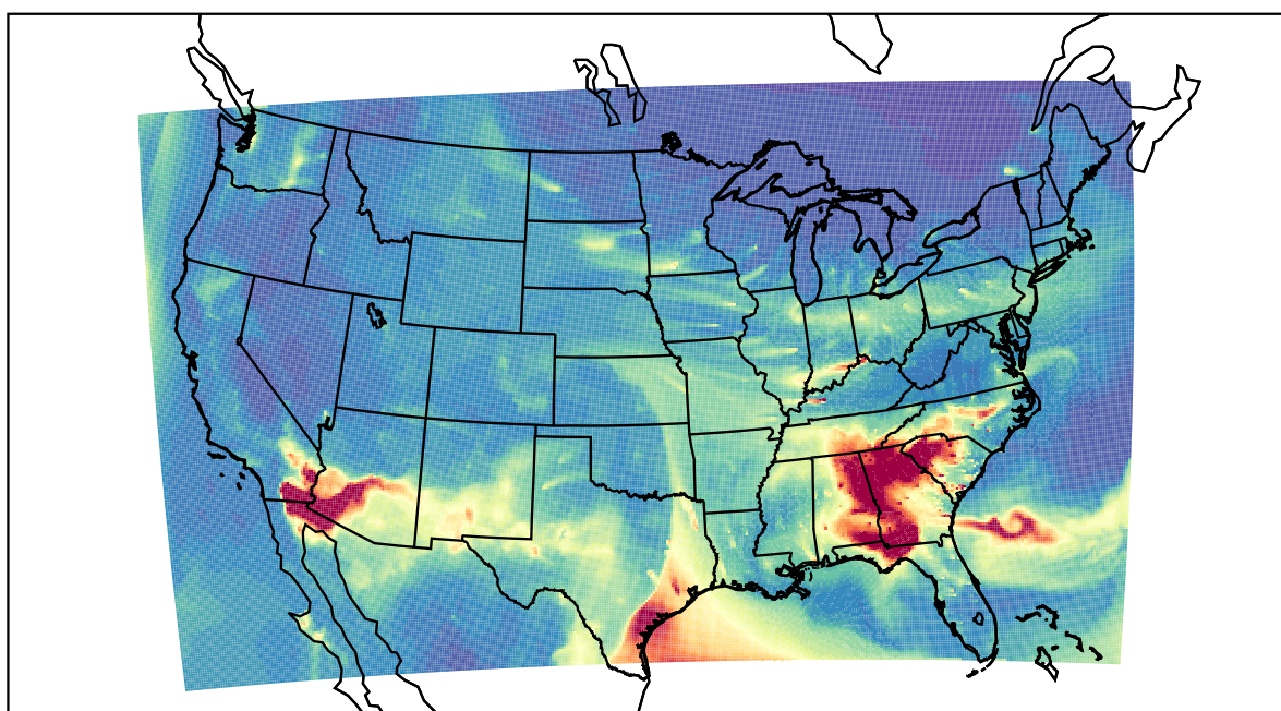
WRF 2021-03-14_13:00:00
