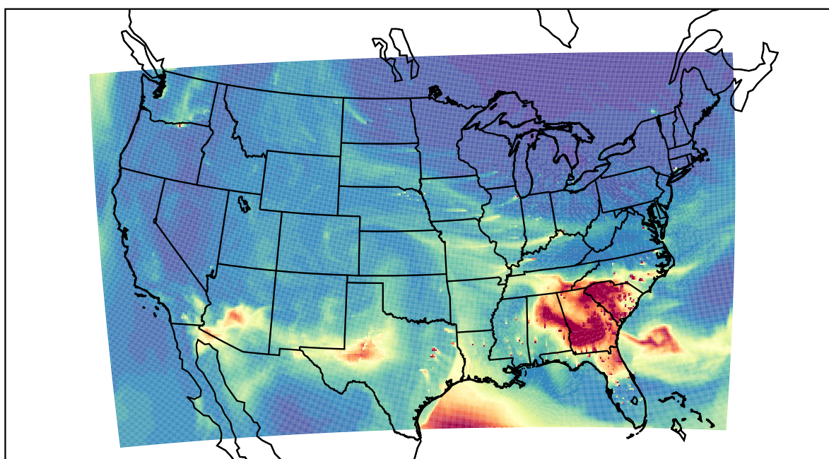
WRF 2021-03-14_19:00:00
