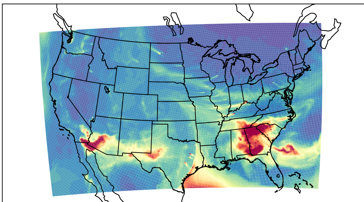
WRF 2021-03-14_16:00:00
