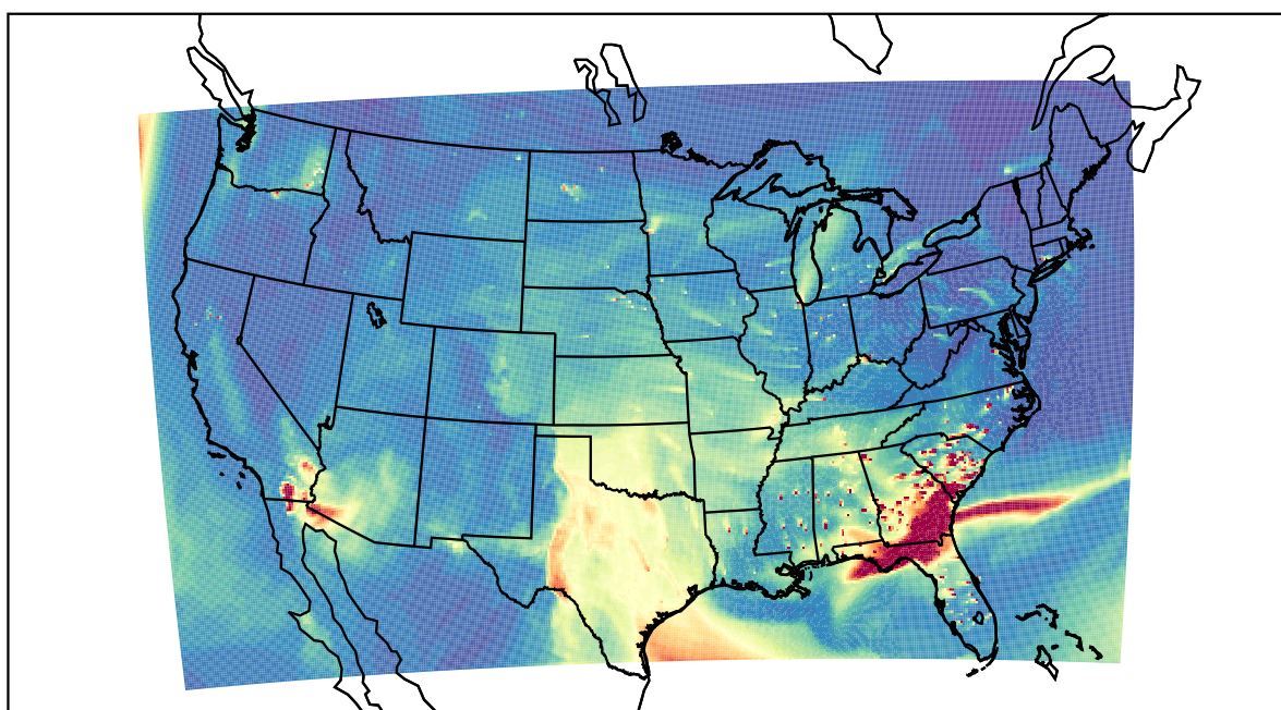
WRF 2021-03-13_21:00:00
