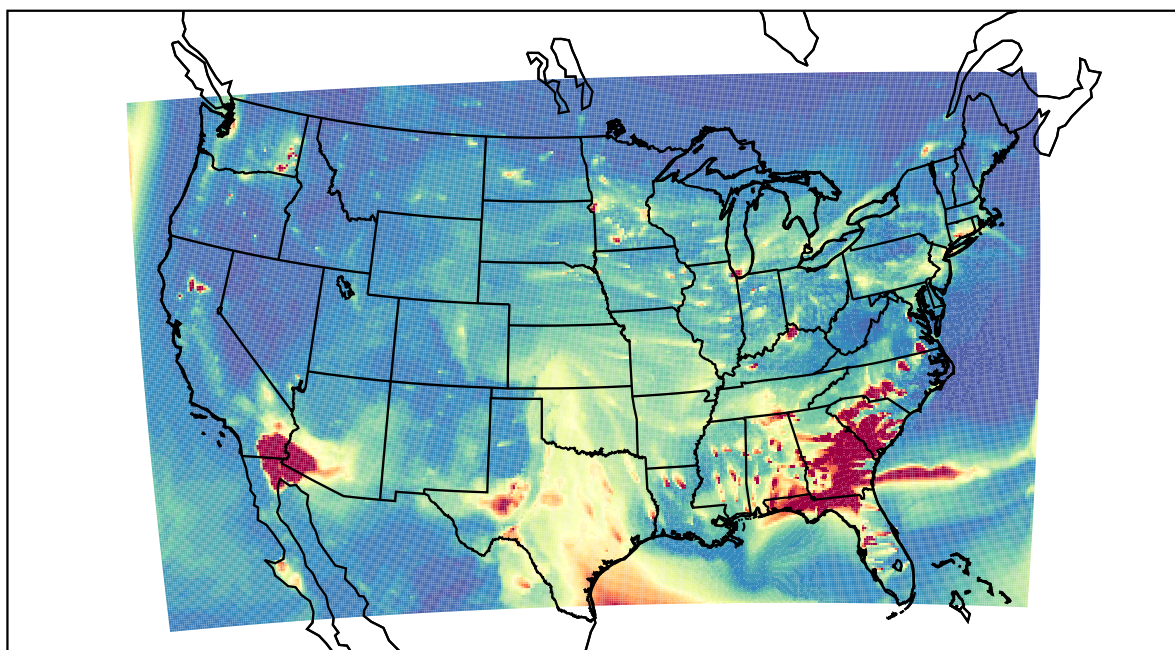
WRF 2021-03-14_02:00:00
