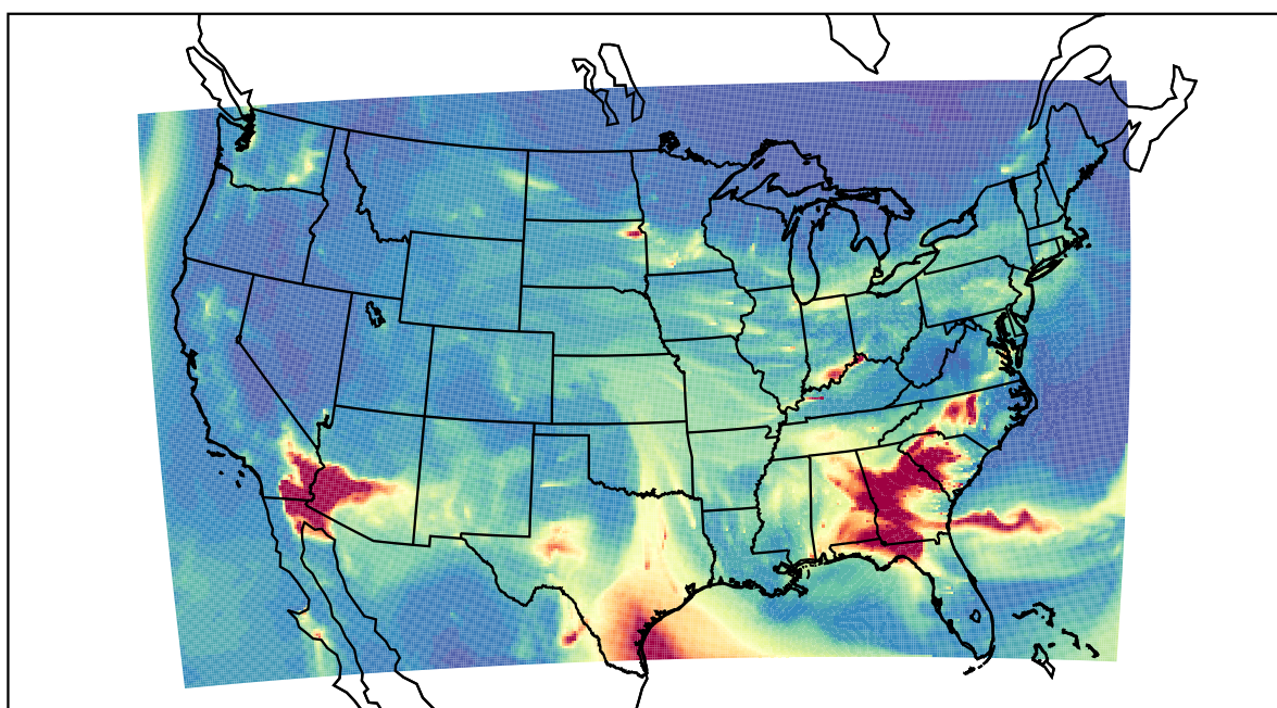
WRF 2021-03-14_08:00:00
