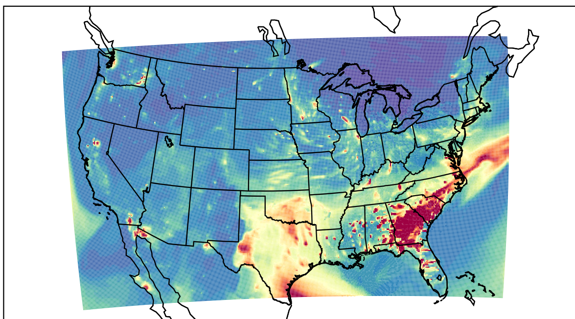
WRF 2021-03-13_02:00:00
