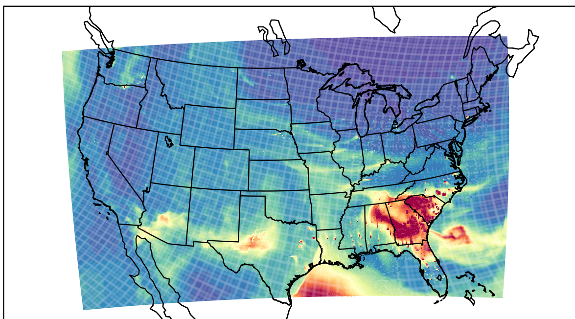
WRF 2021-03-14_20:00:00
