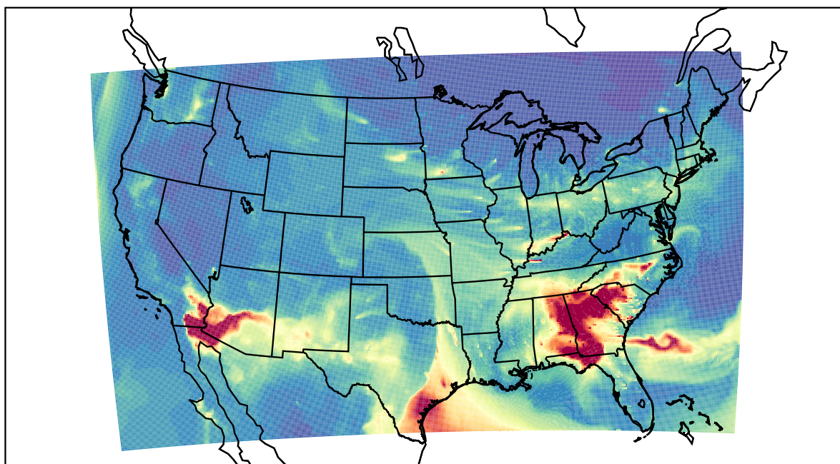
WRF 2021-03-14_12:00:00
