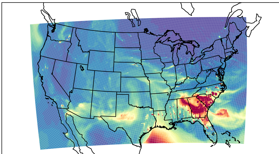
WRF 2021-03-14_22:00:00
