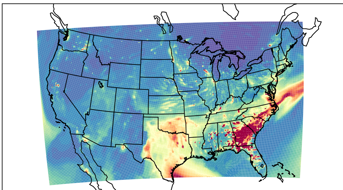
WRF 2021-03-13_01:00:00
