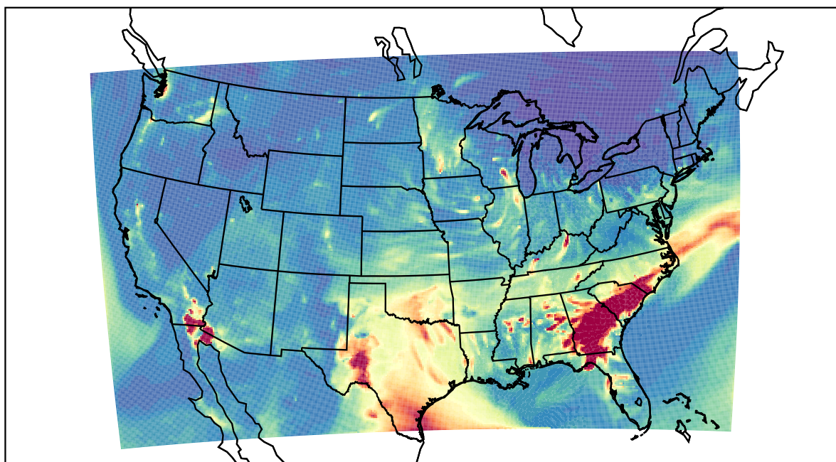
WRF 2021-03-13_05:00:00
