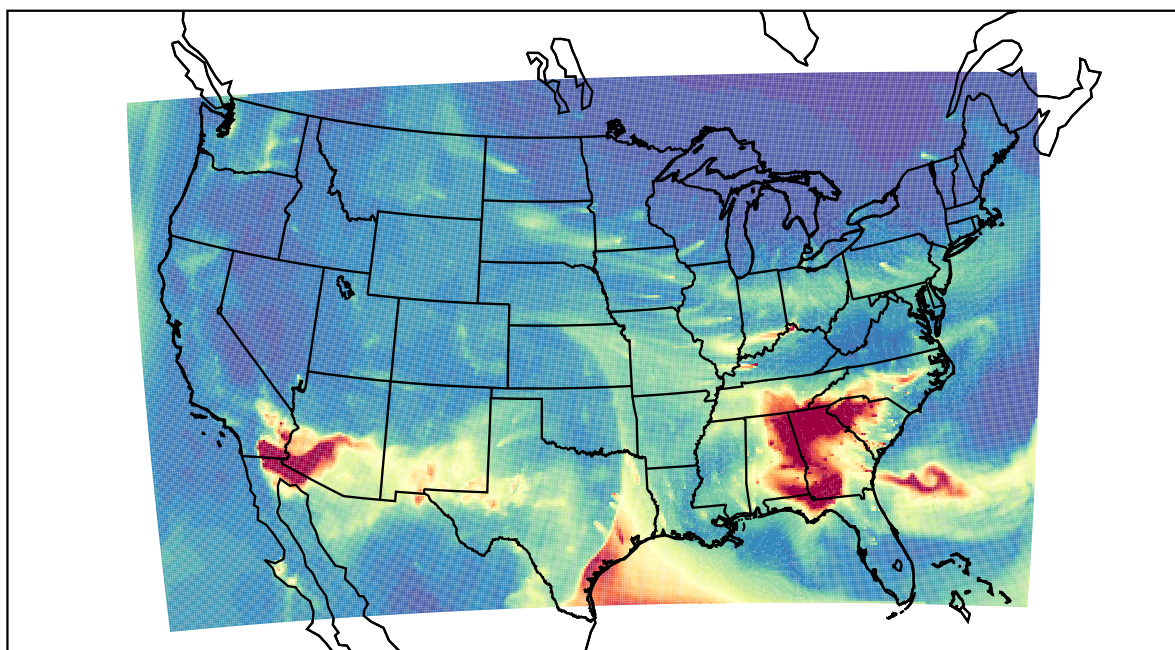
WRF 2021-03-14_14:00:00
