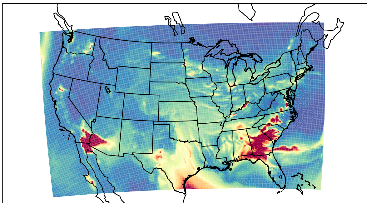
WRF 2021-03-14_05:00:00
