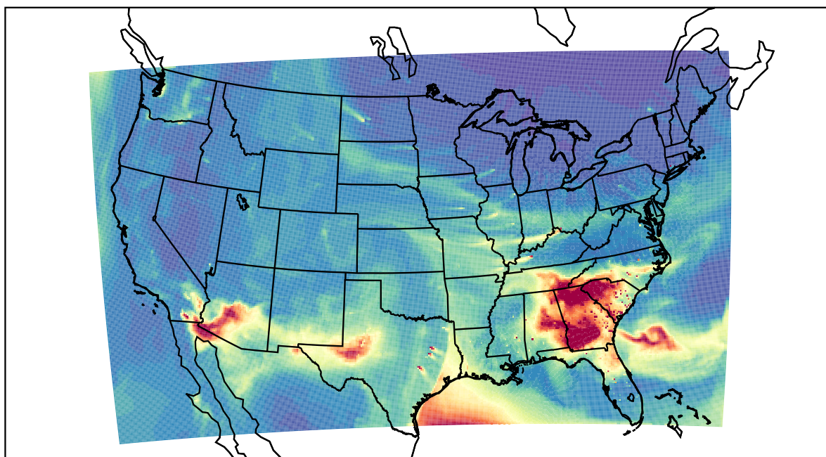
WRF 2021-03-14_17:00:00
