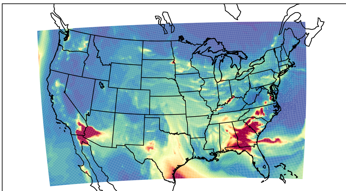
WRF 2021-03-14_06:00:00
