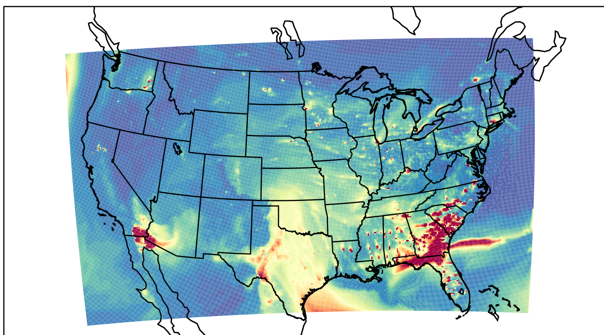
WRF 2021-03-14_00:00:00
