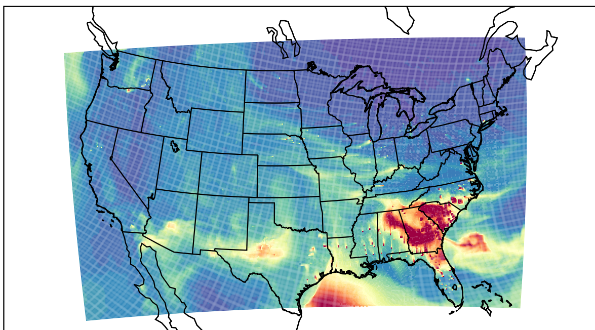
WRF 2021-03-14_21:00:00
