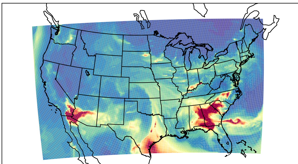
WRF 2021-03-14_10:00:00
