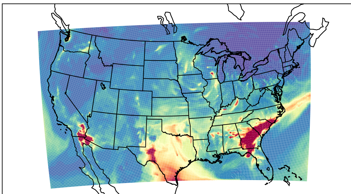
WRF 2021-03-13_07:00:00
