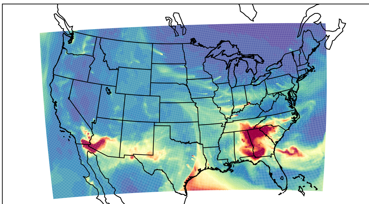
WRF 2021-03-14_15:00:00
