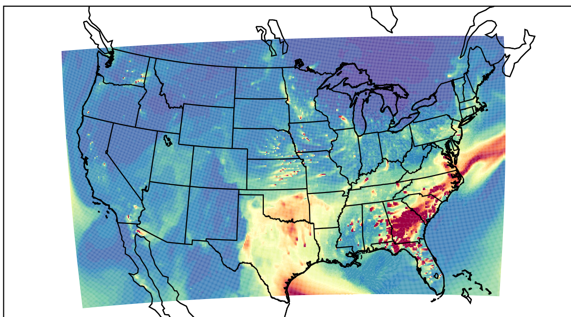
WRF 2021-03-13_00:00:00
