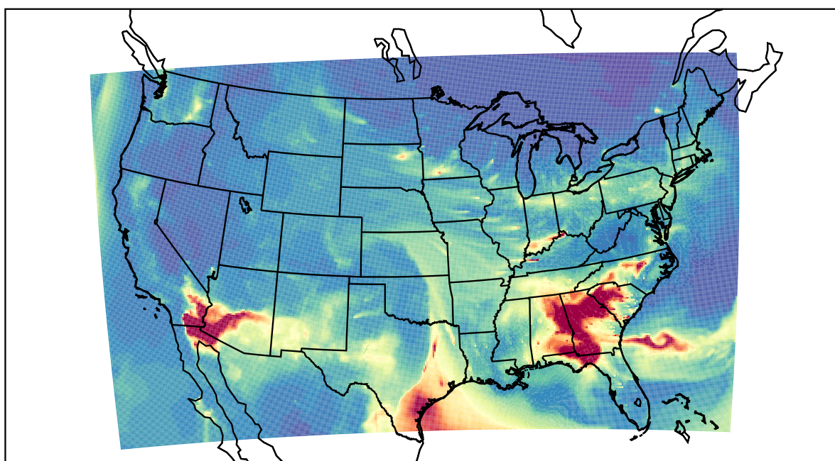
WRF 2021-03-14_11:00:00
