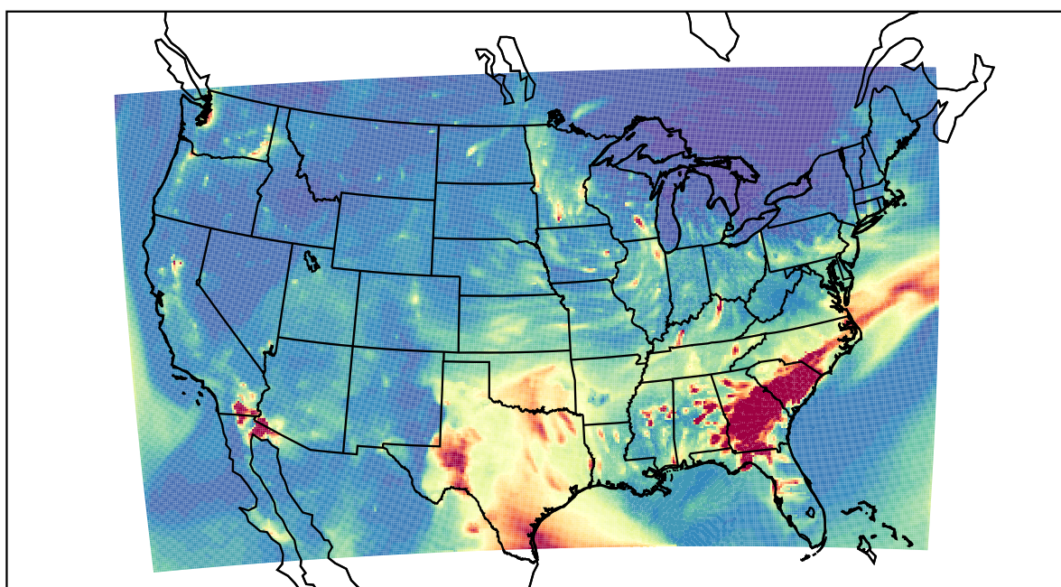
WRF 2021-03-13_04:00:00
