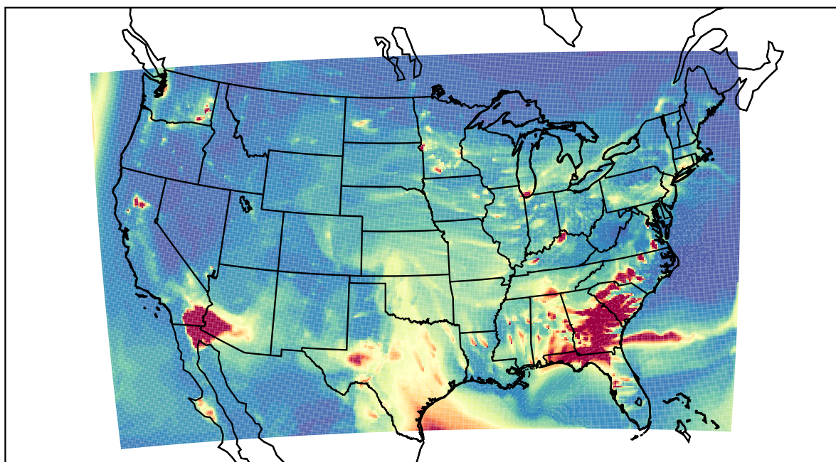
WRF 2021-03-14_03:00:00
