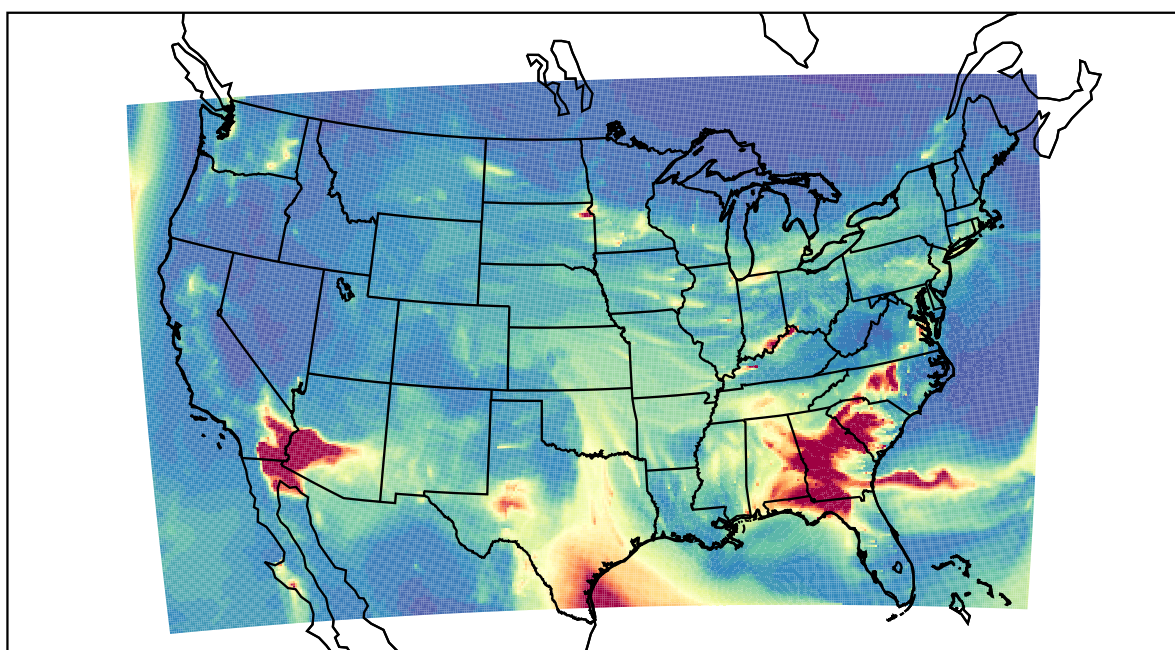
WRF 2021-03-14_07:00:00
