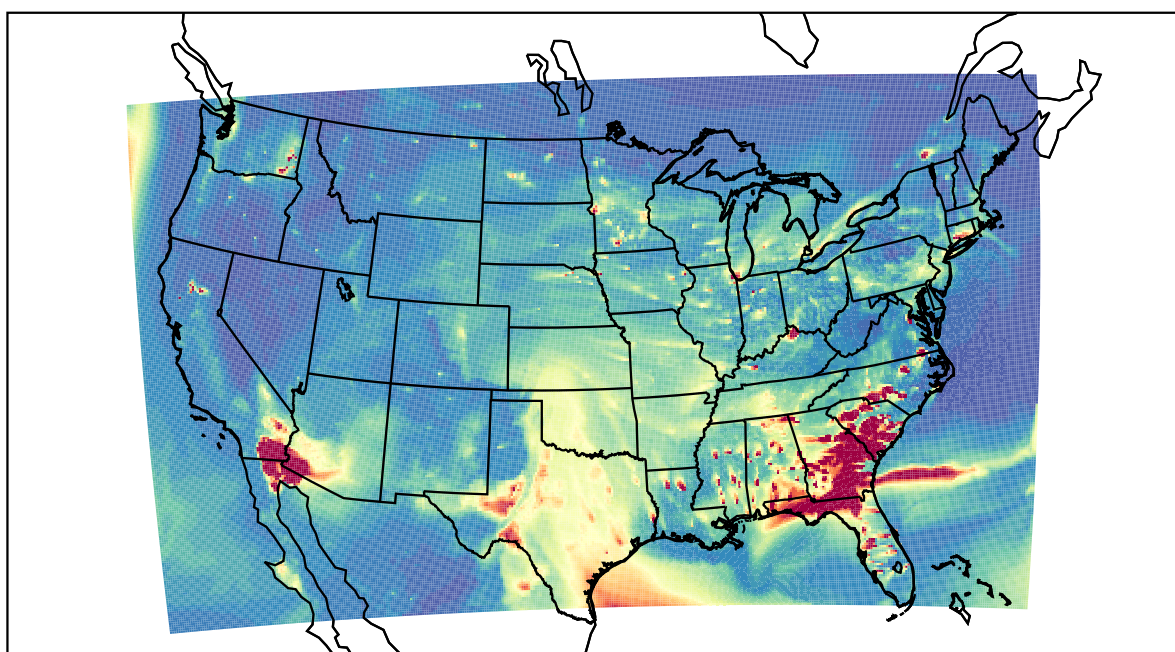
WRF 2021-03-14_01:00:00
