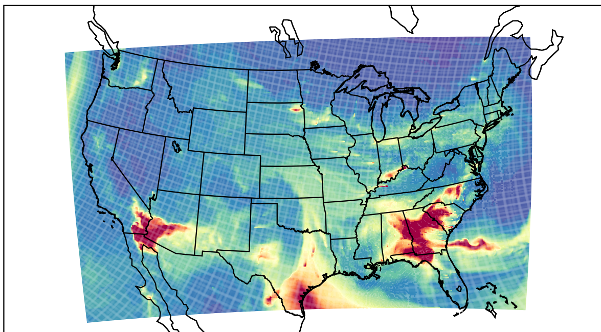
WRF 2021-03-14_09:00:00
