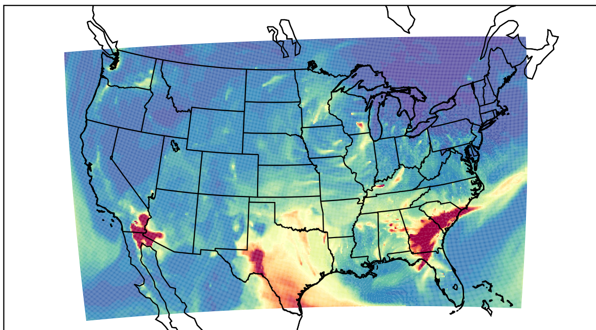
WRF 2021-03-13_09:00:00
