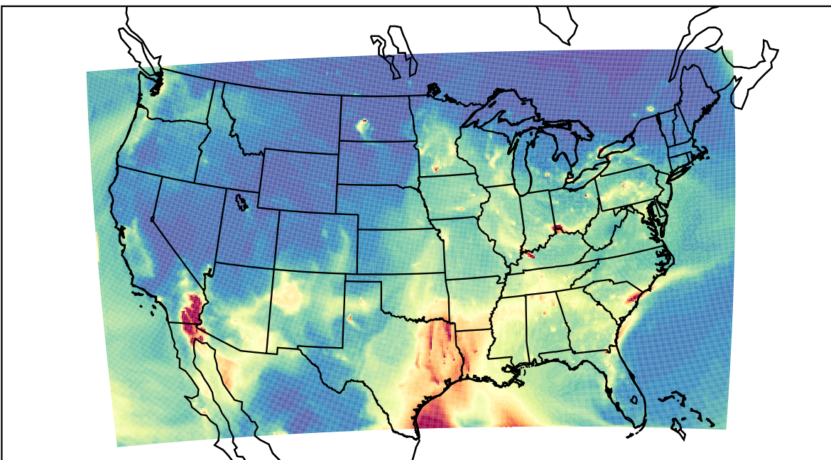
WRF 2021-03-27_13:00:00
