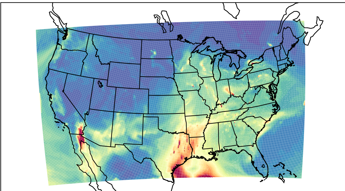
WRF 2021-03-27_17:00:00
