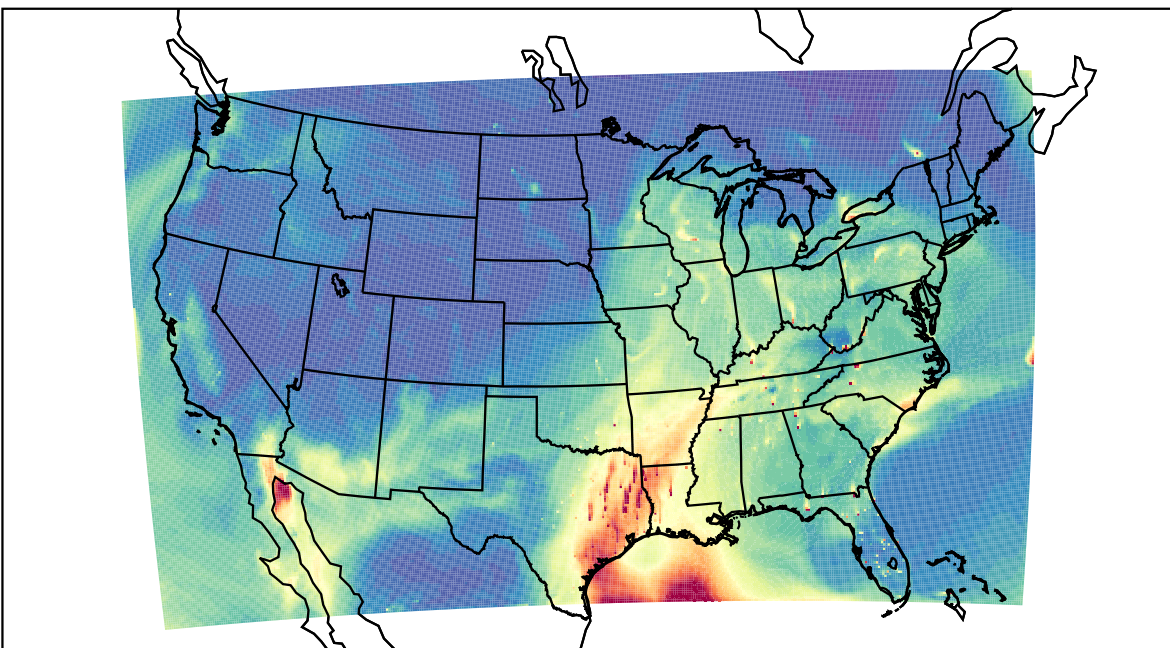
WRF 2021-03-27_20:00:00
