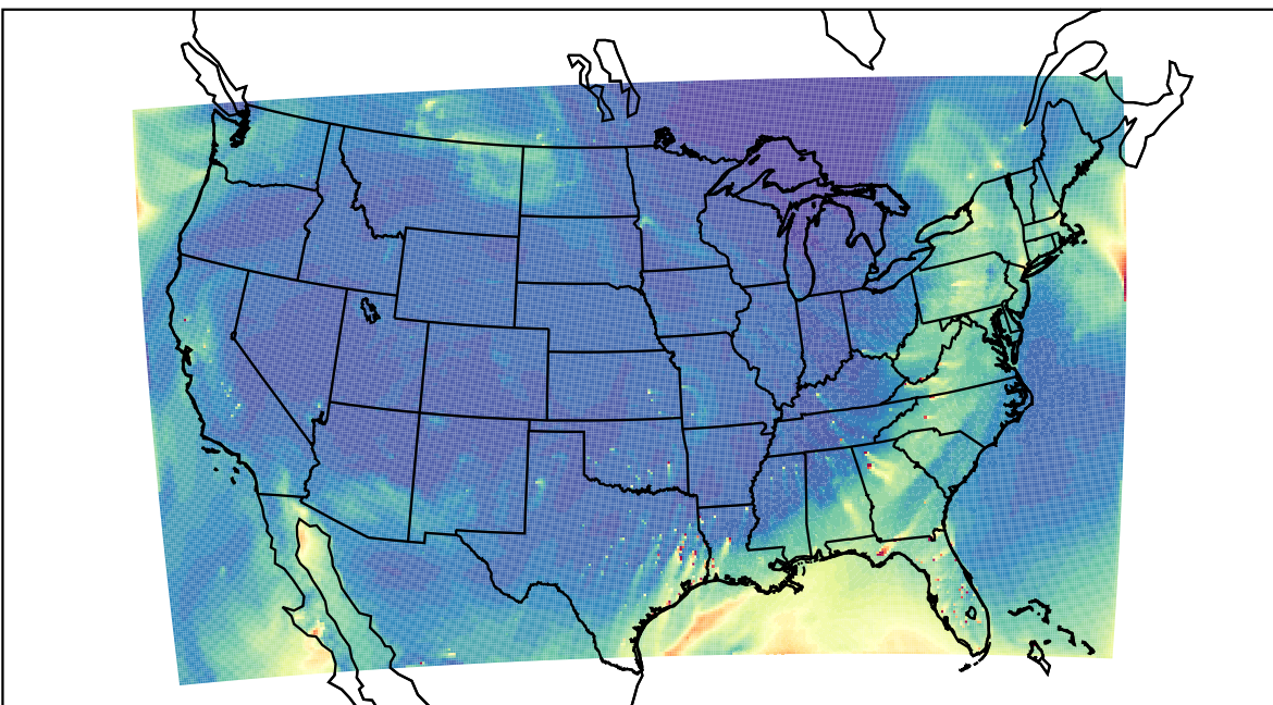
WRF 2021-03-28_22:00:00
