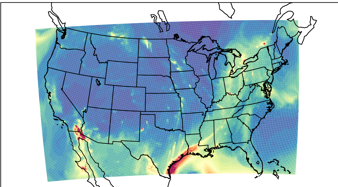
WRF 2021-03-28_14:00:00
