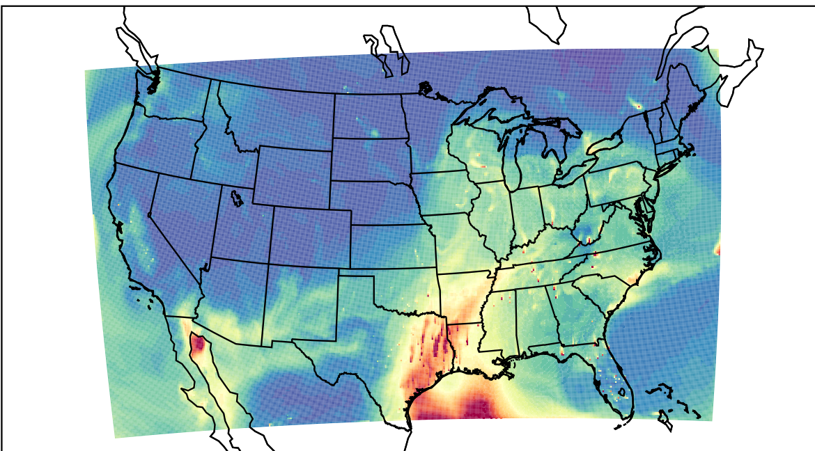
WRF 2021-03-27_21:00:00
