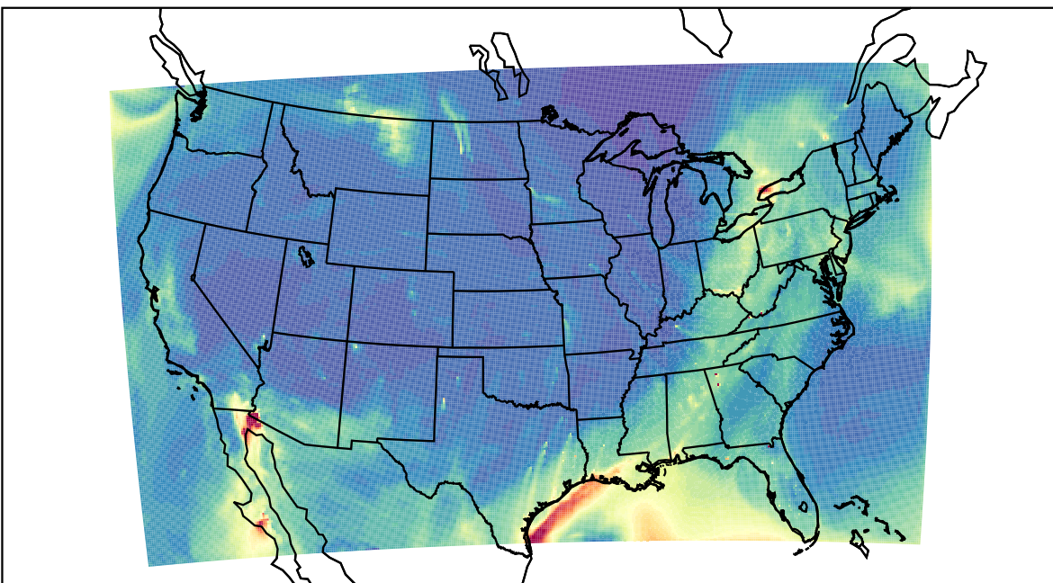
WRF 2021-03-28_17:00:00
