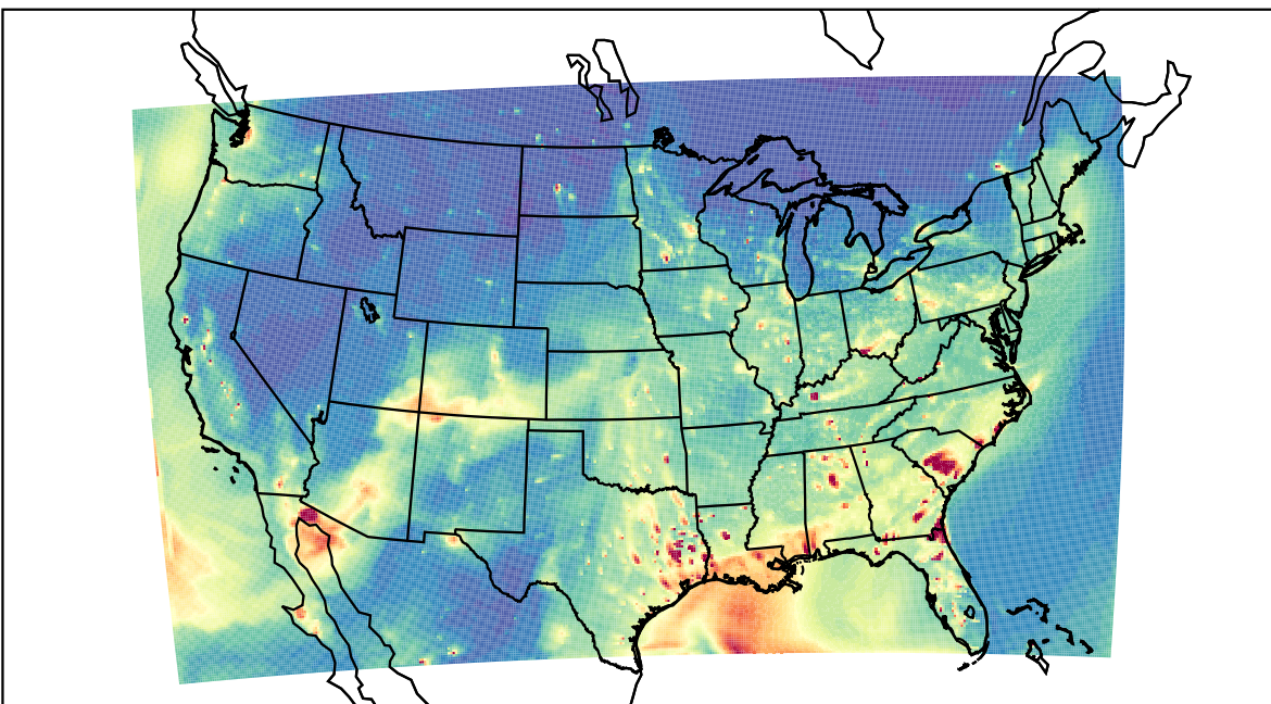
WRF 2021-03-27_02:00:00
