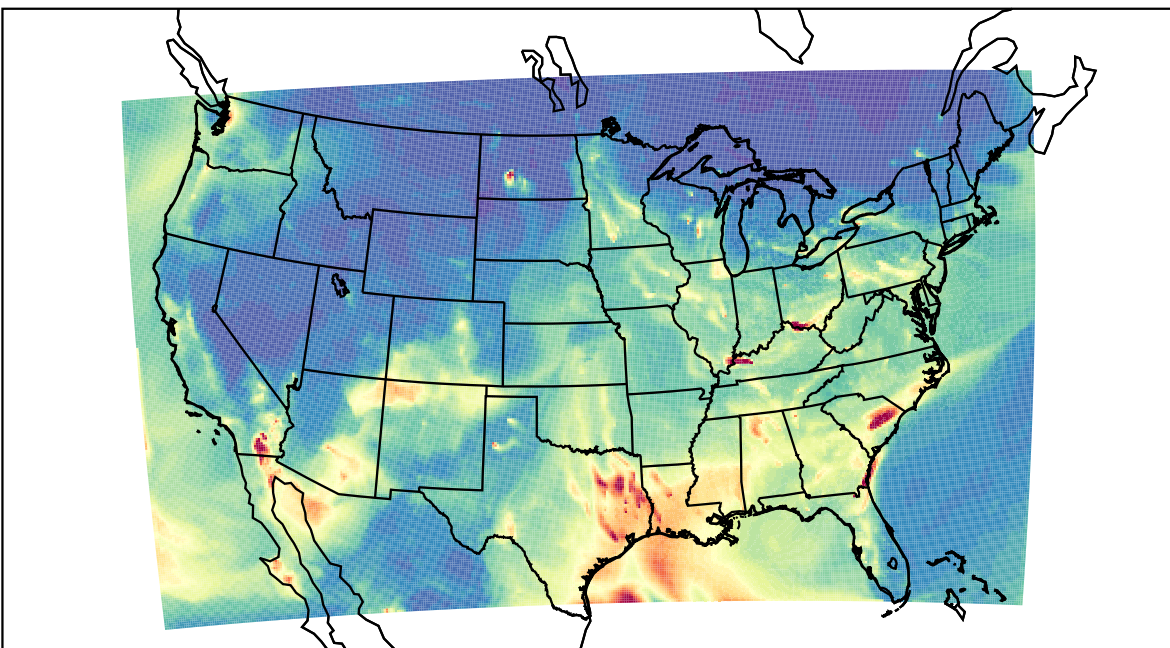
WRF 2021-03-27_07:00:00
