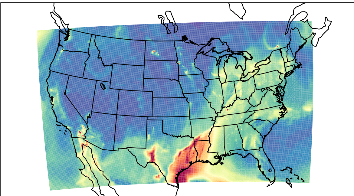
WRF 2021-03-28_07:00:00
