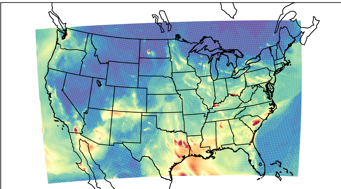
WRF 2021-03-27_06:00:00
