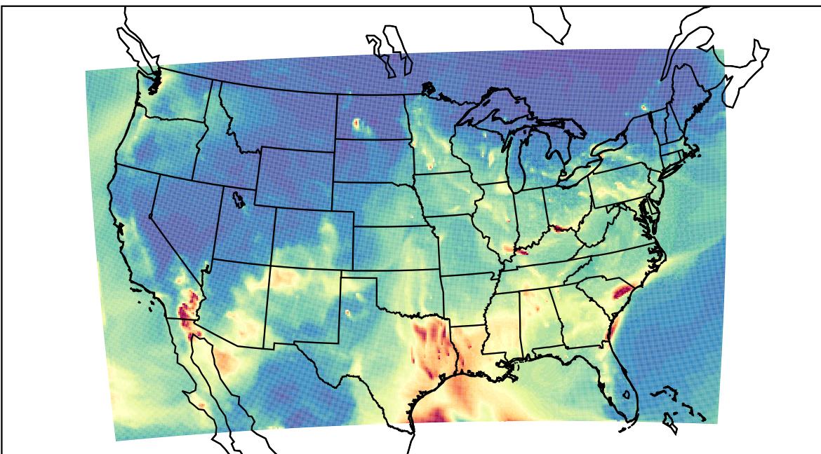
WRF 2021-03-27_09:00:00
