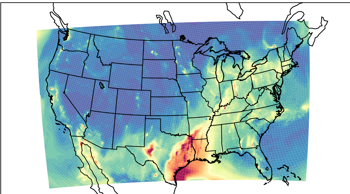
WRF 2021-03-28_05:00:00
