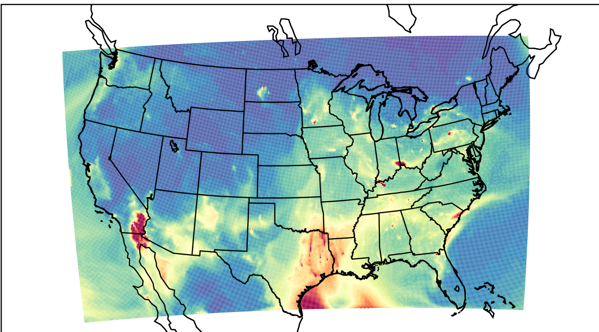
WRF 2021-03-27_14:00:00
