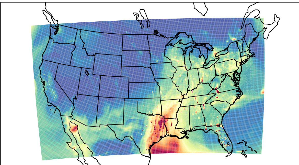
WRF 2021-03-28_00:00:00
