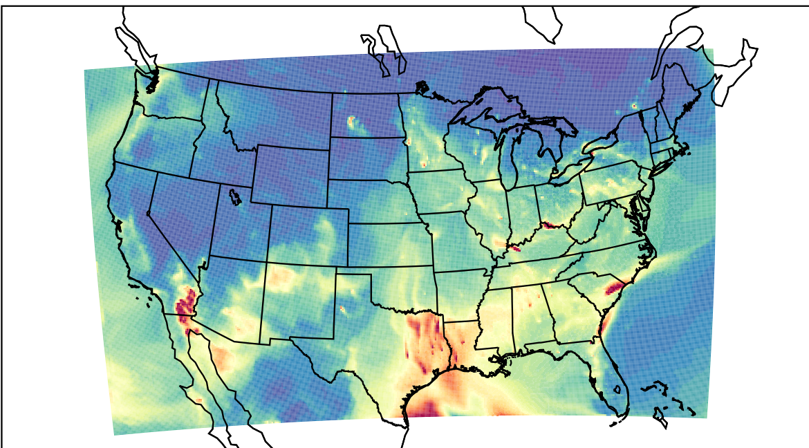
WRF 2021-03-27_10:00:00
