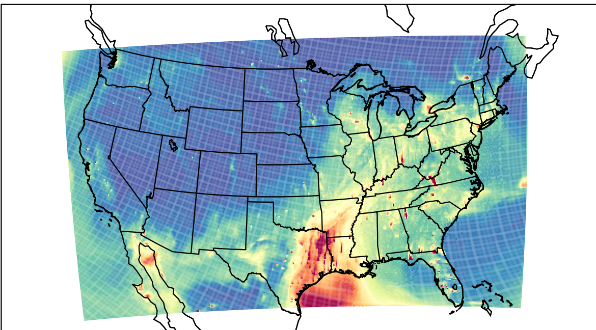
WRF 2021-03-28_01:00:00
