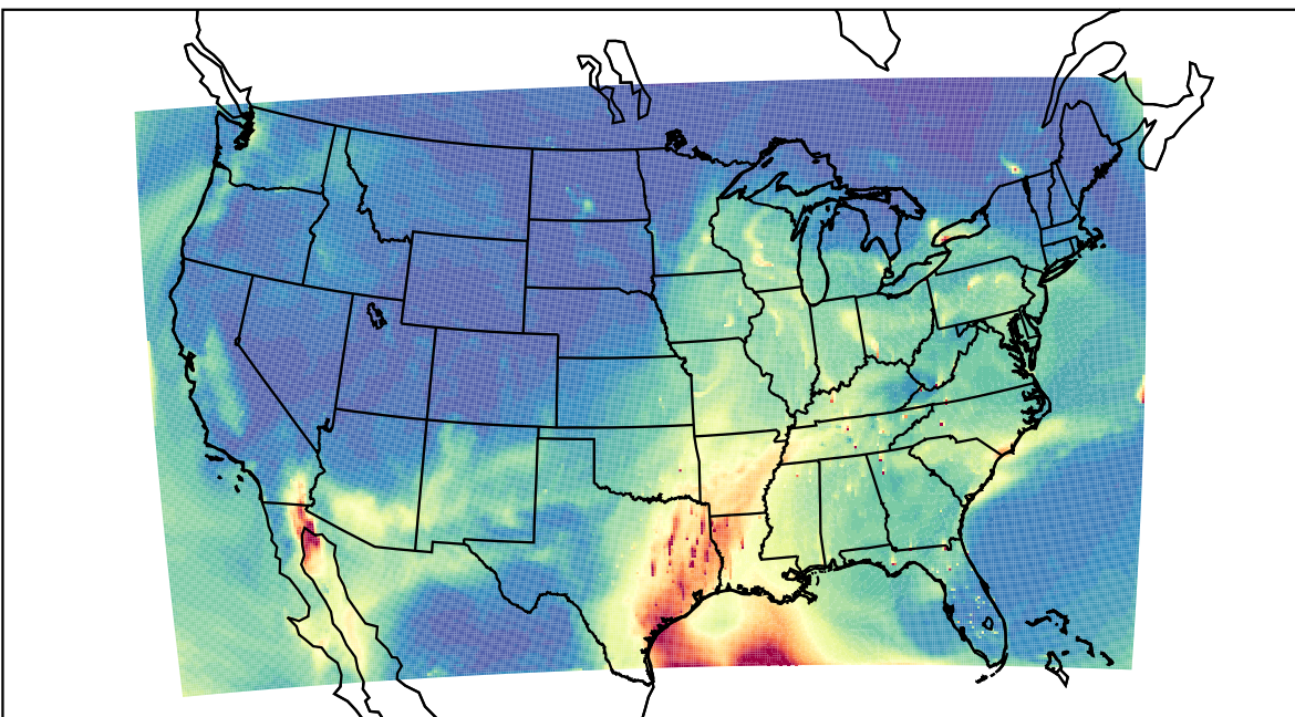
WRF 2021-03-27_19:00:00
