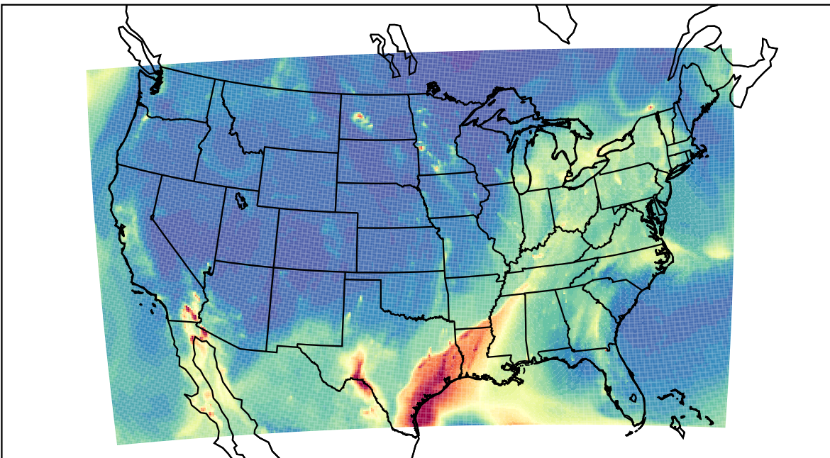
WRF 2021-03-28_09:00:00
