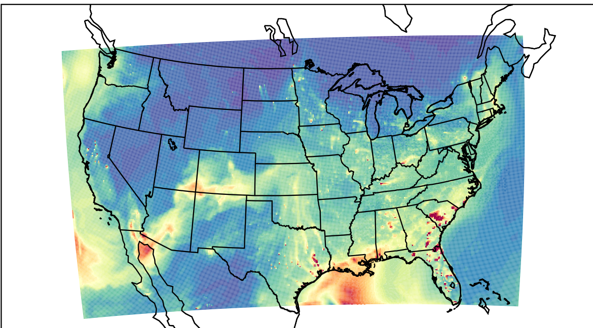
WRF 2021-03-27_00:00:00
