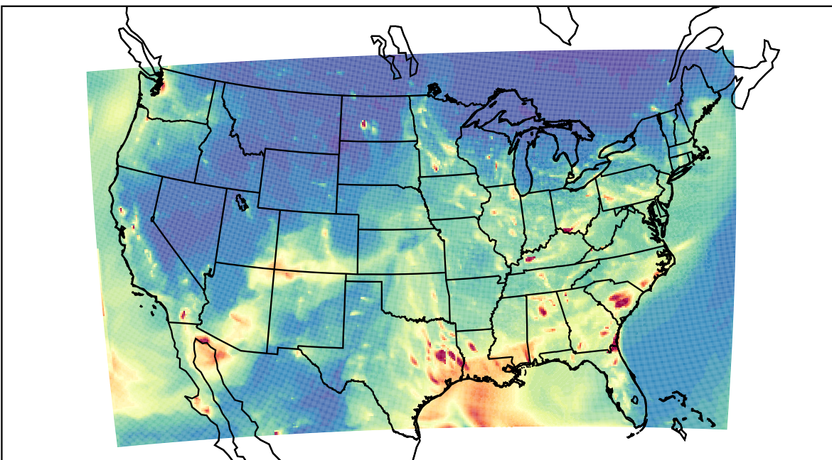
WRF 2021-03-27_04:00:00
