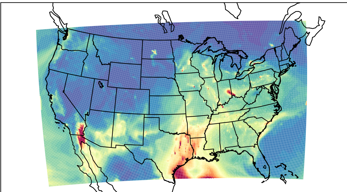
WRF 2021-03-27_16:00:00
