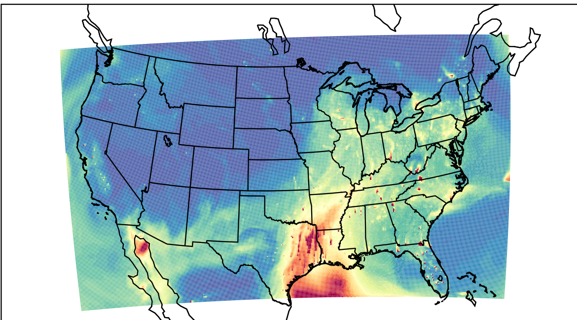
WRF 2021-03-27_23:00:00
