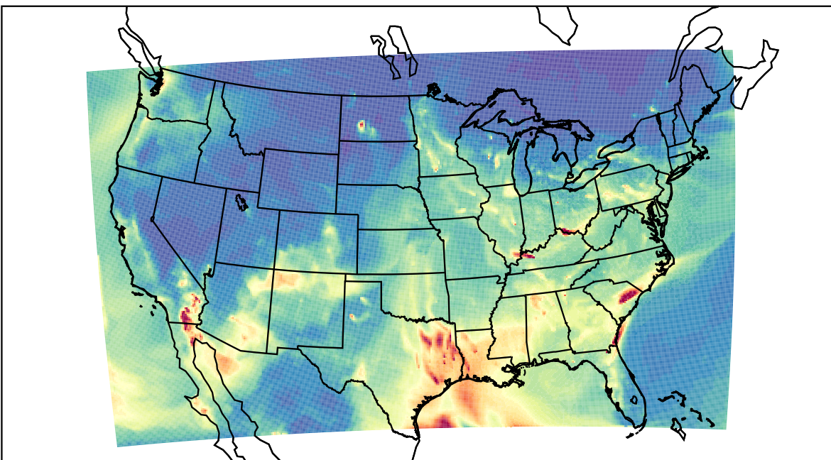
WRF 2021-03-27_08:00:00
