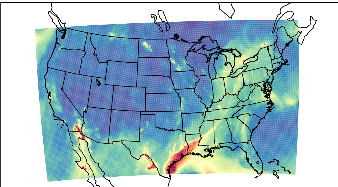
WRF 2021-03-28_12:00:00
