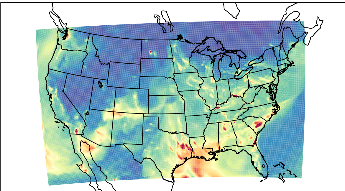
WRF 2021-03-27_05:00:00
