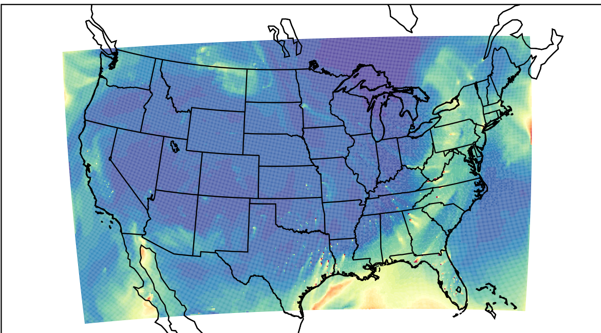
WRF 2021-03-28_21:00:00
