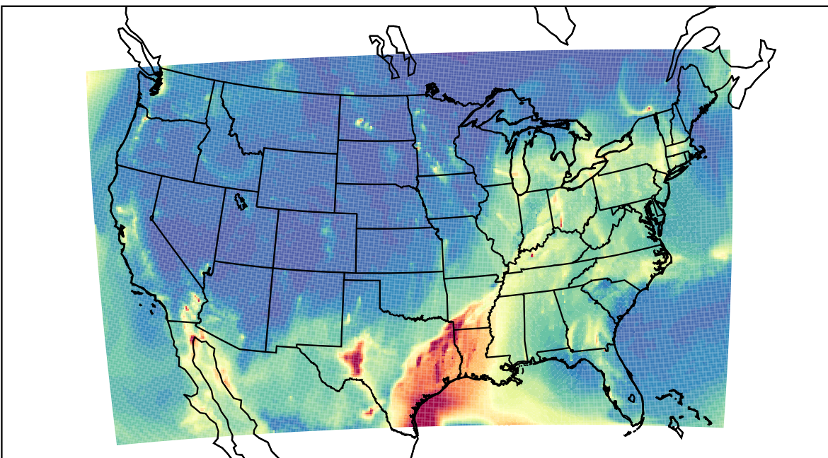
WRF 2021-03-28_06:00:00
