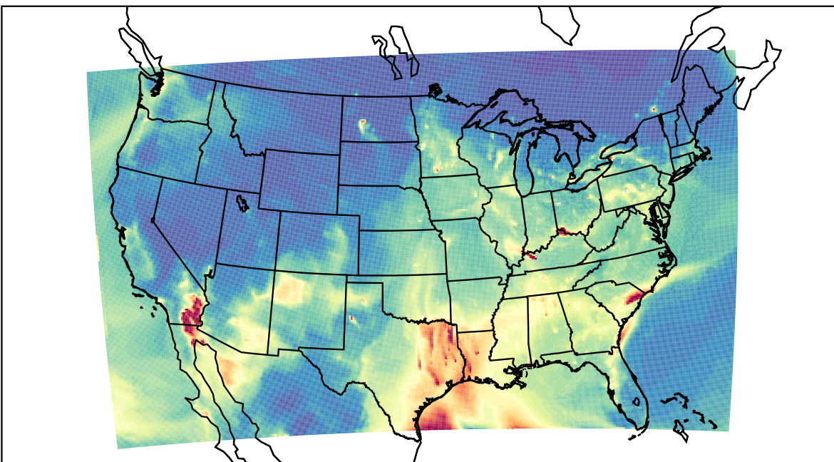
WRF 2021-03-27_11:00:00
