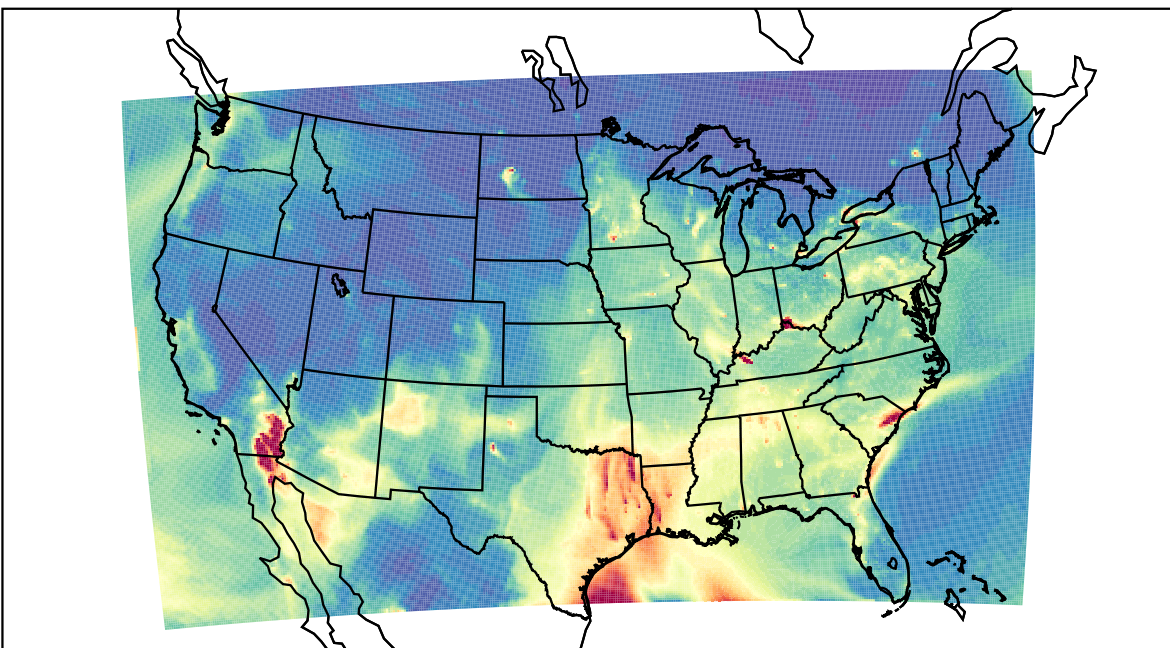
WRF 2021-03-27_12:00:00
