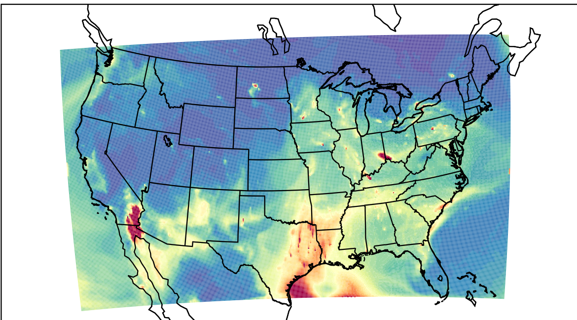
WRF 2021-03-27_15:00:00
