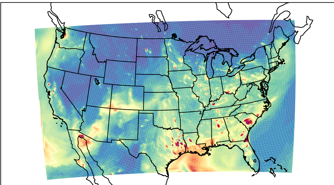
WRF 2021-03-27_03:00:00
