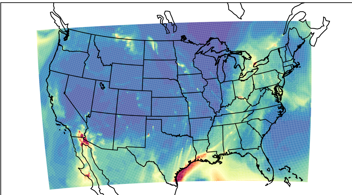
WRF 2021-03-28_15:00:00
