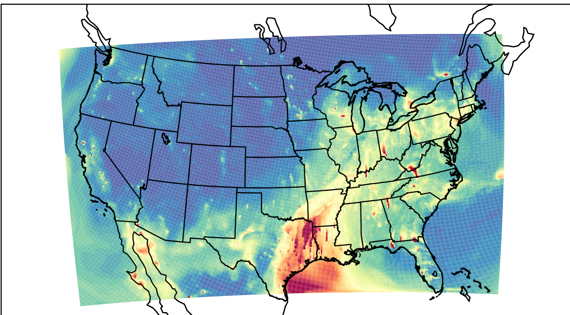
WRF 2021-03-28_02:00:00
