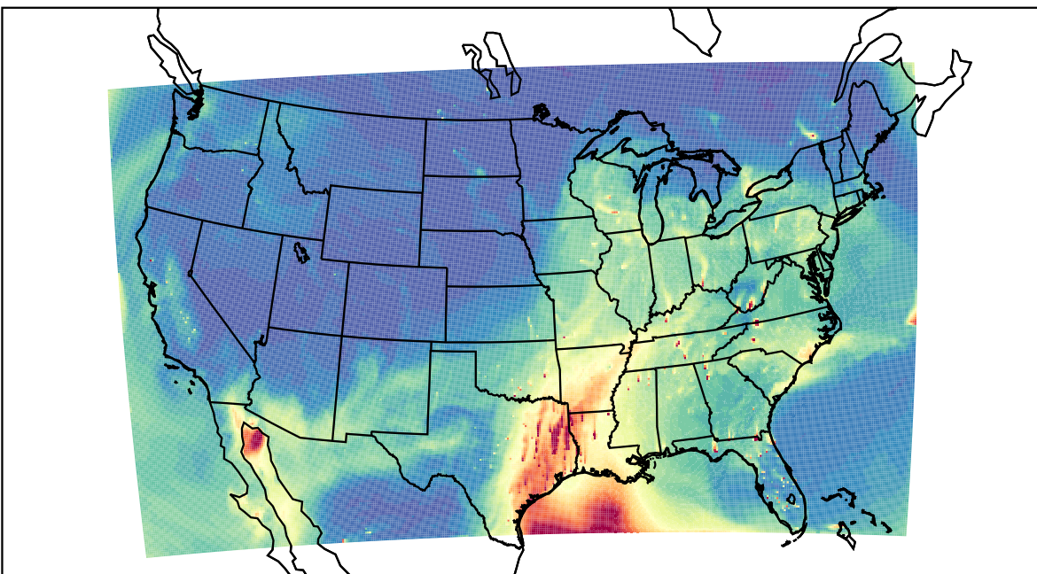
WRF 2021-03-27_22:00:00
