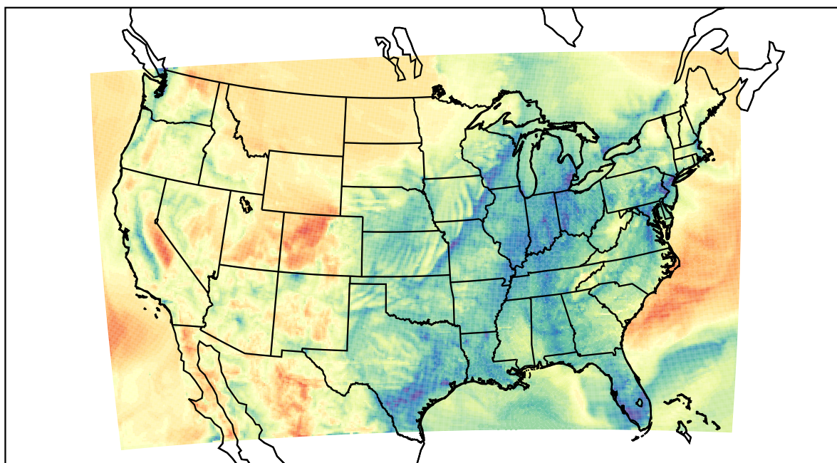
WRF (2021-03-30_12:00:00)
