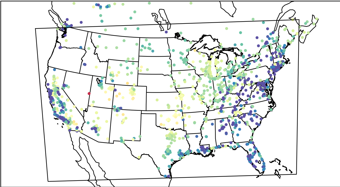
AirNOW (2021-03-30_08:00:00)
