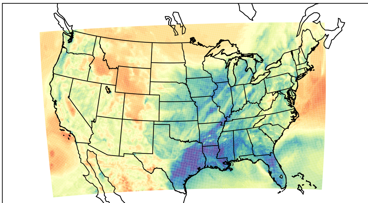
WRF (2021-03-31_05:00:00)
