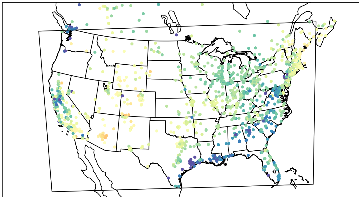
AirNOW (2021-03-31_17:00:00)
