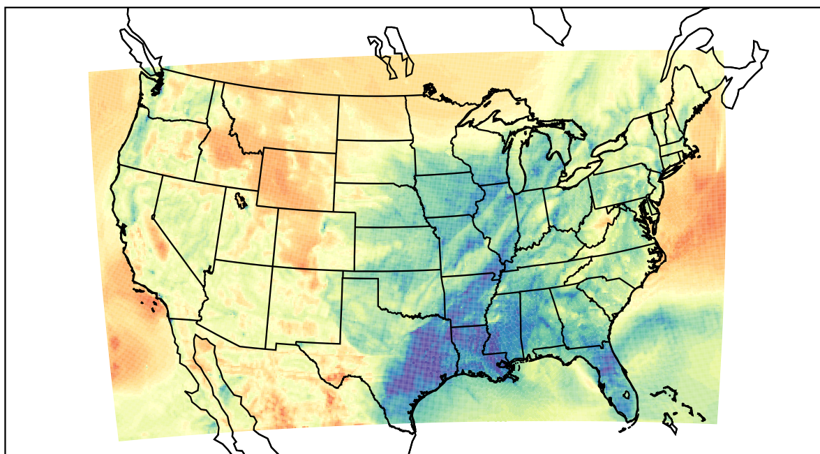
WRF (2021-03-31_04:00:00)
