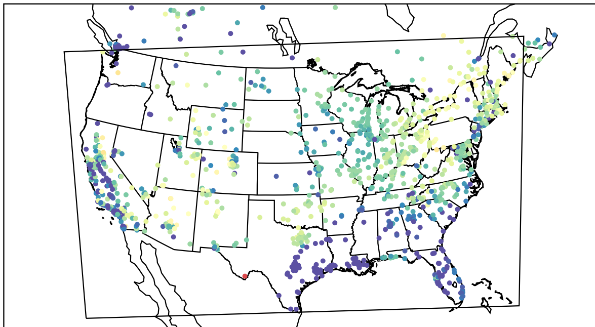
AirNOW (2021-03-31_07:00:00)
