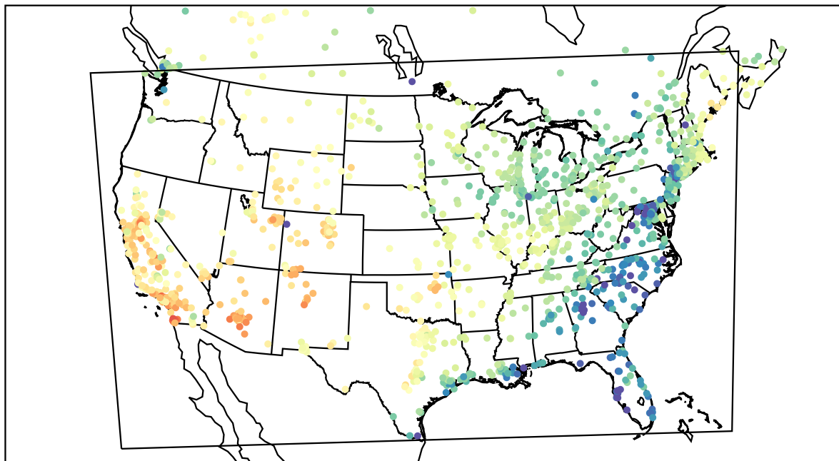
AirNOW (2021-03-31_23:00:00)
