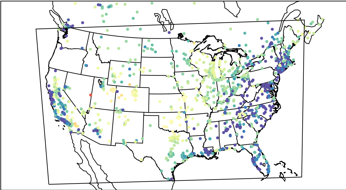
AirNOW (2021-03-30_07:00:00)
