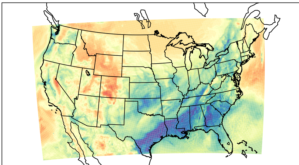
WRF (2021-03-31_14:00:00)
