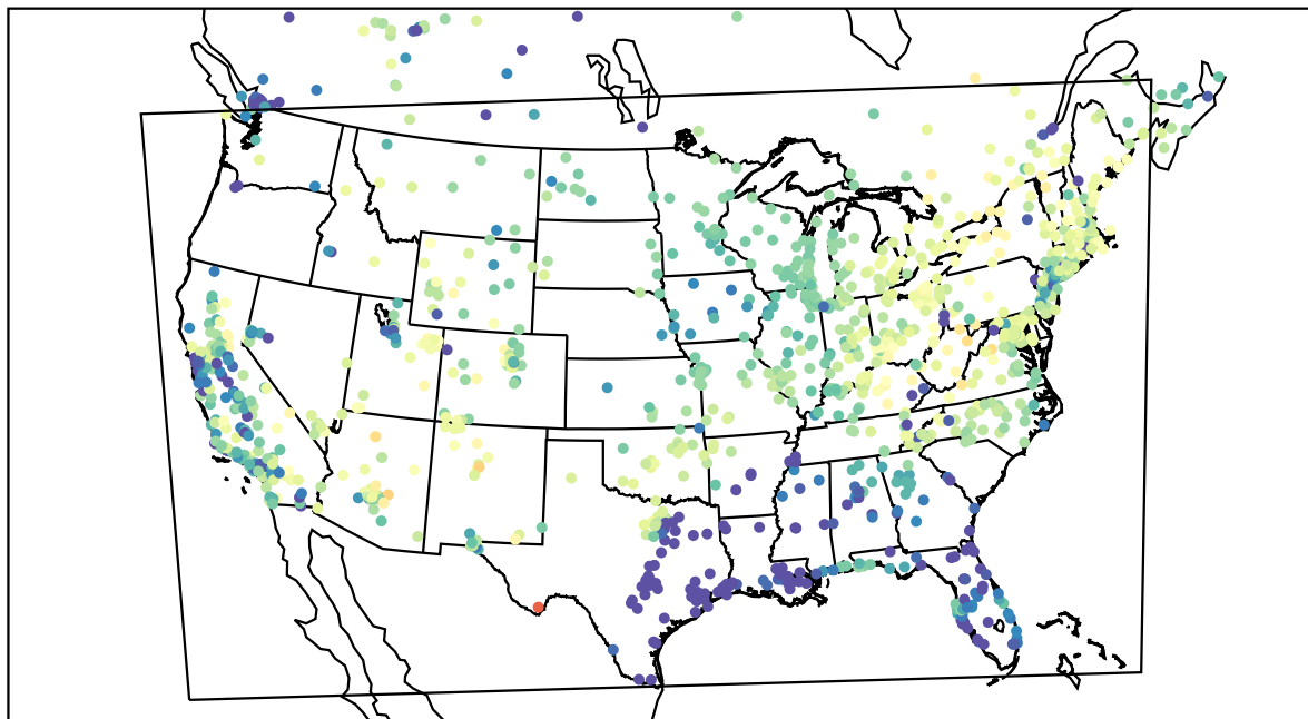
AirNOW (2021-03-31_04:00:00)
