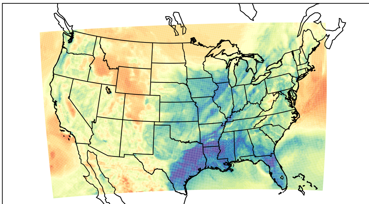
WRF (2021-03-31_06:00:00)
