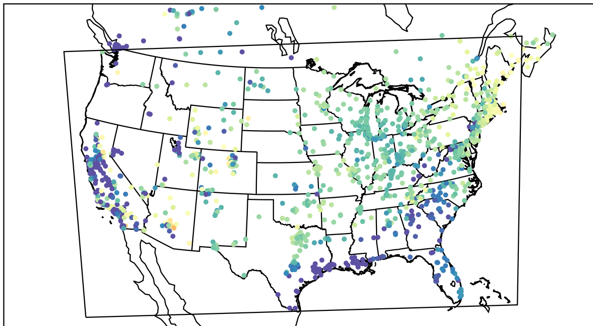
AirNOW (2021-03-31_14:00:00)
