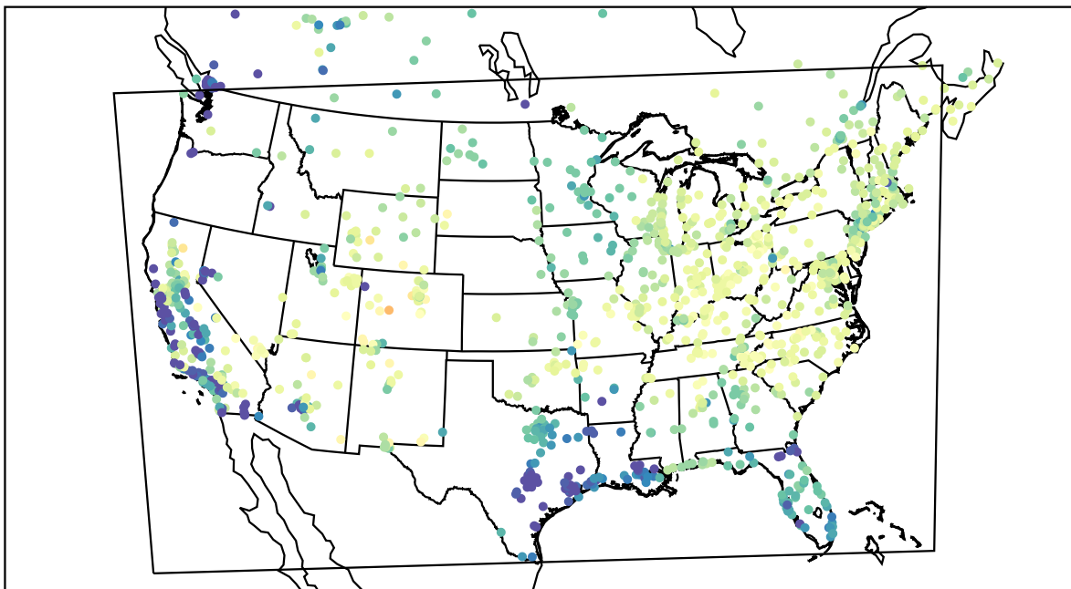
AirNOW (2021-03-30_15:00:00)
