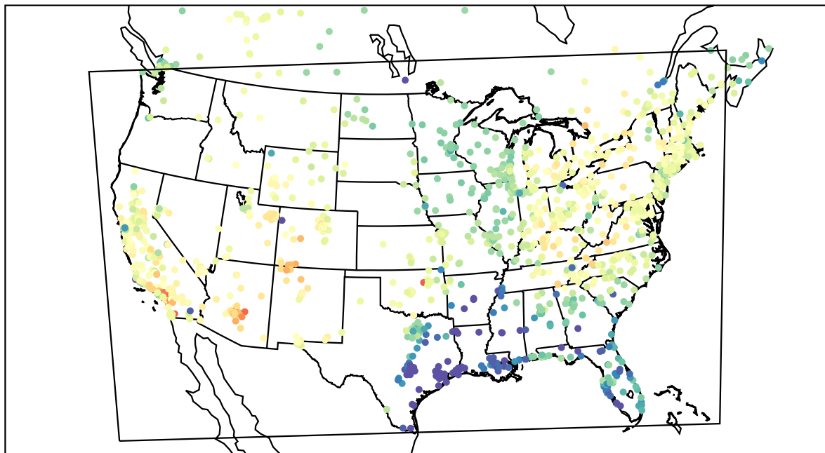
AirNOW (2021-03-31_00:00:00)
