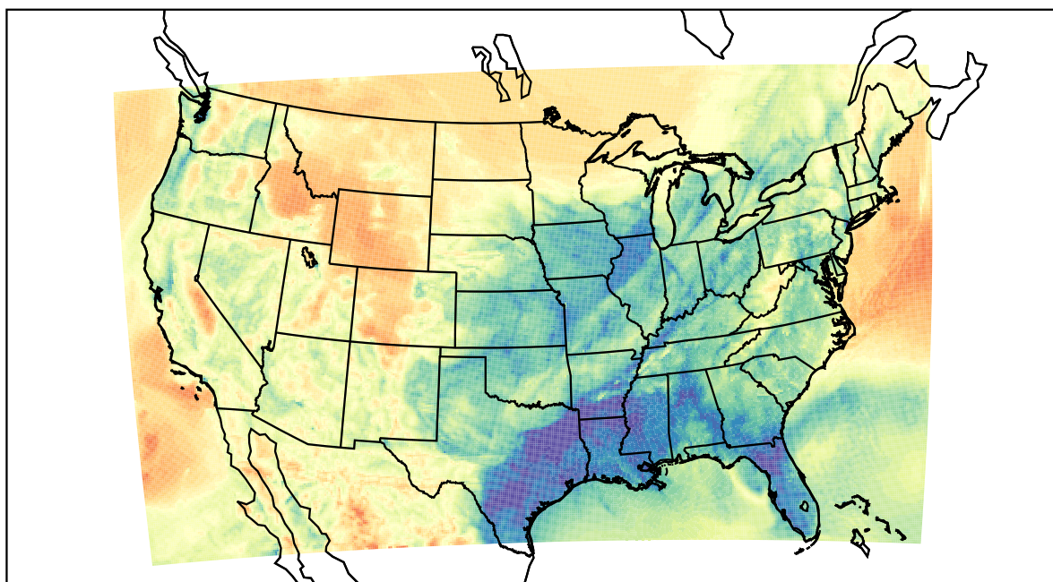
WRF (2021-03-31_07:00:00)
