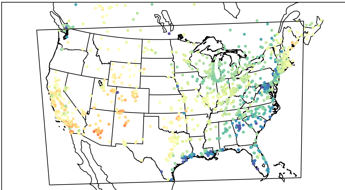
AirNOW (2021-03-31_21:00:00)
