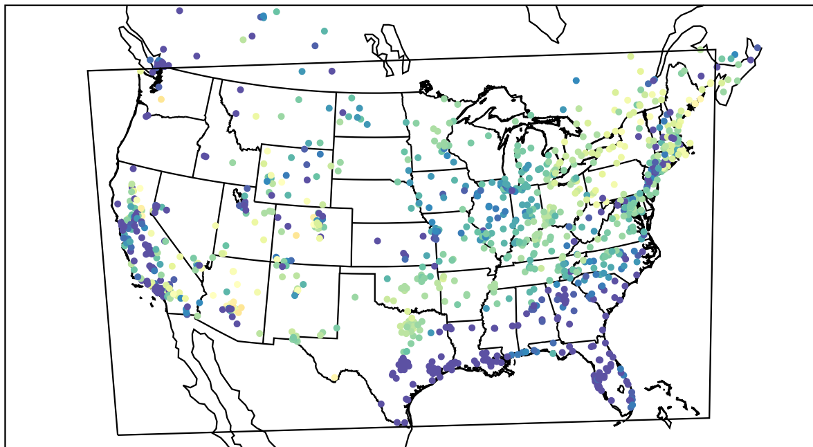
AirNOW (2021-03-31_10:00:00)
