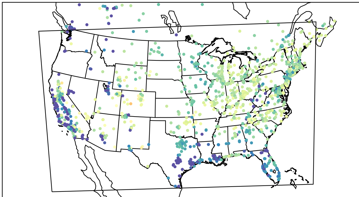
AirNOW (2021-03-30_14:00:00)
