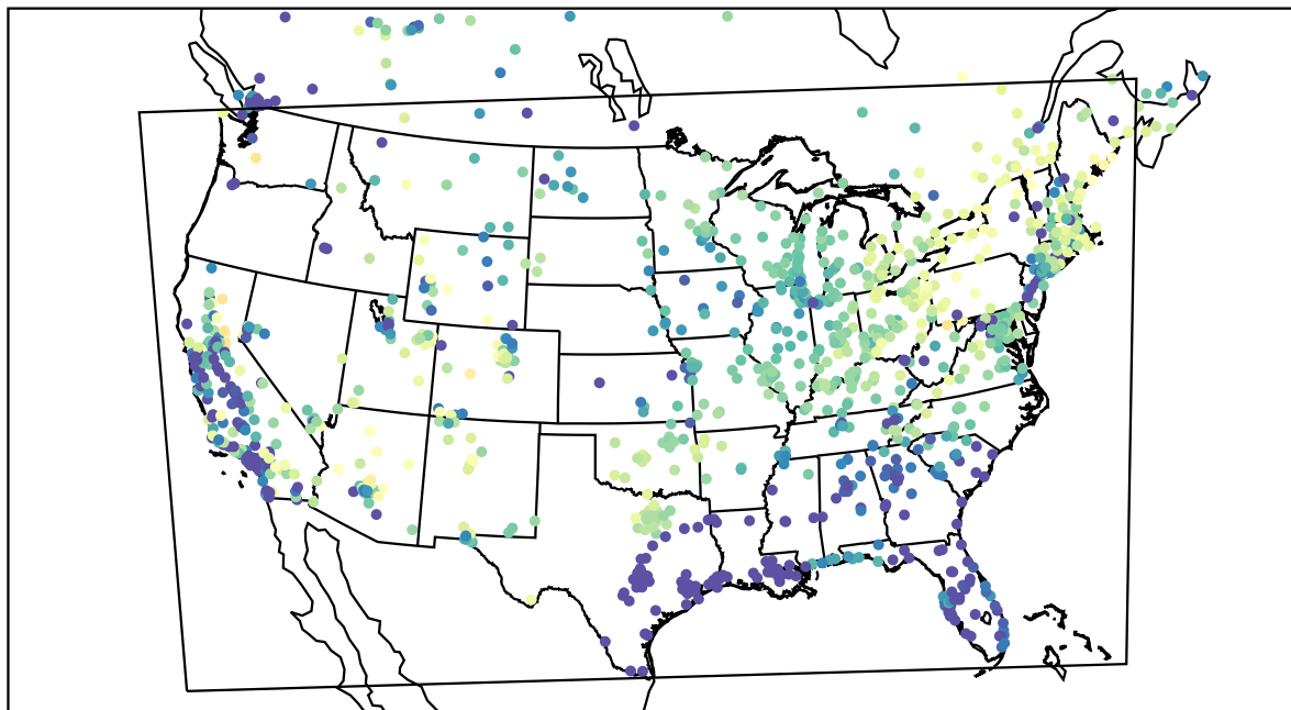
AirNOW (2021-03-31_08:00:00)
