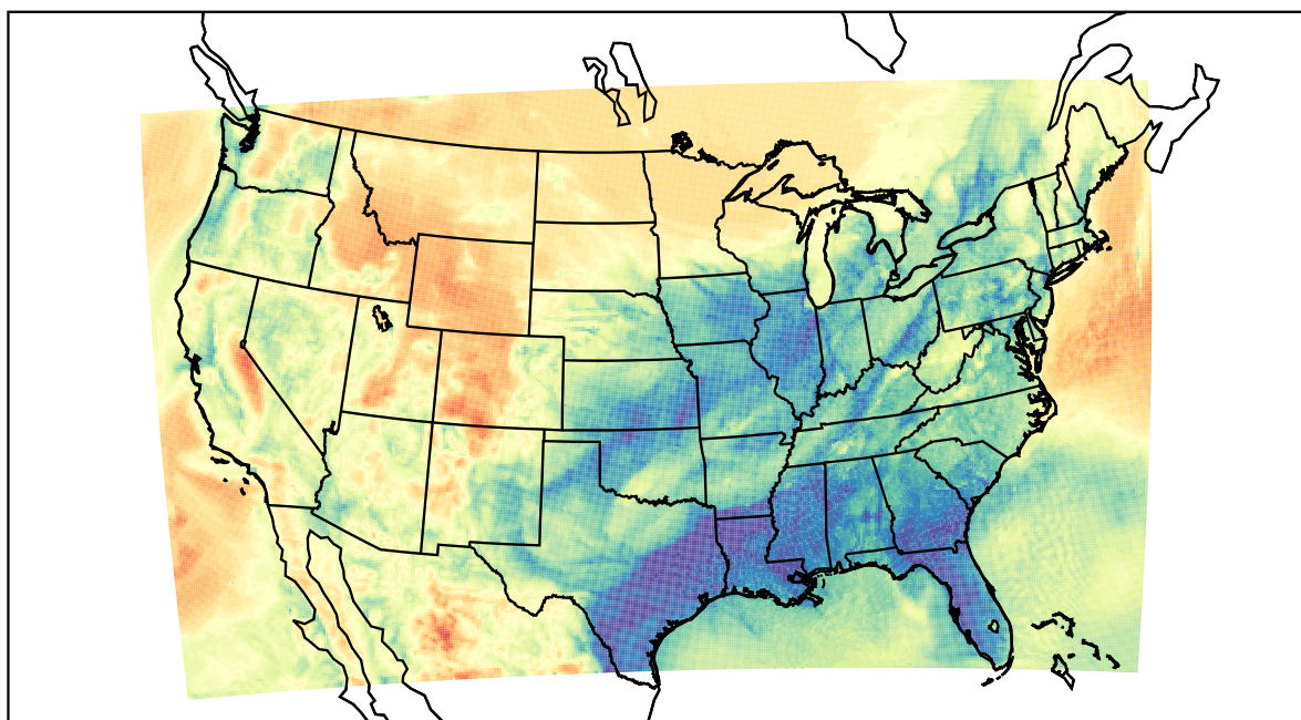
WRF (2021-03-31_11:00:00)
