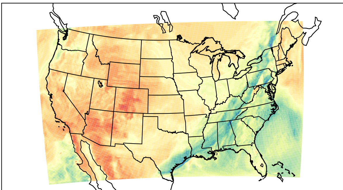
WRF (2021-03-31_21:00:00)
