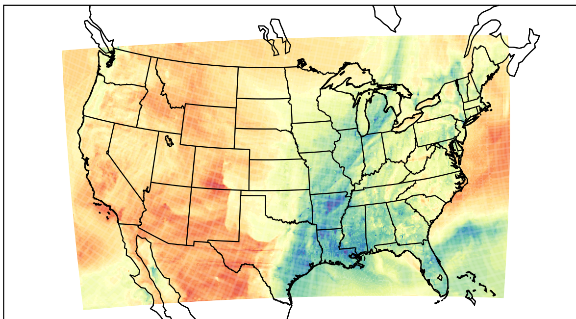
WRF (2021-03-31_00:00:00)
