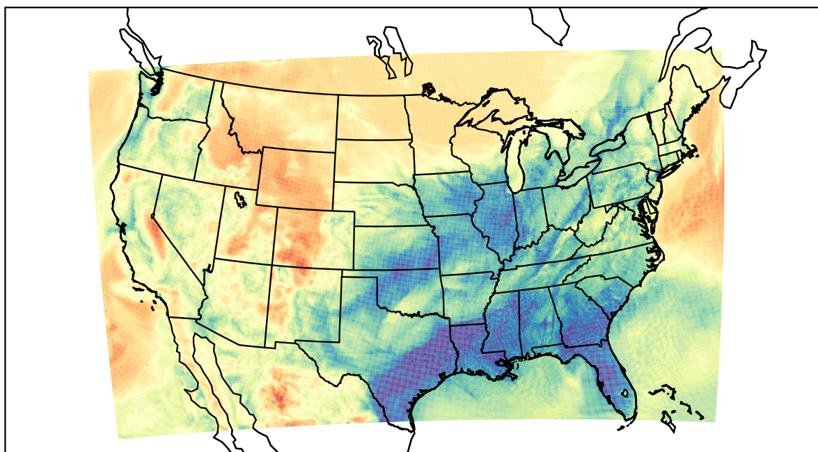
WRF (2021-03-31_12:00:00)
