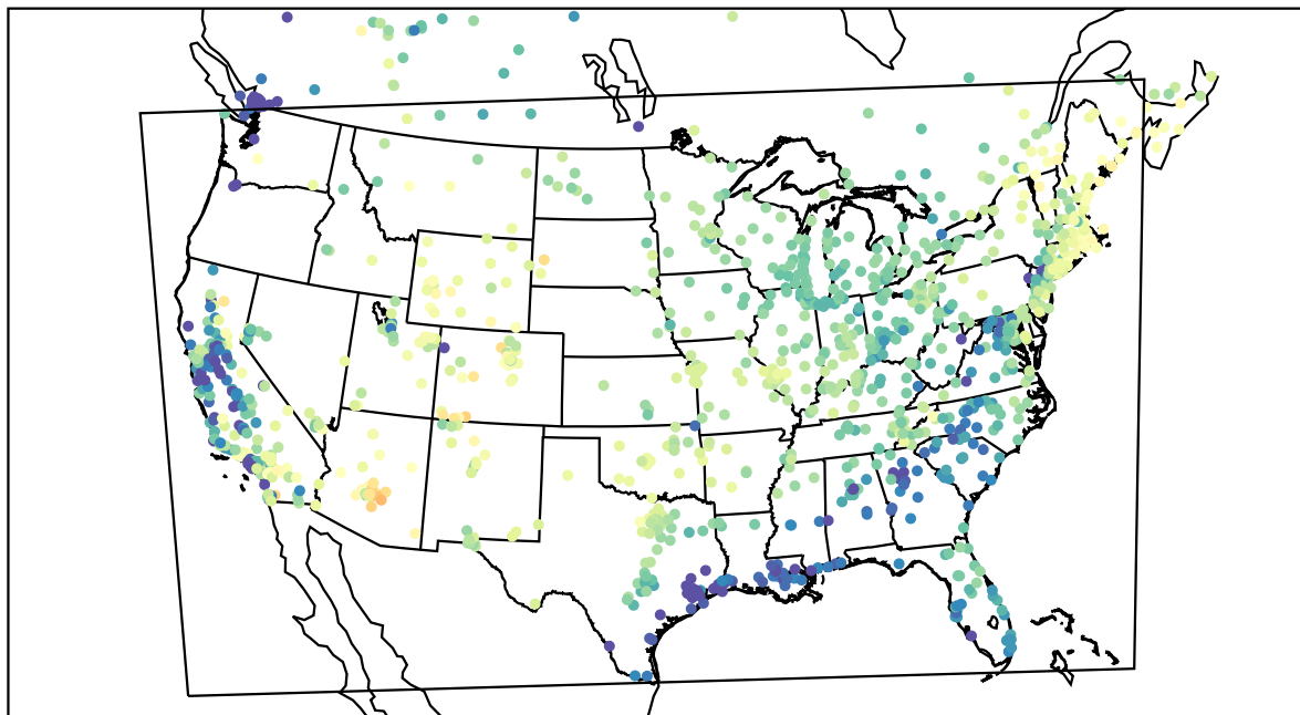
AirNOW (2021-03-31_16:00:00)
