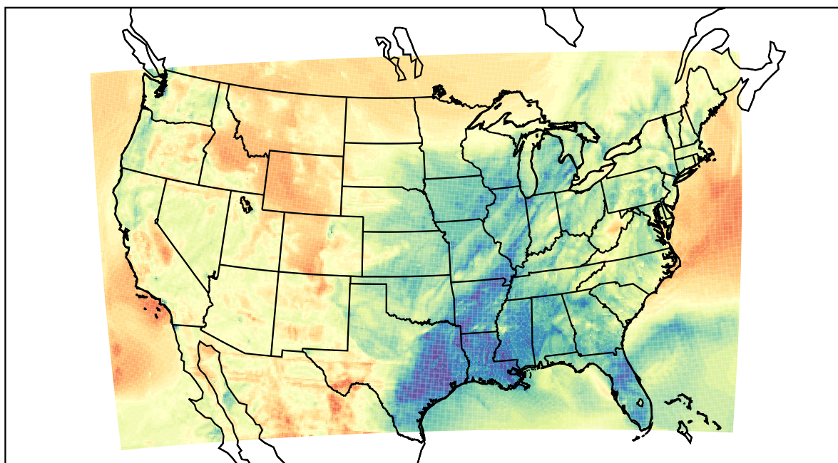
WRF (2021-03-31_03:00:00)
