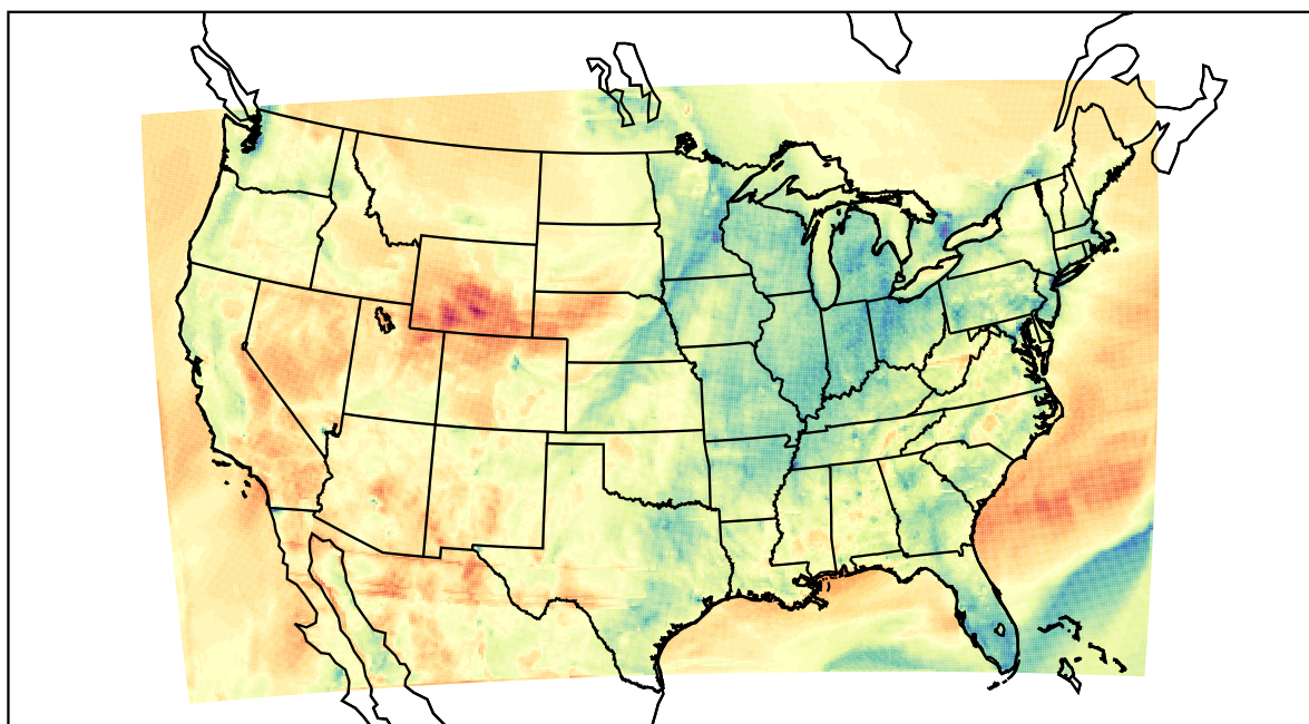
WRF (2021-03-30_02:00:00)
