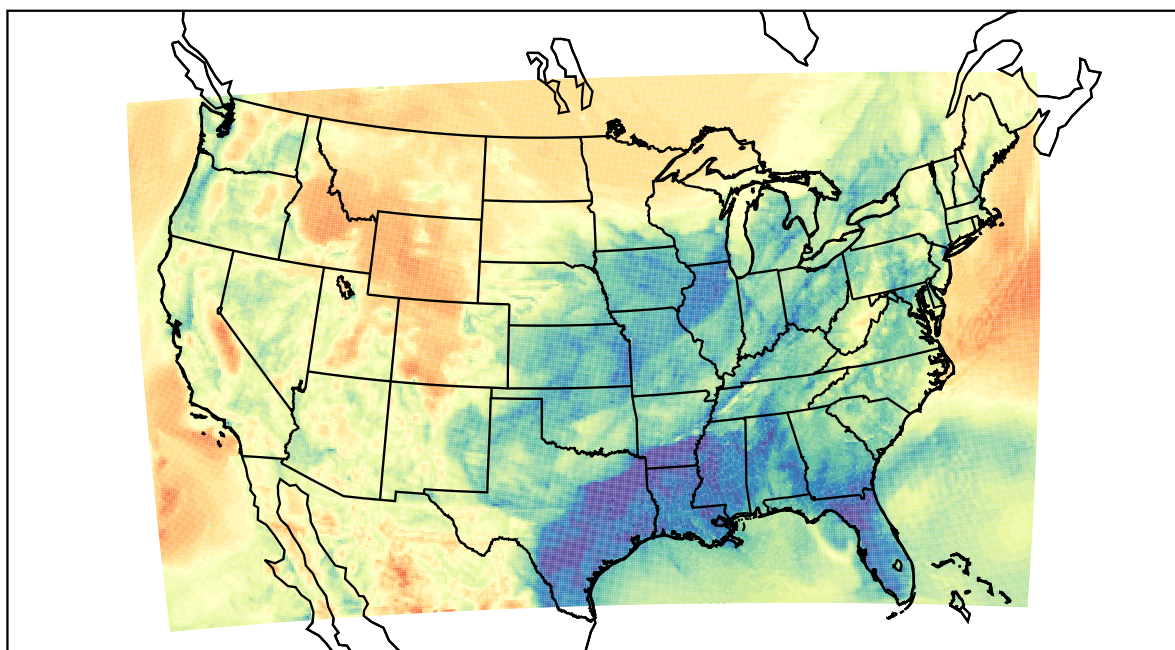
WRF (2021-03-31_08:00:00)
