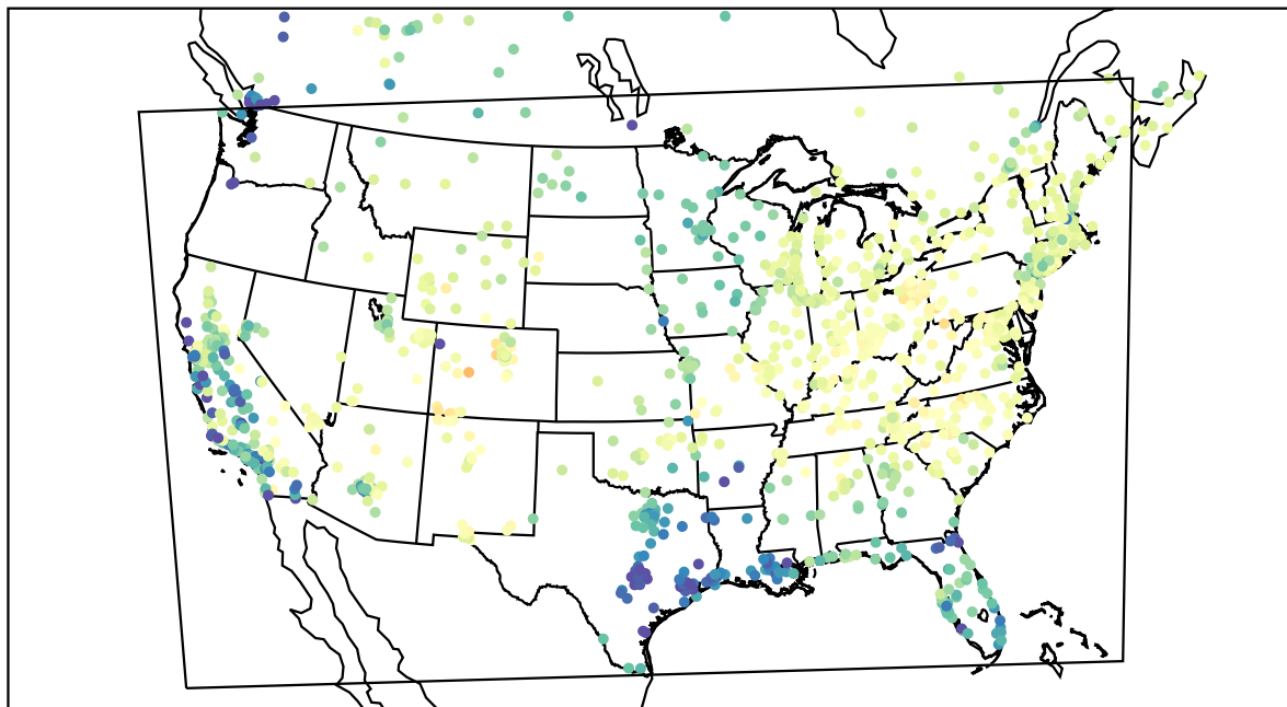
AirNOW (2021-03-30_16:00:00)
