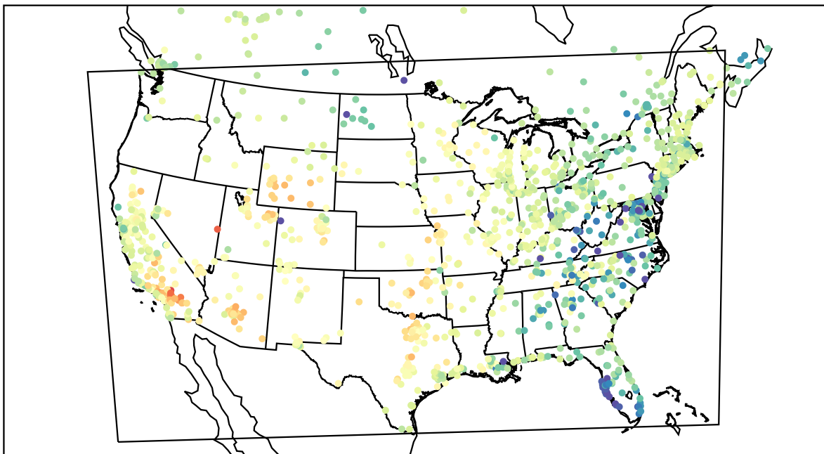
AirNOW (2021-03-30_00:00:00)
