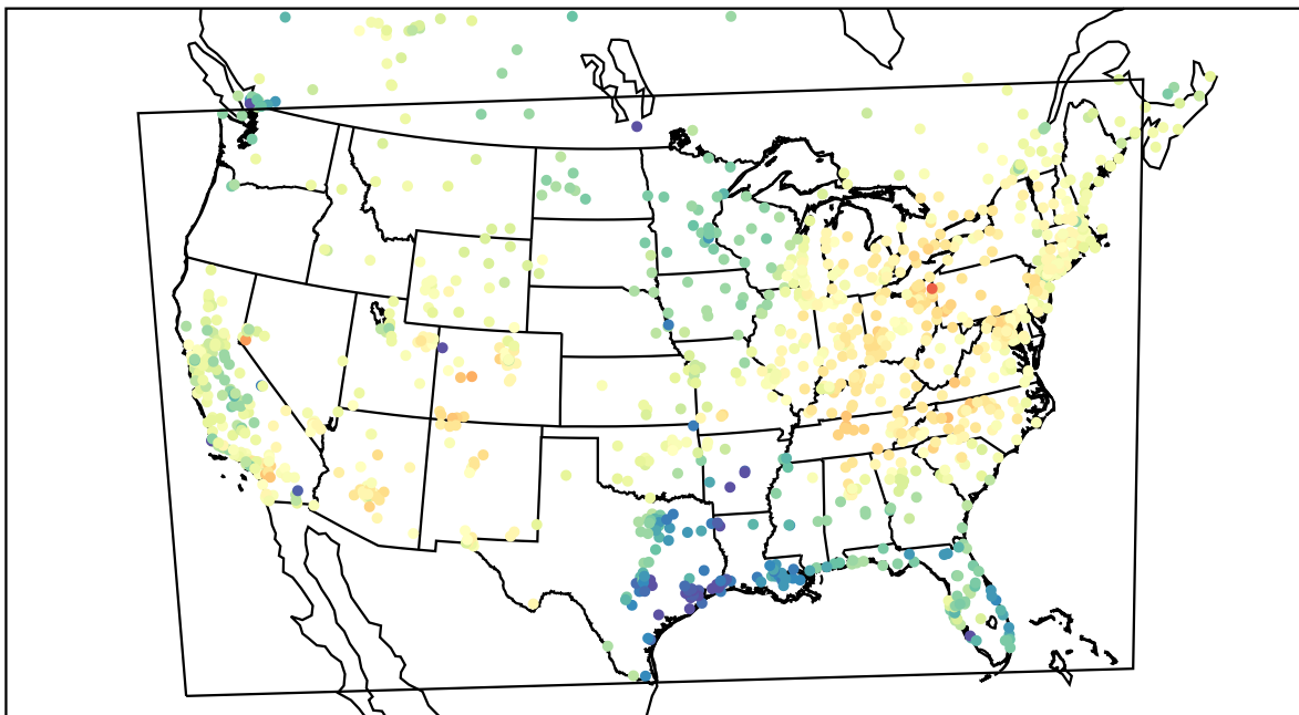
AirNOW (2021-03-30_19:00:00)
