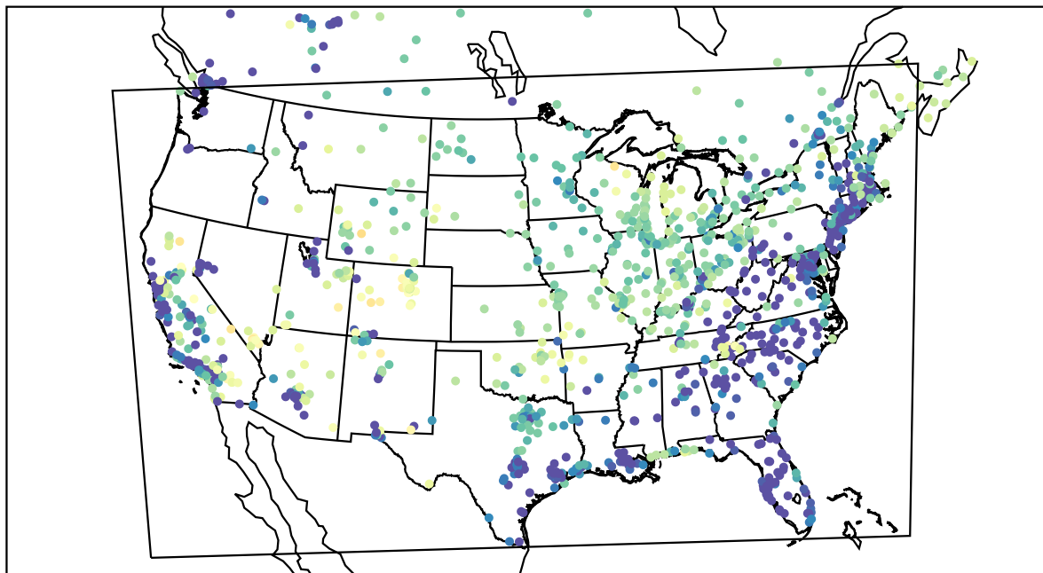
AirNOW (2021-03-30_12:00:00)
