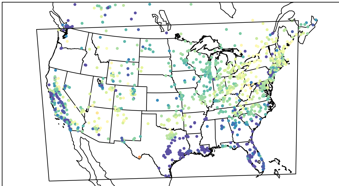
AirNOW (2021-03-31_06:00:00)
