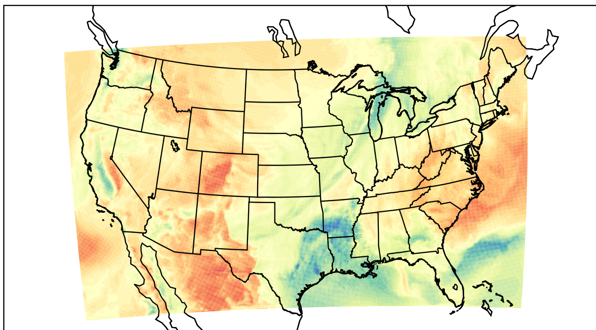
WRF (2021-03-30_17:00:00)
