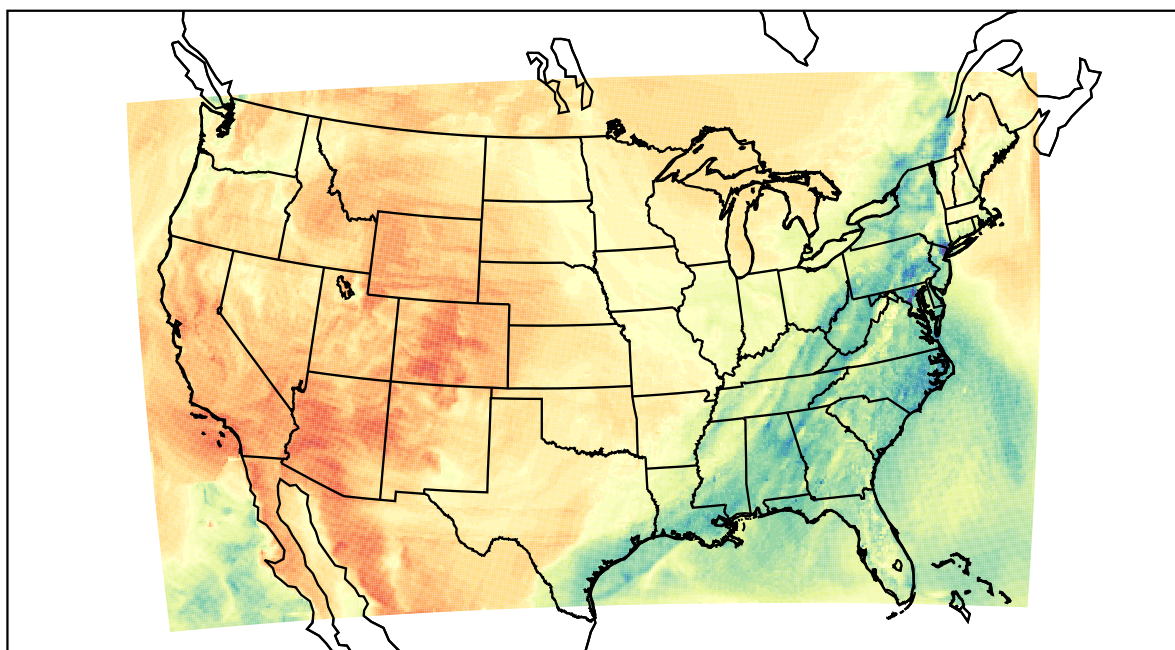
WRF (2021-03-31_23:00:00)
