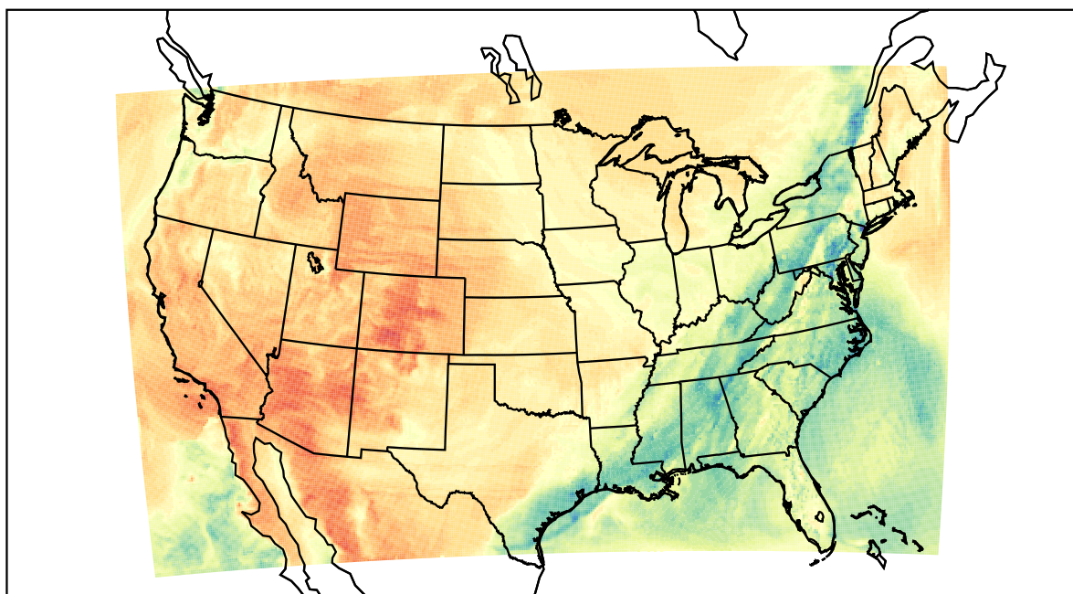
WRF (2021-03-31_22:00:00)
