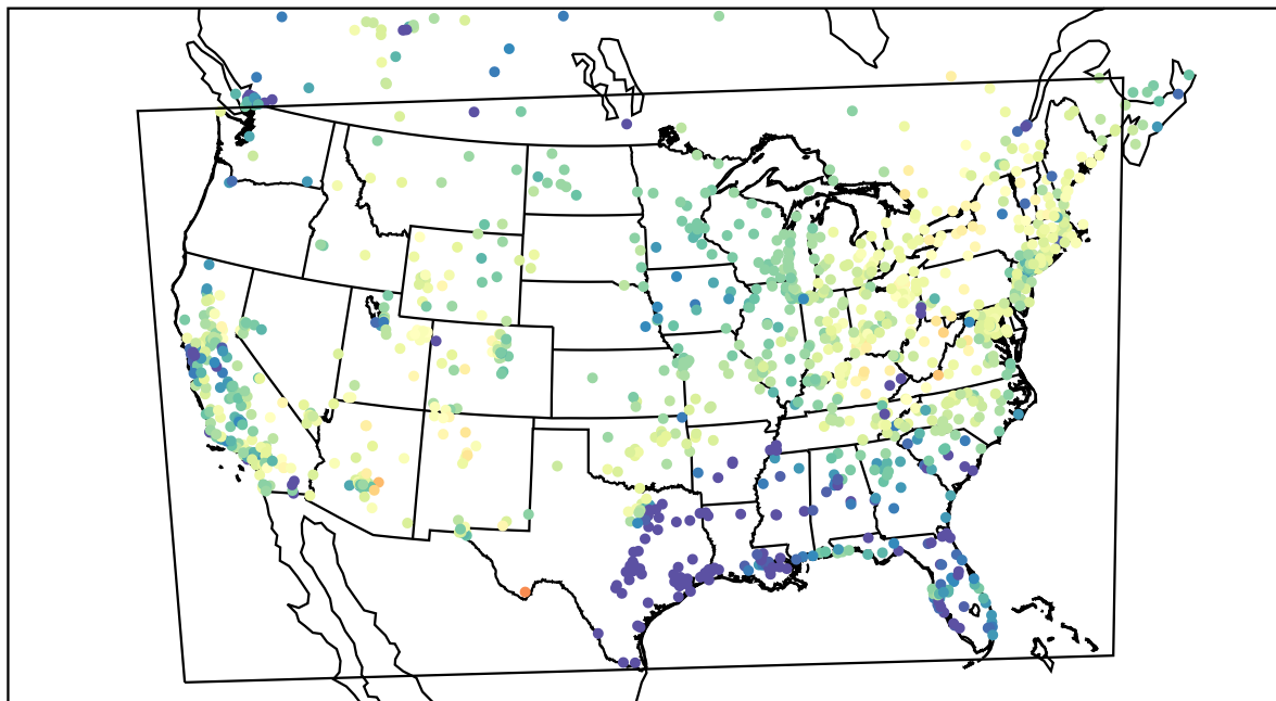
AirNOW (2021-03-31_03:00:00)
