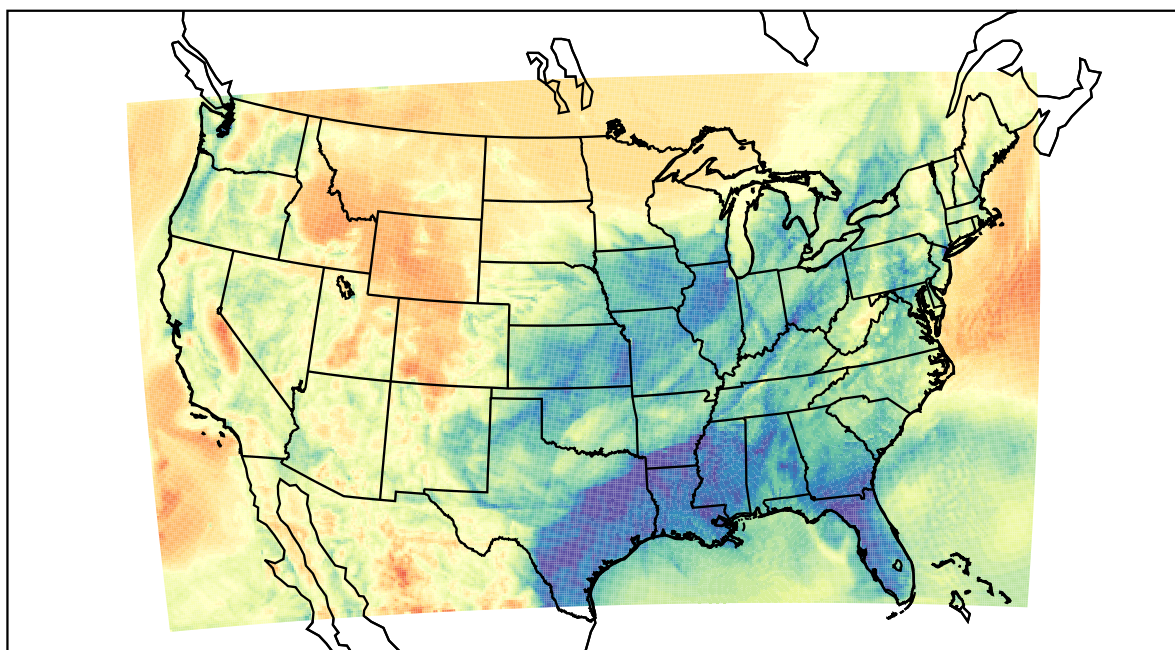
WRF (2021-03-31_09:00:00)
