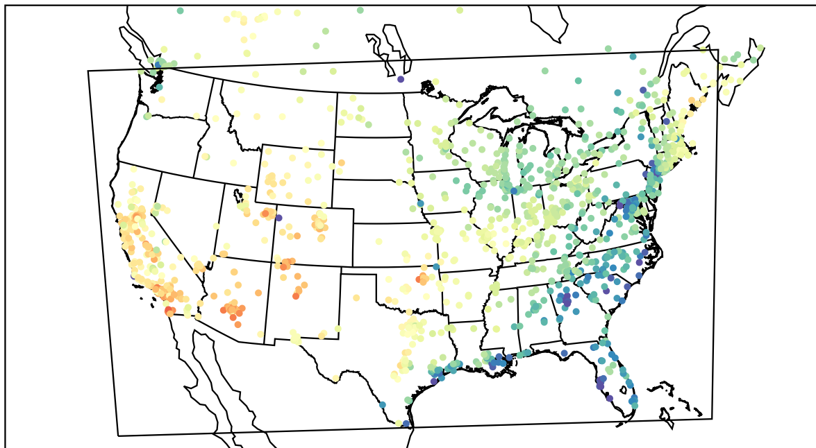
AirNOW (2021-03-31_22:00:00)
