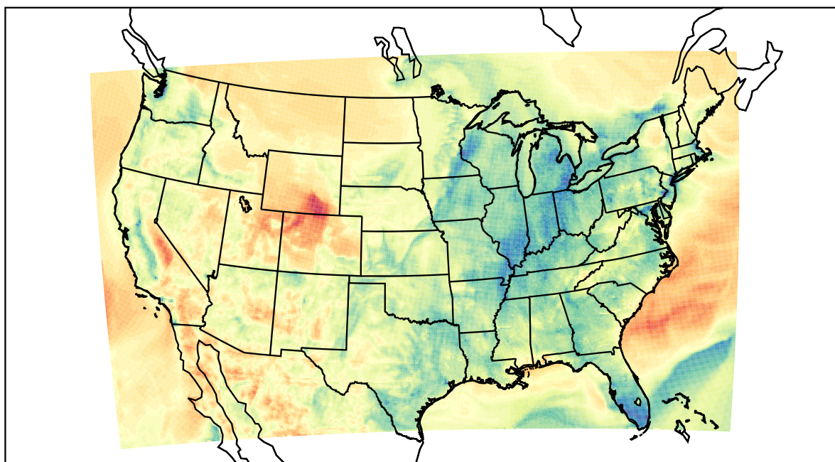
WRF (2021-03-30_06:00:00)
