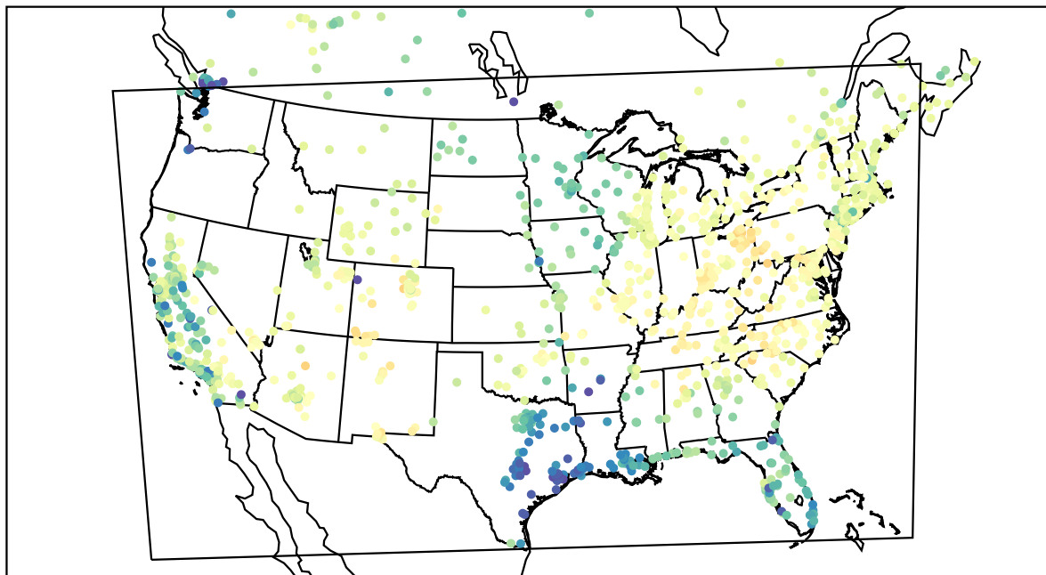
AirNOW (2021-03-30_17:00:00)
