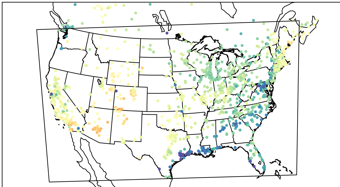
AirNOW (2021-03-31_19:00:00)
