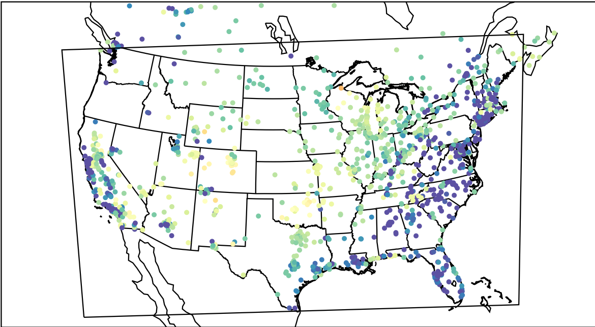
AirNOW (2021-03-30_09:00:00)
