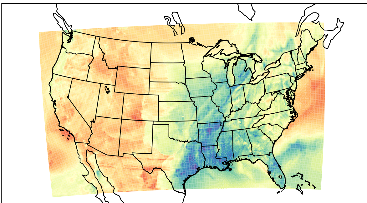
WRF (2021-03-31_01:00:00)
