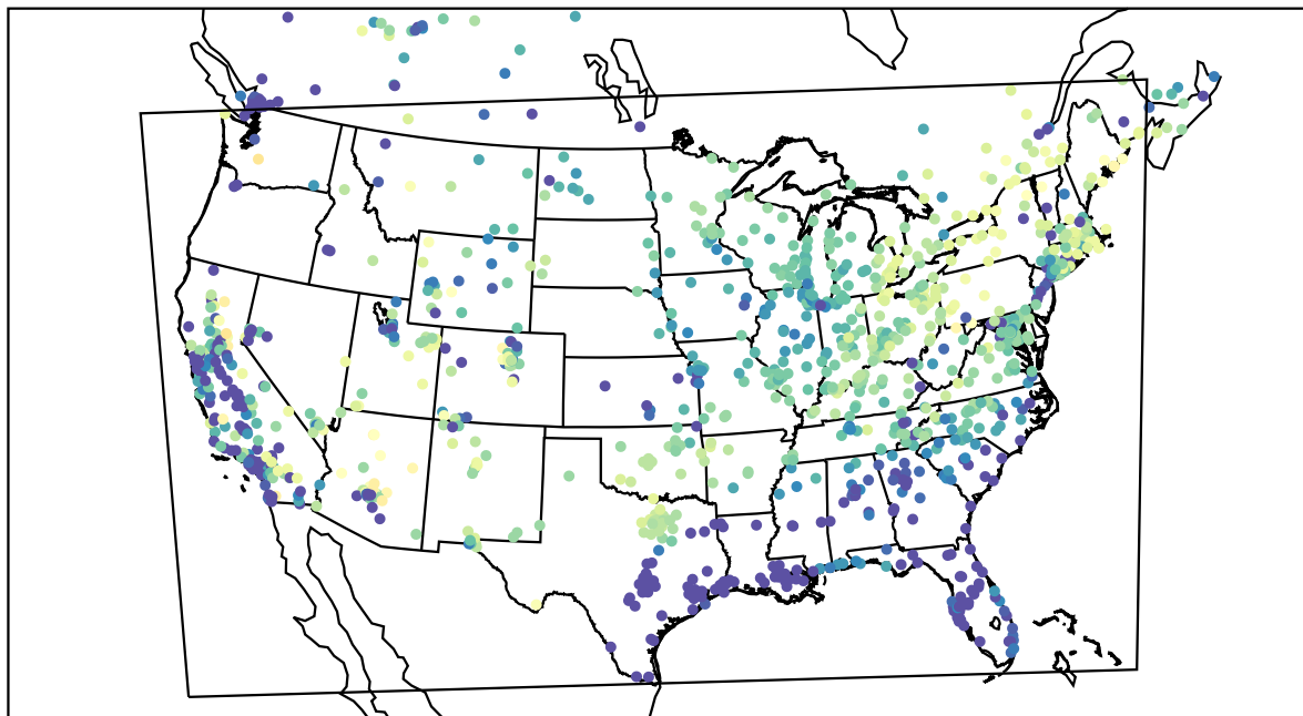
AirNOW (2021-03-31_09:00:00)
