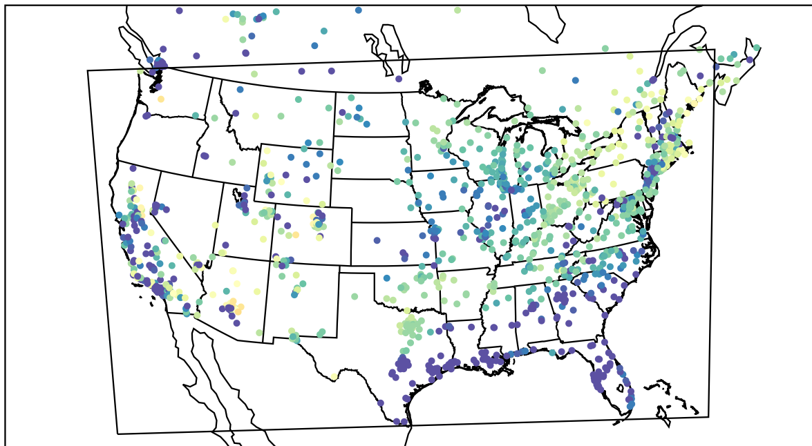
AirNOW (2021-03-31_11:00:00)
