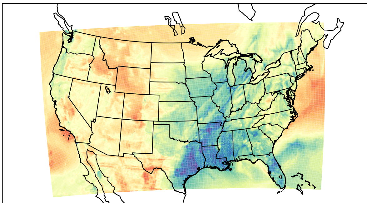
WRF (2021-03-31_02:00:00)
