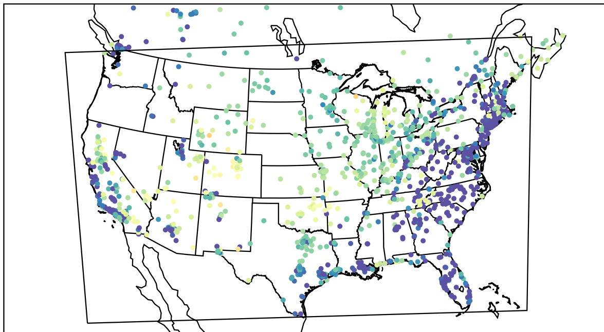
AirNOW (2021-03-30_11:00:00)
