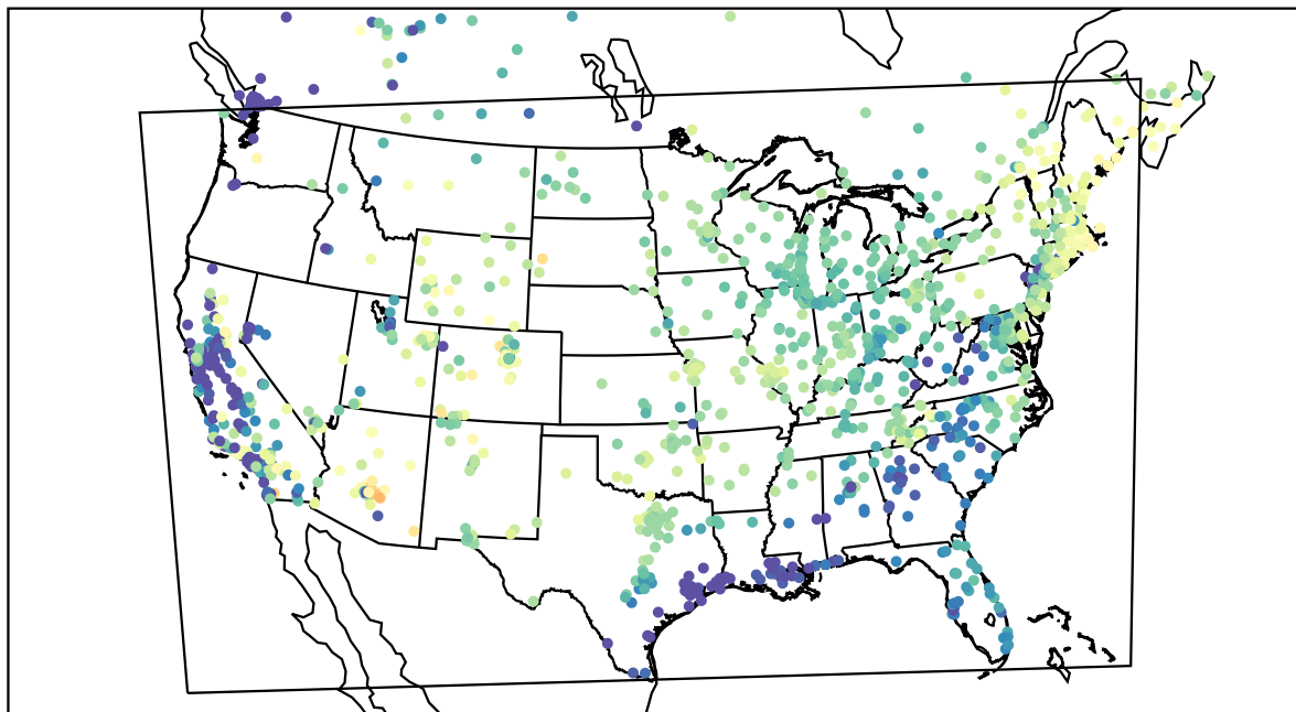
AirNOW (2021-03-31_15:00:00)
