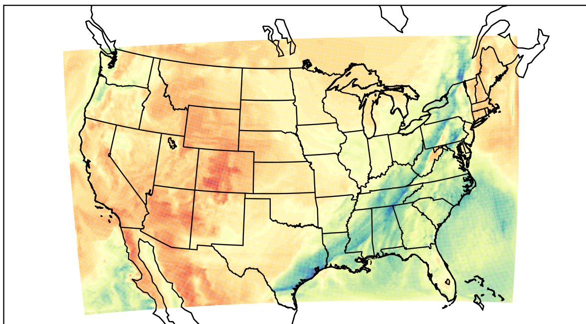
WRF (2021-03-31_20:00:00)
