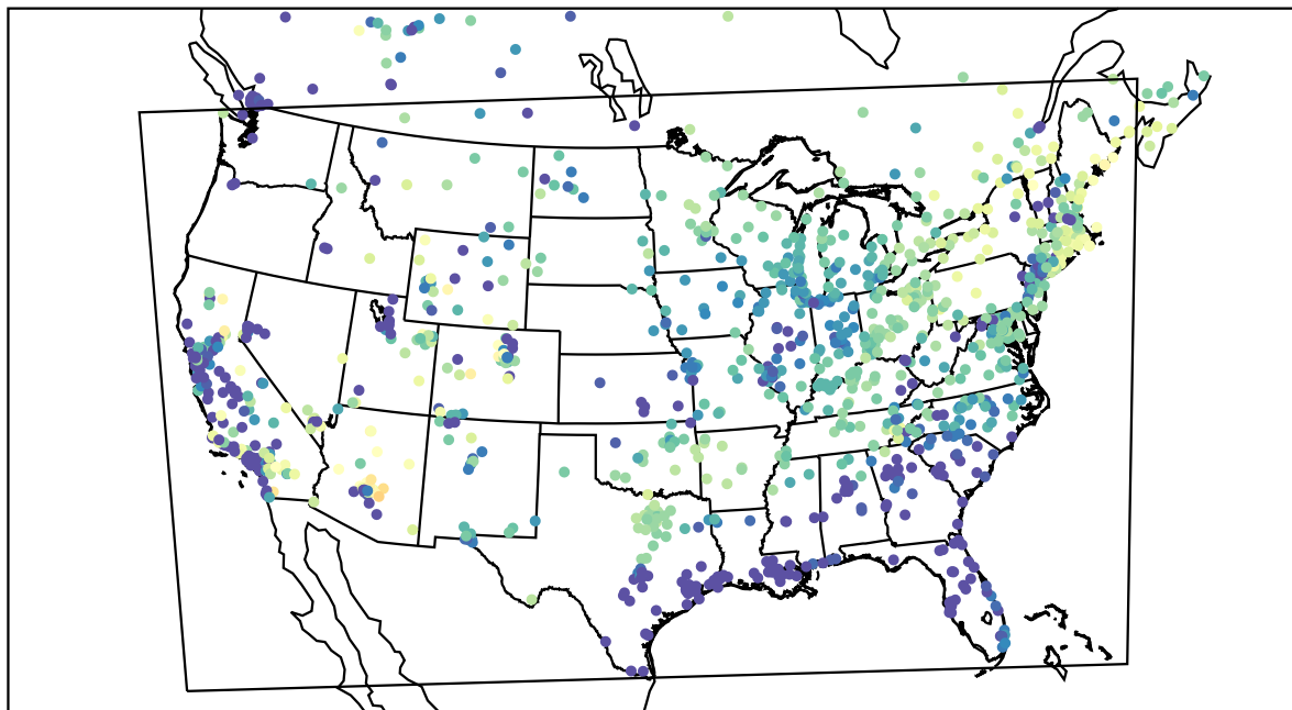
AirNOW (2021-03-31_12:00:00)
