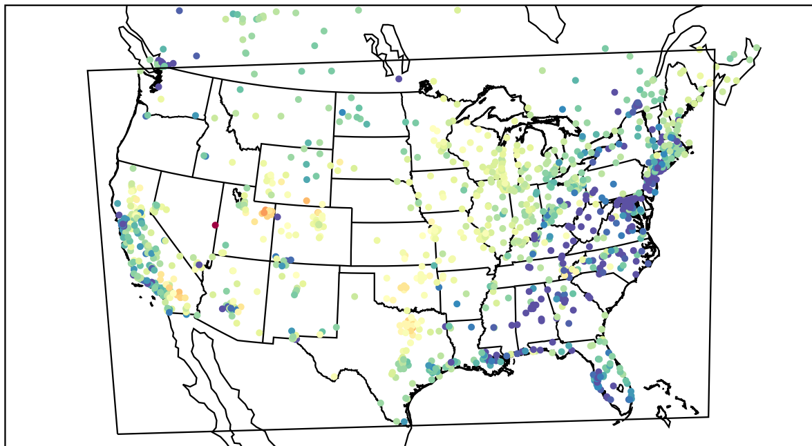
AirNOW (2021-03-30_04:00:00)
