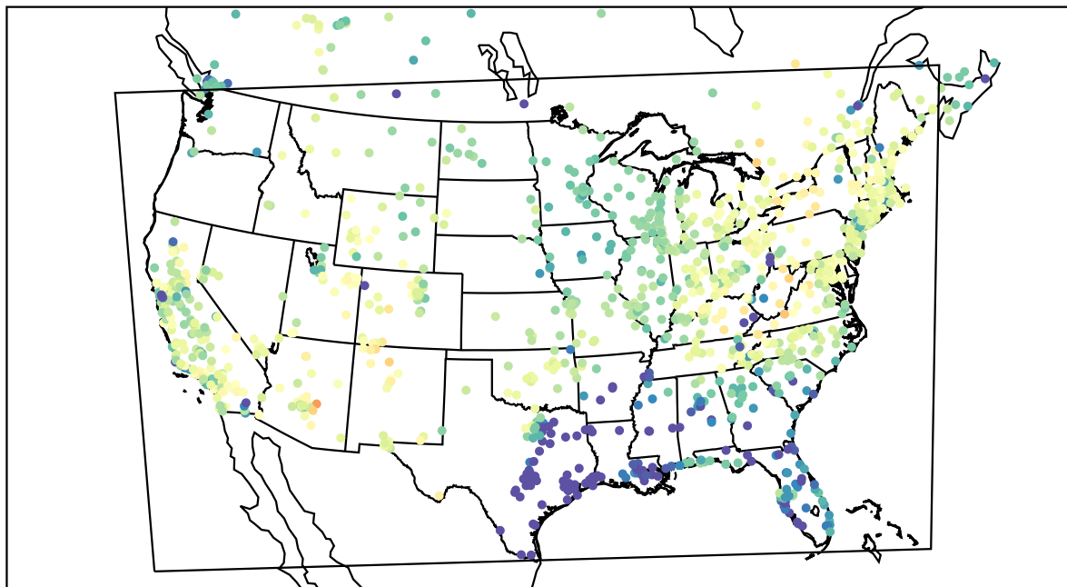
AirNOW (2021-03-31_02:00:00)
