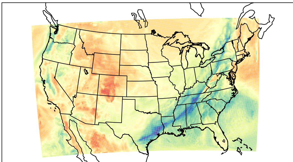
WRF (2021-03-31_17:00:00)
