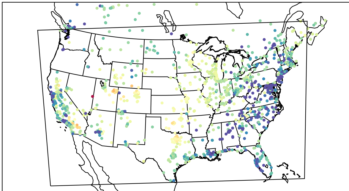
AirNOW (2021-03-30_05:00:00)
