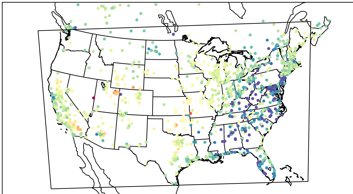
AirNOW (2021-03-30_02:00:00)
