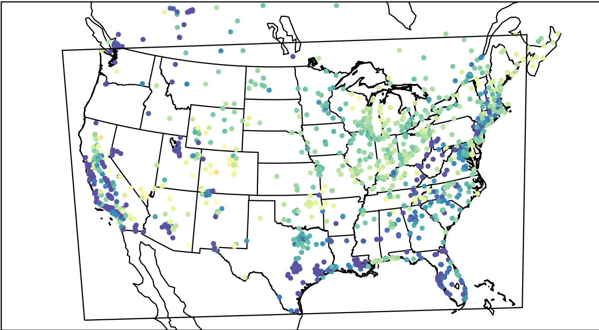
AirNOW (2021-03-30_13:00:00)
