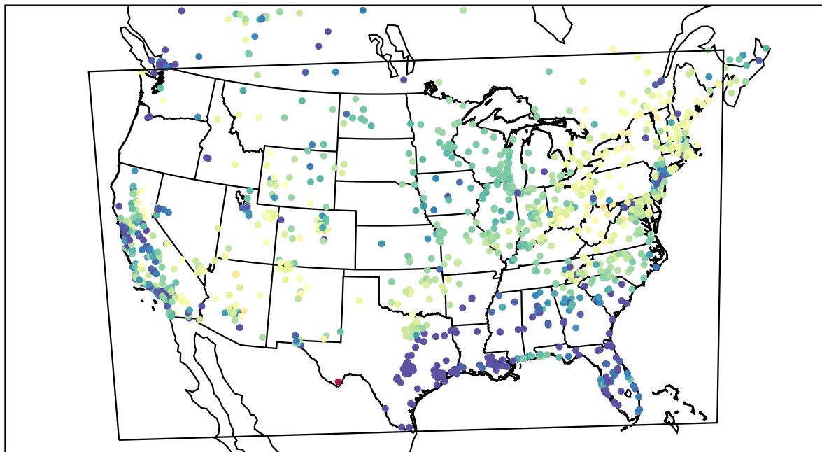
AirNOW (2021-03-31_05:00:00)
