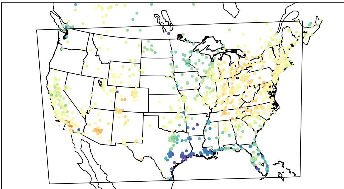
AirNOW (2021-03-30_21:00:00)
