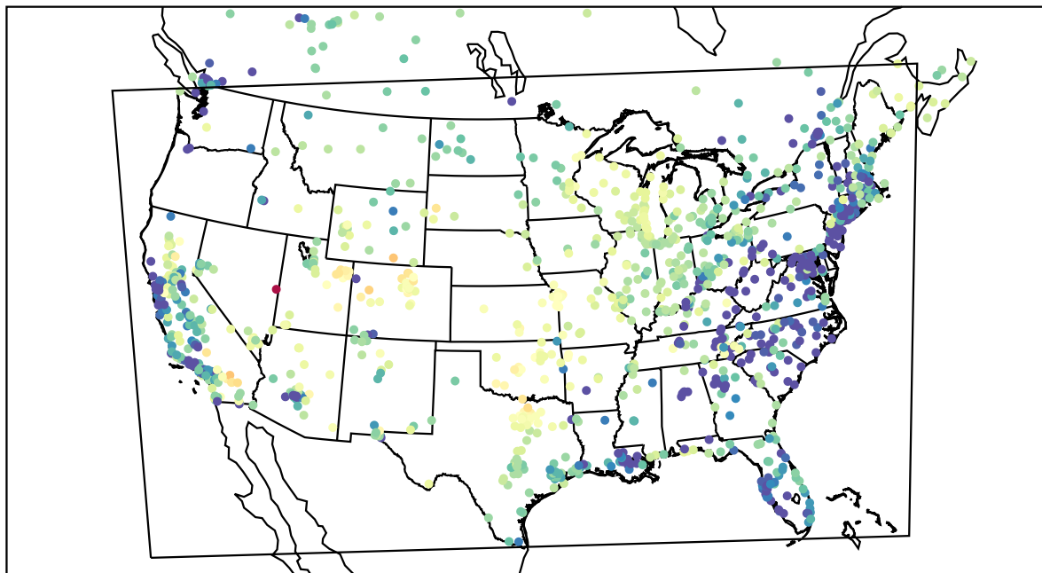
AirNOW (2021-03-30_06:00:00)
