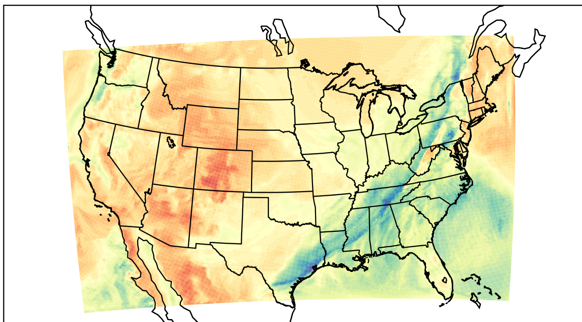
WRF (2021-03-31_19:00:00)
