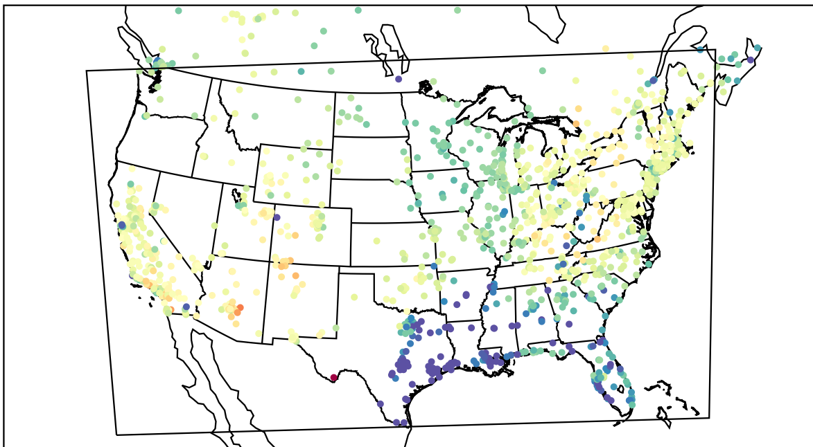
AirNOW (2021-03-31_01:00:00)
