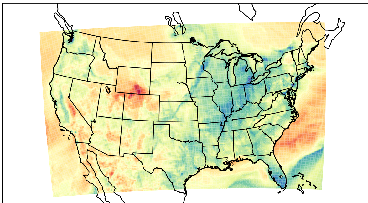
WRF (2021-03-30_05:00:00)
