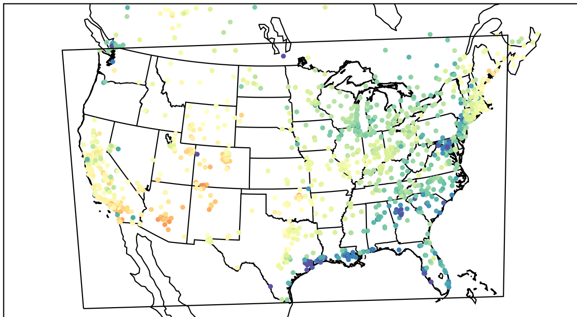
AirNOW (2021-03-31_20:00:00)
