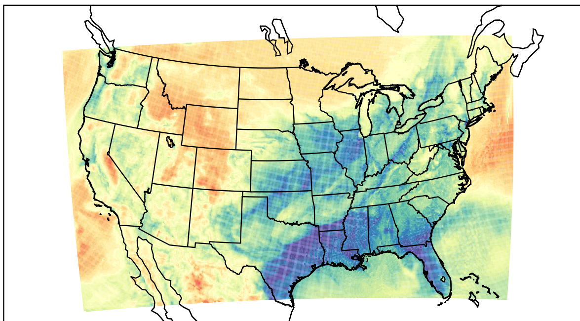
WRF (2021-03-31_10:00:00)
