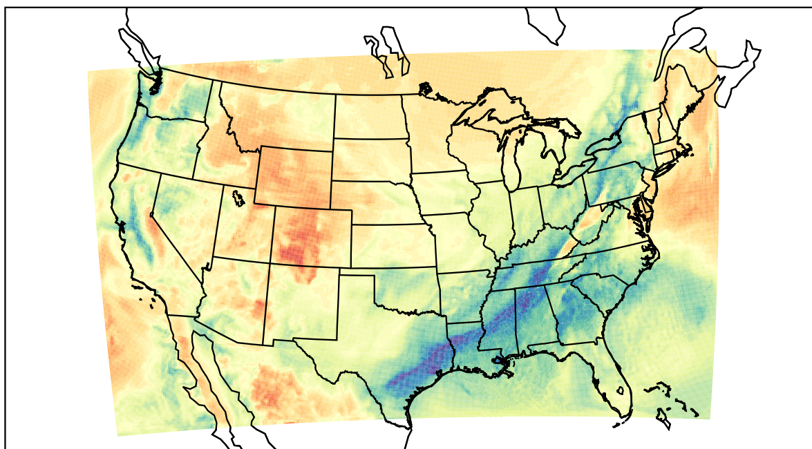
WRF (2021-03-31_16:00:00)
