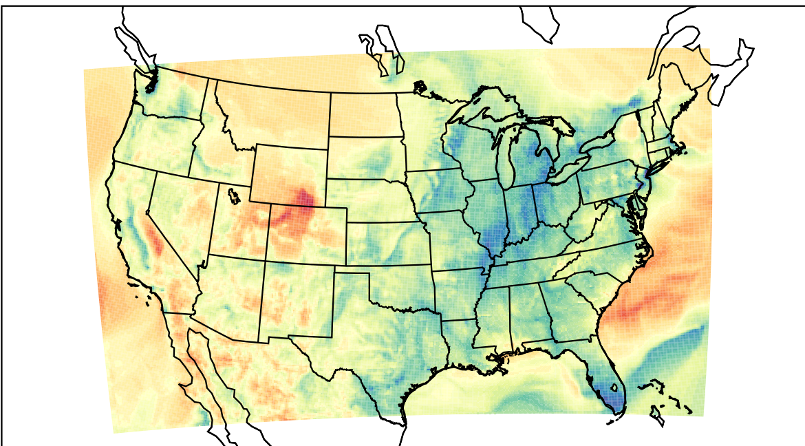
WRF (2021-03-30_07:00:00)
