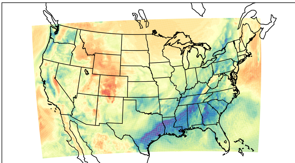
WRF (2021-03-31_15:00:00)
