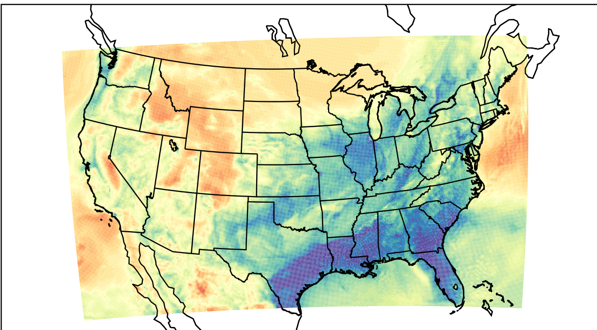
WRF (2021-03-31_11:00:00)
