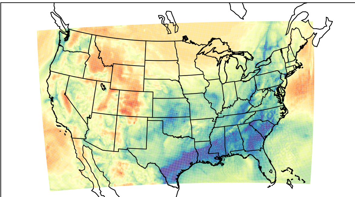
WRF (2021-03-31_14:00:00)
