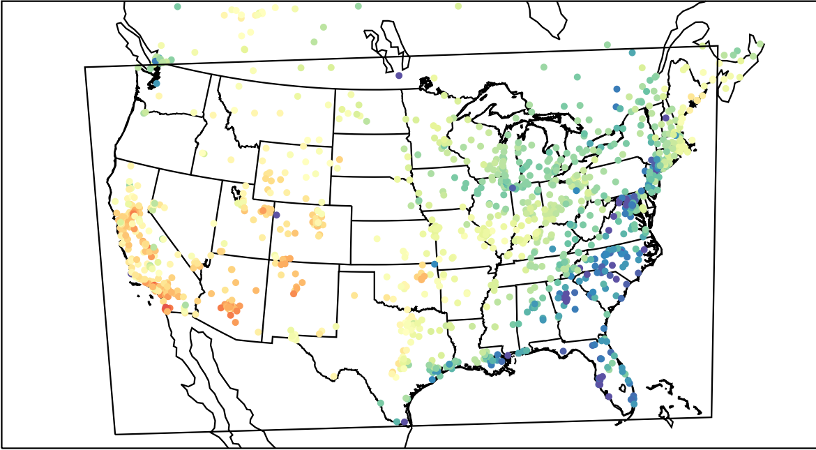
AirNOW (2021-03-31_23:00:00)
