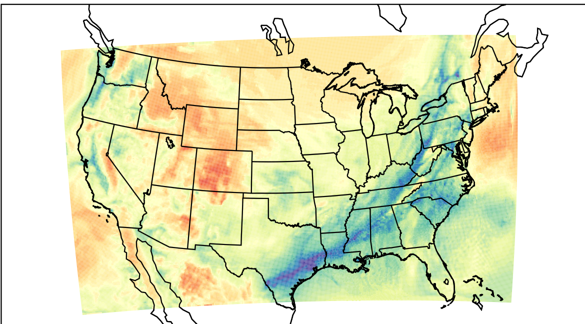
WRF (2021-03-31_16:00:00)
