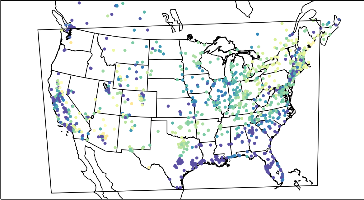
AirNOW (2021-03-31_10:00:00)
