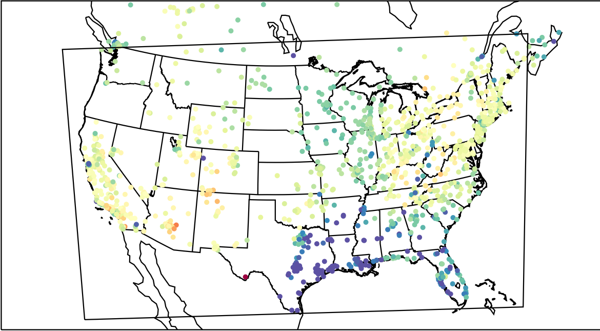
AirNOW (2021-03-31_01:00:00)
