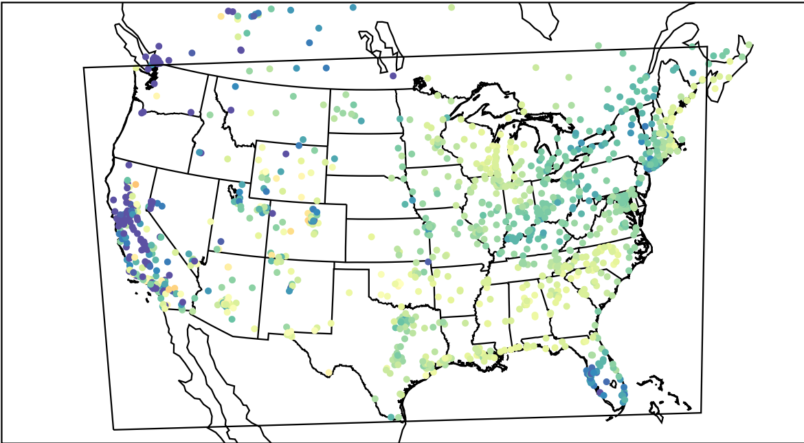
AirNOW (2021-04-01_15:00:00)
