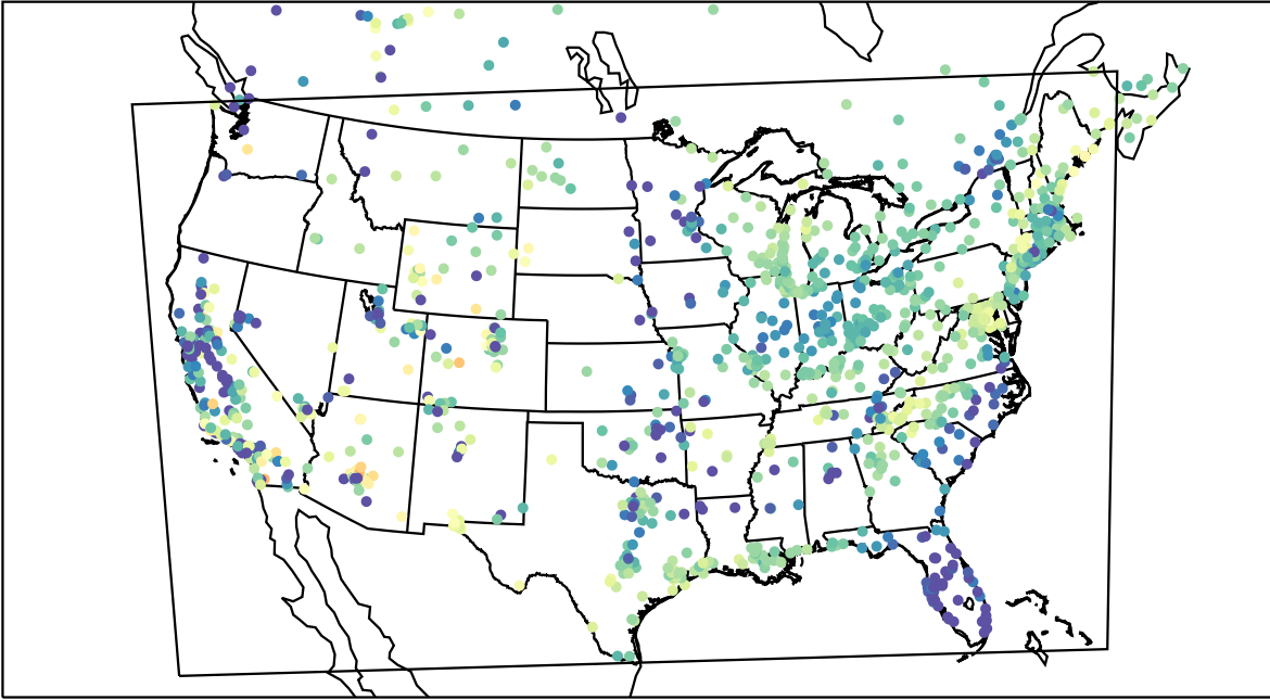
AirNOW (2021-04-01_06:00:00)
