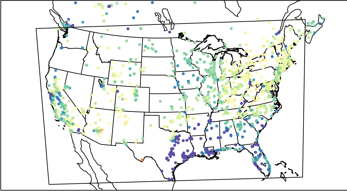
AirNOW (2021-03-31_03:00:00)
