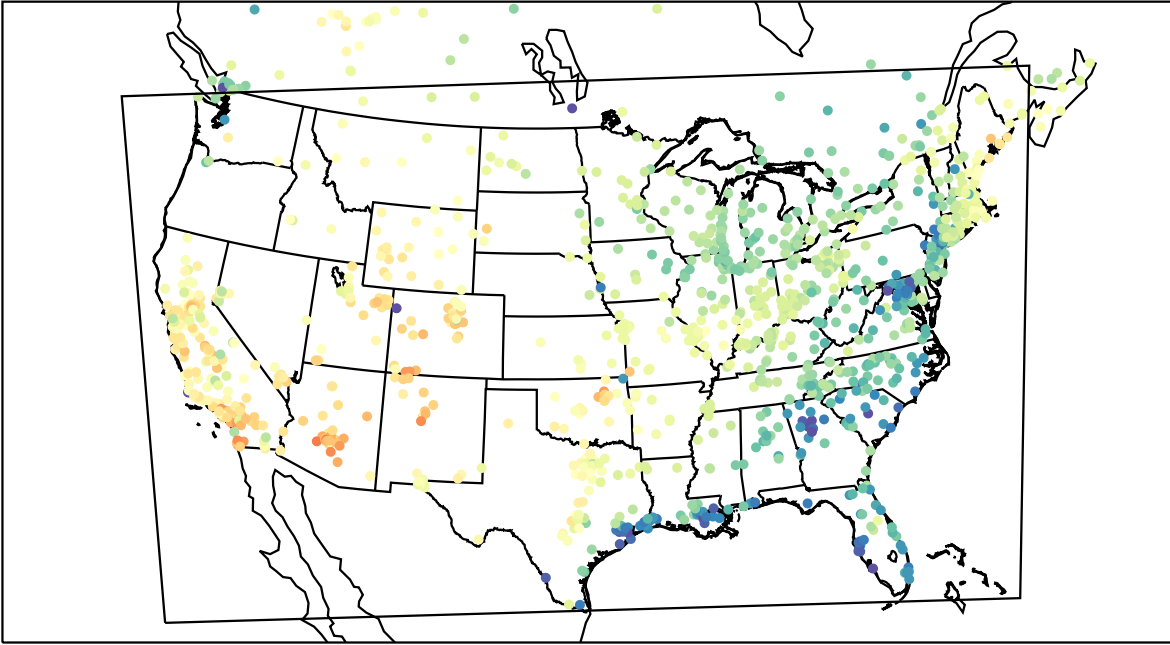
AirNOW (2021-03-31_21:00:00)
