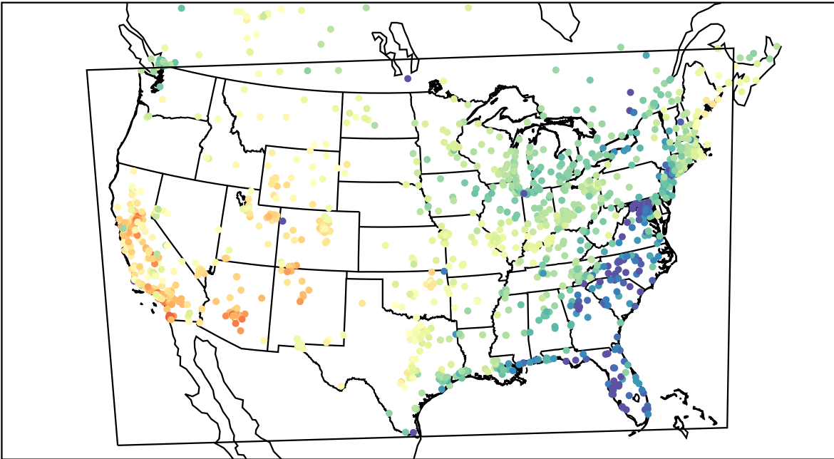
AirNOW (2021-04-01_00:00:00)
