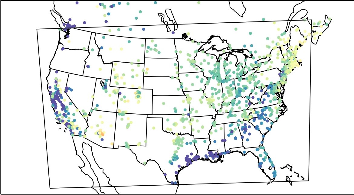
AirNOW (2021-03-31_15:00:00)
