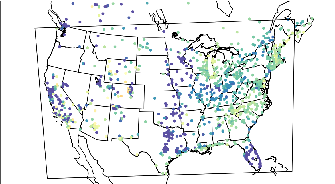
AirNOW (2021-04-01_12:00:00)
