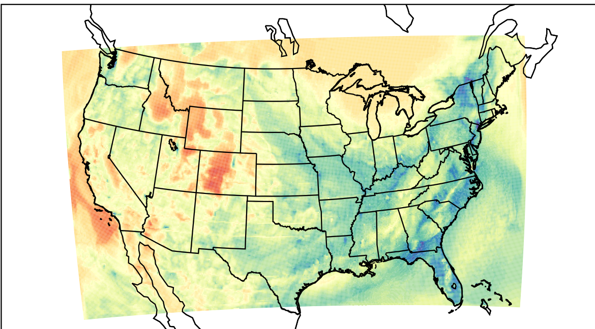
WRF (2021-04-01_04:00:00)
