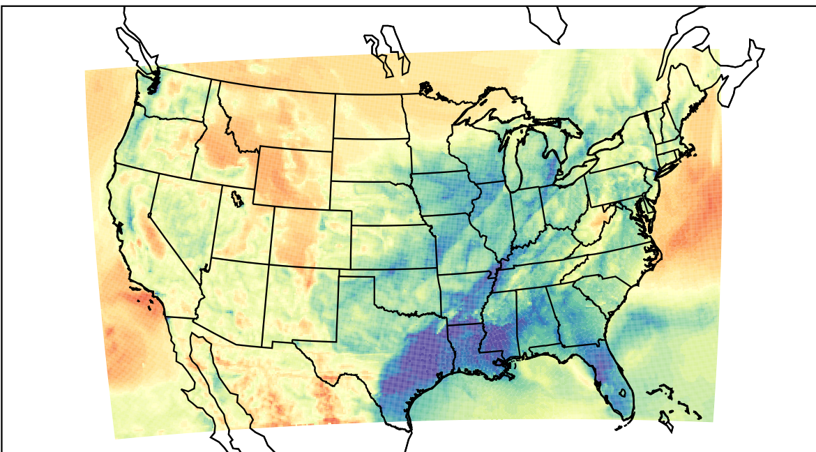
WRF (2021-03-31_05:00:00)
