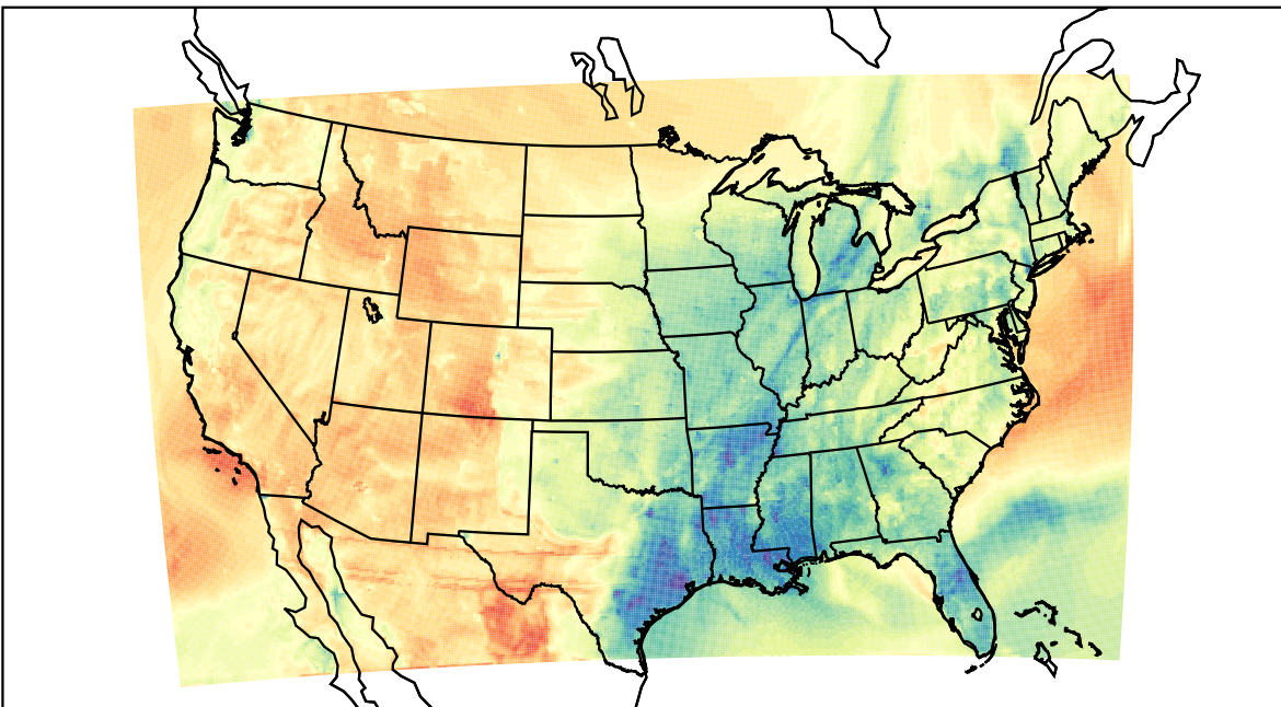
WRF (2021-03-31_01:00:00)
