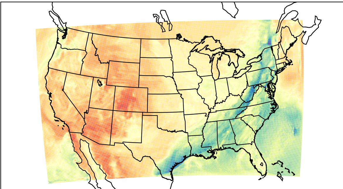
WRF (2021-03-31_21:00:00)
