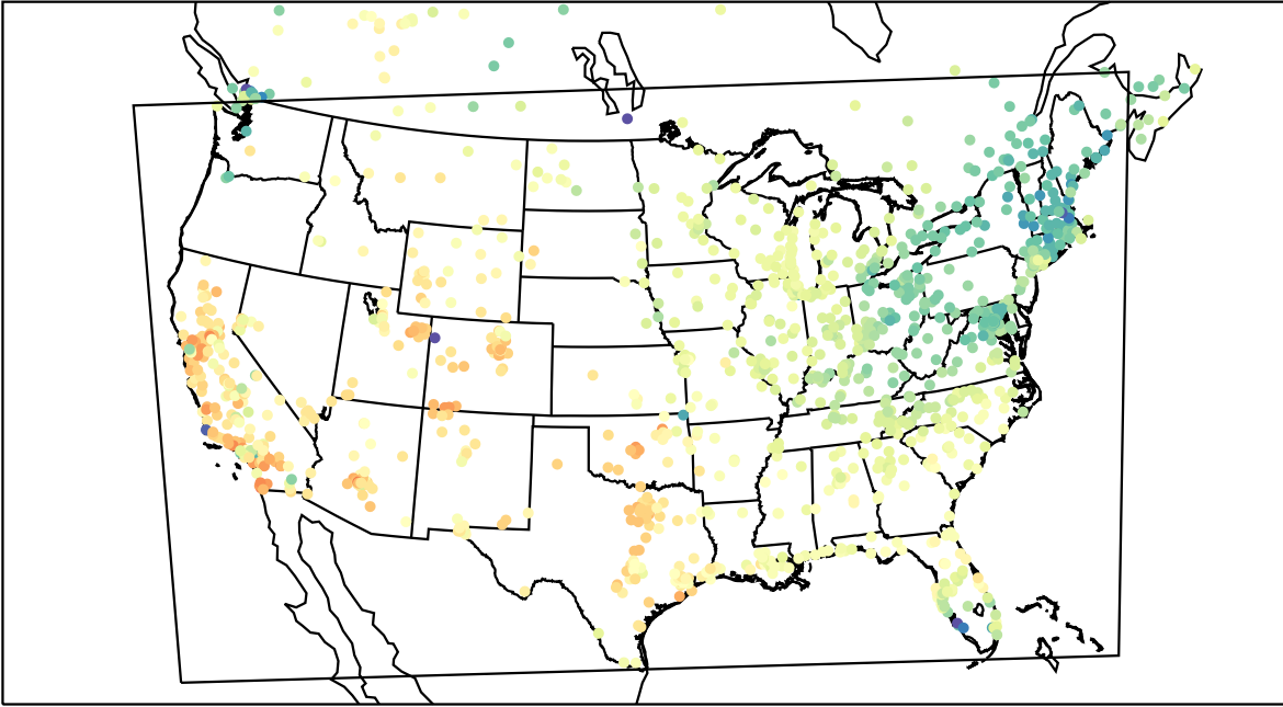
AirNOW (2021-04-01_20:00:00)
