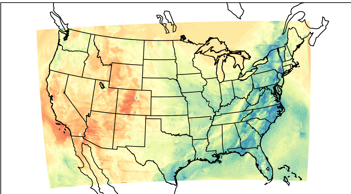
WRF (2021-04-01_01:00:00)
