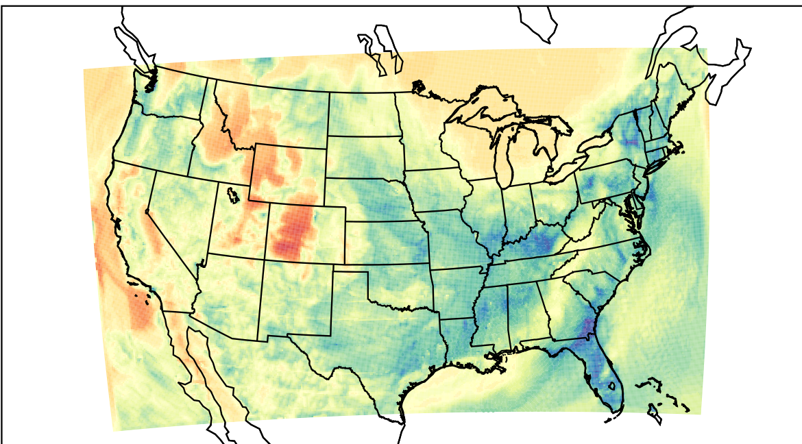
WRF (2021-04-01_08:00:00)
