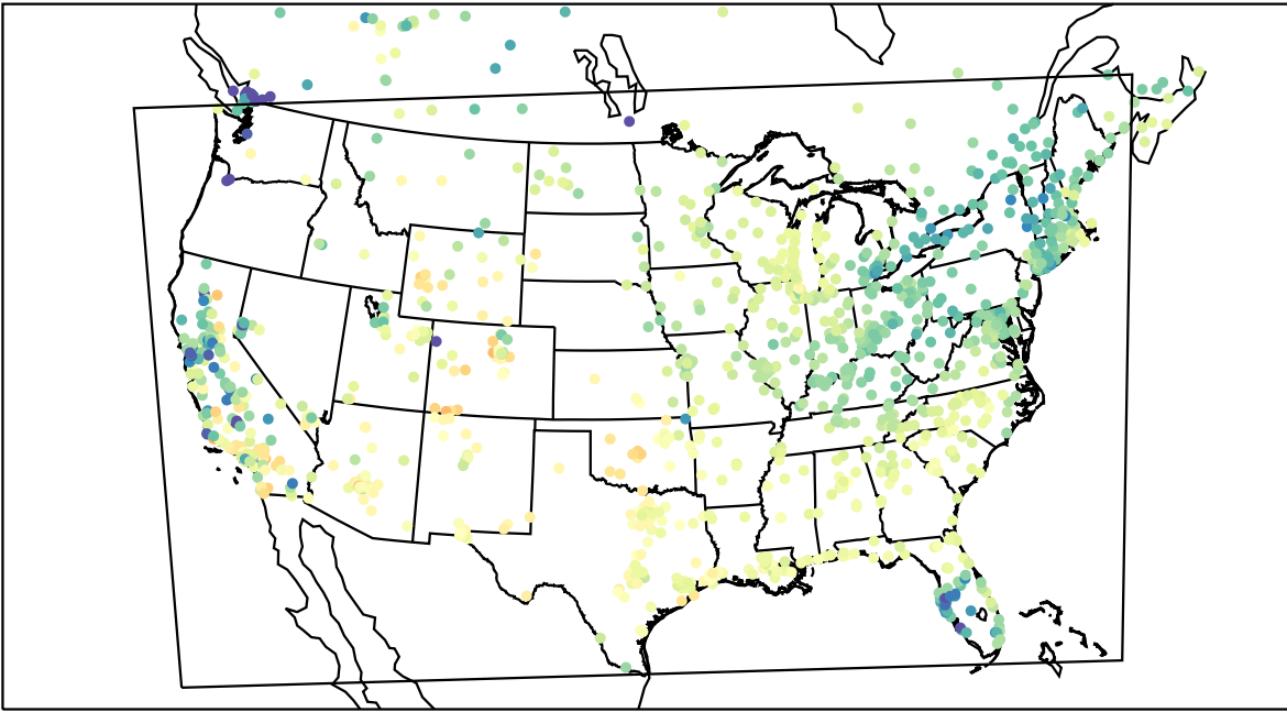
AirNOW (2021-04-01_17:00:00)
