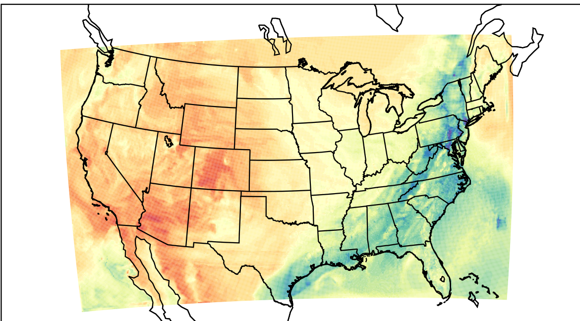
WRF (2021-03-31_23:00:00)
