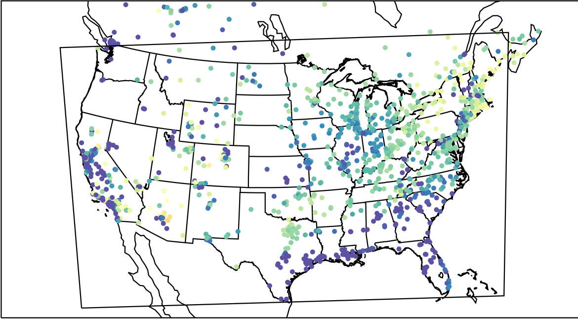
AirNOW (2021-03-31_12:00:00)
