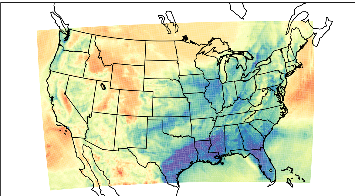
WRF (2021-03-31_09:00:00)
