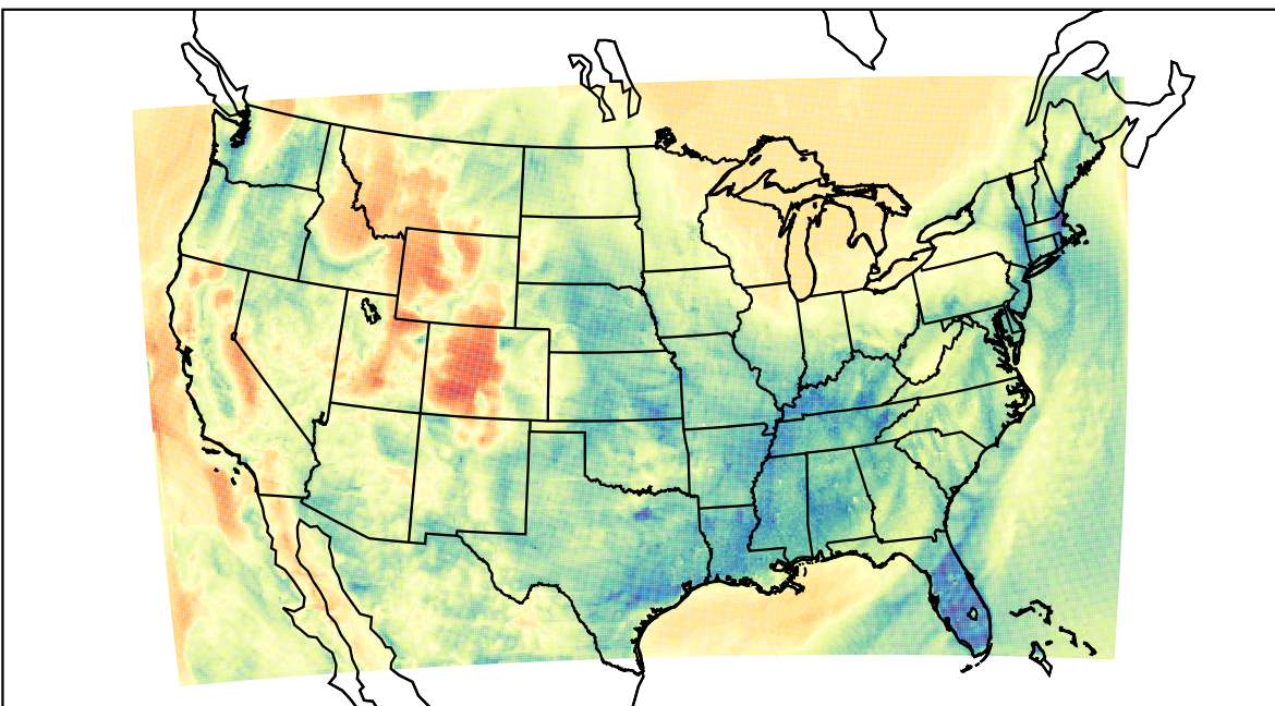
WRF (2021-04-01_12:00:00)
