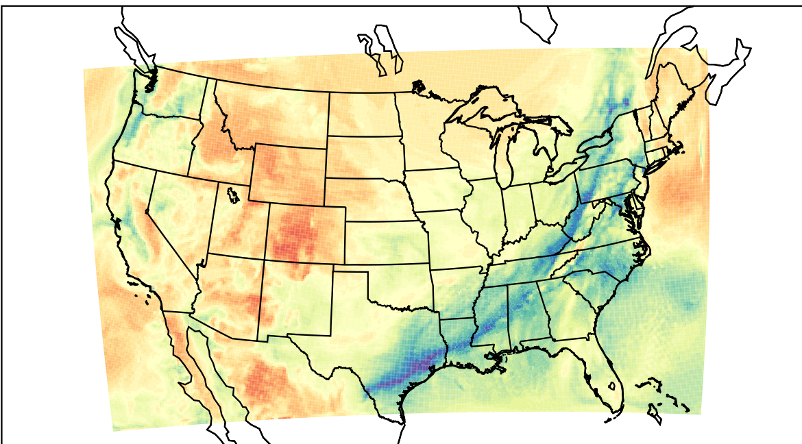
WRF (2021-03-31_17:00:00)
