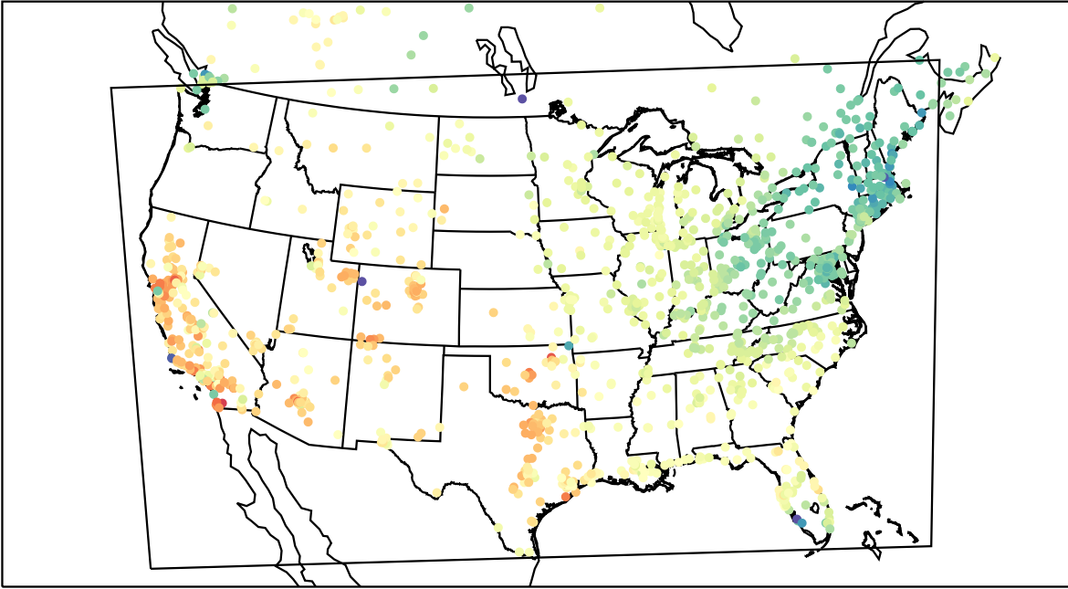
AirNOW (2021-04-01_21:00:00)
