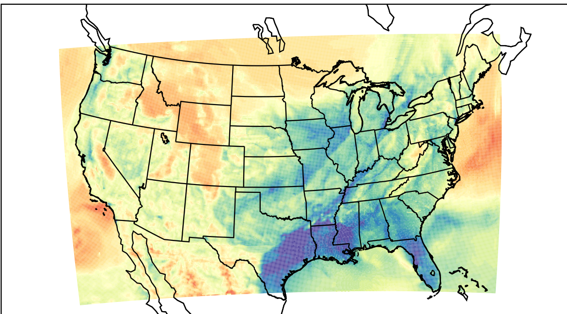
WRF (2021-03-31_06:00:00)
