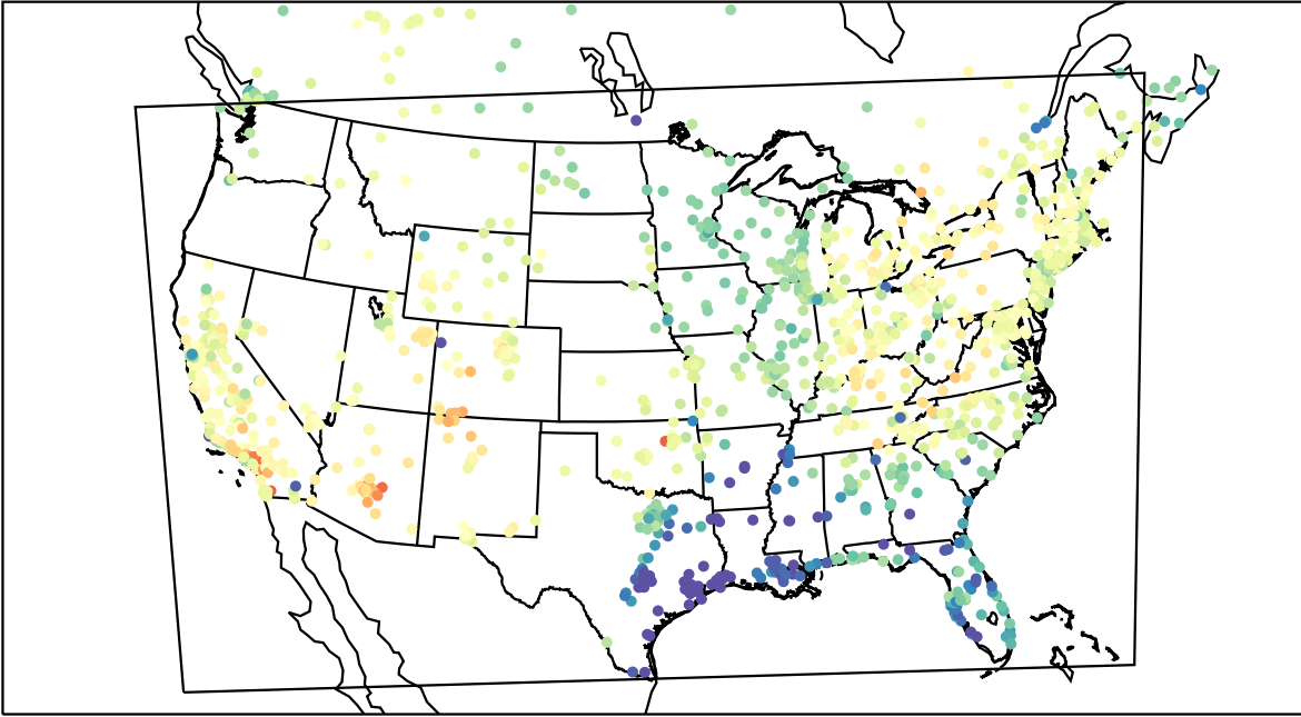
AirNOW (2021-03-31_00:00:00)
