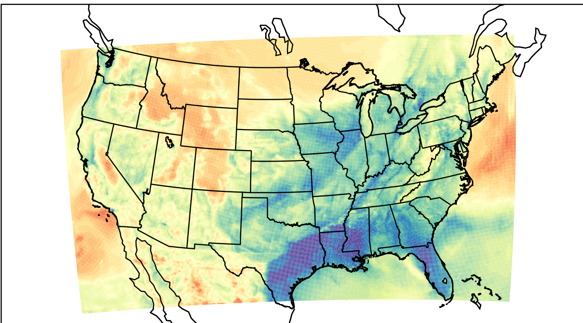
WRF (2021-03-31_07:00:00)
