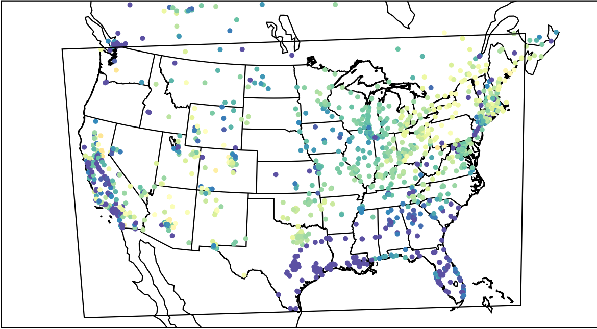
AirNOW (2021-03-31_08:00:00)
