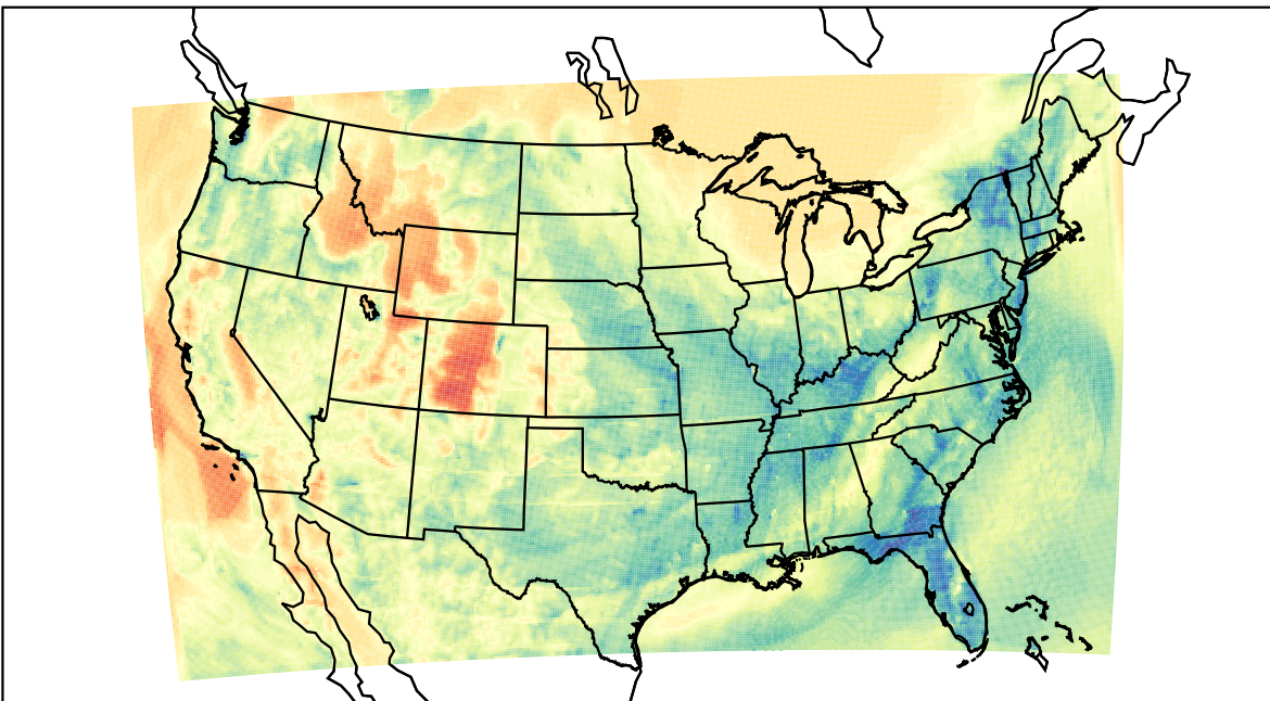
WRF (2021-04-01_06:00:00)
