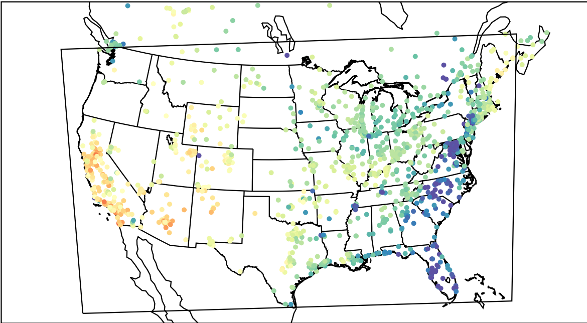
AirNOW (2021-04-01_01:00:00)
