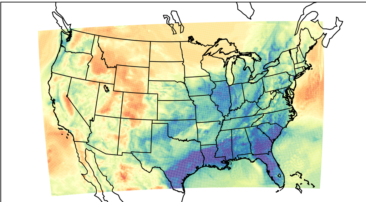
WRF (2021-03-31_12:00:00)
