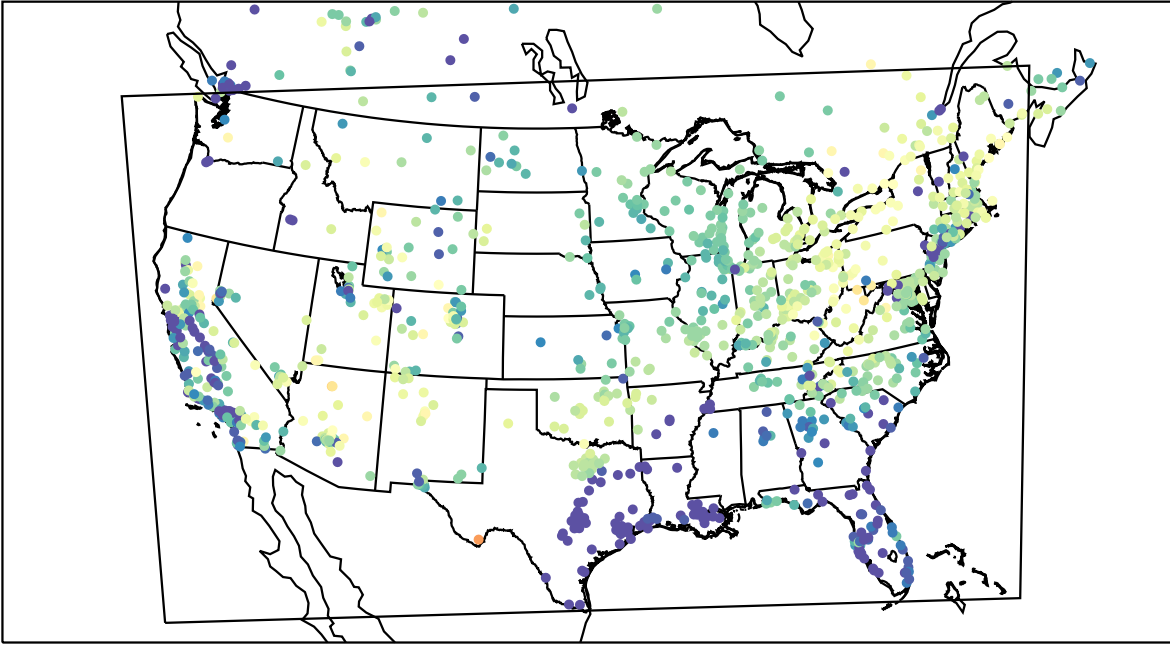
AirNOW (2021-03-31_06:00:00)
