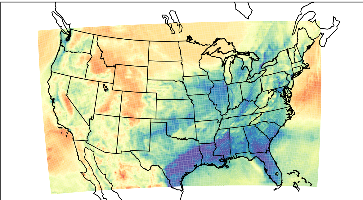
WRF (2021-03-31_10:00:00)
