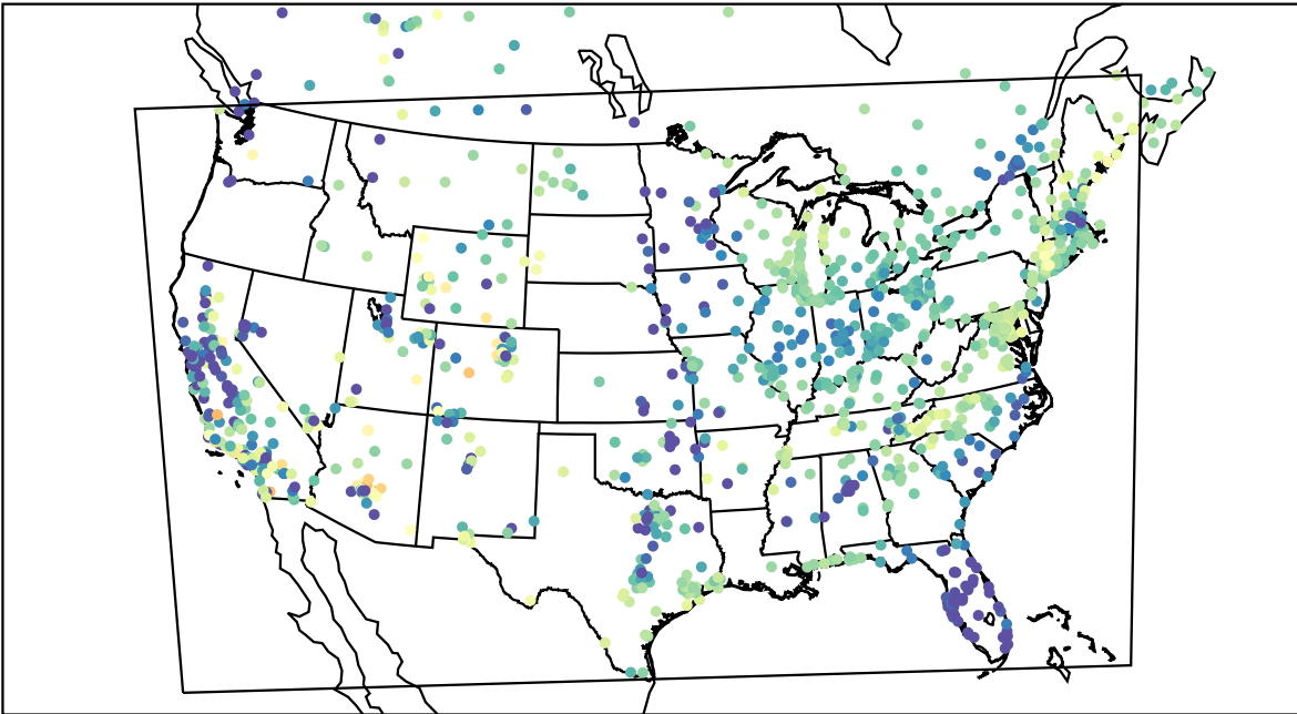
AirNOW (2021-04-01_07:00:00)
