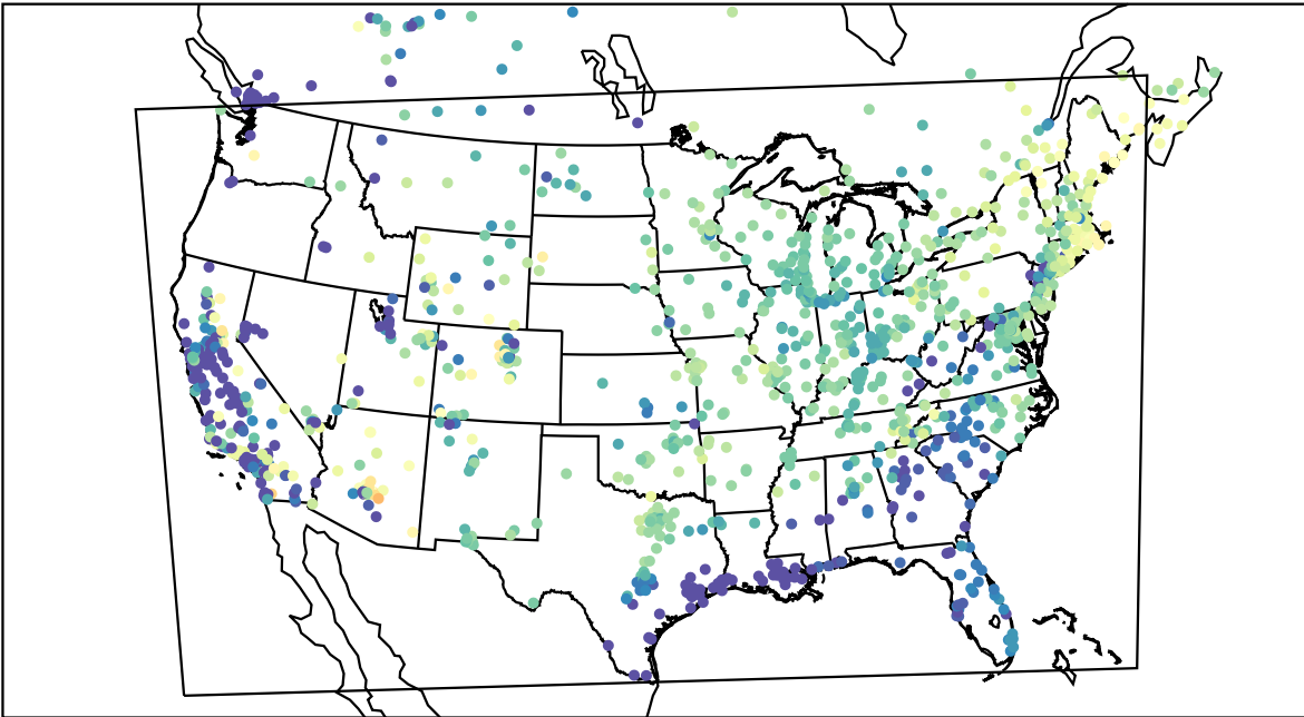
AirNOW (2021-03-31_14:00:00)
