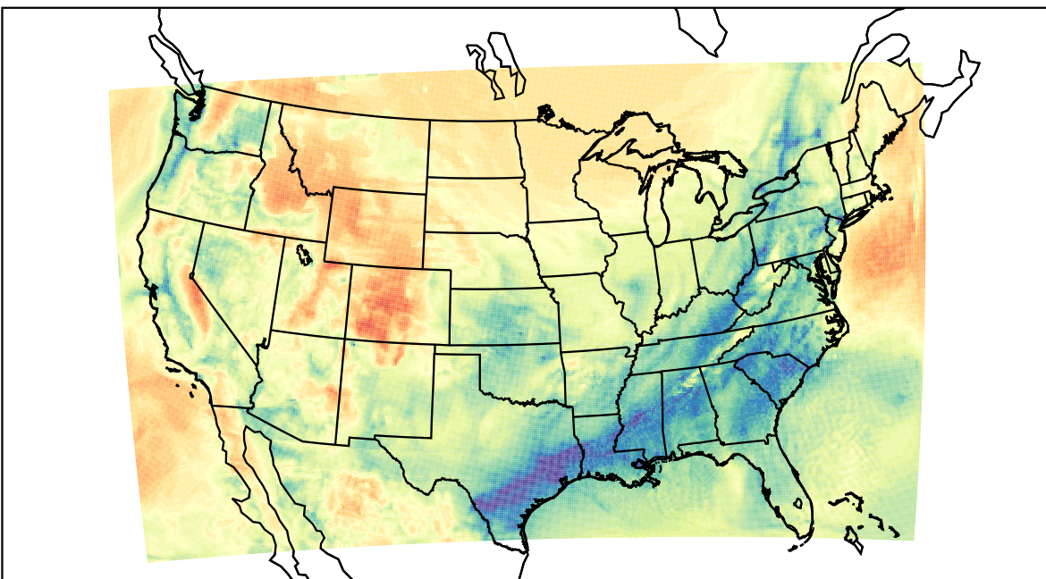
WRF (2021-03-31_15:00:00)
