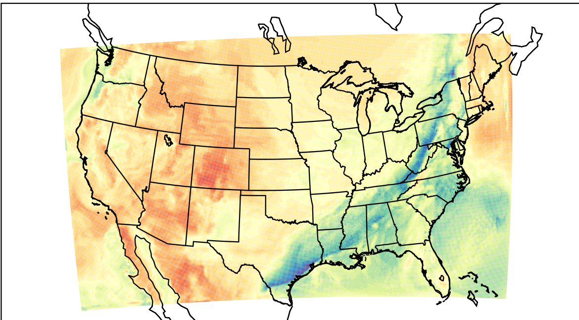
WRF (2021-03-31_19:00:00)
