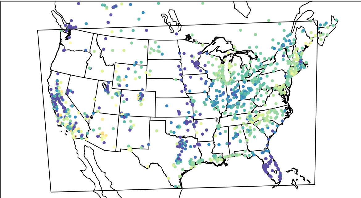
AirNOW (2021-04-01_09:00:00)
