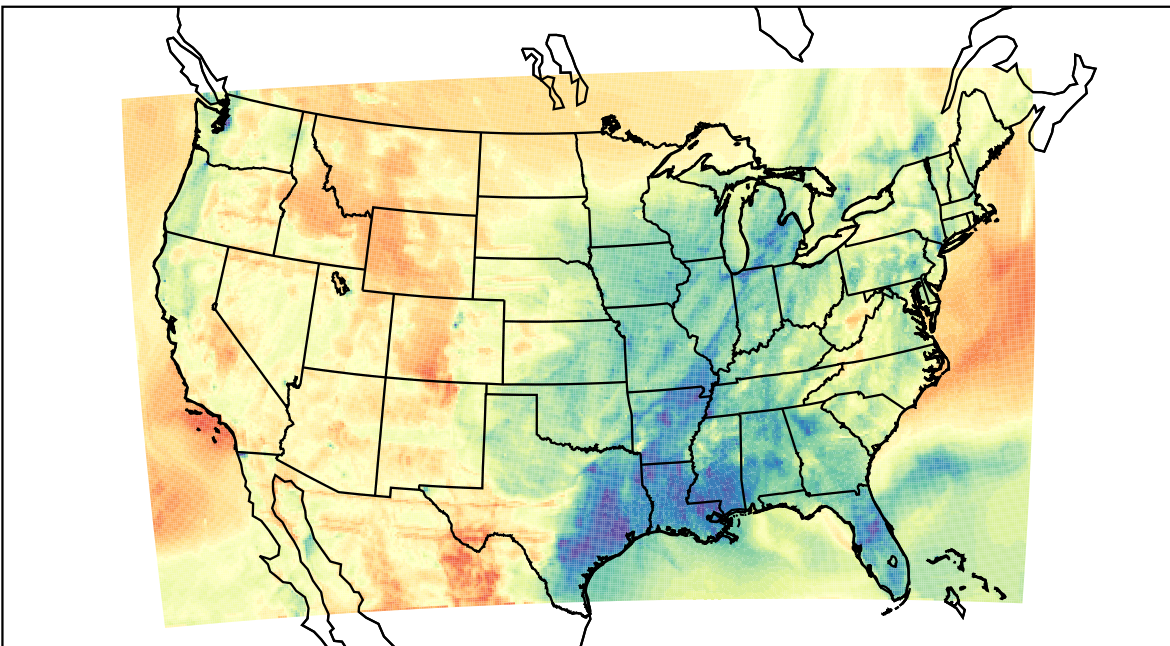
WRF (2021-03-31_02:00:00)
