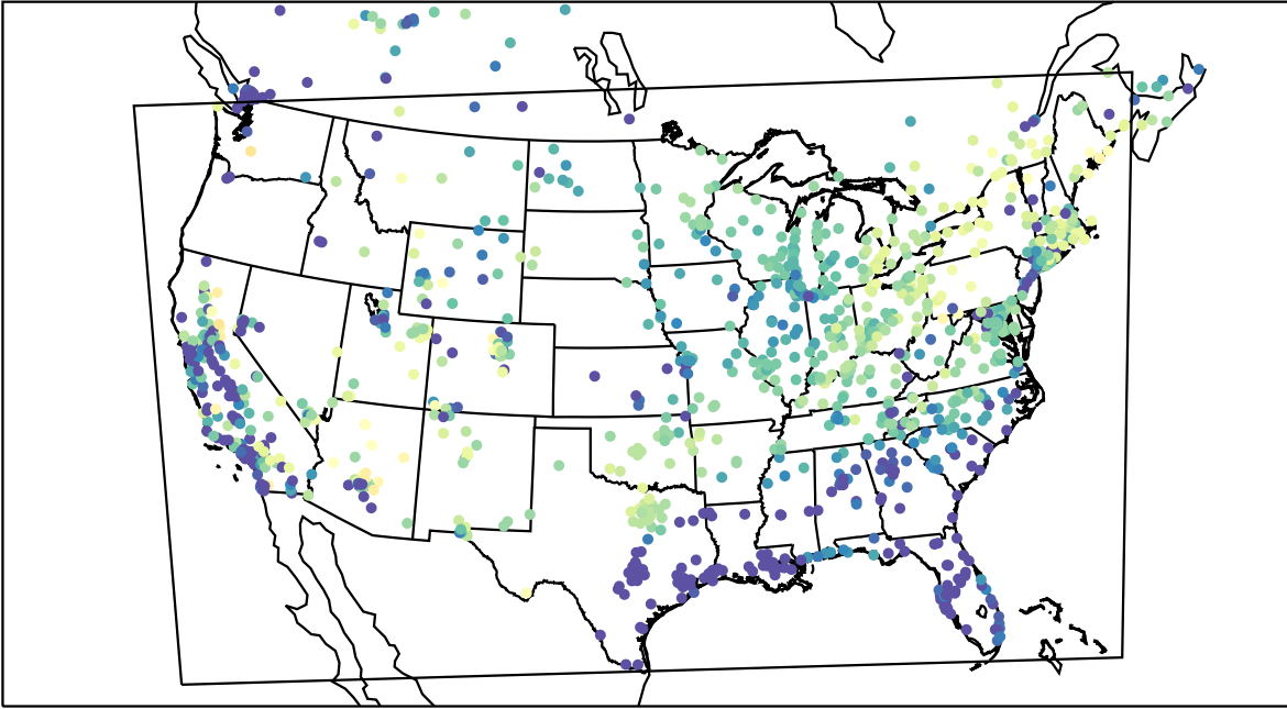
AirNOW (2021-03-31_09:00:00)
