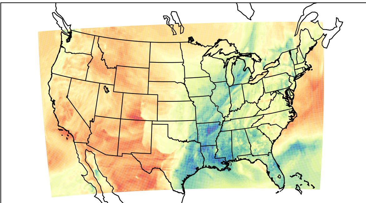
WRF (2021-03-31_00:00:00)
