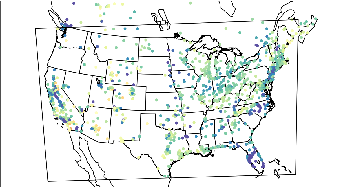
AirNOW (2021-04-01_04:00:00)
