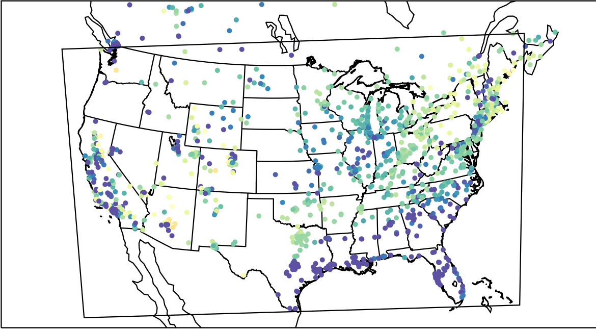
AirNOW (2021-03-31_11:00:00)
