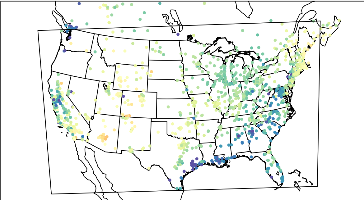
AirNOW (2021-03-31_17:00:00)
