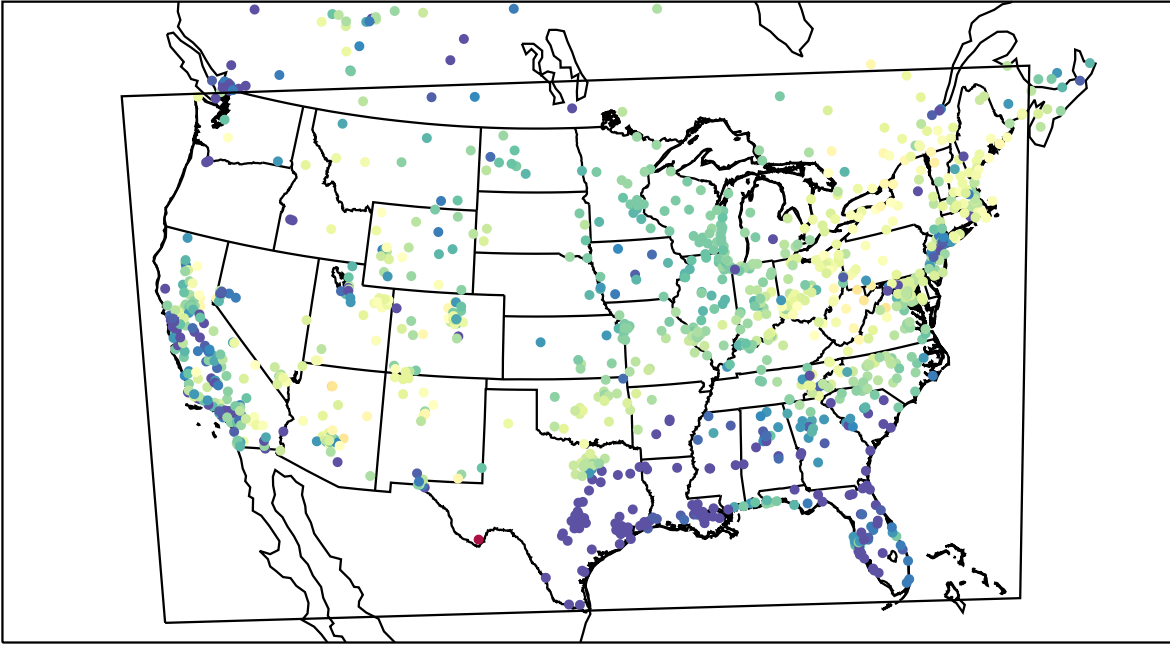
AirNOW (2021-03-31_05:00:00)
