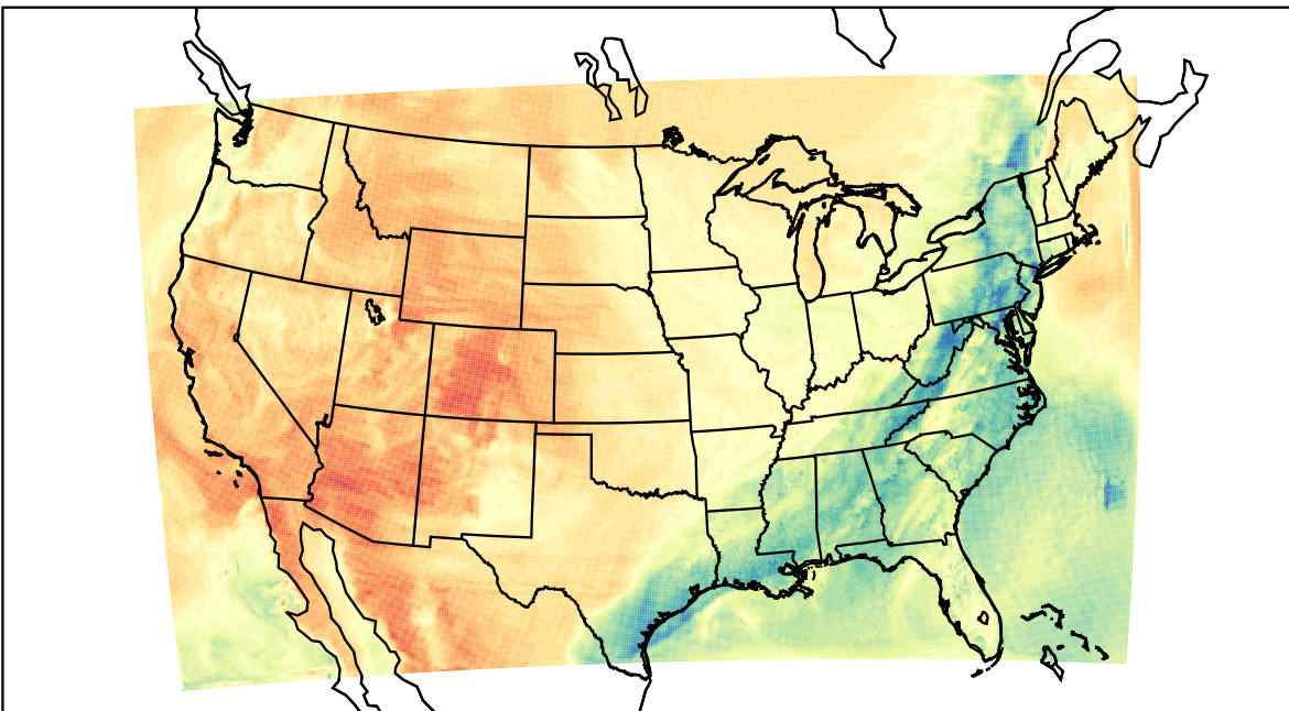
WRF (2021-03-31_22:00:00)
