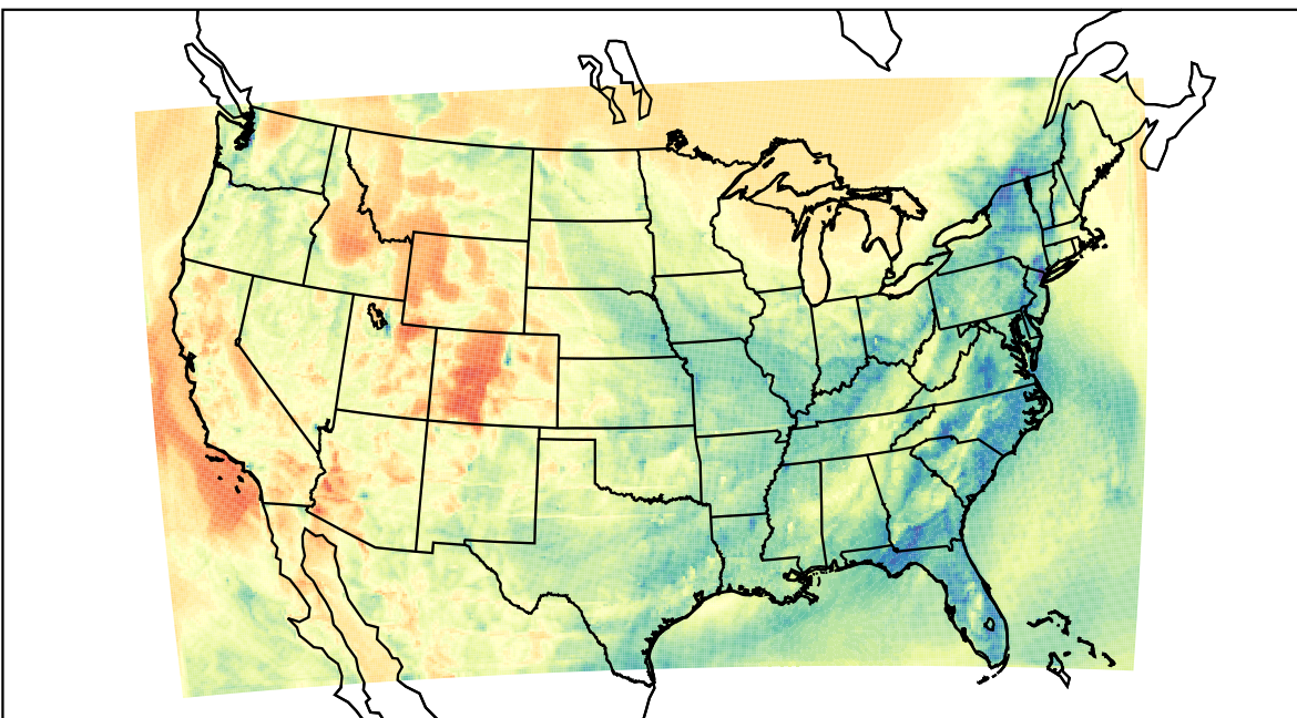
WRF (2021-04-01_03:00:00)
