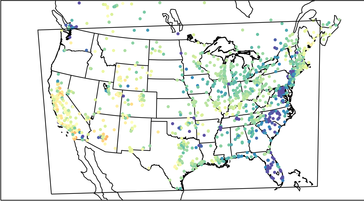
AirNOW (2021-04-01_02:00:00)
