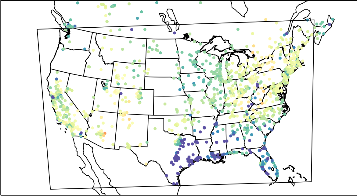
AirNOW (2021-03-31_02:00:00)
