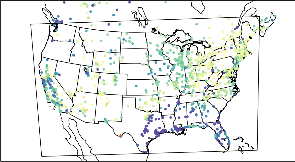
AirNOW (2021-03-31_04:00:00)
