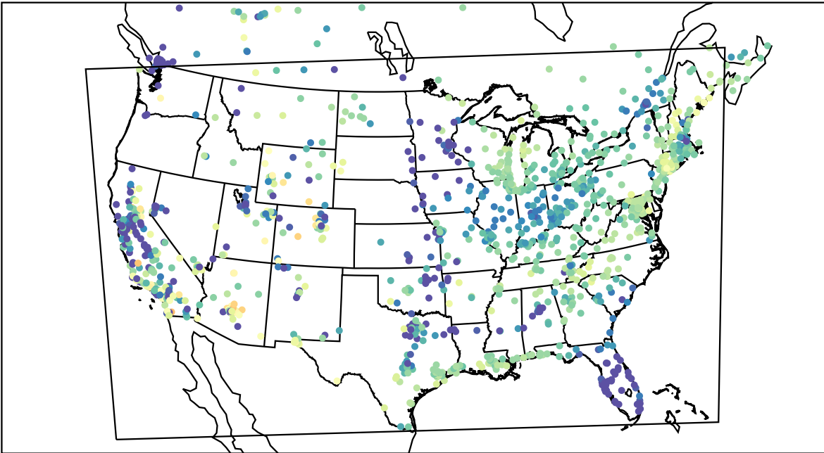
AirNOW (2021-04-01_08:00:00)
