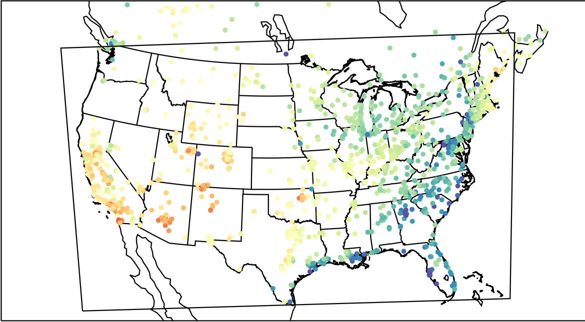
AirNOW (2021-03-31_22:00:00)
