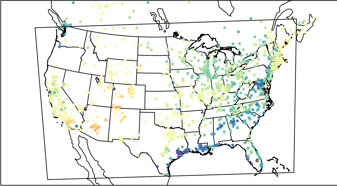
AirNOW (2021-03-31_19:00:00)
