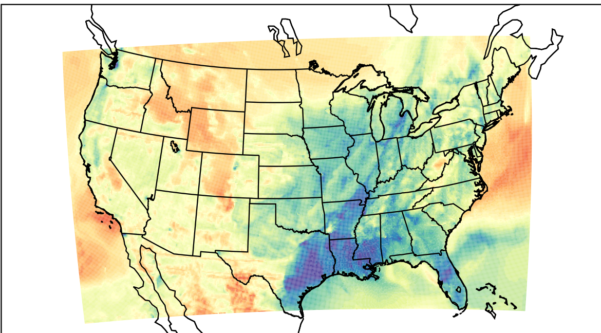
WRF (2021-03-31_03:00:00)
