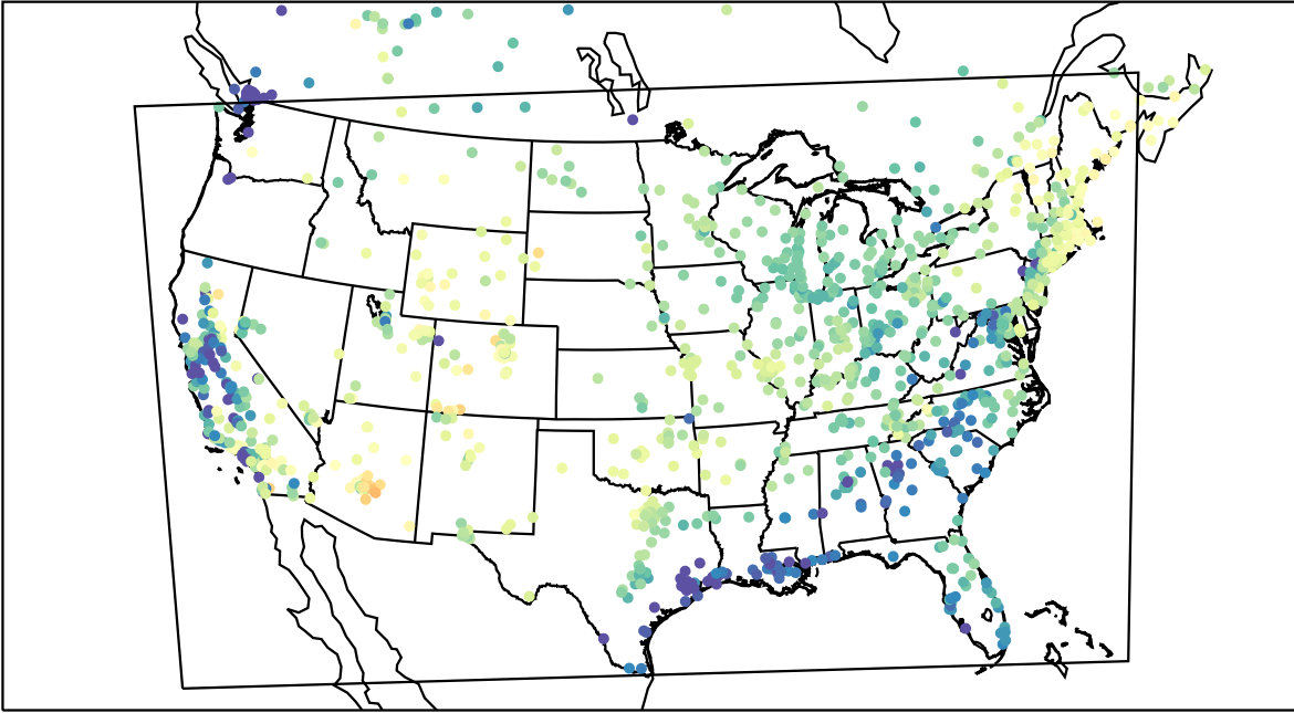
AirNOW (2021-03-31_16:00:00)
