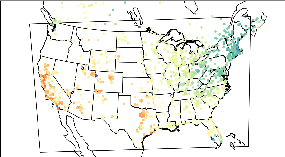
AirNOW (2021-04-01_22:00:00)
