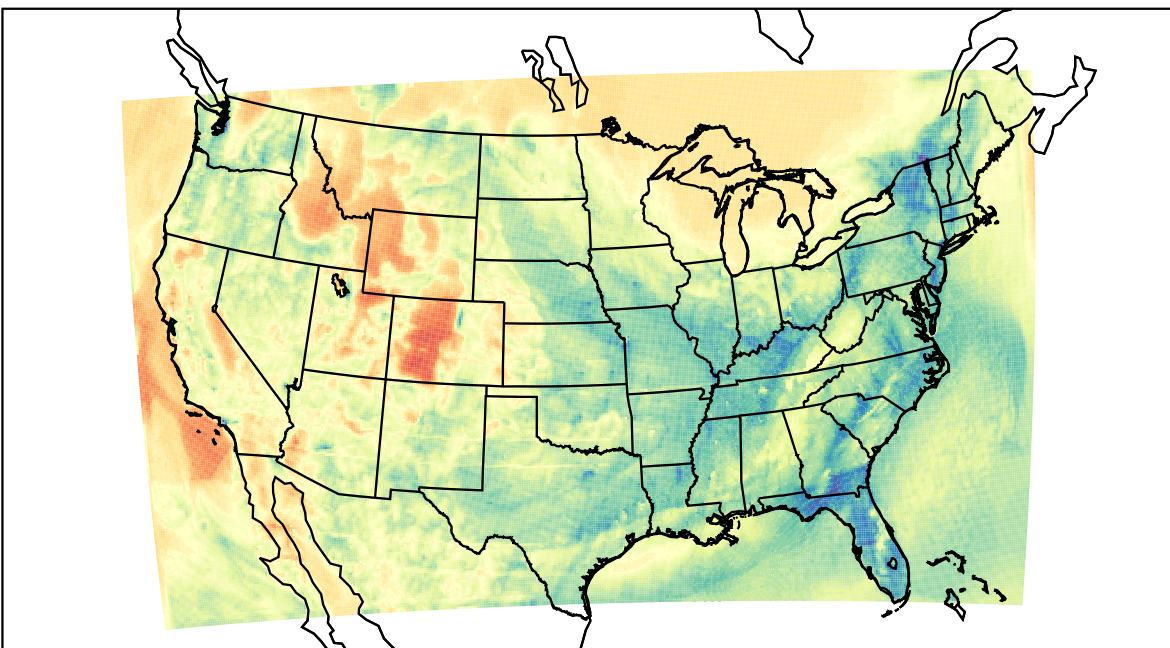
WRF (2021-04-01_05:00:00)
