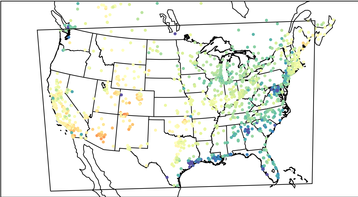
AirNOW (2021-03-31_20:00:00)
