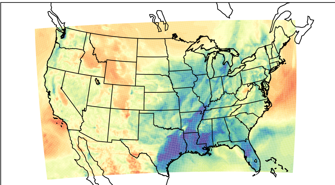
WRF (2021-03-31_04:00:00)
