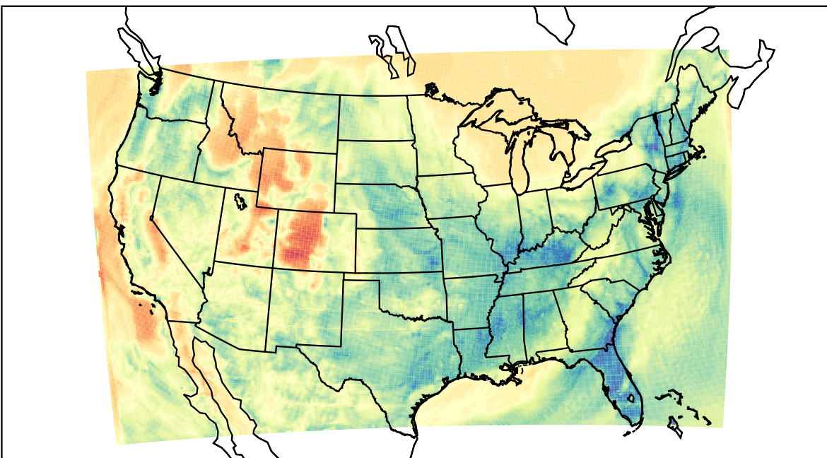
WRF (2021-04-01_09:00:00)
