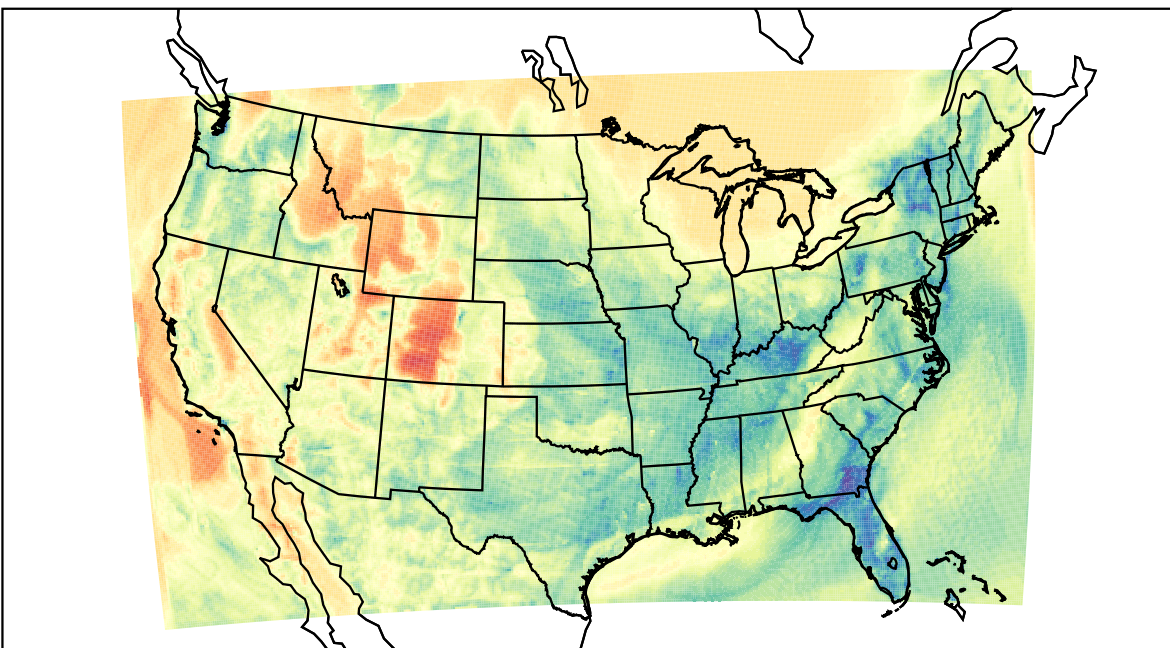
WRF (2021-04-01_07:00:00)
