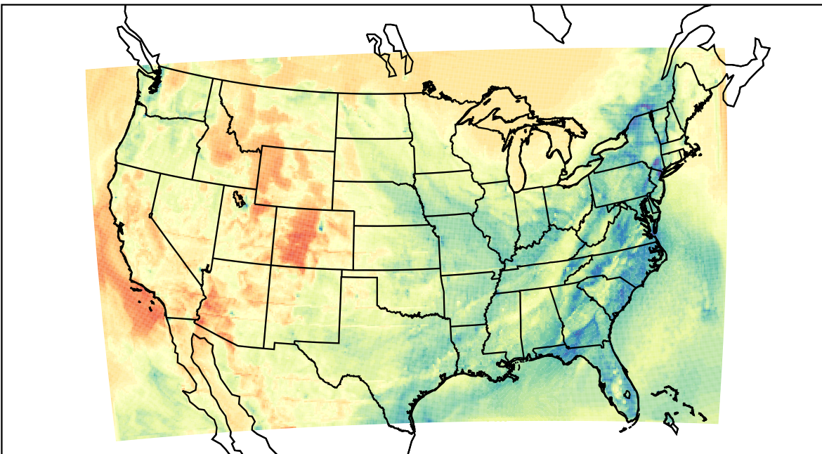
WRF (2021-04-01_02:00:00)
