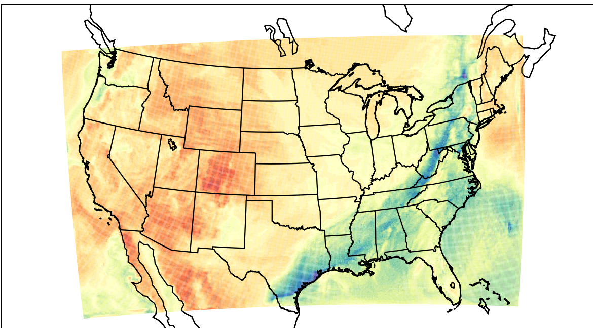
WRF (2021-03-31_20:00:00)
