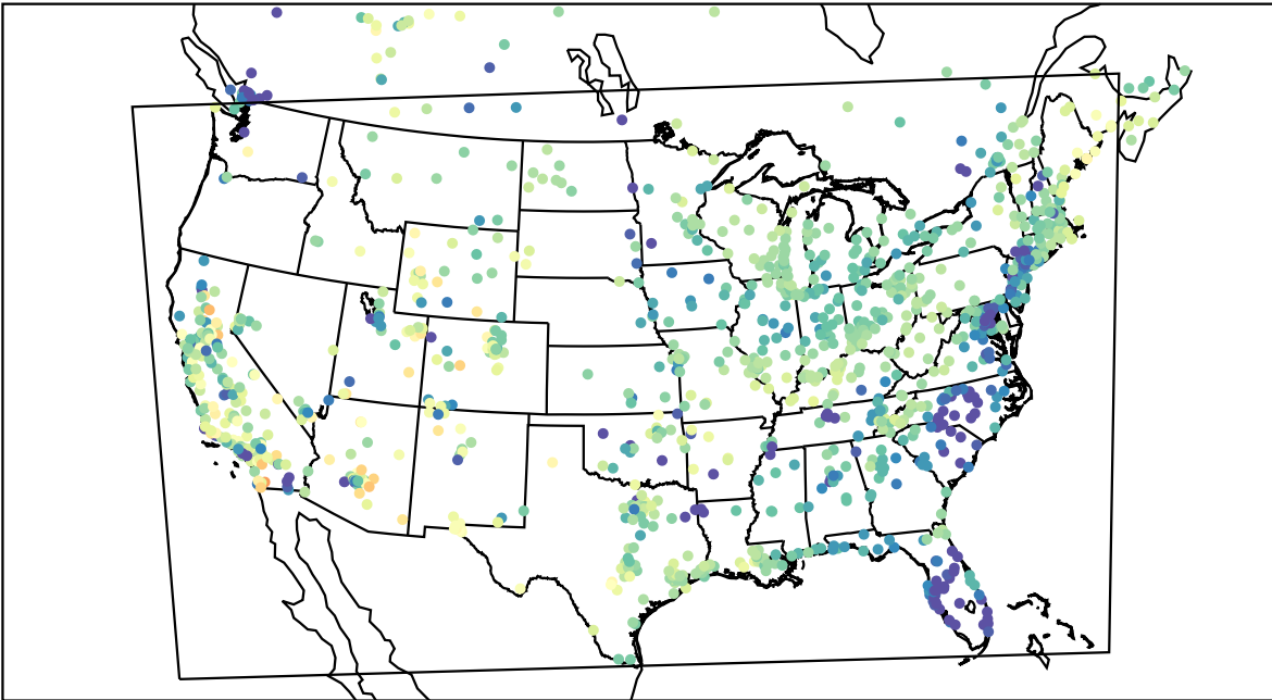
AirNOW (2021-04-01_03:00:00)
