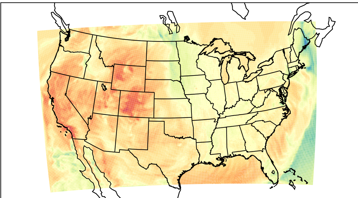
WRF (2021-04-01_21:00:00)
