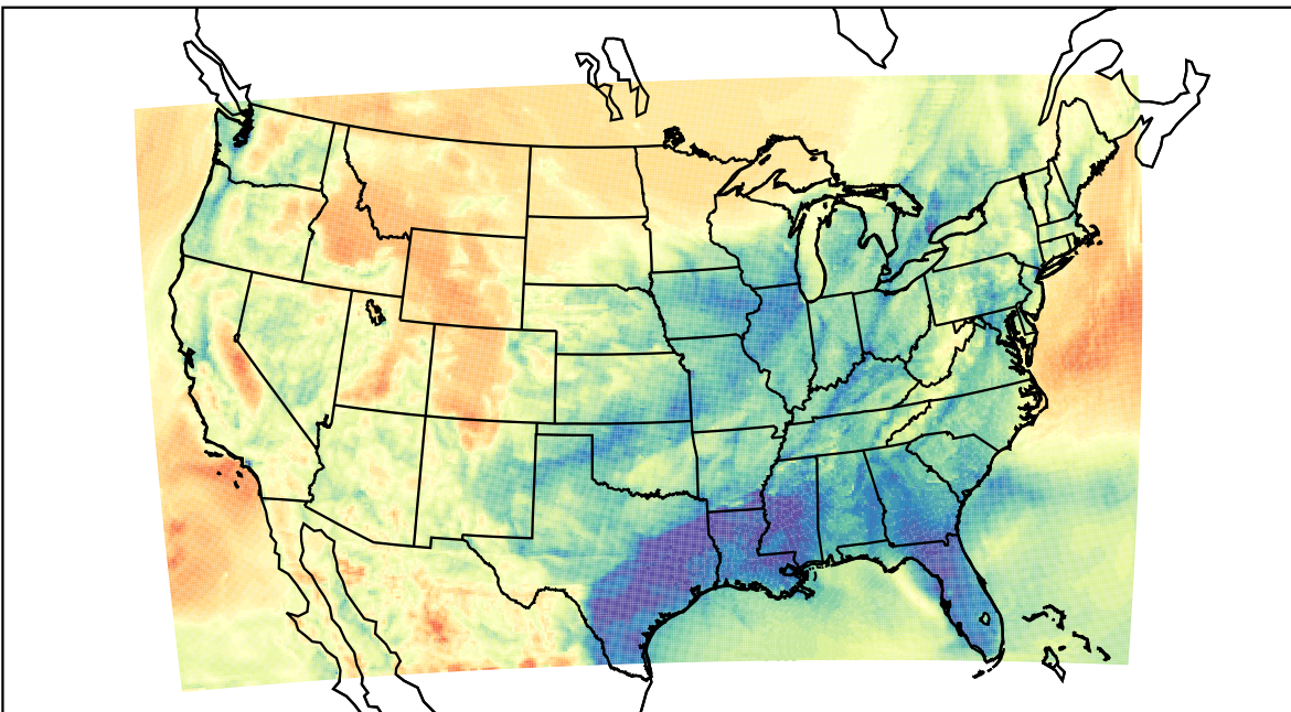
WRF (2021-03-31_08:00:00)
