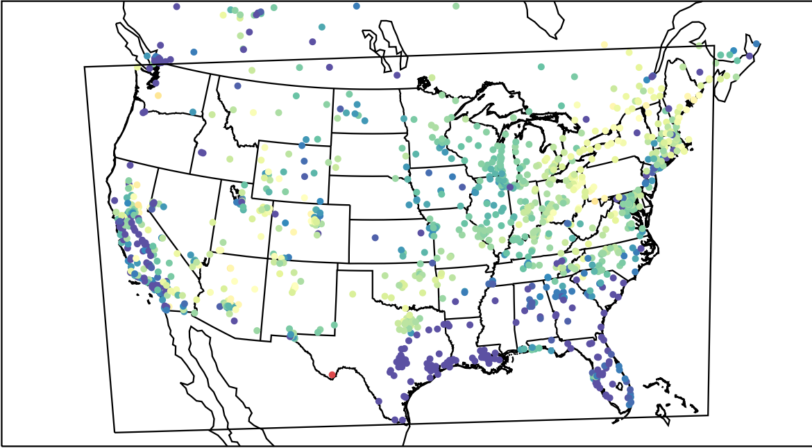
AirNOW (2021-03-31_07:00:00)
