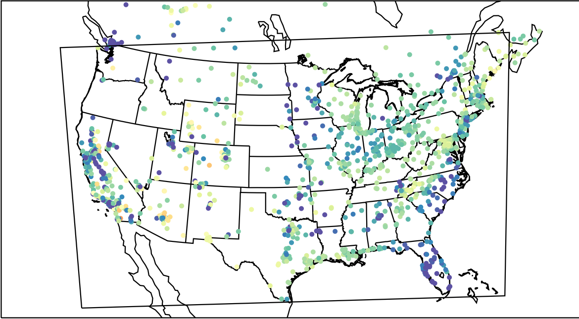
AirNOW (2021-04-01_05:00:00)
