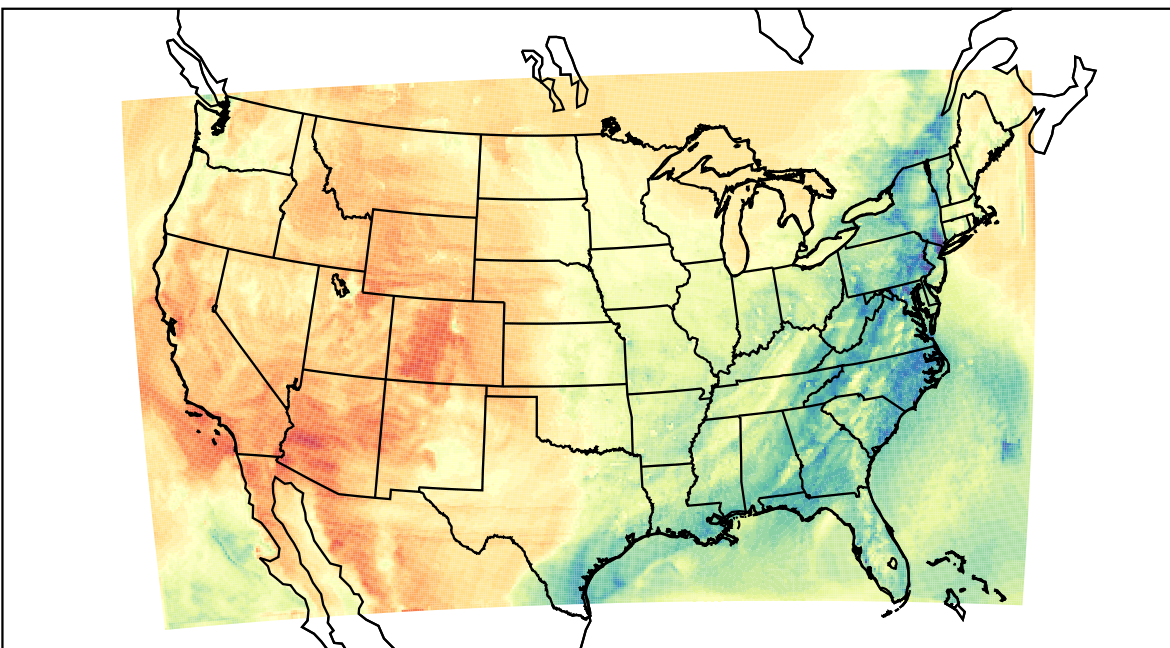
WRF (2021-04-01_00:00:00)
