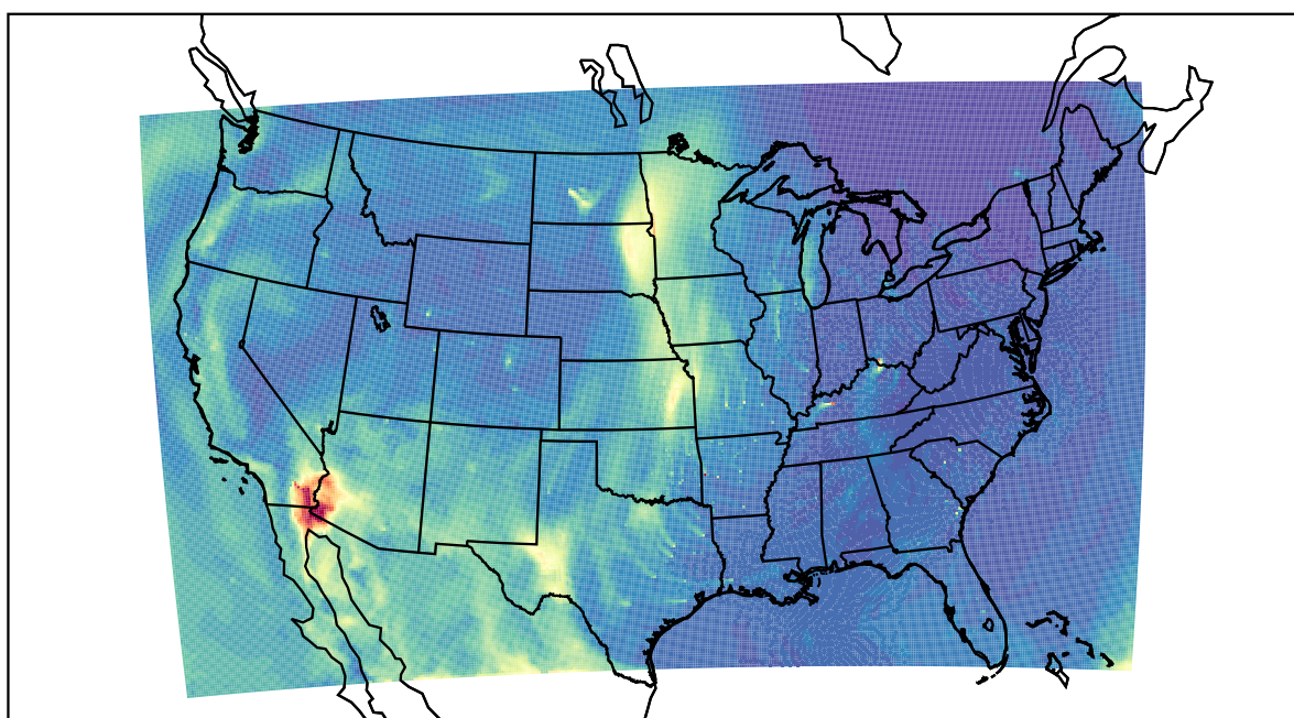
WRF 2021-04-02_17:00:00
