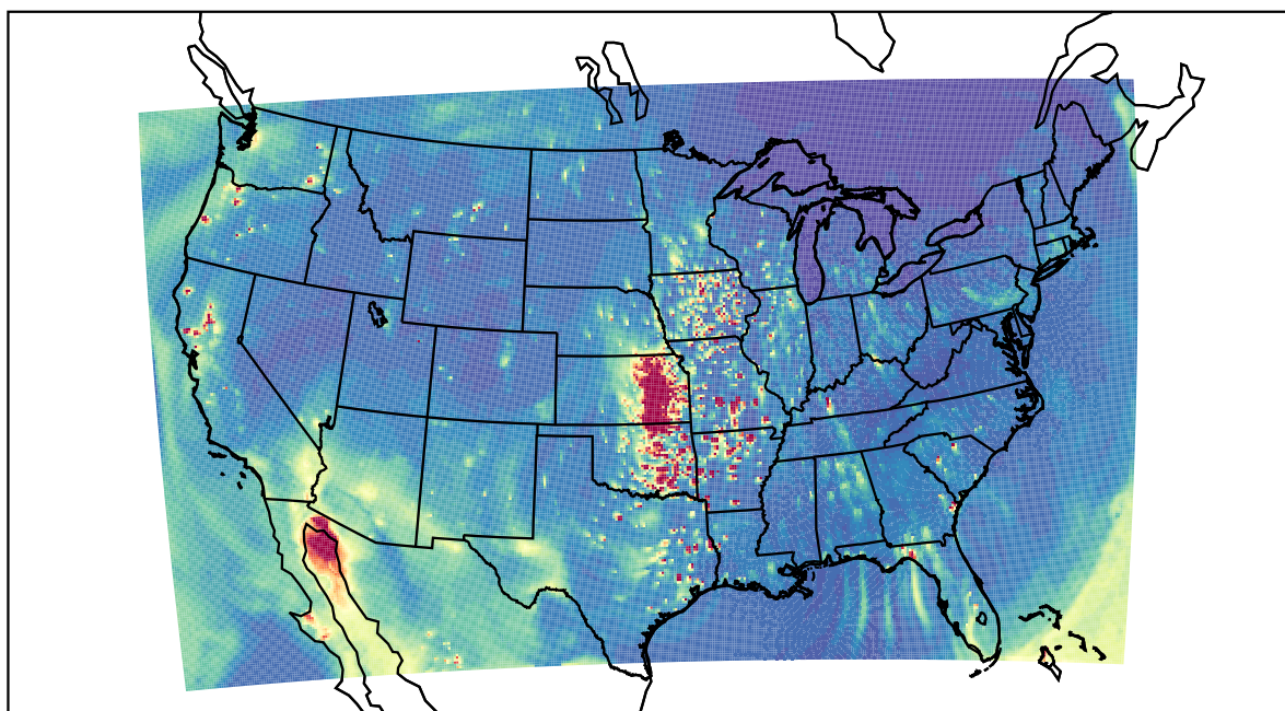
WRF 2021-04-02_02:00:00
