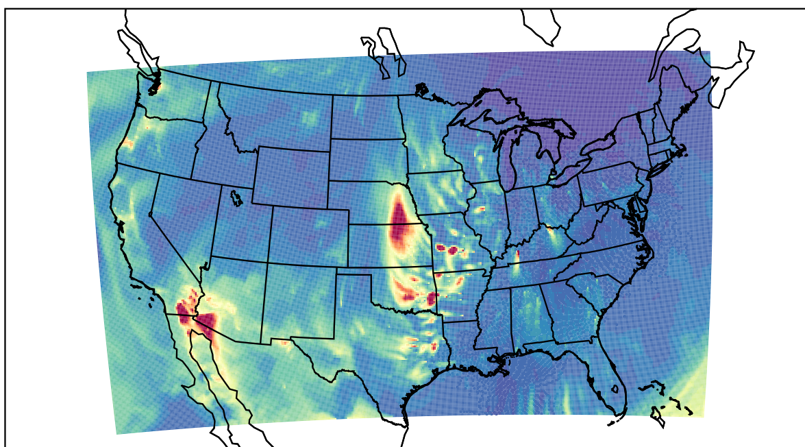
WRF 2021-04-02_07:00:00
