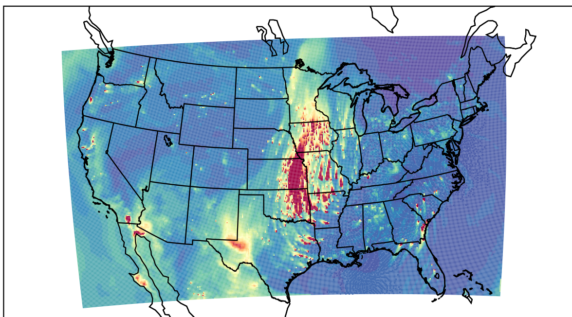
WRF 2021-04-03_01:00:00
