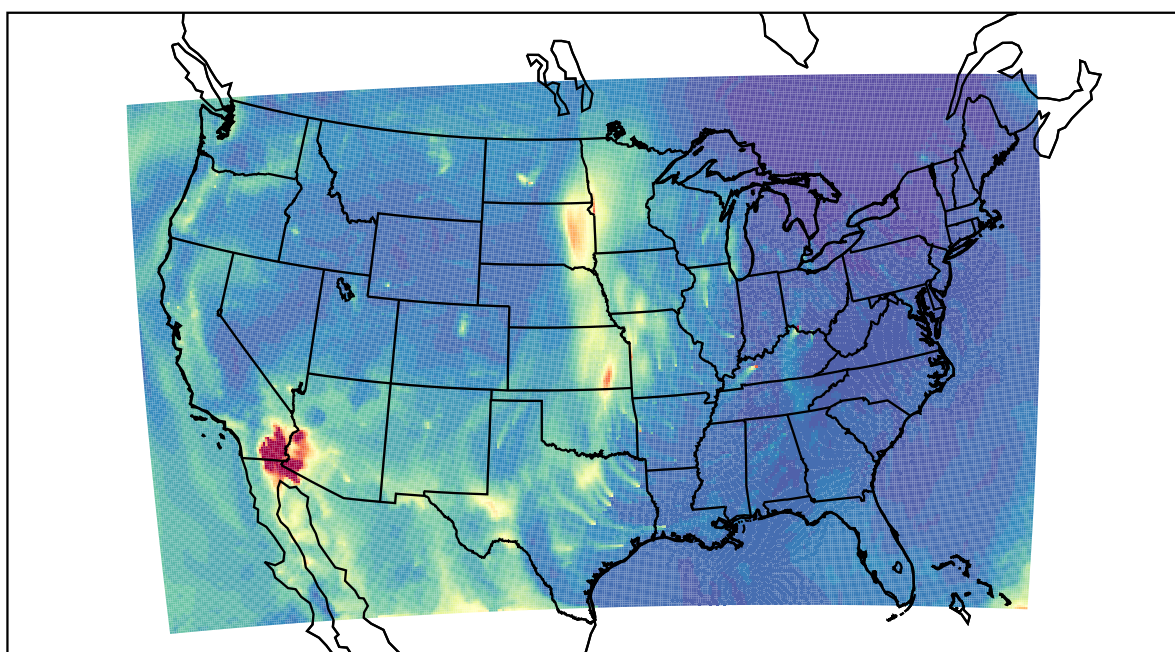
WRF 2021-04-02_15:00:00
