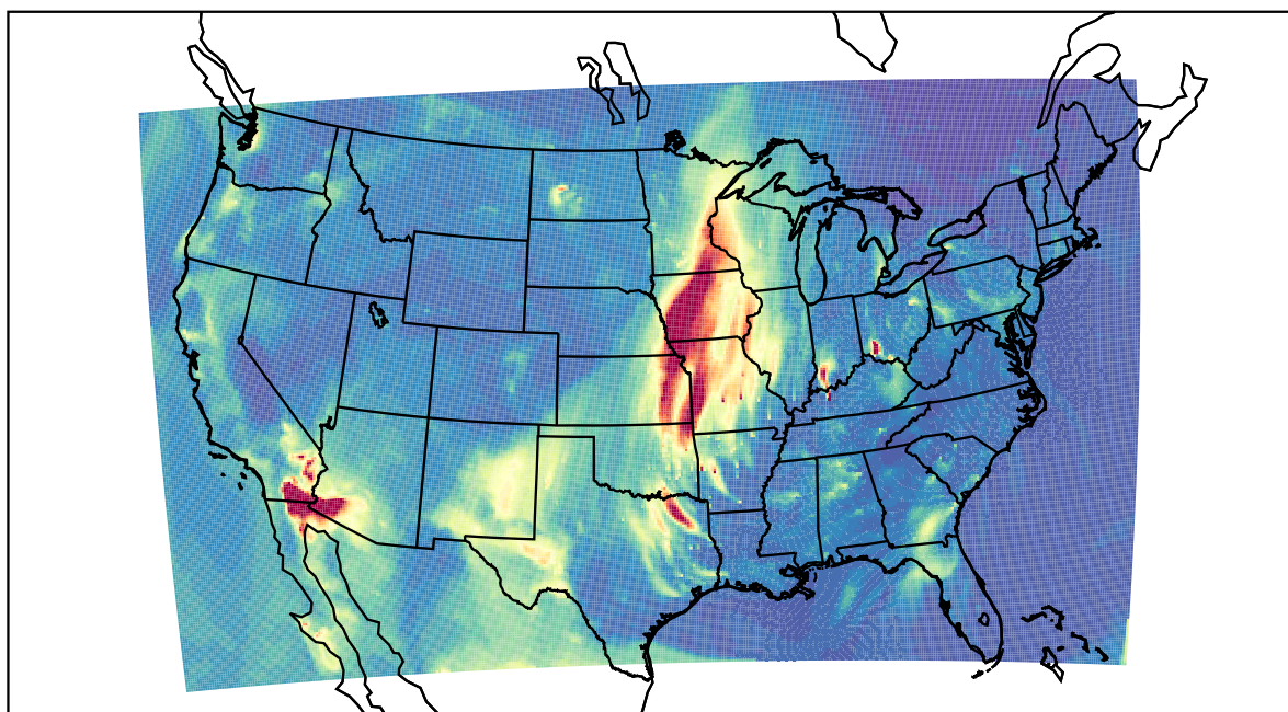
WRF 2021-04-03_08:00:00
