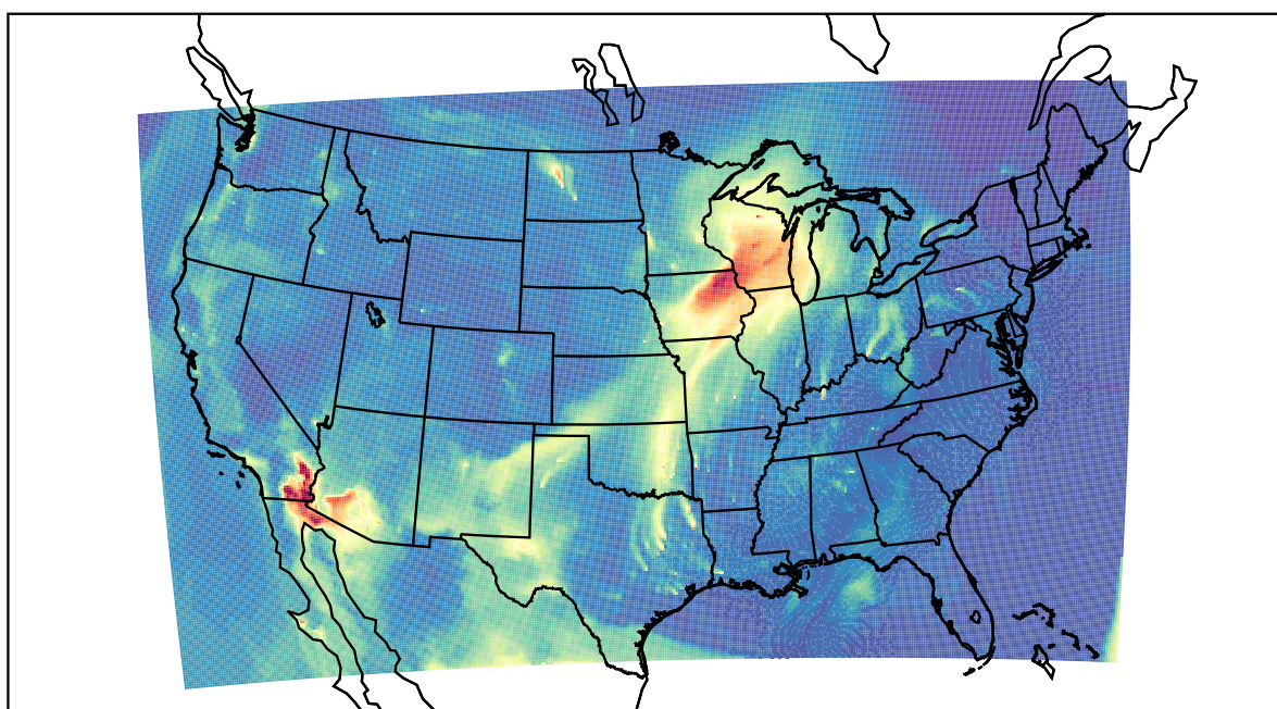
WRF 2021-04-03_15:00:00
