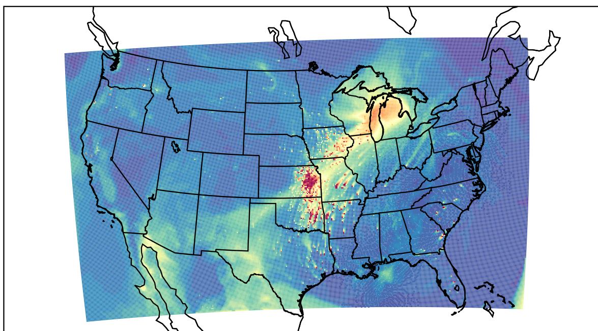
WRF 2021-04-03_21:00:00
