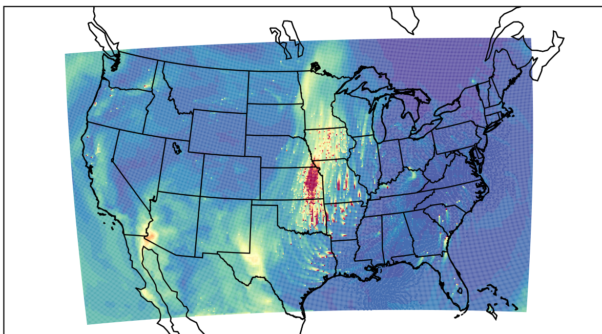
WRF 2021-04-02_22:00:00
