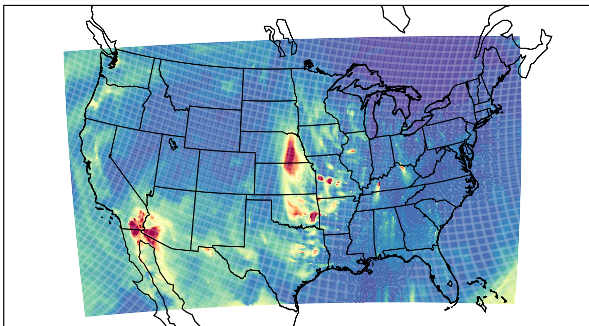
WRF 2021-04-02_08:00:00
