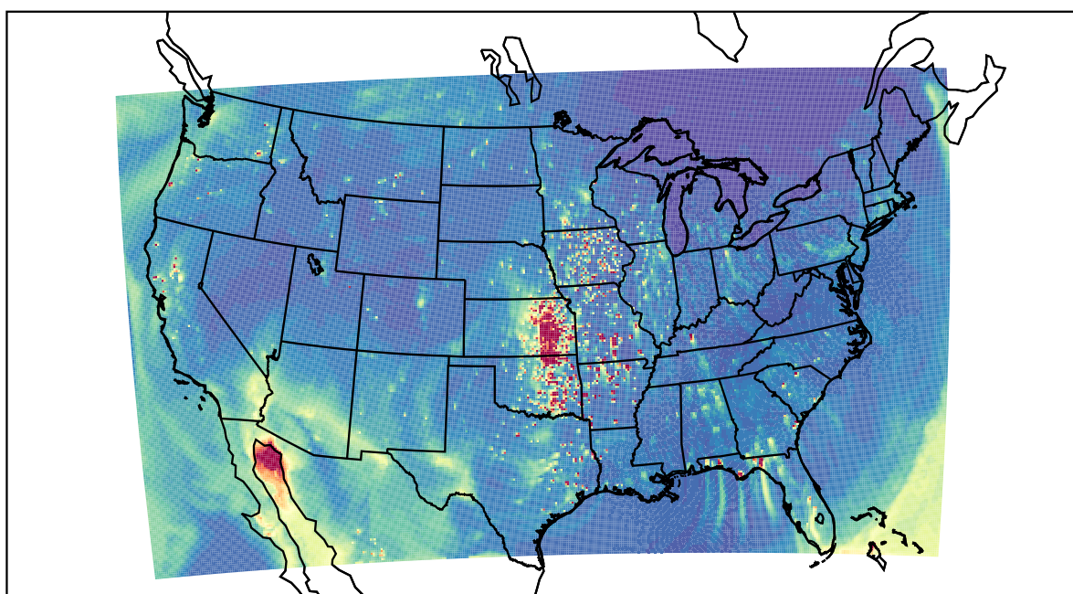
WRF 2021-04-02_01:00:00
