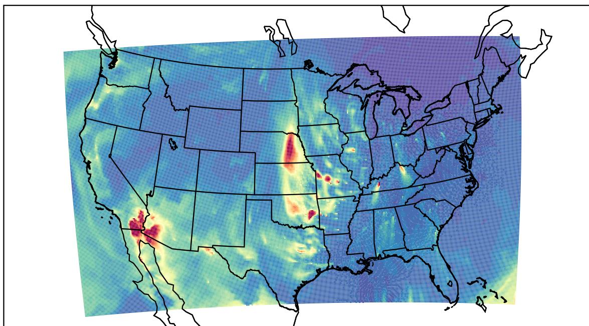
WRF 2021-04-02_09:00:00
