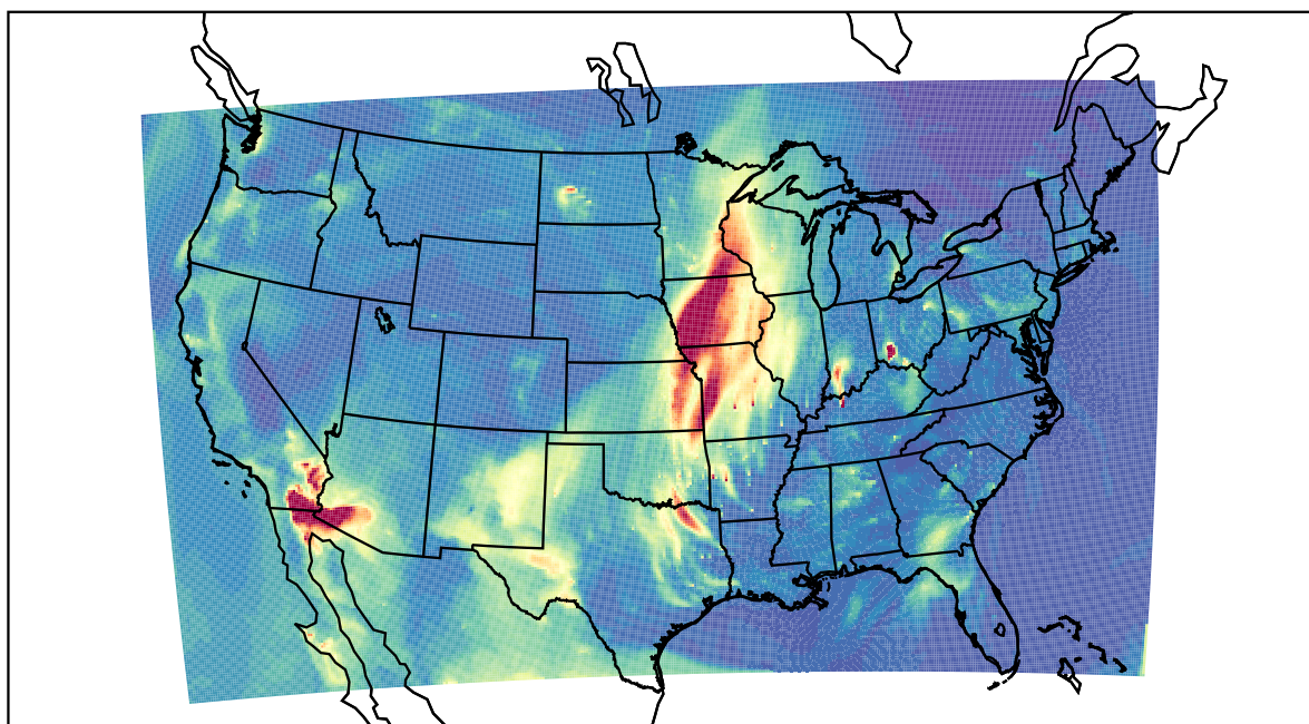
WRF 2021-04-03_09:00:00
