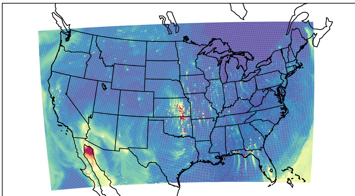
WRF 2021-04-02_00:00:00
