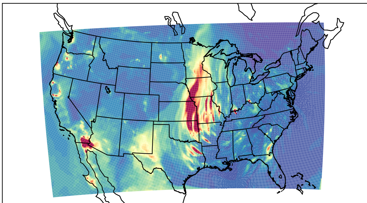
WRF 2021-04-03_05:00:00
