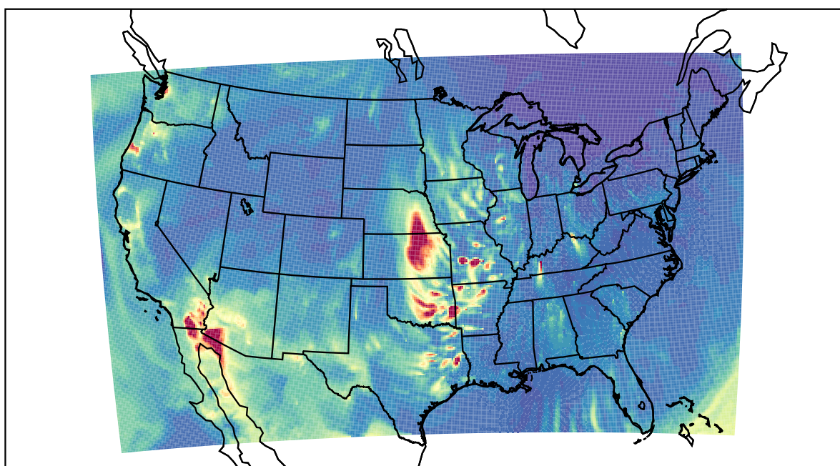
WRF 2021-04-02_06:00:00
