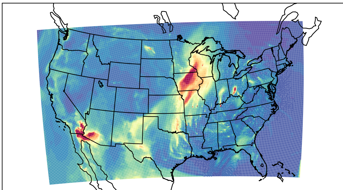
WRF 2021-04-03_12:00:00
