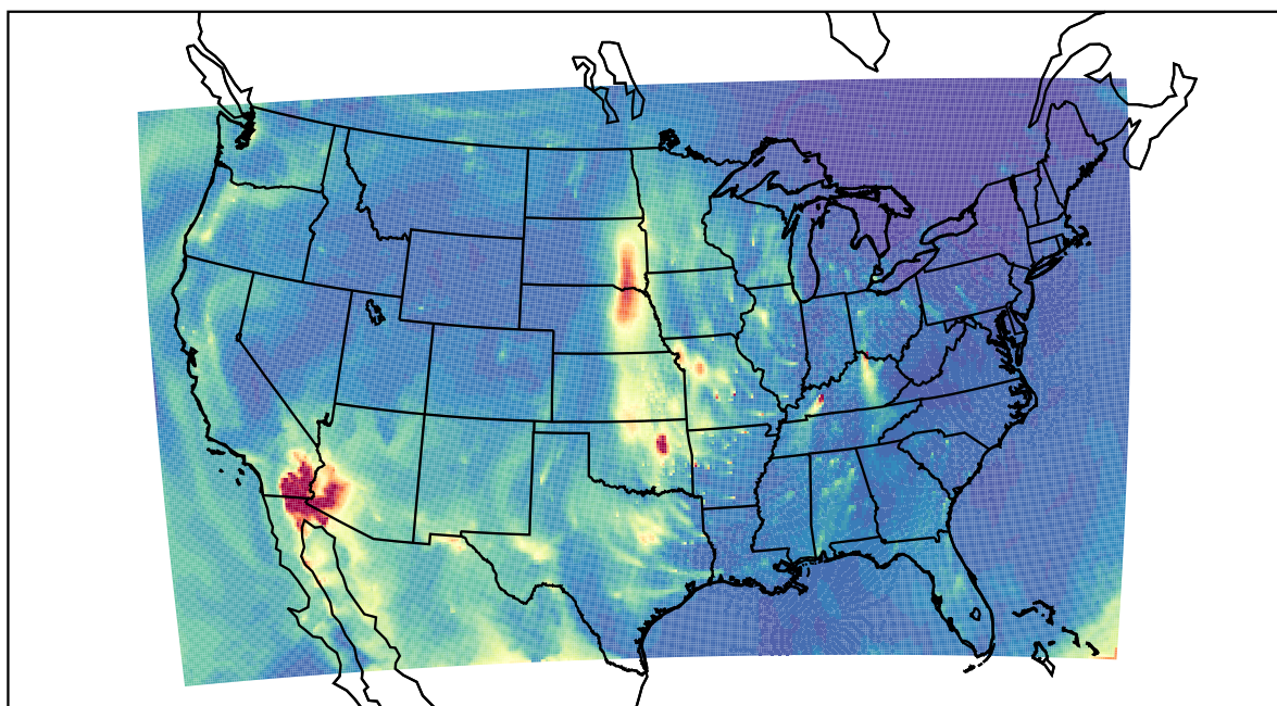
WRF 2021-04-02_12:00:00
