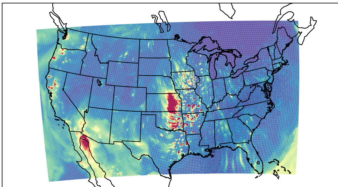
WRF 2021-04-02_03:00:00
