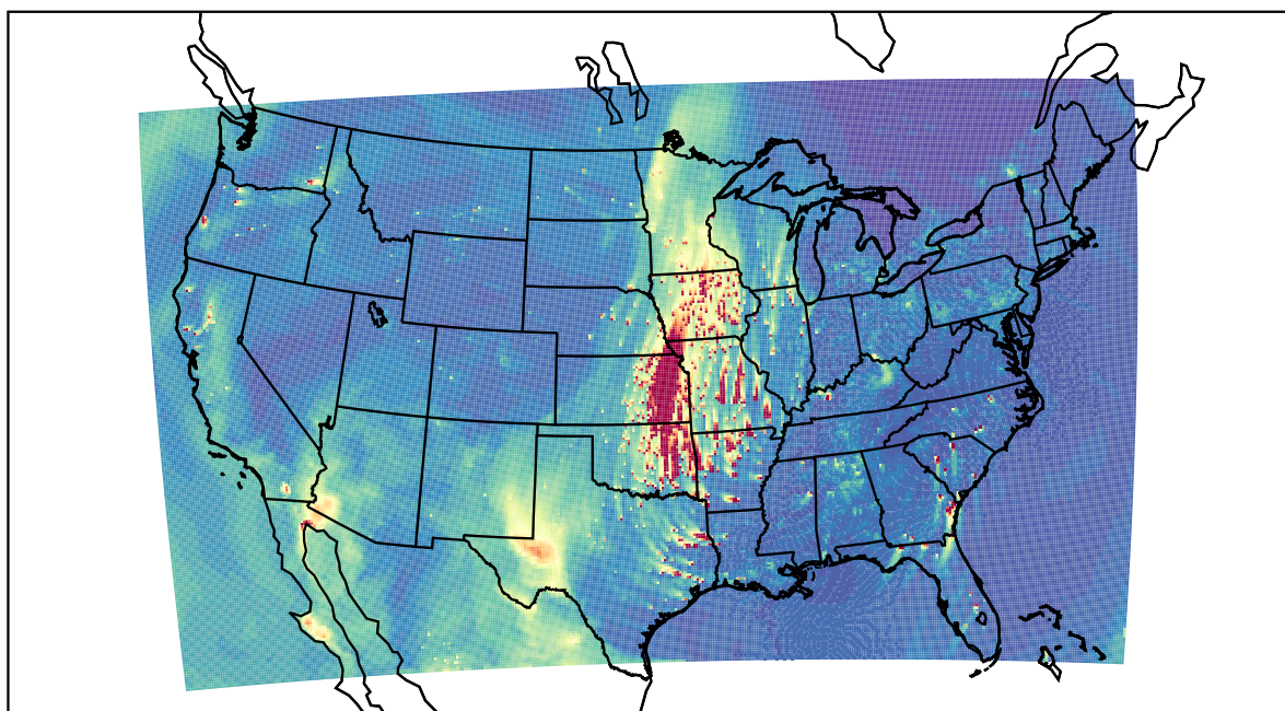
WRF 2021-04-03_00:00:00
