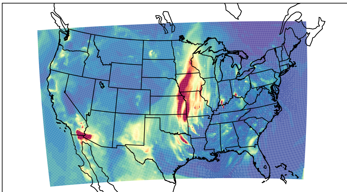
WRF 2021-04-03_07:00:00
