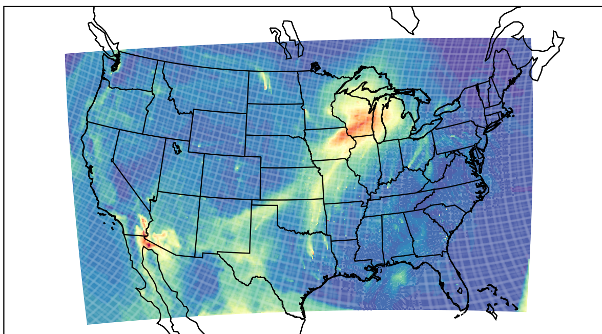
WRF 2021-04-03_17:00:00
