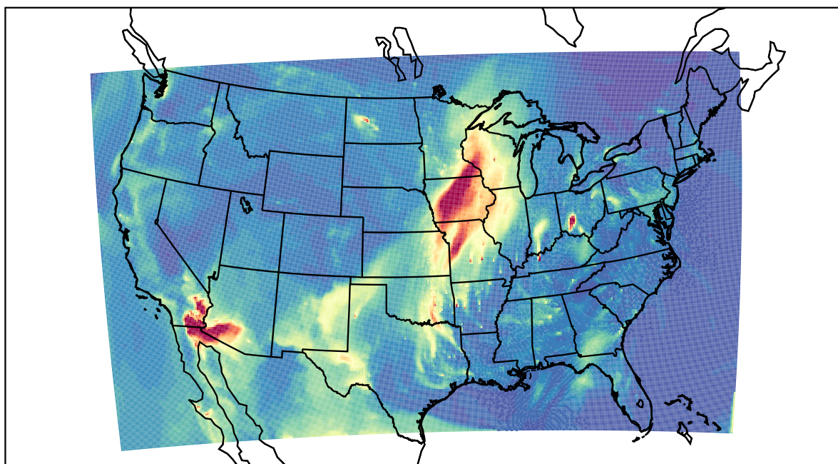
WRF 2021-04-03_11:00:00
