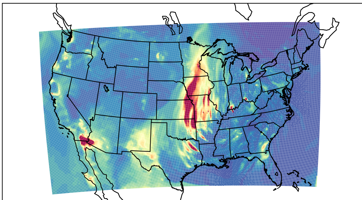
WRF 2021-04-03_06:00:00
