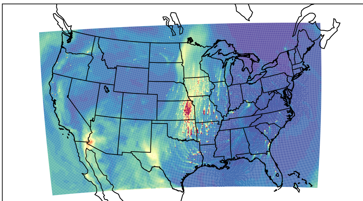
WRF 2021-04-02_21:00:00
