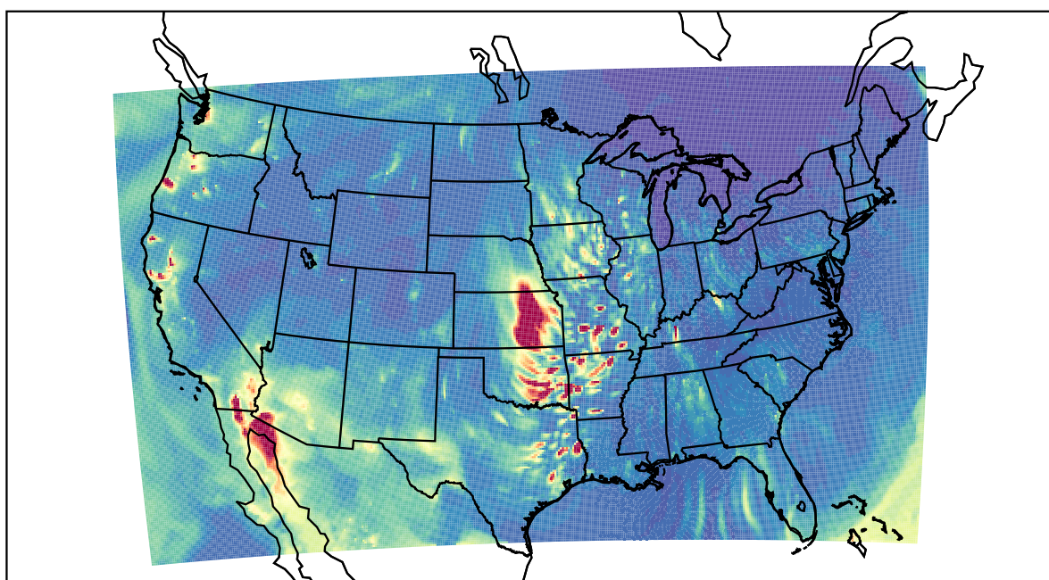
WRF 2021-04-02_04:00:00
