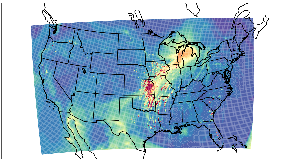
WRF 2021-04-03_22:00:00
