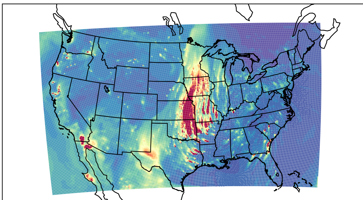
WRF 2021-04-03_02:00:00
