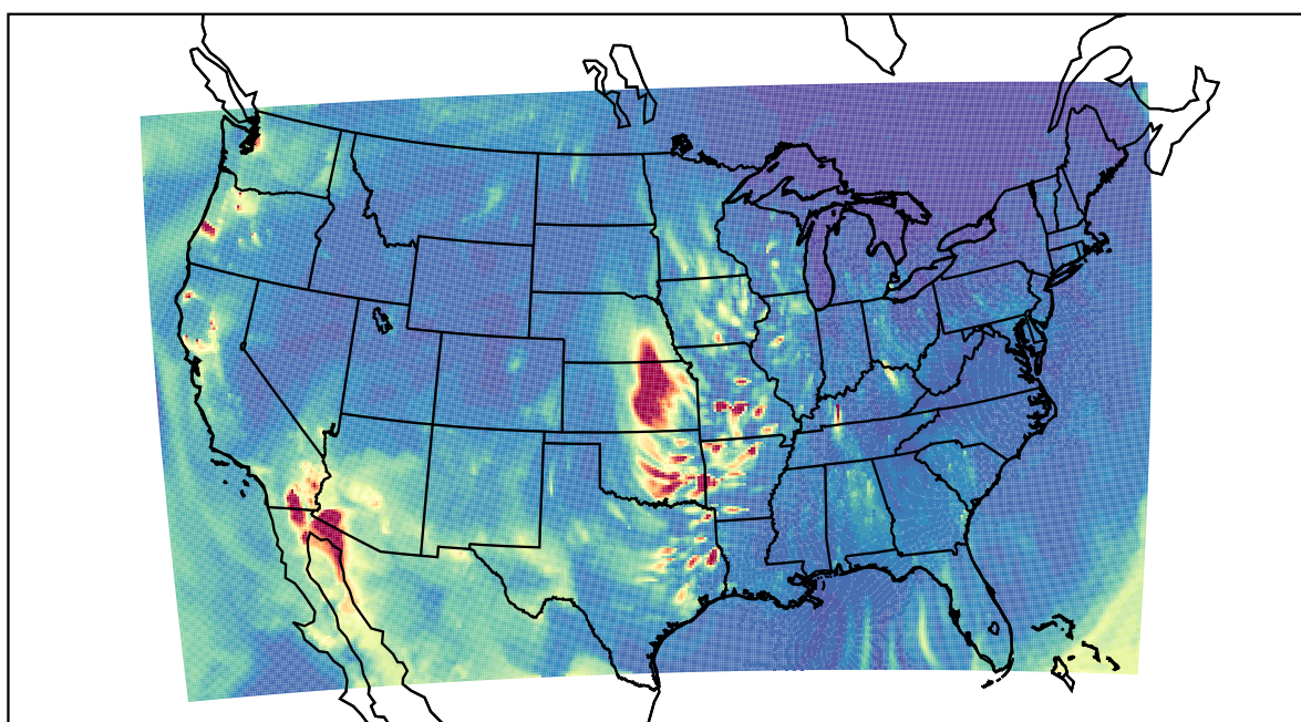
WRF 2021-04-02_05:00:00
