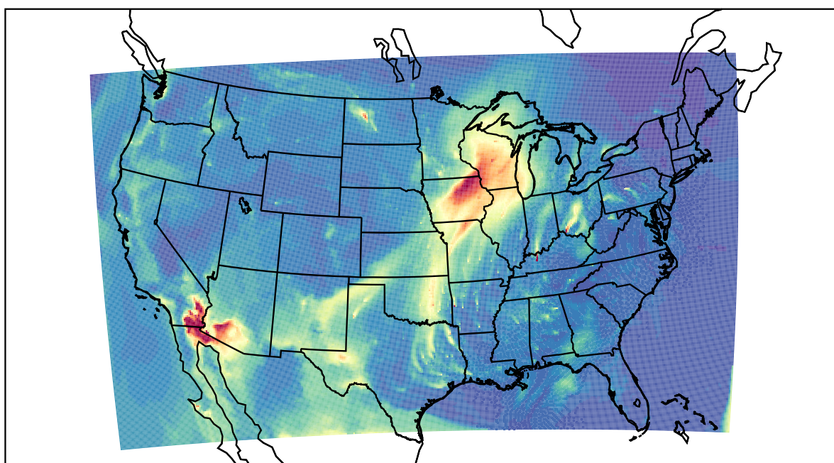
WRF 2021-04-03_14:00:00
