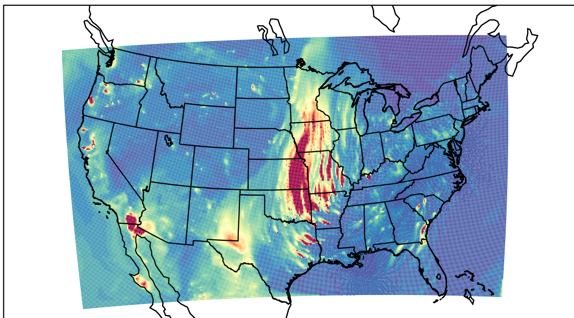
WRF 2021-04-03_03:00:00
