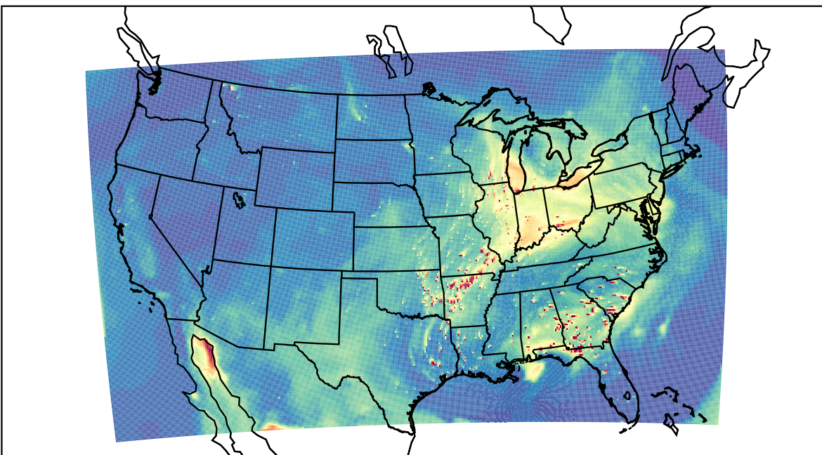
WRF 2021-04-04_21:00:00
