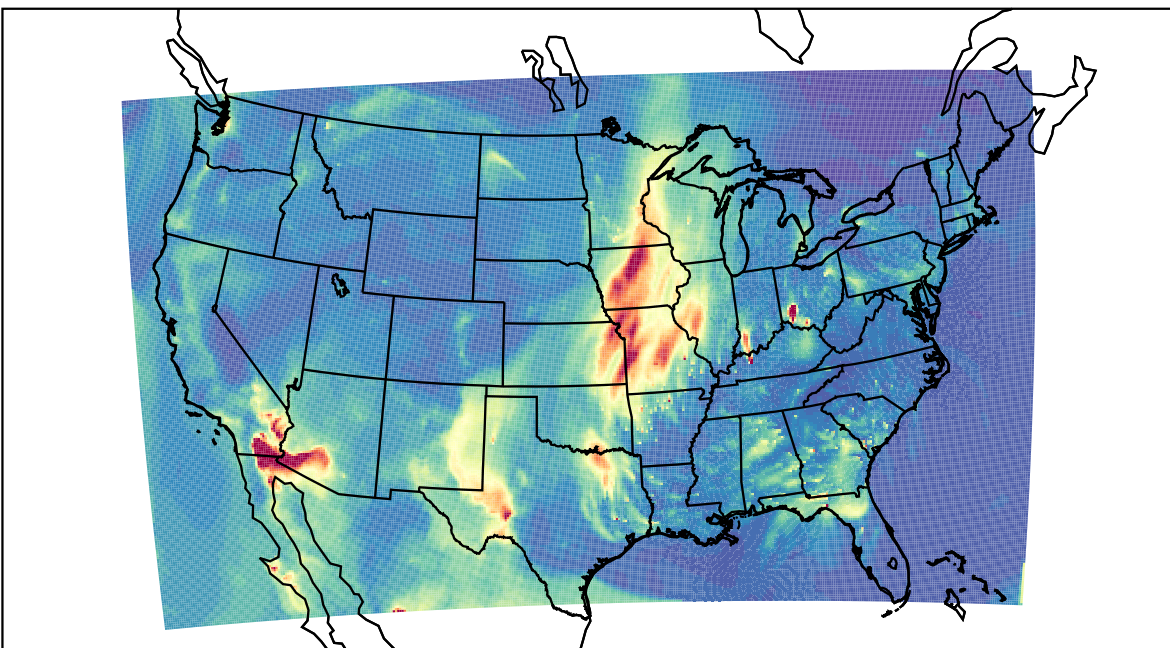
WRF 2021-04-03_09:00:00
