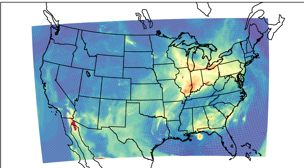
WRF 2021-04-04_17:00:00
