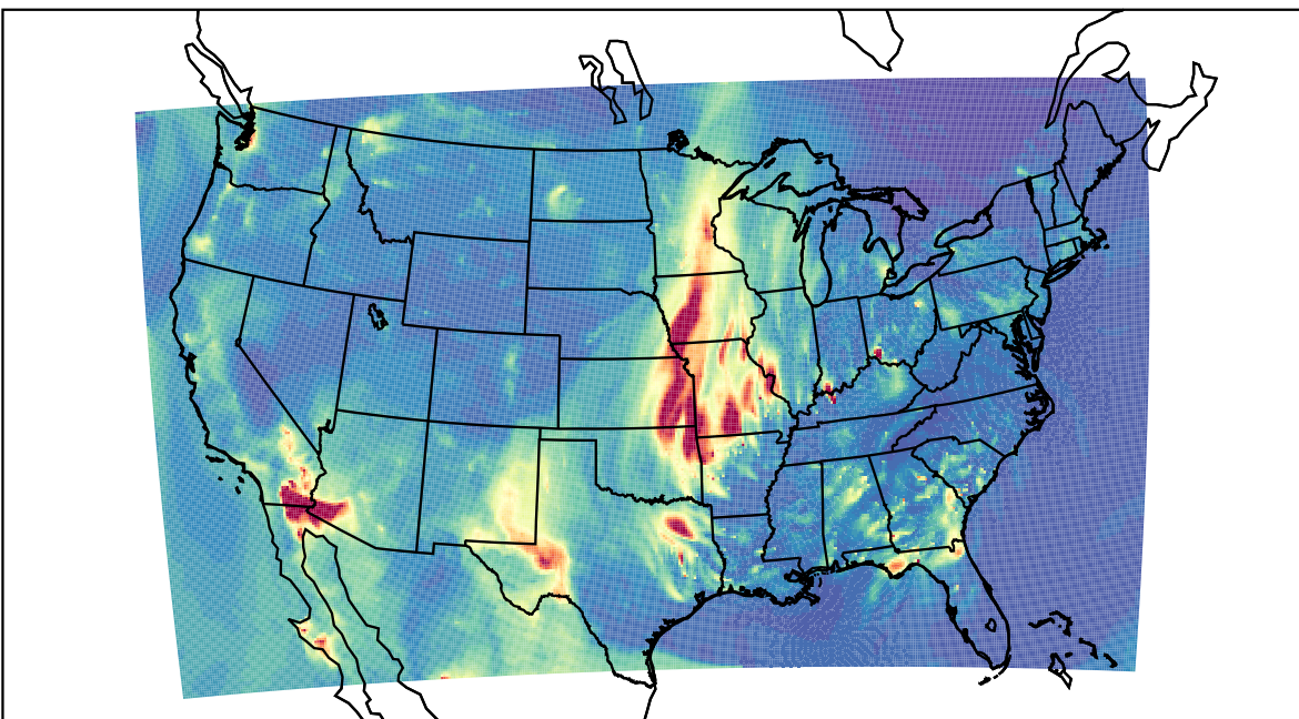
WRF 2021-04-03_06:00:00
