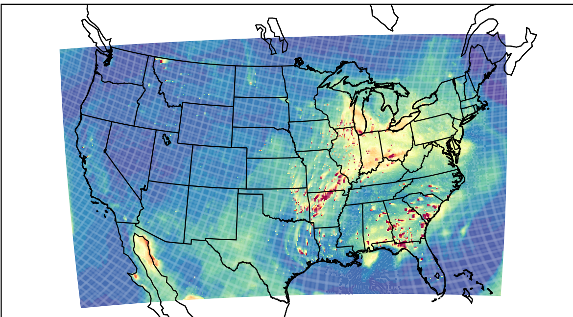
WRF 2021-04-04_23:00:00
