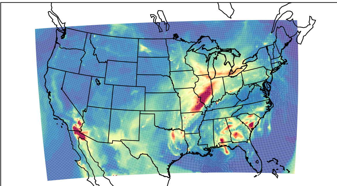
WRF 2021-04-04_12:00:00
