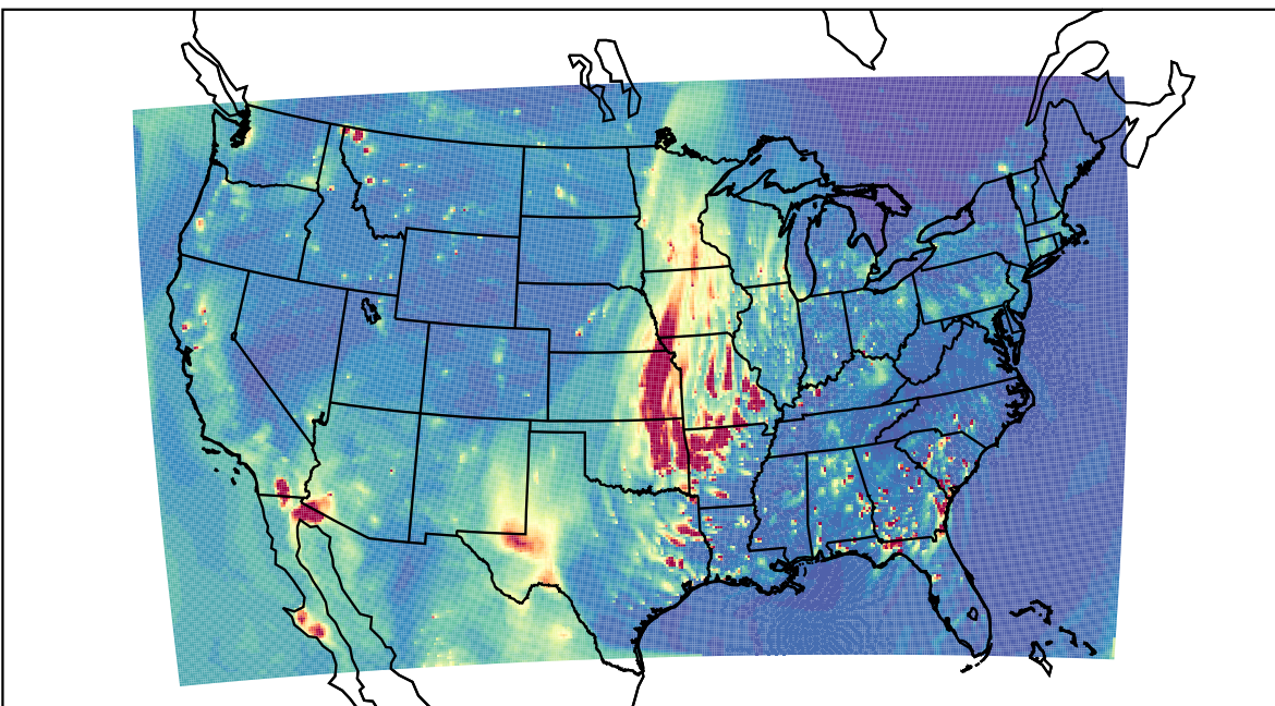
WRF 2021-04-03_02:00:00
