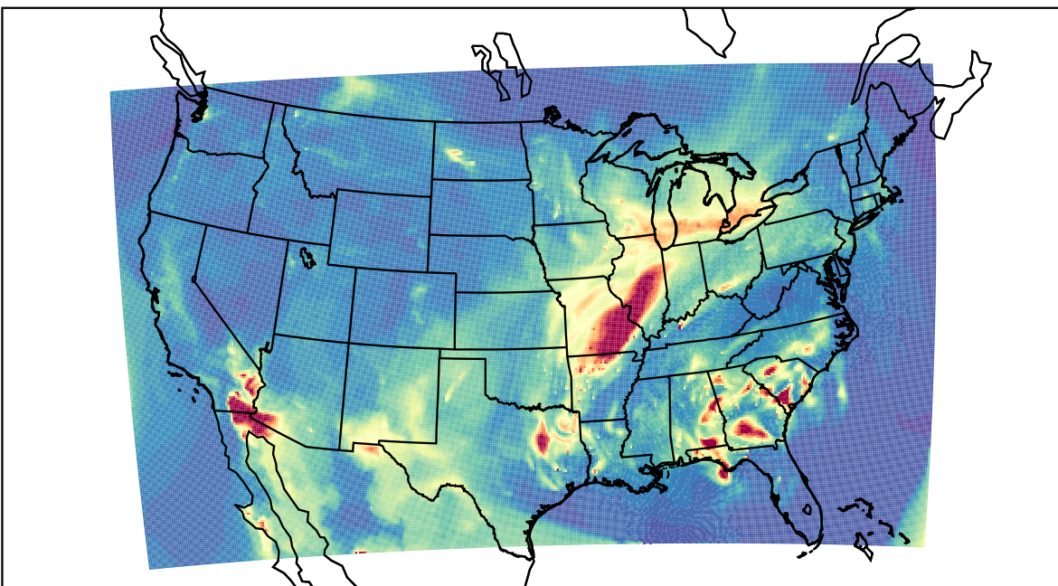
WRF 2021-04-04_09:00:00
