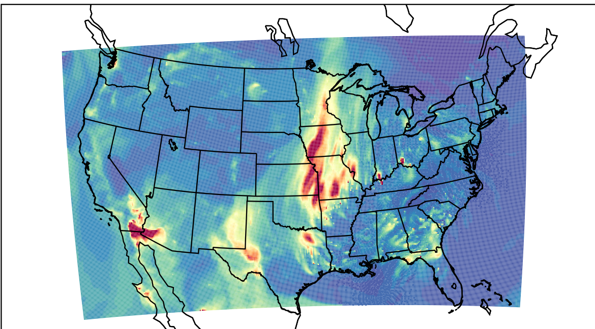
WRF 2021-04-03_07:00:00
