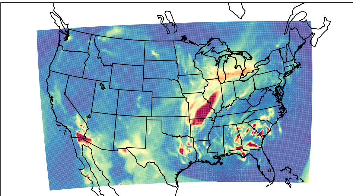
WRF 2021-04-04_07:00:00
