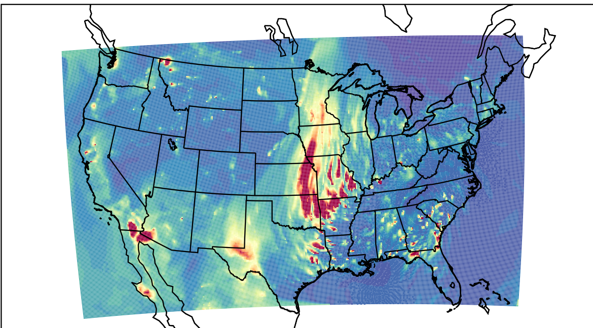
WRF 2021-04-03_03:00:00
