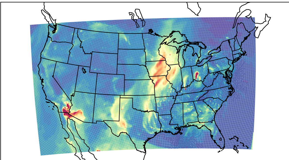
WRF 2021-04-03_12:00:00
