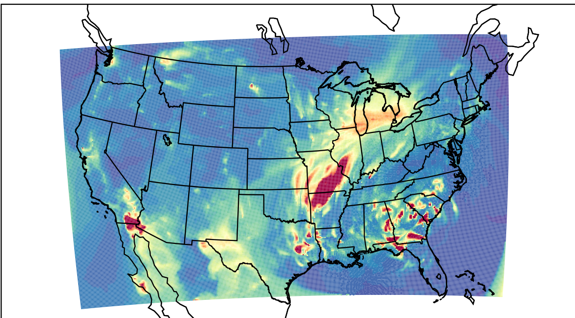
WRF 2021-04-04_05:00:00
