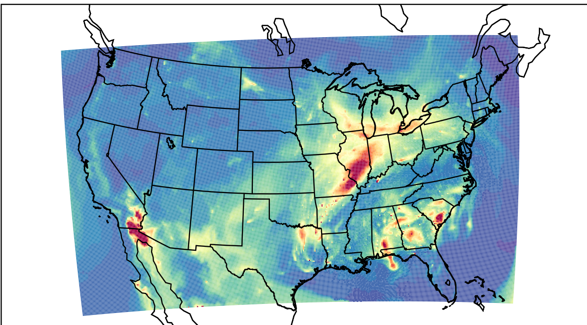
WRF 2021-04-04_13:00:00
