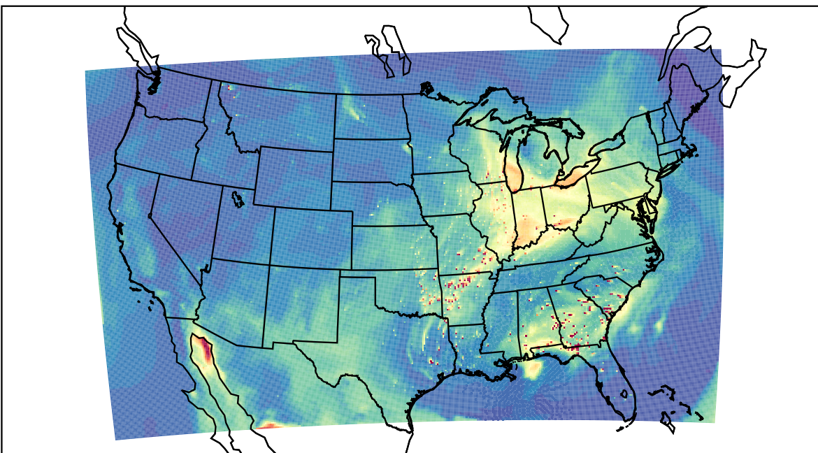
WRF 2021-04-04_20:00:00
