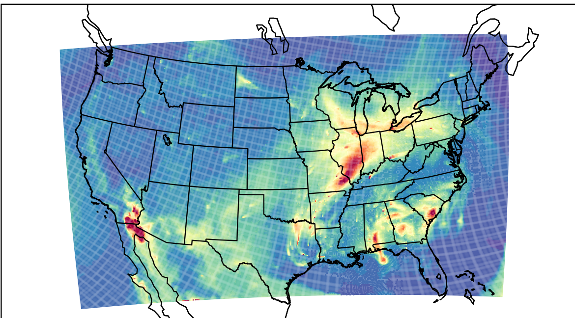
WRF 2021-04-04_14:00:00
