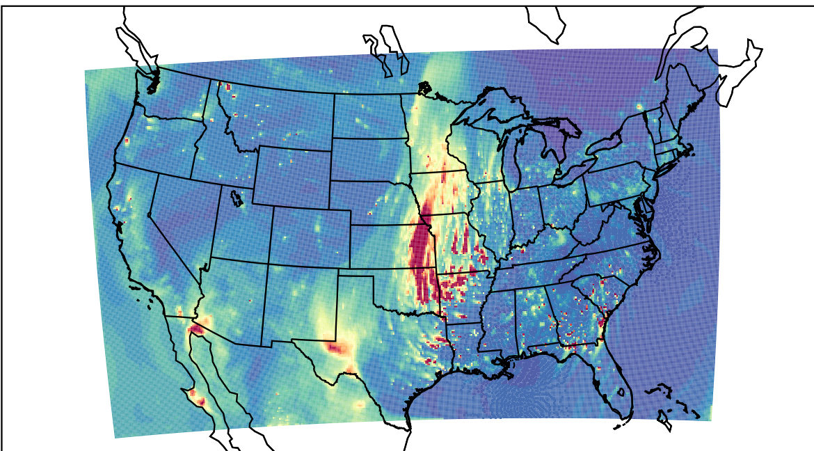
WRF 2021-04-03_01:00:00
