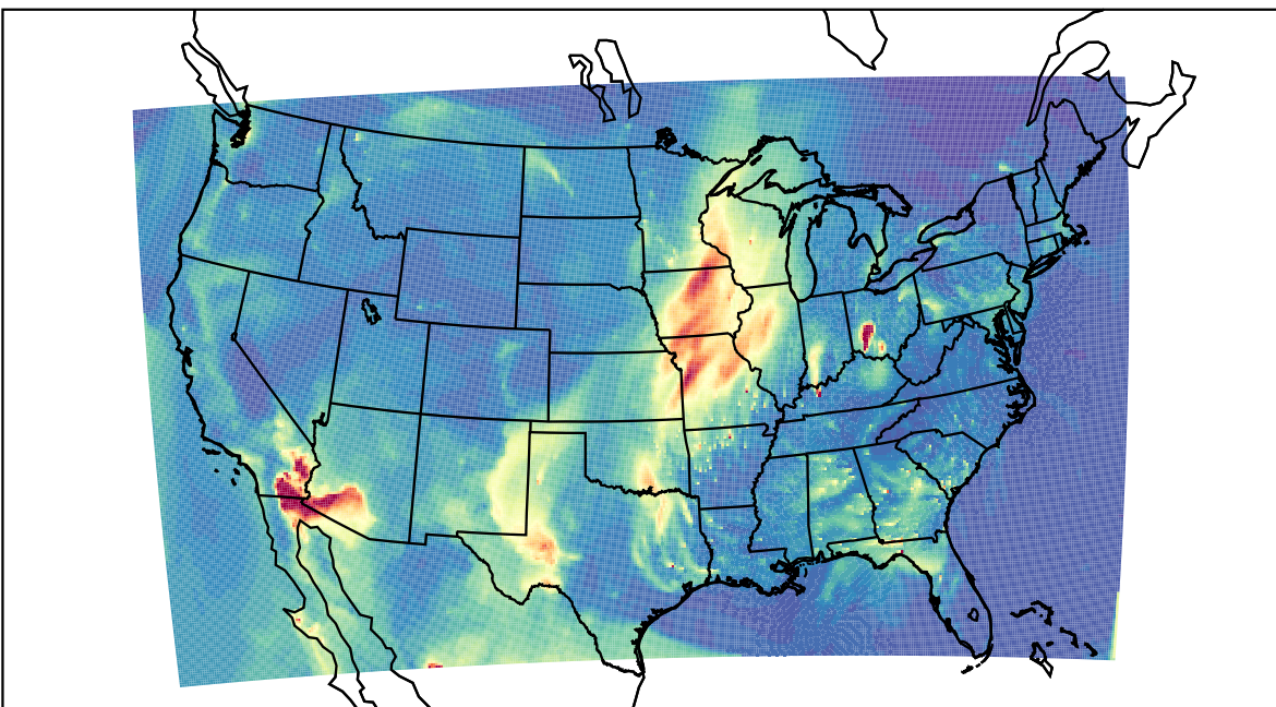
WRF 2021-04-03_11:00:00
