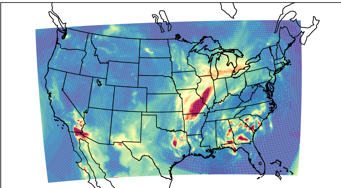
WRF 2021-04-04_08:00:00
