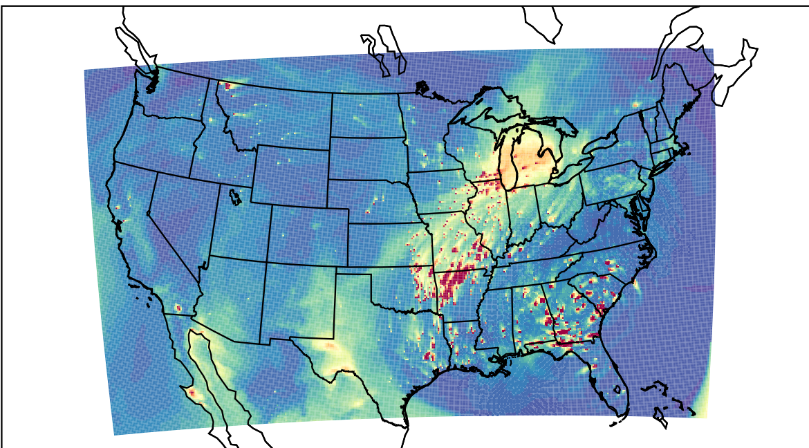
WRF 2021-04-04_00:00:00
