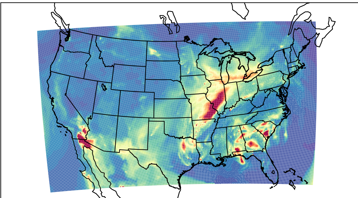
WRF 2021-04-04_11:00:00
