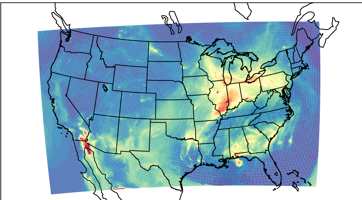
WRF 2021-04-04_16:00:00
