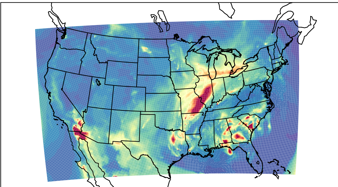
WRF 2021-04-04_10:00:00
