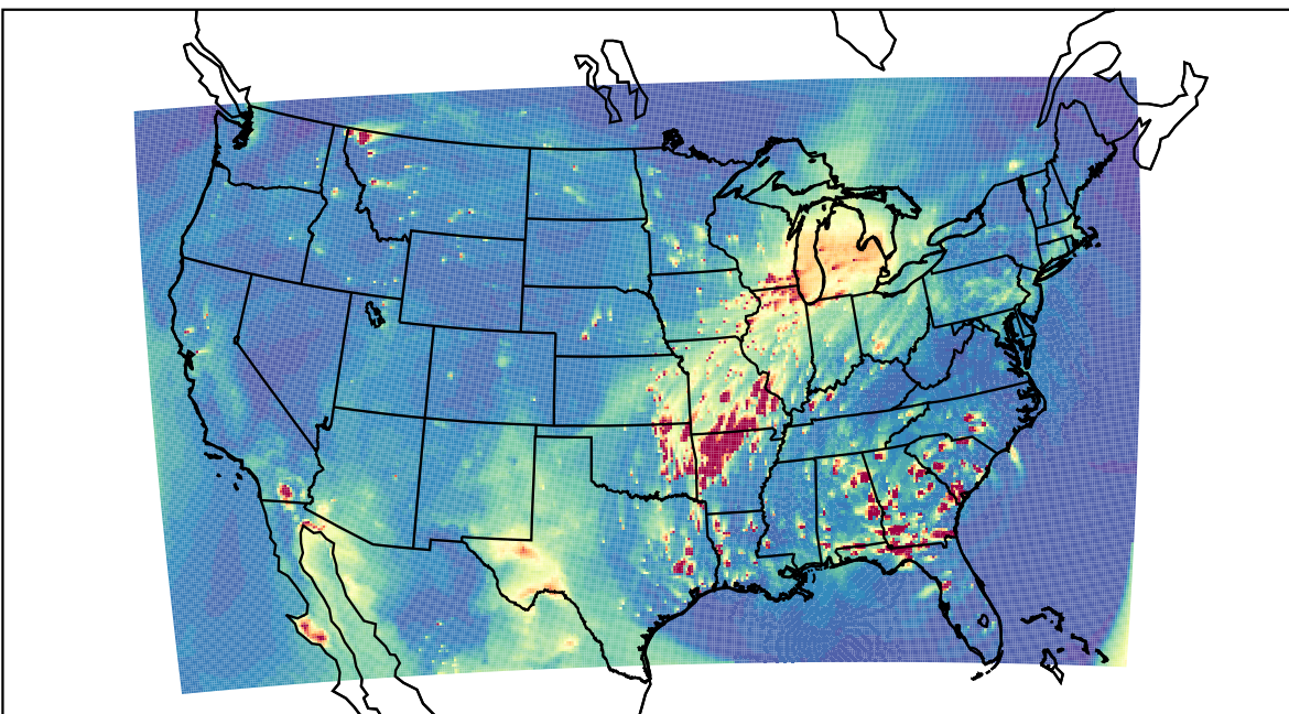
WRF 2021-04-04_01:00:00
