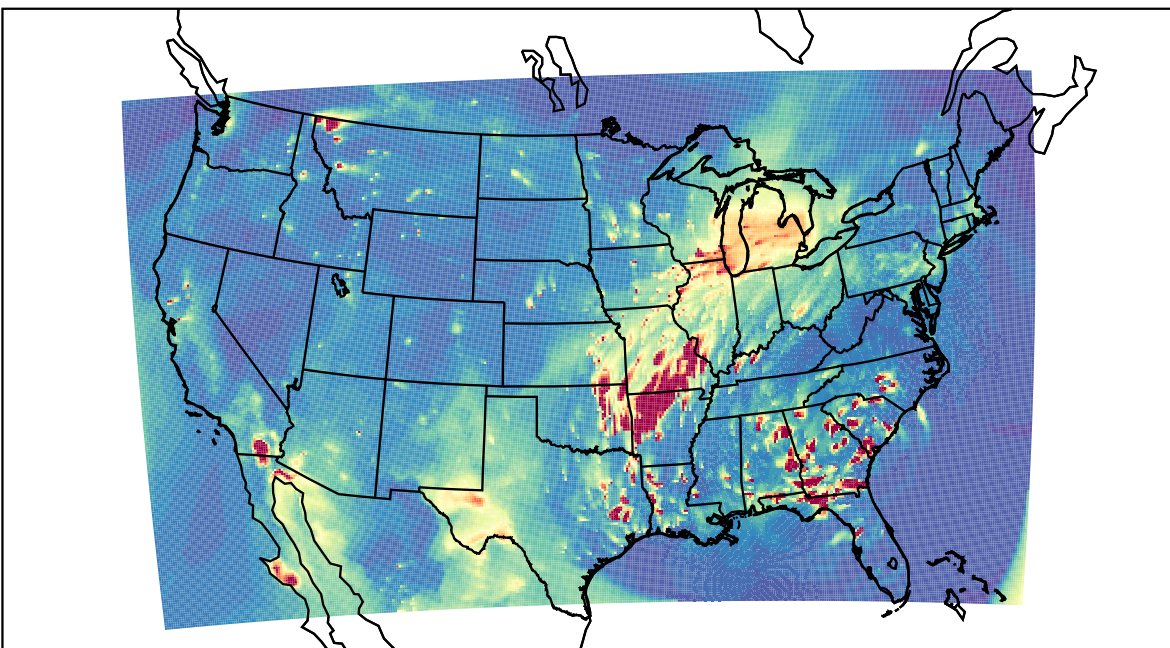
WRF 2021-04-04_02:00:00
