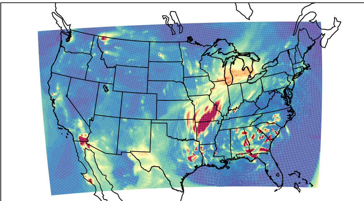
WRF 2021-04-04_04:00:00
