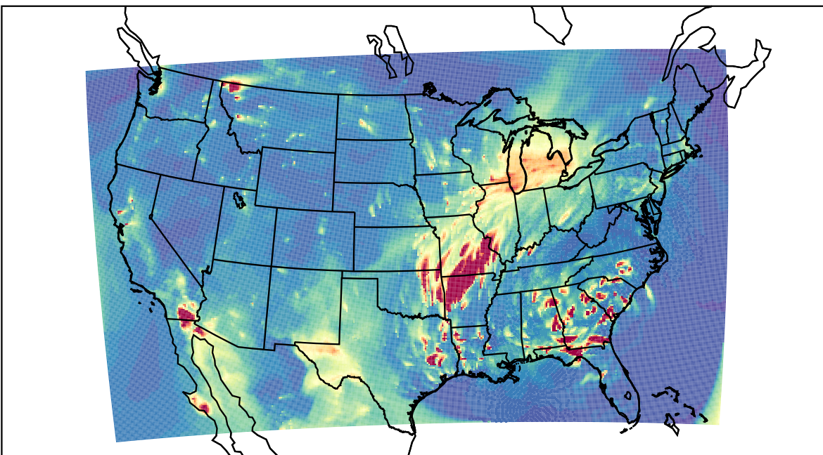
WRF 2021-04-04_03:00:00
