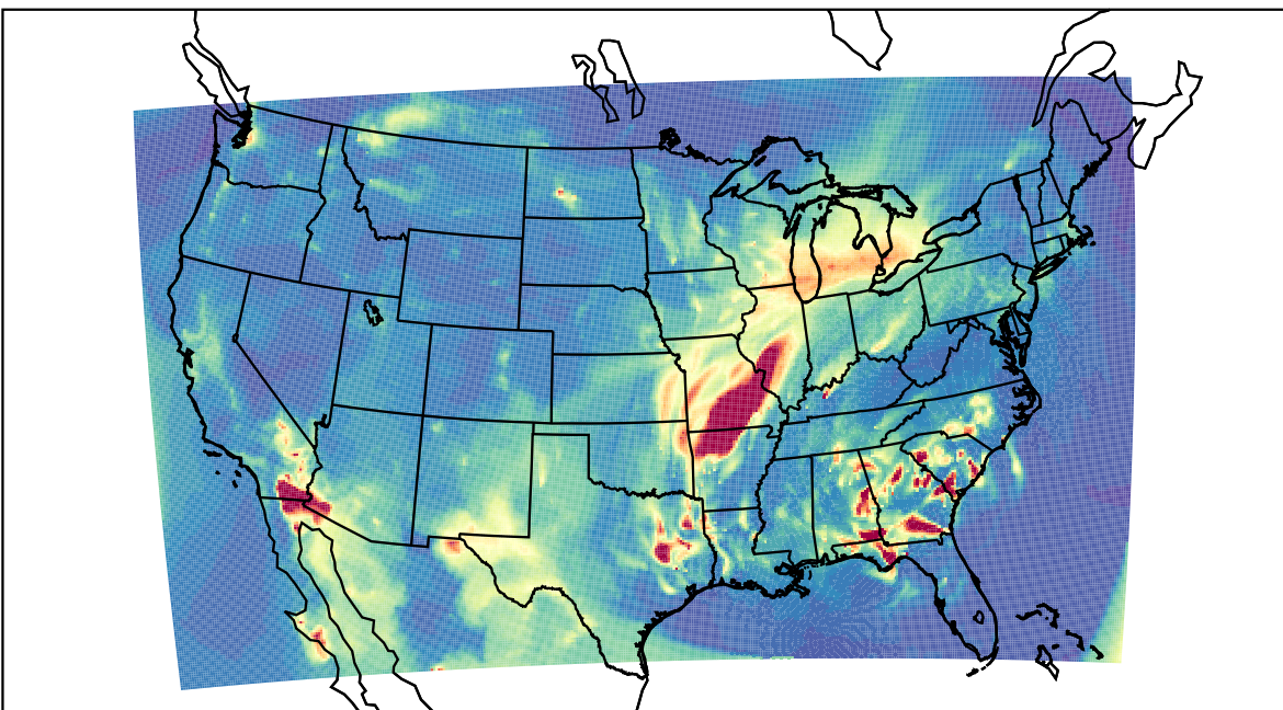
WRF 2021-04-04_06:00:00
