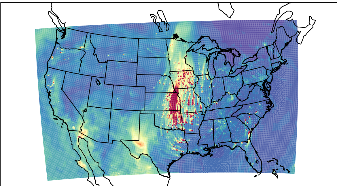
WRF 2021-04-03_00:00:00
