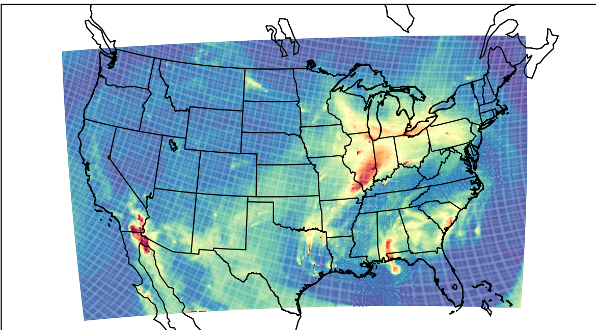
WRF 2021-04-04_15:00:00
