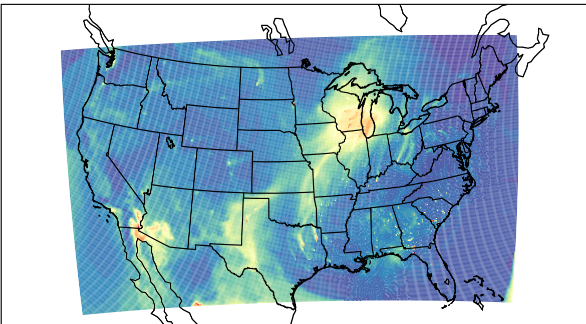
WRF 2021-04-03_17:00:00
