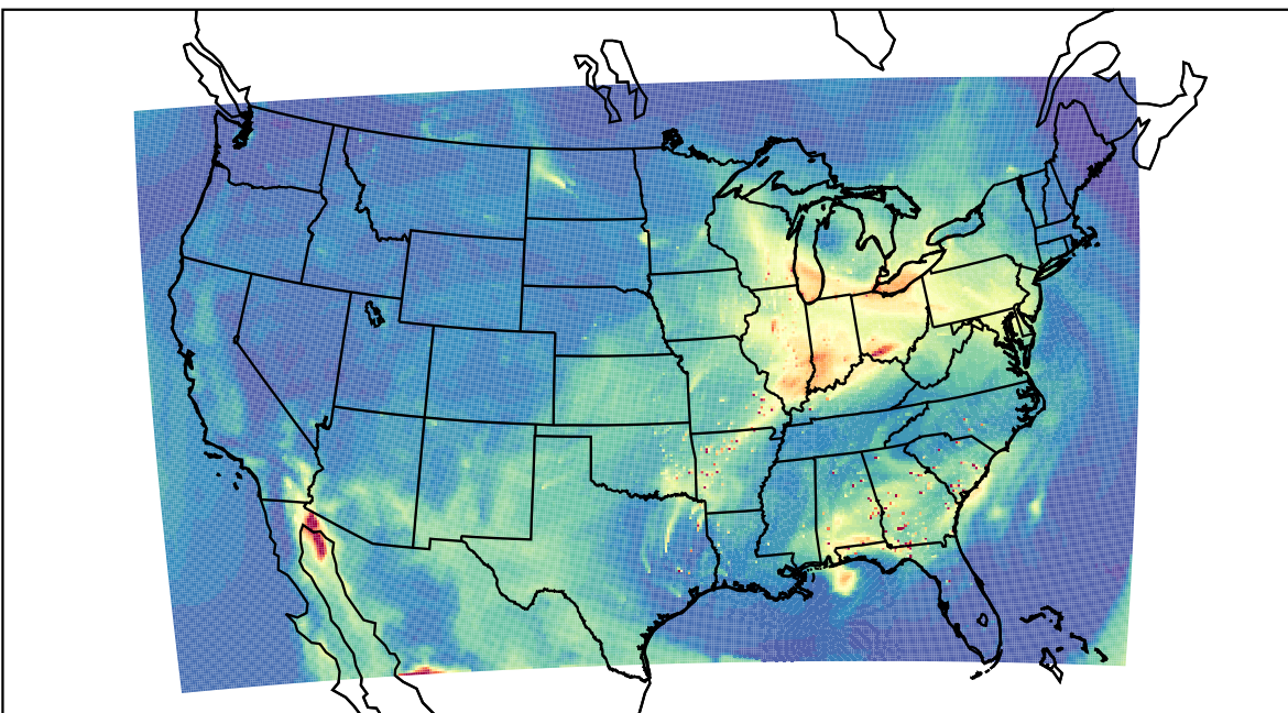
WRF 2021-04-04_18:00:00
