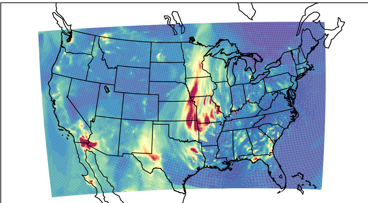
WRF 2021-04-03_05:00:00
