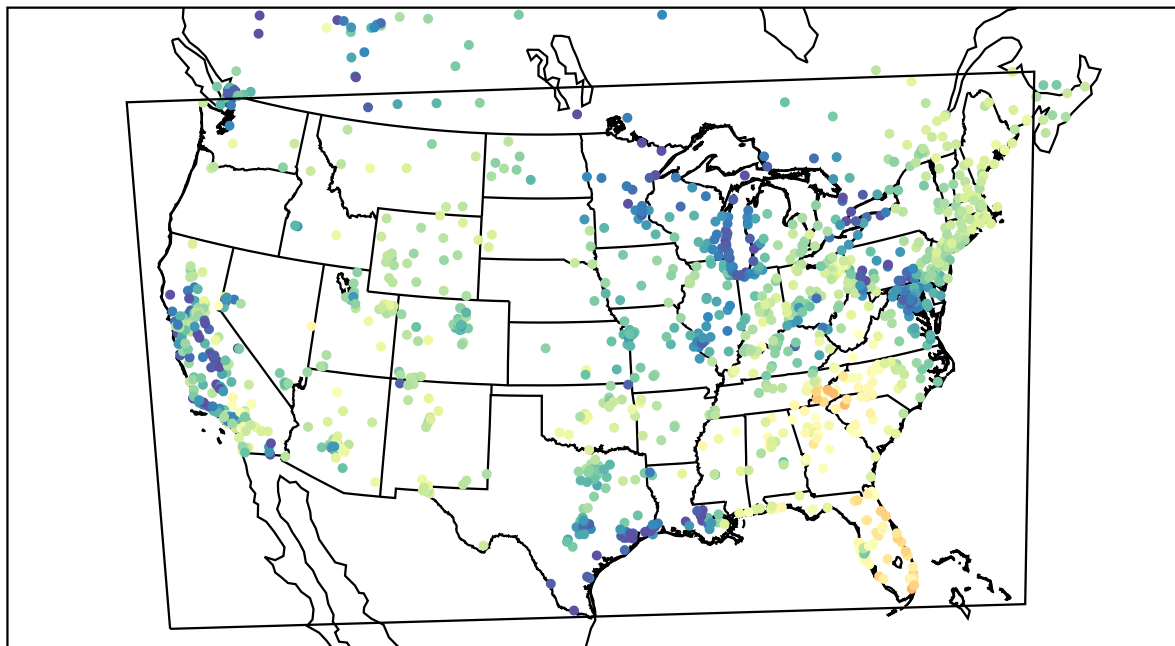
AirNOW (2021-04-13_15:00:00)
