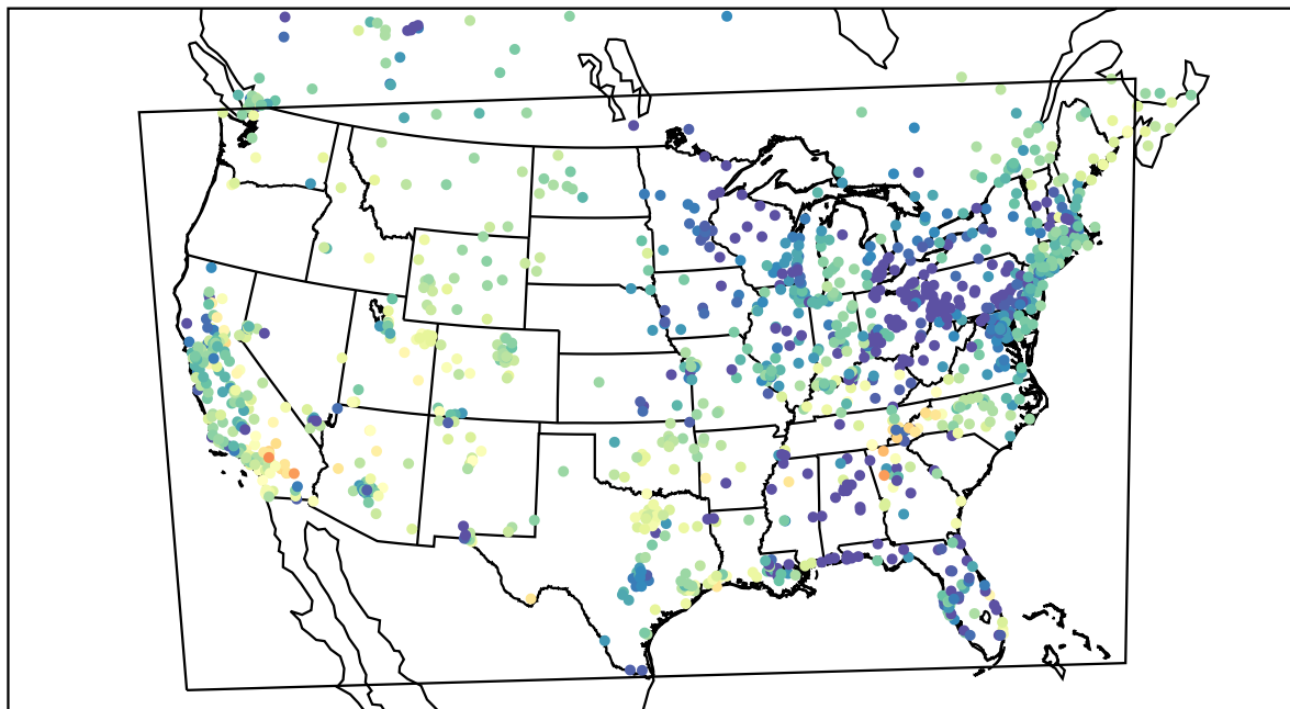
AirNOW (2021-04-13_04:00:00)
