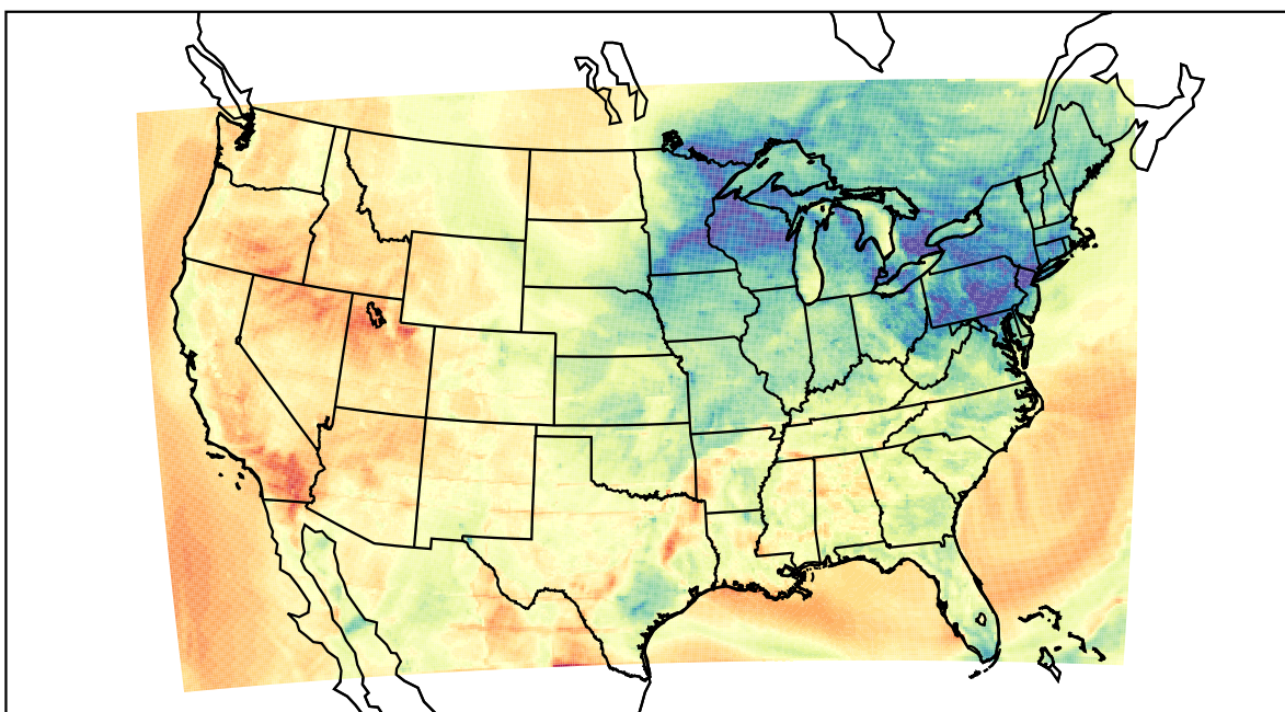
WRF (2021-04-13_01:00:00)
