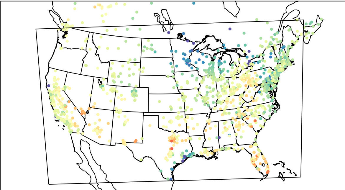
AirNOW (2021-04-13_23:00:00)
