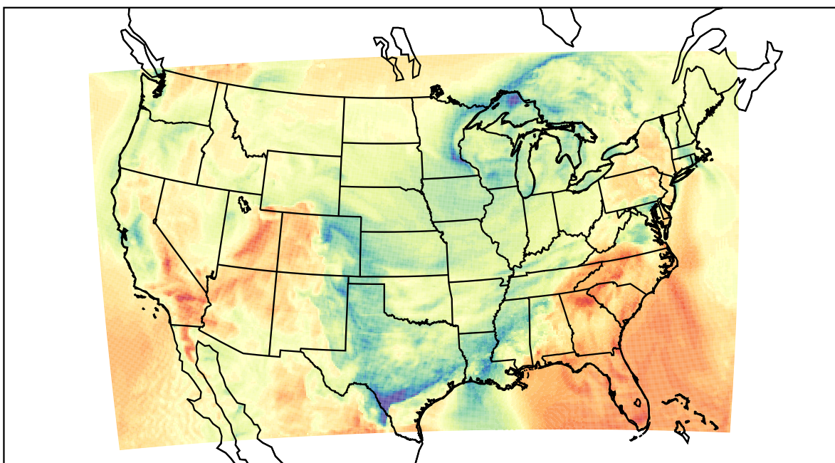
WRF (2021-04-14_17:00:00)
