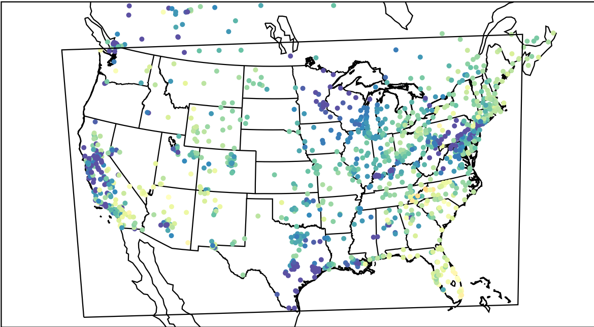
AirNOW (2021-04-14_14:00:00)
