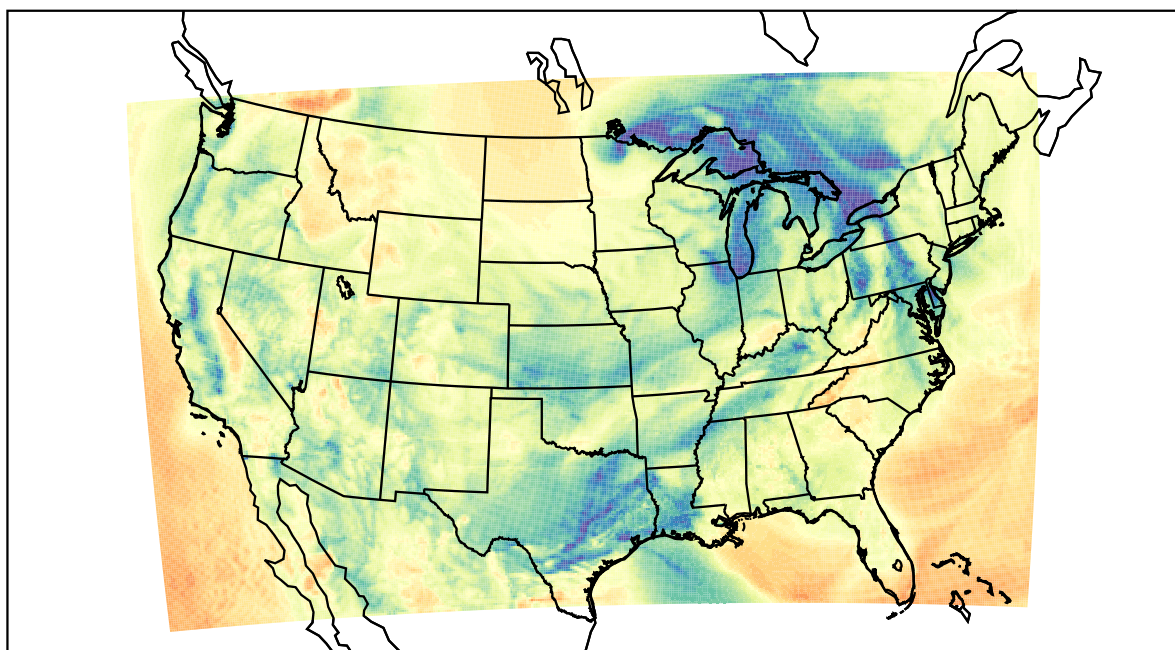
WRF (2021-04-13_15:00:00)
