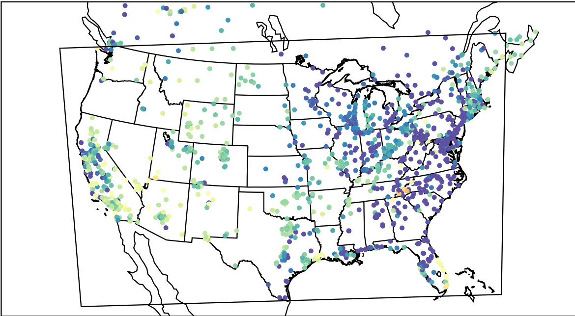
AirNOW (2021-04-14_09:00:00)
