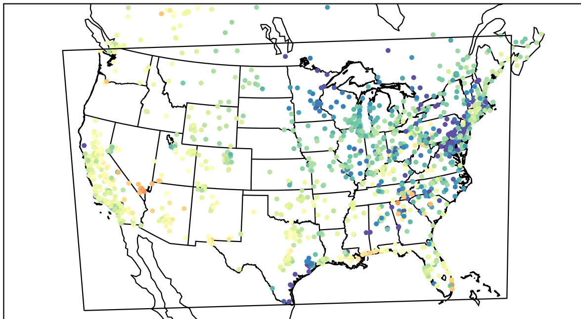
AirNOW (2021-04-14_01:00:00)
