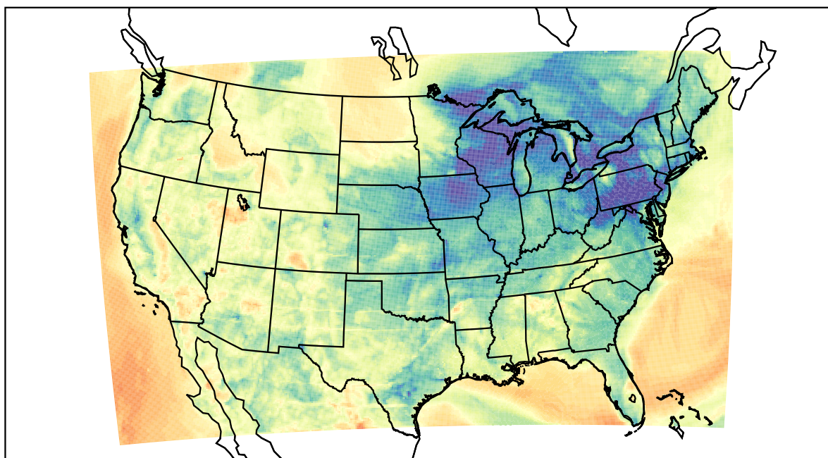
WRF (2021-04-13_06:00:00)
