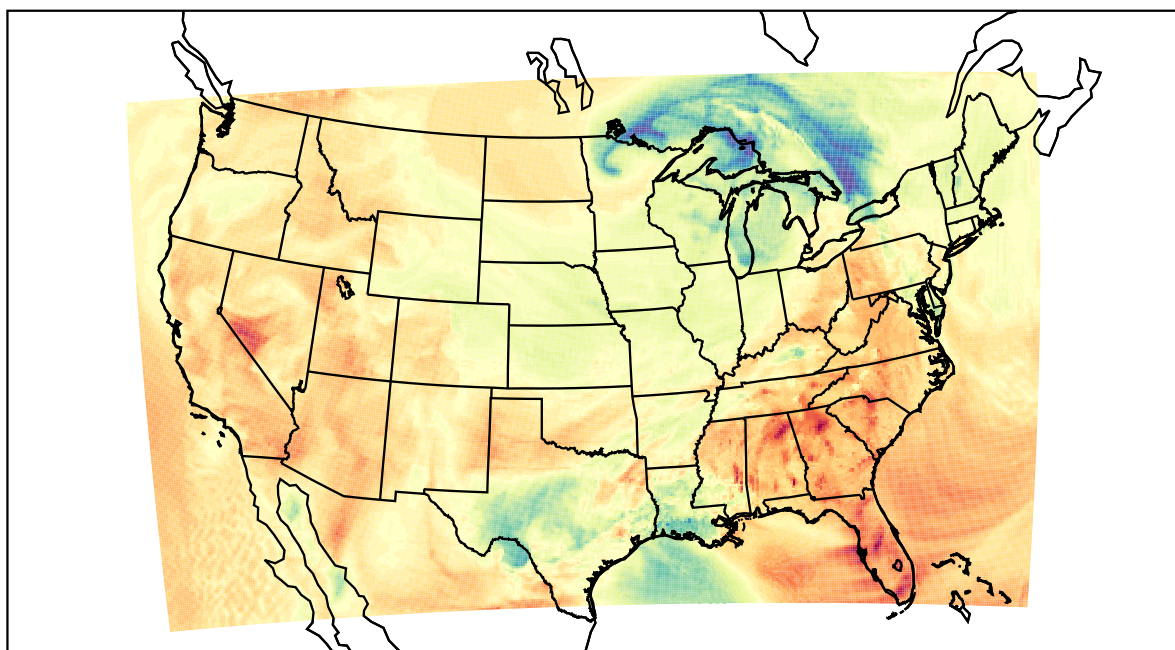
WRF (2021-04-13_21:00:00)
