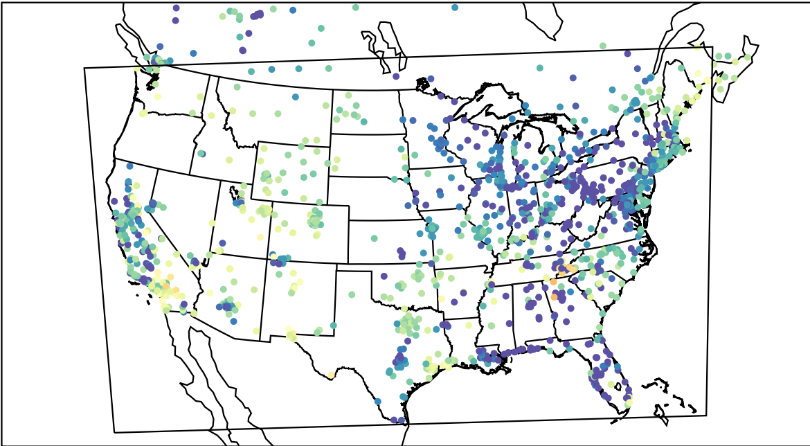
AirNOW (2021-04-13_07:00:00)
