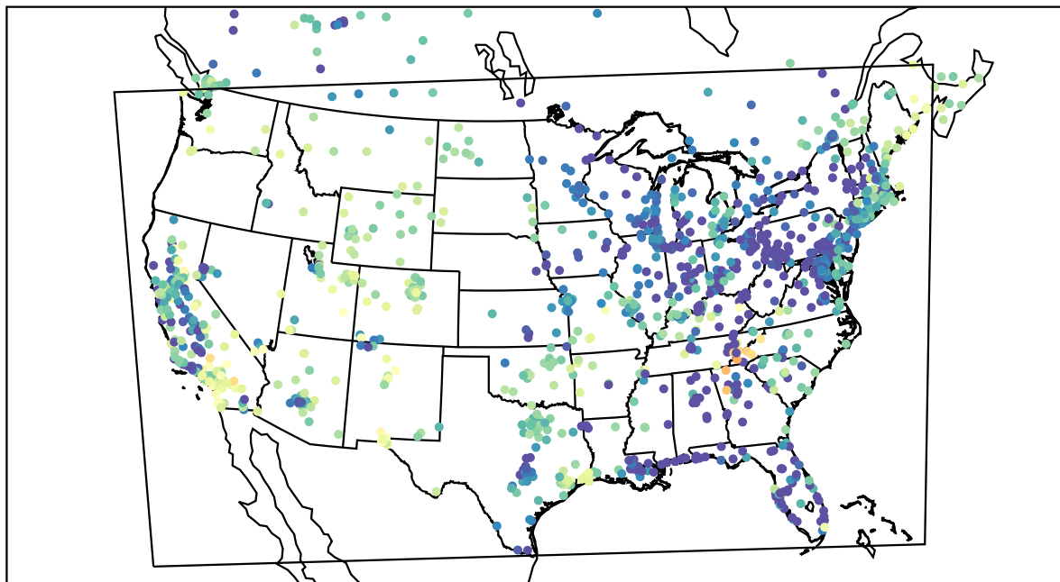
AirNOW (2021-04-13_08:00:00)
