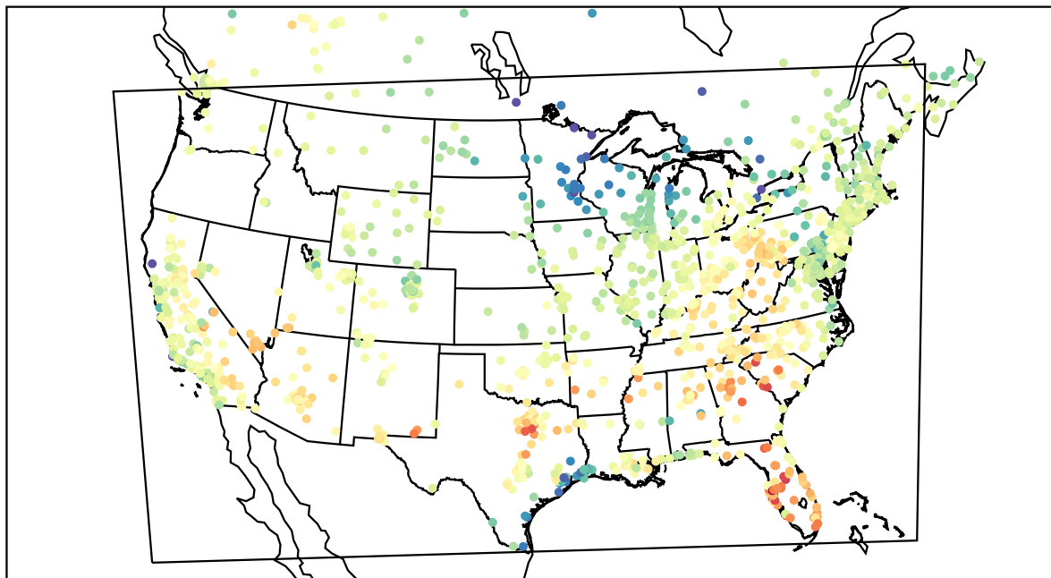
AirNOW (2021-04-13_22:00:00)
