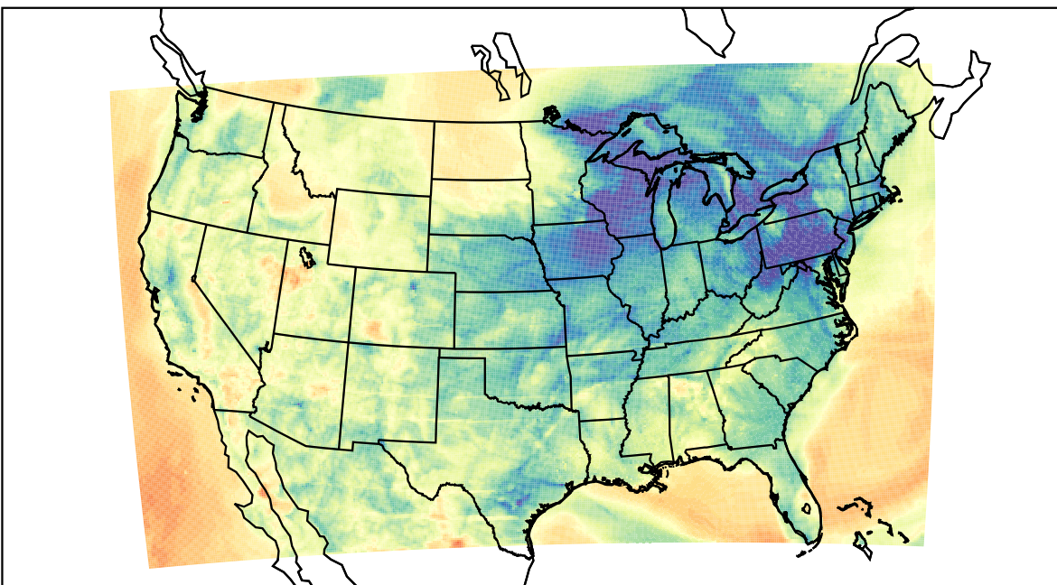
WRF (2021-04-13_07:00:00)
