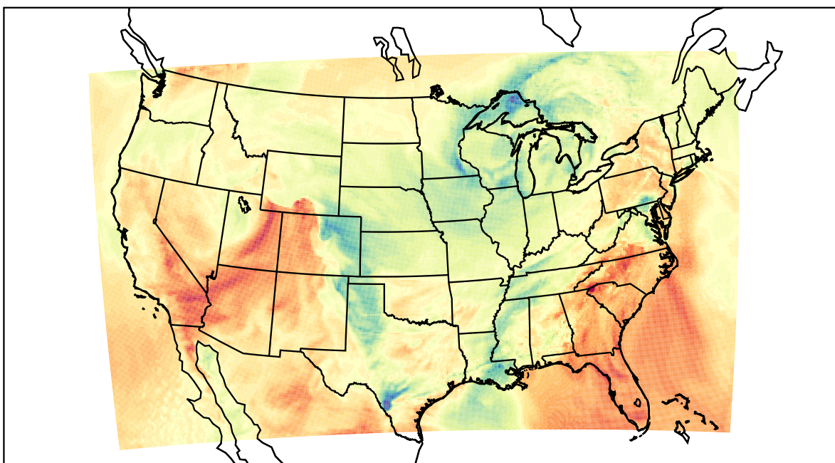
WRF (2021-04-14_20:00:00)
