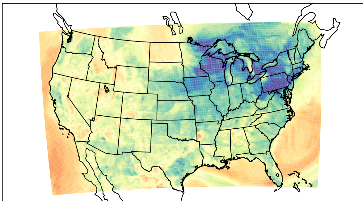
WRF (2021-04-13_04:00:00)
