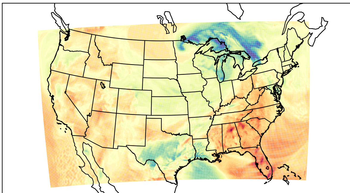
WRF (2021-04-13_19:00:00)
