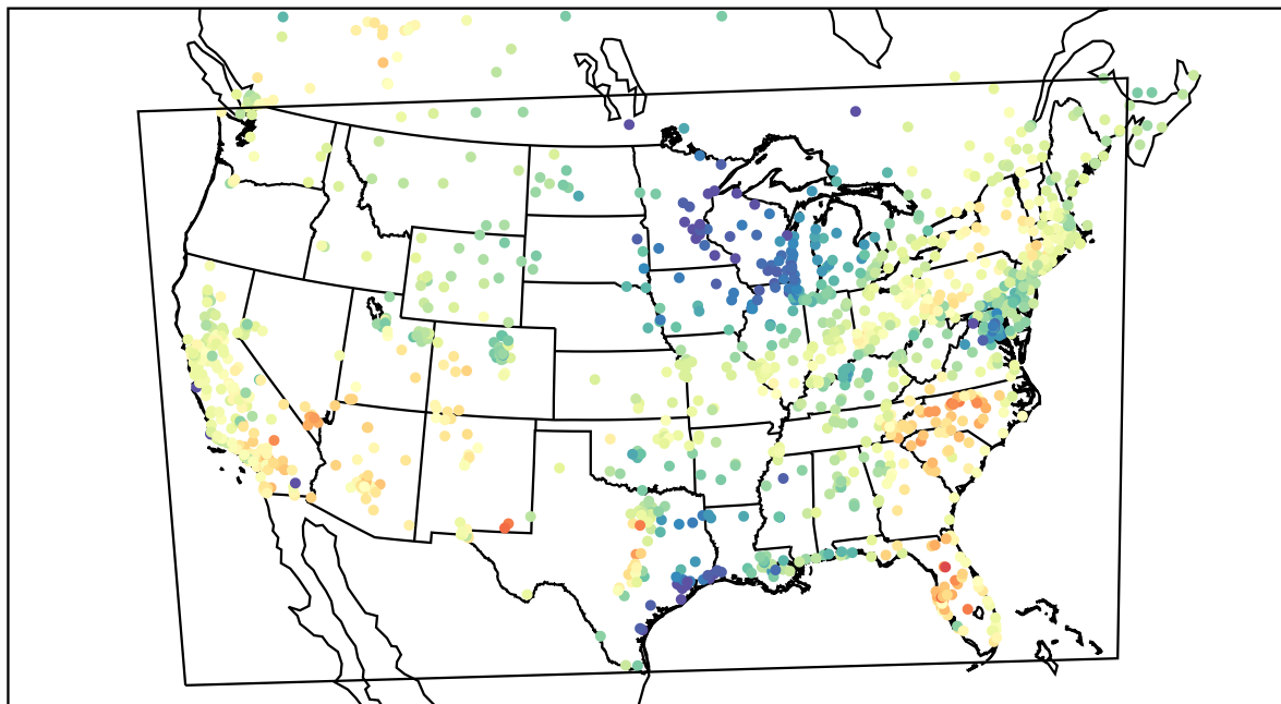
AirNOW (2021-04-14_21:00:00)
