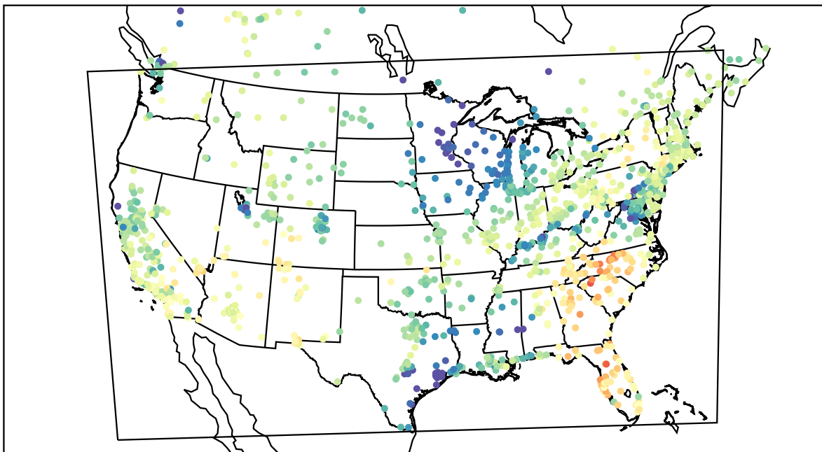
AirNOW (2021-04-14_17:00:00)
