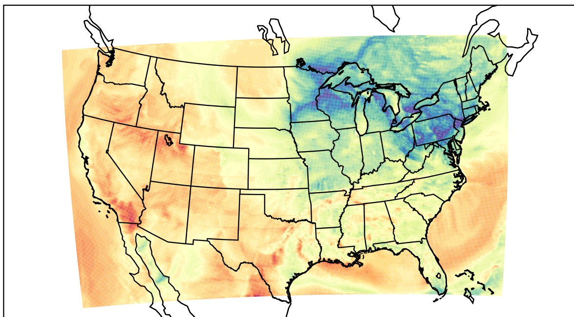
WRF (2021-04-13_00:00:00)
