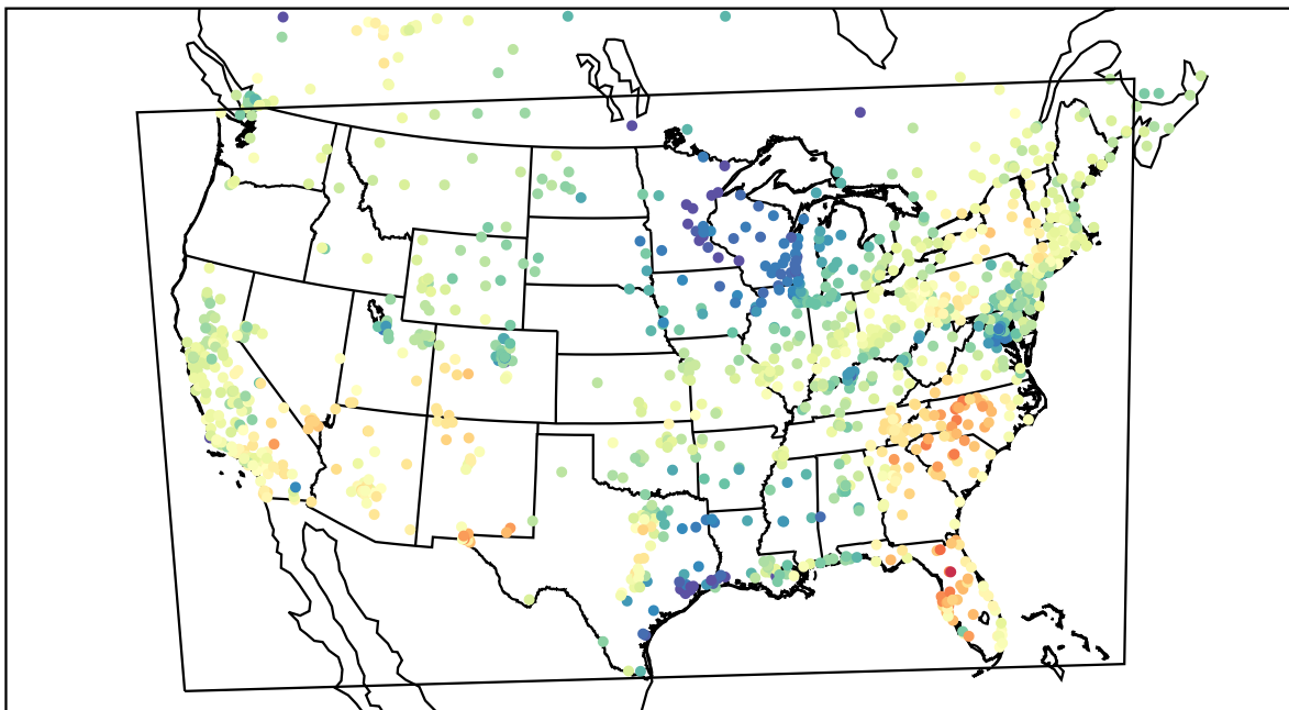
AirNOW (2021-04-14_19:00:00)
