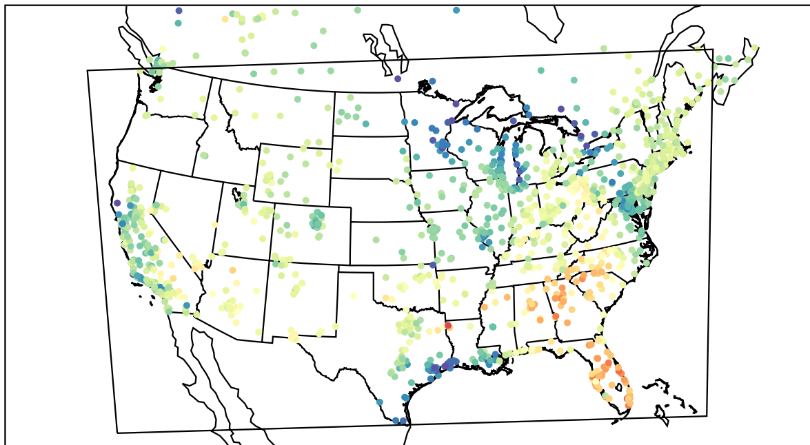
AirNOW (2021-04-13_17:00:00)
