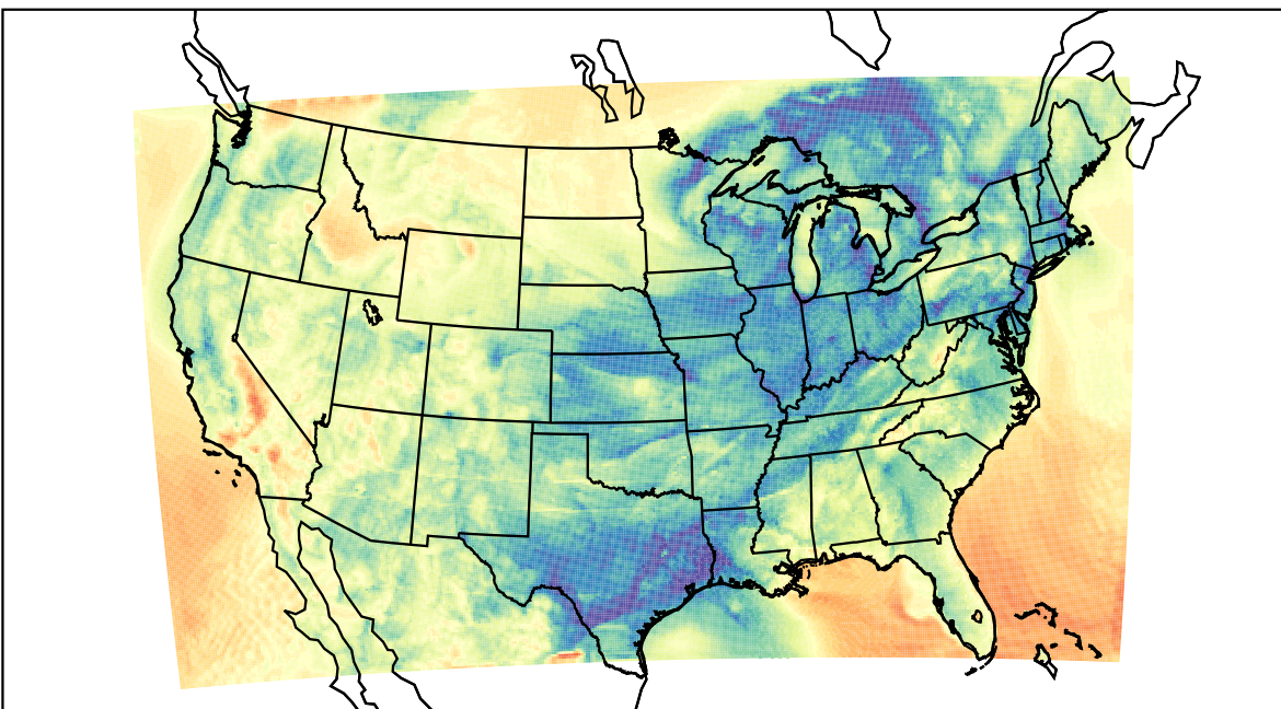
WRF (2021-04-14_09:00:00)
