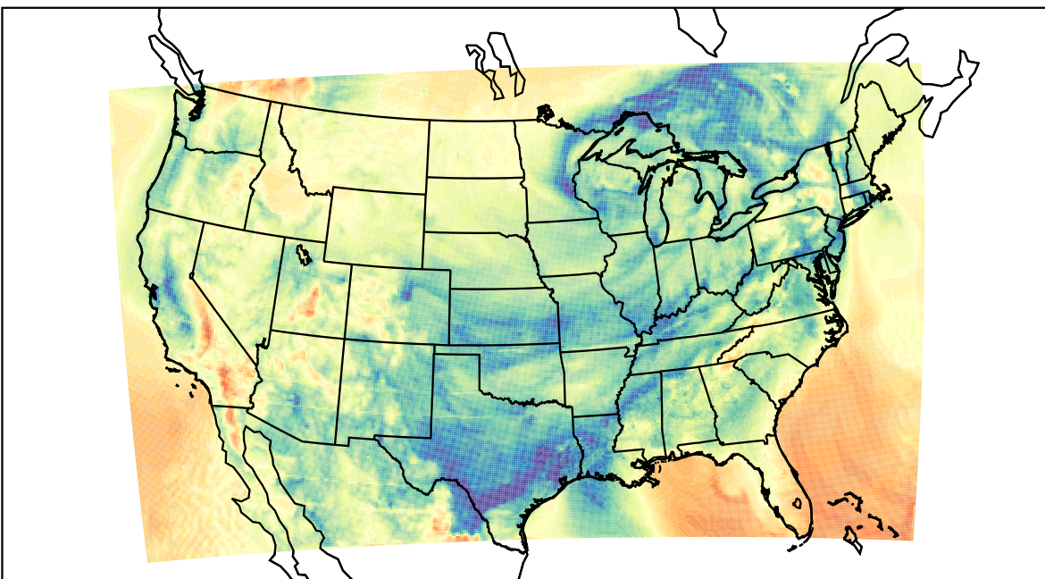
WRF (2021-04-14_14:00:00)
