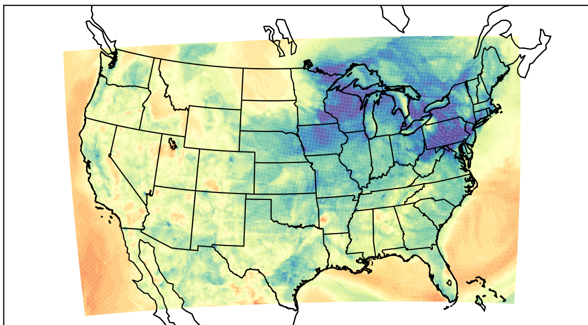
WRF (2021-04-13_05:00:00)
