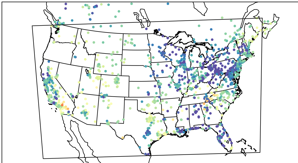
AirNOW (2021-04-13_05:00:00)
