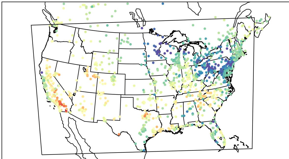
AirNOW (2021-04-13_00:00:00)
