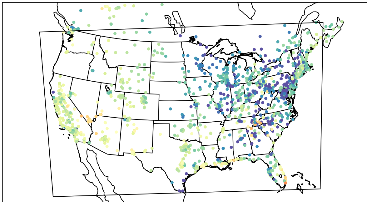
AirNOW (2021-04-14_03:00:00)
