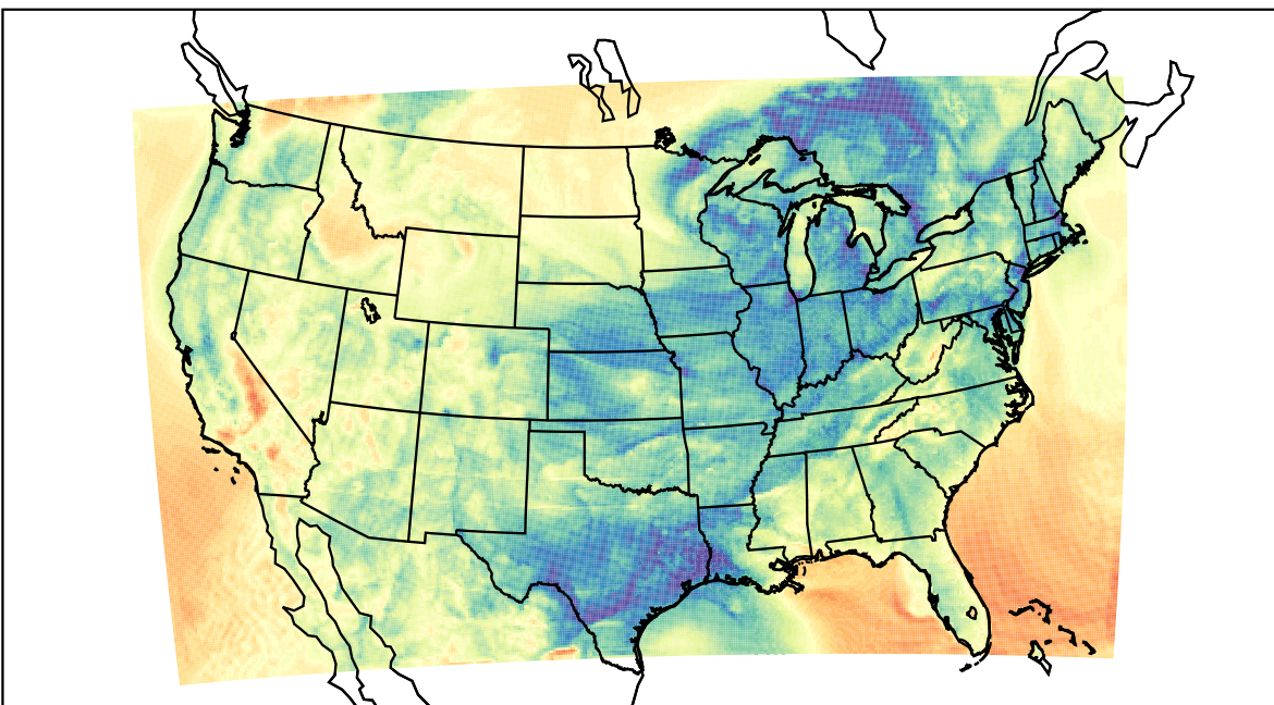
WRF (2021-04-14_08:00:00)
