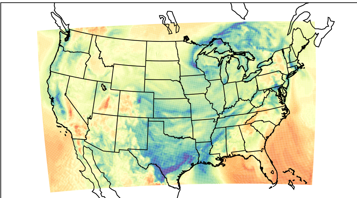
WRF (2021-04-14_15:00:00)
