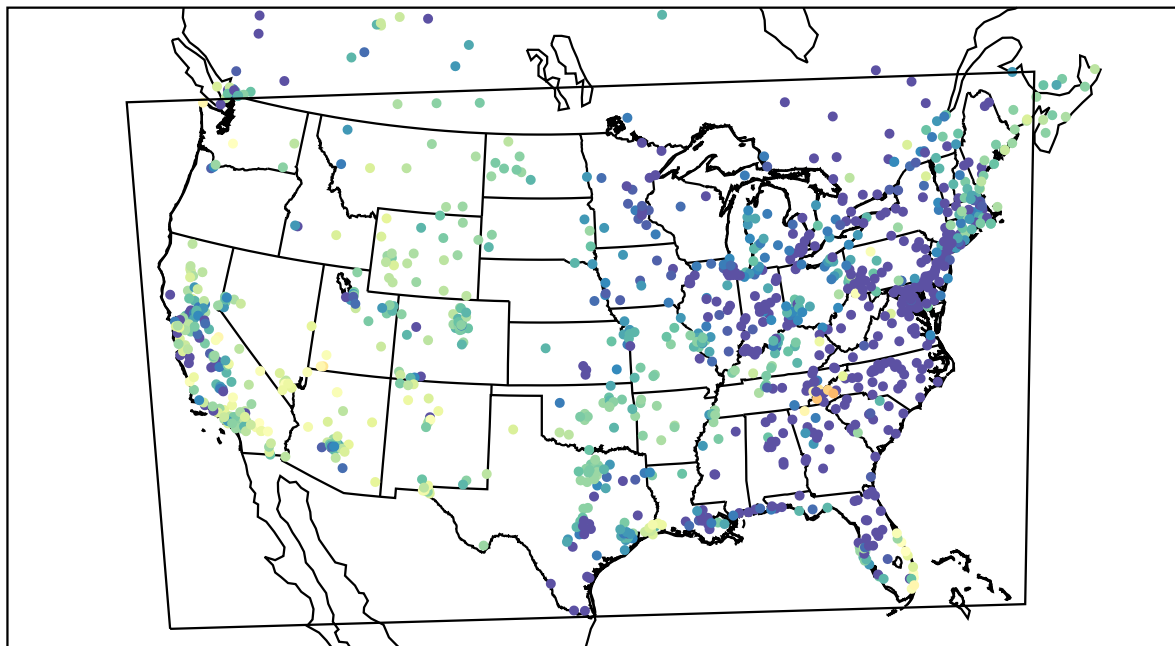
AirNOW (2021-04-14_10:00:00)
