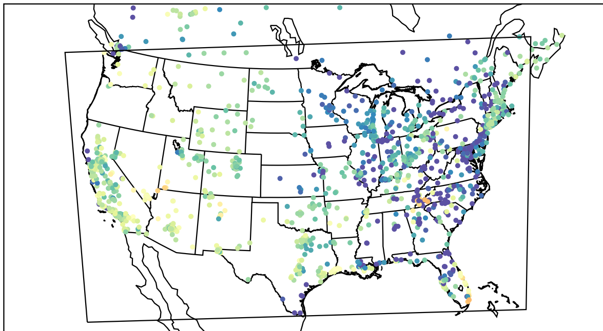
AirNOW (2021-04-14_06:00:00)
