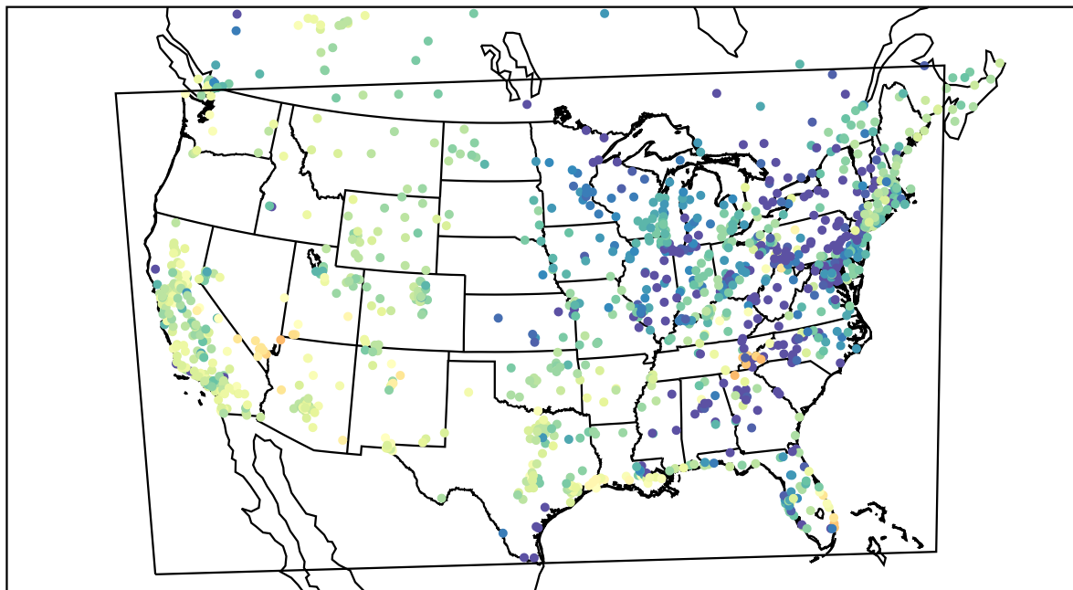
AirNOW (2021-04-14_04:00:00)
