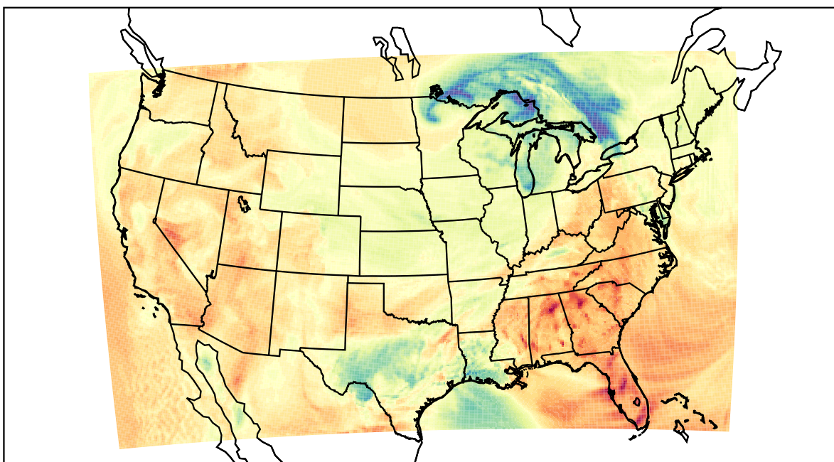
WRF (2021-04-13_20:00:00)
