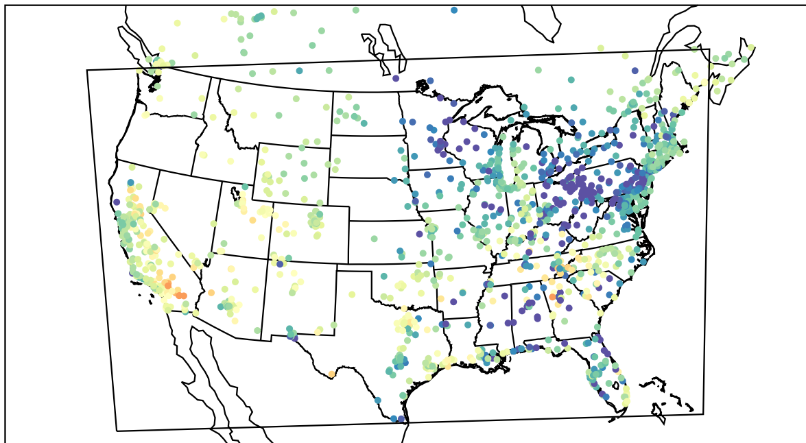
AirNOW (2021-04-13_02:00:00)
