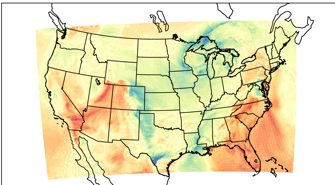
WRF (2021-04-14_19:00:00)
