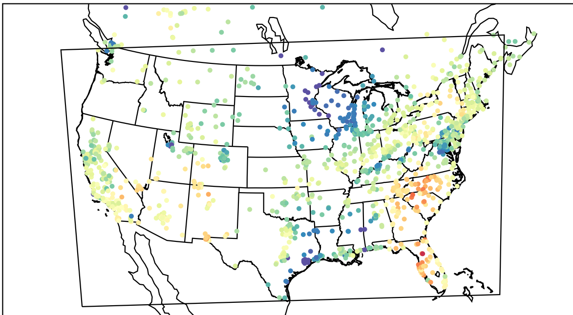
AirNOW (2021-04-14_18:00:00)
