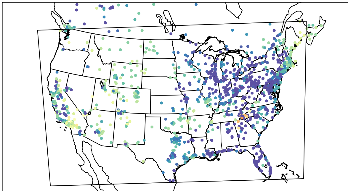
AirNOW (2021-04-13_11:00:00)
