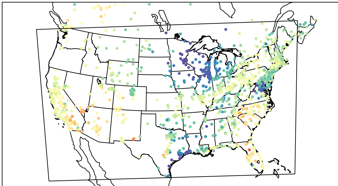
AirNOW (2021-04-14_23:00:00)
