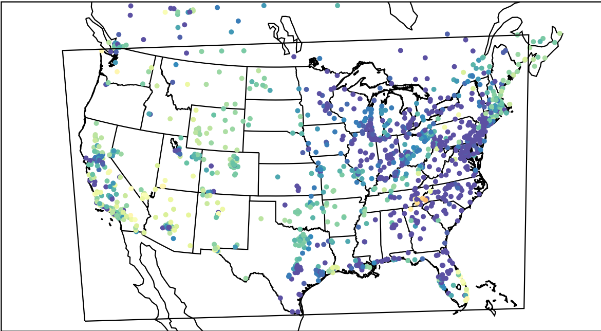
AirNOW (2021-04-14_11:00:00)
