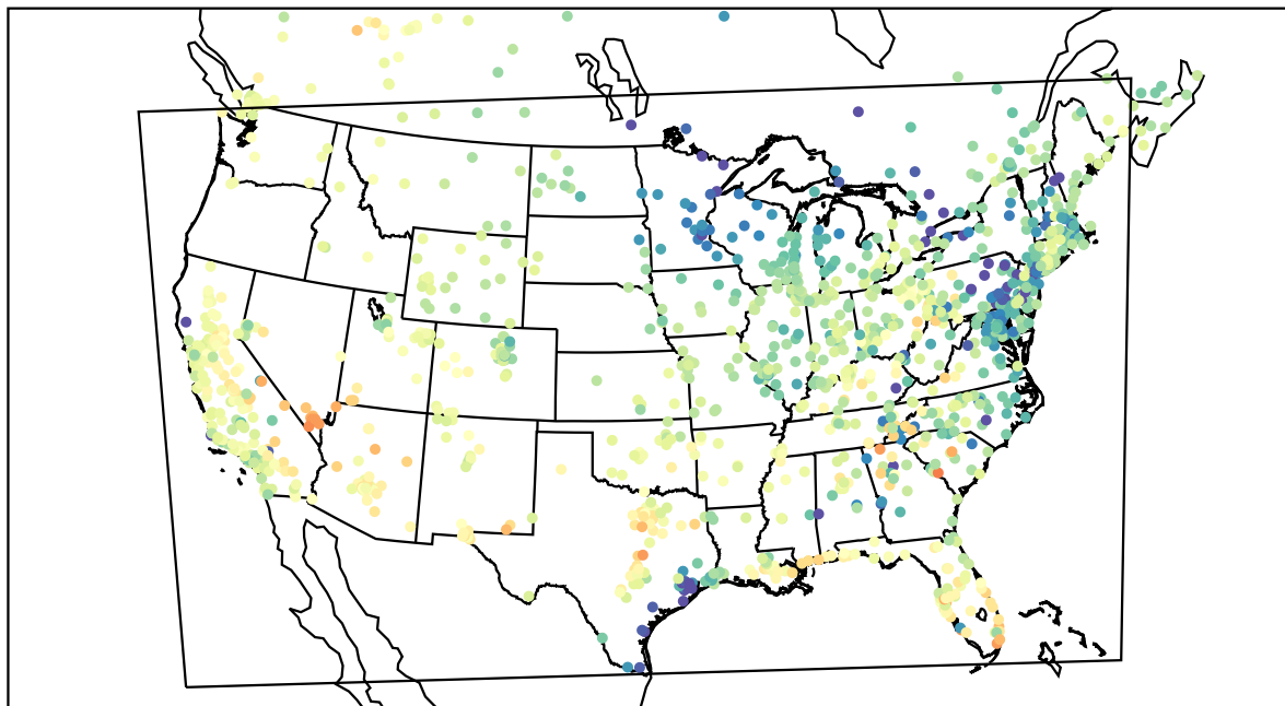
AirNOW (2021-04-14_00:00:00)
