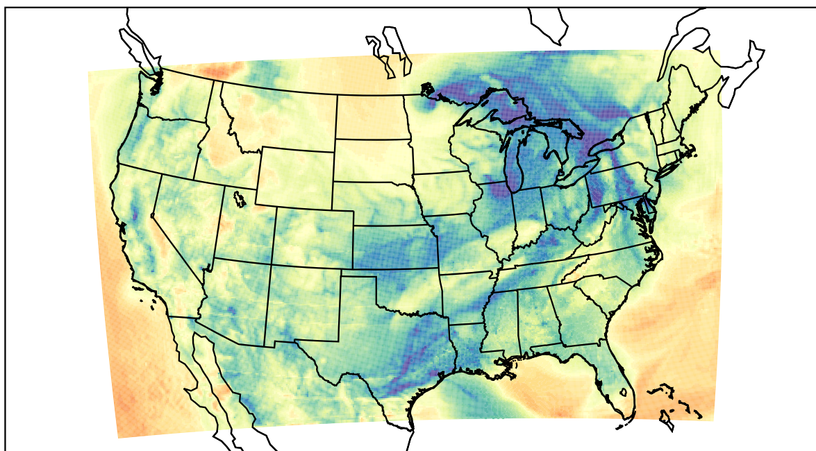
WRF (2021-04-13_14:00:00)
