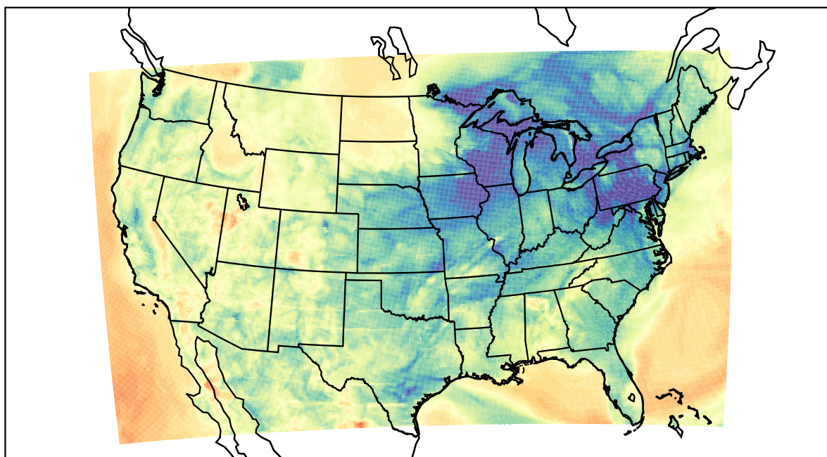
WRF (2021-04-13_08:00:00)
