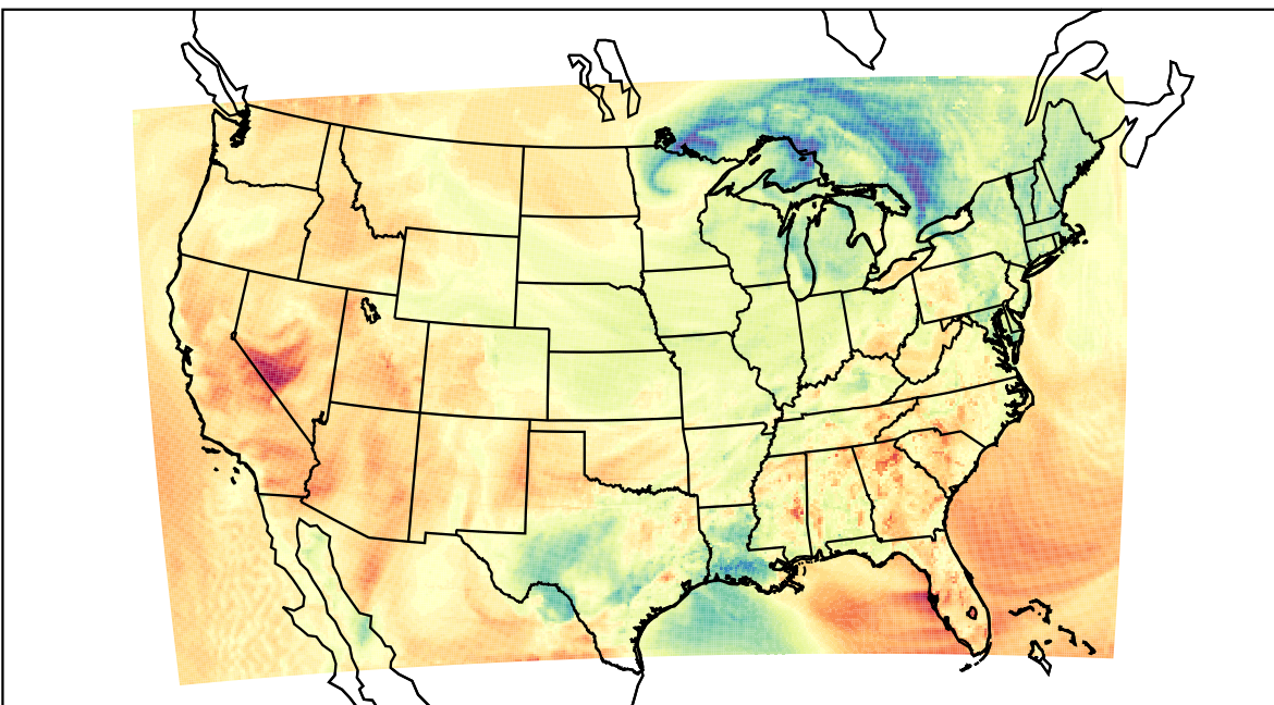
WRF (2021-04-13_23:00:00)
