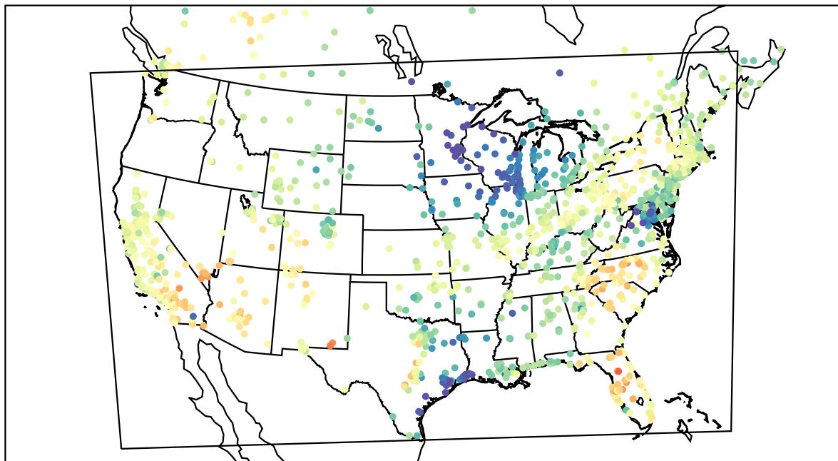
AirNOW (2021-04-14_22:00:00)
