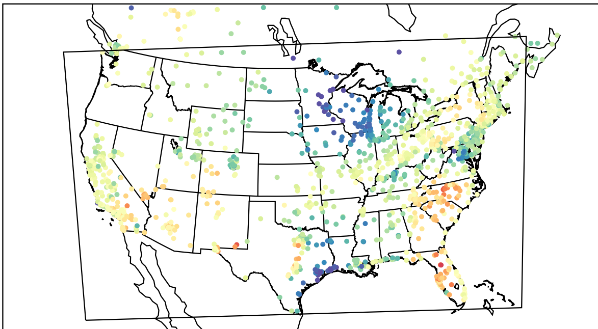
AirNOW (2021-04-14_20:00:00)
