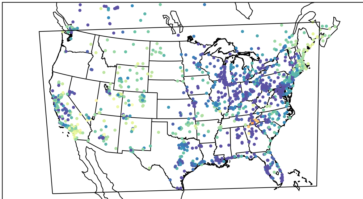
AirNOW (2021-04-13_12:00:00)
