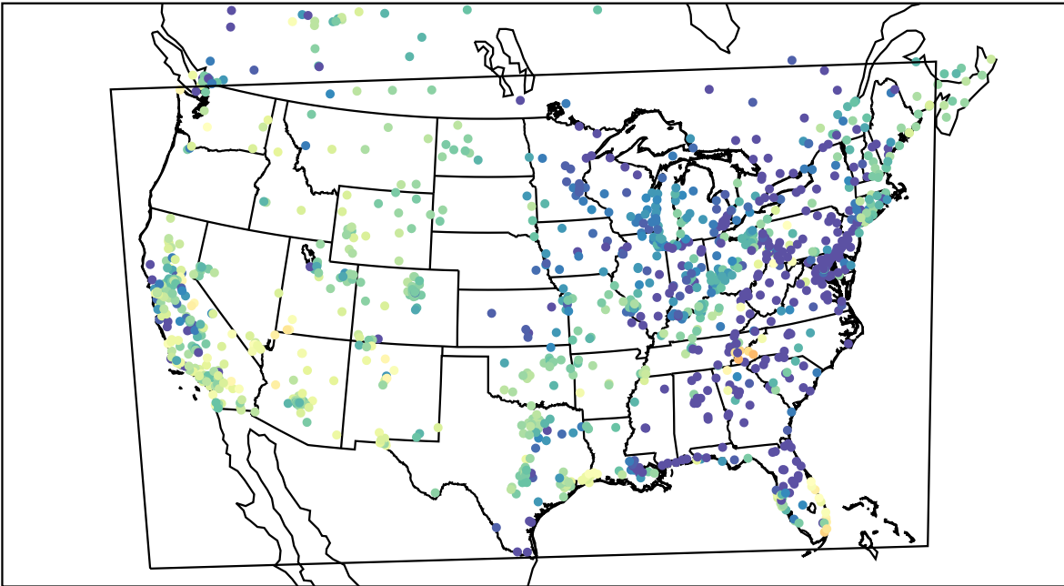
AirNOW (2021-04-14_08:00:00)
