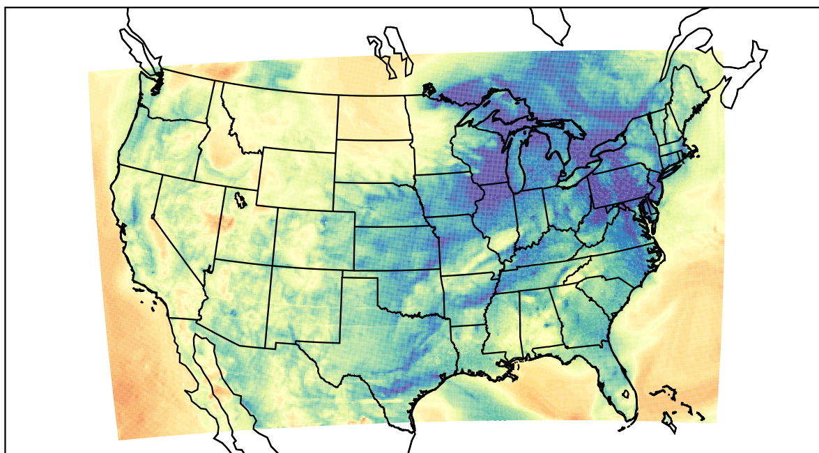
WRF (2021-04-13_11:00:00)
