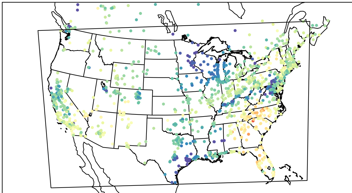
AirNOW (2021-04-14_16:00:00)
