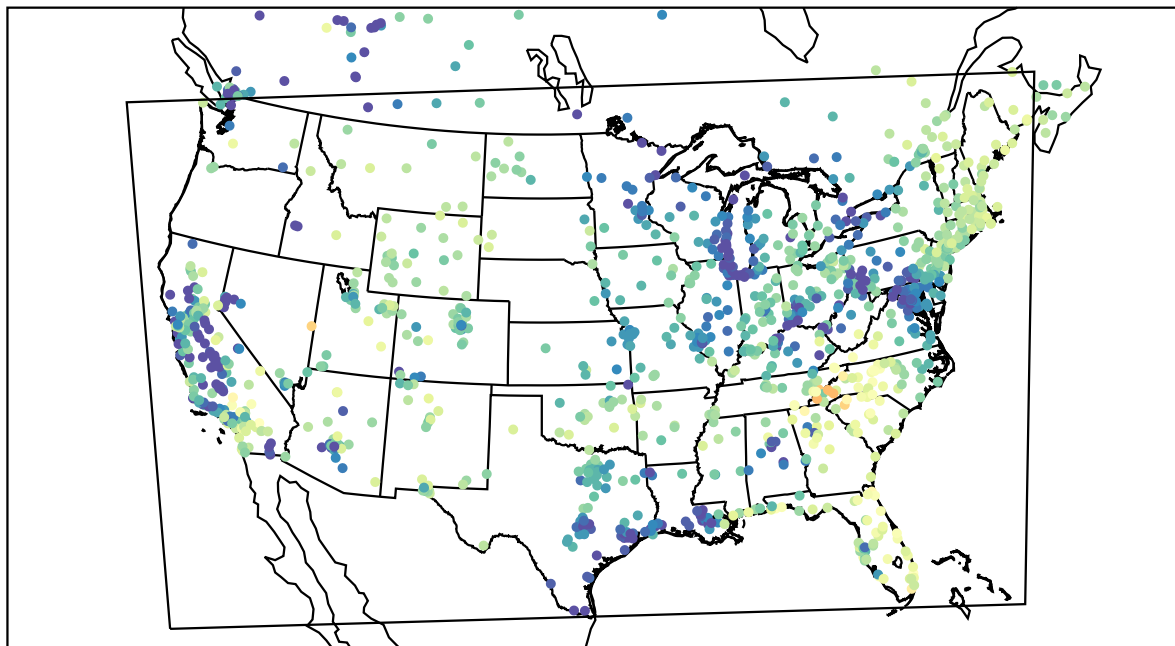
AirNOW (2021-04-13_14:00:00)
