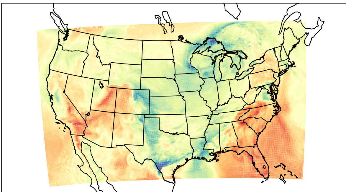
WRF (2021-04-14_18:00:00)
