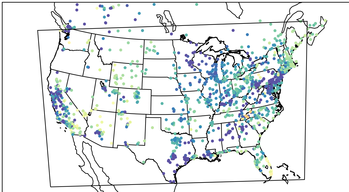
AirNOW (2021-04-14_13:00:00)
