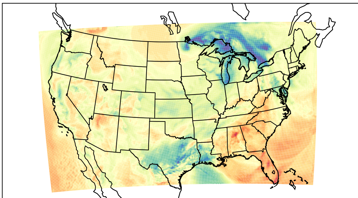
WRF (2021-04-13_17:00:00)
