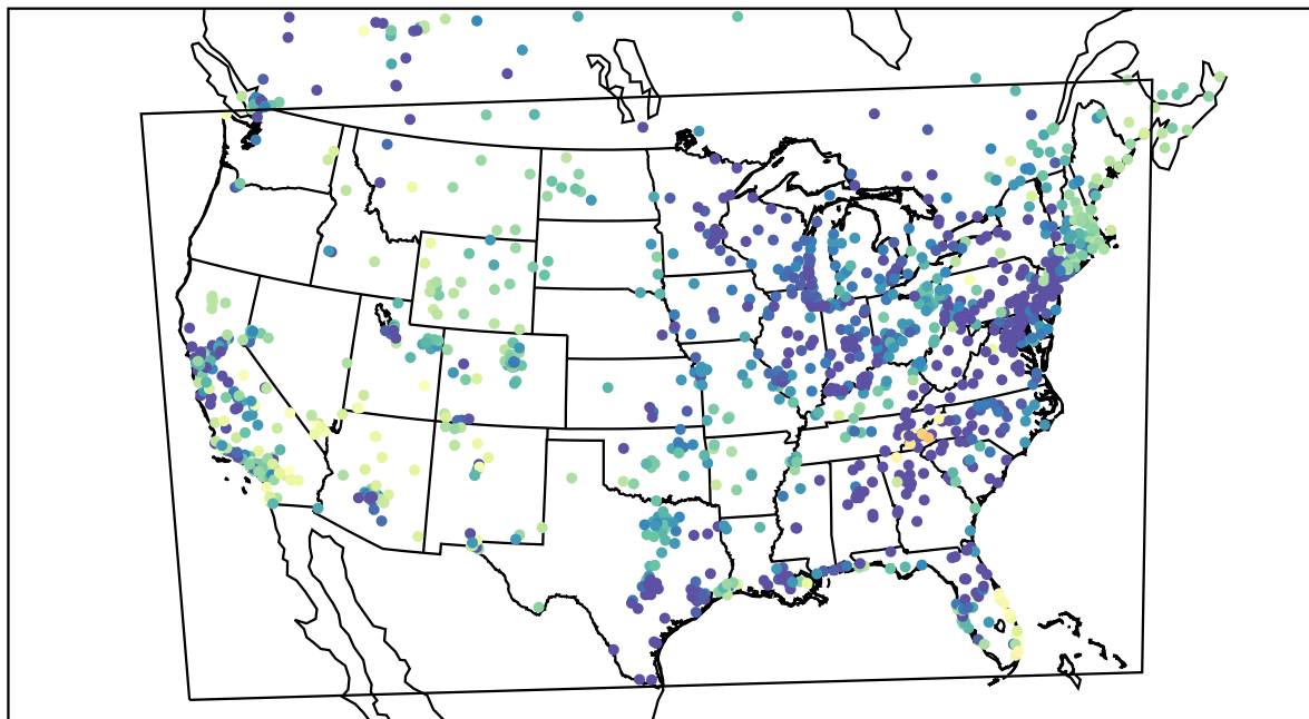
AirNOW (2021-04-14_12:00:00)
