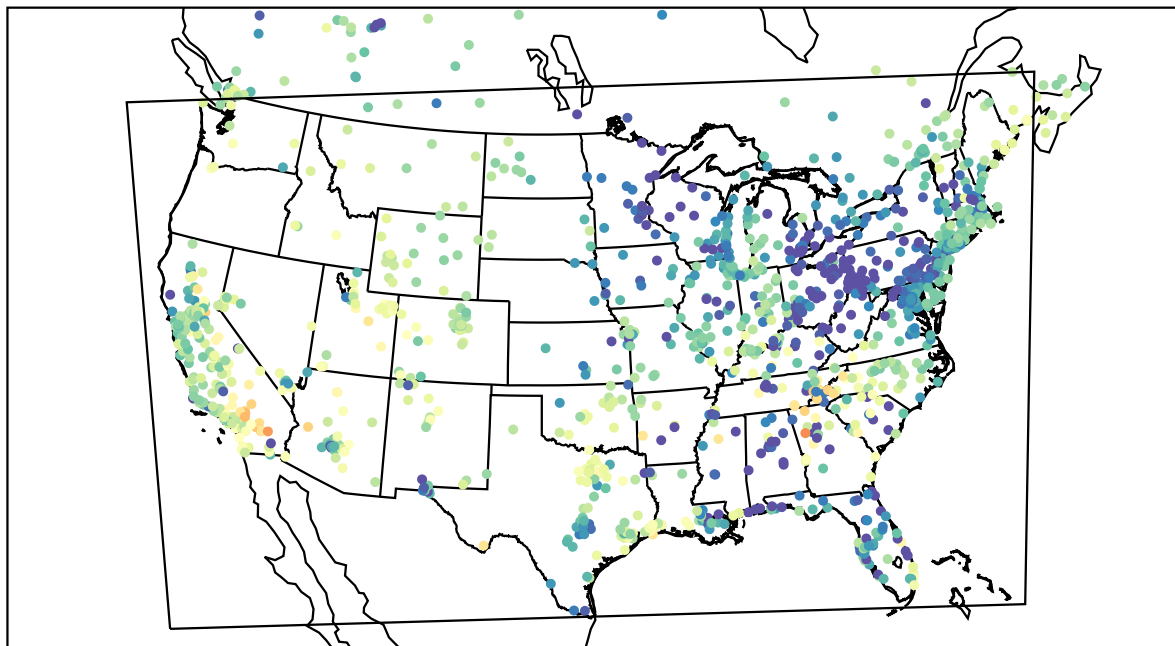
AirNOW (2021-04-13_03:00:00)
