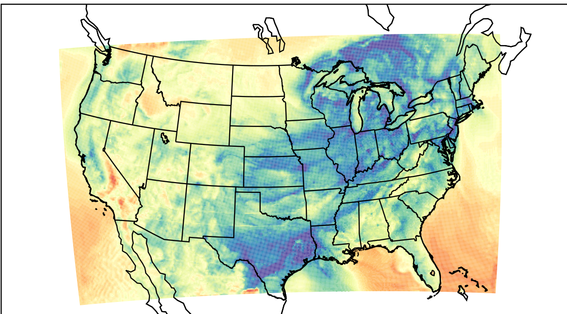
WRF (2021-04-14_11:00:00)
