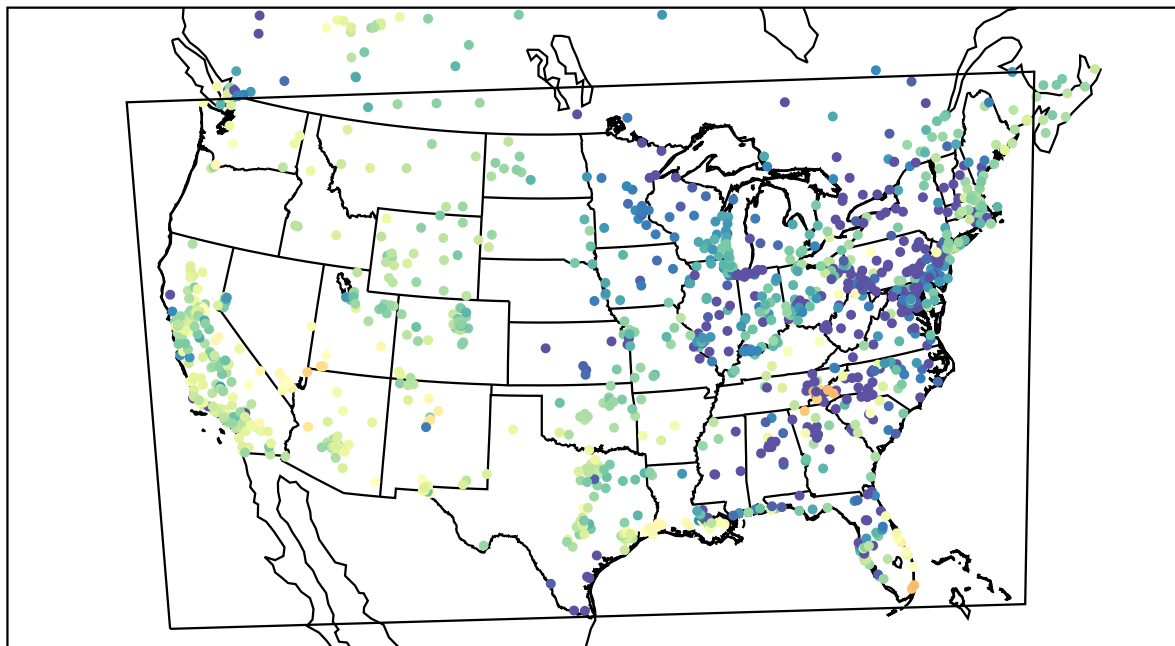
AirNOW (2021-04-14_05:00:00)
