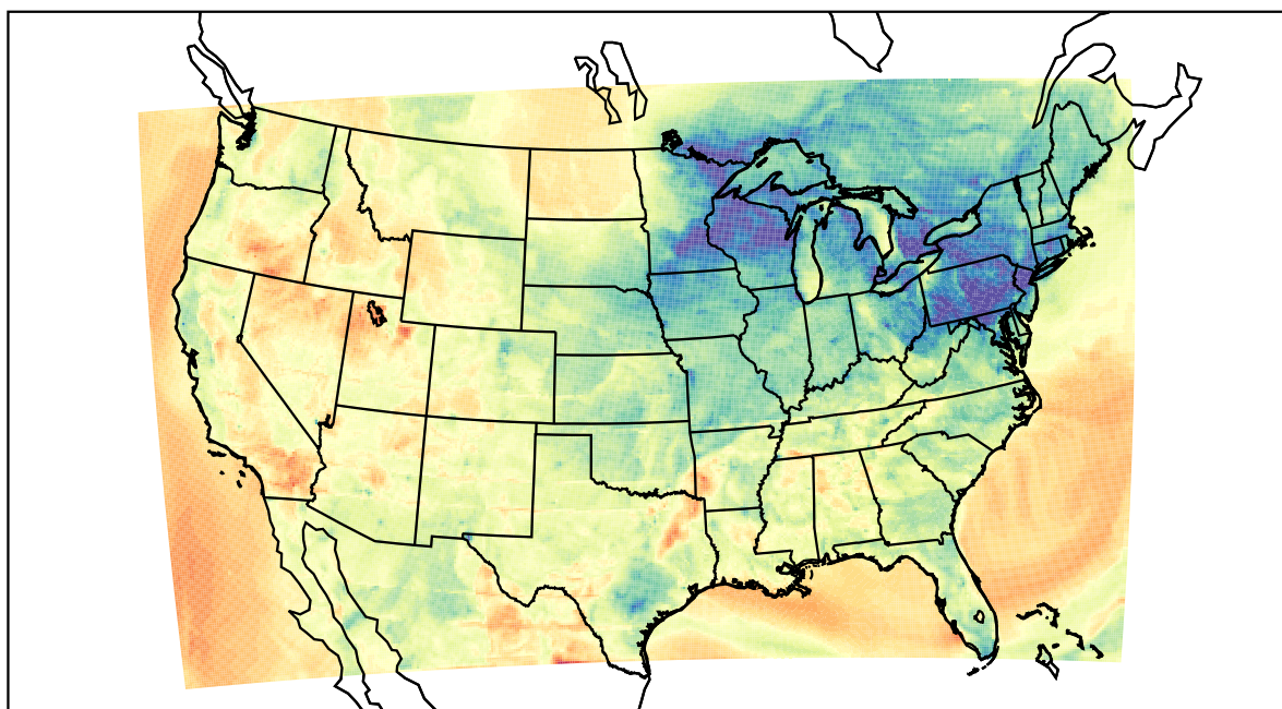
WRF (2021-04-13_02:00:00)
