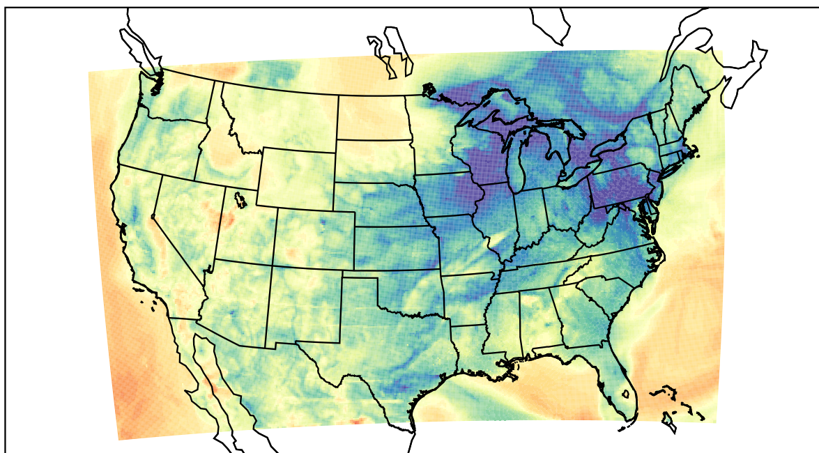
WRF (2021-04-13_09:00:00)
