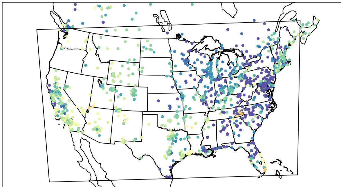
AirNOW (2021-04-14_07:00:00)
