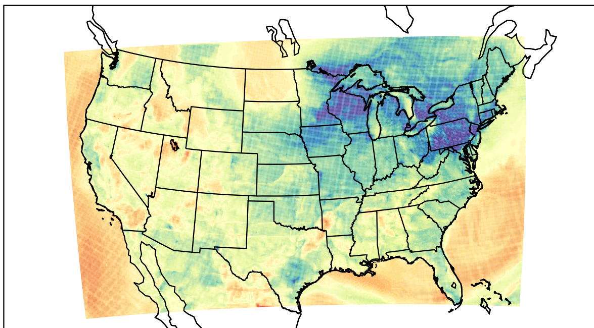
WRF (2021-04-13_03:00:00)
