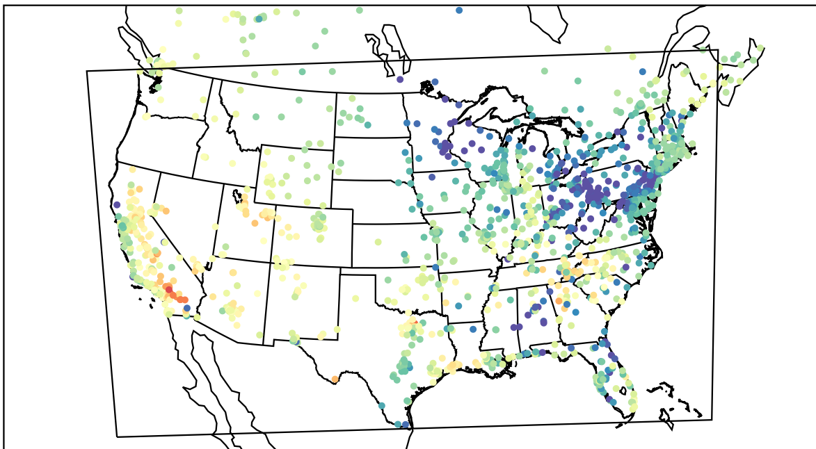
AirNOW (2021-04-13_01:00:00)
