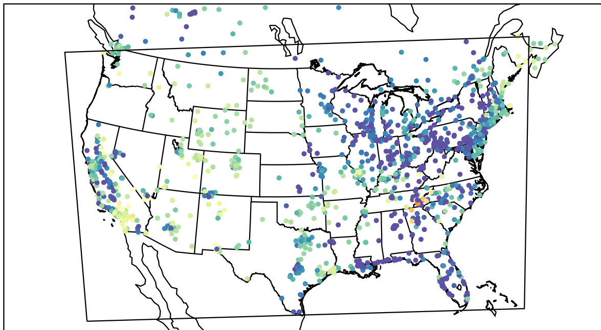
AirNOW (2021-04-13_09:00:00)
