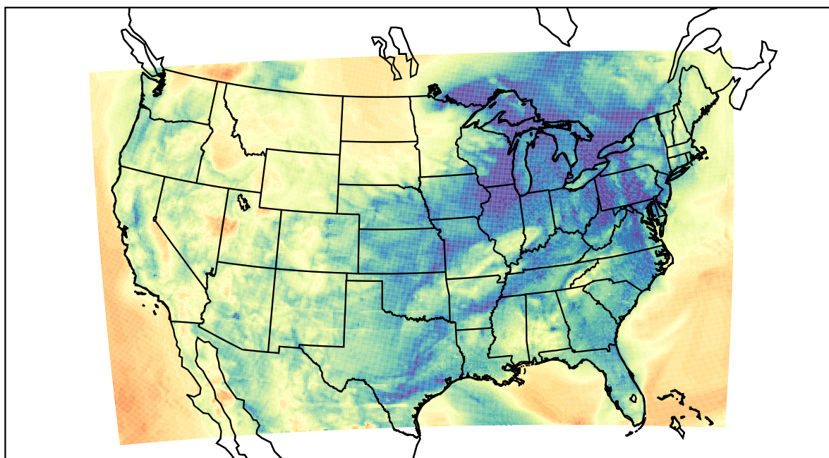
WRF (2021-04-13_12:00:00)
