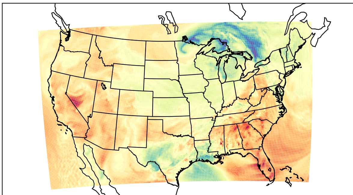
WRF (2021-04-13_22:00:00)
