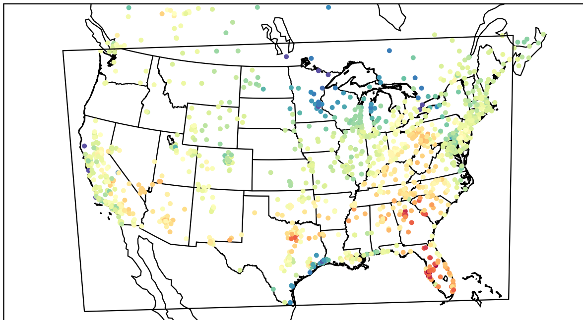
AirNOW (2021-04-13_21:00:00)
