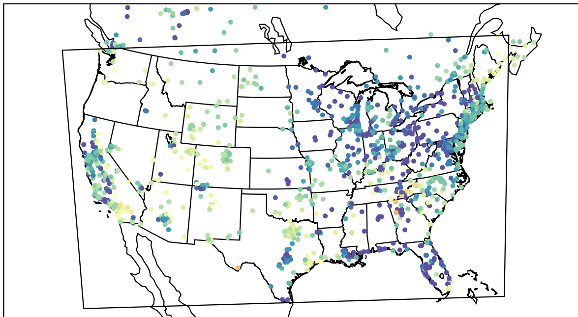
AirNOW (2021-04-13_06:00:00)
