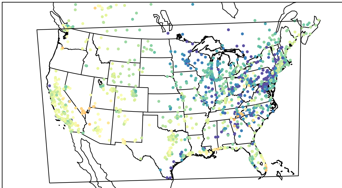
AirNOW (2021-04-14_02:00:00)
