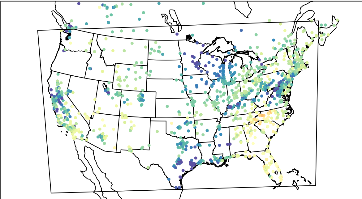
AirNOW (2021-04-14_15:00:00)
