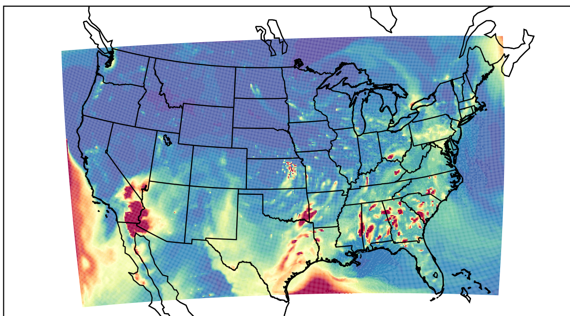
WRF 2021-04-14_03:00:00
