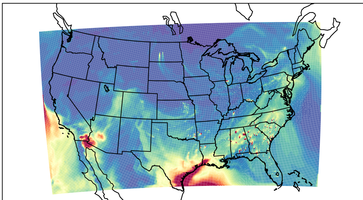
WRF 2021-04-14_19:00:00
