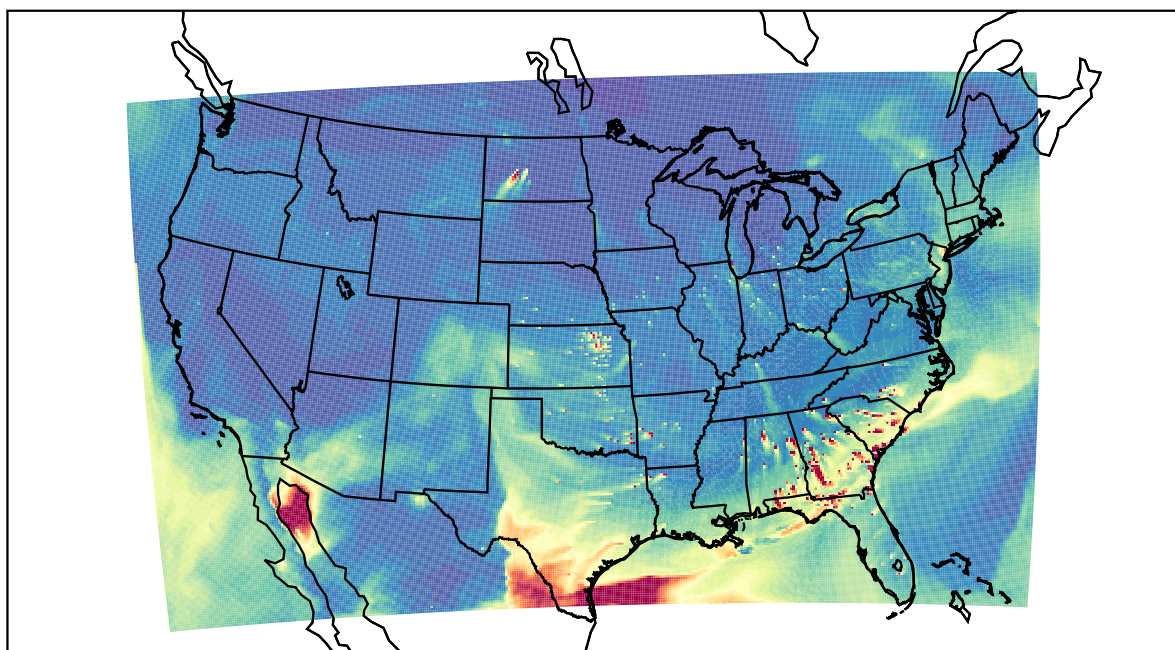
WRF 2021-04-15_21:00:00
