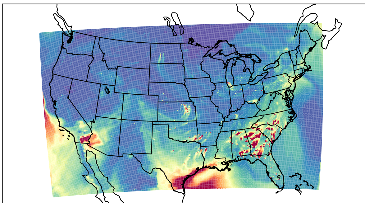
WRF 2021-04-14_23:00:00
