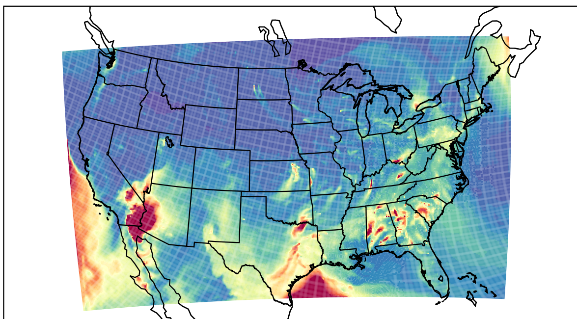
WRF 2021-04-14_06:00:00
