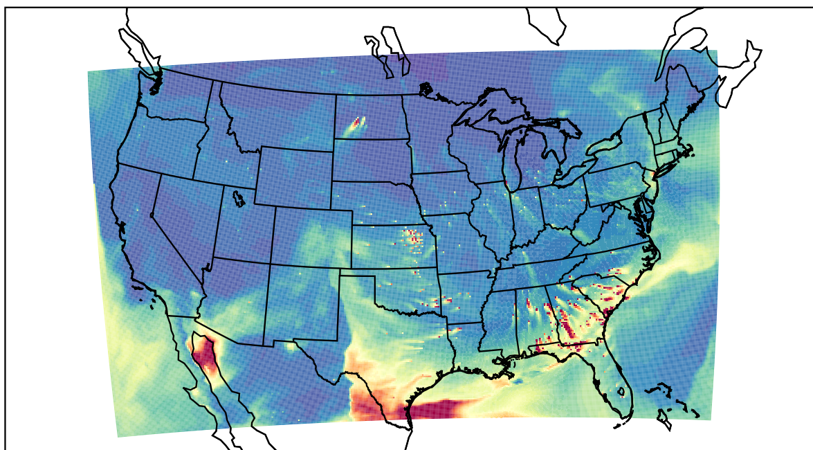
WRF 2021-04-15_22:00:00
