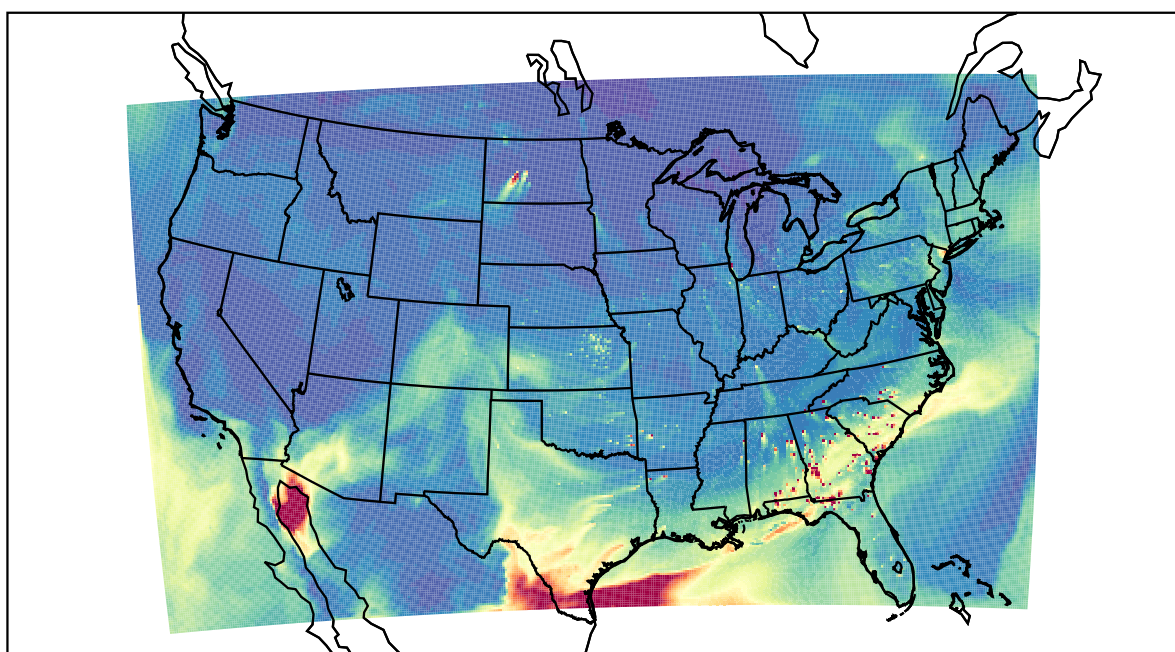
WRF 2021-04-15_19:00:00
