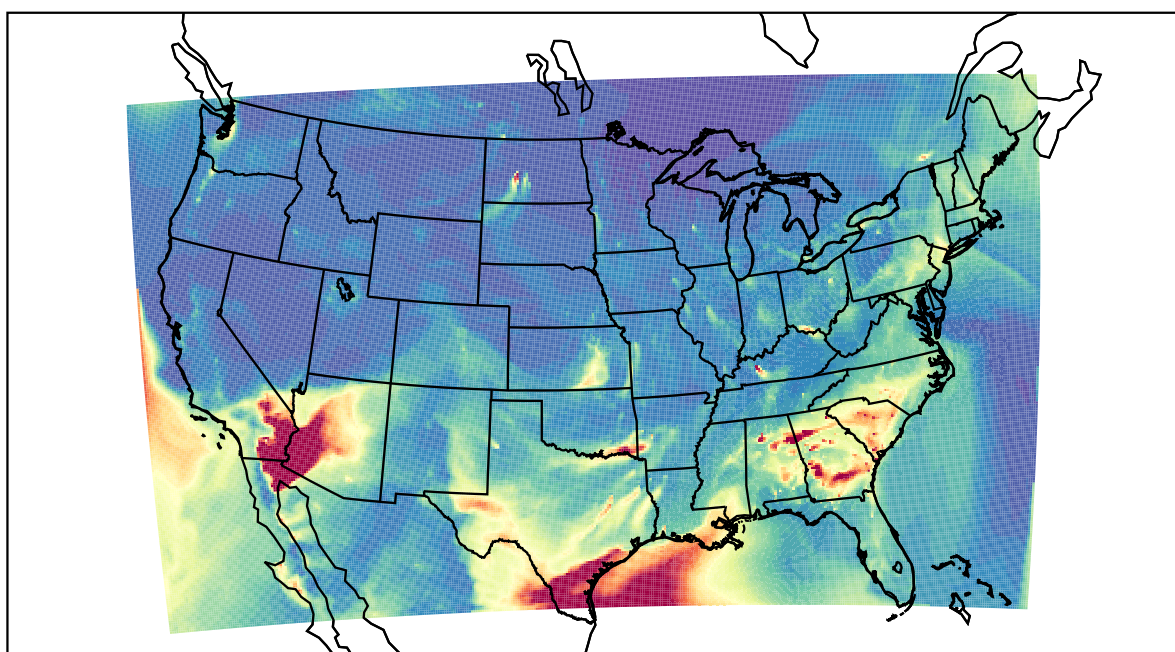
WRF 2021-04-15_06:00:00
