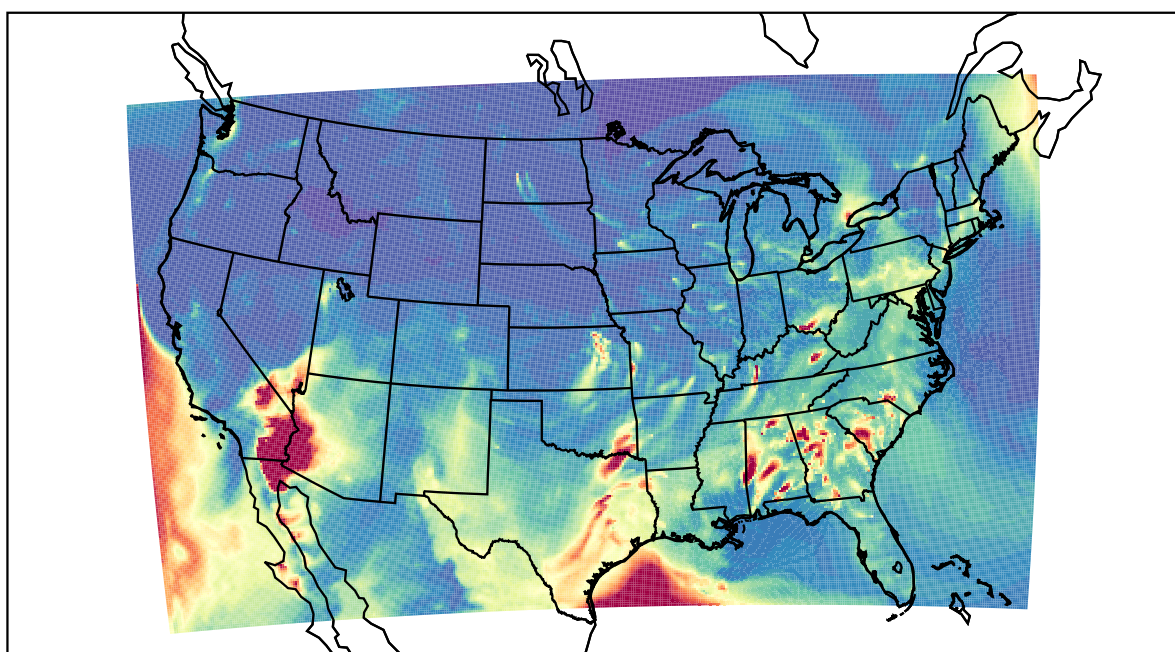
WRF 2021-04-14_05:00:00
