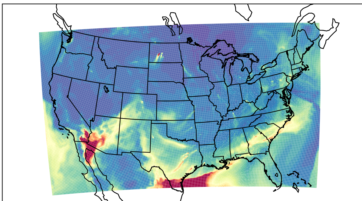
WRF 2021-04-15_15:00:00
