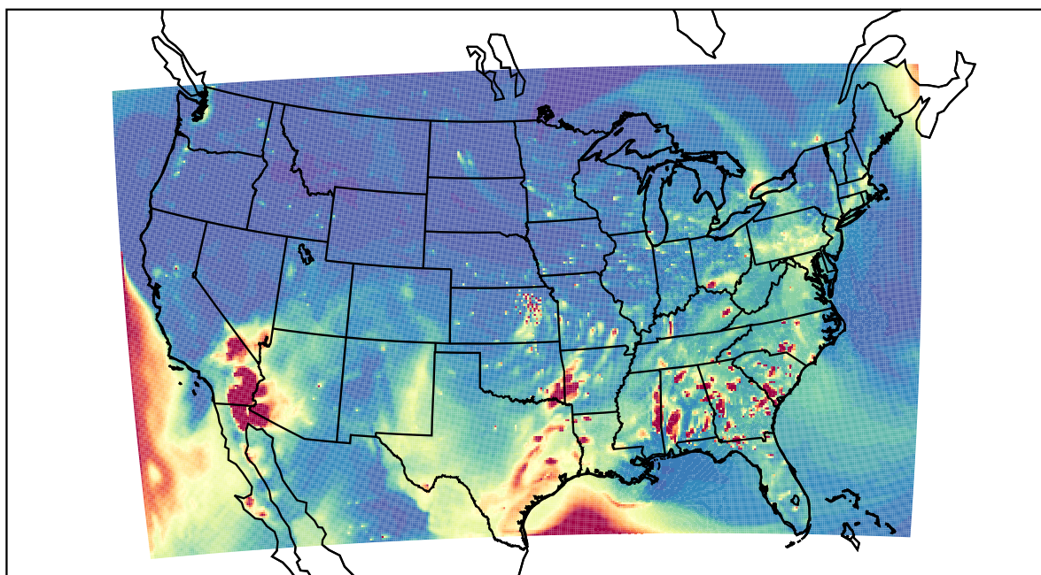
WRF 2021-04-14_02:00:00
