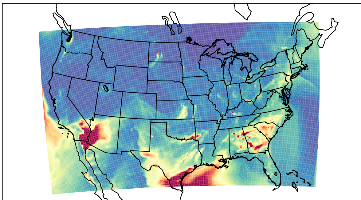
WRF 2021-04-15_05:00:00
