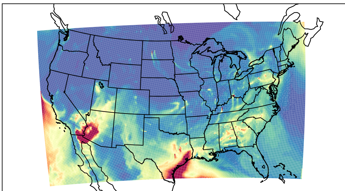
WRF 2021-04-14_14:00:00
