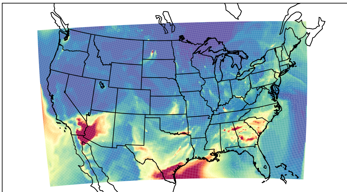
WRF 2021-04-15_07:00:00
