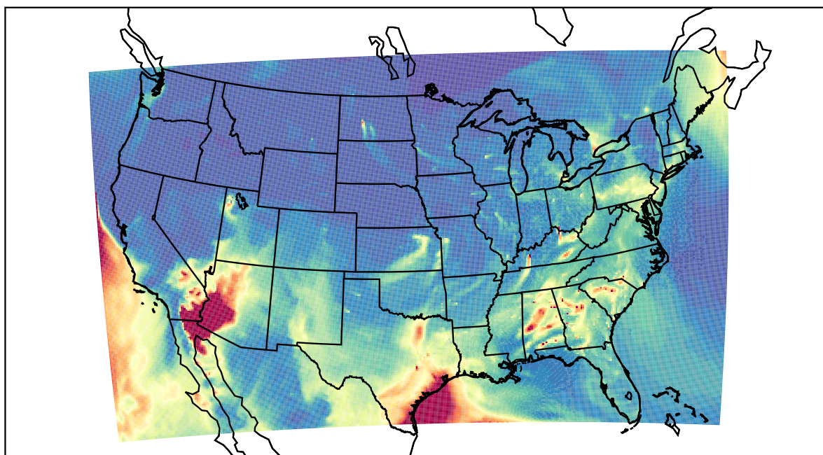
WRF 2021-04-14_10:00:00
