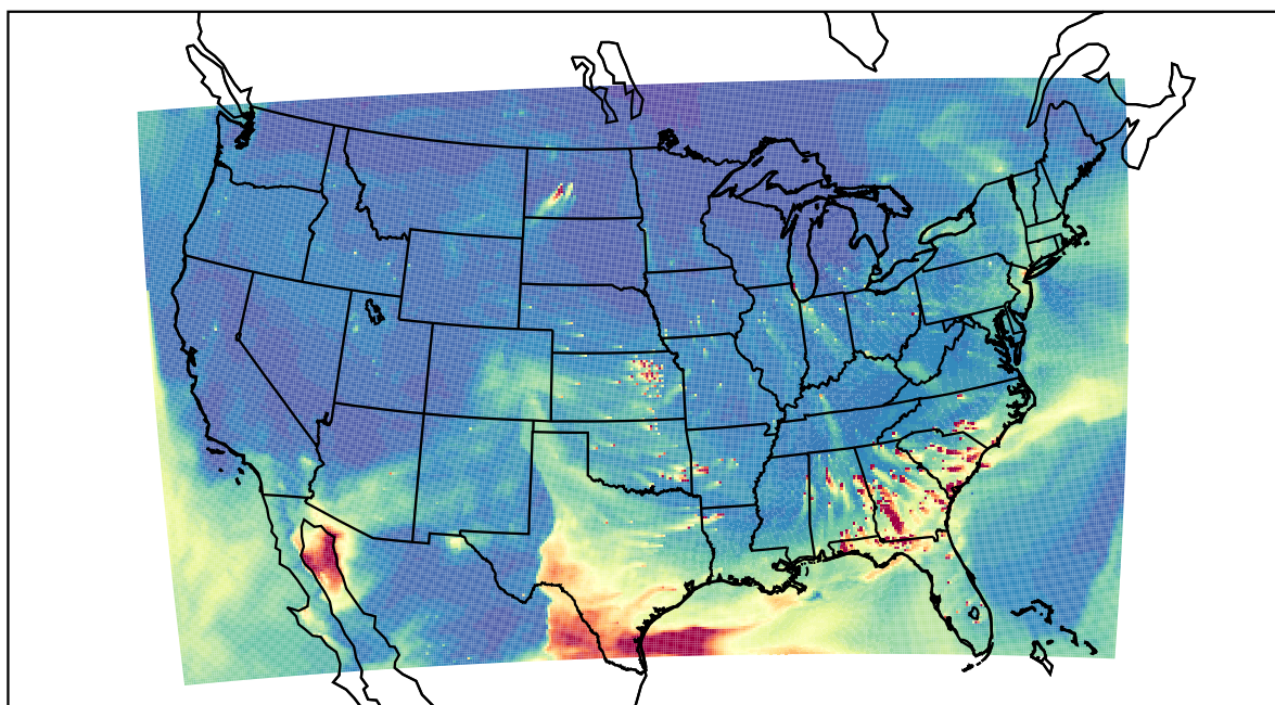
WRF 2021-04-15_23:00:00
