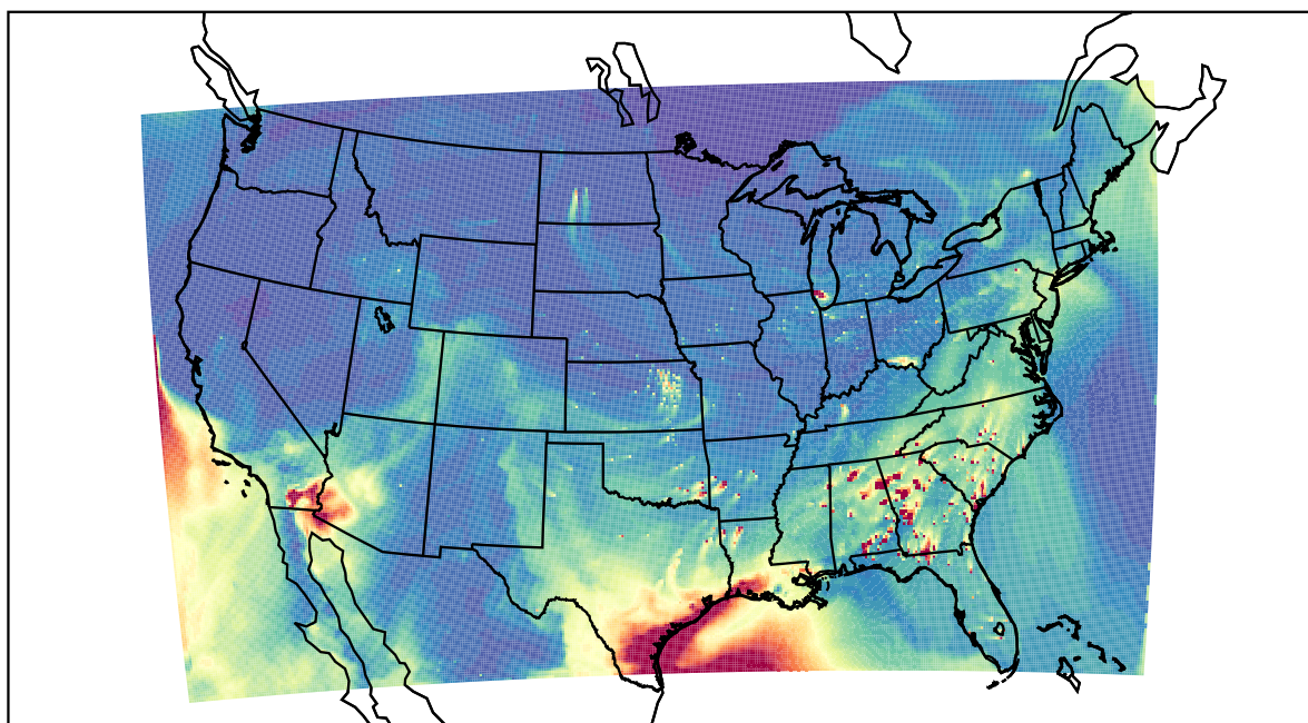
WRF 2021-04-14_21:00:00
