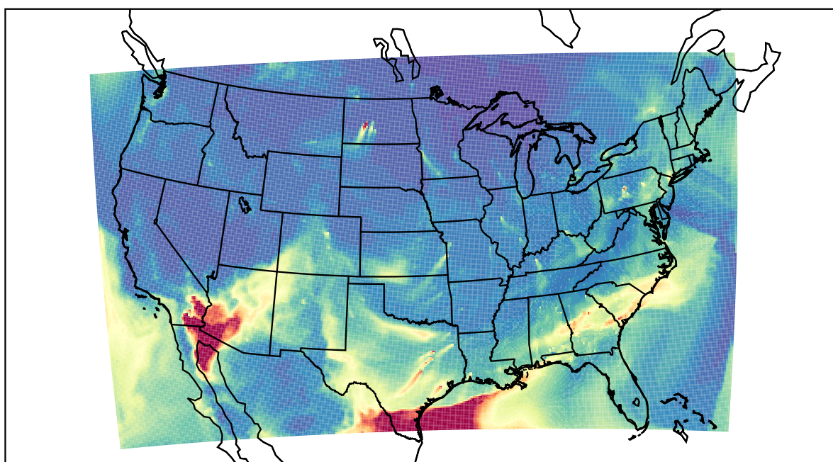
WRF 2021-04-15_14:00:00
