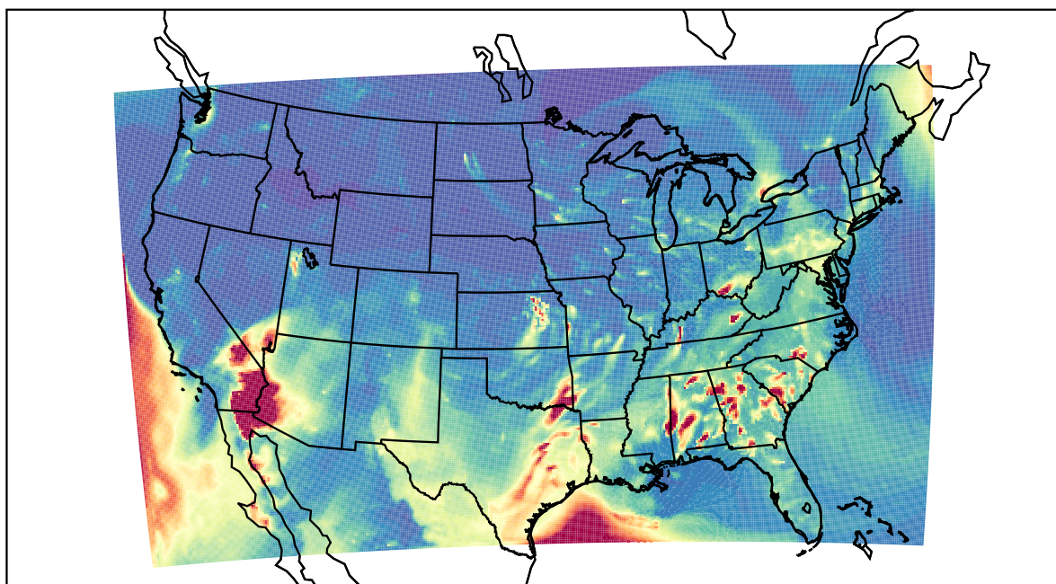
WRF 2021-04-14_04:00:00
