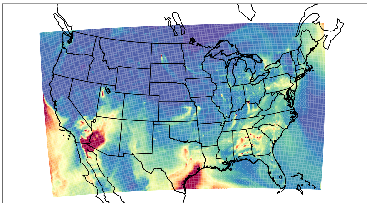
WRF 2021-04-14_12:00:00
