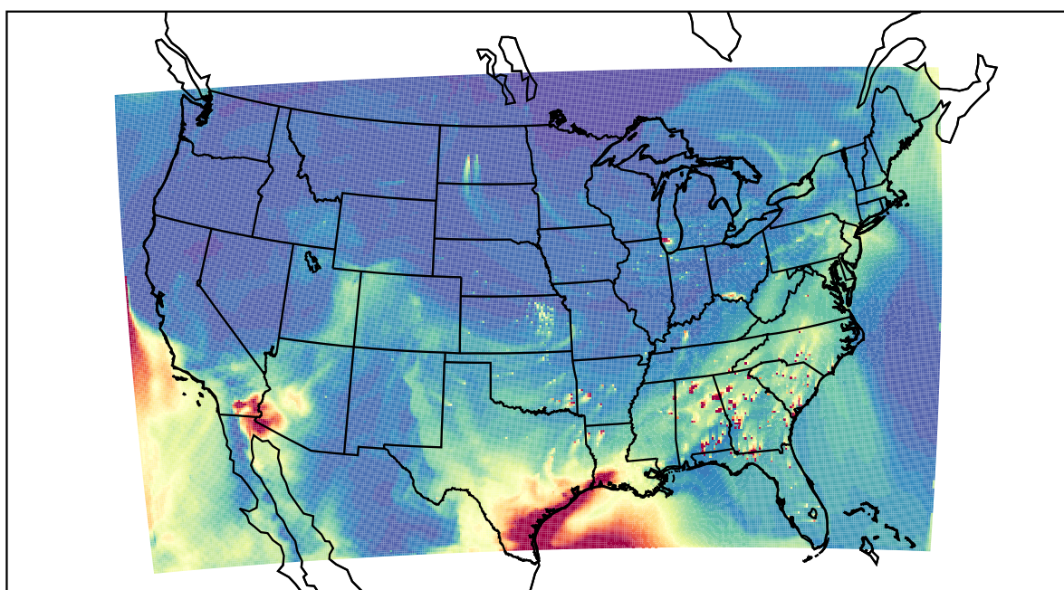
WRF 2021-04-14_20:00:00
