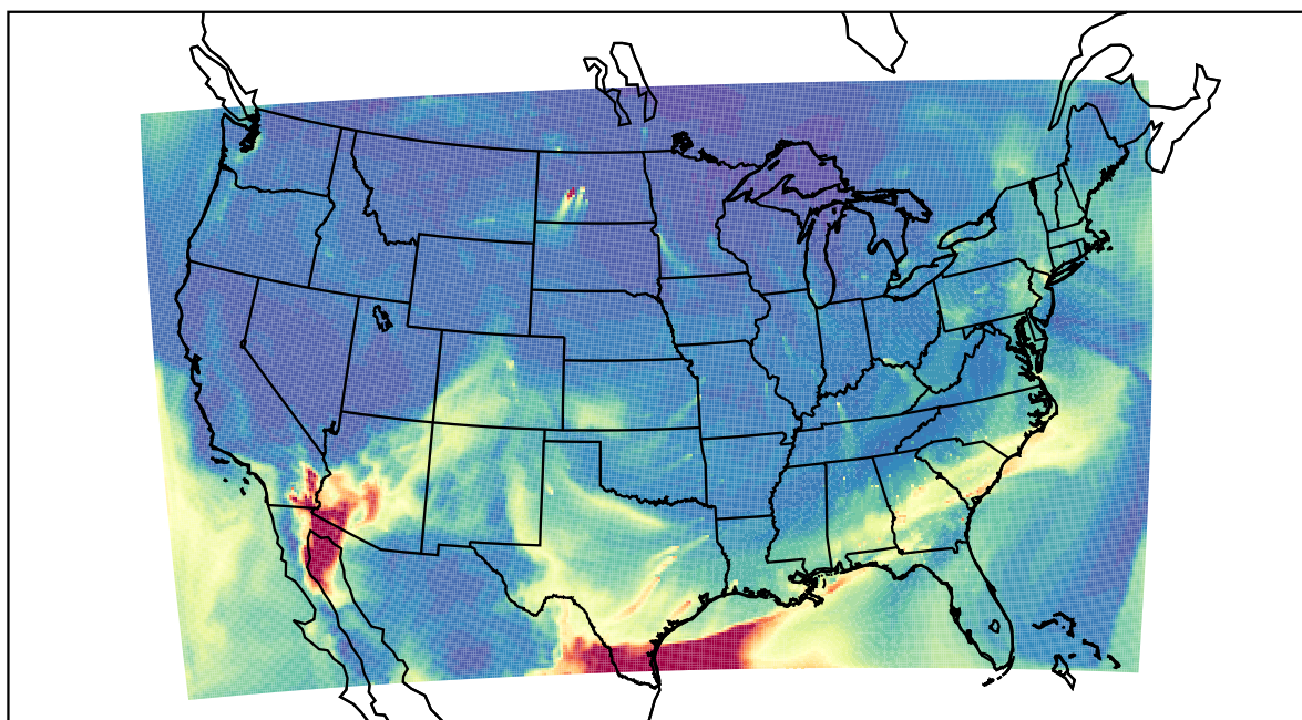
WRF 2021-04-15_16:00:00
