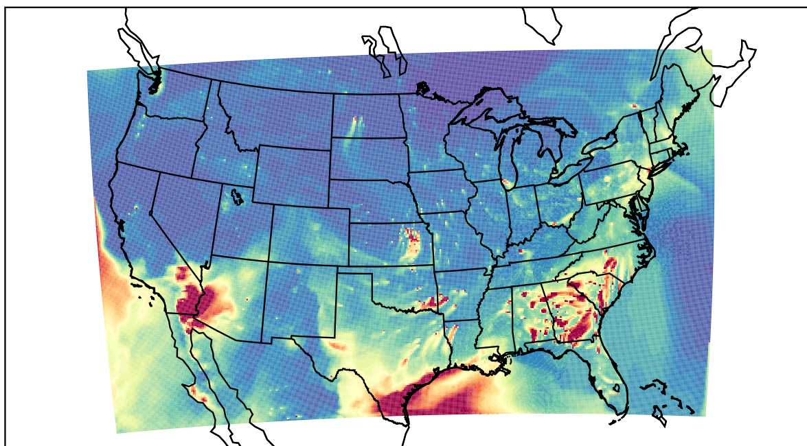
WRF 2021-04-15_02:00:00
