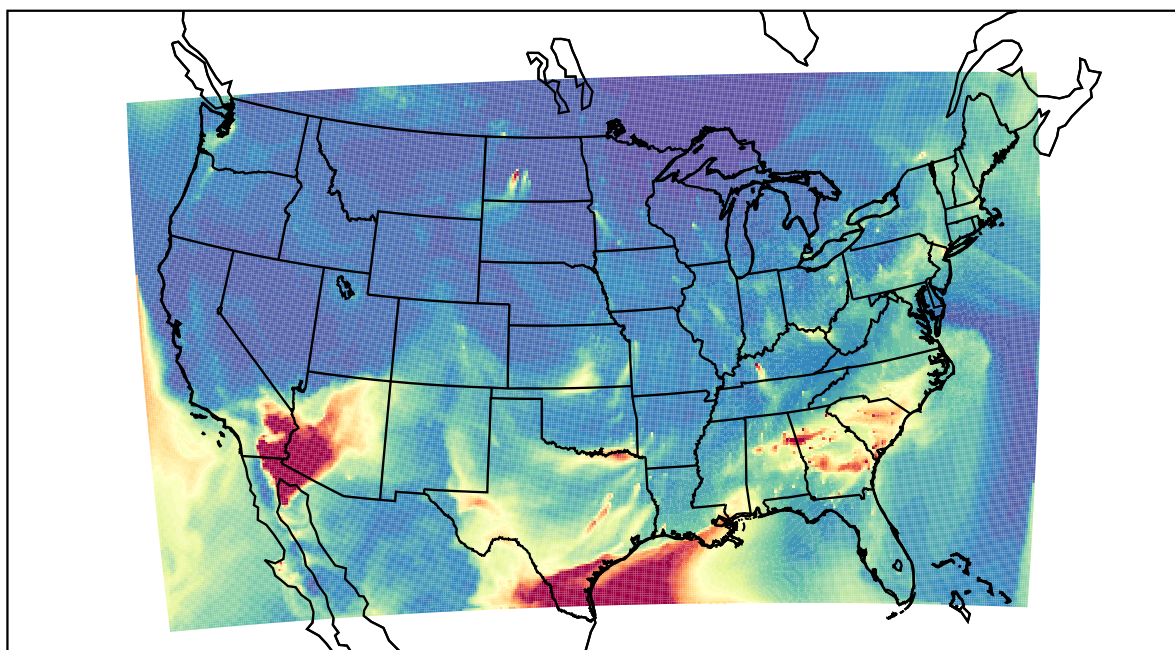
WRF 2021-04-15_09:00:00
