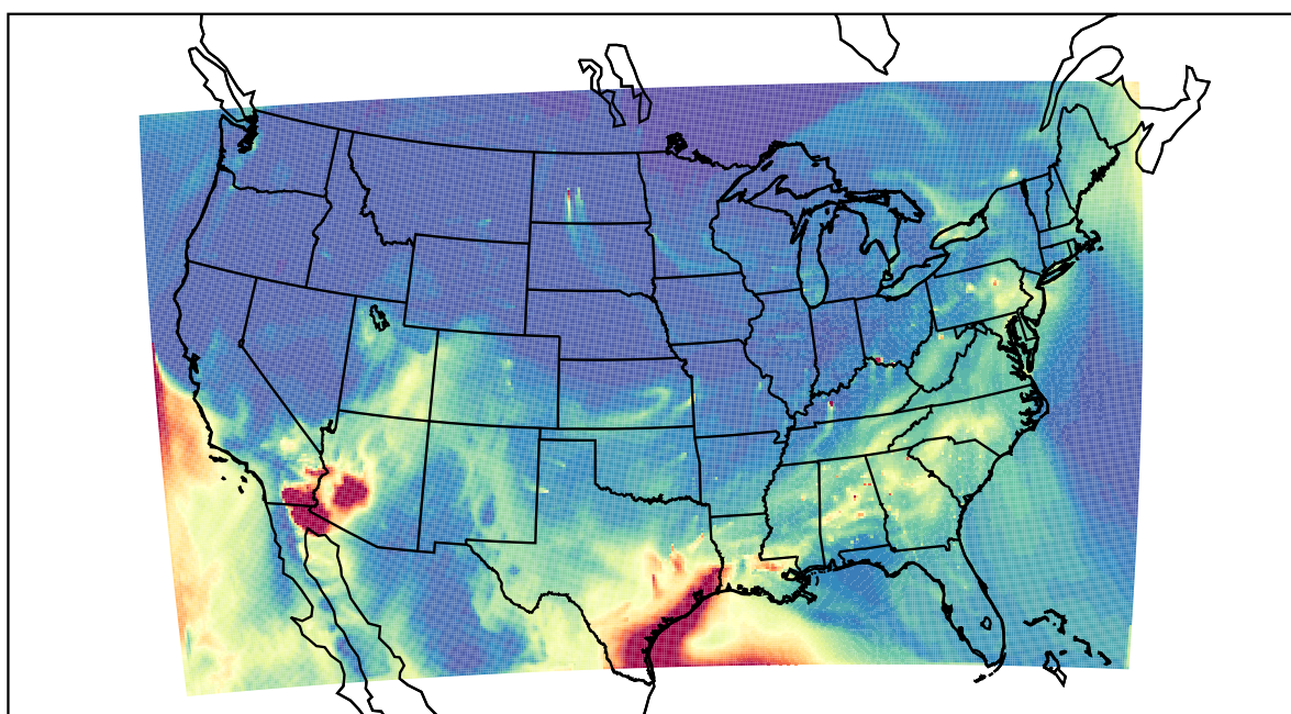
WRF 2021-04-14_16:00:00
