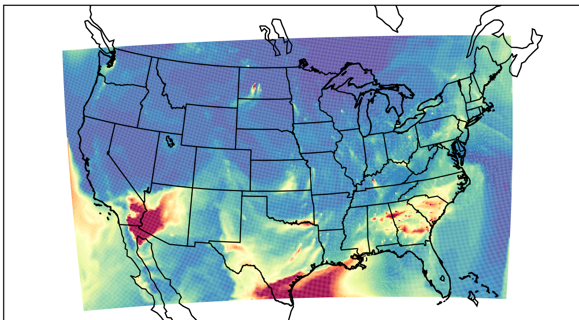
WRF 2021-04-15_08:00:00
