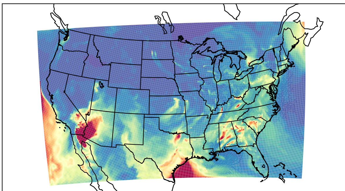
WRF 2021-04-14_08:00:00
