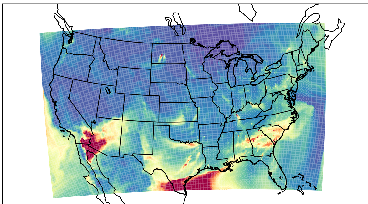
WRF 2021-04-15_11:00:00
