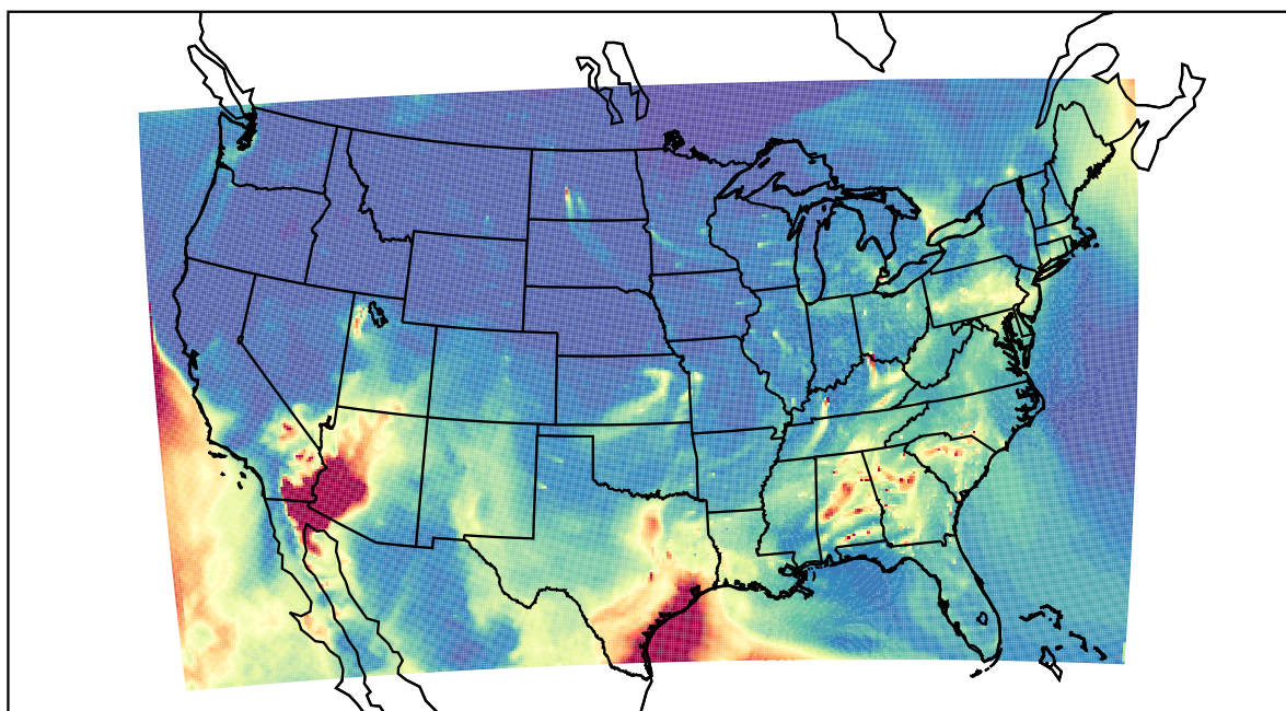
WRF 2021-04-14_11:00:00
