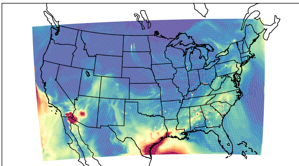
WRF 2021-04-14_18:00:00
