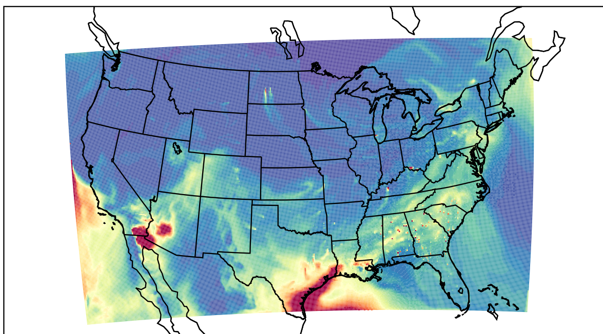
WRF 2021-04-14_17:00:00
