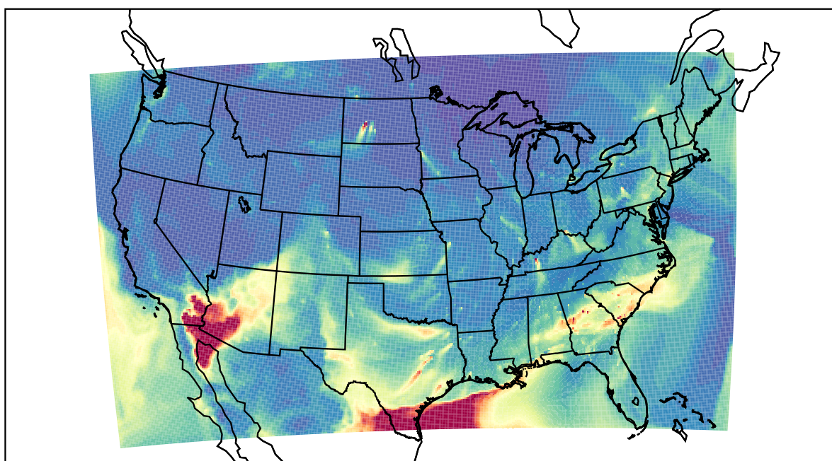
WRF 2021-04-15_13:00:00
