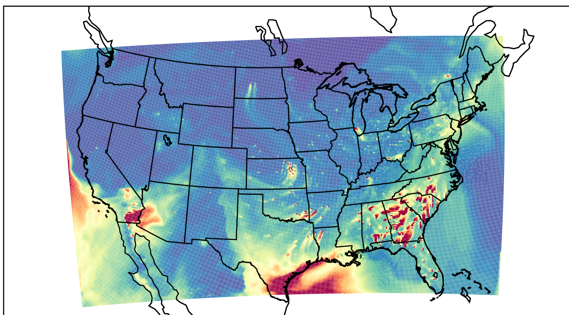
WRF 2021-04-15_00:00:00
