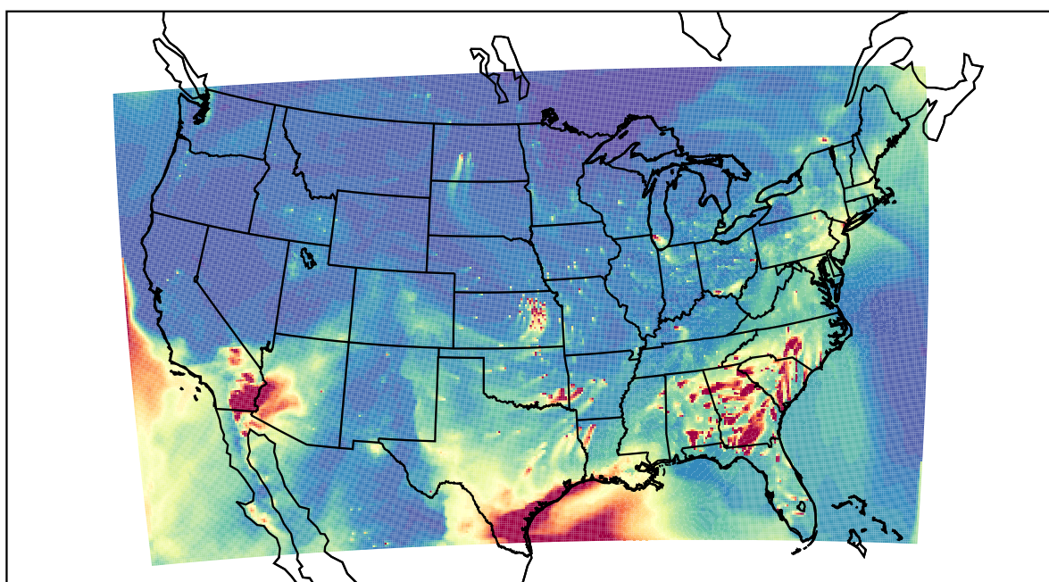
WRF 2021-04-15_01:00:00
