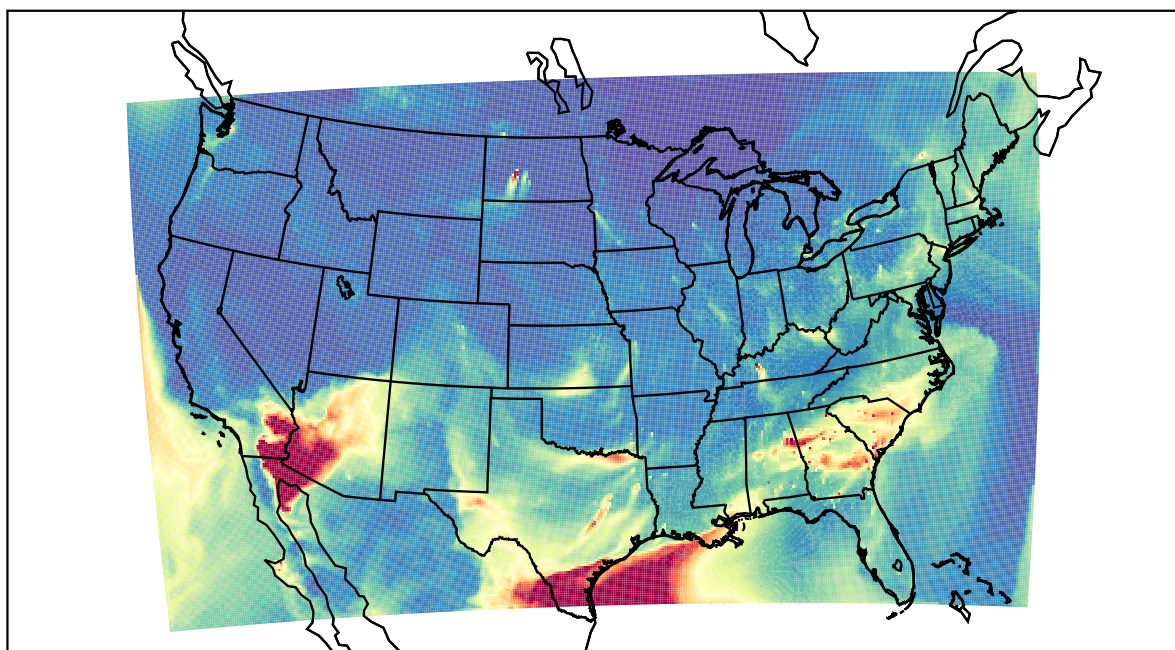
WRF 2021-04-15_10:00:00
