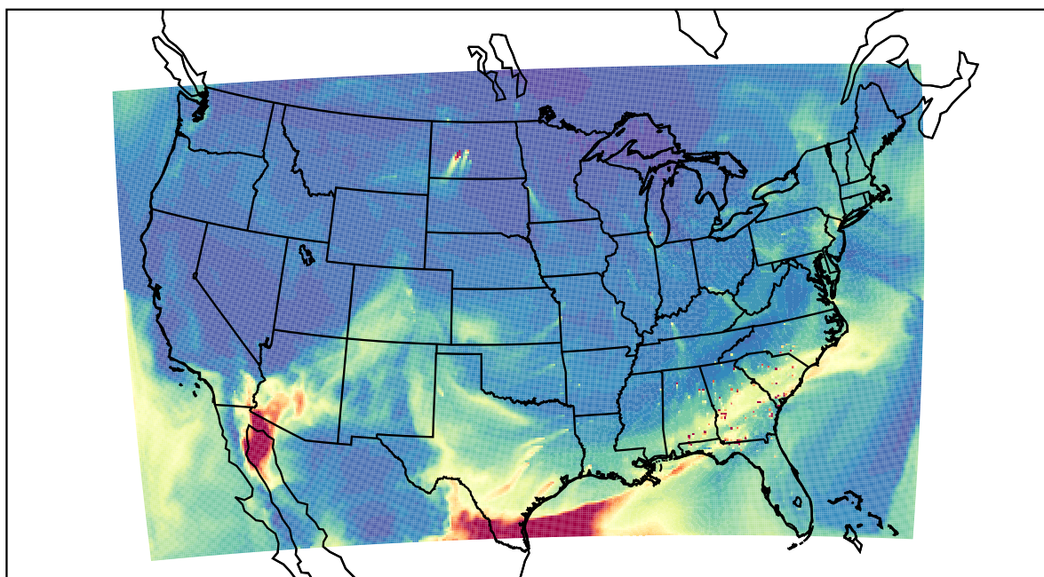
WRF 2021-04-15_17:00:00
