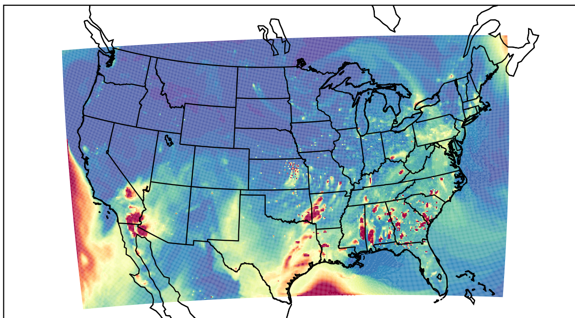
WRF 2021-04-14_01:00:00
