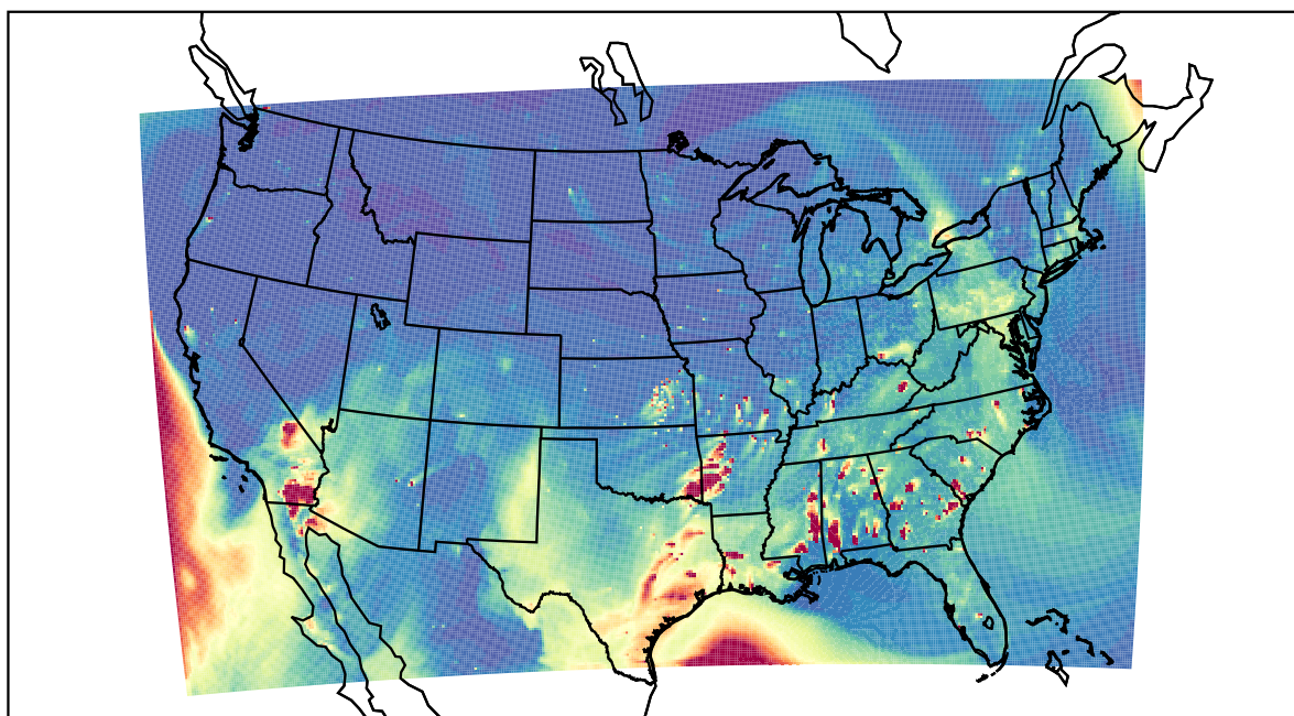
WRF 2021-04-14_00:00:00
