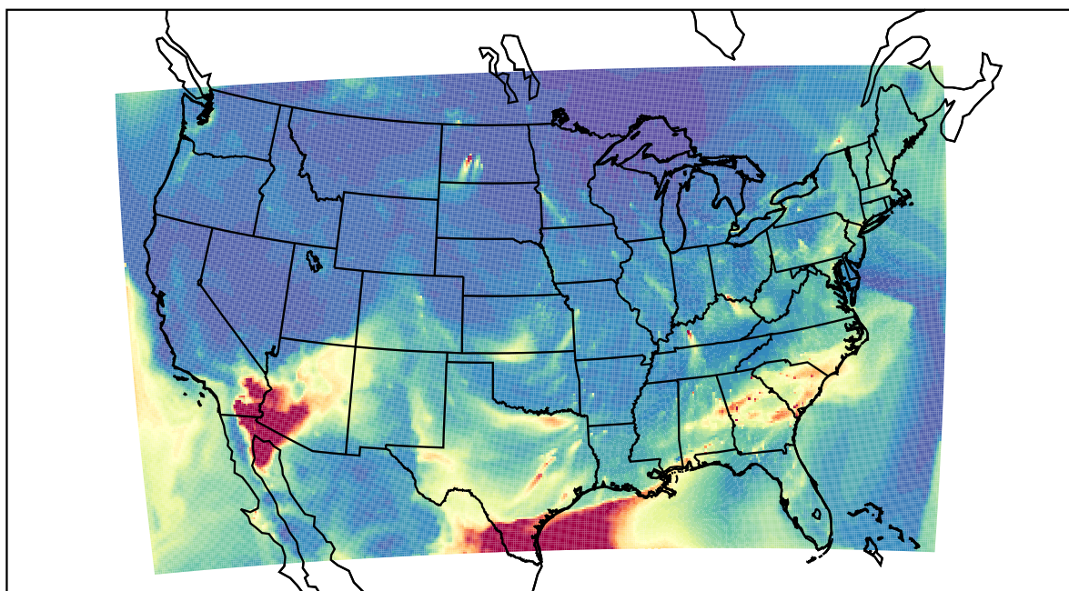
WRF 2021-04-15_12:00:00
