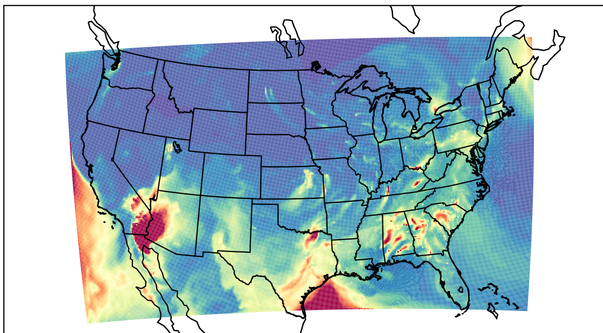
WRF 2021-04-14_07:00:00
