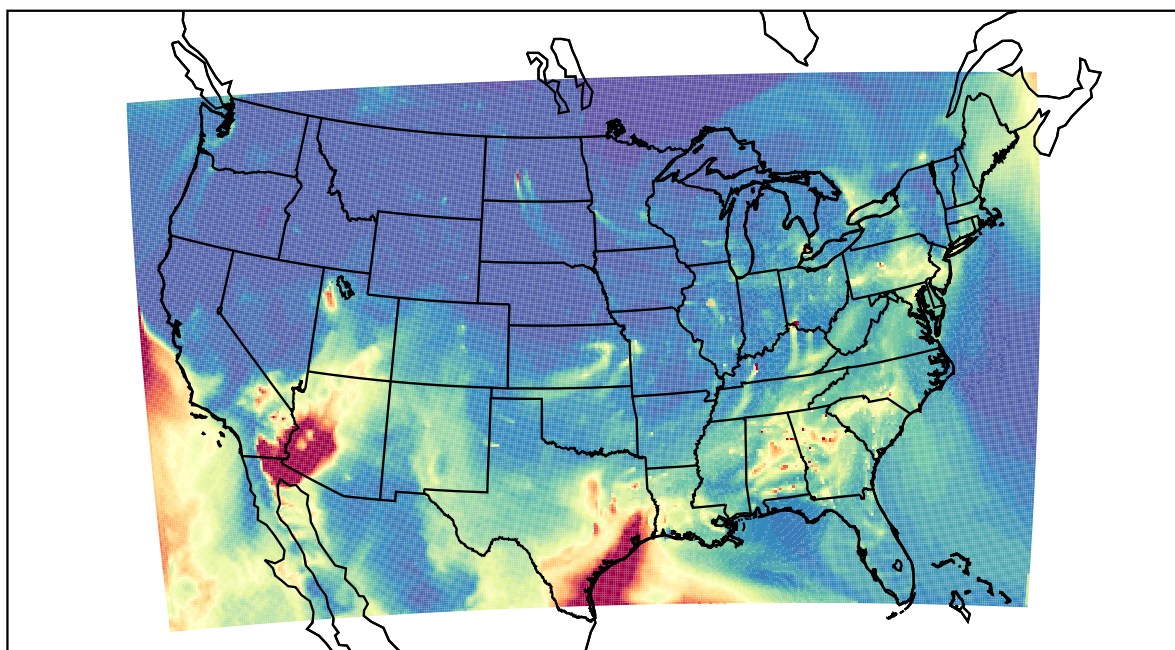
WRF 2021-04-14_13:00:00
