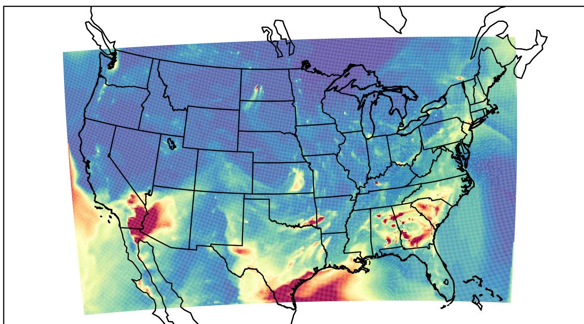
WRF 2021-04-15_04:00:00
