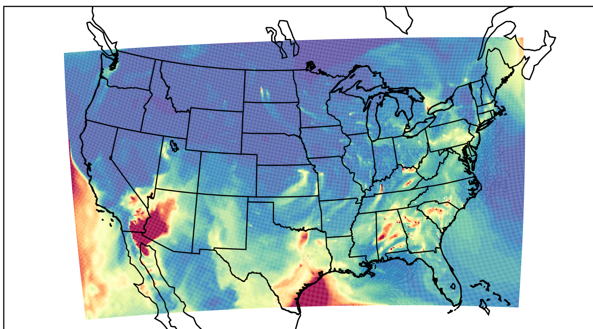
WRF 2021-04-14_09:00:00
