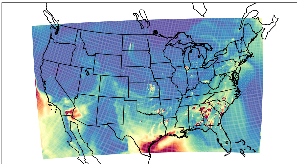
WRF 2021-04-14_22:00:00
