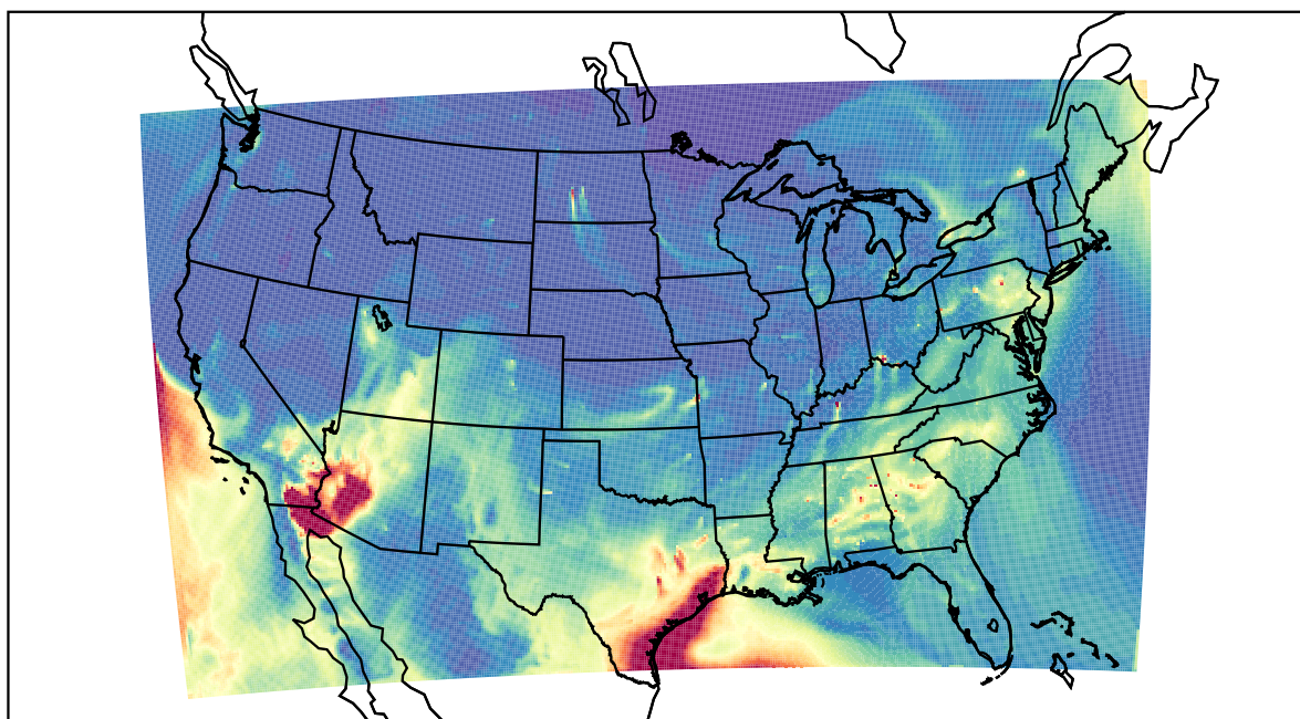
WRF 2021-04-14_15:00:00
