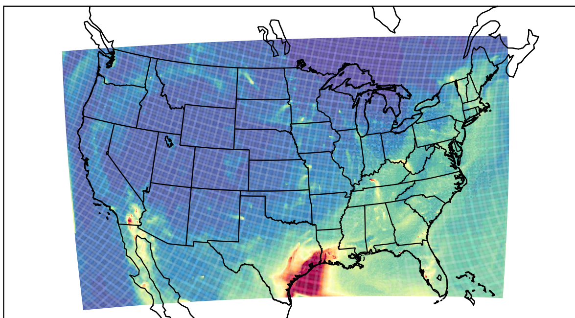
WRF 2021-04-30_11:00:00
