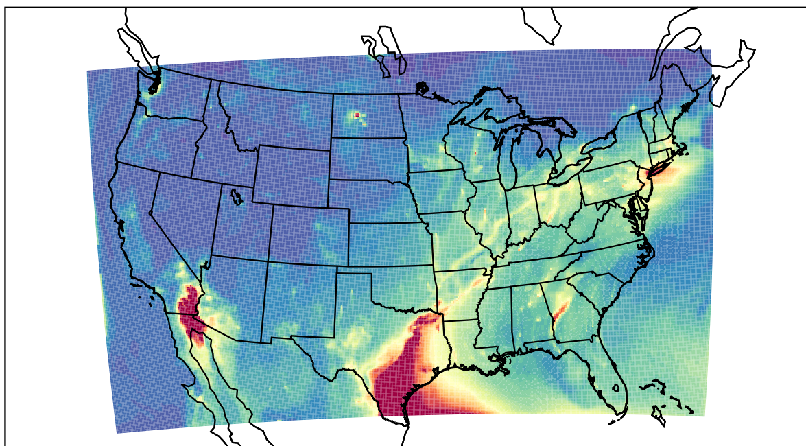
WRF 2021-04-29_13:00:00
