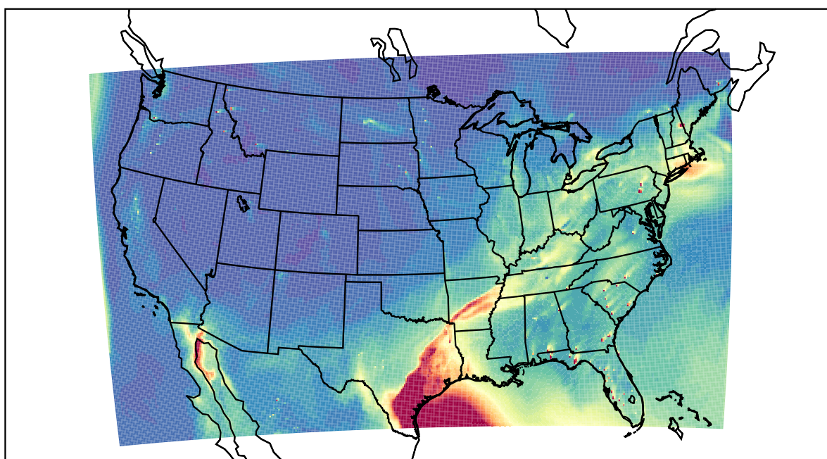
WRF 2021-04-29_21:00:00
