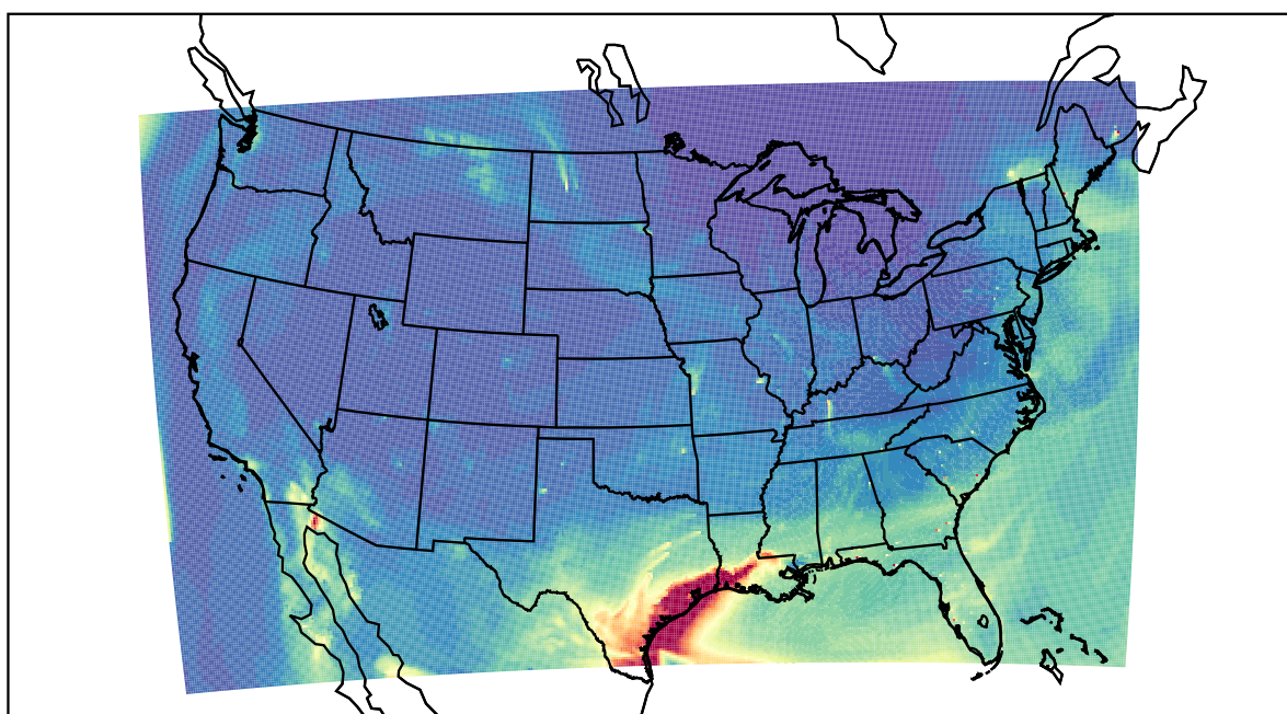
WRF 2021-04-30_17:00:00
