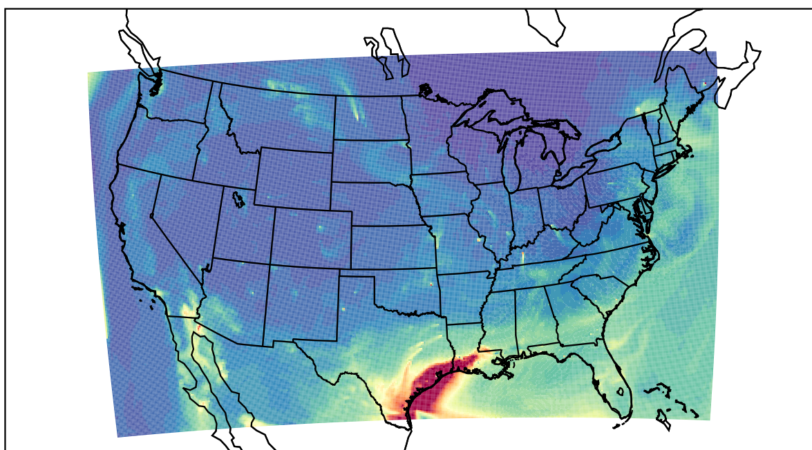
WRF 2021-04-30_16:00:00
