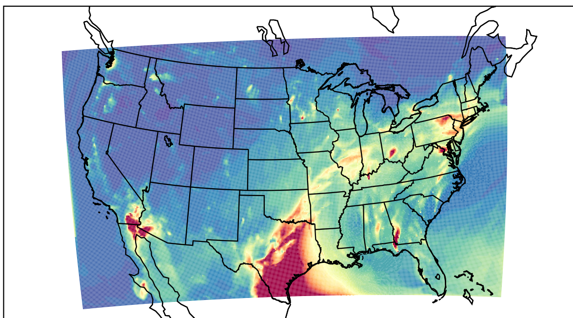
WRF 2021-04-29_06:00:00
