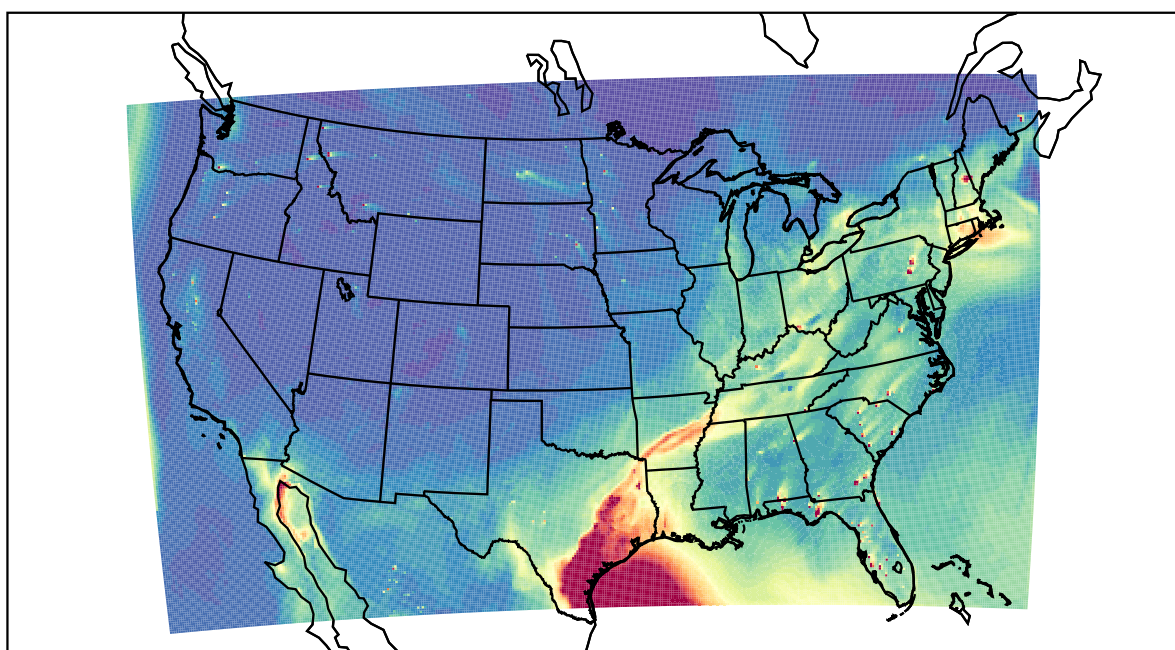
WRF 2021-04-29_22:00:00
