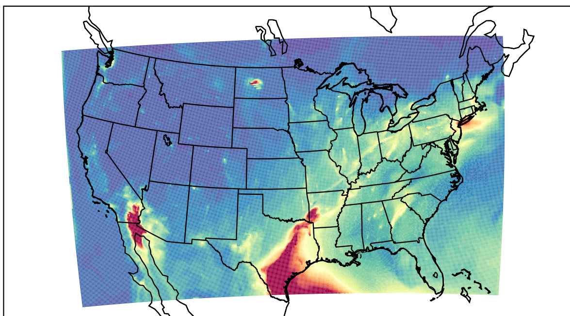
WRF 2021-04-29_15:00:00
