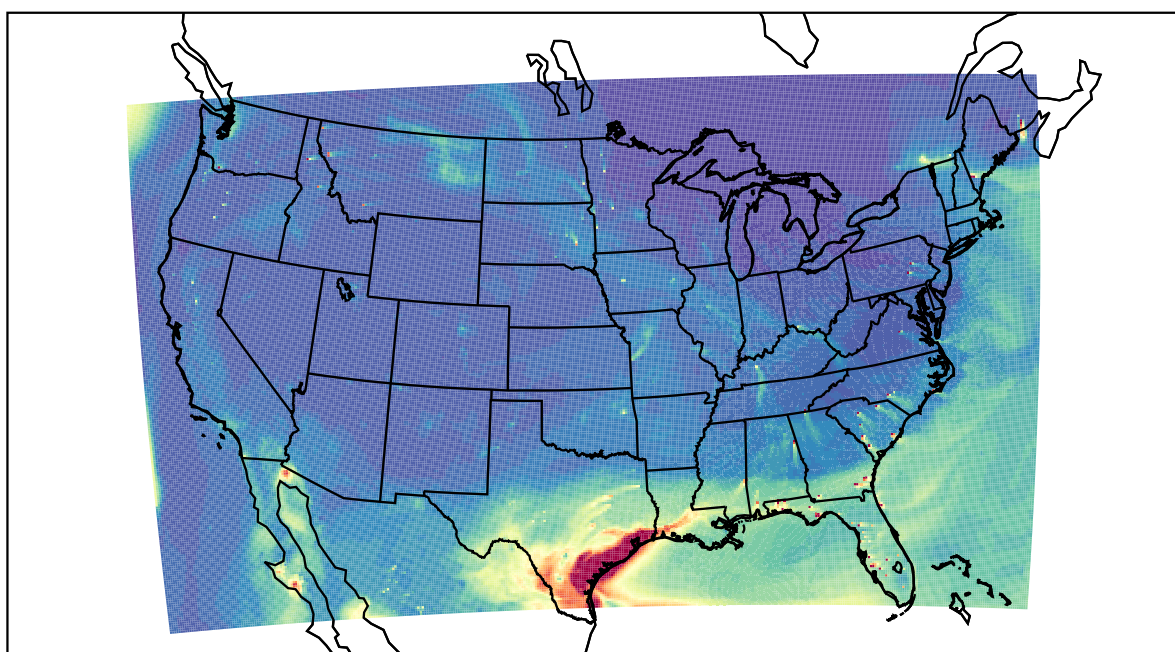
WRF 2021-04-30_21:00:00
