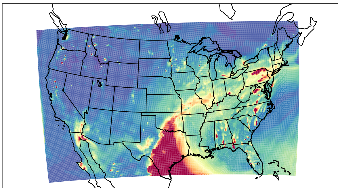
WRF 2021-04-29_02:00:00
