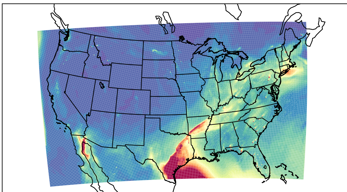
WRF 2021-04-29_20:00:00
