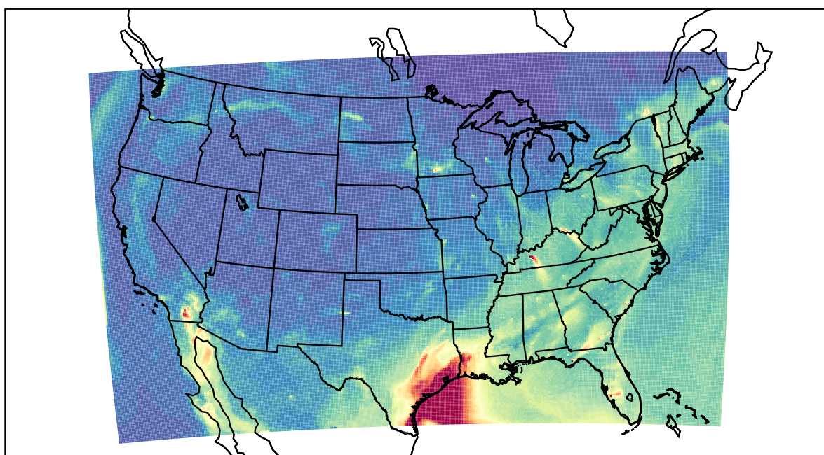
WRF 2021-04-30_08:00:00
