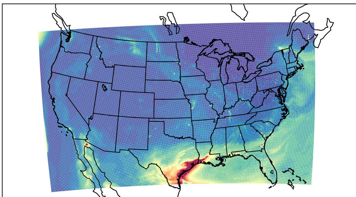
WRF 2021-04-30_19:00:00
