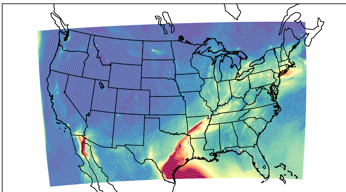
WRF 2021-04-29_19:00:00
