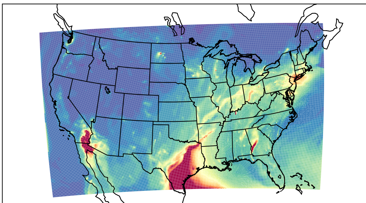
WRF 2021-04-29_11:00:00
