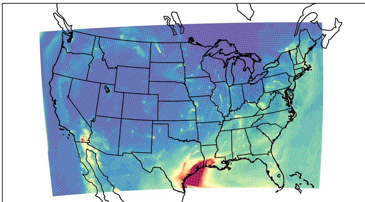
WRF 2021-04-30_13:00:00
