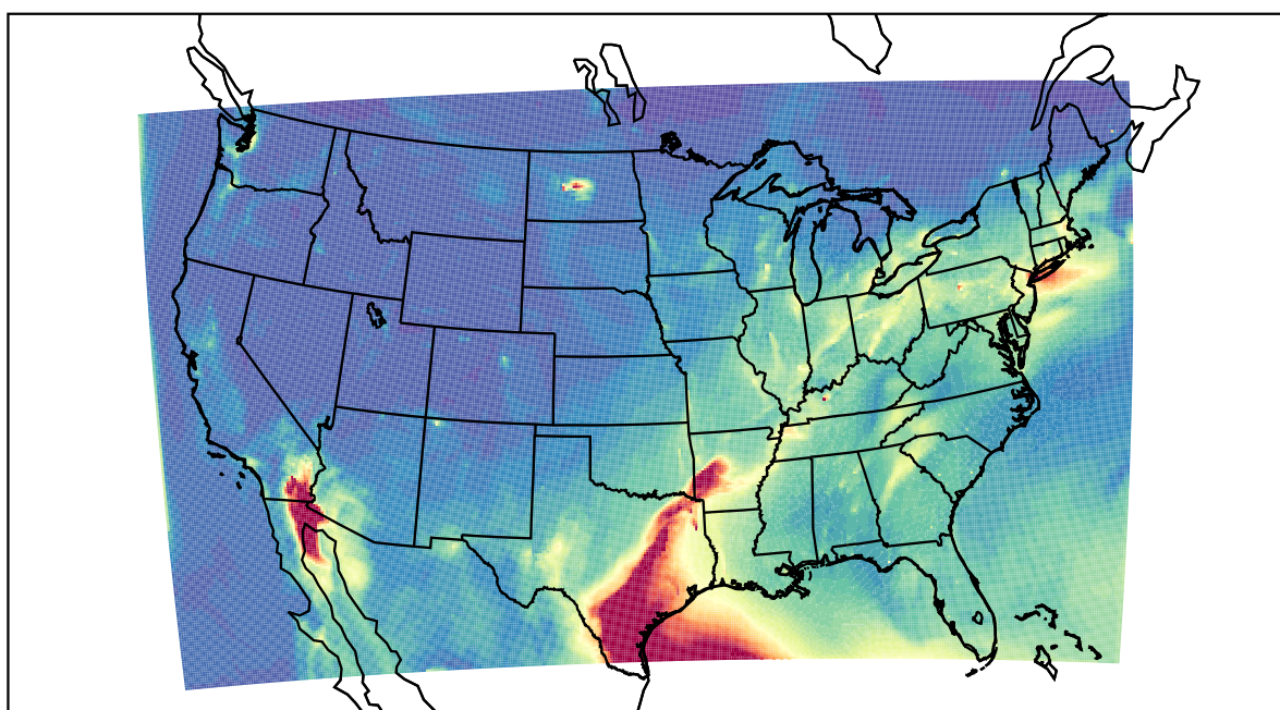
WRF 2021-04-29_16:00:00
