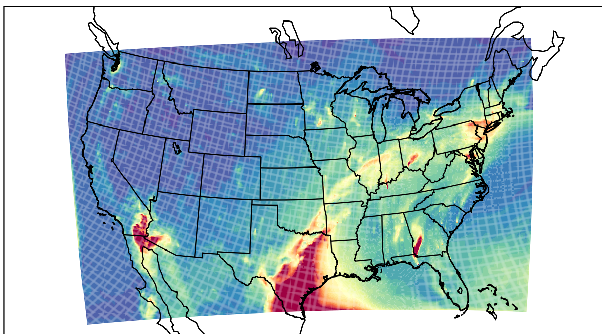
WRF 2021-04-29_08:00:00
