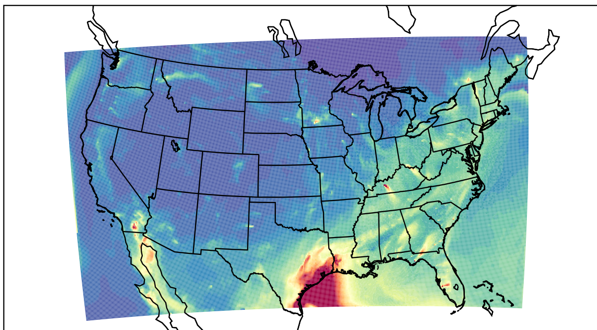
WRF 2021-04-30_07:00:00
