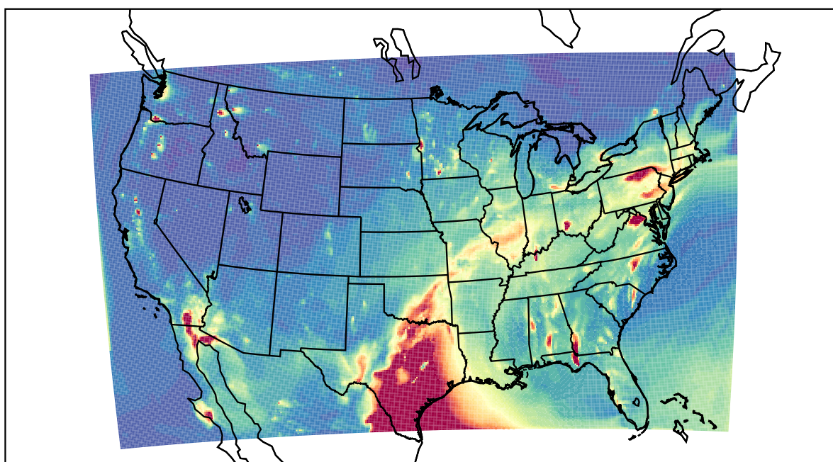
WRF 2021-04-29_04:00:00
