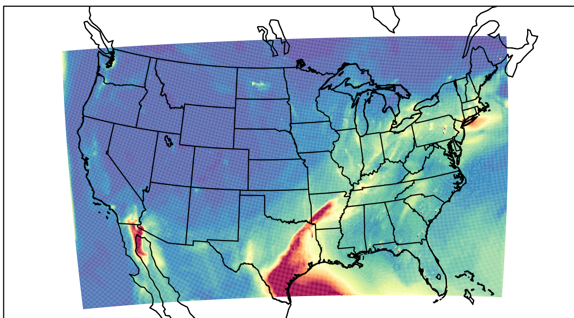
WRF 2021-04-29_18:00:00
