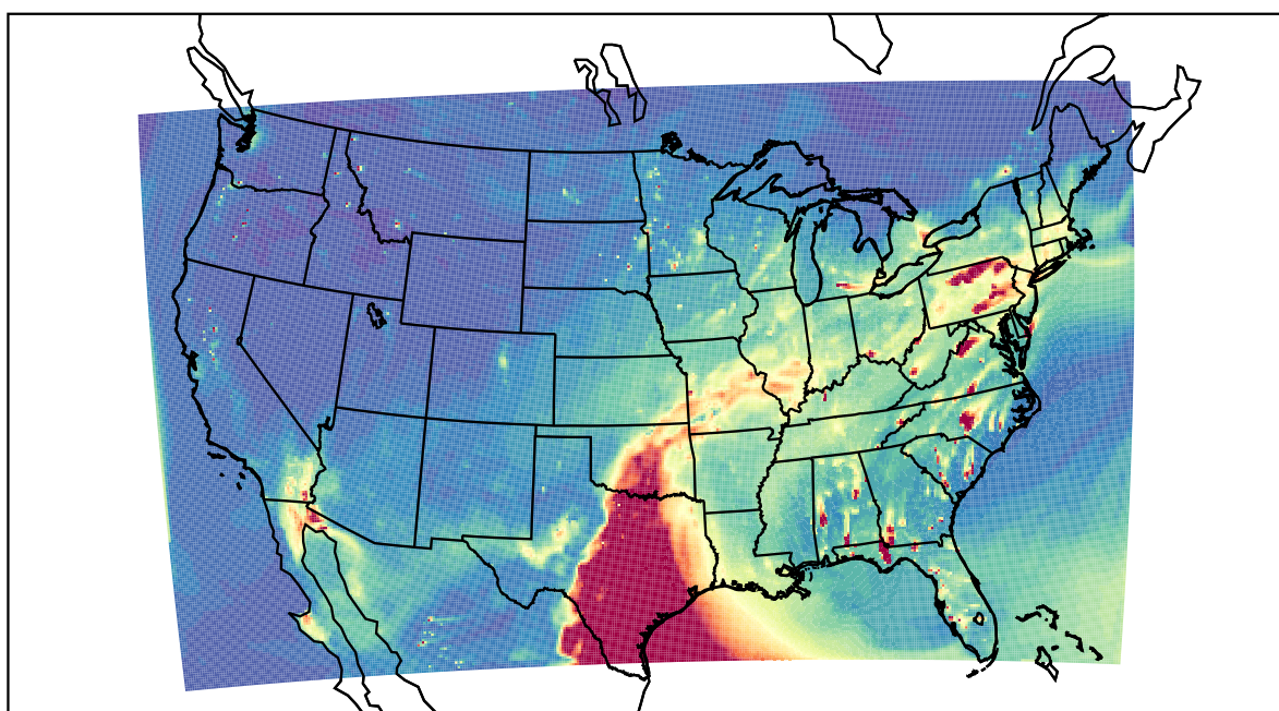
WRF 2021-04-29_01:00:00
