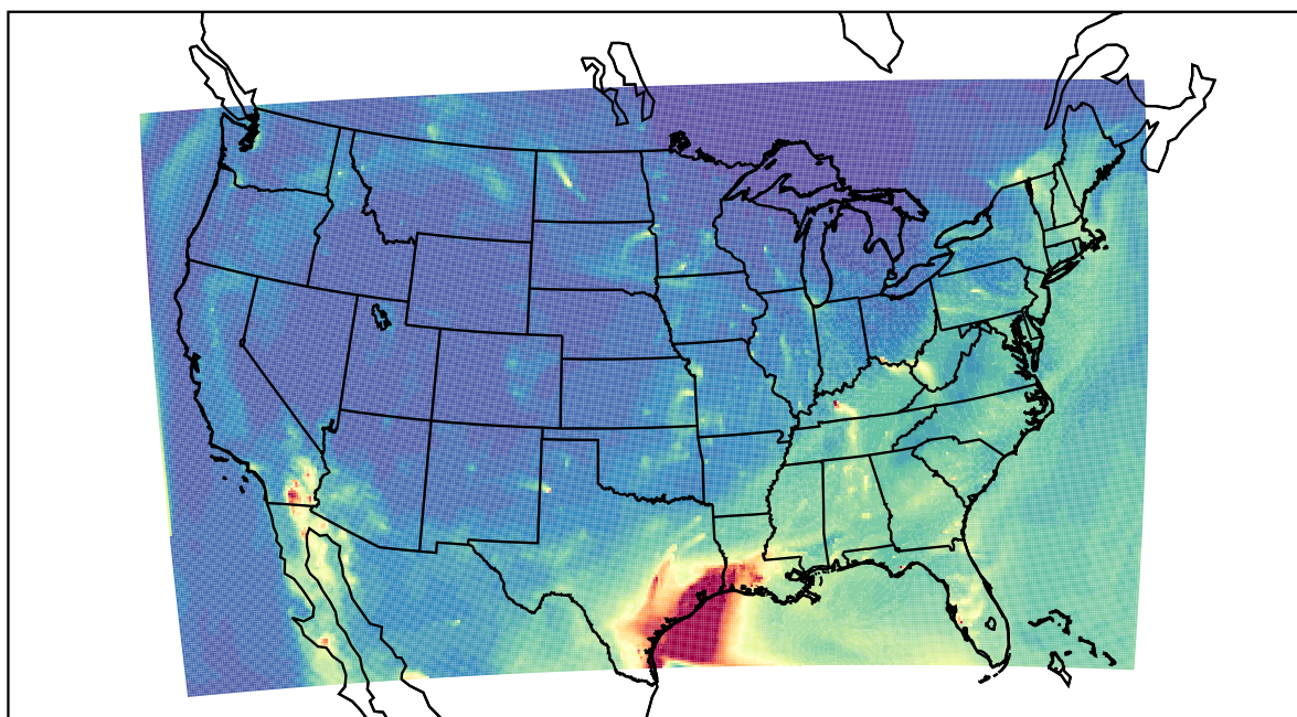
WRF 2021-04-30_12:00:00
