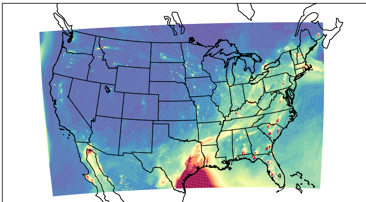
WRF 2021-04-30_01:00:00
