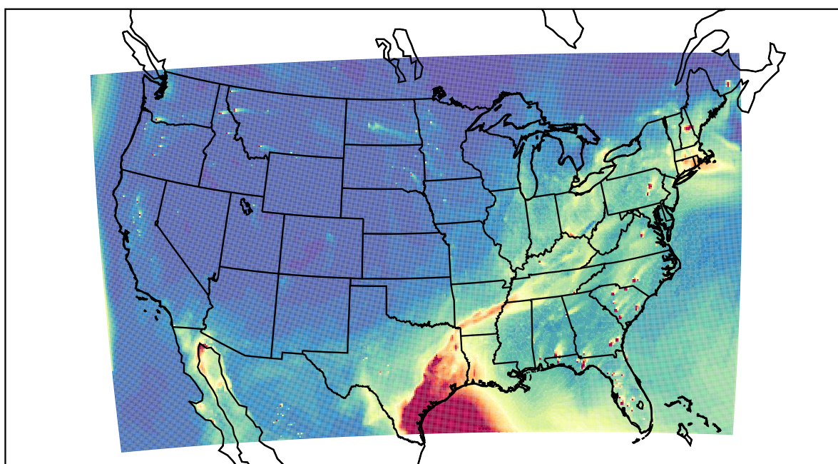
WRF 2021-04-29_23:00:00
