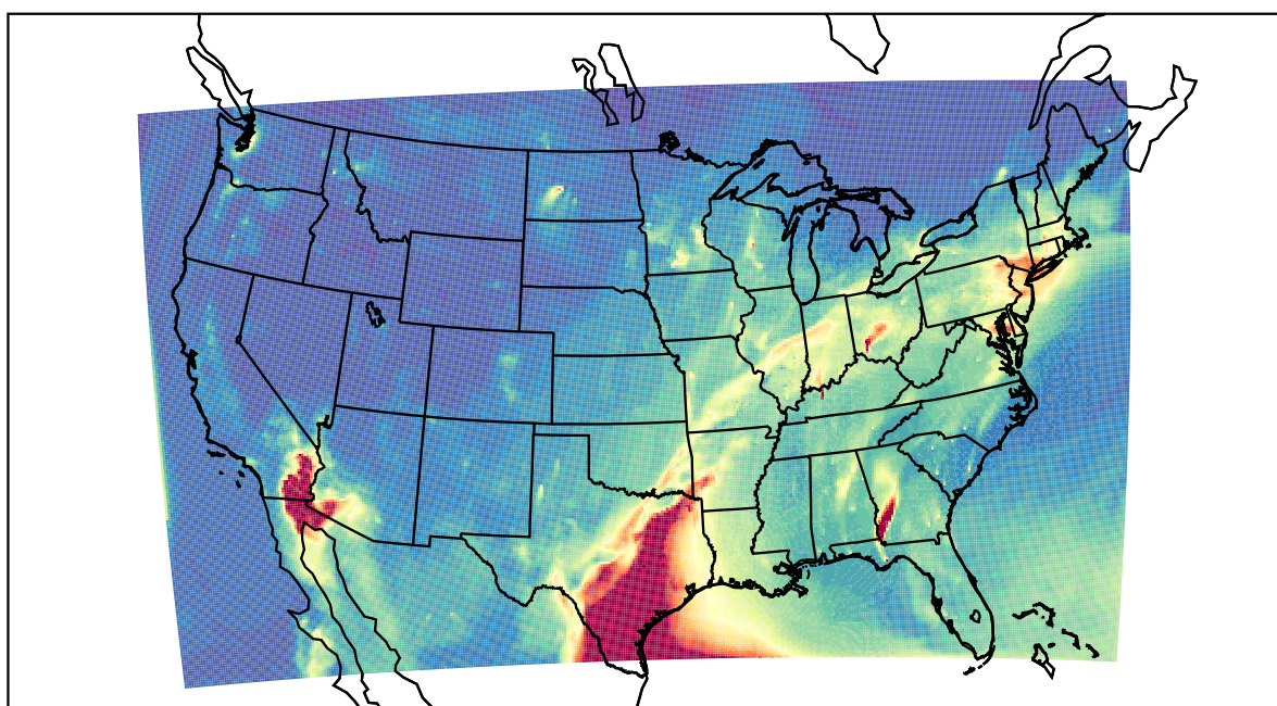
WRF 2021-04-29_09:00:00
