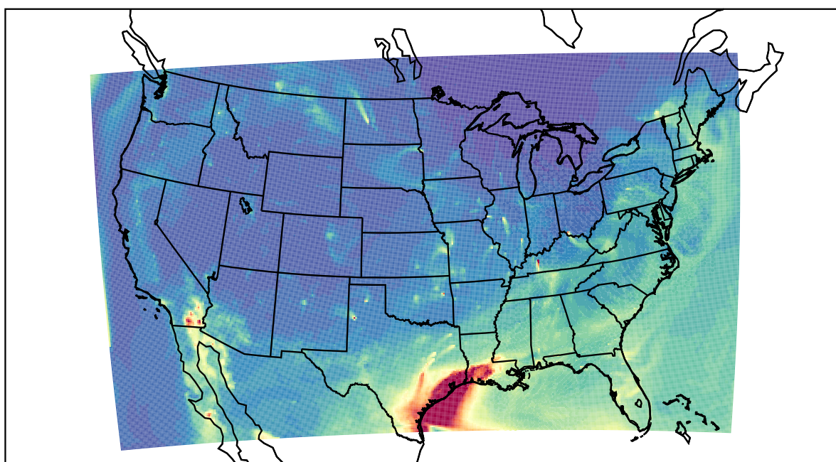
WRF 2021-04-30_14:00:00
