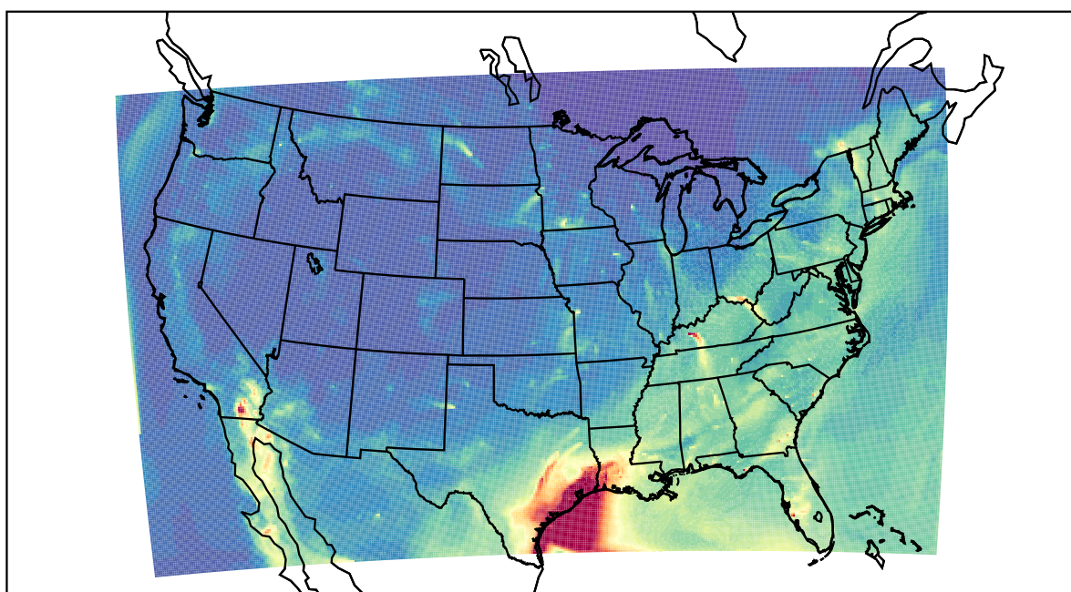
WRF 2021-04-30_10:00:00
