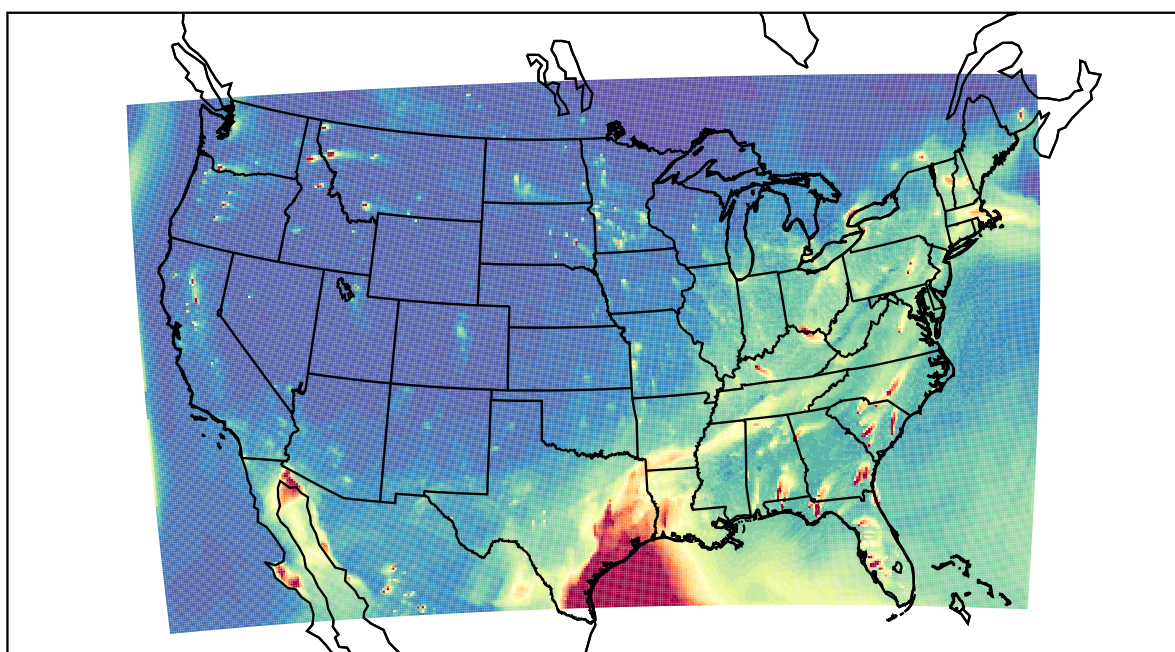
WRF 2021-04-30_02:00:00
