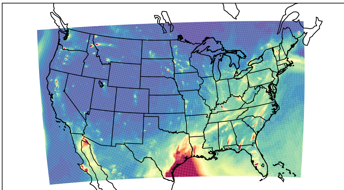
WRF 2021-04-30_03:00:00
