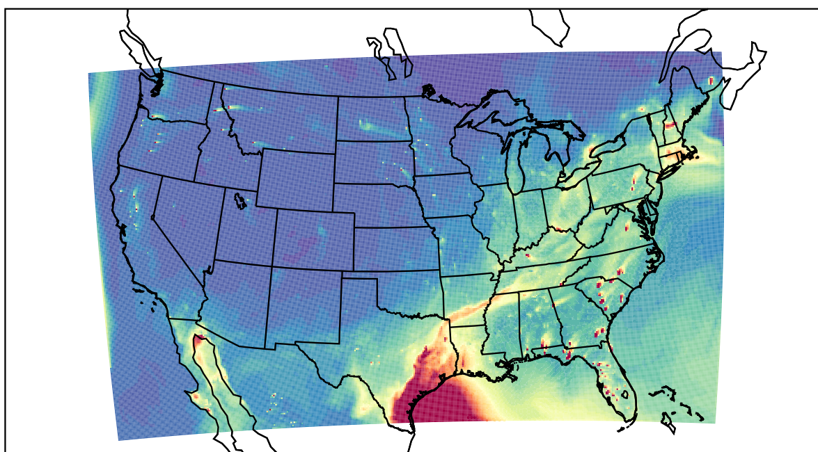
WRF 2021-04-30_00:00:00
