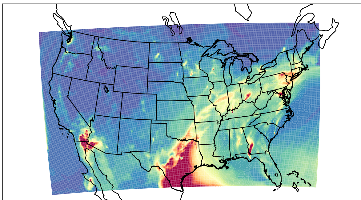
WRF 2021-04-29_07:00:00
