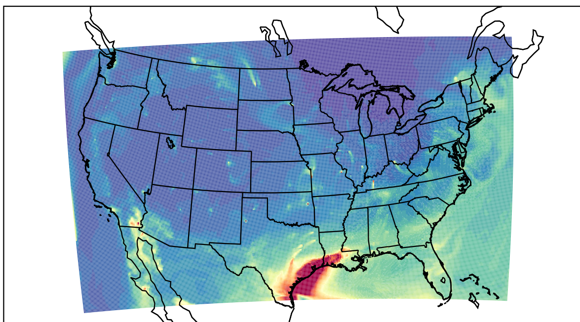
WRF 2021-04-30_15:00:00
