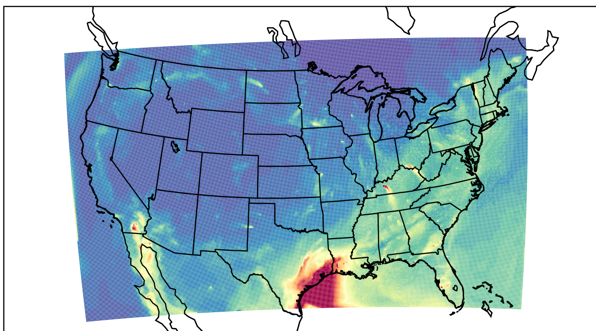
WRF 2021-04-30_09:00:00
