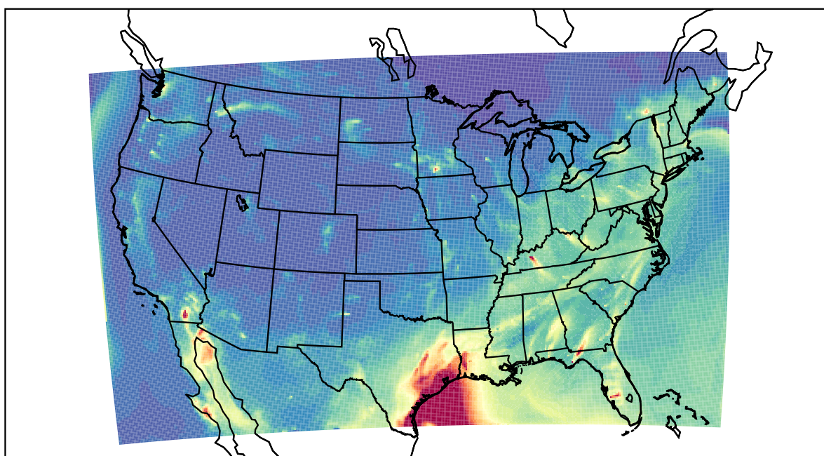
WRF 2021-04-30_06:00:00
