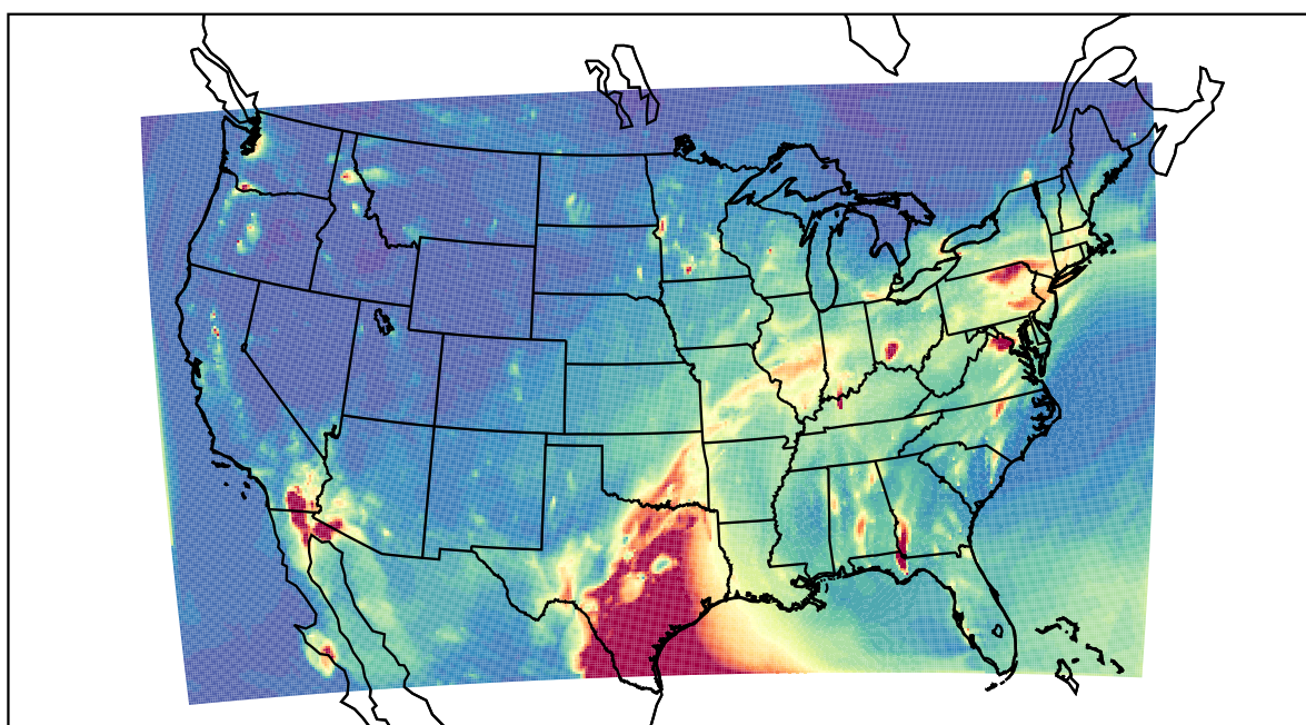
WRF 2021-04-29_05:00:00
