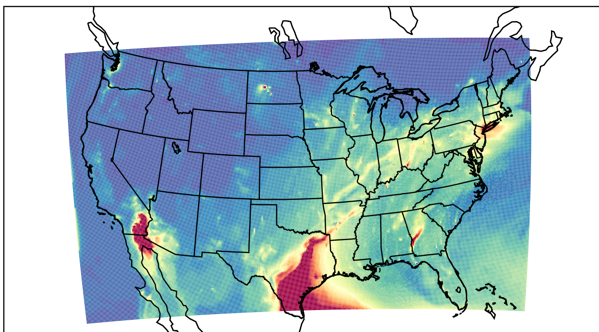
WRF 2021-04-29_12:00:00
