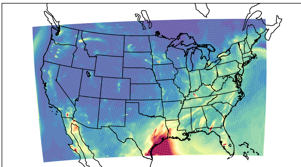
WRF 2021-04-30_05:00:00
