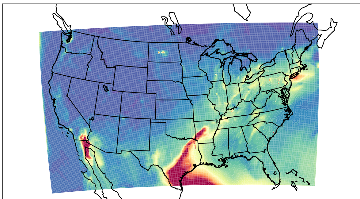
WRF 2021-04-29_17:00:00
