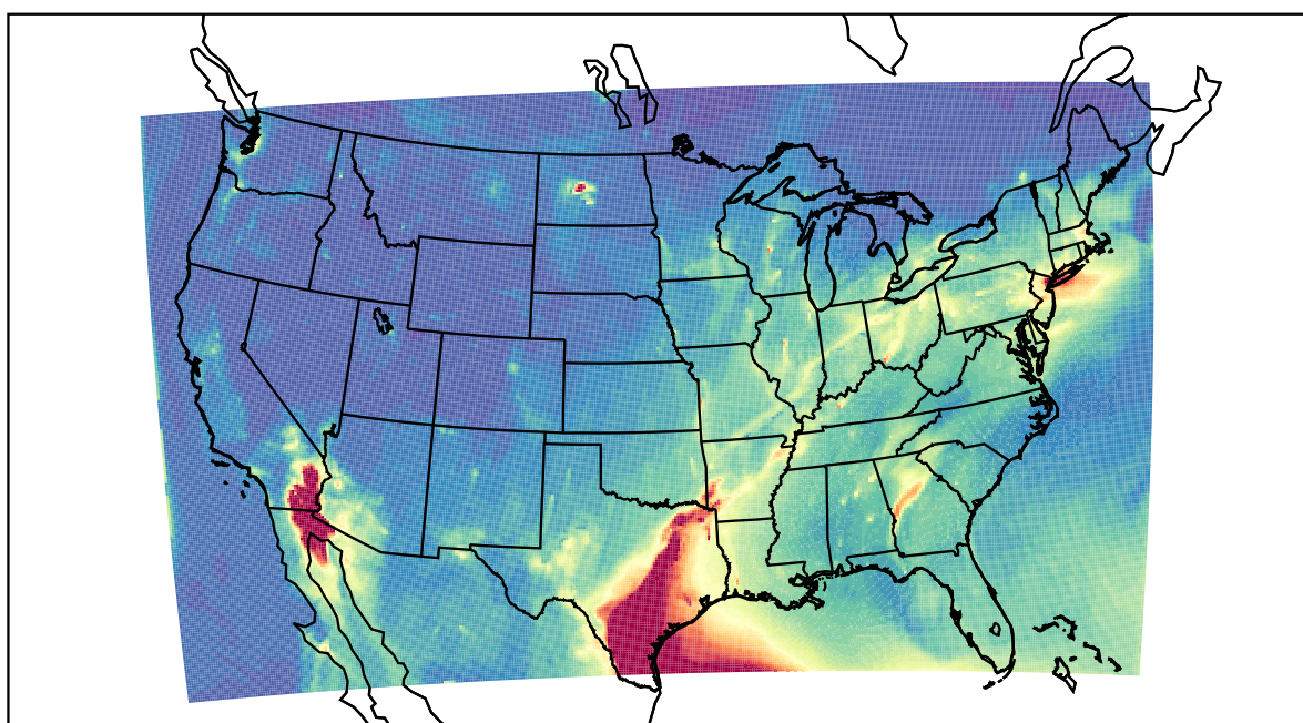
WRF 2021-04-29_14:00:00
