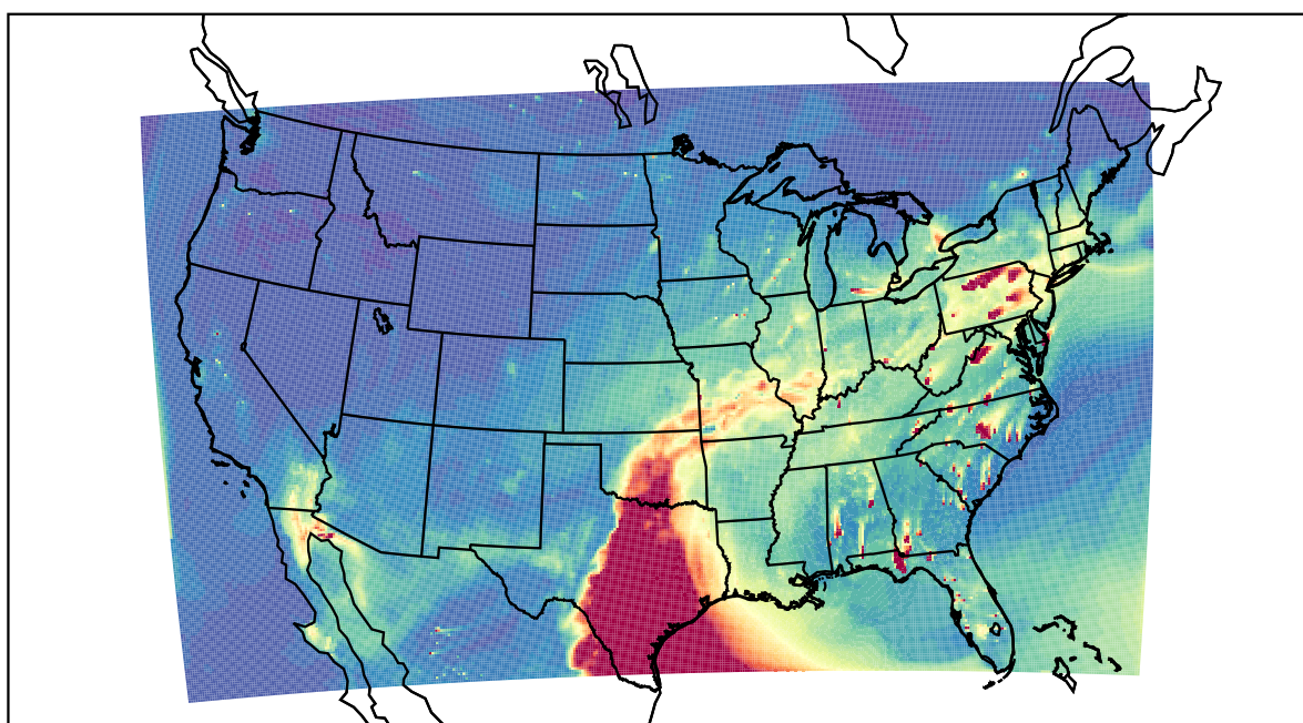
WRF 2021-04-29_00:00:00
