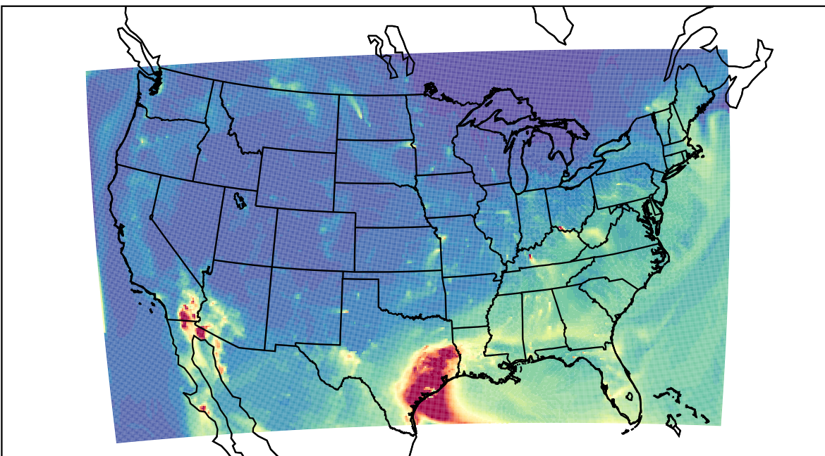
WRF 2021-04-30_13:00:00
