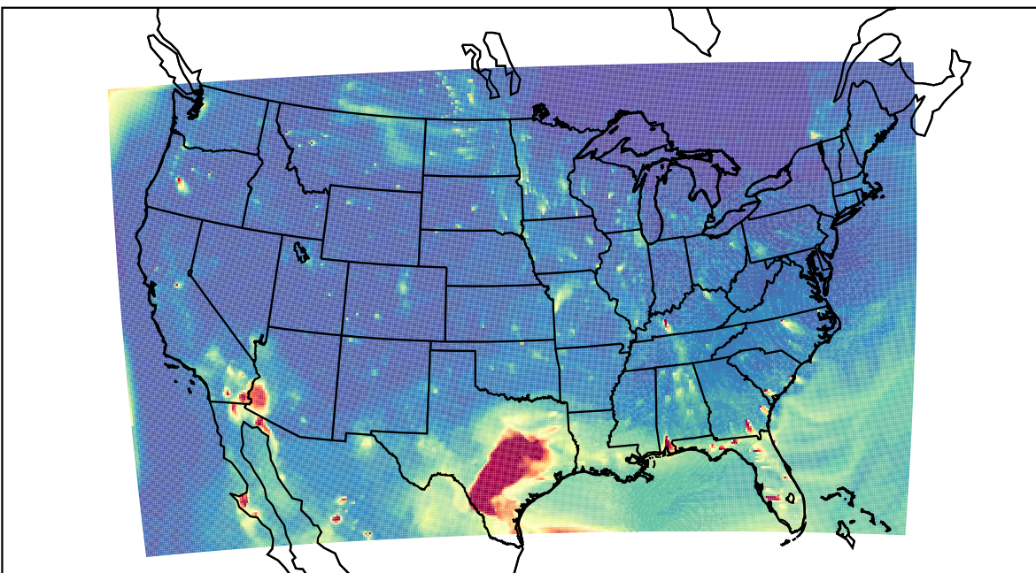
WRF 2021-05-01_02:00:00
