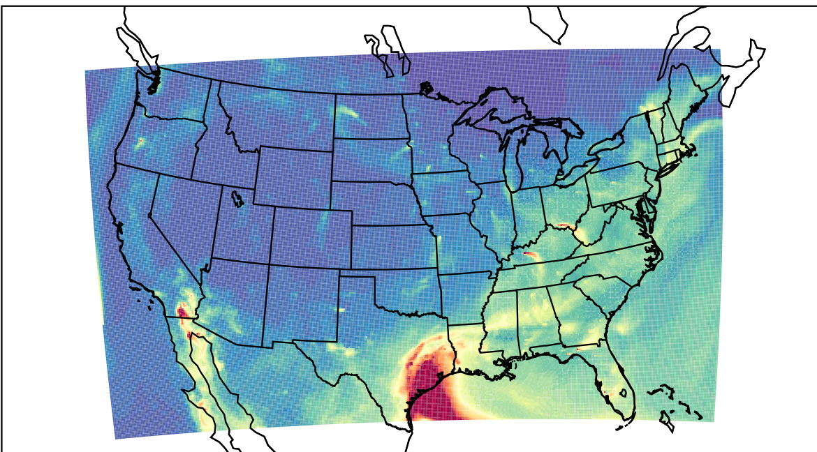
WRF 2021-04-30_09:00:00
