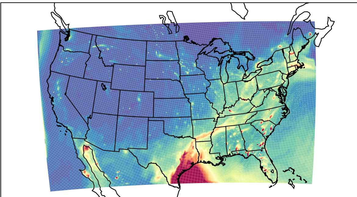
WRF 2021-04-30_01:00:00
