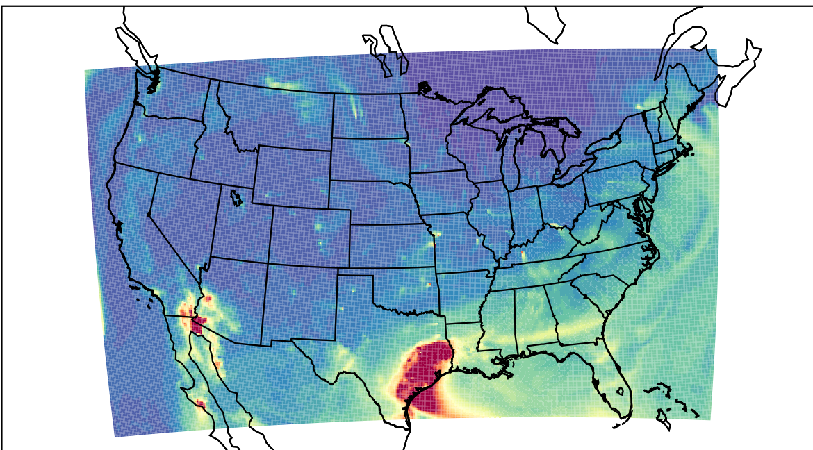
WRF 2021-04-30_15:00:00
