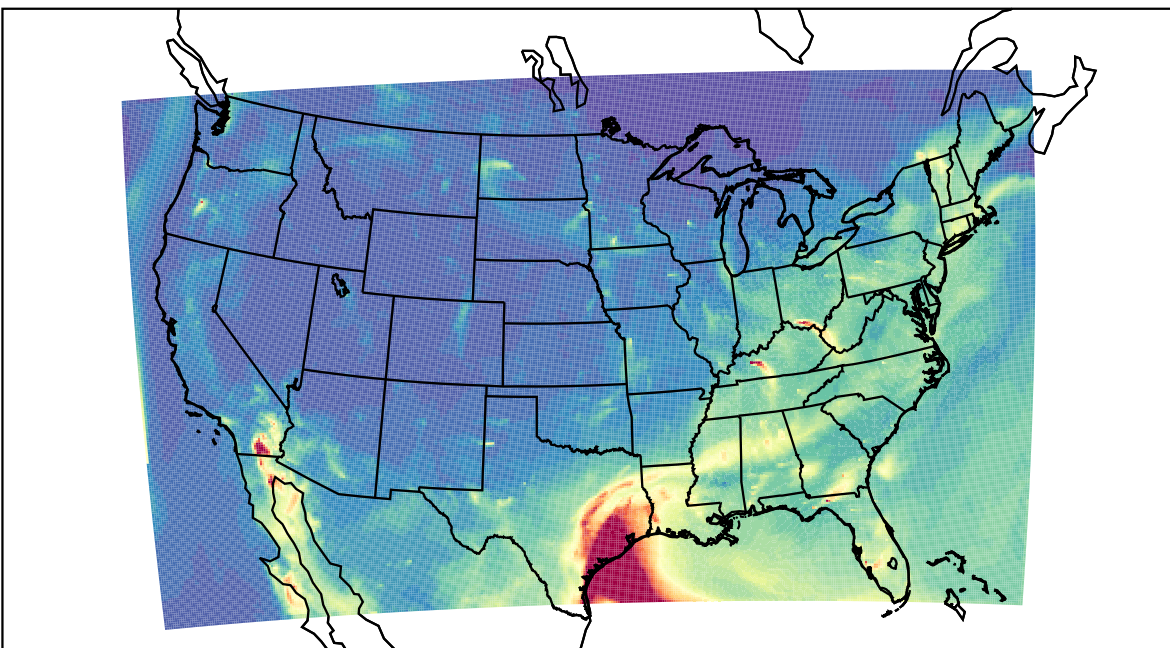
WRF 2021-04-30_08:00:00
