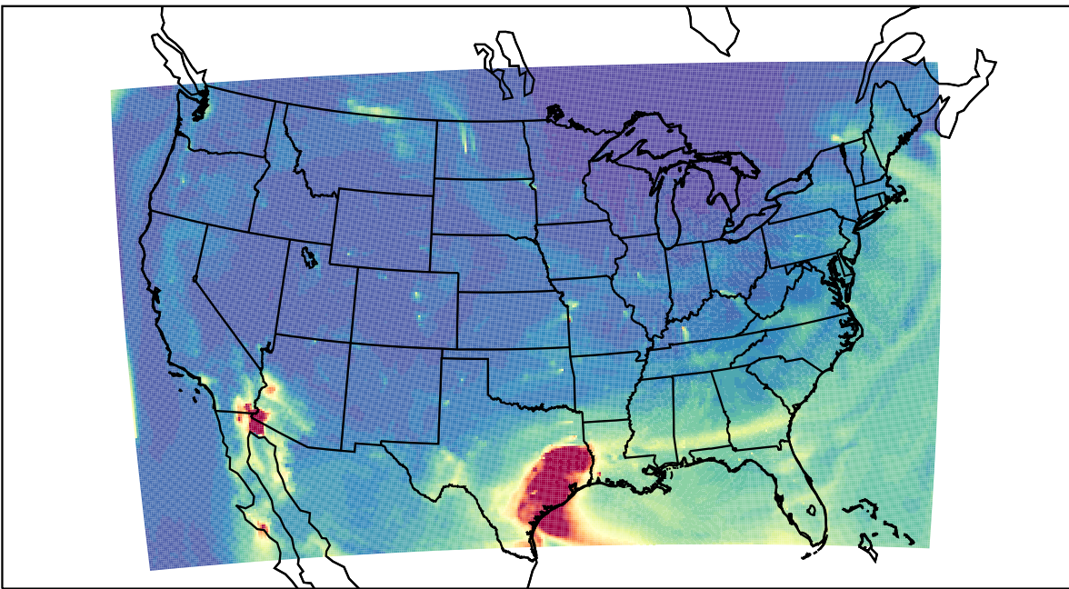
WRF 2021-04-30_16:00:00
