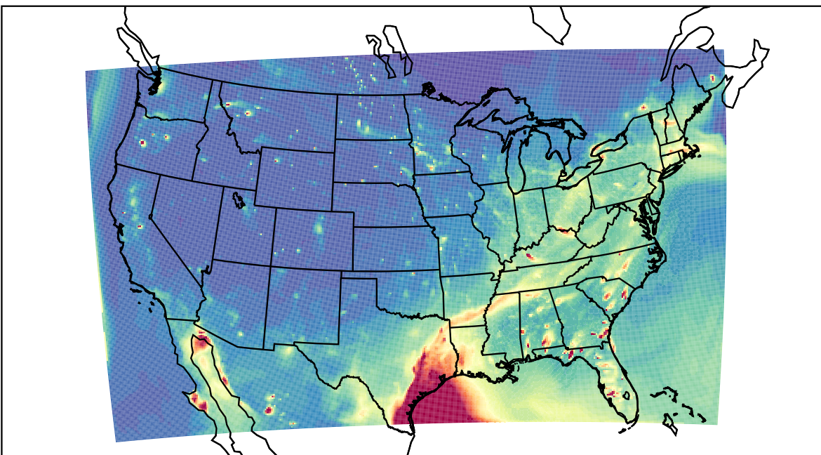
WRF 2021-04-30_02:00:00
