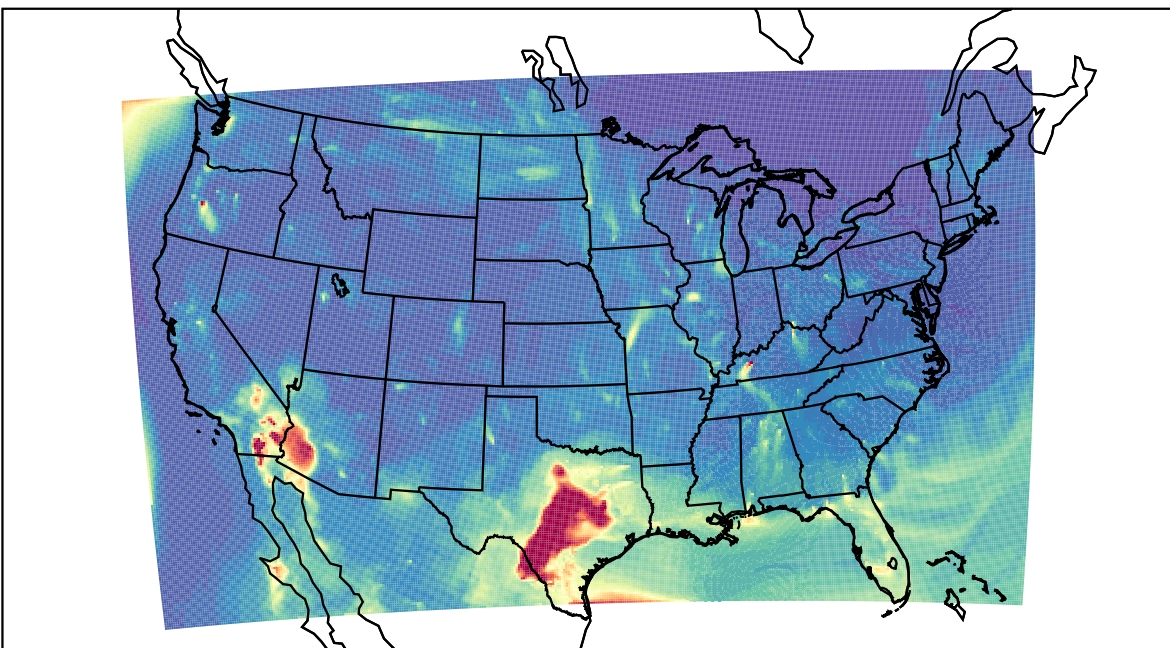
WRF 2021-05-01_05:00:00
