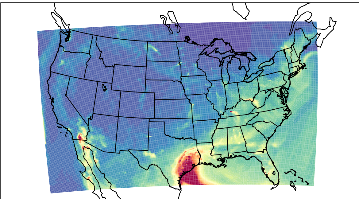
WRF 2021-04-30_10:00:00
