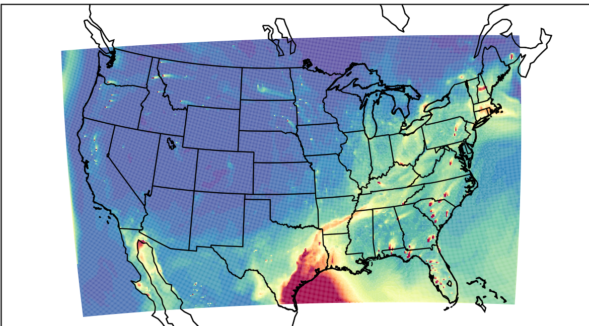
WRF 2021-04-30_00:00:00
