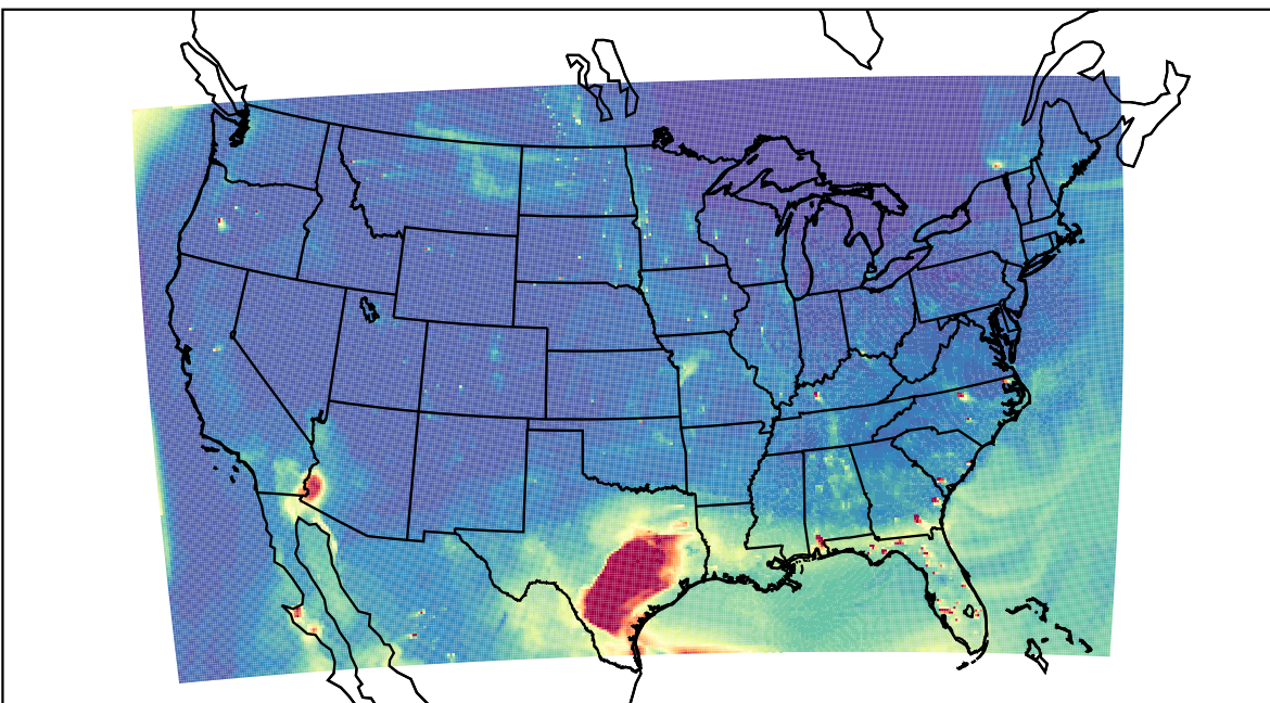
WRF 2021-05-01_00:00:00
