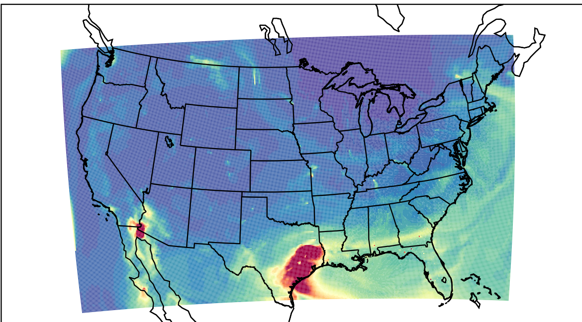
WRF 2021-04-30_17:00:00
