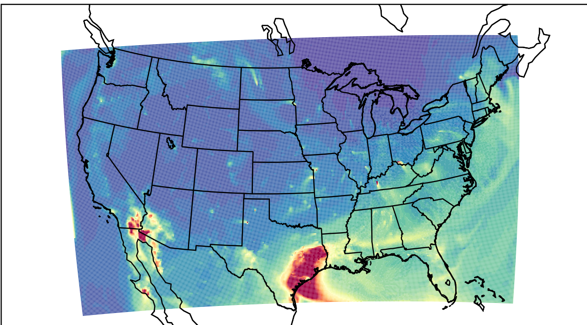
WRF 2021-04-30_14:00:00
