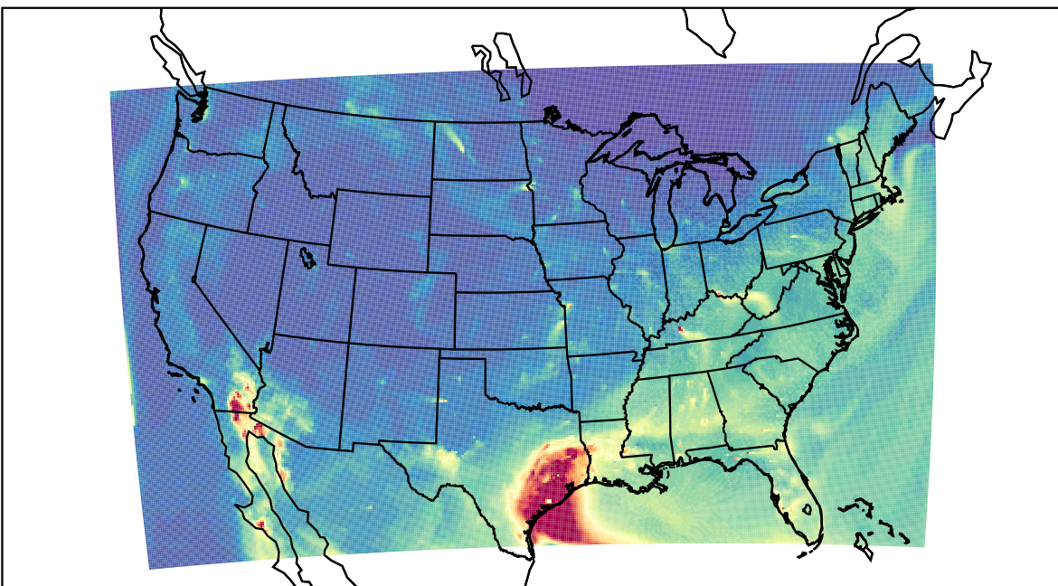
WRF 2021-04-30_12:00:00
