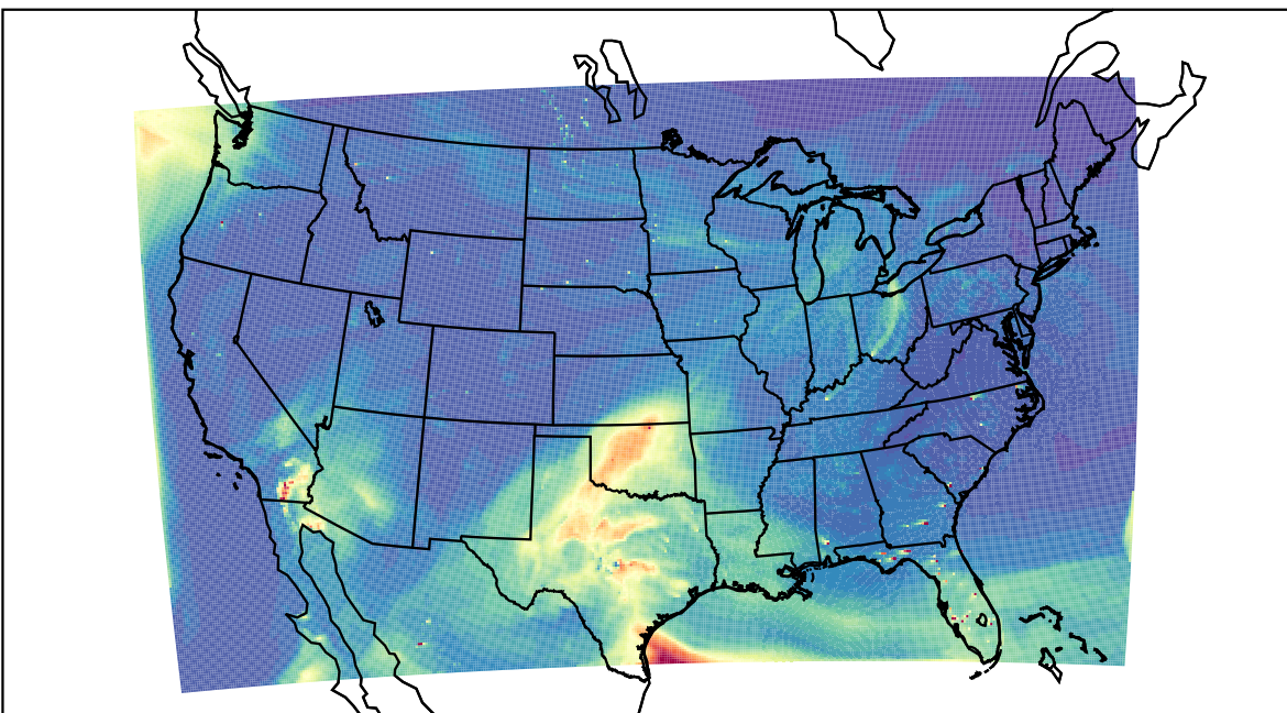
WRF 2021-05-01_21:00:00
