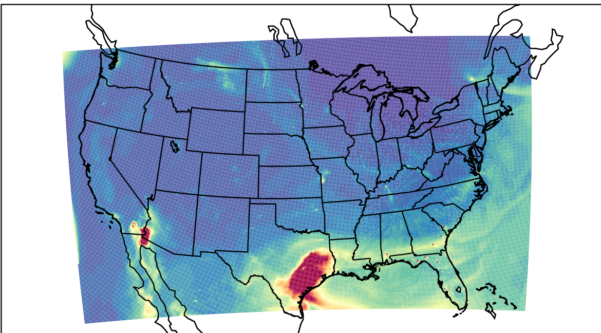
WRF 2021-04-30_19:00:00
