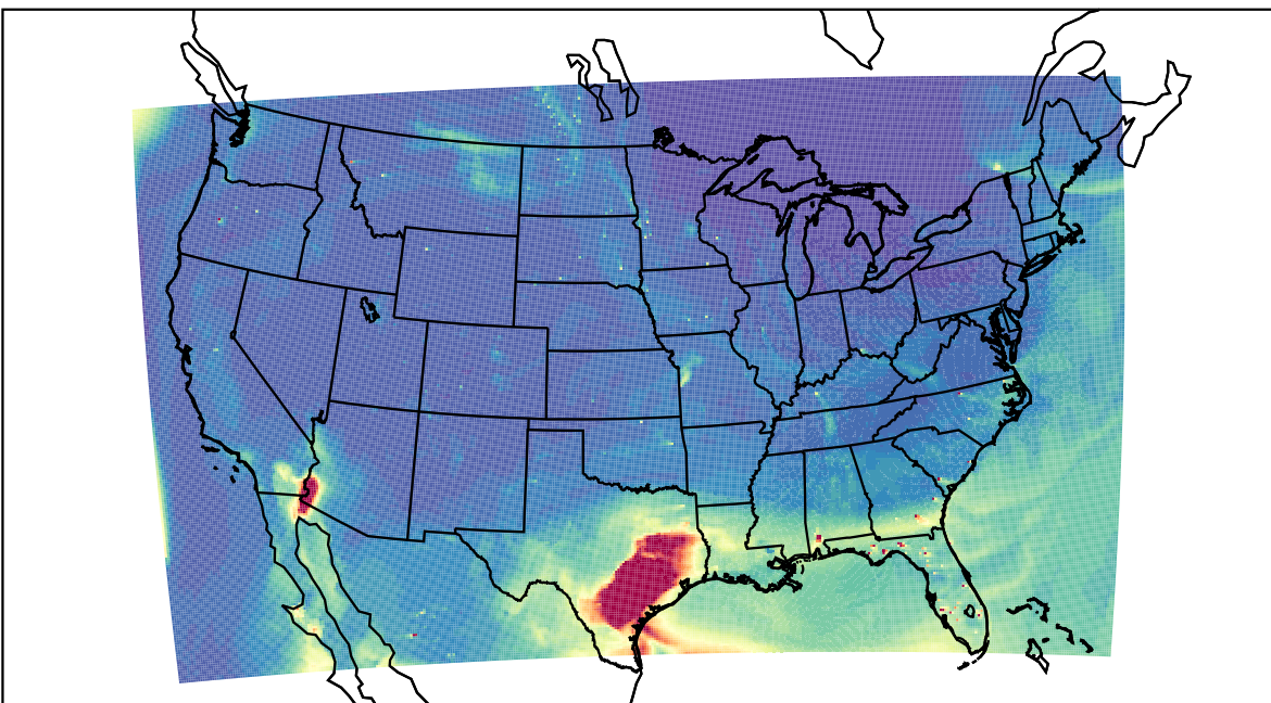
WRF 2021-04-30_21:00:00
