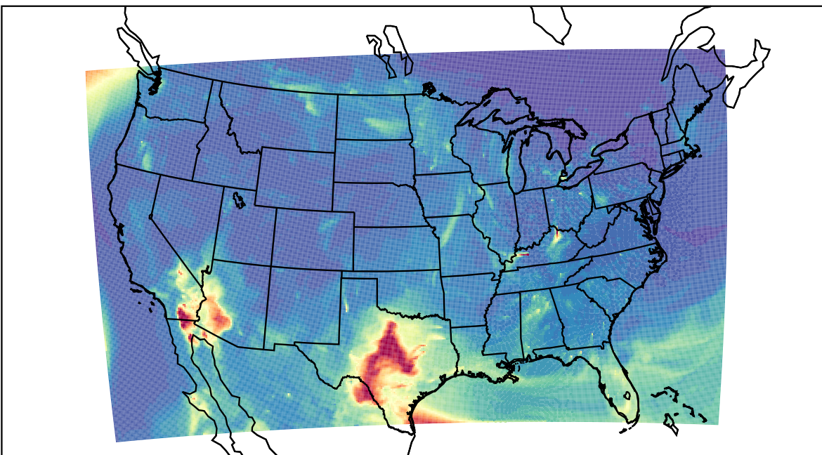
WRF 2021-05-01_09:00:00
