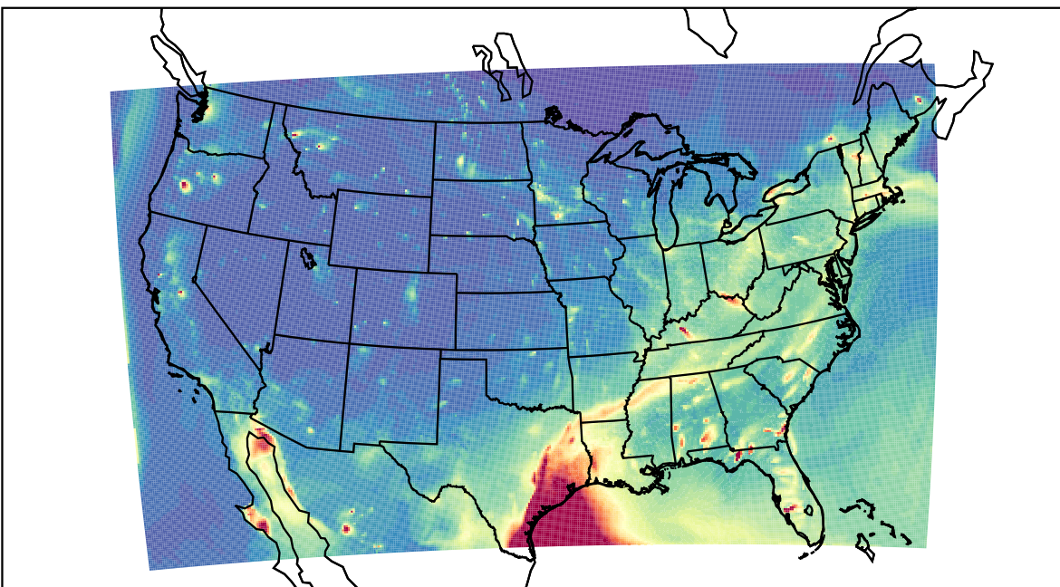
WRF 2021-04-30_03:00:00
