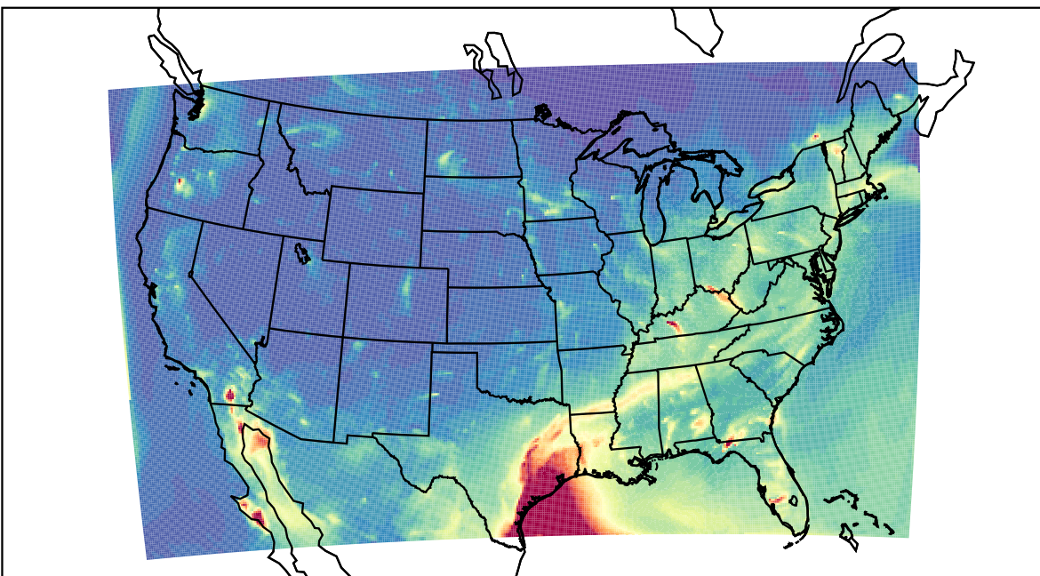
WRF 2021-04-30_05:00:00
