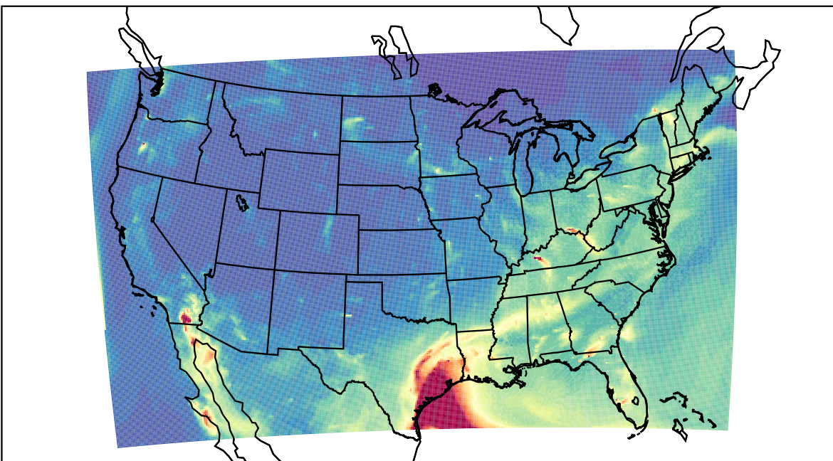
WRF 2021-04-30_07:00:00
