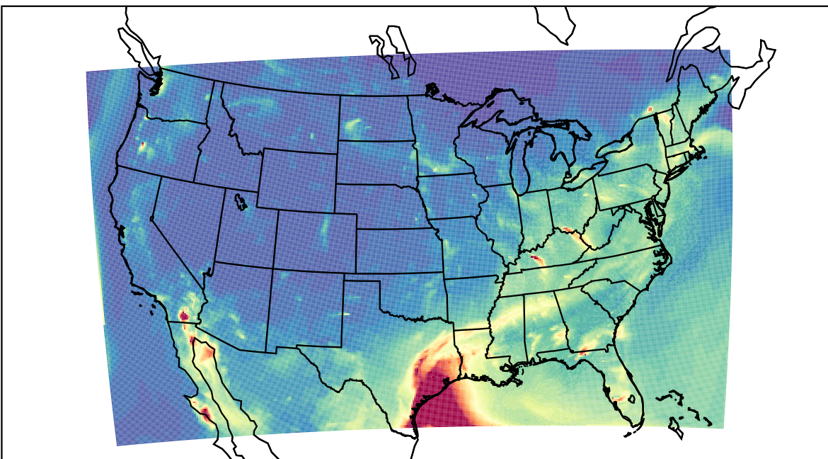
WRF 2021-04-30_06:00:00
