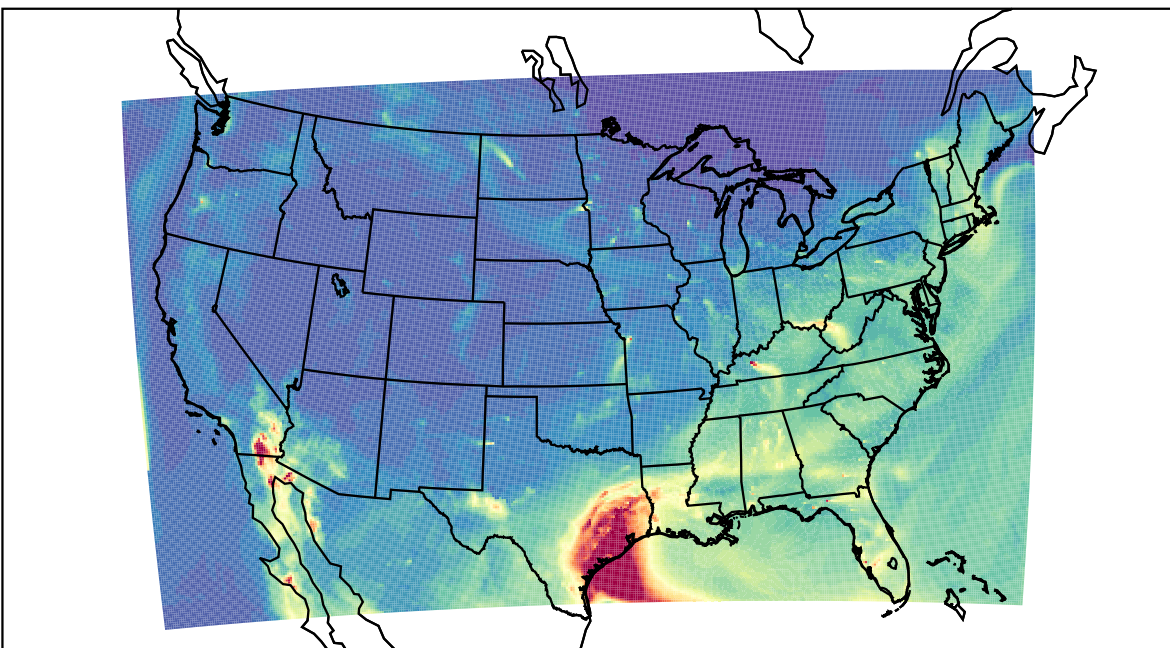
WRF 2021-04-30_11:00:00
