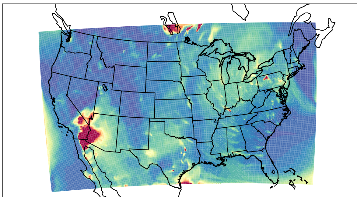
WRF 2021-05-20_05:00:00
