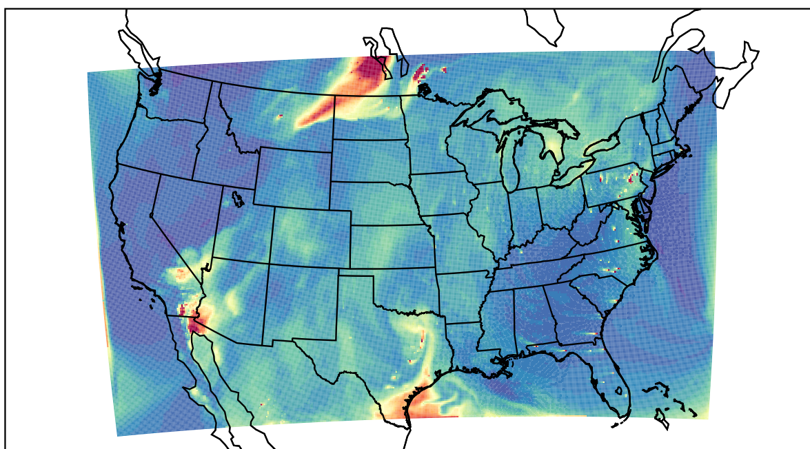
WRF 2021-05-20_21:00:00
