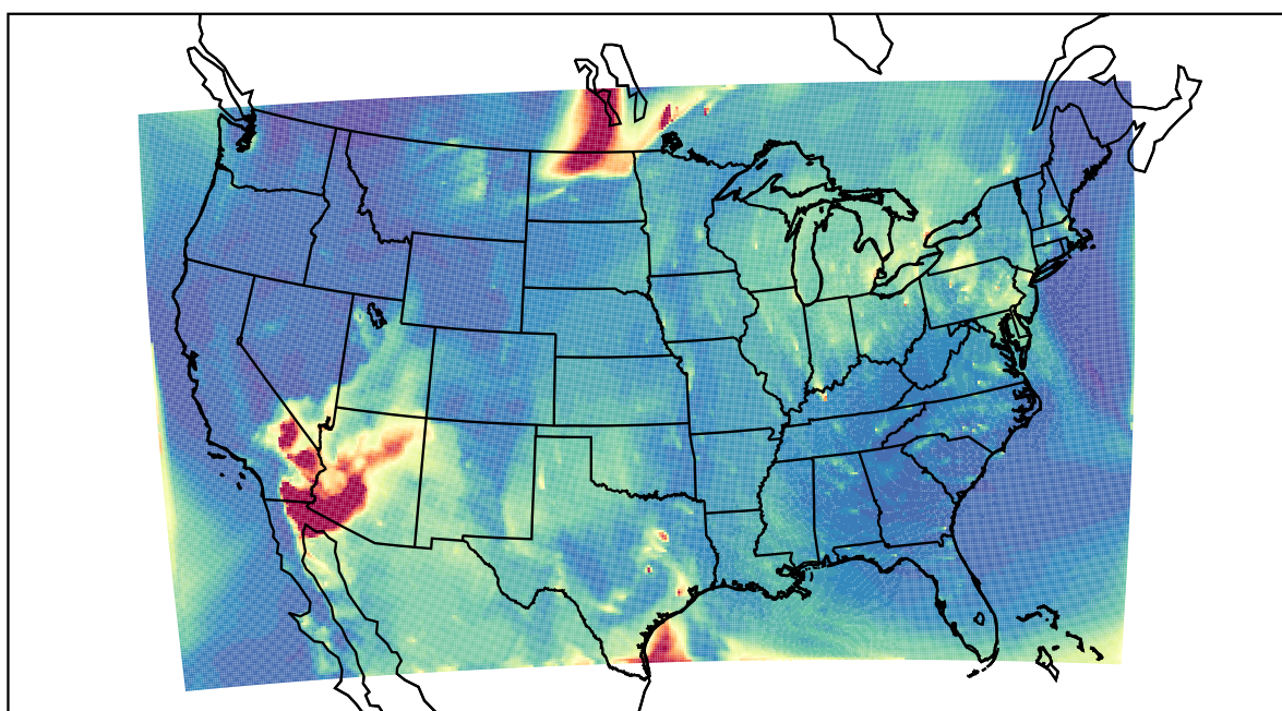
WRF 2021-05-20_12:00:00
