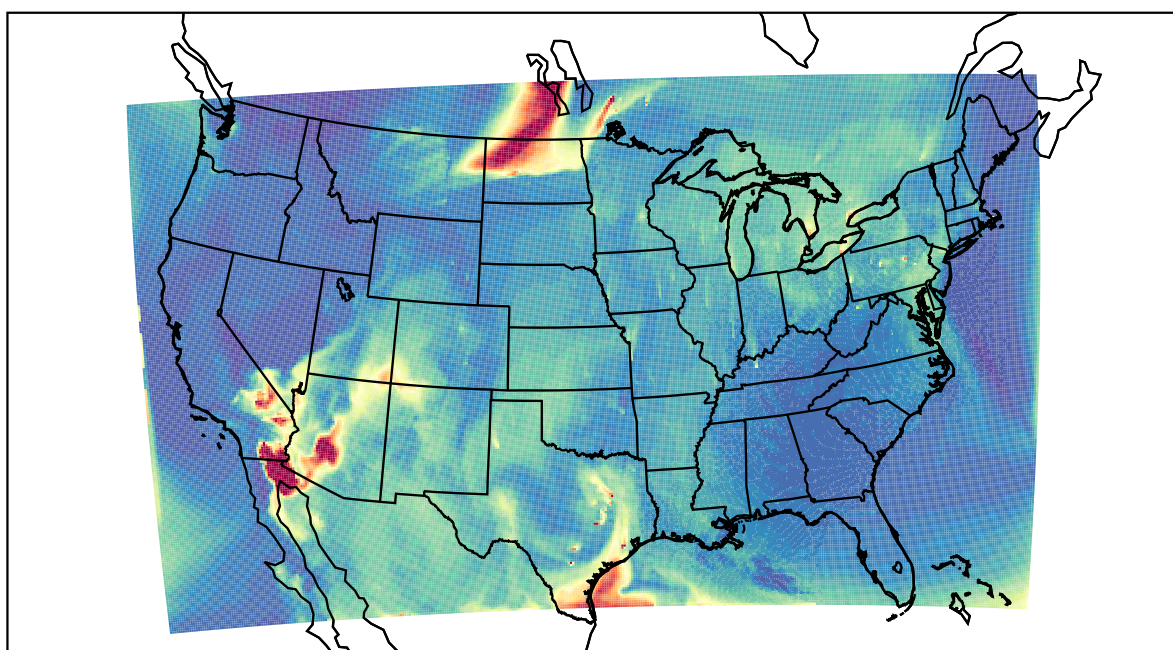
WRF 2021-05-20_16:00:00
