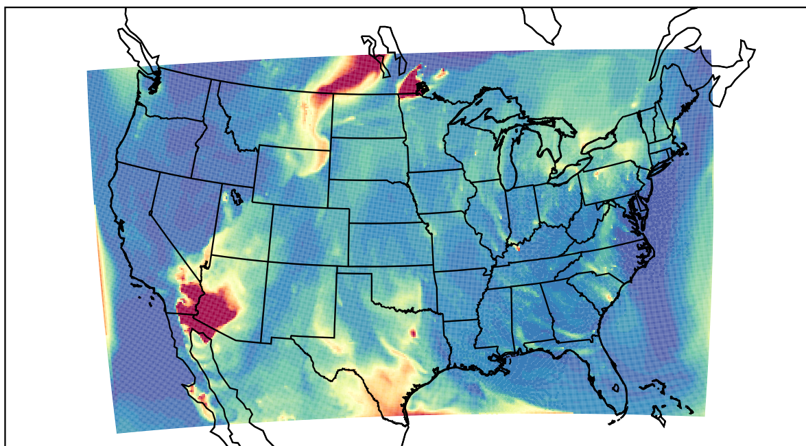
WRF 2021-05-21_07:00:00
