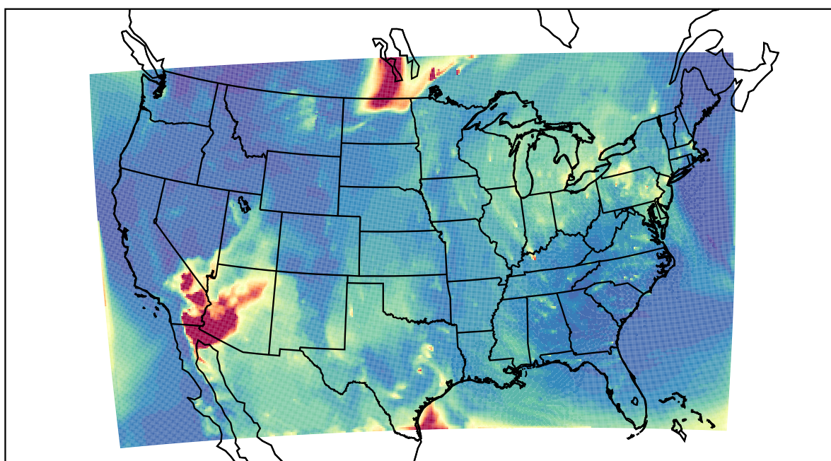
WRF 2021-05-20_11:00:00
