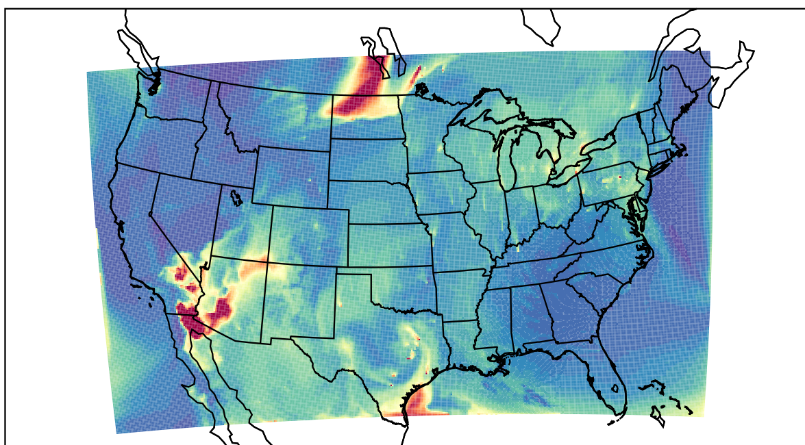
WRF 2021-05-20_15:00:00
