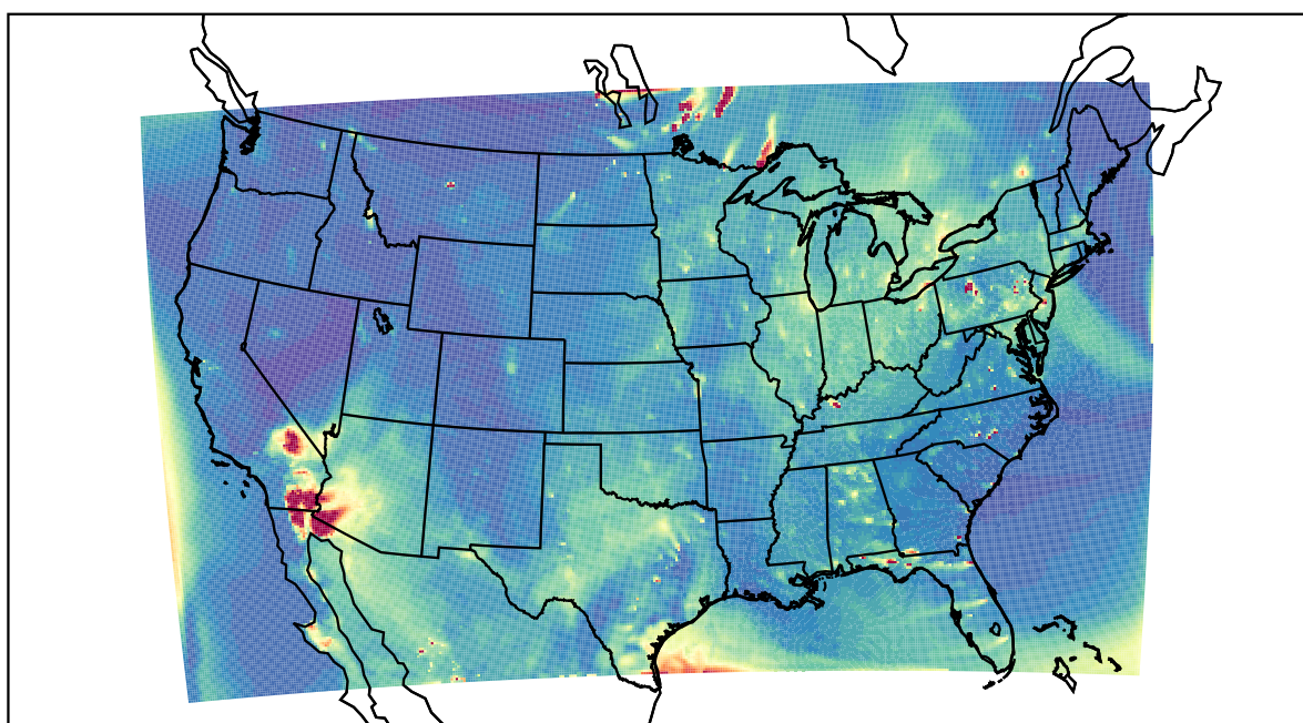
WRF 2021-05-20_01:00:00
