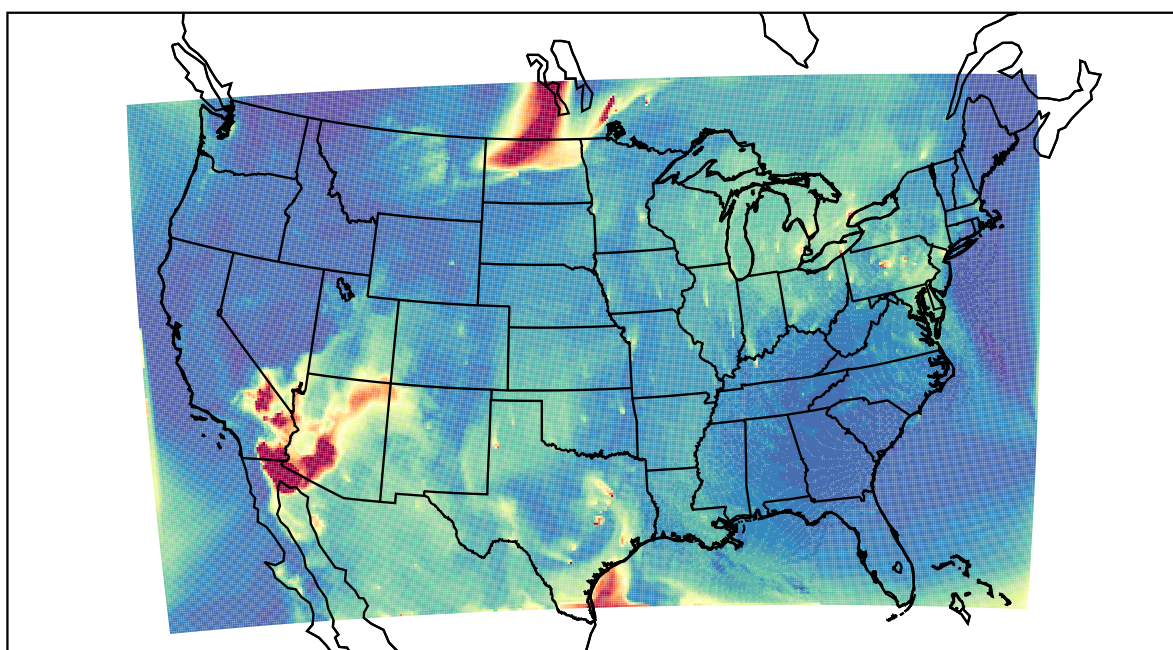
WRF 2021-05-20_14:00:00
