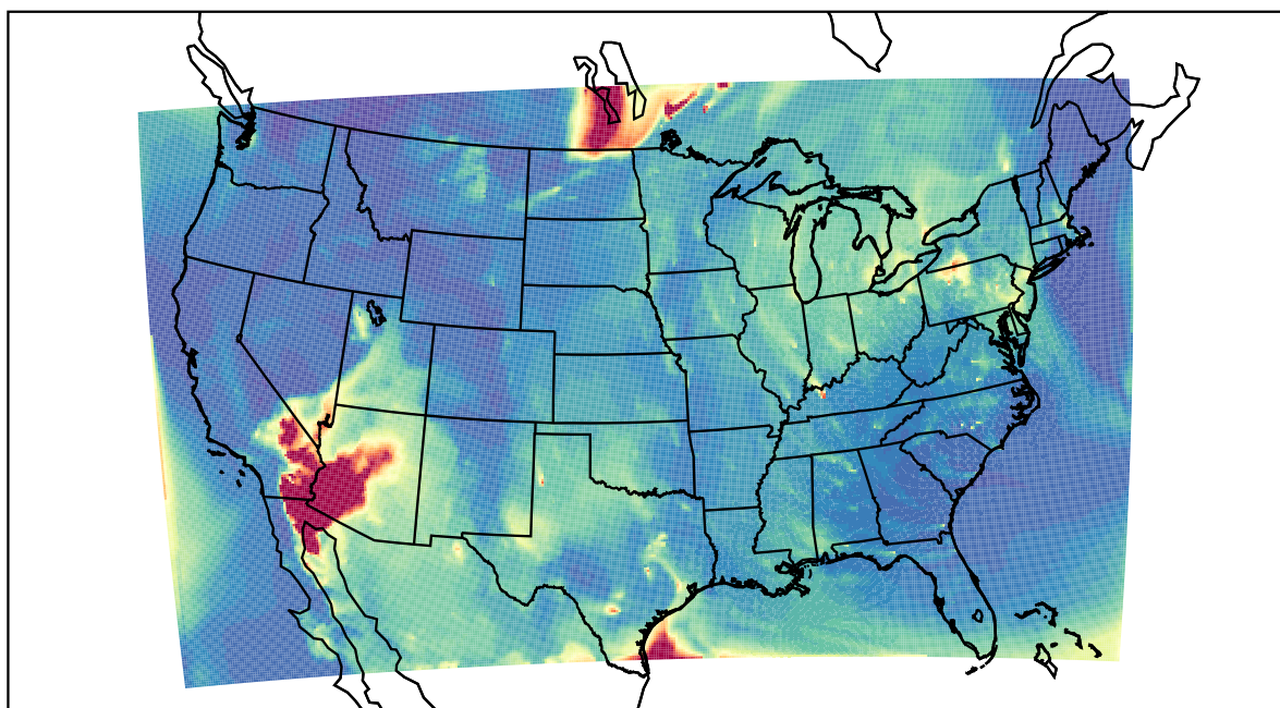
WRF 2021-05-20_09:00:00
