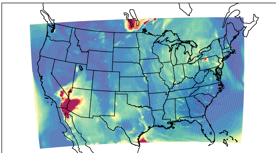
WRF 2021-05-20_07:00:00
