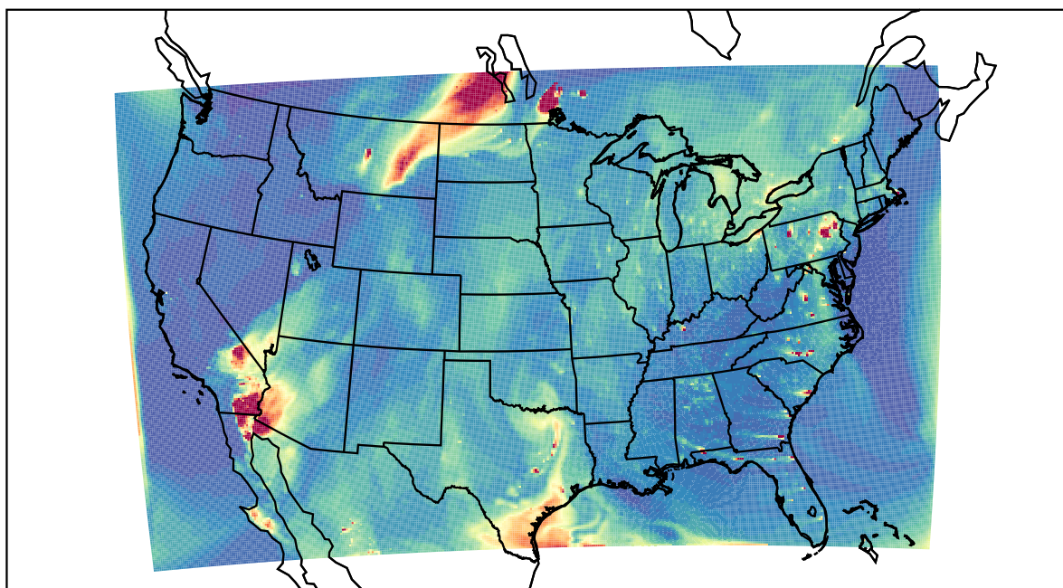
WRF 2021-05-21_00:00:00
