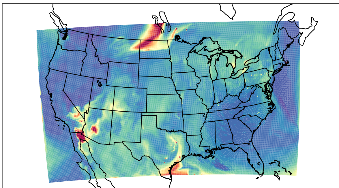
WRF 2021-05-20_17:00:00
