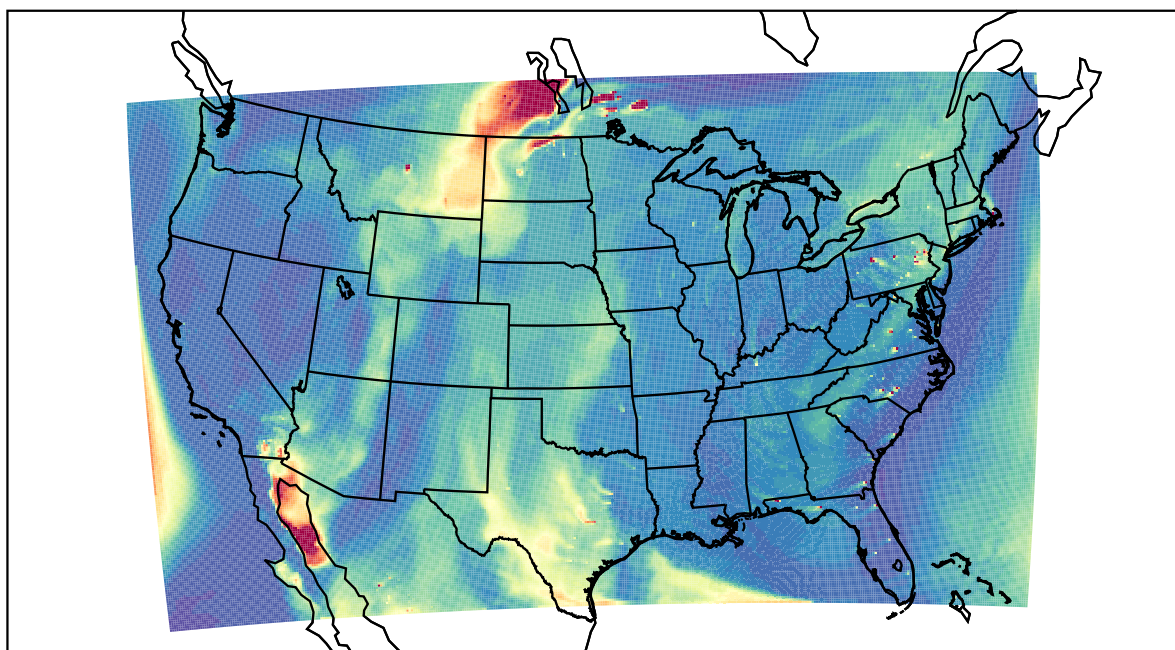
WRF 2021-05-21_21:00:00
