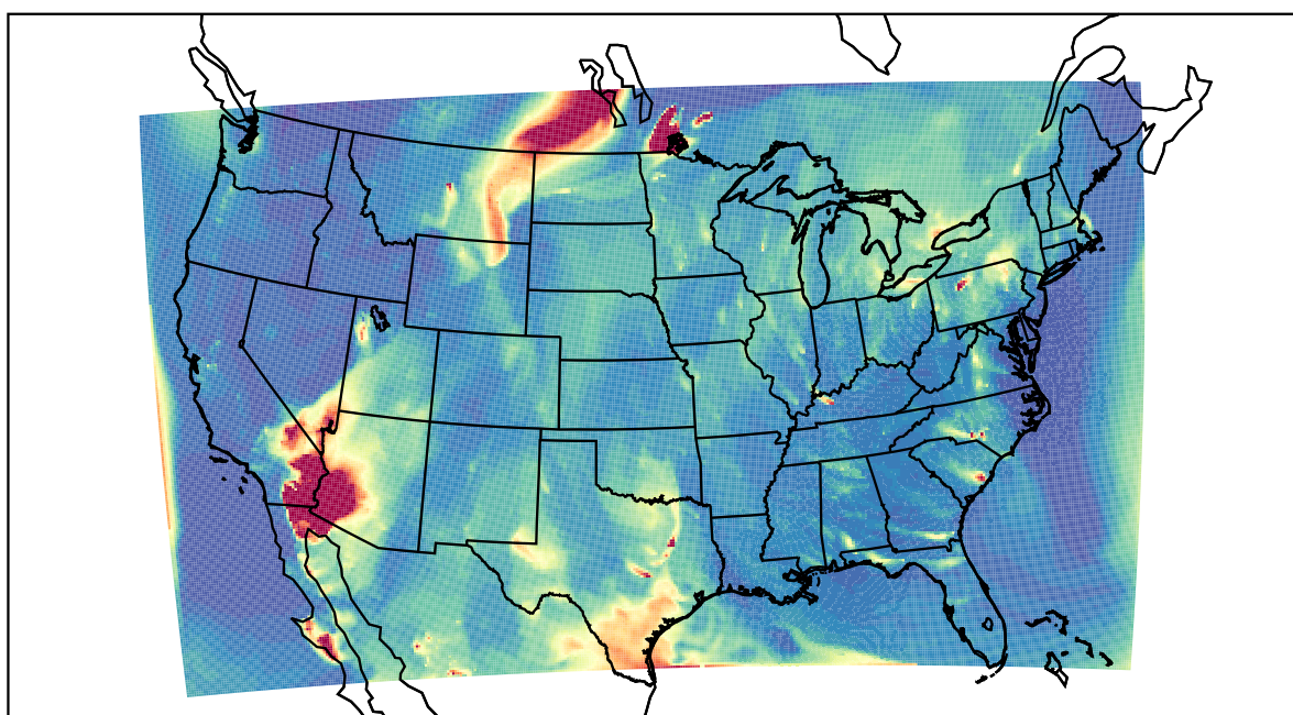
WRF 2021-05-21_04:00:00
