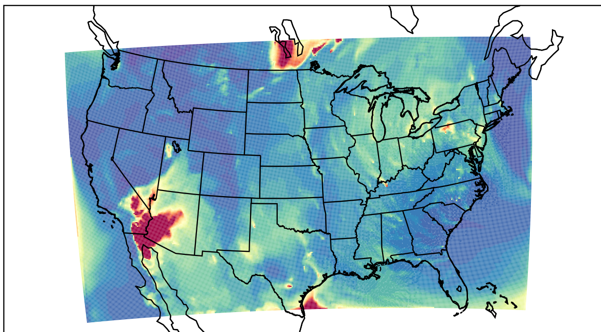
WRF 2021-05-20_08:00:00
