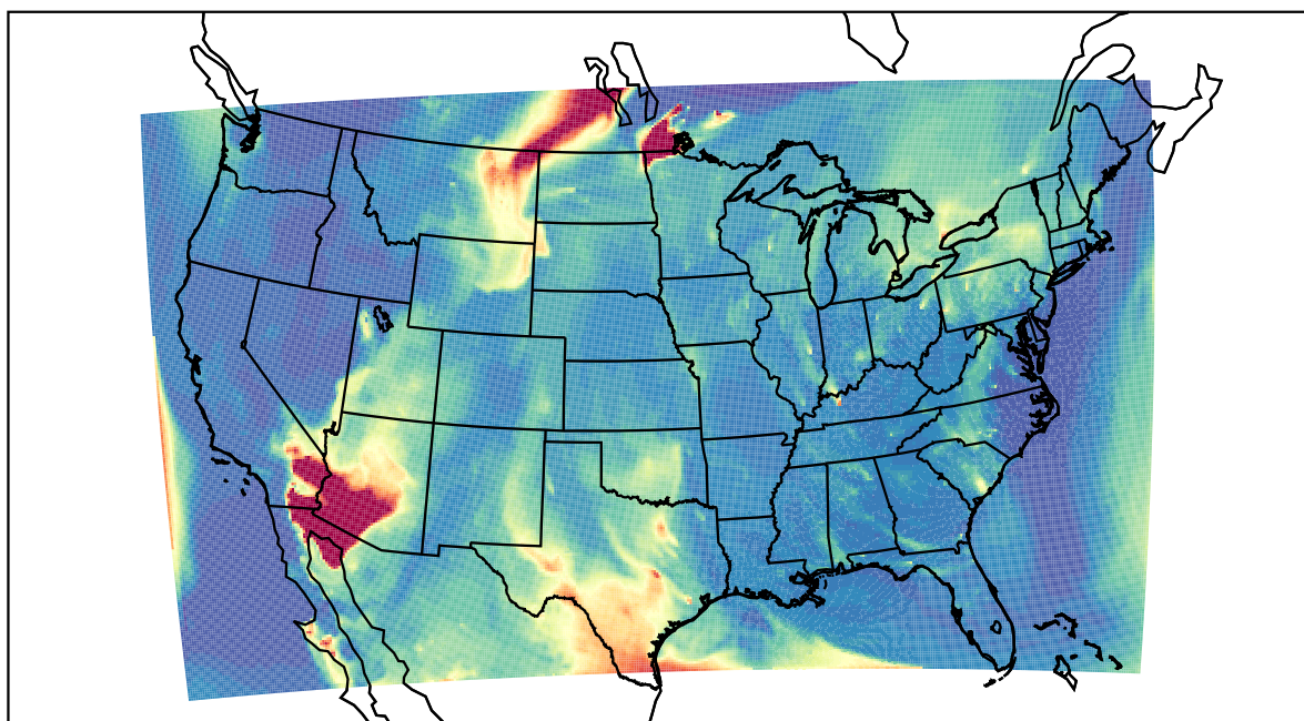
WRF 2021-05-21_09:00:00
