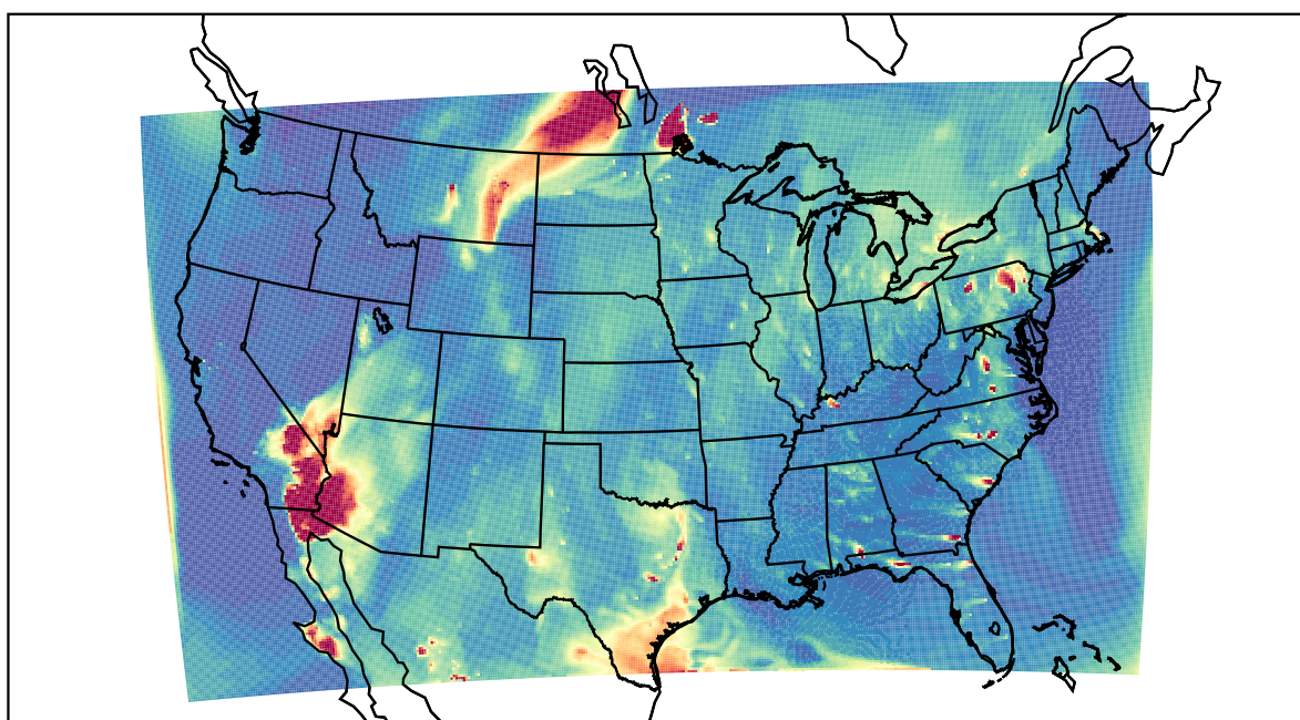
WRF 2021-05-21_02:00:00
