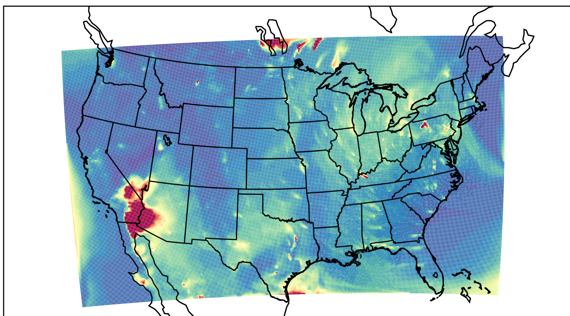
WRF 2021-05-20_04:00:00
