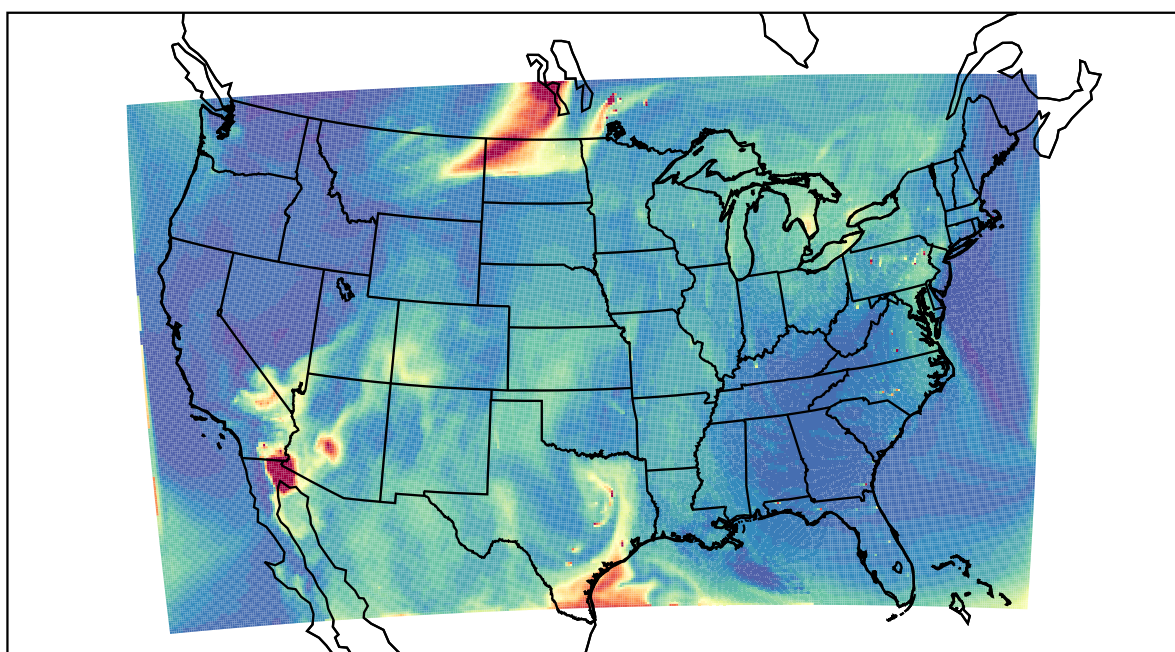
WRF 2021-05-20_18:00:00
