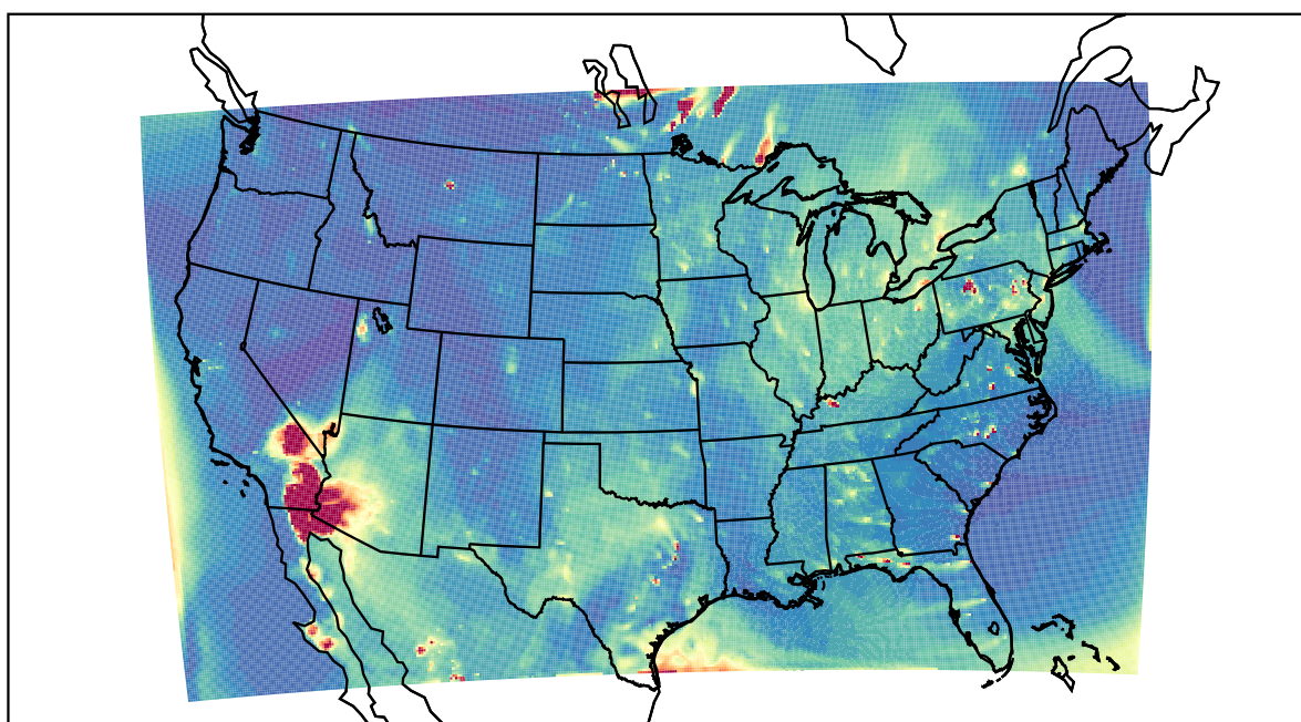
WRF 2021-05-20_02:00:00
