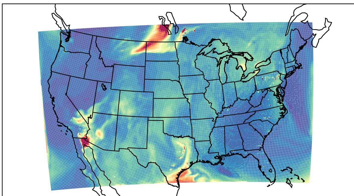
WRF 2021-05-20_19:00:00
