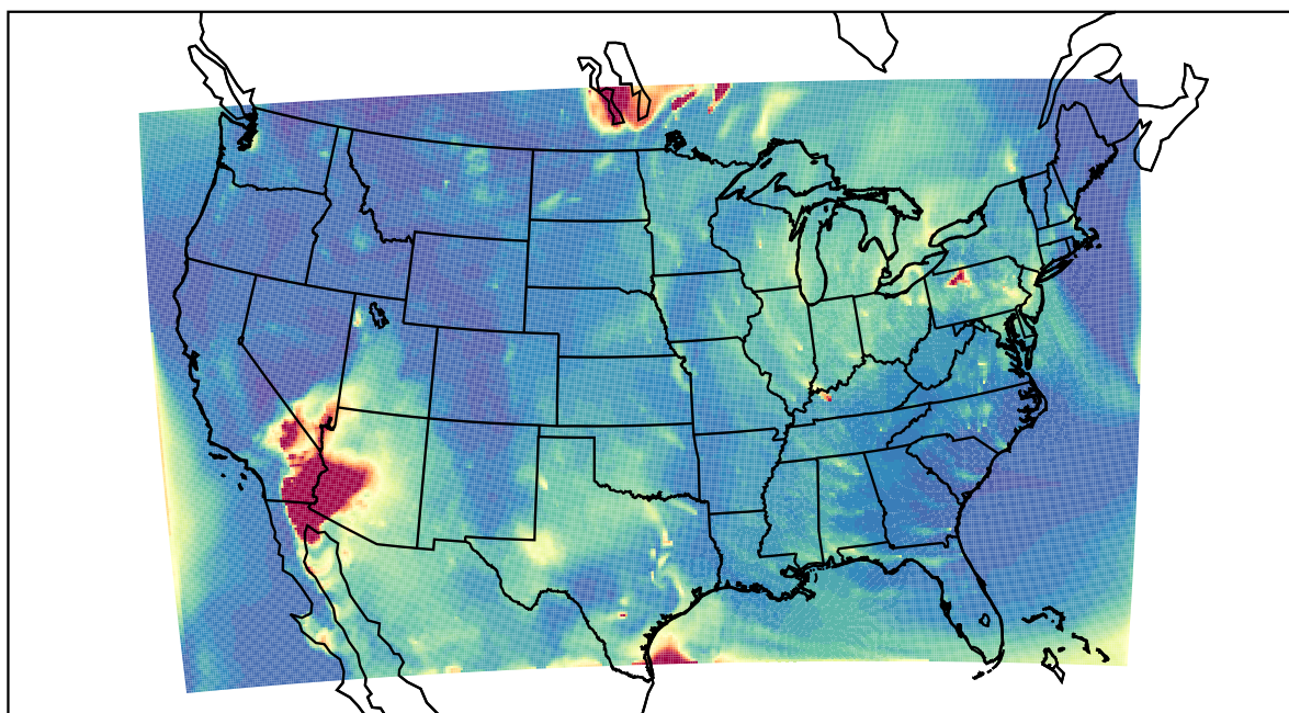
WRF 2021-05-20_06:00:00
