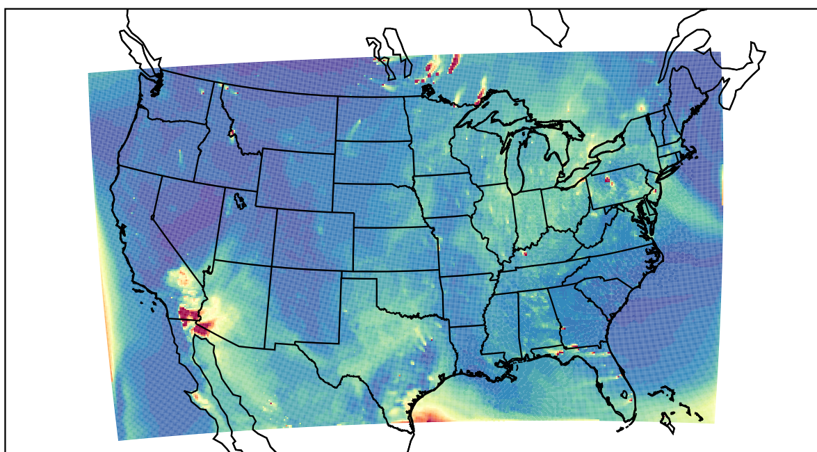
WRF 2021-05-20_00:00:00
