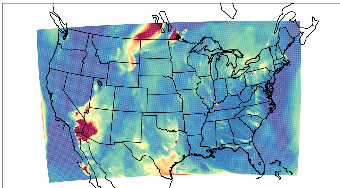
WRF 2021-05-21_05:00:00
