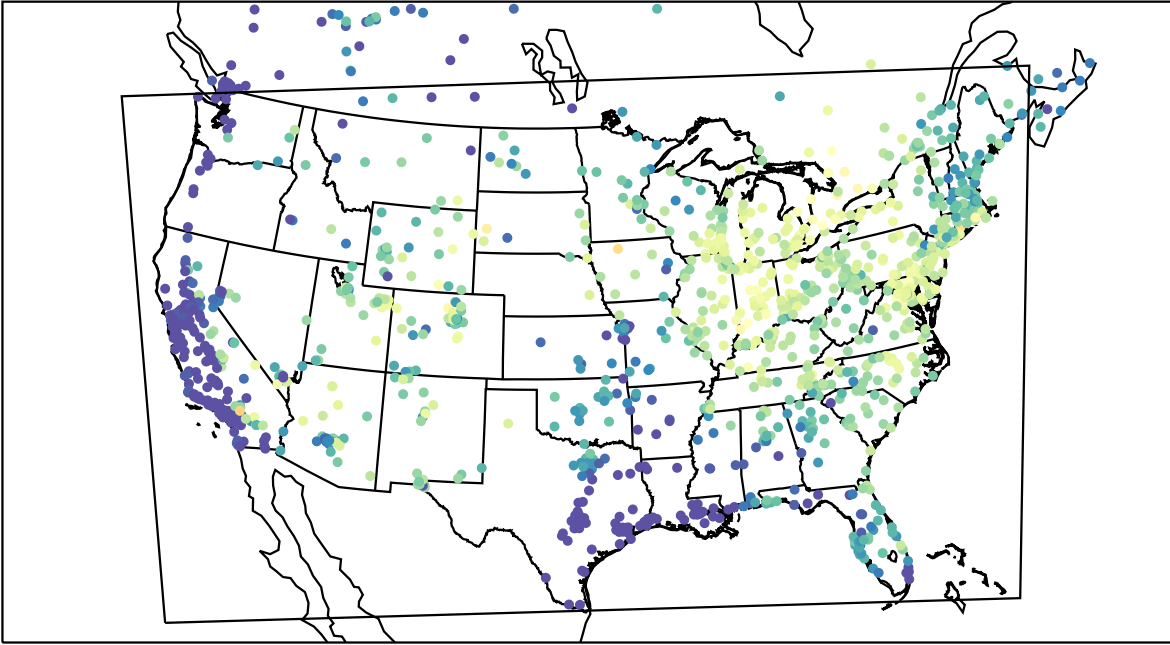
AirNOW (2021-06-24_14:00:00)
