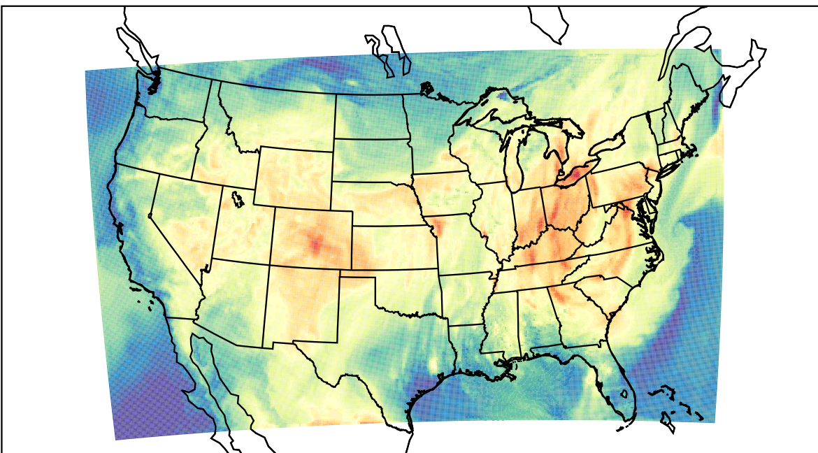
WRF (2021-06-24_17:00:00)
