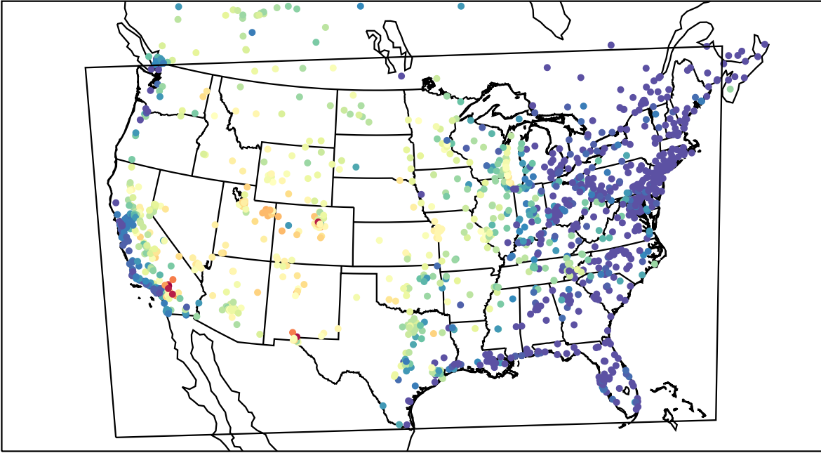
AirNOW (2021-06-23_02:00:00)
