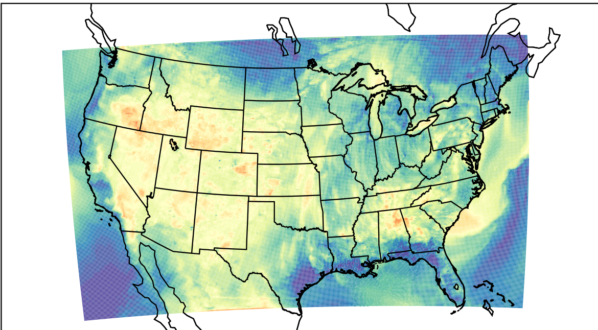
WRF (2021-06-24_02:00:00)
