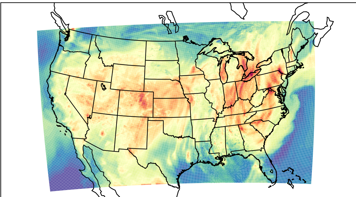
WRF (2021-06-24_22:00:00)
