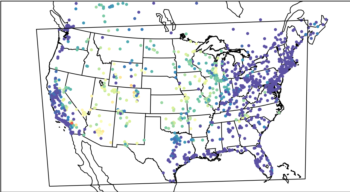
AirNOW (2021-06-23_08:00:00)
