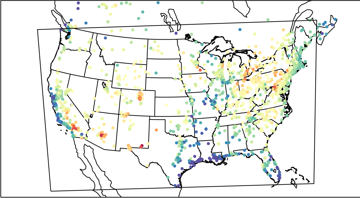
AirNOW (2021-06-24_22:00:00)
