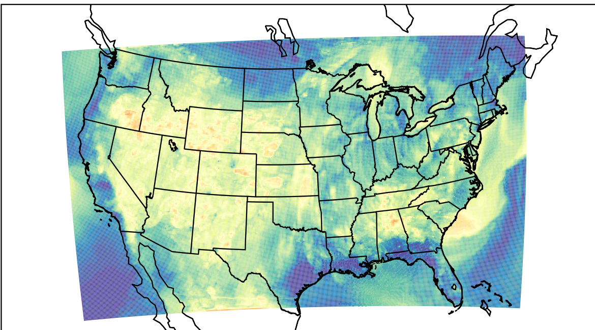
WRF (2021-06-24_03:00:00)
