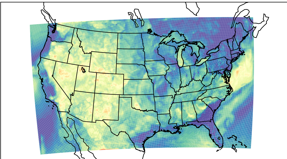
WRF (2021-06-23_04:00:00)
