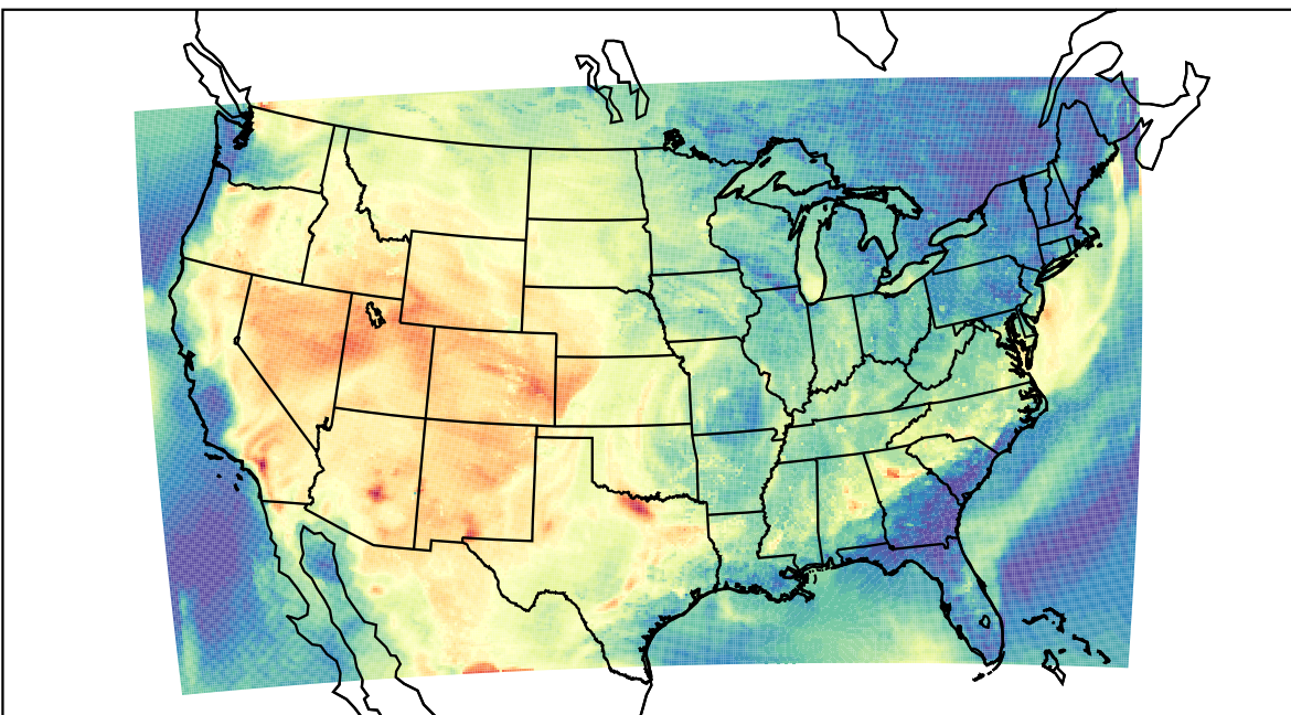
WRF (2021-06-23_00:00:00)
