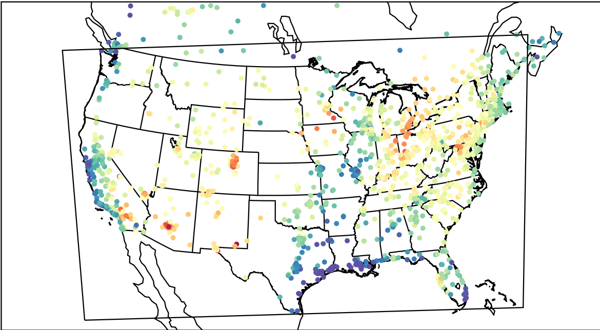
AirNOW (2021-06-24_19:00:00)
