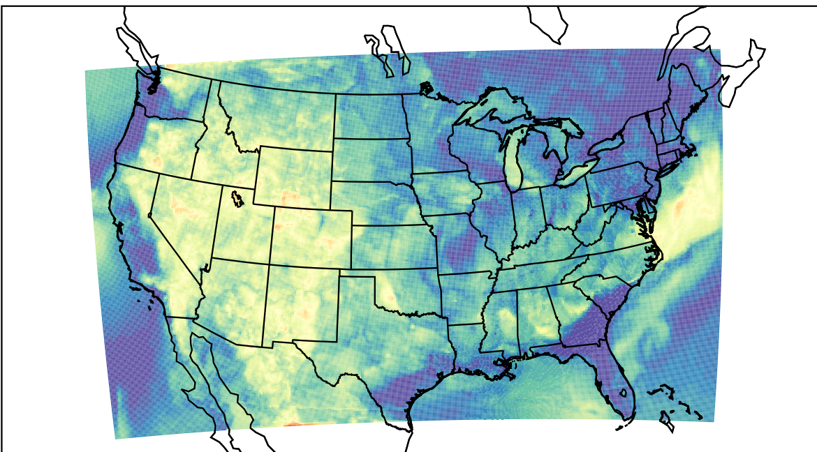
WRF (2021-06-23_05:00:00)
