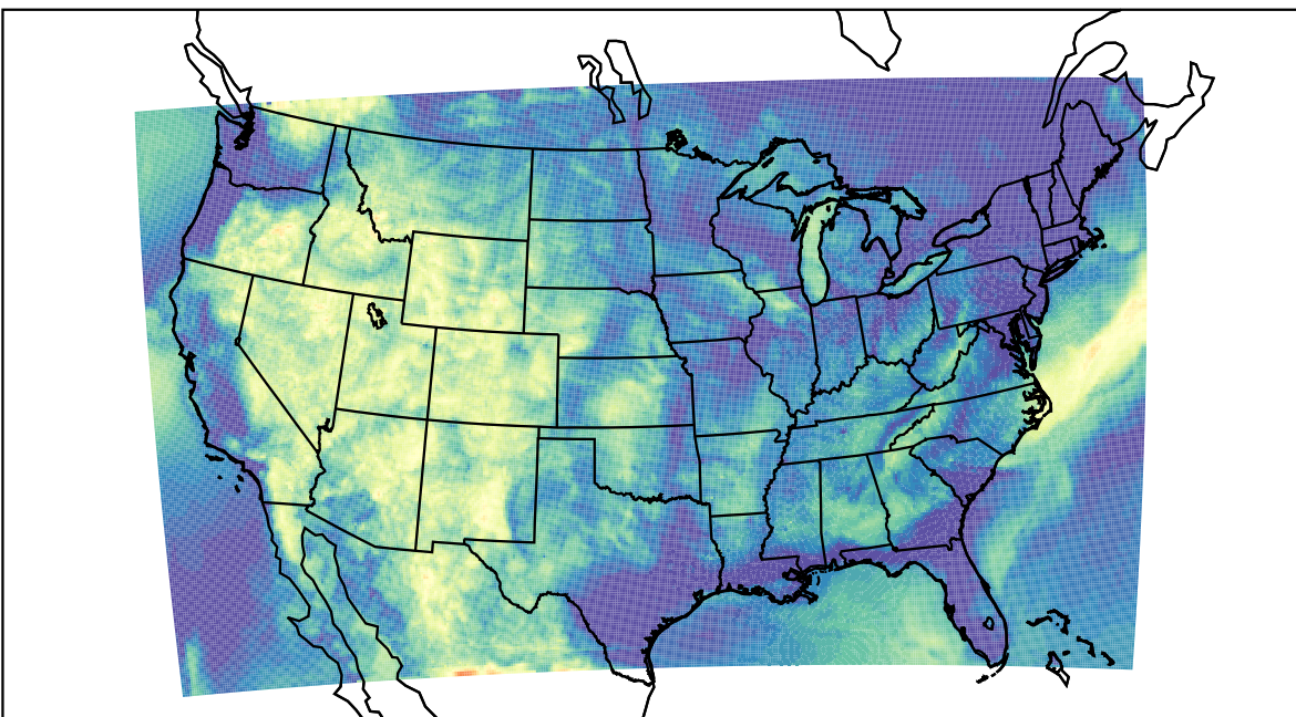
WRF (2021-06-23_10:00:00)
