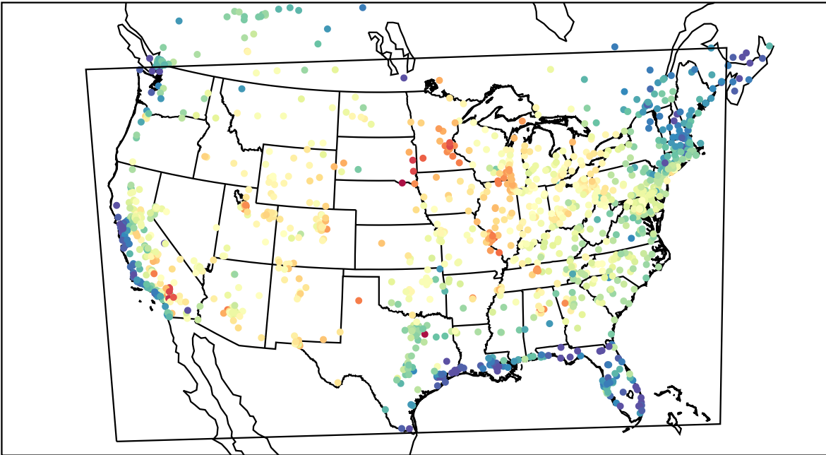
AirNOW (2021-06-23_23:00:00)
