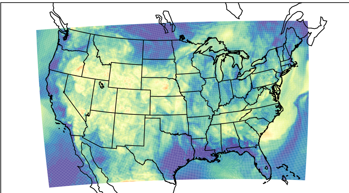
WRF (2021-06-24_06:00:00)
