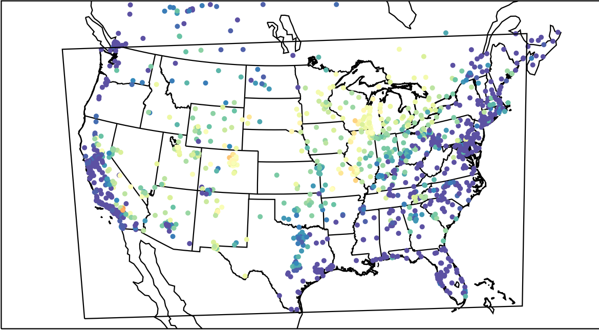
AirNOW (2021-06-24_07:00:00)
