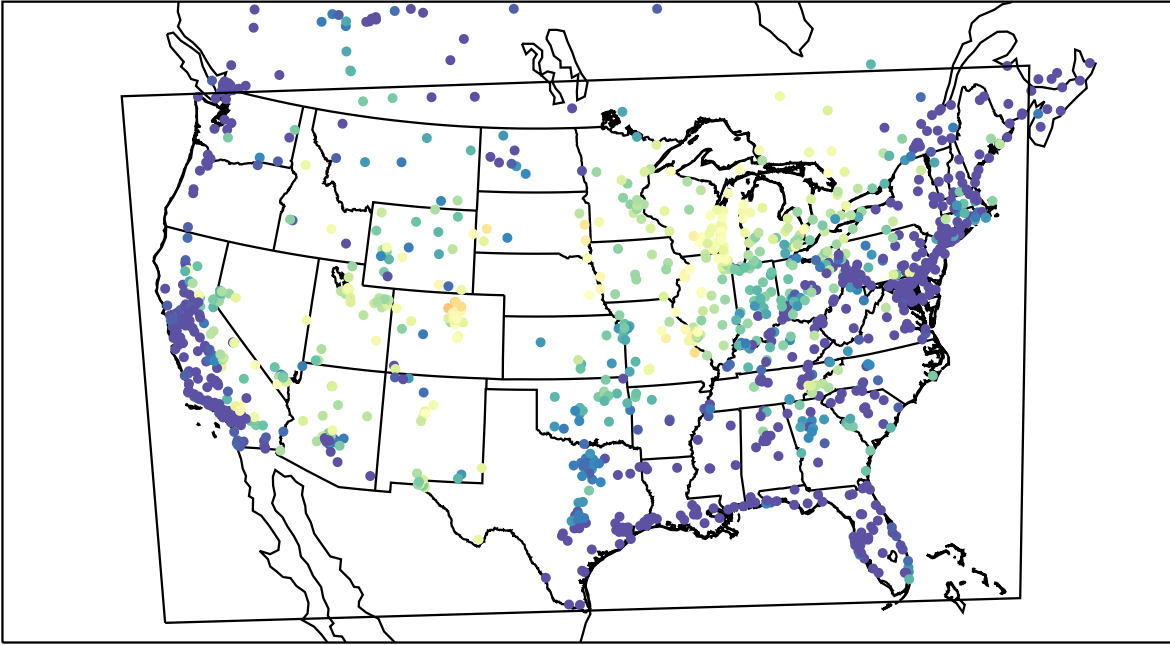
AirNOW (2021-06-24_08:00:00)
