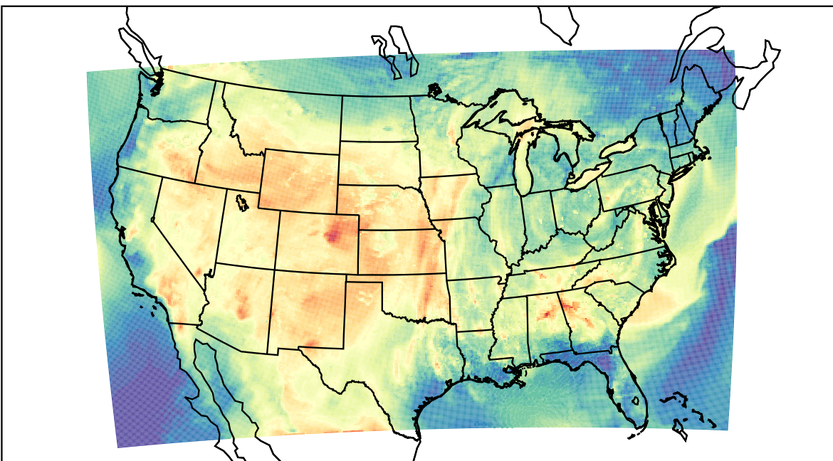
WRF (2021-06-24_00:00:00)
