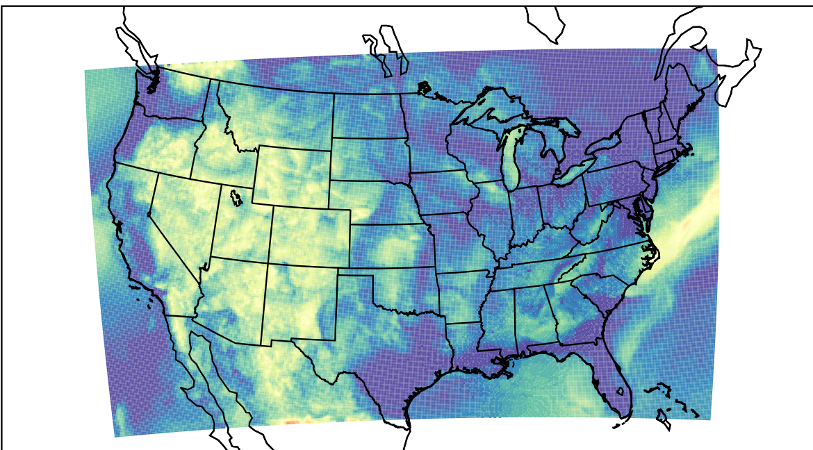
WRF (2021-06-23_11:00:00)
