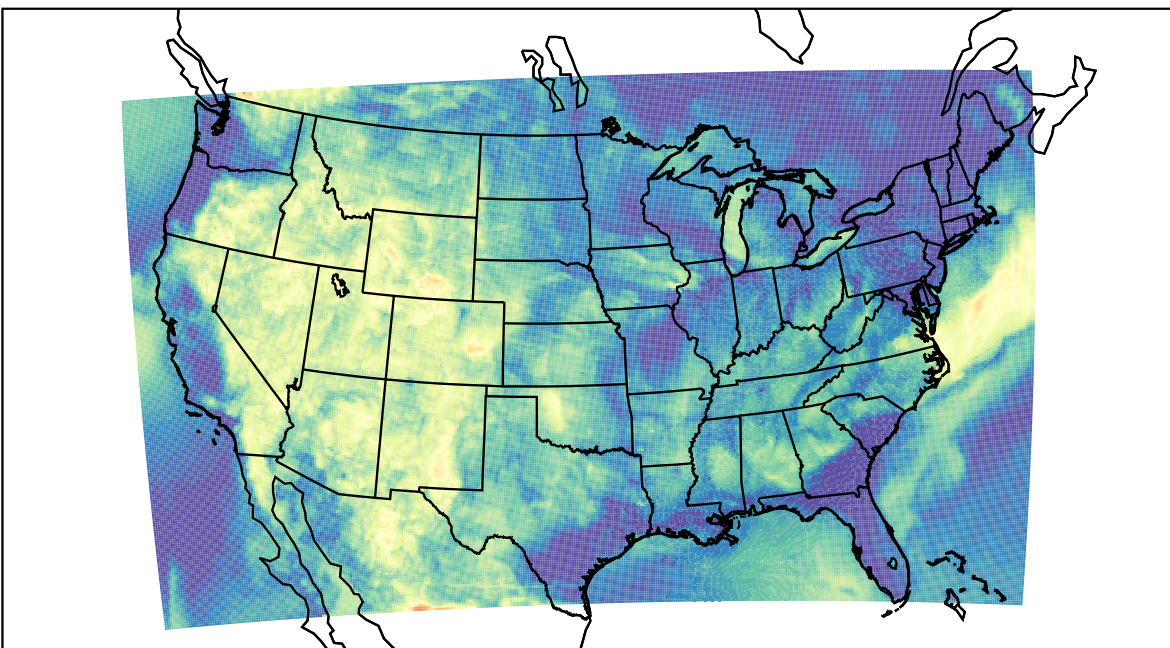
WRF (2021-06-23_07:00:00)
