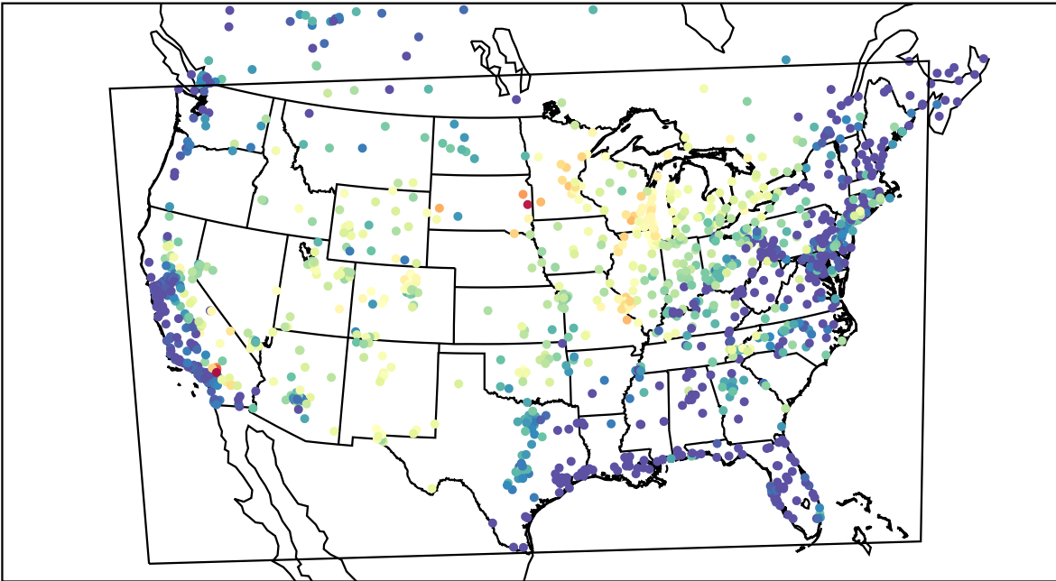
AirNOW (2021-06-24_04:00:00)
