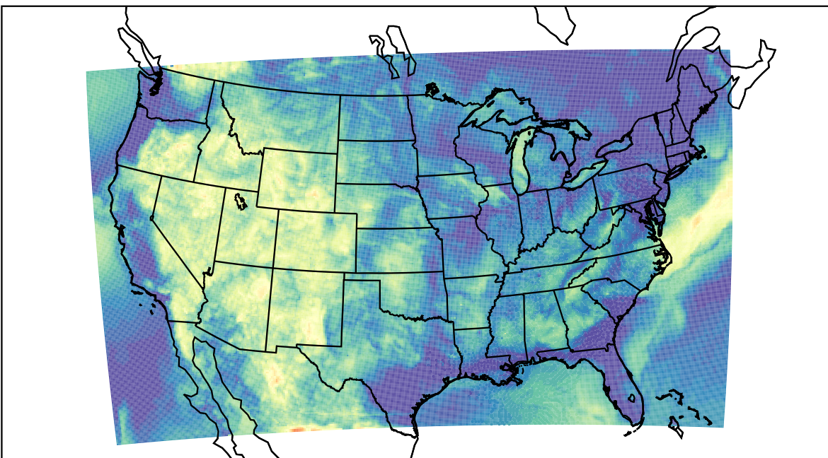
WRF (2021-06-23_09:00:00)
