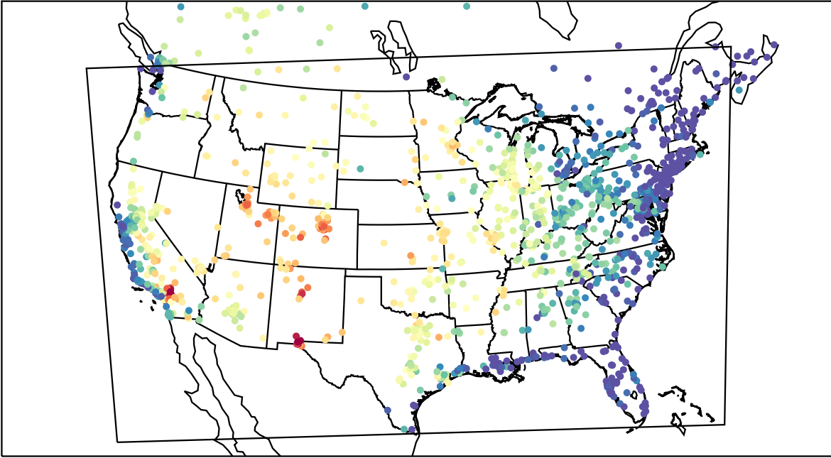
AirNOW (2021-06-23_00:00:00)
