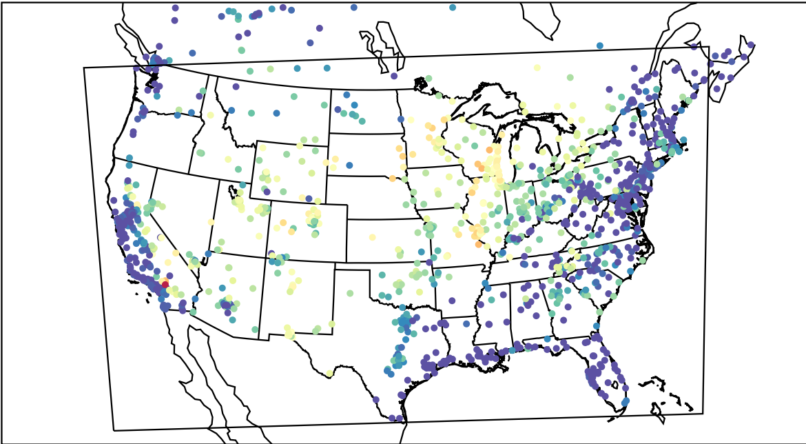
AirNOW (2021-06-24_05:00:00)
