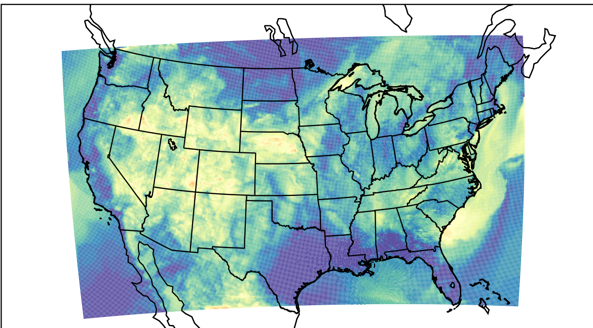
WRF (2021-06-24_09:00:00)
