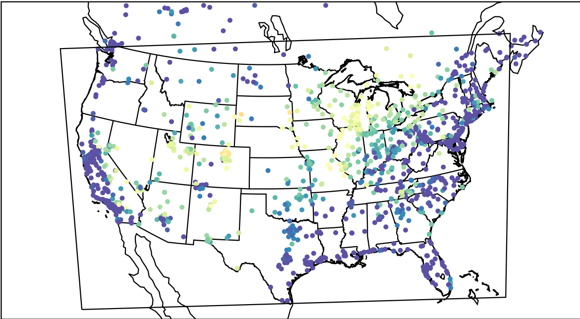
AirNOW (2021-06-24_09:00:00)
