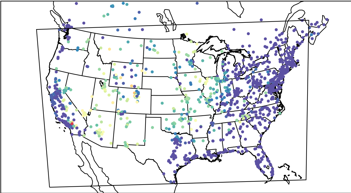
AirNOW (2021-06-23_10:00:00)
