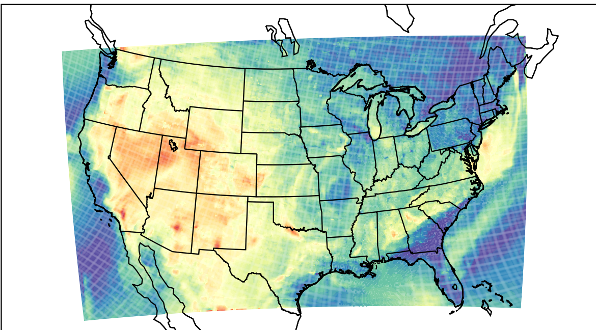
WRF (2021-06-23_01:00:00)
