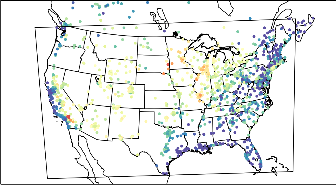
AirNOW (2021-06-24_02:00:00)
