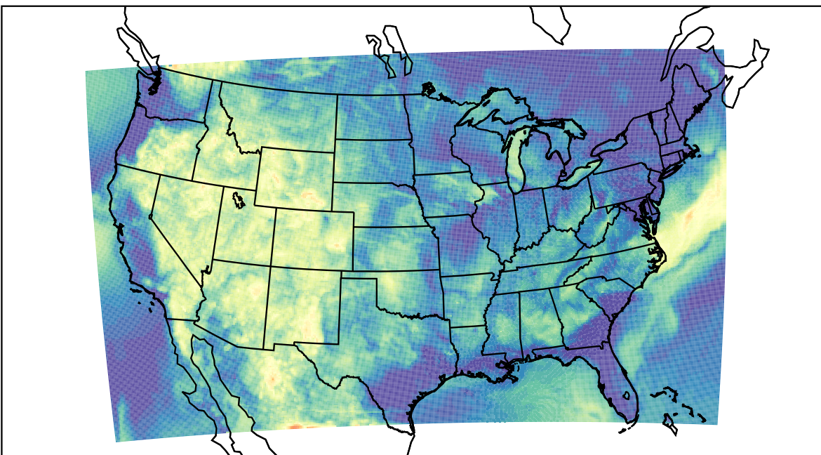
WRF (2021-06-23_08:00:00)
