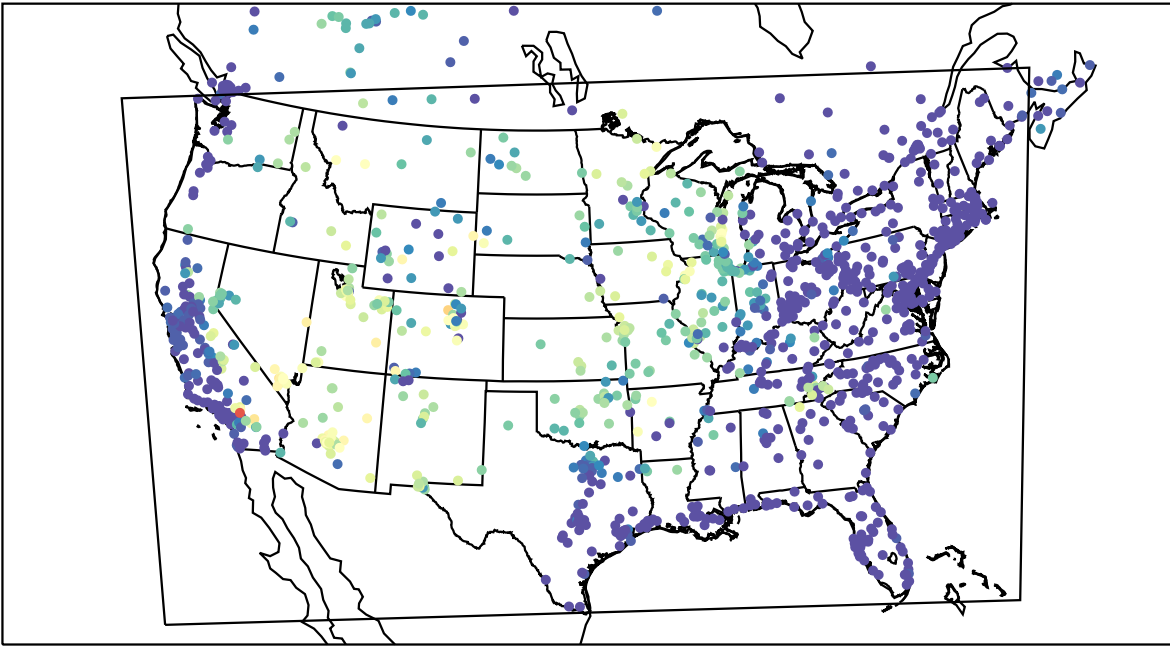
AirNOW (2021-06-23_09:00:00)
