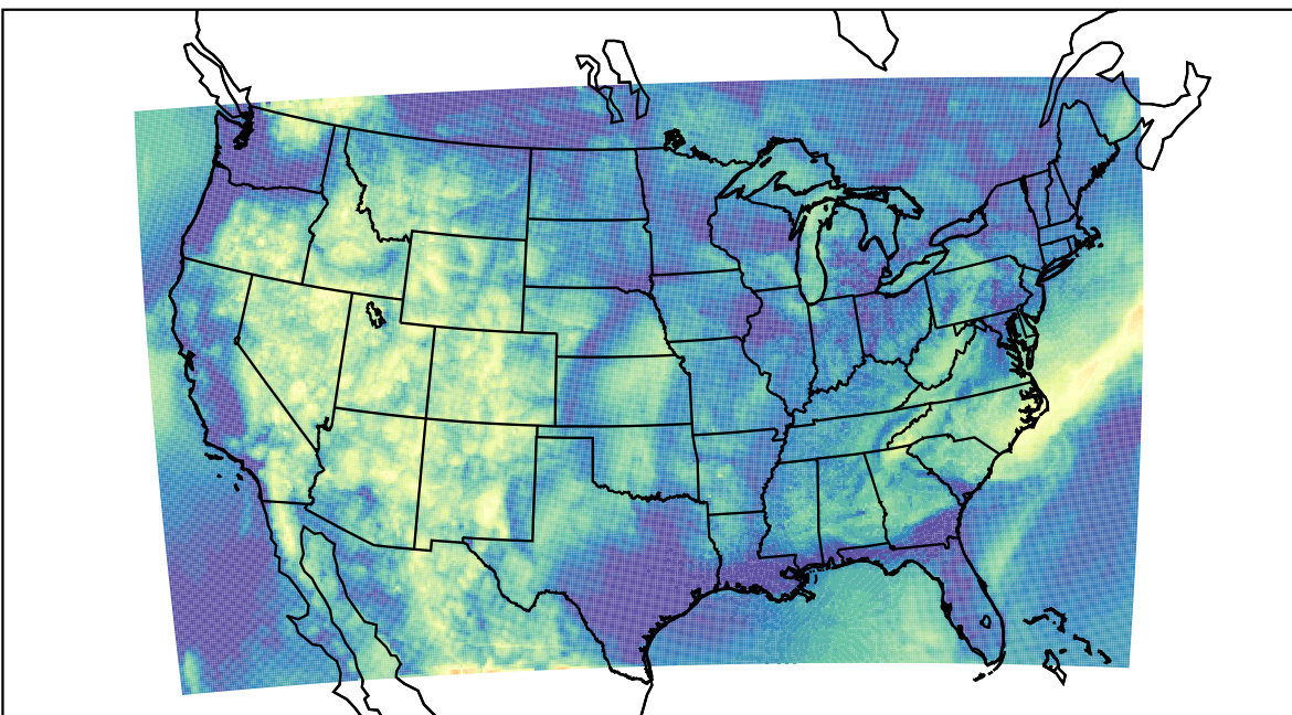
WRF (2021-06-23_13:00:00)
