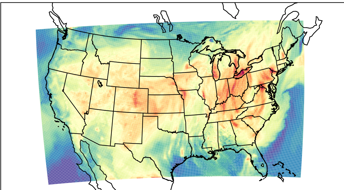
WRF (2021-06-24_19:00:00)
