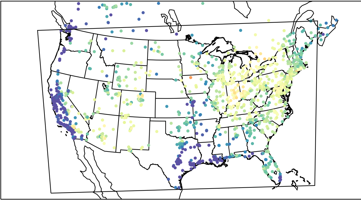
AirNOW (2021-06-24_15:00:00)
