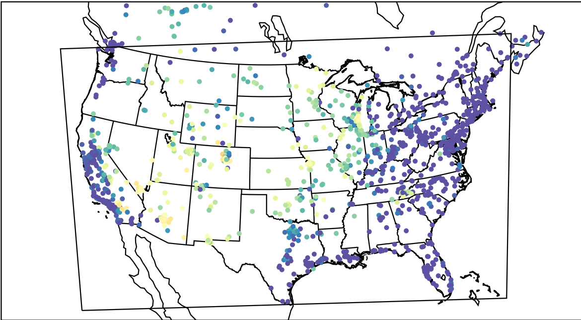
AirNOW (2021-06-23_07:00:00)
