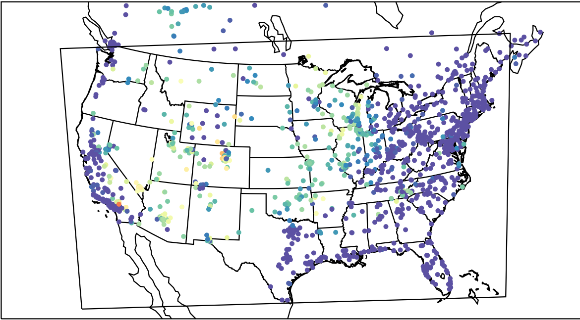
AirNOW (2021-06-23_11:00:00)
