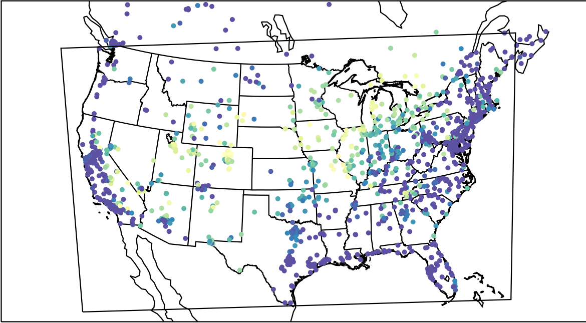
AirNOW (2021-06-24_10:00:00)
