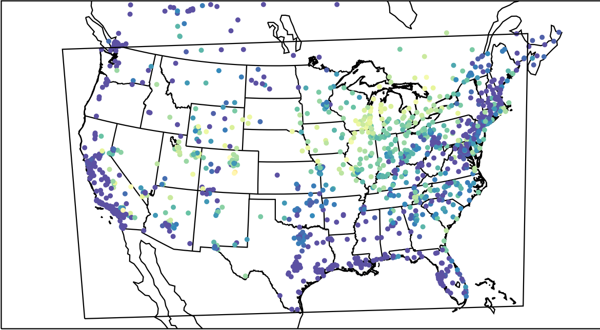
AirNOW (2021-06-24_12:00:00)
