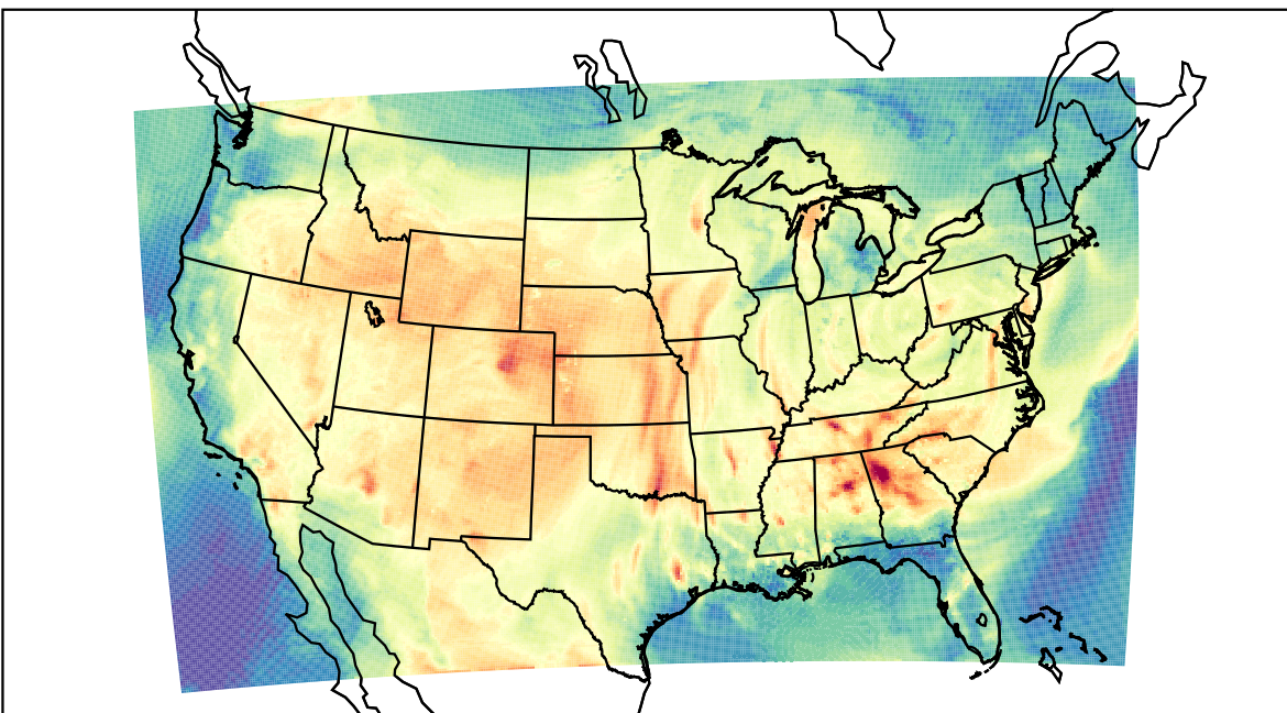
WRF (2021-06-23_21:00:00)
