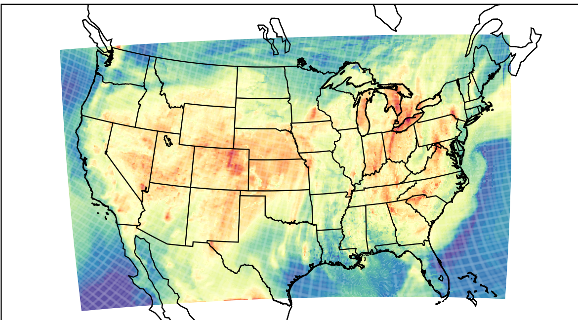
WRF (2021-06-24_23:00:00)
