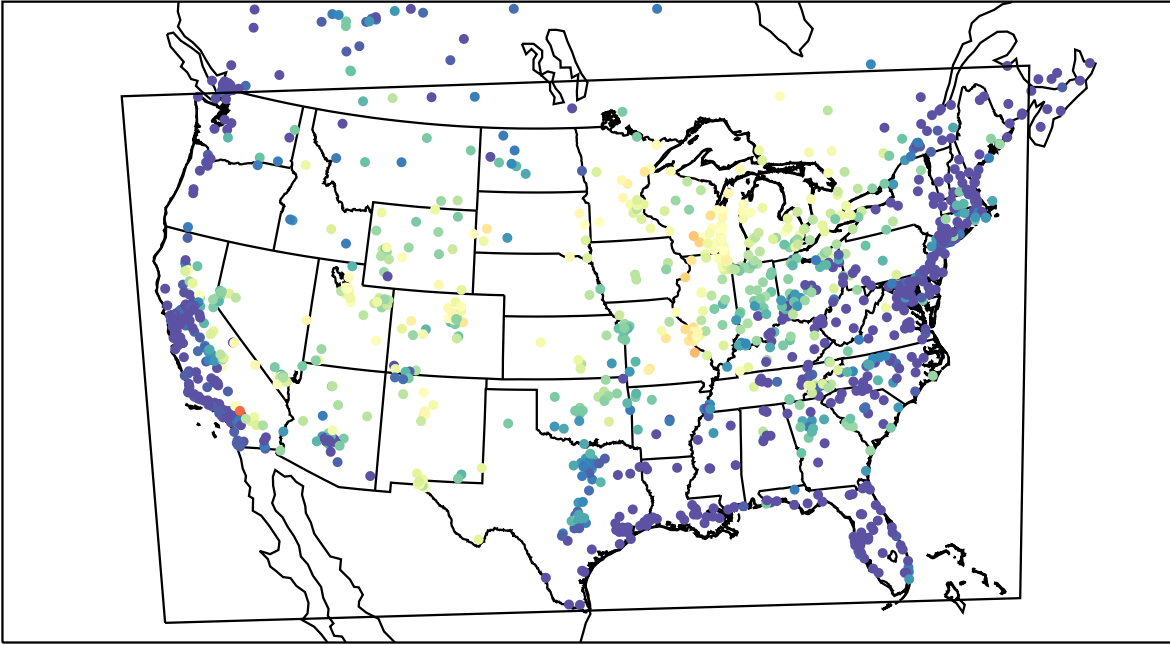
AirNOW (2021-06-24_06:00:00)
