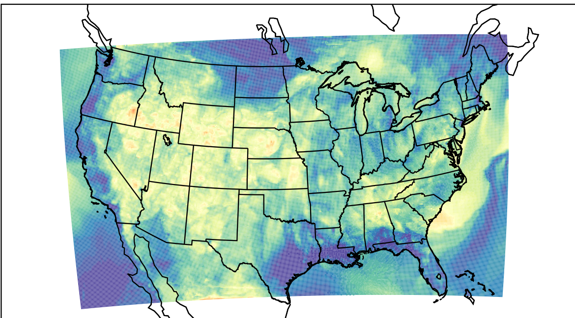
WRF (2021-06-24_05:00:00)
