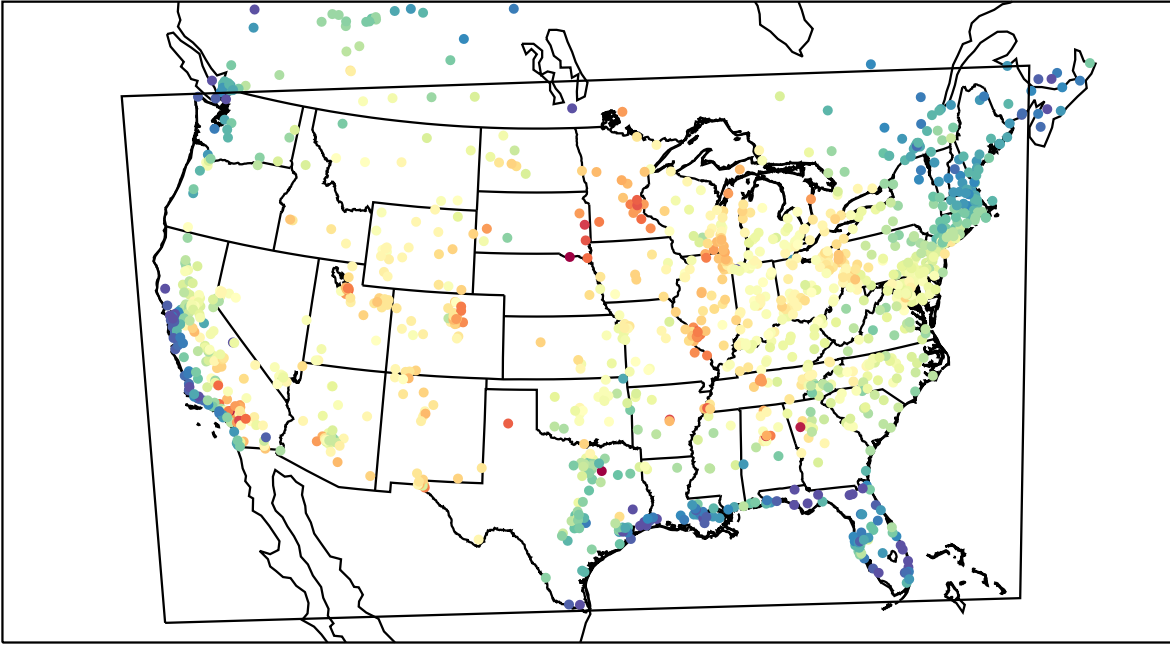
AirNOW (2021-06-23_22:00:00)
