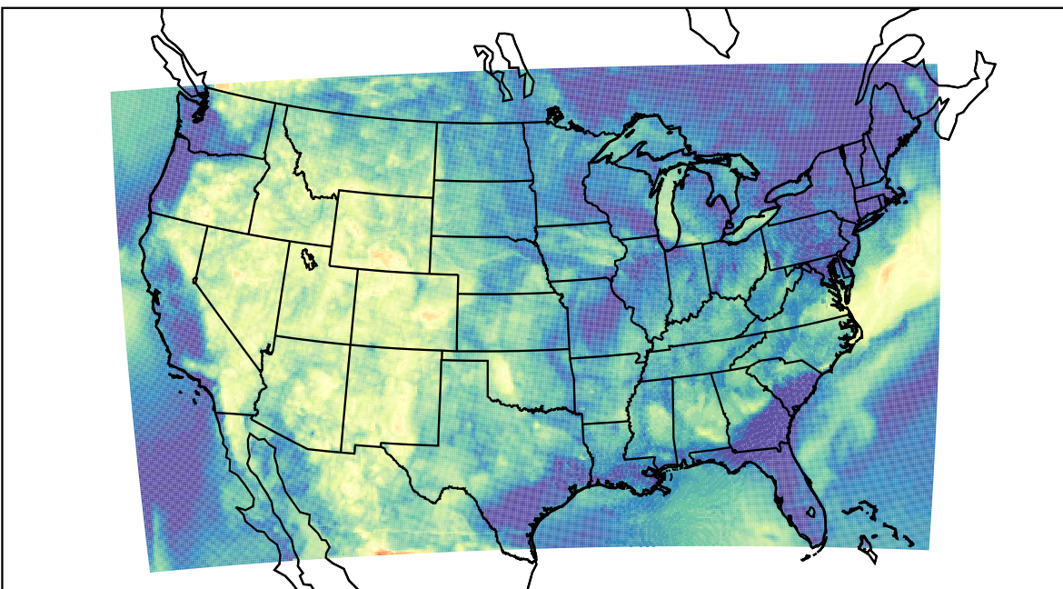
WRF (2021-06-23_06:00:00)
