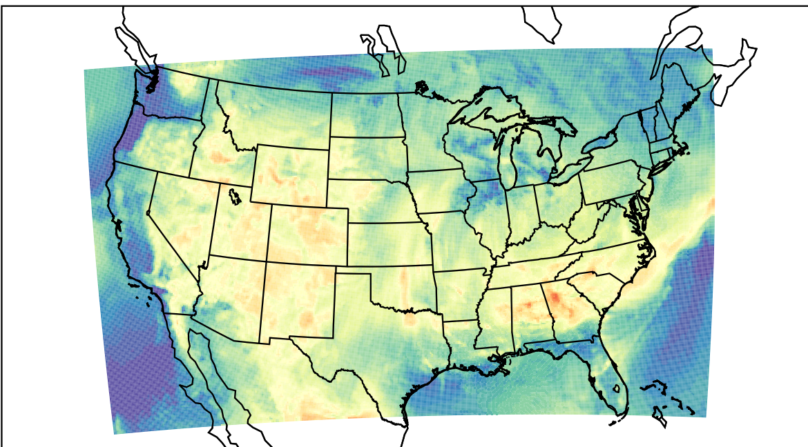
WRF (2021-06-23_16:00:00)
