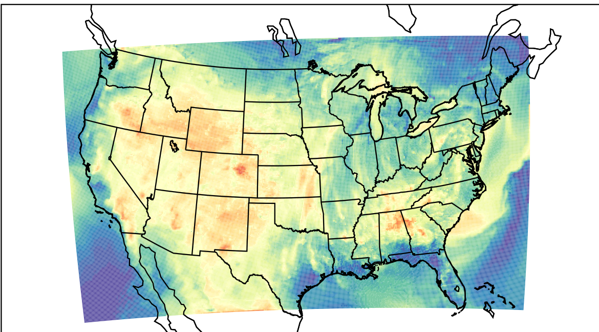
WRF (2021-06-24_01:00:00)
