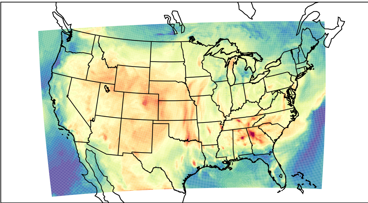
WRF (2021-06-23_20:00:00)
