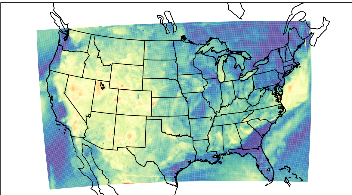
WRF (2021-06-23_03:00:00)
