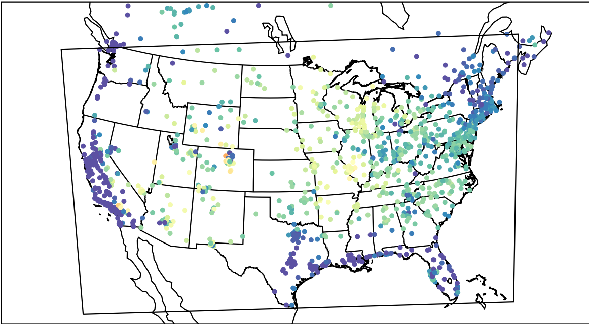
AirNOW (2021-06-23_14:00:00)
