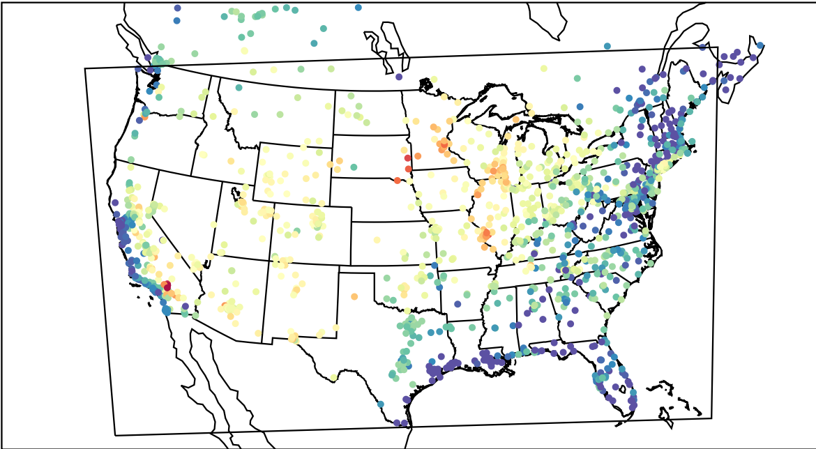
AirNOW (2021-06-24_01:00:00)
