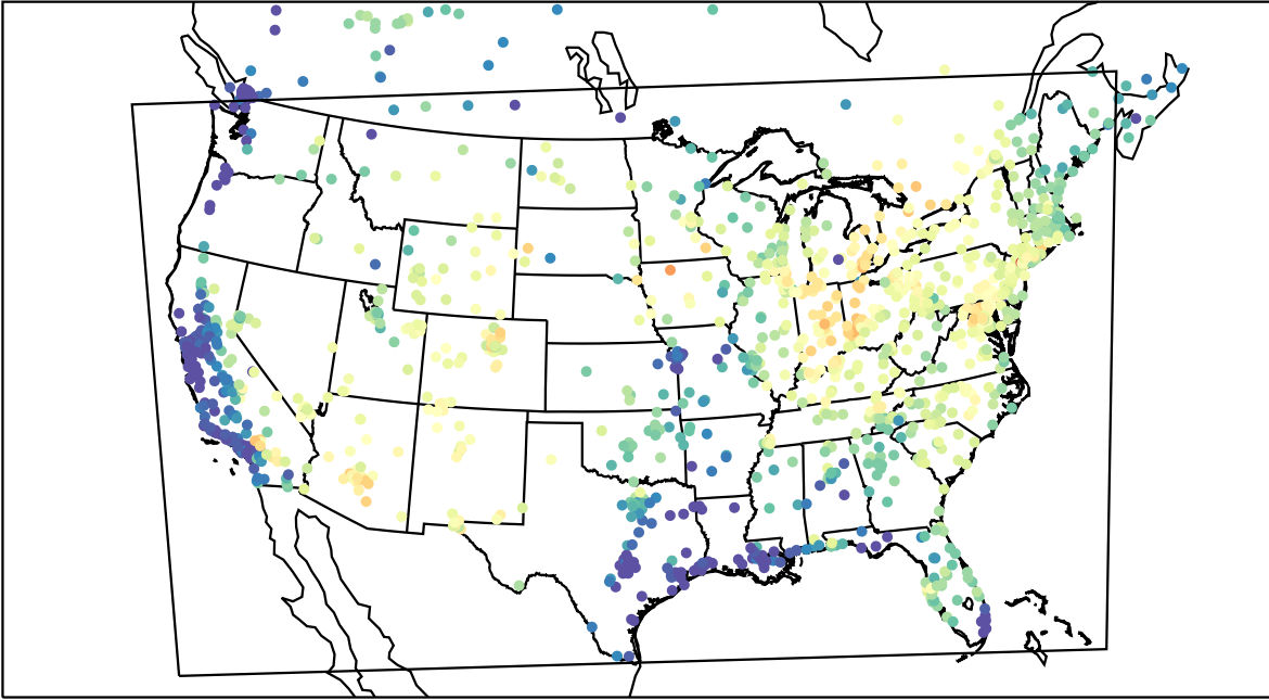
AirNOW (2021-06-24_16:00:00)
