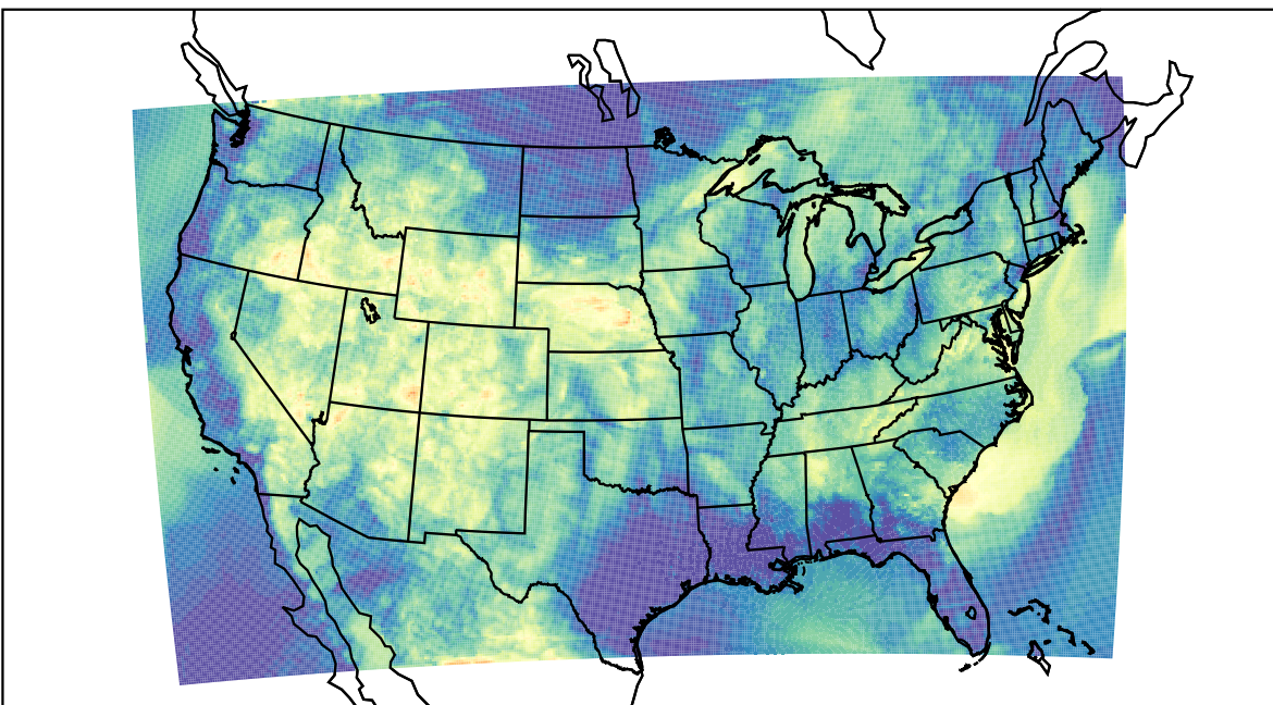
WRF (2021-06-24_08:00:00)
