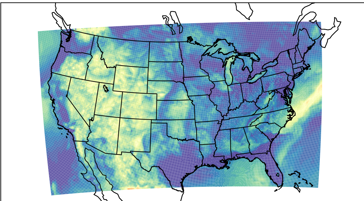
WRF (2021-06-23_12:00:00)
