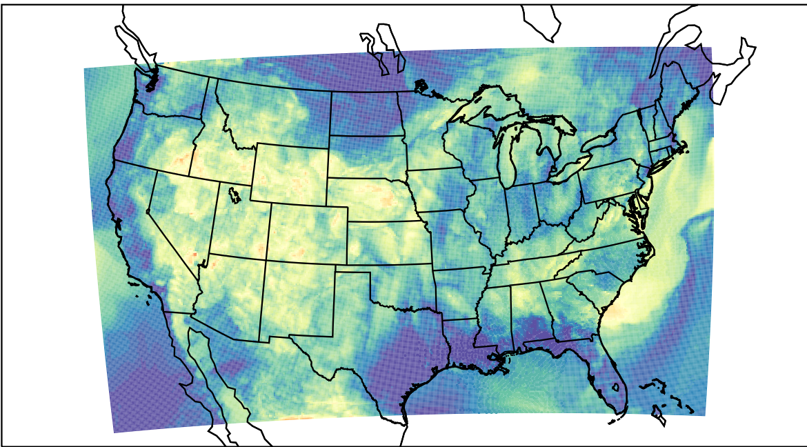
WRF (2021-06-24_07:00:00)
