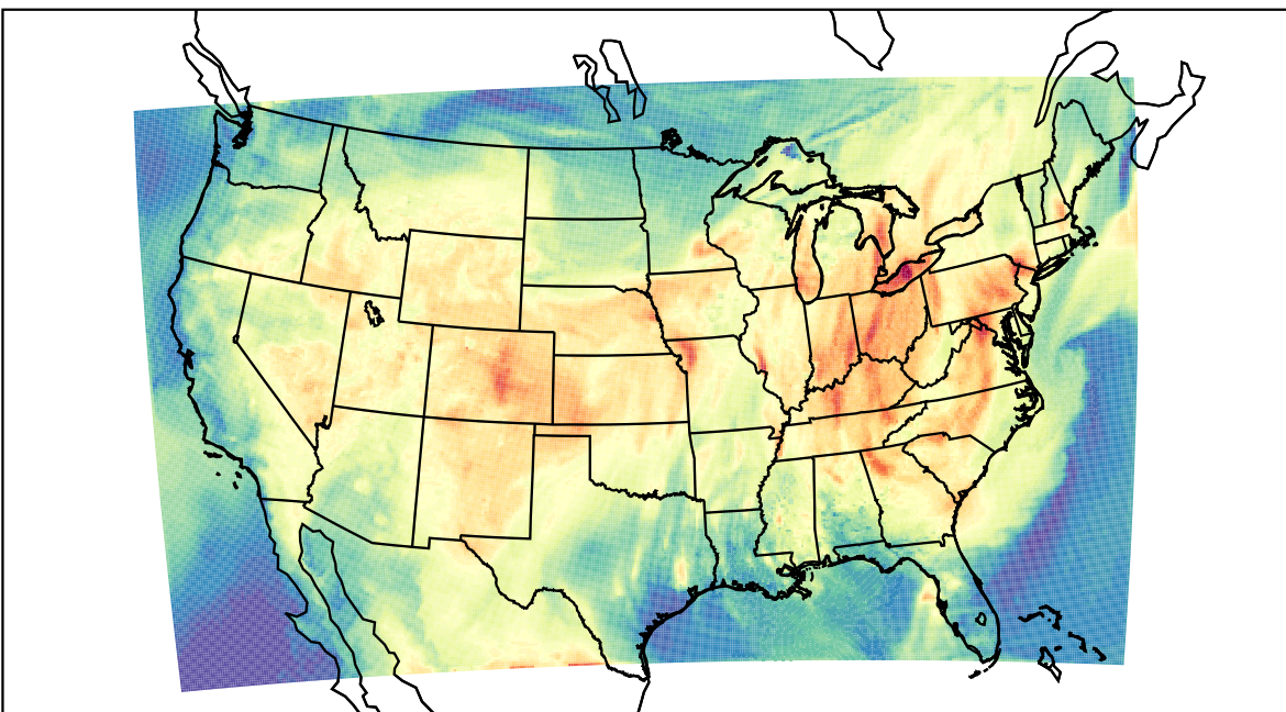
WRF (2021-06-24_18:00:00)
