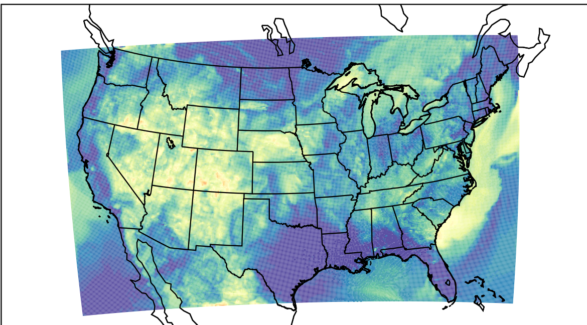
WRF (2021-06-24_11:00:00)
