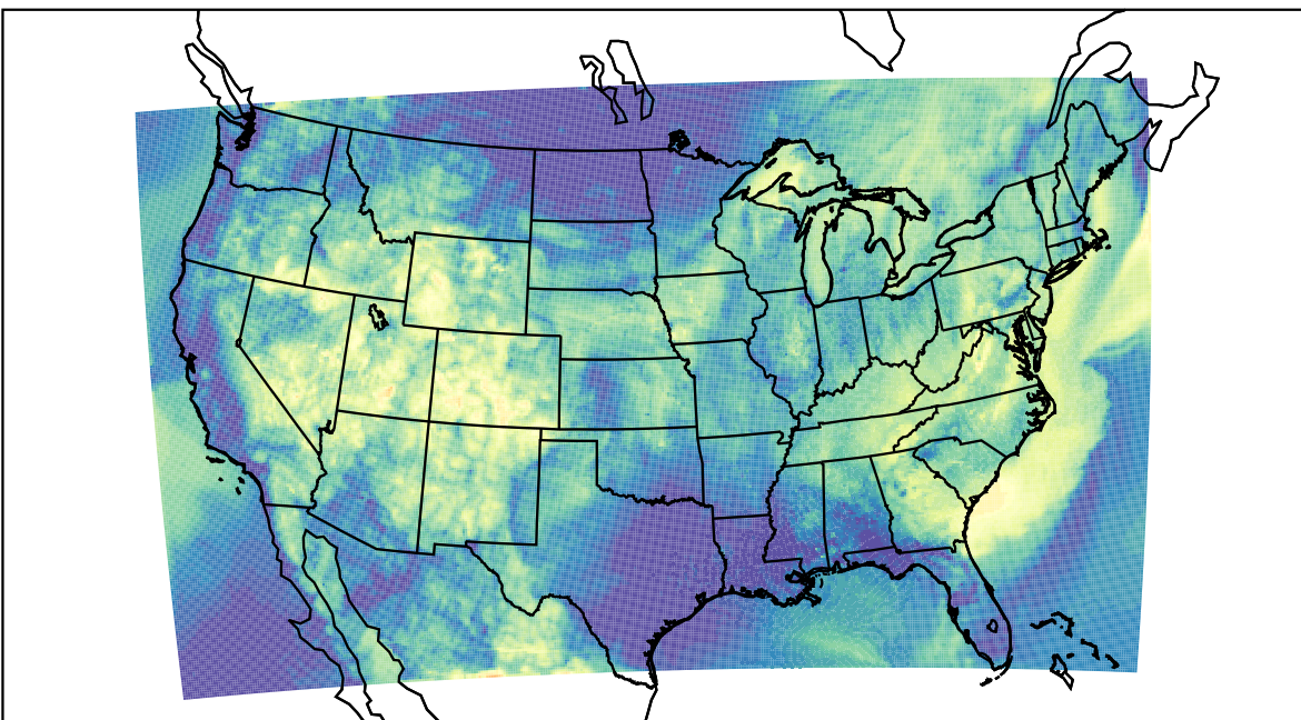
WRF (2021-06-24_13:00:00)
