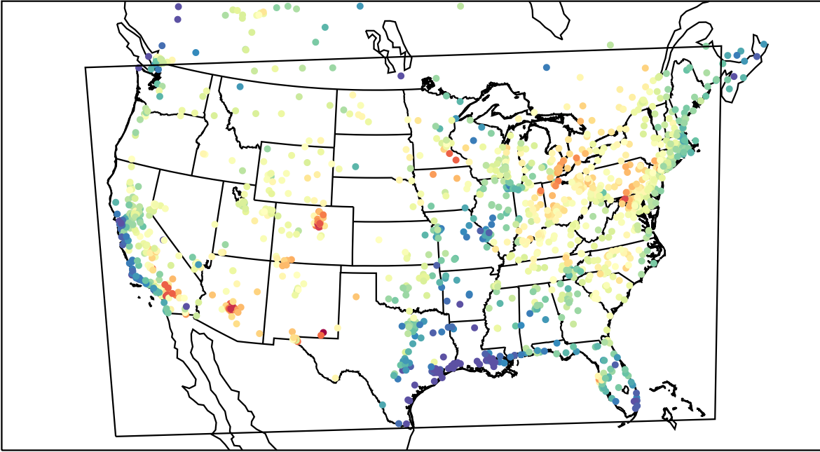
AirNOW (2021-06-24_21:00:00)
