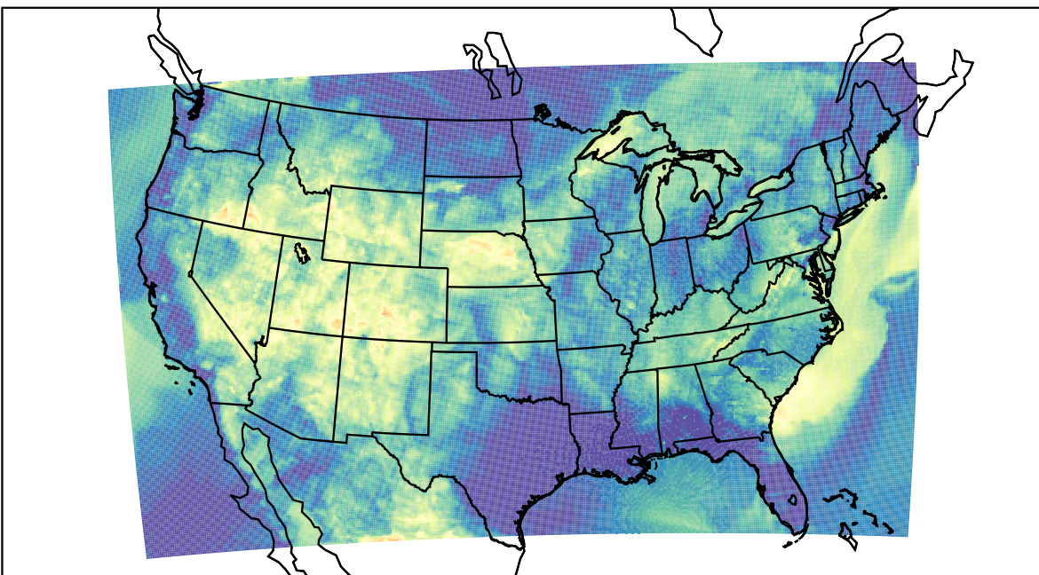
WRF (2021-06-24_10:00:00)
