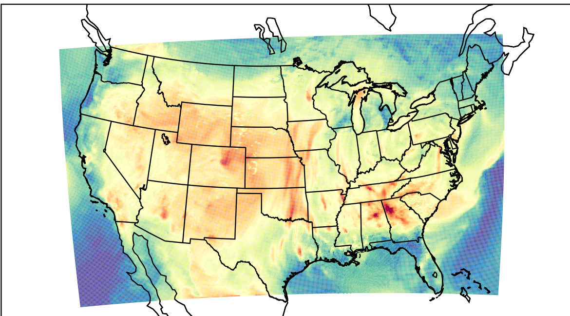
WRF (2021-06-23_22:00:00)
