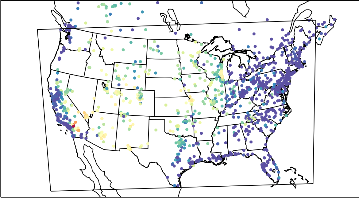
AirNOW (2021-06-23_05:00:00)
