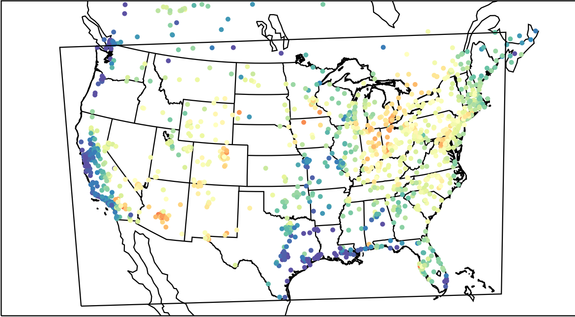
AirNOW (2021-06-24_17:00:00)
