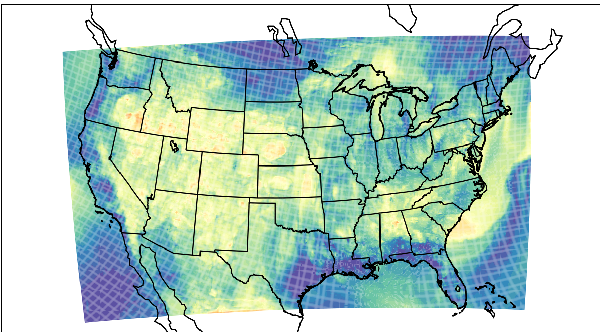
WRF (2021-06-24_04:00:00)
