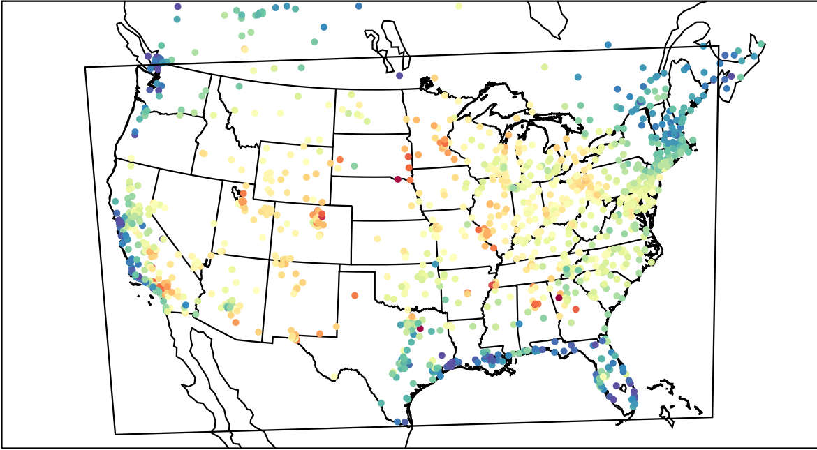
AirNOW (2021-06-23_20:00:00)
