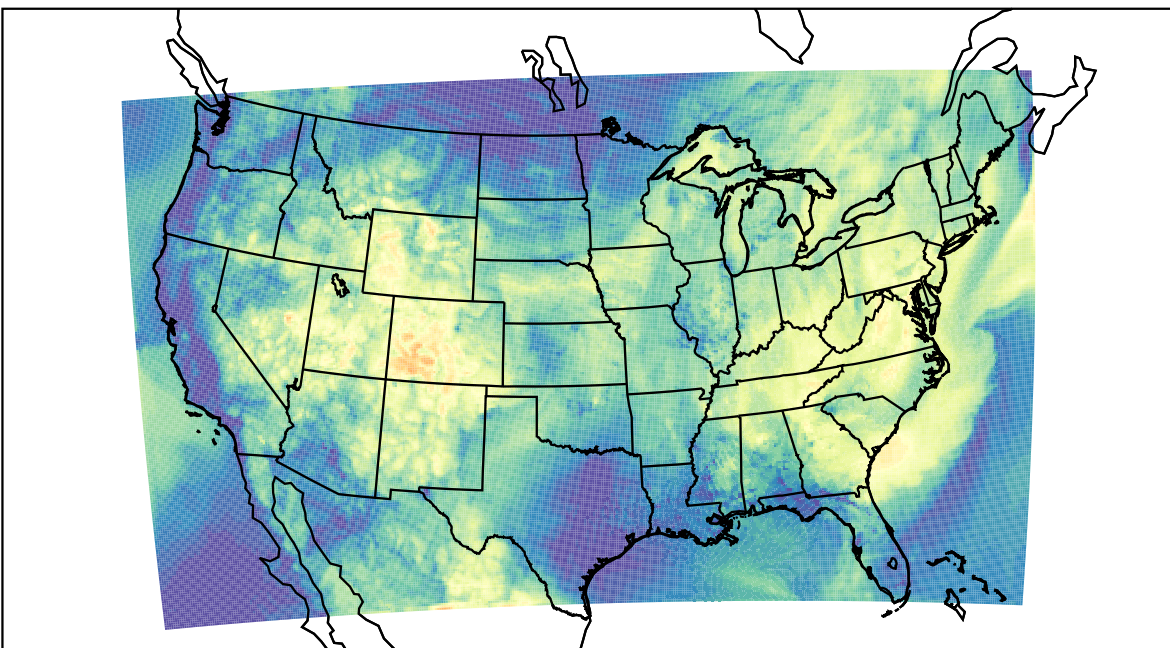
WRF (2021-06-24_14:00:00)
