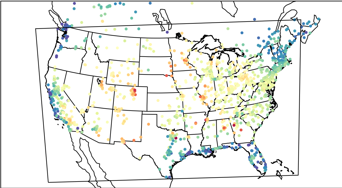
AirNOW (2021-06-23_19:00:00)
