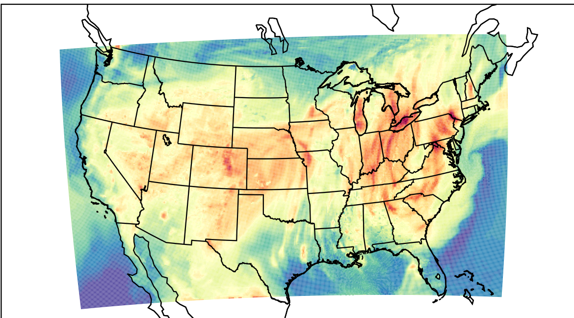
WRF (2021-06-24_21:00:00)
