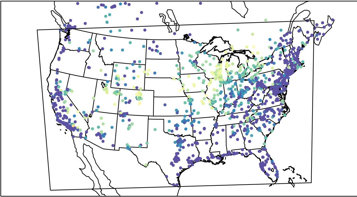
AirNOW (2021-06-24_11:00:00)
