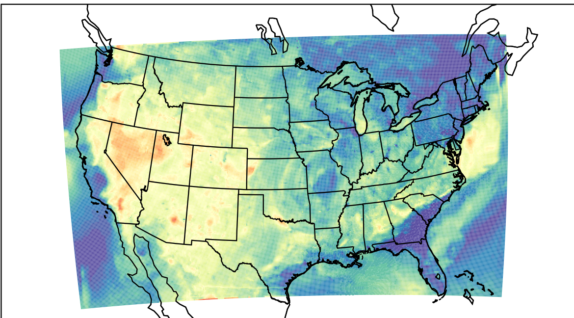
WRF (2021-06-23_02:00:00)
