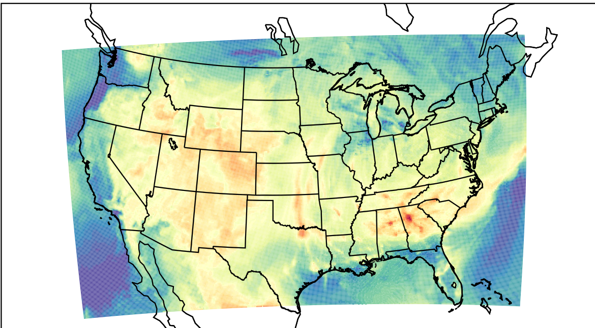
WRF (2021-06-23_17:00:00)
