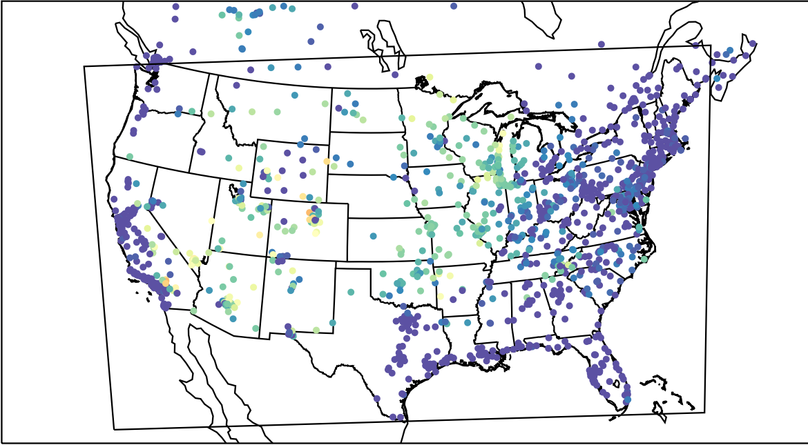
AirNOW (2021-06-23_12:00:00)
