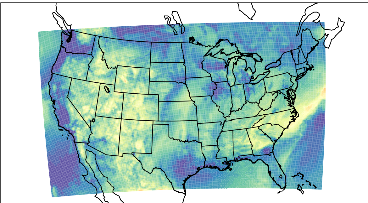
WRF (2021-06-23_14:00:00)
