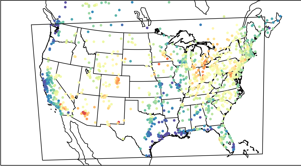
AirNOW (2021-06-24_18:00:00)
