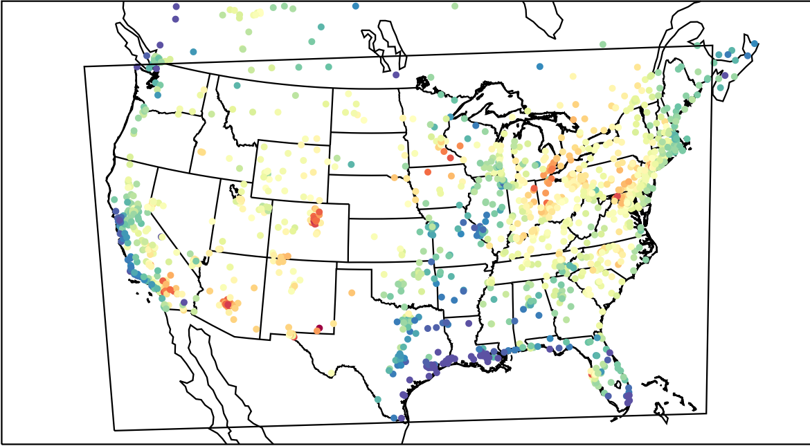
AirNOW (2021-06-24_20:00:00)
