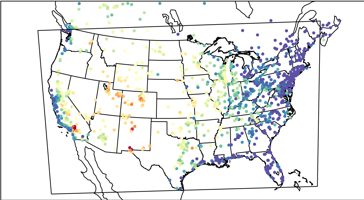
AirNOW (2021-06-23_01:00:00)
