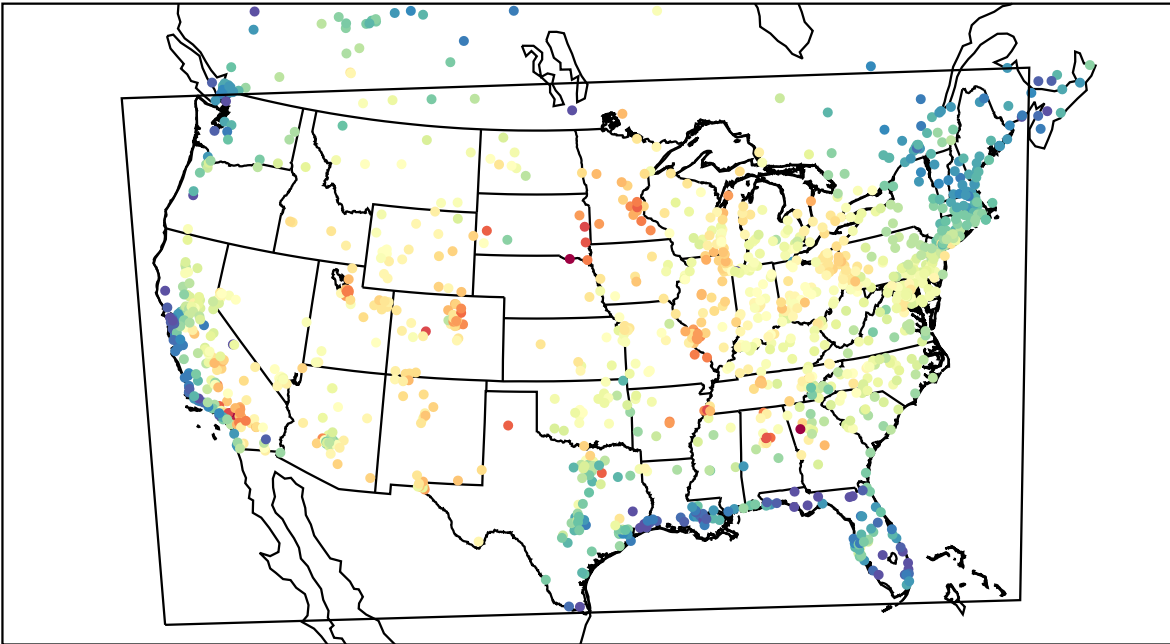
AirNOW (2021-06-23_21:00:00)
