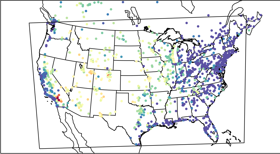
AirNOW (2021-06-23_03:00:00)
