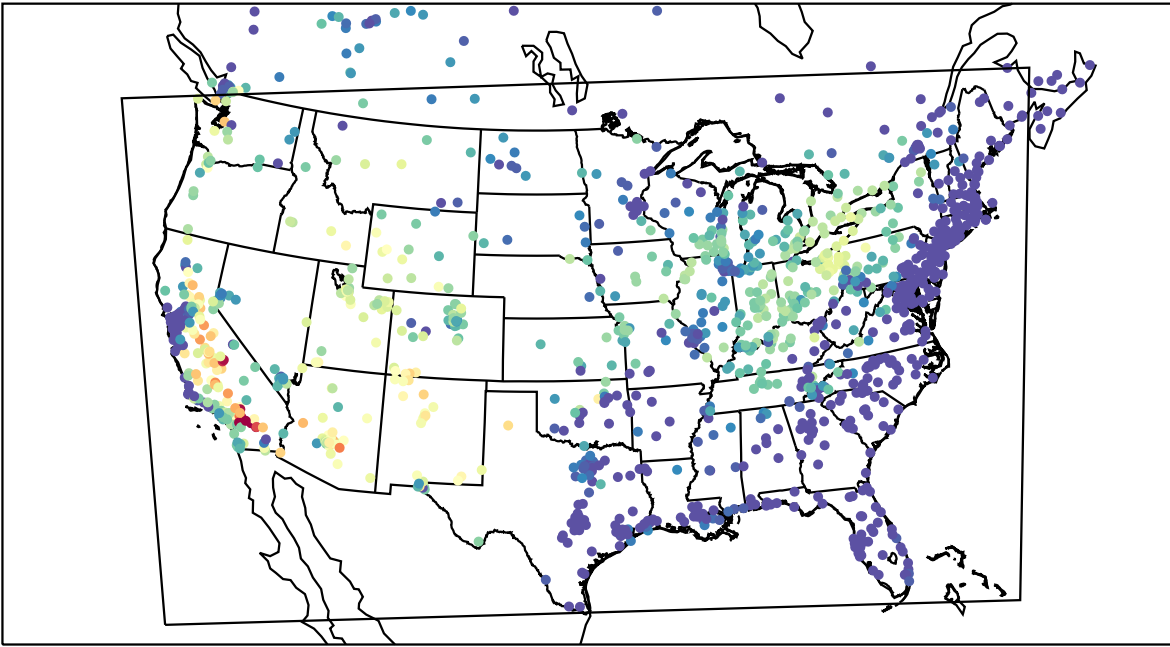
AirNOW (2021-06-27_03:00:00)
