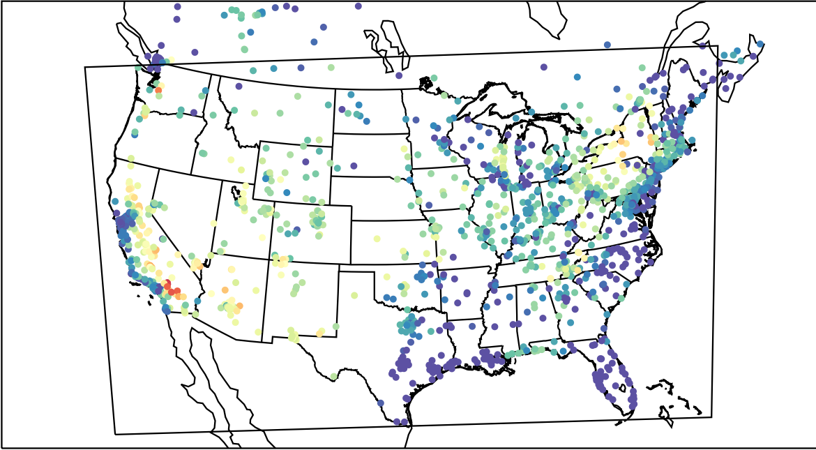
AirNOW (2021-06-26_03:00:00)
