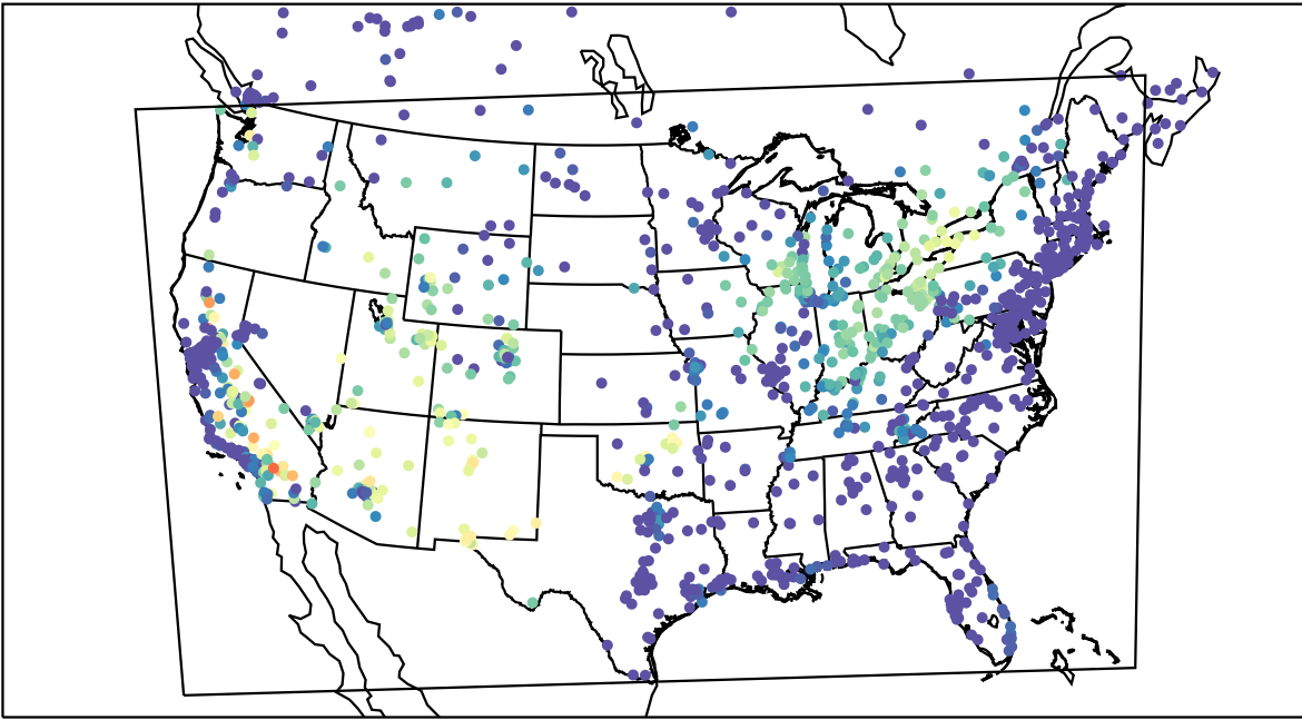
AirNOW (2021-06-27_07:00:00)
