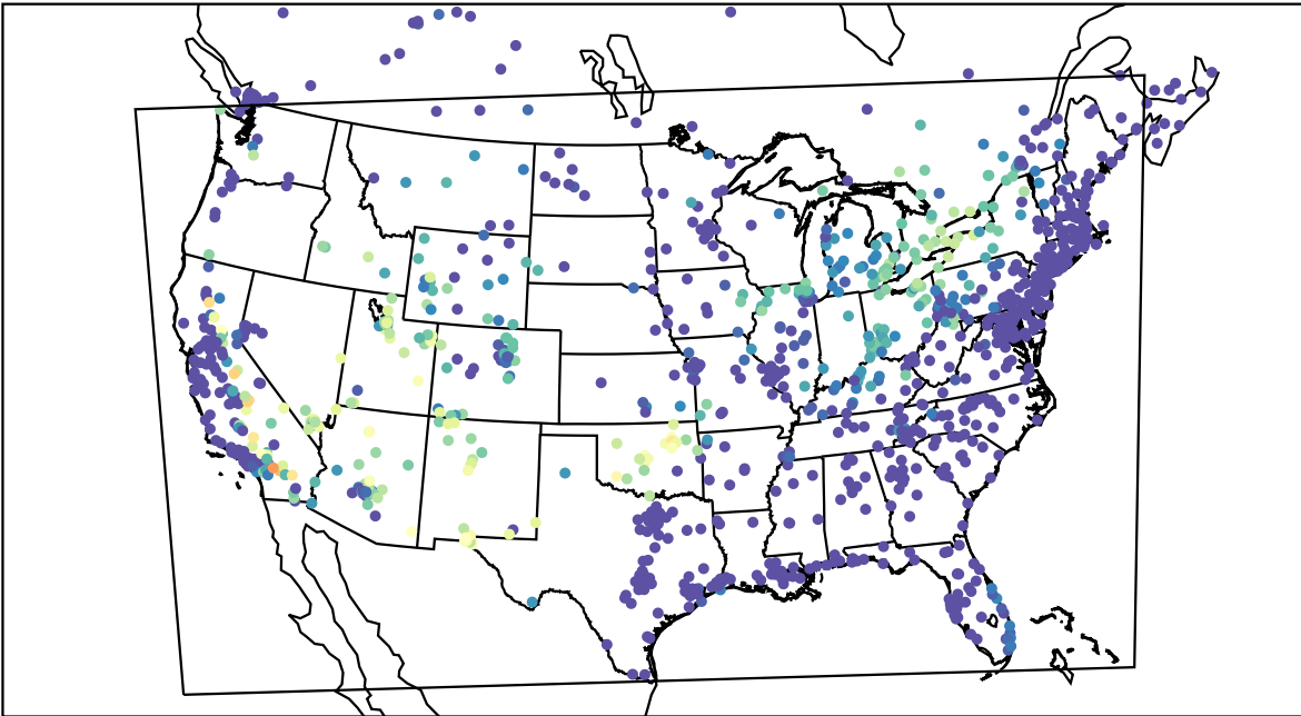
AirNOW (2021-06-27_10:00:00)
