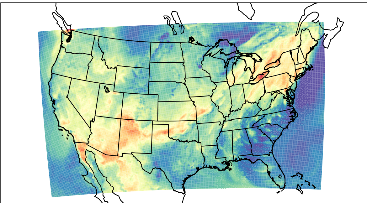
WRF (2021-06-27_17:00:00)
