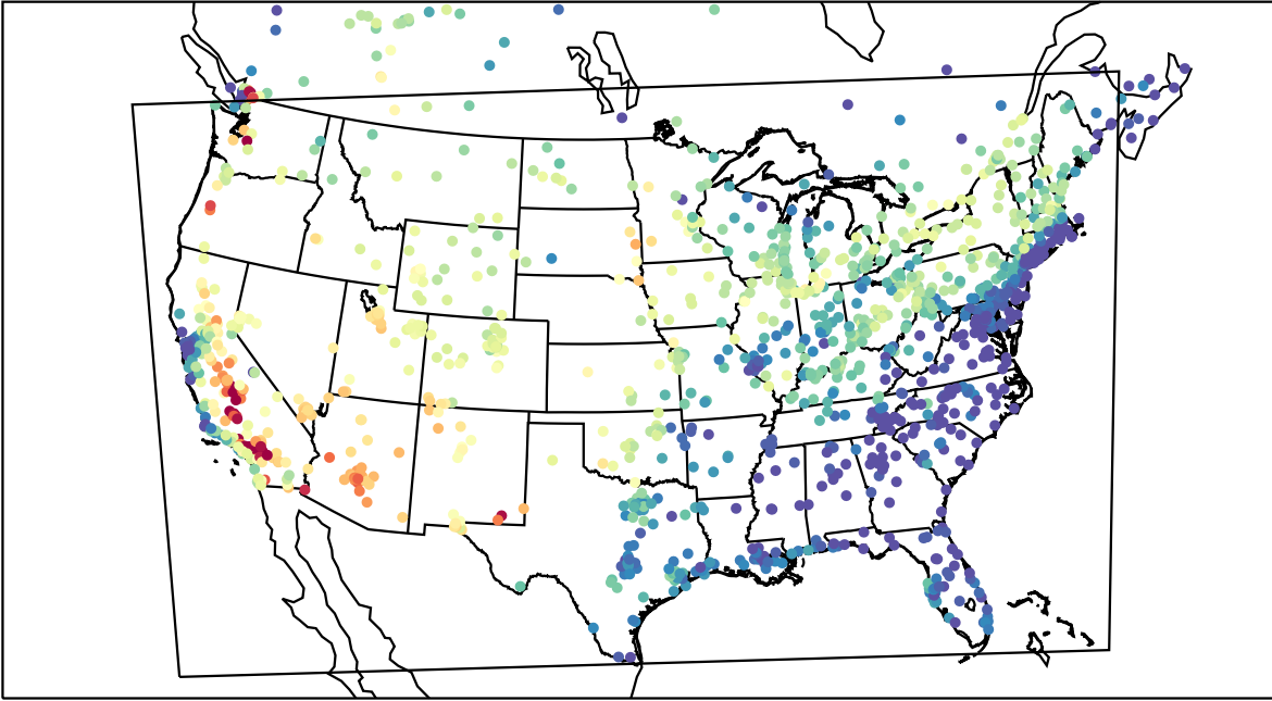
AirNOW (2021-06-27_23:00:00)
