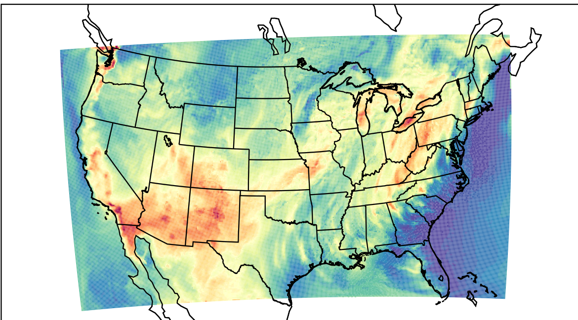
WRF (2021-06-26_21:00:00)
