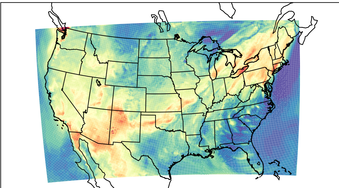
WRF (2021-06-27_18:00:00)
