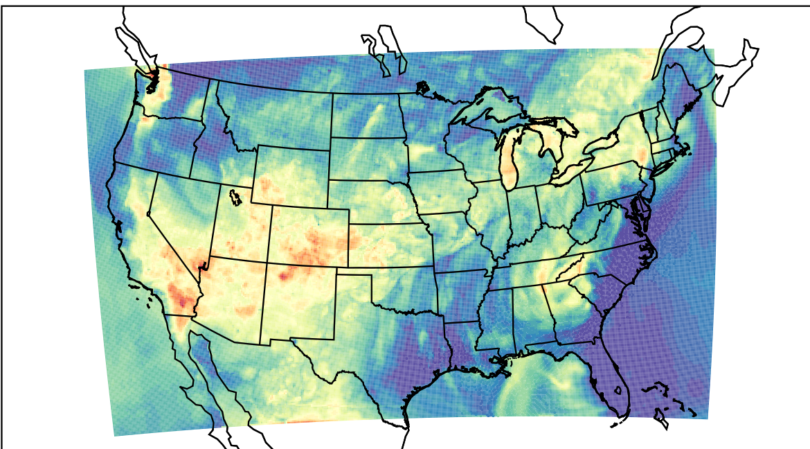
WRF (2021-06-26_03:00:00)
