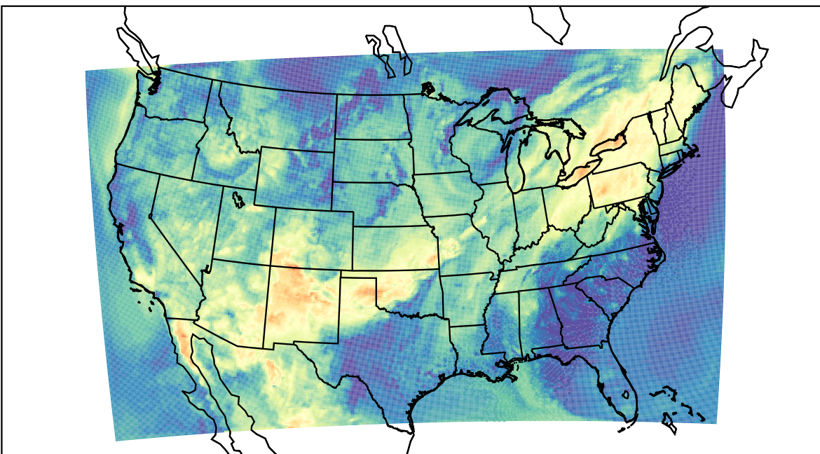
WRF (2021-06-27_15:00:00)
