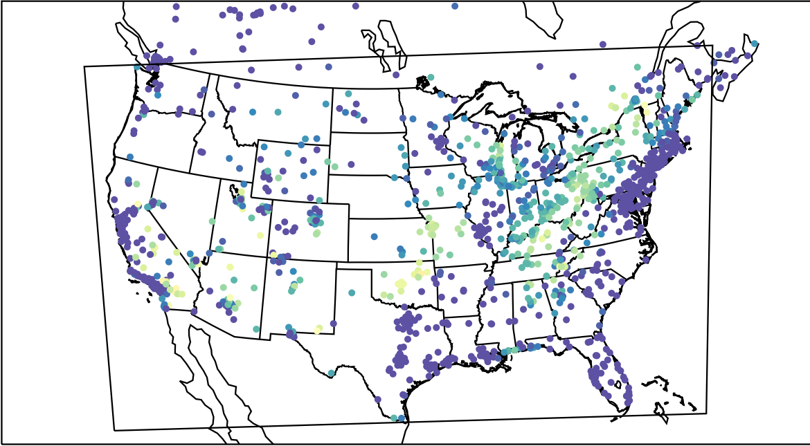
AirNOW (2021-06-26_12:00:00)
