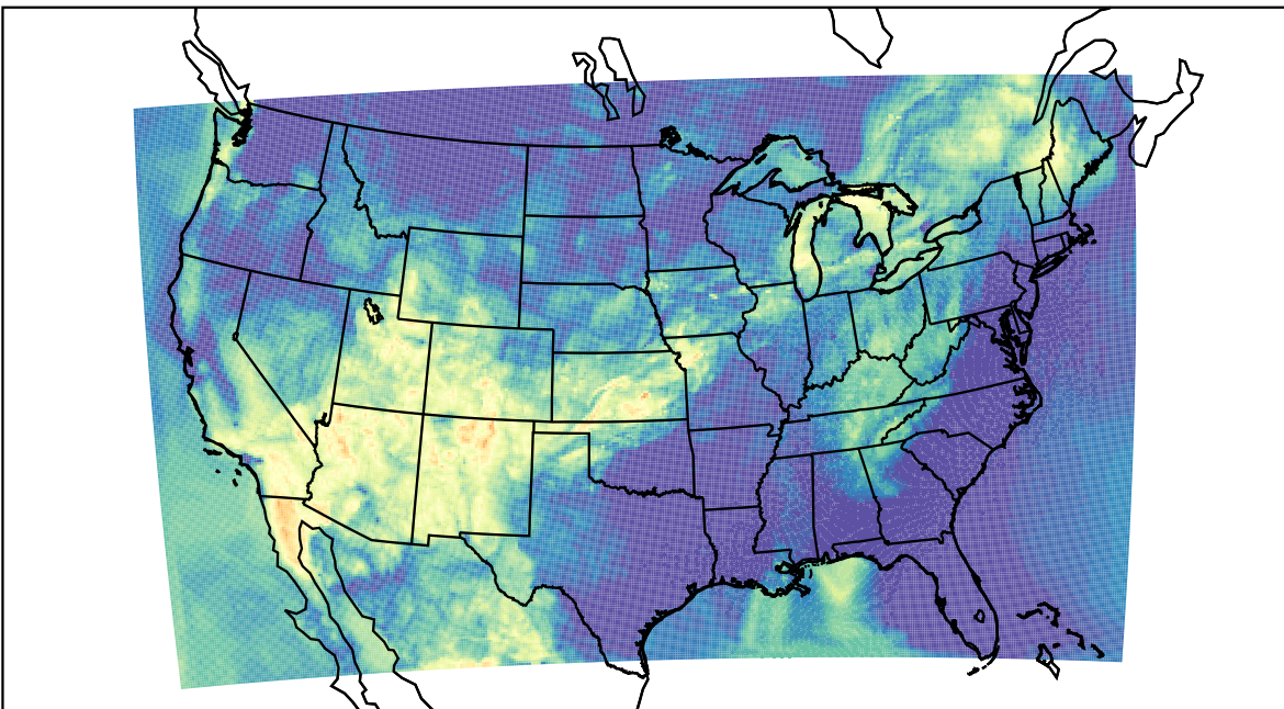
WRF (2021-06-26_12:00:00)
