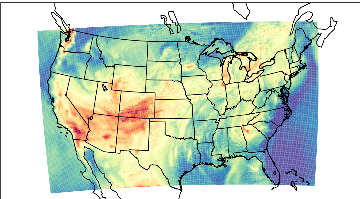
WRF (2021-06-26_00:00:00)
