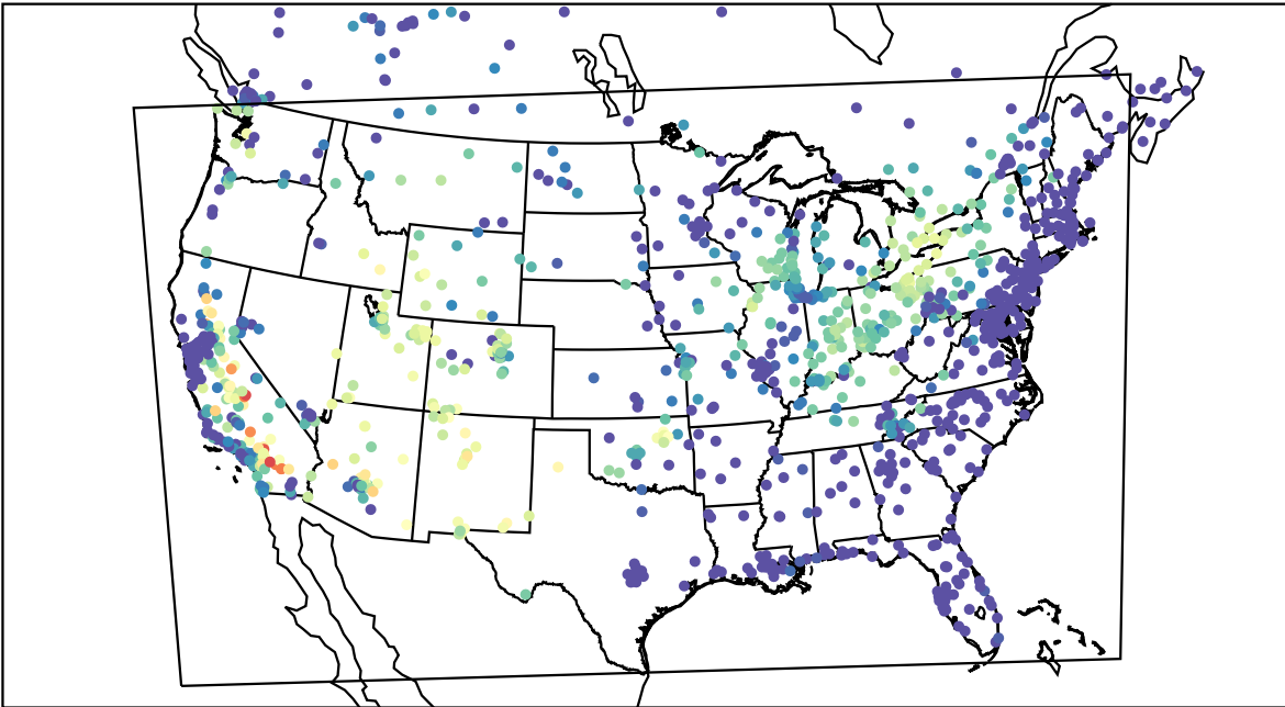
AirNOW (2021-06-27_05:00:00)
