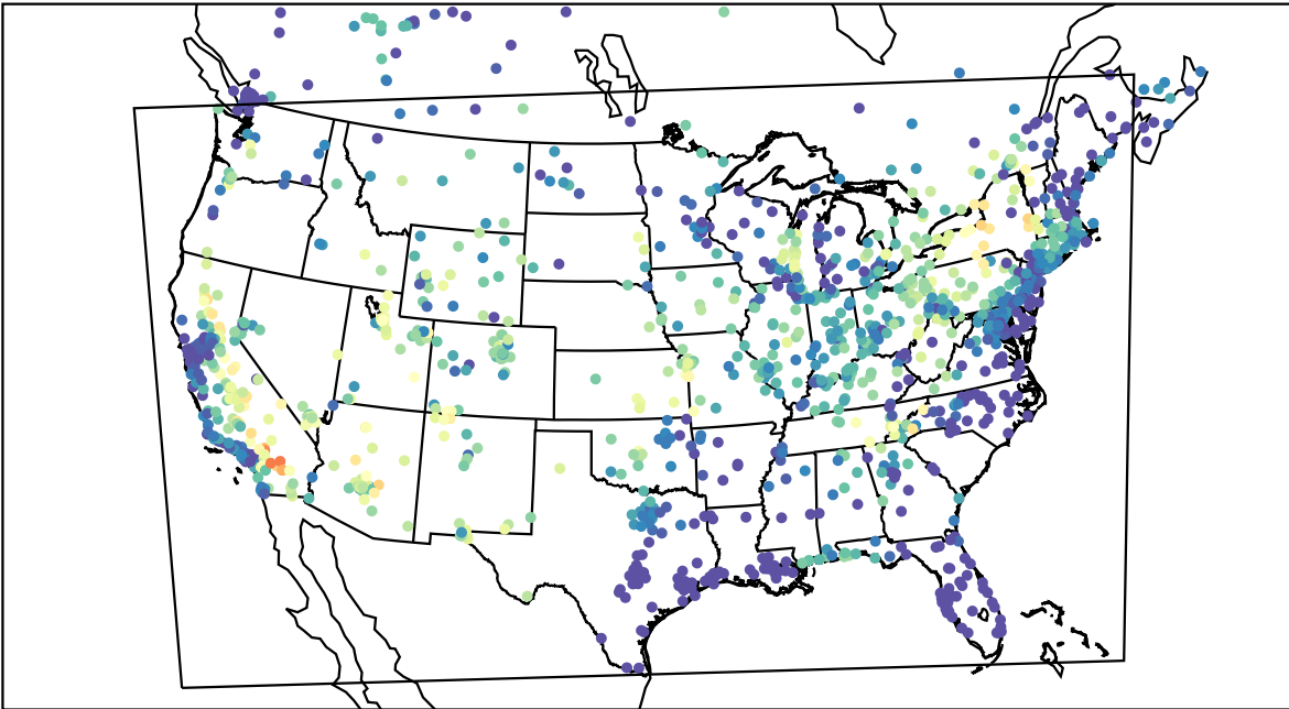
AirNOW (2021-06-26_04:00:00)
