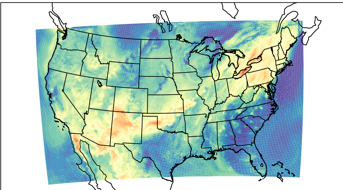
WRF (2021-06-27_16:00:00)
