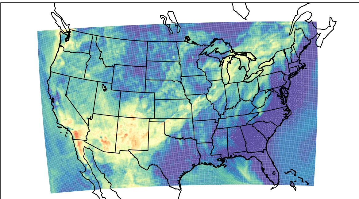
WRF (2021-06-27_06:00:00)
