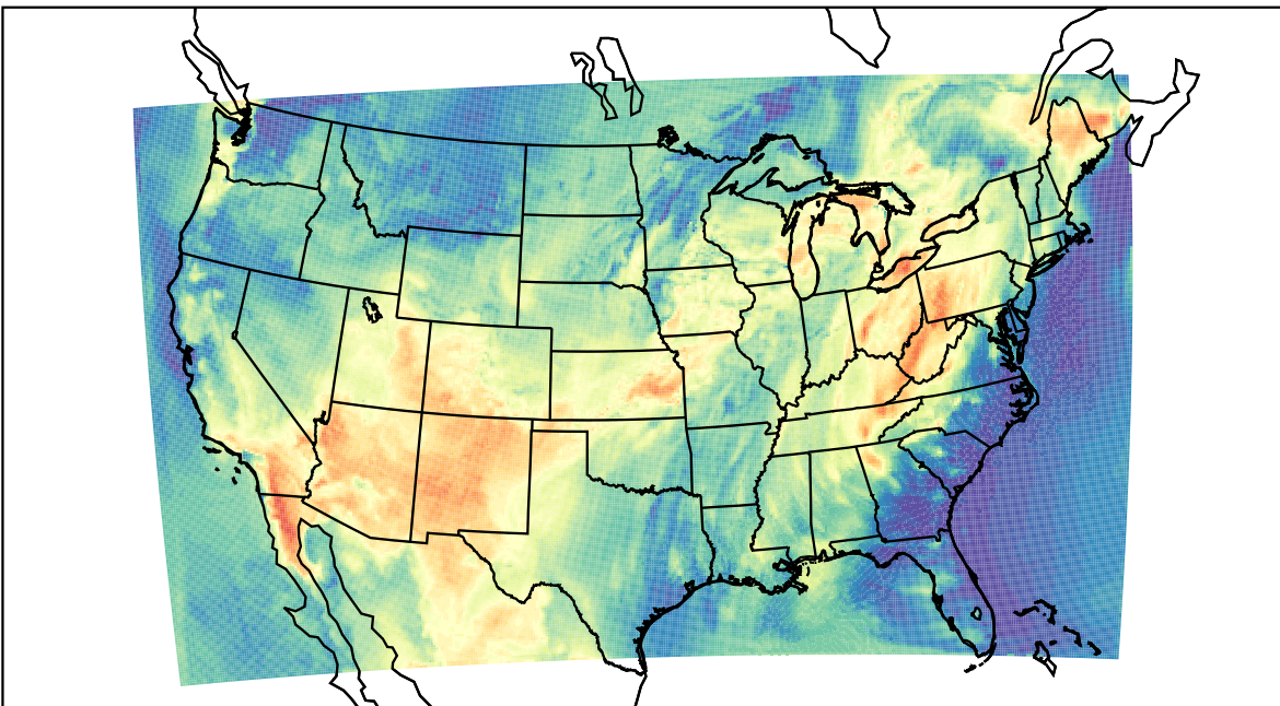
WRF (2021-06-26_17:00:00)
