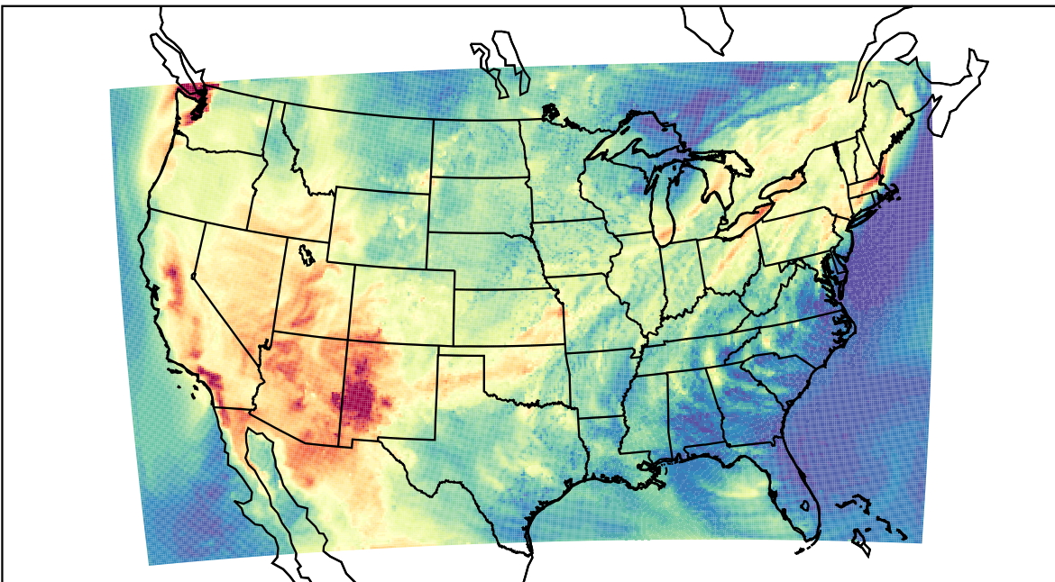
WRF (2021-06-27_23:00:00)
