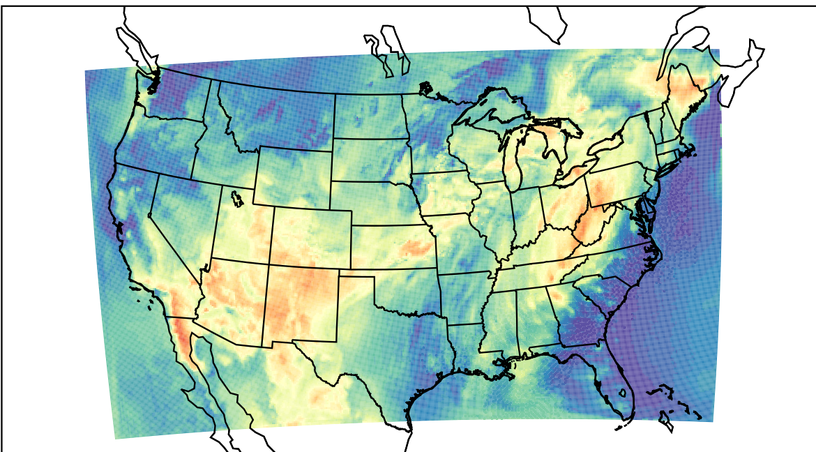
WRF (2021-06-26_16:00:00)
