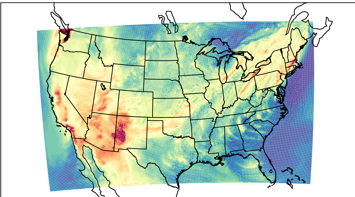
WRF (2021-06-27_22:00:00)
