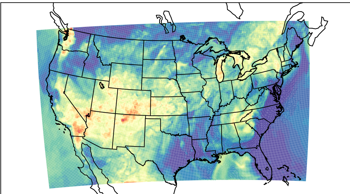
WRF (2021-06-26_04:00:00)
