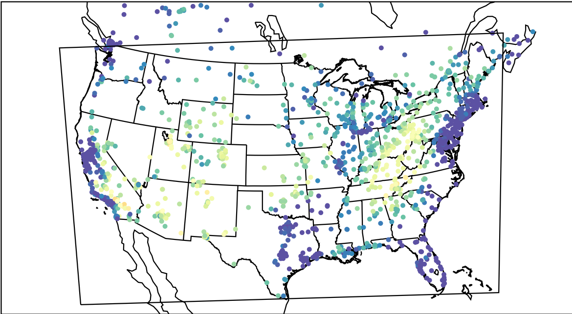
AirNOW (2021-06-26_15:00:00)
