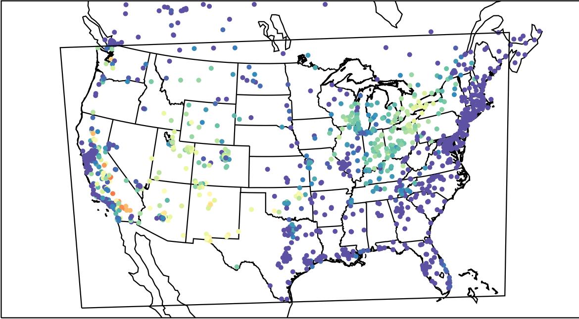
AirNOW (2021-06-27_06:00:00)
