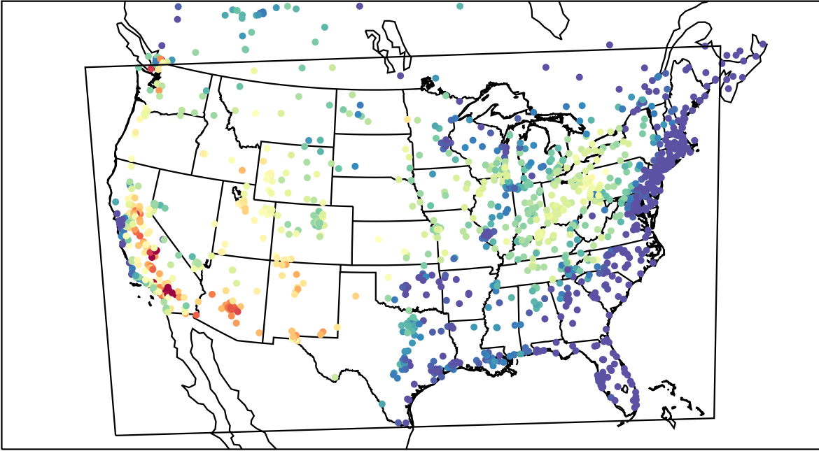
AirNOW (2021-06-27_00:00:00)
