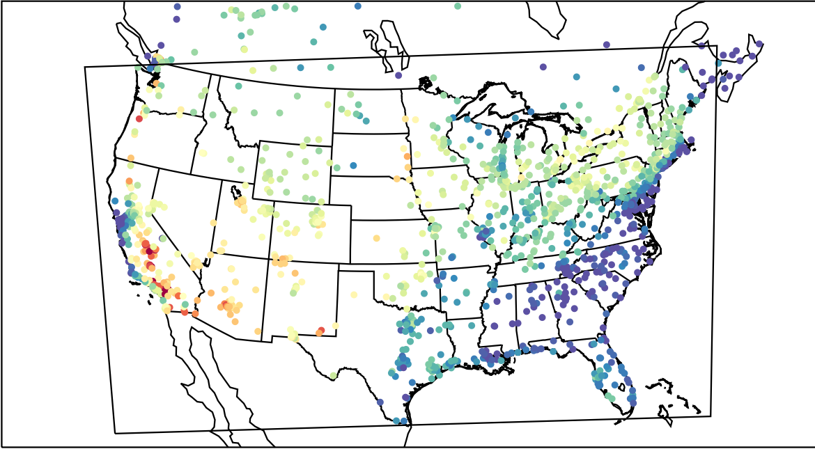
AirNOW (2021-06-27_19:00:00)
