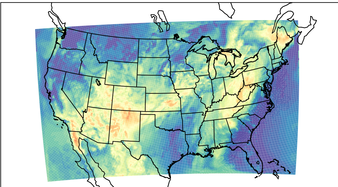
WRF (2021-06-26_15:00:00)
