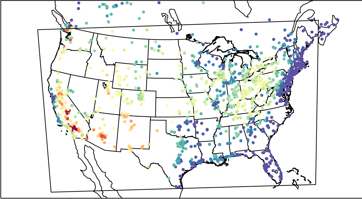
AirNOW (2021-06-26_23:00:00)
