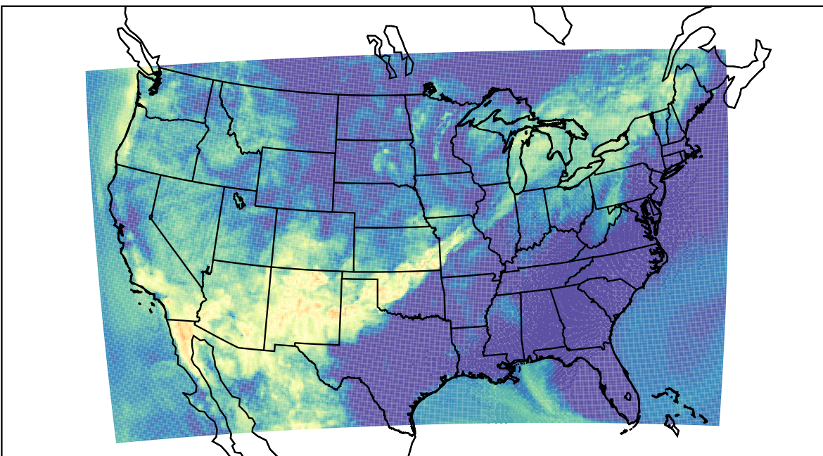
WRF (2021-06-27_11:00:00)
