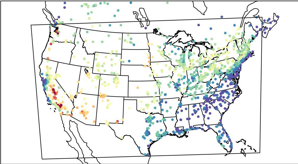
AirNOW (2021-06-27_20:00:00)
