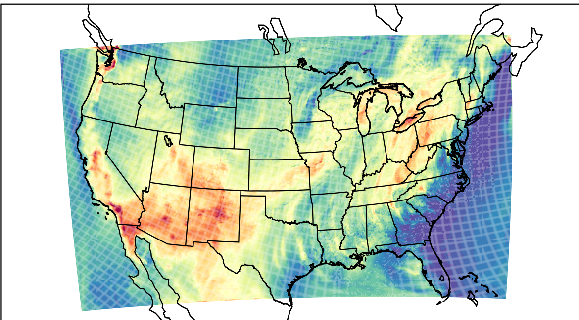
WRF (2021-06-26_22:00:00)
