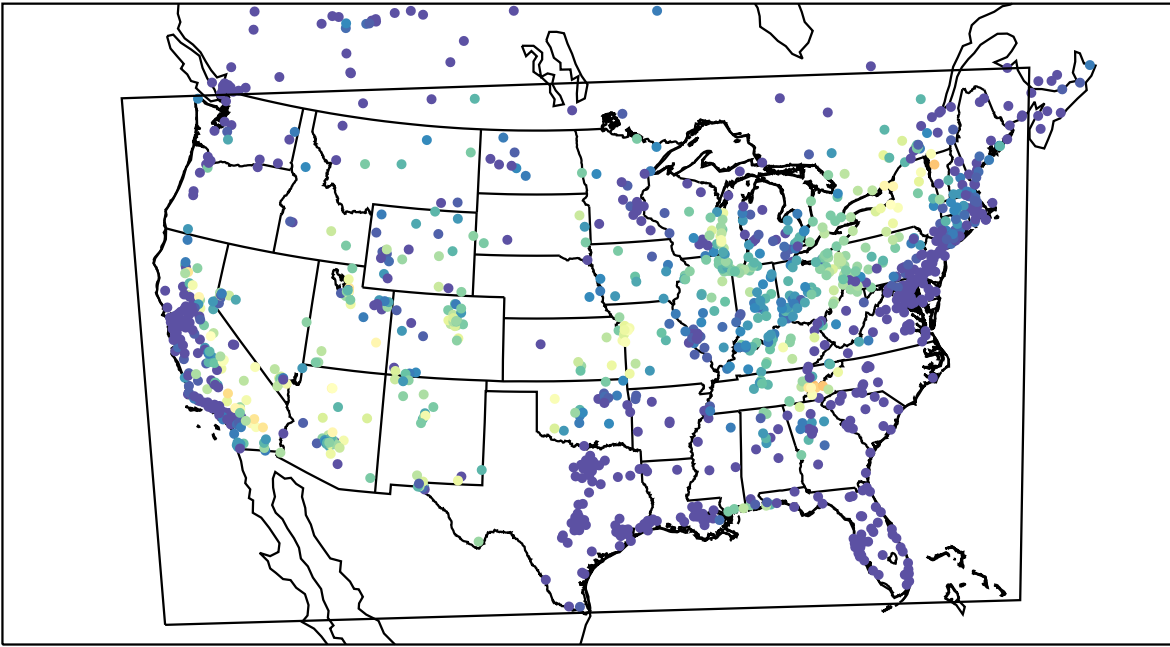
AirNOW (2021-06-26_08:00:00)
