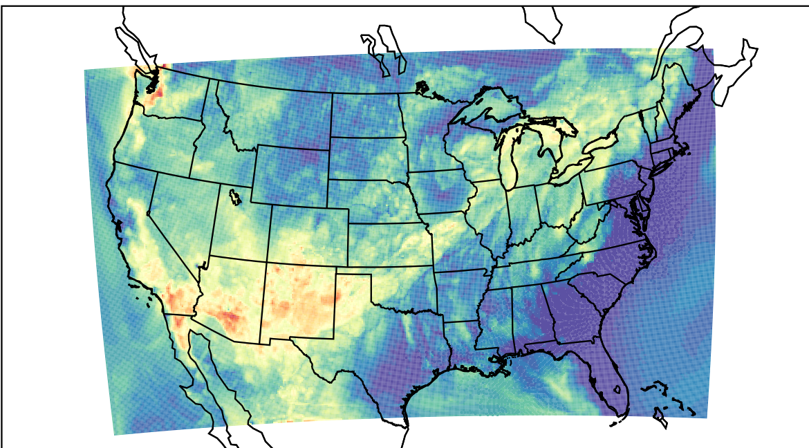
WRF (2021-06-27_04:00:00)
