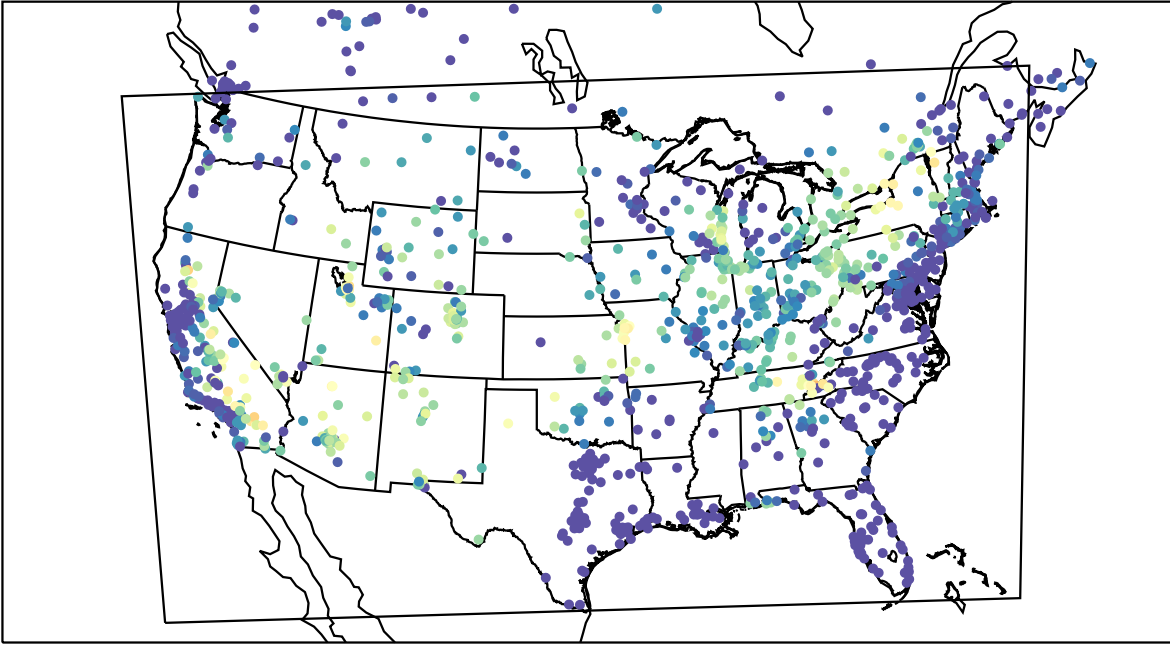
AirNOW (2021-06-26_07:00:00)
