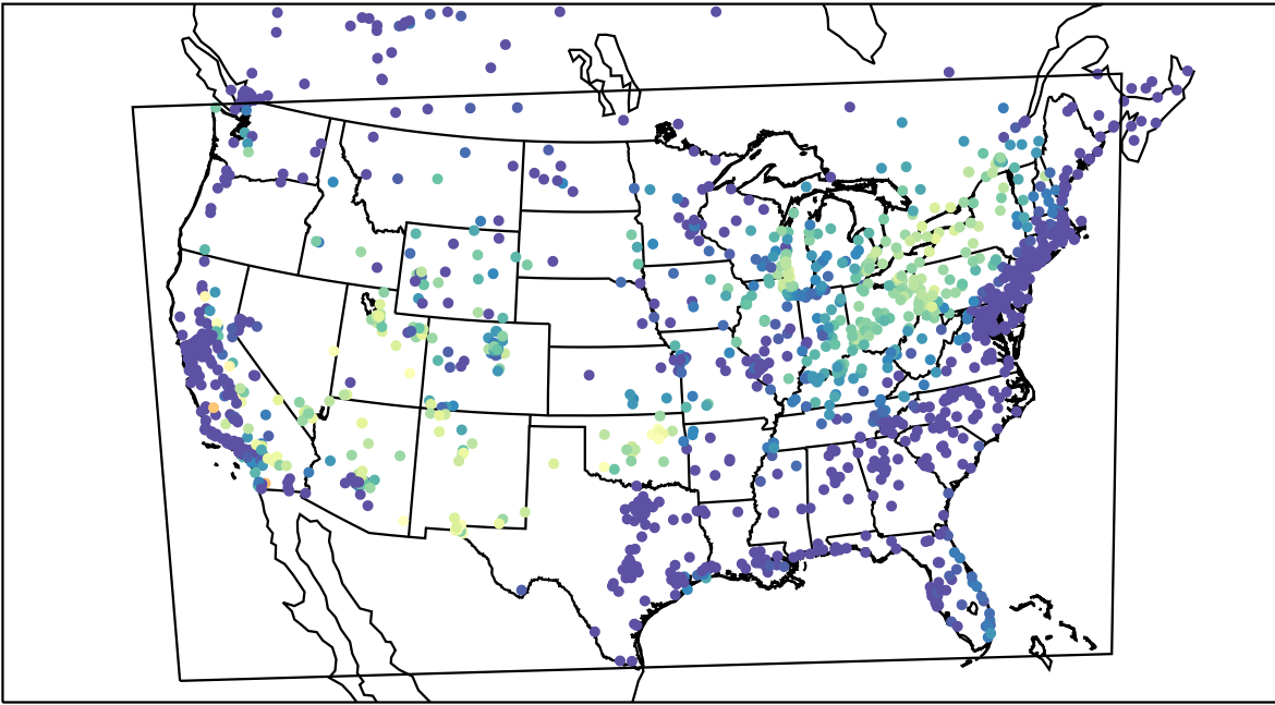
AirNOW (2021-06-27_13:00:00)
