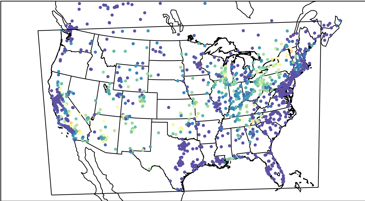
AirNOW (2021-06-26_09:00:00)
