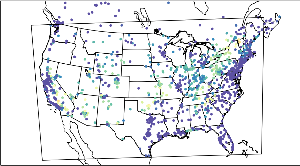
AirNOW (2021-06-26_10:00:00)
