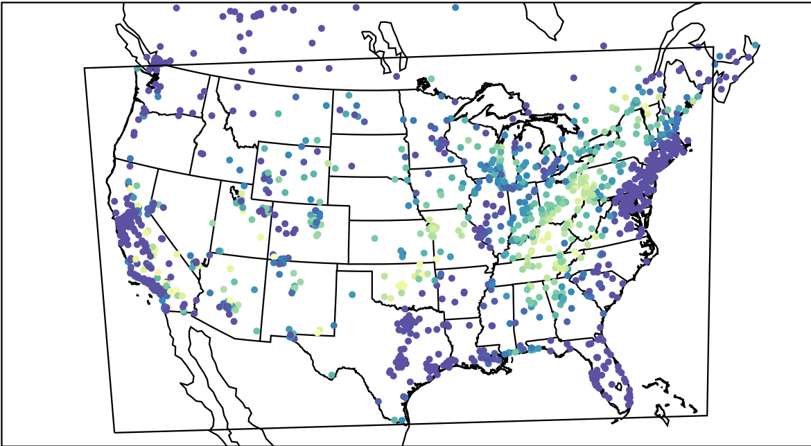
AirNOW (2021-06-26_13:00:00)
