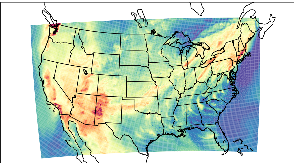
WRF (2021-06-27_21:00:00)
