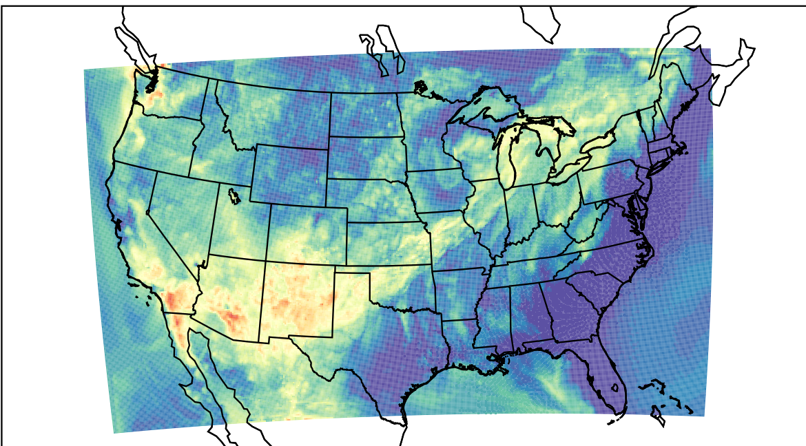
WRF (2021-06-27_05:00:00)
