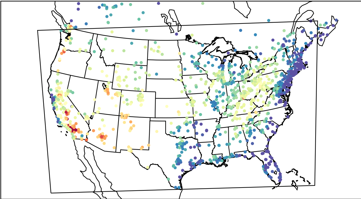
AirNOW (2021-06-26_20:00:00)
