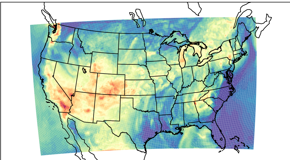
WRF (2021-06-26_02:00:00)
