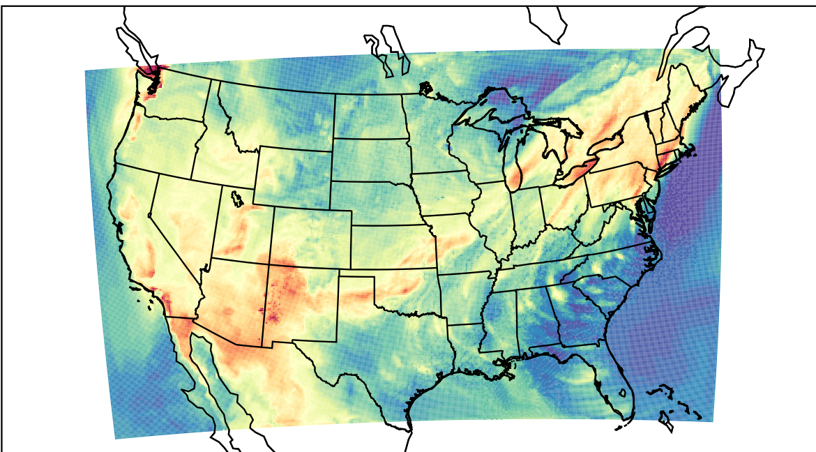
WRF (2021-06-27_19:00:00)
