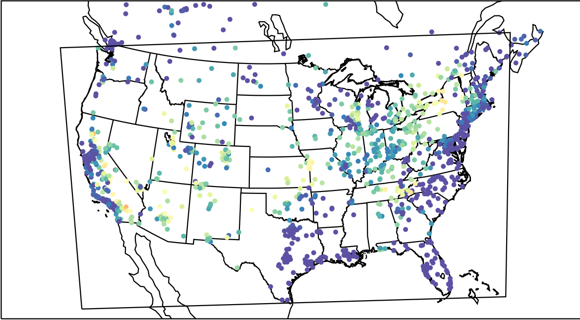
AirNOW (2021-06-26_06:00:00)
