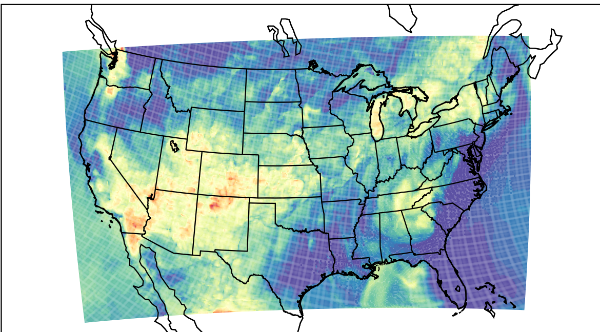
WRF (2021-06-26_05:00:00)
