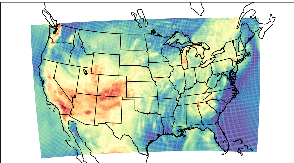
WRF (2021-06-26_01:00:00)
