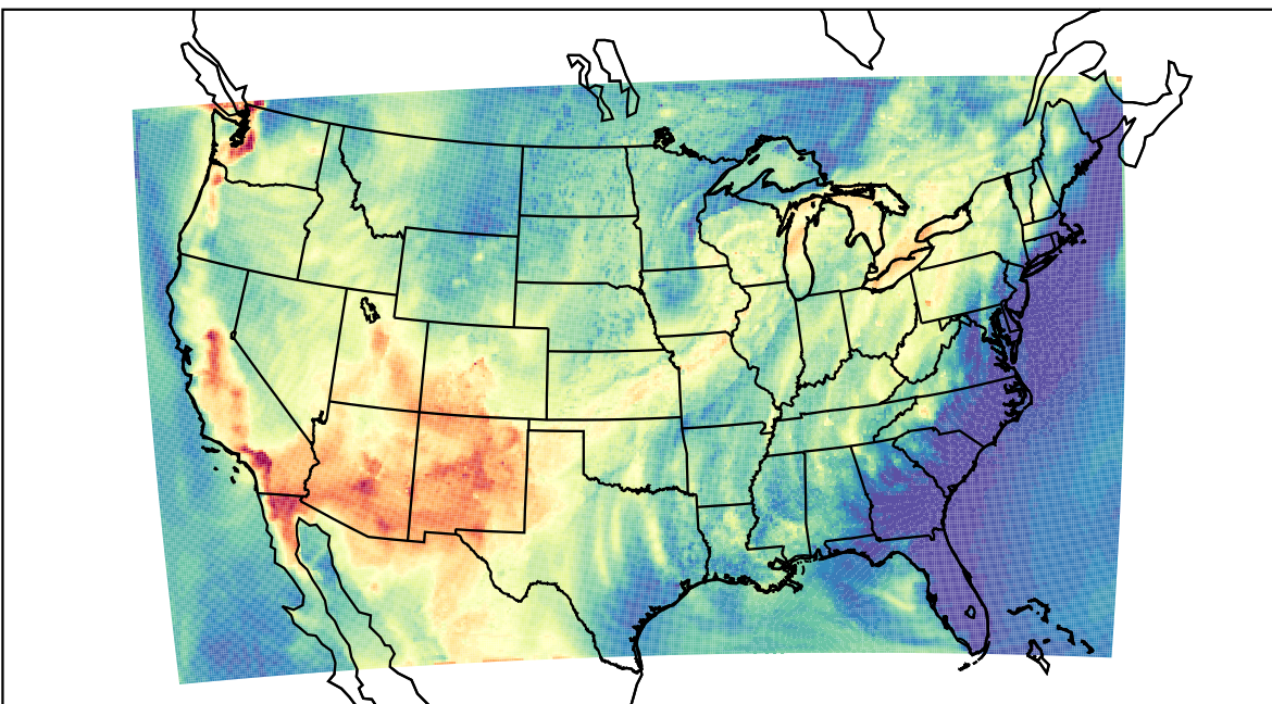
WRF (2021-06-27_00:00:00)
