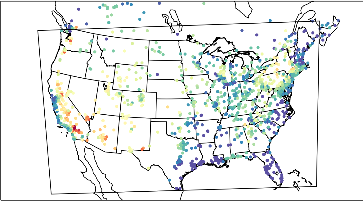
AirNOW (2021-06-26_01:00:00)
