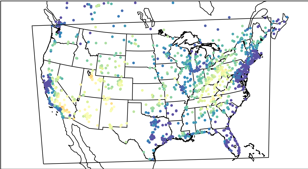
AirNOW (2021-06-26_16:00:00)
