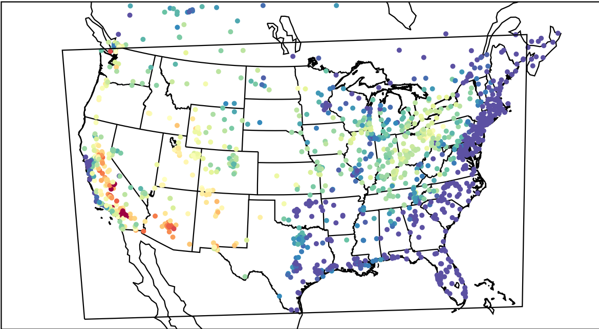
AirNOW (2021-06-27_01:00:00)
