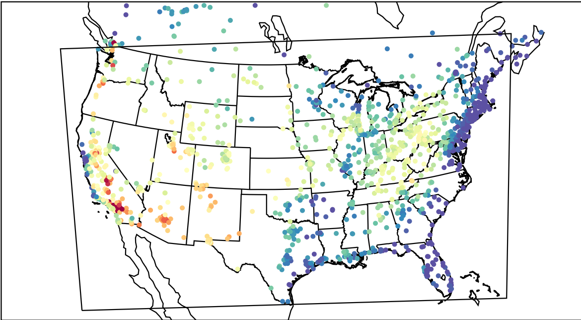
AirNOW (2021-06-26_21:00:00)
