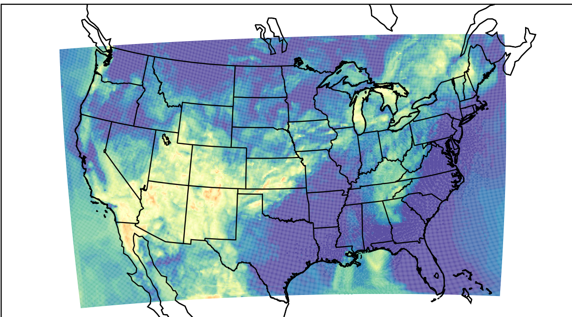
WRF (2021-06-26_11:00:00)
