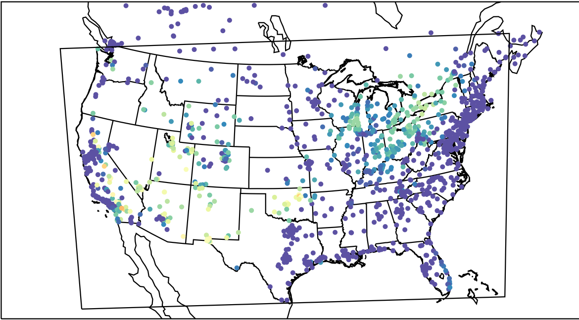
AirNOW (2021-06-27_11:00:00)
