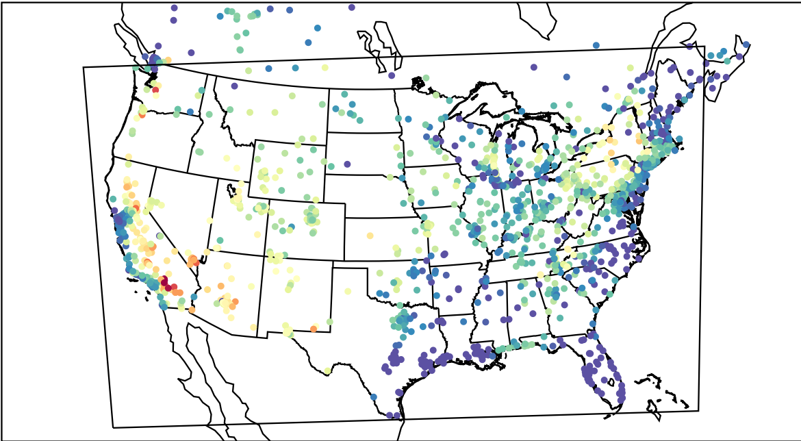
AirNOW (2021-06-26_02:00:00)
