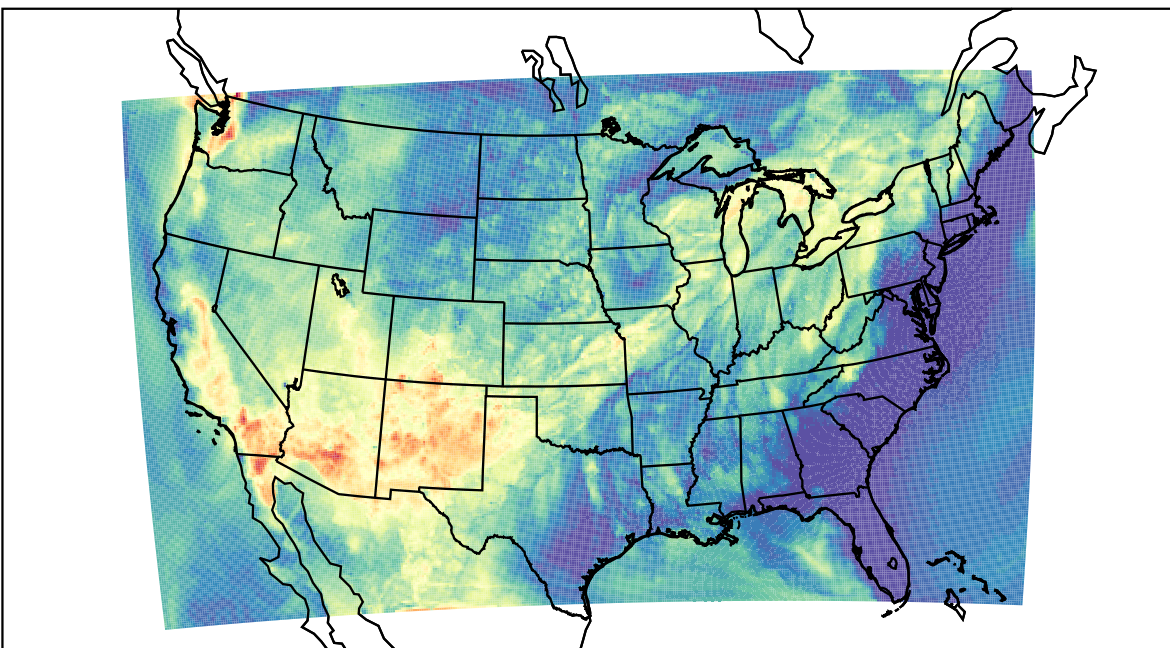
WRF (2021-06-27_03:00:00)
