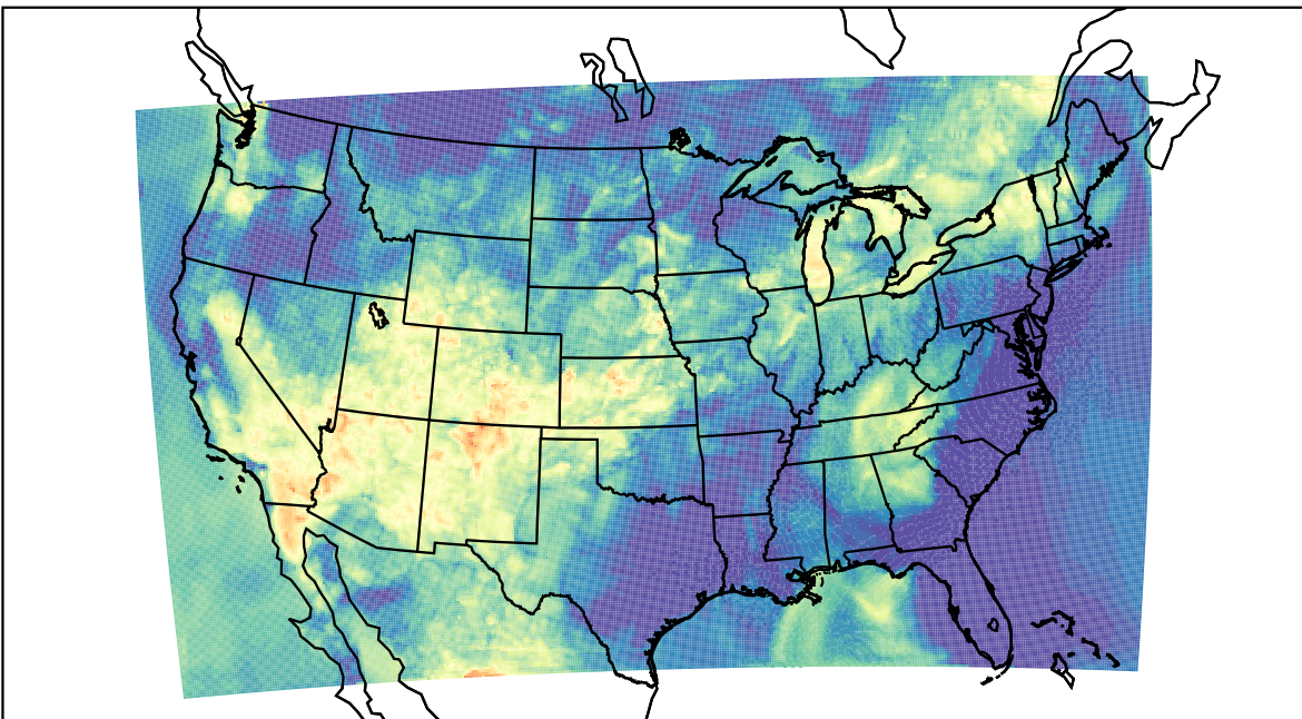
WRF (2021-06-26_07:00:00)
