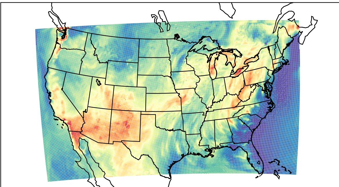
WRF (2021-06-26_20:00:00)
