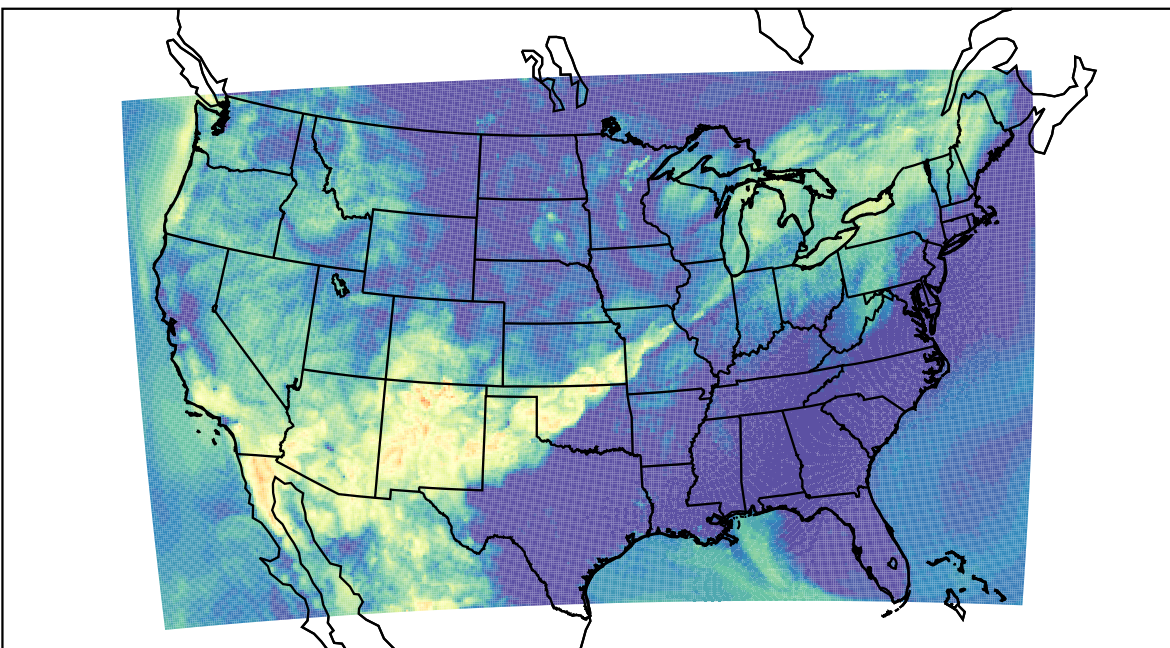
WRF (2021-06-27_12:00:00)
