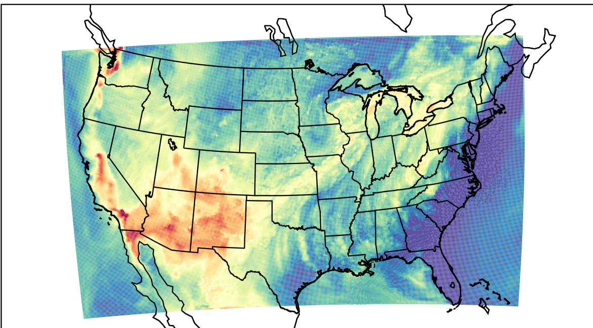
WRF (2021-06-27_01:00:00)
