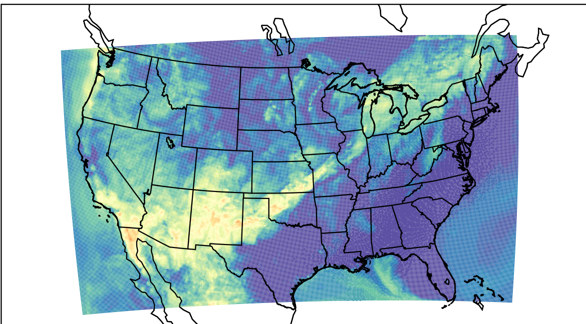
WRF (2021-06-27_10:00:00)
