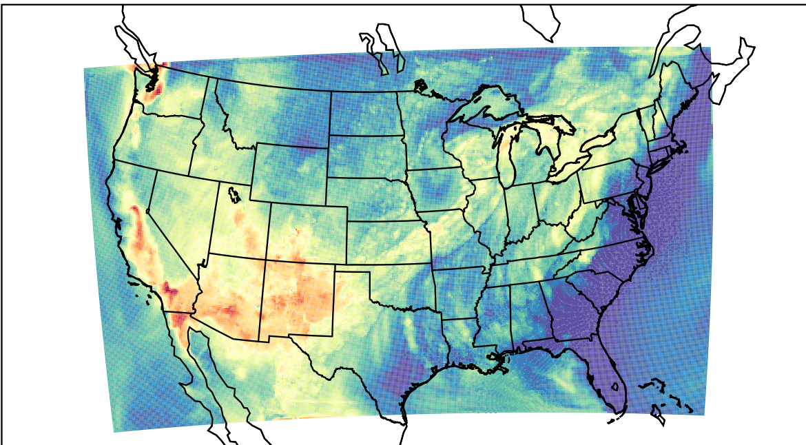
WRF (2021-06-27_02:00:00)
