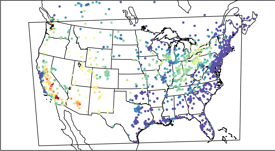
AirNOW (2021-06-27_02:00:00)
