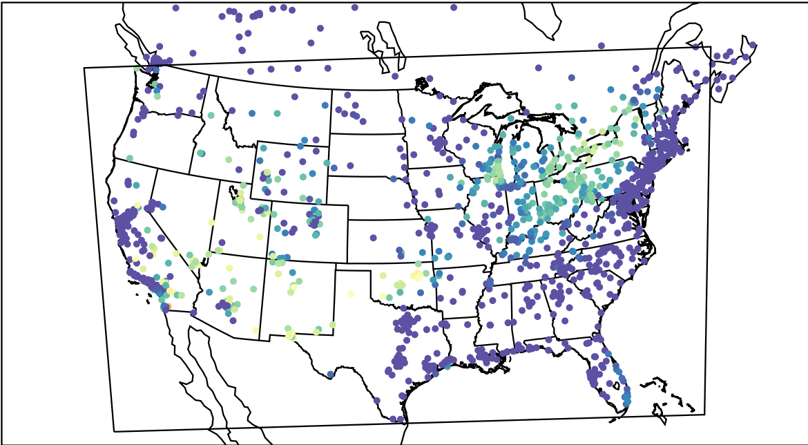
AirNOW (2021-06-27_12:00:00)
