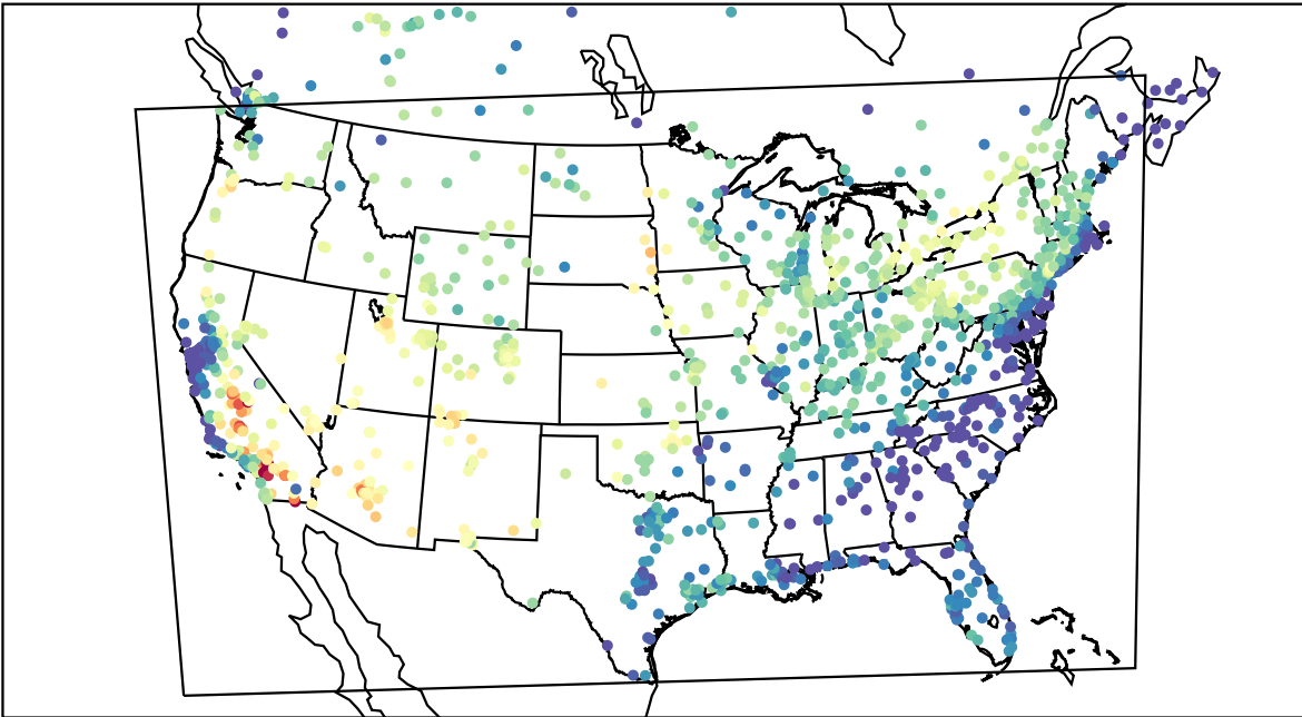
AirNOW (2021-06-27_17:00:00)
