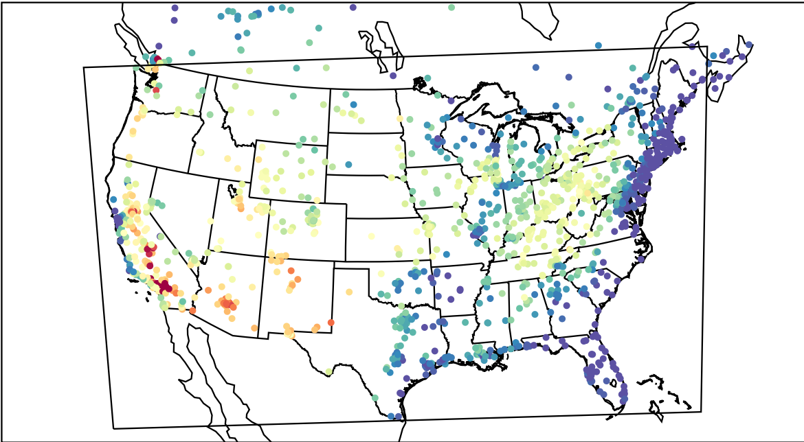
AirNOW (2021-06-26_22:00:00)
