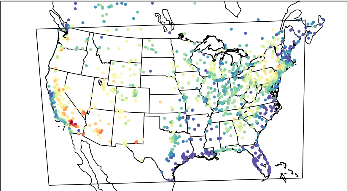
AirNOW (2021-06-26_00:00:00)
