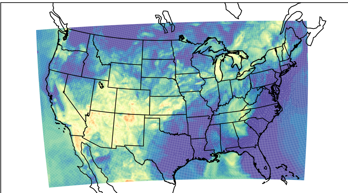
WRF (2021-06-26_09:00:00)
