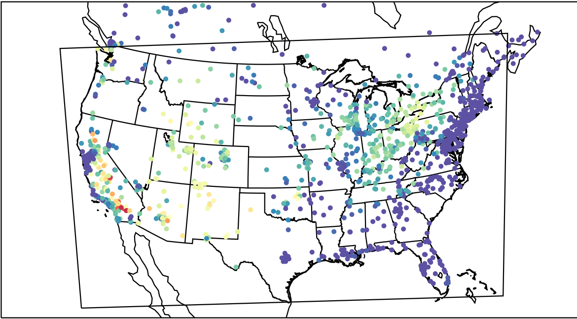
AirNOW (2021-06-27_04:00:00)
