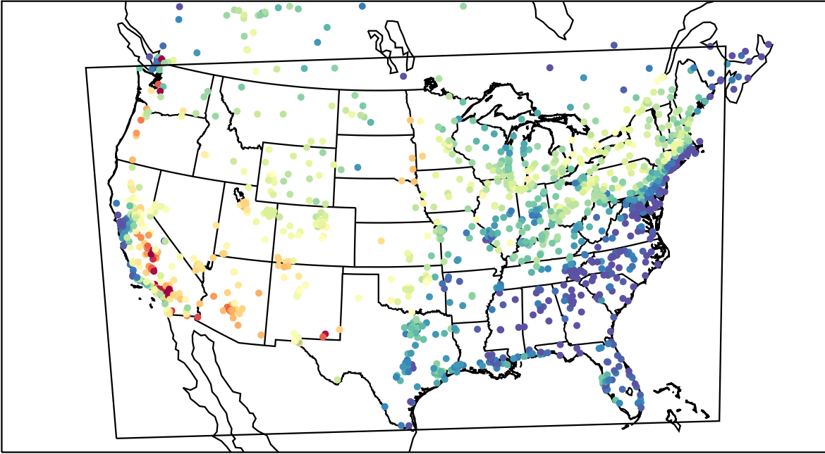
AirNOW (2021-06-27_21:00:00)
