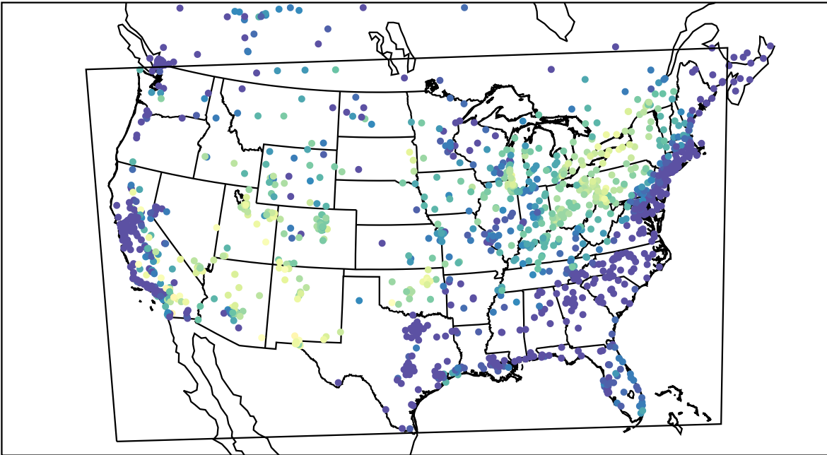
AirNOW (2021-06-27_14:00:00)
