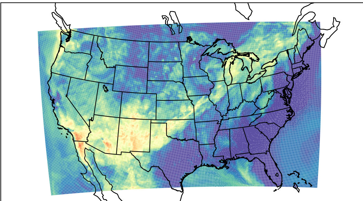
WRF (2021-06-27_07:00:00)
