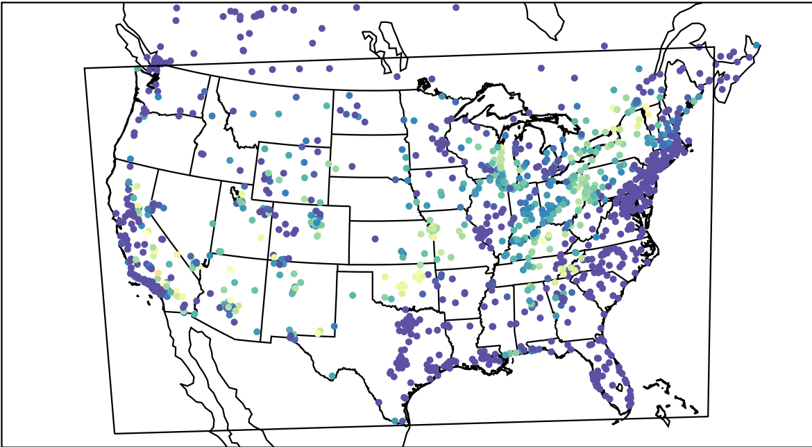
AirNOW (2021-06-26_11:00:00)
