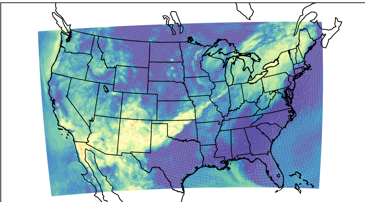
WRF (2021-06-27_13:00:00)
