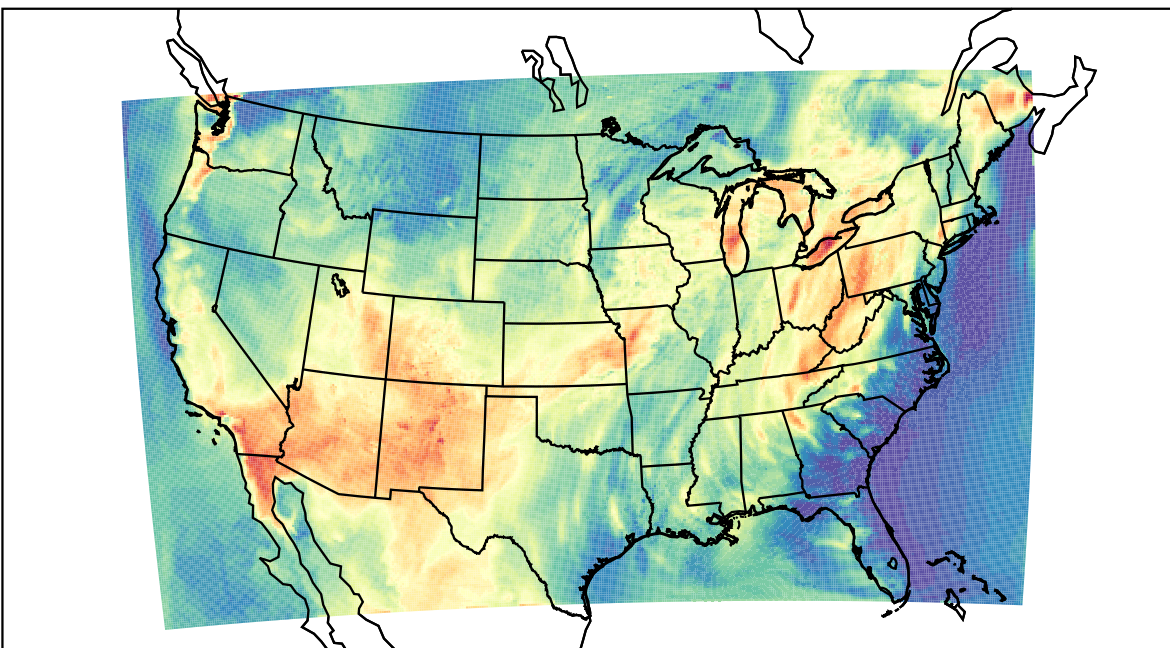
WRF (2021-06-26_19:00:00)
