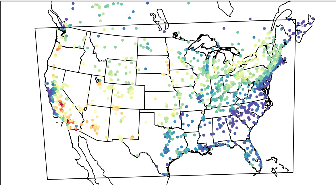
AirNOW (2021-06-27_18:00:00)
