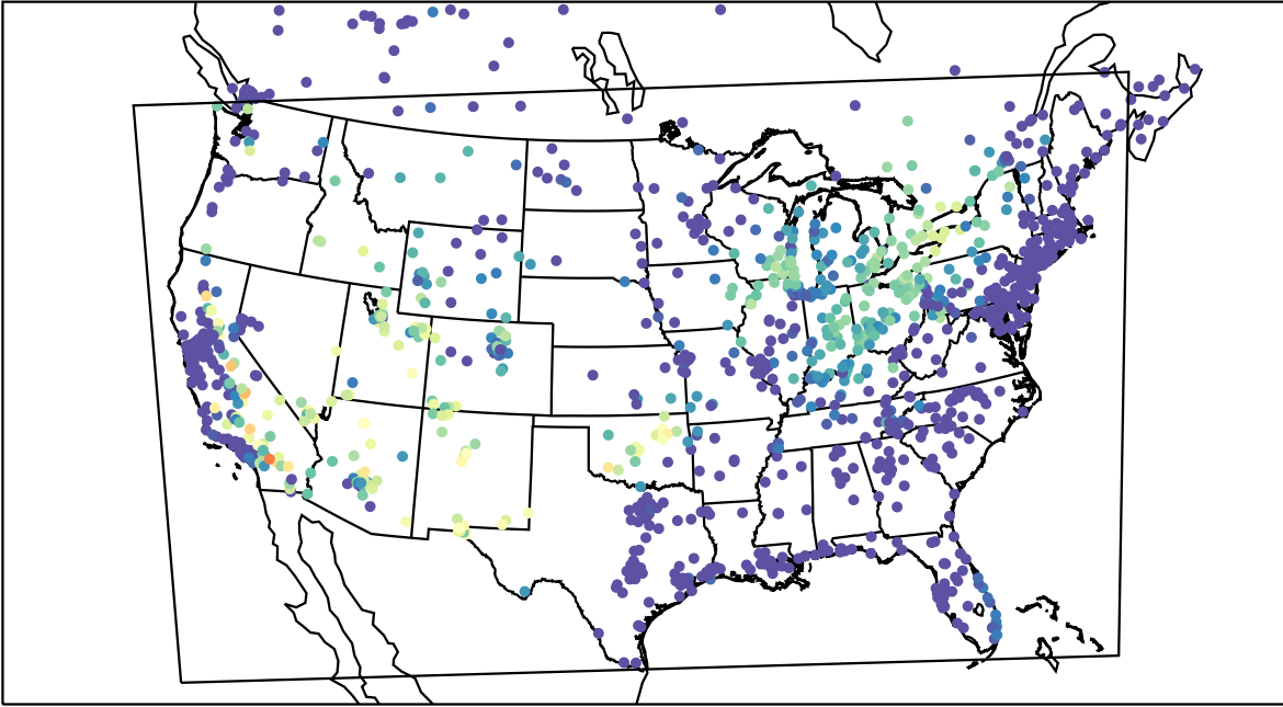
AirNOW (2021-06-27_09:00:00)
