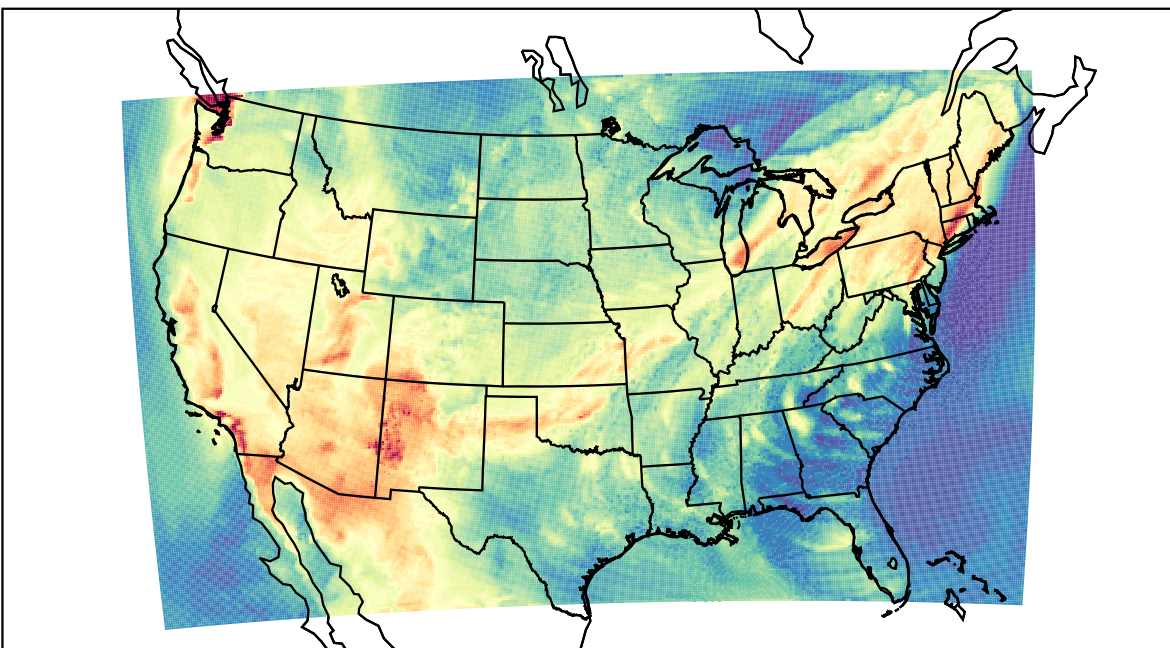
WRF (2021-06-27_20:00:00)
