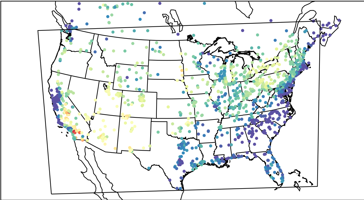
AirNOW (2021-06-27_16:00:00)
