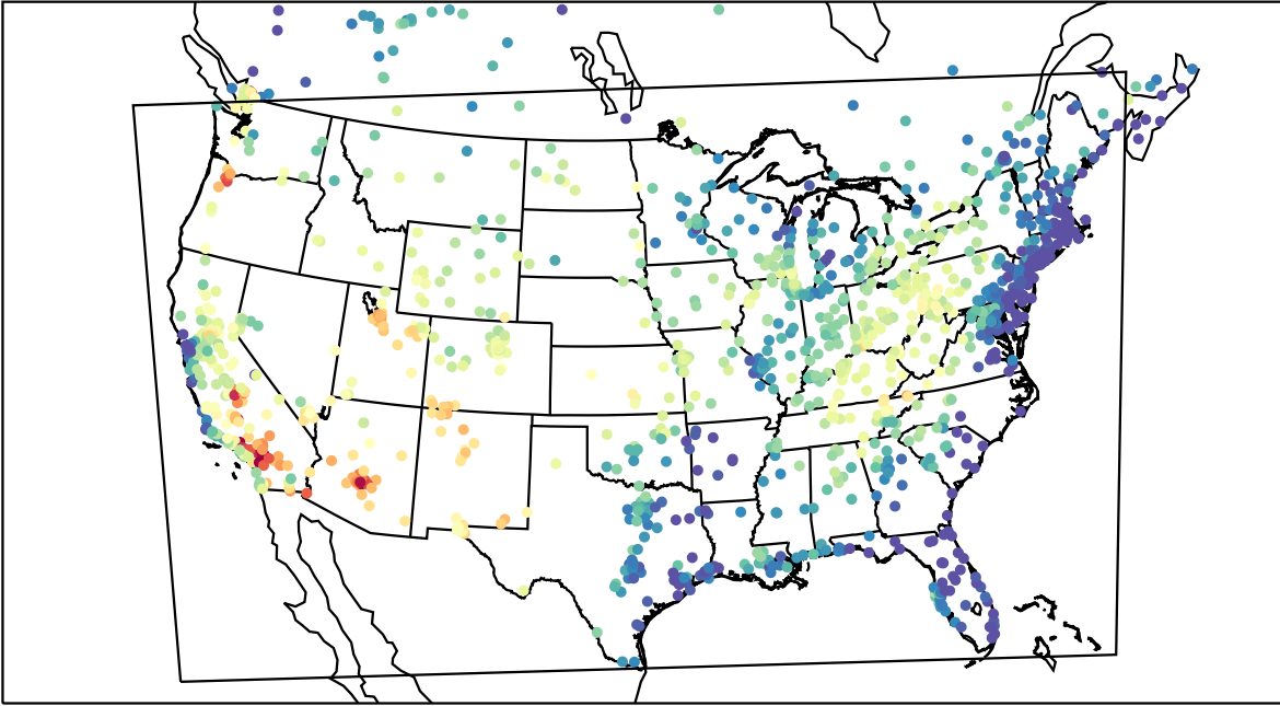
AirNOW (2021-06-26_19:00:00)
