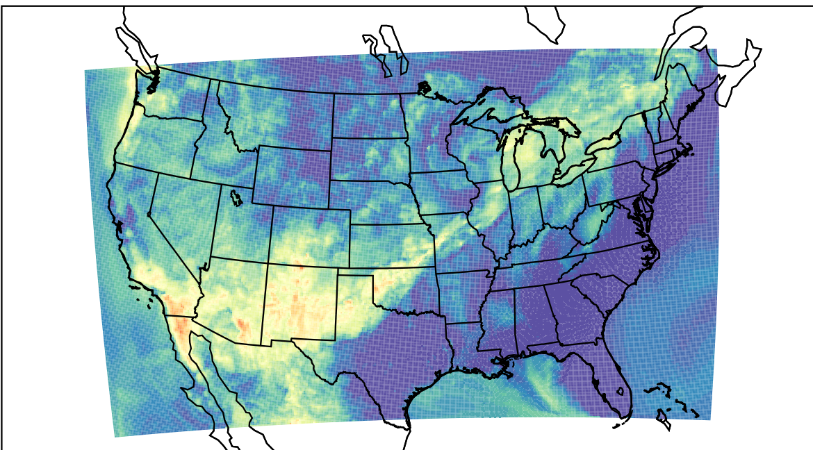
WRF (2021-06-27_08:00:00)
