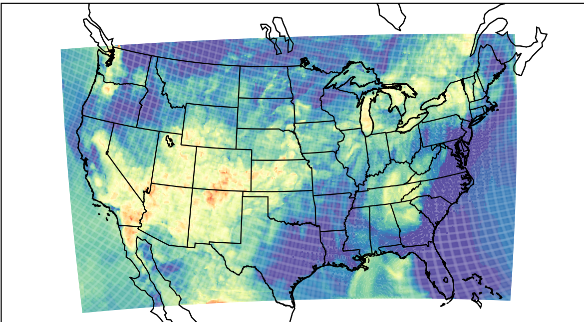
WRF (2021-06-26_06:00:00)
