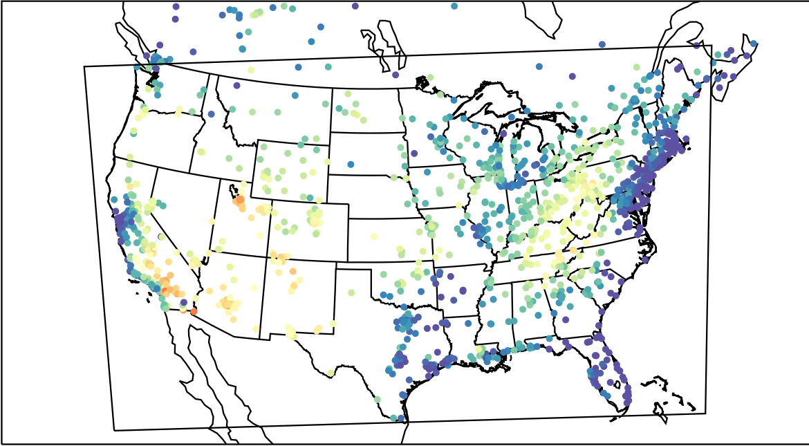
AirNOW (2021-06-26_17:00:00)
