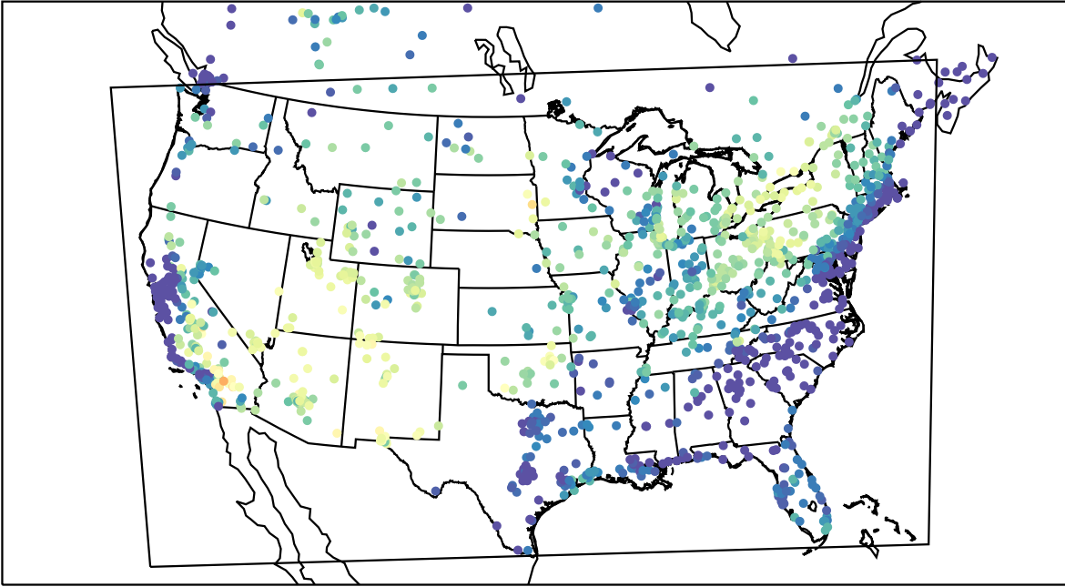
AirNOW (2021-06-27_15:00:00)
