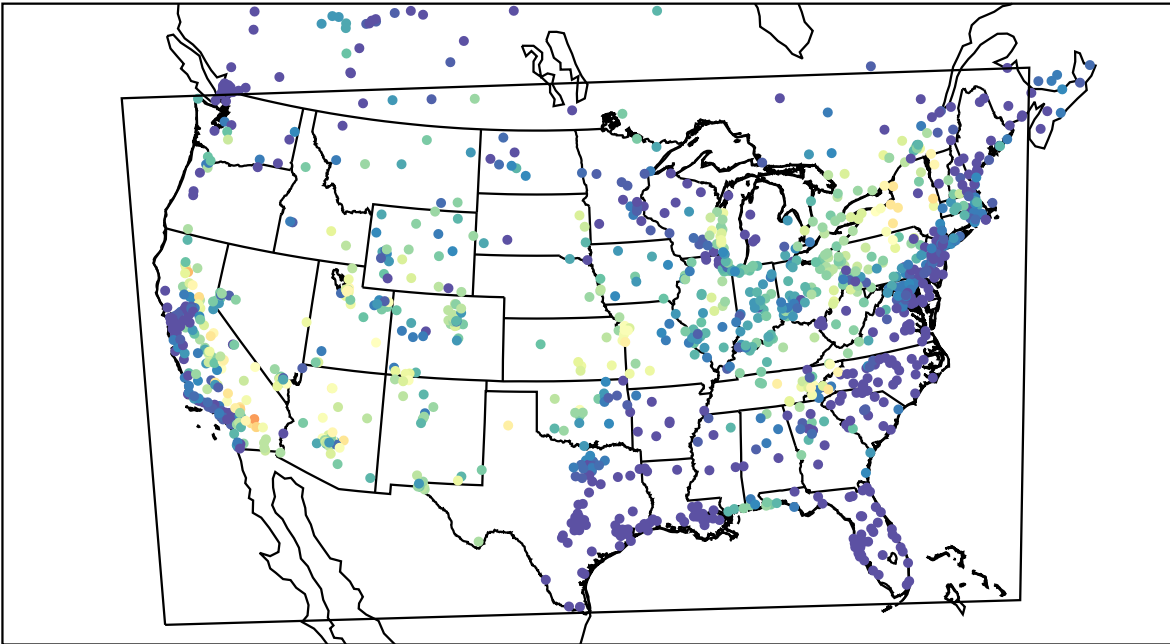
AirNOW (2021-06-26_05:00:00)
