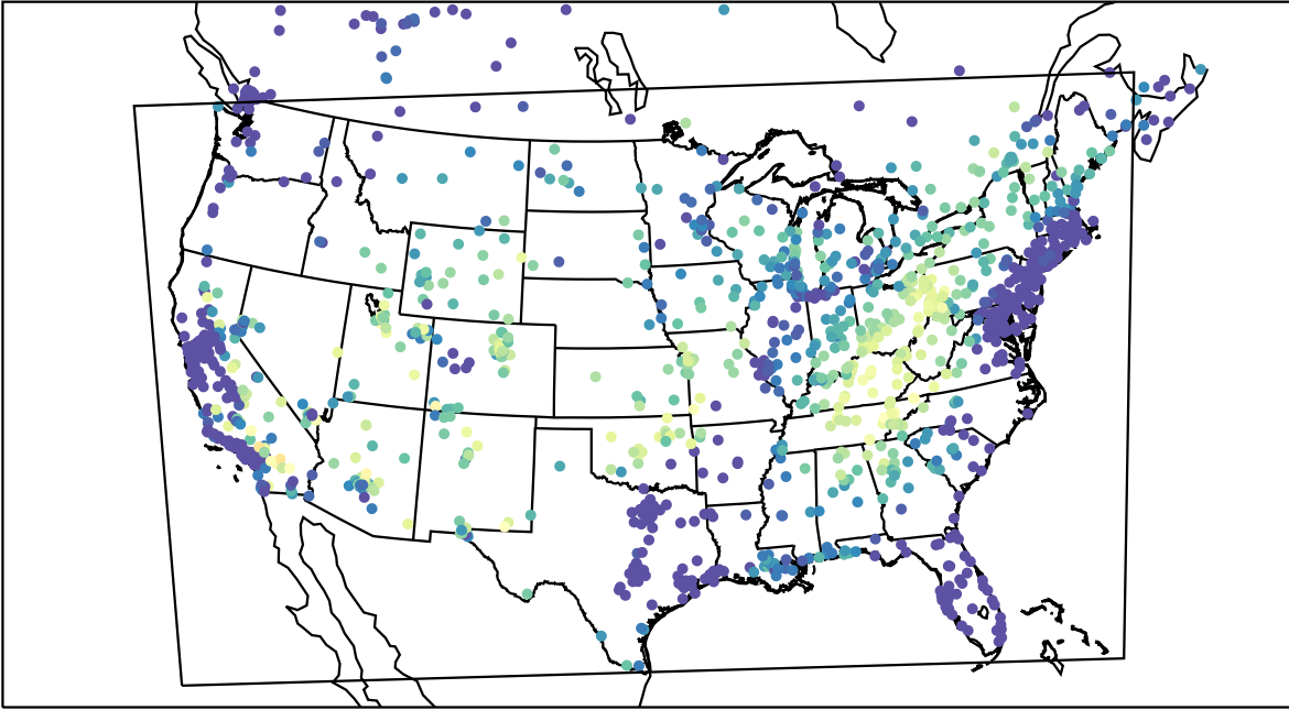
AirNOW (2021-06-26_14:00:00)
