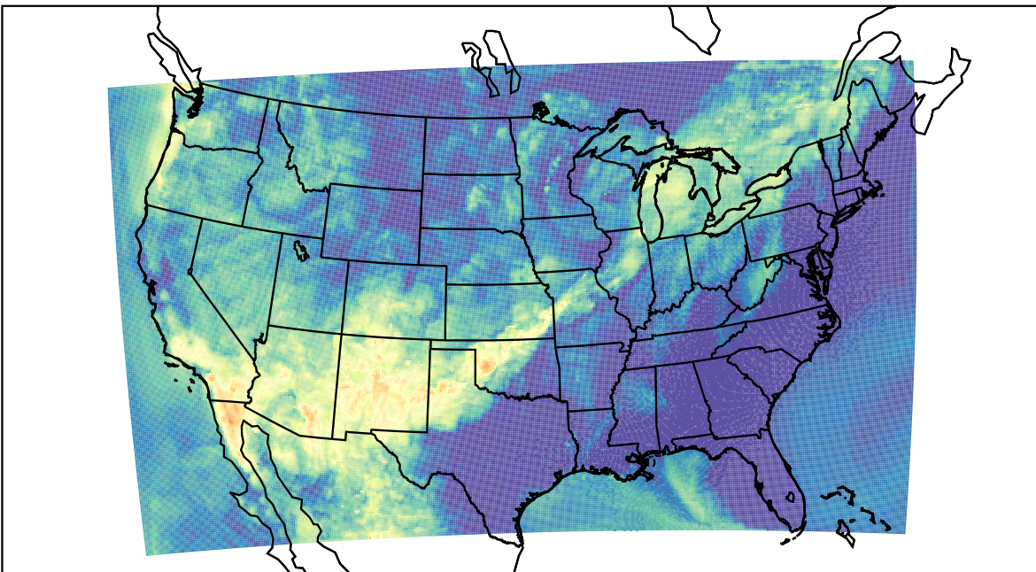
WRF (2021-06-27_09:00:00)
