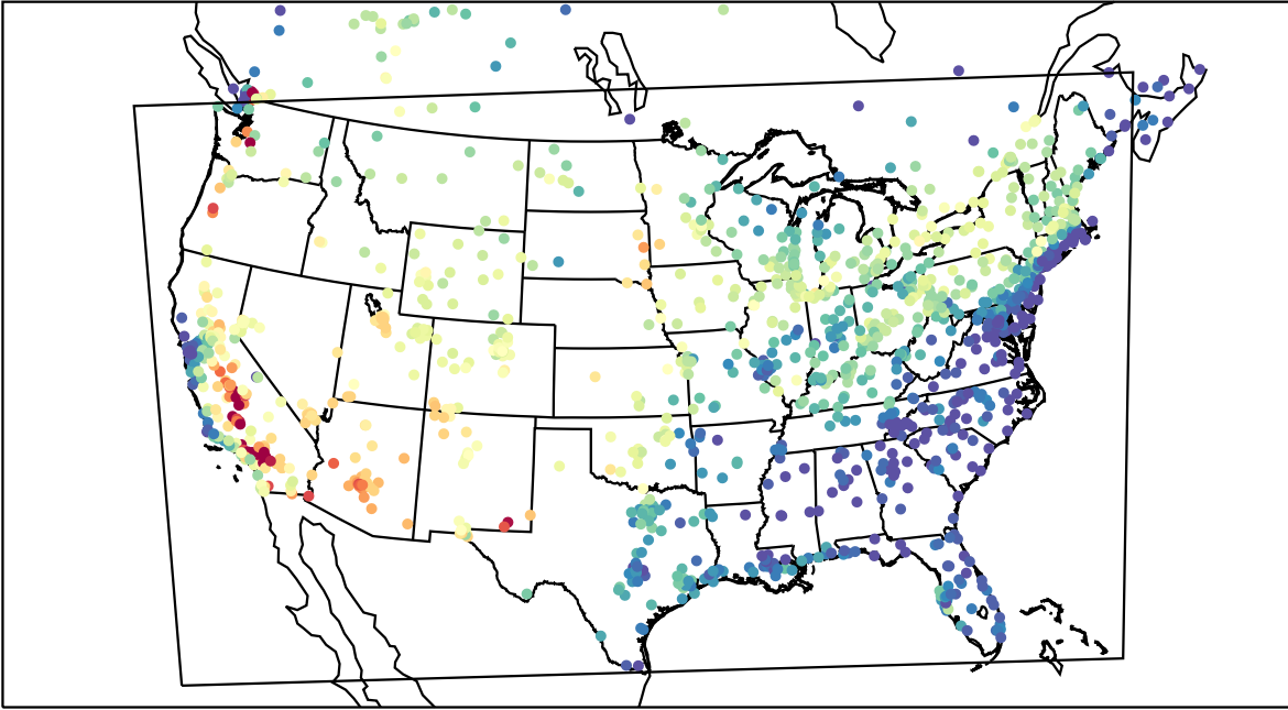
AirNOW (2021-06-27_22:00:00)
