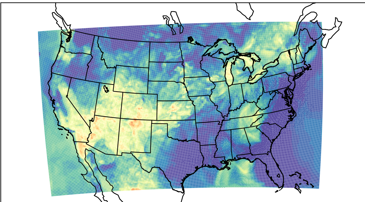
WRF (2021-06-26_08:00:00)
