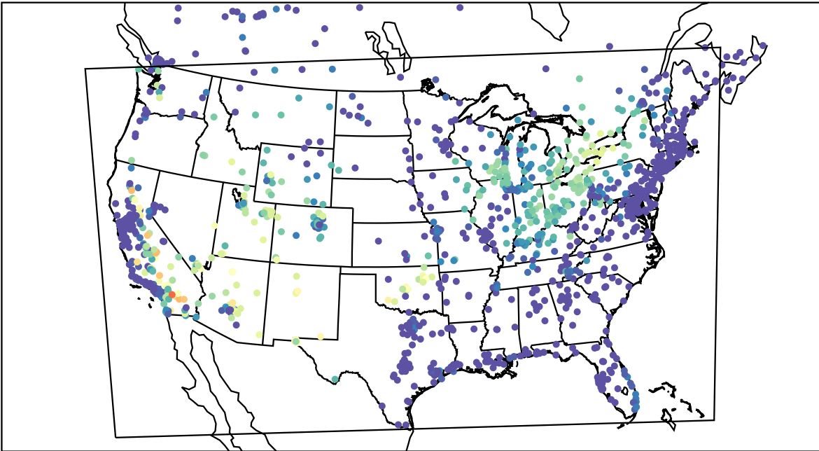
AirNOW (2021-06-27_08:00:00)
