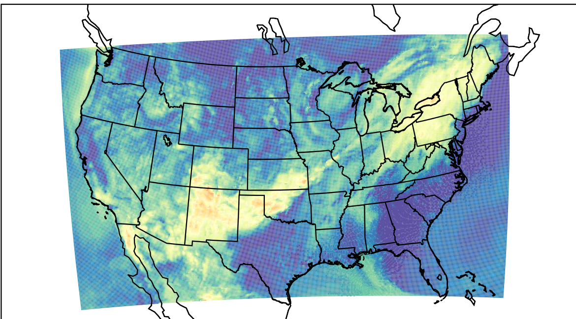
WRF (2021-06-27_14:00:00)
