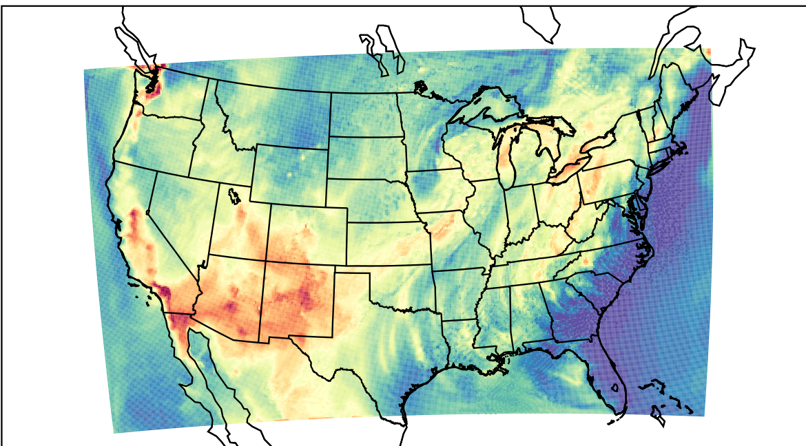
WRF (2021-06-26_23:00:00)
