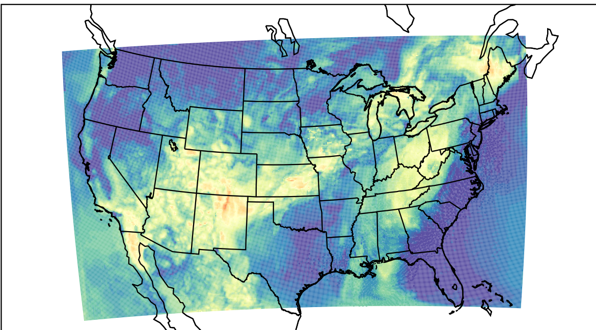
WRF (2021-06-26_14:00:00)
