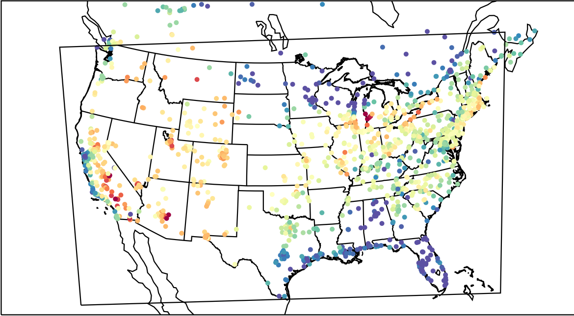
AirNOW (2021-07-06_23:00:00)
