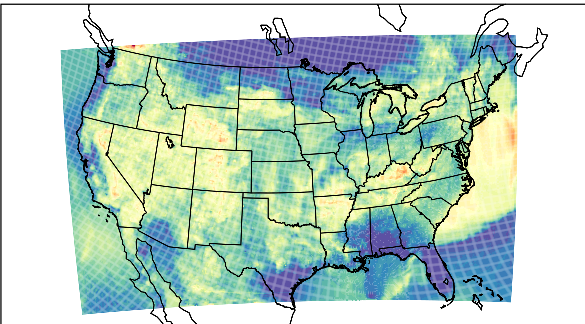
WRF (2021-07-06_07:00:00)
