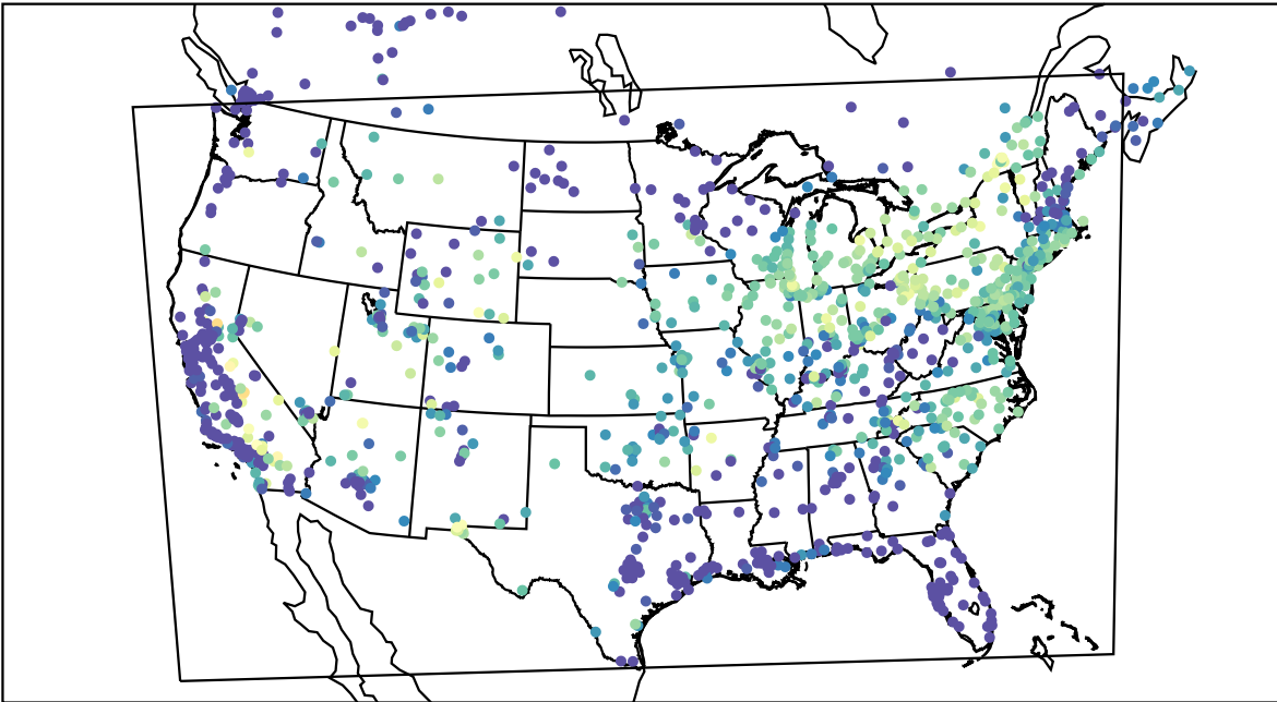
AirNOW (2021-07-06_13:00:00)
