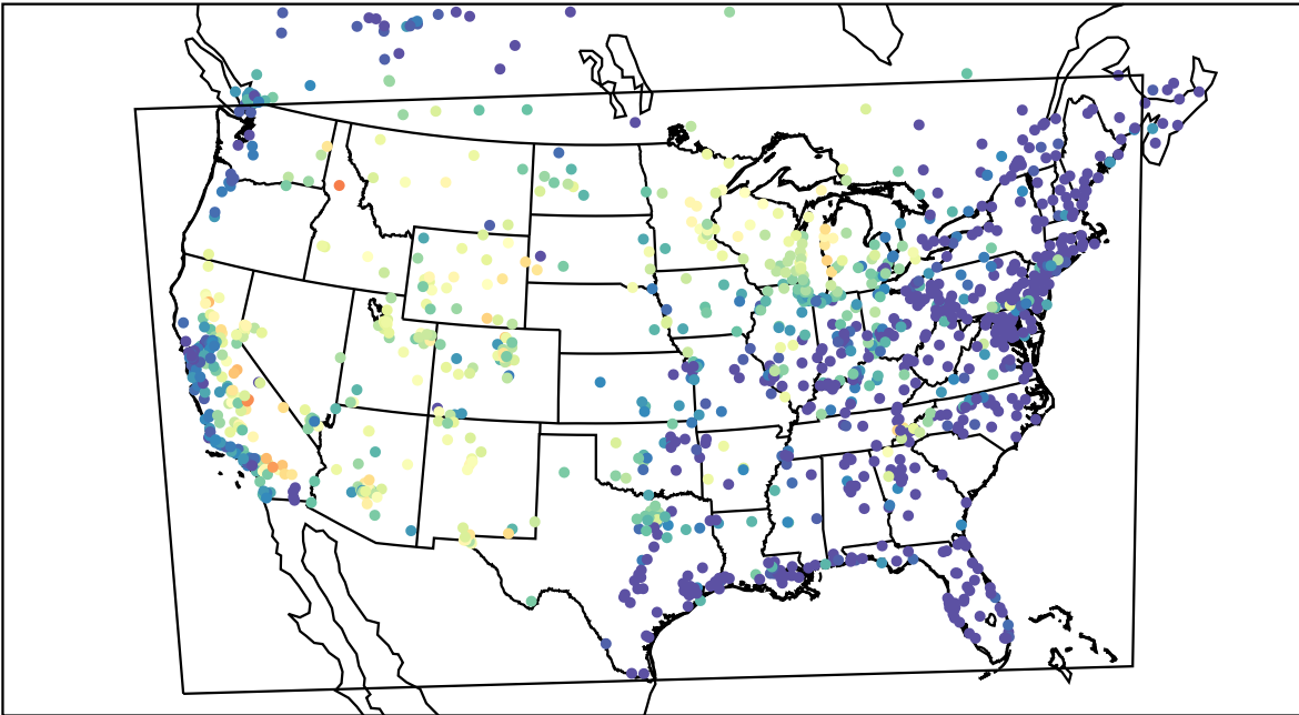
AirNOW (2021-07-05_04:00:00)
