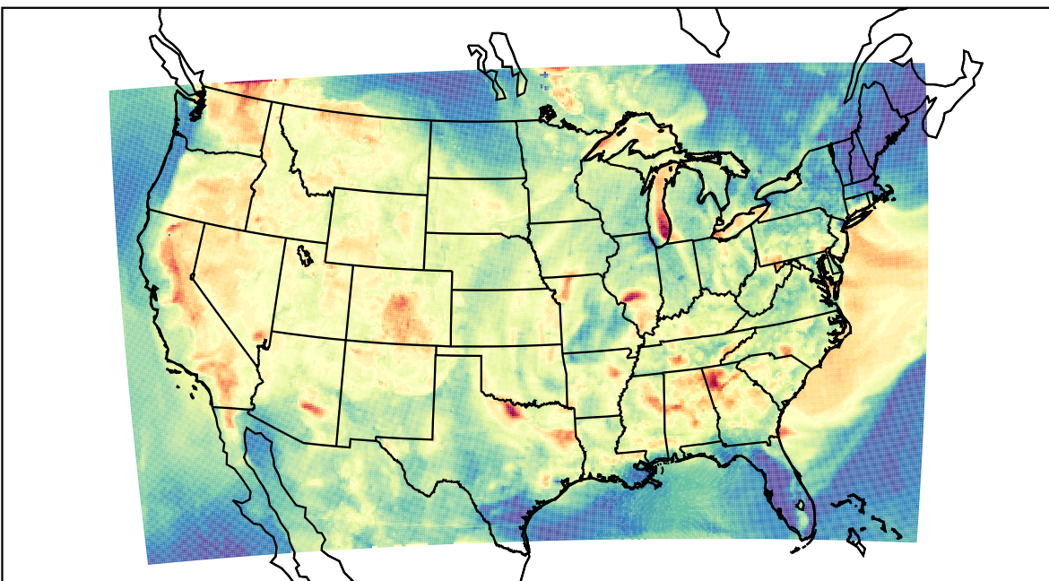
WRF (2021-07-05_02:00:00)
