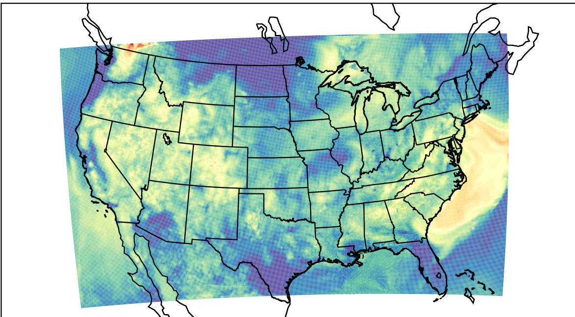
WRF (2021-07-05_13:00:00)
