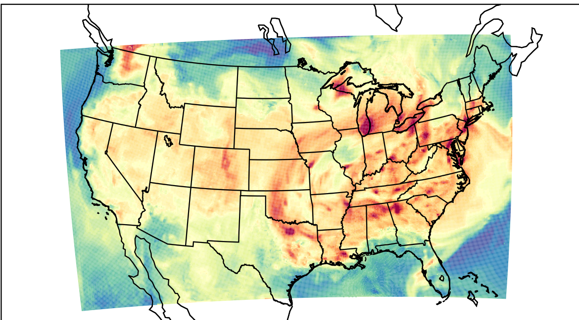
WRF (2021-07-05_18:00:00)
