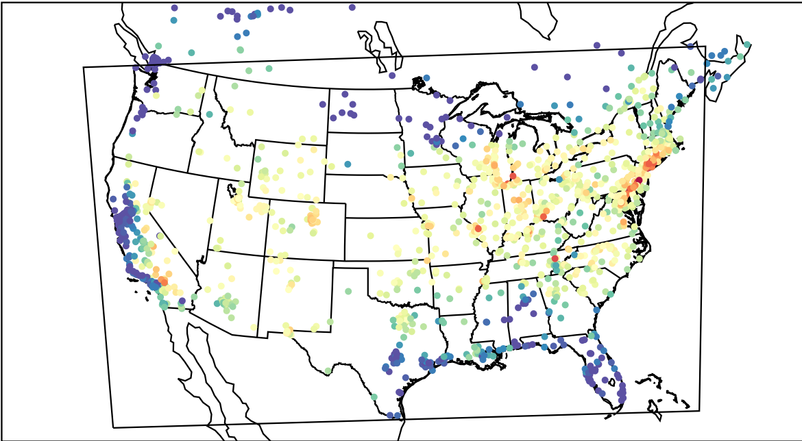
AirNOW (2021-07-06_16:00:00)
