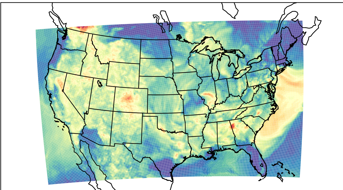
WRF (2021-07-05_06:00:00)
