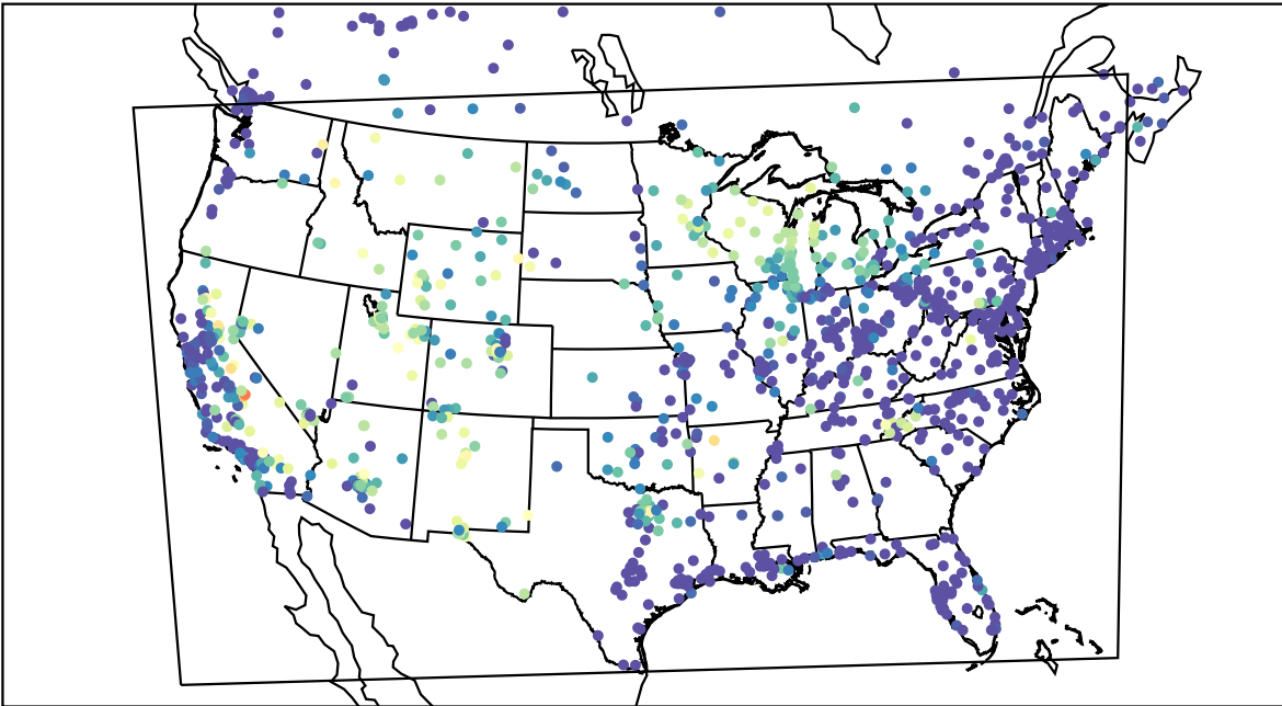
AirNOW (2021-07-05_09:00:00)
