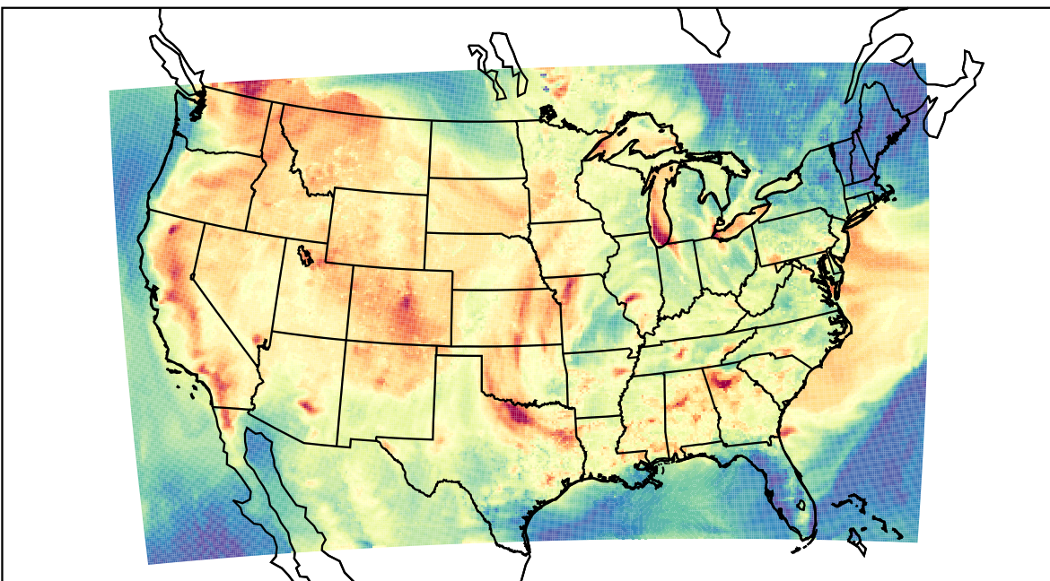
WRF (2021-07-05_00:00:00)
