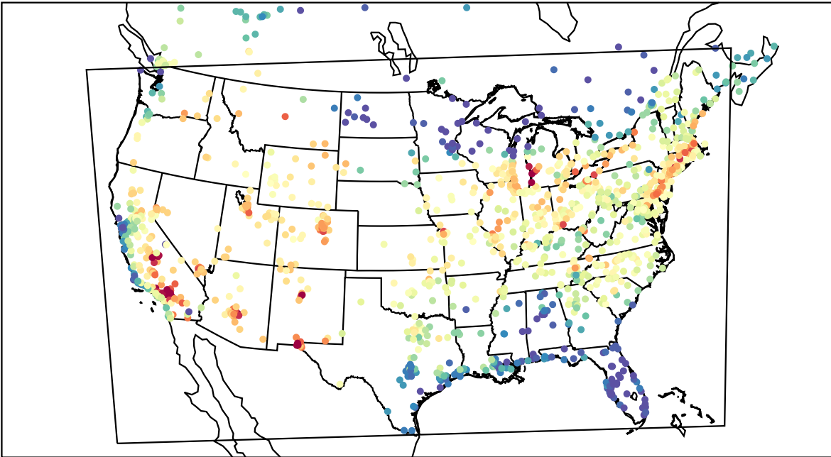
AirNOW (2021-07-06_21:00:00)
