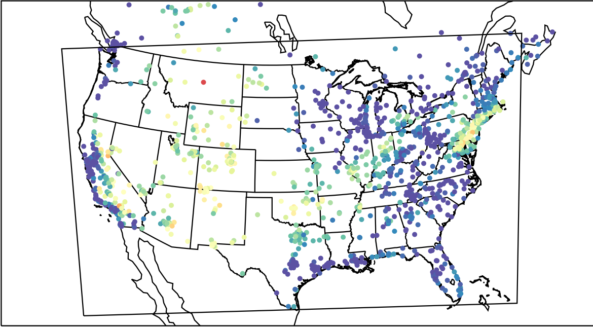
AirNOW (2021-07-08_15:00:00)
