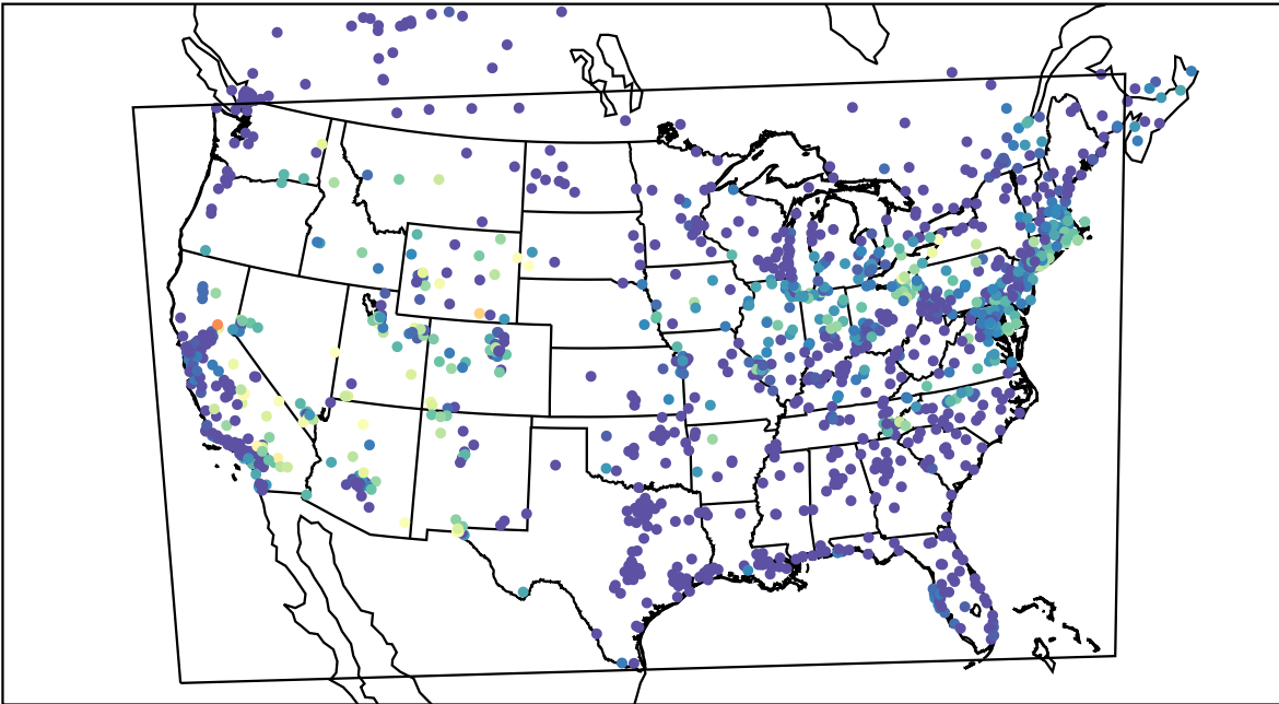
AirNOW (2021-07-07_12:00:00)
