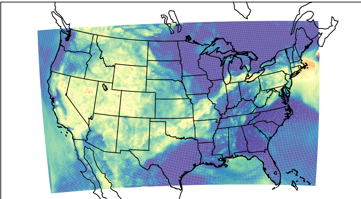
WRF (2021-07-08_08:00:00)
