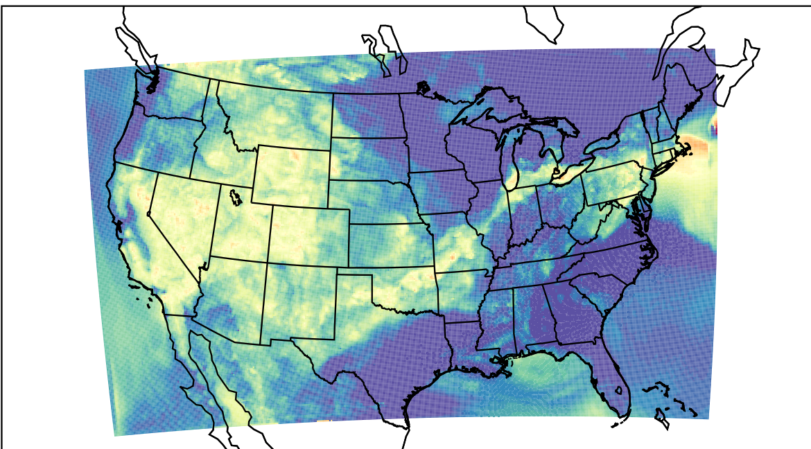
WRF (2021-07-08_09:00:00)
