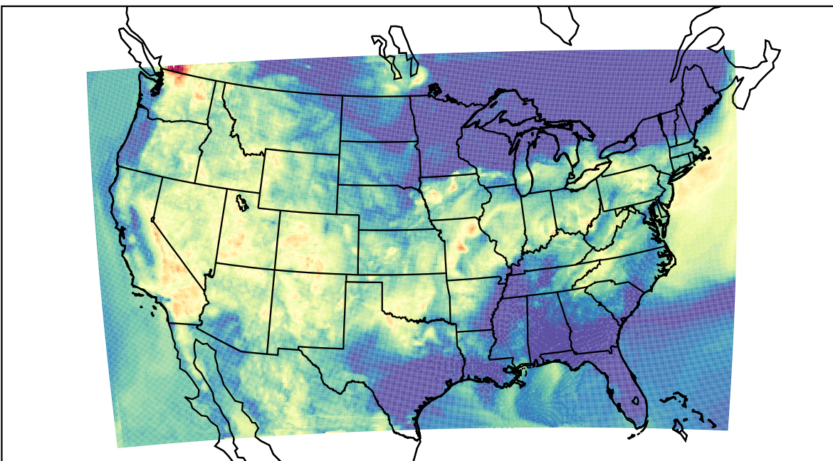
WRF (2021-07-07_08:00:00)
