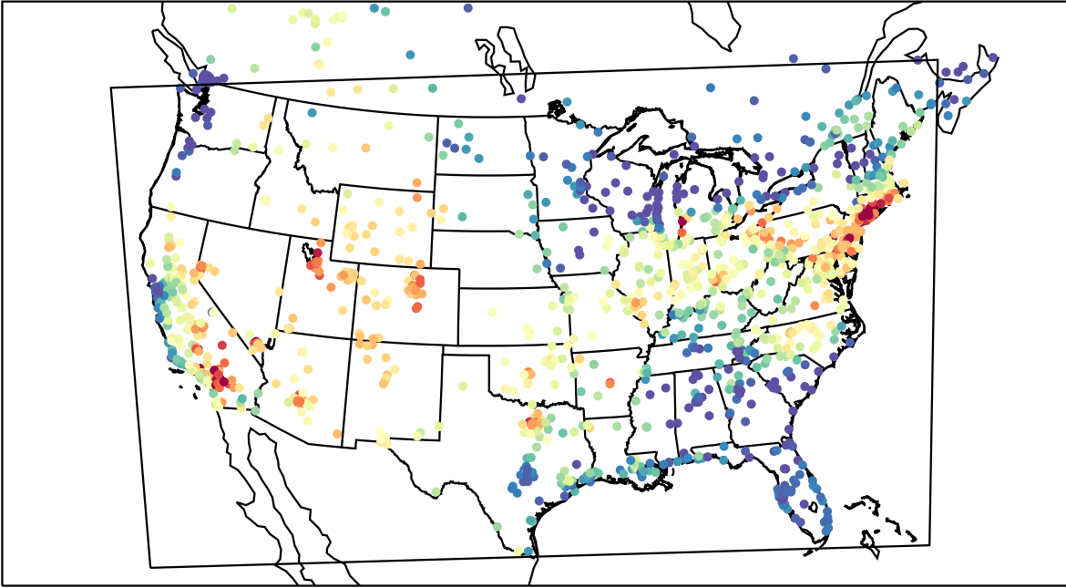
AirNOW (2021-07-07_19:00:00)
