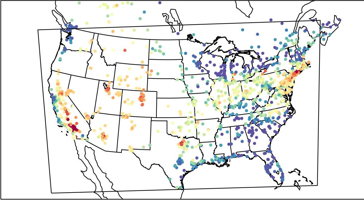
AirNOW (2021-07-07_22:00:00)
