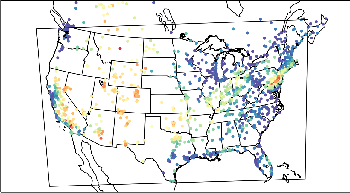
AirNOW (2021-07-08_17:00:00)
