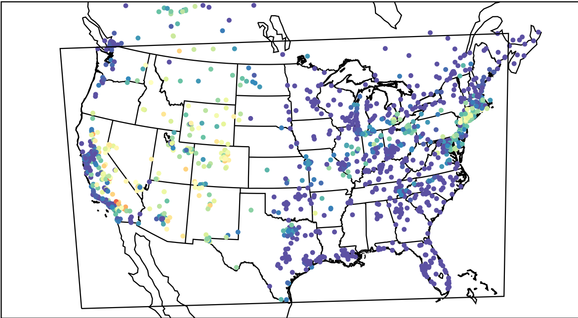
AirNOW (2021-07-08_06:00:00)
