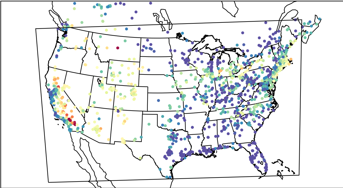
AirNOW (2021-07-07_03:00:00)
