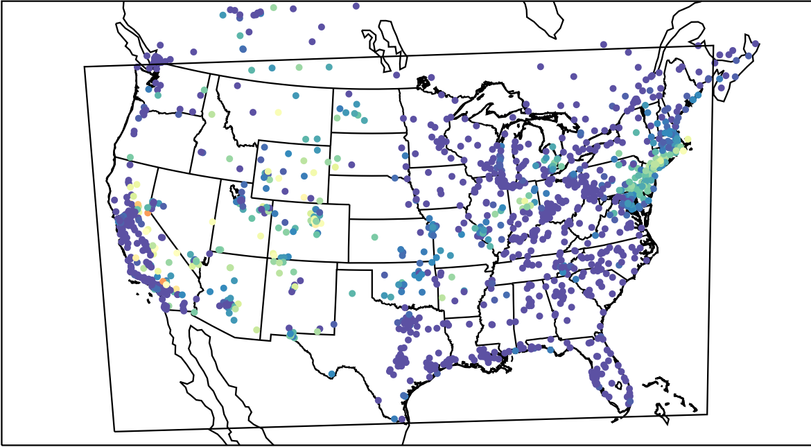
AirNOW (2021-07-08_13:00:00)
