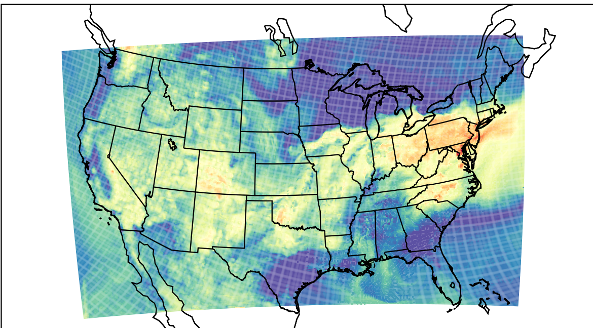
WRF (2021-07-07_14:00:00)
