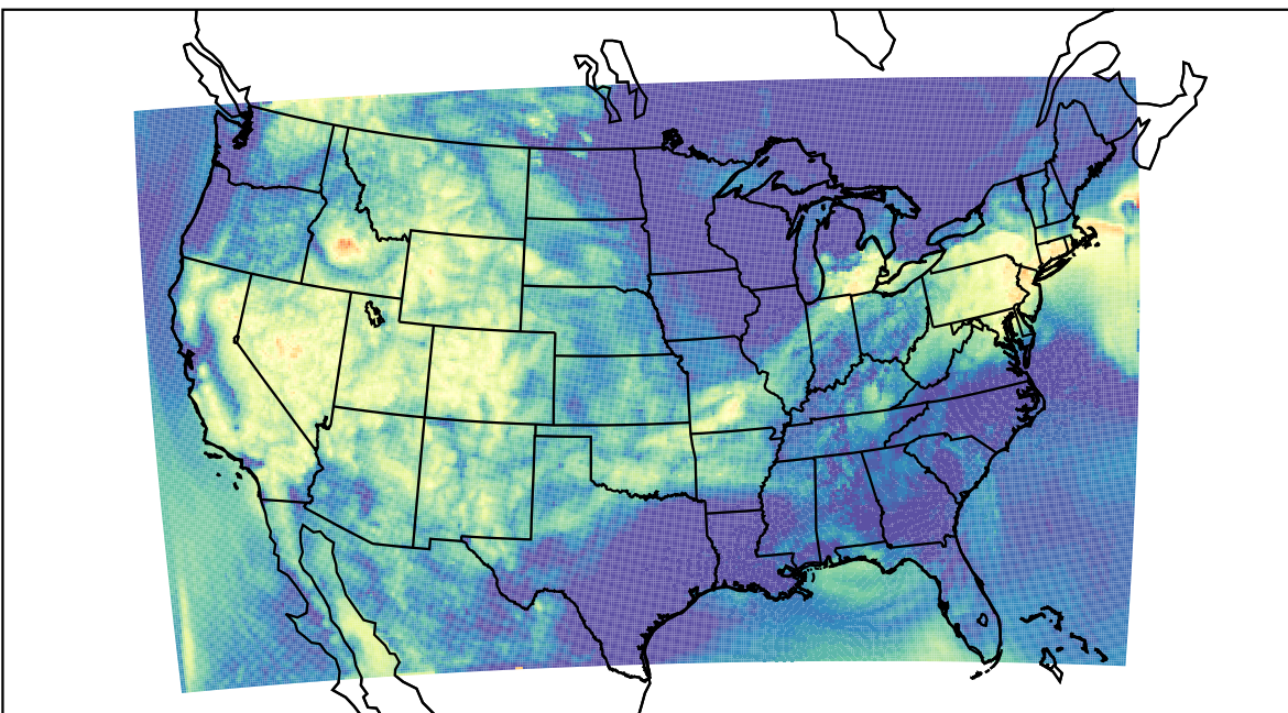
WRF (2021-07-08_13:00:00)
