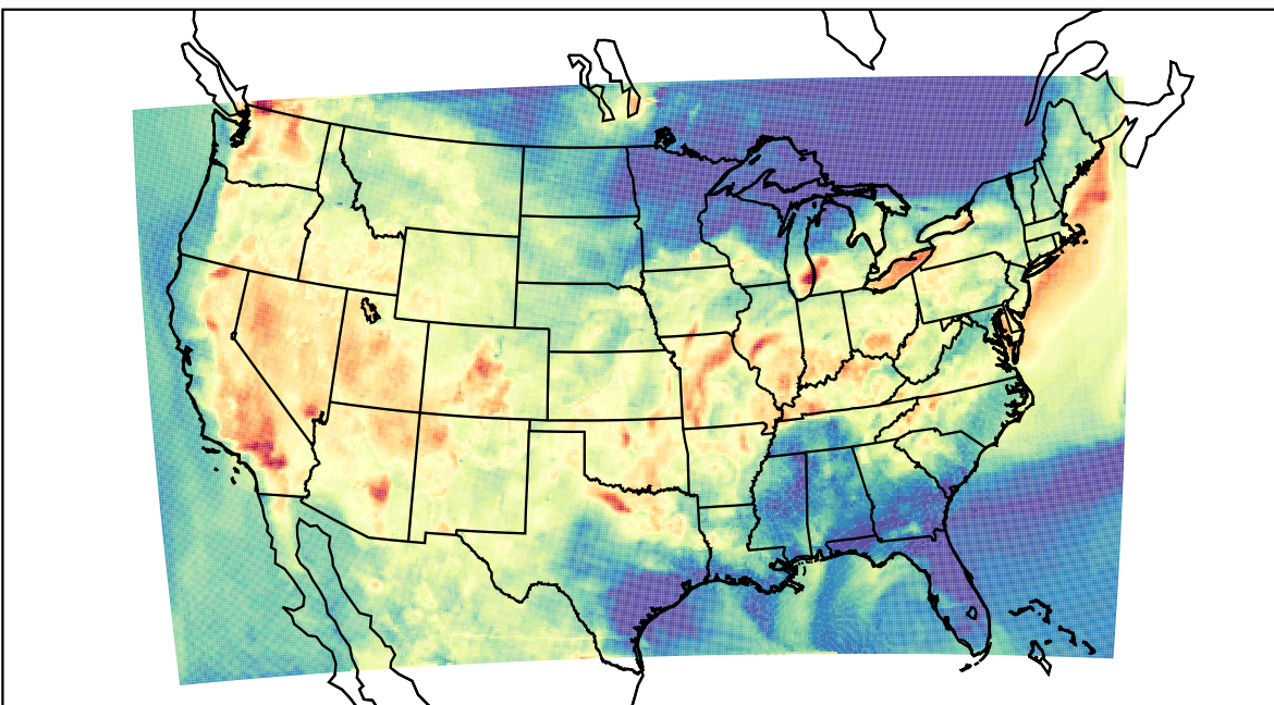
WRF (2021-07-07_02:00:00)
