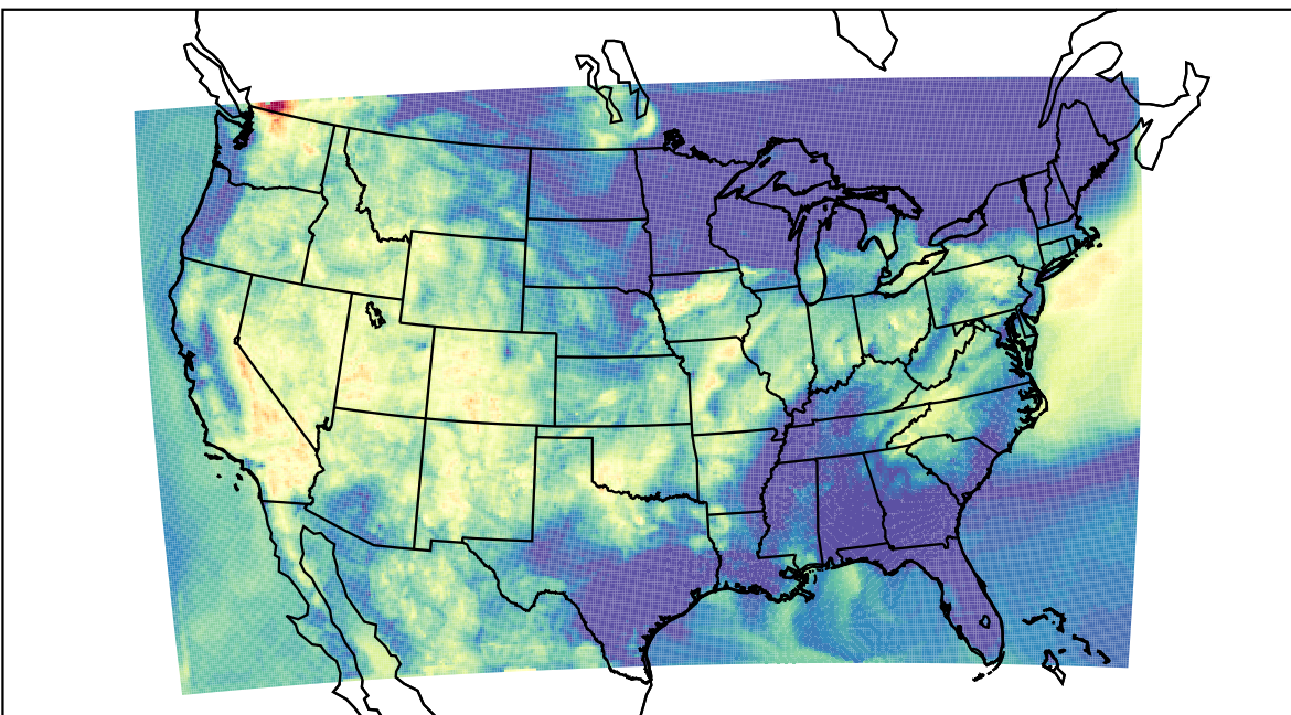
WRF (2021-07-07_10:00:00)
