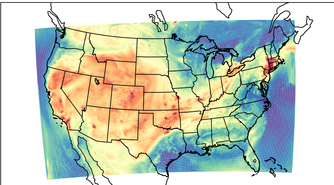
WRF (2021-07-08_21:00:00)
