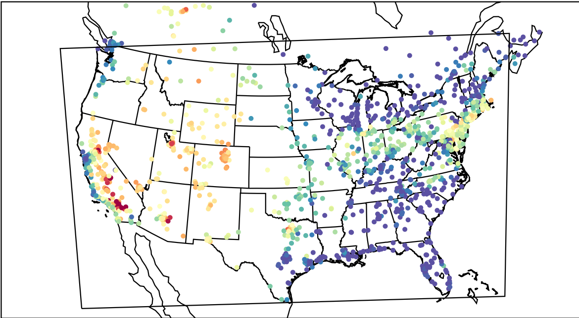
AirNOW (2021-07-08_01:00:00)
