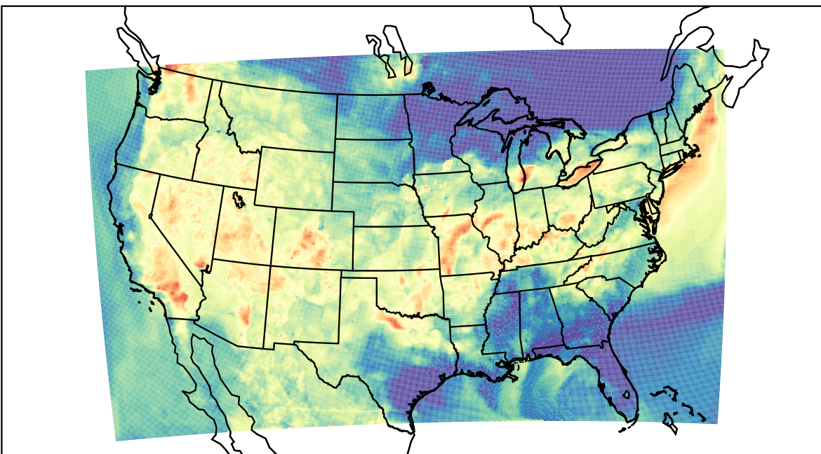
WRF (2021-07-07_03:00:00)
