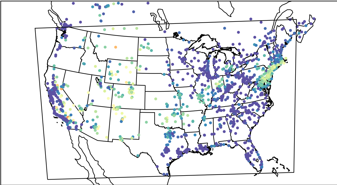
AirNOW (2021-07-08_14:00:00)
