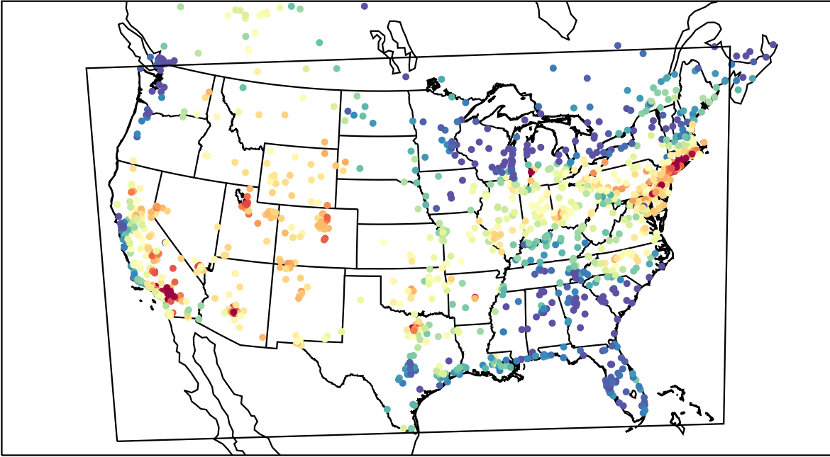
AirNOW (2021-07-07_20:00:00)
