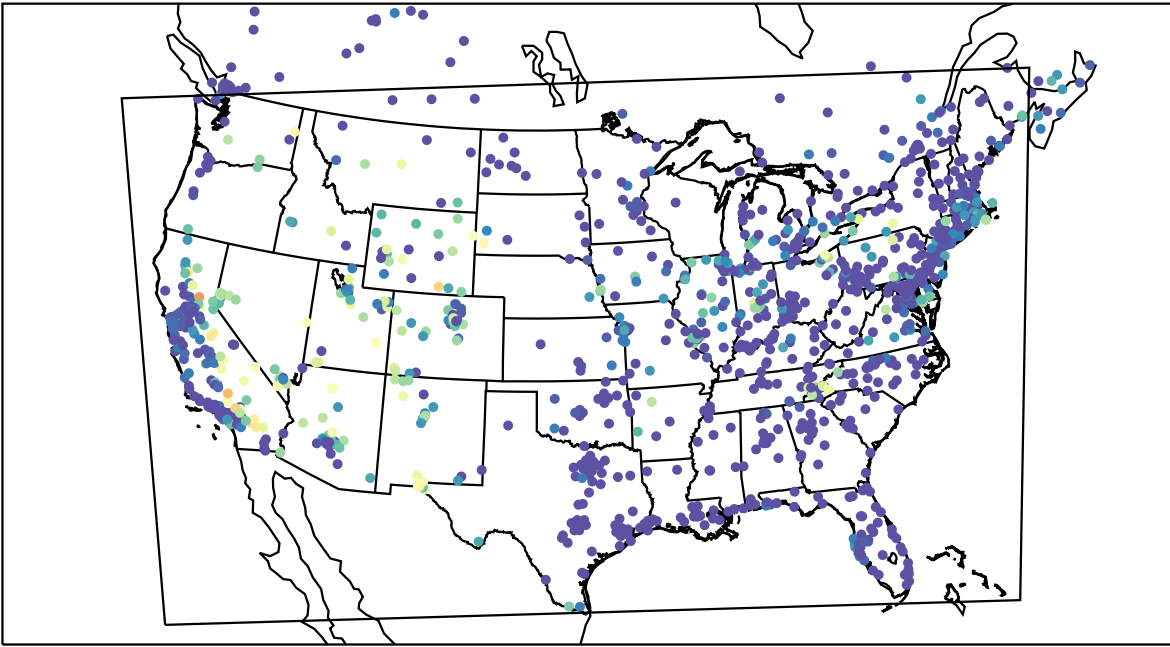
AirNOW (2021-07-07_10:00:00)
