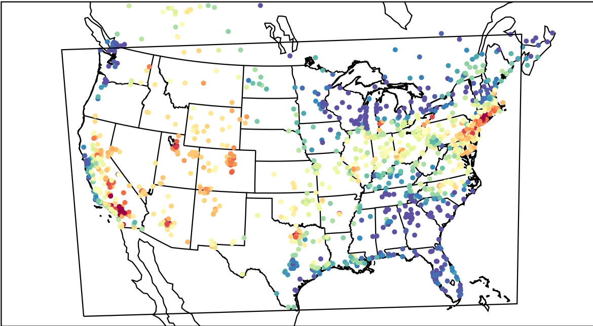
AirNOW (2021-07-07_21:00:00)
