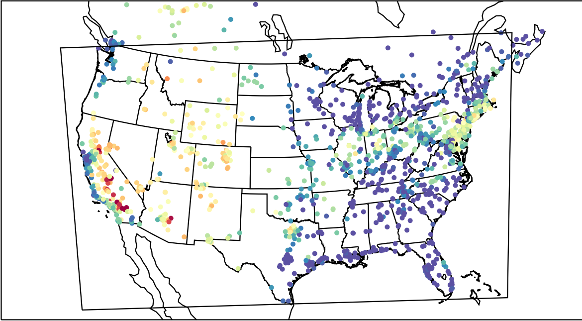
AirNOW (2021-07-08_02:00:00)
