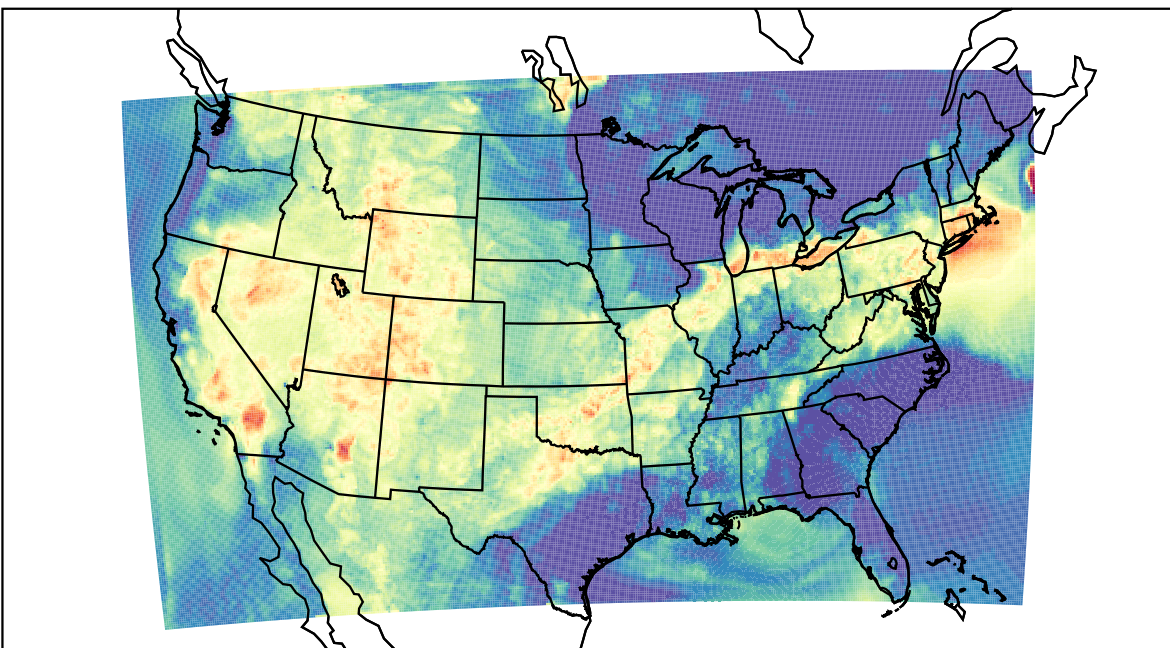
WRF (2021-07-08_04:00:00)
