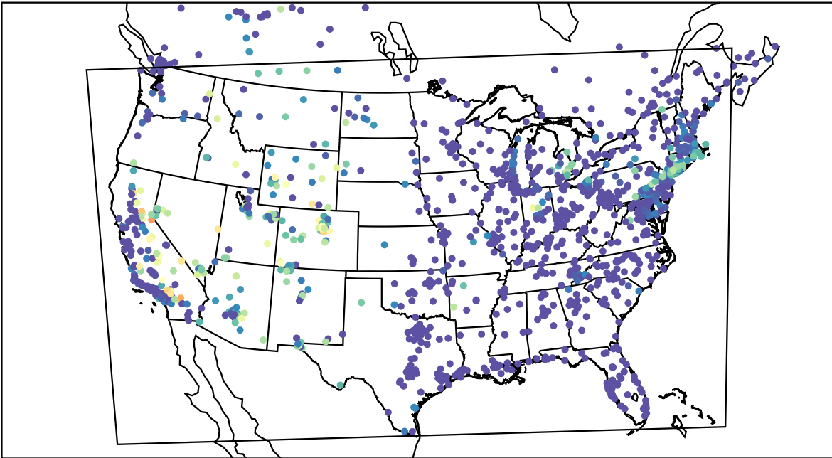
AirNOW (2021-07-08_11:00:00)
