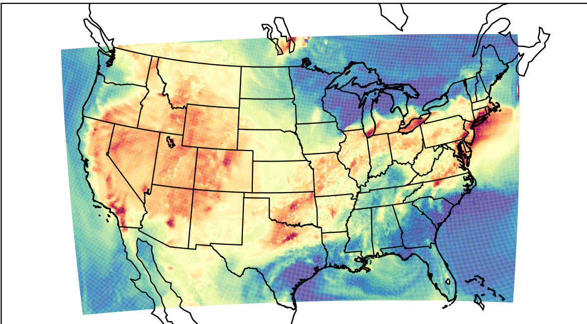
WRF (2021-07-07_23:00:00)
