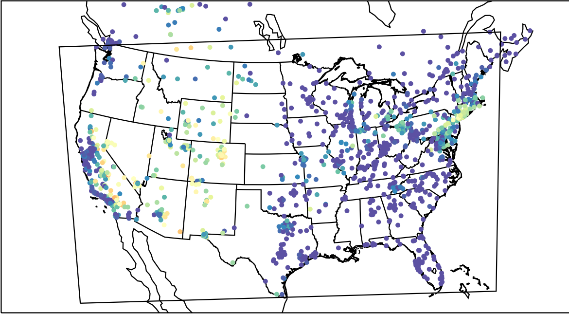
AirNOW (2021-07-08_07:00:00)
