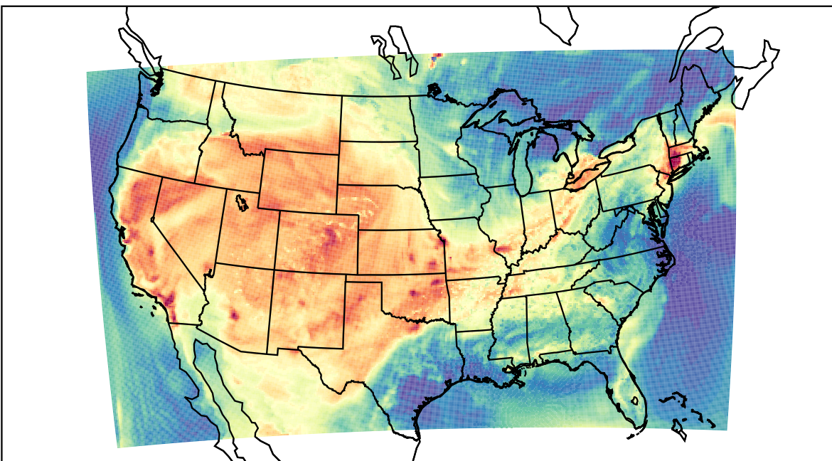
WRF (2021-07-08_22:00:00)
