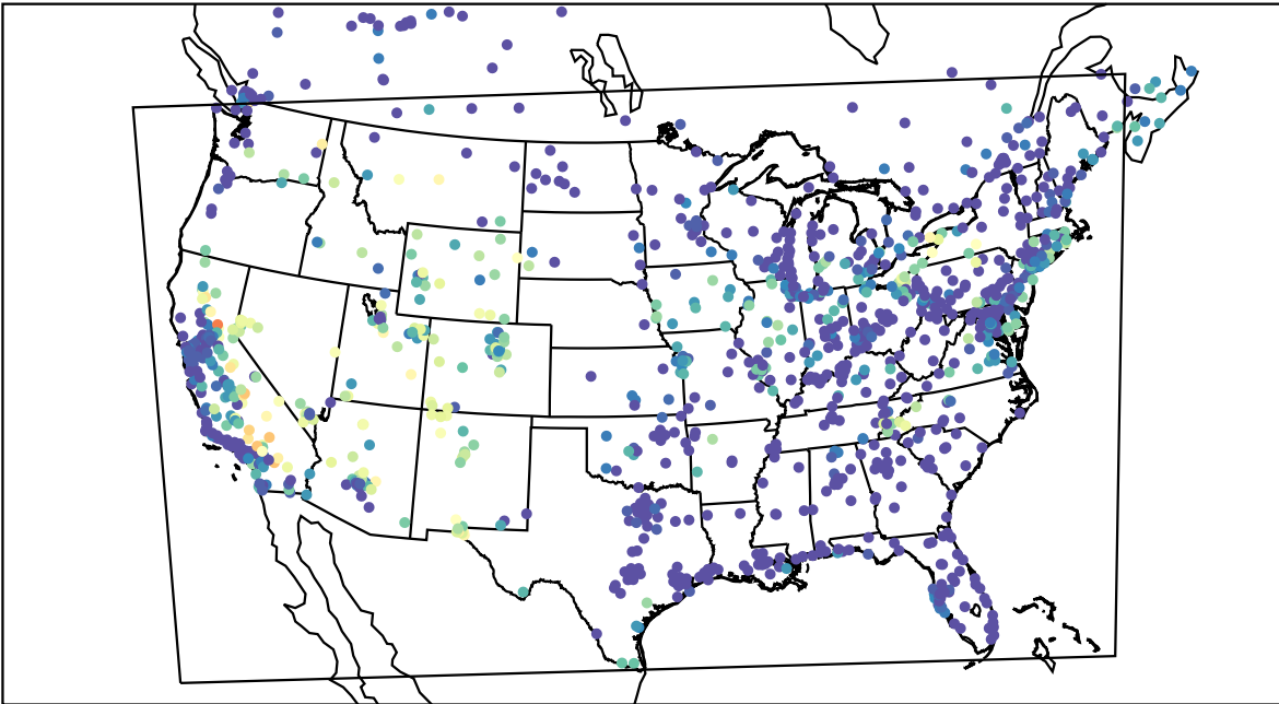
AirNOW (2021-07-07_08:00:00)
