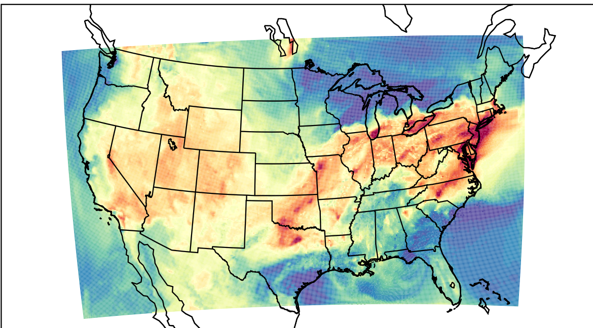
WRF (2021-07-07_18:00:00)
