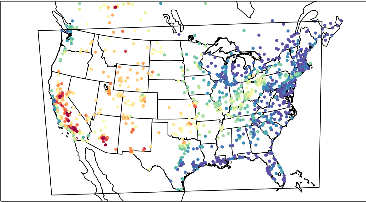
AirNOW (2021-07-08_23:00:00)
