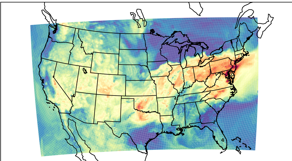
WRF (2021-07-07_15:00:00)
