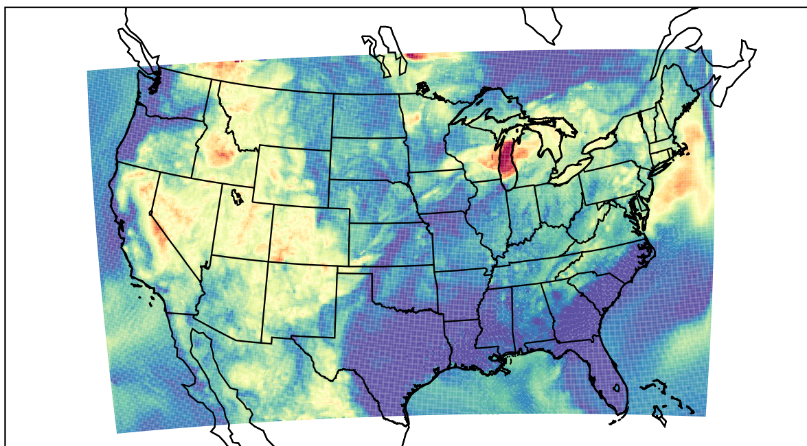
WRF (2021-07-15_12:00:00)
