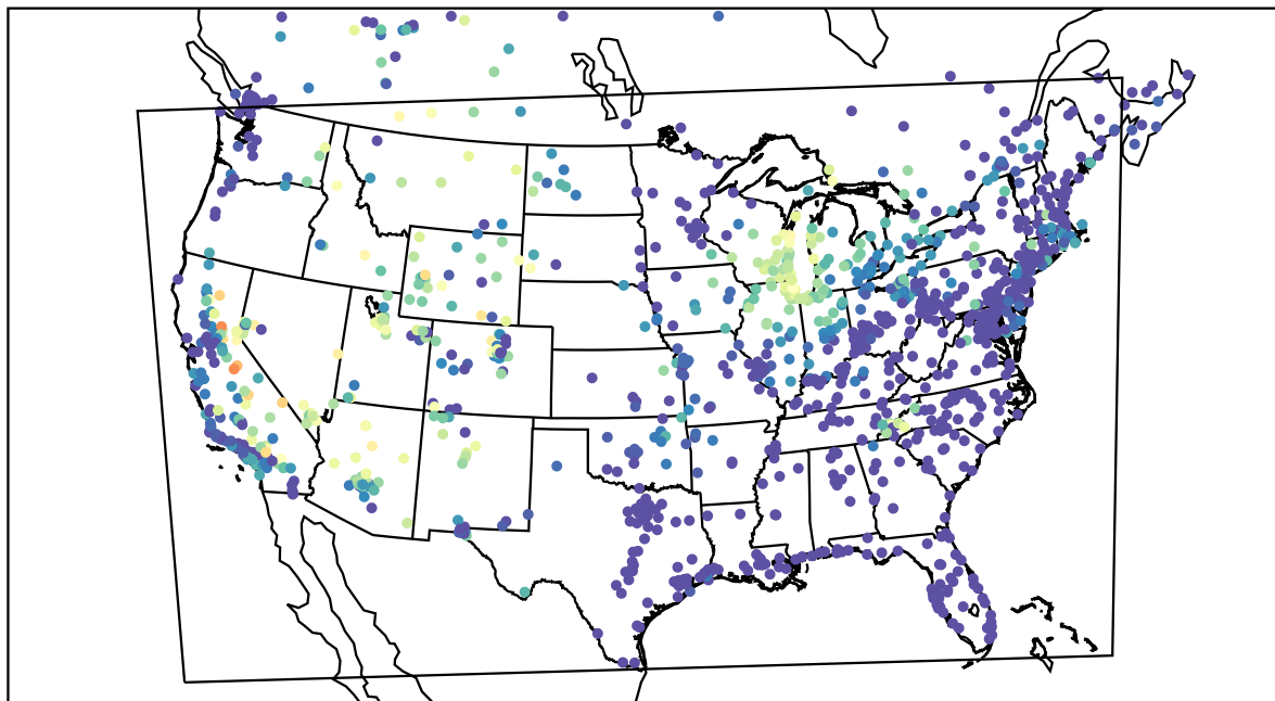
AirNOW (2021-07-15_11:00:00)
