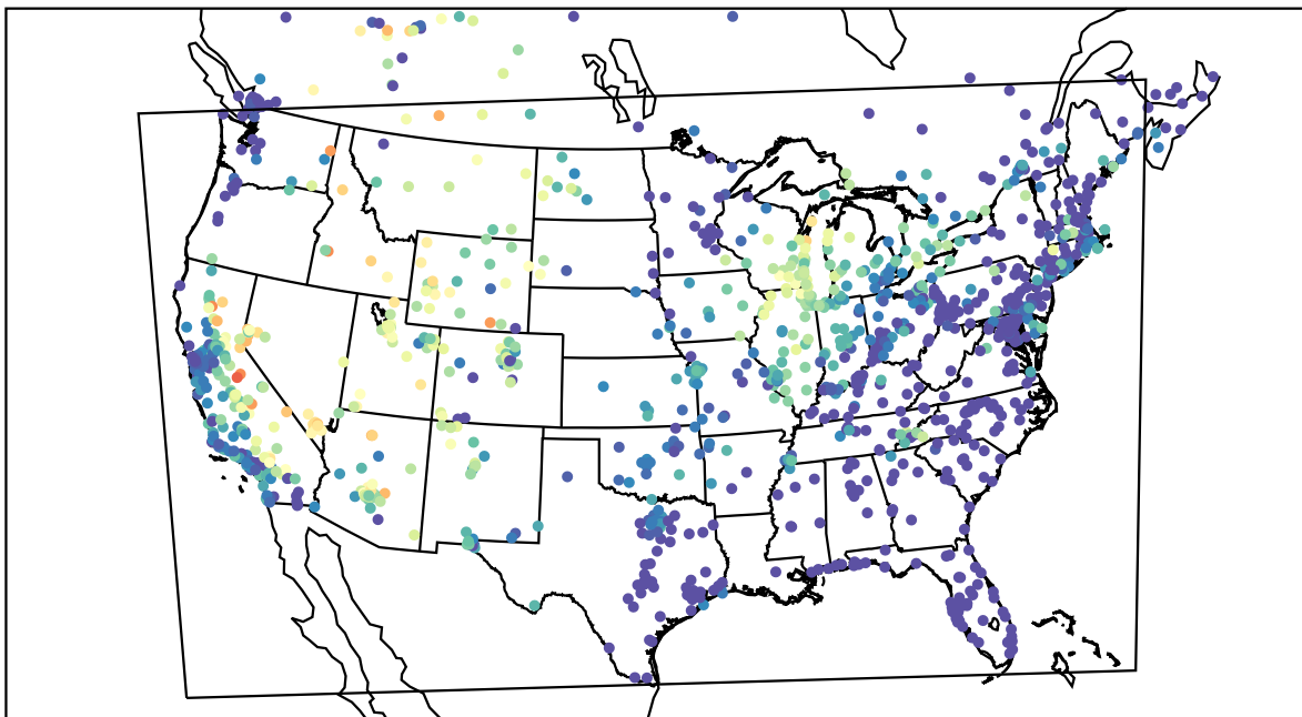
AirNOW (2021-07-15_07:00:00)
