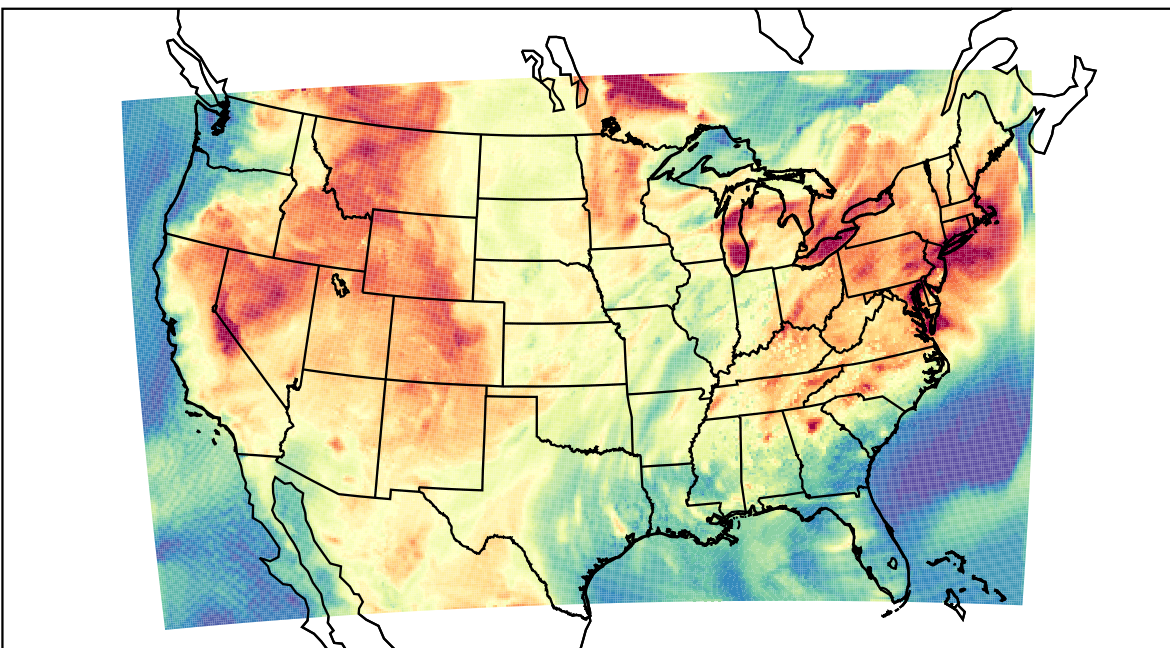
WRF (2021-07-15_19:00:00)
