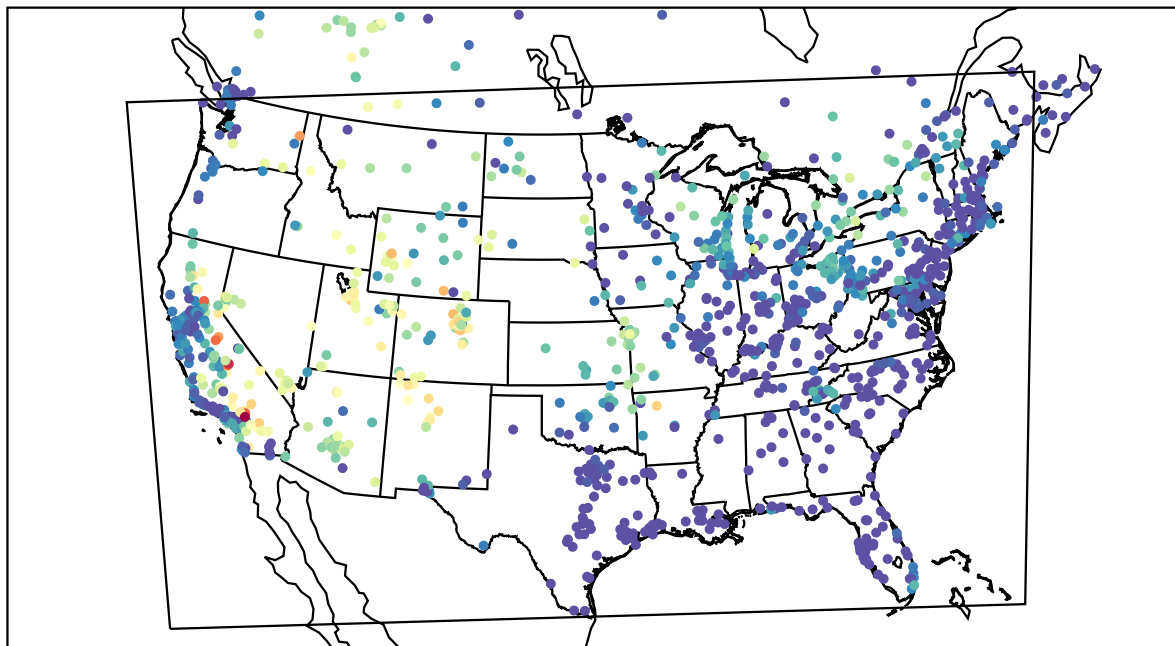
AirNOW (2021-07-14_07:00:00)
