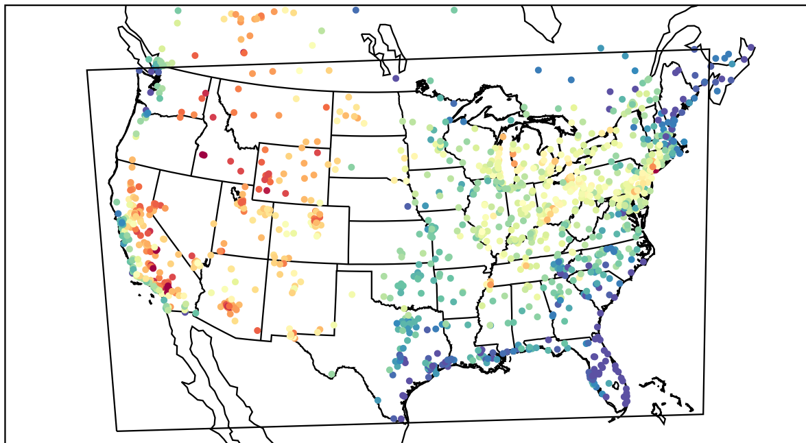
AirNOW (2021-07-14_22:00:00)
