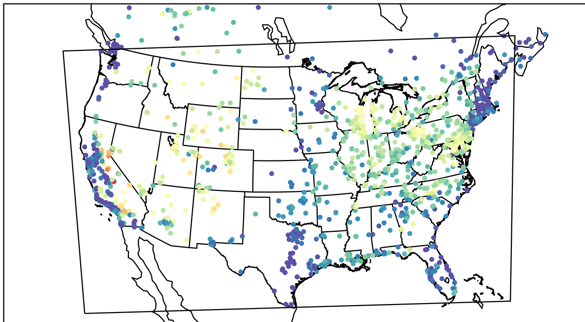
AirNOW (2021-07-14_15:00:00)
