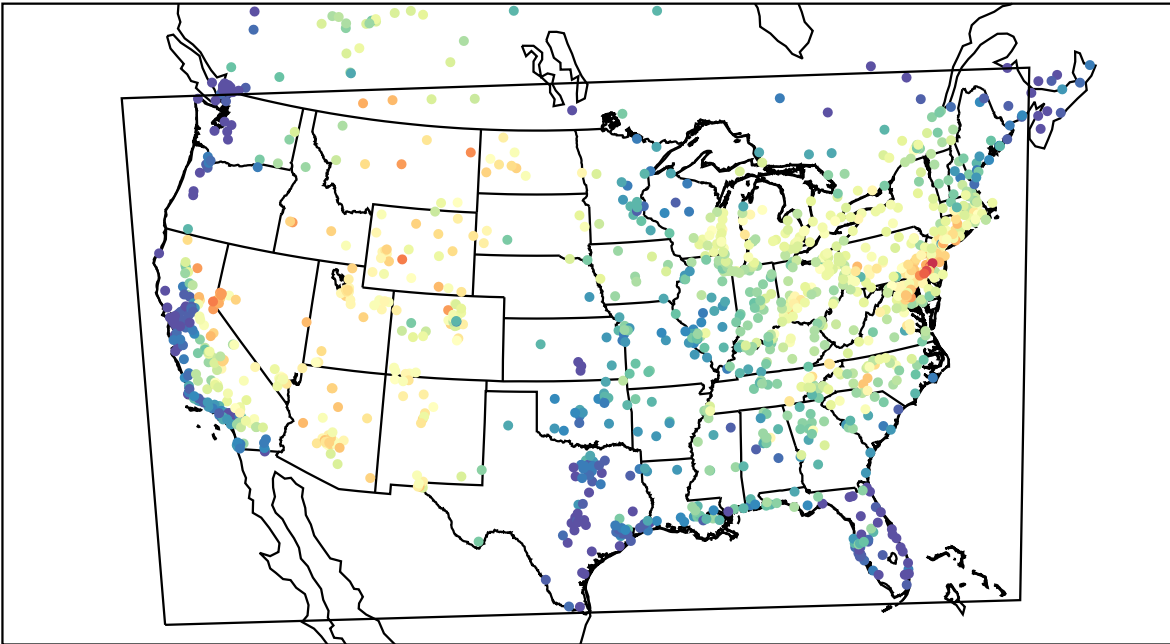
AirNOW (2021-07-15_16:00:00)
