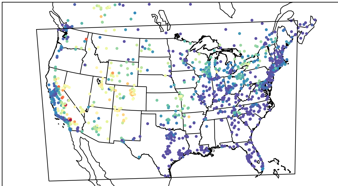
AirNOW (2021-07-14_06:00:00)
