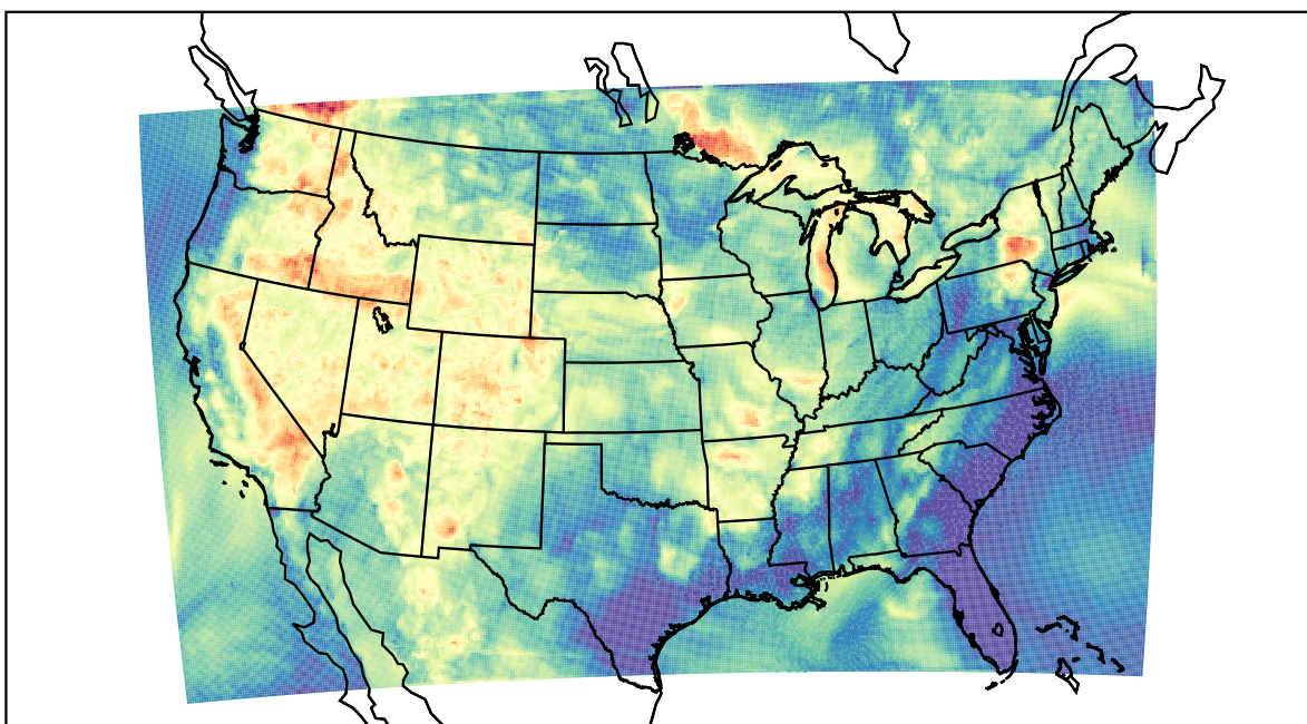
WRF (2021-07-14_05:00:00)
