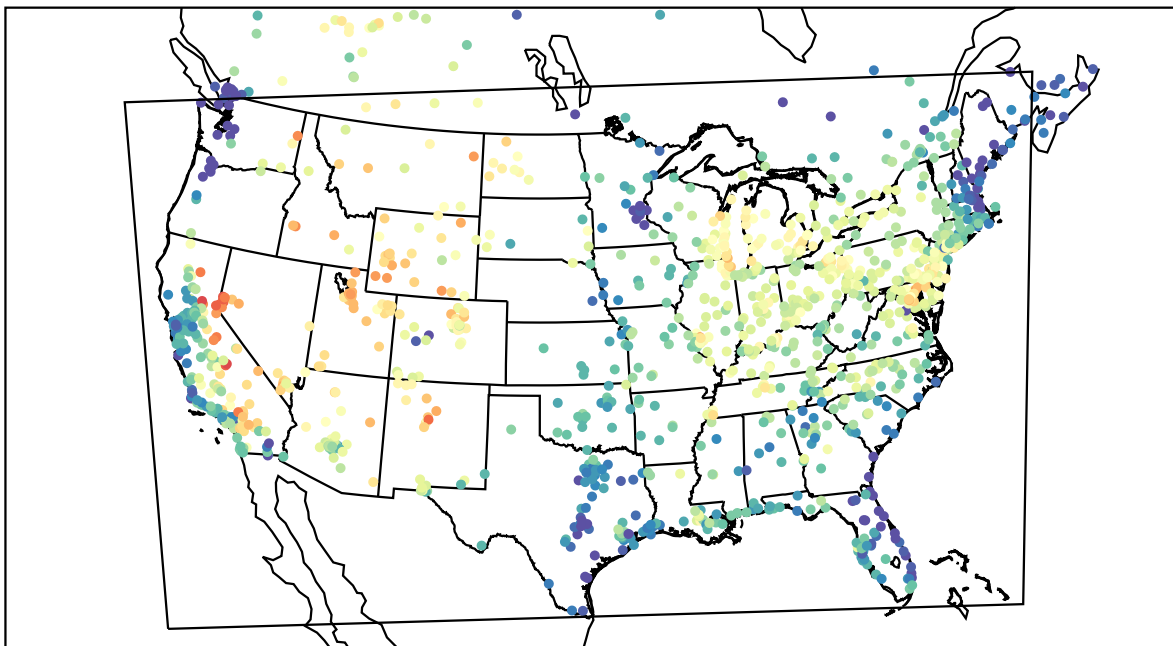
AirNOW (2021-07-14_17:00:00)
