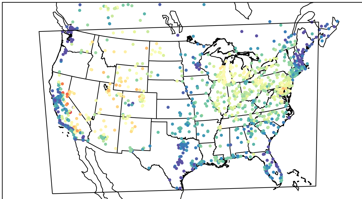
AirNOW (2021-07-14_16:00:00)
