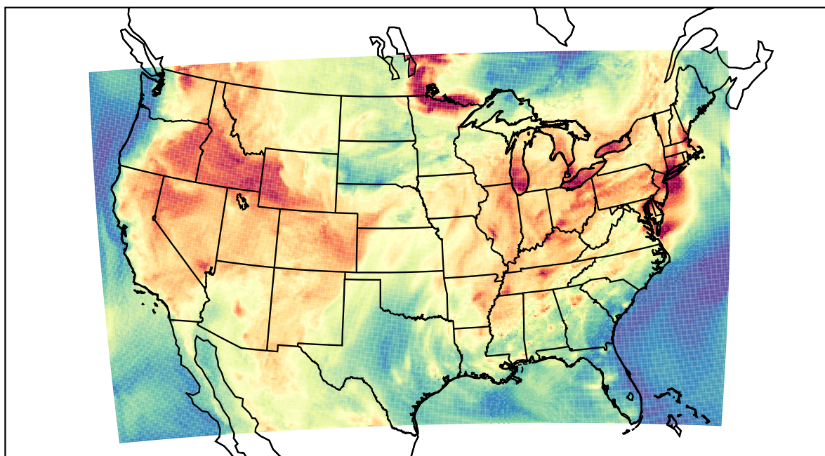
WRF (2021-07-14_19:00:00)
