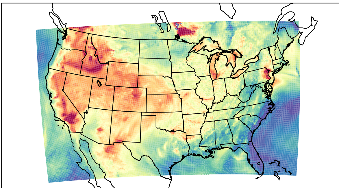
WRF (2021-07-14_00:00:00)
