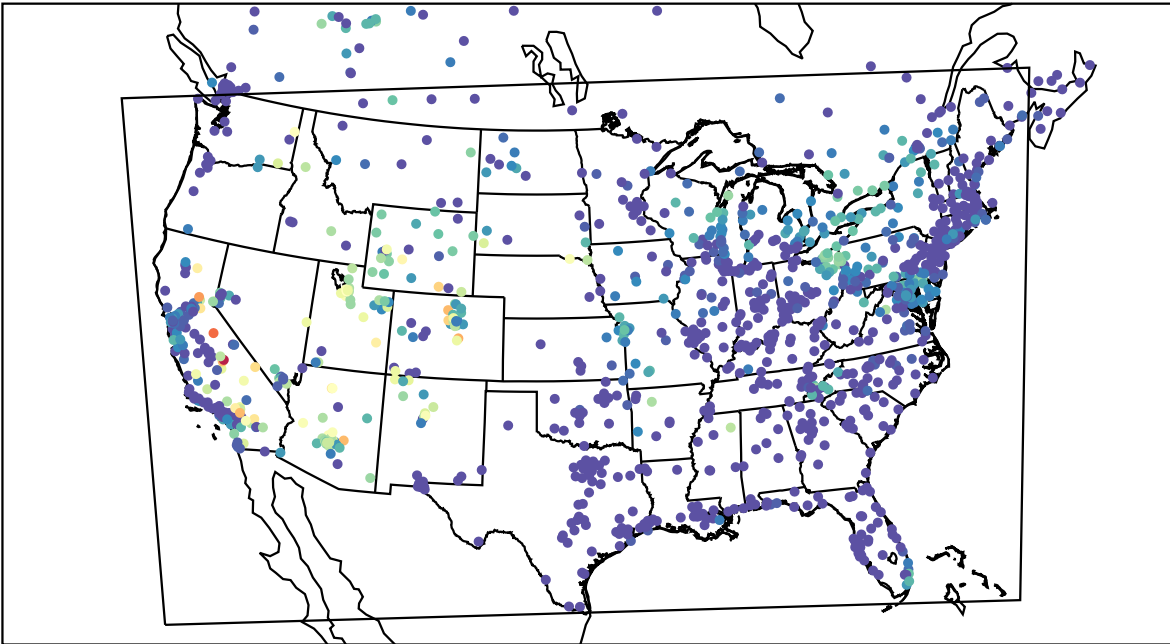
AirNOW (2021-07-14_12:00:00)
