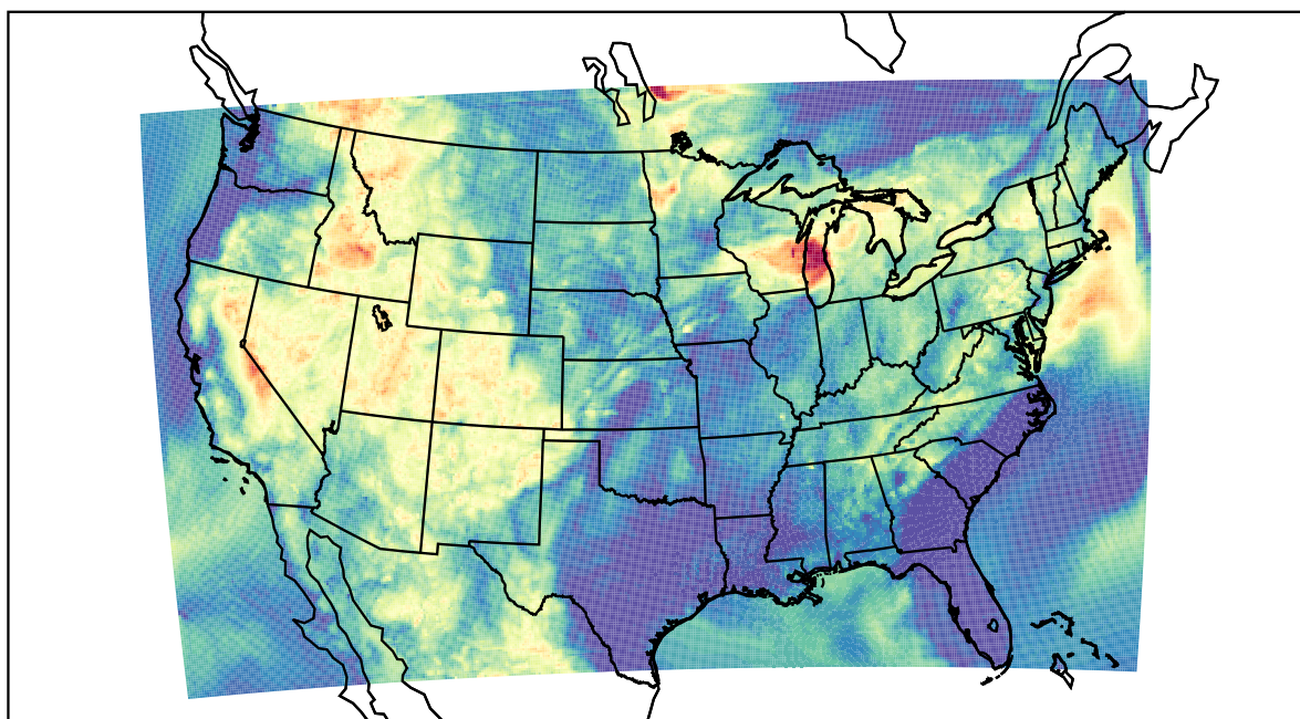
WRF (2021-07-15_10:00:00)
