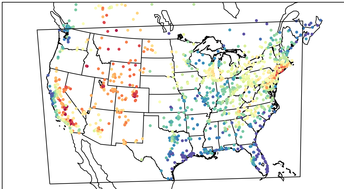
AirNOW (2021-07-15_22:00:00)
