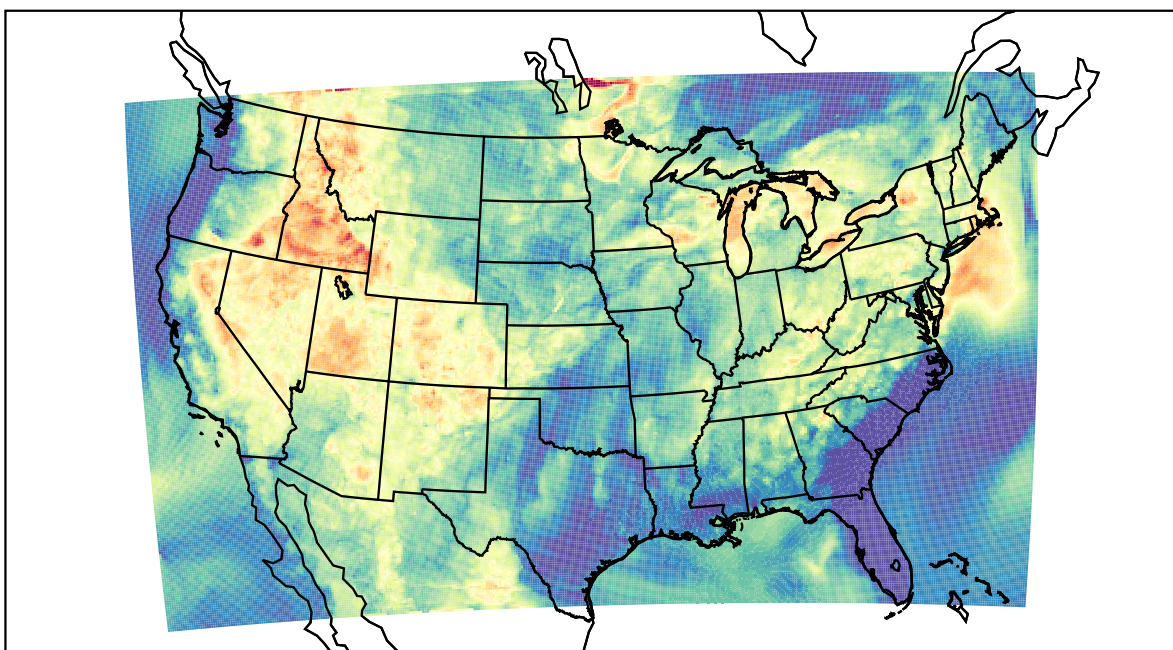
WRF (2021-07-15_05:00:00)
