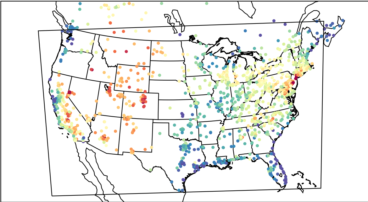
AirNOW (2021-07-15_19:00:00)
