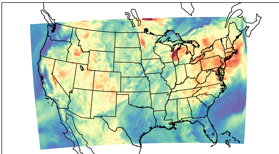
WRF (2021-07-15_15:00:00)
