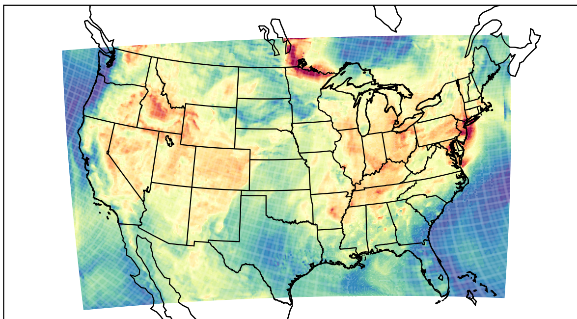
WRF (2021-07-14_16:00:00)
