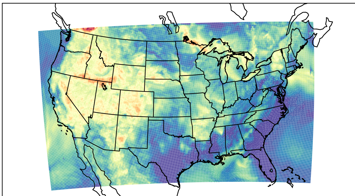
WRF (2021-07-14_08:00:00)
