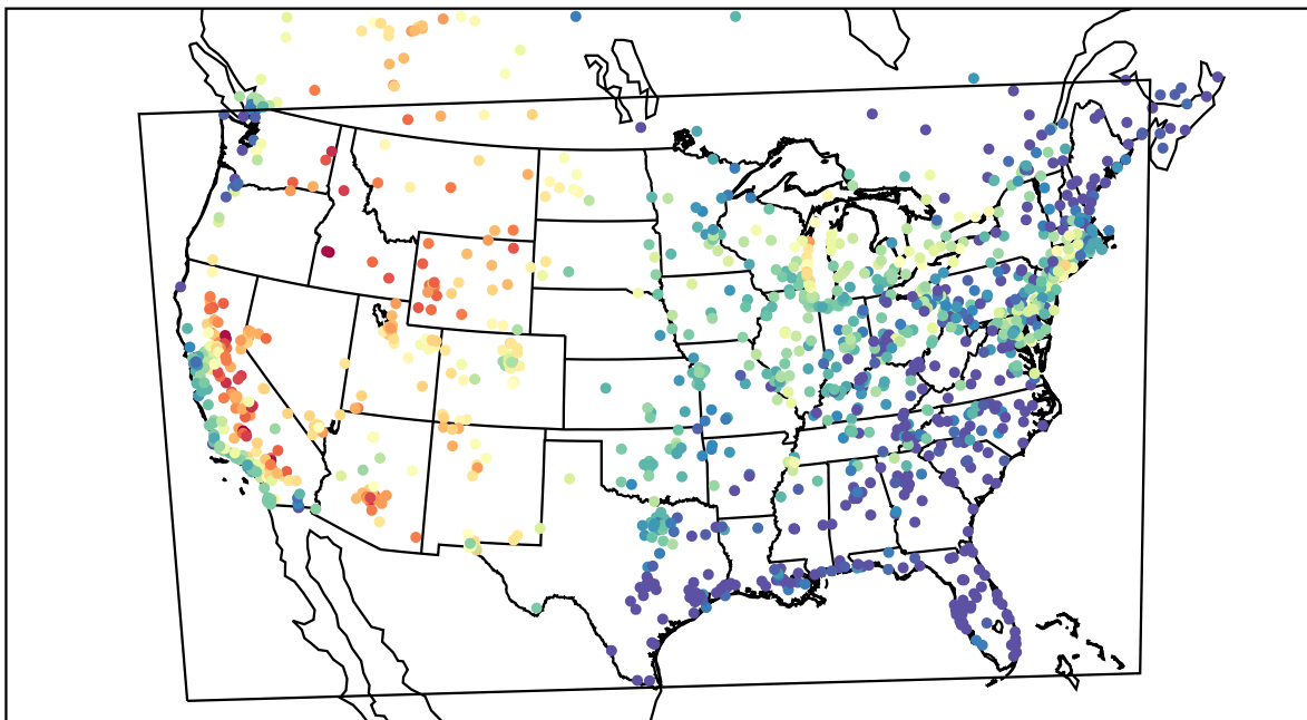
AirNOW (2021-07-15_01:00:00)
