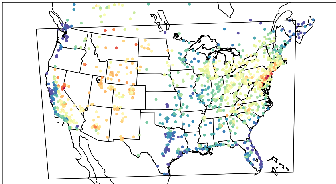
AirNOW (2021-07-15_17:00:00)
