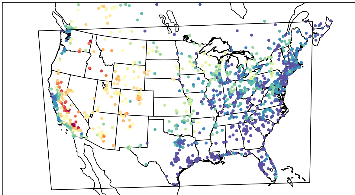
AirNOW (2021-07-14_02:00:00)
