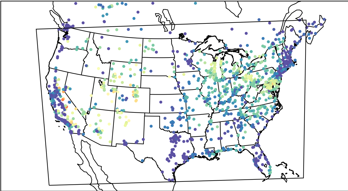
AirNOW (2021-07-14_14:00:00)
