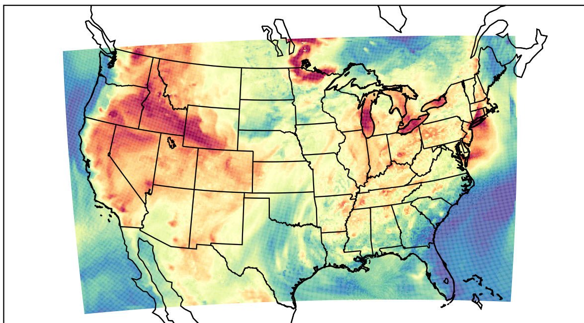
WRF (2021-07-14_23:00:00)
