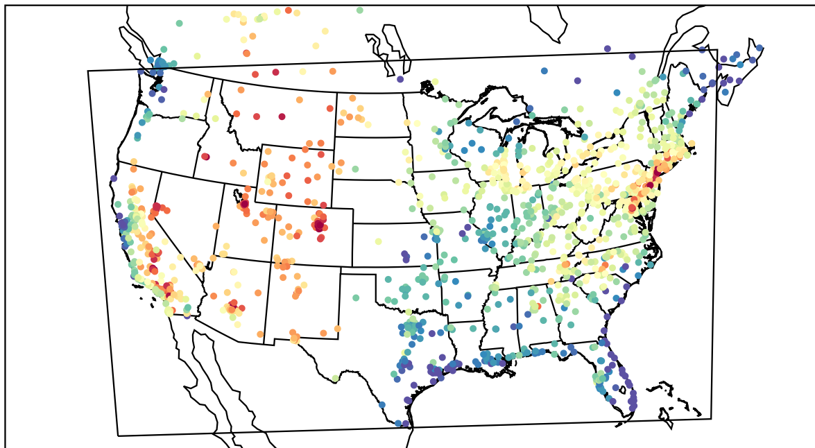
AirNOW (2021-07-15_20:00:00)
