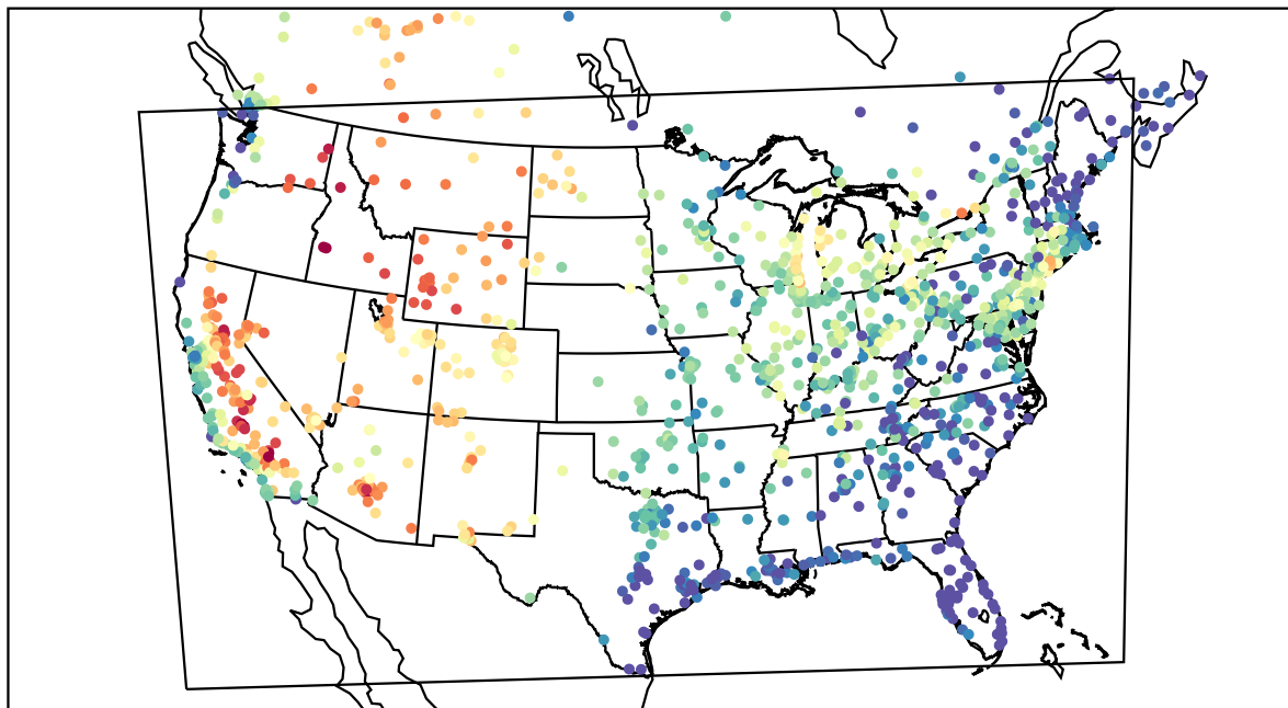
AirNOW (2021-07-15_00:00:00)
