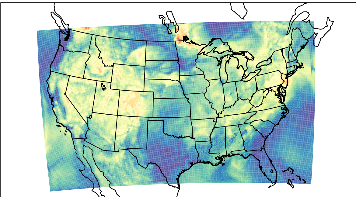
WRF (2021-07-14_14:00:00)
