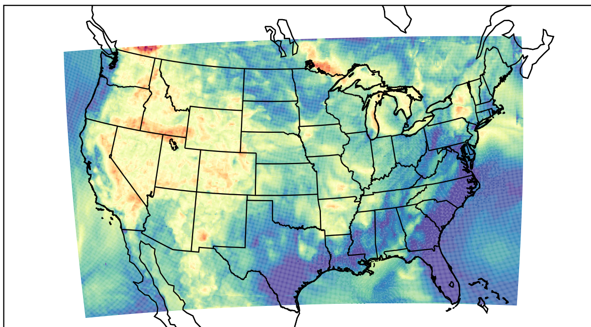
WRF (2021-07-14_06:00:00)
