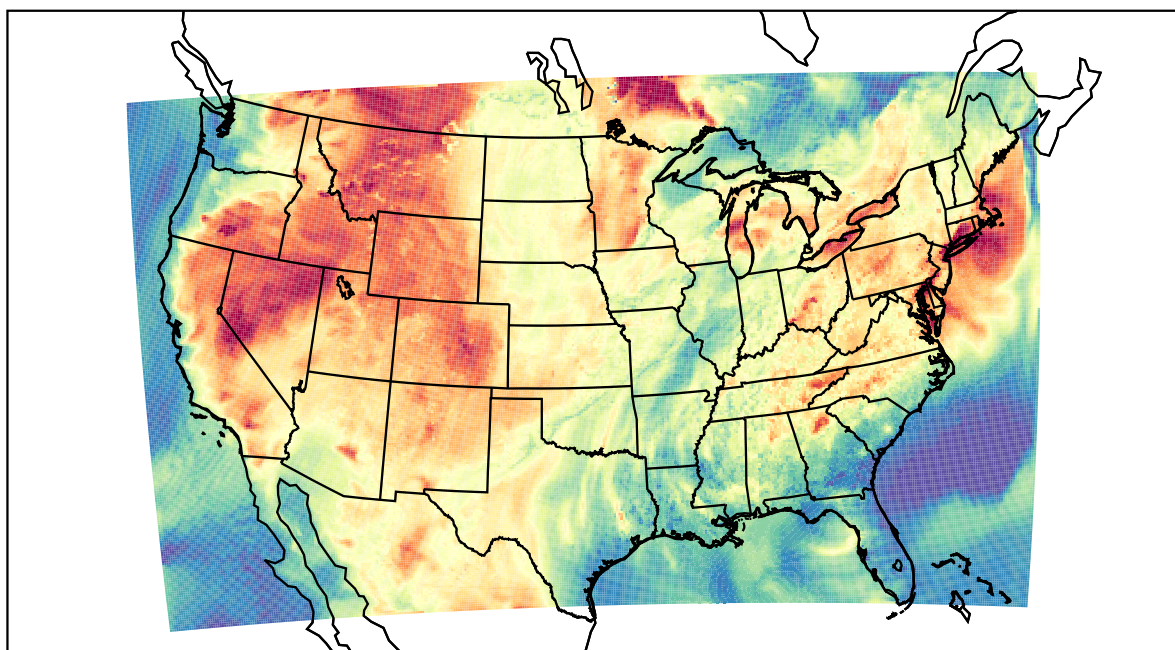
WRF (2021-07-15_23:00:00)
