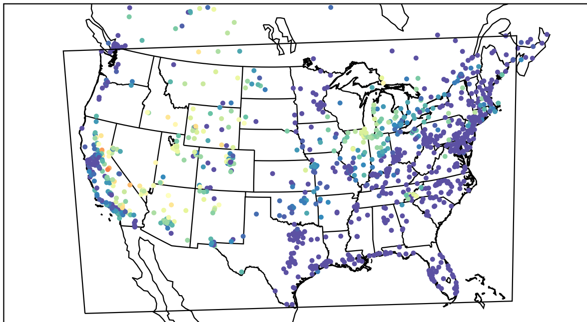
AirNOW (2021-07-15_10:00:00)
