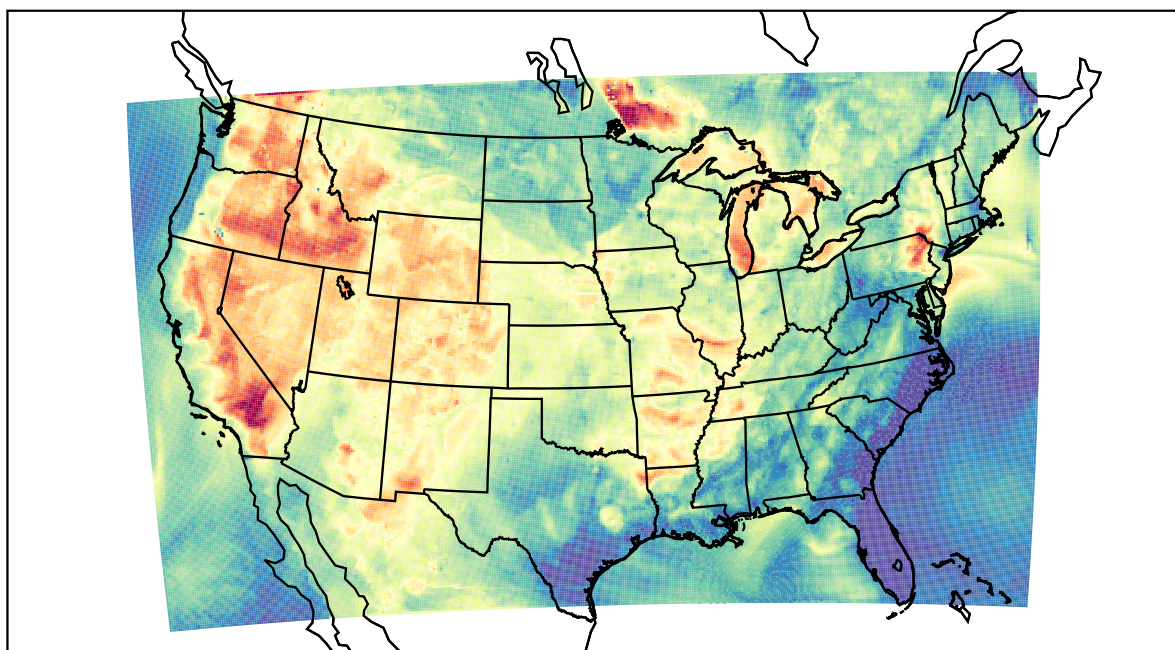
WRF (2021-07-14_02:00:00)
