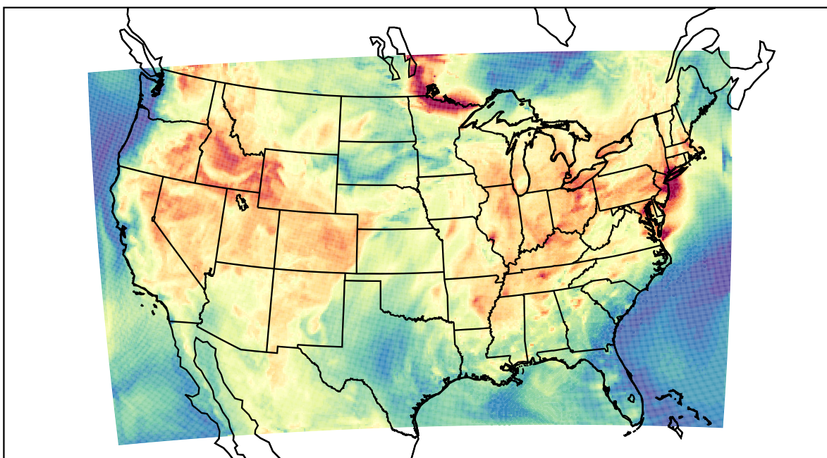
WRF (2021-07-14_17:00:00)
