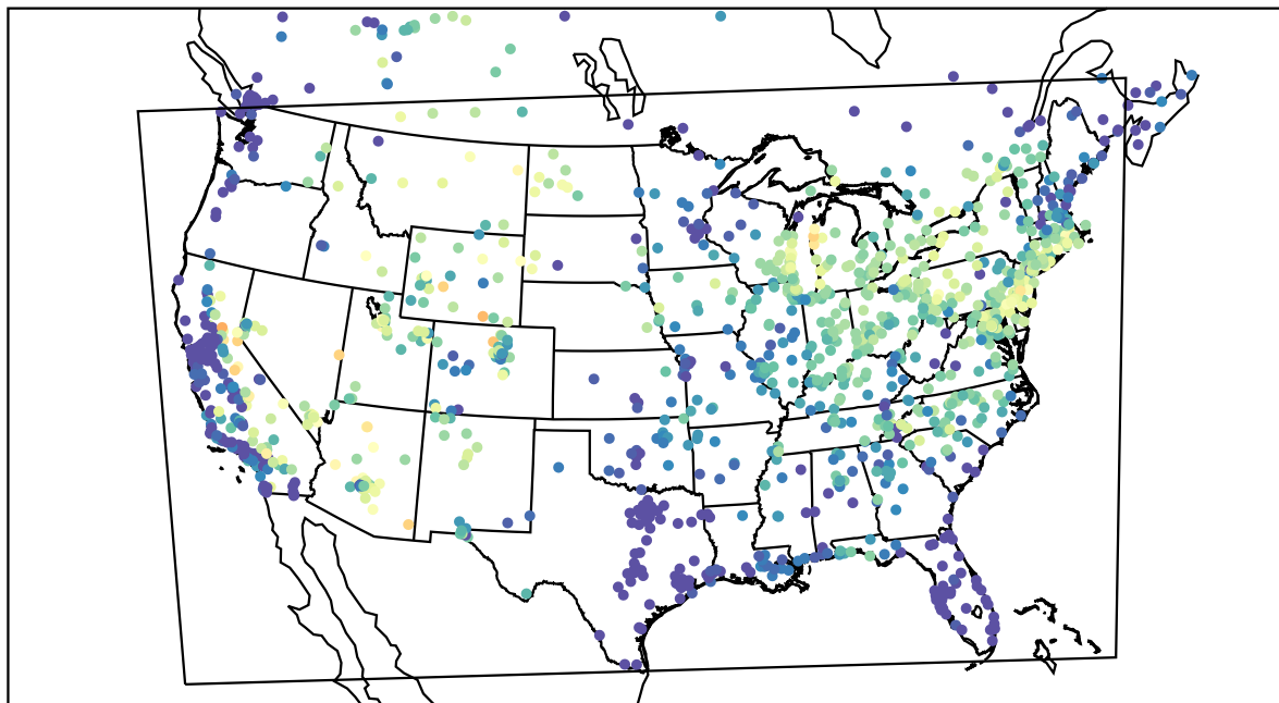
AirNOW (2021-07-15_14:00:00)
