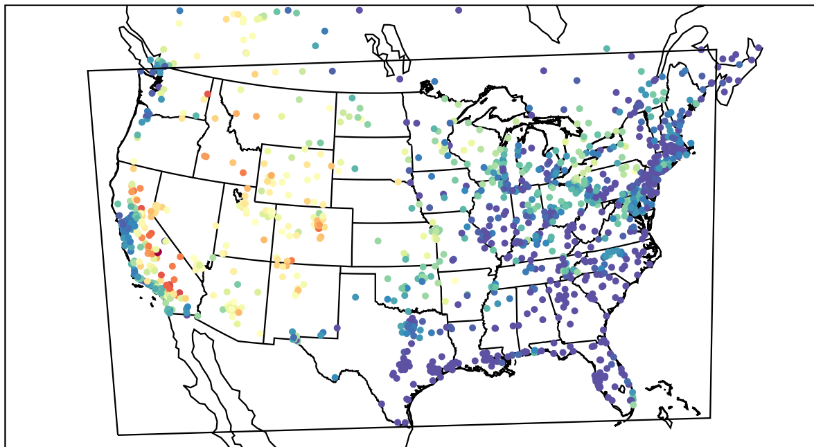
AirNOW (2021-07-14_03:00:00)
