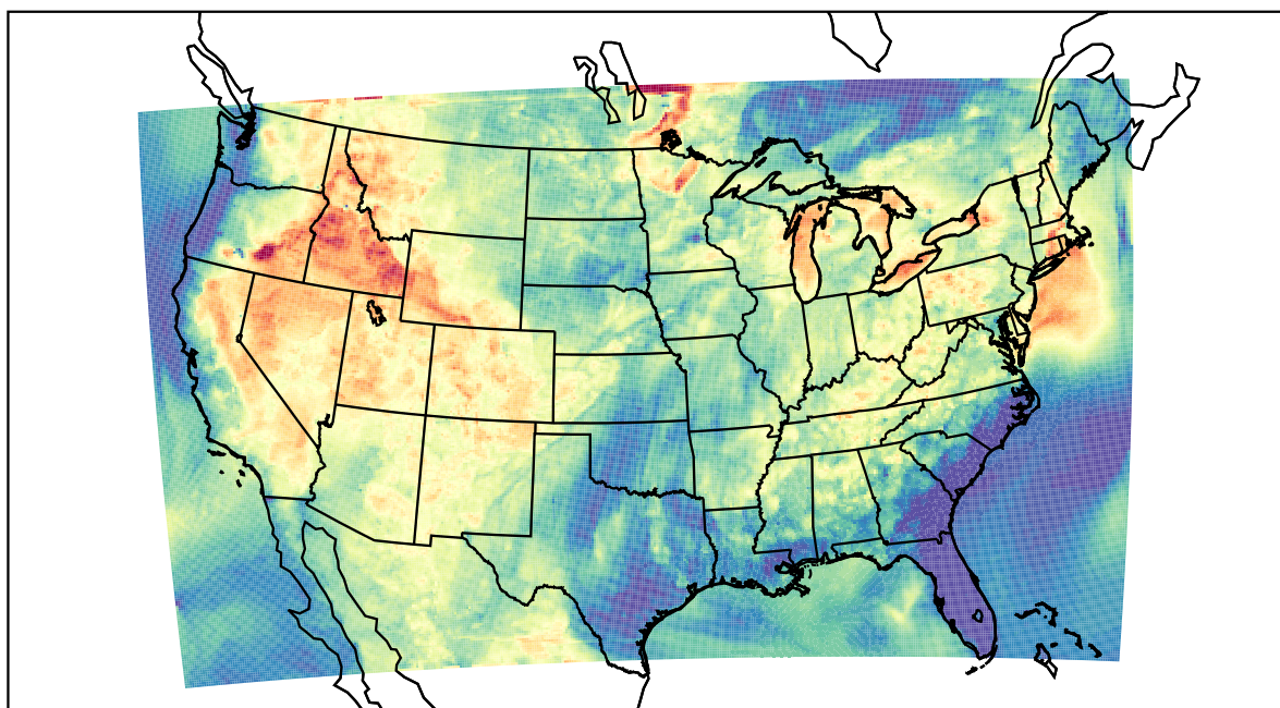
WRF (2021-07-15_03:00:00)
