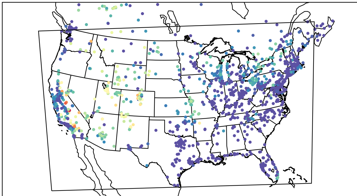
AirNOW (2021-07-14_09:00:00)
