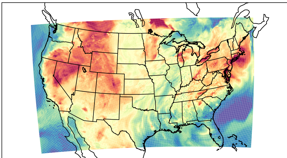
WRF (2021-07-15_22:00:00)
