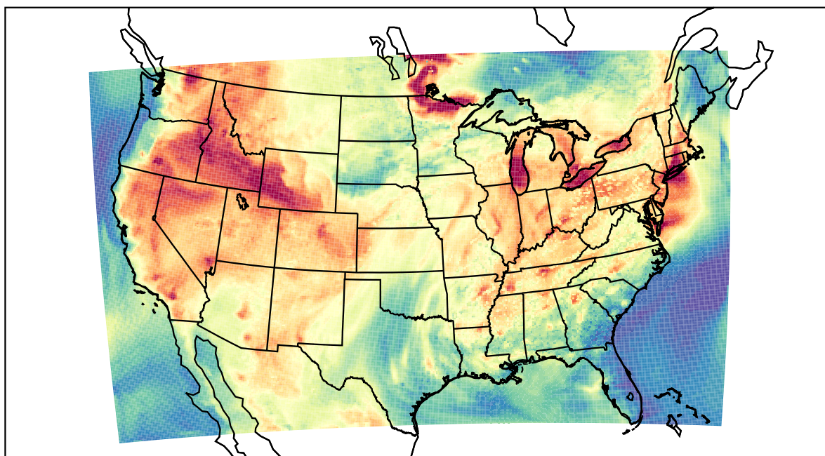
WRF (2021-07-14_22:00:00)
