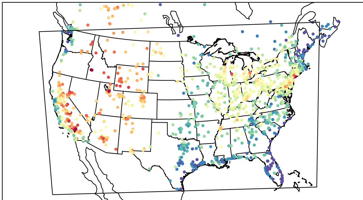
AirNOW (2021-07-14_21:00:00)
