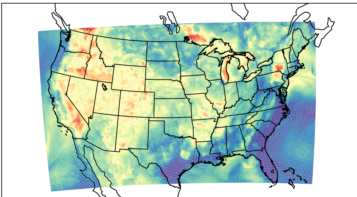
WRF (2021-07-14_04:00:00)
