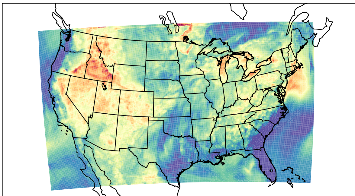
WRF (2021-07-15_04:00:00)
