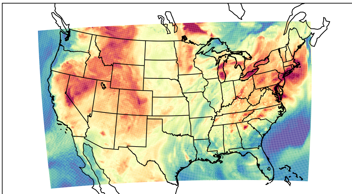
WRF (2021-07-15_20:00:00)
