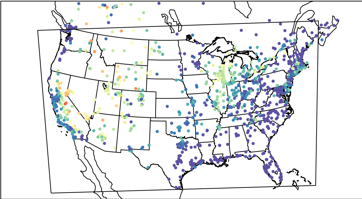
AirNOW (2021-07-15_06:00:00)
