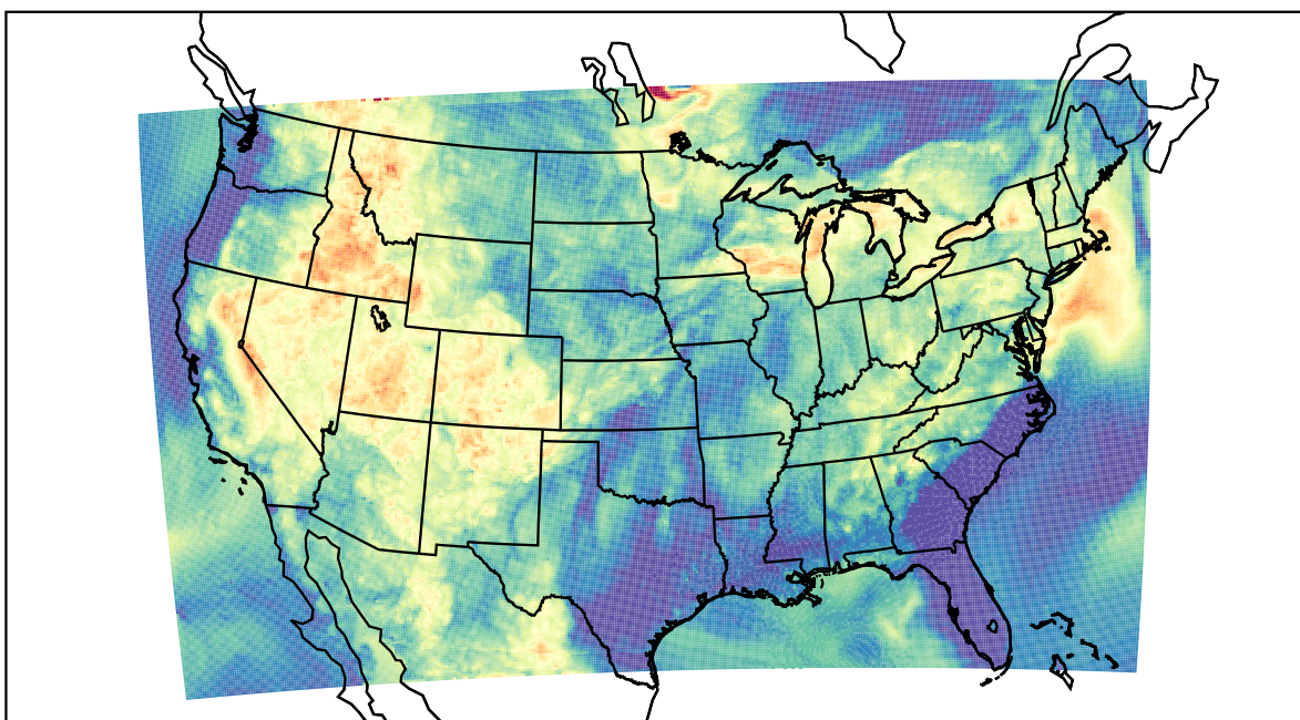
WRF (2021-07-15_07:00:00)
