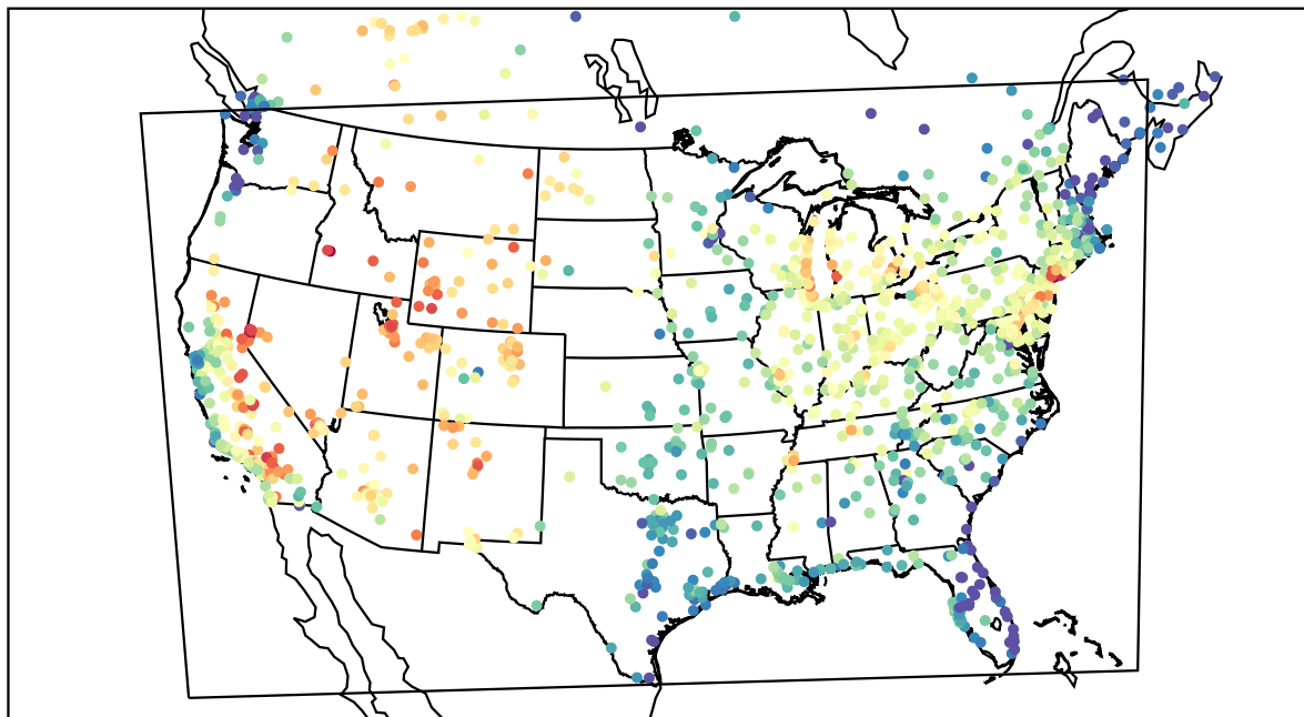
AirNOW (2021-07-14_19:00:00)
