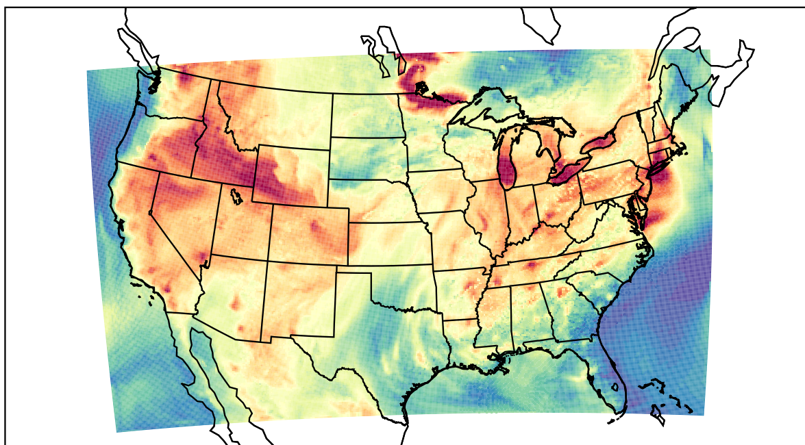
WRF (2021-07-14_21:00:00)
