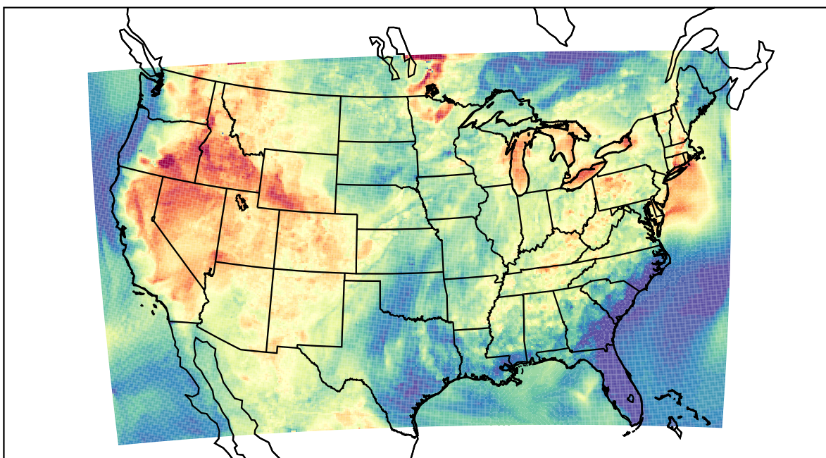
WRF (2021-07-15_02:00:00)
