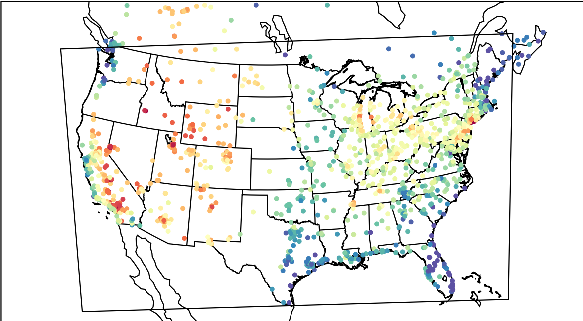
AirNOW (2021-07-14_20:00:00)
