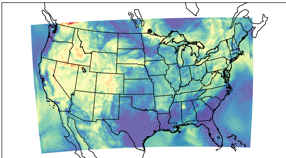
WRF (2021-07-14_13:00:00)
