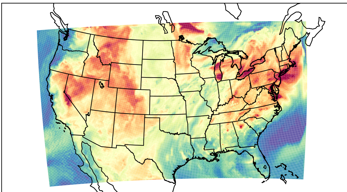
WRF (2021-07-15_18:00:00)
