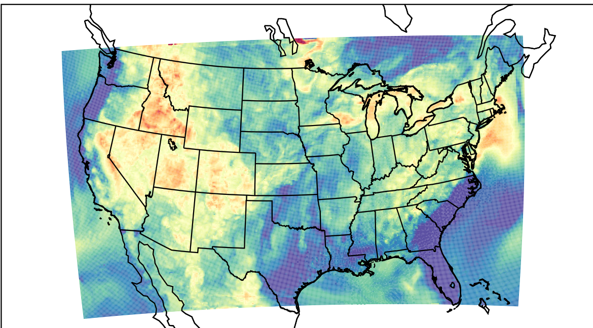
WRF (2021-07-15_06:00:00)
