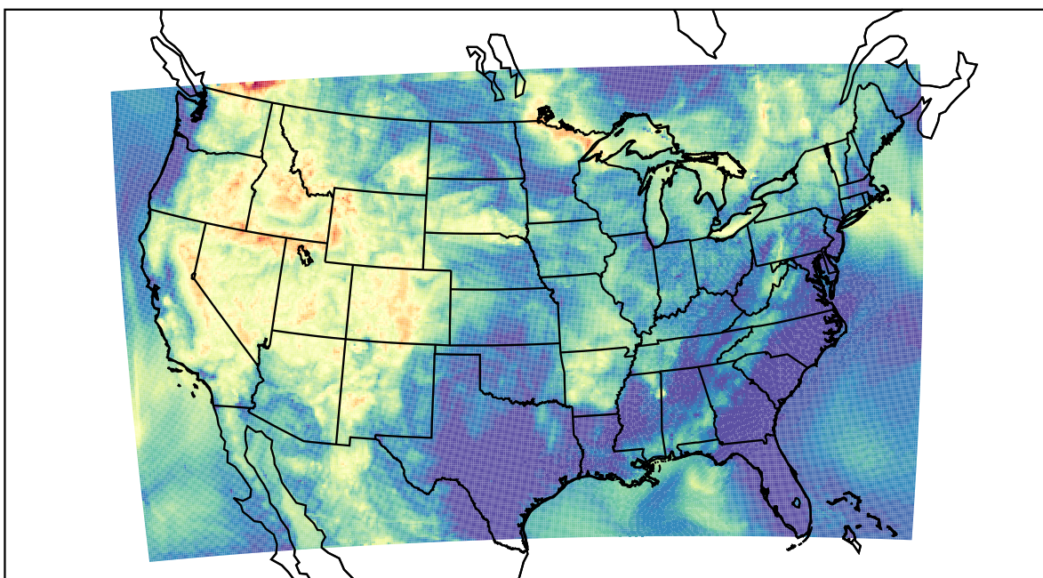
WRF (2021-07-14_11:00:00)
