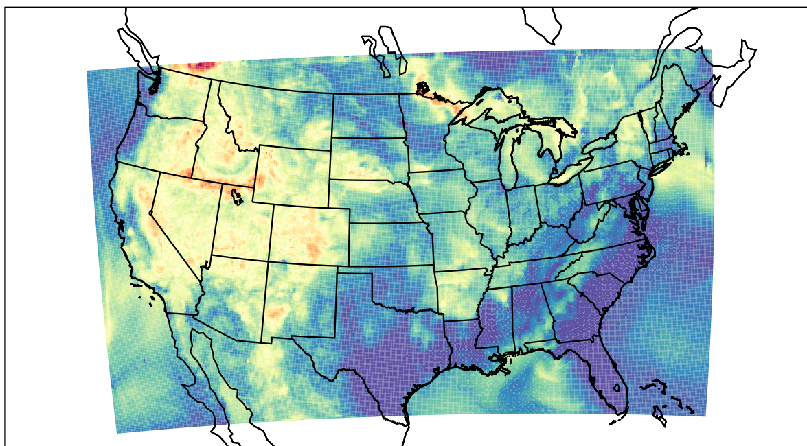
WRF (2021-07-14_09:00:00)
