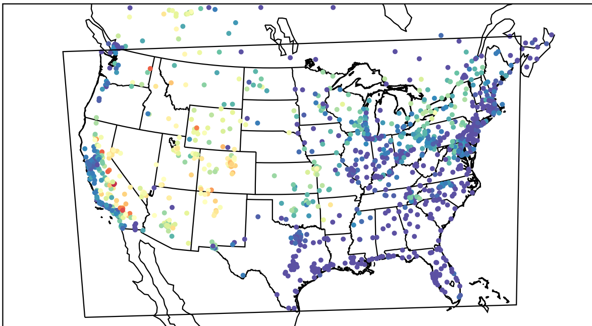
AirNOW (2021-07-14_05:00:00)
