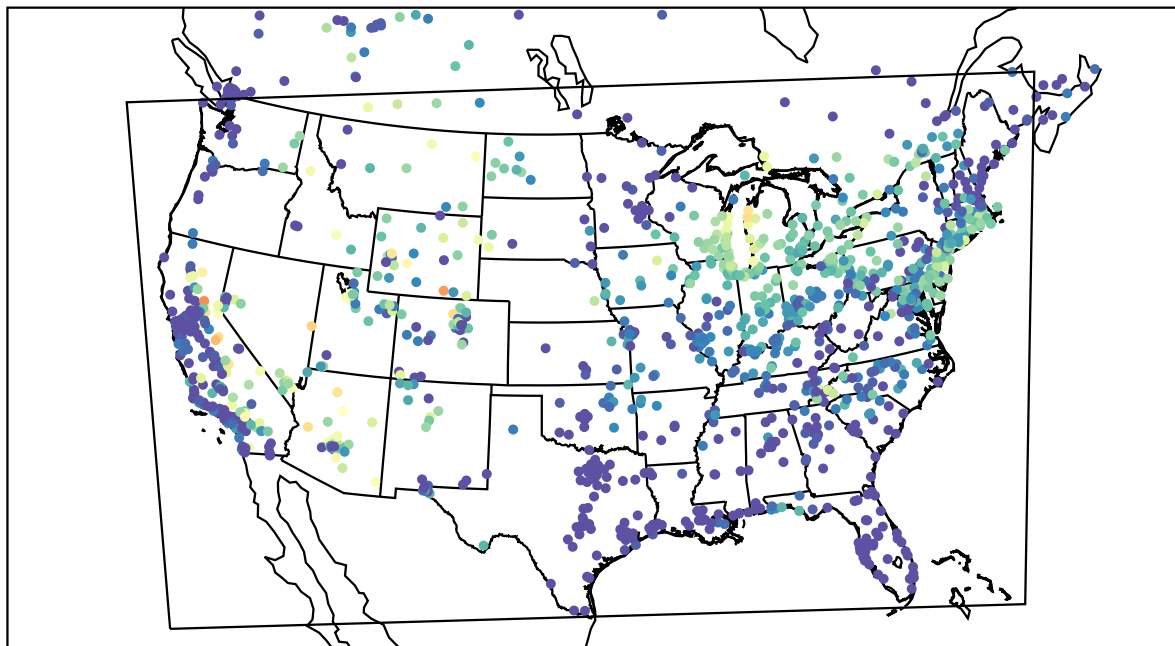
AirNOW (2021-07-15_13:00:00)
