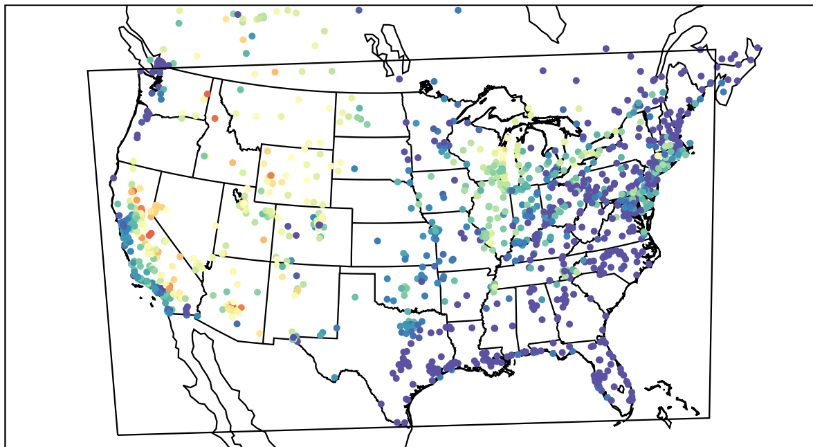
AirNOW (2021-07-15_04:00:00)
