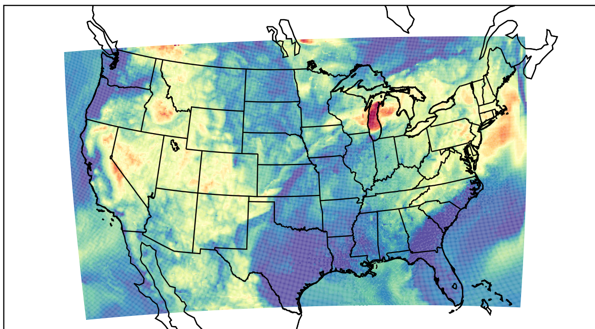
WRF (2021-07-15_13:00:00)
