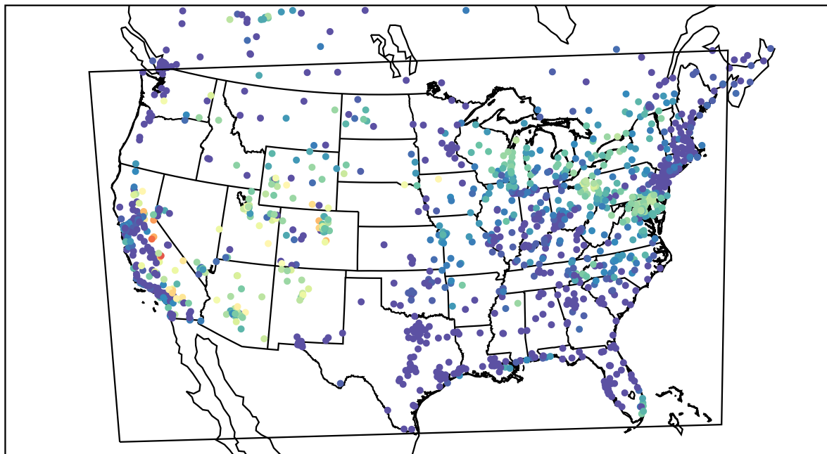
AirNOW (2021-07-14_13:00:00)
