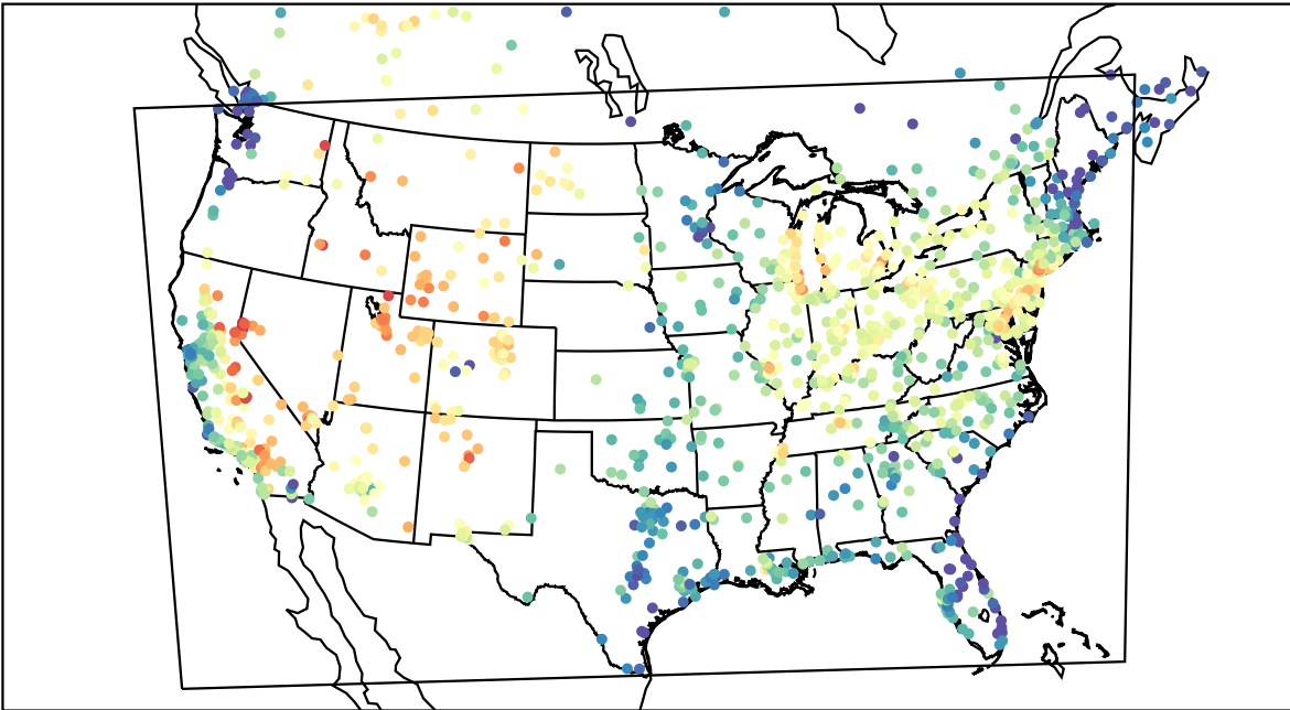
AirNOW (2021-07-14_18:00:00)
