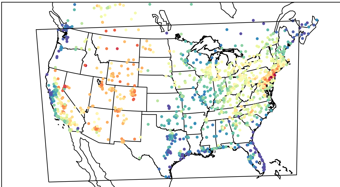
AirNOW (2021-07-15_18:00:00)
