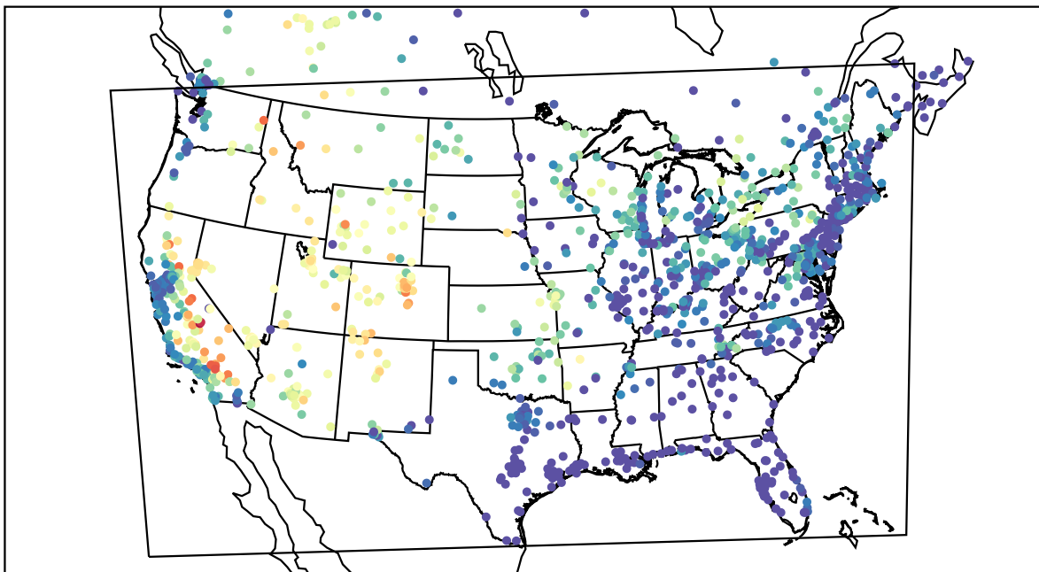
AirNOW (2021-07-14_04:00:00)
