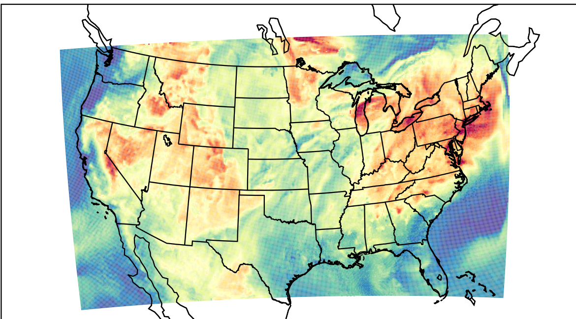
WRF (2021-07-15_16:00:00)
