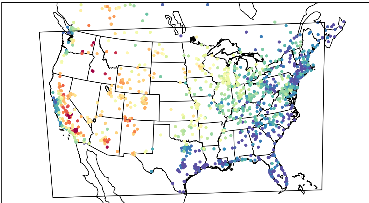
AirNOW (2021-07-14_00:00:00)
