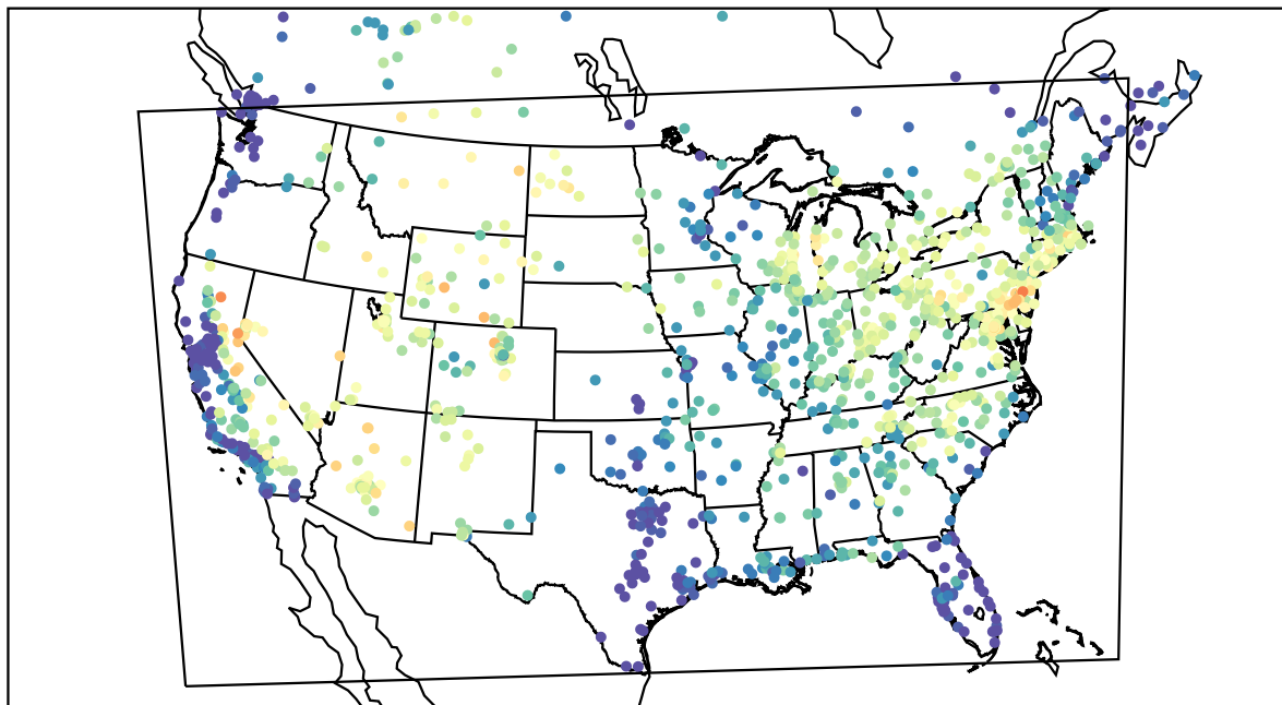
AirNOW (2021-07-15_15:00:00)
