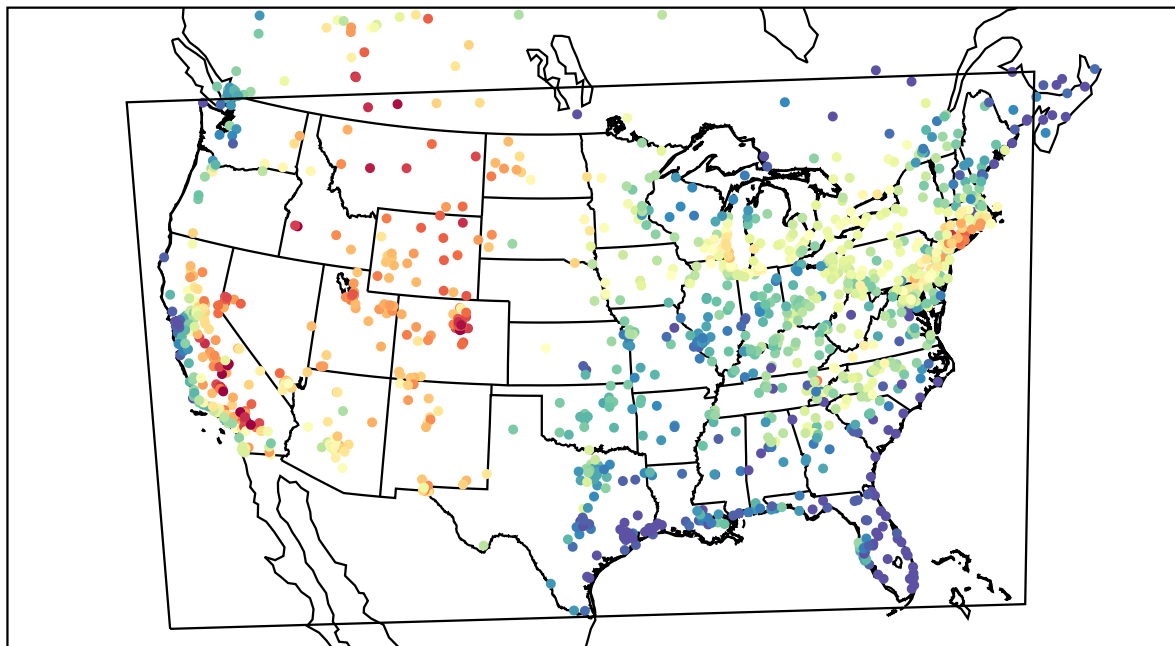
AirNOW (2021-07-15_23:00:00)
