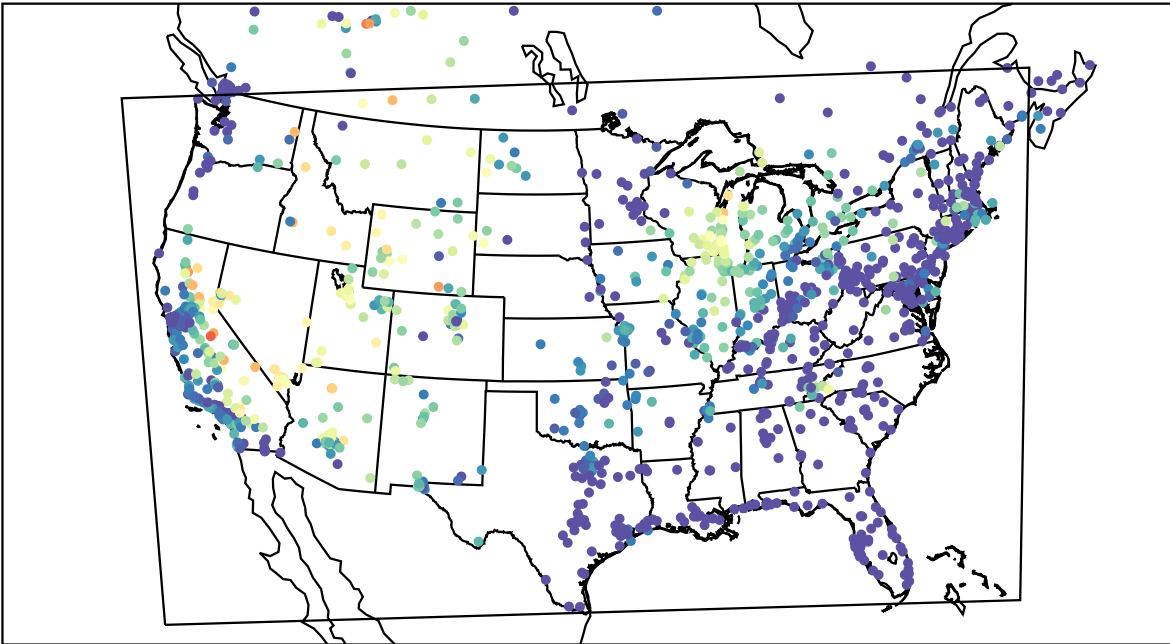
AirNOW (2021-07-15_08:00:00)
