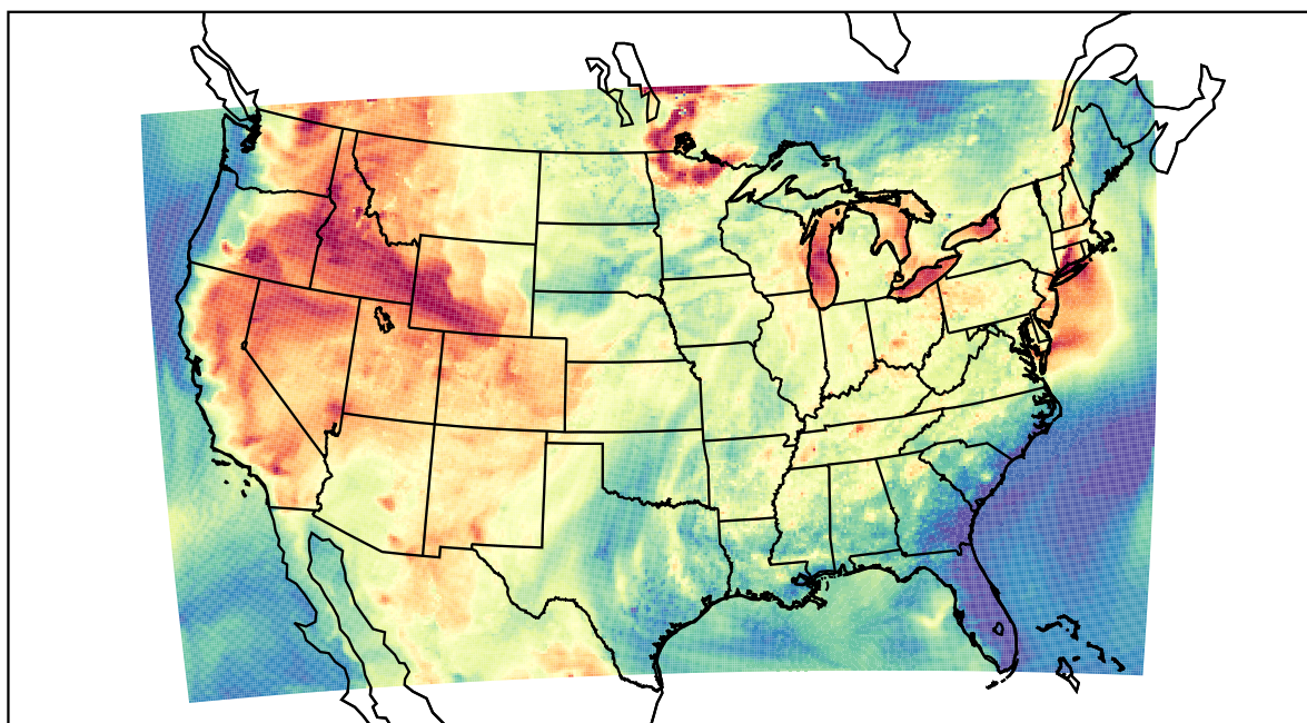
WRF (2021-07-15_00:00:00)
