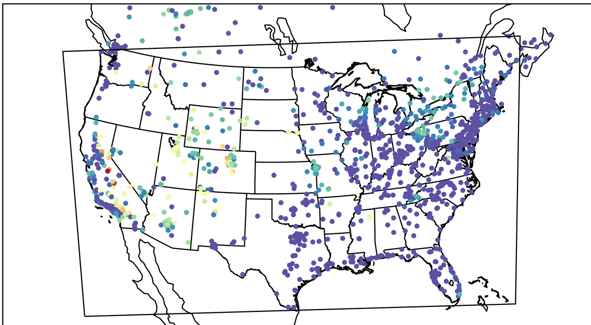
AirNOW (2021-07-14_11:00:00)
