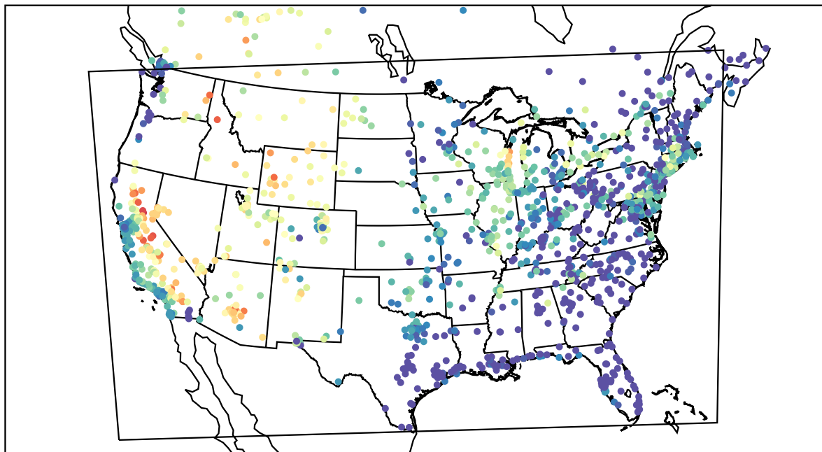
AirNOW (2021-07-15_03:00:00)
