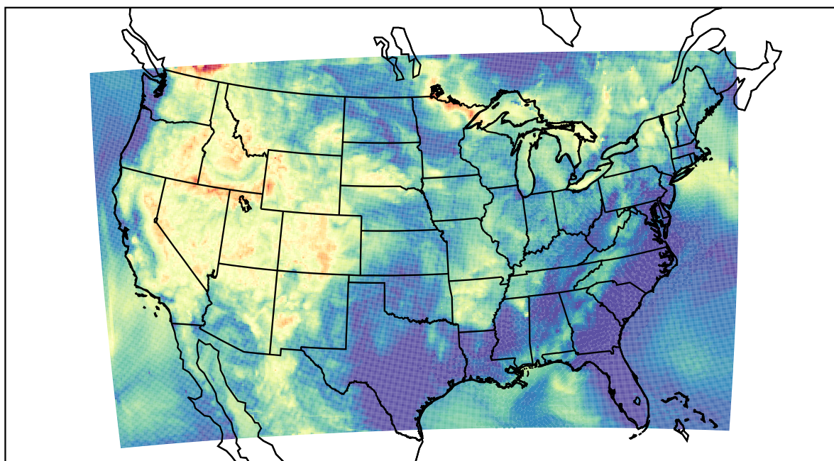
WRF (2021-07-14_10:00:00)
