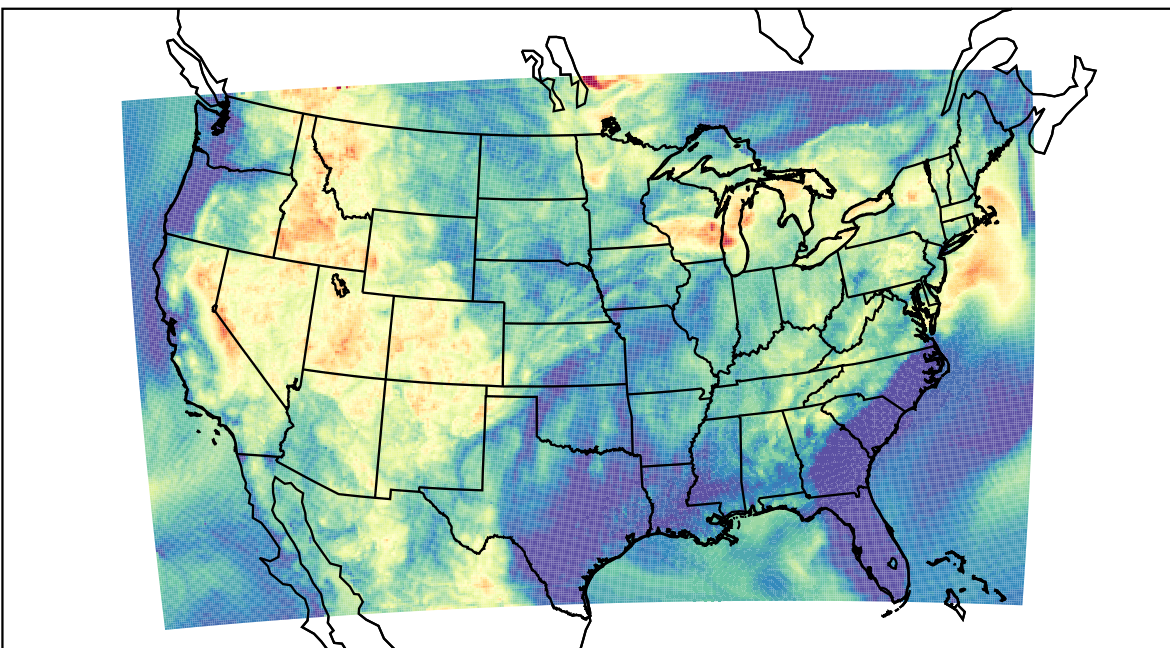
WRF (2021-07-15_08:00:00)
