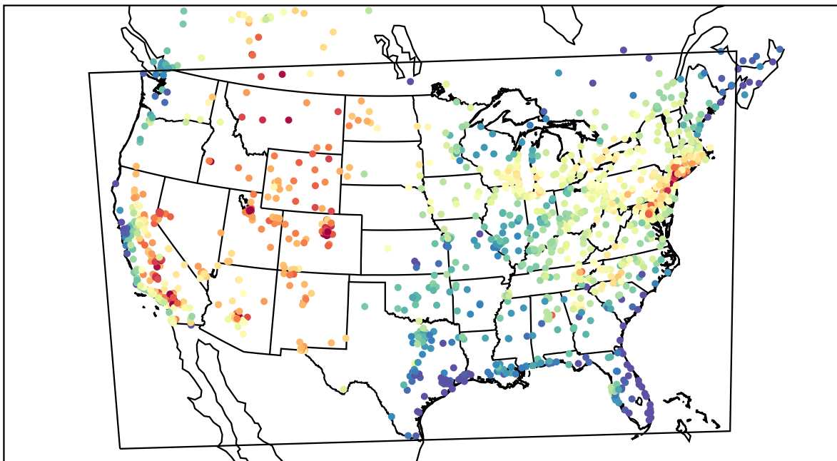
AirNOW (2021-07-15_21:00:00)
