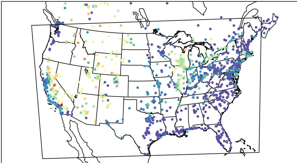
AirNOW (2021-07-15_05:00:00)
