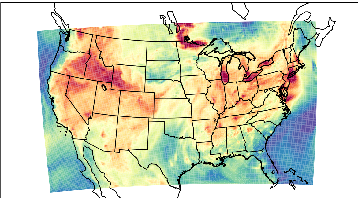
WRF (2021-07-14_20:00:00)
