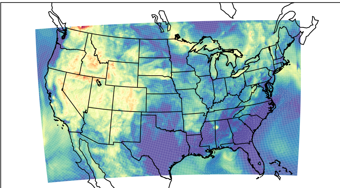
WRF (2021-07-14_12:00:00)
