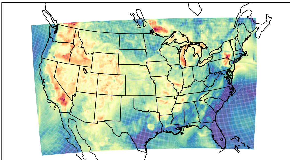
WRF (2021-07-14_03:00:00)
