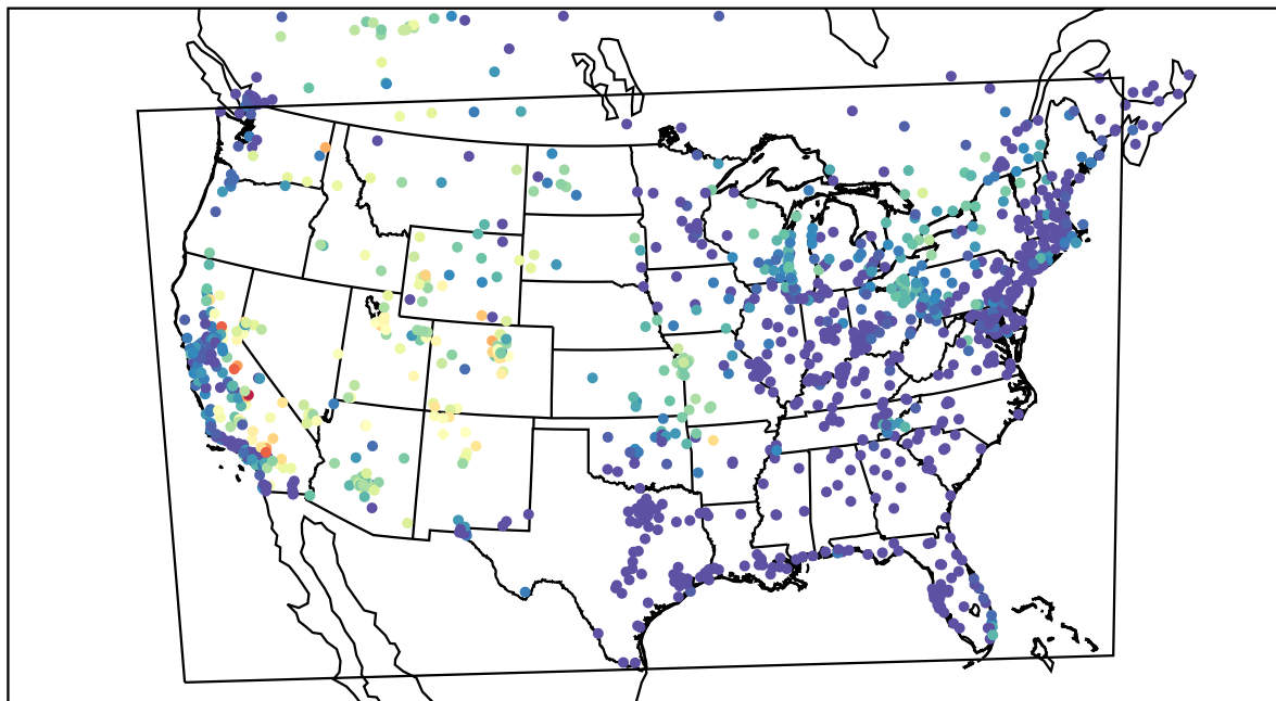
AirNOW (2021-07-14_08:00:00)
