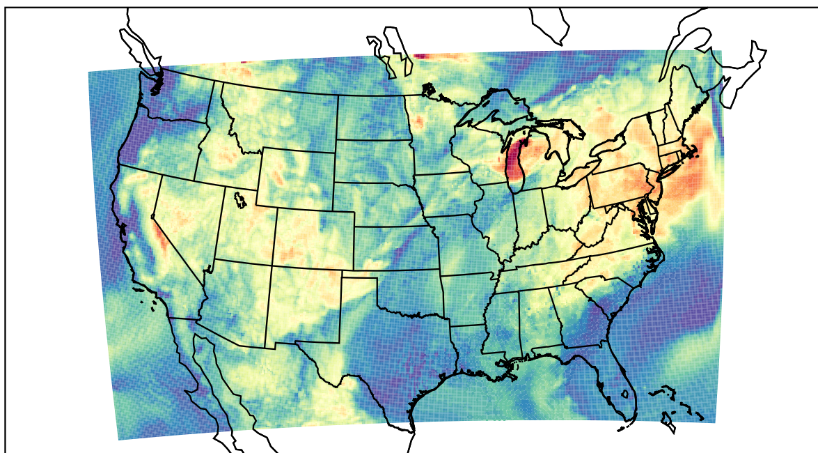
WRF (2021-07-15_14:00:00)
