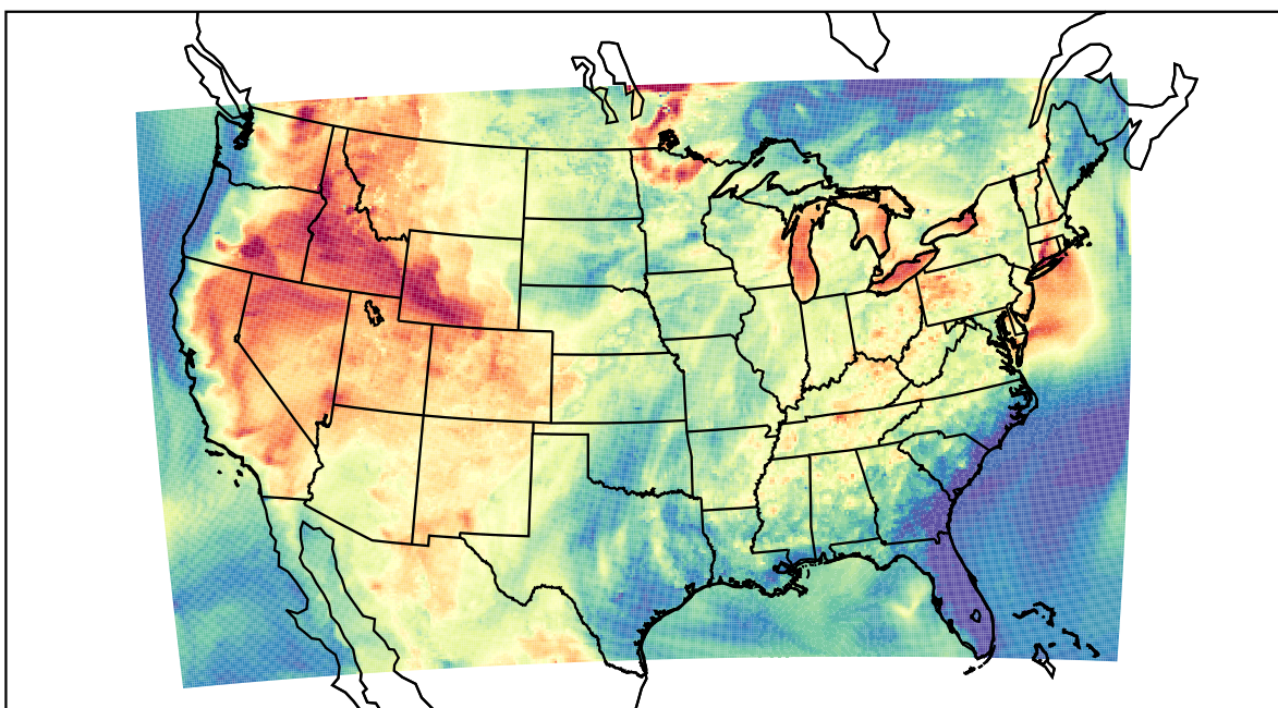
WRF (2021-07-15_01:00:00)
