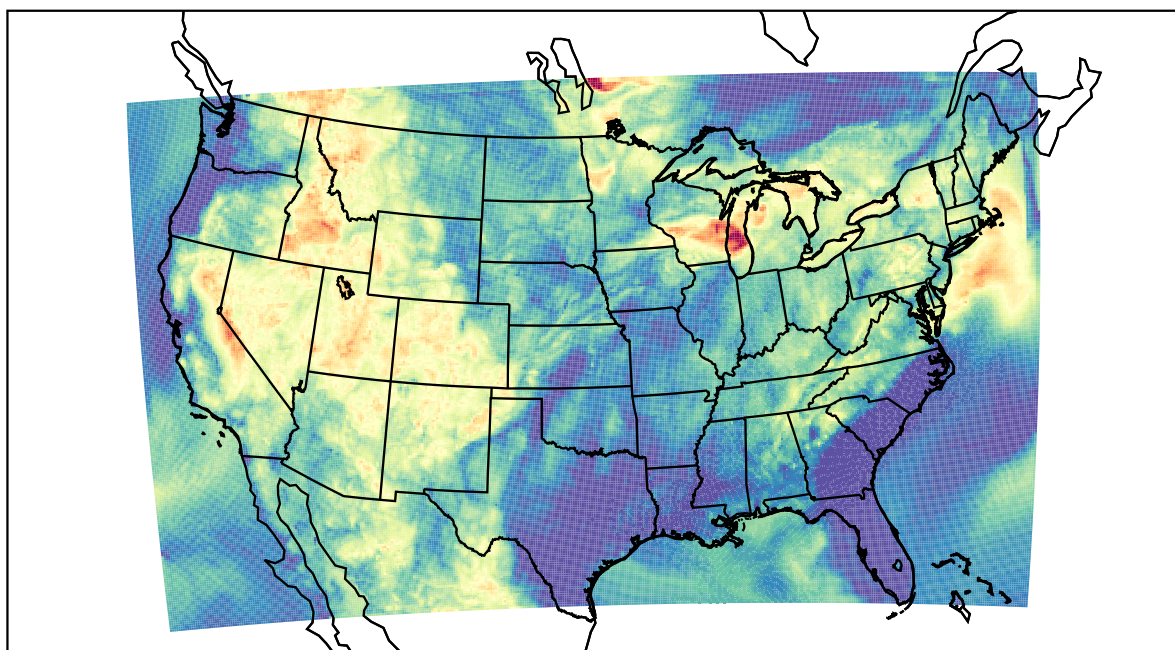
WRF (2021-07-15_09:00:00)
