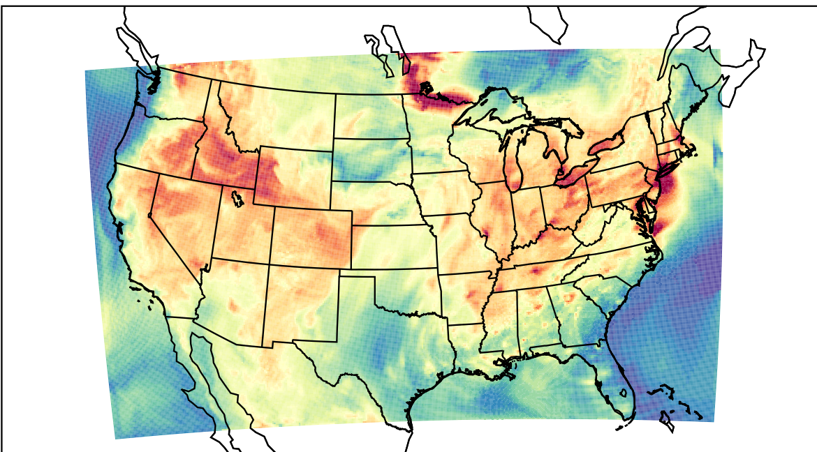
WRF (2021-07-14_18:00:00)
