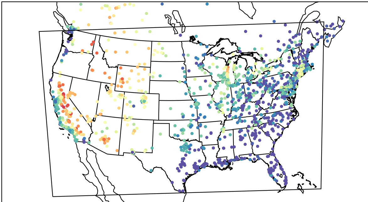
AirNOW (2021-07-15_02:00:00)
