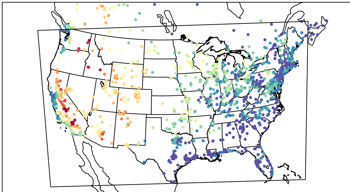
AirNOW (2021-07-14_01:00:00)
