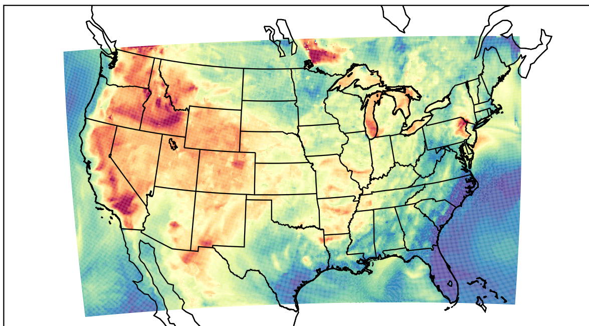
WRF (2021-07-14_01:00:00)
