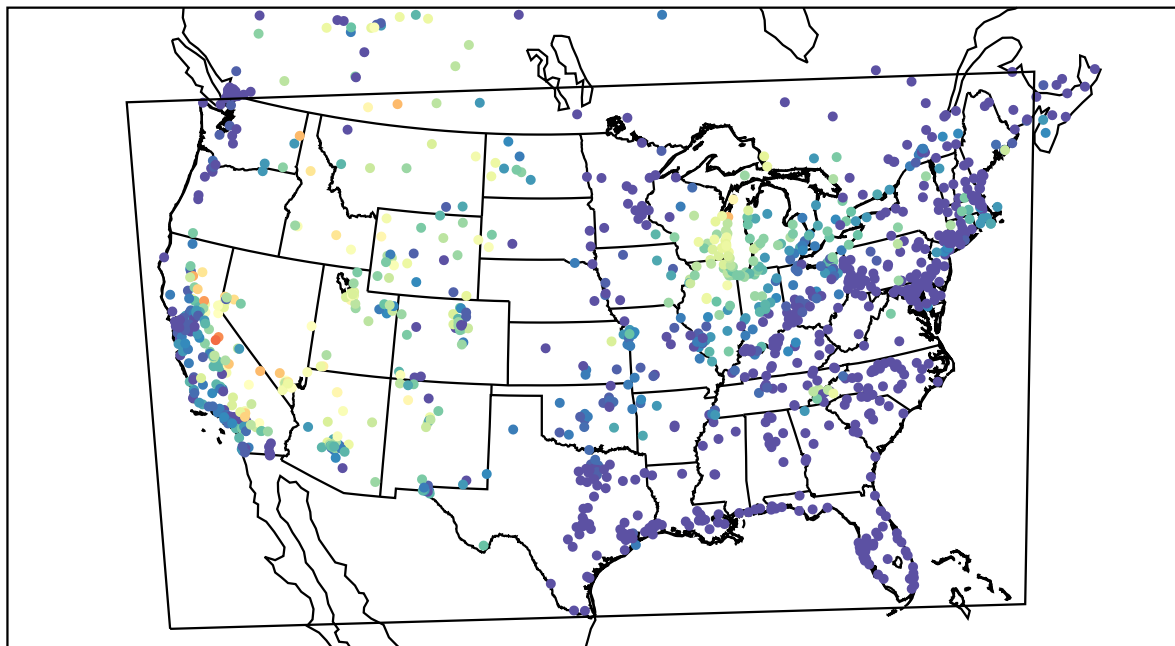
AirNOW (2021-07-15_09:00:00)
