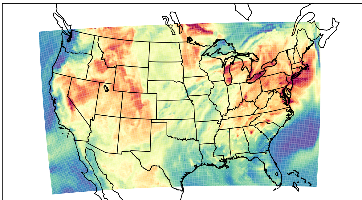
WRF (2021-07-15_17:00:00)
