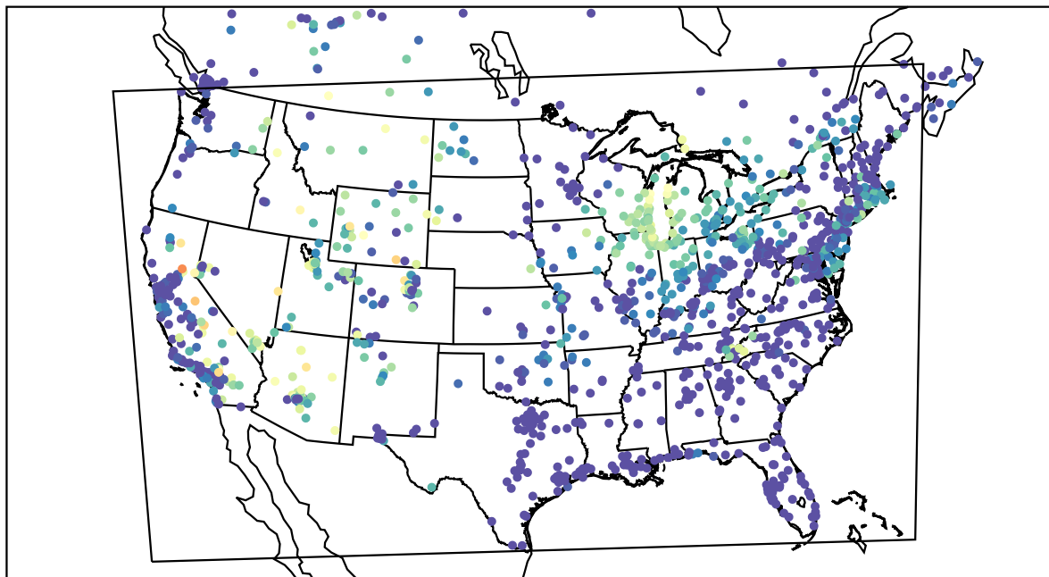
AirNOW (2021-07-15_12:00:00)
