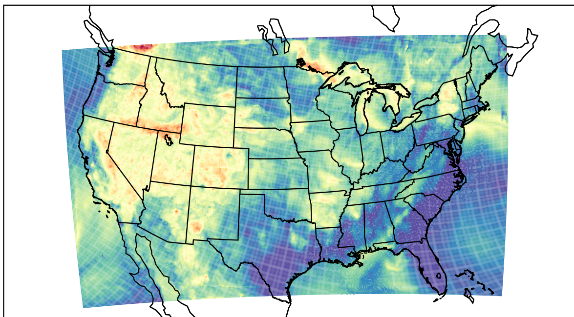
WRF (2021-07-14_07:00:00)
