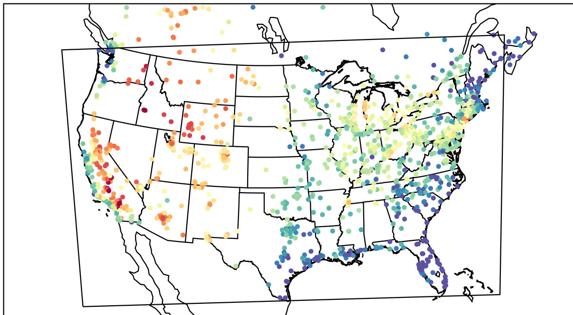
AirNOW (2021-07-14_23:00:00)
