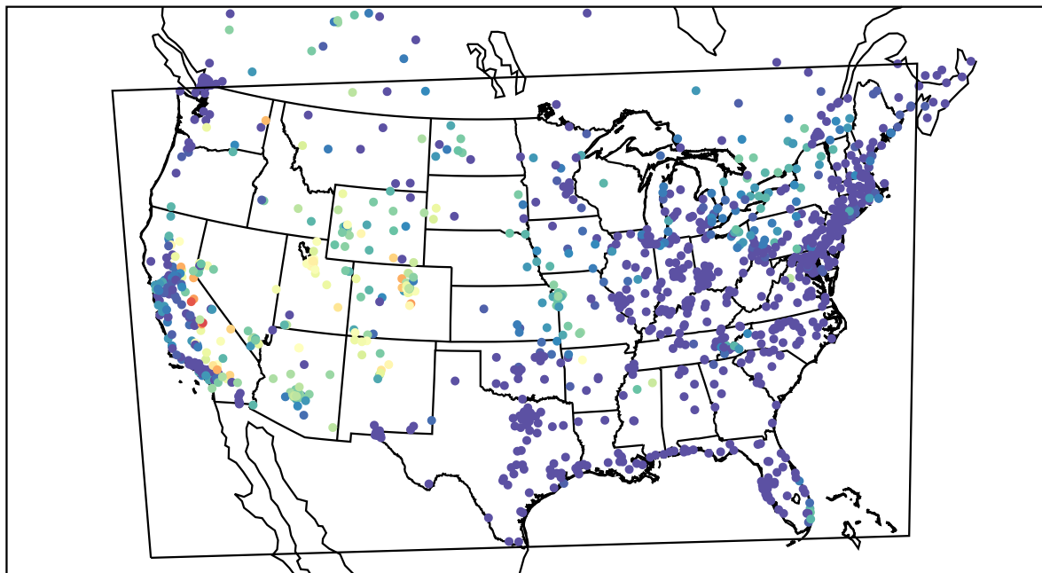
AirNOW (2021-07-14_10:00:00)
