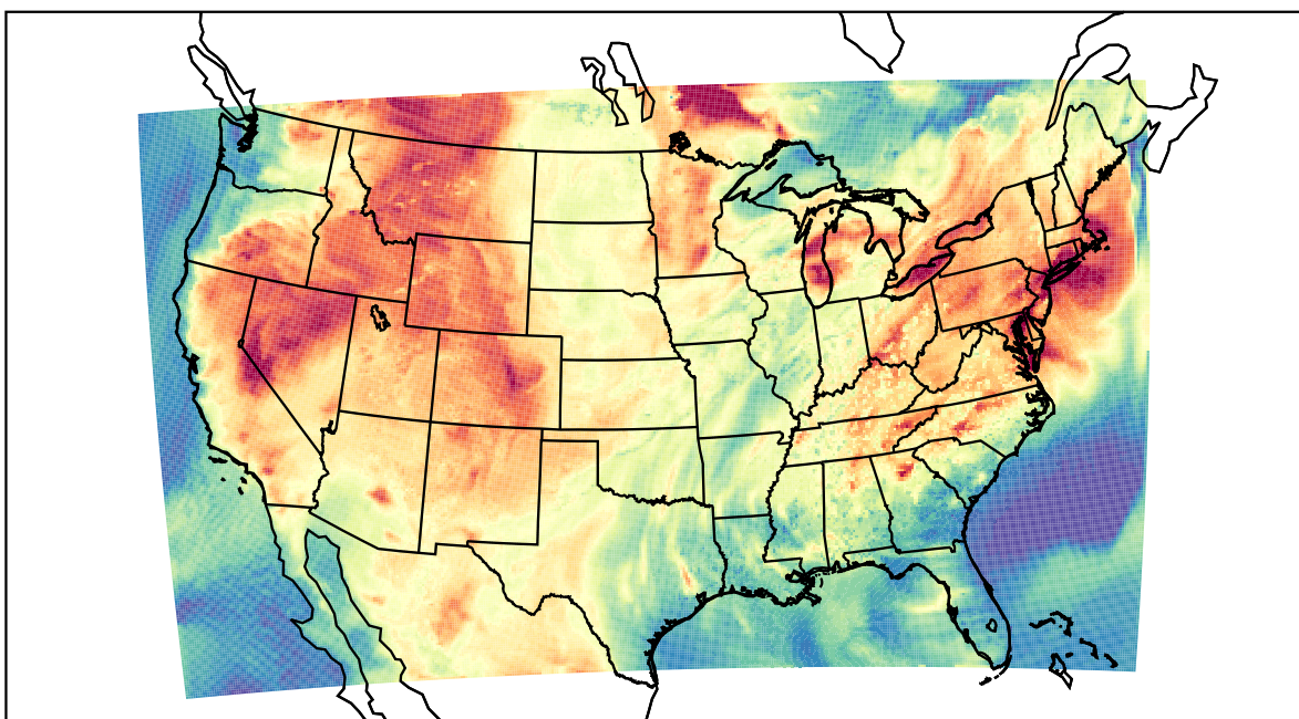
WRF (2021-07-15_21:00:00)
