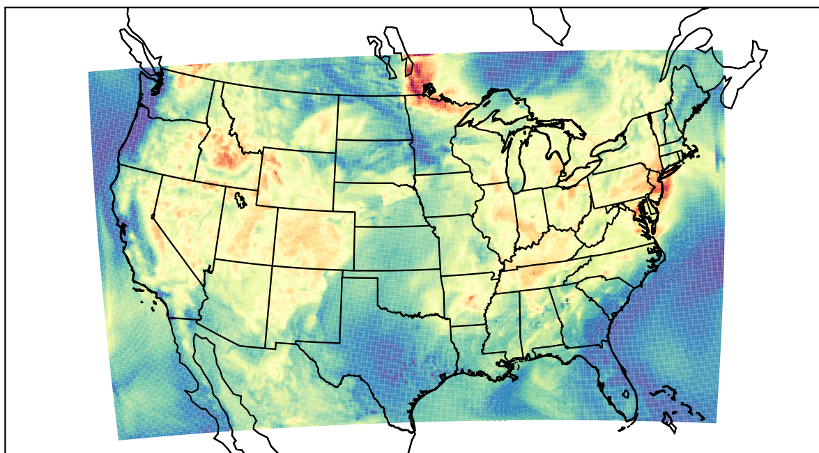
WRF (2021-07-14_15:00:00)
