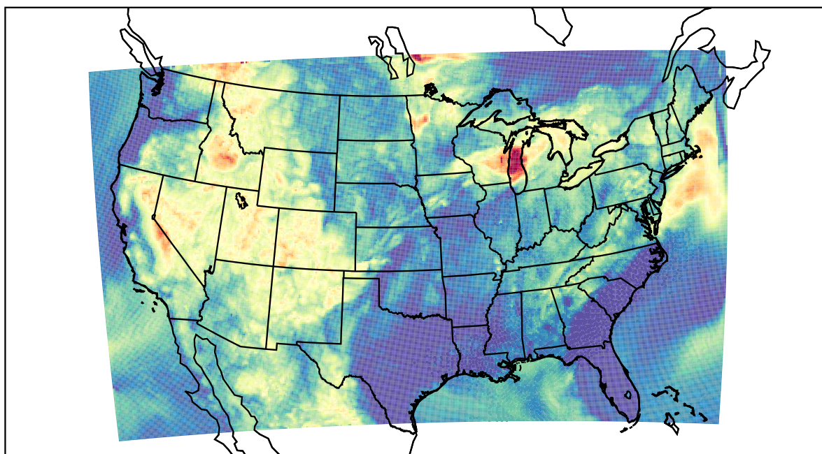
WRF (2021-07-15_11:00:00)
