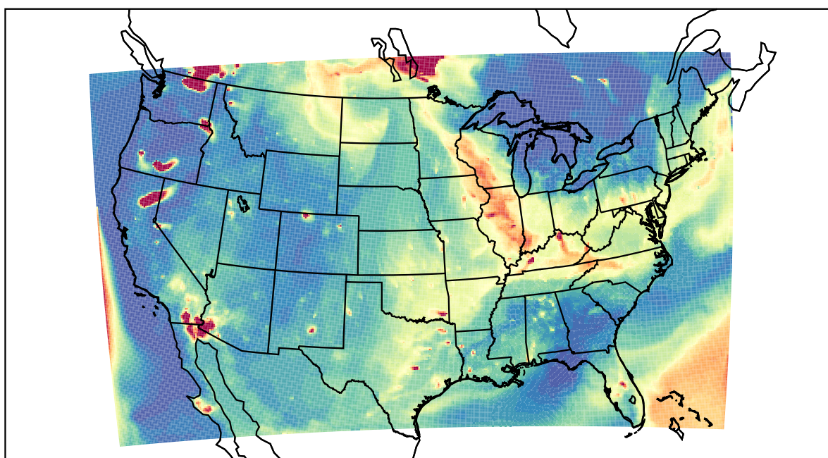
WRF 2021-07-22_03:00:00
