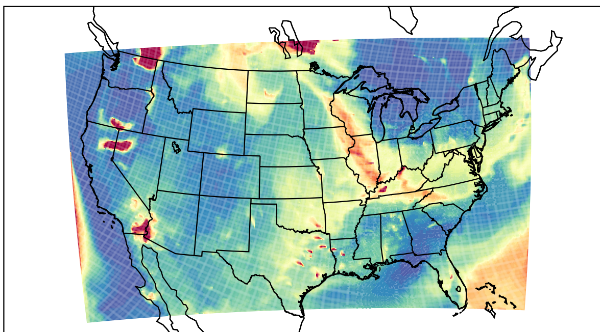
WRF 2021-07-22_06:00:00
