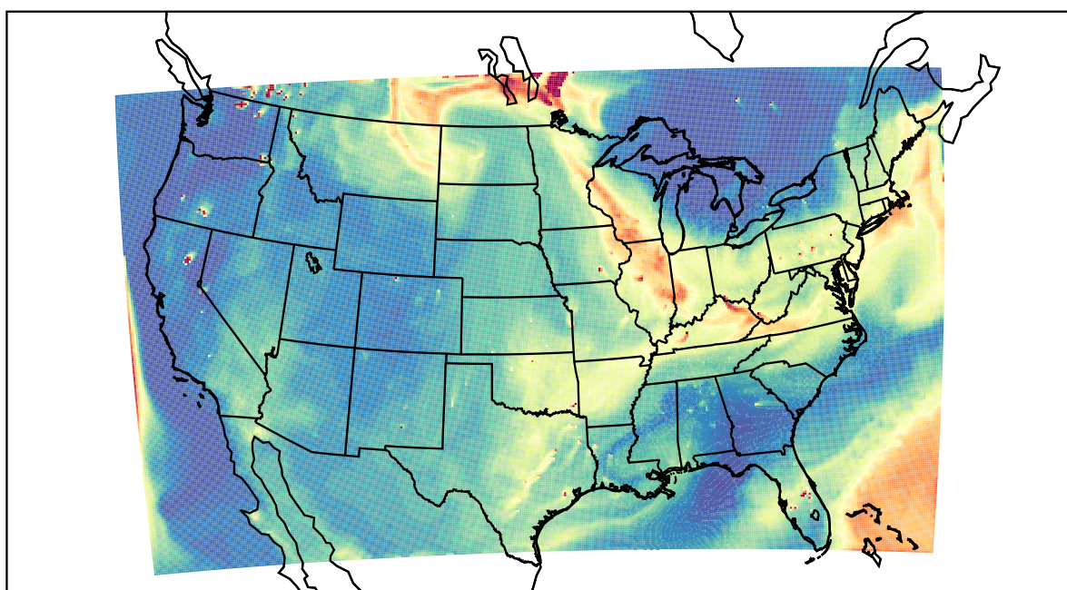
WRF 2021-07-21_21:00:00
