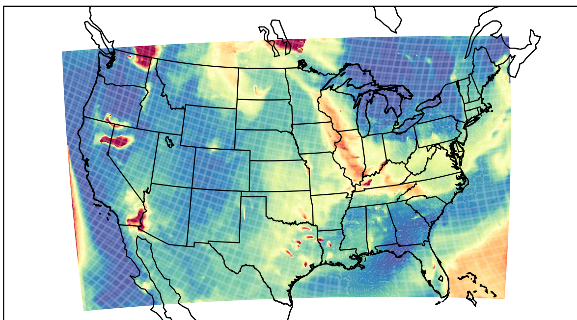
WRF 2021-07-22_07:00:00
