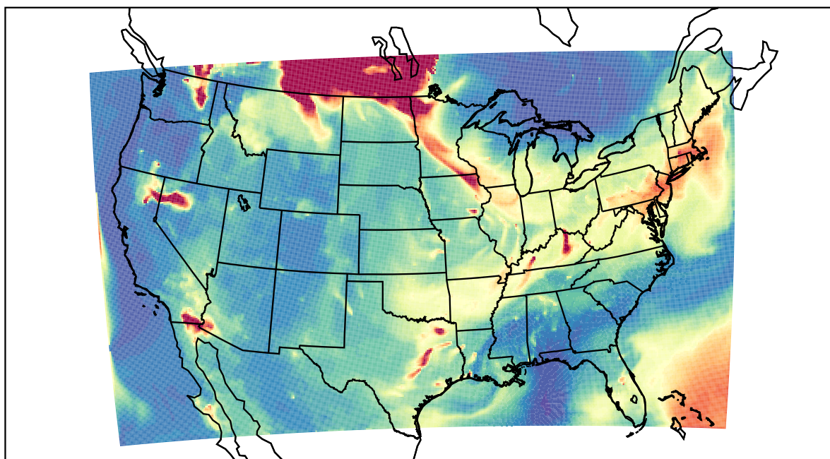
WRF 2021-07-21_09:00:00
