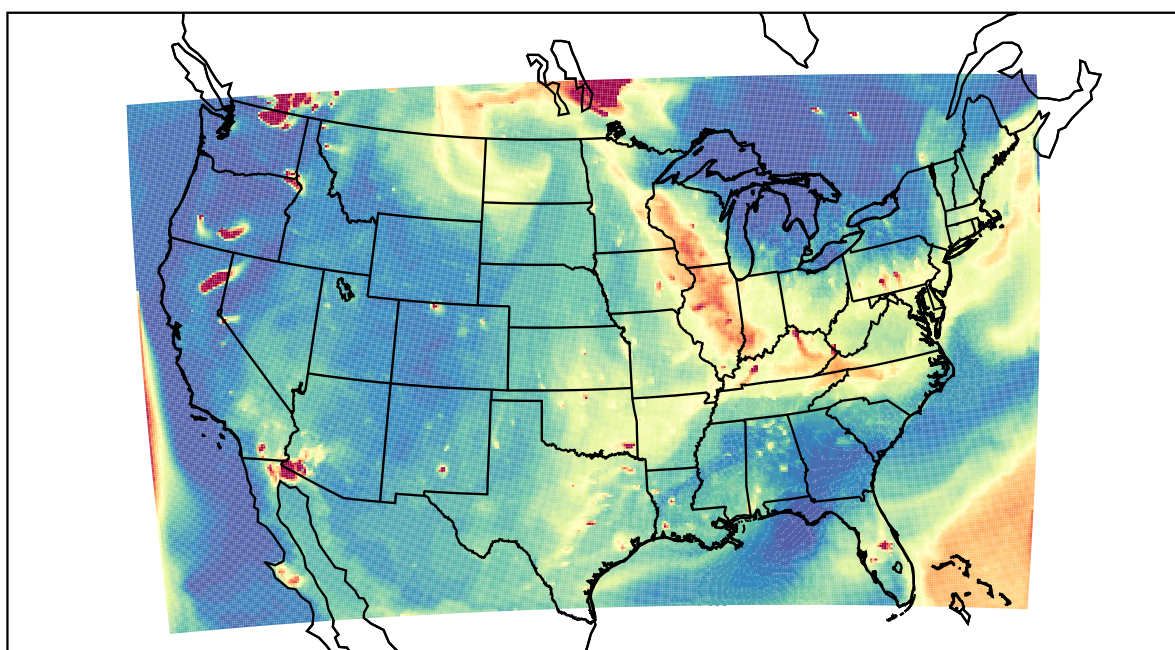
WRF 2021-07-22_02:00:00
