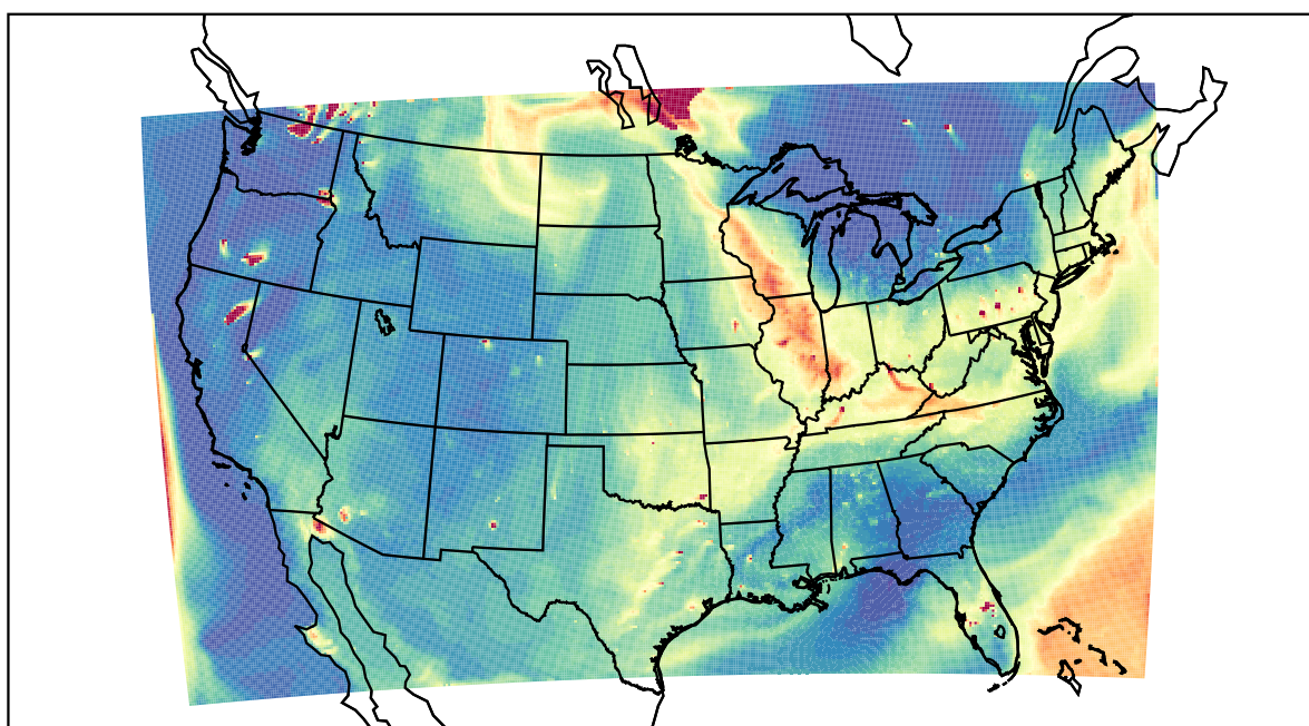
WRF 2021-07-22_00:00:00
