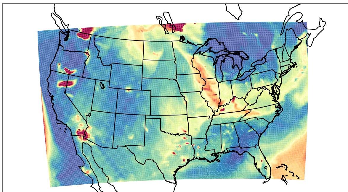
WRF 2021-07-22_05:00:00
