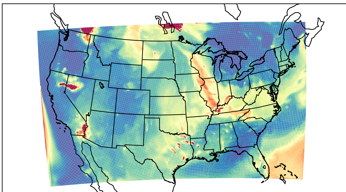
WRF 2021-07-22_09:00:00
