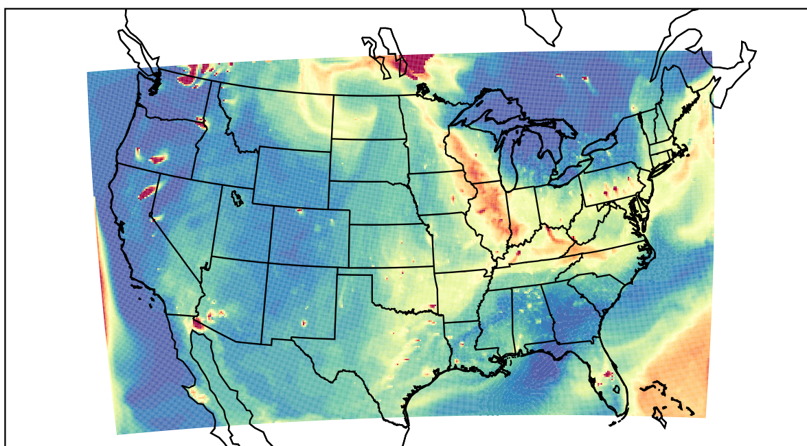
WRF 2021-07-22_01:00:00
