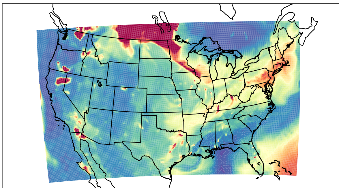
WRF 2021-07-21_05:00:00
