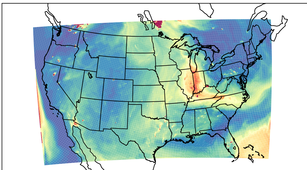
WRF 2021-07-22_21:00:00
