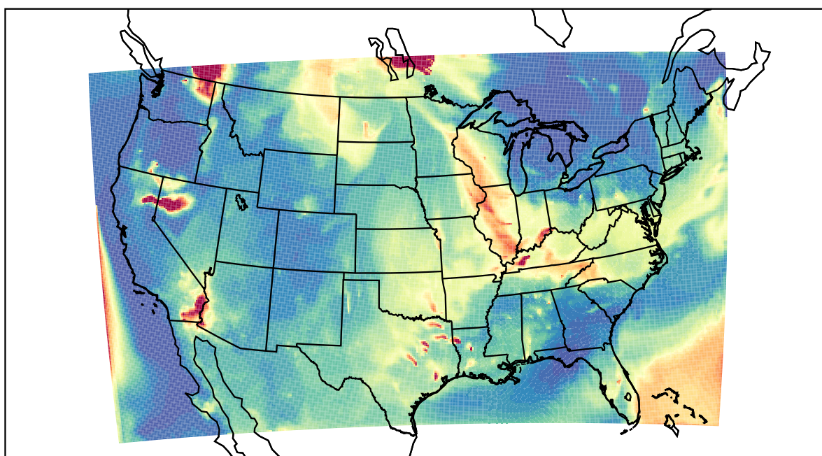
WRF 2021-07-22_08:00:00
