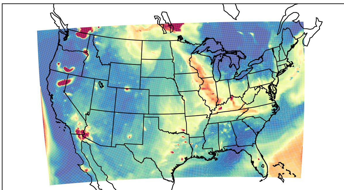
WRF 2021-07-22_04:00:00
