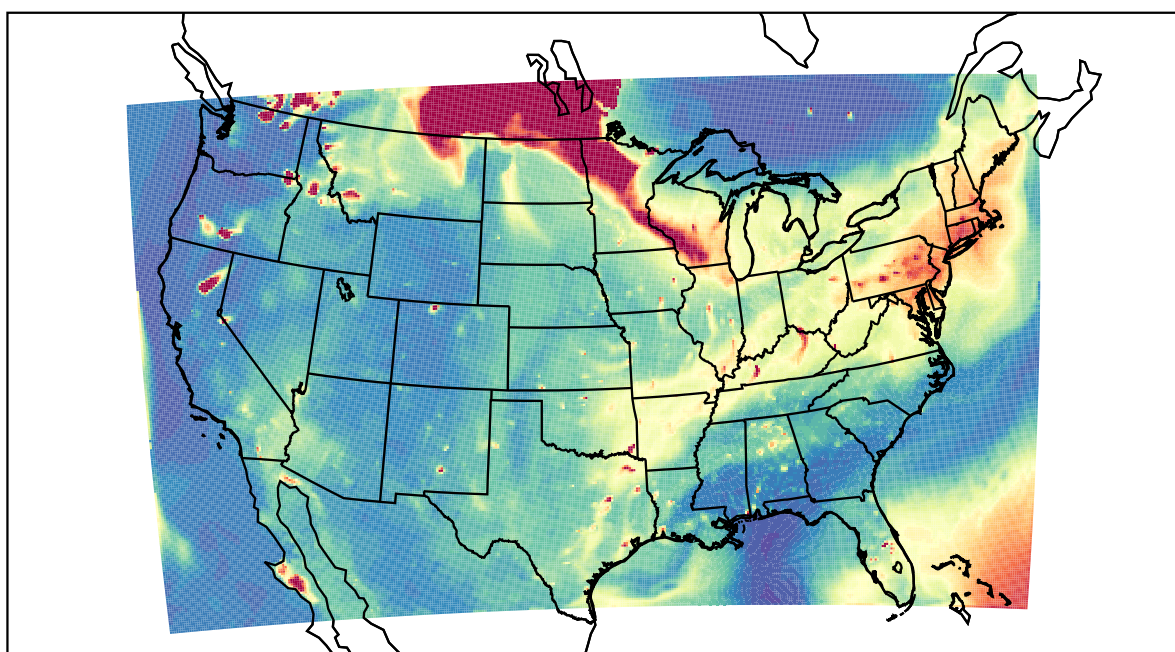
WRF 2021-07-21_02:00:00
